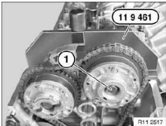
Fig. 363: Identifying Special Tool (11 9 461) Courtesy of BMW OF NORTH AMERICA, INC.
