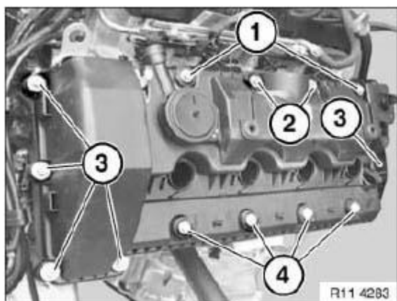
Fig. 32: Identifying Screw Connections Courtesy of BMW OF NORTH AMERICA, INC.
