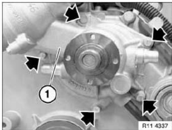
Fig. 588: Identifying Water Pump And Screws Courtesy of BMW OF NORTH AMERICA, INC.
