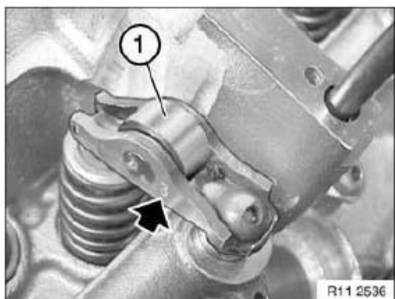
Fig. 379: Locating Rocker Arms On Inlet Side Courtesy of BMW OF NORTH AMERICA, INC.
