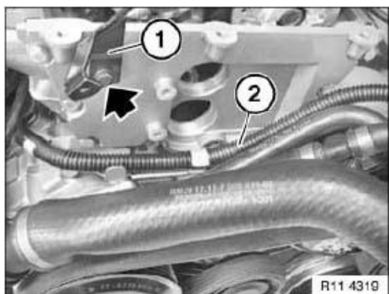
Fig. 108: Identifying Holder And Line Courtesy of BMW OF NORTH AMERICA, INC.
