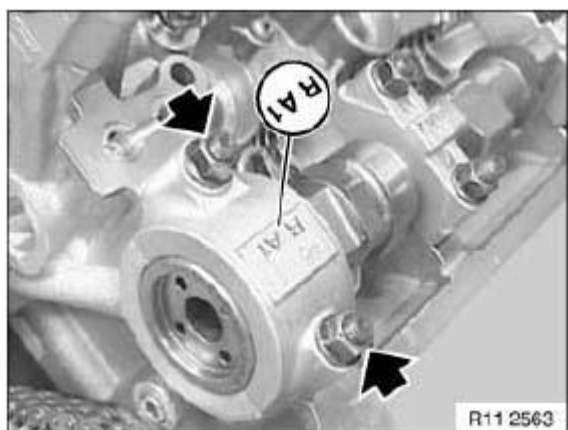
Fig. 304: Identifying Bearing Cap Mark Courtesy of BMW OF NORTH AMERICA, INC.
