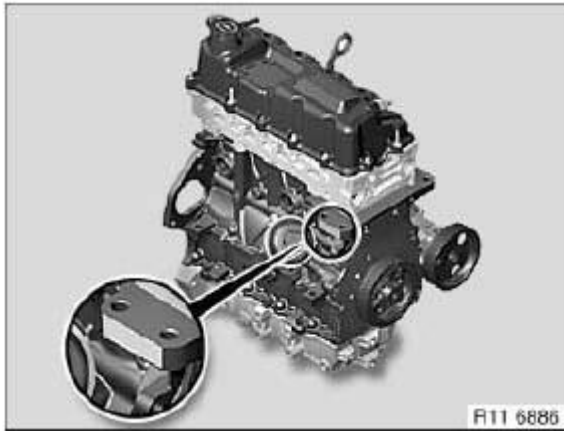
Fig. 25: Identifying Engine Identification Number - W10 / W11 Courtesy of BMW OF NORTH AMERICA, INC.
