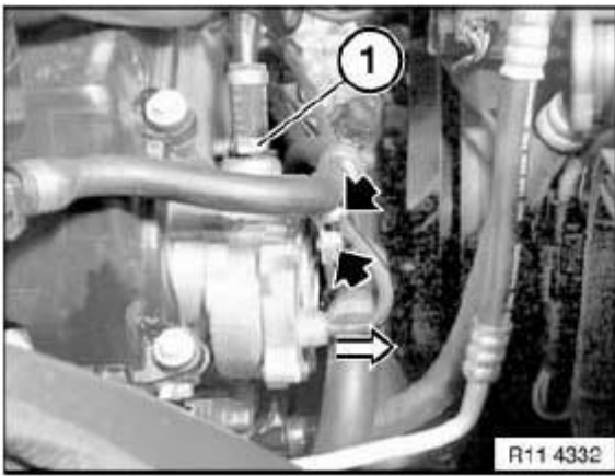
Fig. 601: Identifying Hose Clip
