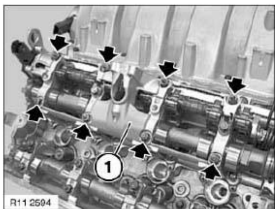
Fig. 389: Locating Bearing Bracket Courtesy of BMW OF NORTH AMERICA, INC.
