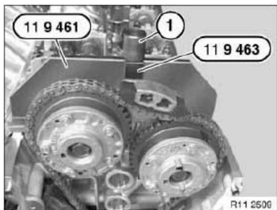
Fig. 349: Identifying Special Tool (11 9 461) And (11 9 463) Courtesy of BMW OF NORTH AMERICA, INC.
