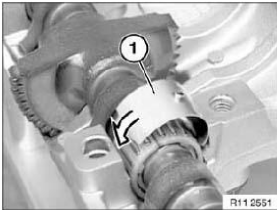
Fig. 510: Installing Bearing Shells Courtesy of BMW OF NORTH AMERICA, INC.
