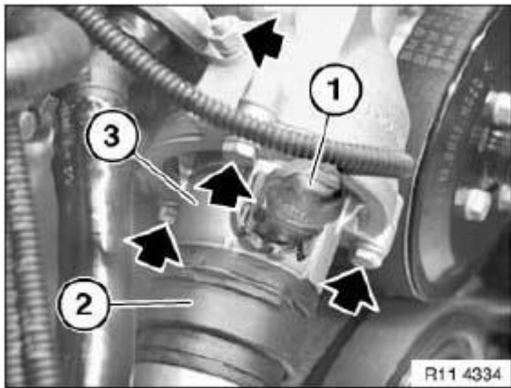
Fig. 595: Locating Coolant Thermostat, Water Hose And Unlock Plug Courtesy of BMW OF NORTH AMERICA, INC.
