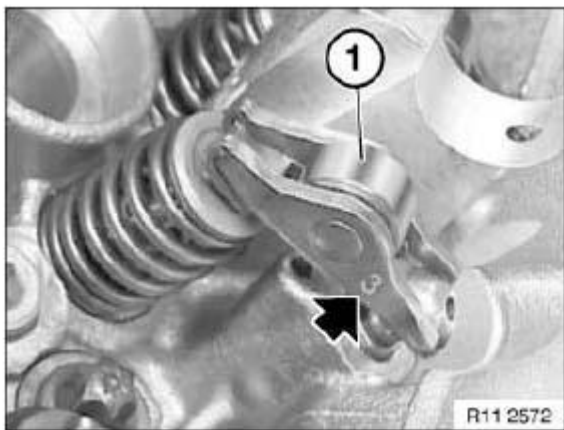
Fig. 319: Identifying Rocker Arm Courtesy of BMW OF NORTH AMERICA, INC.
