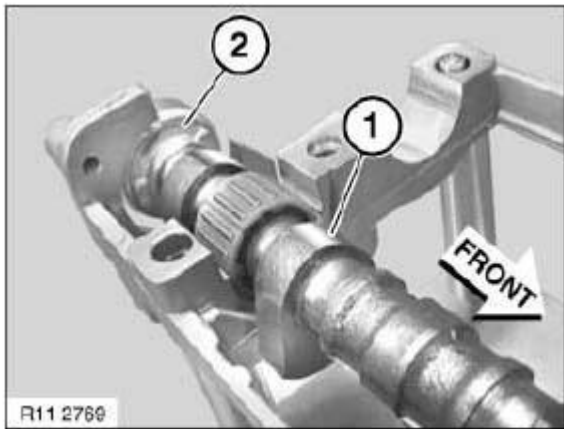
Fig. 509: Installing Eccentric Shaft Courtesy of BMW OF NORTH AMERICA, INC.
