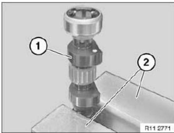
Fig. 499: Clamping Eccentric Shaft Installation With Protective Jaws In Vice Courtesy of BMW OF NORTH AMERICA, INC.
