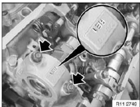
Fig. 373: Locating Camshaft Bearing Caps Of Cylinders Courtesy of BMW OF NORTH AMERICA, INC.
