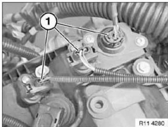
Fig. 43: Identifying Plug
