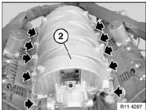
Fig. 598: Identifying Intake Air Manifold Courtesy of BMW OF NORTH AMERICA, INC.
