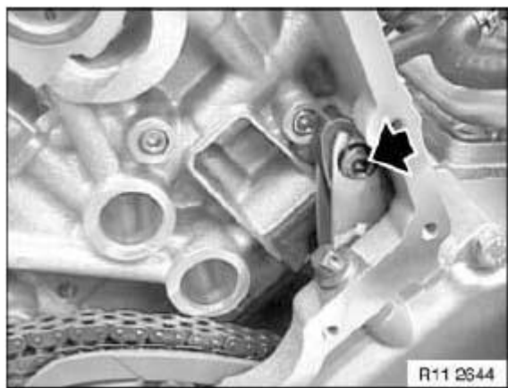
Fig. 84: Identifying Guide Rail Screw Courtesy of BMW OF NORTH AMERICA, INC.
