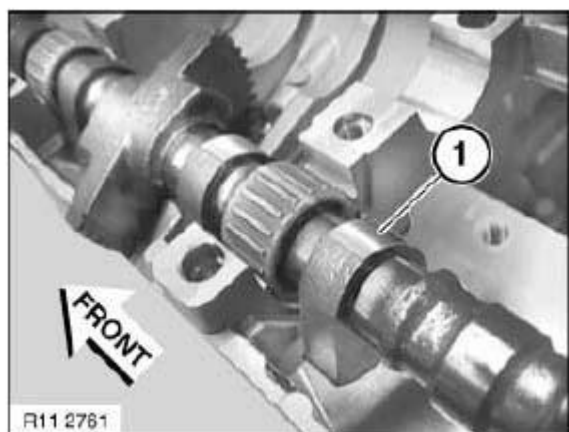
Fig. 494: Identifying Machined Curvature Of Eccentric Points Courtesy of BMW OF NORTH AMERICA, INC.
