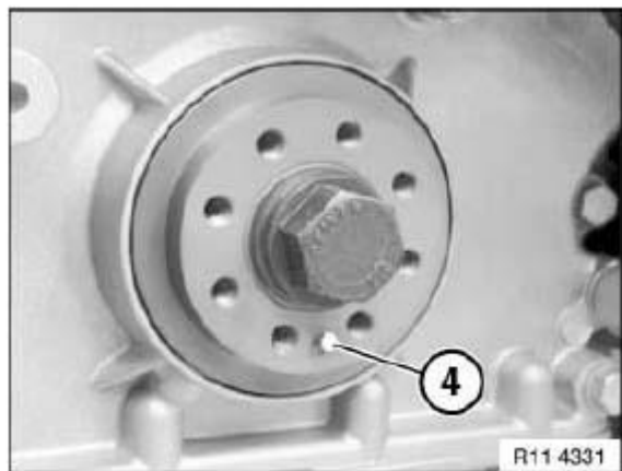
Fig. 149: Identifying Vibration Damper Alignment Pin Courtesy of BMW OF NORTH AMERICA, INC.
