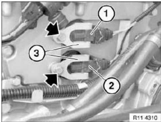
Fig. 474: Locating Solenoid Valves And Holder Courtesy of BMW OF NORTH AMERICA, INC.
