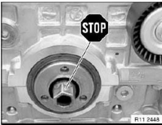
Fig. 66: Identifying Central Bolt
