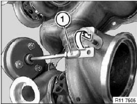
Fig. 421: Engaging Turnbuckle On Adjusting Lever Courtesy of BMW OF NORTH AMERICA, INC.
