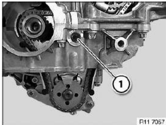
Fig. 327: Identifying Screw
