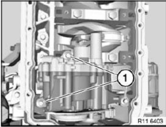
Fig. 126: Identifying Screws
