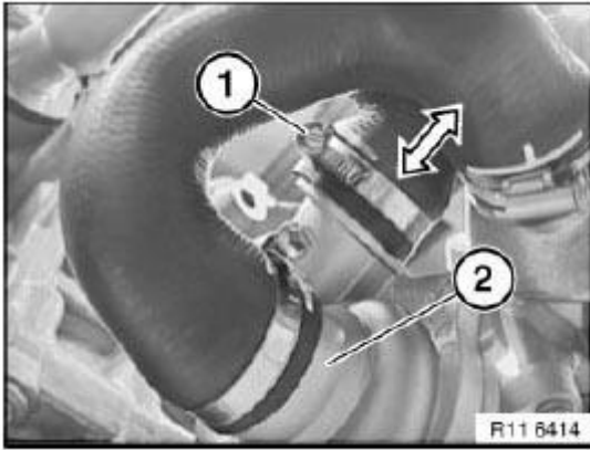
Fig. 350: Identifying Coolant Hose And Coolant Pump Courtesy of BMW OF NORTH AMERICA, INC.
