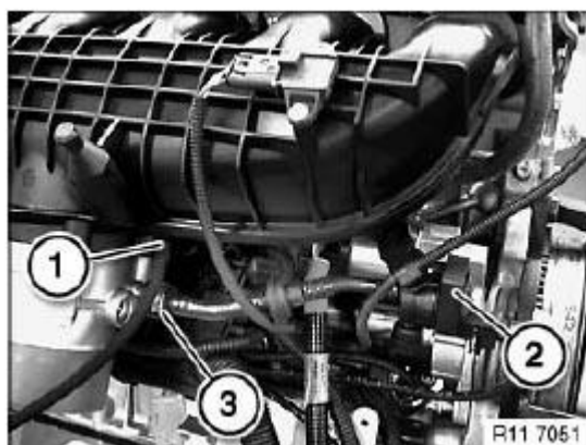
Fig. 354: Identifying Vacuum Hose, Tank Vent Valve And Hose Courtesy of BMW OF NORTH AMERICA, INC.
