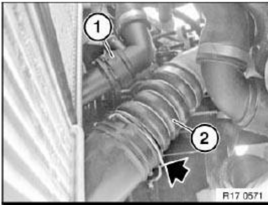
Fig. 364: Identifying Coolant Hose And Charge-Air Duct
