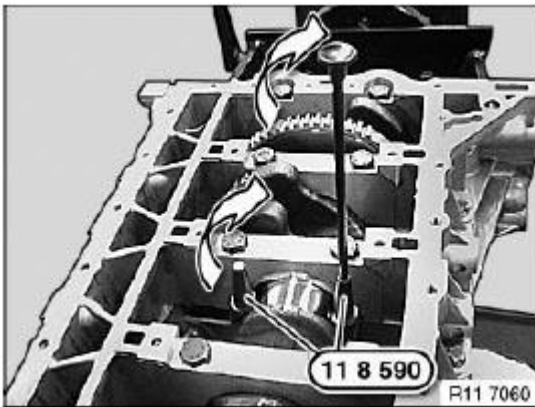
Fig. 191: Screwing Special Tool (11 8 590) Into Base Of Connecting Rod
