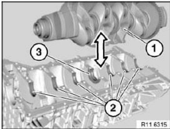
Fig. 173: Identifying Bearing Shells Courtesy of BMW OF NORTH AMERICA, INC.
