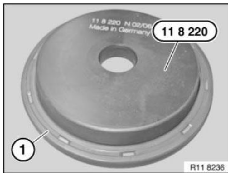
Fig. 99: Identifying Radial Shaft Seal On Special Tool 11 8 220 Courtesy of BMW OF NORTH AMERICA, INC.
