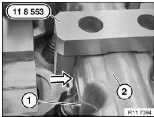
Fig. 256: Positioning Special Tool (11 8 553) Over Screw Connection Of Bearing Banks Courtesy of BMW OF NORTH AMERICA, INC.
