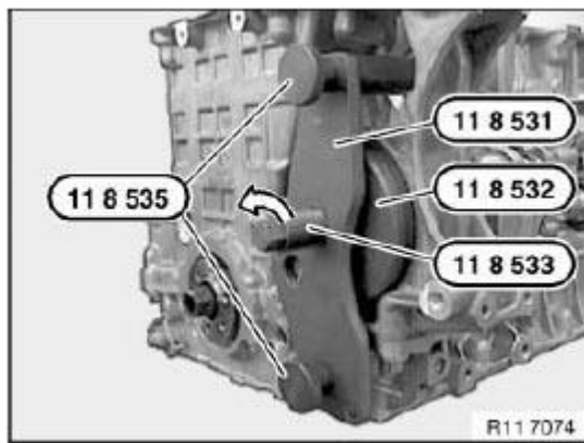
Fig. 79: Twisting Out Special Tool (11 8 533) And (11 8 532) Courtesy of BMW OF NORTH AMERICA, INC.
