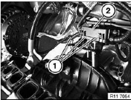
Fig. 357: Identifying Distributor Housing With Bolts Courtesy of BMW OF NORTH AMERICA, INC.
