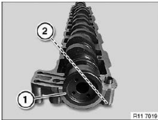
Fig. 234: Rotating Intake Camshaft At Cylinder No. 1 Courtesy of BMW OF NORTH AMERICA, INC.
