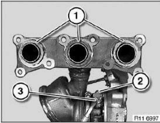
Fig. 342: Identifying Turbocharger
