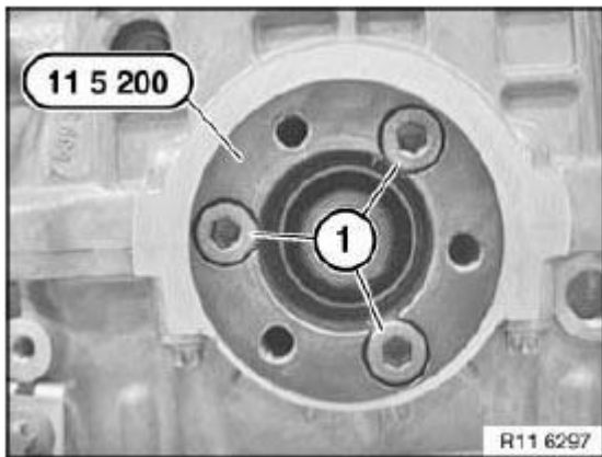
Fig. 336: Identifying Screws With Special Tool (11 5 200) Courtesy of BMW OF NORTH AMERICA, INC.
