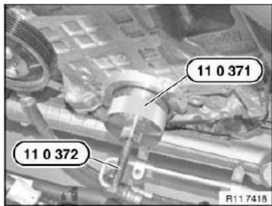
Fig. 68: Screwing Special Tool (11 0 371) Into Crankshaft Seal Courtesy of BMW OF NORTH AMERICA, INC.
