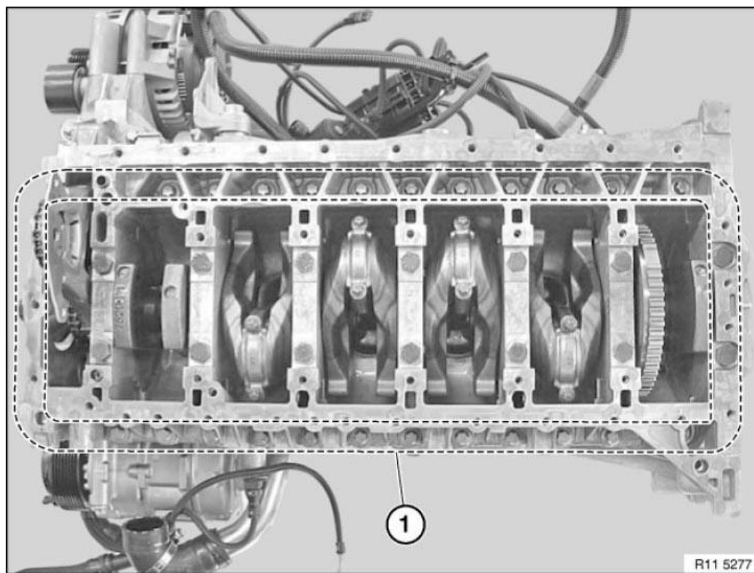
Fig. 144: Identifying Crankcase Bolts
