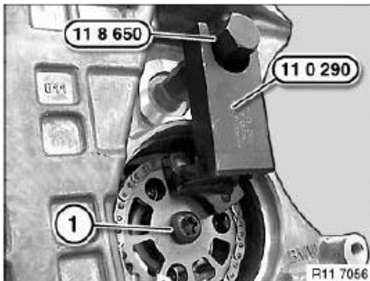
Fig. 423: Identifying Central Bolt With Special Tools (11 8 650) And (11 0 290) Courtesy of BMW OF NORTH AMERICA, INC.
