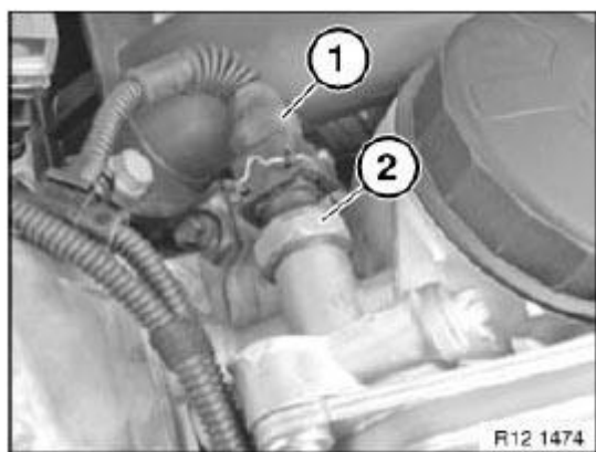
Fig. 355: Identifying Plug Connection On Oil Pressure Switch Courtesy of BMW OF NORTH AMERICA, INC.
