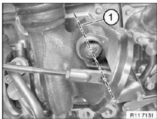
Fig. 382: Positioning Of Wastegate Linkage Depressurized Courtesy of BMW OF NORTH AMERICA, INC.
