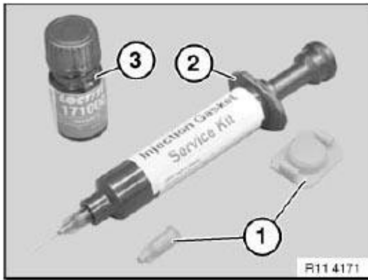
Fig. 73: Identifying Screw Caps And Injector Courtesy of BMW OF NORTH AMERICA, INC.
