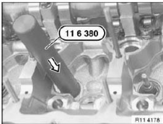
Fig. 297: Pressing Valve Stem Seal With Special Tool (11 6 380) Courtesy of BMW OF NORTH AMERICA, INC.
