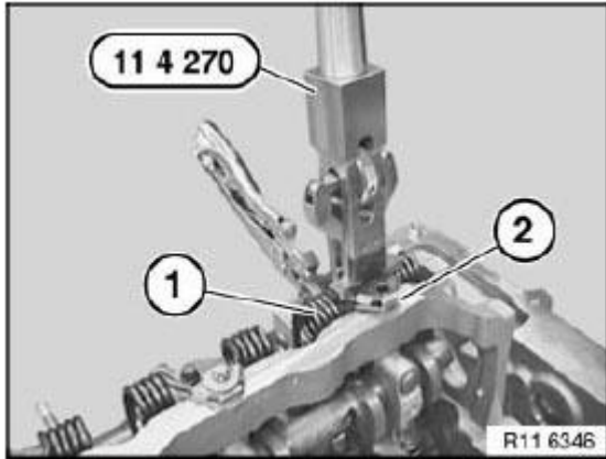
Fig. 294: Identifying Special Tool 11 4 270 Courtesy of BMW OF NORTH AMERICA, INC.
