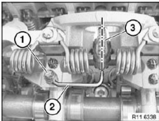
Fig. 337: Identifying Oil Spray Nozzle, Spline Teeth And Screw Courtesy of BMW OF NORTH AMERICA, INC.
