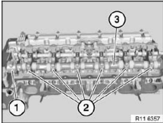
Fig. 220: Identifying Bearing Cap Courtesy of BMW OF NORTH AMERICA, INC.
