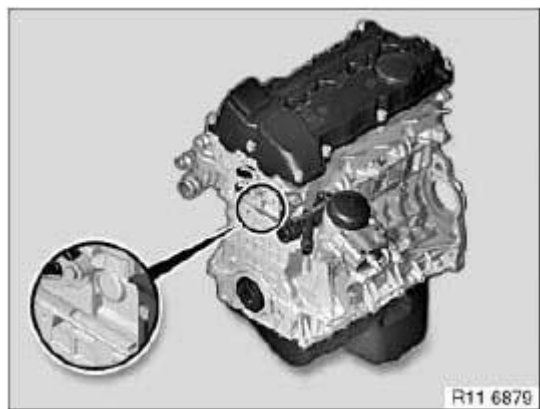
Fig. 25: Identifying Engine Identification - N40 / N45 / N45T / N43 Courtesy of BMW OF NORTH AMERICA, INC.
