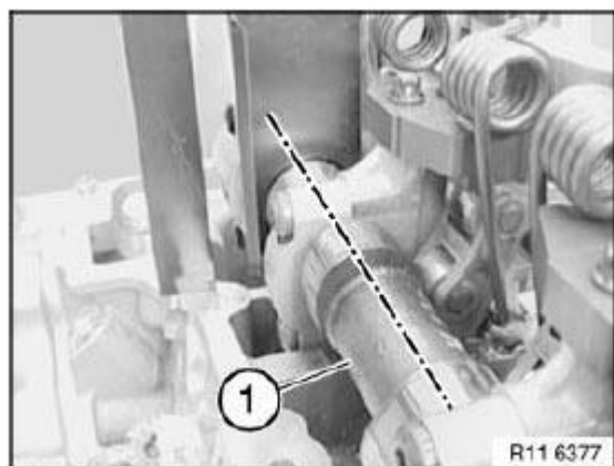
Fig. 216: Identifying Inlet Camshaft Courtesy of BMW OF NORTH AMERICA, INC.
