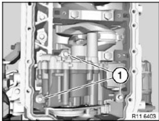
Fig. 137: Identifying Screws
