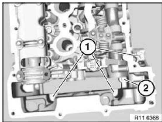
Fig. 44: Identifying Bolt
