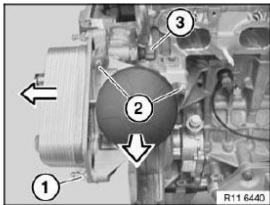
Fig. 346: Releasing Screws
