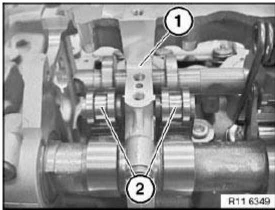
Fig. 326: Identifying Contact Surfaces And Intermediate Levers Courtesy of BMW OF NORTH AMERICA, INC.
