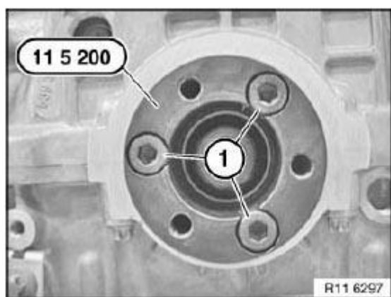
Fig. 362: Identifying Special Tool 11 5 200 And Screws Courtesy of BMW OF NORTH AMERICA, INC.
