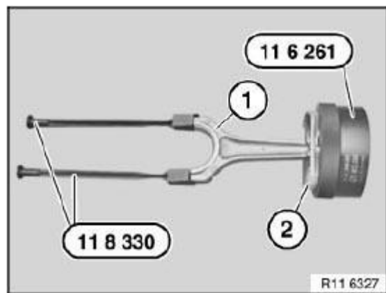
Fig. 196: Identifying Piston And Connecting Rod Courtesy of BMW OF NORTH AMERICA, INC.
