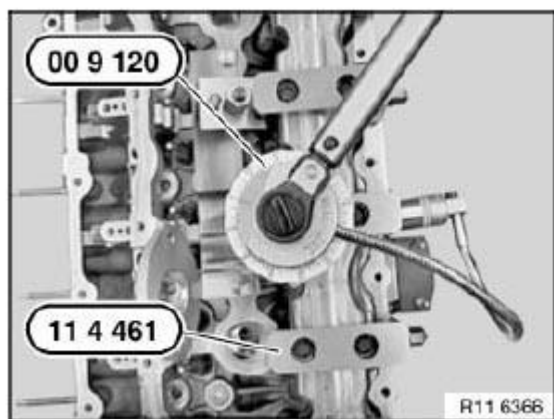
Fig. 242: Identifying Special Tool 11 4 461 And 00 9 120 Courtesy of BMW OF NORTH AMERICA, INC.
