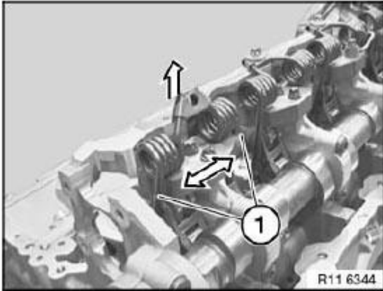
Fig. 322: Pressing Torsion Spring Apart Courtesy of BMW OF NORTH AMERICA, INC.
