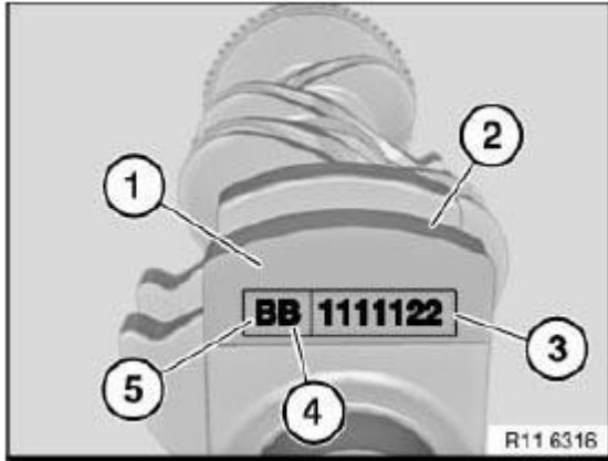
Fig. 123: Identifying Seven-Digit Part Number And Bearing Classification Courtesy of BMW OF NORTH AMERICA, INC.
