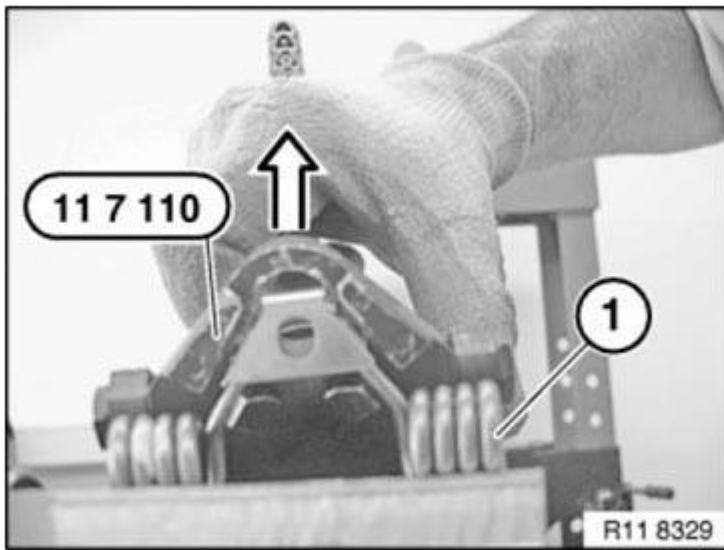
Fig. 332: Positioning Special Tool 11 7 110 On Return Spring Courtesy of BMW OF NORTH AMERICA, INC.
