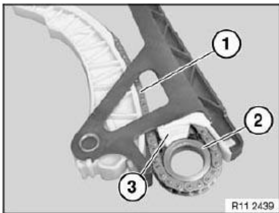
Fig. 253: Identifying Timing Chain, Chain Guide And Sprocket Wheel Courtesy of BMW OF NORTH AMERICA, INC.
