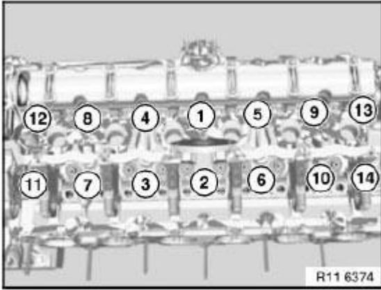
Fig. 52: Identifying Cylinder Head Bolts In Sequence Courtesy of BMW OF NORTH AMERICA, INC.
