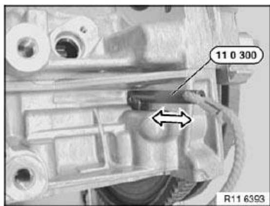
Fig. 141: Securing Crankshaft
