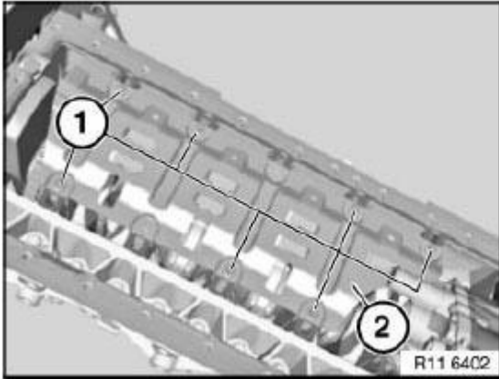
Fig. 108: Identifying Bolts And Screws Courtesy of BMW OF NORTH AMERICA, INC.
