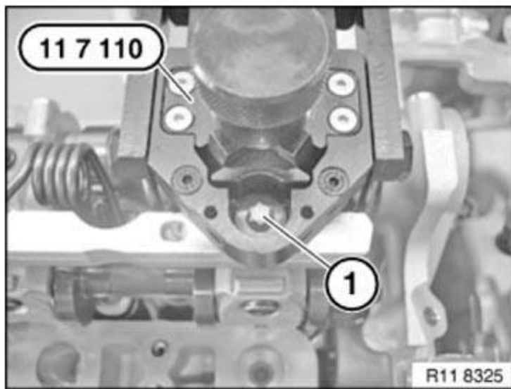
Fig. 364: Tightening Bolt
