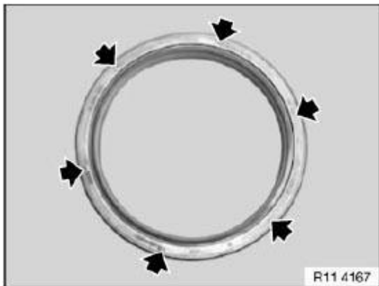
Fig. 96: Locating Crankshaft Radial Seal Openings Courtesy of BMW OF NORTH AMERICA, INC.
