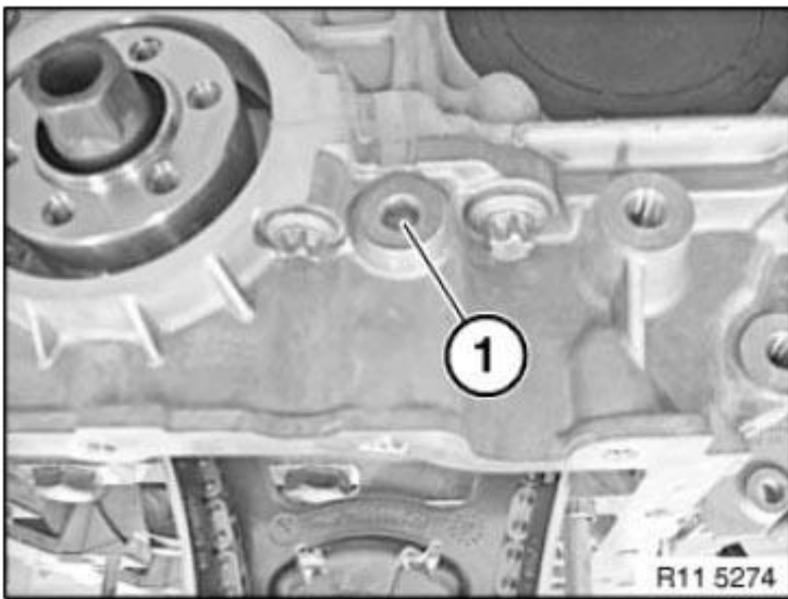
Fig. 157: Identifying Crankcase Screws Plug Courtesy of BMW OF NORTH AMERICA, INC.
