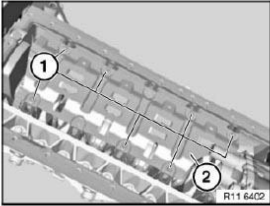
Fig. 154: Identifying Oil Deflector And Screws Courtesy of BMW OF NORTH AMERICA, INC.
