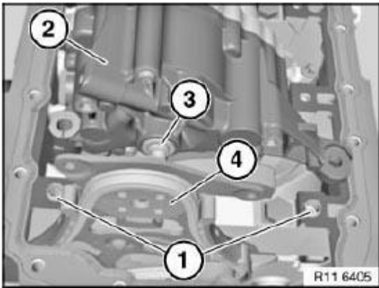
Fig. 396: Identifying Spacer, Oil Pump And Sprocket Wheel
