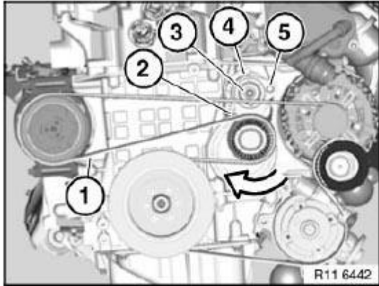
Fig. 234: Turning Belt Tensioner And Drive Belt Routing (E9X) Courtesy of BMW OF NORTH AMERICA, INC.
