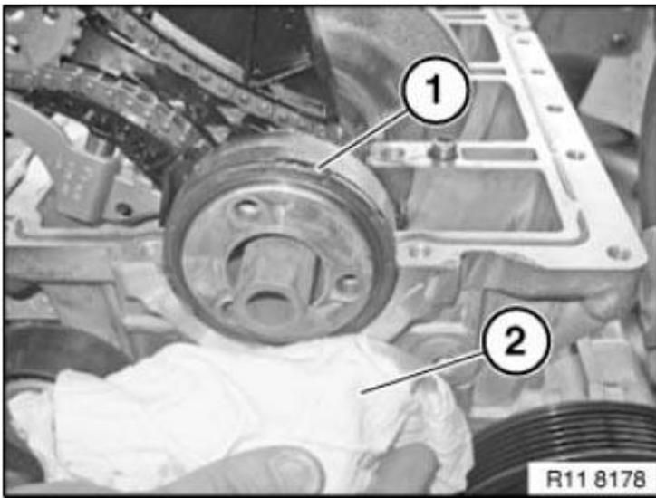
Fig. 171: Stopping Engine Oil Using Cloth Courtesy of BMW OF NORTH AMERICA, INC.
