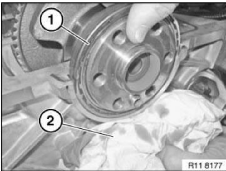
Fig. 170: Removing Radial Shaft Seal Courtesy of BMW OF NORTH AMERICA, INC.
