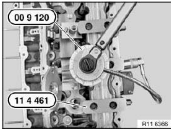
Fig. 269: Tightening Lower/Upper Bearing Strips Courtesy of BMW OF NORTH AMERICA, INC.
