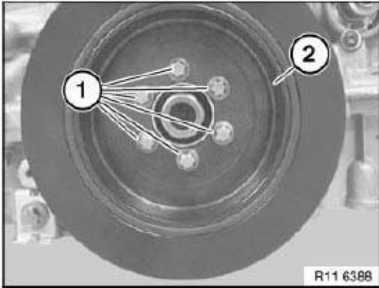
Fig. 200: Identifying Vibration Damper And Screws Courtesy of BMW OF NORTH AMERICA, INC.
