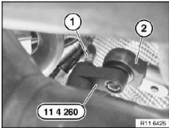
Fig. 412: Releasing Lambda Control Sensor Courtesy of BMW OF NORTH AMERICA, INC.
