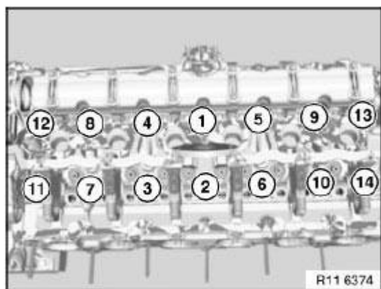
Fig. 58: Cylinder Head Bolts Tightening Sequence Courtesy of BMW OF NORTH AMERICA, INC.
