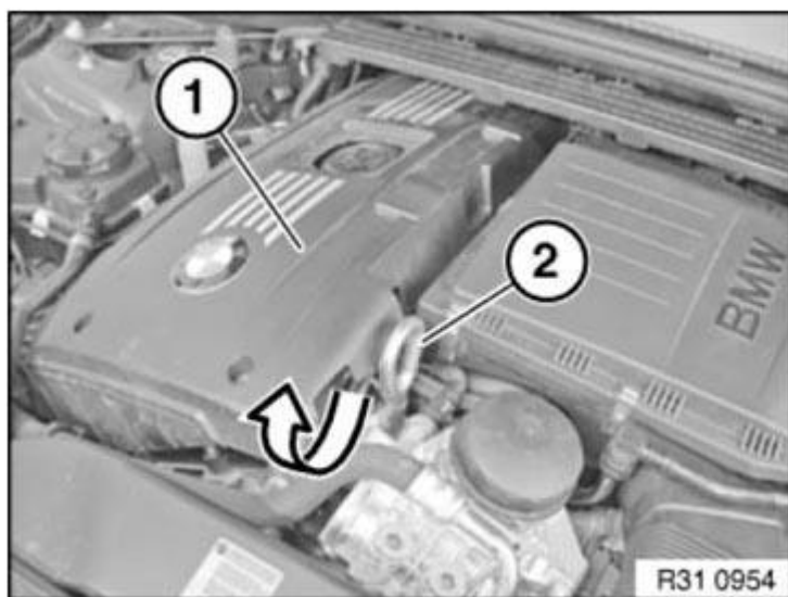
Fig. 36: Raising Acoustic Cover Courtesy of BMW OF NORTH AMERICA, INC.
