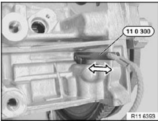
Fig. 276: Sliding Special Tool (11 0 300) Courtesy of BMW OF NORTH AMERICA, INC.
