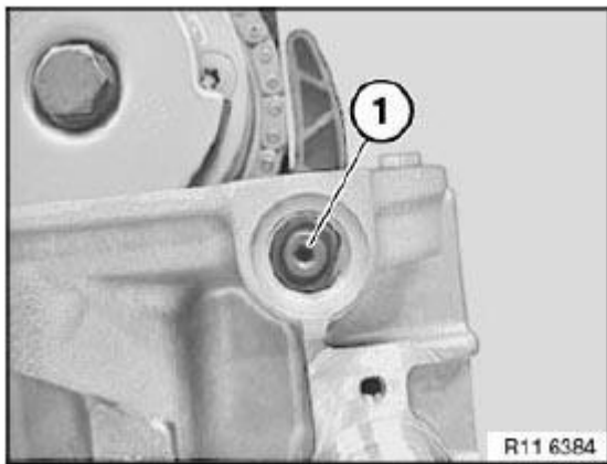
Fig. 280: Identifying Timing Chain Module Bearing Pin (Cylinder Head) Courtesy of BMW OF NORTH AMERICA, INC.
