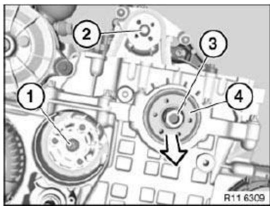
Fig. 385: Removing Hub
