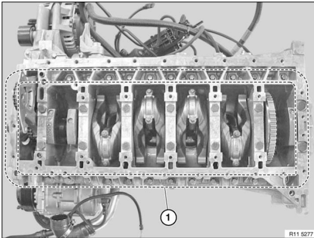
Fig. 167: Identifying Crankcase Bolts
