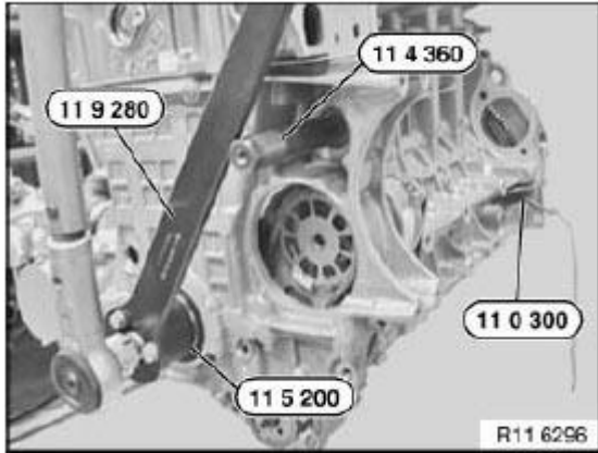
Fig. 289: Tightening Central Bolt Courtesy of BMW OF NORTH AMERICA, INC.
