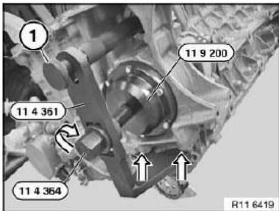
Fig. 124: Attaching Special Tool (11 4 361) To Bedplate Construction Screw Connection
