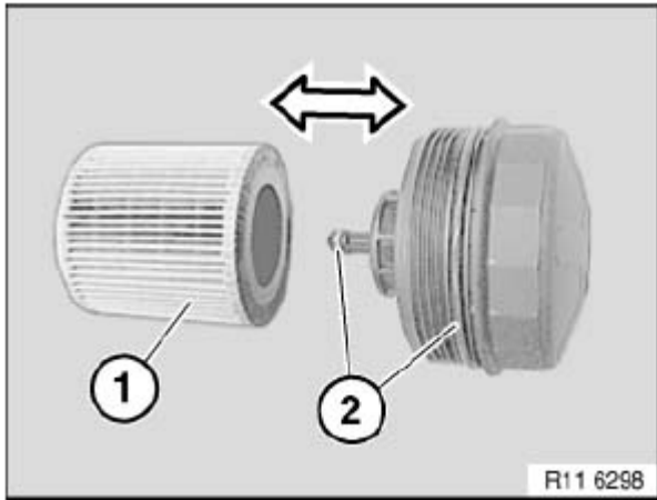
Fig. 20: Removing Oil Filter Element Courtesy of BMW OF NORTH AMERICA, INC.
