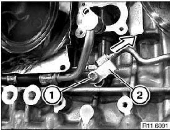
Fig. 283: Detaching Oil Feed Line Courtesy of BMW OF NORTH AMERICA, INC.
