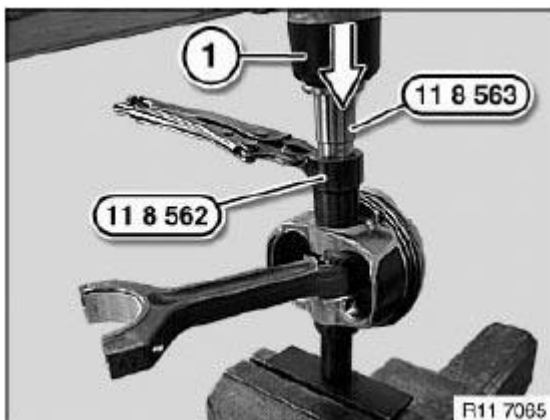
Fig. 117: Identifying Special Tool (11 8 562) To Piston Crown Courtesy of BMW OF NORTH AMERICA, INC.
