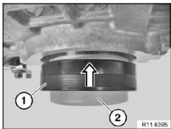
Fig. 64: Pushing On Radial Shaft Seal Courtesy of BMW OF NORTH AMERICA, INC.
