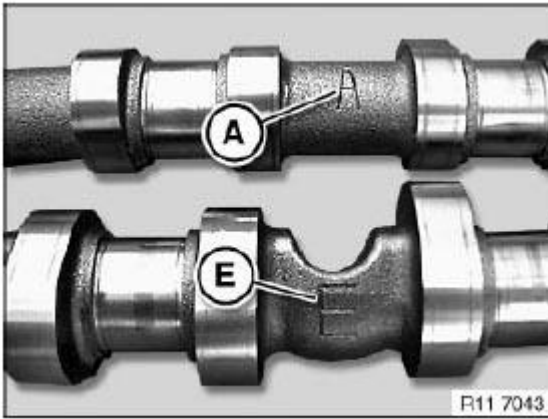
Fig. 146: Identifying Camshafts Identification Mark Courtesy of BMW OF NORTH AMERICA, INC.
