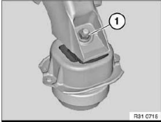
Fig. 15: Identifying Self-Locking Nuts Courtesy of BMW OF NORTH AMERICA, INC.
