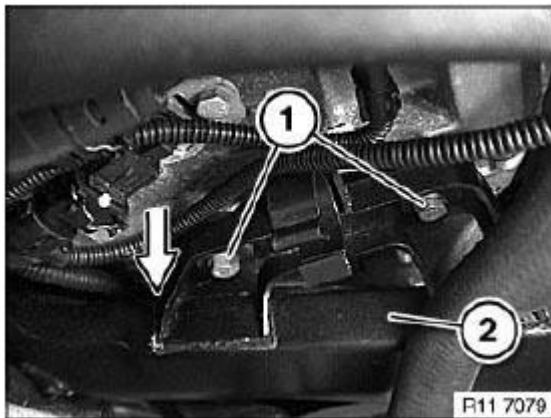
Fig. 134: Identifying Air Duct With Screw Courtesy of BMW OF NORTH AMERICA, INC.
