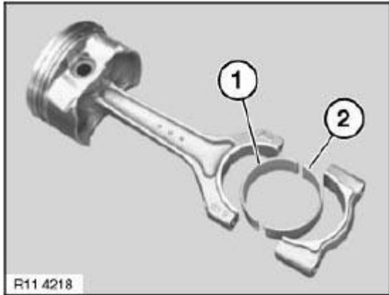
Fig. 102: Identifying Connecting Rod Bearing Shell Courtesy of BMW OF NORTH AMERICA, INC.
