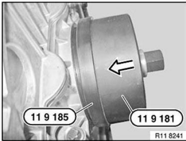
Fig. 112: Installing Rear Crankshaft Seal Using Tool 119 180/181 Courtesy of BMW OF NORTH AMERICA, INC.
