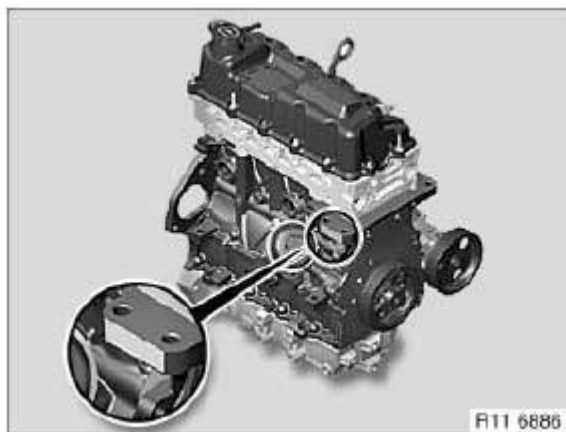
Fig. 42: Identifying Engine Number Location (W10/W11) Courtesy of BMW OF NORTH AMERICA, INC.
