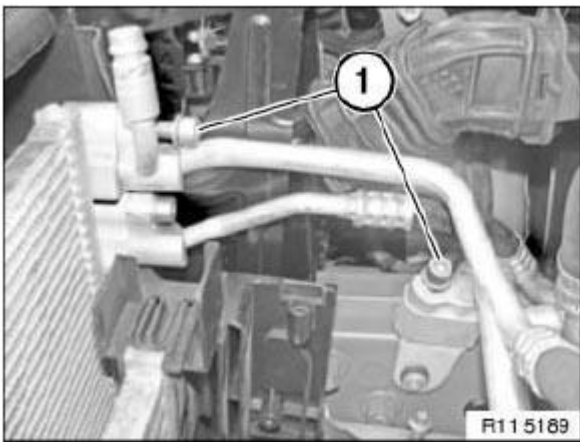
Fig. 13: Identifying A/C Lines Screws Courtesy of BMW OF NORTH AMERICA, INC.
