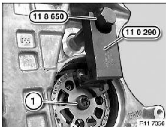
Fig. 346: Positioning Special Tool 11 0 290 On Sprocket Wheel And On Special Tool 11 8 650
