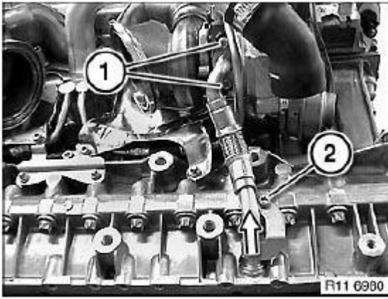
Fig. 389: Identifying Screws
