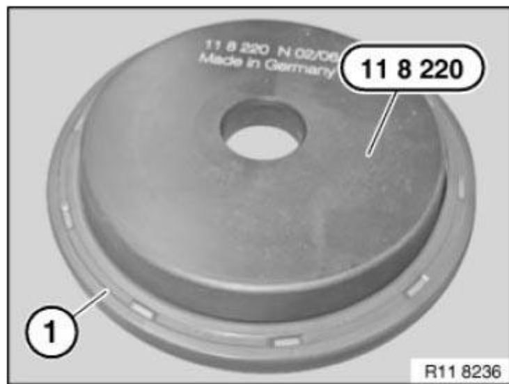
Fig. 107: Identifying Radial Shaft Seal On Special Tool 11 8 220 Courtesy of BMW OF NORTH AMERICA, INC.
