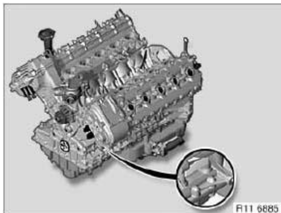
Fig. 41: Identifying Engine Number Location (S85/S65) Courtesy of BMW OF NORTH AMERICA, INC.
