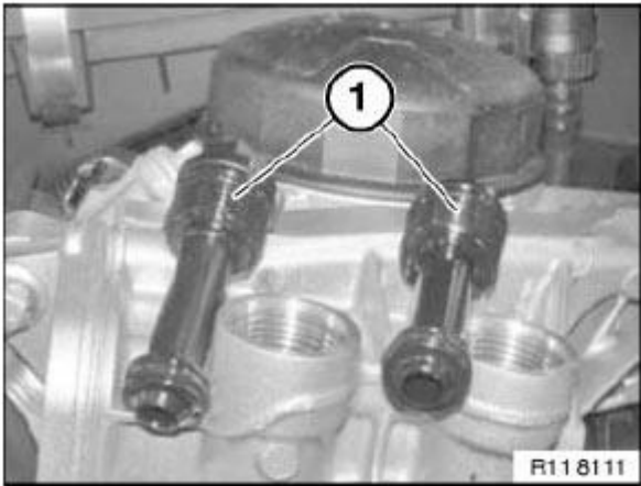
Fig. 20: Identifying Transportation Locks Courtesy of BMW OF NORTH AMERICA, INC.
