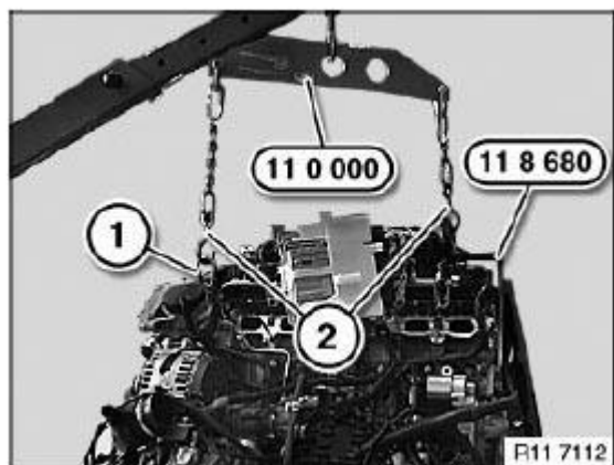
Fig. 17: Identifying Special Tools 11 0 000 And 11 8 680 Courtesy of BMW OF NORTH AMERICA, INC.
