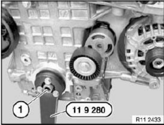
Fig. 337: Identifying Central Bolt With Special Tool 11 9 280 Courtesy of BMW OF NORTH AMERICA, INC.
