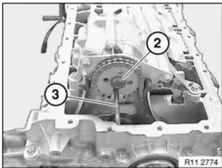
Fig. 143: Identifying Oil Pump Drive Gear And Steel Pin Courtesy of BMW OF NORTH AMERICA, INC.
