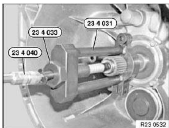
Fig. 189: Identifying Special Tools 23 4 033, 23 4 031 And 23 4 040 Courtesy of BMW OF NORTH AMERICA, INC.
