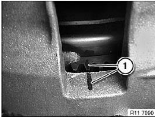
Fig. 272: Identifying Line On Flywheel And Transmission Housing Courtesy of BMW OF NORTH AMERICA, INC.
