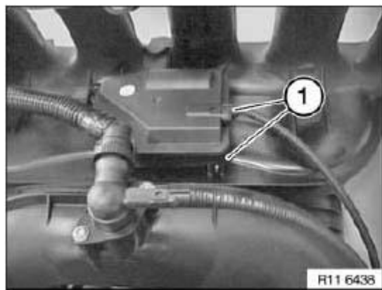
Fig. 299: Identifying Plug Connection At Bottom Courtesy of BMW OF NORTH AMERICA, INC.
