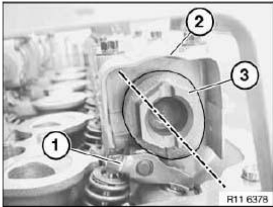
Fig. 165: Identifying Roller Cam Follower And Exhaust Camshaft Courtesy of BMW OF NORTH AMERICA, INC.
