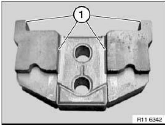
Fig. 245: Identifying Guide Block Contact Surfaces Courtesy of BMW OF NORTH AMERICA, INC.
