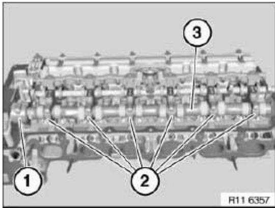
Fig. 166: Identifying Thrust Bearing Screws And Cap Courtesy of BMW OF NORTH AMERICA, INC.
