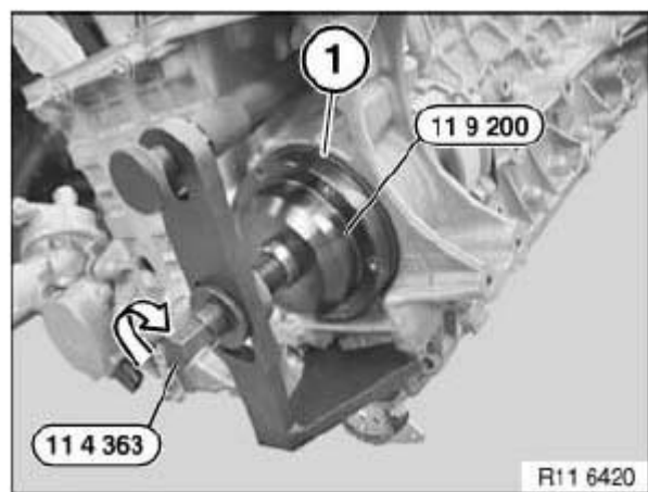
Fig. 85: Identifying Special Tool (11 4 363), (11 9 200) And New Sealing Cover Courtesy of BMW OF NORTH AMERICA, INC.
