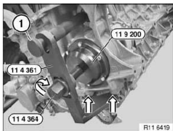
Fig. 84: Identifying Special Tool (11 4 361), (11 4 364), (11 9 200) And Knurled Screw Courtesy of BMW OF NORTH AMERICA, INC.
