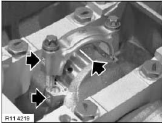
Fig. 129: Locating Conrod Bearing Clearance Courtesy of BMW OF NORTH AMERICA, INC.
