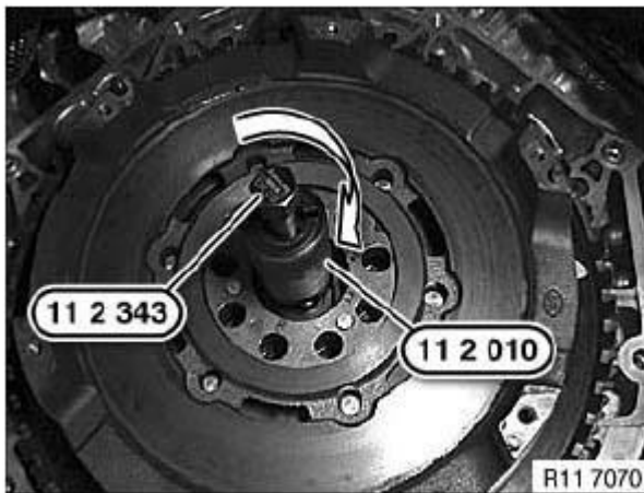
Fig. 121: Identifying Special Tool (11 2 010) And (11 2 343) Courtesy of BMW OF NORTH AMERICA, INC.
