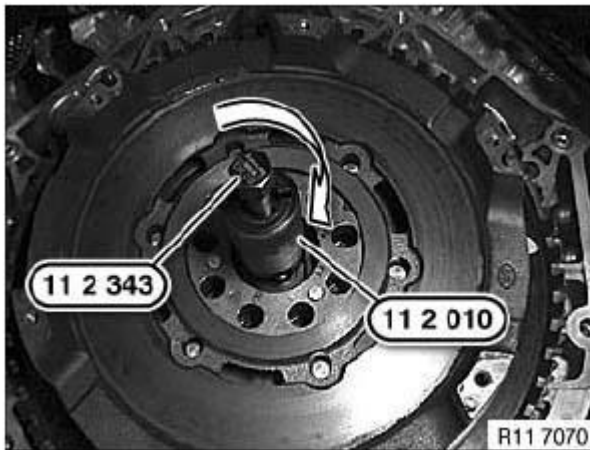
Fig. 123: Identifying Special Tool (11 2 010) And (11 2 343) Courtesy of BMW OF NORTH AMERICA, INC.
