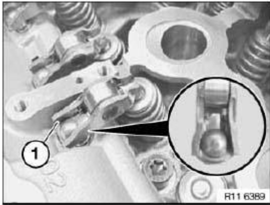
Fig. 175: Identifying Rocker Arms Position Courtesy of BMW OF NORTH AMERICA, INC.
