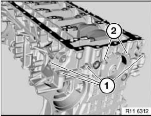
Fig. 99: Identifying Engine Screws Courtesy of BMW OF NORTH AMERICA, INC.
