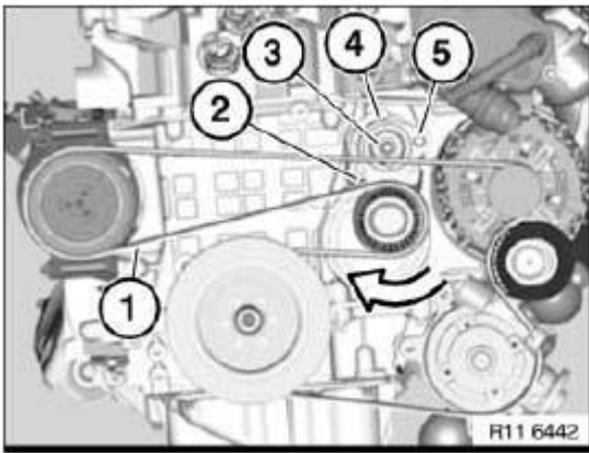
Fig. 156: Identifying Belt Tensioner And Bore Courtesy of BMW OF NORTH AMERICA, INC.
