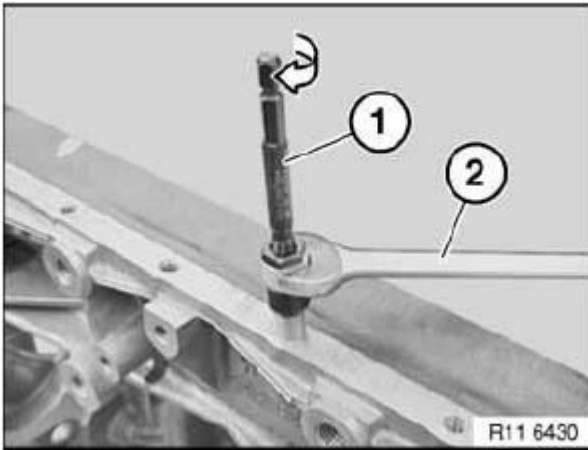
Fig. 12: Identifying Helicoil-Plus
