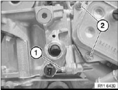
Fig. 315: Identifying Screws
