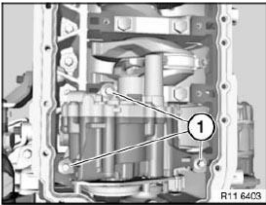
Fig. 298: Screws
