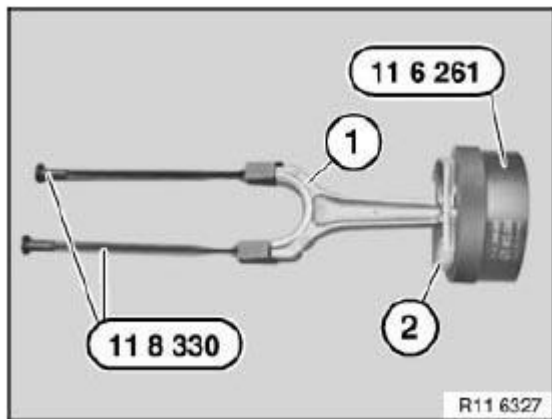
Fig. 181: Connecting Rod, Piston And Special Tools (11 8 330) And (11 6 261) Courtesy of BMW OF NORTH AMERICA, INC.
