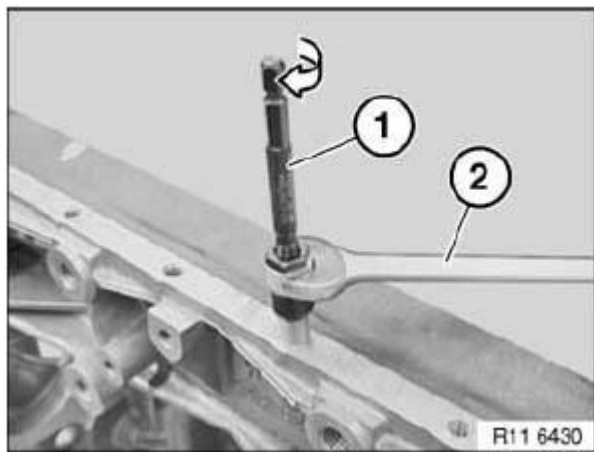
Fig. 12: Identifying Helicoil-Plus
