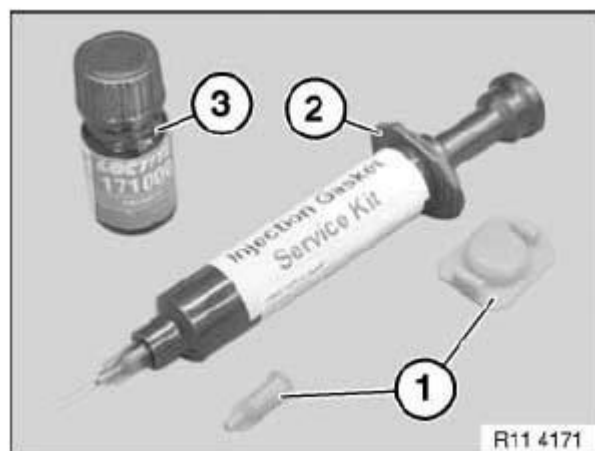
Fig. 75: Identifying Screw Caps, Injector And Loctite Sealing Compound (128357) Courtesy of BMW OF NORTH AMERICA, INC.
