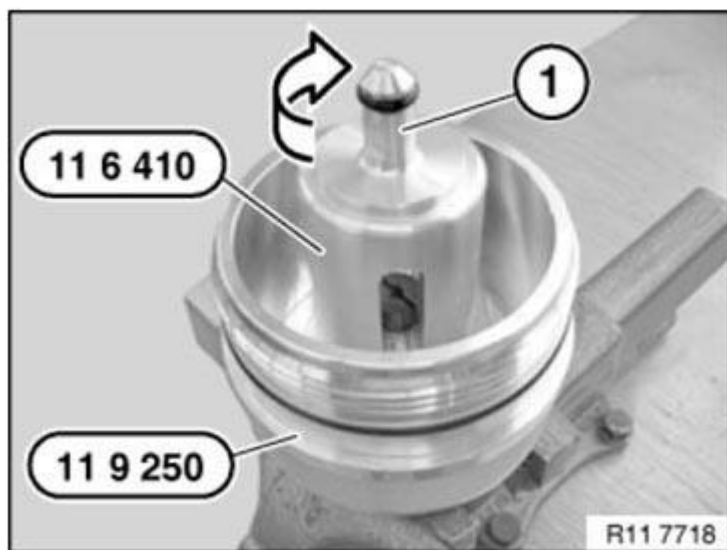
Fig. 363: Tightening Screw Piece Courtesy of BMW OF NORTH AMERICA, INC.
