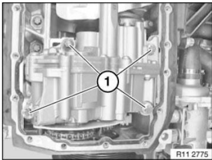
Fig. 148: Identifying Screws
