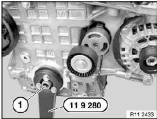
Fig. 371: Identifying Central Bolt With Special Tool (11 9 280) Courtesy of BMW OF NORTH AMERICA, INC.
