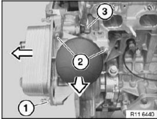
Fig. 389: Releasing Screws
