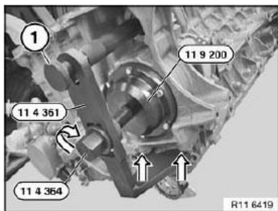
Fig. 112: Connecting Special Tool 11 4 364 Into Special Tool 11 9 200 And Screwing Out Courtesy of BMW OF NORTH AMERICA, INC.
