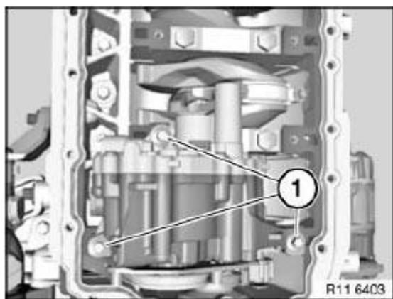
Fig. 385: Identifying Screws
