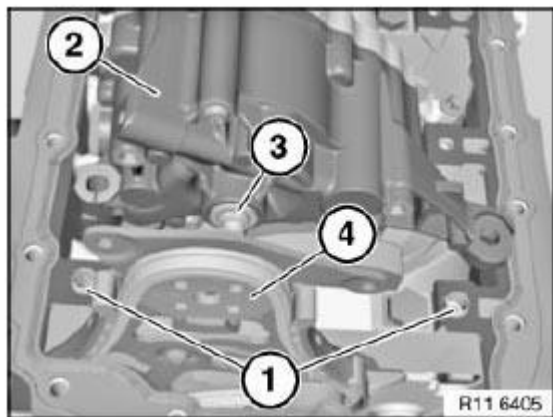
Fig. 387: Identifying Spacer Bushings And Oil Pump Courtesy of BMW OF NORTH AMERICA, INC.
