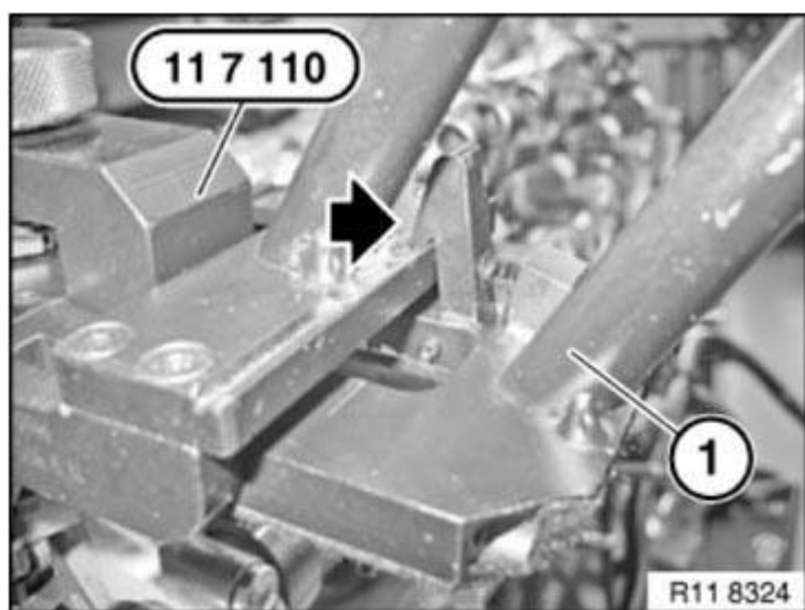
Fig. 352: Clamping Return Spring With Knurled Screw Courtesy of BMW OF NORTH AMERICA, INC.
