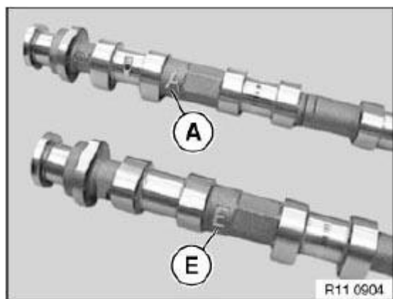
Fig. 264: Identifying Exhaust Camshaft And Inlet Camshaft Courtesy of BMW OF NORTH AMERICA, INC.
