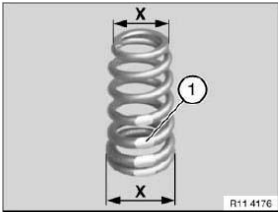
Fig. 286: Identifying Valve Spring Dimensions Courtesy of BMW OF NORTH AMERICA, INC.
