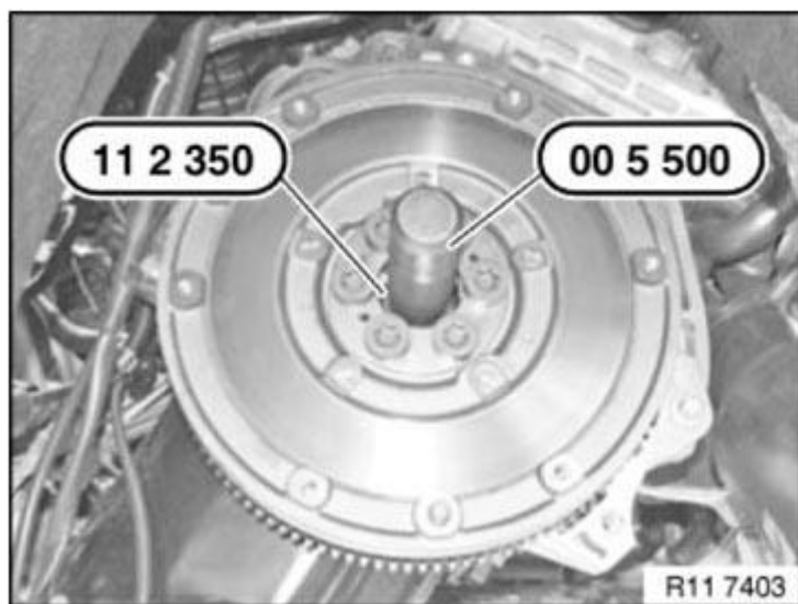
Fig. 140: Installing New Thrust Bearing Using Special Tool 11 2 350 And 00 5 500 Courtesy of BMW OF NORTH AMERICA, INC.
