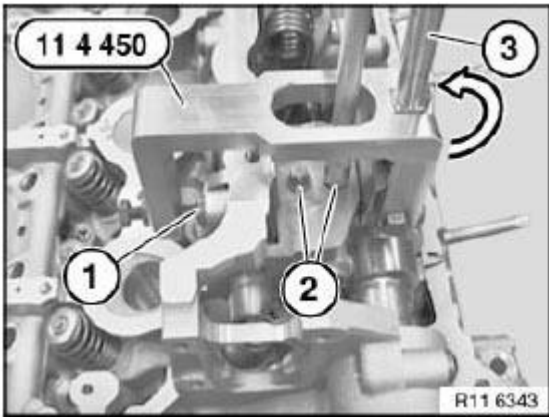
Fig. 349: Turning Eccentric Lever Courtesy of BMW OF NORTH AMERICA, INC.
