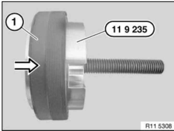
Fig. 176: Pushing Radial Shaft Seal (11 9 235) On Special Tool Courtesy of BMW OF NORTH AMERICA, INC.
