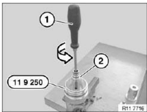
Fig. 360: Releasing Insert Using Screwdriver Courtesy of BMW OF NORTH AMERICA, INC.
