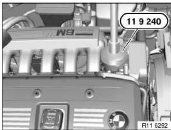
Fig. 18: Removing Oil Filter Cap With Special Tool Courtesy of BMW OF NORTH AMERICA, INC.
