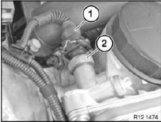
Fig. 395: Identifying Oil Pressure Switch And Plug Connection Courtesy of BMW OF NORTH AMERICA, INC.
