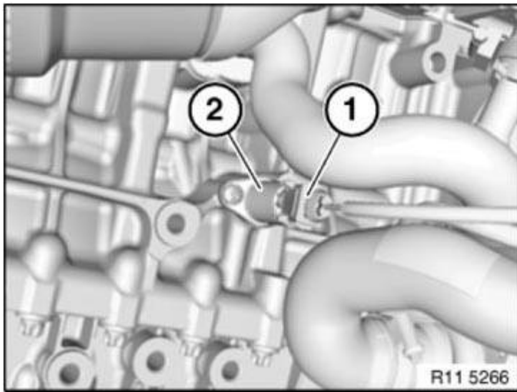
Fig. 380: Identifying Hydraulic Valve With Plug Courtesy of BMW OF NORTH AMERICA, INC.
