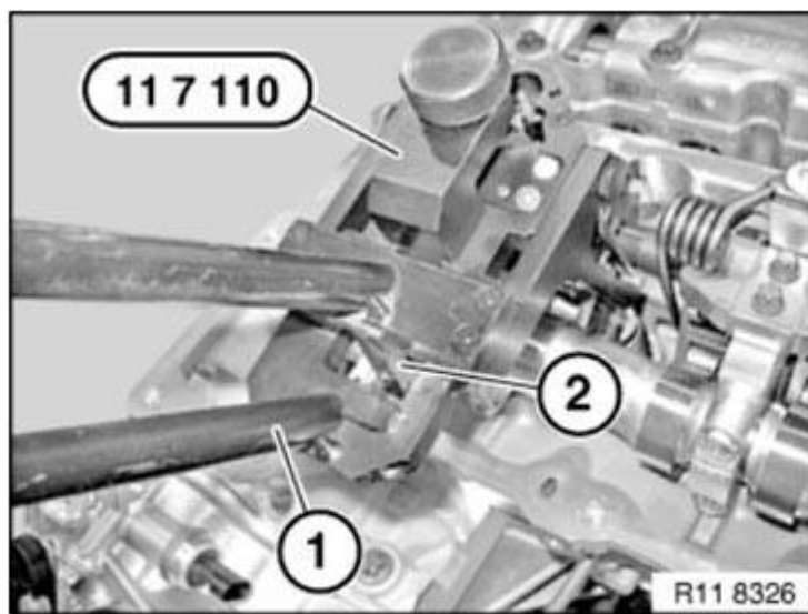
Fig. 338: Identifying Latching Hook, Lever With Special Tool 11 7 110 Courtesy of BMW OF NORTH AMERICA, INC.
