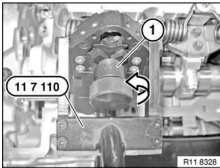
Fig. 339: Releasing Knurled Screw On Special Tool 11 7 110 Courtesy of BMW OF NORTH AMERICA, INC.
