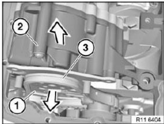
Fig. 386: Pulling Drive Gear Courtesy of BMW OF NORTH AMERICA, INC.
