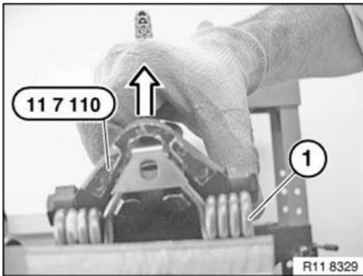
Fig. 351: Positioning Special Tool 11 7 110 On Return Spring Courtesy of BMW OF NORTH AMERICA, INC.
