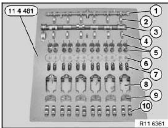
Fig. 342: Identifying Components With Special Tool (11 4 481) Courtesy of BMW OF NORTH AMERICA, INC.
