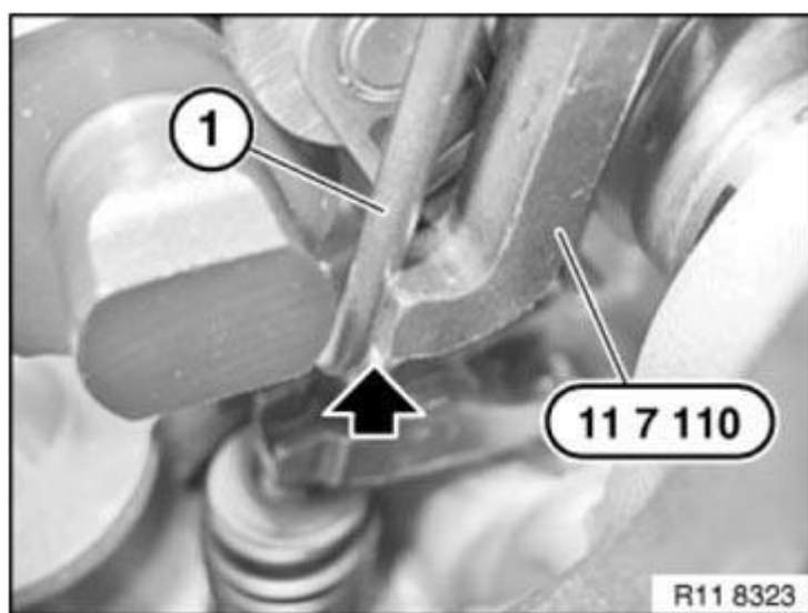
Fig. 270: Positioning Return Spring Courtesy of BMW OF NORTH AMERICA, INC.
