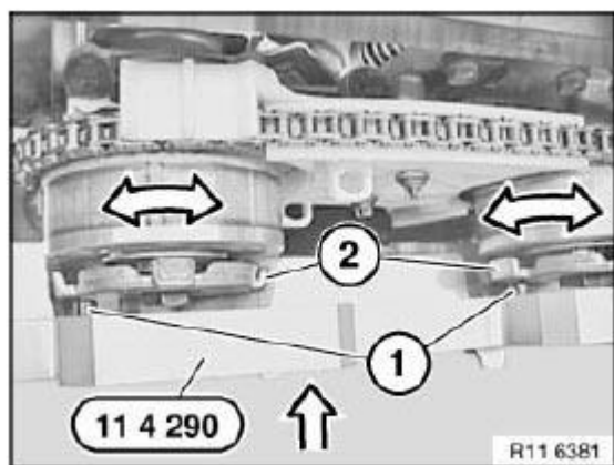
Fig. 217: Identifying Sensor Gears And Pins Courtesy of BMW OF NORTH AMERICA, INC.
