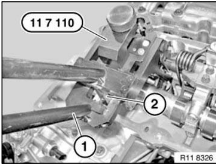
Fig. 274: Pressing Latching Hook Courtesy of BMW OF NORTH AMERICA, INC.
