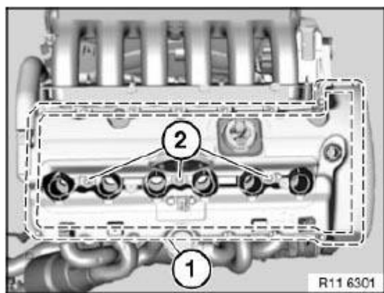
Fig. 34: Identifying Screws
