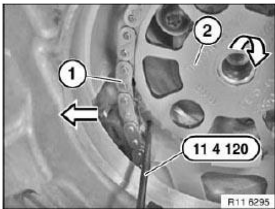
Fig. 327: Removing Camshaft Sprocket Courtesy of BMW OF NORTH AMERICA, INC.
