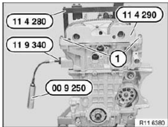
Fig. 218: Identifying Special Tools Courtesy of BMW OF NORTH AMERICA, INC.
