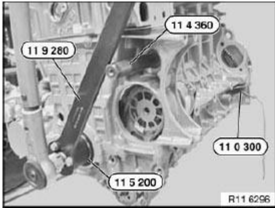
Fig. 207: Identifying Special Tools Courtesy of BMW OF NORTH AMERICA, INC.
