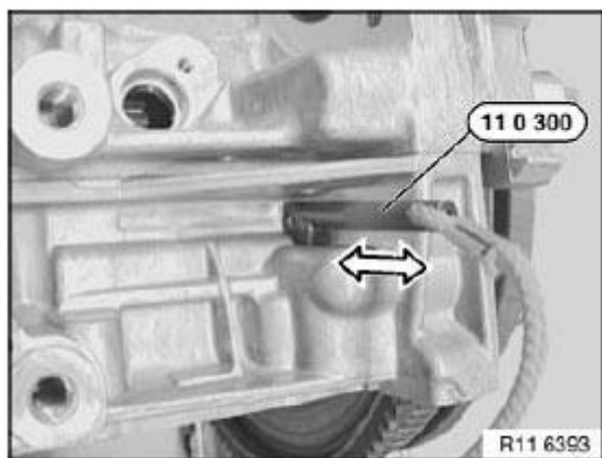
Fig. 194: Securing Crankshaft
