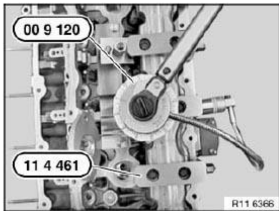
Fig. 192: Tightening Lower And Upper Bearing Banks With Special Tool Courtesy of BMW OF NORTH AMERICA, INC.
