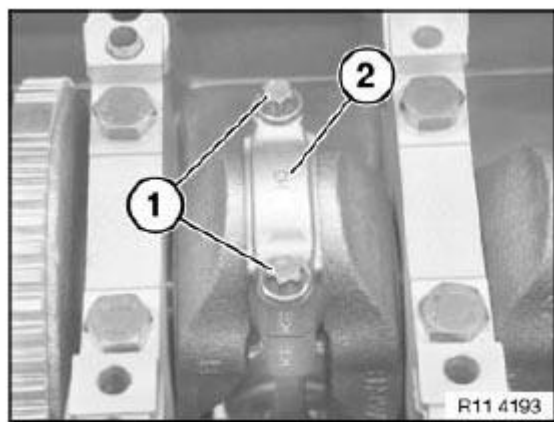
Fig. 155: Identifying Bearing Caps And Conrod Bolts
