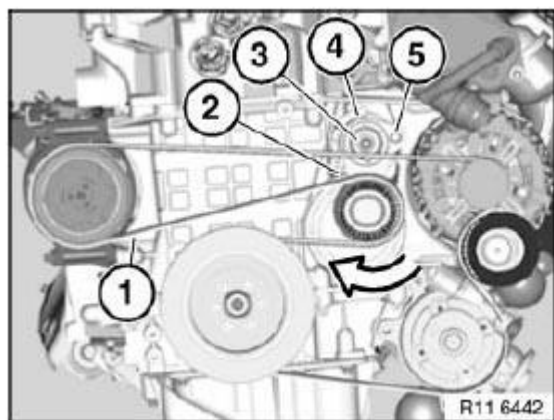
Fig. 166: Removing Drive Belt Towards Top Courtesy of BMW OF NORTH AMERICA, INC.
