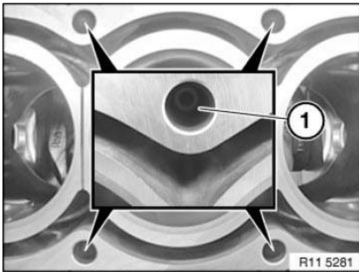
Fig. 49: Identifying Threaded Hole Courtesy of BMW OF NORTH AMERICA, INC.
