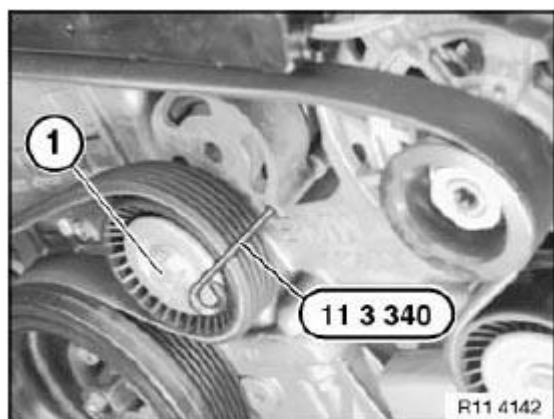
Fig. 165: Securing Belt Tensioner With Special Tool Courtesy of BMW OF NORTH AMERICA, INC.
