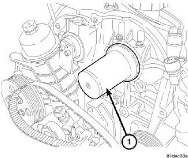
Fig. 125: CAMSHAFT OIL SEAL INSTALLATION Courtesy of CHRYSLER LLC
