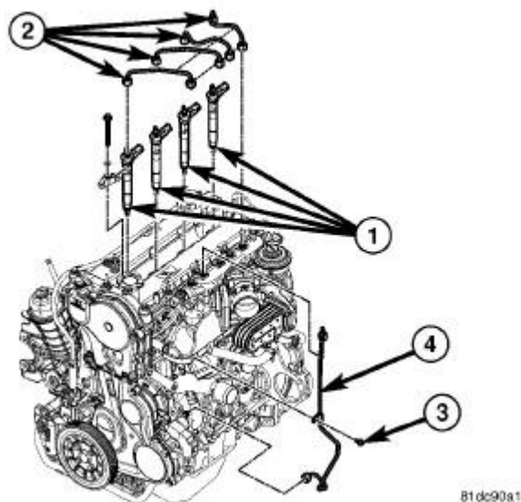
Fig. 104: DIESEL FUEL INJECTORS Courtesy of CHRYSLER LLC
