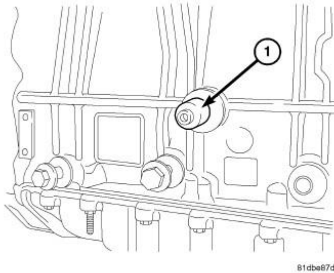
Fig. 324: CRANKSHAFT LOCKING TOOL Courtesy of CHRYSLER LLC
