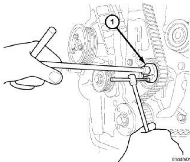
Fig. 329: TIMING BELT TENSIONER TIGHTEN Courtesy of CHRYSLER LLC
