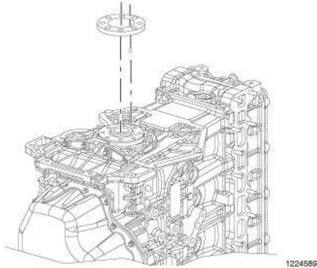
Fig. 209: FLYWHEEL & CRANKSHAFT Courtesy of CHRYSLER LLC
