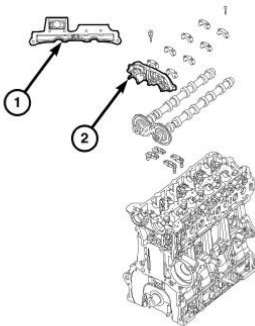
Fig. 80: CAMSHAFT CAP RTV LOCATION Courtesy of CHRYSLER LLC
