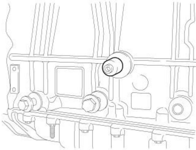
Fig. 158: CRANKSHAFT LOCKING TOOL Courtesy of CHRYSLER LLC
