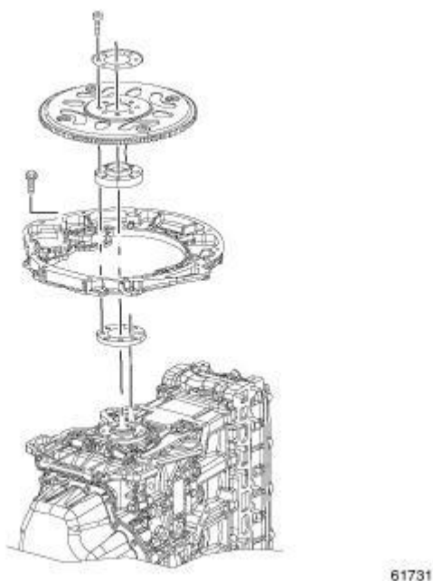
Fig. 176: FLYWHEEL AND FLEX PLATE
