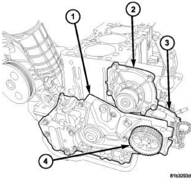
Fig. 138: OIL PUMP COVER ASSEMBLY
