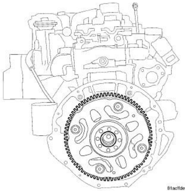
Fig. 153: FLEX PLATE - INSTALLED Courtesy of CHRYSLER LLC
