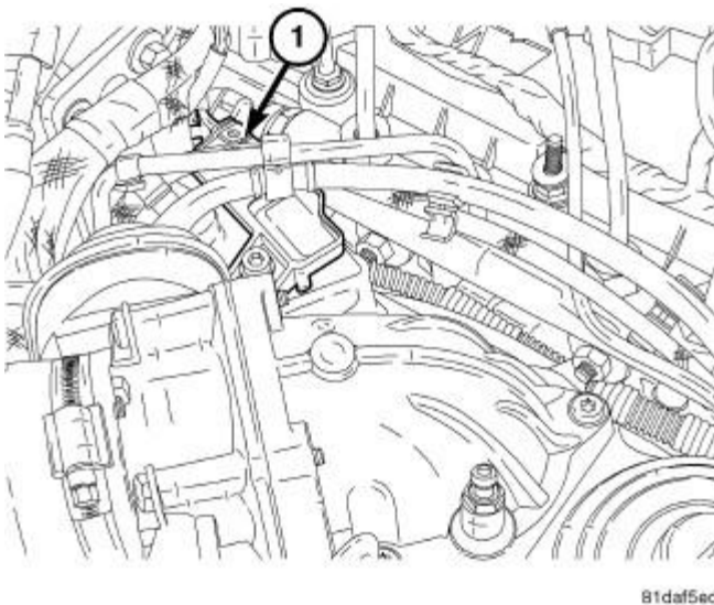
Fig. 30: IAT/BPS SENSOR Courtesy of CHRYSLER LLC
