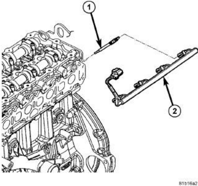
Fig. 284: Glow Plugs & Wiring Harness Courtesy of CHRYSLER LLC
