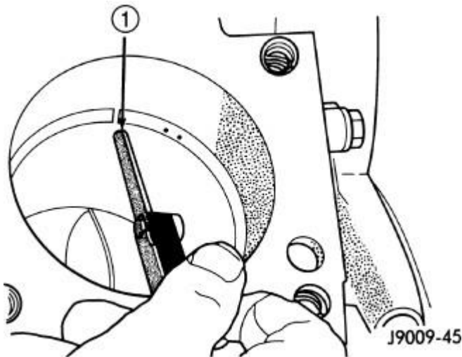
Fig. 187: RING END GAP MEASUREMENT
