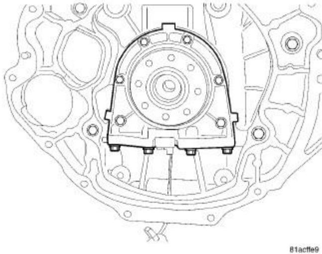
Fig. 244: REAR MAIN SEAL AND OIL PAN BOLTS Courtesy of CHRYSLER LLC
