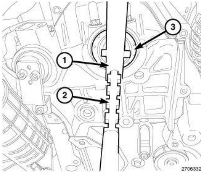
Fig. 124: IDENTIFYING SEAL REMOVER HANDLE, SEAL REMOVER & INTAKE CAMSHAFT OIL SEAL Courtesy of CHRYSLER LLC
