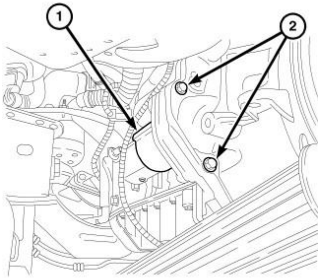
Fig. 42: STARTER MOUNTING 2.8L DIESEL Courtesy of CHRYSLER LLC
