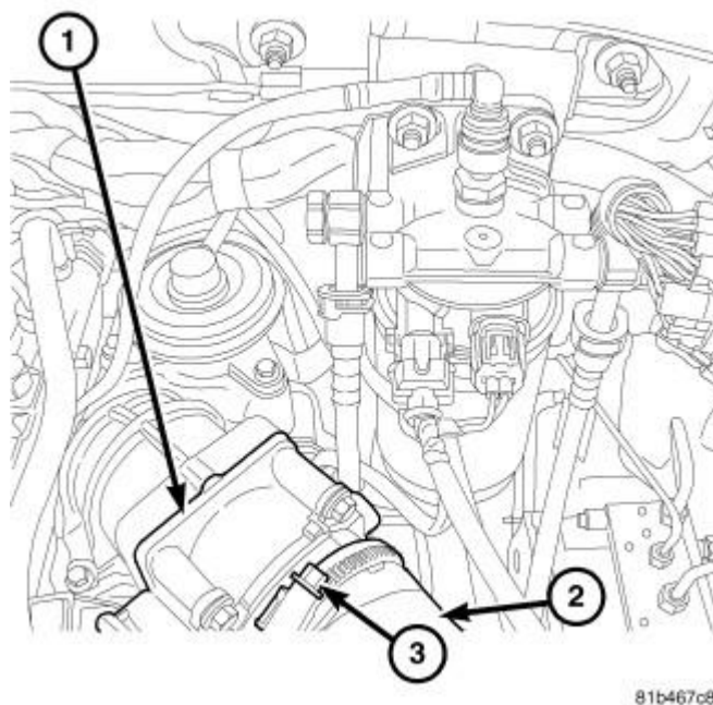
Fig. 274: AIR TUBE - EGR AIR VALVE
