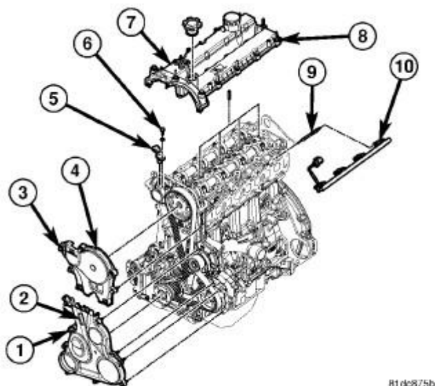
Fig. 352: UPPER FRONT COVER Courtesy of CHRYSLER LLC
