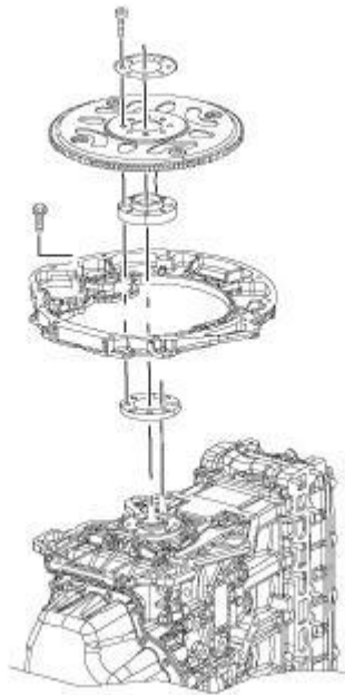
Fig. 155: FLYWHEEL AND FLEX PLATE
