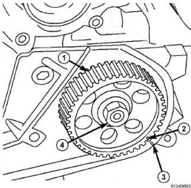
Fig. 330: FUEL INJECTION PUMP TIMING MARKS Courtesy of CHRYSLER LLC
