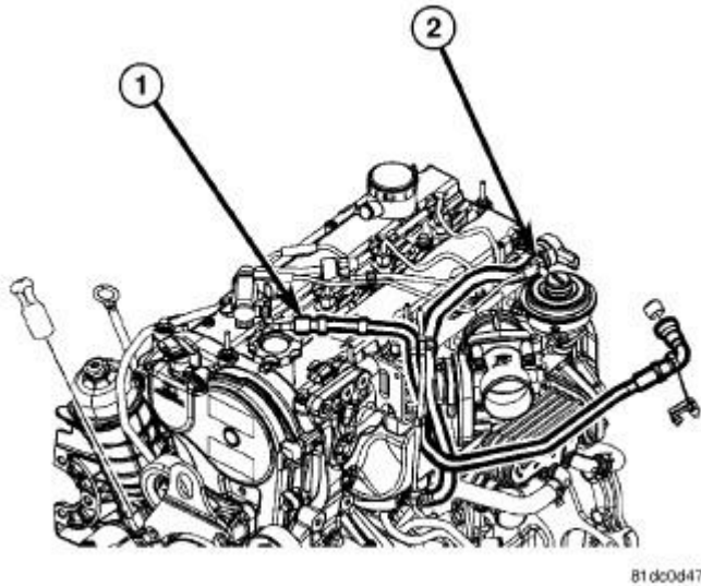
Fig. 100: FUEL RETURN LINES-TOP Courtesy of CHRYSLER LLC
