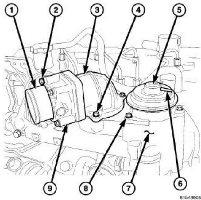
Fig. 297: EGR VALVE/EGR AIRFLOW CONTROL VALVE
