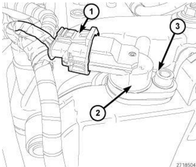
Fig. 310: CAMSHAFT POSITION SENSOR HARNESS CONNECTOR Courtesy of CHRYSLER LLC
