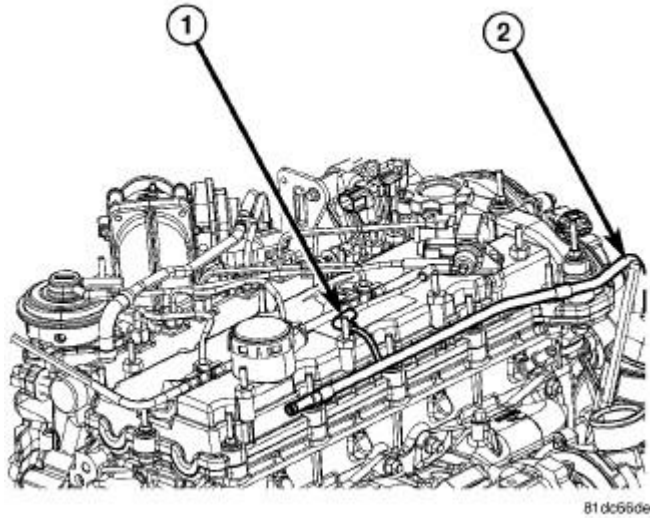
Fig. 112: VACUUM SUPPLY TUBE Courtesy of CHRYSLER LLC
