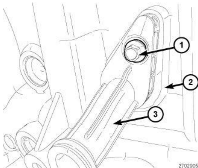
Fig. 228: IDENTIFYING COOLANT TUBE, ENGINE BLOCK & BOLT Courtesy of CHRYSLER LLC
