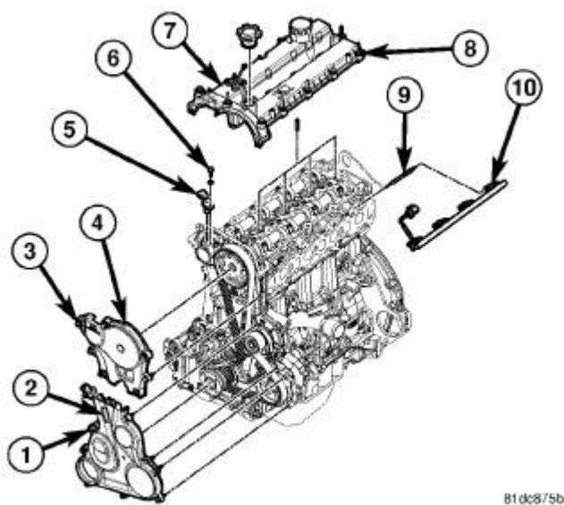
Fig. 321: UPPER AND LOWER FRONT COVERS Courtesy of CHRYSLER LLC
