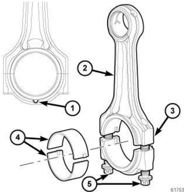
Fig. 137: CONNECTING ROD IDENTIFICATION Courtesy of CHRYSLER LLC
