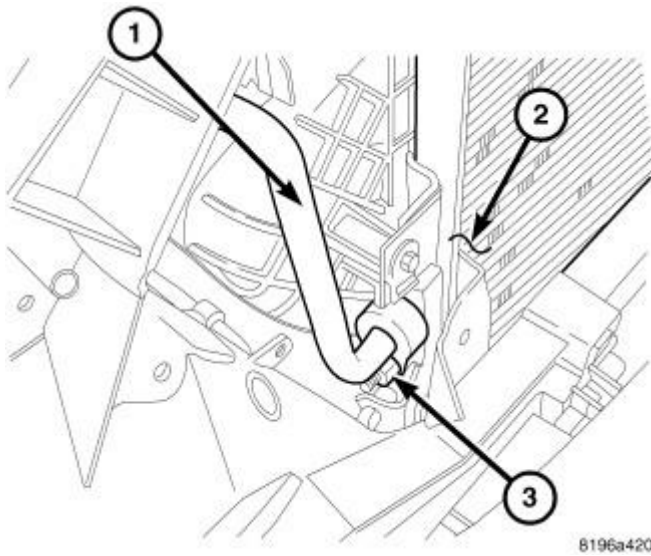
Fig. 12: Identifying Discharge Line To Condenser Diesel Courtesy of CHRYSLER LLC
