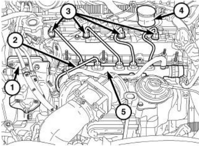
Fig. 110: FUEL RAIL
