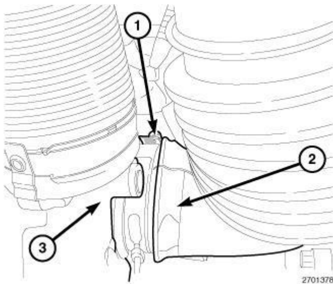
Fig. 378: IDENTIFYING WORM CLAMP, TURBOCHARGER AIR INLET TUBE & TURBOCHARGER
