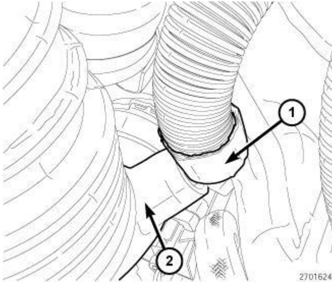
Fig. 375: OIL SEPARATOR HOSE & TURBOCHARGER AIR INLET TUBE Courtesy of CHRYSLER LLC
