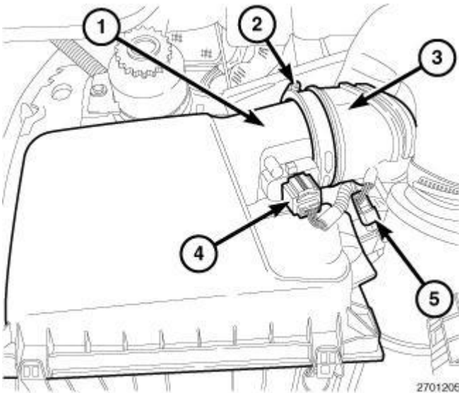
Fig. 376: IDENTIFYING AIR CLEANER HOUSING, WORM CLAMP, AIR CLEANER OUTLET TUBE, MAF SENSOR & IAT SENSOR Courtesy of CHRYSLER LLC
