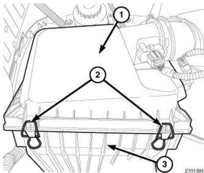
Fig. 383: IDENTIFYING AIR CLEANER HOUSING & CLIPS
