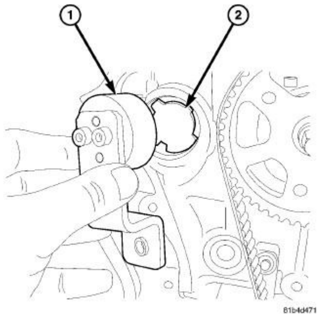
Fig. 337: INSTALLING CAMSHAFT LOCK TOOL Courtesy of CHRYSLER LLC
