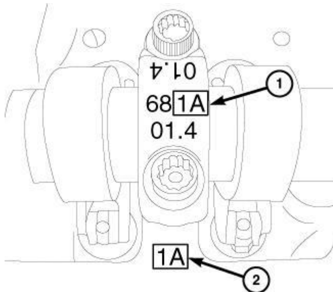
Fig. 82: CAM CAP 1A Courtesy of CHRYSLER LLC
