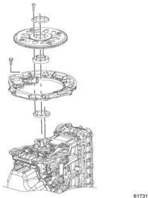
Fig. 175: FLYWHEEL AND FLEX PLATE Courtesy of CHRYSLER LLC
