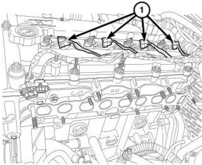
Fig. 111: FUEL INJECTORS
