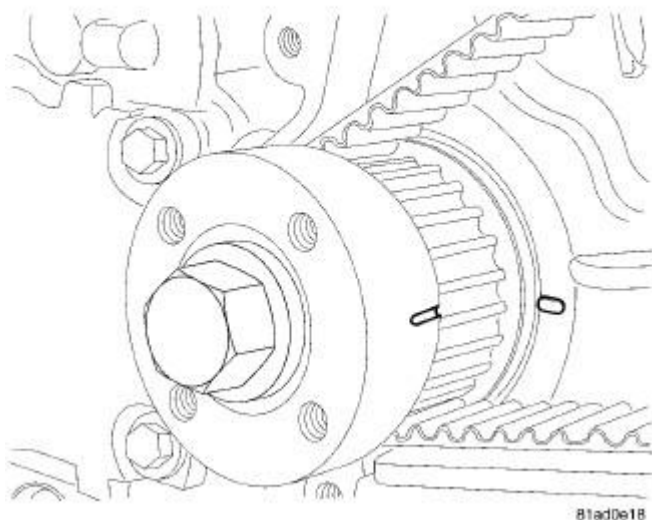
Fig. 364: CRANKSHAFT TIMING MARKS
