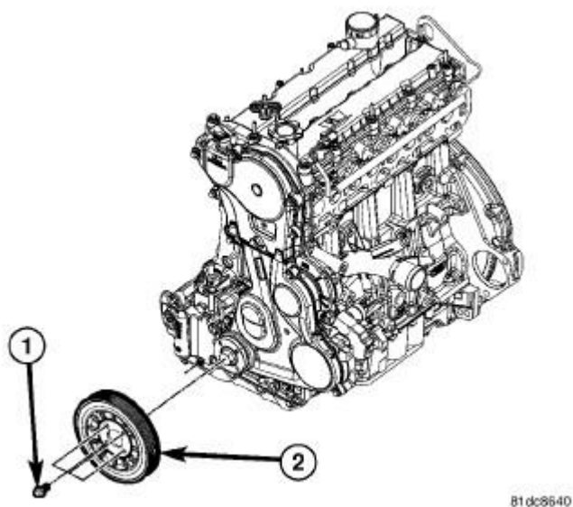
Fig. 353: LOWER FRONT COVER Courtesy of CHRYSLER LLC
