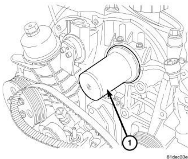
Fig. 94: CAMSHAFT OIL SEAL Courtesy of CHRYSLER LLC
