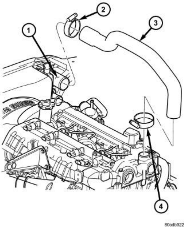
Fig. 308: CHARGE AIR COOLER INLET HOSE
