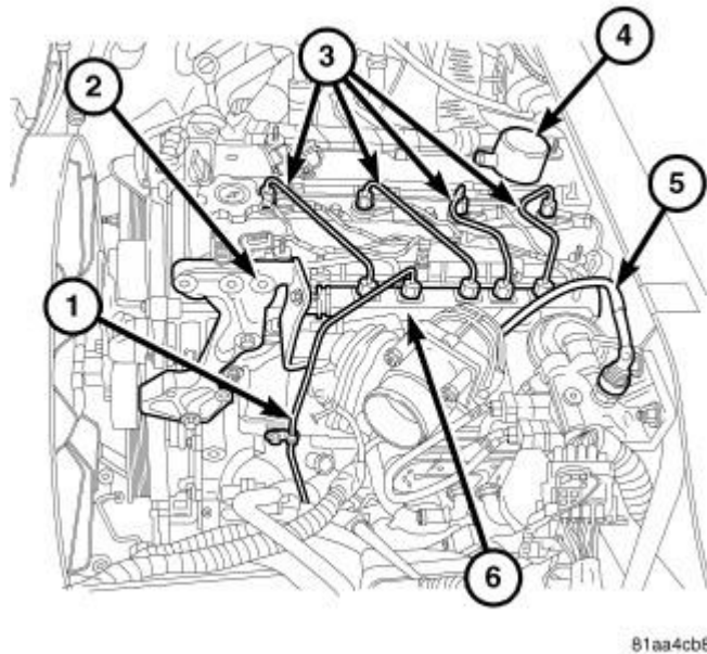
Fig. 291: FUEL RAIL
