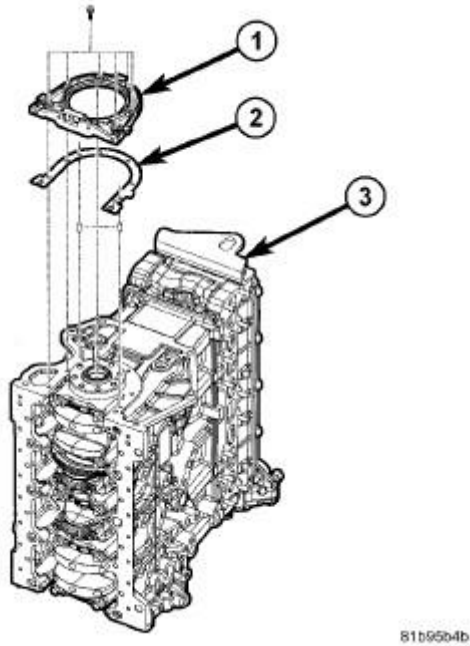
Fig. 205: REAR MAIN SEAL GASKET
