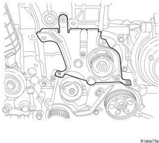
Fig. 74: INNER FRONT COVER
