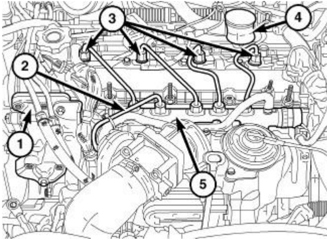
Fig. 18: FUEL RAIL
