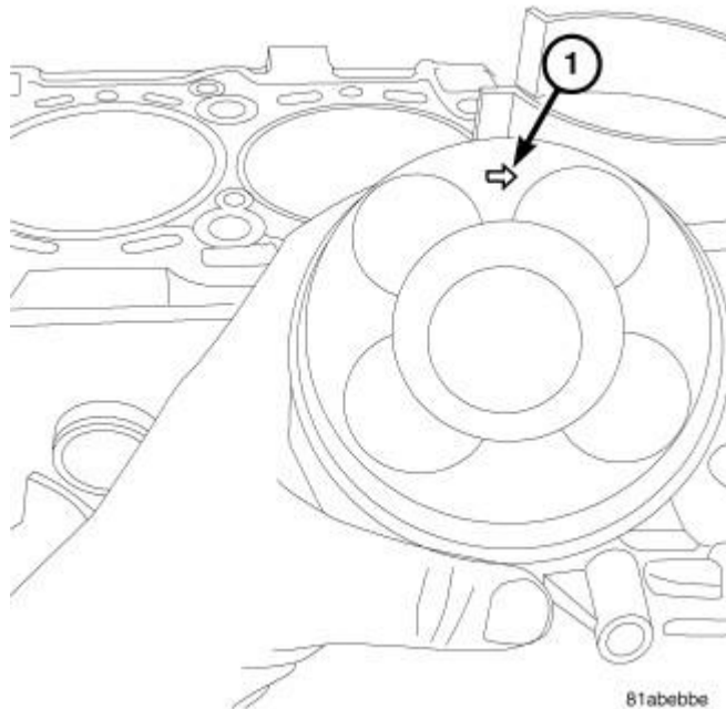
Fig. 197: PISTON DIRECTION Courtesy of CHRYSLER LLC
