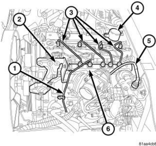
Fig. 265: FUEL RAIL
