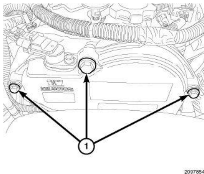
Fig. 105: UPPER COVER BOLTS Courtesy of CHRYSLER LLC
