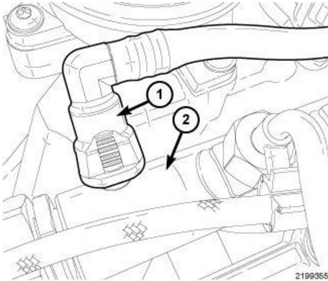
Fig. 292: FUEL RAIL & FUEL RETURN LINE Courtesy of CHRYSLER LLC
