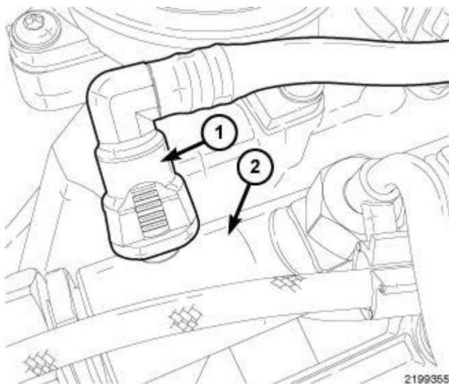
Fig. 281: FUEL RAIL & FUEL RETURN LINE Courtesy of CHRYSLER LLC
