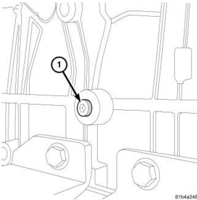
Fig. 313: CRANKSHAFT LOCK PLUG LOCATION
