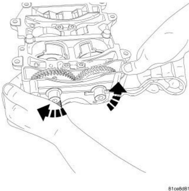
Fig. 165: BALANCE SHAFT TOOL INSTALLATION Courtesy of CHRYSLER LLC
