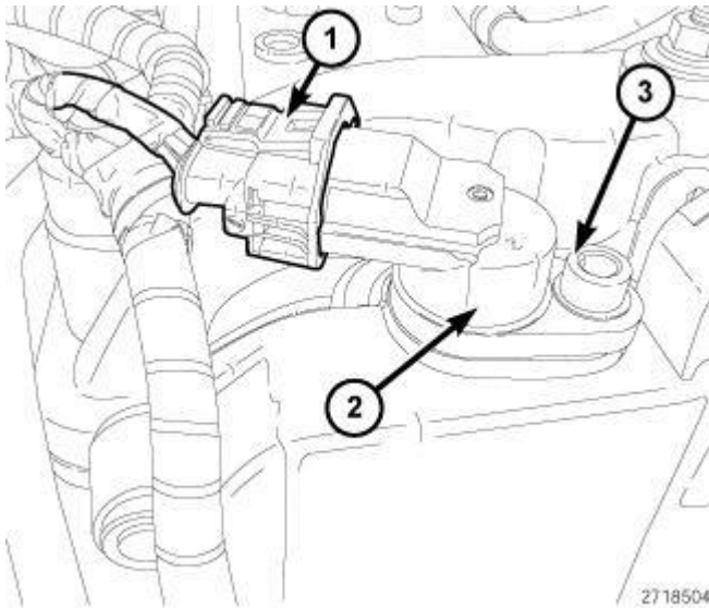
Fig. 316: CAMSHAFT POSITION SENSOR HARNESS CONNECTOR Courtesy of CHRYSLER LLC
