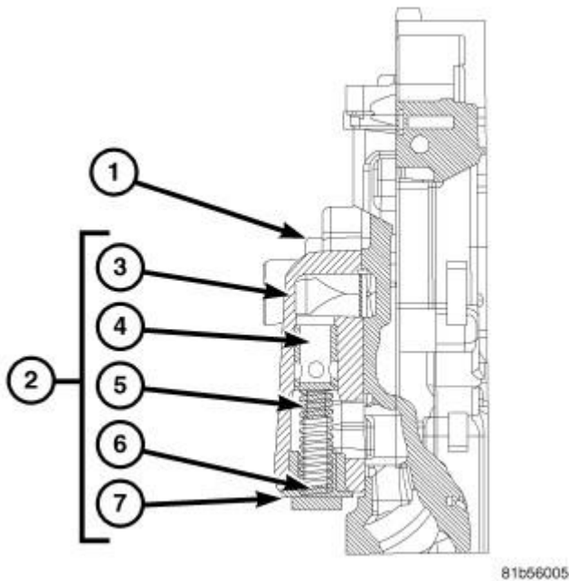
Fig. 266: FRONT COVER COMPONENTS
