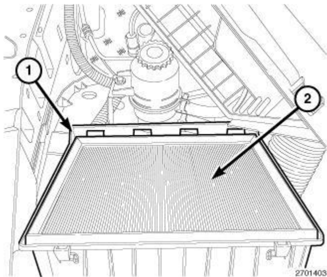
Fig. 381: AIR CLEANER HOUSING & AIR CLEANER FILTER Courtesy of CHRYSLER LLC
