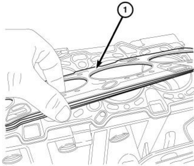
Fig. 71: MLS GASKET Courtesy of CHRYSLER LLC
