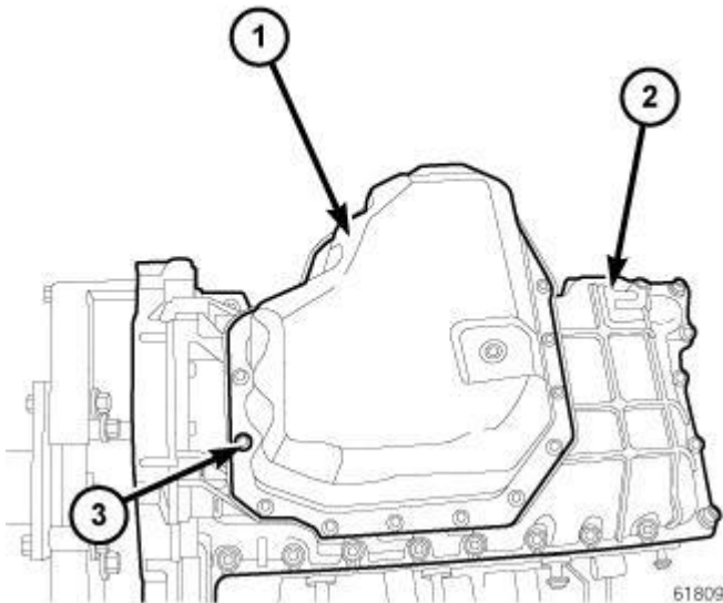
Fig. 257: LOWER OIL PAN Courtesy of CHRYSLER LLC
