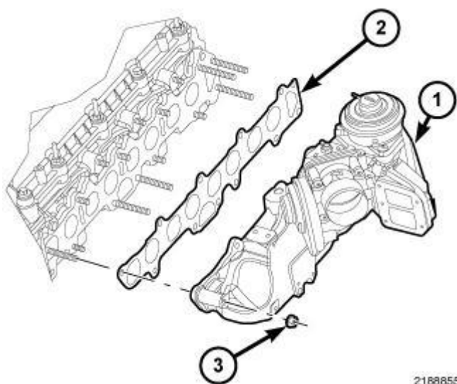
Fig. 287: IDENTIFYING MANIFOLD RETAINING NUTS, INTAKE MANIFOLD & INTAKE MANIFOLD GASKET
