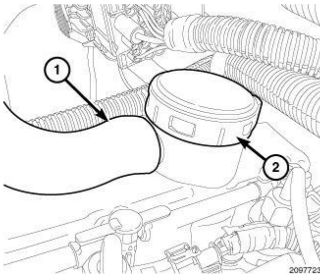
Fig. 99: CRANKCASE VENT HOSE & OIL SEPARATOR Courtesy of CHRYSLER LLC
