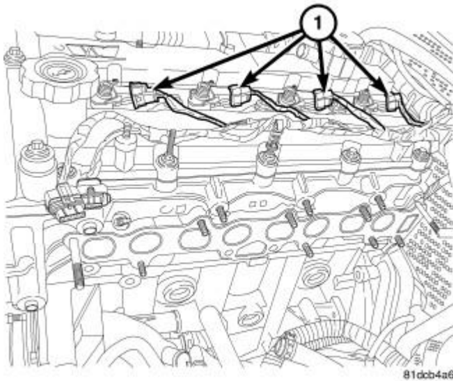
Fig. 102: FUEL INJECTORS Courtesy of CHRYSLER LLC
