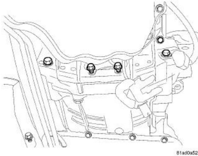
Fig. 177: BELL HOUSING BOLTS Courtesy of CHRYSLER LLC
