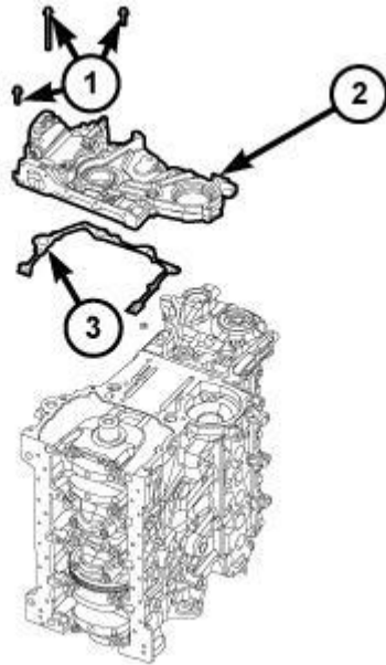
Fig. 182: FRONT COVER AND GASKET Courtesy of CHRYSLER LLC
