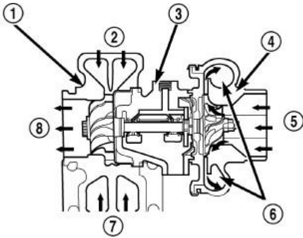
Fig. 301: Turbocharger Operation Courtesy of CHRYSLER LLC
