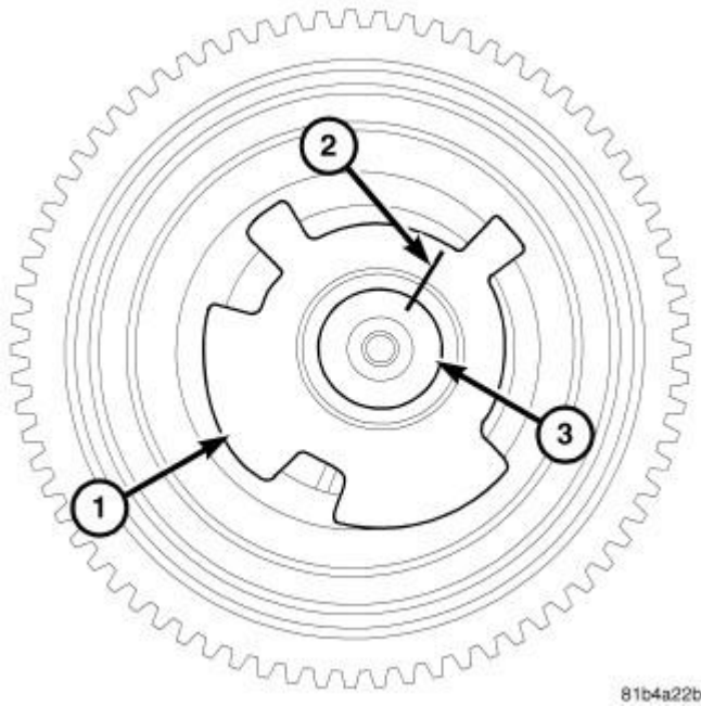
Fig. 340: MARK THE CAMSHAFT Courtesy of CHRYSLER LLC
