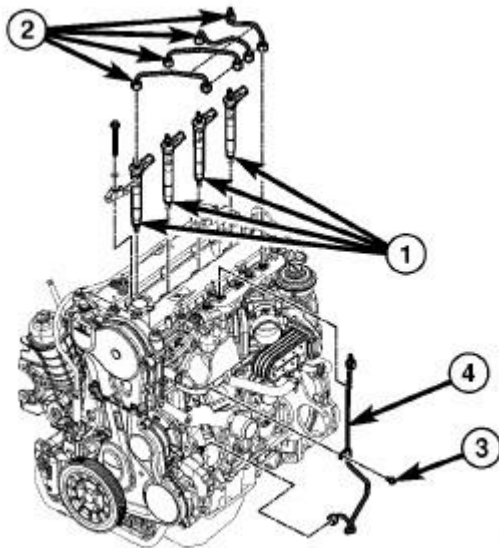
Fig. 109: DIESEL FUEL INJECTORS Courtesy of CHRYSLER LLC
