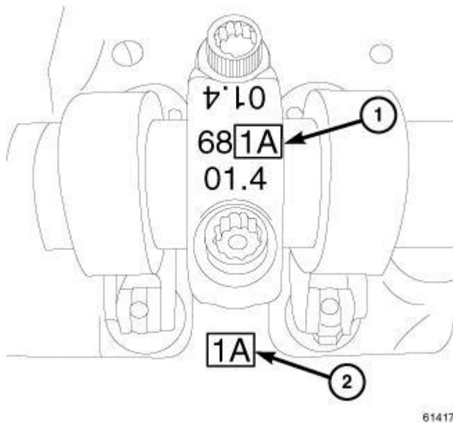
Fig. 86: CAM CAP 1A Courtesy of CHRYSLER LLC
