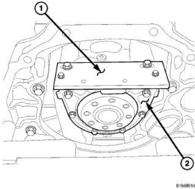
Fig. 207: REAR SEAL TOOL INSTALLED Courtesy of CHRYSLER LLC
