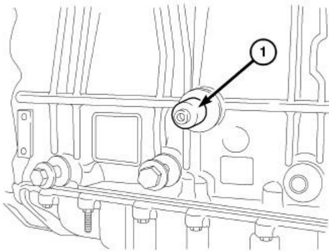
Fig. 314: CRANKSHAFT LOCKING TOOL Courtesy of CHRYSLER LLC
