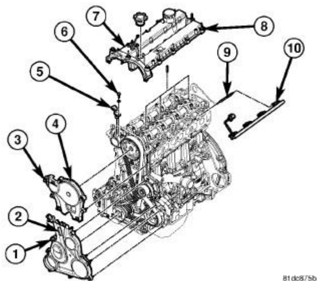
Fig. 344: UPPER AND LOWER FRONT COVERS
