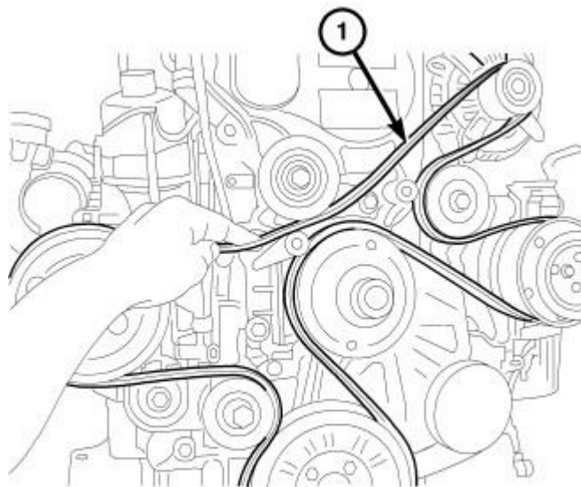
Fig. 185: ACCESSORY DRIVE BELT REMOVED
