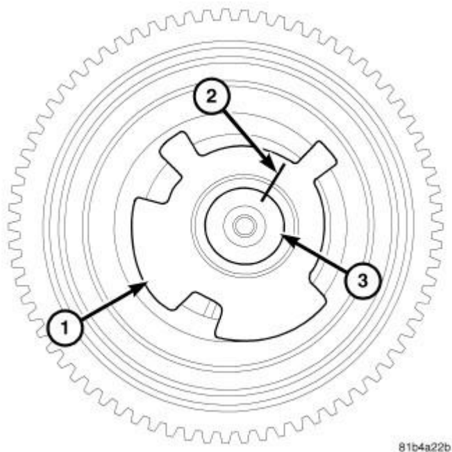
Fig. 327: MARK THE CAMSHAFT Courtesy of CHRYSLER LLC
