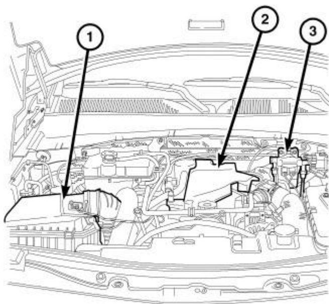
Fig. 267: ENGINE COVER
