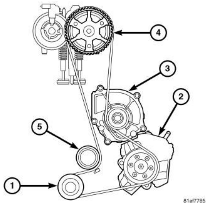
Fig. 140: TIMING BELT TENSIONER Courtesy of CHRYSLER LLC
