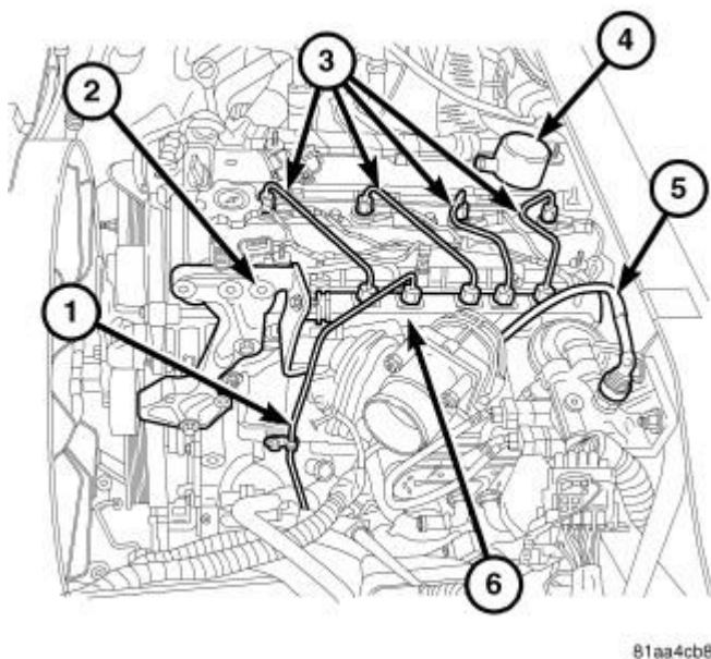
Fig. 264: FUEL RAIL
