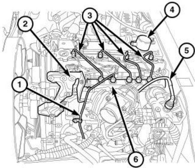
Fig. 282: FUEL RAIL
