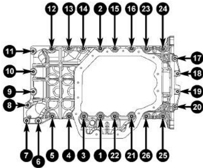
Fig. 170: OIL SUMP TORQUE SEQUENCE
