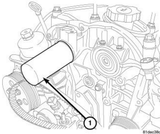
Fig. 341: CAMSHAFT OIL SEAL Courtesy of CHRYSLER LLC
