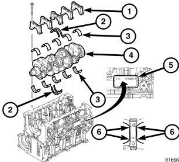
Fig. 133: CRANKSHAFT BEARING SIZE MARK Courtesy of CHRYSLER LLC
