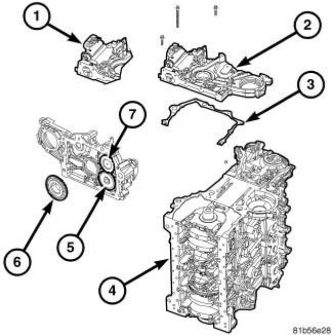
Fig. 262: VACUUM PUMP AND OIL PUMP Courtesy of CHRYSLER LLC
