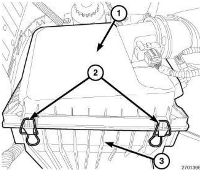
Fig. 379: IDENTIFYING AIR CLEANER HOUSING & CLIPS
