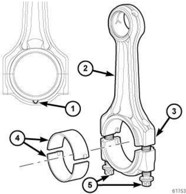
Fig. 134: CONNECTING ROD IDENTIFICATION
