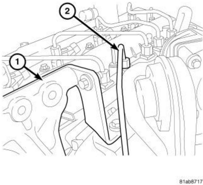
Fig. 293: GENERATOR BRACKET Courtesy of CHRYSLER LLC
