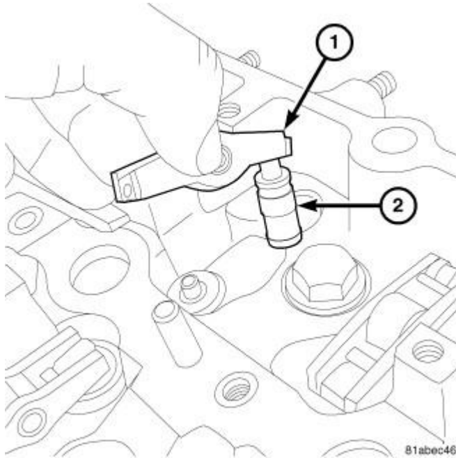
Fig. 121: ROCKER ARM AND LIFTER ASSEMBLY Courtesy of CHRYSLER LLC
