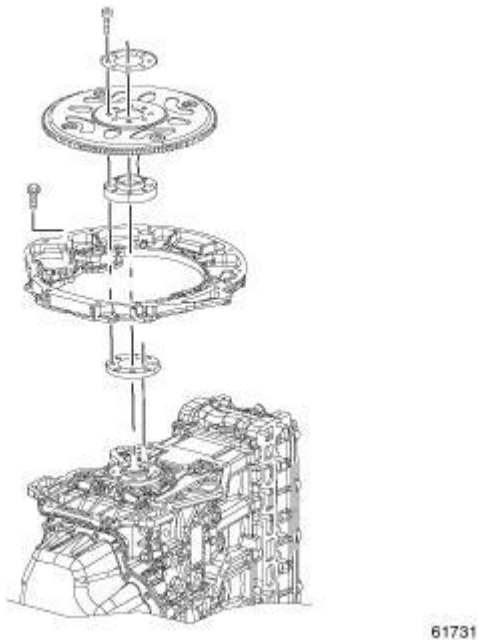
Fig. 173: FLYWHEEL AND FLEX PLATE Courtesy of CHRYSLER LLC
