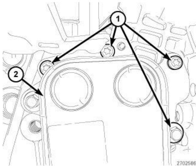
Fig. 215: ENGINE OIL COOLER & BOLTS Courtesy of CHRYSLER LLC
