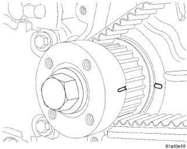
Fig. 312: CRANKSHAFT TIMING MARKS
