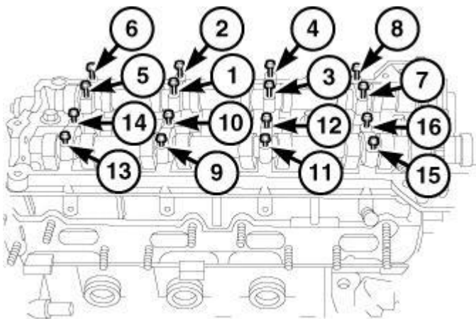
Fig. 88: IDENTIFYING TIGHTENING SEQUENCE
