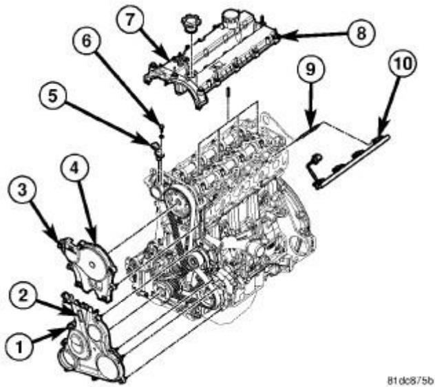
Fig. 79: CYLINDER HEAD COVER Courtesy of CHRYSLER LLC
