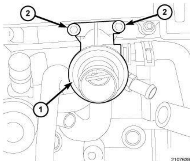
Fig. 288: THERMOSTAT HOUSING
