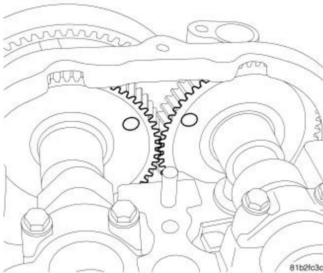
Fig. 91: CAMSHAFT MARKS AT 90° ATDC Courtesy of CHRYSLER LLC
