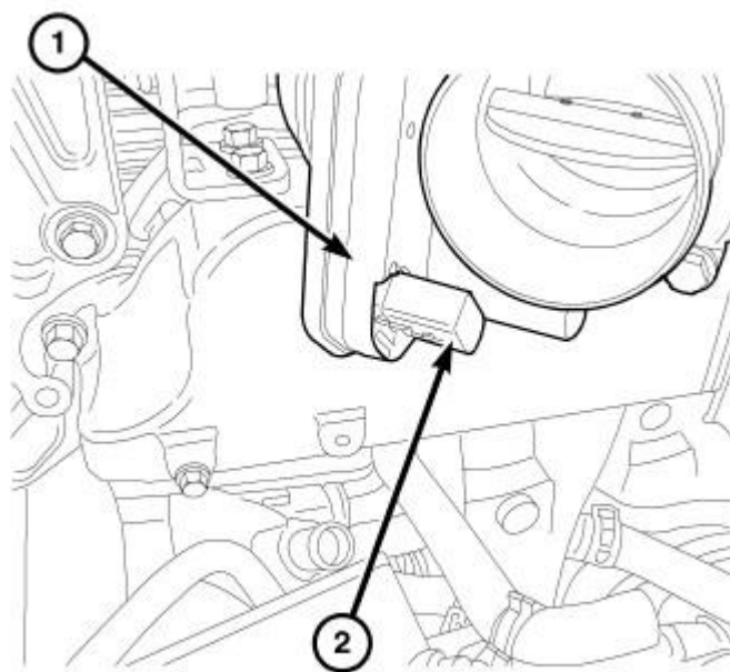
Fig. 298: ELECTRICAL CONNECTOR - EGR AIR VALVE Courtesy of CHRYSLER LLC
