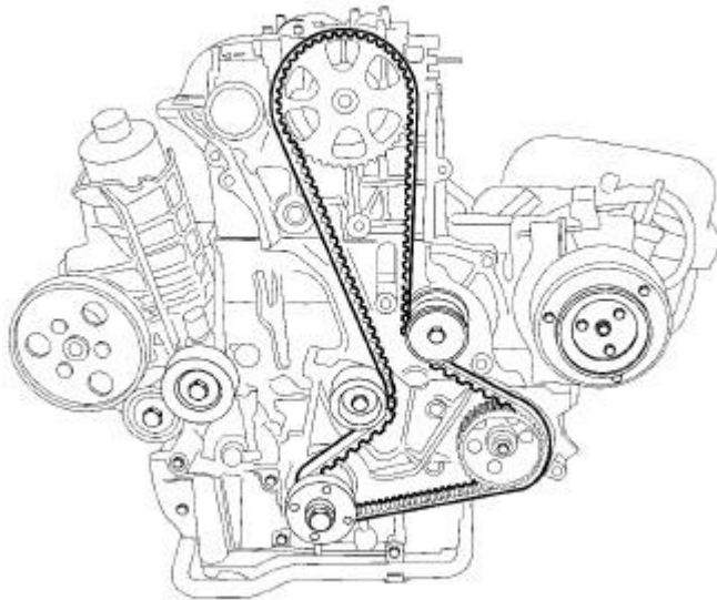
Fig. 333: TIMING BELT
