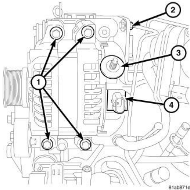
Fig. 296: GENERATOR Courtesy of CHRYSLER LLC
