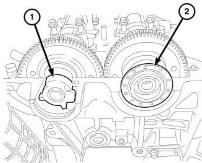
Fig. 81: CAMSHAFT OIL SEAL Courtesy of CHRYSLER LLC
