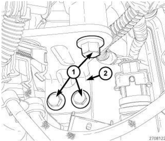
Fig. 278: GENERATOR BRACKET SUPPORT & BOLTS Courtesy of CHRYSLER LLC
