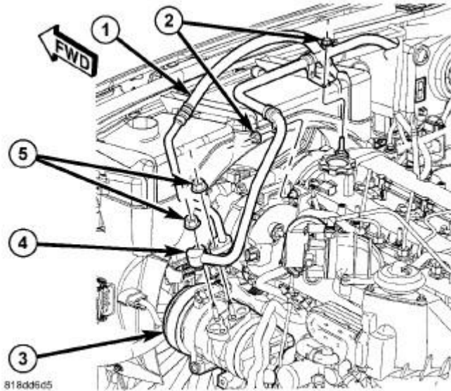
Fig. 35: Refrigerant Lines To Compressor - 2.8L Courtesy of CHRYSLER LLC
