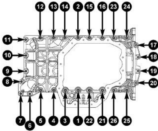
Fig. 252: OIL SUMP TORQUE SEQUENCE
