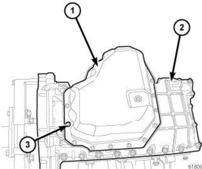
Fig. 261: LOWER OIL PAN
