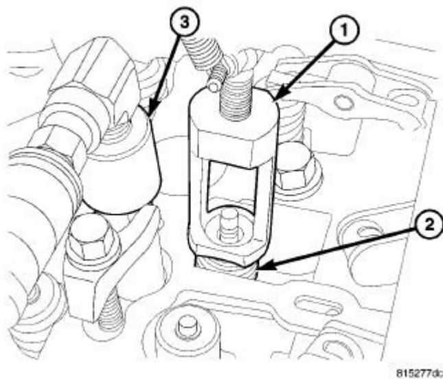
Fig. 59: MD998772A-15 ADAPTOR Courtesy of CHRYSLER LLC
