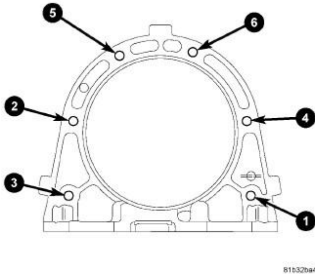
Fig. 208: REAR COVER TORQUE Courtesy of CHRYSLER LLC
