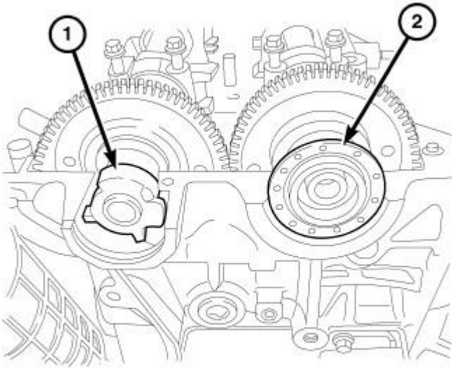
Fig. 76: CAMSHAFT OIL SEAL Courtesy of CHRYSLER LLC
