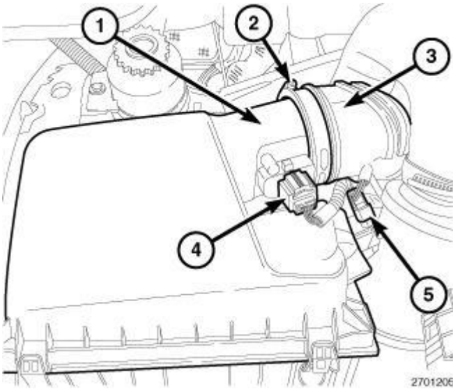
Fig. 373: IDENTIFYING AIR CLEANER HOUSING, WORM CLAMP, AIR CLEANER OUTLET TUBE, MAF SENSOR & IAT SENSOR
