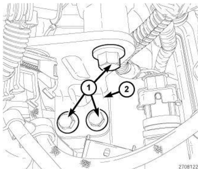
Fig. 295: GENERATOR BRACKET SUPPORT & BOLTS
