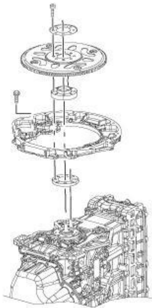
Fig. 152: FLYWHEEL AND FLEX PLATE
