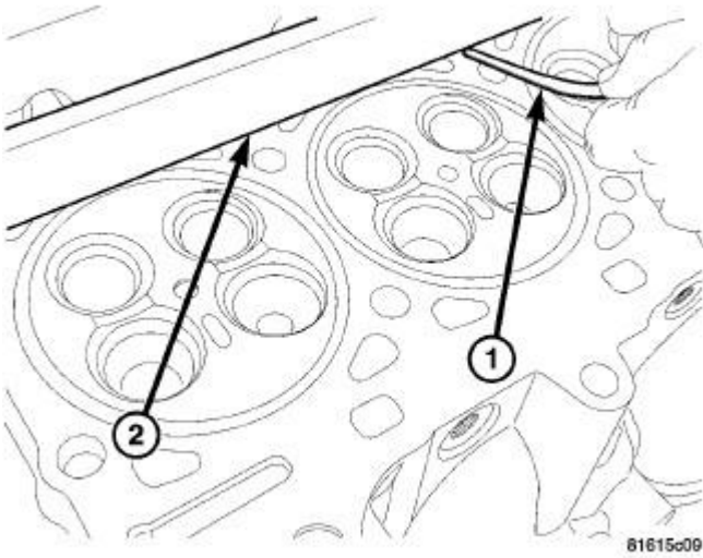
Fig. 66: CYLINDER HEAD FLATNESS - 1 Courtesy of CHRYSLER LLC
