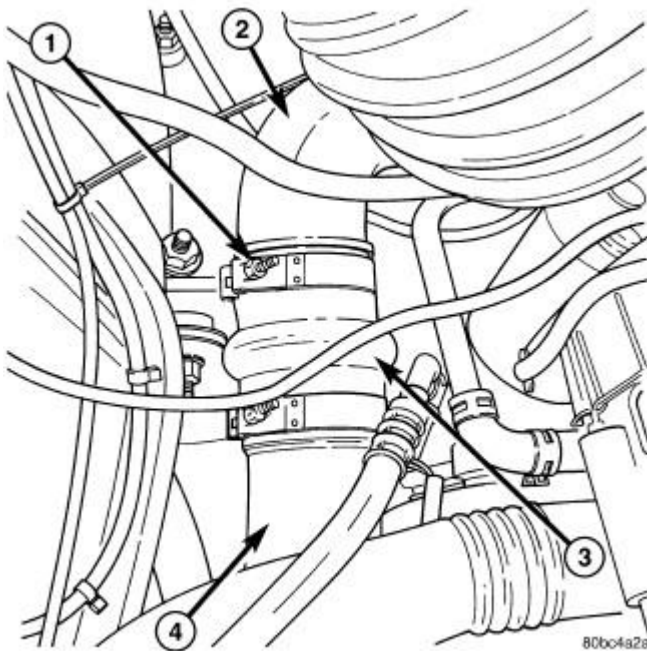
Fig. 305: AIR INLET DUCT RUBBER SLEEVE Courtesy of CHRYSLER LLC
