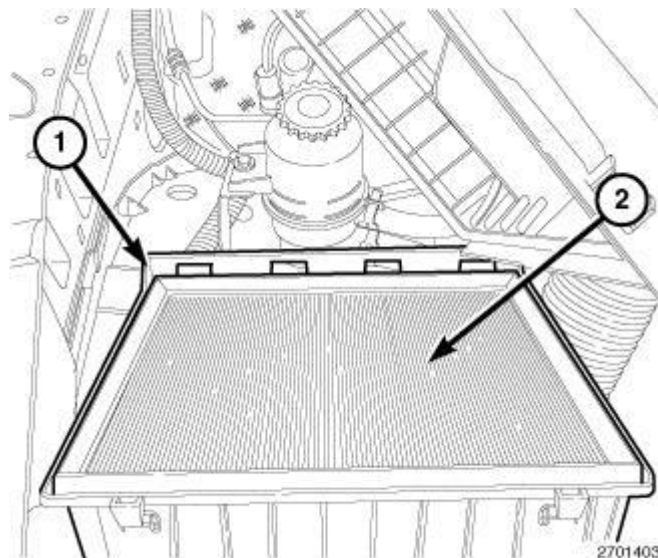
Fig. 380: AIR CLEANER HOUSING & AIR CLEANER FILTER Courtesy of CHRYSLER LLC
