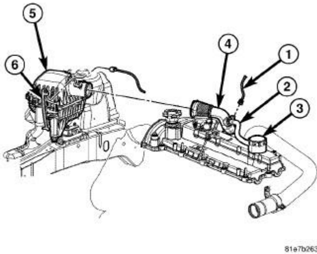
Fig. 98: CYLINDER HEAD COVER Courtesy of CHRYSLER LLC
