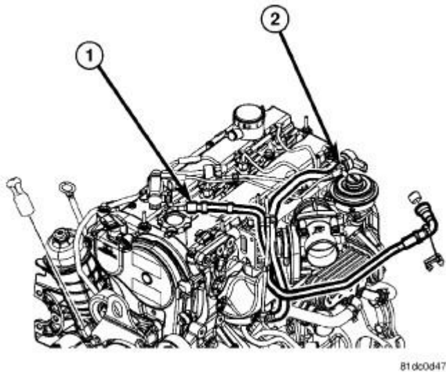
Fig. 113: FUEL RETURN LINES-TOP Courtesy of CHRYSLER LLC
