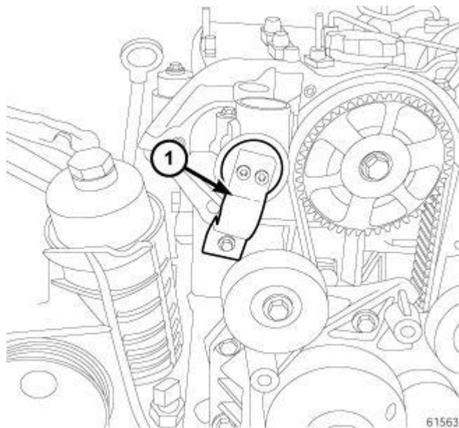
Fig. 93: CAMSHAFT LOCKING TOOL INSTALLED Courtesy of CHRYSLER LLC
