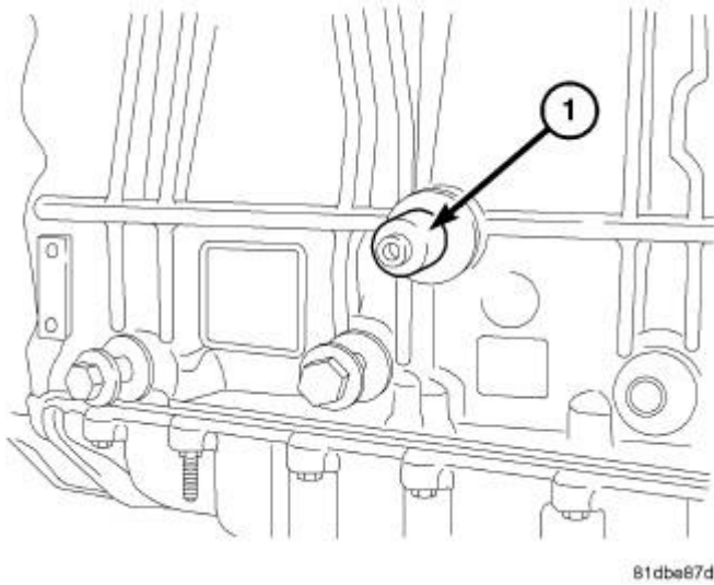
Fig. 338: CRANKSHAFT LOCKING TOOL Courtesy of CHRYSLER LLC
