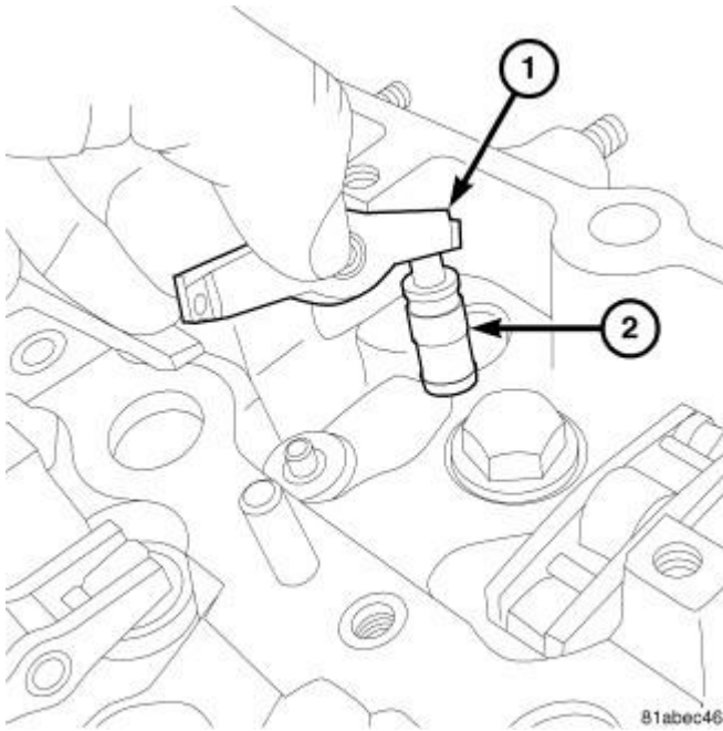
Fig. 116: LIFTERS
