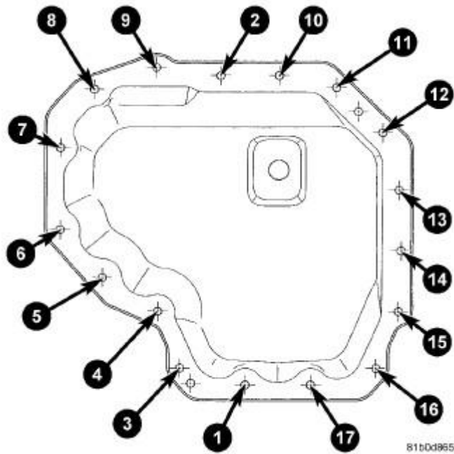
Fig. 249: LOWER OIL PAN TORQUE SEQUENCE
