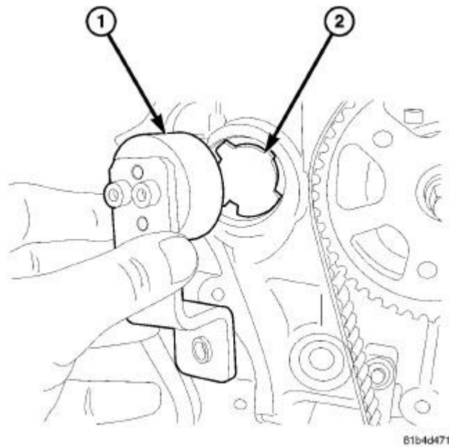
Fig. 319: INSTALLING CAMSHAFT LOCK TOOL
