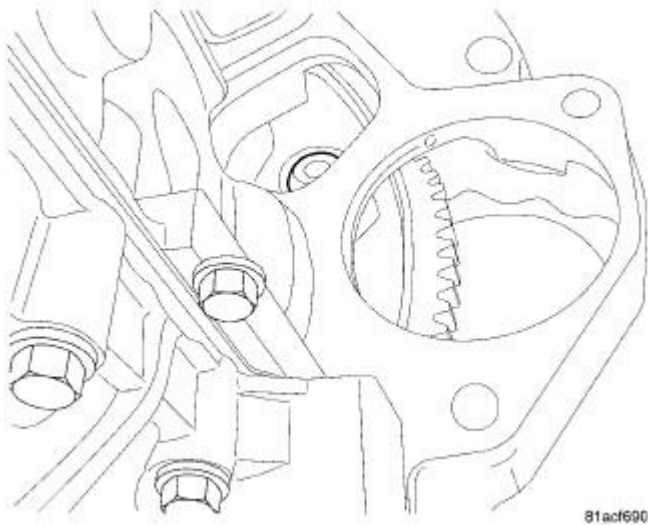
Fig. 29: FLEX PLATE BOLTS Courtesy of CHRYSLER LLC
