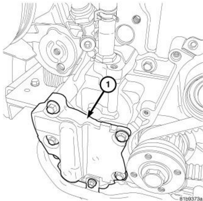
Fig. 183: VACUUM PUMP COVER
