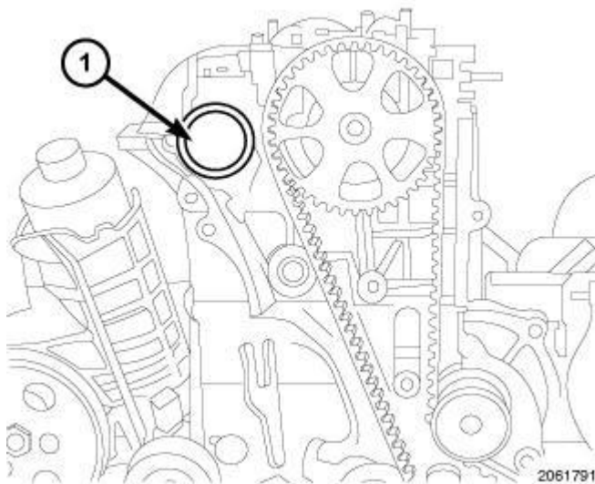
Fig. 326: EXHAUST CAMSHAFT OIL SEAL Courtesy of CHRYSLER LLC
