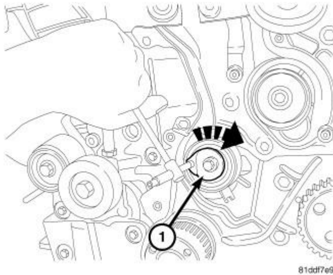
Fig. 332: TIMING BELT TENSIONER ADJUSTMENT Courtesy of CHRYSLER LLC
