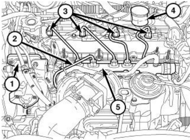
Fig. 31: FUEL RAIL Courtesy of CHRYSLER LLC
