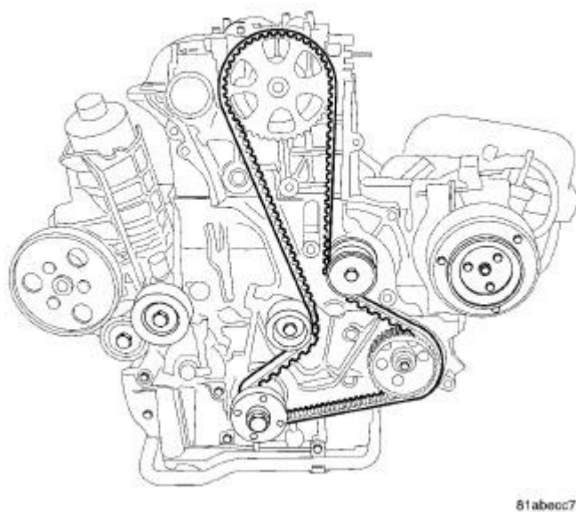
Fig. 144: TIMING BELT
