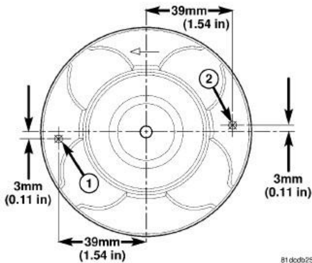
Fig. 70: PISTON PROTRUSION MEASUREMENT Courtesy of CHRYSLER LLC
