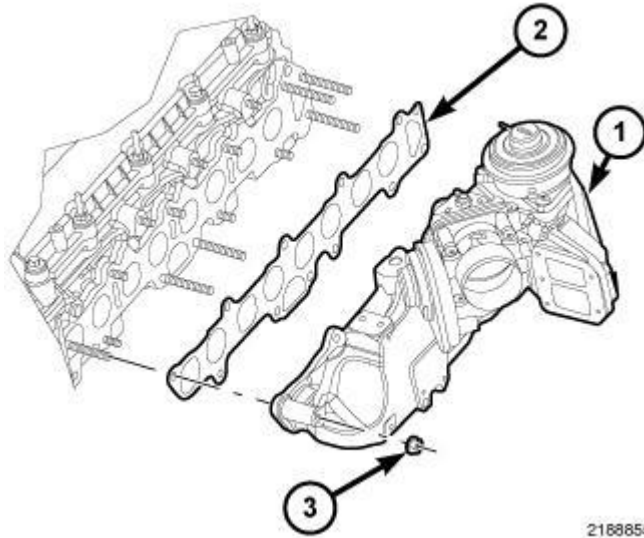
Fig. 286: IDENTIFYING MANIFOLD RETAINING NUTS, INTAKE MANIFOLD & INTAKE MANIFOLD GASKET
