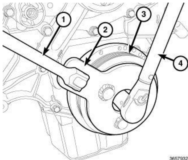
Fig. 269: Installing Vibration Damper Courtesy of CHRYSLER GROUP, LLC
