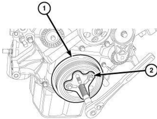
Fig. 183: Vibration Damper & Bolt Grip Puller Courtesy of CHRYSLER GROUP, LLC
