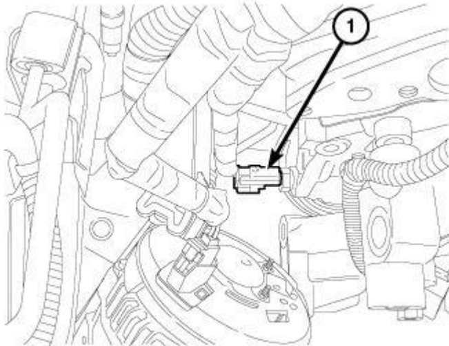
Fig. 380: Oil Temperature Sensor Electrical Connector Courtesy of CHRYSLER GROUP, LLC
