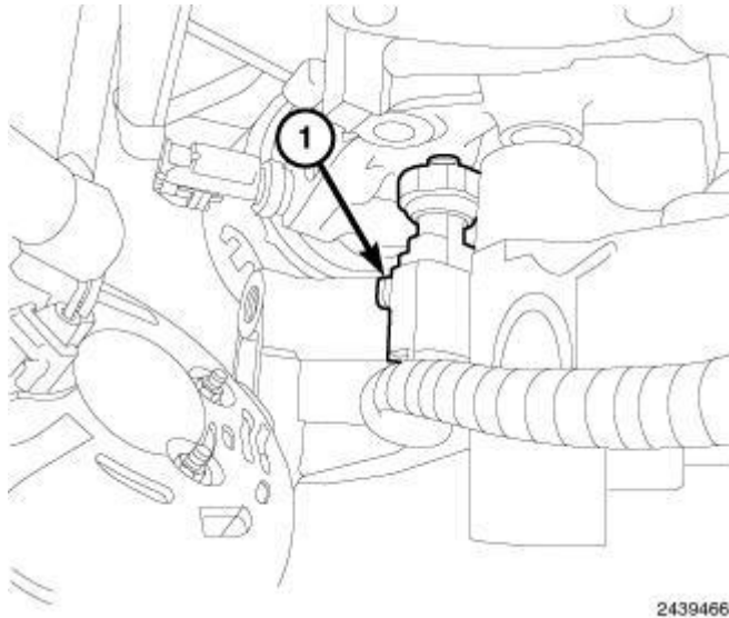
Fig. 38: Oil Pressure Sensor Electrical Connector Courtesy of CHRYSLER GROUP, LLC
