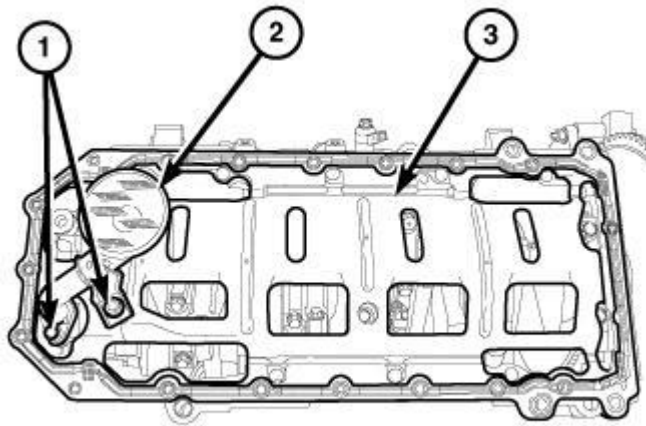
Fig. 446: Integral Windage Tray, Oil Pump Pickup Tube & Bolts Courtesy of CHRYSLER GROUP, LLC
