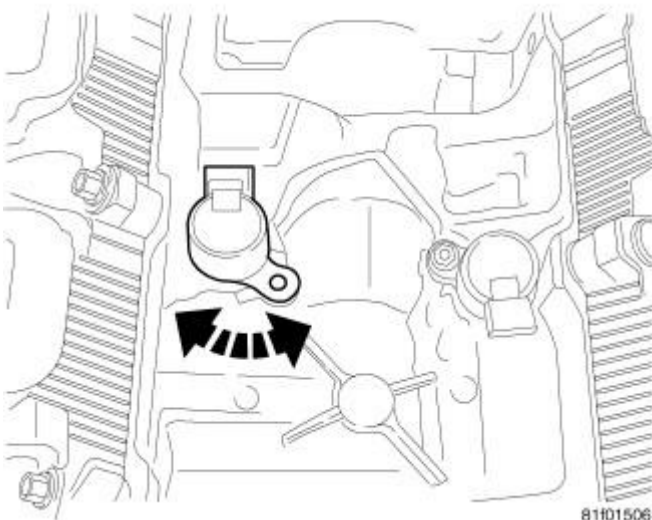
Fig. 276: Removing/Installing MDS Solenoid Courtesy of CHRYSLER GROUP, LLC
