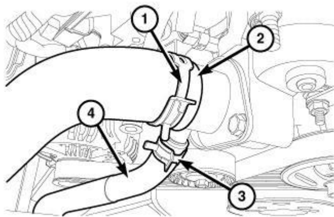
Fig. 69: Upper Radiator Hose, Clamp, Oil Cooler Return Line Hose & Clamp Courtesy of CHRYSLER GROUP, LLC
