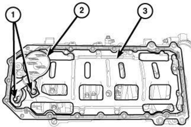
Fig. 251: Integral Windage Tray, Oil Pump Pickup Tube & Bolts
