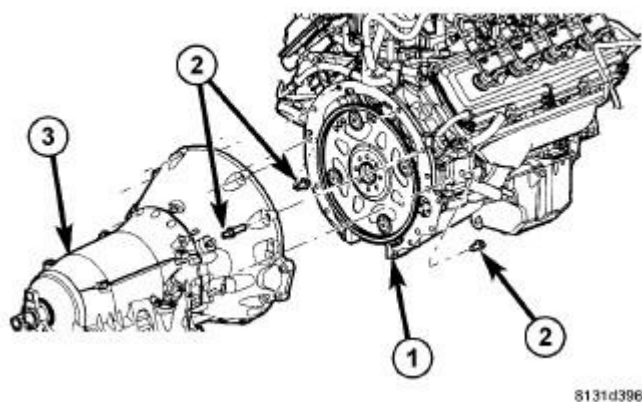
Fig. 35: Remove/Install Transmission To Engine Bolts Courtesy of CHRYSLER GROUP, LLC
