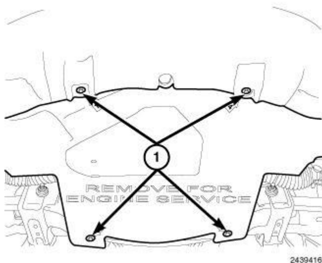
Fig. 330: Lower Splash Shield & Fasteners Courtesy of CHRYSLER GROUP, LLC
