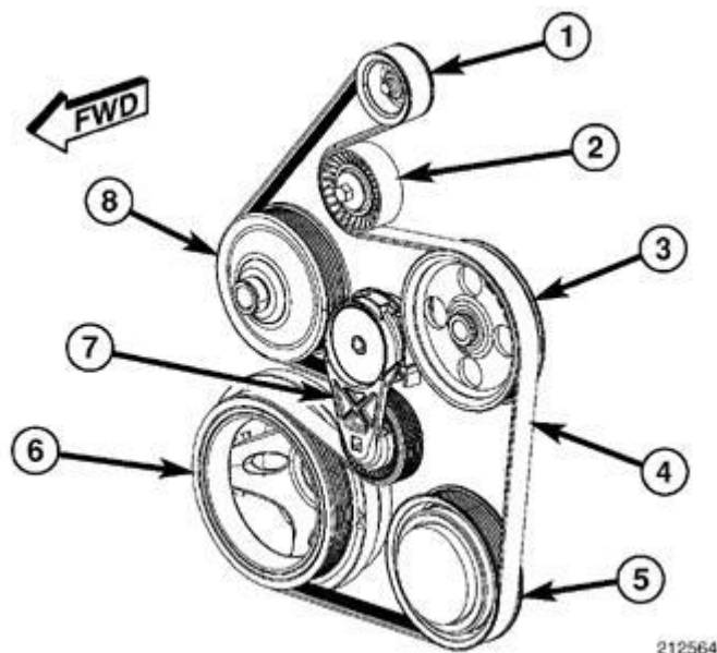
Fig. 178: Drive Belt Tensioners & Assembly With Drive Belt Routing Courtesy of CHRYSLER GROUP, LLC
