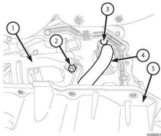
Fig. 349: Oil Pan Gasket/Windage Tray, Oil Pump Pickup Tube, Oil Pan & Fasteners Courtesy of CHRYSLER GROUP, LLC
