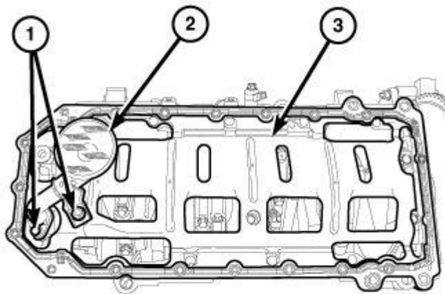
Fig. 369: Integral Windage Tray, Oil Pump Pickup Tube & Bolts Courtesy of CHRYSLER GROUP, LLC
