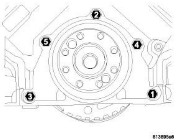
Fig. 238: Rear Seal Retainer Torque Sequence Courtesy of CHRYSLER GROUP, LLC
