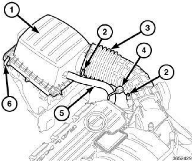
Fig. 77: Intake Air Temperature (IAT) Sensor, Air Cleaner Housing & Duct Courtesy of CHRYSLER GROUP, LLC
