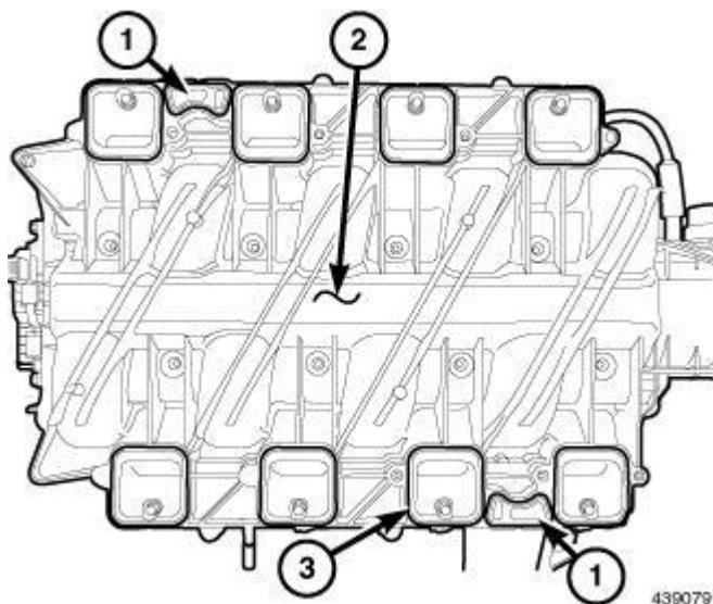
Fig. 400: Intake Manifold & PCV Seals Courtesy of CHRYSLER GROUP, LLC
