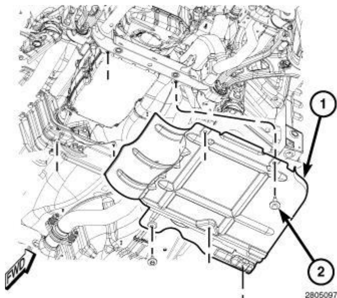
Fig. 75: Transmission Skid Plate & Fasteners Courtesy of CHRYSLER GROUP, LLC
