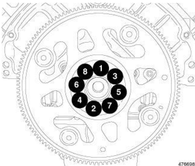
Fig. 229: Flexplate Retaining Bolt Removal & Tightening Sequence
