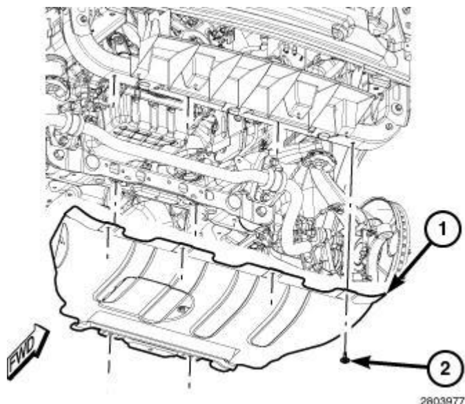
Fig. 7: Skid Plate & Fasteners Courtesy of CHRYSLER GROUP, LLC
