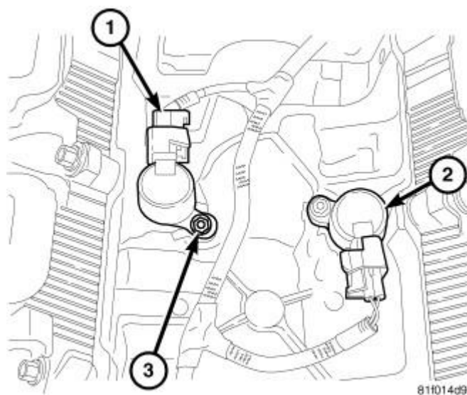
Fig. 274: MDS Solenoid Connector Courtesy of CHRYSLER GROUP, LLC
