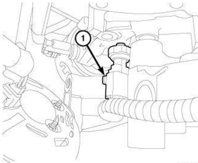
Fig. 64: Oil Pressure Sensor Electrical Connector Courtesy of CHRYSLER GROUP, LLC
