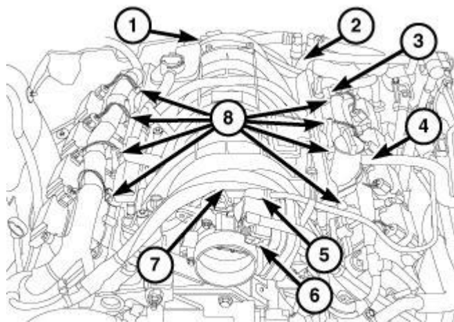
Fig. 305: Map Sensor, Brake Booster Vacuum Hose, Fuel Supply Line, Make Up Air Hose, EVAP Vacuum Purge Hose, Electrical Connector & Electrical Harness Courtesy of CHRYSLER GROUP, LLC
