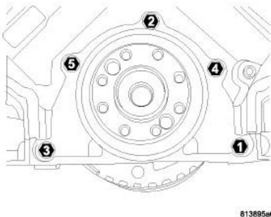
Fig. 207: Rear Seal Retainer Torque Sequence Courtesy of CHRYSLER GROUP, LLC
