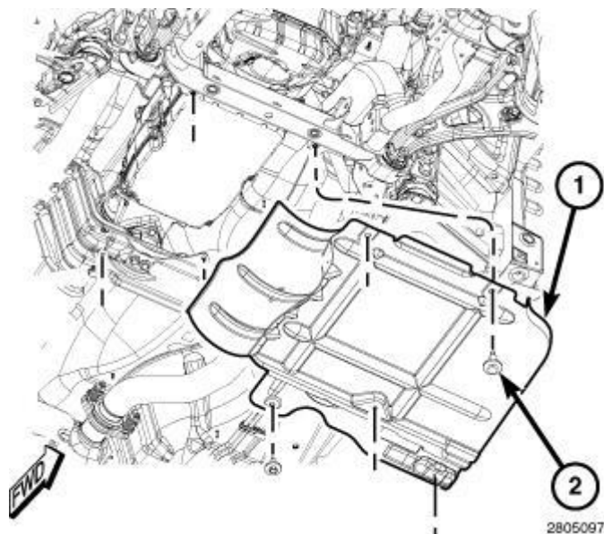
Fig. 8: Transmission Skid Plate & Fasteners Courtesy of CHRYSLER GROUP, LLC
