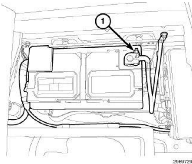
Fig. 249: Negative Battery Cable Courtesy of CHRYSLER GROUP, LLC
