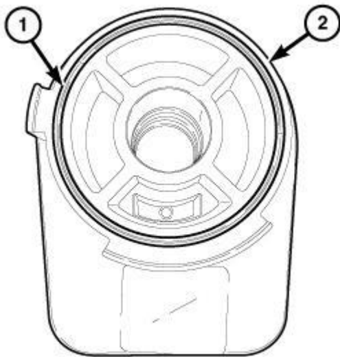
Fig. 322: O-Ring Seal & Oil Cooler Courtesy of CHRYSLER GROUP, LLC
