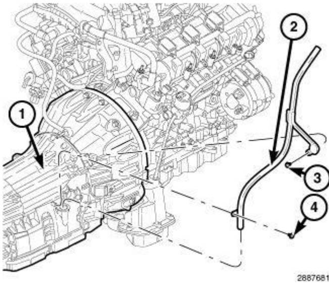
Fig. 27: Identifying Transmission, Transmission Fill Tube & Bolts Courtesy of CHRYSLER GROUP, LLC
