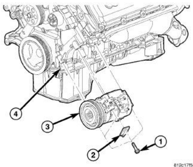
Fig. 36: Removing/Installing A/C Compressor Courtesy of CHRYSLER GROUP, LLC
