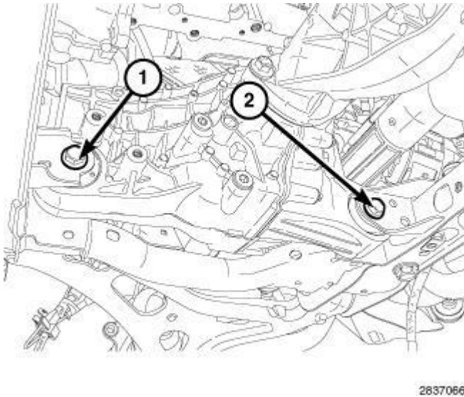
Fig. 353: Front Axle Cover Bushing Bolt & Pinion Nose Bushing Bolt Courtesy of CHRYSLER GROUP, LLC
