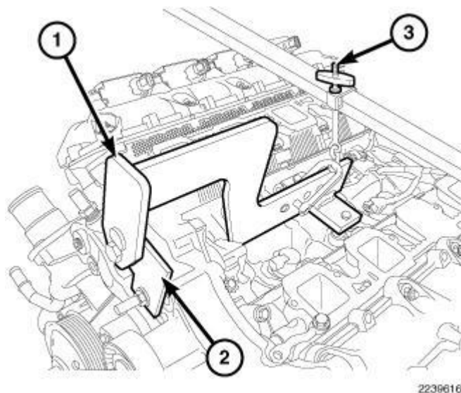
Fig. 297: Engine Lift Fixture & Adapter Courtesy of CHRYSLER GROUP, LLC
