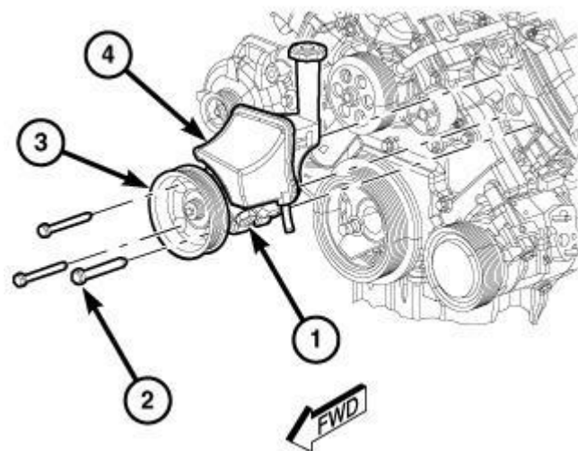
Fig. 20: Power Steering Reservoir, Pump, Pulley & Bolts
