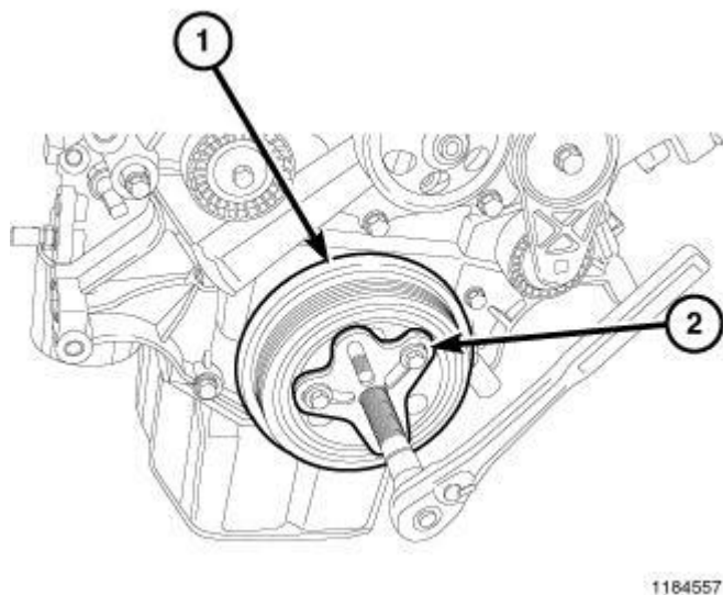
Fig. 441: Vibration Damper & Bolt Grip Puller Courtesy of CHRYSLER GROUP, LLC
