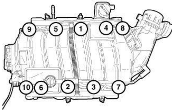
Fig. 16: Intake Manifold Removal/Tightening Sequence Courtesy of CHRYSLER GROUP, LLC
