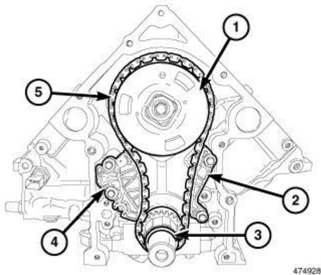
Fig. 163: Timing Chain, Sprockets, Timing Chain Tensioner & Guide Courtesy of CHRYSLER GROUP, LLC
