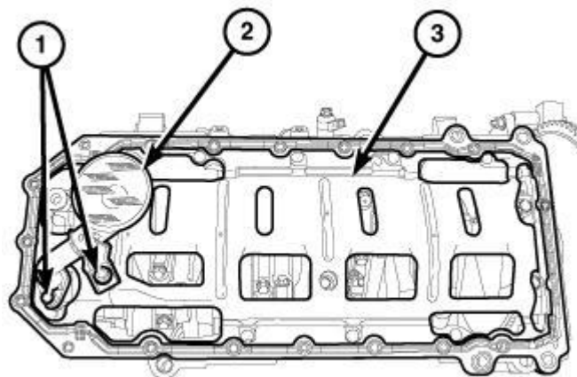
Fig. 431: Integral Windage Tray, Oil Pump Pickup Tube & Bolts
