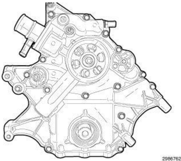
Fig. 445: Engine Timing Cover Courtesy of CHRYSLER GROUP, LLC
