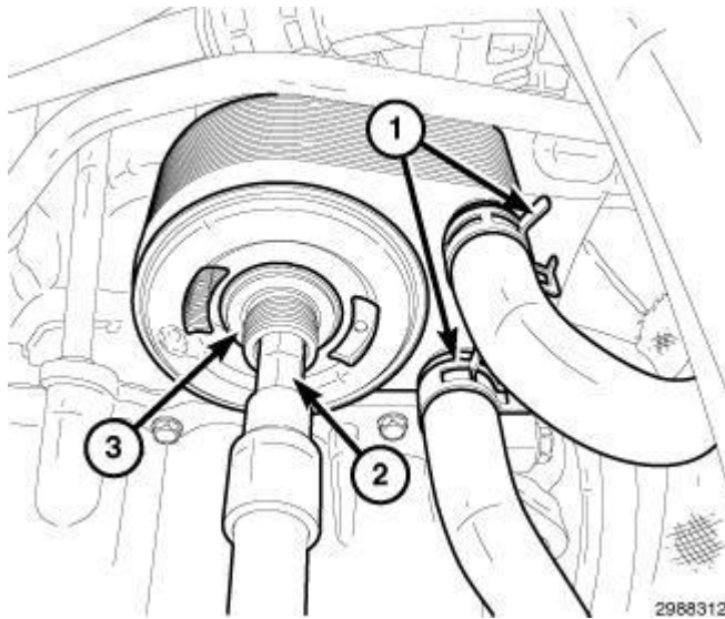
Fig. 321: Clamps, Allen Wrench Socket & Oil Cooler Retaining Bolt Courtesy of CHRYSLER GROUP, LLC
