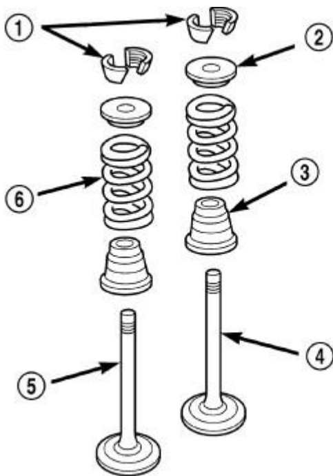
Fig. 145: Valve Assembly Configuration Courtesy of CHRYSLER GROUP, LLC
