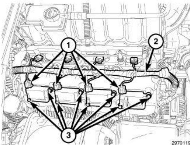
Fig. 105: Ignition Coil Electrical Connectors, Harness & Bolts
