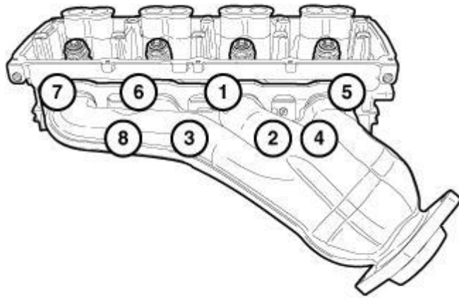
Fig. 91: Exhaust Manifold Removal/Tightening Sequence Courtesy of CHRYSLER GROUP, LLC
