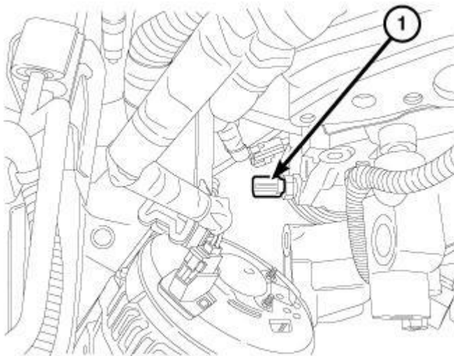
Fig. 381: Oil Temperature Sensor Courtesy of CHRYSLER GROUP, LLC
