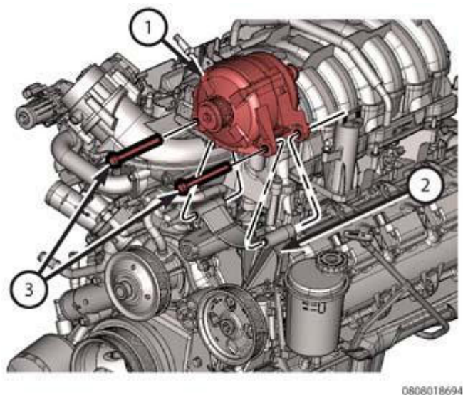
Fig. 440: Generator, Bolts & Connector Courtesy of CHRYSLER GROUP, LLC
