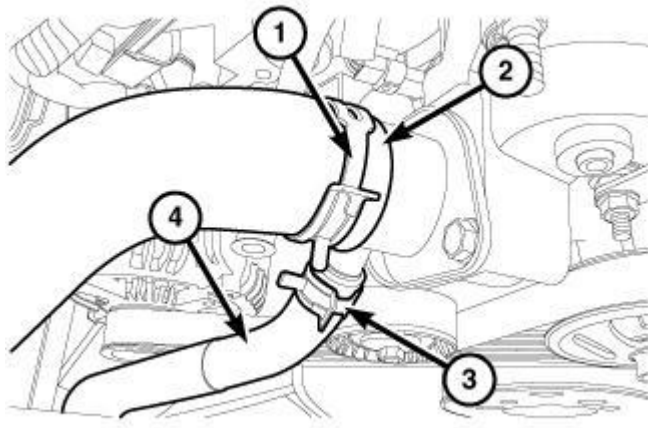
Fig. 218: Upper Radiator Hose, Clamp, Oil Cooler Return Line Hose & Clamp Courtesy of CHRYSLER GROUP, LLC
