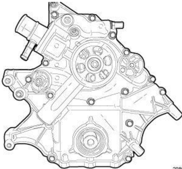
Fig. 426: Engine Timing Cover Courtesy of CHRYSLER GROUP, LLC
