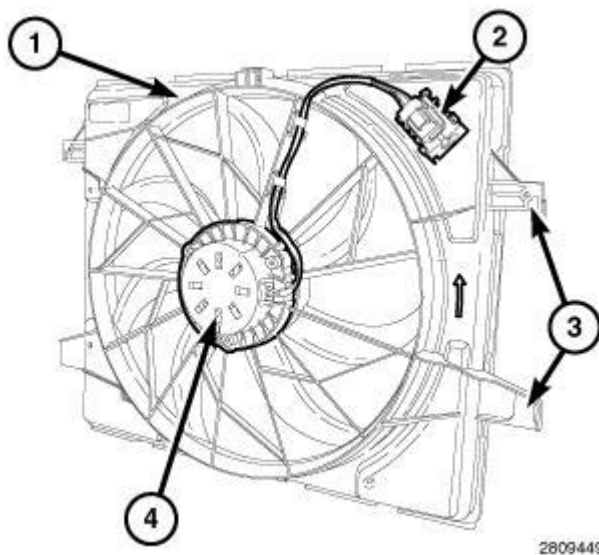
Fig. 68: Cooling Fan Module Components Courtesy of CHRYSLER GROUP, LLC
