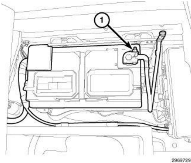
Fig. 231: Negative Battery Cable
