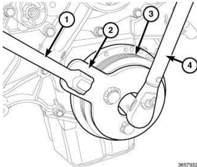
Fig. 224: Installing Vibration Damper Courtesy of CHRYSLER GROUP, LLC
