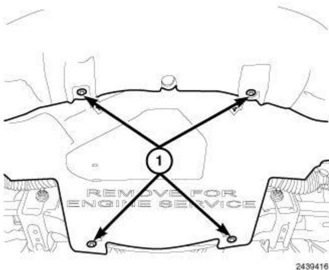
Fig. 327: Lower Splash Shield & Fasteners Courtesy of CHRYSLER GROUP, LLC
