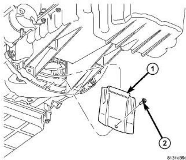
Fig. 32: Remove/Install Torque Converter Access Cover Courtesy of CHRYSLER GROUP, LLC
