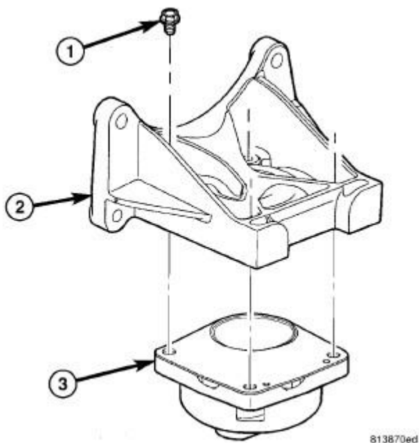
Fig. 286: Rear Transmission Mount Isolator
