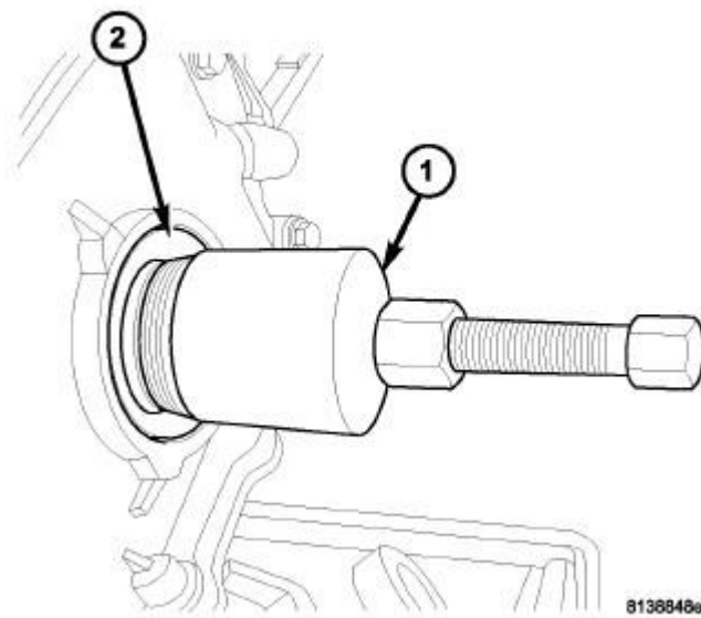
Fig. 265: Front Crankshaft Seal Removal Courtesy of CHRYSLER GROUP, LLC
