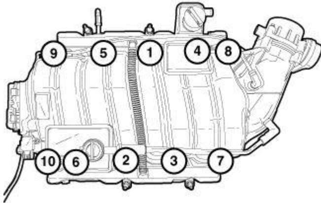
Fig. 401: Intake Manifold Removal/Tightening Sequence Courtesy of CHRYSLER GROUP, LLC
