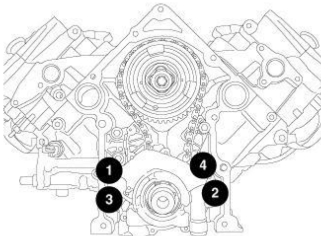
Fig. 424: Oil Pump Retaining Bolt Tightening Sequence Courtesy of CHRYSLER GROUP, LLC
