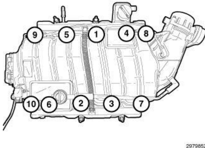
Fig. 62: Intake Manifold Removal/Tightening Sequence Courtesy of CHRYSLER GROUP, LLC
