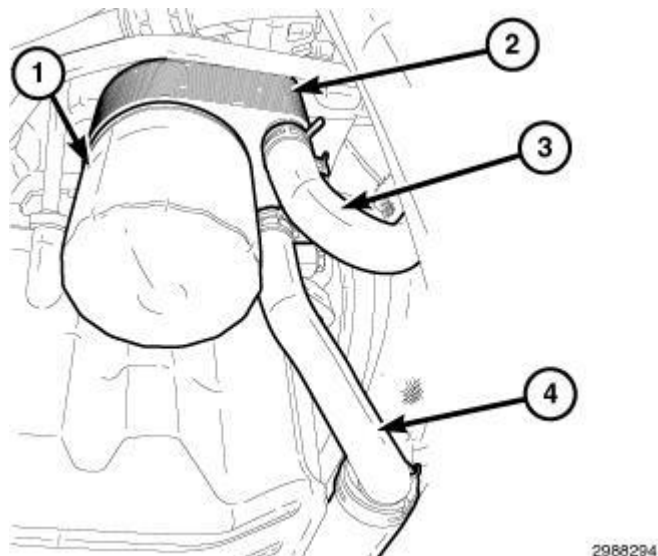
Fig. 328: Oil Filter, Oil Cooler & Hoses Courtesy of CHRYSLER GROUP, LLC
