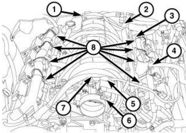
Fig. 337: Map Sensor, Brake Booster Vacuum Hose, Fuel Supply Line, Make Up Air Hose, EVAP Vacuum Purge Hose, Electrical Connector & Electrical Harness Courtesy of CHRYSLER GROUP, LLC
