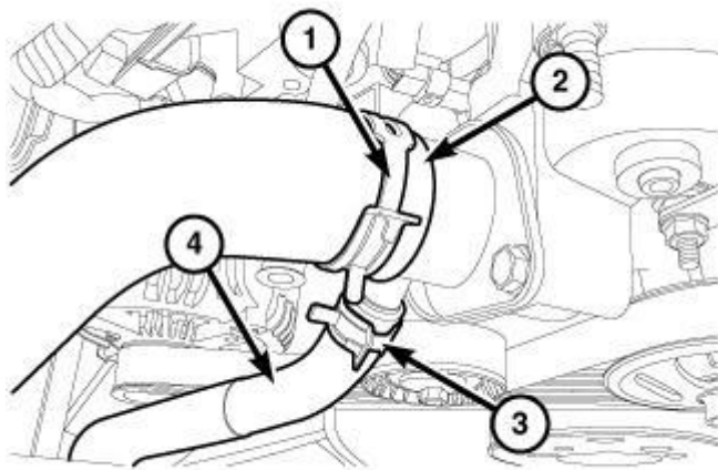
Fig. 227: Upper Radiator Hose, Clamp, Oil Cooler Return Line Hose & Clamp Courtesy of CHRYSLER GROUP, LLC
