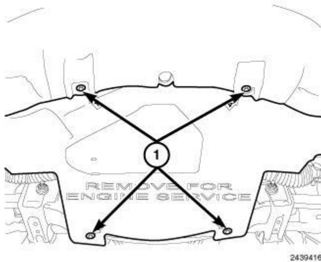
Fig. 293: Lower Splash Shield & Fasteners Courtesy of CHRYSLER GROUP, LLC
