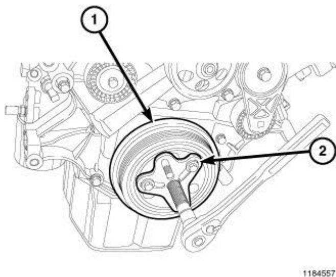
Fig. 264: Vibration Damper & Bolt Grip Puller Courtesy of CHRYSLER GROUP, LLC
