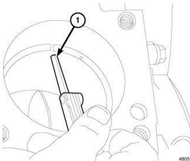
Fig. 242: Using Feeler Gauge To Check Ring End Gap Courtesy of CHRYSLER GROUP, LLC
