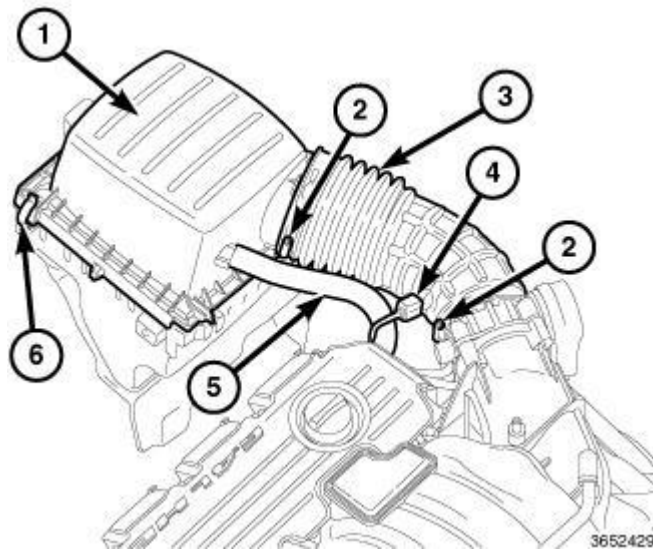
Fig. 228: Intake Air Temperature (IAT) Sensor, Air Cleaner Housing & Duct Courtesy of CHRYSLER GROUP, LLC
