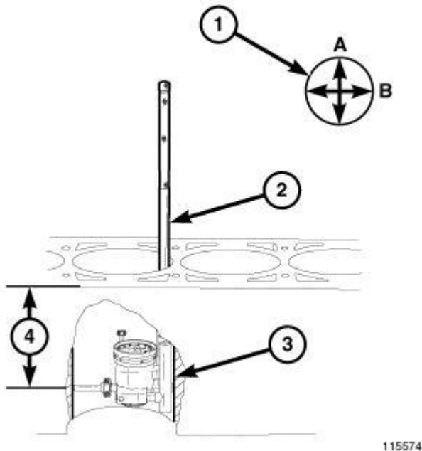
Fig. 152: Measuring Cylinder Bore Diameter Courtesy of CHRYSLER GROUP, LLC
