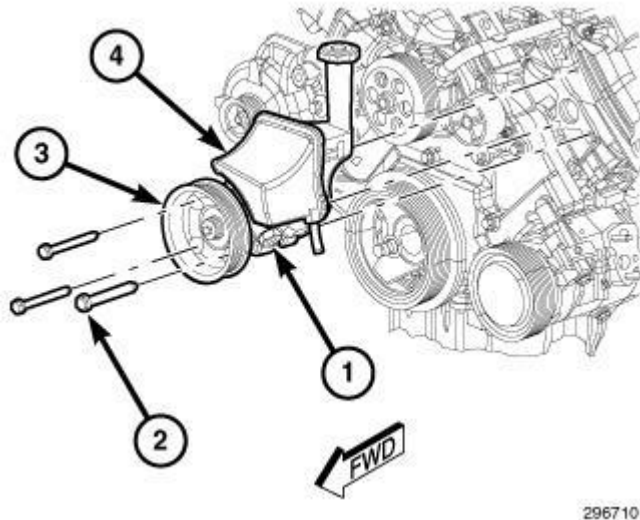
Fig. 86: Power Steering Reservoir, Pump, Pulley & Bolts Courtesy of CHRYSLER GROUP, LLC
