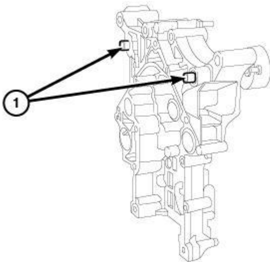
Fig. 407: Front Cover Slide Bushings Courtesy of CHRYSLER GROUP, LLC
