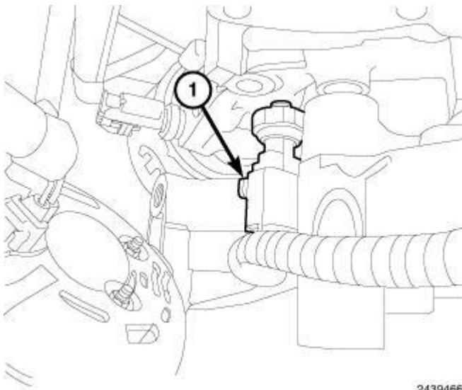
Fig. 372: Oil Pressure Sensor Electrical Connector Courtesy of CHRYSLER GROUP, LLC
