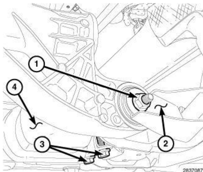
Fig. 344: Nut And Bolt, Front Axle Tube Bushing & Bolts Courtesy of CHRYSLER GROUP, LLC
