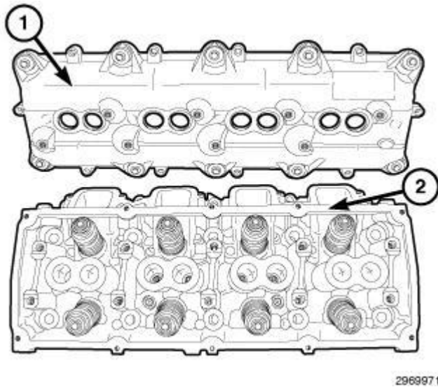
Fig. 110: Cylinder Head & Cover Courtesy of CHRYSLER GROUP, LLC
