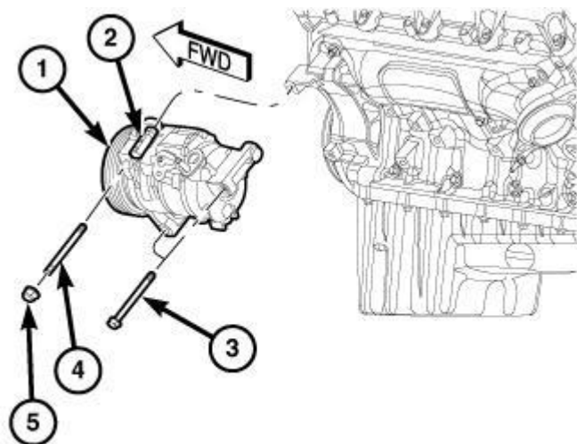
Fig. 294: A/C Clutch Electrical Connector, Two Bolts, A/C Compressor, Nut & Stud Courtesy of CHRYSLER GROUP, LLC
