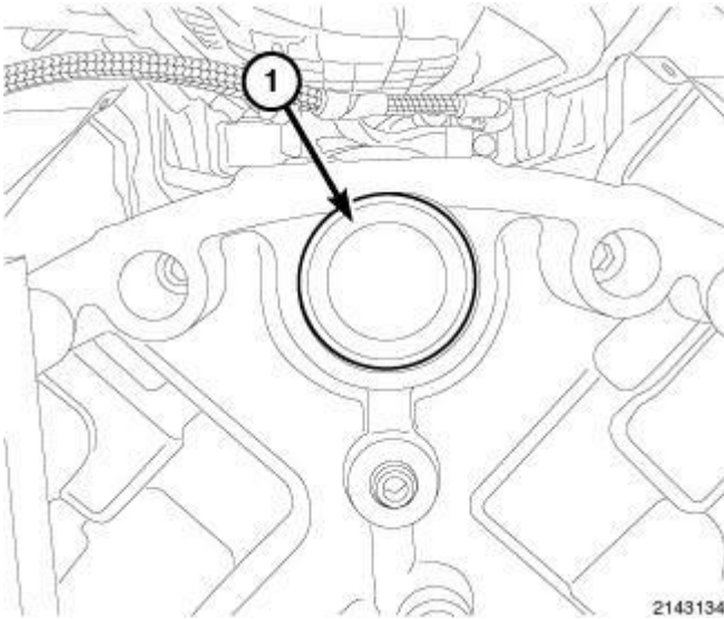
Fig. 166: Camshaft Core Hole Plug Courtesy of CHRYSLER GROUP, LLC
