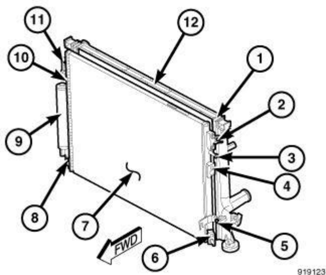
Fig. 173: A/C Condenser & Radiator Courtesy of CHRYSLER GROUP, LLC
