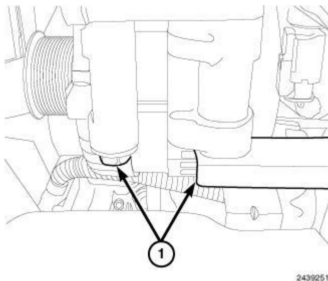
Fig. 379: Lower Generator Retaining Bolts Courtesy of CHRYSLER GROUP, LLC
