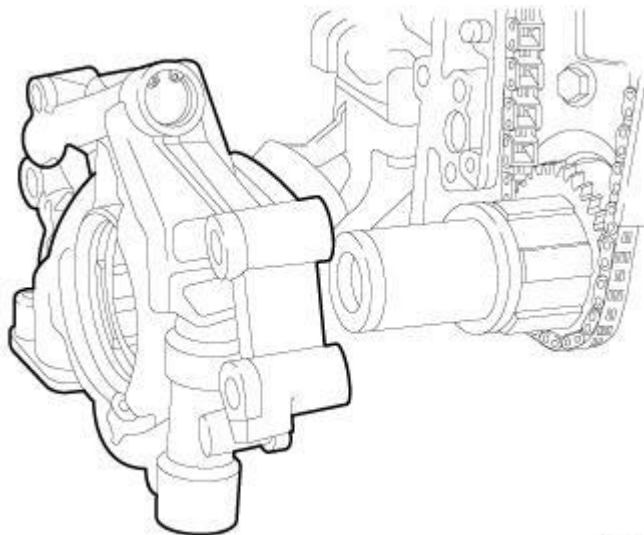
Fig. 162: Remove/Install Oil Pump Courtesy of CHRYSLER GROUP, LLC
