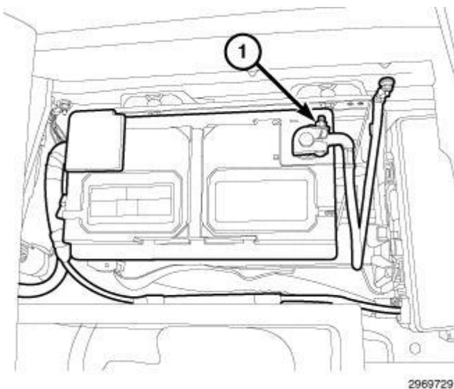
Fig. 81: Negative Battery Cable
