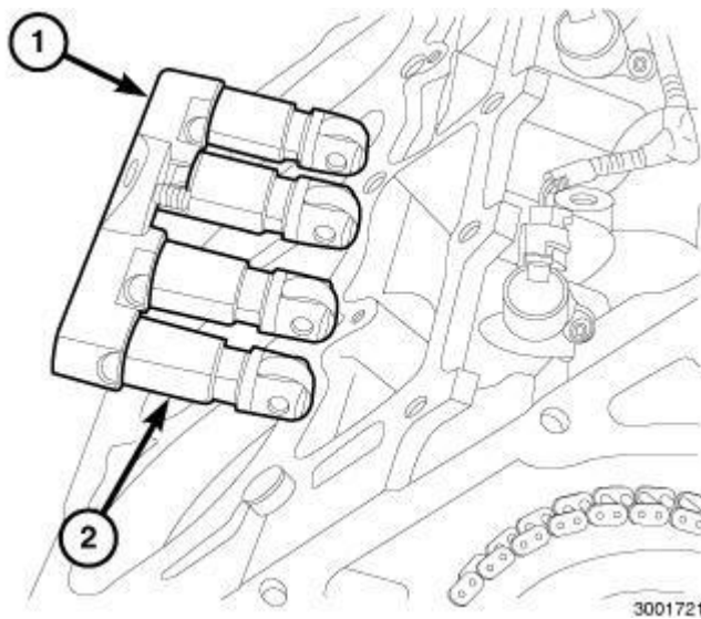
Fig. 175: Hydraulic Lifters/Tappets & Retainer/Guide Holder Courtesy of CHRYSLER GROUP, LLC
