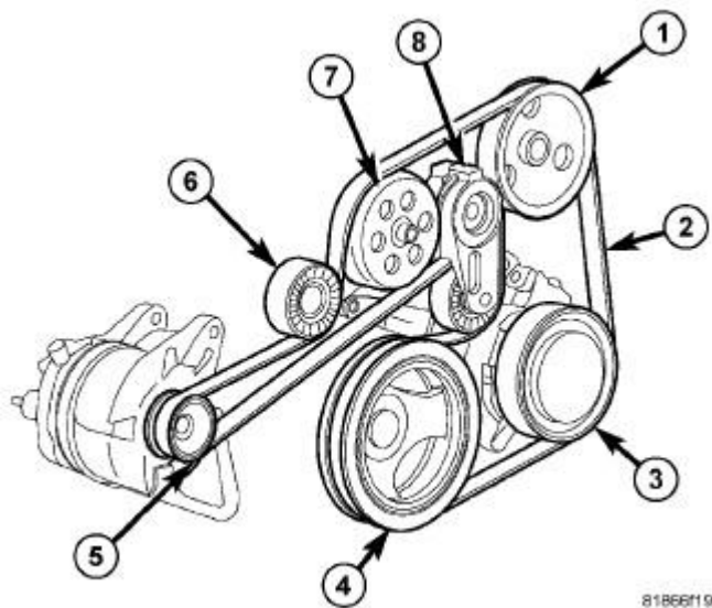
Fig. 85: Accessory Drive Belt Routing, Tensioner & Pulleys Courtesy of CHRYSLER GROUP, LLC
