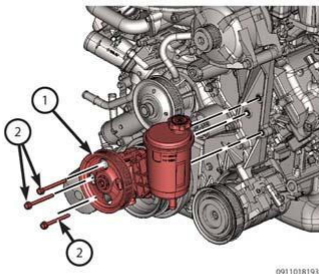
Fig. 438: Power Steering Pump Pulley & Bolts Courtesy of CHRYSLER GROUP, LLC
