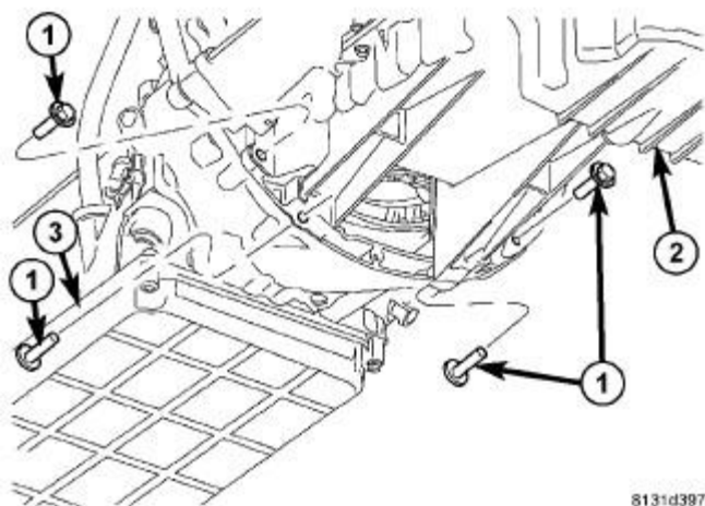
Fig. 34: Remove/Install Transmission To Oil Pan Bolts Courtesy of CHRYSLER GROUP, LLC
