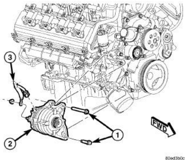
Fig. 296: Generator & Retaining Bolts Courtesy of CHRYSLER GROUP, LLC
