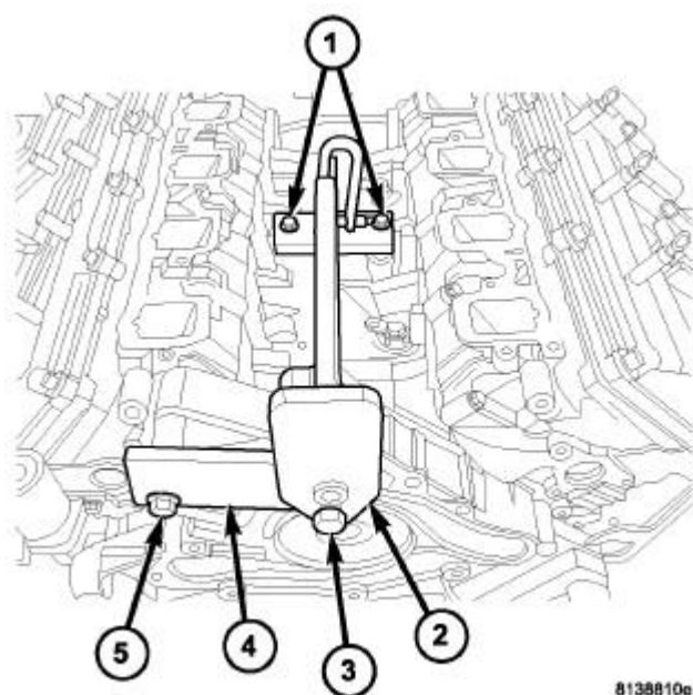
Fig. 55: Engine Lift Fixture & Adapter Courtesy of CHRYSLER GROUP, LLC
