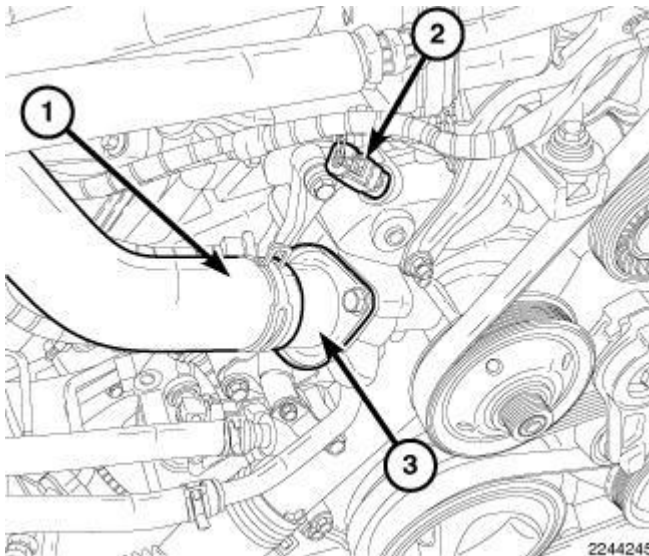
Fig. 435: Engine Coolant Temperature (ECT) Sensor & Thermostat Courtesy of CHRYSLER GROUP, LLC
