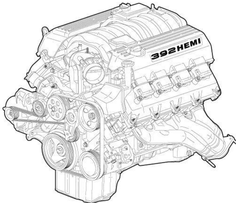
Fig. 212: 6.4L HEMI® V-8 Engine
