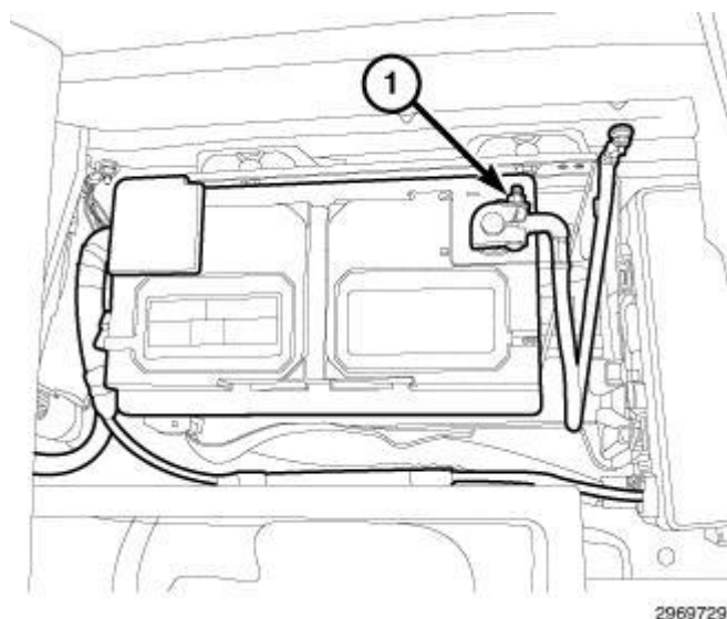
Fig. 457: Negative Battery Cable Courtesy of CHRYSLER GROUP, LLC
