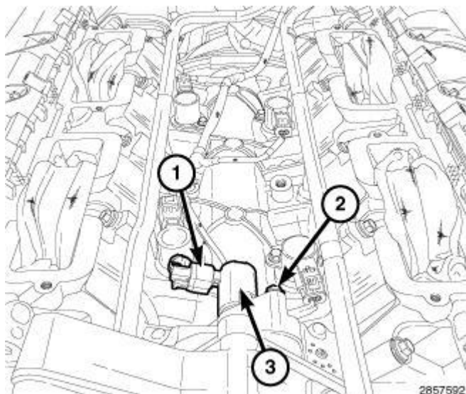
Fig. 314: Oil Control Valve, Electrical Connector & Retaining Bolt Courtesy of CHRYSLER GROUP, LLC
