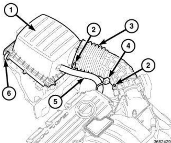
Fig. 78: Intake Air Temperature (IAT) Sensor, Air Cleaner Housing & Duct Courtesy of CHRYSLER GROUP, LLC
