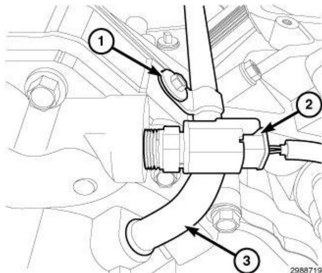
Fig. 57: Coolant Temperature (ECT) Sensor Electrical Connector, Heater Tube & Retaining Bolt Courtesy of CHRYSLER GROUP, LLC
