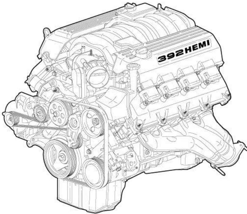
Fig. 182: 6.4L HEMI® V-8 Engine
