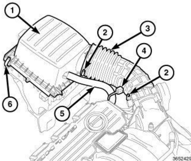
Fig. 72: Intake Air Temperature (IAT) Sensor, Air Cleaner Housing & Duct Courtesy of CHRYSLER GROUP, LLC
