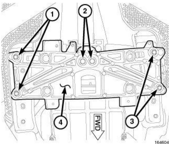
Fig. 280: Rear Cross Member & Bolts Courtesy of CHRYSLER GROUP, LLC
