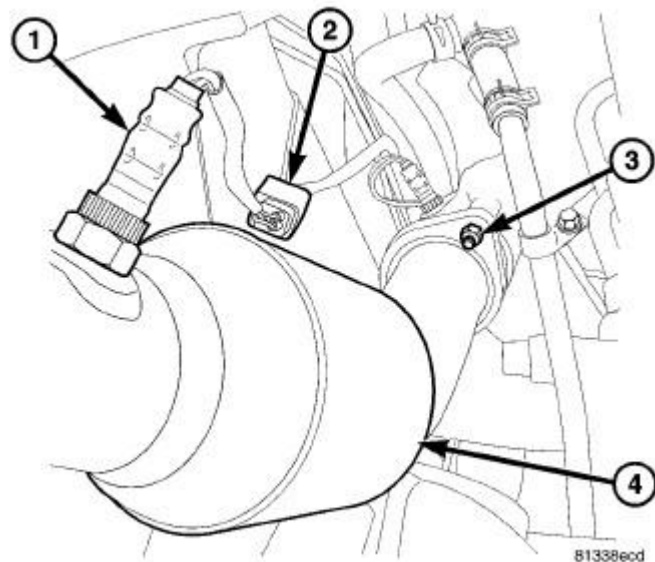
Fig. 52: Oxygen Sensor, Oxygen Sensor Connector, Ball Flange Nut & LH Catalytic Converter Courtesy of CHRYSLER GROUP, LLC
