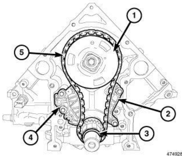
Fig. 189: Timing Chain, Sprockets, Timing Chain Tensioner & Guide Courtesy of CHRYSLER GROUP, LLC
