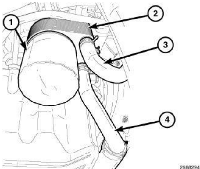
Fig. 329: Oil Filter, Oil Cooler & Hoses Courtesy of CHRYSLER GROUP, LLC
