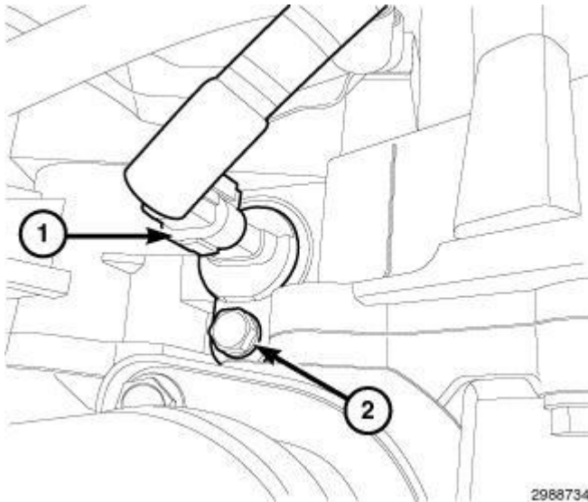
Fig. 454: Camshaft Position Sensor Electrical Connector & Bolt Courtesy of CHRYSLER GROUP, LLC
