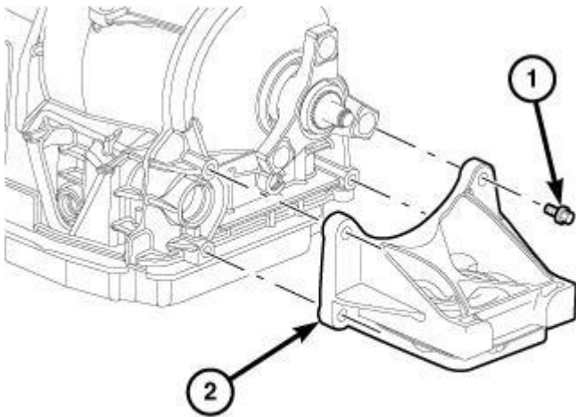
Fig. 285: Rear Transmission Mount Bracket Courtesy of CHRYSLER GROUP, LLC
