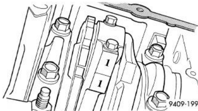
Fig. 202: Mark On Connecting Rod & Bearing Cap Courtesy of CHRYSLER GROUP, LLC
