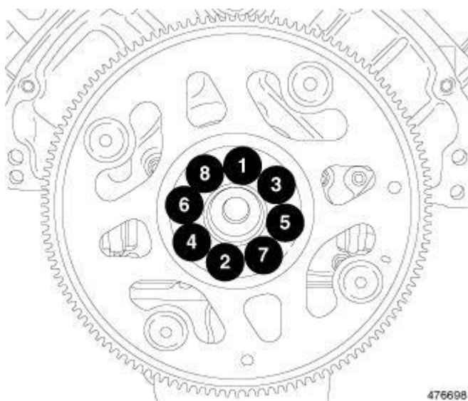
Fig. 230: Flexplate Retaining Bolt Removal & Tightening Sequence
