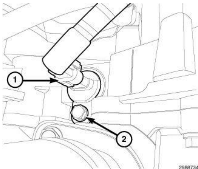
Fig. 14: Camshaft Position Sensor Electrical Connector & Bolt Courtesy of CHRYSLER GROUP, LLC
