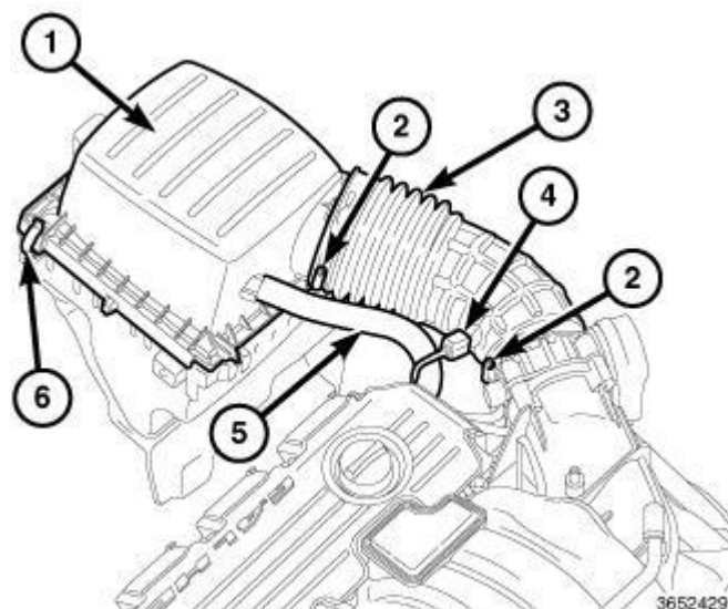
Fig. 398: Intake Air Temperature (IAT) Sensor, Air Cleaner Housing & Duct Courtesy of CHRYSLER GROUP, LLC
