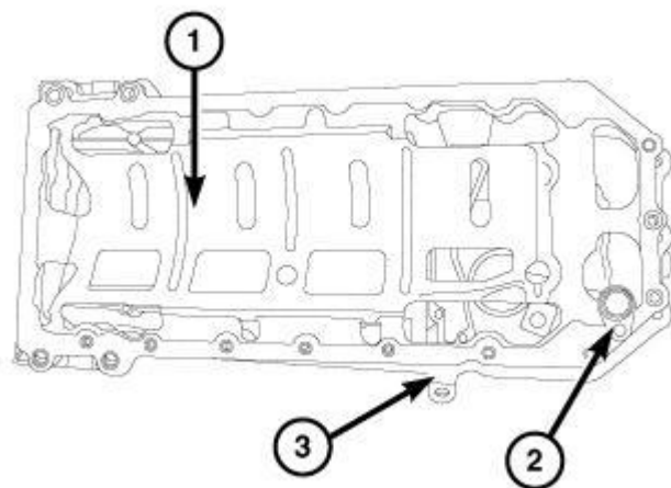
Fig. 348: Oil Pan Gasket/Windage Tray, Oil Pump Pickup Tube & Oil Pan Courtesy of CHRYSLER GROUP, LLC
