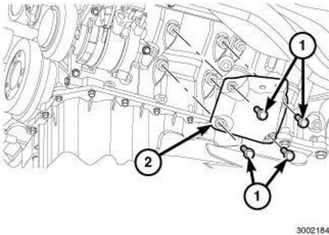
Fig. 300: Engine Mount-To-Engine Block Mounting Brackets & Retaining Bolts Courtesy of CHRYSLER GROUP, LLC
