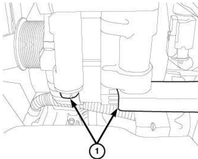
Fig. 376: Lower Generator Retaining Bolts Courtesy of CHRYSLER GROUP, LLC
