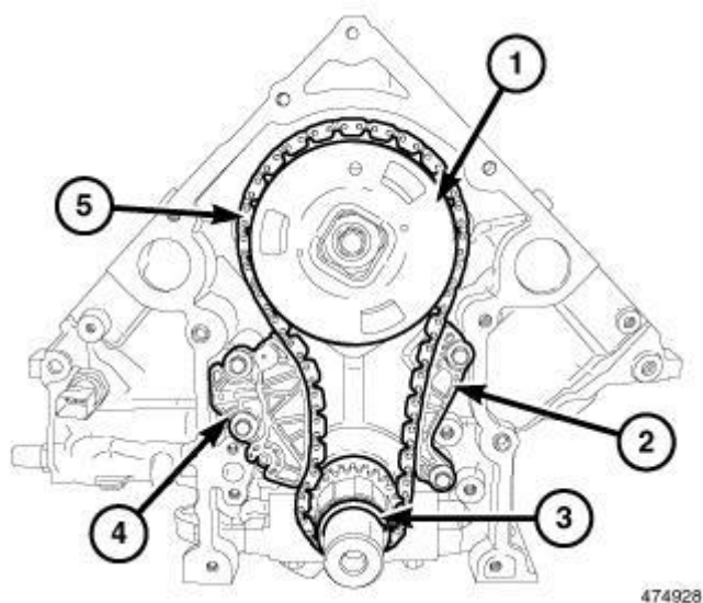
Fig. 204: Timing Chain, Sprockets, Timing Chain Tensioner & Guide Courtesy of CHRYSLER GROUP, LLC
