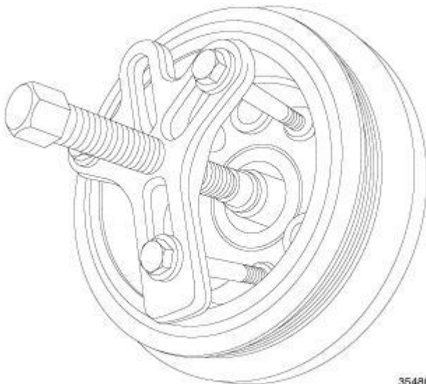
Fig. 215: Removing Vibration Damper Courtesy of CHRYSLER GROUP, LLC
