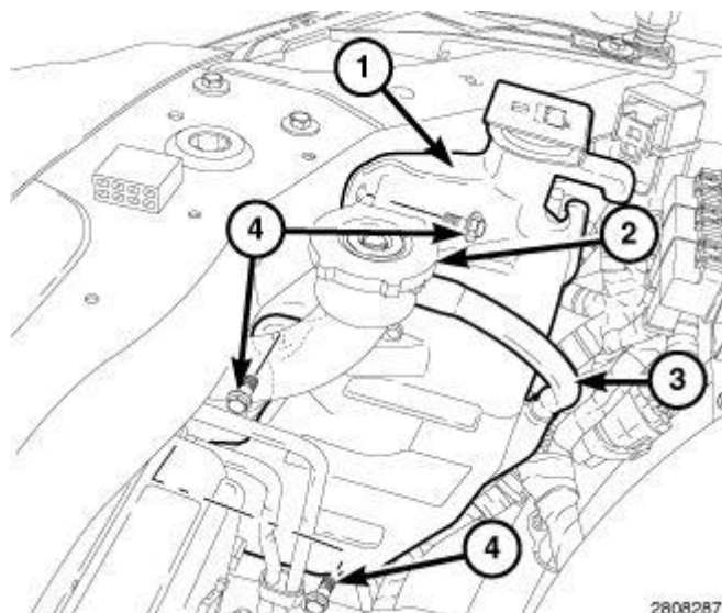
Fig. 40: Coolant Recovery Bottle, Radiator Neck, Overflow Tube & Fasteners Courtesy of CHRYSLER GROUP, LLC
