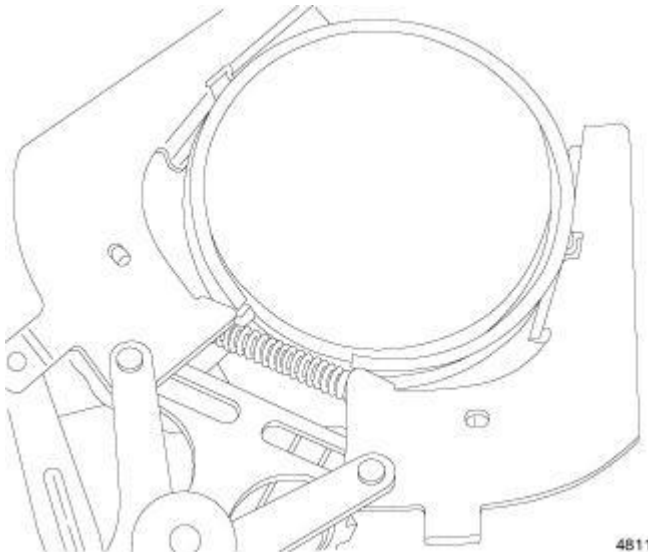
Fig. 245: Installing Upper & Intermediate Rings Courtesy of CHRYSLER GROUP, LLC
