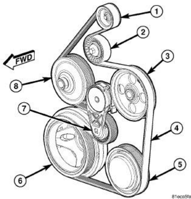
Fig. 437: Drive Belt Routing Courtesy of CHRYSLER GROUP, LLC
