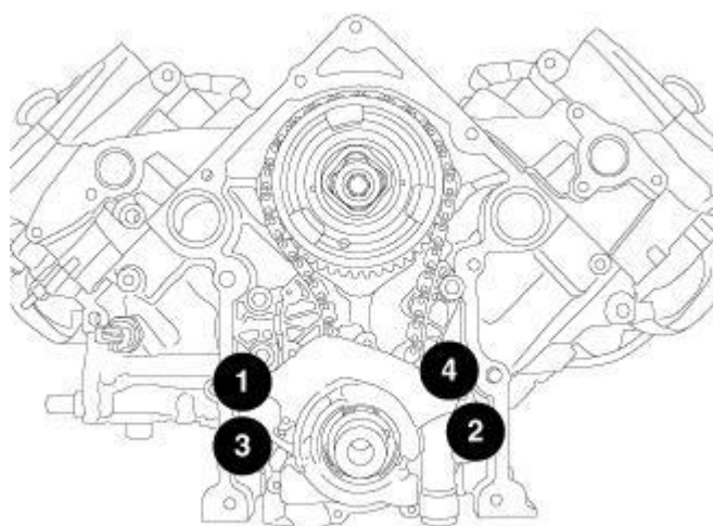
Fig. 205: Oil Pump Retaining Bolt Tightening Sequence Courtesy of CHRYSLER GROUP, LLC
