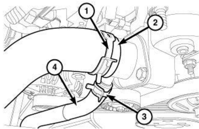
Fig. 12: Upper Radiator Hose, Clamp, Oil Cooler Return Line Hose & Clamp Courtesy of CHRYSLER GROUP, LLC
