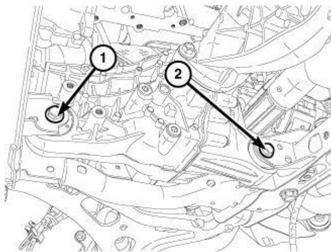
Fig. 343: Front Axle Cover Bushing Bolt & Pinion Nose Bushing Bolt Courtesy of CHRYSLER GROUP, LLC
