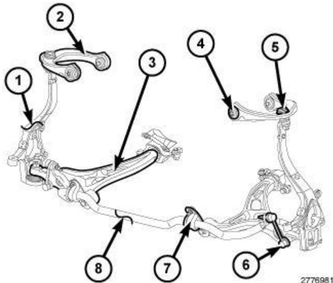
Fig. 352: Suspension Components With Rubber/Urethane Bushings Courtesy of CHRYSLER GROUP, LLC
