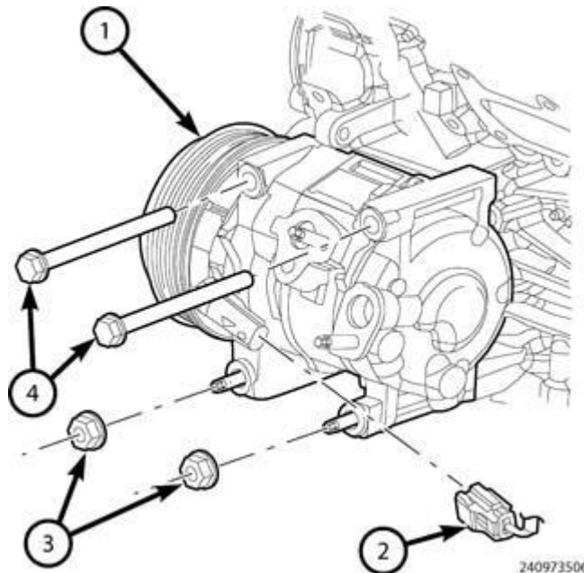
Fig. 451: Removing/Installing A/C Compressor Courtesy of CHRYSLER GROUP, LLC
