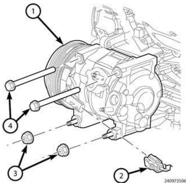
Fig. 439: Removing/Installing A/C Compressor Courtesy of CHRYSLER GROUP, LLC
