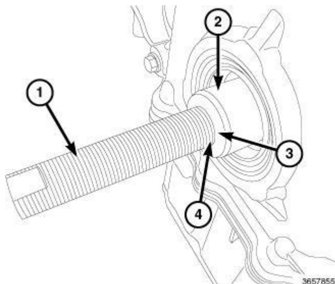
Fig. 448: Installing Vibration Damper Onto Crankshaft Using Special Tool Courtesy of CHRYSLER GROUP, LLC
