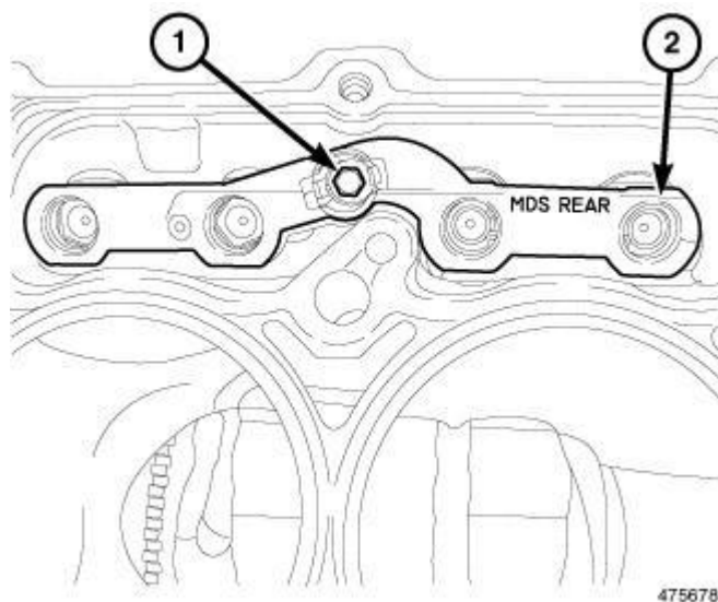
Fig. 234: Rear MDS Lifter Assembly Courtesy of CHRYSLER GROUP, LLC
