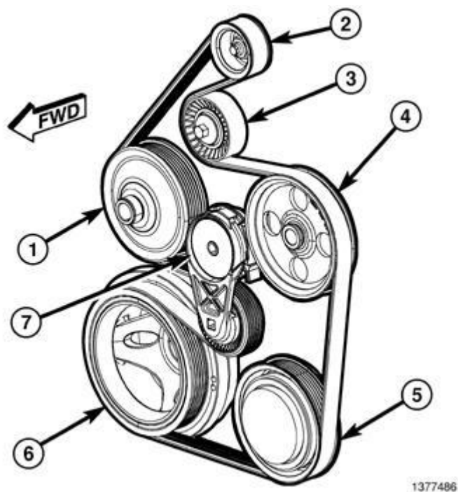
Fig. 453: Accessory Drive Belt Routing, Tensioner & Pulleys Courtesy of CHRYSLER GROUP, LLC
