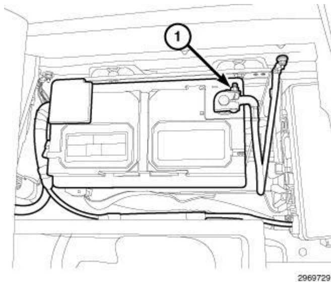
Fig. 405: Negative Battery Cable Courtesy of CHRYSLER GROUP, LLC
