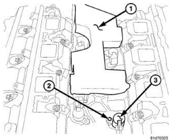
Fig. 278: Intake Manifold Foam Insulator Pad, MDS Solenoids & Bolts Courtesy of CHRYSLER GROUP, LLC
