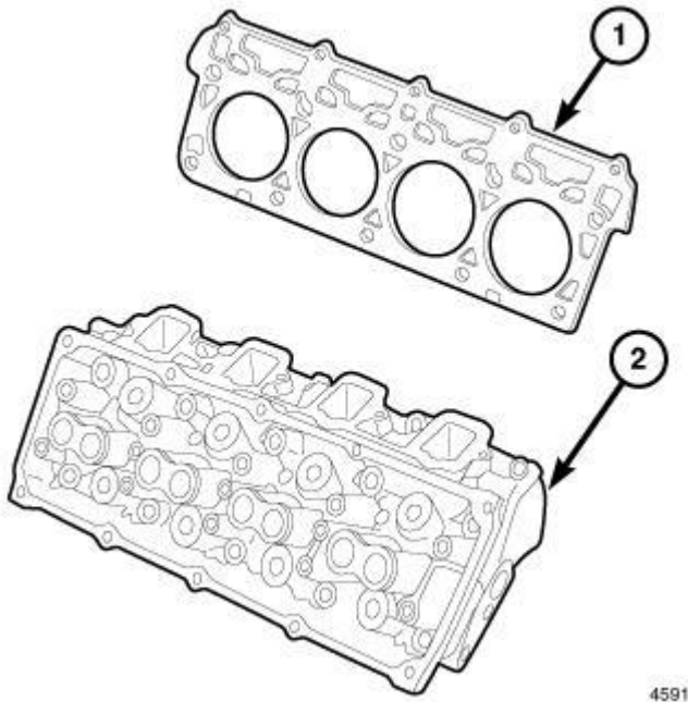
Fig. 156: Cylinder Head & Gasket Courtesy of CHRYSLER GROUP, LLC
