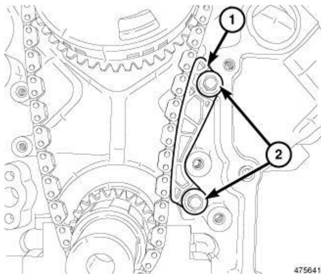
Fig. 414: Timing Chain Guide Courtesy of CHRYSLER GROUP, LLC
