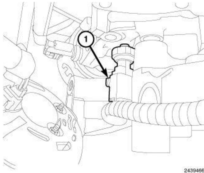
Fig. 375: Oil Pressure Sensor Electrical Connector Courtesy of CHRYSLER GROUP, LLC
