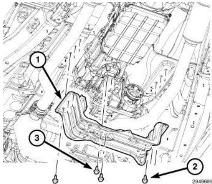
Fig. 24: Crossmember, Crossmember Bolts & Transmission Mount Bolts
