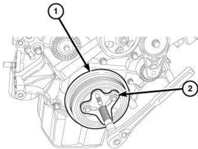
Fig. 221: Vibration Damper & Bolt Grip Puller
