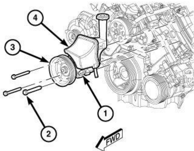
Fig. 63: Power Steering Reservoir, Pump, Pulley & Bolts Courtesy of CHRYSLER GROUP, LLC
