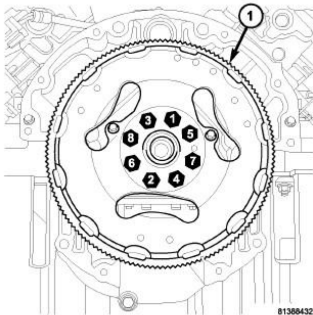
Fig. 240: Flex Plate Bolt Removal/Tightening Sequence Courtesy of CHRYSLER GROUP, LLC
