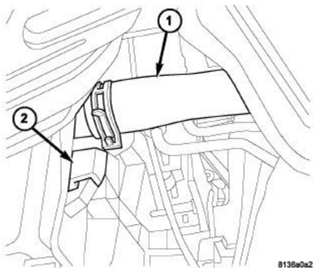
Fig. 54: Lower Radiator Hose Courtesy of CHRYSLER GROUP, LLC
