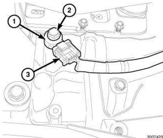
Fig. 30: Knock Sensor, Electrical Connector & Bolt Courtesy of CHRYSLER GROUP, LLC
