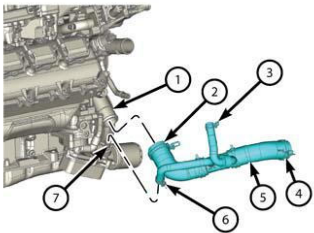
Fig. 447: Lower Radiator Hose Courtesy of CHRYSLER GROUP, LLC
