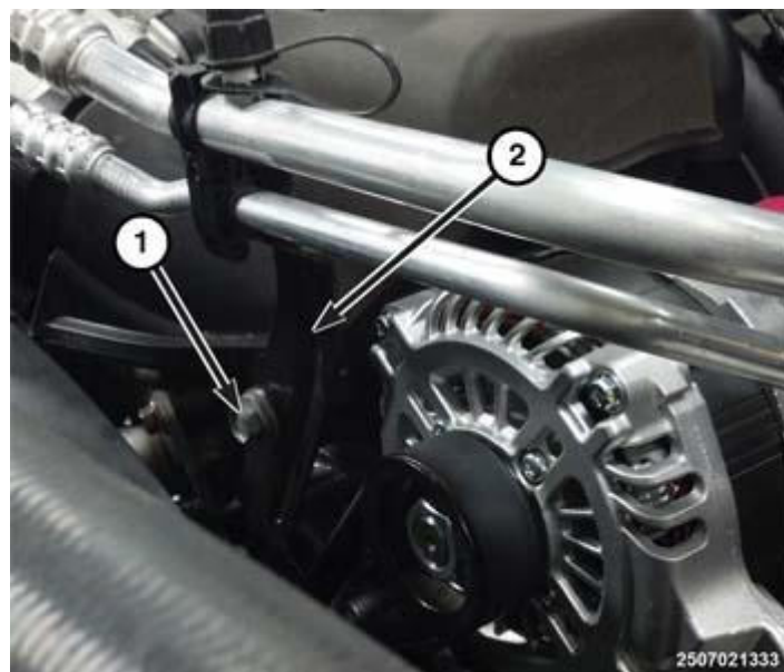
Fig. 456: A/C Line Support Bracket Courtesy of CHRYSLER GROUP, LLC
