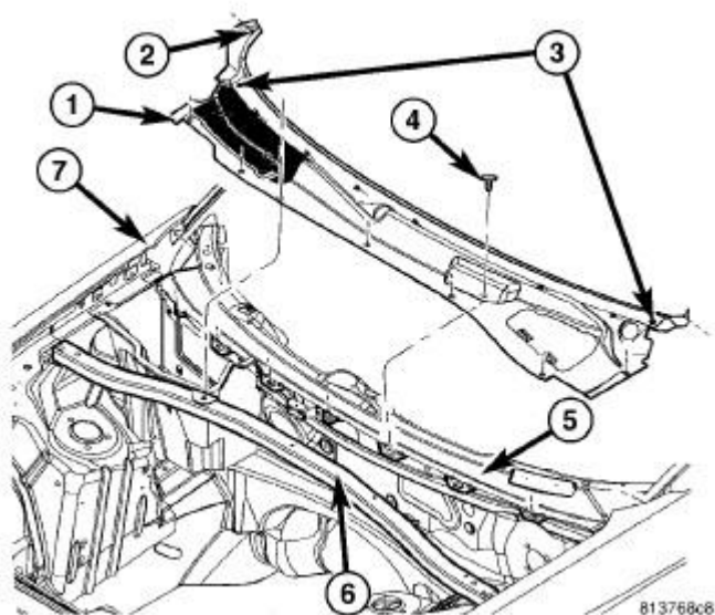
Fig. 11: Removing/Installing Cowl Panel Courtesy of CHRYSLER GROUP, LLC
