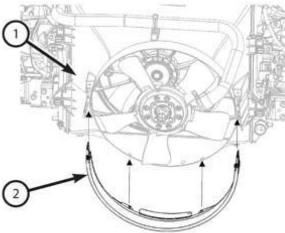
Fig. 433: Upper & Lower Shrouds Courtesy of CHRYSLER GROUP, LLC
