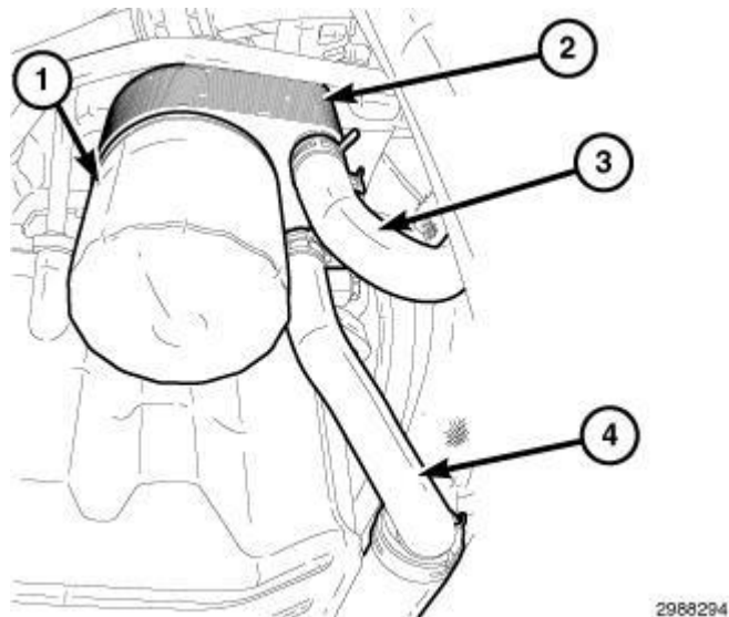
Fig. 320: Oil Filter, Oil Cooler & Hoses Courtesy of CHRYSLER GROUP, LLC
