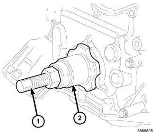
Fig. 267: Front Seal Installation Courtesy of CHRYSLER GROUP, LLC
