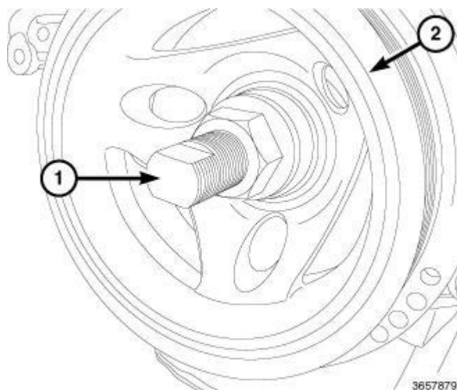
Fig. 449: Installing Vibration Damper Courtesy of CHRYSLER GROUP, LLC
