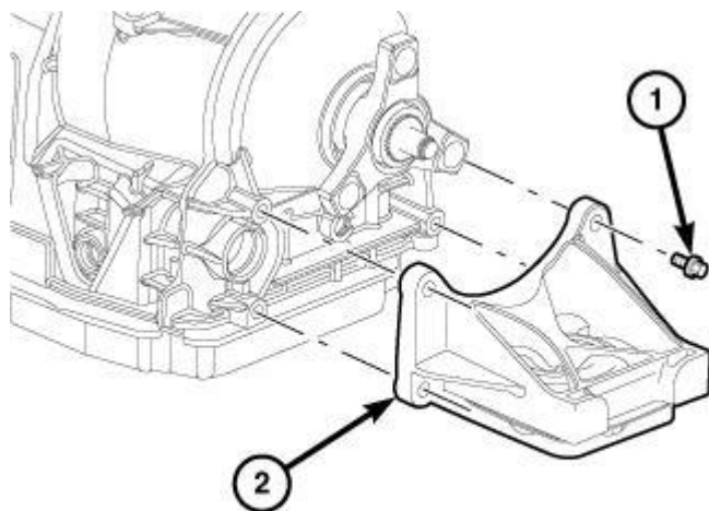
Fig. 282: Rear Transmission Mount Bracket Courtesy of CHRYSLER GROUP, LLC
