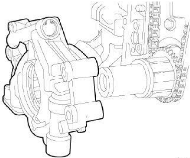
Fig. 423: Remove/Install Oil Pump Courtesy of CHRYSLER GROUP, LLC
