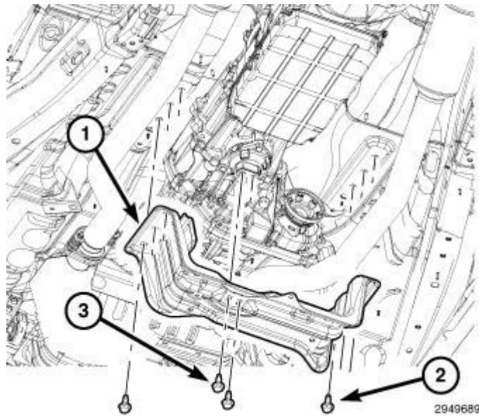
Fig. 73: Crossmember, Crossmember Bolts & Transmission Mount Bolts Courtesy of CHRYSLER GROUP, LLC
