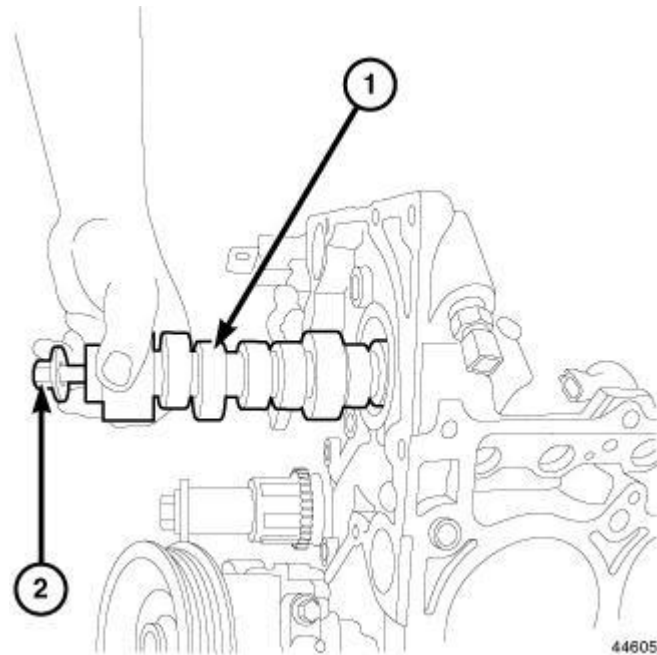
Fig. 165: Removing/Installing Camshaft Courtesy of CHRYSLER GROUP, LLC
