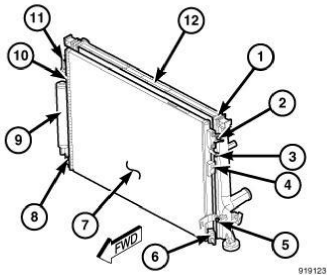
Fig. 159: A/C Condenser & Radiator Courtesy of CHRYSLER GROUP, LLC
