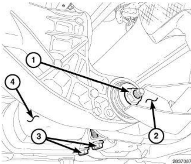
Fig. 354: Nut And Bolt, Front Axle Tube Bushing & Bolts Courtesy of CHRYSLER GROUP, LLC
