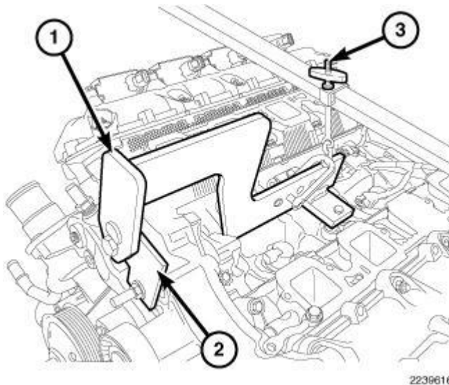
Fig. 302: Engine Lift Fixture & Adapter Courtesy of CHRYSLER GROUP, LLC
