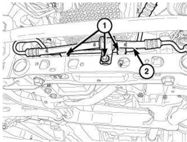
Fig. 342: Steering Gear Pressure Line Retainers & Pressure Line Courtesy of CHRYSLER GROUP, LLC
