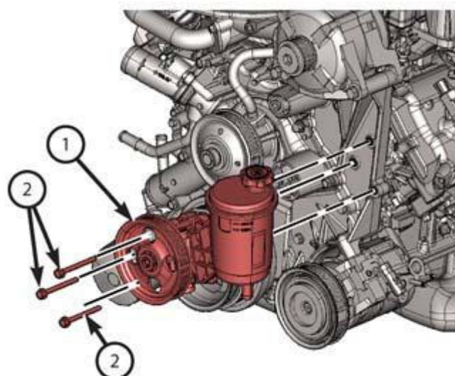
Fig. 452: Power Steering Pump Pulley & Bolts Courtesy of CHRYSLER GROUP, LLC
