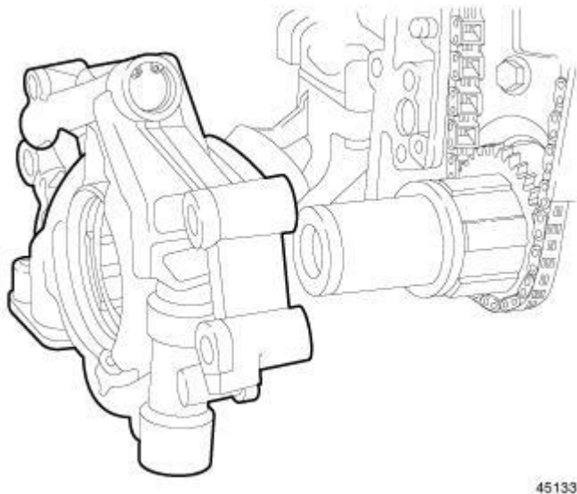
Fig. 170: Remove/Install Oil Pump Courtesy of CHRYSLER GROUP, LLC
