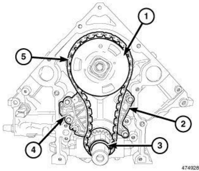
Fig. 169: Timing Chain, Sprockets, Timing Chain Tensioner & Guide Courtesy of CHRYSLER GROUP, LLC
