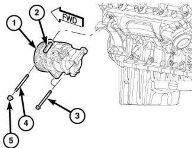
Fig. 306: A/C Clutch Electrical Connector, Two Bolts, A/C Compressor, Nut & Stud Courtesy of CHRYSLER GROUP, LLC
