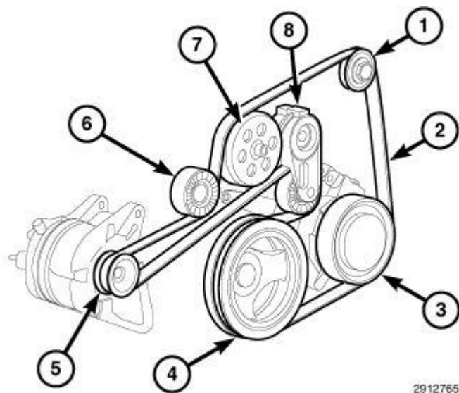
Fig. 19: Drive Belt Tensioner And Drive Belt Routing Courtesy of CHRYSLER GROUP, LLC
