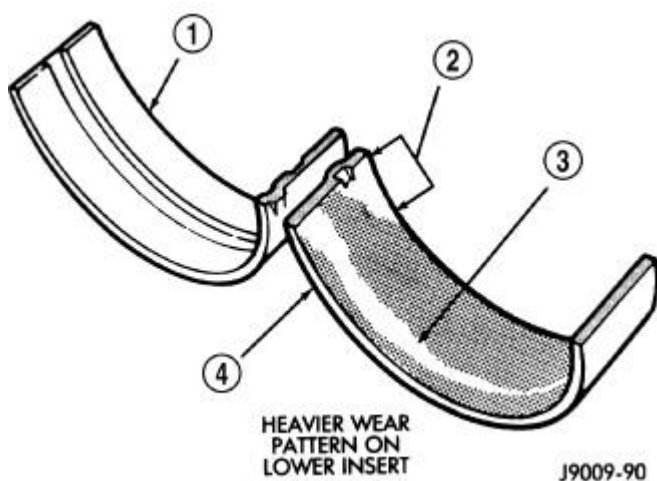
Fig. 154: Main Bearing Wear Patterns Courtesy of CHRYSLER GROUP, LLC
