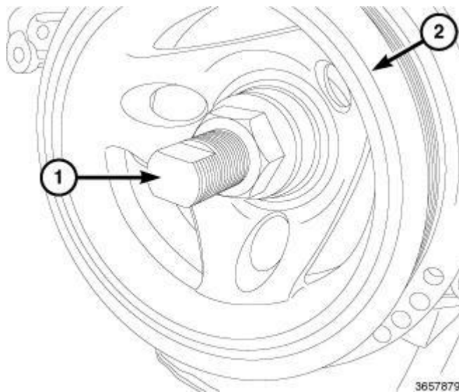
Fig. 223: Installing Vibration Damper Courtesy of CHRYSLER GROUP, LLC
