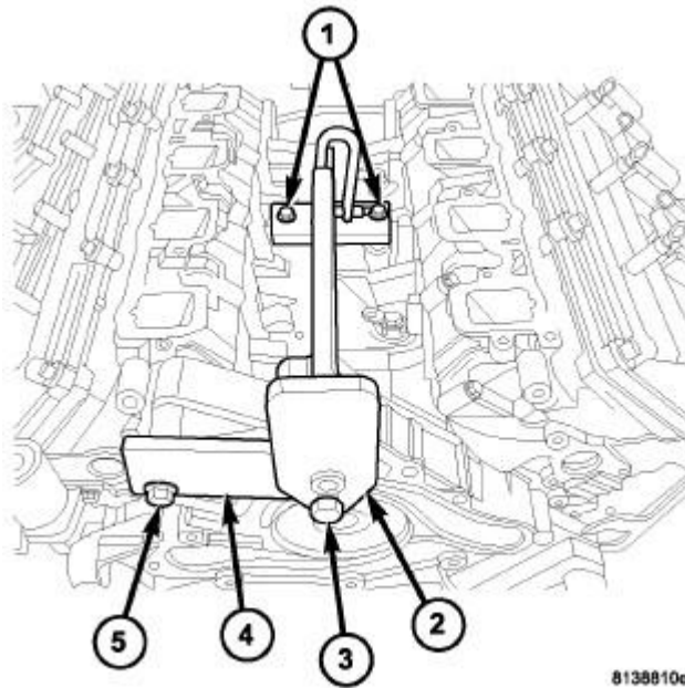
Fig. 43: Engine Lift Fixture & Adapter Courtesy of CHRYSLER GROUP, LLC
