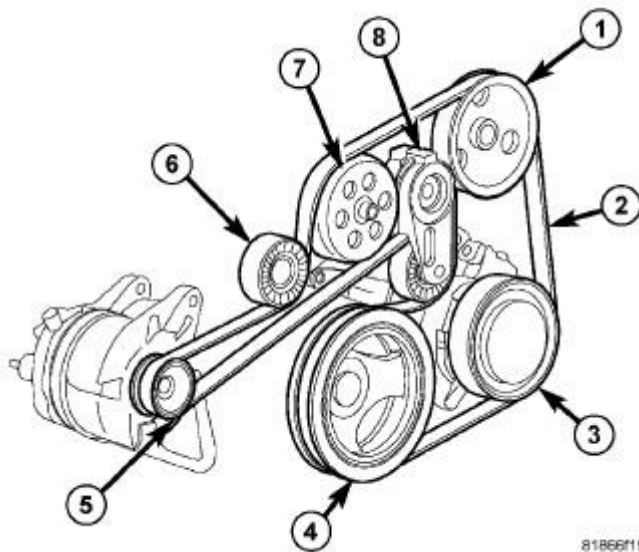
Fig. 98: Accessory Drive Belt Routing, Tensioner & Pulleys Courtesy of CHRYSLER GROUP, LLC
