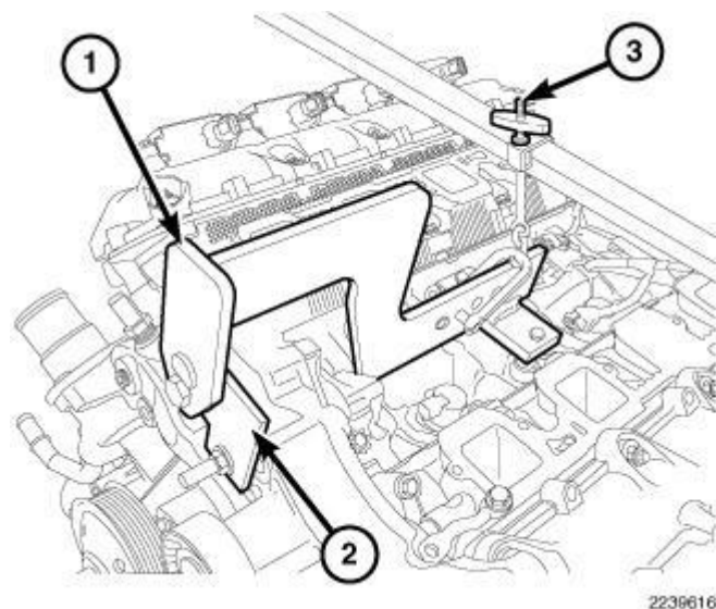
Fig. 357: Engine Lift Fixture & Adapter Courtesy of CHRYSLER GROUP, LLC
