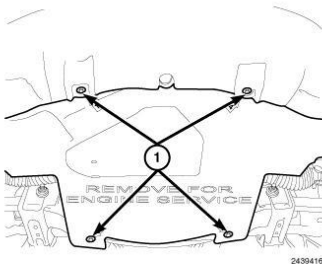
Fig. 370: Lower Splash Shield & Fasteners Courtesy of CHRYSLER GROUP, LLC
