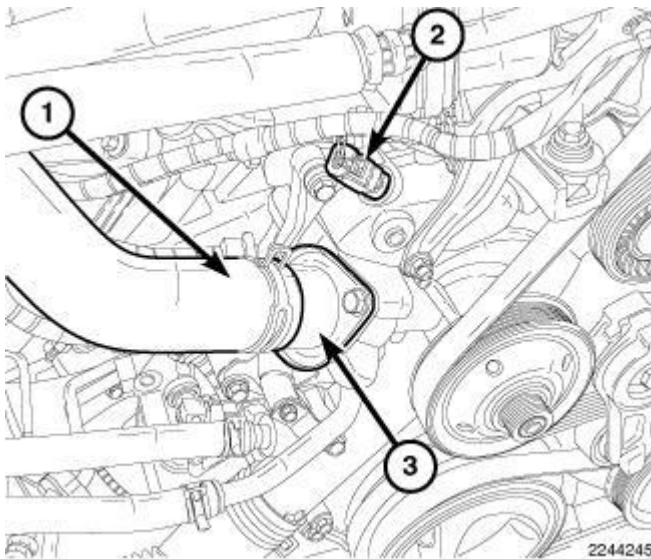
Fig. 455: Engine Coolant Temperature (ECT) Sensor & Thermostat Courtesy of CHRYSLER GROUP, LLC
