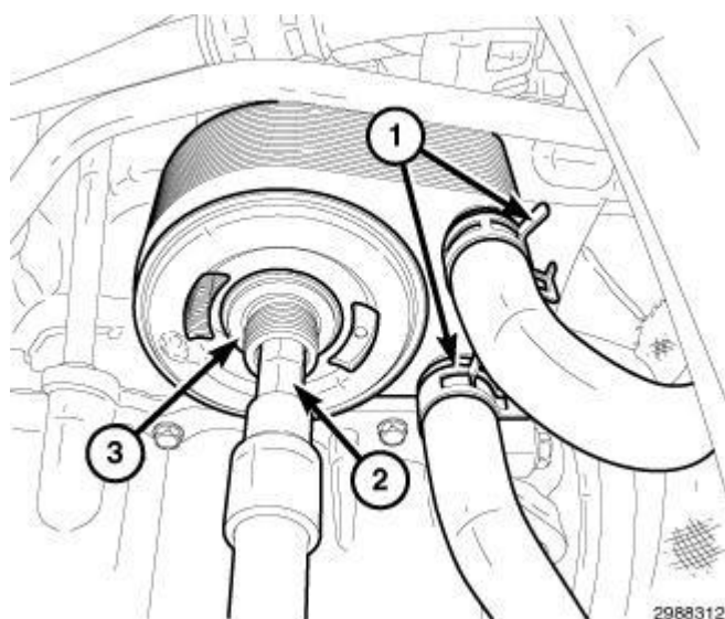
Fig. 324: Clamps, Allen Wrench Socket & Oil Cooler Retaining Bolt
