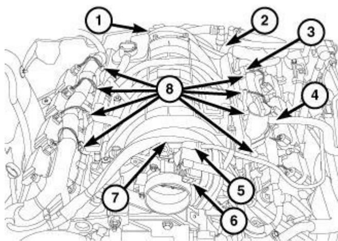
Fig. 359: Map Sensor, Brake Booster Vacuum Hose, Fuel Supply Line, Make Up Air Hose, EVAP Vacuum Purge Hose, Electrical Connector & Electrical Harness Courtesy of CHRYSLER GROUP, LLC
