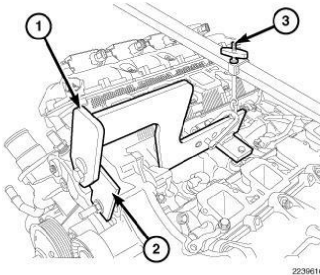
Fig. 339: Engine Lift Fixture & Adapter Courtesy of CHRYSLER GROUP, LLC
