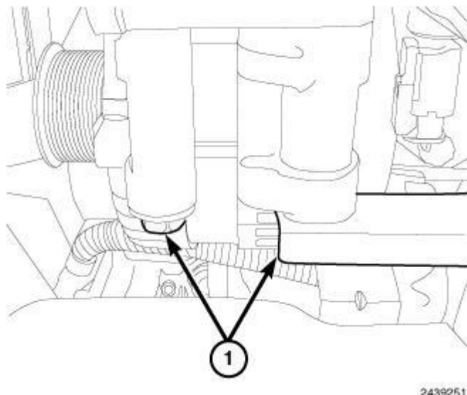
Fig. 384: Lower Generator Retaining Bolts Courtesy of CHRYSLER GROUP, LLC
