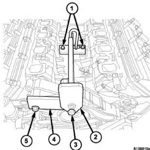
Fig. 42: Engine Lift Fixture & Adapter Courtesy of CHRYSLER GROUP, LLC
