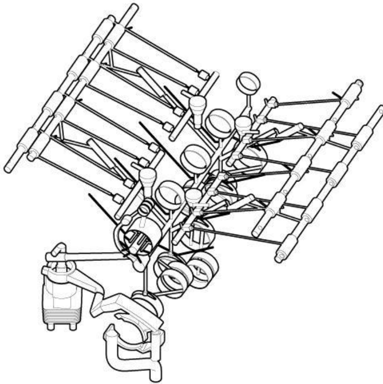
Fig. 310: 6.4L Lubrication System Courtesy of CHRYSLER GROUP, LLC
