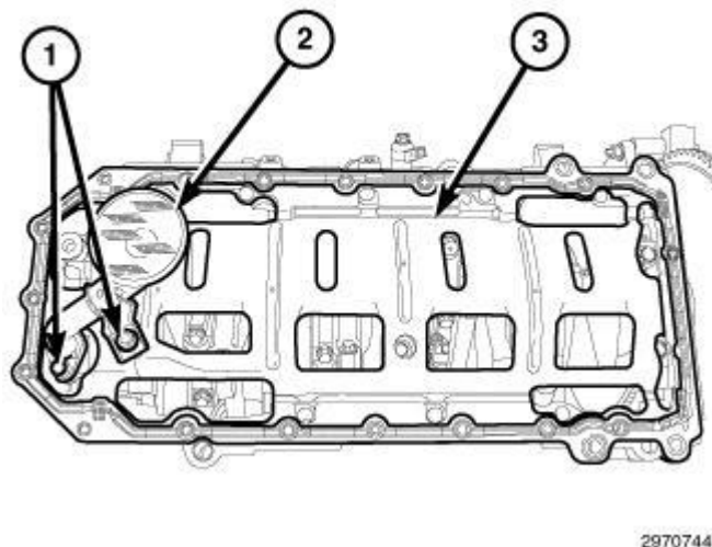
Fig. 362: Integral Windage Tray, Oil Pump Pickup Tube & Bolts Courtesy of CHRYSLER GROUP, LLC
