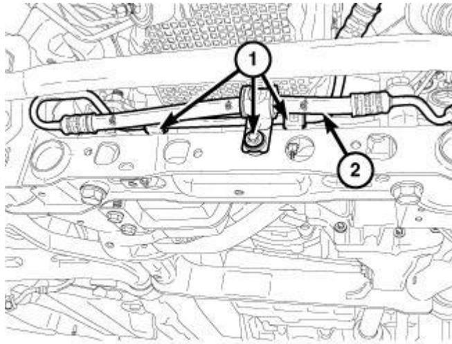
Fig. 351: Steering Gear Pressure Line Retainers & Pressure Line Courtesy of CHRYSLER GROUP, LLC
