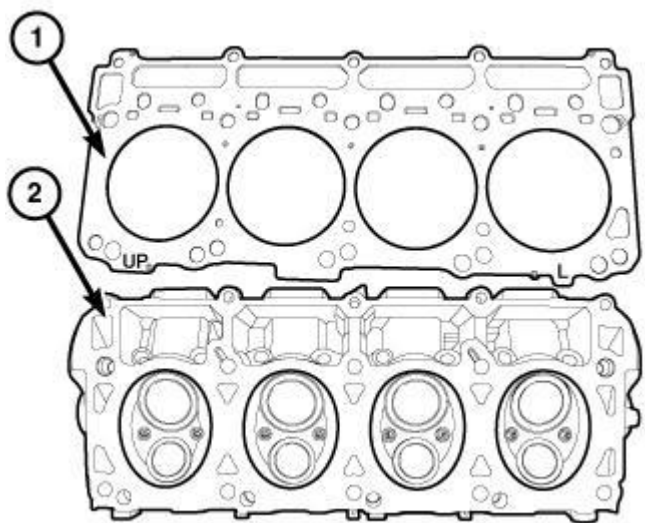
Fig. 90: Cylinder Head Gasket & Cylinder Head
