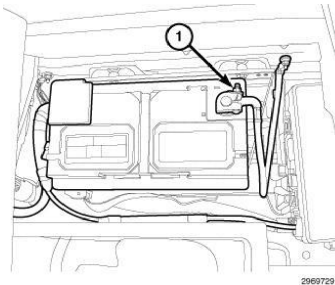
Fig. 143: Negative Battery Cable Courtesy of CHRYSLER GROUP, LLC
