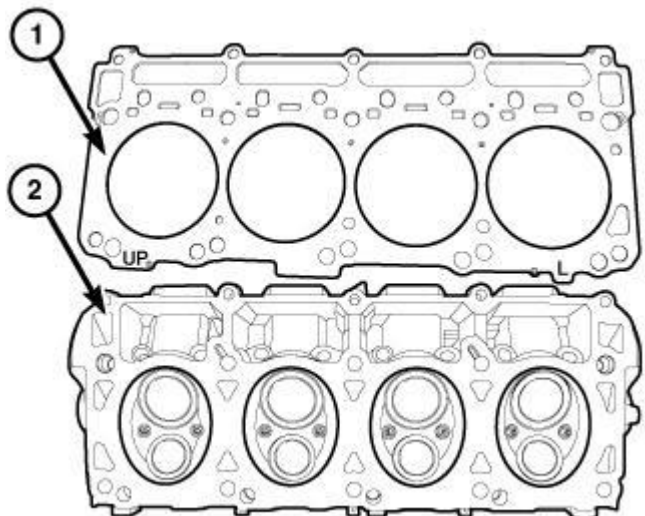
Fig. 93: Cylinder Head Gasket & Cylinder Head
