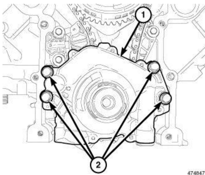
Fig. 367: Oil Pump Retaining Bolts
