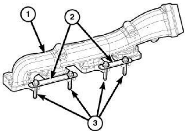
Fig. 389: Exhaust Manifold, Tie Bars & Bolts Courtesy of CHRYSLER GROUP, LLC
