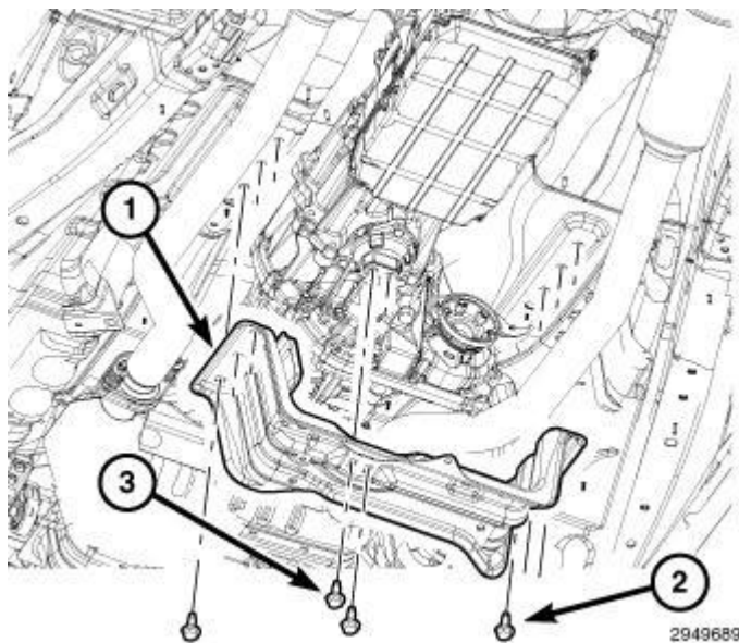
Fig. 29: Crossmember, Crossmember Bolts & Transmission Mount Bolts Courtesy of CHRYSLER GROUP, LLC
