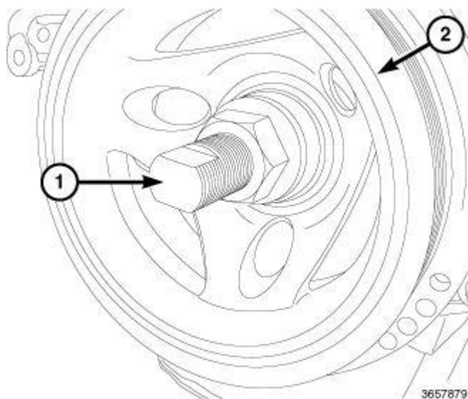
Fig. 268: Installing Vibration Damper Courtesy of CHRYSLER GROUP, LLC
