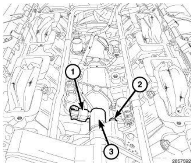
Fig. 56: Oil Control Valve, Electrical Connector & Retaining Bolt Courtesy of CHRYSLER GROUP, LLC
