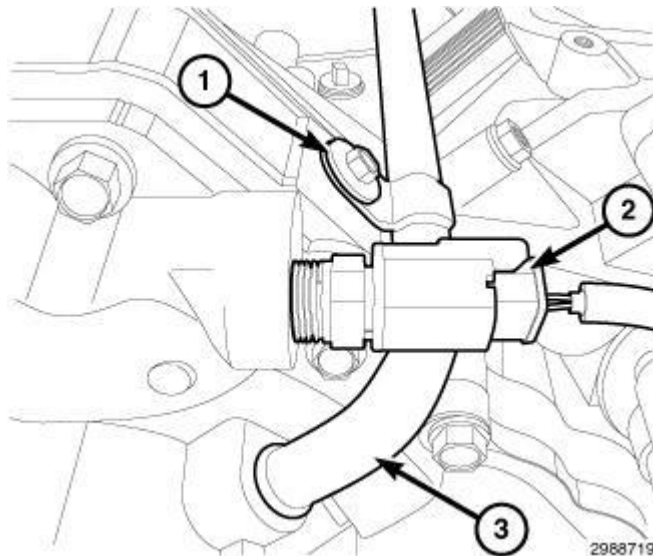
Fig. 13: Coolant Temperature (ECT) Sensor Electrical Connector, Heater Tube & Retaining Bolt Courtesy of CHRYSLER GROUP, LLC
