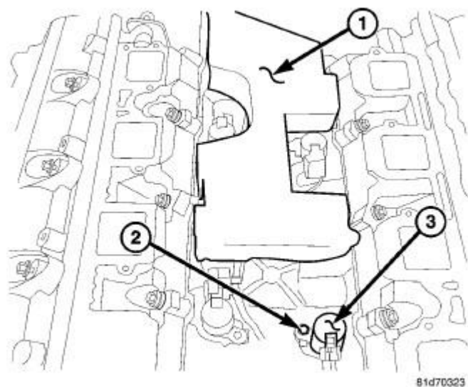
Fig. 273: Intake Manifold Foam Insulator Pad, MDS Solenoids & Bolts Courtesy of CHRYSLER GROUP, LLC
