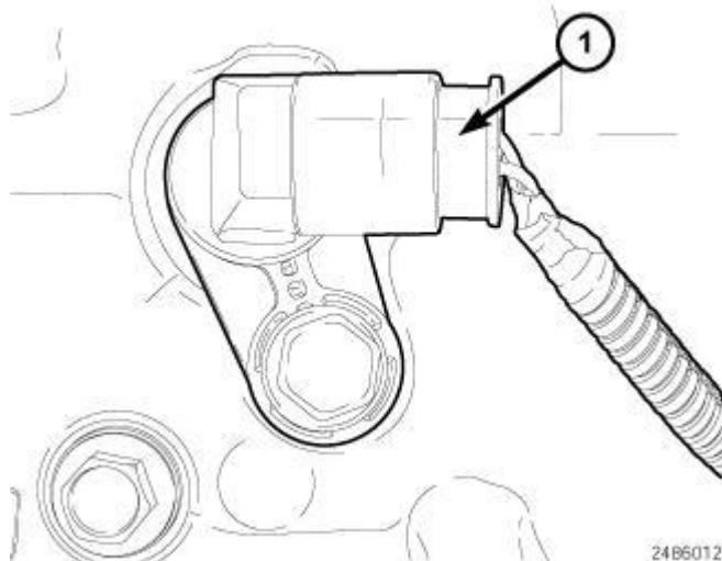
Fig. 31: Crankshaft Position Sensor Electrical Connector Courtesy of CHRYSLER GROUP, LLC
