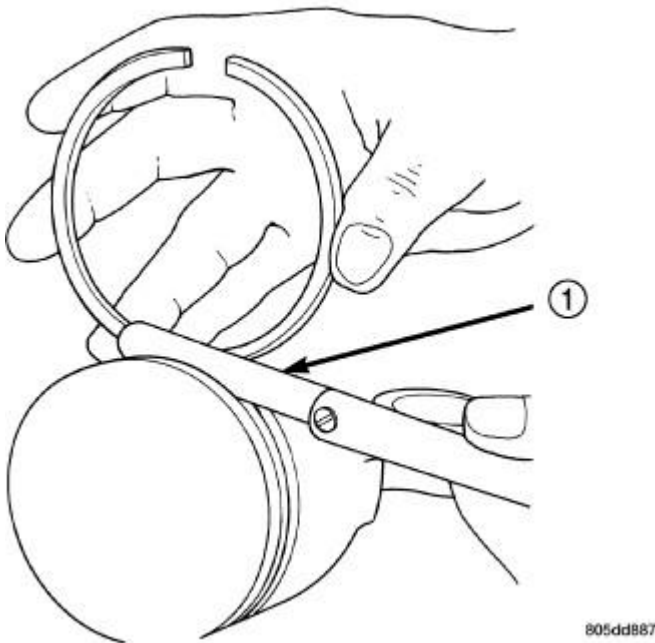
Fig. 243: Measuring Piston Ring Side Clearance Courtesy of CHRYSLER GROUP, LLC
