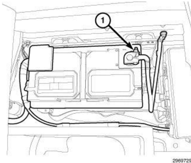
Fig. 394: Negative Battery Cable Courtesy of CHRYSLER GROUP, LLC
