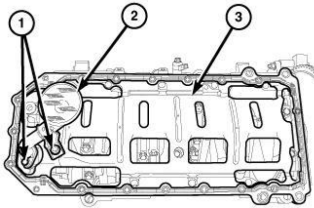
Fig. 406: Integral Windage Tray, Oil Pump Pickup Tube & Bolts Courtesy of CHRYSLER GROUP, LLC
