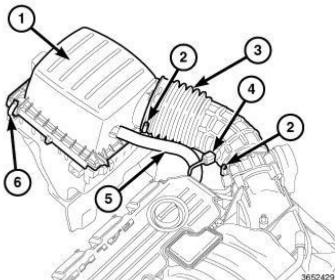
Fig. 79: Intake Air Temperature (IAT) Sensor, Air Cleaner Housing & Duct Courtesy of CHRYSLER GROUP, LLC
