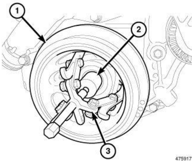
Fig. 216: Removing Vibration Damper Courtesy of CHRYSLER GROUP, LLC
