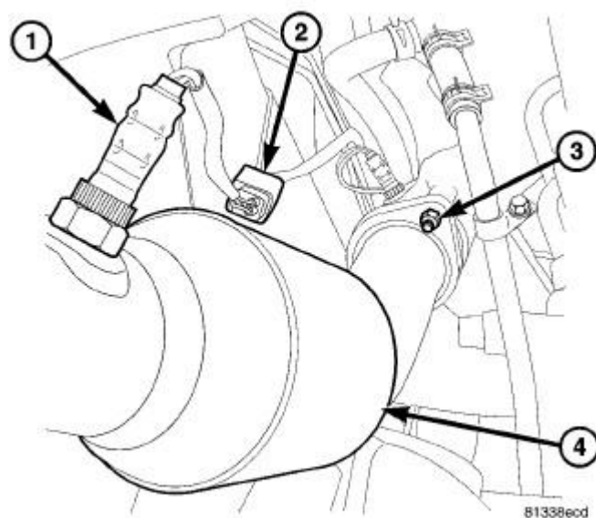
Fig. 26: Oxygen Sensor, Oxygen Sensor Connector, Ball Flange Nut & LH Catalytic Converter Courtesy of CHRYSLER GROUP, LLC
