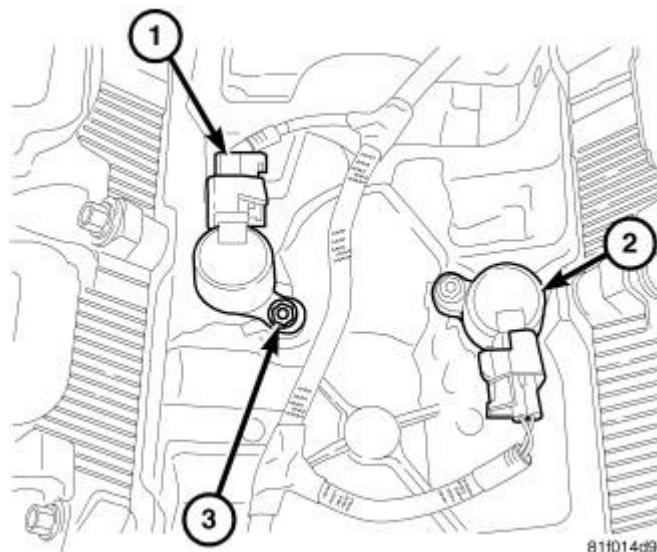
Fig. 277: MDS Solenoid Connector Courtesy of CHRYSLER GROUP, LLC
