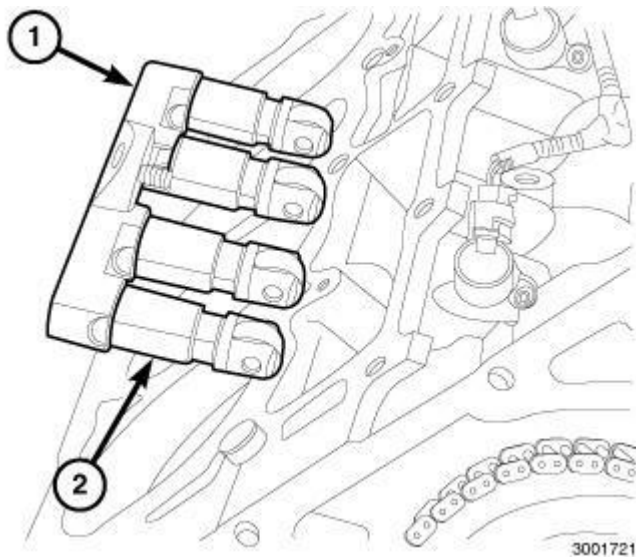
Fig. 233: Hydraulic Lifters/Tappets & Retainer/Guide Holder Courtesy of CHRYSLER GROUP, LLC
