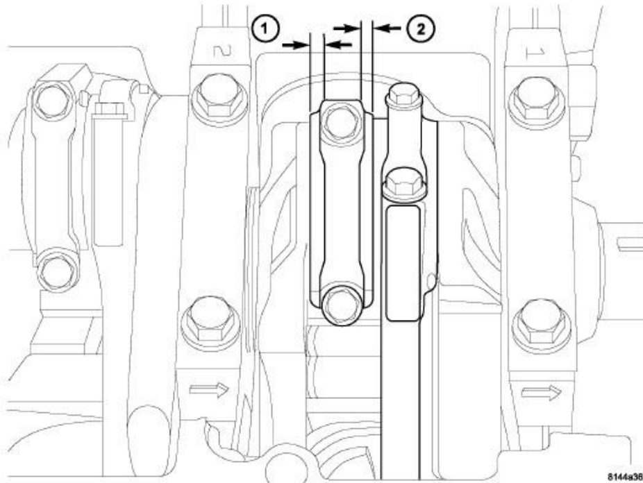
Fig. 203: Connecting Rod Proper Installation Courtesy of CHRYSLER GROUP, LLC
