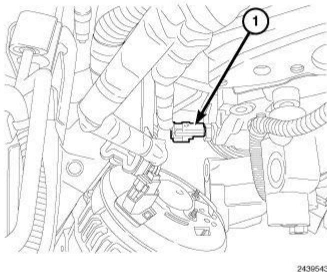
Fig. 383: Oil Temperature Sensor Electrical Connector Courtesy of CHRYSLER GROUP, LLC
