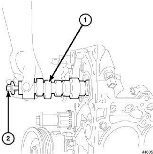
Fig. 167: Removing/Installing Camshaft Courtesy of CHRYSLER GROUP, LLC
