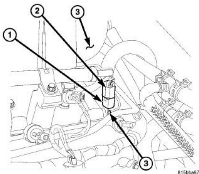
Fig. 18: Ignition Capacitor, Electrical Connector & Intake Manifold Courtesy of CHRYSLER GROUP, LLC
