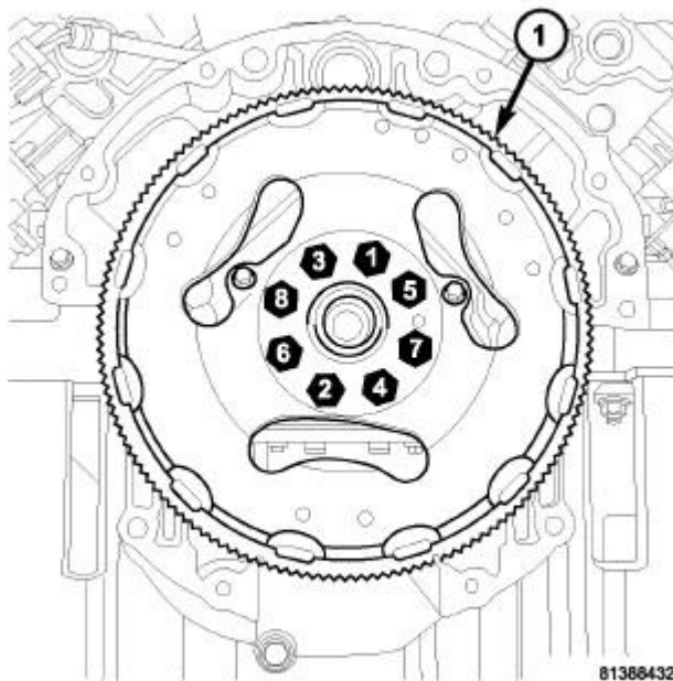
Fig. 184: Flex Plate Bolt Removal/Tightening Sequence
