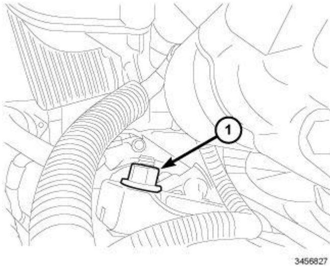
Fig. 338: Engine Mount Retaining Nut Courtesy of CHRYSLER GROUP, LLC
