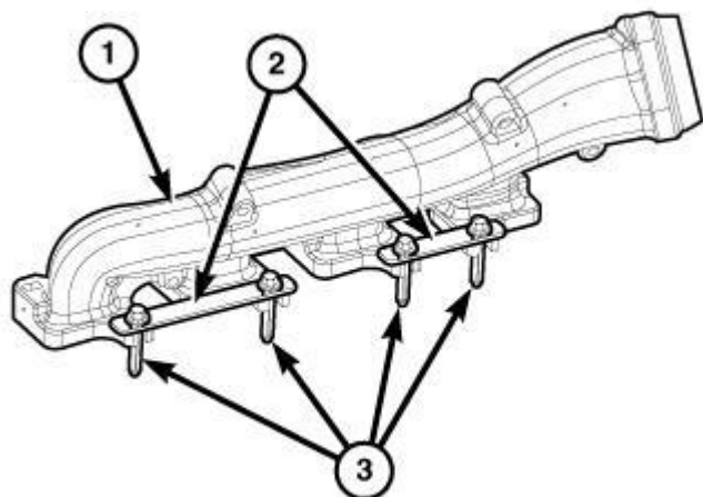
Fig. 390: Exhaust Manifold, Tie Bars & Bolts
