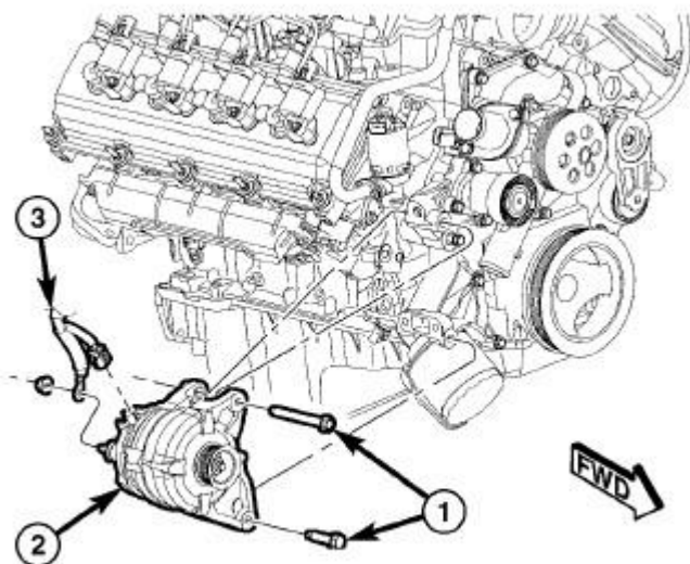
Fig. 304: Generator & Retaining Bolts Courtesy of CHRYSLER GROUP, LLC
