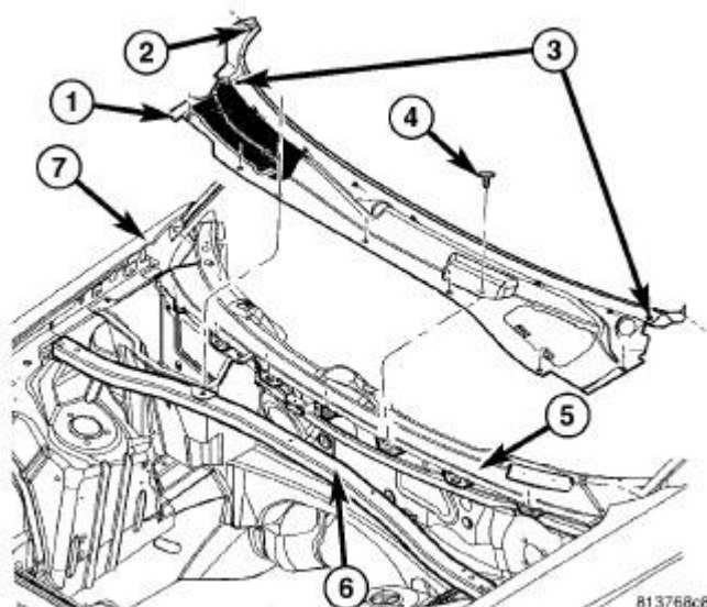
Fig. 70: Removing/Installing Cowl Panel Courtesy of CHRYSLER GROUP, LLC
