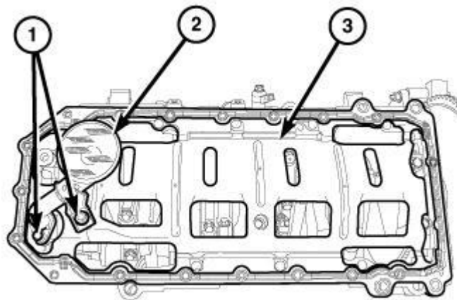
Fig. 427: Integral Windage Tray, Oil Pump Pickup Tube & Bolts Courtesy of CHRYSLER GROUP, LLC
