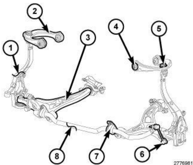
Fig. 341: Suspension Components With Rubber/Urethane Bushings Courtesy of CHRYSLER GROUP, LLC
