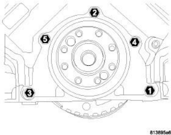
Fig. 186: Rear Seal Retainer Removal/Tightening Sequence Courtesy of CHRYSLER GROUP, LLC
