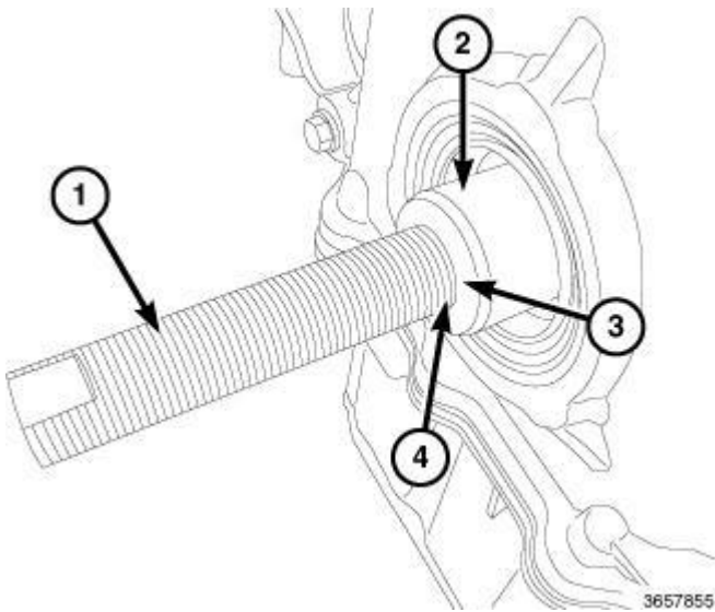
Fig. 222: Installing Vibration Damper Onto Crankshaft Using Special Tool Courtesy of CHRYSLER GROUP, LLC
