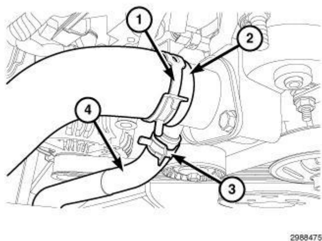
Fig. 270: Upper Radiator Hose, Clamp, Oil Cooler Return Line Hose & Clamp Courtesy of CHRYSLER GROUP, LLC
