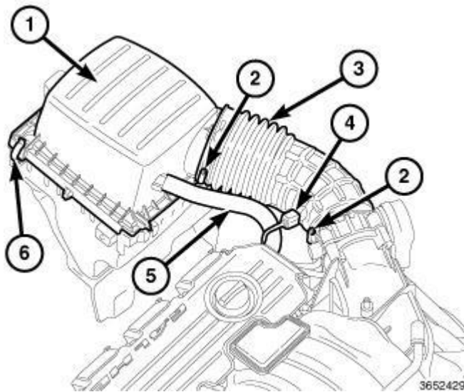
Fig. 9: Intake Air Temperature (IAT) Sensor, Air Cleaner Housing & Duct Courtesy of CHRYSLER GROUP, LLC
