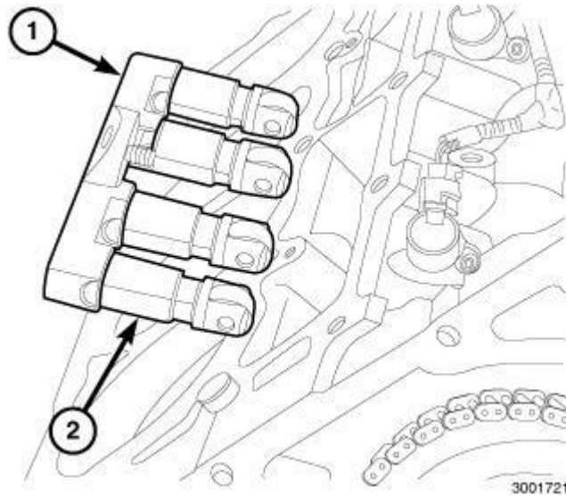
Fig. 157: Hydraulic Lifters/Tappets & Retainer/Guide Holder Courtesy of CHRYSLER GROUP, LLC
