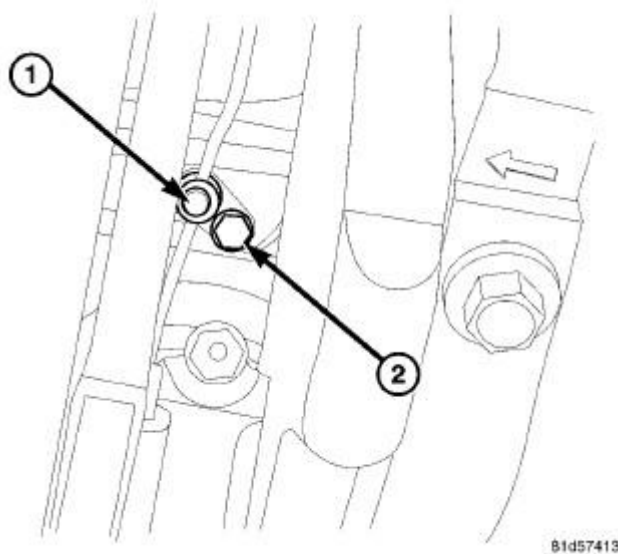
Fig. 333: Piston Oil Jet & Bolt Courtesy of CHRYSLER GROUP, LLC
