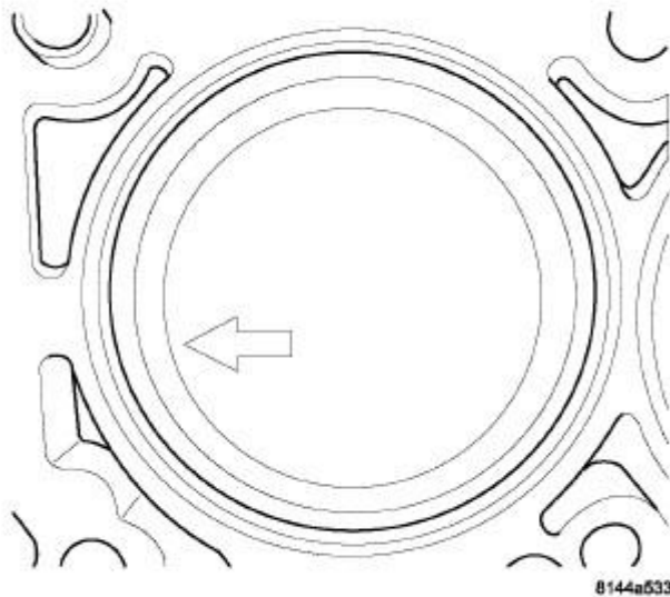
Fig. 254: Piston Direction Arrow Courtesy of CHRYSLER GROUP, LLC
