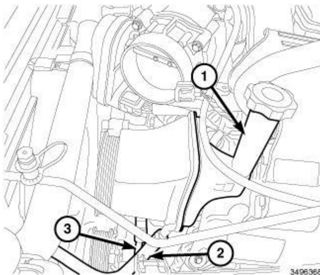
Fig. 107: Power Steering Pump, Pressure Hose & Return Hose Courtesy of CHRYSLER GROUP, LLC
