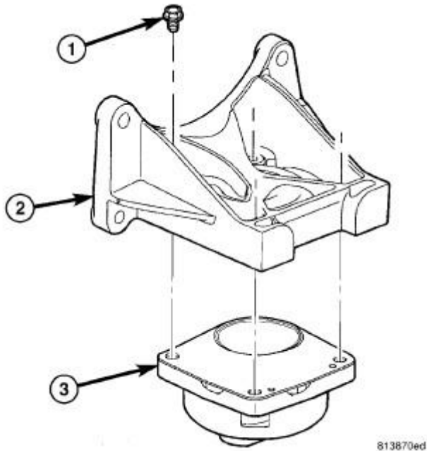
Fig. 281: Rear Transmission Mount Isolator Courtesy of CHRYSLER GROUP, LLC
