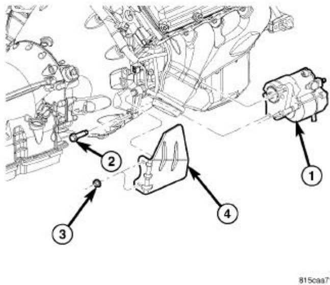
Fig. 28: Removing/Installing Starter Courtesy of CHRYSLER GROUP, LLC
