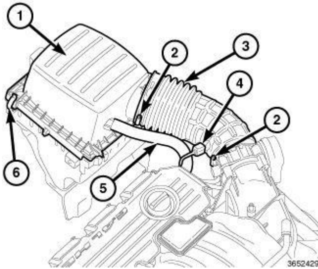
Fig. 402: Intake Air Temperature (IAT) Sensor, Air Cleaner Housing & Duct Courtesy of CHRYSLER GROUP, LLC
