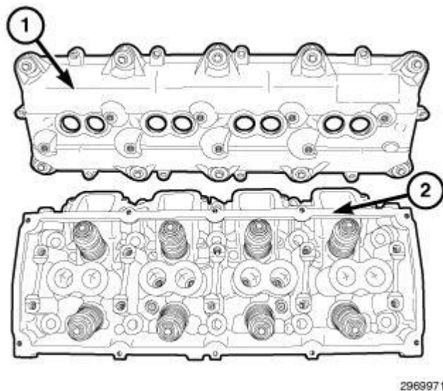
Fig. 109: Cylinder Head & Cover Courtesy of CHRYSLER GROUP, LLC
