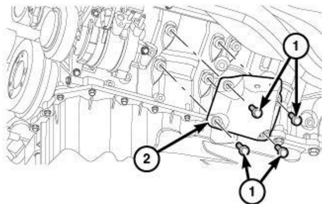
Fig. 299: Engine Mount-To-Engine Block Mounting Brackets & Retaining Bolts Courtesy of CHRYSLER GROUP, LLC
