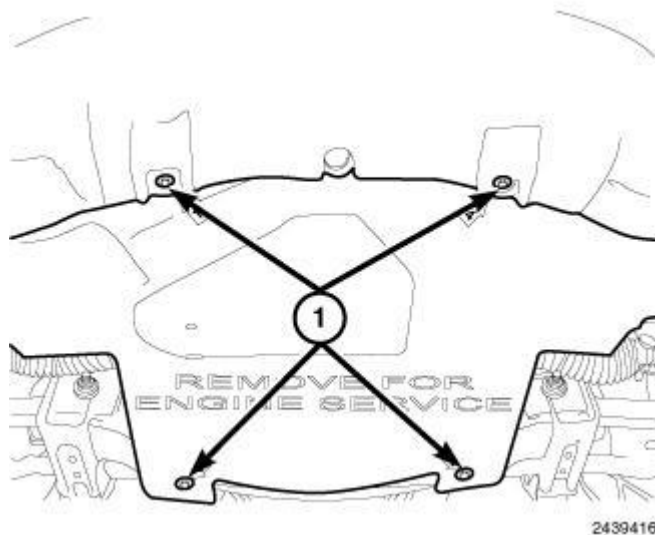
Fig. 378: Lower Splash Shield & Fasteners Courtesy of CHRYSLER GROUP, LLC
