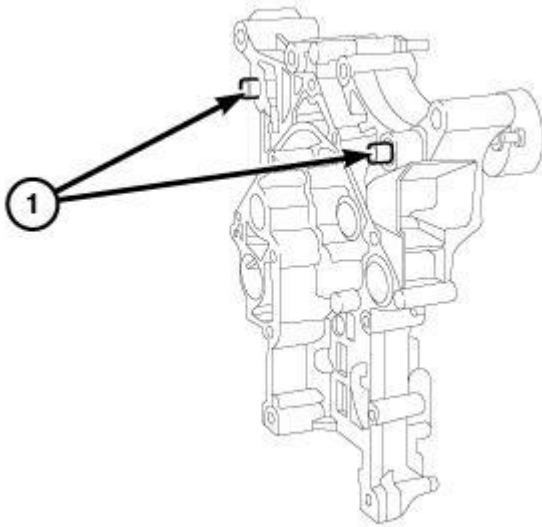
Fig. 443: Front Cover Slide Bushings Courtesy of CHRYSLER GROUP, LLC
