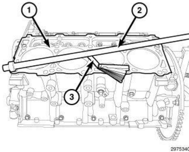
Fig. 151: Checking Engine Block Deck Surface With Precision Straightedge & Feeler Gauge Courtesy of CHRYSLER GROUP, LLC
