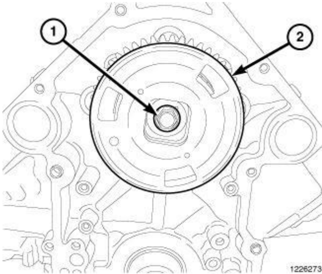
Fig. 313: Camshaft Phaser & Bolt Courtesy of CHRYSLER GROUP, LLC
