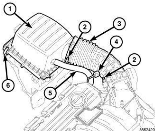
Fig. 80: Intake Air Temperature (IAT) Sensor, Air Cleaner Housing & Duct Courtesy of CHRYSLER GROUP, LLC
