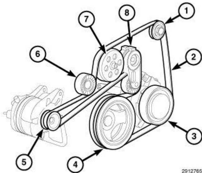
Fig. 67: Drive Belt Tensioner And Drive Belt Routing Courtesy of CHRYSLER GROUP, LLC
