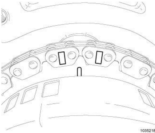
Fig. 416: Aligning Timing Chain & Camshaft Phaser Marks Courtesy of CHRYSLER GROUP, LLC
