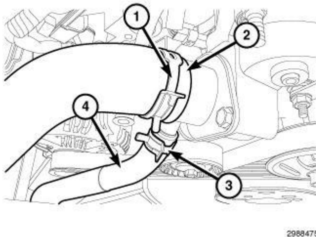
Fig. 262: Upper Radiator Hose, Clamp, Oil Cooler Return Line Hose & Clamp Courtesy of CHRYSLER GROUP, LLC
