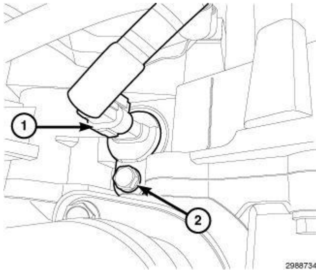
Fig. 436: Camshaft Position Sensor Electrical Connector & Bolt Courtesy of CHRYSLER GROUP, LLC
