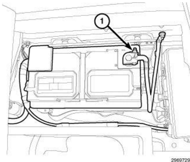
Fig. 116: Negative Battery Cable
