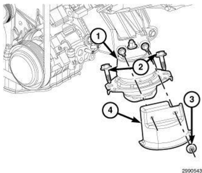
Fig. 41: Engine Mount Heat Shield Retaining Nuts, Lower Mount Retaining Bolts & Heat Shields Courtesy of CHRYSLER GROUP, LLC
