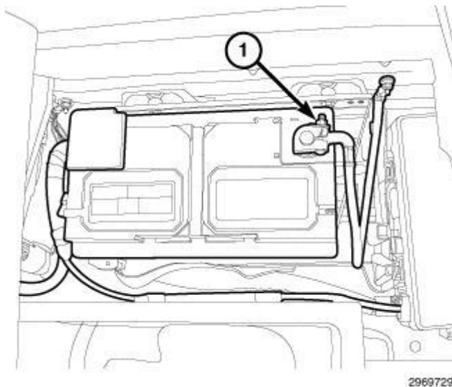
Fig. 241: Negative Battery Cable Courtesy of CHRYSLER GROUP, LLC
