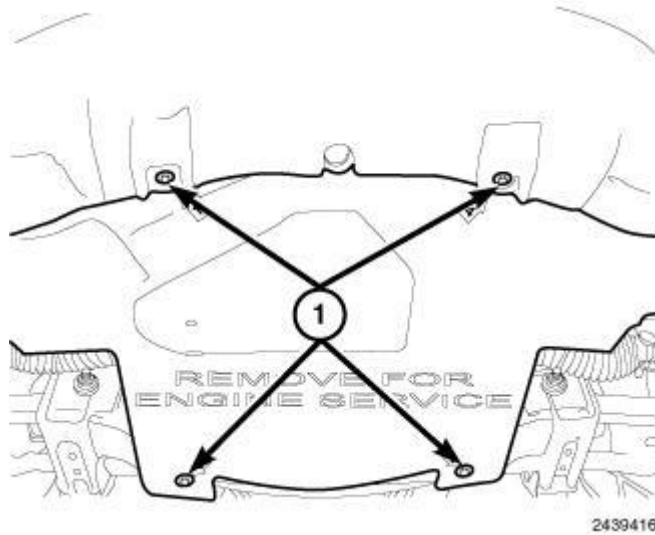
Fig. 377: Lower Splash Shield & Fasteners Courtesy of CHRYSLER GROUP, LLC
