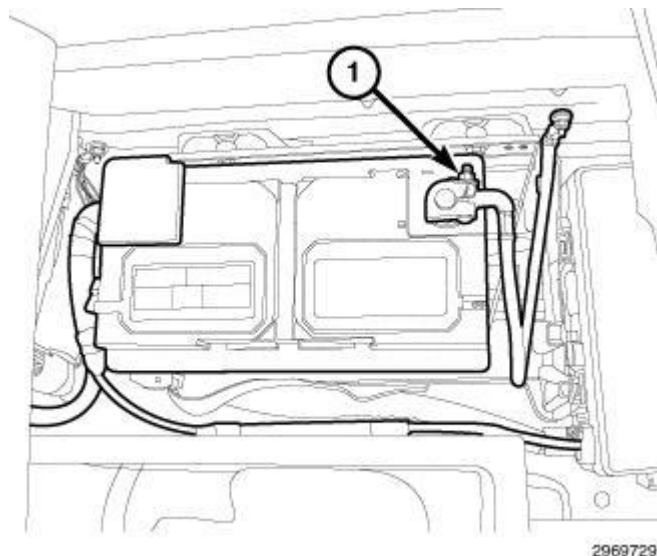
Fig. 180: Negative Battery Cable Courtesy of CHRYSLER GROUP, LLC
