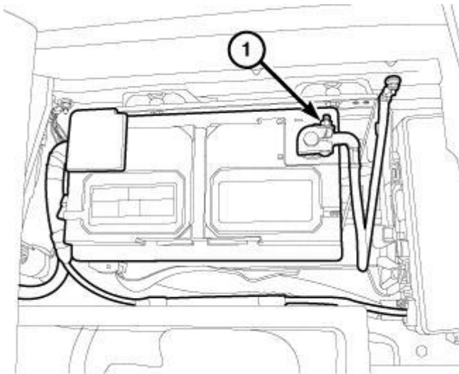
Fig. 260: Negative Battery Cable Courtesy of CHRYSLER GROUP, LLC
