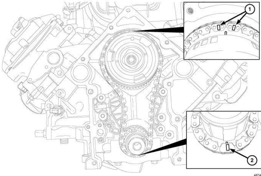
Fig. 409: Aligning Timing Marks With Timing Chain Sprockets Courtesy of CHRYSLER GROUP, LLC
