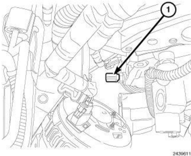
Fig. 382: Oil Temperature Sensor Courtesy of CHRYSLER GROUP, LLC
