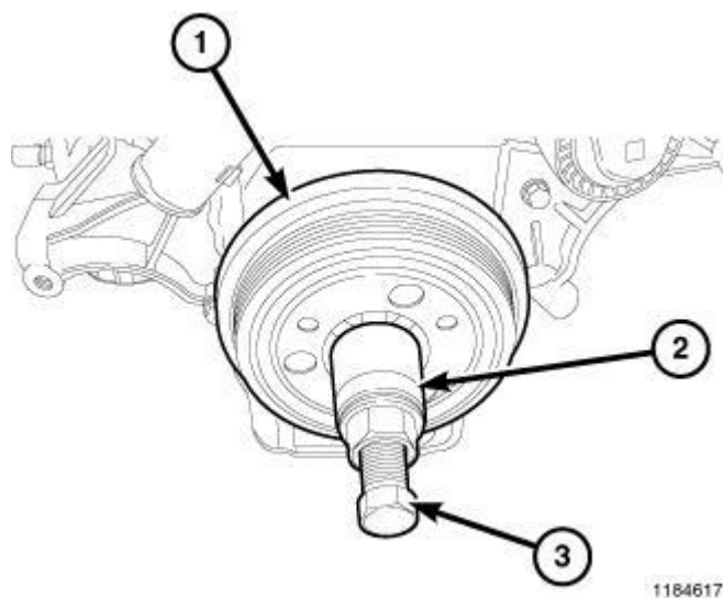
Fig. 210: Pressing Damper Onto Crankshaft Courtesy of CHRYSLER GROUP, LLC
