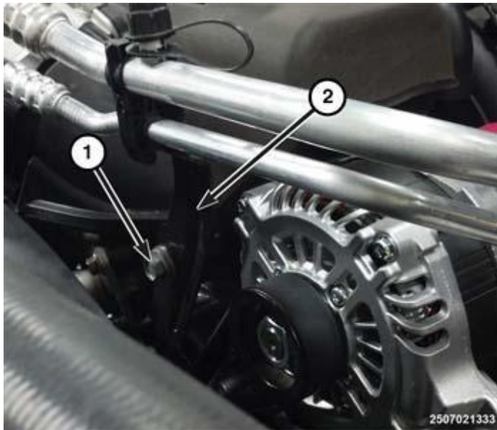
Fig. 434: A/C Line Support Bracket Courtesy of CHRYSLER GROUP, LLC
