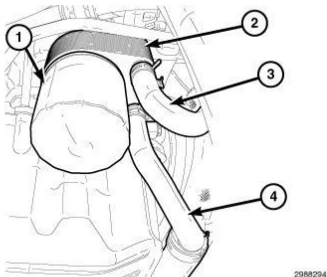
Fig. 355: Oil Filter, Oil Cooler & Hoses Courtesy of CHRYSLER GROUP, LLC
