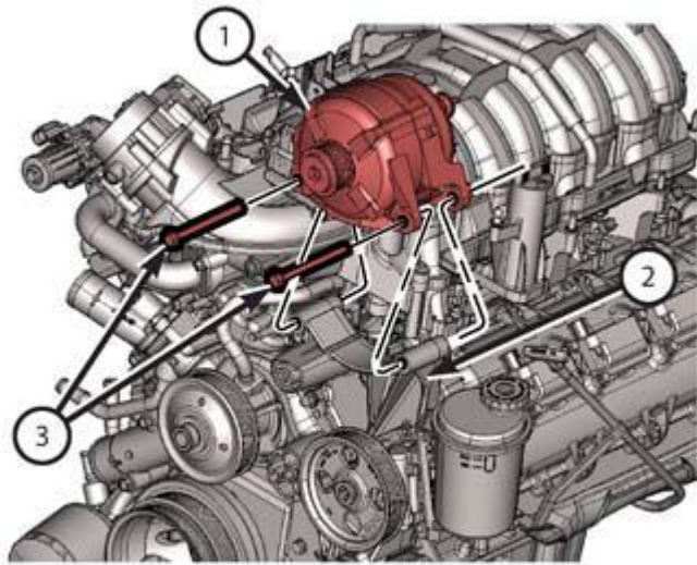
Fig. 450: Generator, Bolts & Connector Courtesy of CHRYSLER GROUP, LLC
