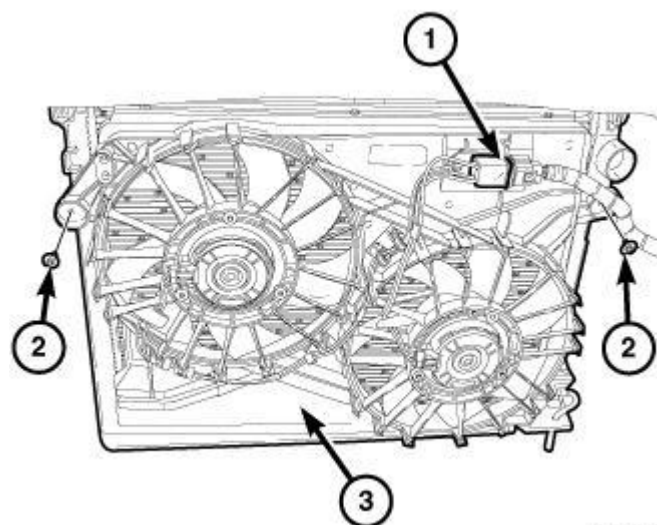
Fig. 220: Cooling Fan Electrical Connector, Cooling Fan Mounting Bolts & Radiator Cooling Fan Assembly
