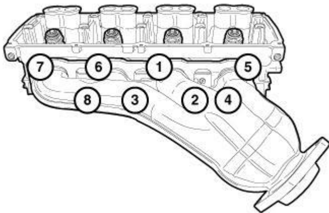
Fig. 92: Exhaust Manifold Removal/Tightening Sequence Courtesy of CHRYSLER GROUP, LLC
