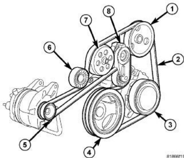
Fig. 308: Accessory Drive Belt Routing, Tensioner & Pulleys Courtesy of CHRYSLER GROUP, LLC
