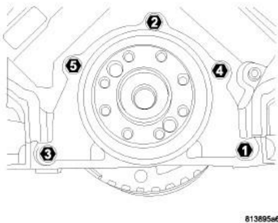
Fig. 239: Rear Seal Retainer Torque Sequence Courtesy of CHRYSLER GROUP, LLC
