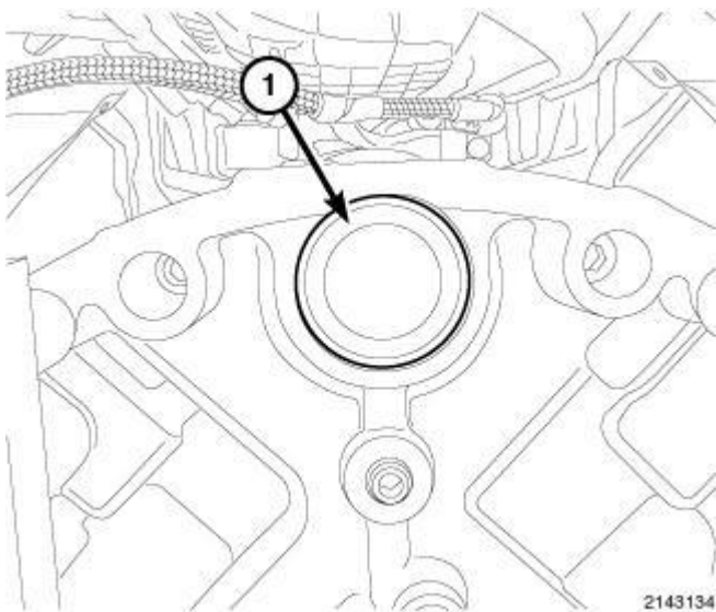
Fig. 155: Camshaft Core Hole Plug Courtesy of CHRYSLER GROUP, LLC
