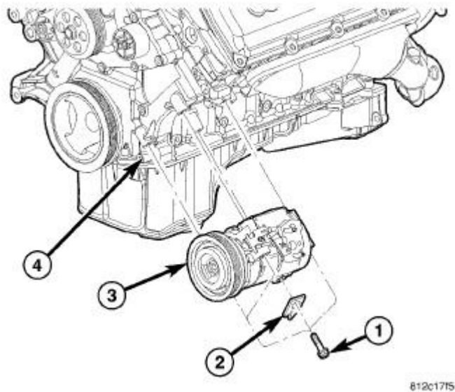
Fig. 53: Removing/Installing A/C Compressor Courtesy of CHRYSLER GROUP, LLC
