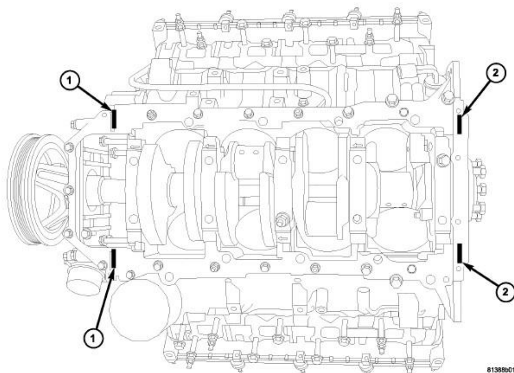
Fig. 347: T-Joint RTV Sealant Application Locations
