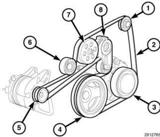
Fig. 226: Drive Belt Tensioner And Drive Belt Routing Courtesy of CHRYSLER GROUP, LLC
