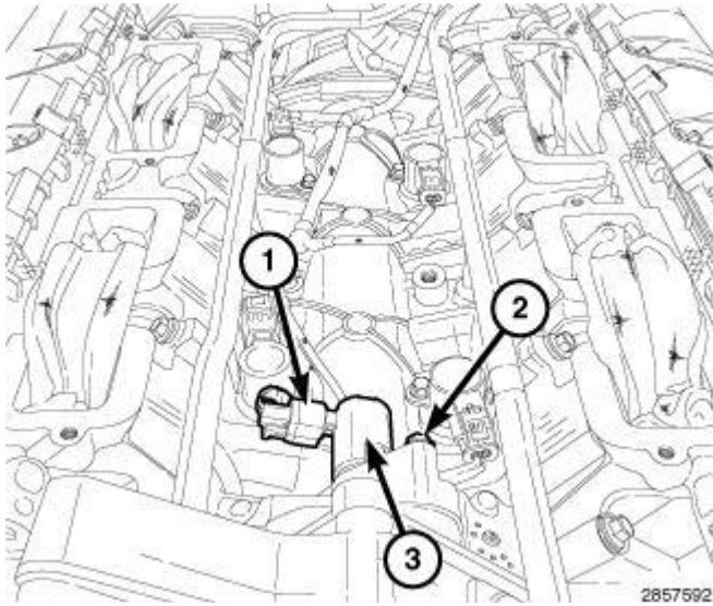
Fig. 312: Oil Control Valve, Electrical Connector & Retaining Bolt
