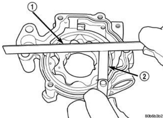
Fig. 366: Measuring Clearance Over Rotors Courtesy of CHRYSLER GROUP, LLC
