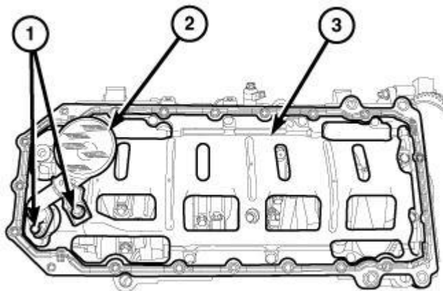
Fig. 172: Integral Windage Tray, Oil Pump Pickup Tube & Bolts Courtesy of CHRYSLER GROUP, LLC
