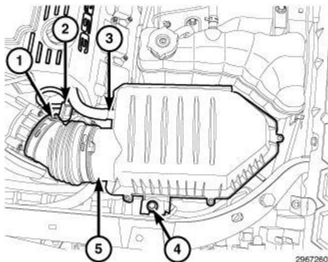
Fig. 179: Air Duct Retaining Clamp, Intake Air Temperature Sensor Electrical Connector, Makeup Air Hose, Bolt & Air Cleaner Housing Courtesy of CHRYSLER GROUP, LLC
