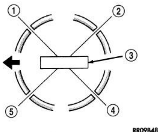
Fig. 246: Piston Ring End Gap Position Courtesy of CHRYSLER GROUP, LLC
