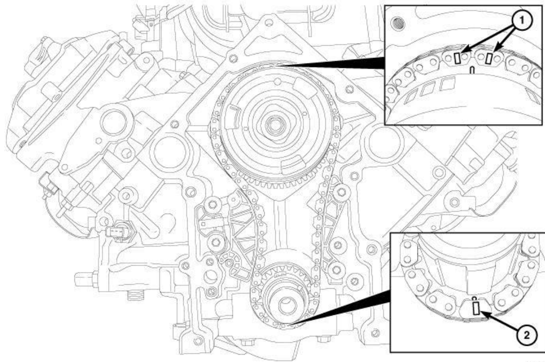
Fig. 421: Aligning Timing Marks With Timing Chain Sprockets Courtesy of CHRYSLER GROUP, LLC
