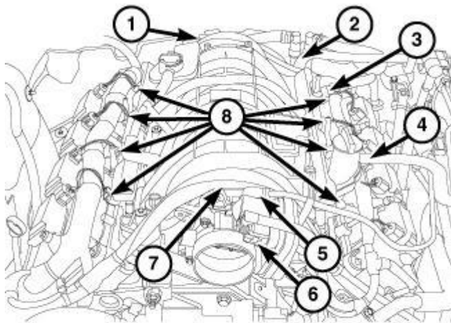
Fig. 291: Map Sensor, Brake Booster Vacuum Hose, Fuel Supply Line, Make Up Air Hose, EVAP Vacuum Purge Hose, Electrical Connector & Electrical Harness Courtesy of CHRYSLER GROUP, LLC
