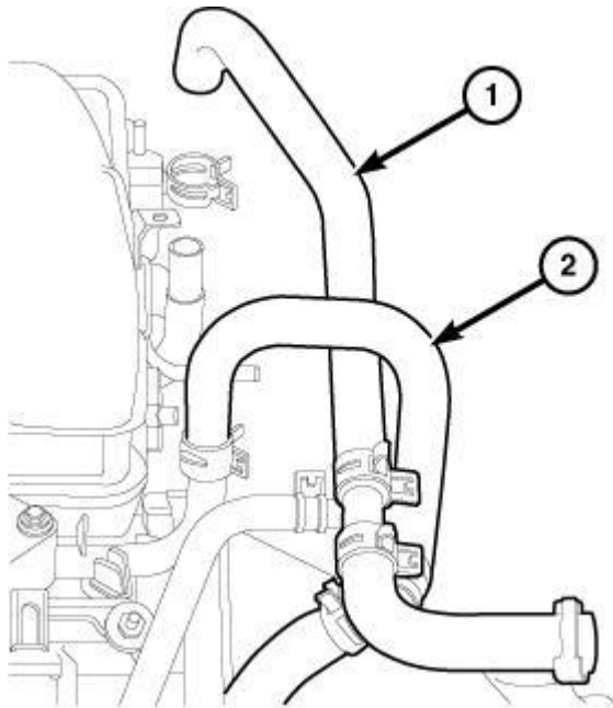
Fig. 39: Heater Hose Supply Courtesy of CHRYSLER GROUP, LLC
