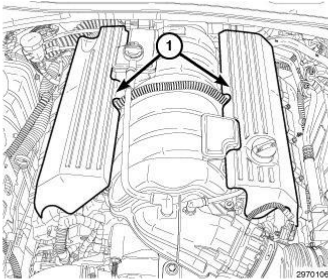
Fig. 429: Engine Covers
