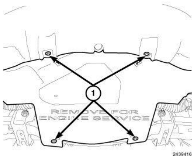
Fig. 356: Lower Splash Shield & Fasteners Courtesy of CHRYSLER GROUP, LLC
