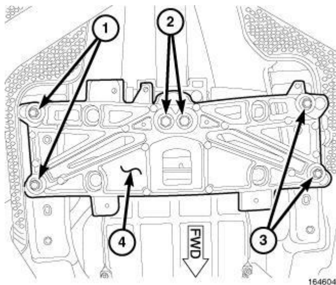
Fig. 287: Rear Cross Member & Bolts Courtesy of CHRYSLER GROUP, LLC
