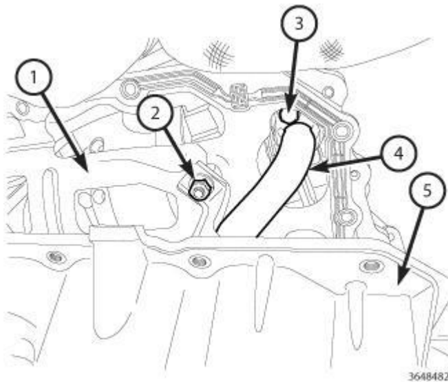
Fig. 346: Oil Pan Gasket/Windage Tray, Oil Pump Pickup Tube, Oil Pan & Fasteners Courtesy of CHRYSLER GROUP, LLC
