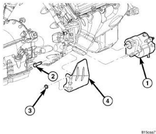
Fig. 51: Removing/Installing Starter Courtesy of CHRYSLER GROUP, LLC
