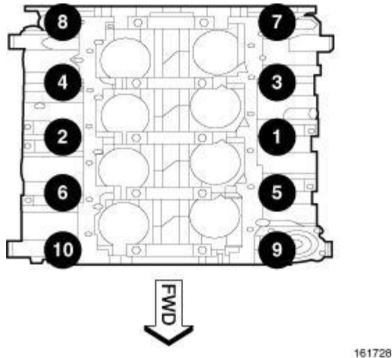
Fig. 201: Crossbolt Tightening Sequence Courtesy of CHRYSLER GROUP, LLC
