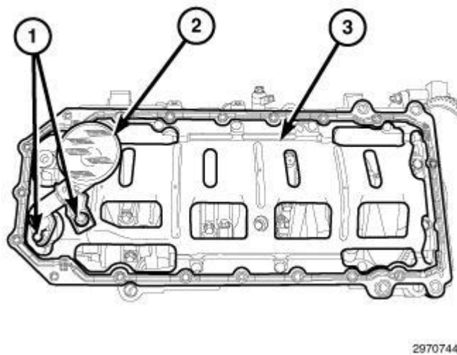
Fig. 258: Integral Windage Tray, Oil Pump Pickup Tube & Bolts
