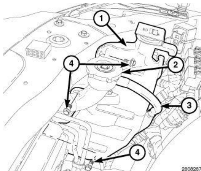
Fig. 66: Coolant Recovery Bottle, Radiator Neck, Overflow Tube & Fasteners
