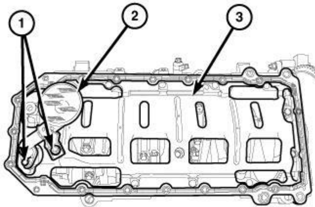
Fig. 160: Integral Windage Tray, Oil Pump Pickup Tube & Bolts Courtesy of CHRYSLER GROUP, LLC
