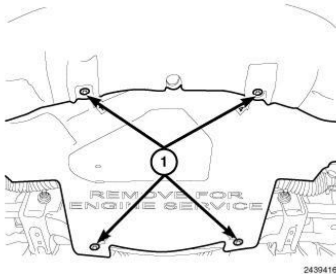
Fig. 307: Lower Splash Shield & Fasteners Courtesy of CHRYSLER GROUP, LLC
