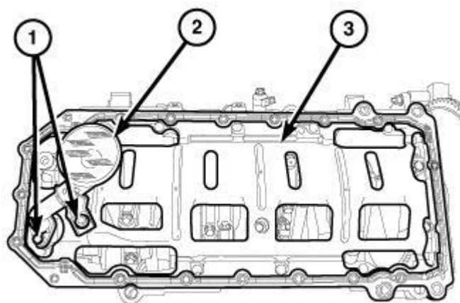
Fig. 208: Integral Windage Tray, Oil Pump Pickup Tube & Bolts Courtesy of CHRYSLER GROUP, LLC
