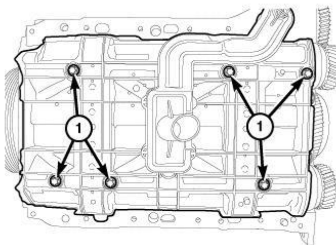
Fig. 329: Oil Pump Pickup Bolts Courtesy of CHRYSLER GROUP, LLC
