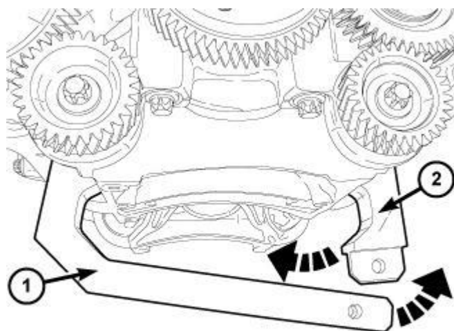
Fig. 330: Installing Balance Shaft Lock Tool Halves & Rotating Into Locked Position Courtesy of CHRYSLER GROUP, LLC
