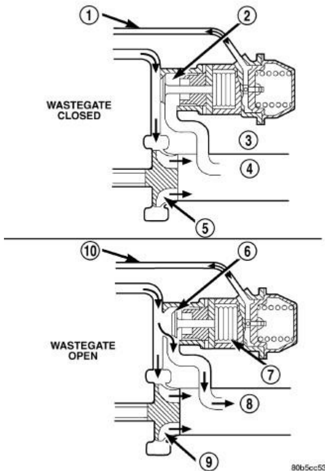
Fig. 568: Wastegate Operation
