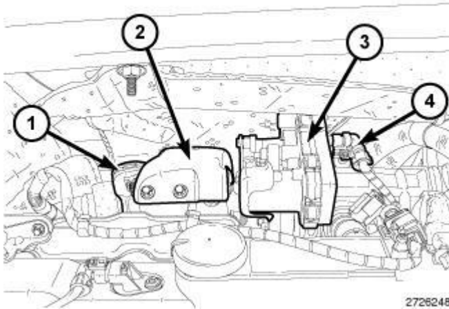
Fig. 571: Catalytic Converter, Turbocharger Heat Shield, Catalytic Converter Band Clamp & Upstream Temperature Sensor Courtesy of CHRYSLER GROUP, LLC
