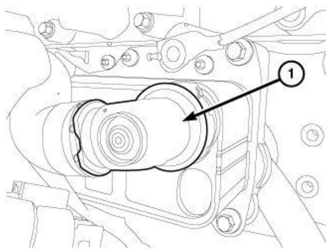
Fig. 494: Coolant Hose To Oil Cooler Courtesy of CHRYSLER GROUP, LLC
