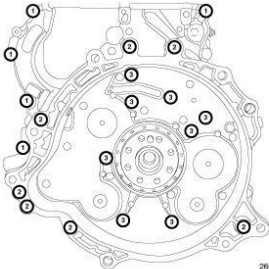
Fig. 634: Timing Chain Cover At Engine Bolts
