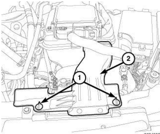
Fig. 489: Quarter Turn Lock Tabs & Air Inlet Duct Courtesy of CHRYSLER GROUP, LLC
