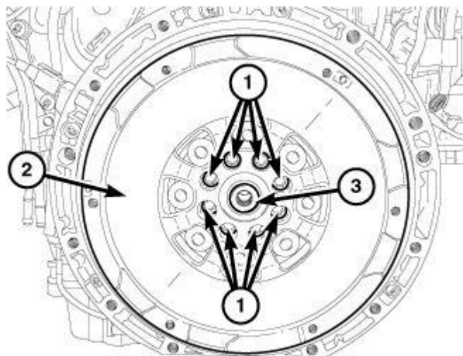
Fig. 250: Flywheel & Bolts
