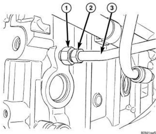
Fig. 555: Coolant Supply Line & Fittings
