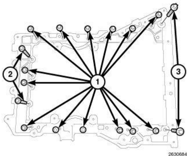
Fig. 224: Oil Pan Bolts
