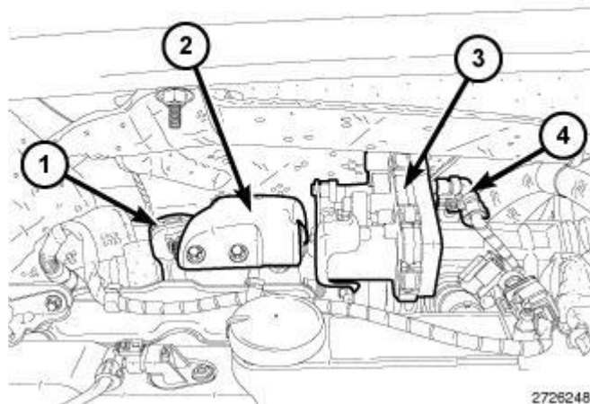
Fig. 583: Catalytic Converter, Turbocharger Heat Shield, Catalytic Converter Band Clamp & Upstream Temperature Sensor Courtesy of CHRYSLER GROUP, LLC
