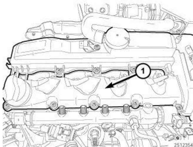
Fig. 168: Cylinder Head Cover Courtesy of CHRYSLER GROUP, LLC
