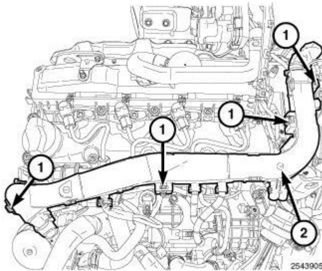
Fig. 176: Lock Tabs & Engine Wire Harness Courtesy of CHRYSLER GROUP, LLC
