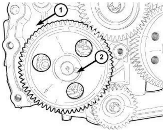
Fig. 334: Oil Pump And Drive Gear Assembly At Engine Block Courtesy of CHRYSLER LLC
