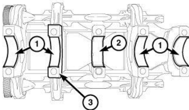
Fig. 207: Installing Bearing Halves Into Bearing Caps
