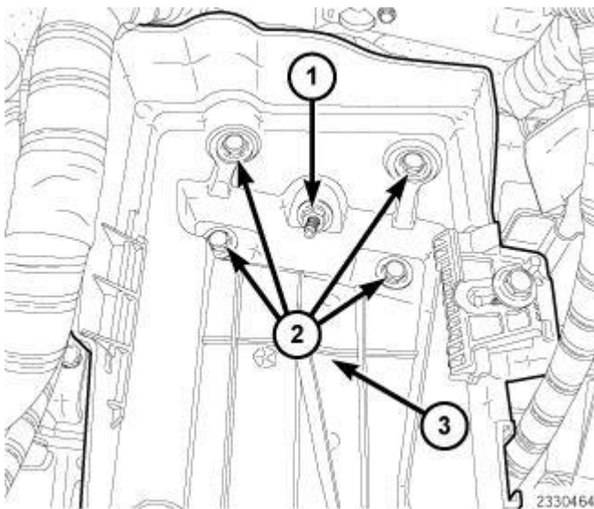
Fig. 264: Battery Tray, Nut & Retaining Bolts
