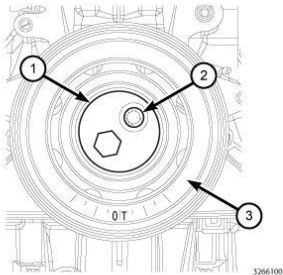
Fig. 209: Vibration Damper Holder Tool, Vibration Damper & Bolts Courtesy of CHRYSLER LLC
