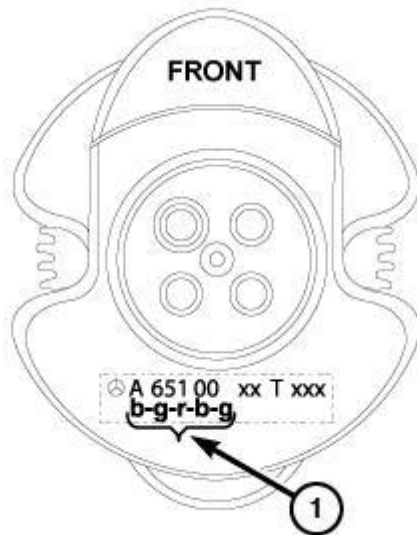
Fig. 206: Letters Stamped On Crankshaft Courtesy of CHRYSLER LLC
