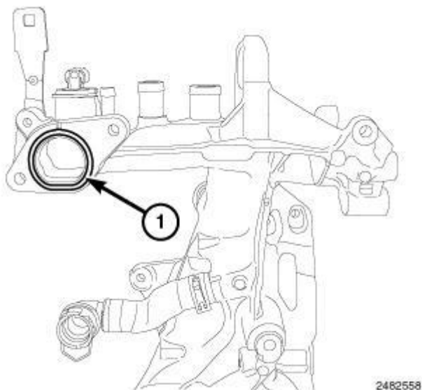
Fig. 307: Accessory Carrier & O-Ring Gasket Courtesy of CHRYSLER LLC
