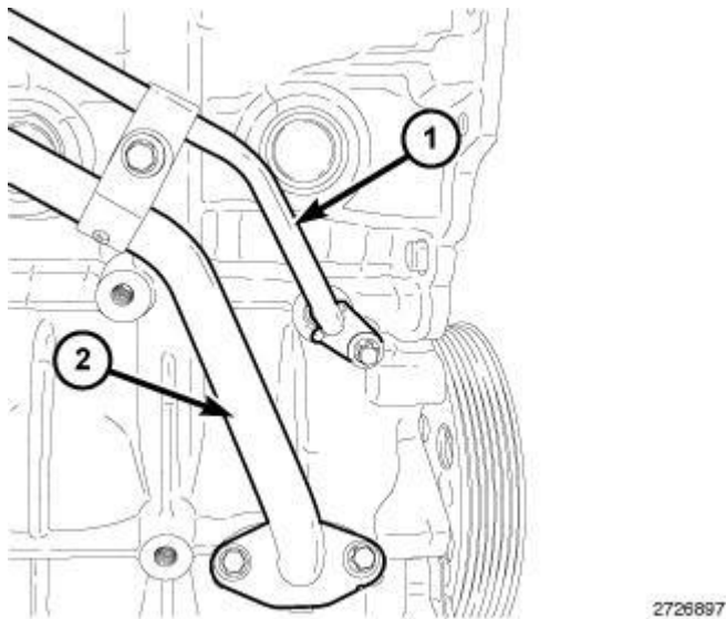
Fig. 574: Oil Supply & Return Lines Courtesy of CHRYSLER LLC
