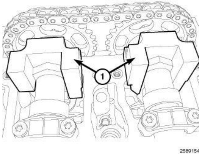
Fig. 148: Camshaft Lock Tools Courtesy of CHRYSLER LLC
