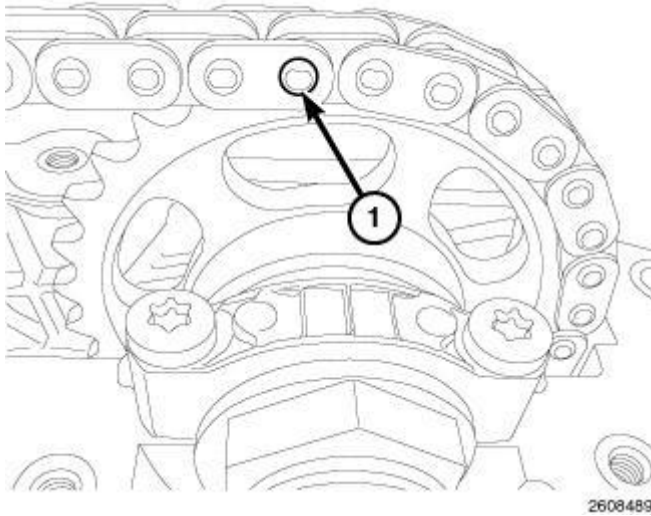
Fig. 580: Timing Chain Pin At Chain Link Courtesy of CHRYSLER LLC
