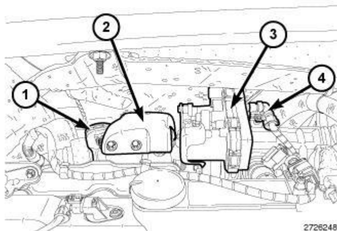
Fig. 578: Catalytic Converter, Turbocharger Heat Shield, Catalytic Converter Band Clamp & Upstream Temperature Sensor Courtesy of CHRYSLER LLC
