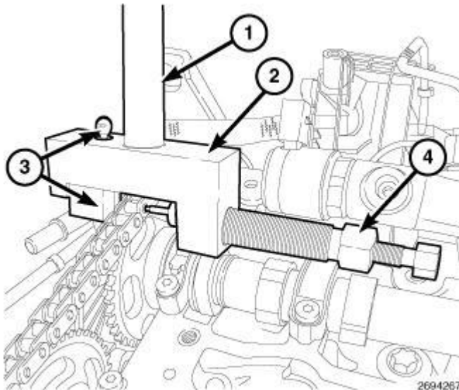
Fig. 581: Chain Link Tool, Handle, Insert & Thrust Screw/Pin Courtesy of CHRYSLER LLC
