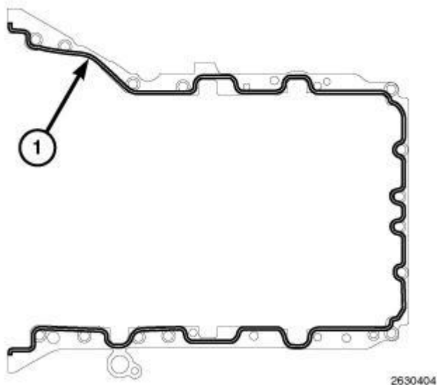
Fig. 322: Applying Engine Sealant RTV Onto Oil Pan Mating Surface Courtesy of CHRYSLER LLC
