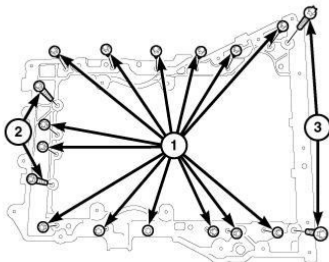
Fig. 325: Locating Oil Pan Bolts Courtesy of CHRYSLER LLC
