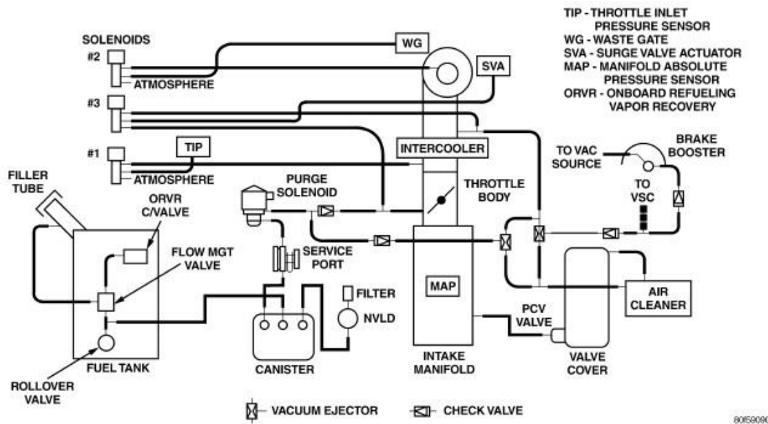
Fig. 555: Vacuum Harness Schematic Courtesy of CHRYSLER LLC
