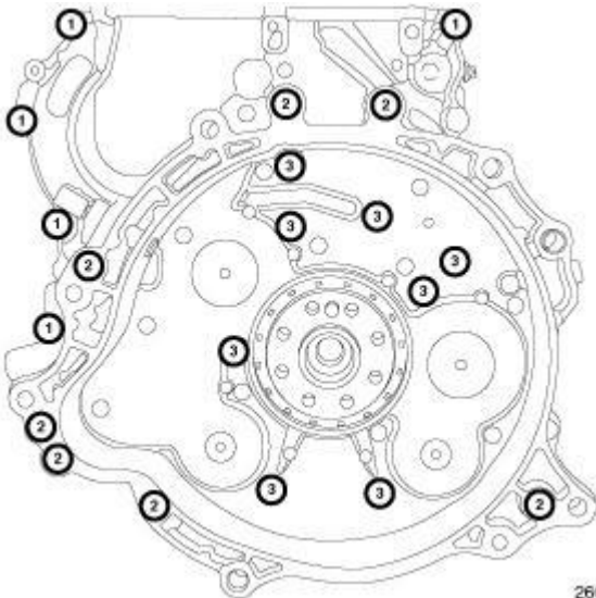
Fig. 629: Timing Chain Cover At Engine Bolts Courtesy of CHRYSLER LLC
