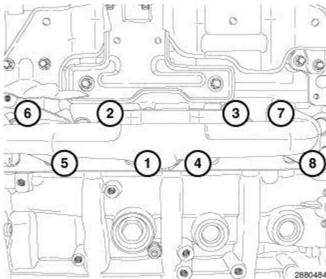
Fig. 414: Exhaust Manifold Bolt Tightening Sequence
