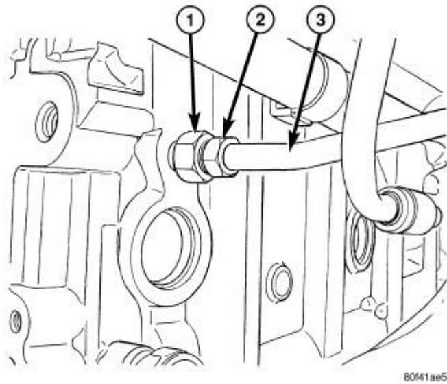
Fig. 550: Coolant Supply Line & Fittings Courtesy of CHRYSLER LLC
