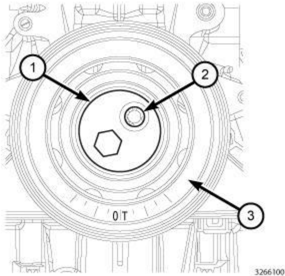
Fig. 135: Vibration Damper Holder Tool, Vibration Damper & Bolts Courtesy of CHRYSLER LLC
