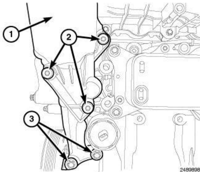
Fig. 306: Oil Filter Housing & Bolts
