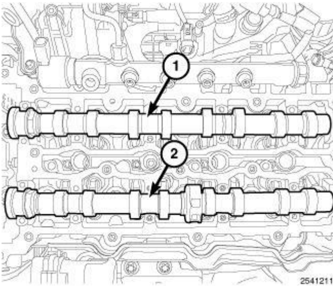
Fig. 146: Camshafts Courtesy of CHRYSLER LLC
