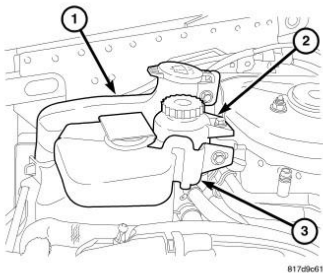
Fig. 54: Coolant Reservoir Courtesy of CHRYSLER LLC
