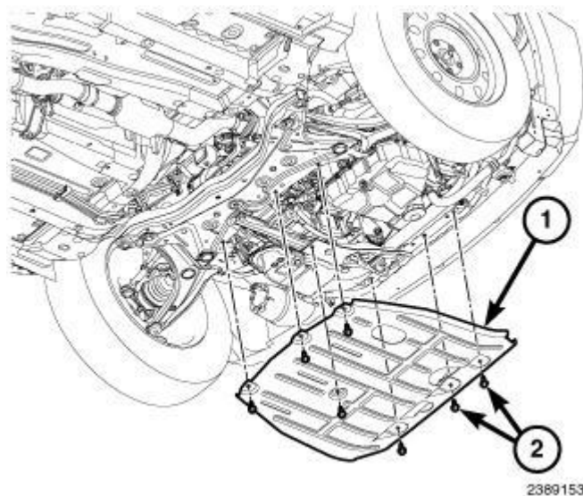
Fig. 333: Removal/Installation Front Skid Plate And Bolts Courtesy of CHRYSLER LLC
