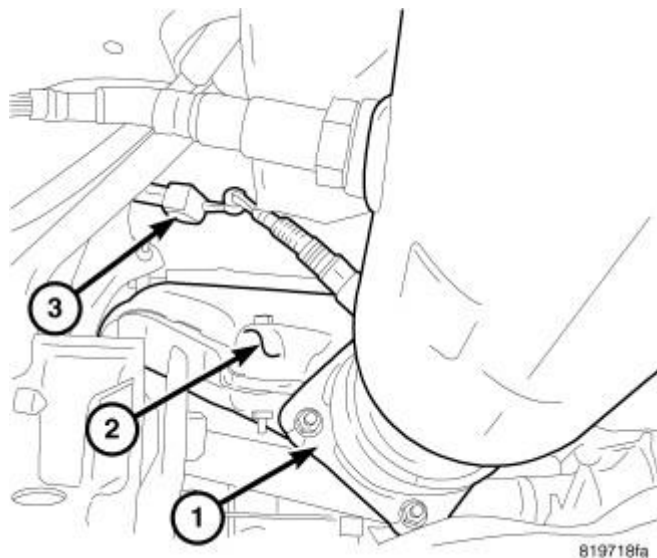
Fig. 350: Exhaust Pipe To Manifold Bolts & Oxygen Sensor Courtesy of CHRYSLER LLC
