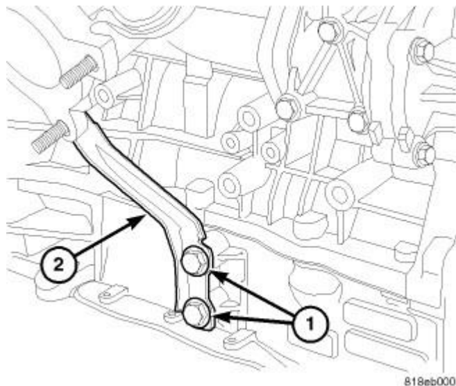
Fig. 351: Exhaust Manifold Support Bracket Courtesy of CHRYSLER LLC
