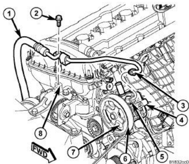
Fig. 78: Power Steering Assembly Components Courtesy of CHRYSLER LLC
