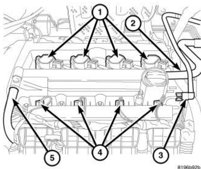
Fig. 51: Coil Connector Courtesy of CHRYSLER LLC
