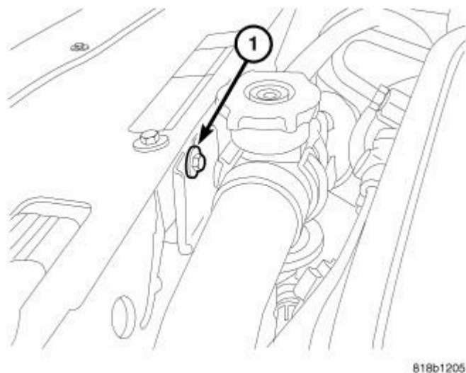
Fig. 387: Radiator Hose Support Courtesy of CHRYSLER LLC
