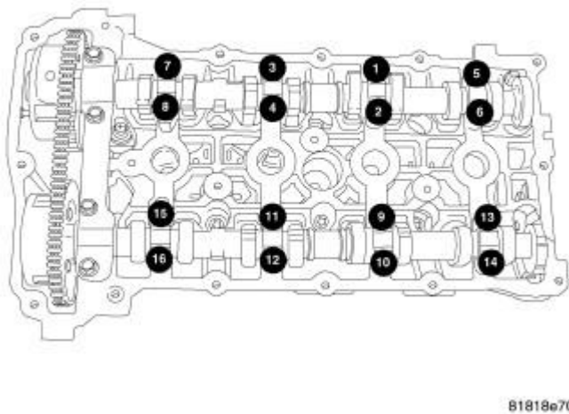
Fig. 118: Removing/Installing Intake & Exhaust Camshaft Bearing Caps - Torque Sequence
