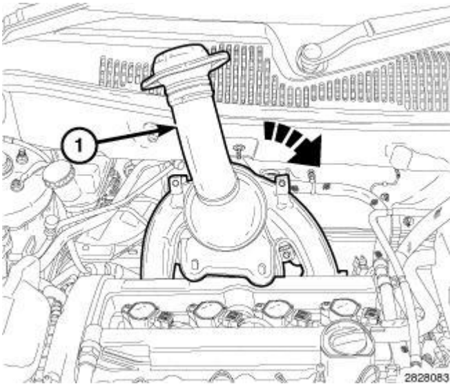
Fig. 353: Rotating Maniverter Clockwise Courtesy of CHRYSLER LLC
