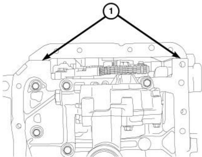
Fig. 305: Sealer Location Courtesy of CHRYSLER LLC
