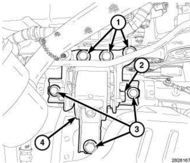
Fig. 354: Engine Mount Isolator, Right Engine Mount & Engine Mount Bracket Retaining Bolts Courtesy of CHRYSLER LLC
