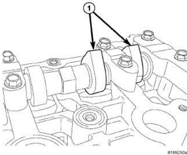
Fig. 135: Identifying Camshaft So Lobes Are Vertical Courtesy of CHRYSLER LLC
