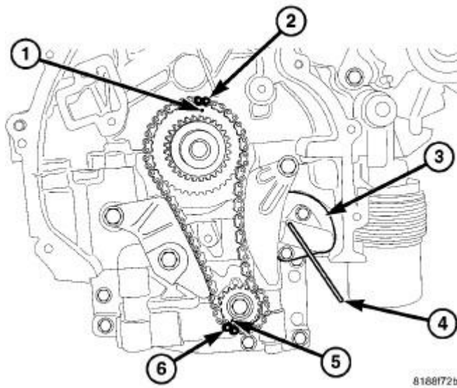
Fig. 406: Oil Pump Drive Chain, Oil Pump Drive Chain Tensioner & Timing Marks On Chain Courtesy of CHRYSLER LLC
