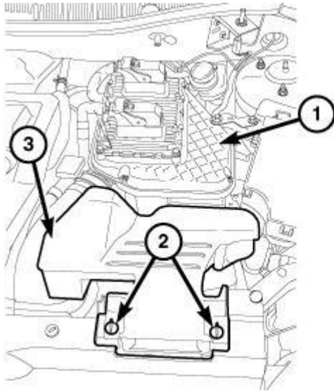
Fig. 72: Retainers, Fresh Air Inlet Duct & Air Cleaner Body Courtesy of CHRYSLER LLC
