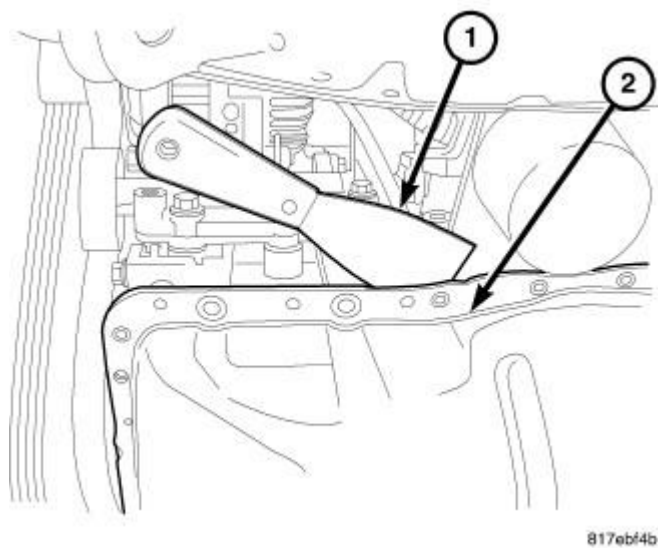
Fig. 217: Oil Pan Removal Courtesy of CHRYSLER LLC
