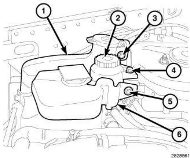
Fig. 356: Coolant Reservoir, Power Steering Fluid Reservoir, Washer Fluid Reservoir & Bolts Courtesy of CHRYSLER LLC
