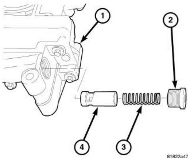
Fig. 327: Oil Pressure Relief Valve Courtesy of CHRYSLER LLC
