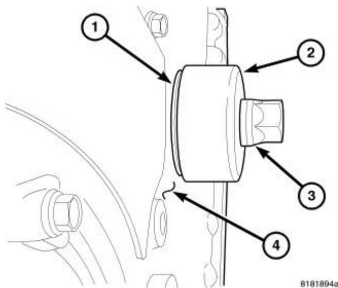
Fig. 262: Installing Front Seal Courtesy of CHRYSLER LLC
