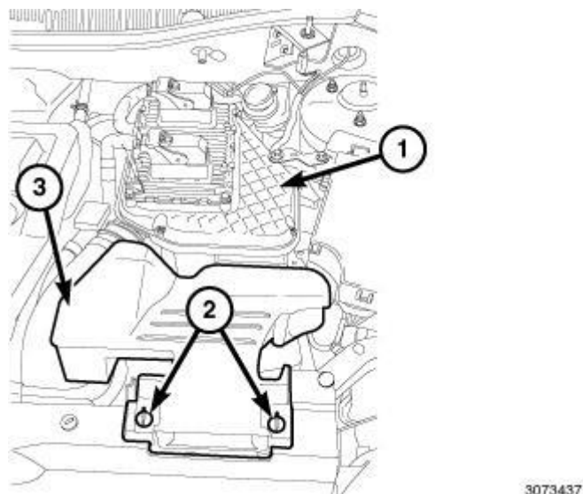
Fig. 331: Retainers, Fresh Air Inlet Duct & Air Cleaner Body Courtesy of CHRYSLER LLC
