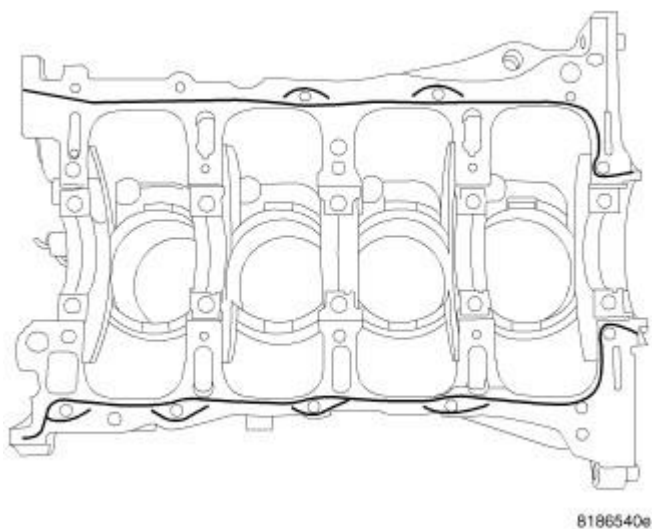
Fig. 240: Sealing Ladder Frame Courtesy of CHRYSLER LLC
