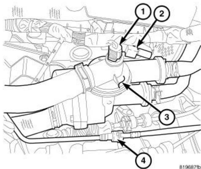
Fig. 126: Coolant Adapter Courtesy of CHRYSLER LLC
