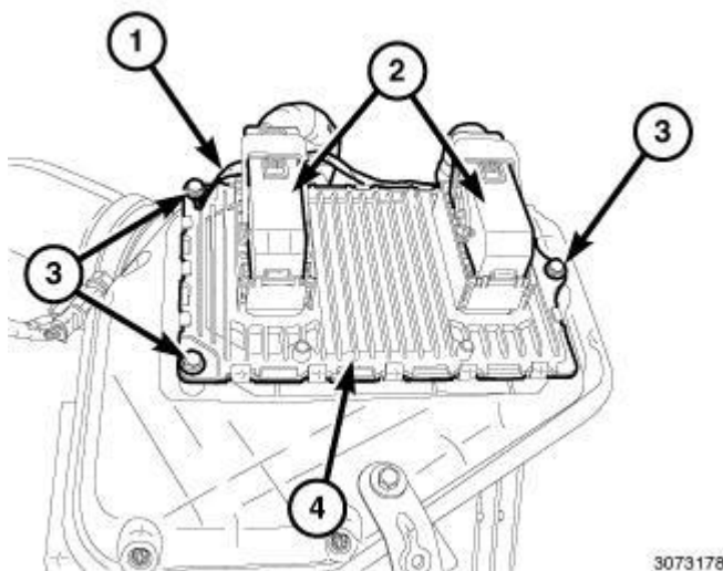
Fig. 71: Electrical Connectors, PCM, Three Mounting Bolts & Ground Wire Courtesy of CHRYSLER LLC
