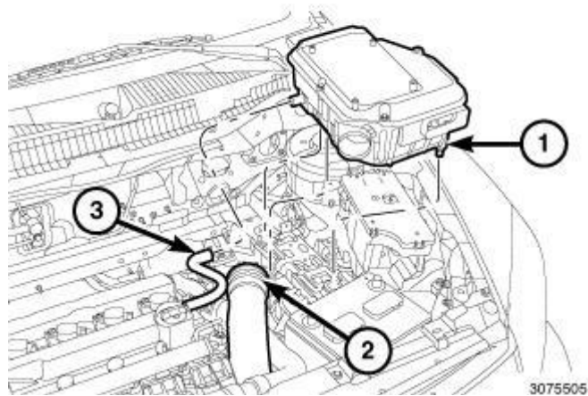
Fig. 69: Air Cleaner Body, Air Inlet Tube & Make-Up Air Hose Courtesy of CHRYSLER LLC
