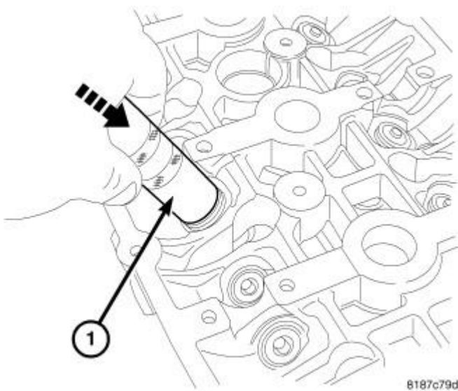
Fig. 179: Valve Removal Courtesy of CHRYSLER LLC
