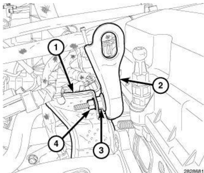
Fig. 342: Heatshield, Stud Bolt, Engine Lift Bracket & Nut Courtesy of CHRYSLER LLC
