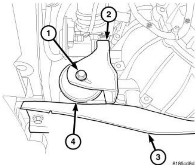
Fig. 186: Front Mount Through Bolt Courtesy of CHRYSLER LLC
