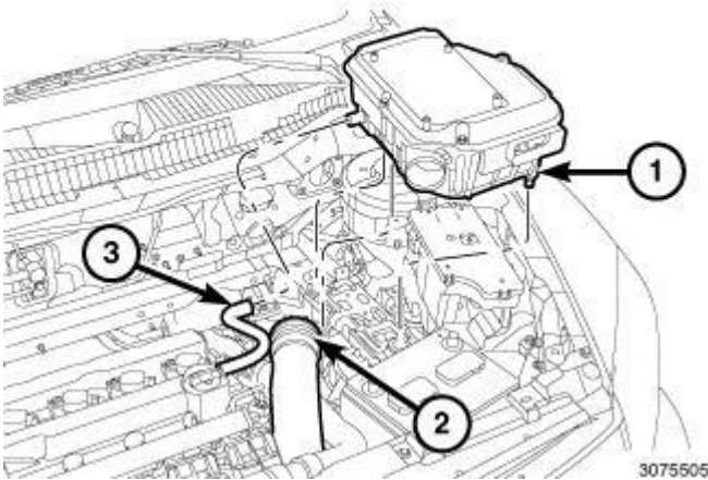
Fig. 70: Air Cleaner Body, Air Inlet Tube & Make-Up Air Hose Courtesy of CHRYSLER LLC
