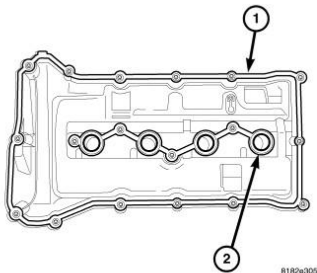
Fig. 172: Cylinder Head Cover Gaskets Location Courtesy of CHRYSLER LLC
