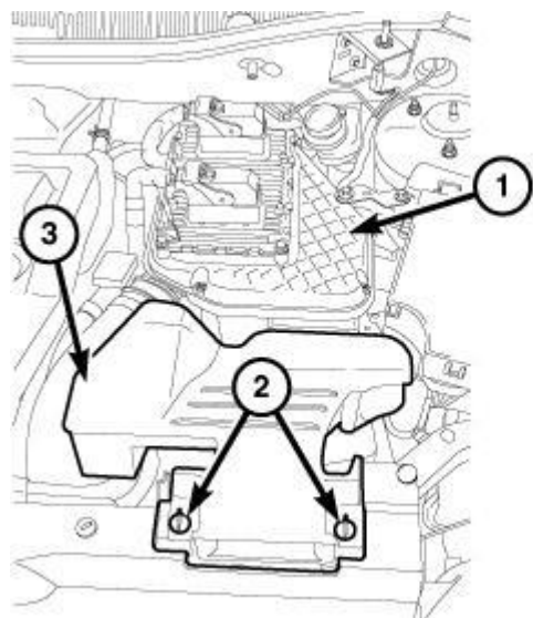
Fig. 66: Retainers, Fresh Air Inlet Duct & Air Cleaner Body Courtesy of CHRYSLER LLC
