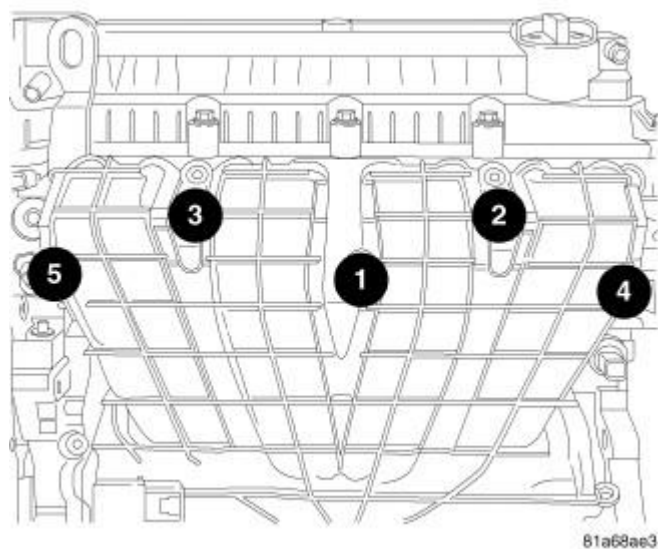
Fig. 385: Intake Manifold Bolt Removal & Tightening Sequence Courtesy of CHRYSLER LLC
