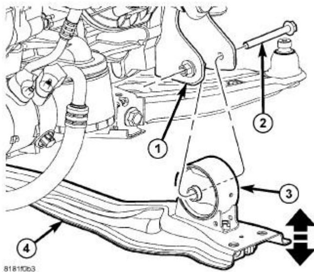
Fig. 337: Removing/Installing Fore/Aft Crossmember Courtesy of CHRYSLER LLC
