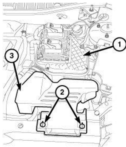
Fig. 370: Retainers, Fresh Air Inlet Duct & Air Cleaner Body Courtesy of CHRYSLER LLC
