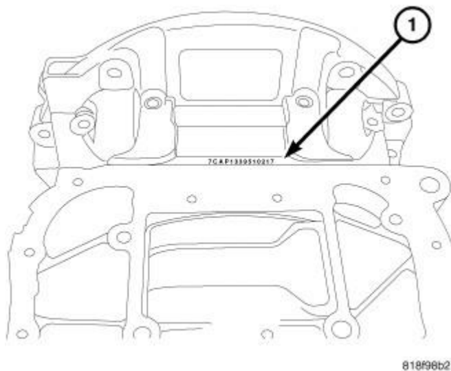
Fig. 60: Locating Engine Serial Number Courtesy of CHRYSLER LLC
