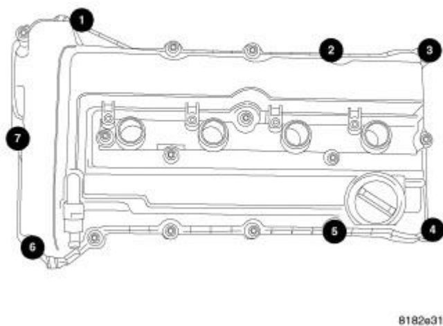
Fig. 173: Cylinder Head Stud Installation Sequence Courtesy of CHRYSLER LLC
