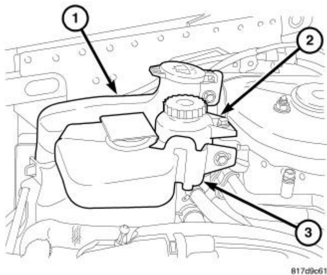
Fig. 202: Coolant Reservoir Courtesy of CHRYSLER LLC
