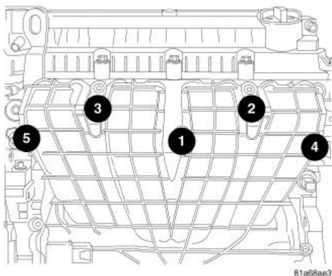
Fig. 386: Intake Manifold Bolt Removal & Tightening Sequence Courtesy of CHRYSLER LLC
