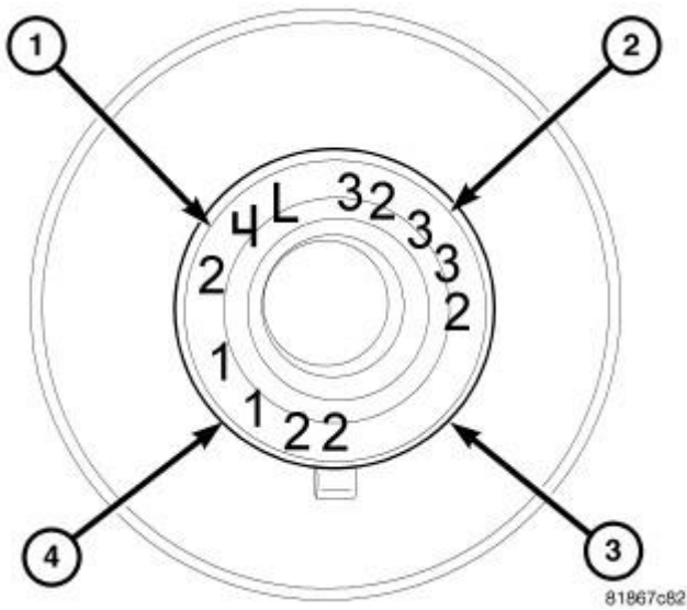
Fig. 206: Connecting Rod Bearing Identification Courtesy of CHRYSLER LLC
