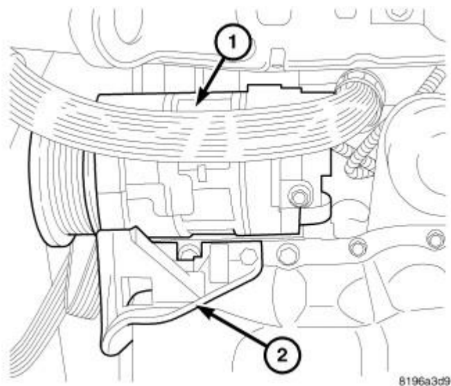
Fig. 30: A/C Compressor Courtesy of CHRYSLER LLC
