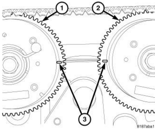
Fig. 117: Camshaft Timing Courtesy of CHRYSLER LLC
