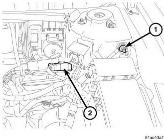
Fig. 375: Battery Cables Courtesy of CHRYSLER LLC
