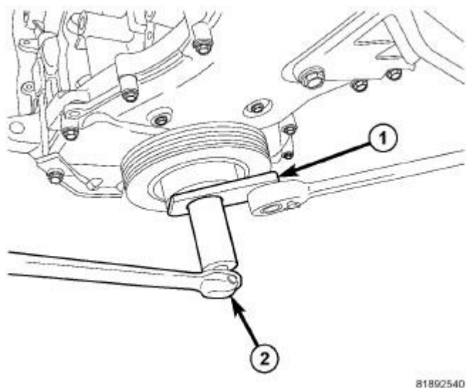
Fig. 259: Damper Removal & Installation Courtesy of CHRYSLER LLC
