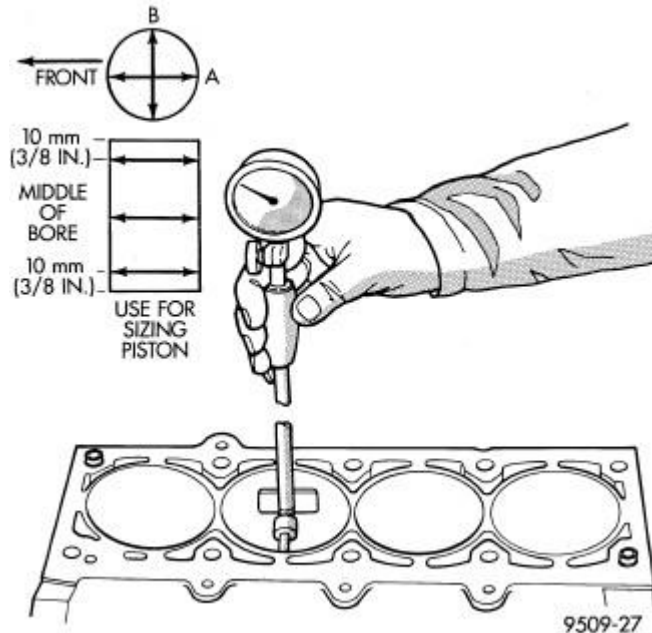
Fig. 205: Checking Cylinder Bore Size Courtesy of CHRYSLER LLC
