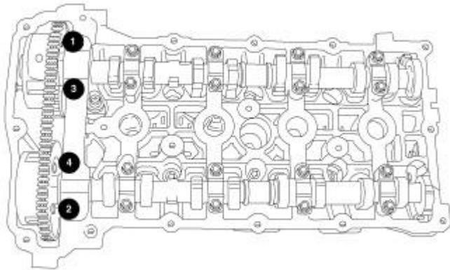
Fig. 151: Removing/Installing Front Camshaft Bearing Caps Courtesy of CHRYSLER LLC
