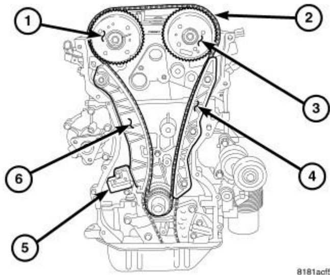
Fig. 400: Timing Drive Courtesy of CHRYSLER LLC
