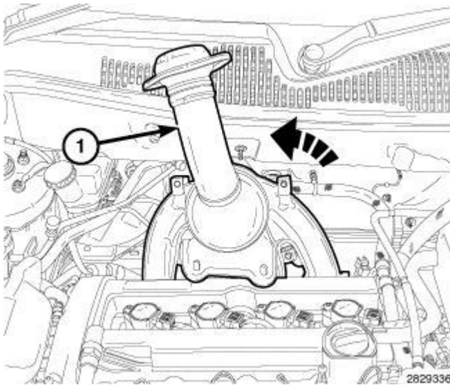
Fig. 347: Rotating Maniverter Counterclockwise Courtesy of CHRYSLER LLC
