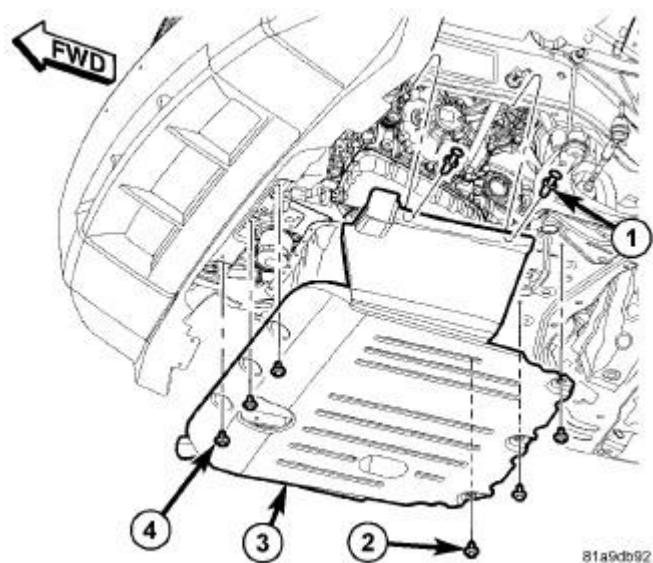
Fig. 366: Belly Pan Courtesy of CHRYSLER LLC
