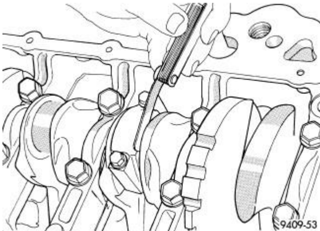
Fig. 208: Connecting Rod Side Clearance Courtesy of CHRYSLER LLC
