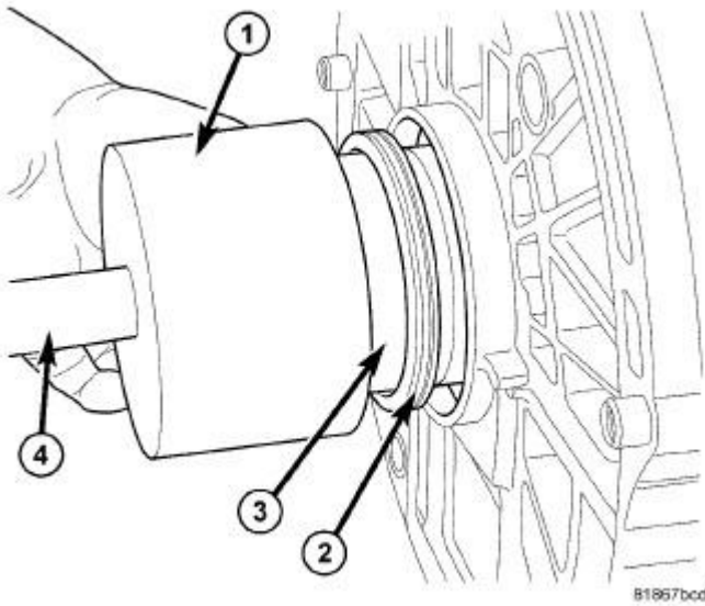
Fig. 267: Driving Seal Into Block Using Seal Driver 9706 And Driver Handle C-4171 Until Seal Driver 9706 Bottoms Out Against Block Courtesy of CHRYSLER LLC
