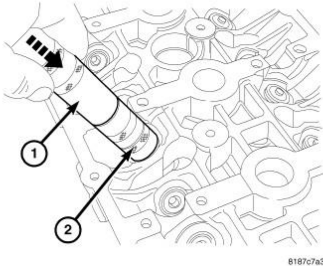
Fig. 183: Valve Installation Courtesy of CHRYSLER LLC
