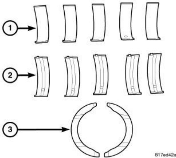
Fig. 223: Bearing Identification Courtesy of CHRYSLER LLC
