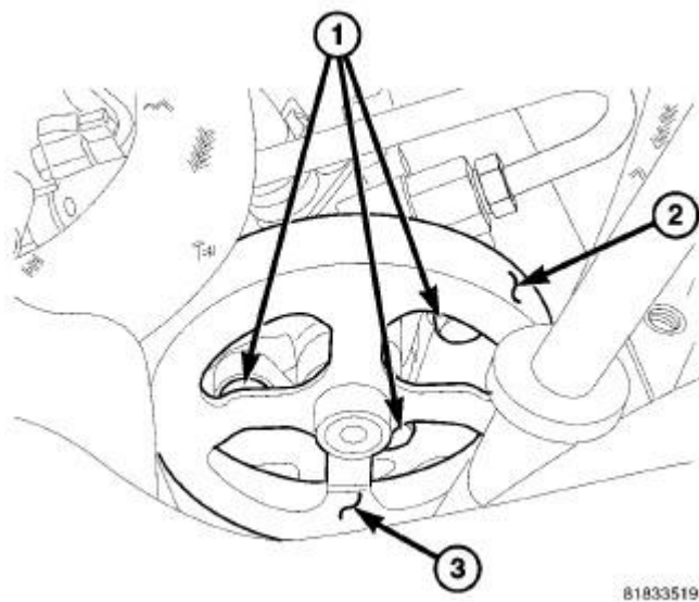
Fig. 79: Power Steering Pump Bolts & Pulley Courtesy of CHRYSLER LLC
