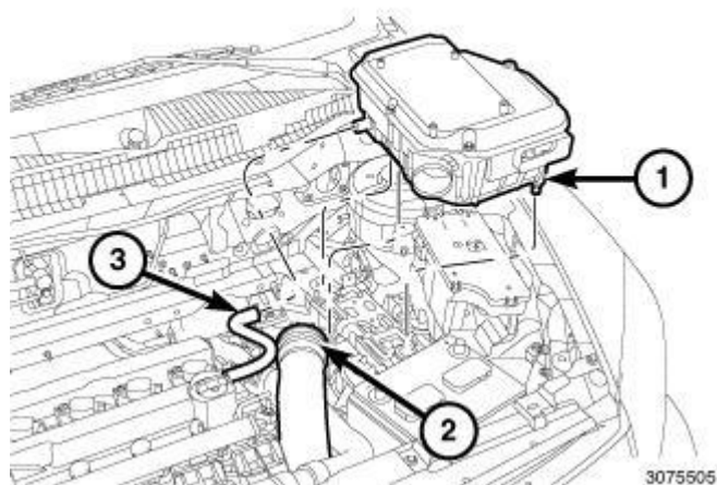
Fig. 76: Air Cleaner Body, Air Inlet Tube & Make-Up Air Hose Courtesy of CHRYSLER LLC
