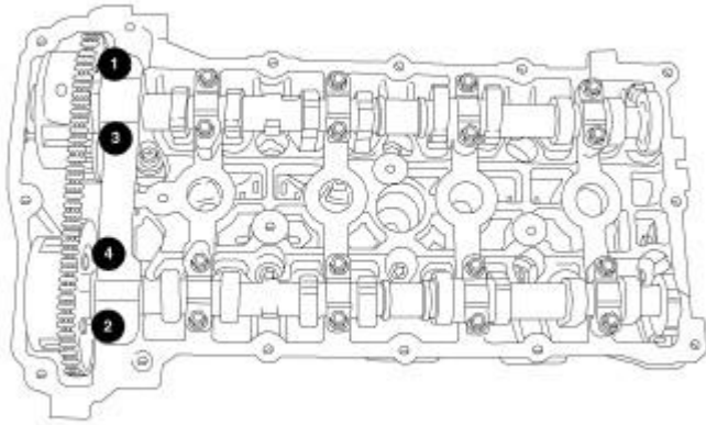
Fig. 161: Removing/Installing Front Intake & Exhaust Bearing Caps - Torque Sequence Courtesy of CHRYSLER LLC
