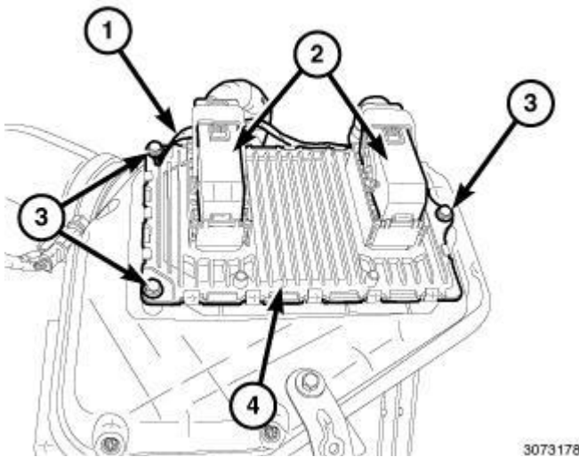
Fig. 193: Electrical Connectors, PCM, Three Mounting Bolts & Ground Wire Courtesy of CHRYSLER LLC
