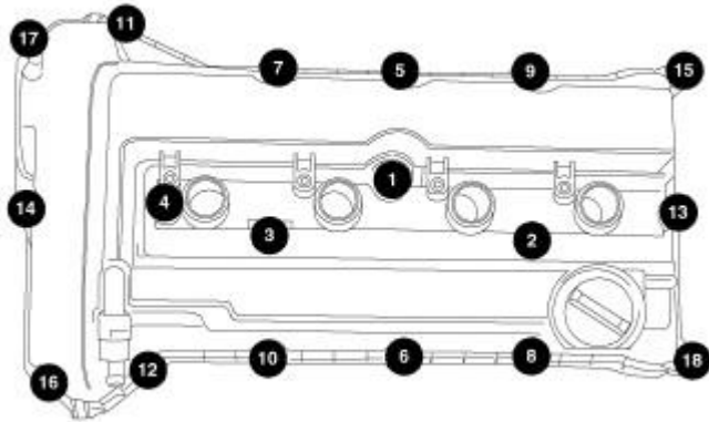
Fig. 121: Cylinder Head Cover Bolt Torque Sequence Courtesy of CHRYSLER LLC
