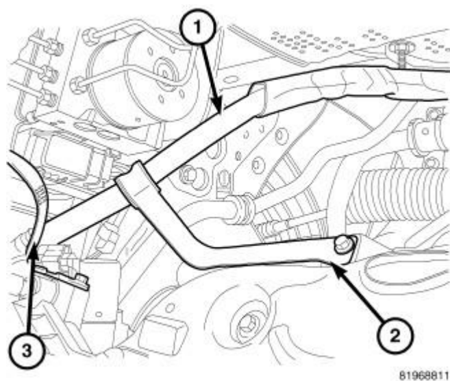
Fig. 48: P/S Hose Support - FWD Courtesy of CHRYSLER LLC
