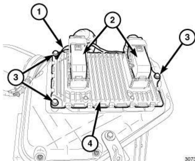
Fig. 12: Electrical Connectors, PCM, Three Mounting Bolts & Ground Wire Courtesy of CHRYSLER LLC
