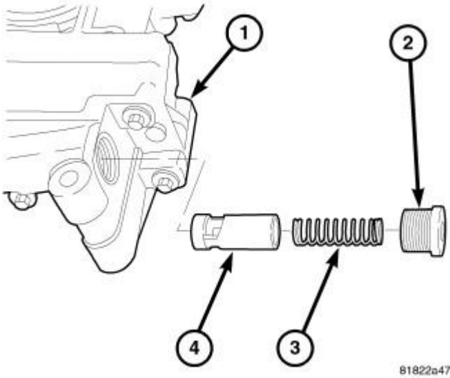
Fig. 329: Oil Pressure Relief Valve Courtesy of CHRYSLER LLC
