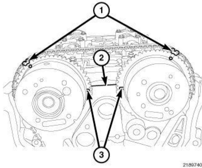
Fig. 399: Timing Chain Timing Marks Courtesy of CHRYSLER LLC
