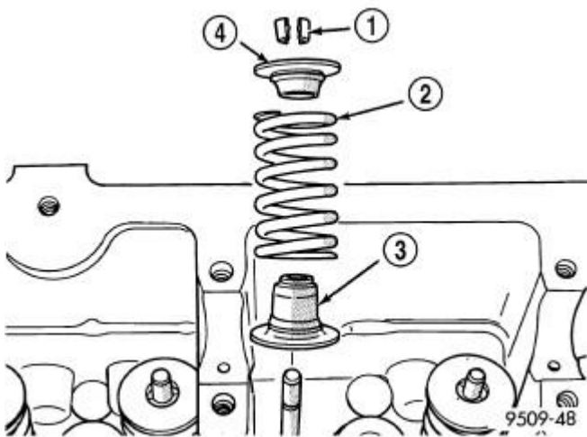
Fig. 180: Valve Spring Assembly Courtesy of CHRYSLER LLC
