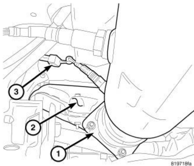
Fig. 26: Exhaust Pipe To Manifold Bolts & Oxygen Sensor Courtesy of CHRYSLER LLC
