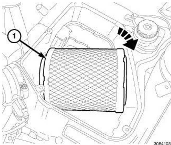
Fig. 64: Air Cleaner Element Courtesy of CHRYSLER LLC
