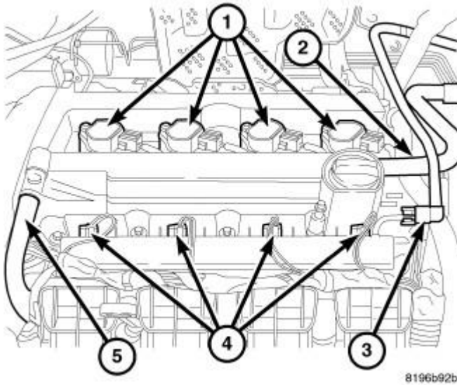
Fig. 390: Coil Connectors Courtesy of CHRYSLER LLC
