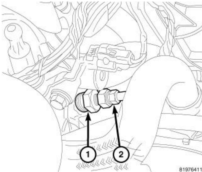
Fig. 276: Oil Pressure Adapter 9879 Courtesy of CHRYSLER LLC
