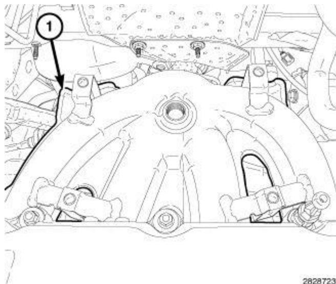
Fig. 359: Lower Maniverter Heatshield Courtesy of CHRYSLER LLC
