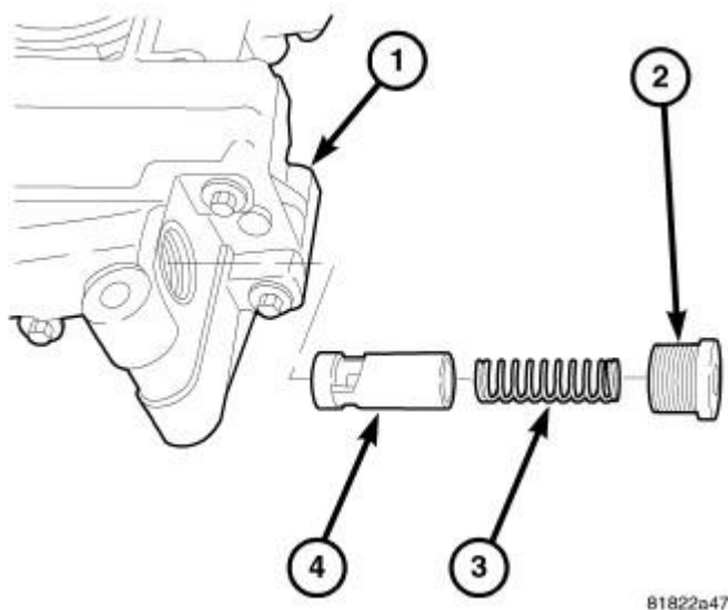
Fig. 328: Oil Pressure Relief Valve Courtesy of CHRYSLER LLC
