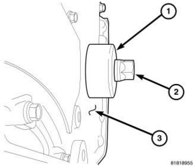
Fig. 263: Front Seal Installed Courtesy of CHRYSLER LLC
