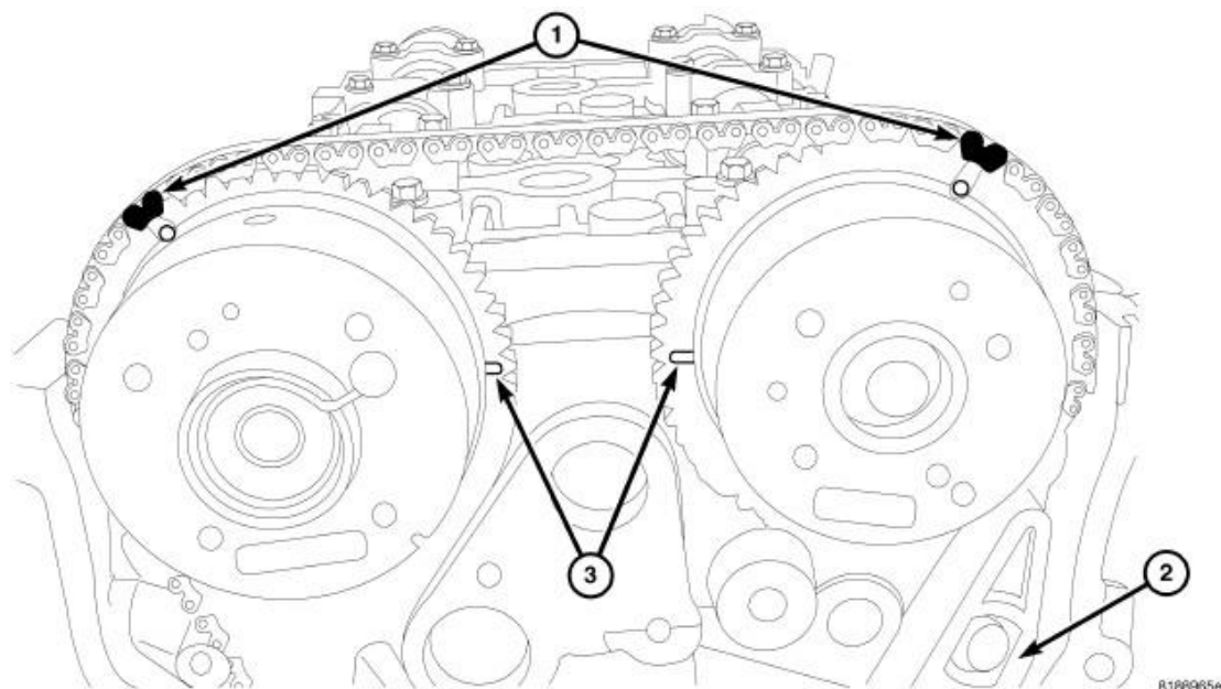
Fig. 162: Timing Chain Timing Marks Courtesy of CHRYSLER LLC
