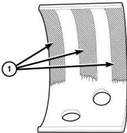
Fig. 142: Identifying Uneven Wear Patterns On Cam Bearing Courtesy of CHRYSLER LLC
