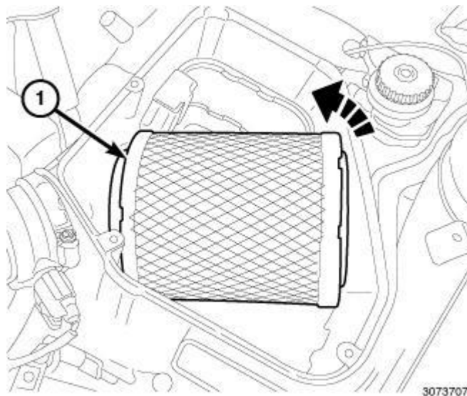
Fig. 63: Air Cleaner Element Courtesy of CHRYSLER LLC
