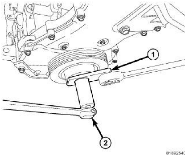
Fig. 264: Damper Removal & Installation Courtesy of CHRYSLER LLC
