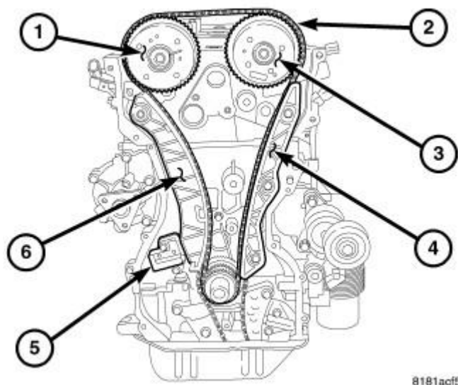
Fig. 91: Removing/Installing Timing Chain, Tensioner, Chain Guide, & Chain Pivot Guide Courtesy of CHRYSLER LLC
