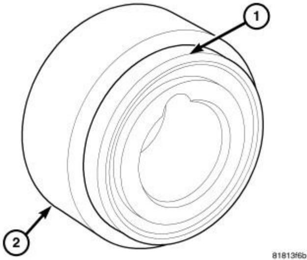
Fig. 261: Crankshaft Oil Seal & Seal Installer 9506 Courtesy of CHRYSLER LLC
