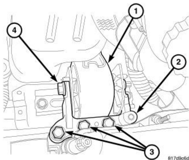
Fig. 423: Right Engine Mount Assembly Courtesy of CHRYSLER LLC
