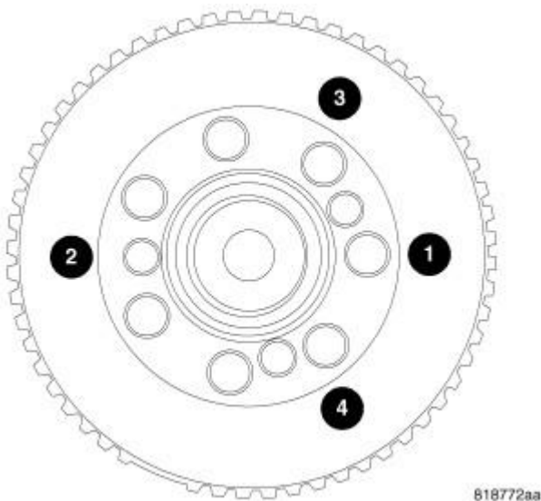
Fig. 224: Target Wheel Courtesy of CHRYSLER LLC
