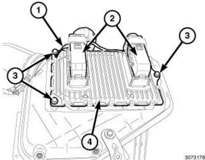
Fig. 188: Electrical Connectors, PCM, Three Mounting Bolts & Ground Wire Courtesy of CHRYSLER LLC
