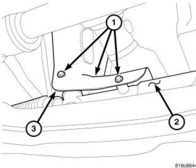
Fig. 364: Removing/Installing Bolts Securing Steering Gear Heat Shield Courtesy of CHRYSLER LLC
