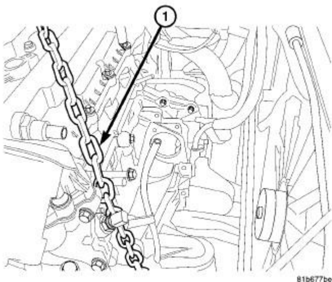
Fig. 35: Identifying Lift Chain Courtesy of CHRYSLER LLC
