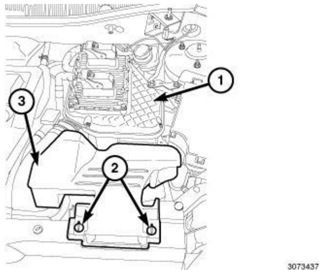
Fig. 130: Retainers, Fresh Air Inlet Duct & Air Cleaner Body Courtesy of CHRYSLER LLC
