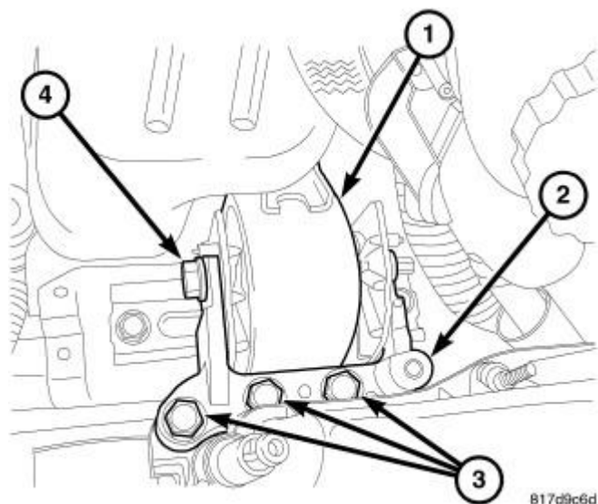
Fig. 33: Right Engine Mount Courtesy of CHRYSLER LLC
