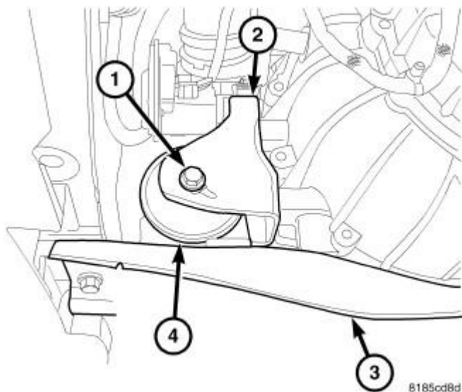
Fig. 185: Front Mount Through Bolt Courtesy of CHRYSLER LLC
