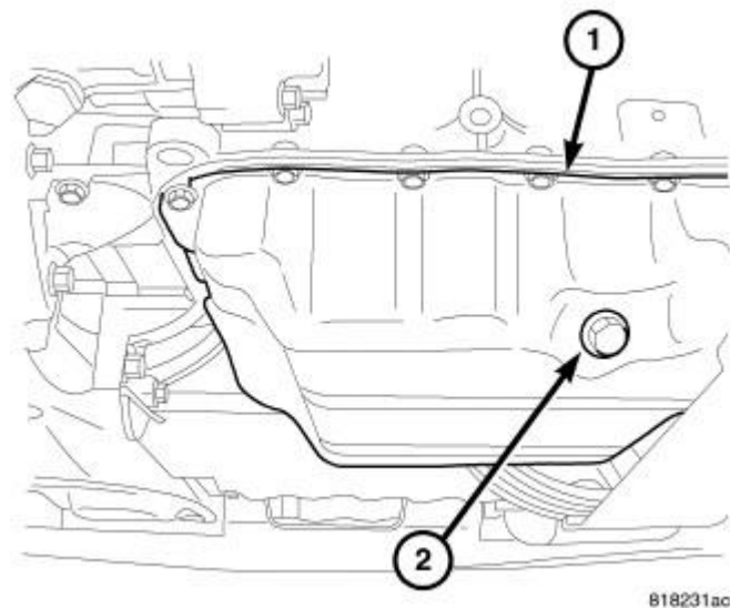
Fig. 300: Oil Drain Plug
