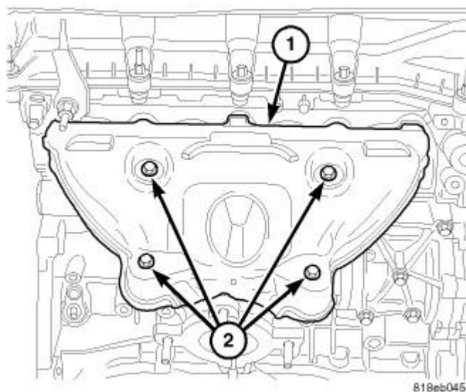
Fig. 372: Exhaust Manifold Heat Shield Courtesy of CHRYSLER LLC
