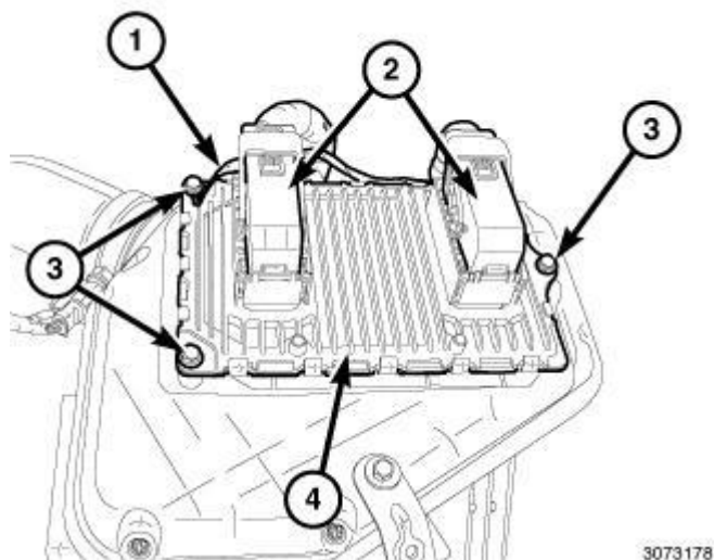
Fig. 392: Electrical Connectors, PCM, Three Mounting Bolts & Ground Wire Courtesy of CHRYSLER LLC
