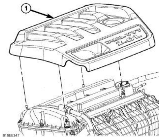
Fig. 177: Engine Cover Courtesy of CHRYSLER LLC
