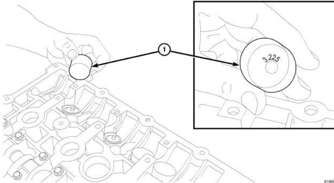
Fig. 139: Tappet Identification Courtesy of CHRYSLER LLC
