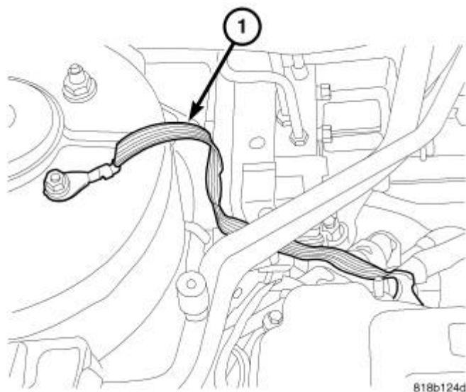
Fig. 40: Ground Strap Courtesy of CHRYSLER LLC
