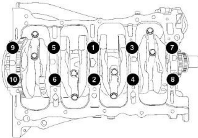
Fig. 228: Main Bearing Cap Torque Sequence Courtesy of CHRYSLER LLC
