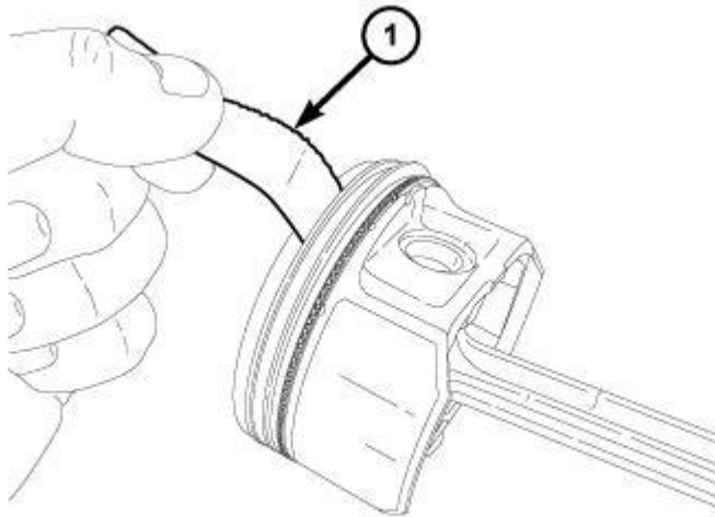
Fig. 243: Piston Ring To Groove Side Clearance Courtesy of CHRYSLER LLC
