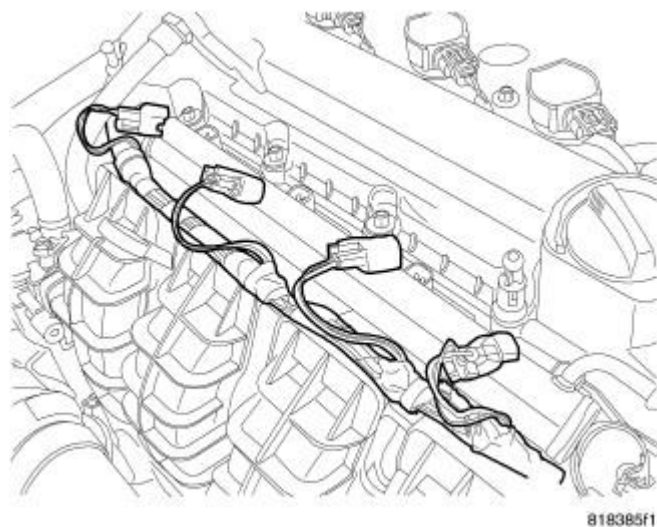
Fig. 93: Identifying Fuel Injector Electrical Connectors Courtesy of CHRYSLER LLC
