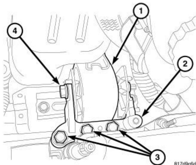
Fig. 36: Right Engine Mount
