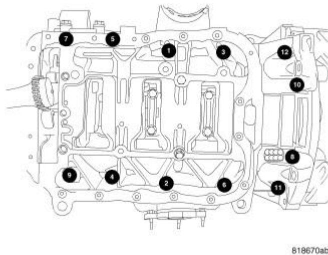
Fig. 241: Ladder Frame Bolts Tightening Sequence Courtesy of CHRYSLER LLC
