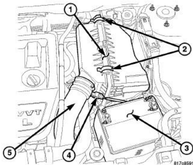
Fig. 444: Air Cleaner Housing, Snap Clasps, Battery, Intake Air Temperature Sensor Connector & Clean Air Hose Courtesy of CHRYSLER LLC
