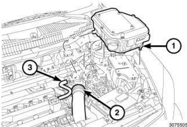
Fig. 391: Air Cleaner Body, Air Inlet Tube & Make-Up Air Hose Courtesy of CHRYSLER LLC
