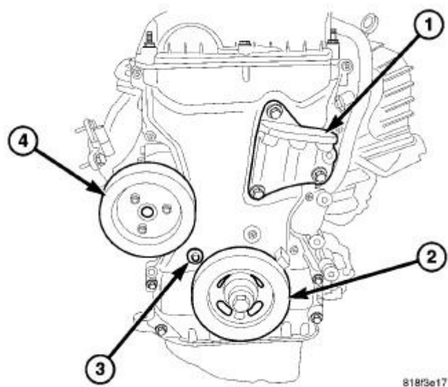
Fig. 84: Right Side Engine Mount Bracket, Crankshaft Damper & Water Pump Pulley Courtesy of CHRYSLER LLC
