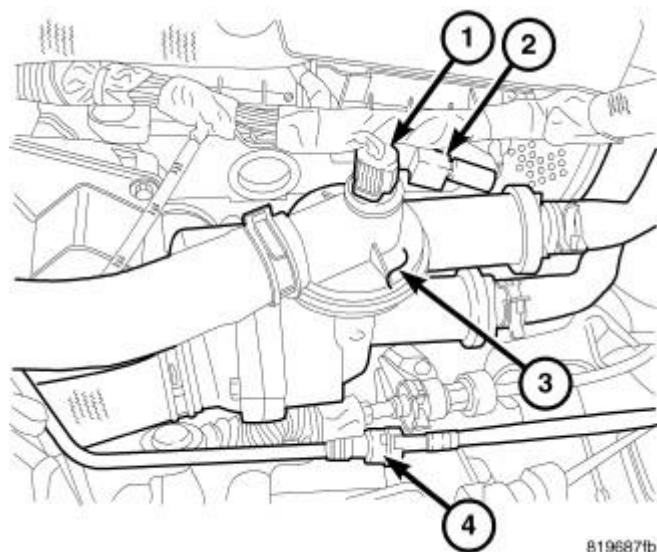
Fig. 53: Coolant Adapter Courtesy of CHRYSLER LLC
