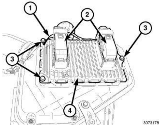
Fig. 129: Electrical Connectors, PCM, Three Mounting Bolts & Ground Wire Courtesy of CHRYSLER LLC
