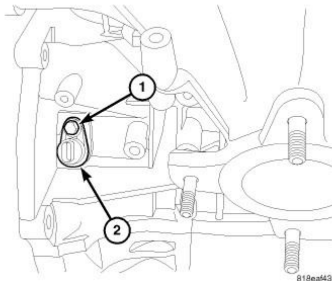
Fig. 39: Crankshaft Position Sensor Courtesy of CHRYSLER LLC
