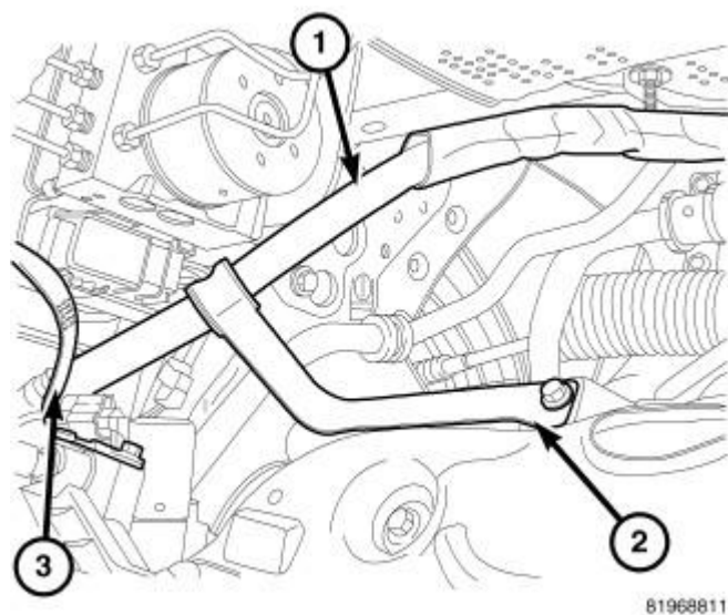
Fig. 22: P/S Hose Support - FWD Courtesy of CHRYSLER LLC
