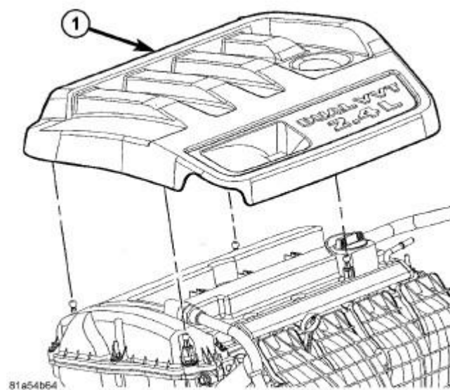
Fig. 369: Engine Cover Courtesy of CHRYSLER LLC
