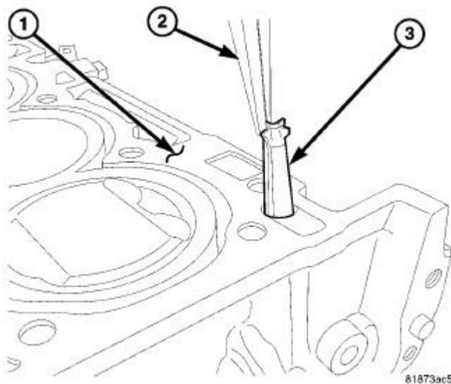
Fig. 106: VVT Filter Courtesy of CHRYSLER LLC
