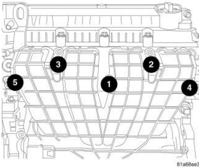
Fig. 20: Intake Manifold Bolt Removal & Tightening Sequence Courtesy of CHRYSLER LLC
