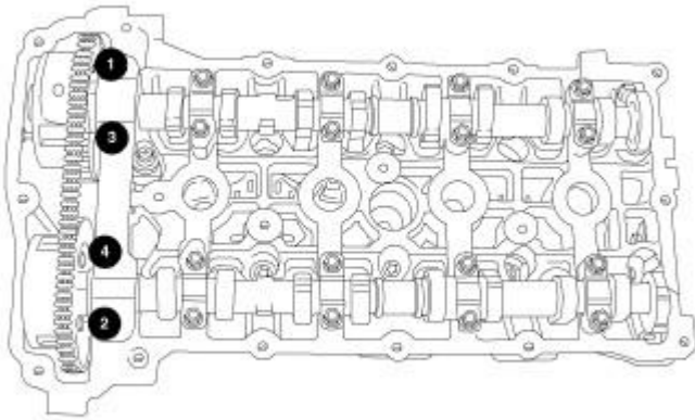
Fig. 119: Removing/Installing Front Intake & Exhaust Bearing Caps - Torque Sequence
