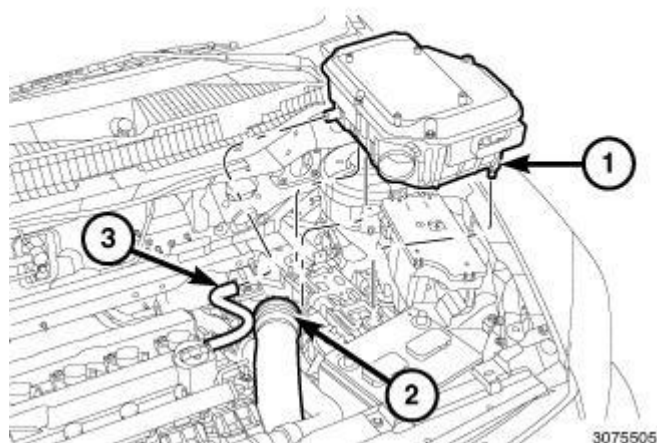
Fig. 380: Air Cleaner Body, Air Inlet Tube & Make-Up Air Hose Courtesy of CHRYSLER LLC
