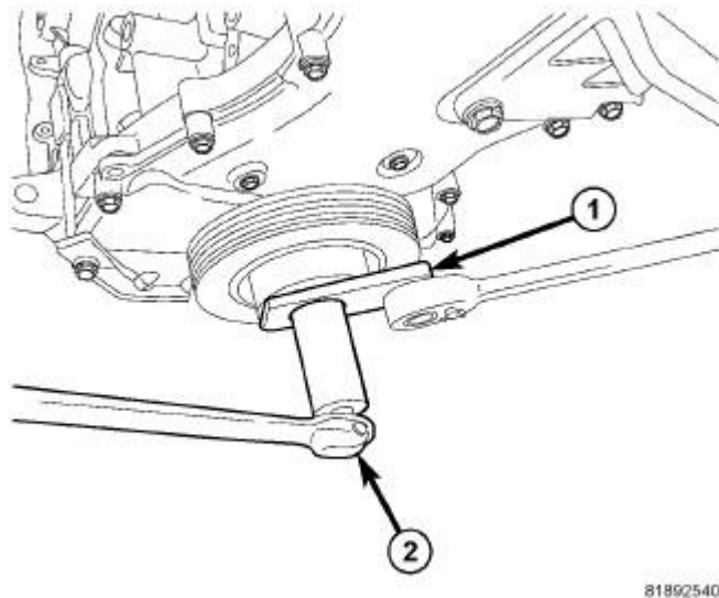
Fig. 24: Damper Removal & Installation Courtesy of CHRYSLER LLC
