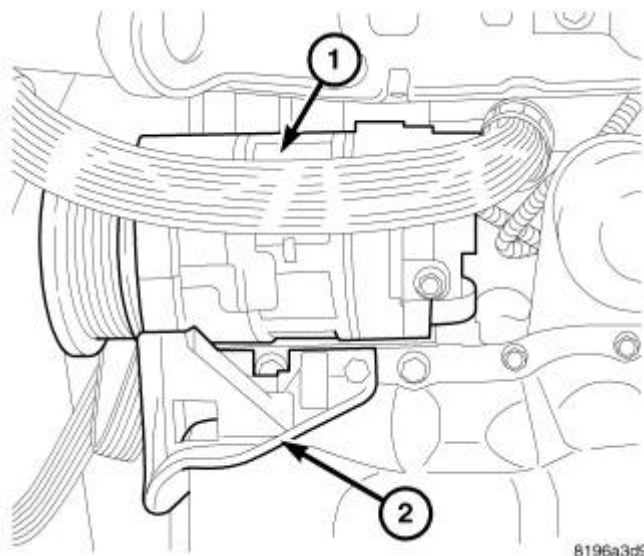
Fig. 439: A/C Compressor & Mounting Bracket Courtesy of CHRYSLER LLC
