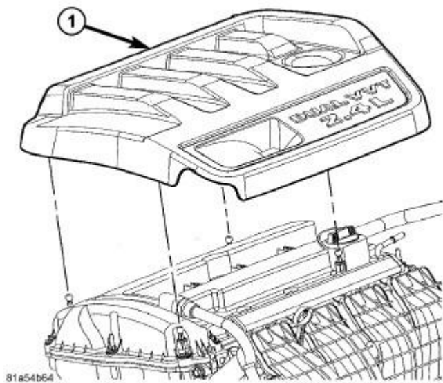
Fig. 8: Engine Cover - 2.4L Courtesy of CHRYSLER LLC
