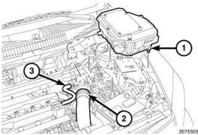
Fig. 192: Air Cleaner Body, Air Inlet Tube & Make-Up Air Hose Courtesy of CHRYSLER LLC
