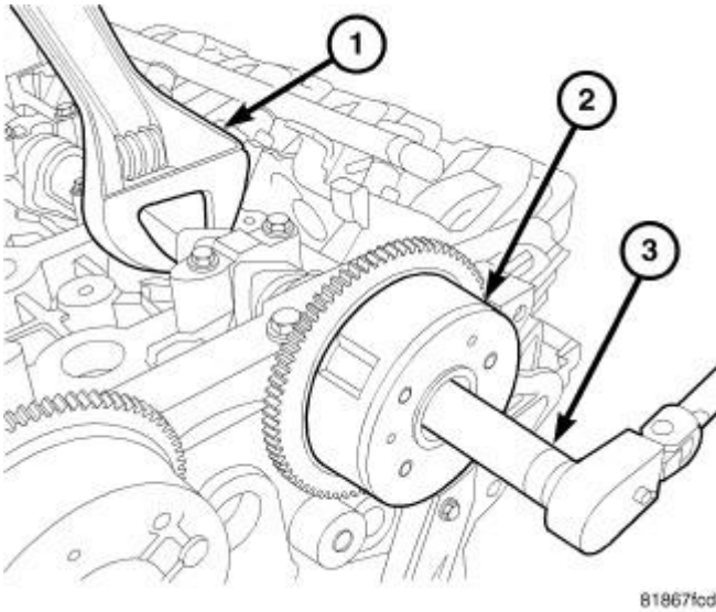
Fig. 133: Camshaft Phaser Removal & Installation Courtesy of CHRYSLER LLC
