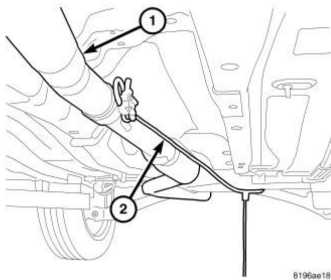
Fig. 42: Exhaust Pipe & Suitable Strap Courtesy of CHRYSLER LLC
