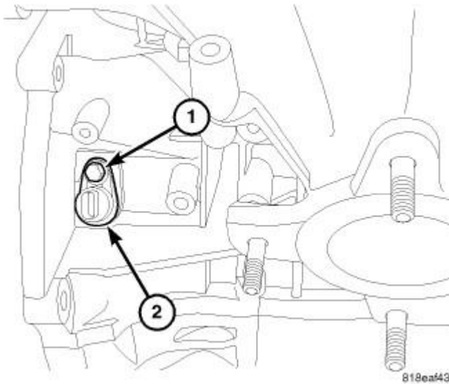
Fig. 229: Crankshaft Position Sensor Courtesy of CHRYSLER LLC
