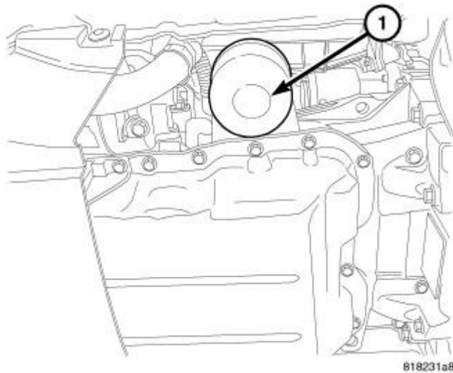
Fig. 301: Oil Filter
