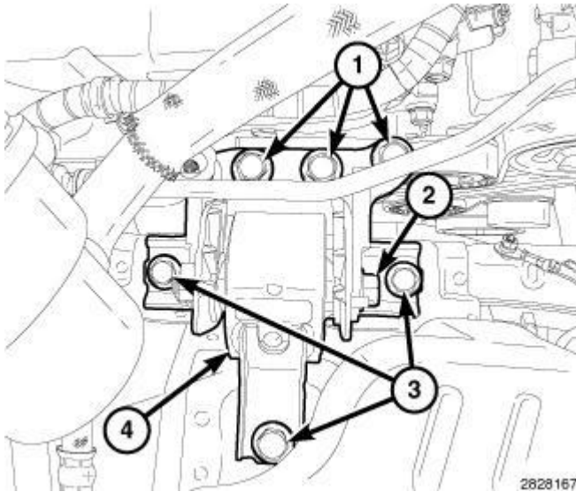
Fig. 346: Engine Mount Isolator, Right Engine Mount & Engine Mount Bracket Retaining Bolts Courtesy of CHRYSLER LLC
