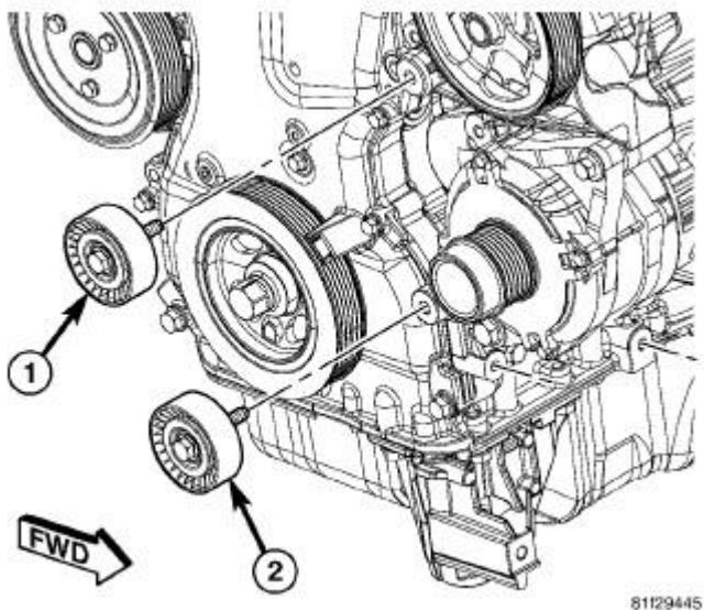
Fig. 434: Removing/Installing Accessory Drive Belt Lower Idler Pulley Courtesy of CHRYSLER LLC
