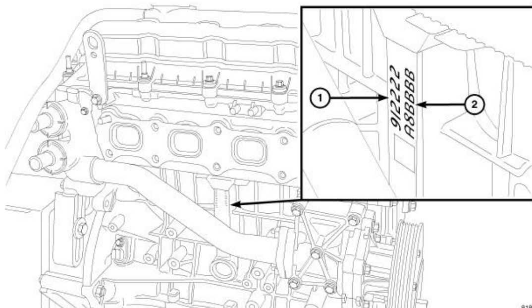
Fig. 210: Upper Main Bearing Shell Identification Courtesy of CHRYSLER LLC
