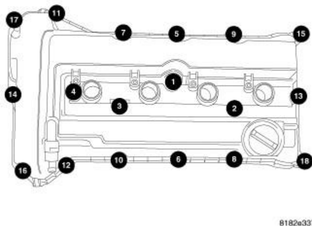
Fig. 167: Cylinder Head Cover Bolt Torque Sequence Courtesy of CHRYSLER LLC
