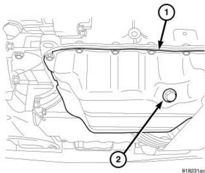
Fig. 25: Oil Drain Plug Courtesy of CHRYSLER LLC
