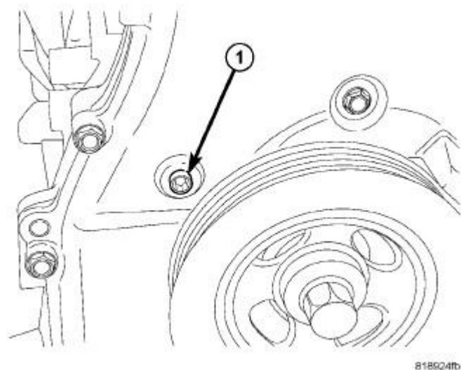
Fig. 147: Tensioner Access Plug
