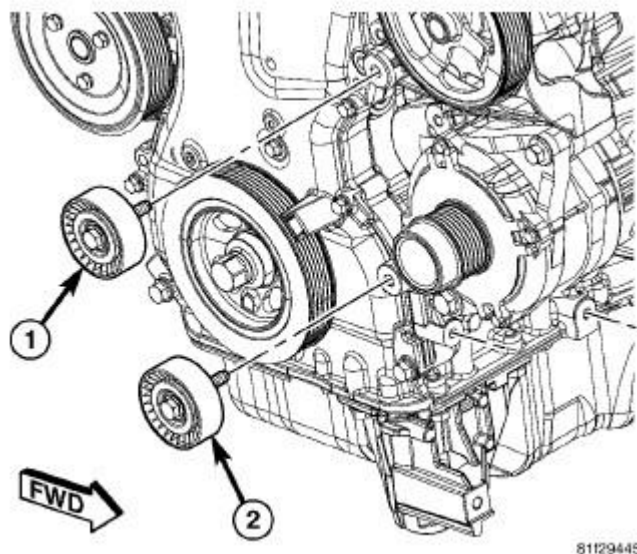
Fig. 438: Removing/Installing Accessory Drive Belt Lower Idler Pulley Courtesy of CHRYSLER LLC
