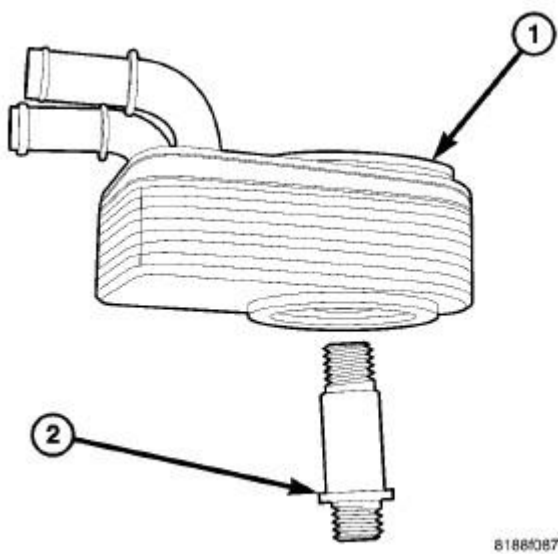
Fig. 293: Oil Cooler & Oil Cooler Connector Bolt Courtesy of CHRYSLER LLC
