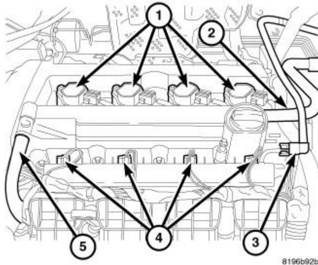
Fig. 10: Coil Connector
