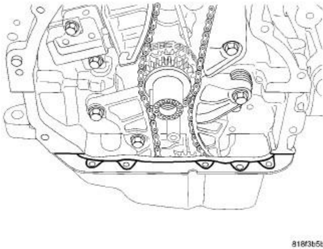
Fig. 430: Applying Mopar® Engine Sealant RTV (Or Equivalent) To Oil Pan
