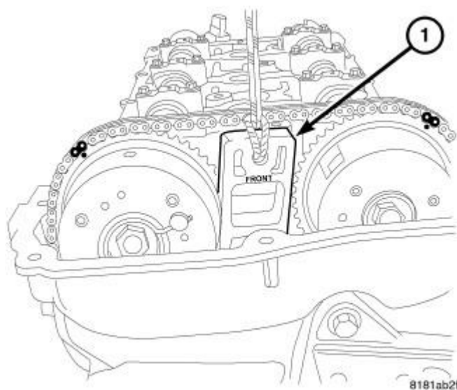
Fig. 149: Inserting Wedge 9701 Between Camshaft Phasers Courtesy of CHRYSLER LLC
