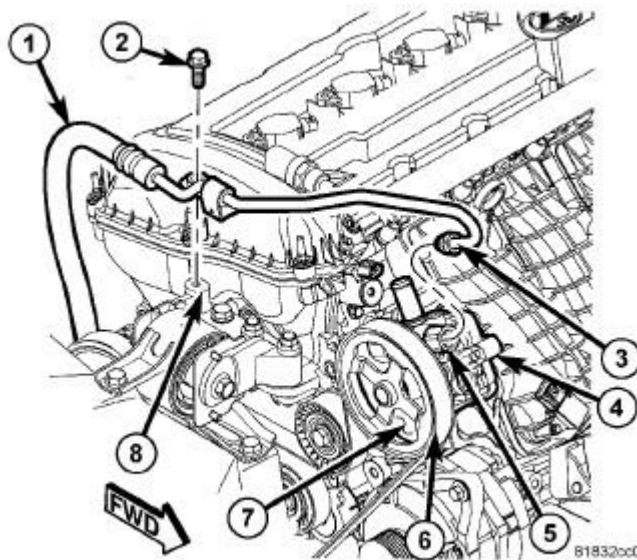
Fig. 345: Power Steering Assembly Components Courtesy of CHRYSLER LLC
