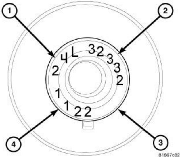
Fig. 209: Lower Main Bearing Identification Courtesy of CHRYSLER LLC
