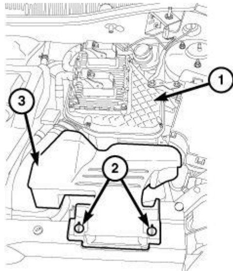
Fig. 58: Retainers, Fresh Air Inlet Duct & Air Cleaner Body Courtesy of CHRYSLER LLC
