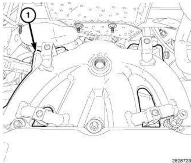
Fig. 341: Lower Manierverter Heatshield Courtesy of CHRYSLER LLC
