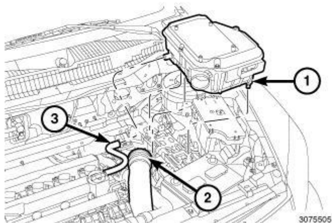
Fig. 56: Air Cleaner Body, Air Inlet Tube & Make-Up Air Hose Courtesy of CHRYSLER LLC
