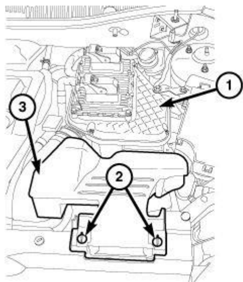
Fig. 194: Retainers, Fresh Air Inlet Duct & Air Cleaner Body Courtesy of CHRYSLER LLC
