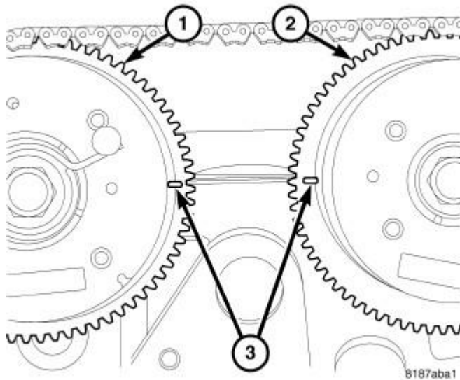
Fig. 397: Camshaft Timing Courtesy of CHRYSLER LLC
