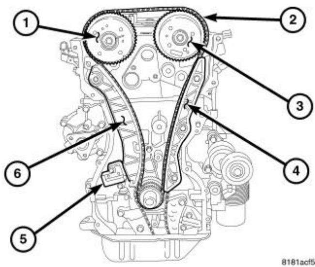
Fig. 446: Timing Drive System Courtesy of CHRYSLER LLC
