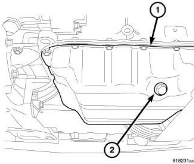
Fig. 214: Oil Drain Plug Courtesy of CHRYSLER LLC
