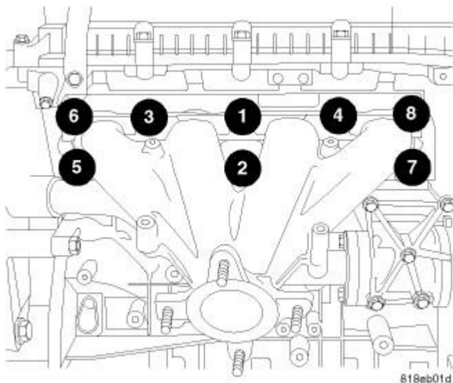
Fig. 371: Exhaust Manifold Retaining Fasteners Tightening Sequence Courtesy of CHRYSLER LLC
