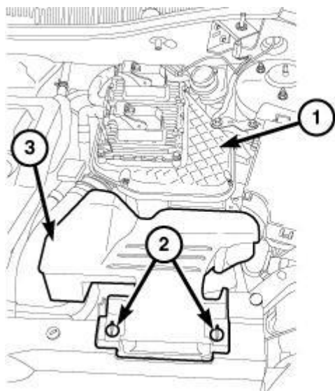
Fig. 67: Retainers, Fresh Air Inlet Duct & Air Cleaner Body Courtesy of CHRYSLER LLC
