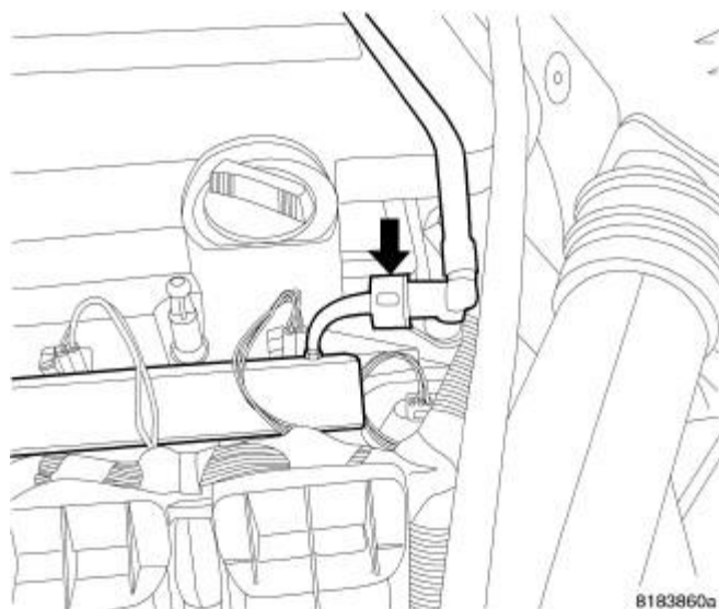
Fig. 92: Fuel Line At Fuel Rail Courtesy of CHRYSLER LLC
