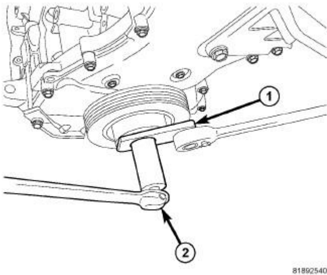
Fig. 235: Damper Removal & Installation Courtesy of CHRYSLER LLC
