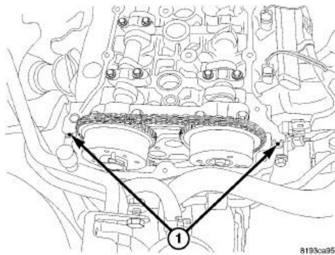
Fig. 174: Applying RTV To Cylinder Head/Front Cover T-Joint Courtesy of CHRYSLER LLC
