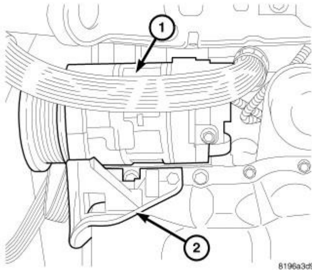
Fig. 419: A/C Compressor & Mounting Bracket Courtesy of CHRYSLER LLC
