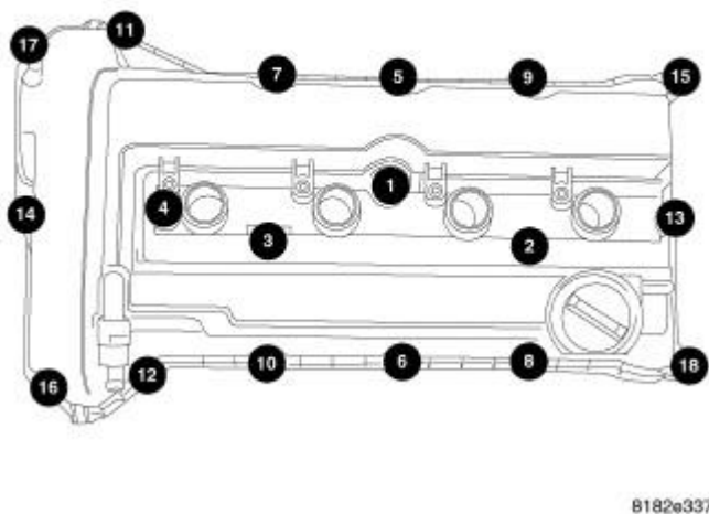
Fig. 171: Removing/Installing Cylinder Head Cover Bolts In Sequence Courtesy of CHRYSLER LLC
