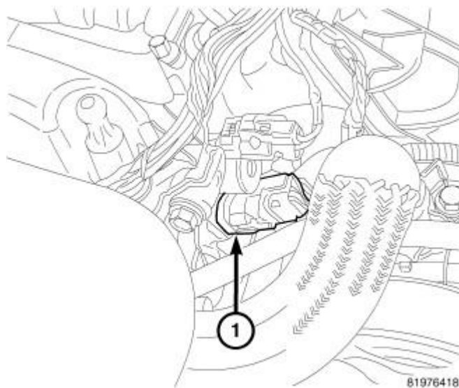
Fig. 389: Oil Temperature Sensor Courtesy of CHRYSLER LLC
