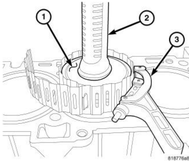
Fig. 256: Piston, Hammer Handle & Ring Compressor Courtesy of CHRYSLER LLC
