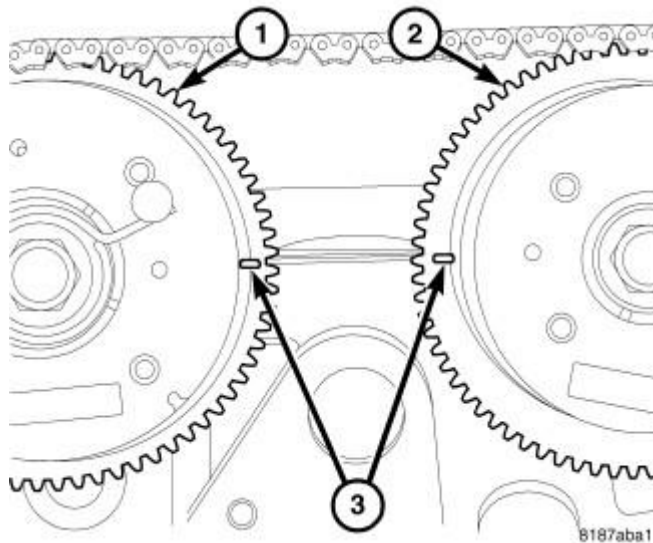
Fig. 412: Camshaft Timing Courtesy of CHRYSLER LLC
