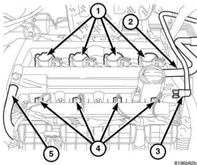
Fig. 381: Coil Connectors Courtesy of CHRYSLER LLC
