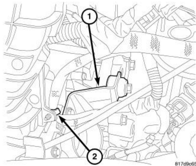
Fig. 383: Throttle Body Support Courtesy of CHRYSLER LLC
