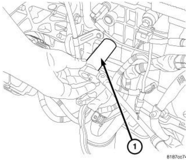
Fig. 324: Oil Sender
