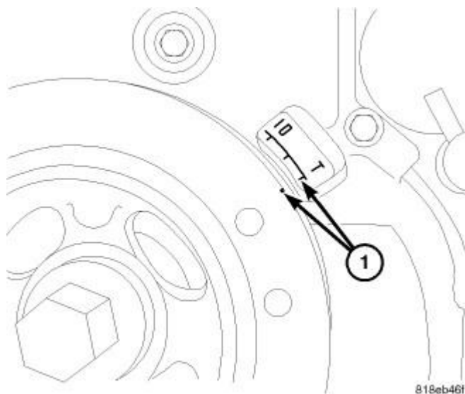
Fig. 81: Setting Crankshaft To Top Dead Center Courtesy of CHRYSLER LLC
