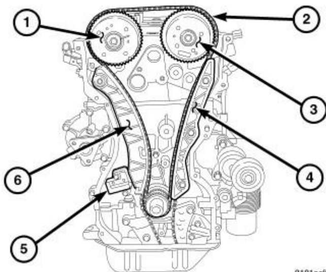
Fig. 120: Timing Drive
