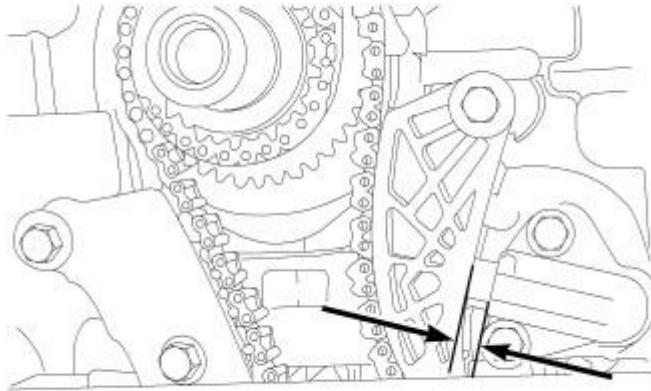
Fig. 316: Oil Pump Chain Stretch Courtesy of CHRYSLER LLC
