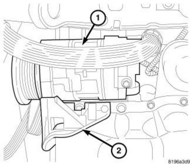
Fig. 303: A/C Compressor Courtesy of CHRYSLER LLC
