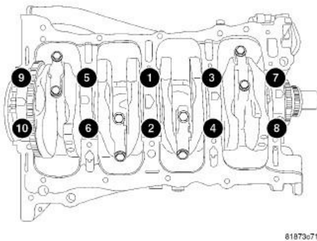
Fig. 221: Main Bearing Cap Torque Sequence Courtesy of CHRYSLER LLC
