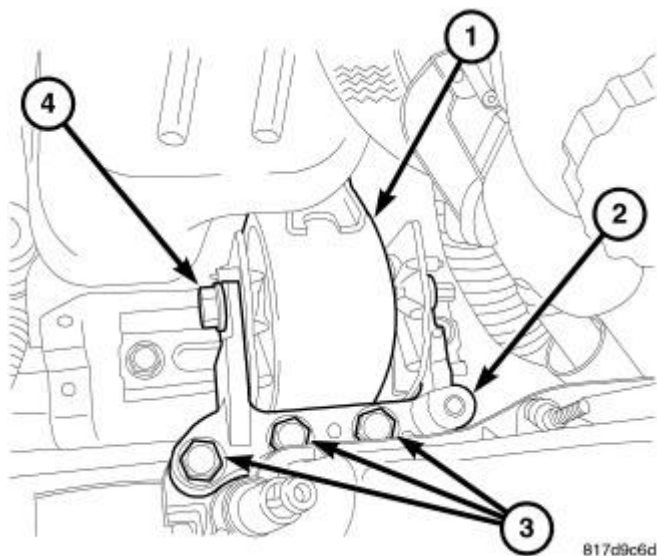
Fig. 200: Right Engine Mount Courtesy of CHRYSLER LLC
