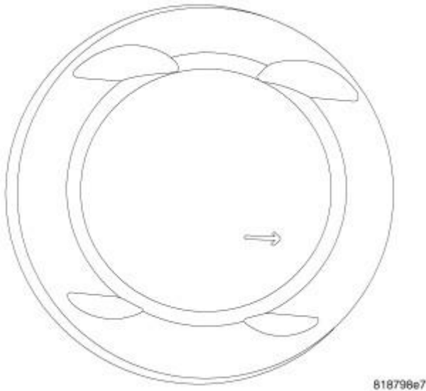
Fig. 255: Piston Installation Courtesy of CHRYSLER LLC
