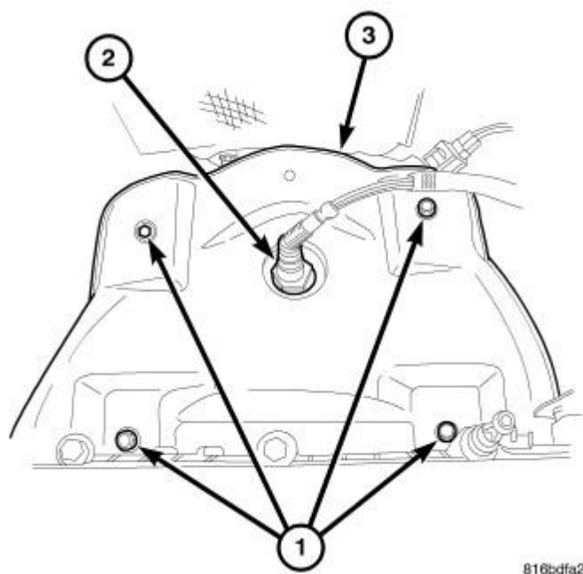
Fig. 368: Maniverter Heat Shield And Bolts Courtesy of CHRYSLER LLC
