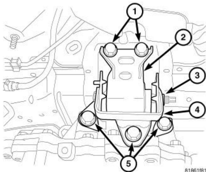
Fig. 190: Left Mount
