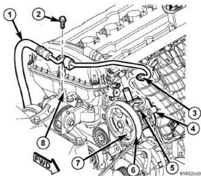
Fig. 415: Power Steering Assembly Components Courtesy of CHRYSLER LLC
