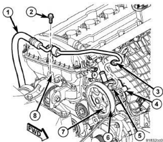
Fig. 355: Power Steering Assembly Components Courtesy of CHRYSLER LLC
