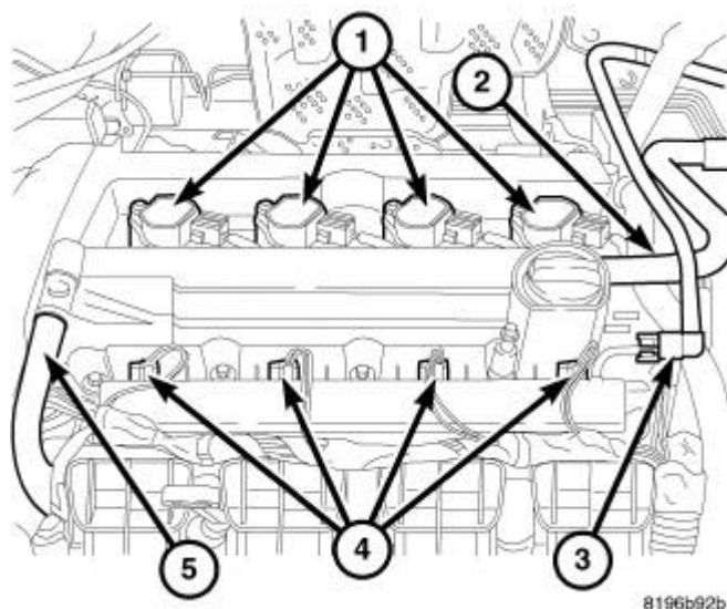
Fig. 125: Coil Connector Courtesy of CHRYSLER LLC
