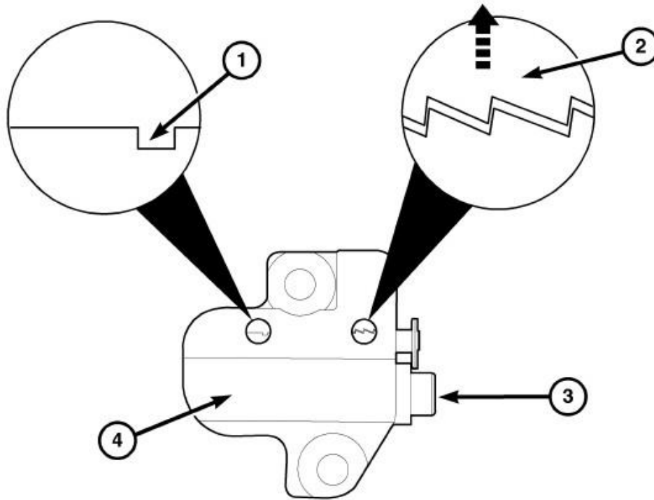
Fig. 447: Tensioner Reset Courtesy of CHRYSLER LLC
