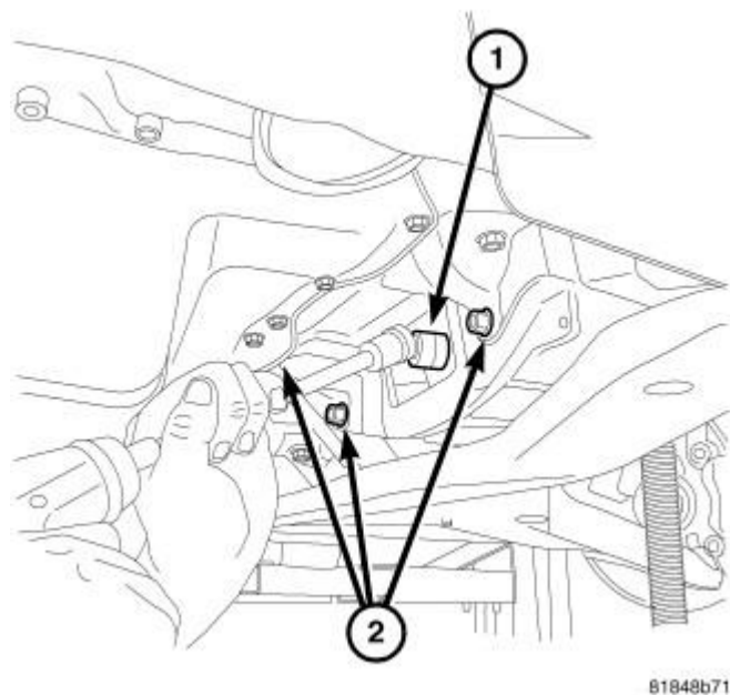
Fig. 37: Modular Clutch To Flex Plate Bolts
