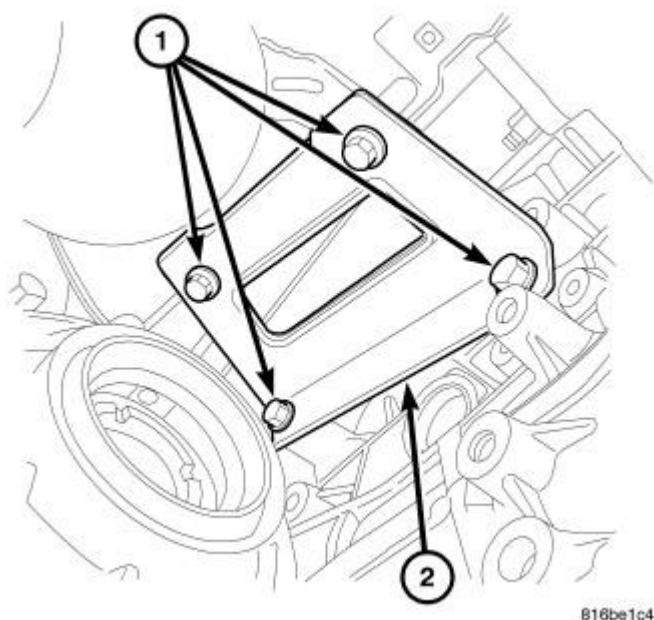
Fig. 338: Maniverter To Block Support Bracket Courtesy of CHRYSLER LLC
