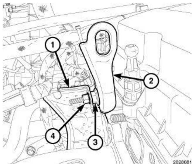
Fig. 358: Heatshield, Stud Bolt, Engine Lift Bracket & Nut Courtesy of CHRYSLER LLC
