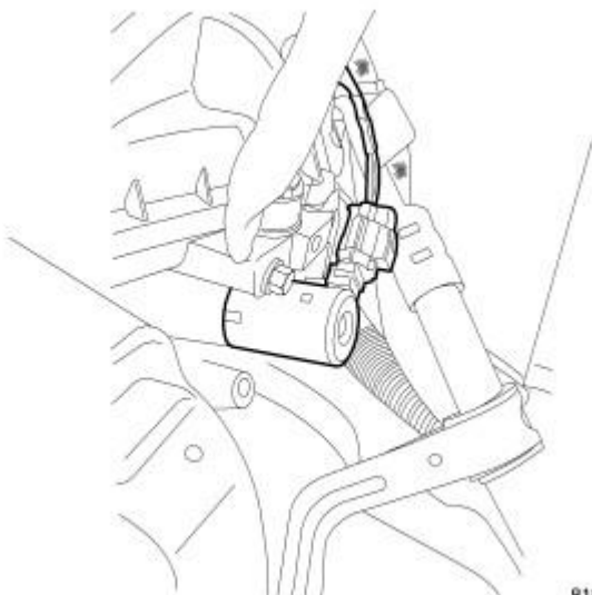
Fig. 291: Solenoid Location 1/2 Courtesy of CHRYSLER LLC
