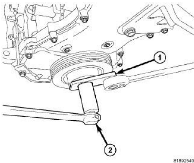
Fig. 234: Damper Removal & Installation Courtesy of CHRYSLER LLC
