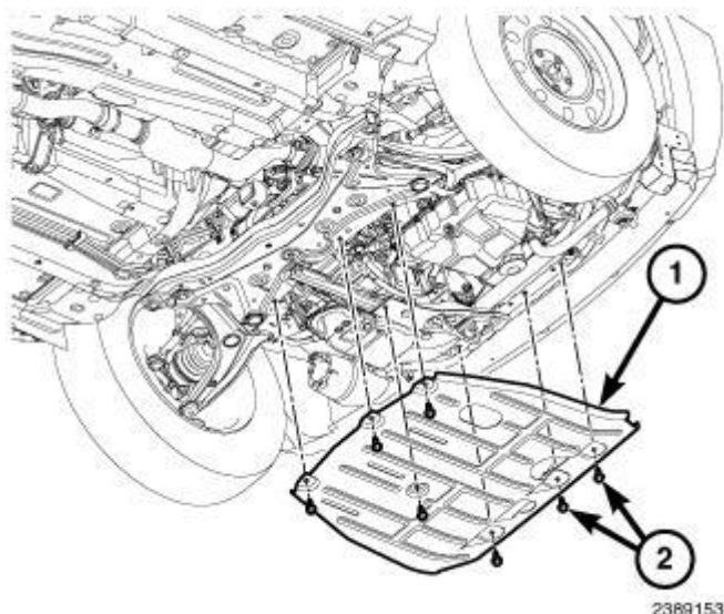
Fig. 367: Removal/Installation Front Skid Plate And Bolts Courtesy of CHRYSLER LLC
