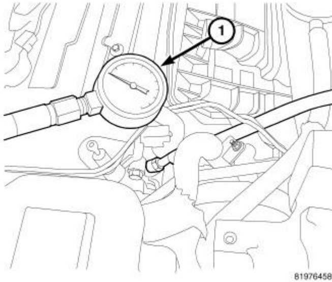
Fig. 277: Oil PSI Gauge Courtesy of CHRYSLER LLC
