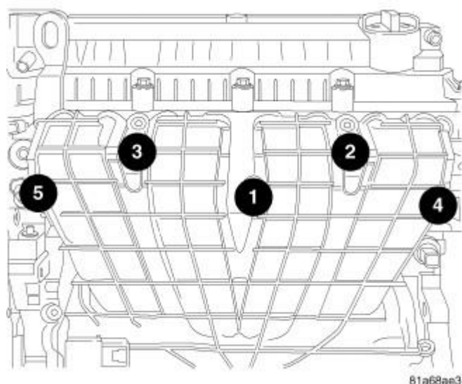
Fig. 98: Intake Manifold Bolt Removal & Tightening Sequence Courtesy of CHRYSLER LLC
