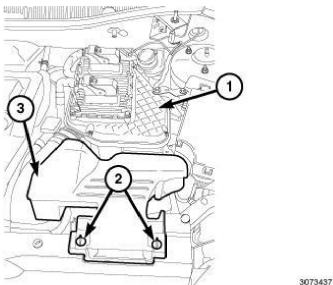
Fig. 187: Retainers, Fresh Air Inlet Duct & Air Cleaner Body Courtesy of CHRYSLER LLC
