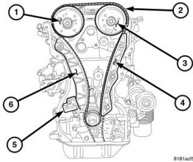
Fig. 411: Timing Drive Courtesy of CHRYSLER LLC
