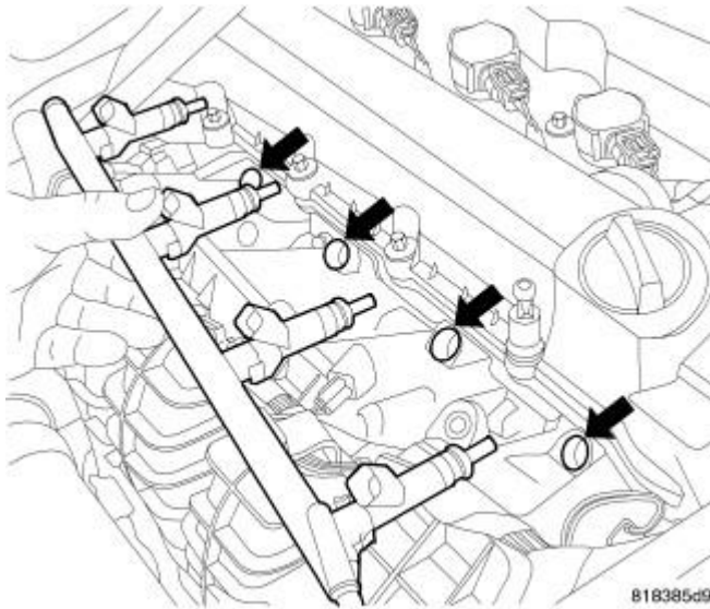
Fig. 94: Removing/Installing Fuel Rail Courtesy of CHRYSLER LLC
