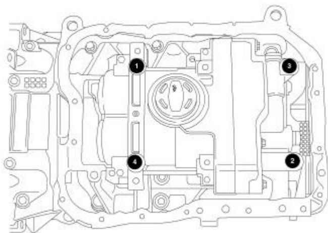
Fig. 319: BSM Mounting Bolts Tightening Sequence Courtesy of CHRYSLER LLC
