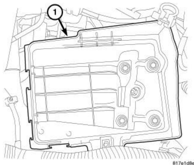
Fig. 14: Battery Tray Courtesy of CHRYSLER LLC
