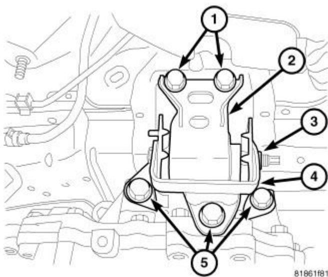
Fig. 191: Left Mount
