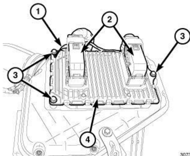
Fig. 379: Electrical Connectors, PCM, Three Mounting Bolts & Ground Wire Courtesy of CHRYSLER LLC
