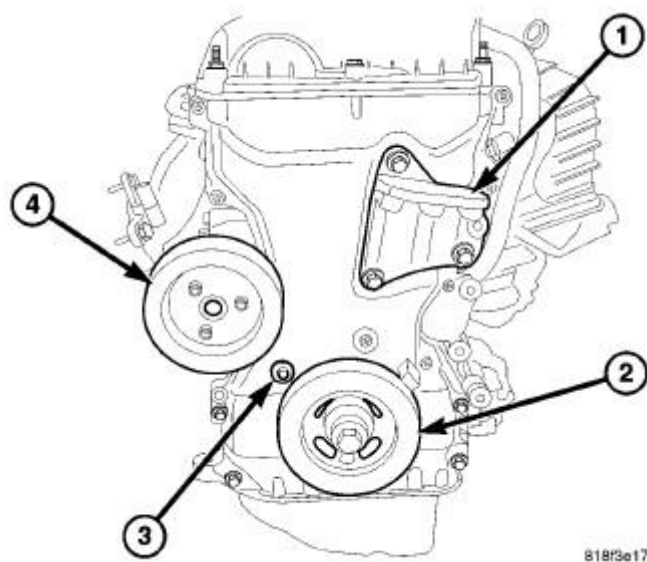
Fig. 425: Right Side Engine Mount Bracket, Crankshaft Damper & Water Pump Pulley Courtesy of CHRYSLER LLC
