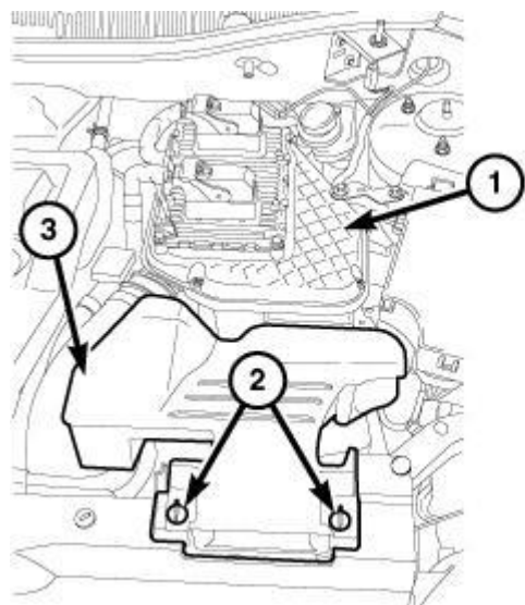
Fig. 378: Retainers, Fresh Air Inlet Duct & Air Cleaner Body Courtesy of CHRYSLER LLC
