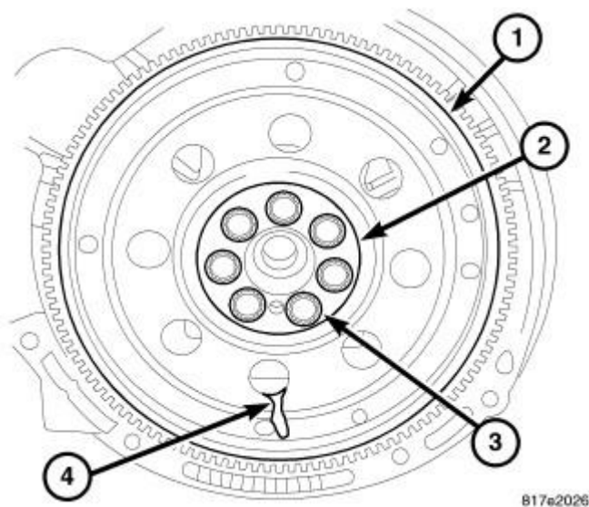
Fig. 212: Flex Plate
