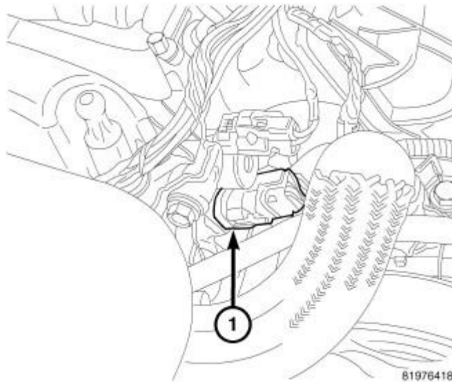
Fig. 382: Oil Temperature Sensor Courtesy of CHRYSLER LLC
