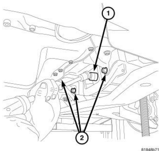
Fig. 29: Modular Clutch To Flex Plate Bolts Courtesy of CHRYSLER LLC
