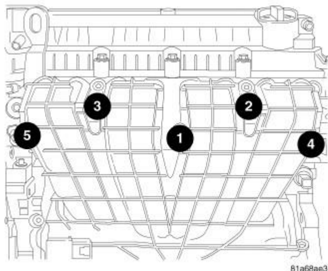
Fig. 49: Intake Manifold Bolt Removal & Tightening Sequence Courtesy of CHRYSLER LLC
