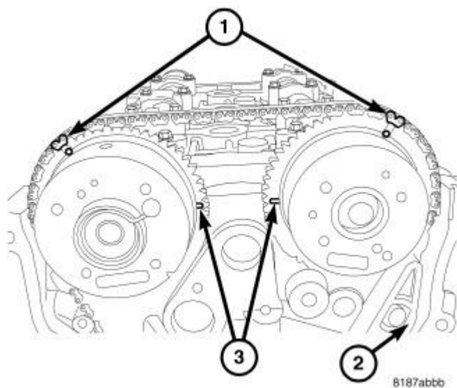
Fig. 146: Timing Chain Timing Marks
