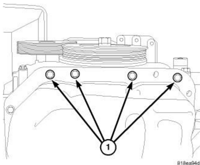
Fig. 436: Oil Pan To Timing Chain Cover Lower Bolts Courtesy of CHRYSLER LLC
