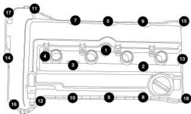
Fig. 440: Remove/Install Cylinder Head Cover Bolts In Sequence Courtesy of CHRYSLER LLC
