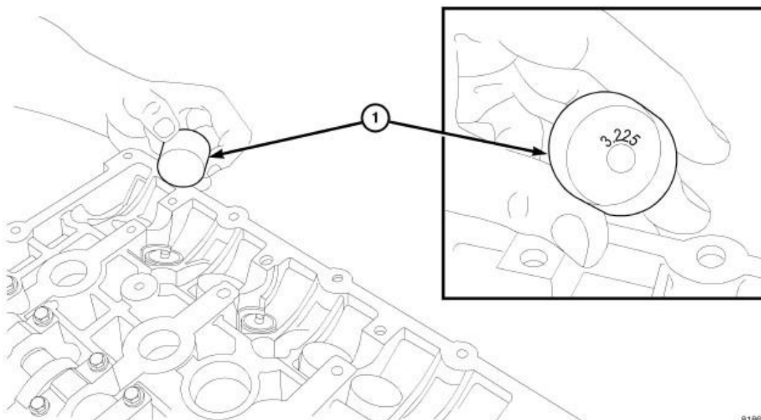
Fig. 140: Tappet Identification Courtesy of CHRYSLER LLC
