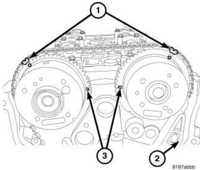
Fig. 151: Timing Chain Timing Marks Courtesy of CHRYSLER LLC
