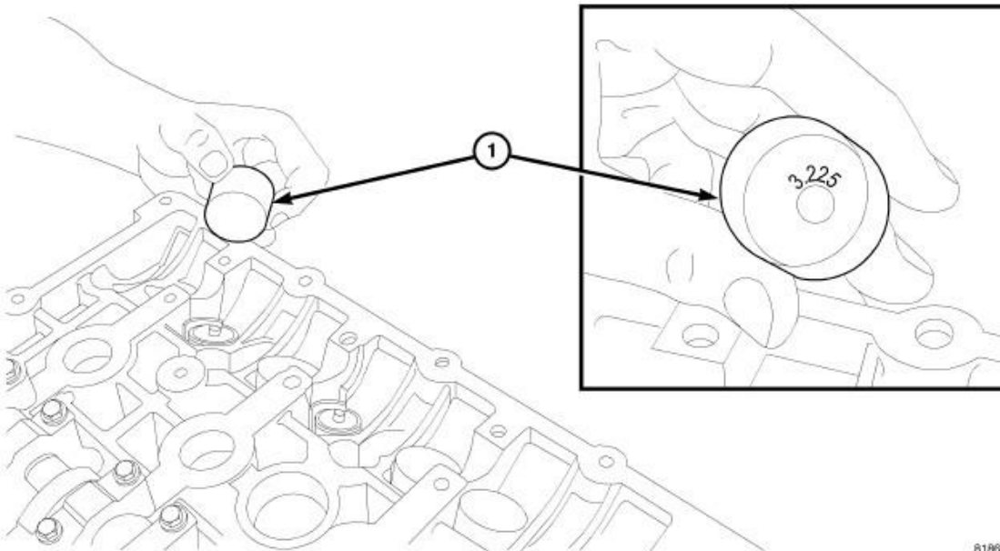
Fig. 145: Tappet Identification Courtesy of CHRYSLER LLC
