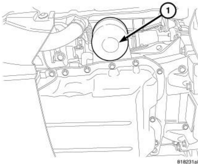
Fig. 236: Oil Filter Courtesy of CHRYSLER LLC
