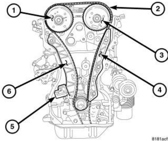
Fig. 378: Timing Drive Courtesy of CHRYSLER LLC
