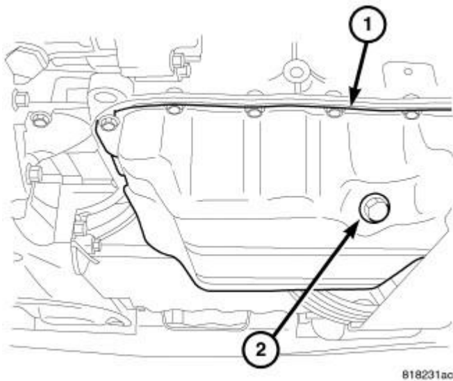
Fig. 306: Oil Drain Plug
