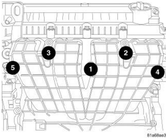
Fig. 47: Torque Sequence Courtesy of CHRYSLER LLC
