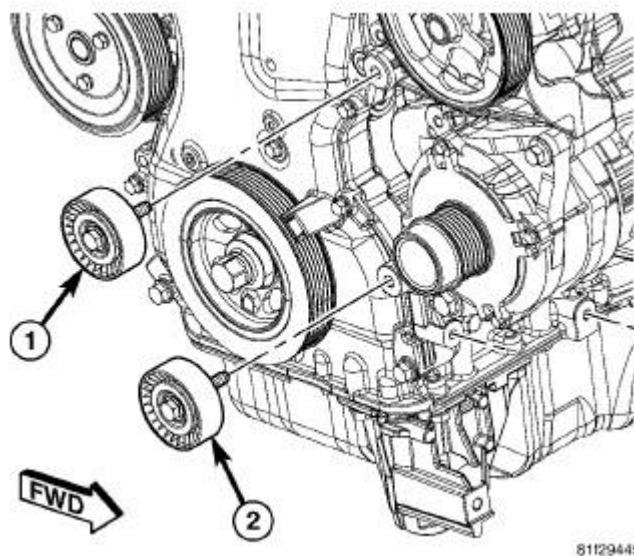
Fig. 397: Accessory Drive Belt Idler Pulley - 2.4L Courtesy of CHRYSLER LLC
