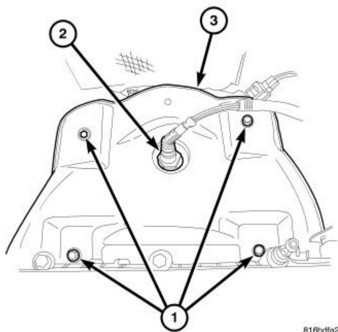
Fig. 347: Maniverter Heat Shield & Bolts Courtesy of CHRYSLER LLC
