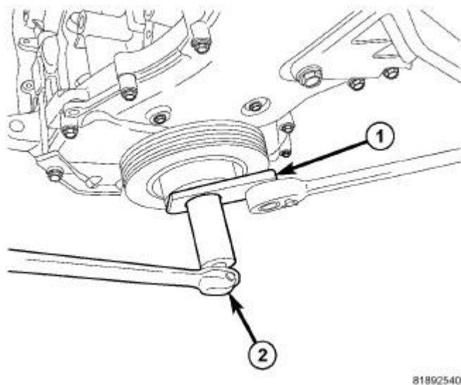
Fig. 262: Damper Removal Courtesy of CHRYSLER LLC
