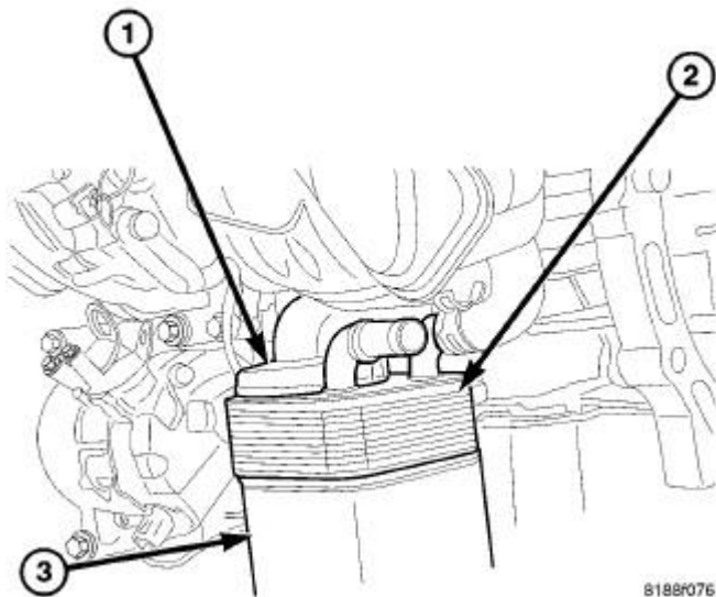
Fig. 44: Oil Cooler Courtesy of CHRYSLER LLC
