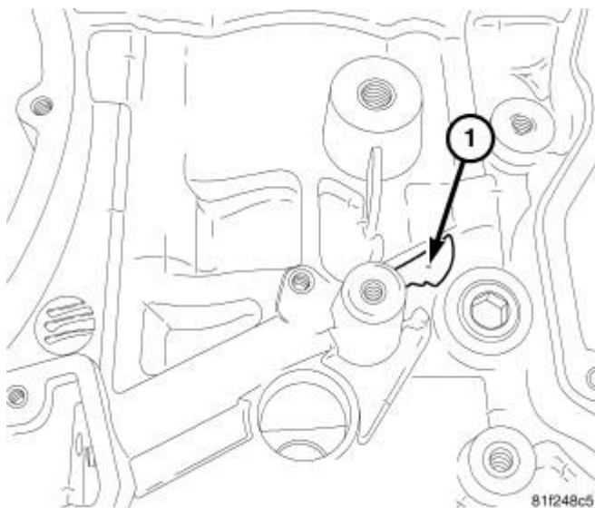
Fig. 273: Oil Hole
