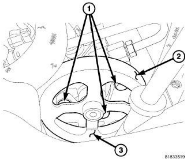
Fig. 393: Power Steering Pump - Gas Courtesy of CHRYSLER LLC
