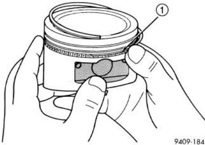
Fig. 248: Installing Side Rail Courtesy of CHRYSLER LLC
