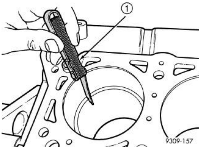
Fig. 245: Check Gap On Piston Rings Courtesy of CHRYSLER LLC
