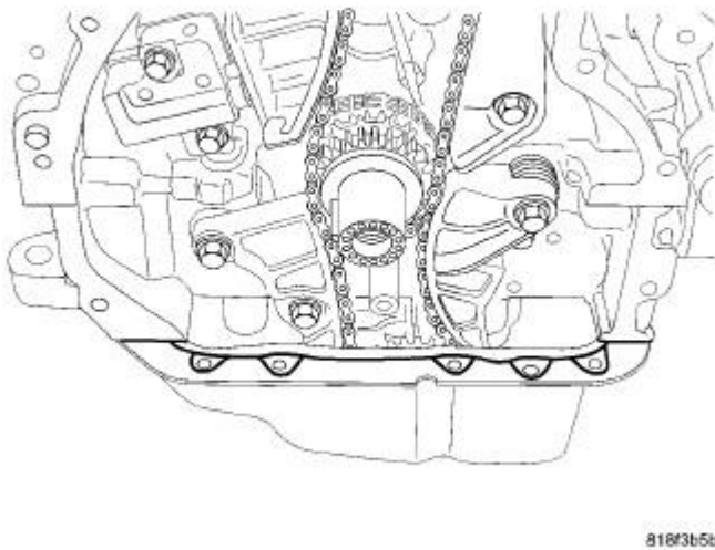
Fig. 407: Sealing Oil Pan Courtesy of CHRYSLER LLC
