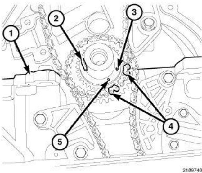
Fig. 386: Crankshaft Timing Marks Courtesy of CHRYSLER LLC
