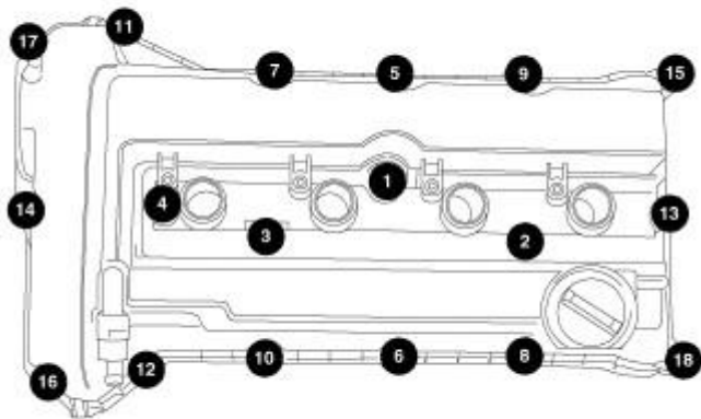
Fig. 139: Torque Sequence Courtesy of CHRYSLER LLC
