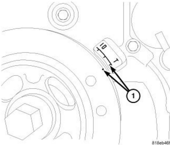
Fig. 88: TDC Courtesy of CHRYSLER LLC
