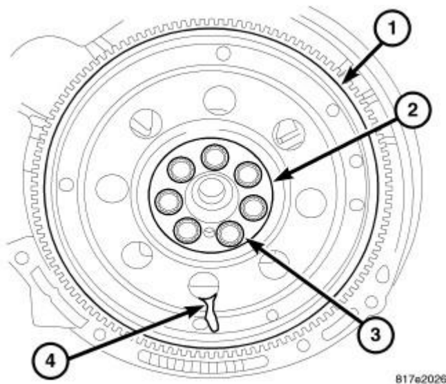
Fig. 240: Flex Plate
