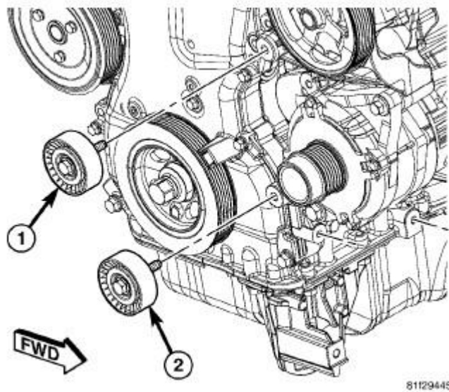
Fig. 401: Accessory Drive Belt Idler Pulley - 2.4L Courtesy of CHRYSLER LLC
