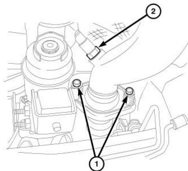
Fig. 349: Exhaust To Maniverter Bolts Courtesy of CHRYSLER LLC
