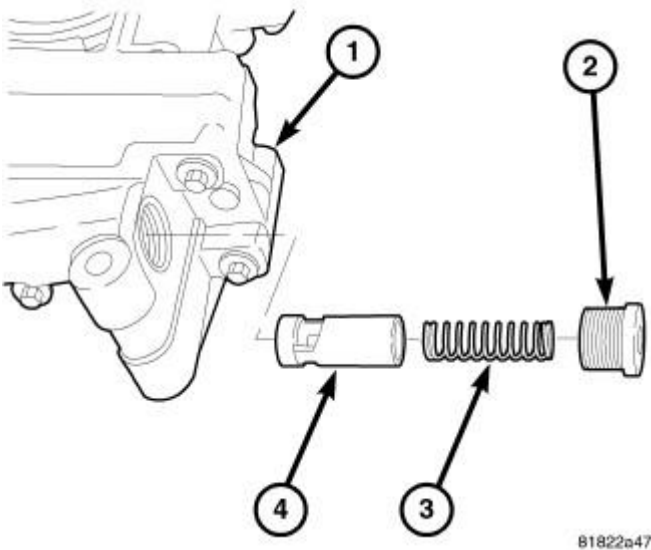
Fig. 332: Oil Pressure Relief Valve Courtesy of CHRYSLER LLC
