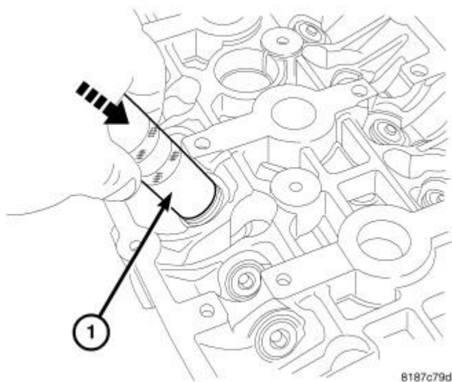
Fig. 183: Valve Removal Courtesy of CHRYSLER LLC
