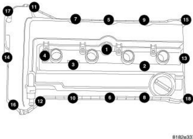
Fig. 180: Torque Sequence
