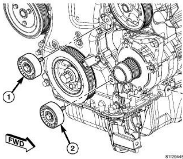
Fig. 415: Accessory Drive Belt Idler Pulley - 2.4L Courtesy of CHRYSLER LLC
