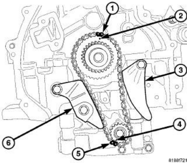
Fig. 321: BSM Timing
