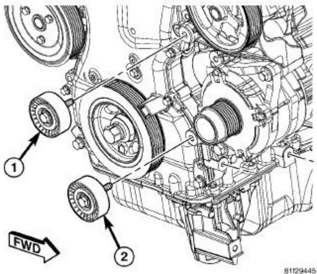
Fig. 411: Accessory Drive Belt Idler Pulley - 2.4L Courtesy of CHRYSLER LLC
