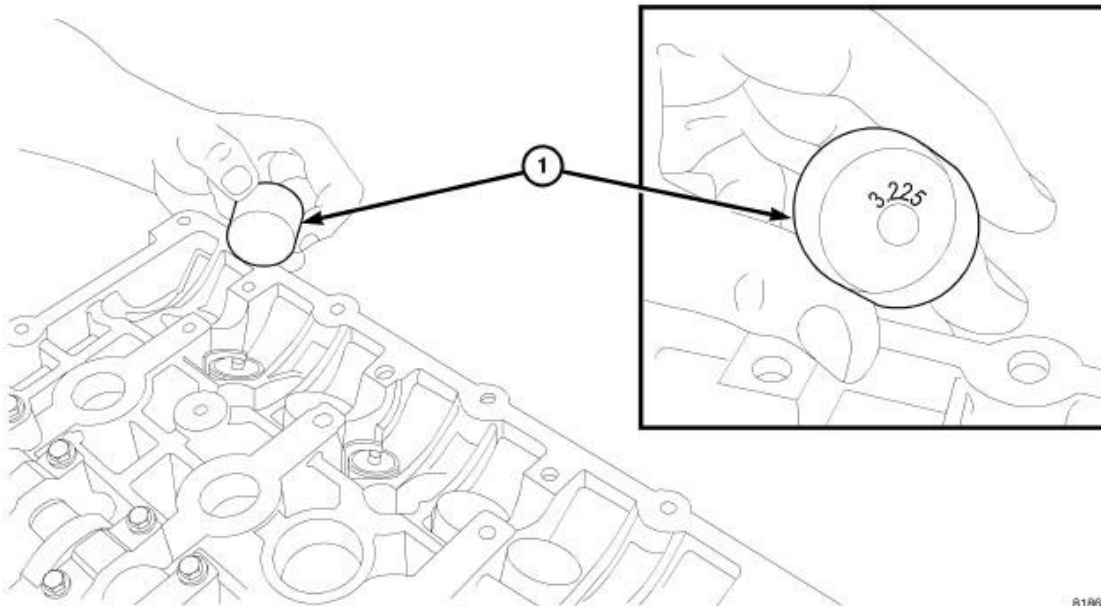
Fig. 142: Tappet Identification Courtesy of CHRYSLER LLC
