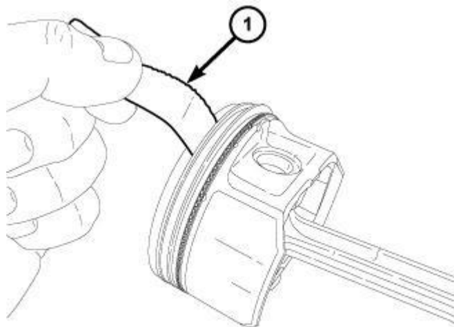
Fig. 246: Piston Ring To Groove Side Clearance Courtesy of CHRYSLER LLC
