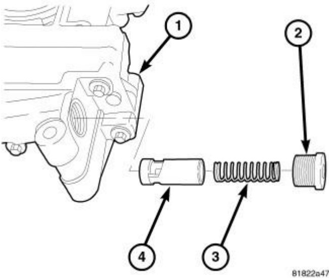
Fig. 331: Oil Pressure Relief Valve Courtesy of CHRYSLER LLC
