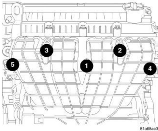
Fig. 130: Torque Sequence Courtesy of CHRYSLER LLC
