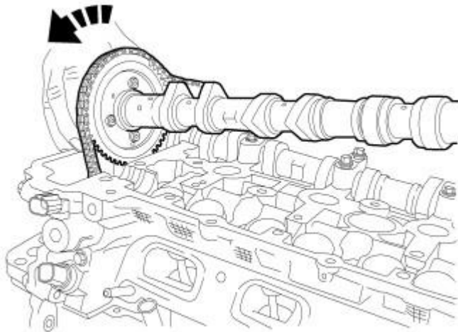
Fig. 158: Roll Camshaft Courtesy of CHRYSLER LLC
