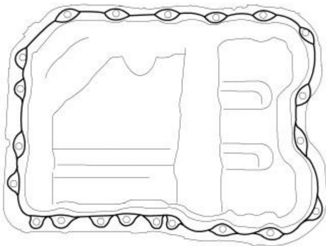
Fig. 310: Sealing Oil Pan
