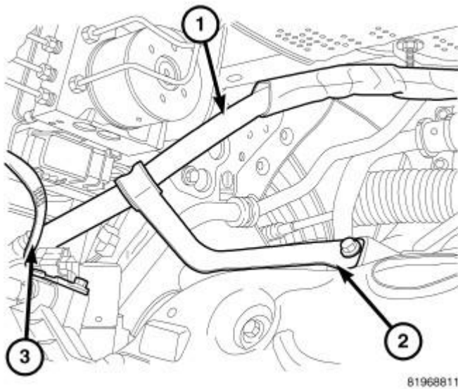
Fig. 46: P/S Hose Support - FWD Courtesy of CHRYSLER LLC
