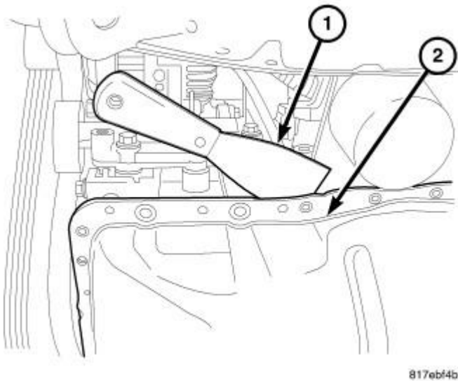
Fig. 220: Oil Pan Removal Courtesy of CHRYSLER LLC
