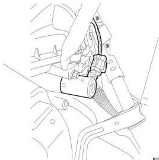
Fig. 287: Solenoid Location 1/2 Courtesy of CHRYSLER LLC
