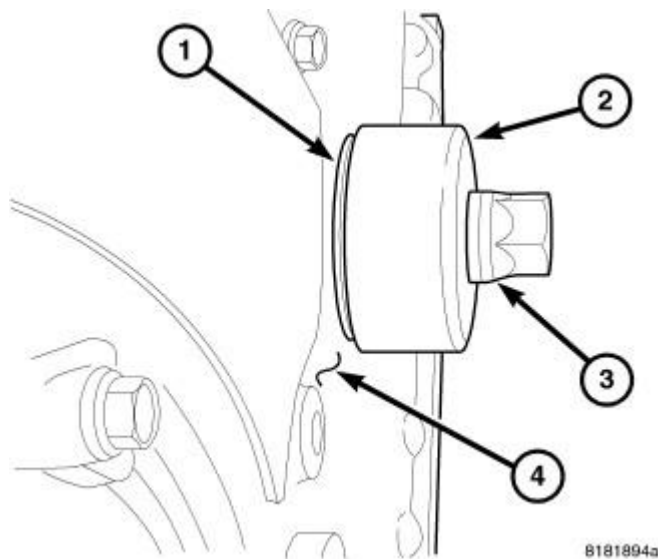
Fig. 265: Installing Front Seal Courtesy of CHRYSLER LLC
