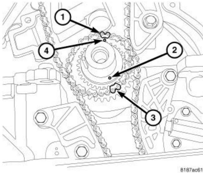
Fig. 377: Crankshaft Timing Marks Courtesy of CHRYSLER LLC
