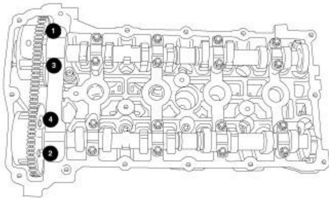
Fig. 156: Front Camshaft Cap Removal Sequence Courtesy of CHRYSLER LLC
