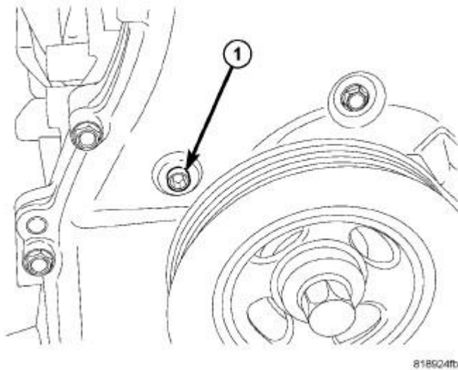
Fig. 169: Tensioner Access Plug Courtesy of CHRYSLER LLC
