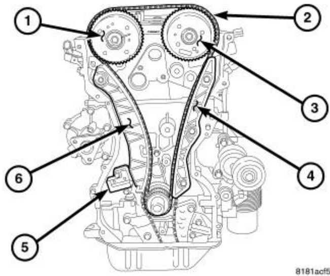
Fig. 389: Timing Drive Courtesy of CHRYSLER LLC
