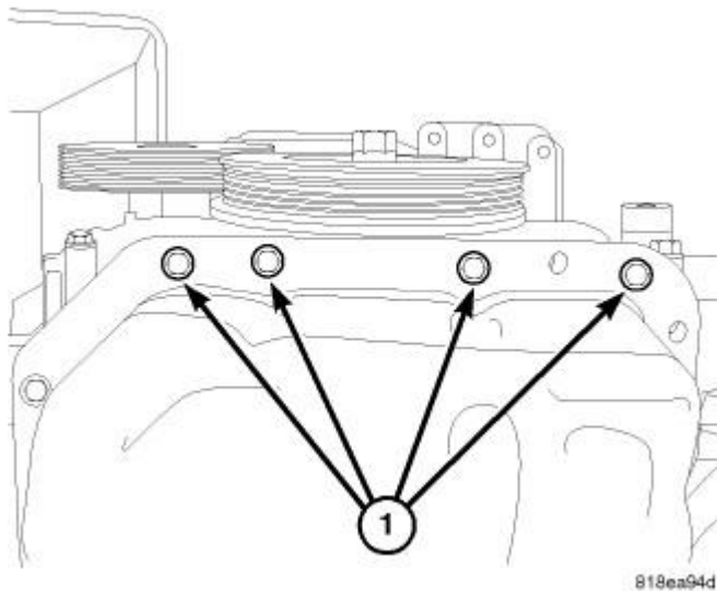
Fig. 413: Timing Chain Cover Lower Bolts Courtesy of CHRYSLER LLC
