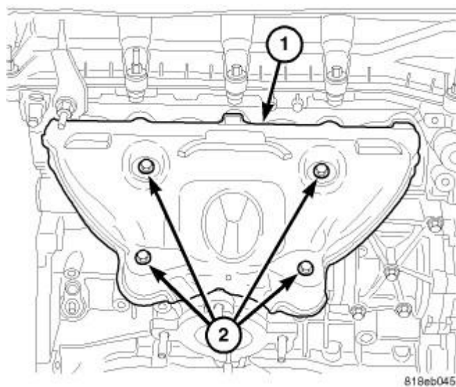
Fig. 341: Exhaust Manifold Heat Shield Courtesy of CHRYSLER LLC
