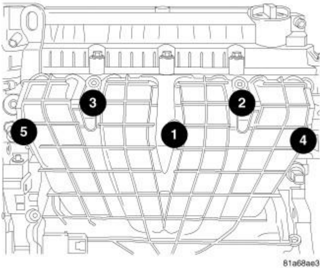
Fig. 368: Torque Sequence Courtesy of CHRYSLER LLC
