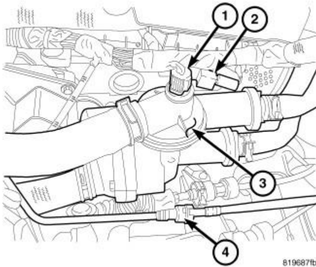
Fig. 338: Coolant Adapter Courtesy of CHRYSLER LLC
