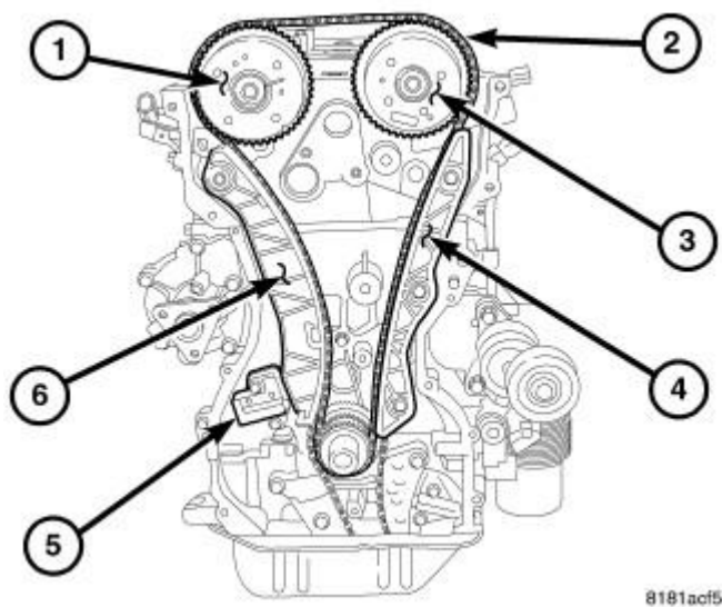
Fig. 372: Timing Drive Courtesy of CHRYSLER LLC
