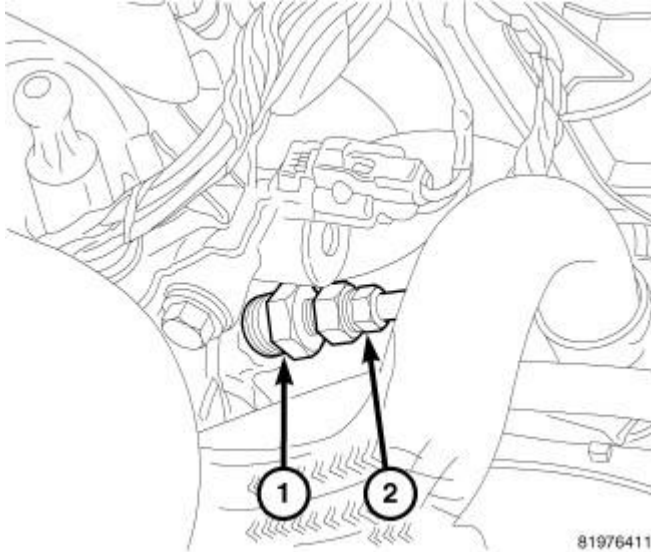
Fig. 275: Oil Pressure Adapter Courtesy of CHRYSLER LLC
