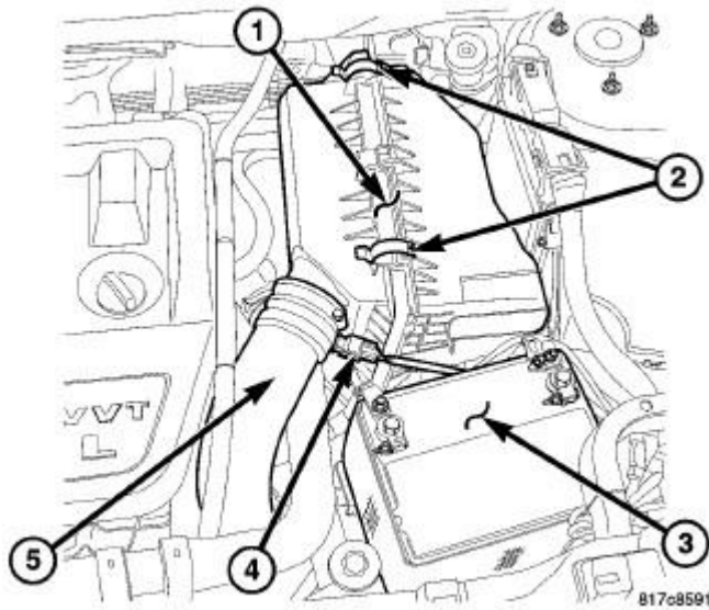
Fig. 369: Air Cleaner Housing Courtesy of CHRYSLER LLC
