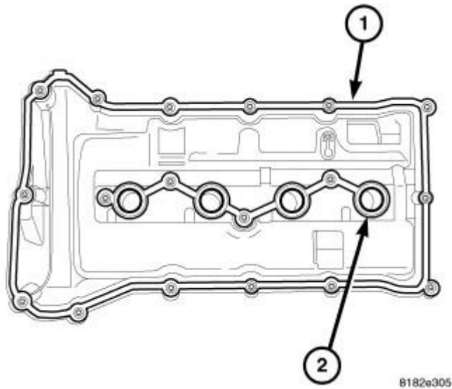
Fig. 171: Gasket Location Courtesy of CHRYSLER LLC
