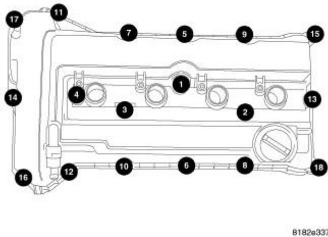
Fig. 417: Torque Sequence Courtesy of CHRYSLER LLC
