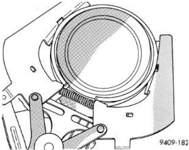
Fig. 247: Piston Rings - Removing & Installing Courtesy of CHRYSLER LLC
