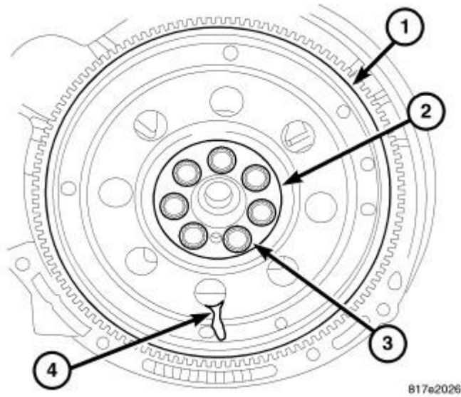
Fig. 215: FLEX PLATE Courtesy of CHRYSLER LLC
