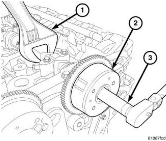
Fig. 138: Camshaft Phaser Installation
