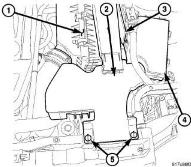
Fig. 192: Air Cleaner Inlet
