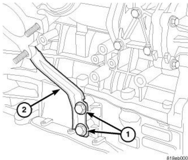
Fig. 343: Exhaust Manifold Support Bracket Courtesy of CHRYSLER LLC
