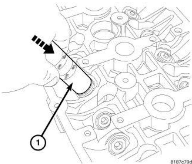
Fig. 184: Valve Removal Courtesy of CHRYSLER LLC
