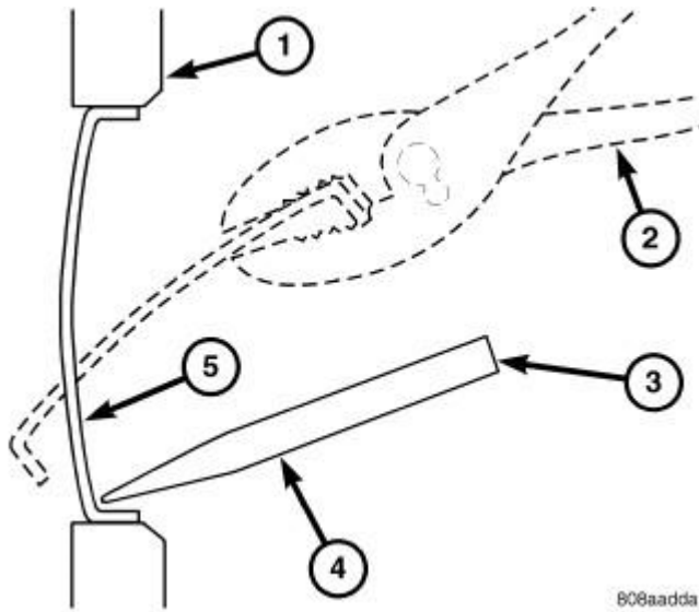
Fig. 4: Core Hole Plug Removal Courtesy of CHRYSLER LLC
