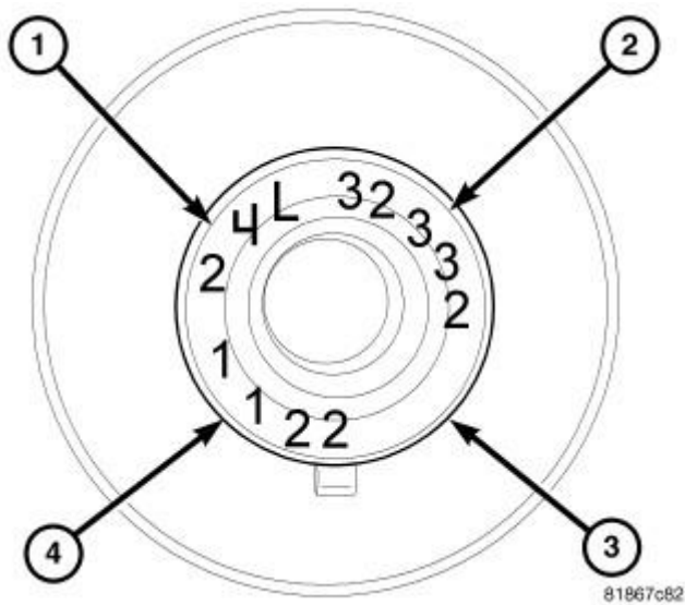
Fig. 209: Connecting Rod Bearing Identification Courtesy of CHRYSLER LLC
