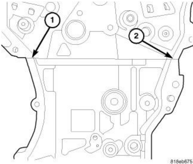
Fig. 405: Front Cover Upper T-Joints
