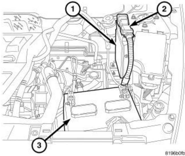
Fig. 193: Battery Courtesy of CHRYSLER LLC
