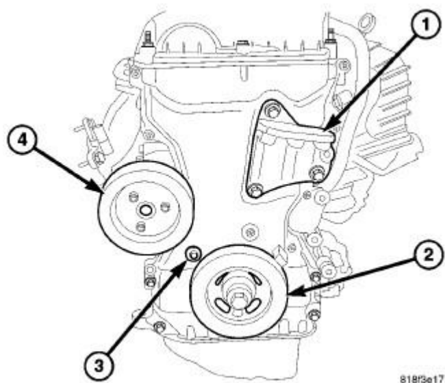
Fig. 402: Engine Front Courtesy of CHRYSLER LLC
