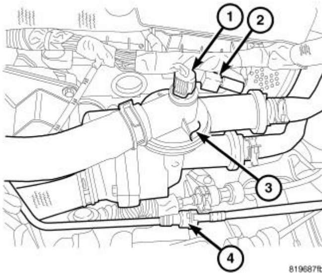
Fig. 346: Coolant Adapter
