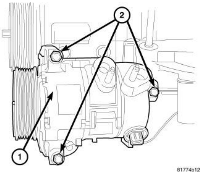
Fig. 326: A/C Compressor - R & I Courtesy of CHRYSLER LLC
