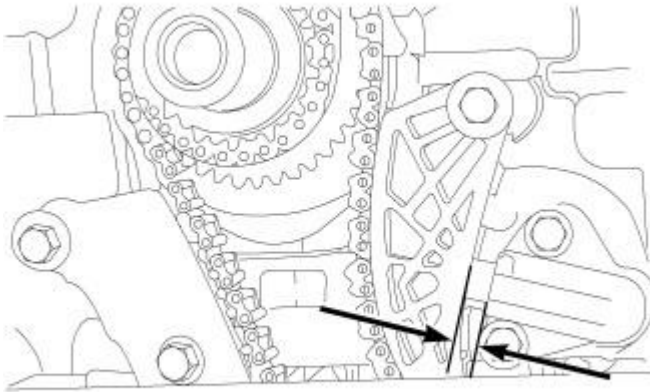
Fig. 320: Oil Pump Chain Stretch Courtesy of CHRYSLER LLC
