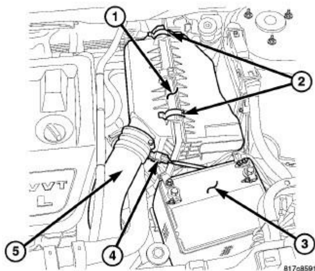
Fig. 352: Air Cleaner Housing Courtesy of CHRYSLER LLC
