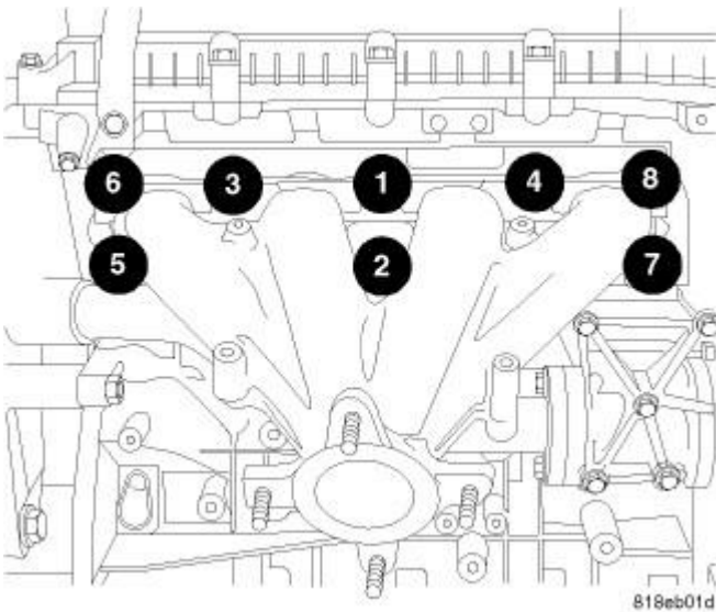
Fig. 354: Torque Sequence Courtesy of CHRYSLER LLC
