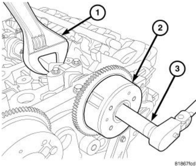
Fig. 385: Cam Phaser Installation Courtesy of CHRYSLER LLC
