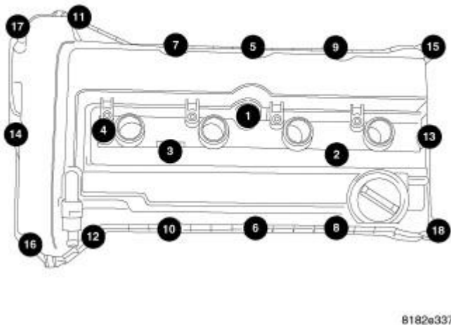
Fig. 176: Torque Sequence Courtesy of CHRYSLER LLC
