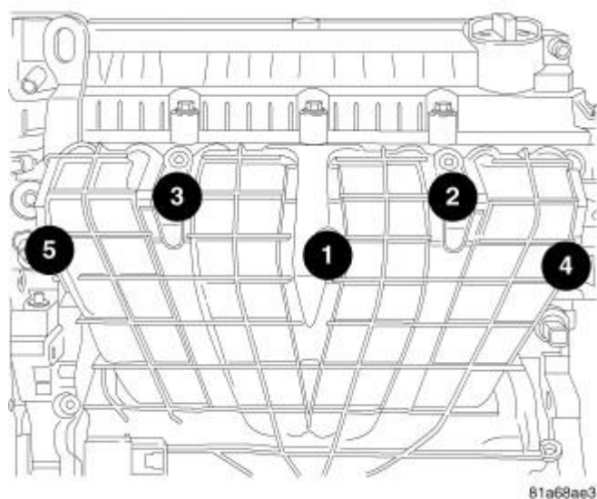
Fig. 105: Intake Torque Sequence Courtesy of CHRYSLER LLC
