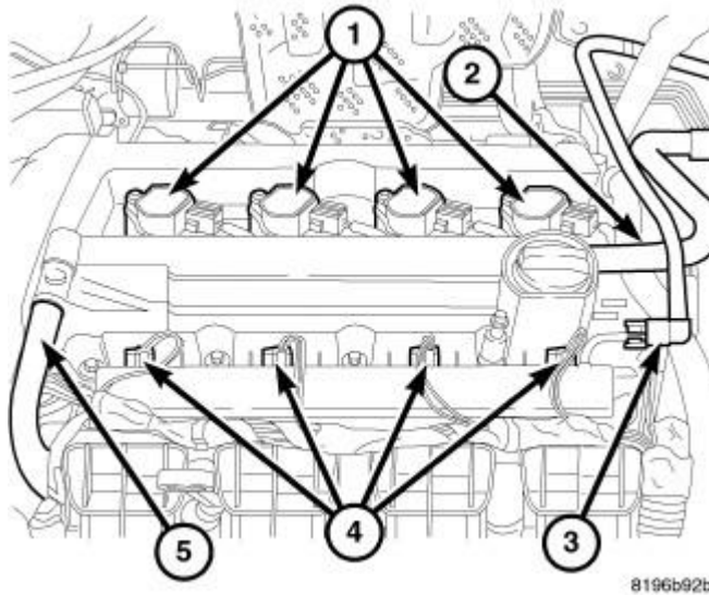
Fig. 363: Coil Connector Courtesy of CHRYSLER LLC
