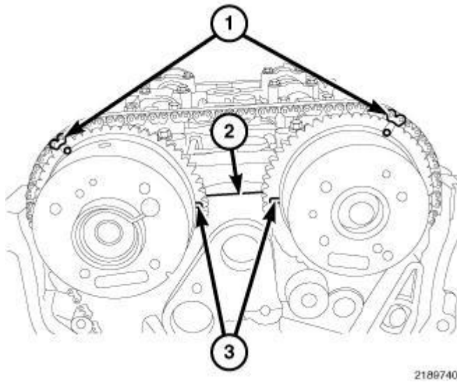
Fig. 164: Timing Chain Timing Marks
