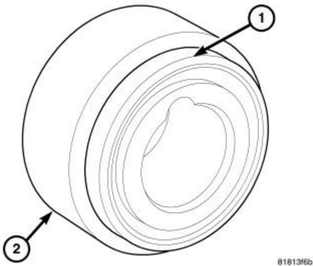
Fig. 264: Front Crankshaft Seal Installer Courtesy of CHRYSLER LLC
