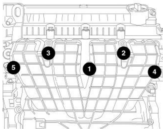
Fig. 367: Torque Sequence Courtesy of CHRYSLER LLC
