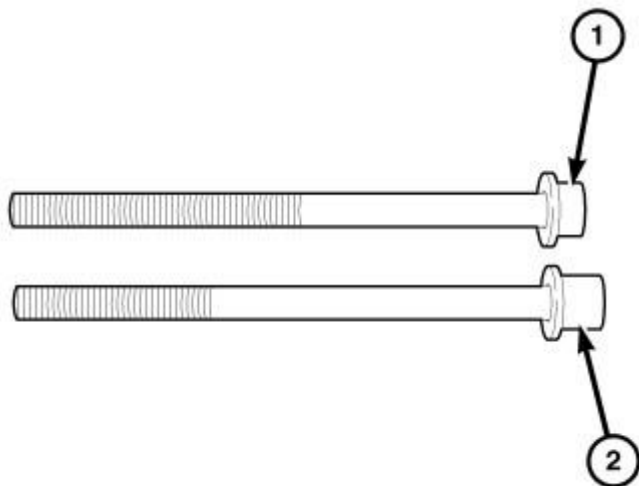
Fig. 116: Cylinder Head Bolt Identification Courtesy of CHRYSLER LLC
