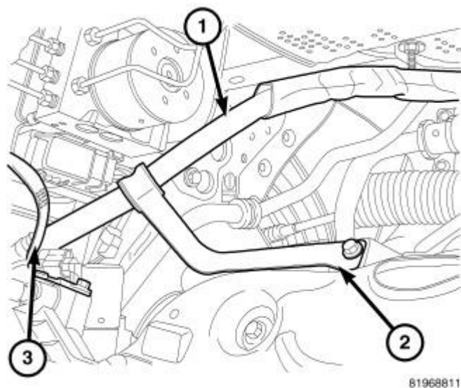
Fig. 20: P/S Hose Support - FWD Courtesy of CHRYSLER LLC
