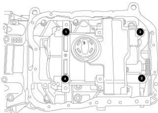
Fig. 322: BSM Torque Sequence
