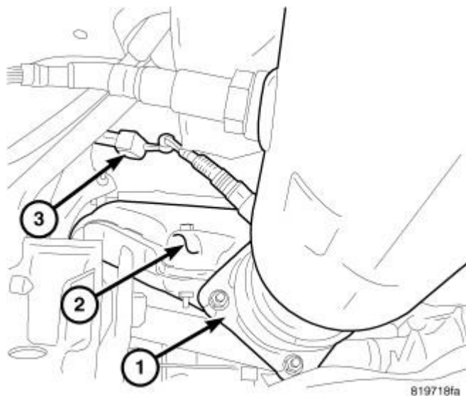
Fig. 342: Exhaust Pipe To Manifold Courtesy of CHRYSLER LLC
