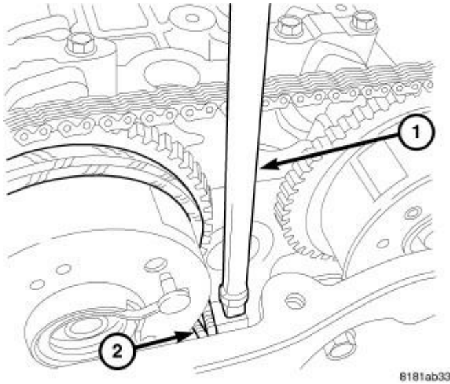
Fig. 155: Seating Wedge Tool Courtesy of CHRYSLER LLC
