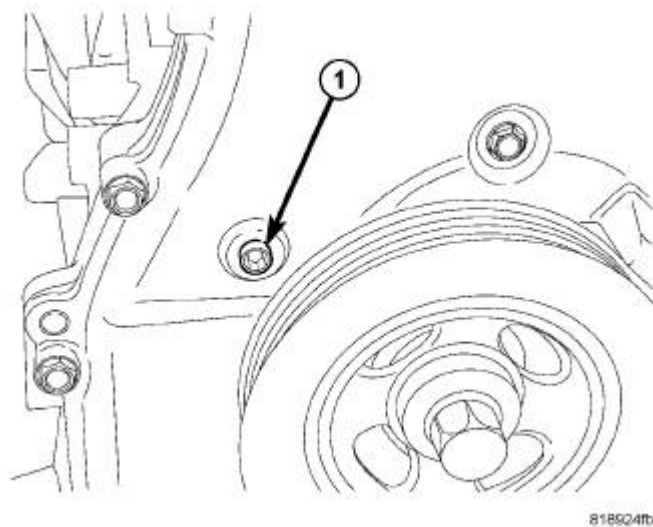
Fig. 152: Tensioner Access Plug Courtesy of CHRYSLER LLC
