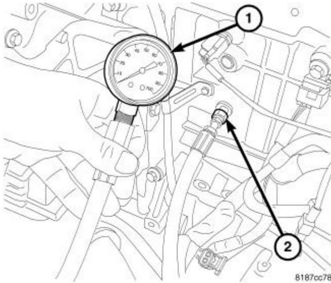
Fig. 280: Oil Pressure Gauge Courtesy of CHRYSLER LLC
