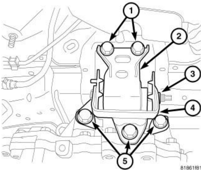
Fig. 194: Left Mount Courtesy of CHRYSLER LLC
