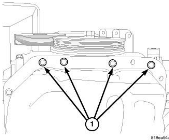
Fig. 399: Timing Chain Cover Lower Bolts Courtesy of CHRYSLER LLC
