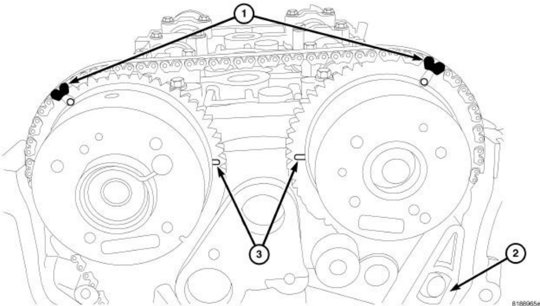
Fig. 376: Timing Chain Timing Marks Courtesy of CHRYSLER LLC
