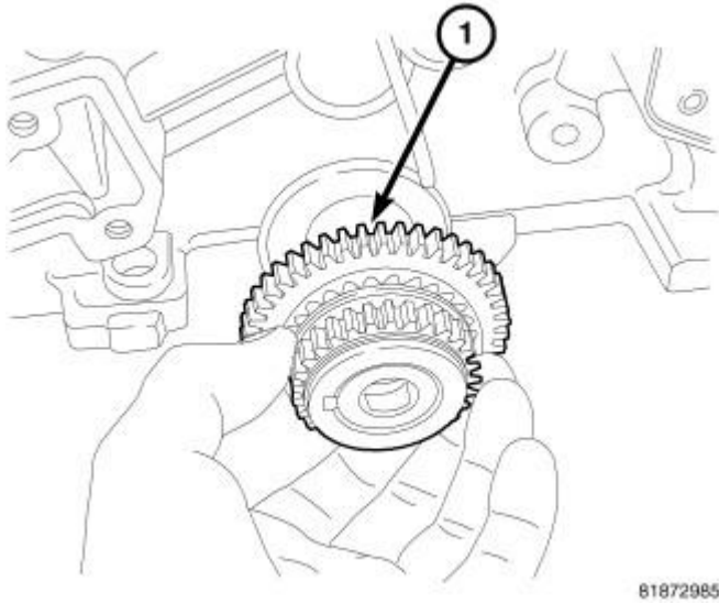
Fig. 379: Crankshaft Sprocket Courtesy of CHRYSLER LLC
