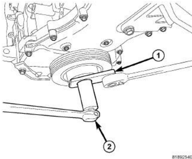
Fig. 43: Damper Removal Courtesy of CHRYSLER LLC
