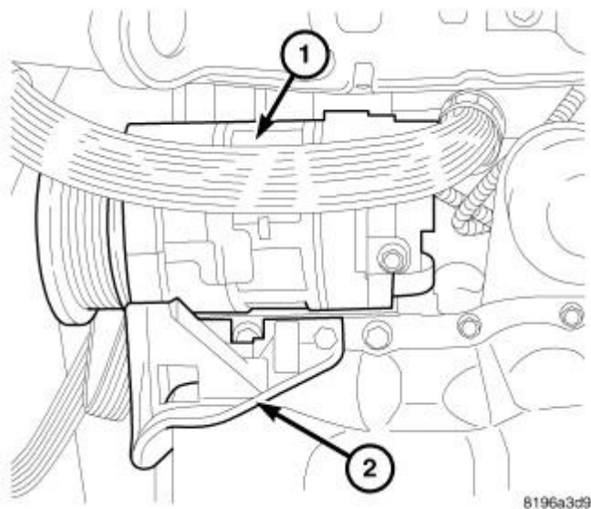
Fig. 396: A/C Compressor Courtesy of CHRYSLER LLC
