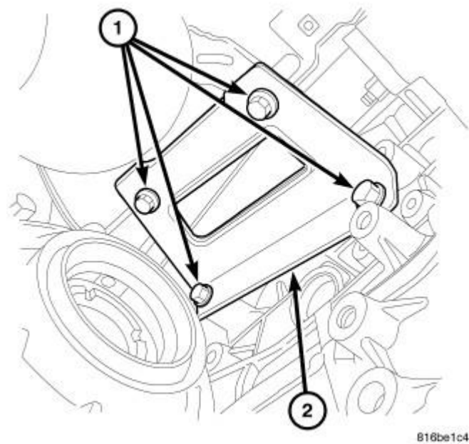
Fig. 348: Maniverter To Block Support Bracket Courtesy of CHRYSLER LLC
