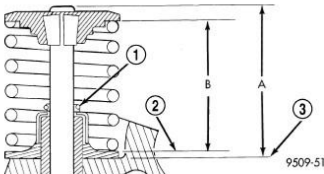
Fig. 189: Spring Installed Height & Valve Tip To Spring Seat Dimensions Courtesy of CHRYSLER LLC
