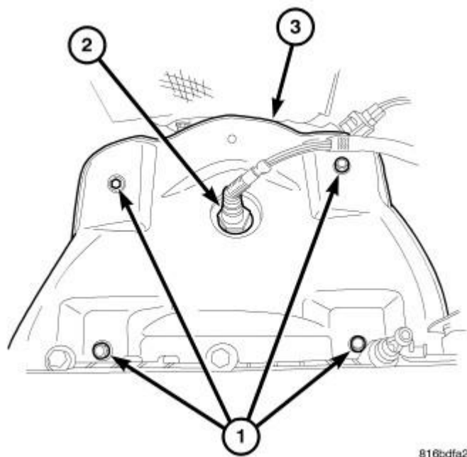
Fig. 350: Oxygen Sensor Courtesy of CHRYSLER LLC
