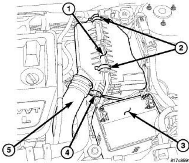
Fig. 421: Air Cleaner Housing Courtesy of CHRYSLER LLC
