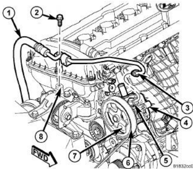
Fig. 392: Pressure Hose Courtesy of CHRYSLER LLC
