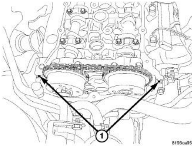
Fig. 179: Cylinder Head/Front Cover T-Joint Courtesy of CHRYSLER LLC
