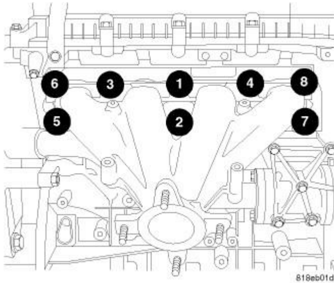
Fig. 344: Torque Sequence Courtesy of CHRYSLER LLC
