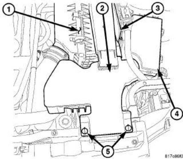
Fig. 353: Air Cleaner Inlet Courtesy of CHRYSLER LLC
