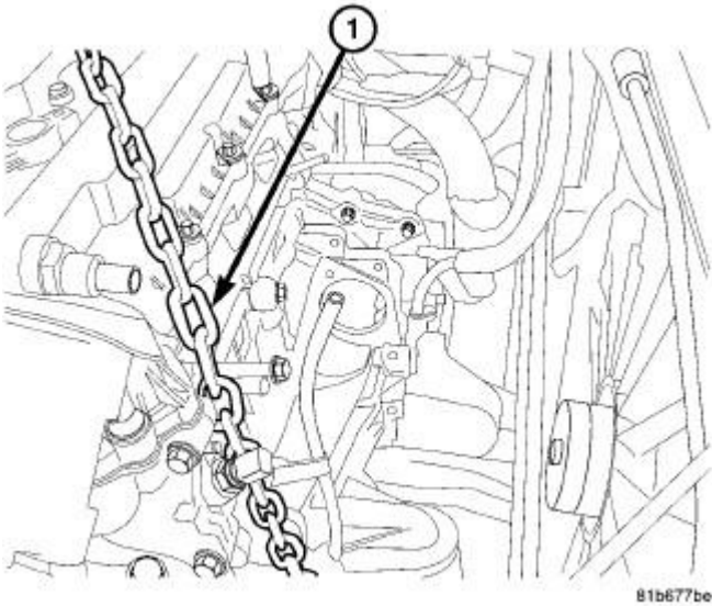
Fig. 33: Lift Chain
