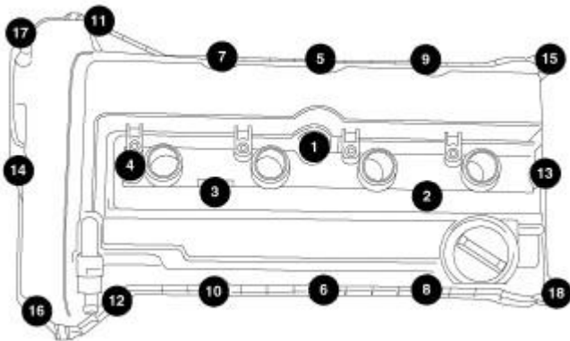
Fig. 172: Torque Sequence Courtesy of CHRYSLER LLC
