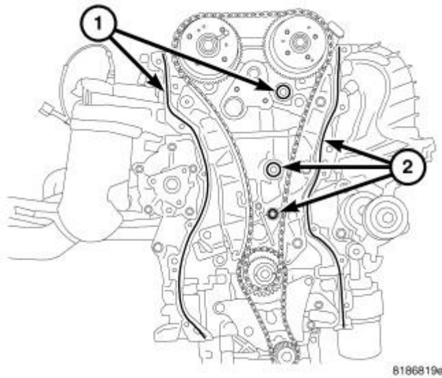
Fig. 408: Timing Chain Cover Sealing Courtesy of CHRYSLER LLC
