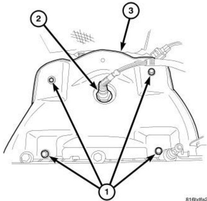
Fig. 335: Maniverter Heat Shield & Bolts Courtesy of CHRYSLER LLC
