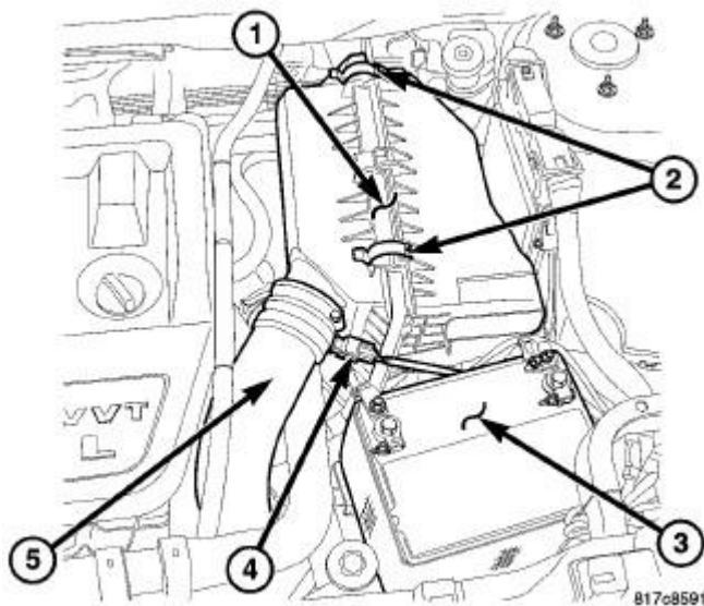
Fig. 370: Air Cleaner Housing Courtesy of CHRYSLER LLC
