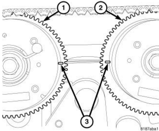
Fig. 374: Camshaft Timing Courtesy of CHRYSLER LLC
