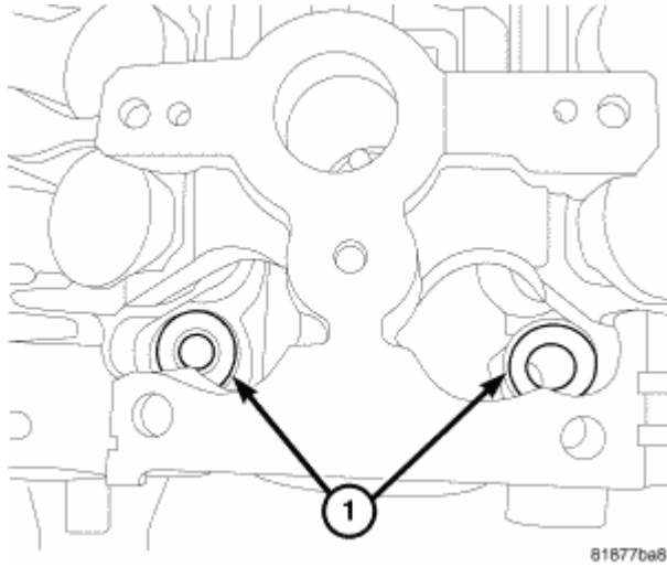
Fig. 101: Front Head Bolt Washers Courtesy of CHRYSLER LLC
