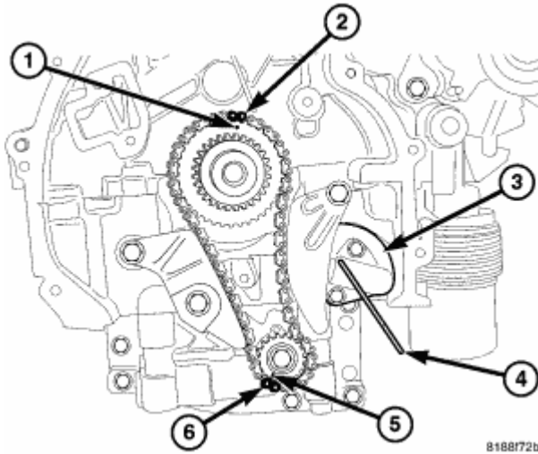
Fig. 411: BSM Tensioner Courtesy of CHRYSLER LLC
