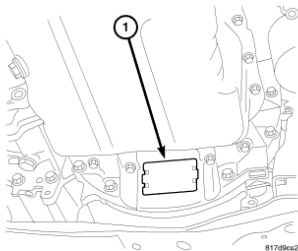
Fig. 26: Inspection Cover Courtesy of CHRYSLER LLC
