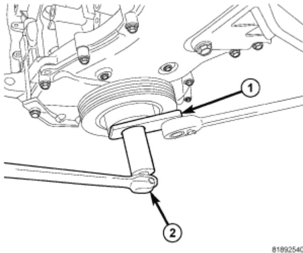
Fig. 222: Removing/Installing Damper Courtesy of CHRYSLER LLC
