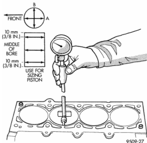
Fig. 193: Checking Cylinder Bore Size Courtesy of CHRYSLER LLC
