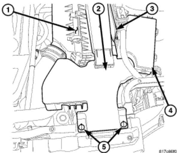
Fig. 73: Air Cleaner Housing Assembly Courtesy of CHRYSLER LLC
