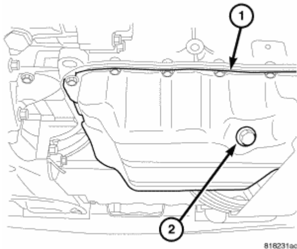
Fig. 231: Oil Drain Plug
