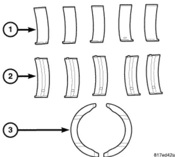
Fig. 209: Bearing Identification
