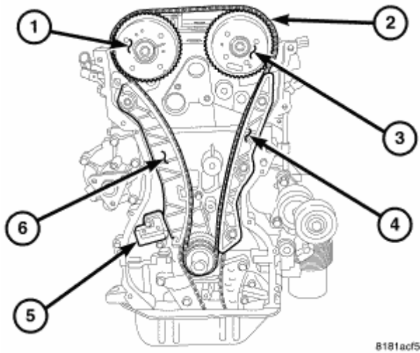
Fig. 371: TIMING DRIVE Courtesy of CHRYSLER LLC
