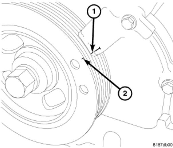
Fig. 402: TDC Courtesy of CHRYSLER LLC
