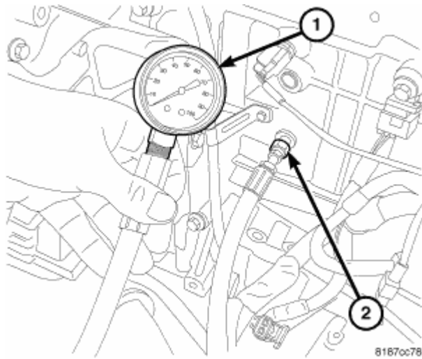
Fig. 262: Checking Engine Oil Pressure Courtesy of CHRYSLER LLC
