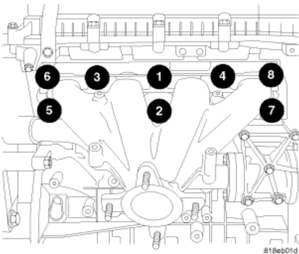
Fig. 353: Exhaust Manifold Bolt Torque Sequence Courtesy of CHRYSLER LLC
