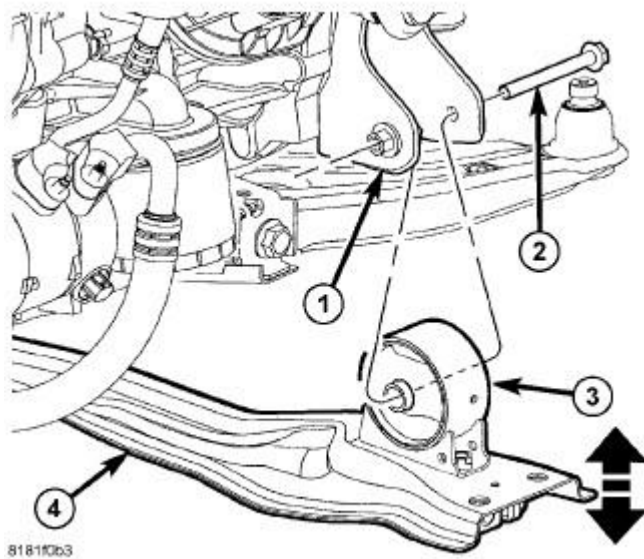
Fig. 345: Removing/Installing Fore/Aft Crossmember Courtesy of CHRYSLER LLC
