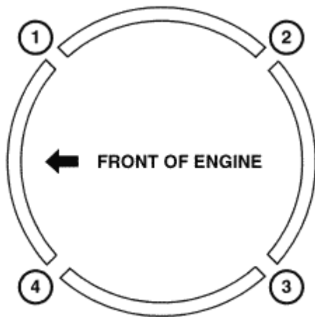
Fig. 248: Piston Ring End Gap Position Courtesy of CHRYSLER LLC
