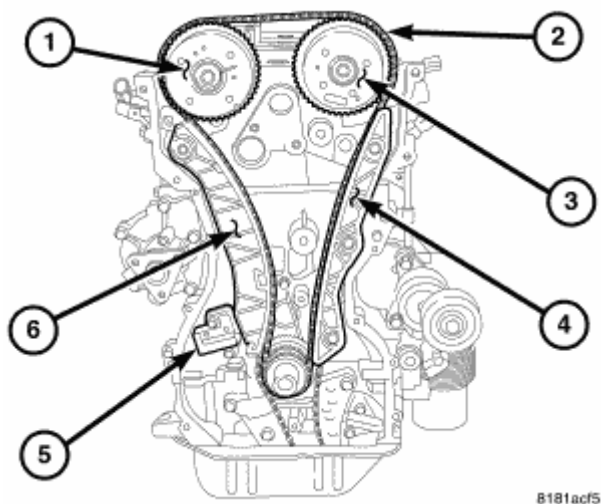
Fig. 424: TIMING DRIVE Courtesy of CHRYSLER LLC
