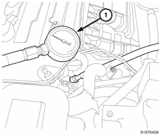
Fig. 258: Checking Engine Oil Pressure Courtesy of CHRYSLER LLC
