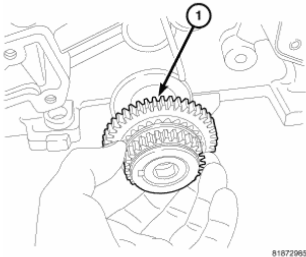
Fig. 201: Crankshaft Sprocket Courtesy of CHRYSLER LLC
