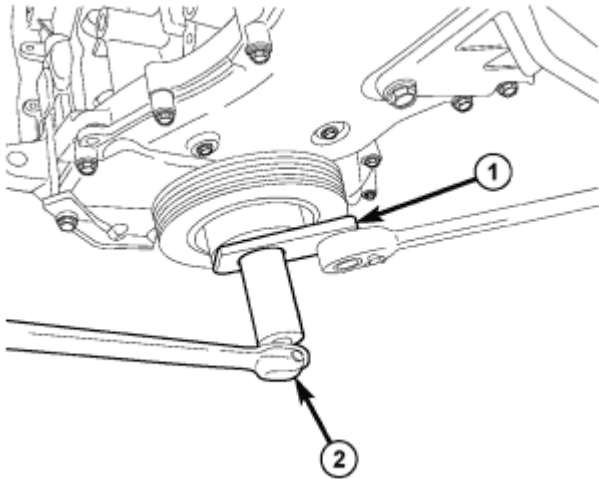
Fig. 250: Removing/Installing Damper Courtesy of CHRYSLER LLC
