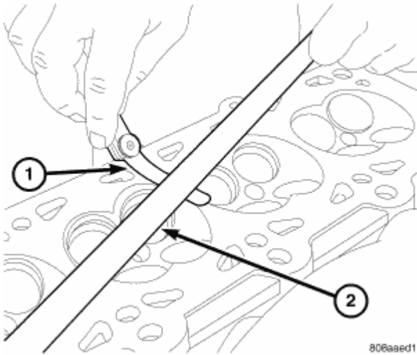
Fig. 102: Checking Cylinder Head Flatness
