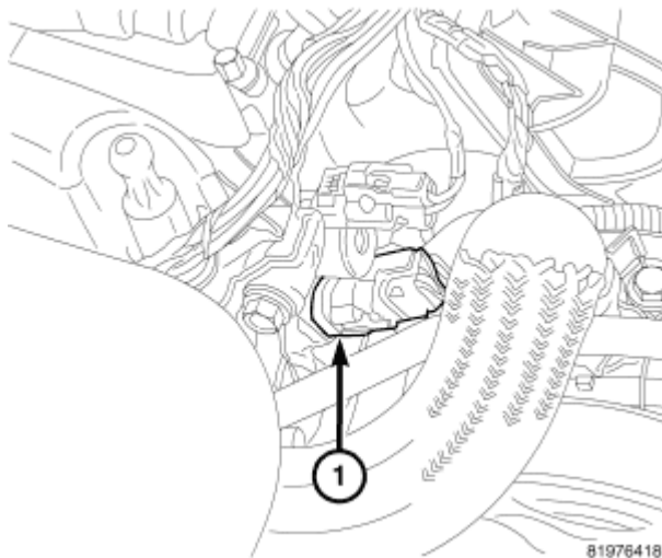
Fig. 260: Oil Temperature Sensor Courtesy of CHRYSLER LLC
