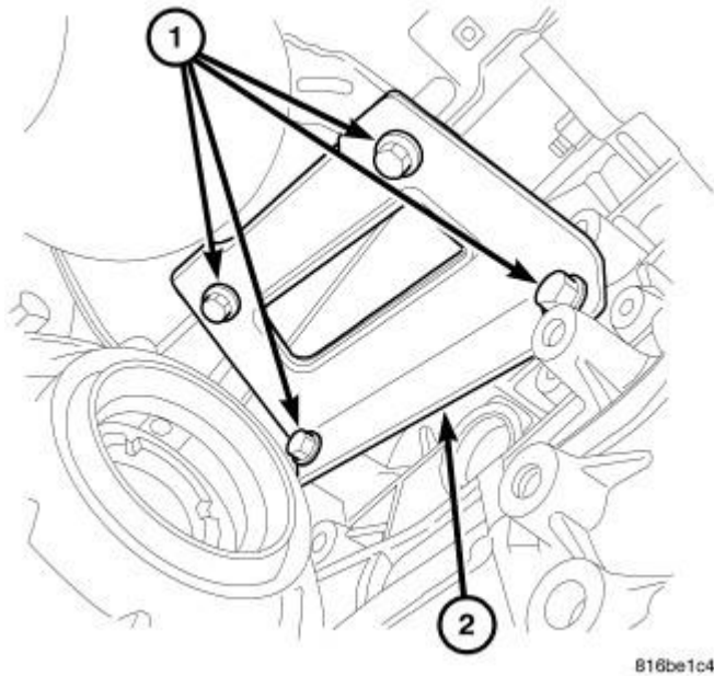
Fig. 344: Maniverter To Block Support Bracket Courtesy of CHRYSLER LLC
