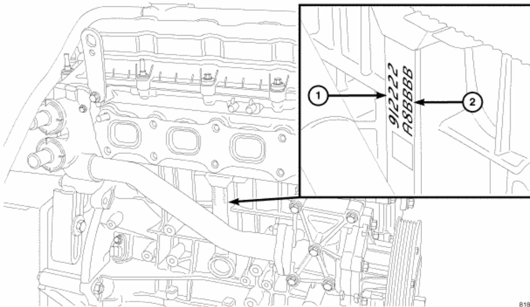
Fig. 227: Piston Identification
