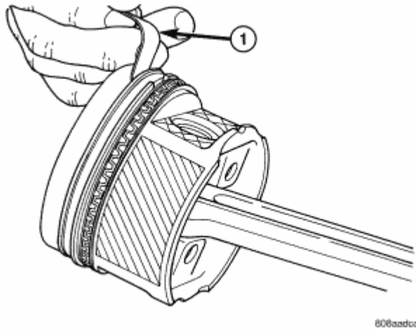
Fig. 245: Checking Ring-To-Groove Side Clearance Courtesy of CHRYSLER LLC
