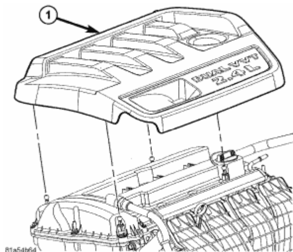
Fig. 329: Engine Cover Courtesy of CHRYSLER LLC
