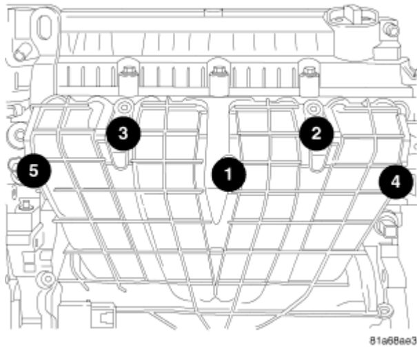
Fig. 47: Intake Manifold Bolt Torque Sequence Courtesy of CHRYSLER LLC
