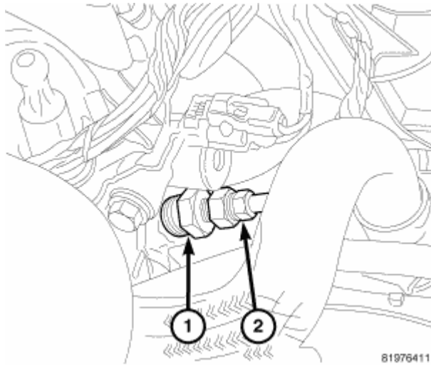
Fig. 257: Threaded Adapter 9879 Courtesy of CHRYSLER LLC
