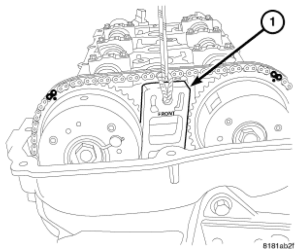
Fig. 147: Wedge Tool Courtesy of CHRYSLER LLC
