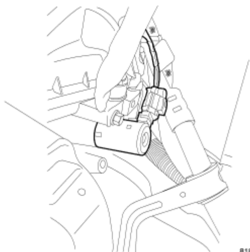
Fig. 284: Variable Valve Timing Solenoid Connector Courtesy of CHRYSLER LLC
