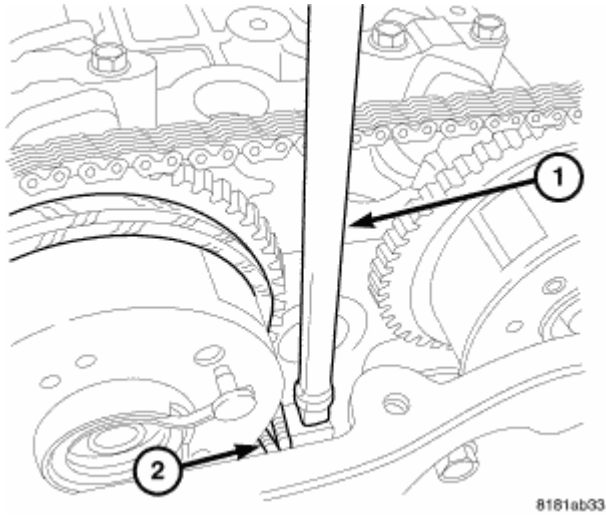
Fig. 133: Seating Wedge Tool Courtesy of CHRYSLER LLC
