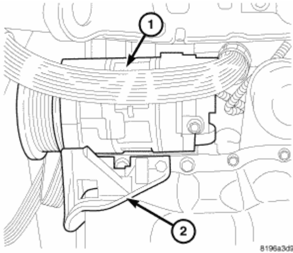
Fig. 378: A/C Compressor Courtesy of CHRYSLER LLC
