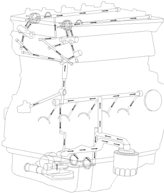
Fig. 255: OIL FLOW DIAGRAM Courtesy of CHRYSLER LLC
