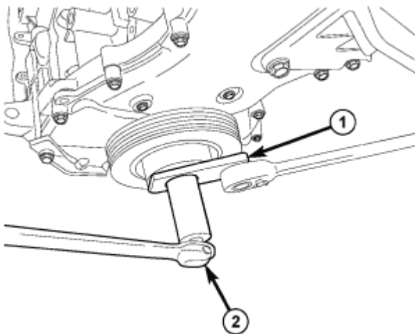
Fig. 249: Removing/Installing Damper Courtesy of CHRYSLER LLC
