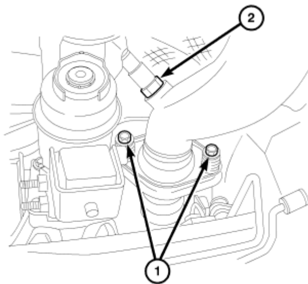
Fig. 39: Exhaust To Maniverter Bolts Courtesy of CHRYSLER LLC
