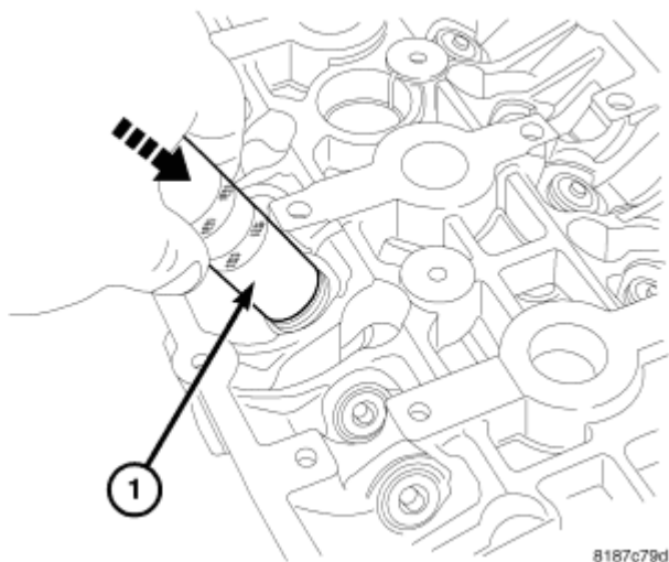
Fig. 167: Removing Valve Keepers Courtesy of CHRYSLER LLC
