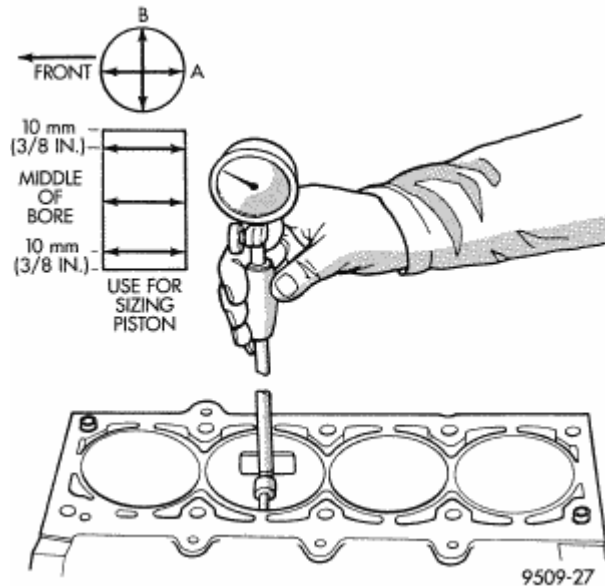
Fig. 229: Checking Cylinder Bore Size Courtesy of CHRYSLER LLC
