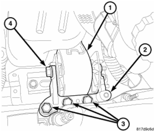
Fig. 184: Right Mount Courtesy of CHRYSLER LLC
