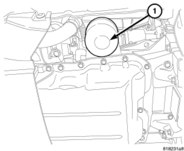
Fig. 266: Oil Filter
