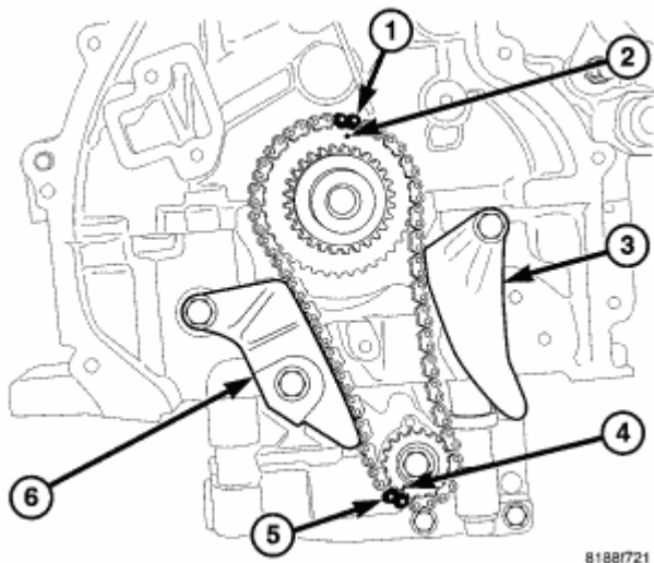
Fig. 300: Aligning Marks On Sprockets & Chain Courtesy of CHRYSLER LLC
