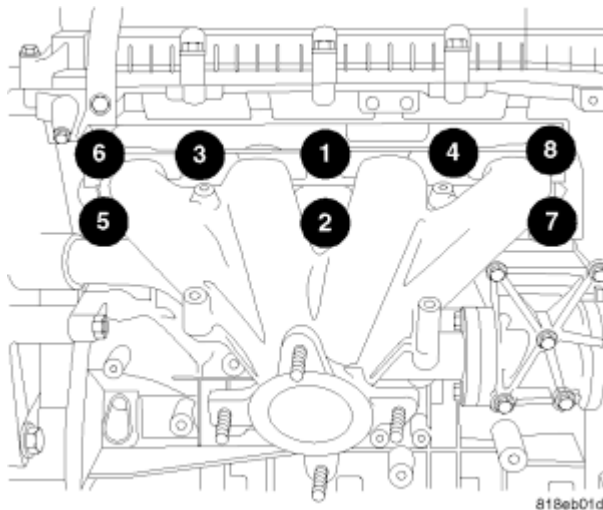
Fig. 334: Exhaust Manifold Bolt Torque Sequence Courtesy of CHRYSLER LLC
