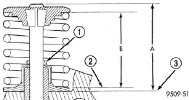
Fig. 170: Checking Spring Installed Height & Valve Tip To Spring Seat Dimensions Courtesy of CHRYSLER LLC
