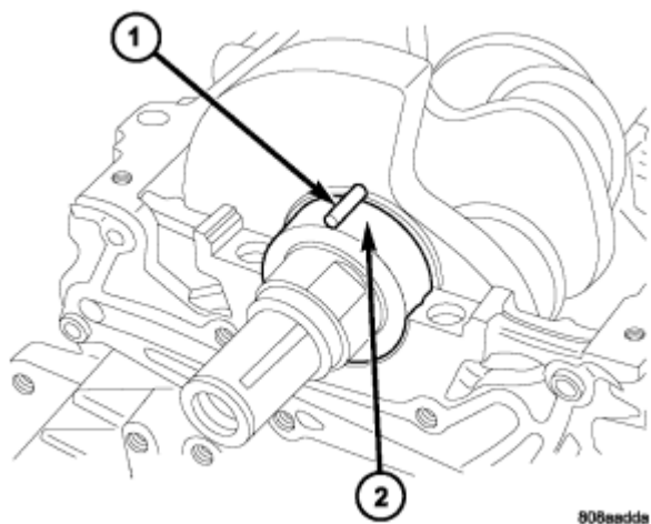
Fig. 6: Identifying Plastigage Courtesy of CHRYSLER LLC
