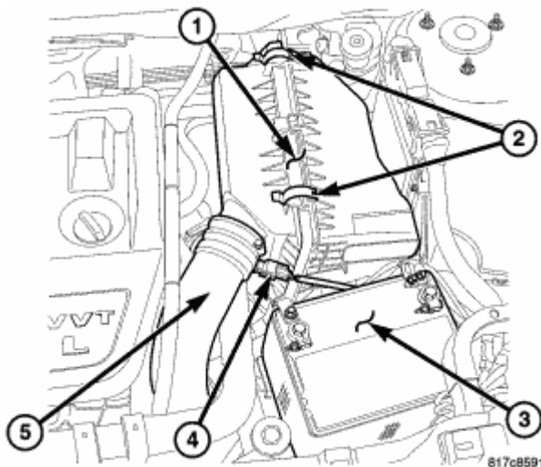
Fig. 10: Air Cleaner Housing Courtesy of CHRYSLER LLC
