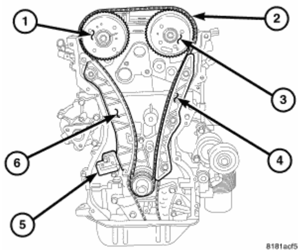
Fig. 414: Timing Drive Courtesy of CHRYSLER LLC
