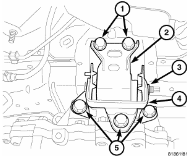
Fig. 177: Left Mount Courtesy of CHRYSLER LLC
