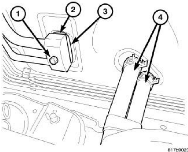
Fig. 320: Refrigerant Lines To Evaporator Bolt Courtesy of CHRYSLER LLC
