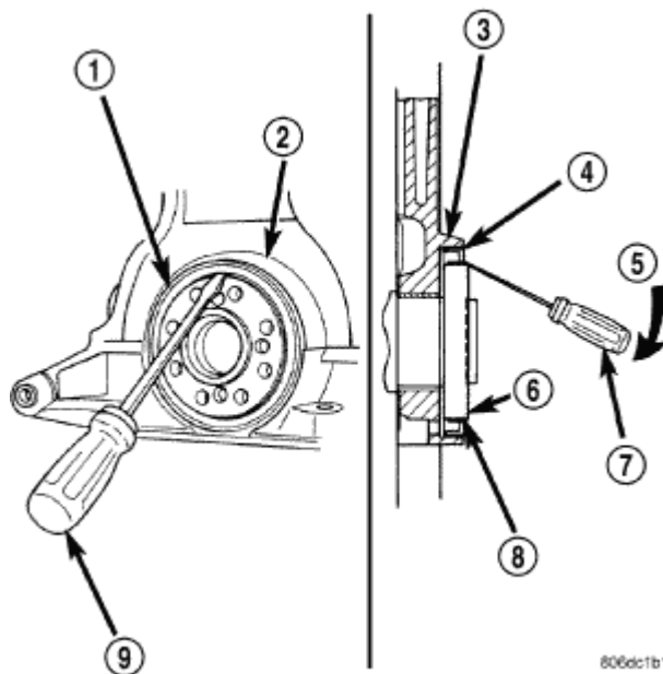
Fig. 224: Rear Crankshaft Oil Seal - Removal
