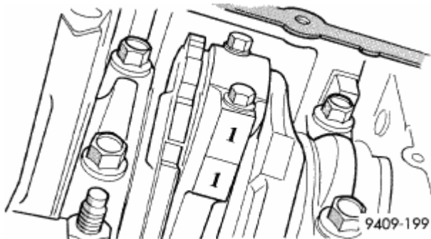
Fig. 233: Identify Connecting Rod to Cylinder-Typical Courtesy of CHRYSLER LLC
