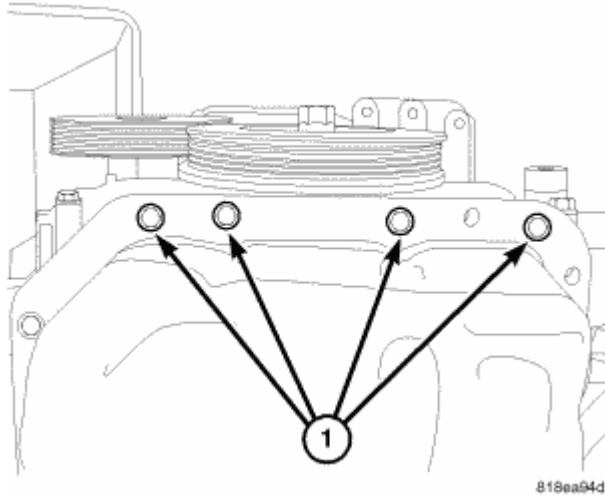
Fig. 380: Timing Chain Cover Lower Bolts Courtesy of CHRYSLER LLC
