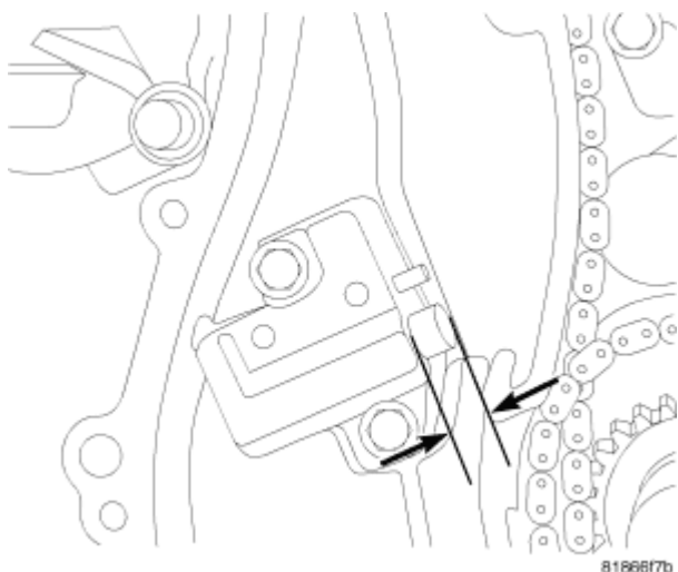
Fig. 406: Checking Timing Chain Stretch Courtesy of CHRYSLER LLC
