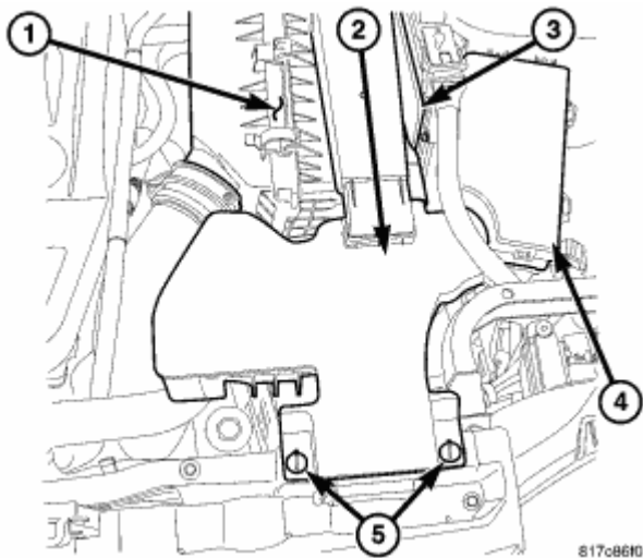
Fig. 175: Air Cleaner Housing Assembly Courtesy of CHRYSLER LLC
