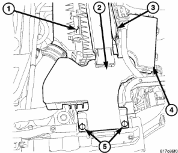
Fig. 399: Air Cleaner Inlet Courtesy of CHRYSLER LLC
