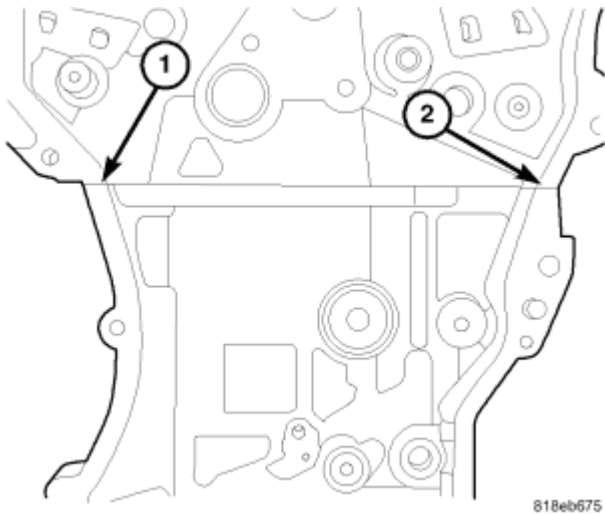
Fig. 386: Front Cover Upper T-Joints Courtesy of CHRYSLER LLC
