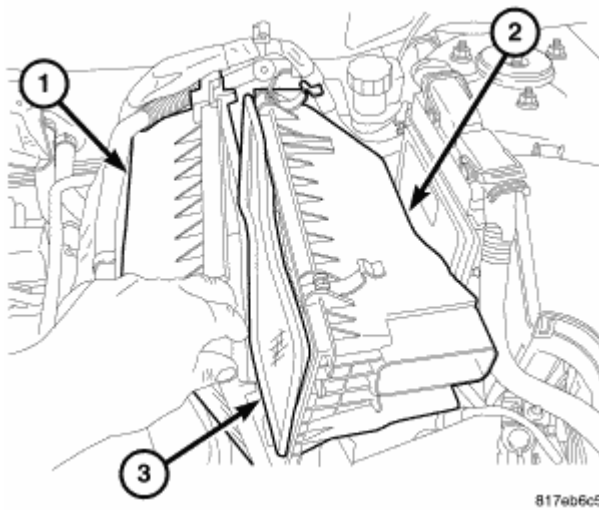
Fig. 75: Air Filter Element Courtesy of CHRYSLER LLC
