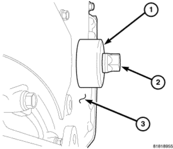
Fig. 221: Front Seal Installed Courtesy of CHRYSLER LLC
