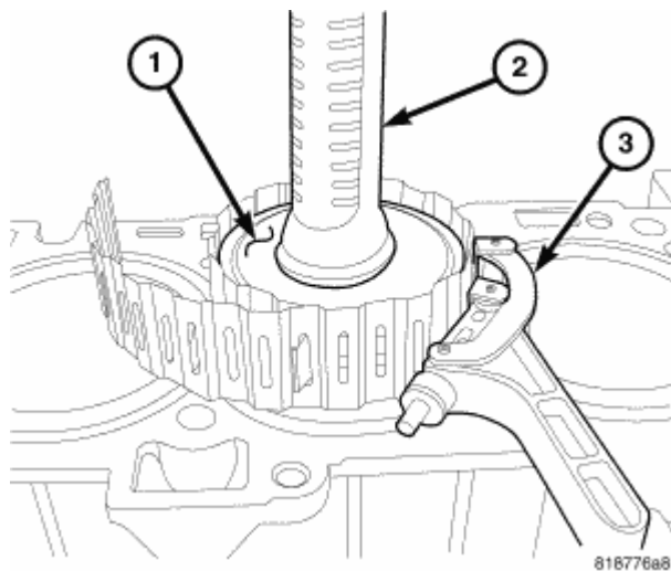
Fig. 236: Ring Compressor Courtesy of CHRYSLER LLC
