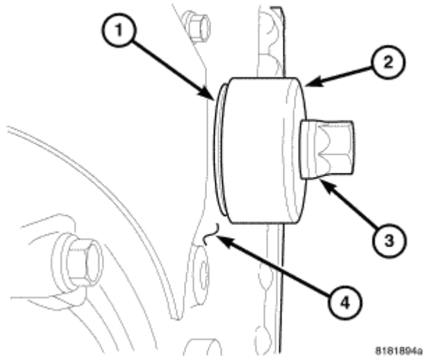
Fig. 220: Installing Front Seal Courtesy of CHRYSLER LLC
