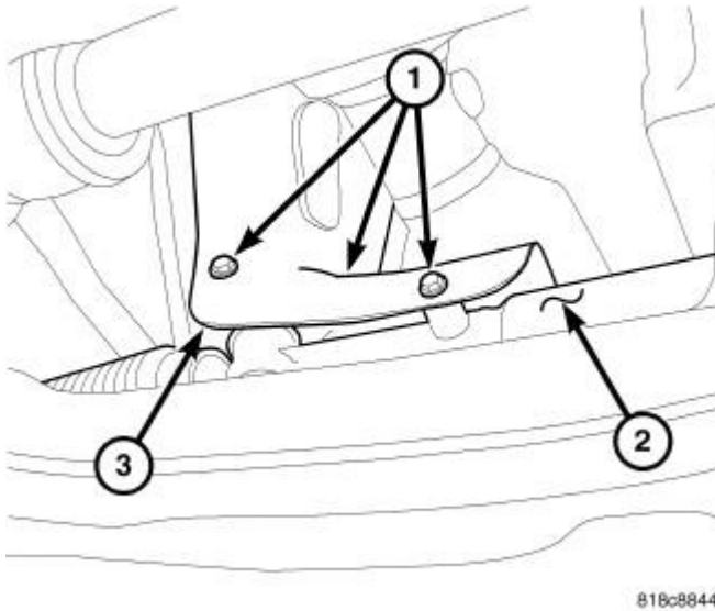
Fig. 346: Removing/Installing Bolts Securing Steering Gear Heat Shield Courtesy of CHRYSLER LLC
