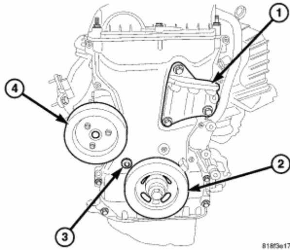
Fig. 383: Engine Front Courtesy of CHRYSLER LLC
