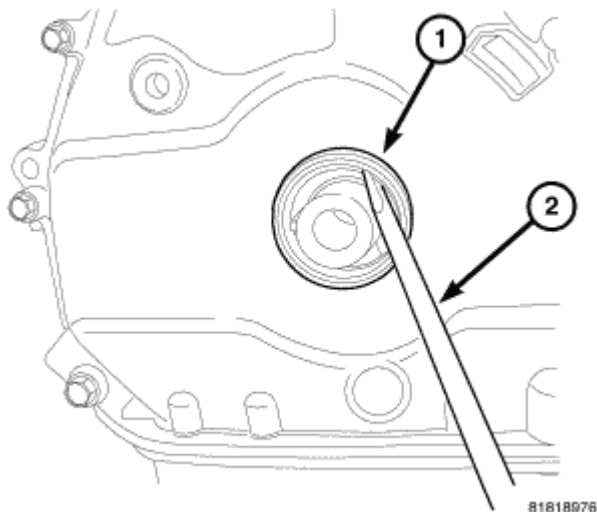
Fig. 218: Front Crankshaft Seal Removal Courtesy of CHRYSLER LLC
