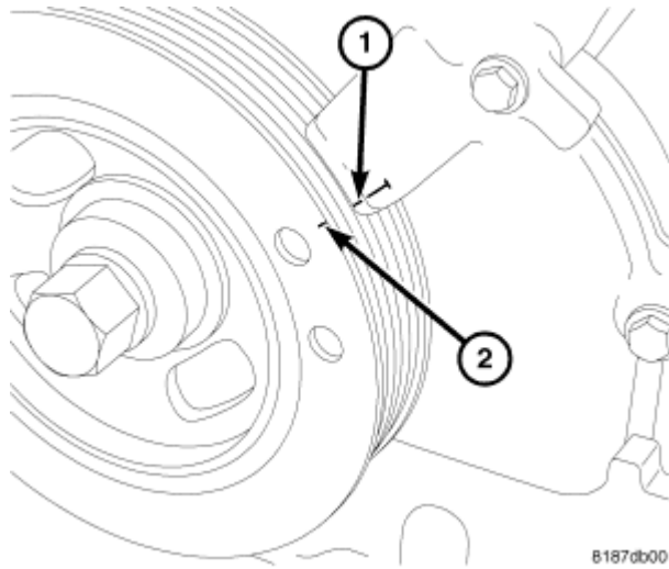
Fig. 422: TDC Courtesy of CHRYSLER LLC
