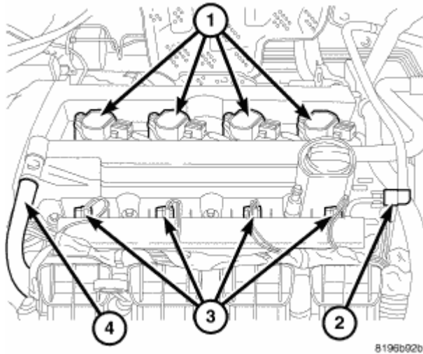
Fig. 85: Coil Connector Courtesy of CHRYSLER LLC
