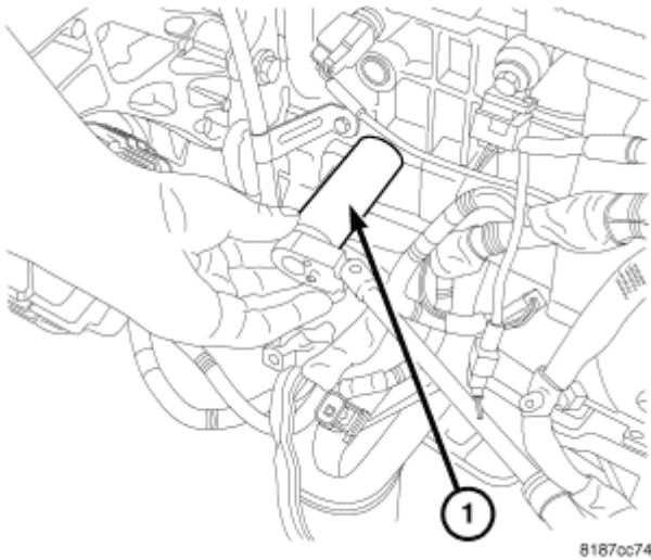
Fig. 304: Oil Pressure Sensor Courtesy of CHRYSLER LLC
