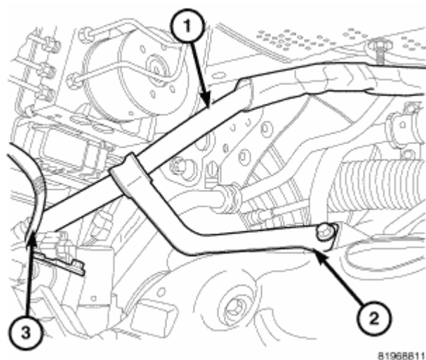
Fig. 46: P/S Hose Support-FWD Courtesy of CHRYSLER LLC
