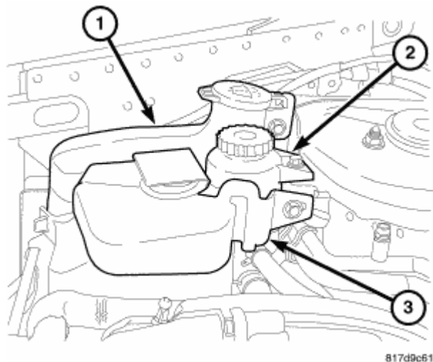
Fig. 375: Coolant Reservoir
