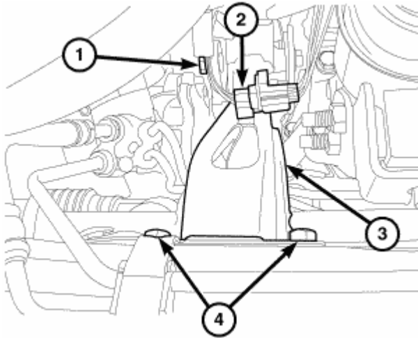
Fig. 190: Rear Mount
