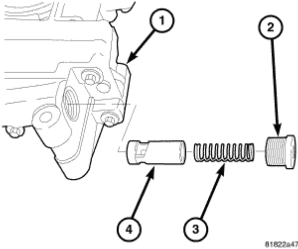
Fig. 293: View Of Pressure Regulating Valve Courtesy of CHRYSLER LLC
