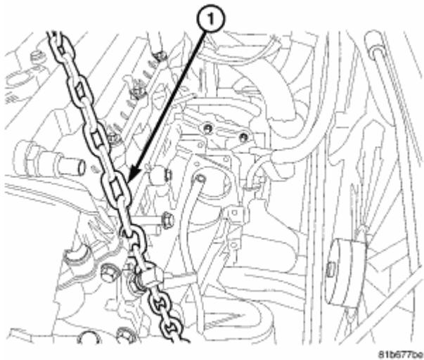
Fig. 30: Lift Chain Courtesy of CHRYSLER LLC
