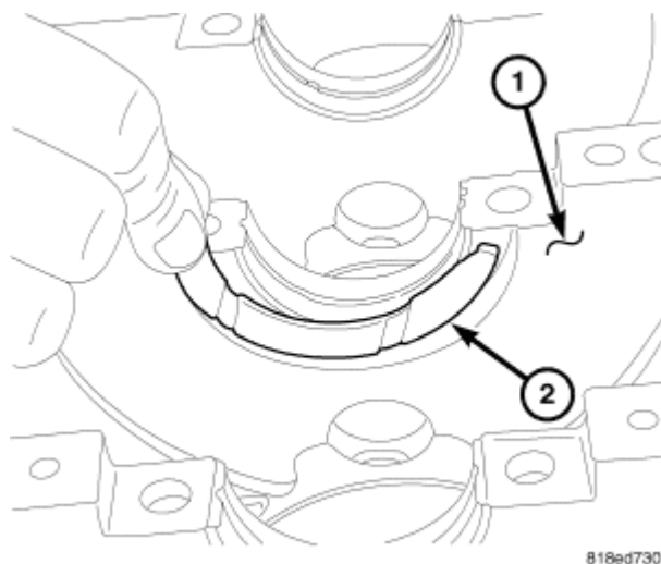
Fig. 208: Installing Thrust Bearing
