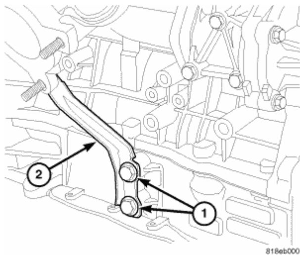
Fig. 355: Exhaust Manifold Support Bracket Courtesy of CHRYSLER LLC
