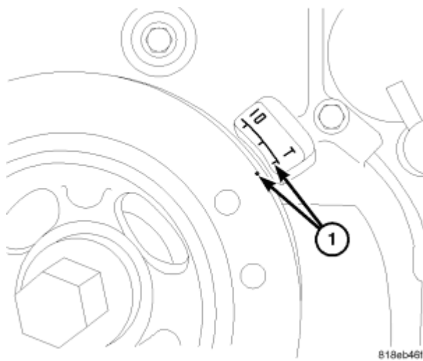
Fig. 377: TDC Courtesy of CHRYSLER LLC
