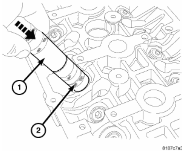
Fig. 169: Valve Installation Courtesy of CHRYSLER LLC
