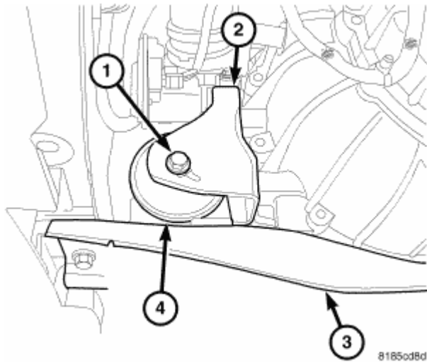
Fig. 187: Front Mount Courtesy of CHRYSLER LLC
