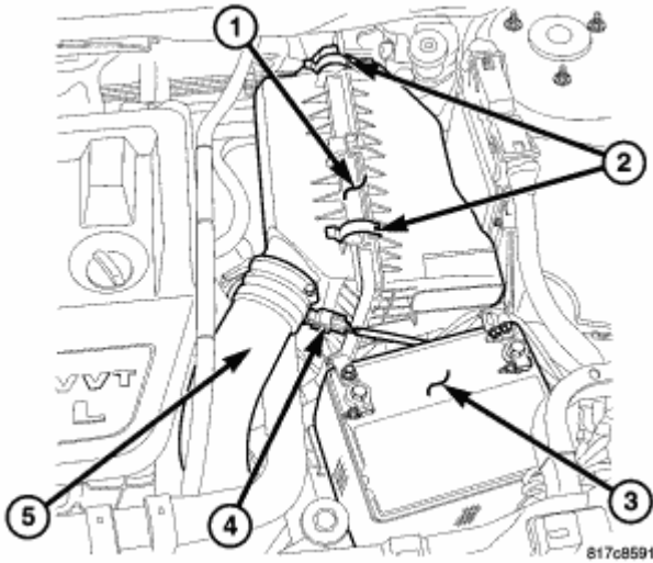
Fig. 83: Air Cleaner Housing Courtesy of CHRYSLER LLC
