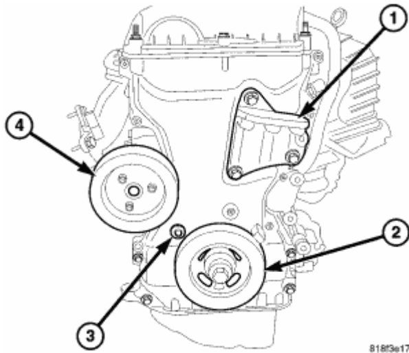
Fig. 88: Engine Front Courtesy of CHRYSLER LLC
