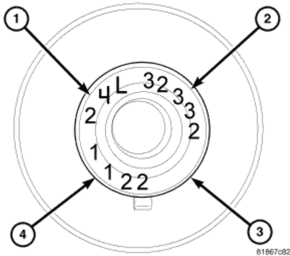
Fig. 241: Connecting Rod Bearing Identification Courtesy of CHRYSLER LLC
