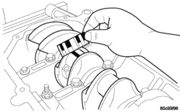
Fig. 242: Connecting Rod Bearing Clearance - Typical Courtesy of CHRYSLER LLC
