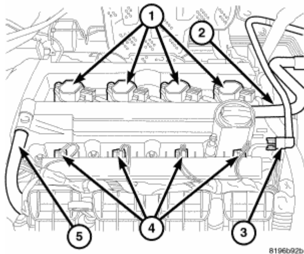
Fig. 8: Coil Connector Courtesy of CHRYSLER LLC
