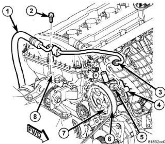
Fig. 337: Power Steering Assembly Components Courtesy of CHRYSLER LLC
