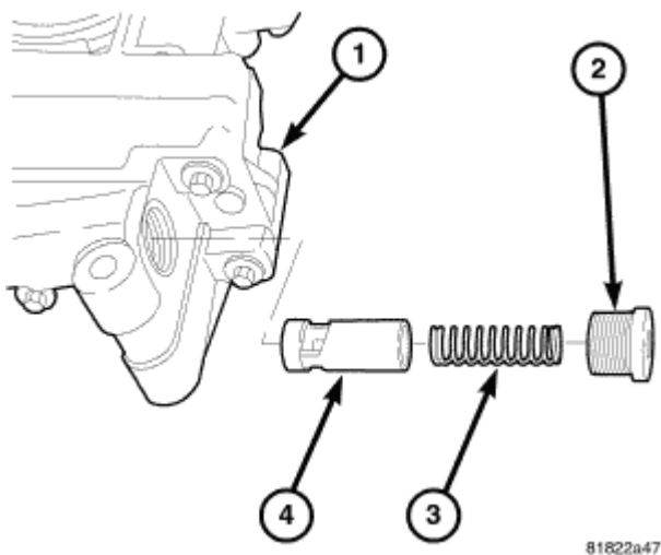
Fig. 292: View Of Pressure Regulating Valve Courtesy of CHRYSLER LLC
