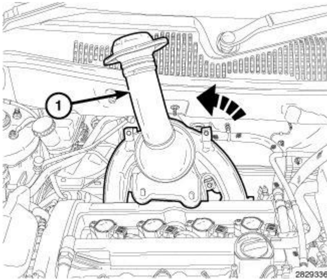
Fig. 328: Rotating Maniverter Counterclockwise Courtesy of CHRYSLER LLC
