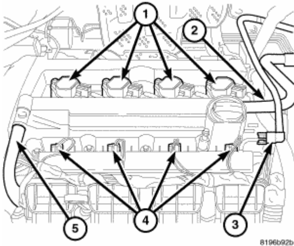
Fig. 397: Coil Connector Courtesy of CHRYSLER LLC
