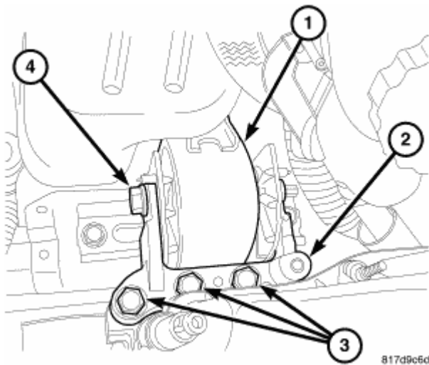
Fig. 34: Right Engine Mount
