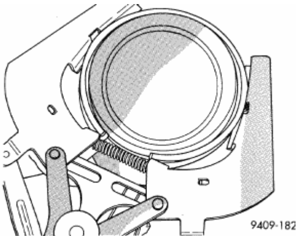
Fig. 246: Ring Expander Courtesy of CHRYSLER LLC
