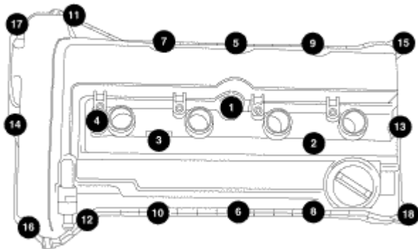
Fig. 157: Cylinder Head Cover Bolt Torque Sequence Courtesy of CHRYSLER LLC
