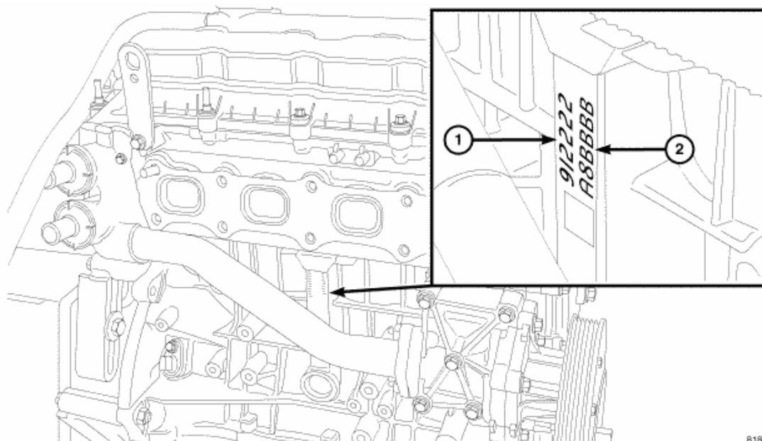
Fig. 240: Upper Main Bearing Shell Identification Courtesy of CHRYSLER LLC
