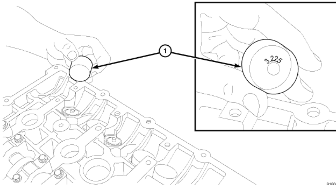
Fig. 163: Tappet Identification Courtesy of CHRYSLER LLC
