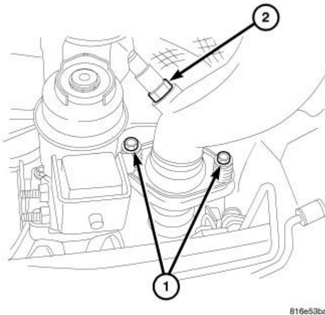
Fig. 316: Exhaust To Manifold Bolts
