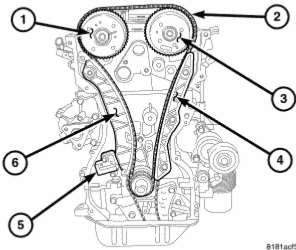
Fig. 423: TIMING DRIVE Courtesy of CHRYSLER LLC
