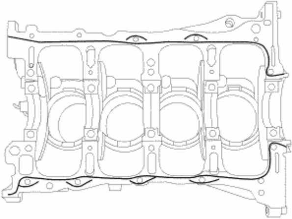
Fig. 253: Bead Of Sealant
