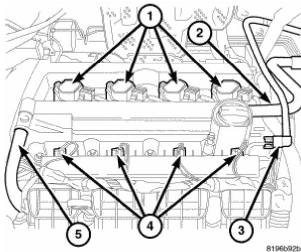
Fig. 126: Coil Connector Courtesy of CHRYSLER LLC
