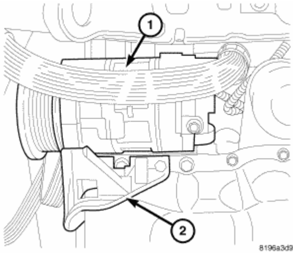
Fig. 28: A/C Compressor
