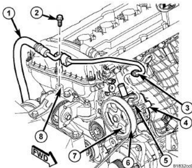
Fig. 326: Power Steering Assembly Components Courtesy of CHRYSLER LLC
