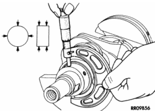
Fig. 205: Checking Crankshaft Main Journal Courtesy of CHRYSLER LLC
