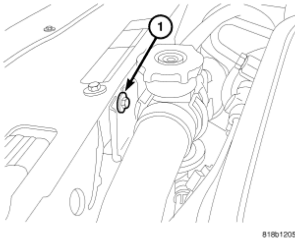
Fig. 99: Radiator Hose Support Courtesy of CHRYSLER LLC
