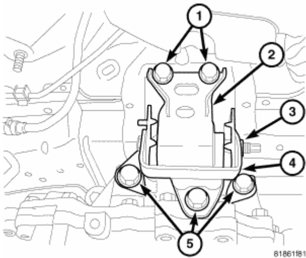
Fig. 178: Left Mount Courtesy of CHRYSLER LLC
