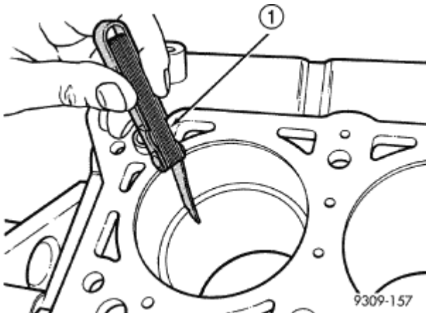
Fig. 244: Checking Ring Gap Courtesy of CHRYSLER LLC
