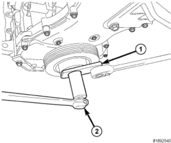
Fig. 217: Removing/Installing Damper Courtesy of CHRYSLER LLC
