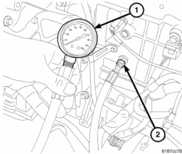
Fig. 263: Checking Engine Oil Pressure Courtesy of CHRYSLER LLC
