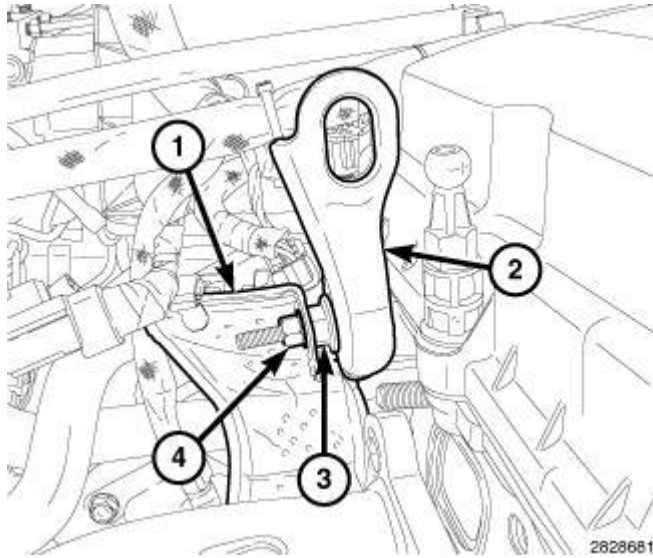
Fig. 340: Heatshield, Stud Bolt, Engine Lift Bracket & Nut Courtesy of CHRYSLER LLC
