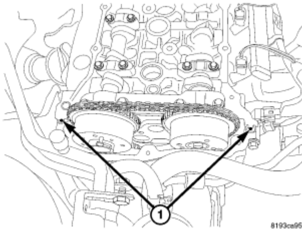
Fig. 156: Cylinder Head/Front Cover T-Joints Courtesy of CHRYSLER LLC
