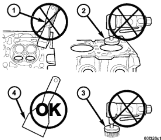
Fig. 5: PROPER TOOL USAGE FOR SURFACE PREPARATION
