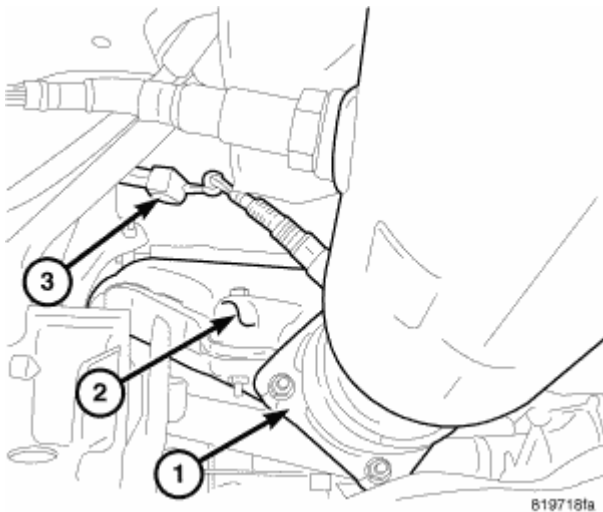
Fig. 332: CAT At Exhaust Manifold Courtesy of CHRYSLER LLC
