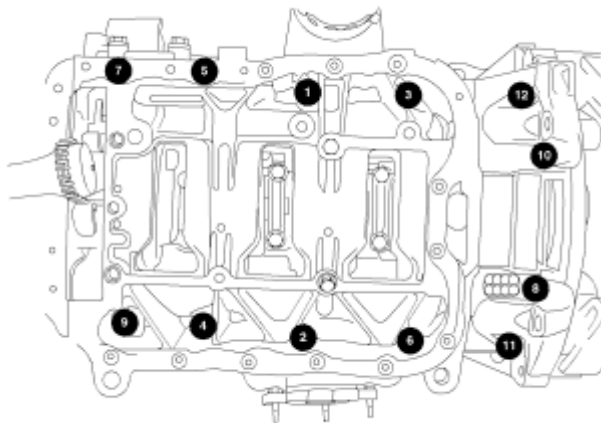
Fig. 254: Ladder Frame Torque Sequence
