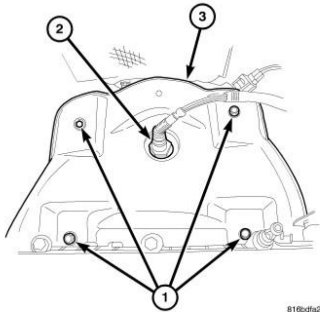
Fig. 350: Maniverter Heat Shield And Bolts Courtesy of CHRYSLER LLC
