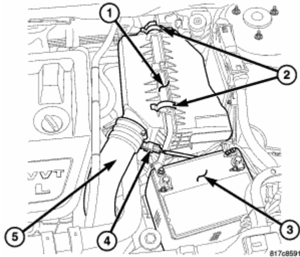
Fig. 369: Air Cleaner Housing Courtesy of CHRYSLER LLC
