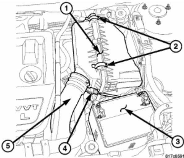
Fig. 81: Air Cleaner Housing Courtesy of CHRYSLER LLC
