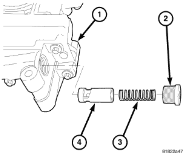
Fig. 291: View Of Pressure Regulating Valve Courtesy of CHRYSLER LLC
