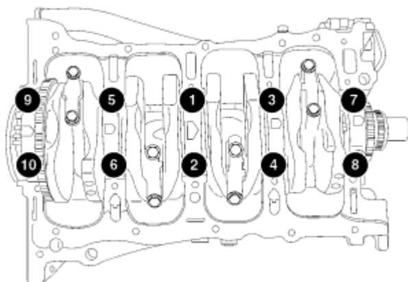
Fig. 211: Main Bearing Cap Torque Sequence
