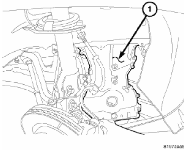
Fig. 390: Timing Chain Cover Removal Courtesy of CHRYSLER LLC
