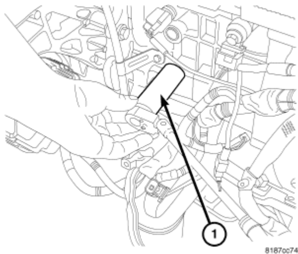
Fig. 264: Oil Pressure Sensor Courtesy of CHRYSLER LLC
