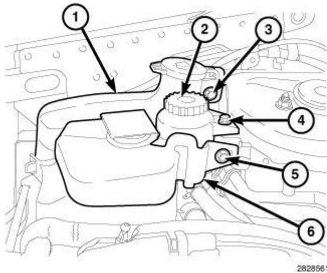
Fig. 325: Coolant Reservoir, Power Steering Fluid Reservoir, Washer Fluid Reservoir & Bolts Courtesy of CHRYSLER LLC
