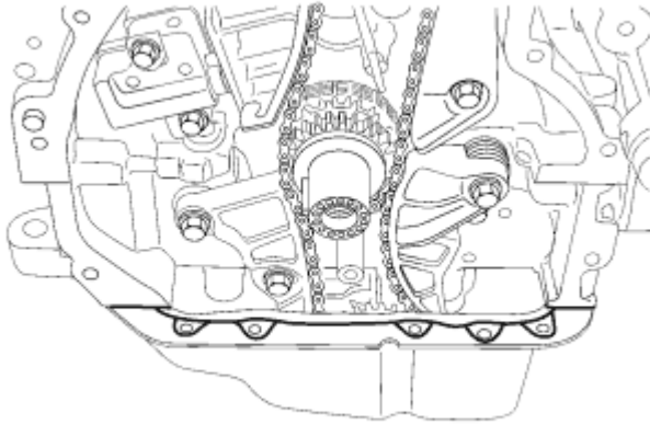
Fig. 388: Sealing Oil Pan Courtesy of CHRYSLER LLC
