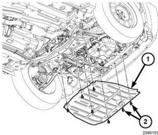
Fig. 349: Removal/Installation Front Skid Plate And Bolts
