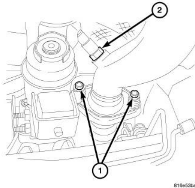
Fig. 347: Exhaust To Maniverter Bolts Courtesy of CHRYSLER LLC
