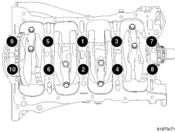
Fig. 204: Main Bearing Cap Torque Sequence Courtesy of CHRYSLER LLC
