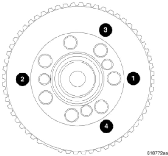
Fig. 207: Target Wheel Courtesy of CHRYSLER LLC
