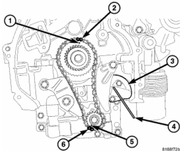
Fig. 302: Timing Chain Mark & Tensioner Pin Courtesy of CHRYSLER LLC
