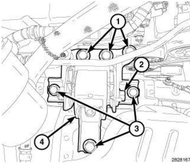
Fig. 327: Engine Mount Isolator, Right Engine Mount & Engine Mount Bracket Retaining Bolts Courtesy of CHRYSLER LLC
