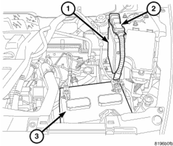
Fig. 179: Battery, Negative Battery Cable & PCM Courtesy of CHRYSLER LLC
