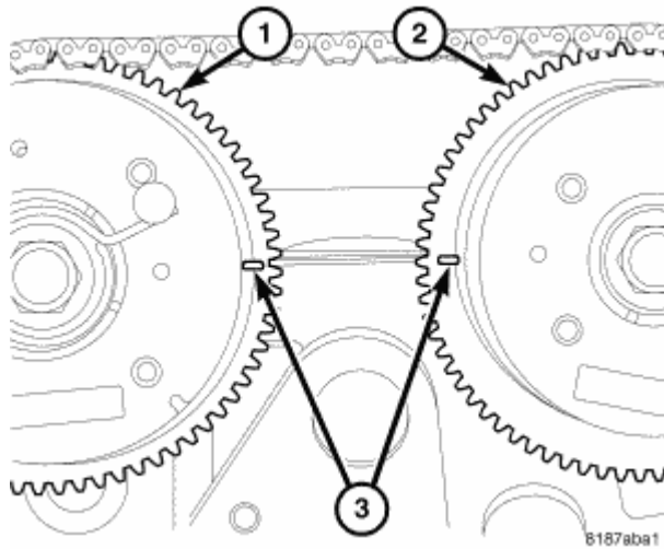
Fig. 413: Camshaft Timing Courtesy of CHRYSLER LLC
