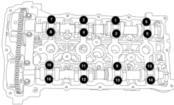
Fig. 150: CAM Cap Torque Sequence Courtesy of CHRYSLER LLC
