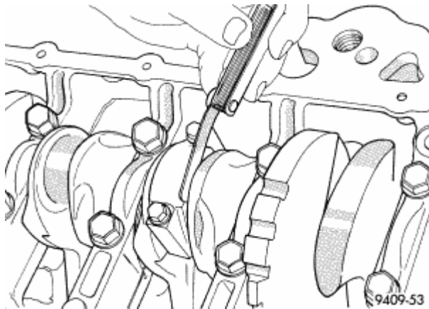
Fig. 237: Connecting Rod Side Clearance Courtesy of CHRYSLER LLC
