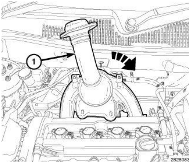
Fig. 335: Rotating Maniverter Clockwise Courtesy of CHRYSLER LLC
