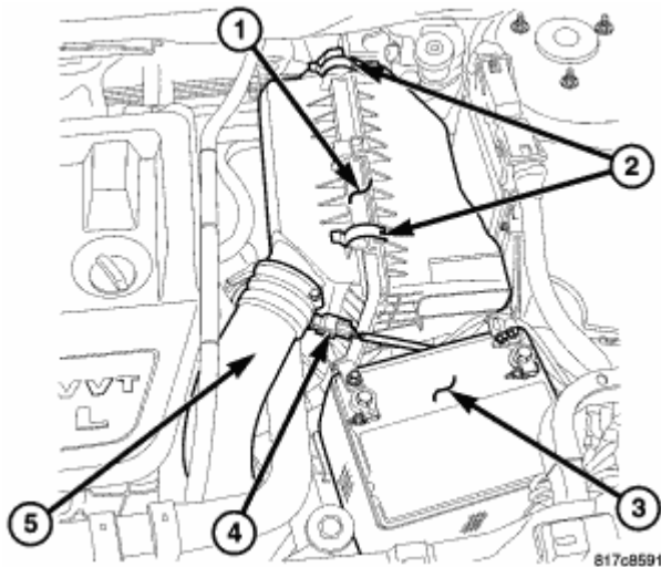
Fig. 122: Air Cleaner Housing Courtesy of CHRYSLER LLC
