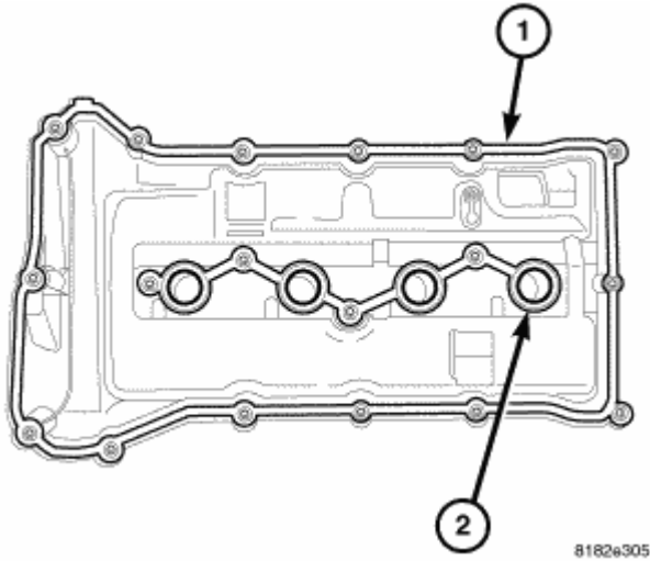
Fig. 154: Gasket Location
