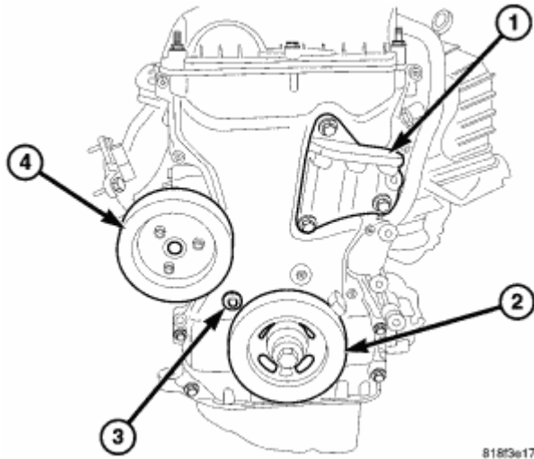
Fig. 379: Engine Front Courtesy of CHRYSLER LLC
