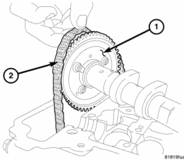
Fig. 137: Lifting Timing Chain Off Sprocket Courtesy of CHRYSLER LLC
