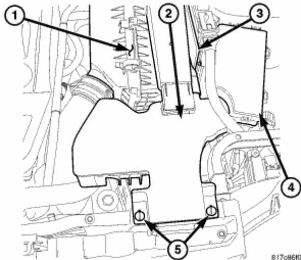
Fig. 180: Air Cleaner Housing Assembly Courtesy of CHRYSLER LLC
