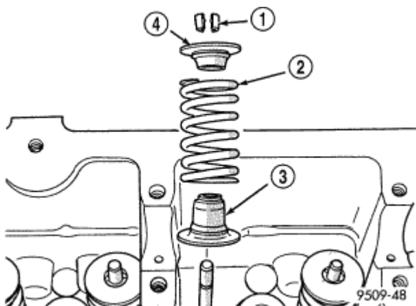
Fig. 171: Valve Stem Seal/Valve Spring Seat Courtesy of CHRYSLER LLC
