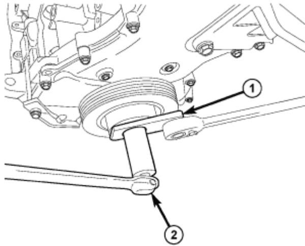
Fig. 43: Damper Removal Courtesy of CHRYSLER LLC
