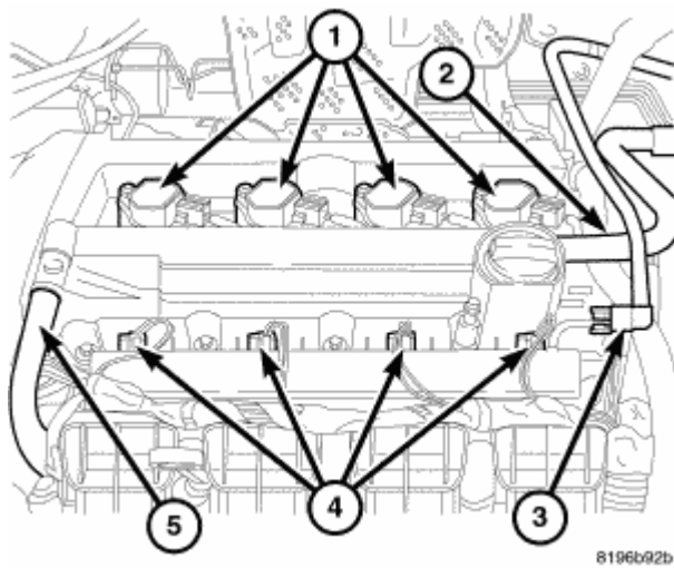
Fig. 121: Coil Connector Courtesy of CHRYSLER LLC
