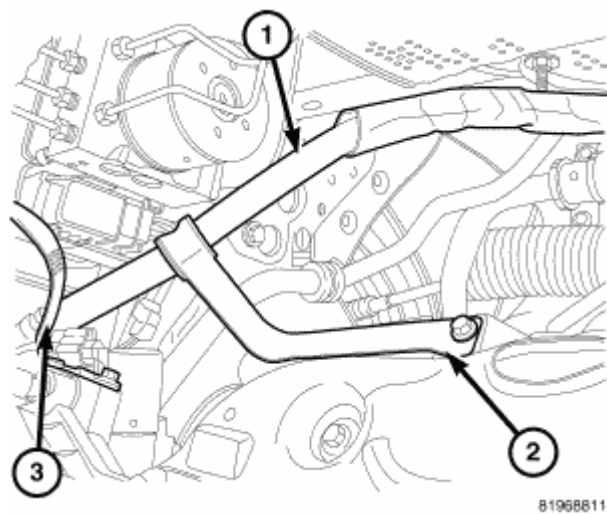
Fig. 20: P/S Hose Support-Fwd Courtesy of CHRYSLER LLC
