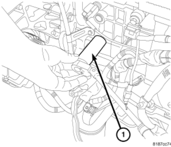
Fig. 261: Oil Pressure Sensor Courtesy of CHRYSLER LLC
