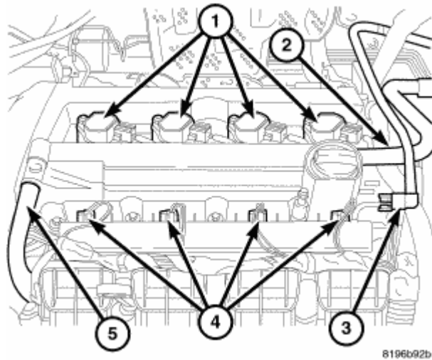
Fig. 376: Coil Connector Courtesy of CHRYSLER LLC
