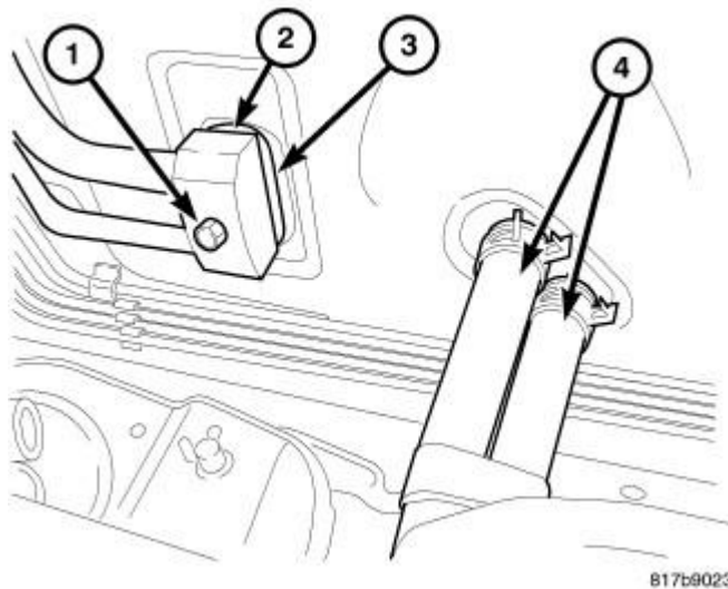
Fig. 343: Refrigerant Lines To Evaporator Bolt Courtesy of CHRYSLER LLC
