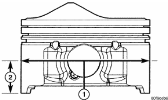
Fig. 228: Piston Measurement
