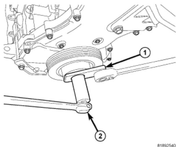
Fig. 22: Damper Removal Courtesy of CHRYSLER LLC
