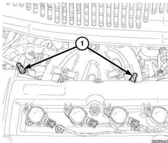
Fig. 324: Engine Cover Mounting Posts Courtesy of CHRYSLER LLC
