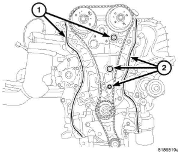
Fig. 389: Timing Chain Cover Sealing Courtesy of CHRYSLER LLC
