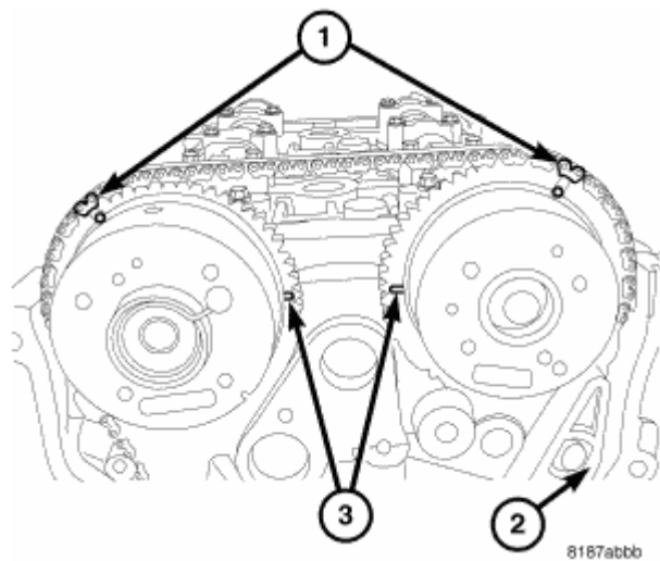
Fig. 415: Timing Chain Timing Marks Courtesy of CHRYSLER LLC
