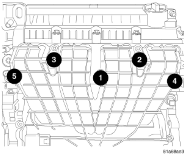
Fig. 366: Intake Manifold Bolt Torque Sequence Courtesy of CHRYSLER LLC
