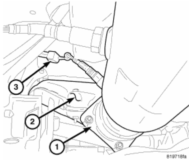
Fig. 41: Cat At Exhaust Manifold
