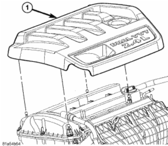
Fig. 57: Engine Cover Courtesy of CHRYSLER LLC
