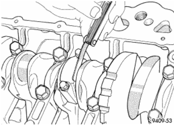
Fig. 243: Connecting Rod Side Clearance Courtesy of CHRYSLER LLC
