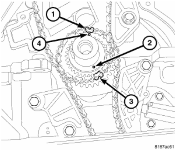
Fig. 412: Crankshaft Timing Marks Courtesy of CHRYSLER LLC
