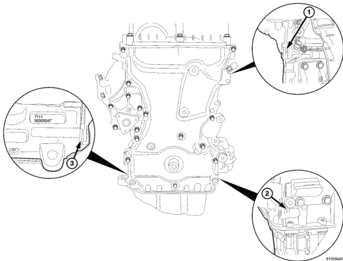
Fig. 384: Timing Chain Cover Pry Points Courtesy of CHRYSLER LLC
