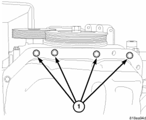
Fig. 393: Timing Chain Cover Lower Bolts Courtesy of CHRYSLER LLC
