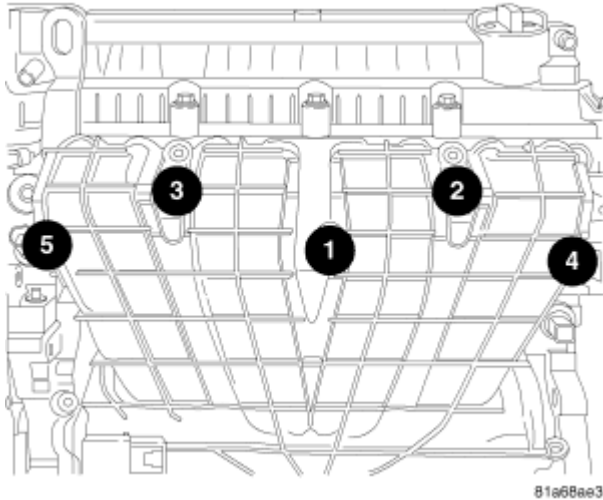
Fig. 367: Intake Manifold Bolt Torque Sequence Courtesy of CHRYSLER LLC
