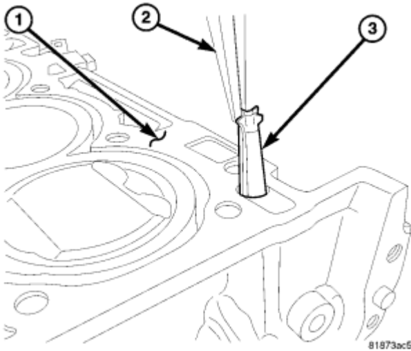
Fig. 104: VVT Filter
