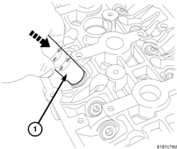
Fig. 166: Removing Valve Keeper Courtesy of CHRYSLER LLC
