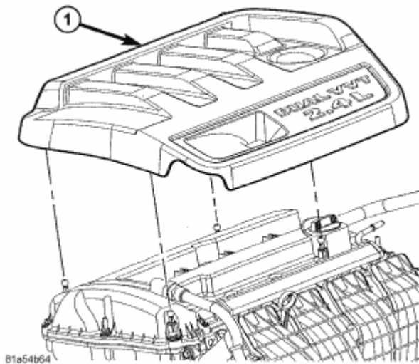
Fig. 370: Engine Cover Courtesy of CHRYSLER LLC
