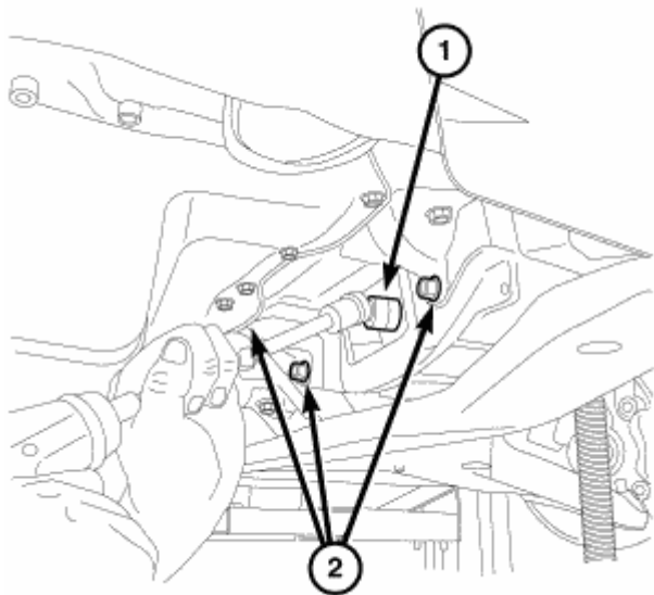
Fig. 27: Bolts
