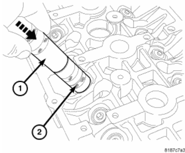
Fig. 172: Valve Installation Courtesy of CHRYSLER LLC
