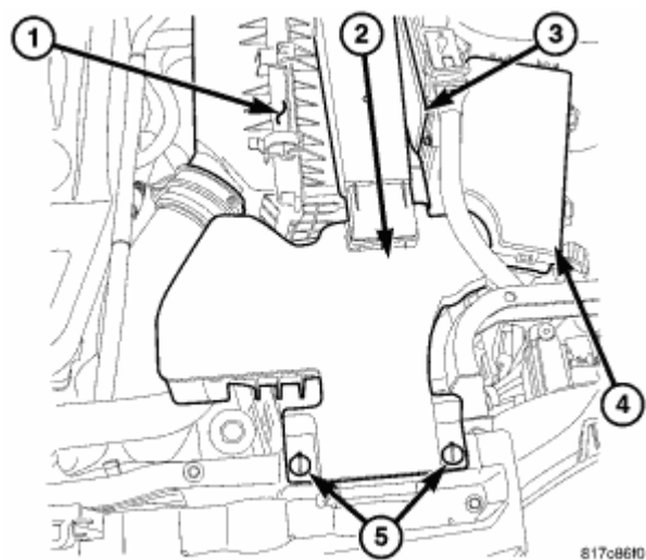
Fig. 9: Air Cleaner Inlet Courtesy of CHRYSLER LLC
