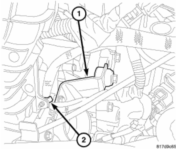
Fig. 48: Throttle Body Support Courtesy of CHRYSLER LLC
