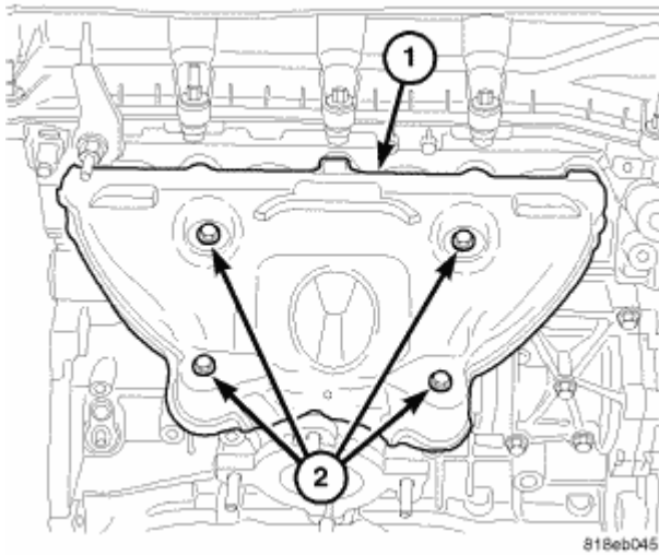
Fig. 331: Exhaust Manifold Heat Shield Courtesy of CHRYSLER LLC
