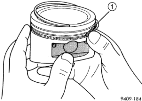
Fig. 247: Installing Side Rail Courtesy of CHRYSLER LLC
