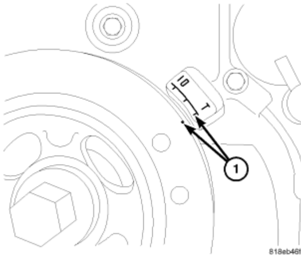
Fig. 86: TDC Courtesy of CHRYSLER LLC
