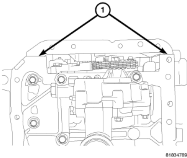
Fig. 276: Engine Block Parting Lines Courtesy of CHRYSLER LLC
