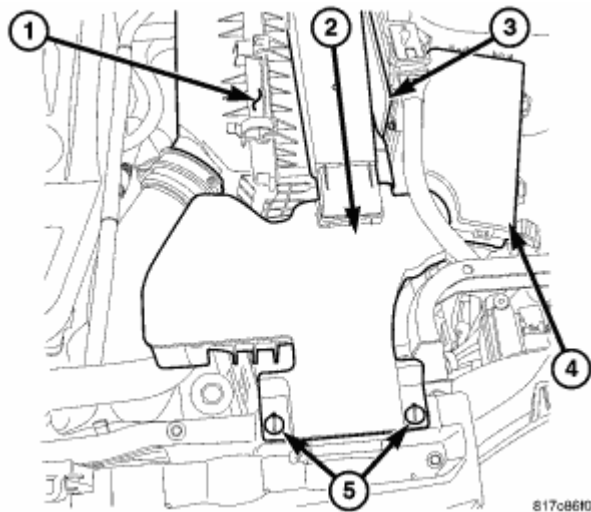
Fig. 312: Air Cleaner Housing Assembly Courtesy of CHRYSLER LLC
