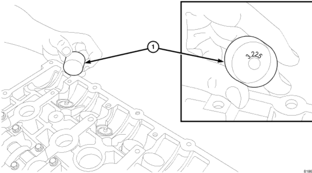
Fig. 161: Tappet Identification Courtesy of CHRYSLER LLC
