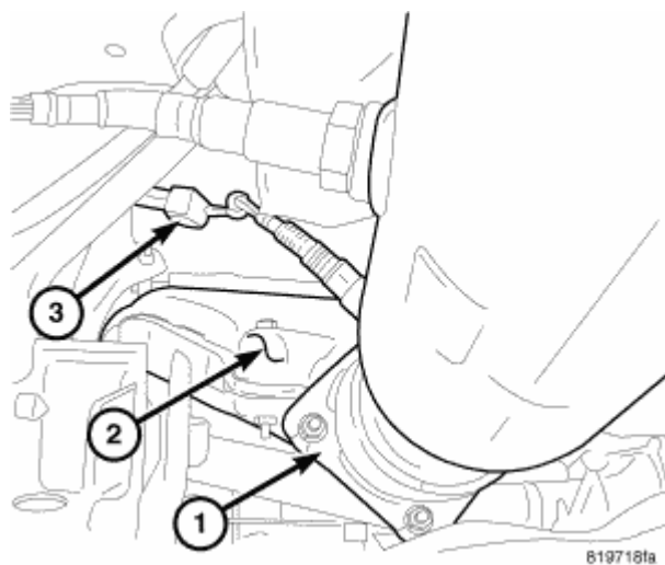
Fig. 90: CAT At Exhaust Manifold Courtesy of CHRYSLER LLC
