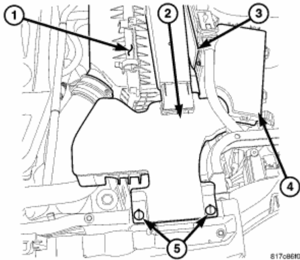
Fig. 360: Air Cleaner Inlet Courtesy of CHRYSLER LLC
