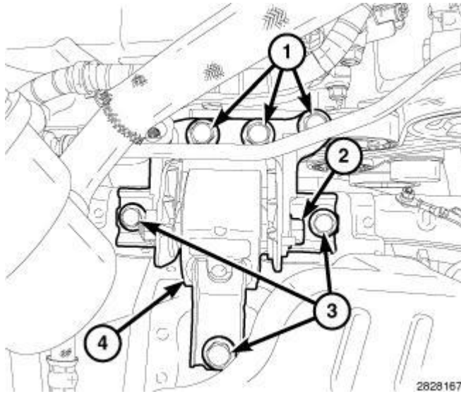
Fig. 336: Engine Mount Isolator, Right Engine Mount & Engine Mount Bracket Retaining Bolts Courtesy of CHRYSLER LLC
