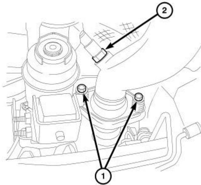
Fig. 365: Exhaust To Maniverter Bolts Courtesy of CHRYSLER GROUP, LLC
