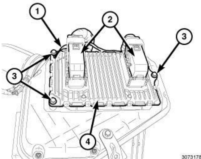
Fig. 392: Electrical Connectors, PCM, Three Mounting Bolts & Ground Wire
