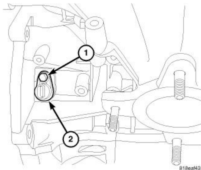
Fig. 39: Crankshaft Position Sensor
