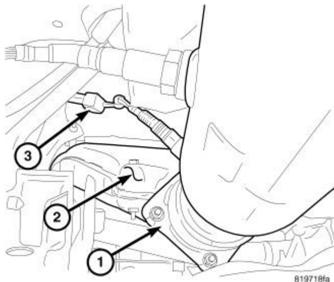
Fig. 350: Exhaust Manifold Bolts, Heat Shield & Oxygen Sensor Connector Courtesy of CHRYSLER GROUP, LLC
