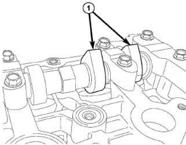
Fig. 135: Identifying Camshaft So Lobes Are Vertical Courtesy of CHRYSLER GROUP, LLC
