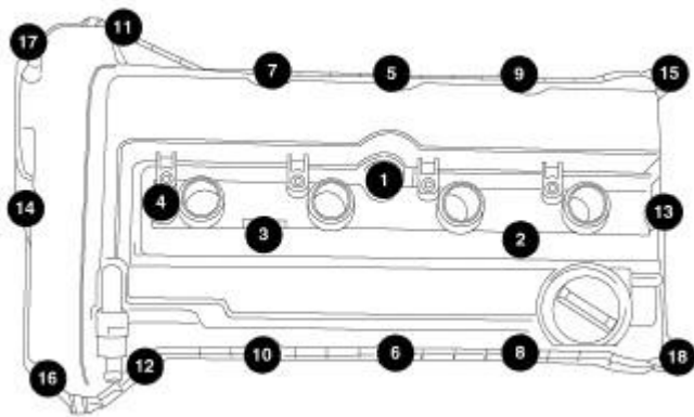
Fig. 417: Removing/Installing Cylinder Head Cover Bolts - Torque Sequence Courtesy of CHRYSLER GROUP, LLC
