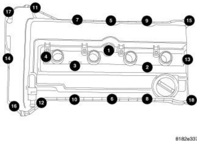
Fig. 440: Remove/Install Cylinder Head Cover Bolts In Sequence
