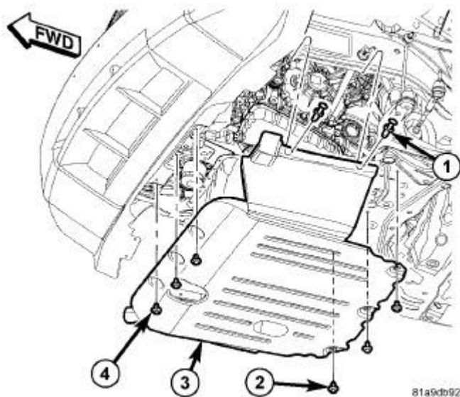
Fig. 334: Belly Pan & Fasteners Courtesy of CHRYSLER GROUP, LLC
