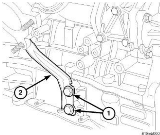
Fig. 351: Exhaust Manifold Support Bracket Courtesy of CHRYSLER GROUP, LLC
