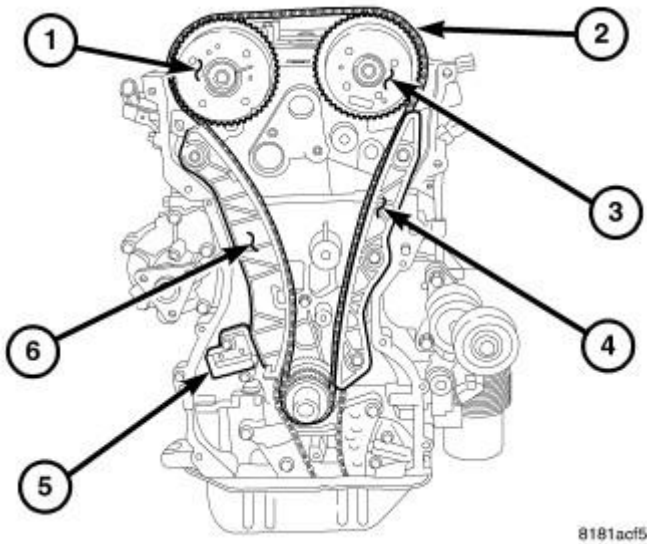
Fig. 395: Timing Drive System
