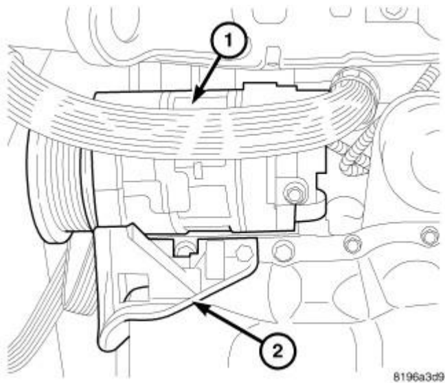
Fig. 82: A/C Compressor Courtesy of CHRYSLER GROUP, LLC
