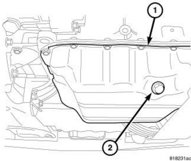
Fig. 251: Oil Drain Plug
