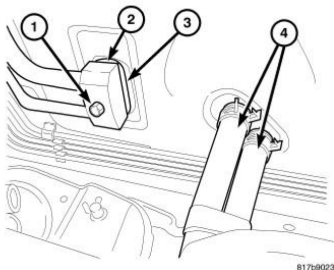
Fig. 339: Refrigerant Lines To Evaporator Bolt Courtesy of CHRYSLER GROUP, LLC
