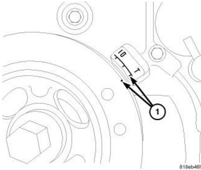
Fig. 81: Setting Engine To Top Dead Center Courtesy of CHRYSLER GROUP, LLC
