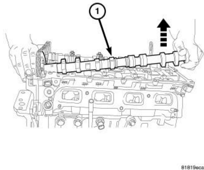
Fig. 158: Removing/Installing Intake Camshaft Courtesy of CHRYSLER GROUP, LLC
