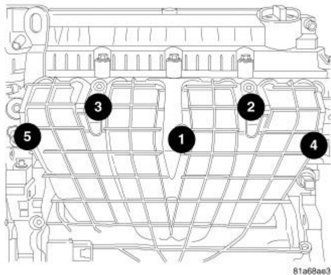
Fig. 123: Removing/Installing Intake Bolts In Sequence Courtesy of CHRYSLER GROUP, LLC
