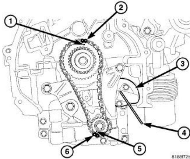
Fig. 404: Oil Pump Drive Chain, Oil Pump Drive Chain Tensioner & Timing Marks On Chain Courtesy of CHRYSLER GROUP, LLC
