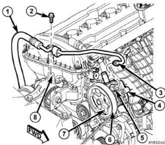
Fig. 442: Removing/Installing Power Steering Hose Hold Down Courtesy of CHRYSLER GROUP, LLC
