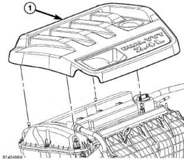
Fig. 59: Engine Cover - 2.4L Courtesy of CHRYSLER GROUP, LLC
