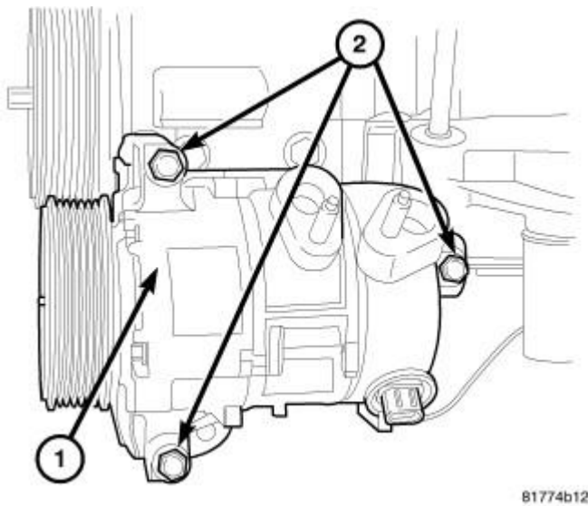
Fig. 326: A/C Compressor Removal/Installation
