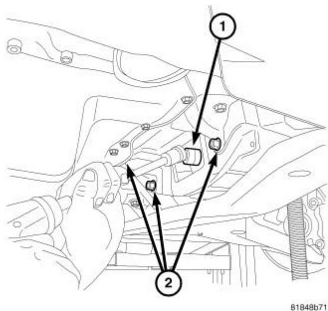
Fig. 37: Modular Clutch To Flex Plate Bolts Courtesy of CHRYSLER GROUP, LLC
