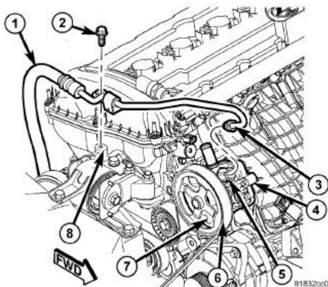
Fig. 78: Removing/Installing Power Steering Hose Hold Down Courtesy of CHRYSLER GROUP, LLC
