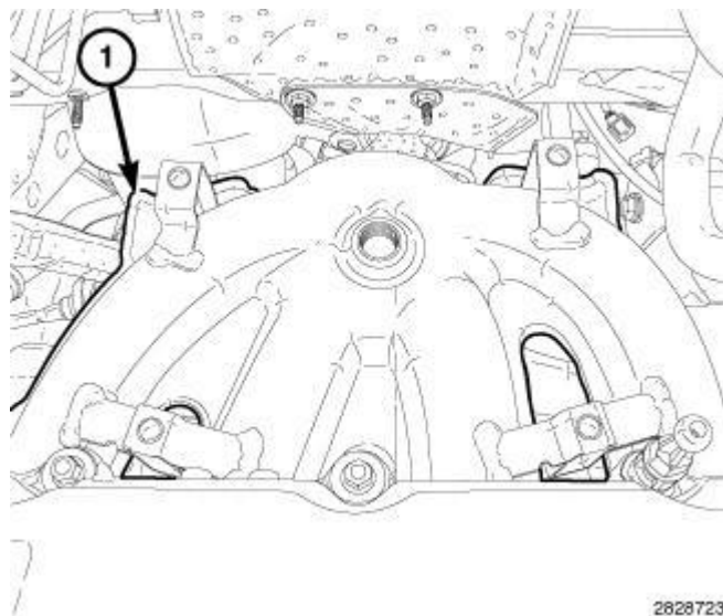
Fig. 359: Lower Maniwerter Heatshield Courtesy of CHRYSLER GROUP, LLC
