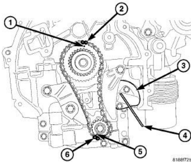
Fig. 320: Oil Pump Drive Chain, Oil Pump Drive Chain Tensioner & Timing Marks On Chain
