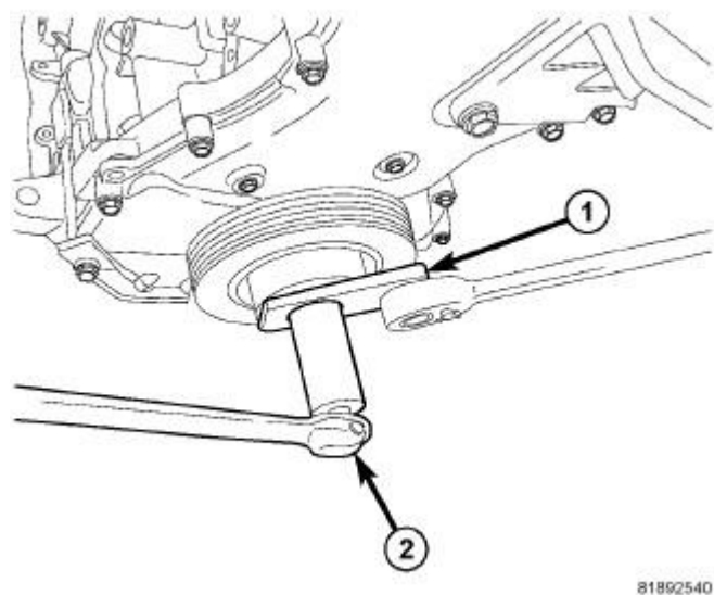
Fig. 24: Damper Removal & Installation
