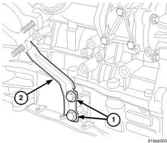
Fig. 373: Exhaust Manifold Support Bracket Courtesy of CHRYSLER GROUP, LLC
