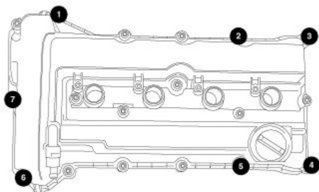
Fig. 173: Identifying Stud Locations In Cylinder Head Cover Courtesy of CHRYSLER GROUP, LLC
