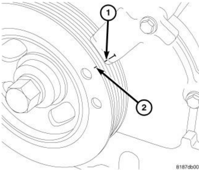
Fig. 396: Setting Engine To Top Dead Center Courtesy of CHRYSLER GROUP, LLC
