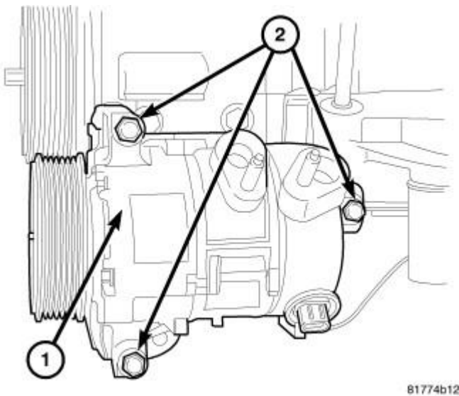
Fig. 323: A/C Compressor Removal/Installation Courtesy of CHRYSLER GROUP, LLC
