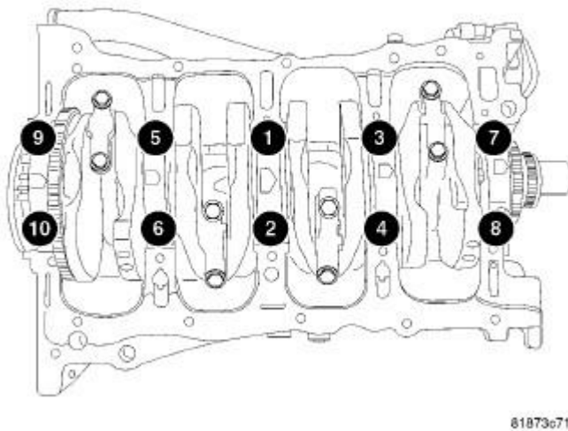
Fig. 221: Main Bearing Cap Torque Sequence Courtesy of CHRYSLER GROUP, LLC
