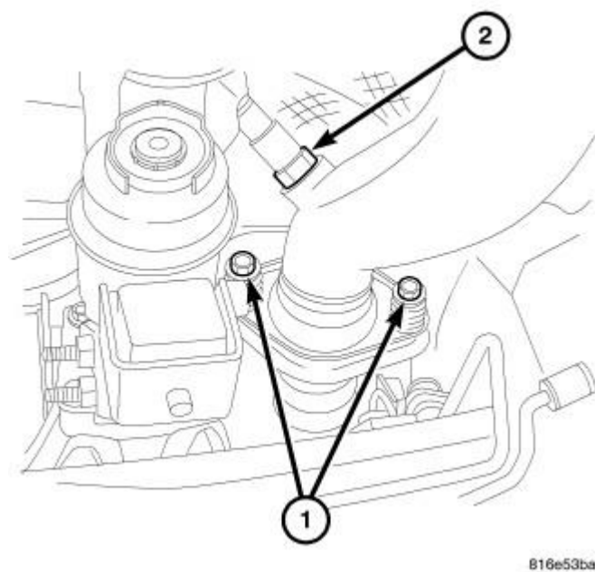
Fig. 41: Exhaust To Maniverter Bolts
