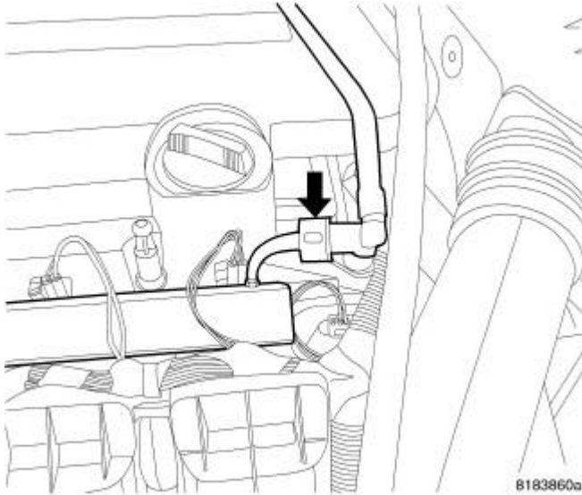
Fig. 92: Disconnecting/Connecting Fuel Line At Fuel Rail Courtesy of CHRYSLER GROUP, LLC
