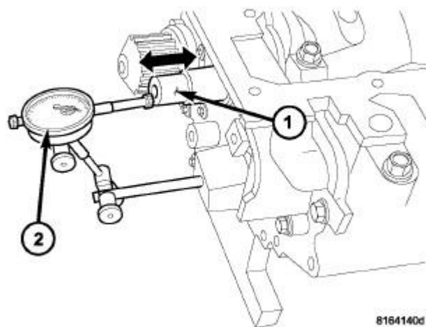
Fig. 211: Checking Crankshaft End Play - Typical Courtesy of CHRYSLER GROUP, LLC
