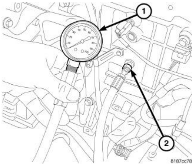
Fig. 272: Oil Pressure Gauge
