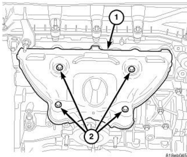
Fig. 372: Exhaust Manifold Heat Shield Courtesy of CHRYSLER GROUP, LLC
