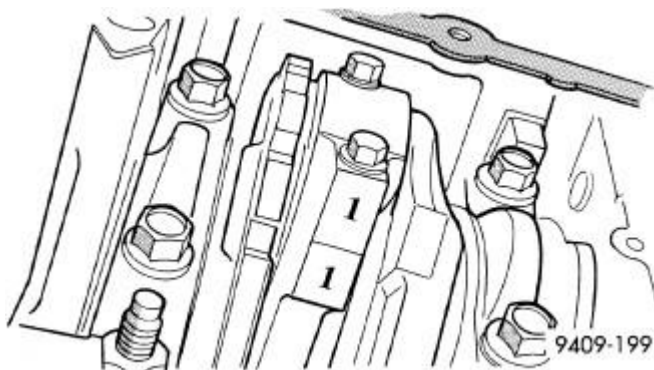
Fig. 253: Identifying Mark On Connecting Rod And Bearing Cap
