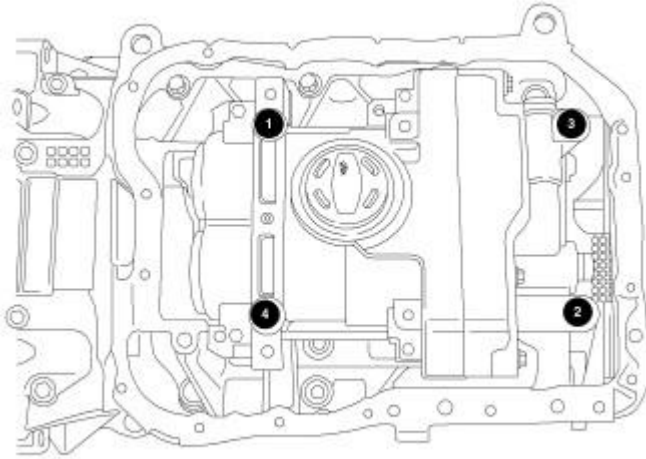
Fig. 319: Balance Shaft Module Torque Sequence Courtesy of CHRYSLER GROUP, LLC
