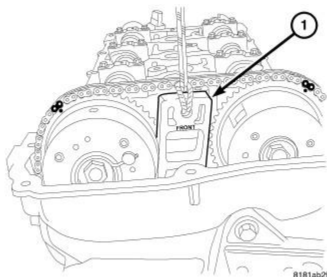
Fig. 149: Inserting Wedge 9701 Between Camshaft Phasers
