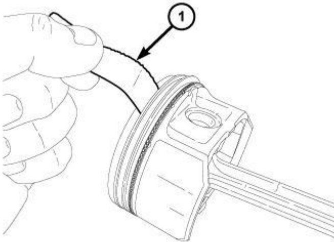
Fig. 243: Piston Ring To Groove Side Clearance Courtesy of CHRYSLER GROUP, LLC
