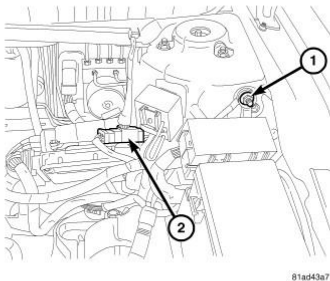
Fig. 375: Identifying Battery Cables Courtesy of CHRYSLER GROUP, LLC
