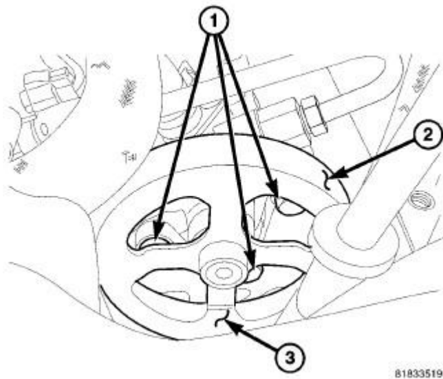
Fig. 441: Removing/Installing Power Steering Pump Mounting Bolts Through Pulley Openings Courtesy of CHRYSLER GROUP, LLC
