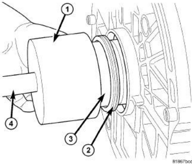
Fig. 267: Driving Seal Into Block Using Seal Driver 9706 And Driver Handle C-4171 Until Seal Driver 9706 Bottoms Out Against Block
