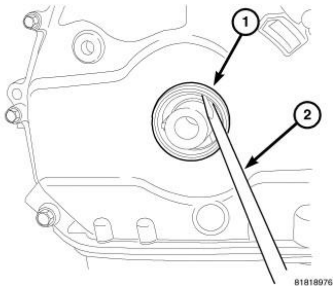
Fig. 260: Front Crankshaft Seal Removal Courtesy of CHRYSLER GROUP, LLC
