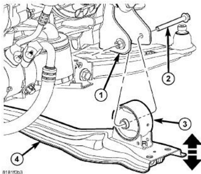
Fig. 363: Removing/Installing Fore/Aft Crossmember Courtesy of CHRYSLER GROUP, LLC
