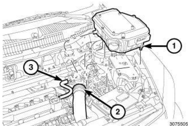
Fig. 56: Air Cleaner Body, Air Inlet Tube & Make-Up Air Hose Courtesy of CHRYSLER GROUP, LLC
