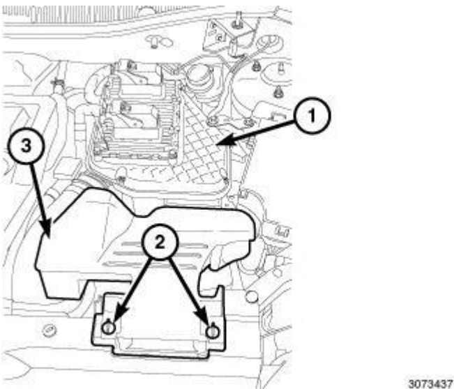
Fig. 187: Retainers, Fresh Air Inlet Duct & Air Cleaner Body Courtesy of CHRYSLER GROUP, LLC
