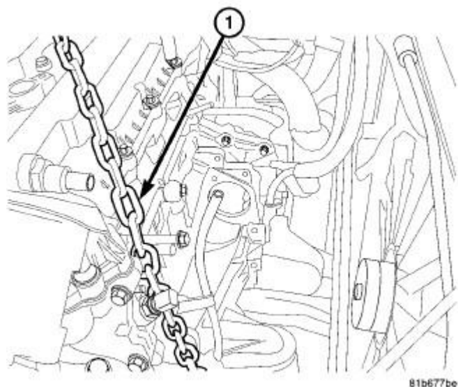
Fig. 258: Identifying Lift Chain Courtesy of CHRYSLER GROUP, LLC
