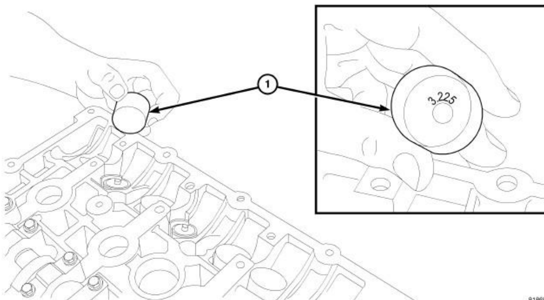
Fig. 140: Tappet Identification
