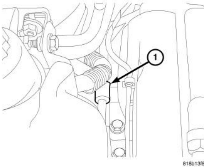
Fig. 201: Power Steering Line Support Courtesy of CHRYSLER GROUP, LLC
