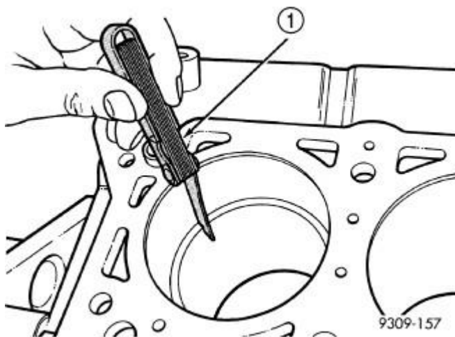
Fig. 242: Check Gap On Piston Rings Courtesy of CHRYSLER GROUP, LLC
