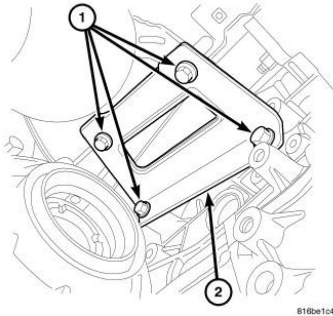
Fig. 362: Maniverter To Block Support Bracket Courtesy of CHRYSLER GROUP, LLC
