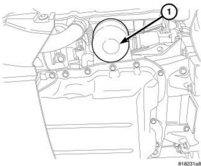
Fig. 296: Oil Filter
