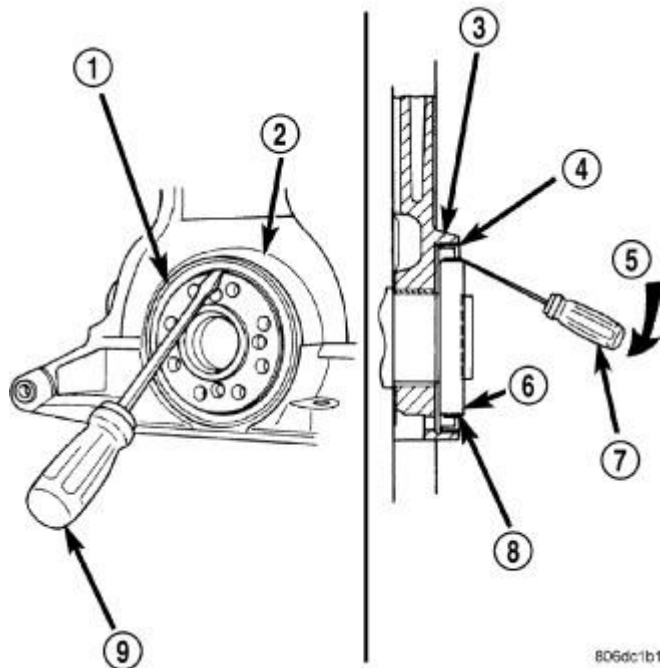
Fig. 266: Rear Crankshaft Oil Seal - Removal
