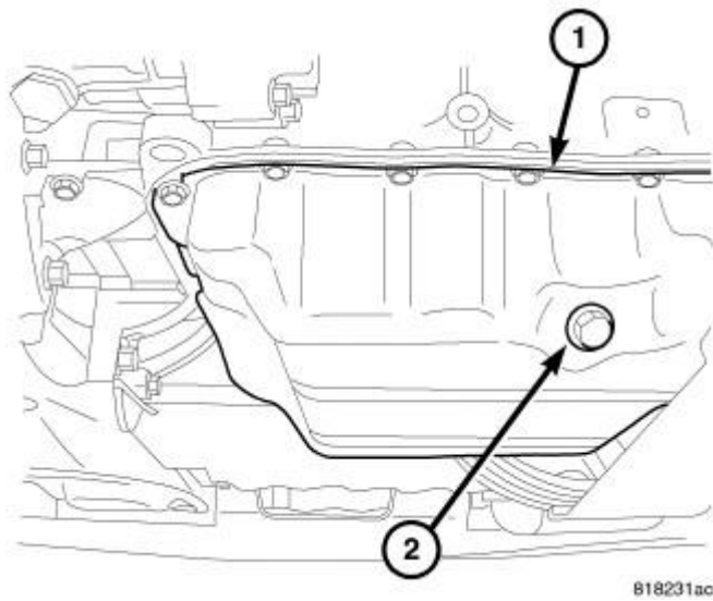
Fig. 214: Oil Drain Plug Courtesy of CHRYSLER GROUP, LLC
