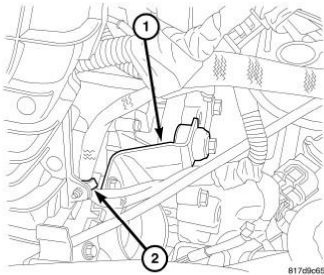
Fig. 388: Throttle Body Support Courtesy of CHRYSLER GROUP, LLC
