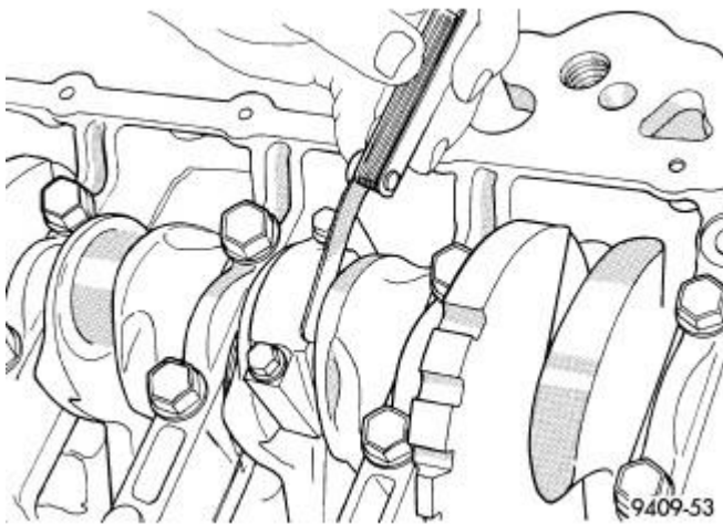
Fig. 257: Connecting Rod Side Clearance Courtesy of CHRYSLER GROUP, LLC
