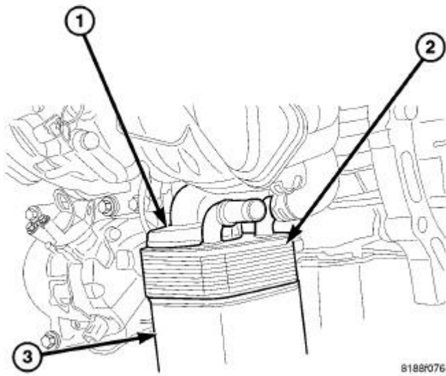
Fig. 46: Oil Cooler
