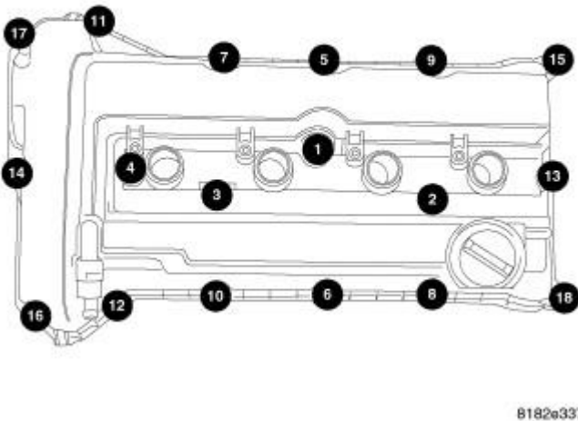
Fig. 167: Cylinder Head Cover Bolt Torque Sequence Courtesy of CHRYSLER GROUP, LLC
