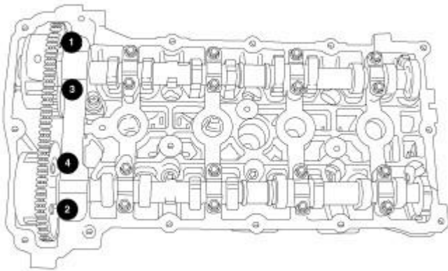
Fig. 161: Front Cam Cap Removal/Tightening Sequence Courtesy of CHRYSLER GROUP, LLC
