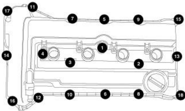
Fig. 171: Removing/Installing Cylinder Head Cover Bolts - Torque Sequence Courtesy of CHRYSLER GROUP, LLC
