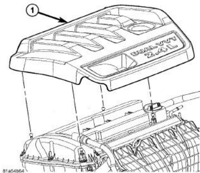
Fig. 330: Engine Cover
