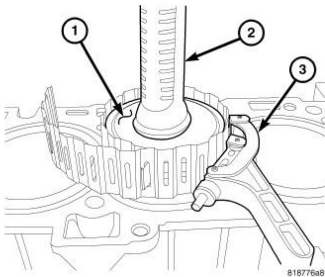
Fig. 256: Piston, Hammer Handle & Ring Compressor
