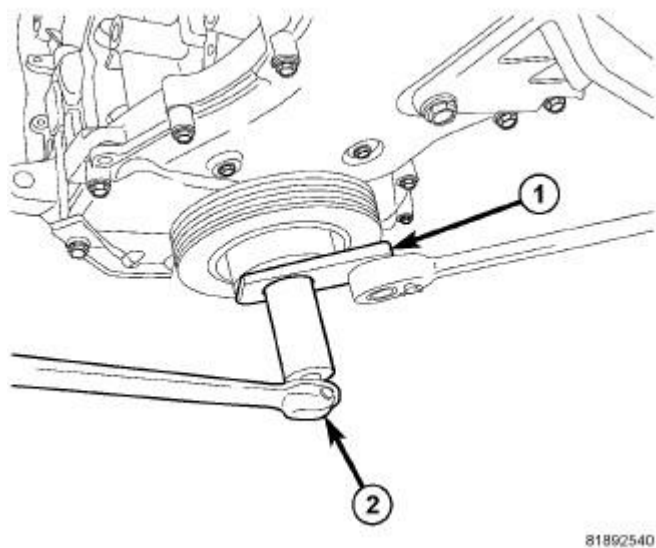
Fig. 259: Damper Removal & Installation Courtesy of CHRYSLER GROUP, LLC
