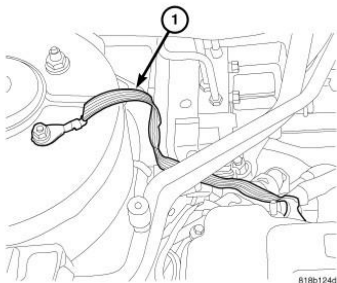
Fig. 23: Ground Strap
