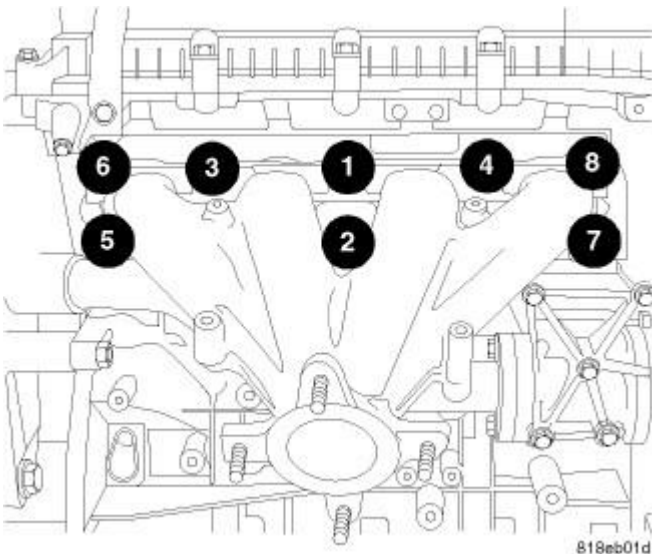
Fig. 371: Exhaust Manifold Retaining Fasteners Tightening Sequence Courtesy of CHRYSLER GROUP, LLC
