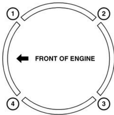
Fig. 254: Identifying Piston Ring End Gap Positions Courtesy of CHRYSLER GROUP, LLC
