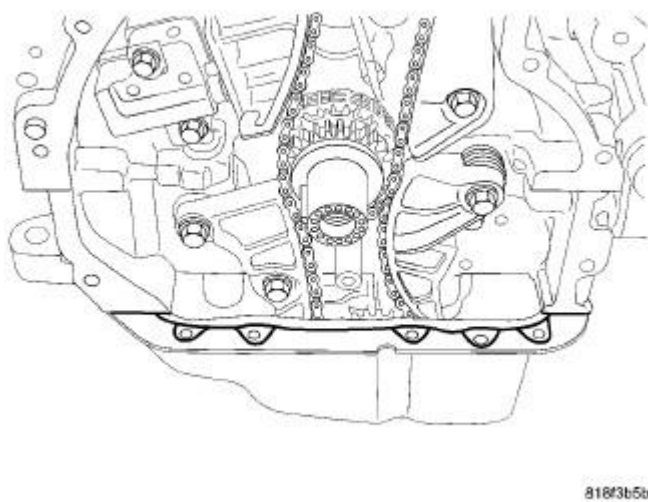
Fig. 430: Sealing Oil Pan
