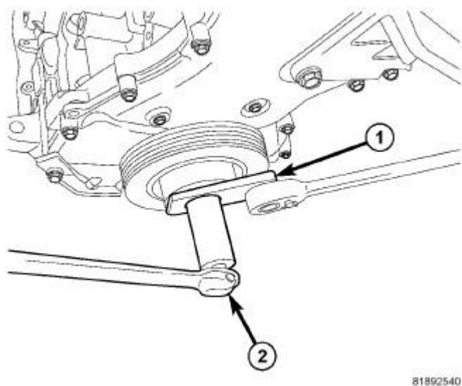
Fig. 235: Damper Removal & Installation Courtesy of CHRYSLER GROUP, LLC
