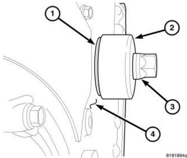
Fig. 262: Installing Front Seal
