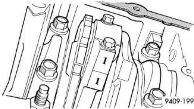
Fig. 220: Identifying Mark On Connecting Rod And Bearing Cap Courtesy of CHRYSLER GROUP, LLC
