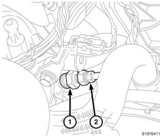
Fig. 276: Oil Pressure Adapter 9879
