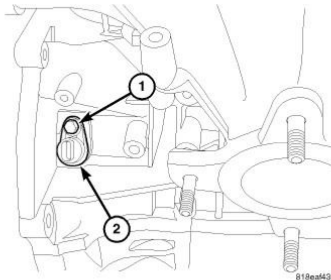
Fig. 31: Crankshaft Position Sensor Courtesy of CHRYSLER GROUP, LLC
