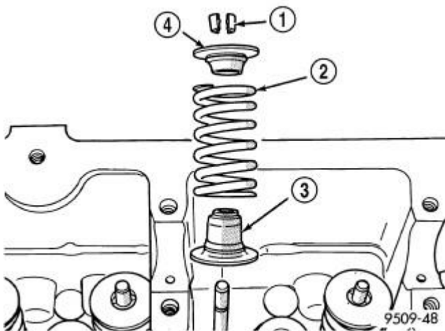
Fig. 182: Valve Spring Assembly
