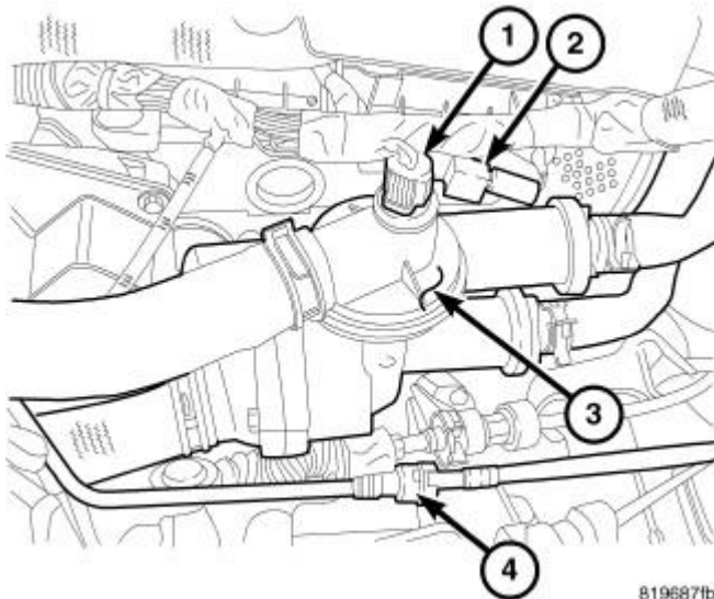
Fig. 114: Coolant Temperature Sensor, Capacitor Electrical Connector & Coolant Adapter Courtesy of CHRYSLER GROUP, LLC
