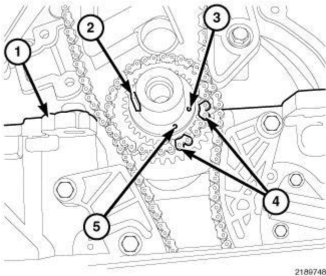
Fig. 408: Crankshaft Timing Marks Courtesy of CHRYSLER GROUP, LLC
