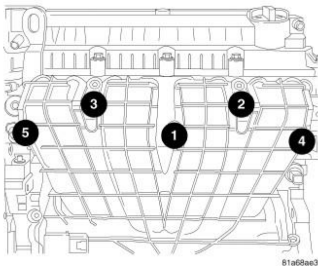
Fig. 20: Intake Manifold Bolt Removal & Tightening Sequence Courtesy of CHRYSLER GROUP, LLC
