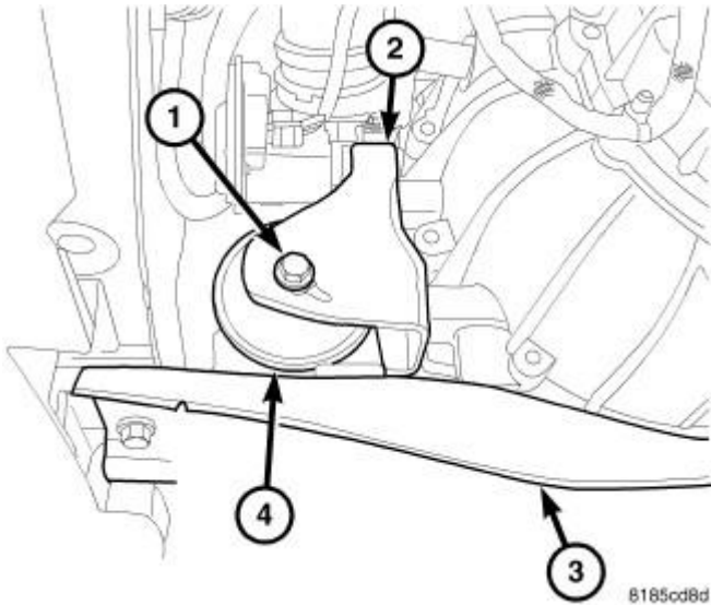
Fig. 186: Front Mount Through Bolt Courtesy of CHRYSLER GROUP, LLC
