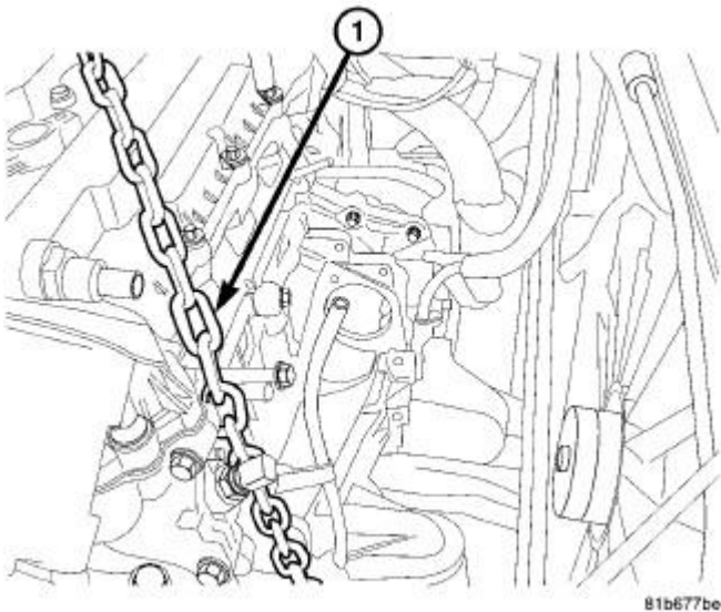
Fig. 35: Identifying Lift Chain Courtesy of CHRYSLER GROUP, LLC
