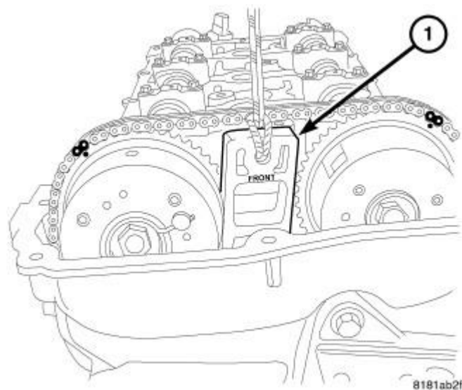
Fig. 163: Inserting Wedge 9701 Between Camshaft Phasers Courtesy of CHRYSLER GROUP, LLC
