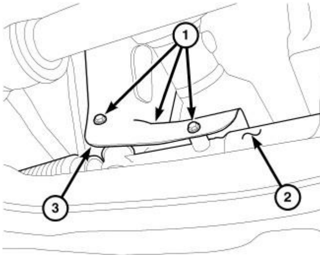
Fig. 364: Steering Gear Heat Shield Bolts Courtesy of CHRYSLER GROUP, LLC
