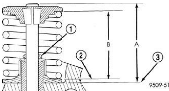
Fig. 184: Spring Installed Height And Valve TIP To Spring Seat Dimensions
