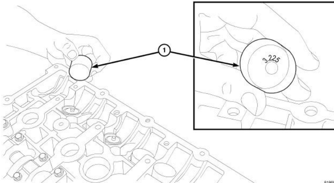
Fig. 139: Tappet Identification Courtesy of CHRYSLER GROUP, LLC
