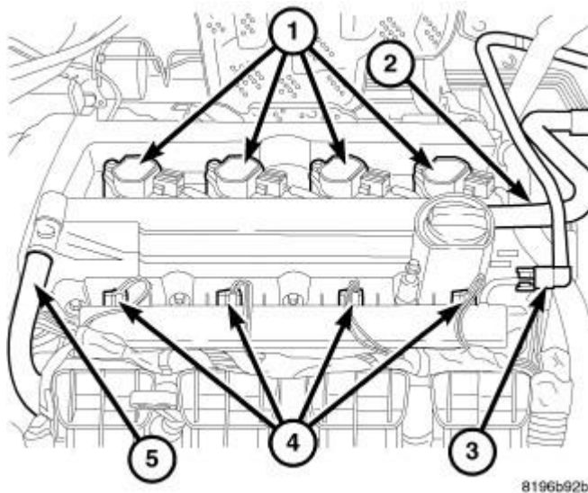
Fig. 390: Ignition Coils, Air Hose, Fuel Line, Injectors & PCV Hose Courtesy of CHRYSLER GROUP, LLC
