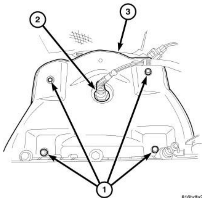
Fig. 332: Maniverter Heat Shield And Bolts Courtesy of CHRYSLER GROUP, LLC
