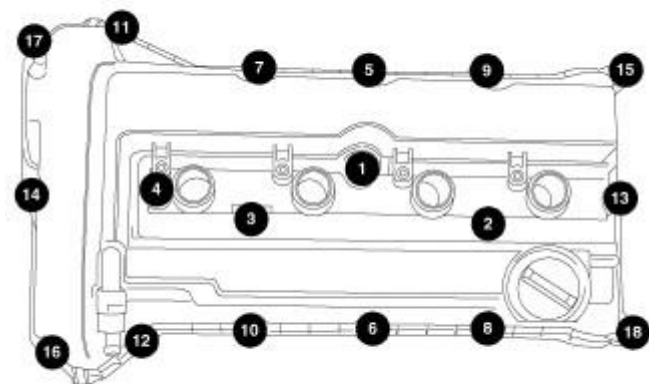
Fig. 138: Cylinder Head Cover Bolts Torque Sequence
