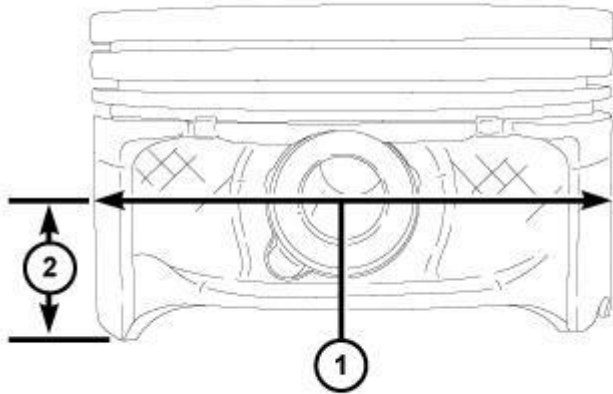
Fig. 247: Identifying Piston Diameter Measurement Location Courtesy of CHRYSLER GROUP, LLC
