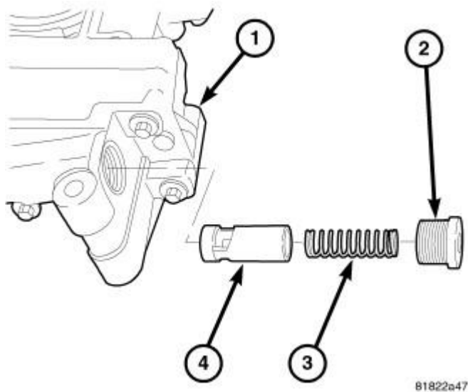
Fig. 327: Oil Pressure Relief Valve
