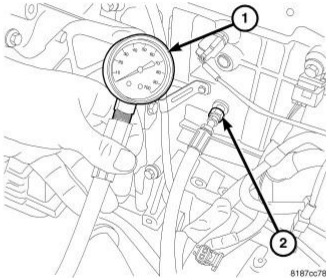
Fig. 273: Oil Pressure Gauge Courtesy of CHRYSLER GROUP, LLC
