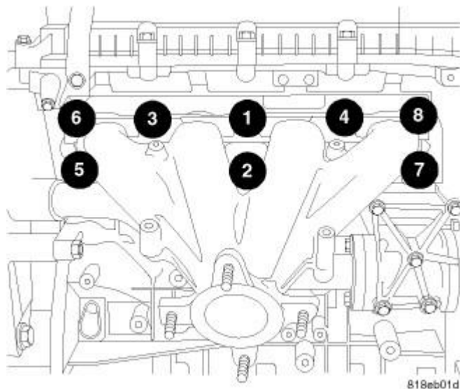
Fig. 352: Exhaust Manifold Retaining Fasteners Tightening Sequence Courtesy of CHRYSLER GROUP, LLC
