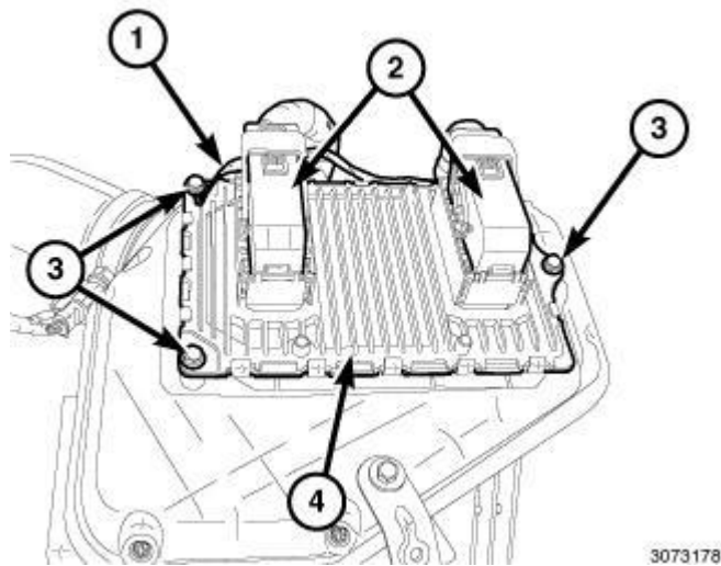
Fig. 379: Electrical Connectors, PCM, Three Mounting Bolts & Ground Wire Courtesy of CHRYSLER GROUP, LLC
