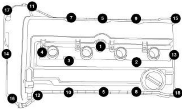
Fig. 121: Cylinder Head Cover Bolt Torque Sequence Courtesy of CHRYSLER GROUP, LLC
