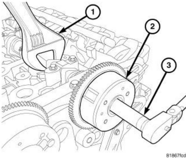
Fig. 132: Camshaft Phaser Removal & Installation Courtesy of CHRYSLER GROUP, LLC
