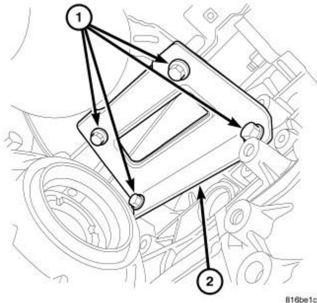
Fig. 338: Maniverter To Block Support Bracket Courtesy of CHRYSLER GROUP, LLC
