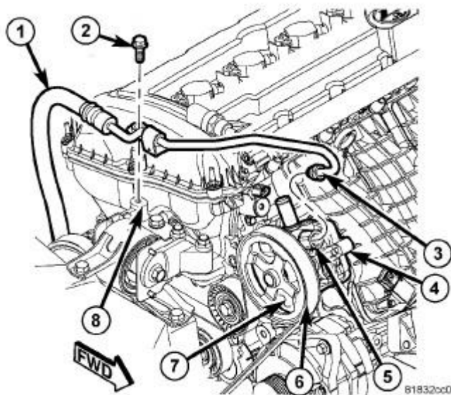
Fig. 355: Removing/Installing Power Steering Hose Hold Down Courtesy of CHRYSLER GROUP, LLC
