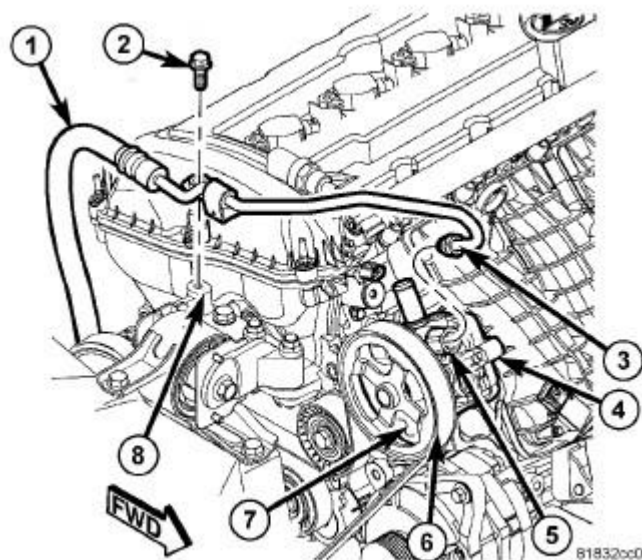
Fig. 345: Removing/Installing Power Steering Hose Hold Down Courtesy of CHRYSLER GROUP, LLC
