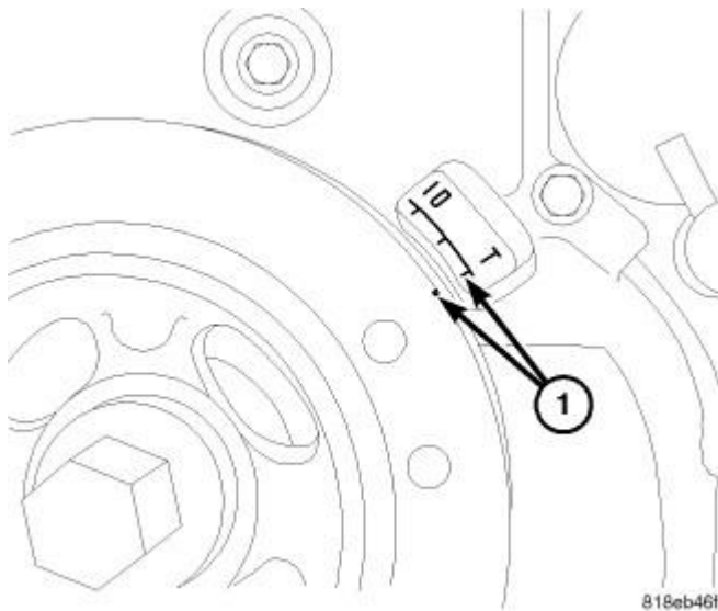
Fig. 145: Setting Engine To Top Dead Center
