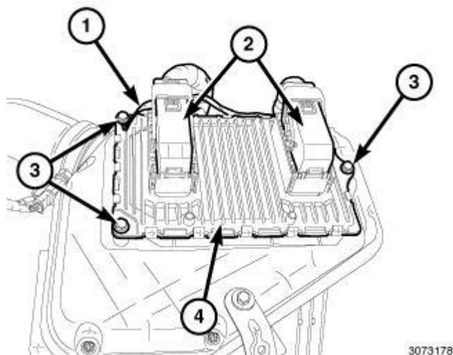
Fig. 12: Electrical Connectors, PCM, Three Mounting Bolts & Ground Wire Courtesy of CHRYSLER GROUP, LLC
