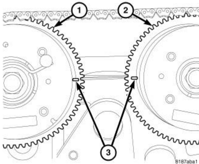
Fig. 165: Camshaft Timing Courtesy of CHRYSLER GROUP, LLC
