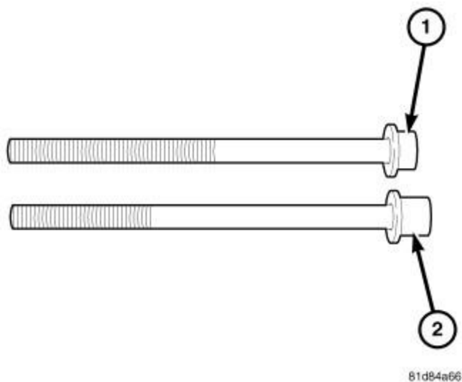
Fig. 109: Cylinder Head Bolt Identification Courtesy of CHRYSLER LLC
