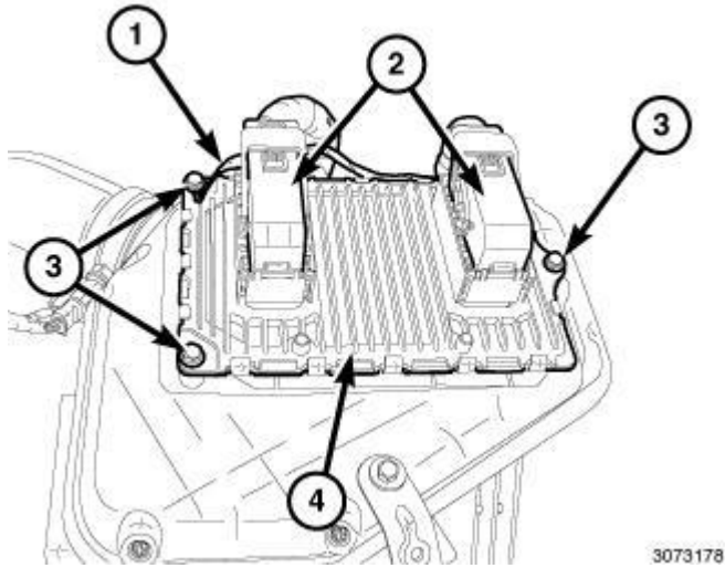
Fig. 57: Electrical Connectors, PCM, Three Mounting Bolts & Ground Wire Courtesy of CHRYSLER LLC
