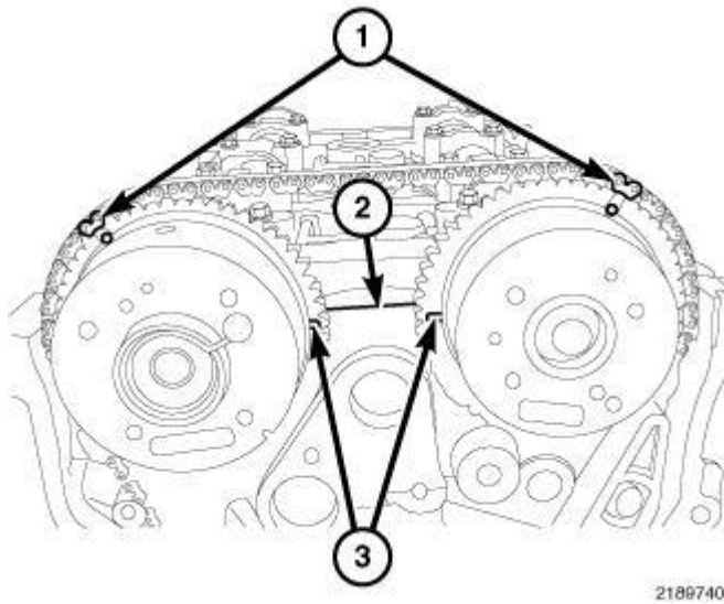
Fig. 409: Timing Chain Timing Marks
