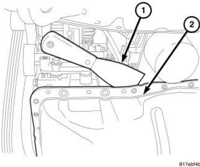
Fig. 217: Oil Pan Removal Courtesy of CHRYSLER LLC
