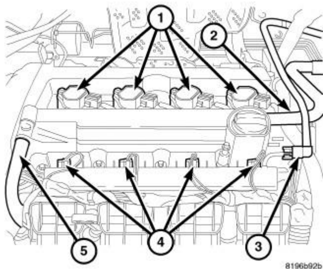
Fig. 390: Coil Connectors Courtesy of CHRYSLER LLC
