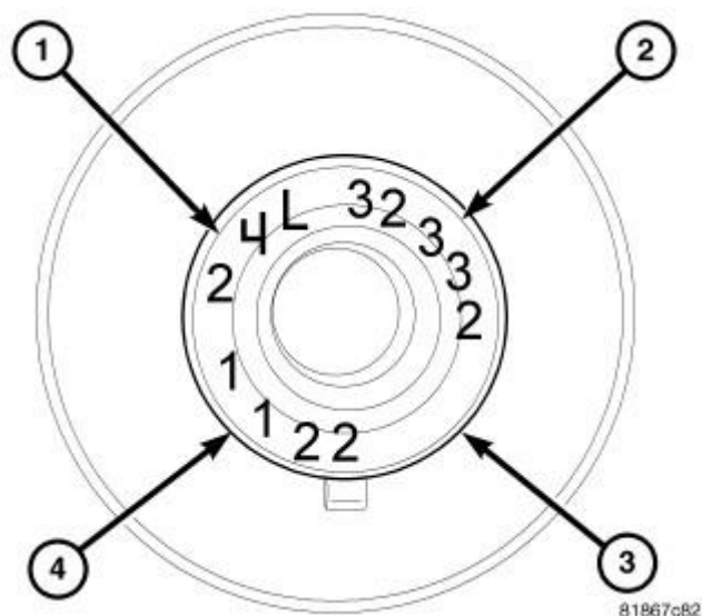
Fig. 206: Connecting Rod Bearing Identification Courtesy of CHRYSLER LLC
