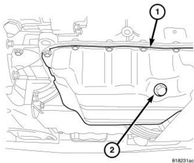
Fig. 298: Oil Drain Plug Courtesy of CHRYSLER LLC
