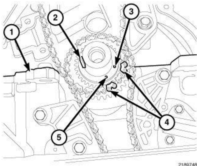
Fig. 398: Crankshaft Timing Marks
