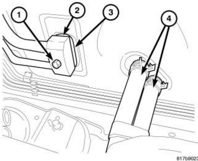
Fig. 339: Refrigerant Lines To Evaporator Bolt Courtesy of CHRYSLER LLC
