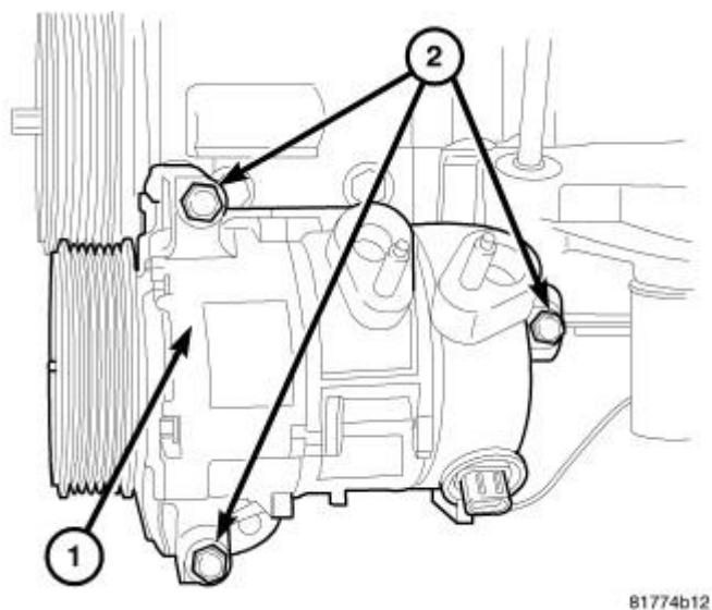
Fig. 323: Removing/Installing A/C Compressor Courtesy of CHRYSLER LLC
