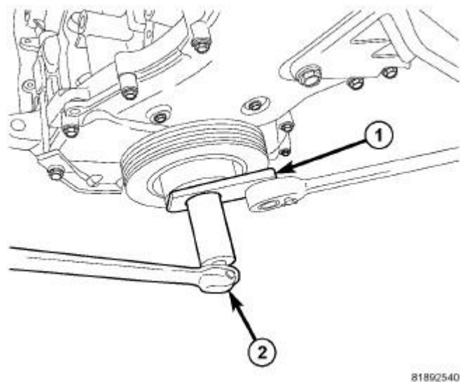
Fig. 264: Damper Removal & Installation Courtesy of CHRYSLER LLC
