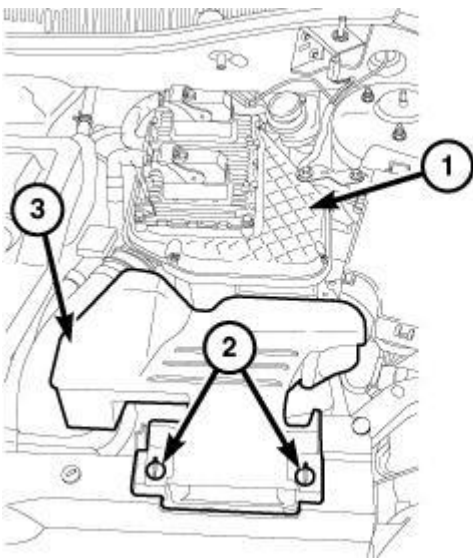
Fig. 187: Retainers, Fresh Air Inlet Duct & Air Cleaner Body Courtesy of CHRYSLER LLC
