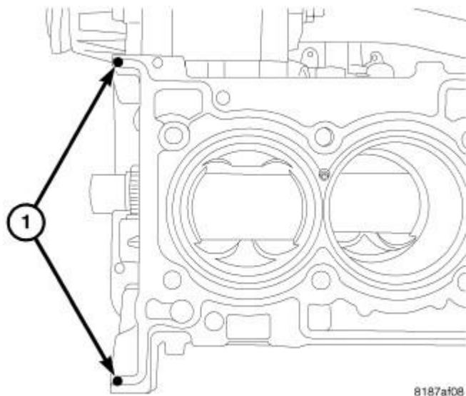
Fig. 108: Cylinder Head Gasket RTV Courtesy of CHRYSLER LLC
