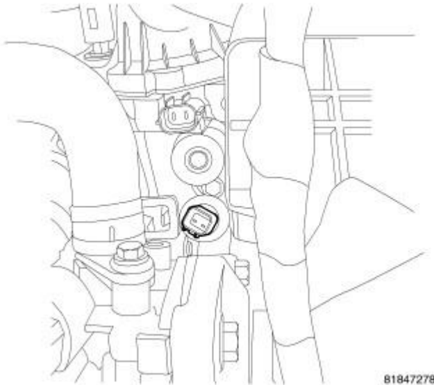
Fig. 289: Oil Pressure Sensor Courtesy of CHRYSLER LLC
