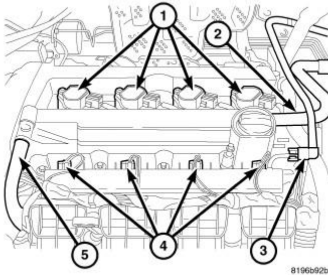
Fig. 10: Coil Connector Courtesy of CHRYSLER LLC
