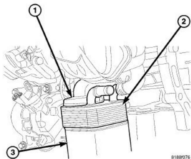
Fig. 46: Oil Cooler Courtesy of CHRYSLER LLC
