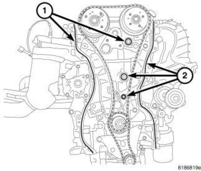
Fig. 431: Timing Chain Cover Sealing Courtesy of CHRYSLER LLC
