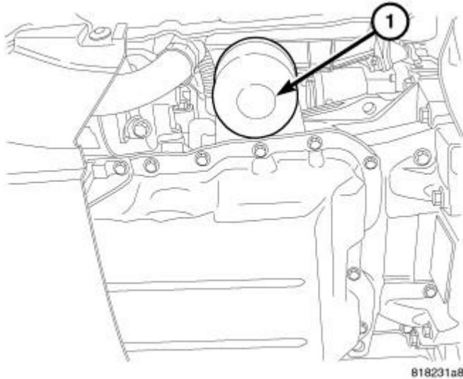
Fig. 252: Oil Filter
