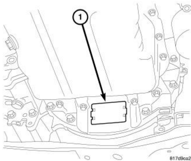
Fig. 38: Inspection Cover
