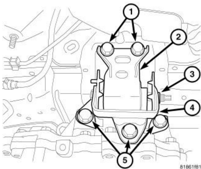
Fig. 191: Left Mount Courtesy of CHRYSLER LLC
