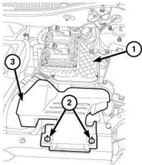
Fig. 74: Retainers, Fresh Air Inlet Duct & Air Cleaner Body Courtesy of CHRYSLER LLC
