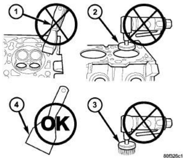
Fig. 103: Proper Tool Usage For Surface Preparation Courtesy of CHRYSLER LLC
