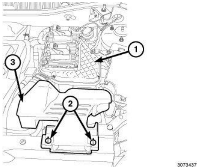
Fig. 58: Retainers, Fresh Air Inlet Duct & Air Cleaner Body Courtesy of CHRYSLER LLC
