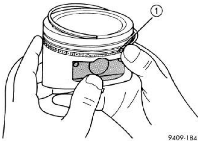
Fig. 245: Installing Side Rail Courtesy of CHRYSLER LLC
