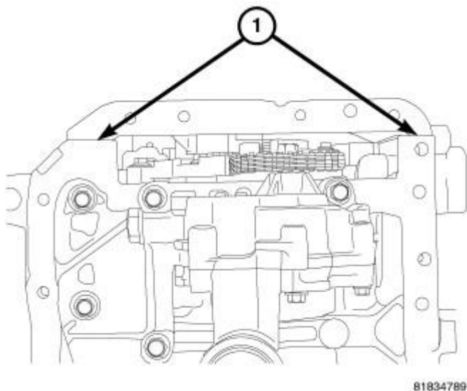
Fig. 305: Sealer Location Courtesy of CHRYSLER LLC
