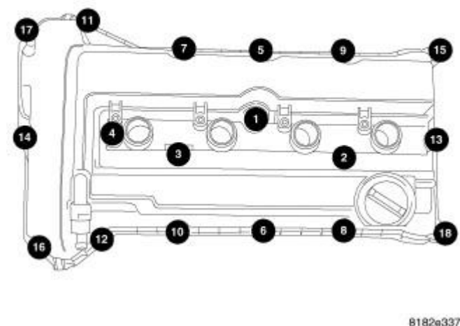
Fig. 171: Removing/Installing Cylinder Head Cover Bolts In Sequence Courtesy of CHRYSLER LLC
