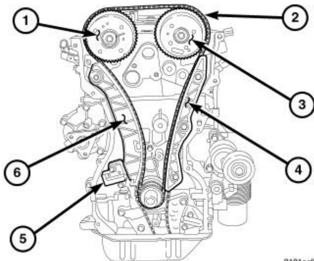
Fig. 120: Timing Drive Courtesy of CHRYSLER LLC
