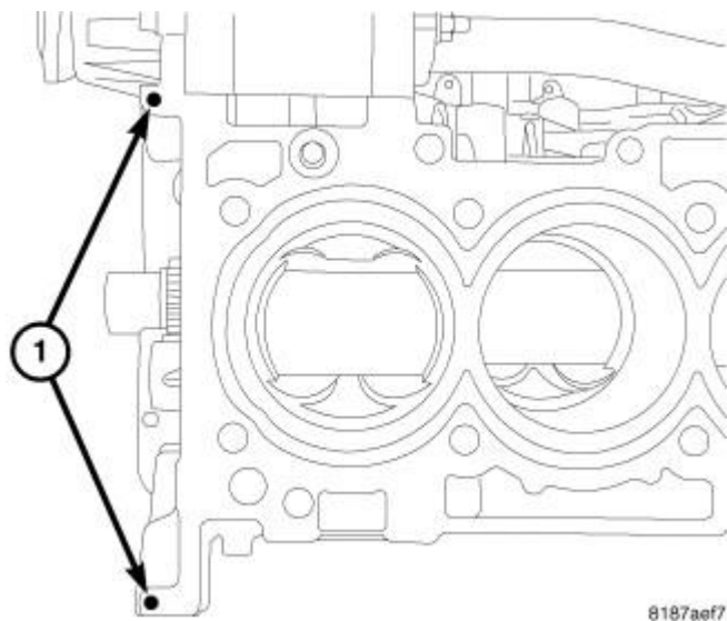
Fig. 107: Applying Cylinder Head RTV On Cylinder Block Courtesy of CHRYSLER LLC
