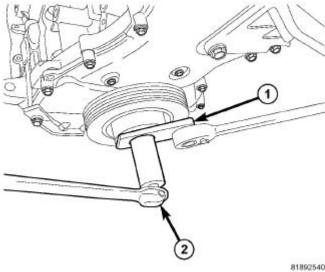
Fig. 259: Damper Removal & Installation Courtesy of CHRYSLER LLC
