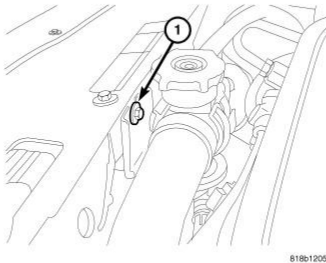
Fig. 52: Radiator Hose Support Courtesy of CHRYSLER LLC
