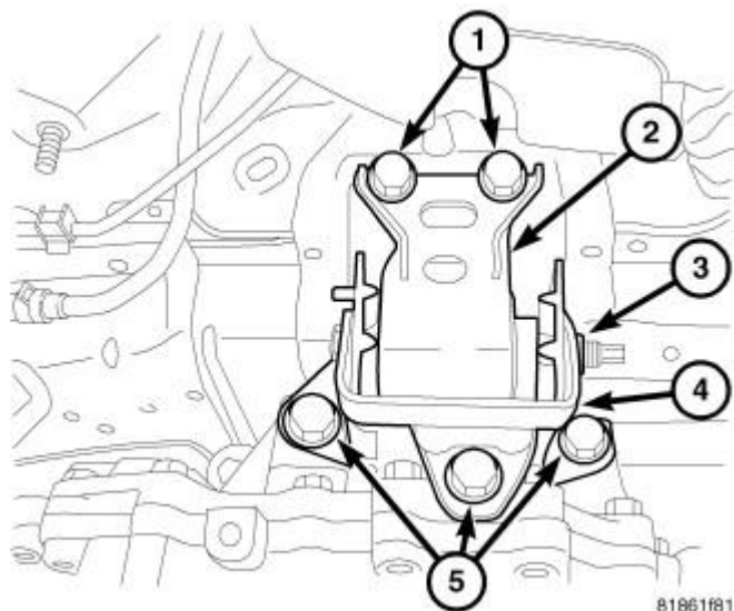
Fig. 190: Left Mount Courtesy of CHRYSLER LLC
