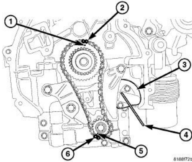
Fig. 404: Oil Pump Drive Chain, Oil Pump Drive Chain Tensioner & Timing Marks On Chain Courtesy of CHRYSLER LLC
