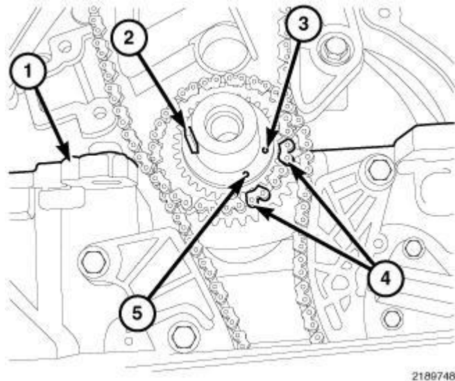
Fig. 410: Crankshaft Timing Marks
