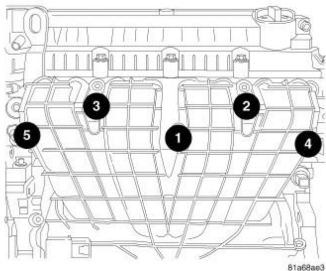
Fig. 20: Intake Manifold Bolt Removal & Tightening Sequence Courtesy of CHRYSLER LLC
