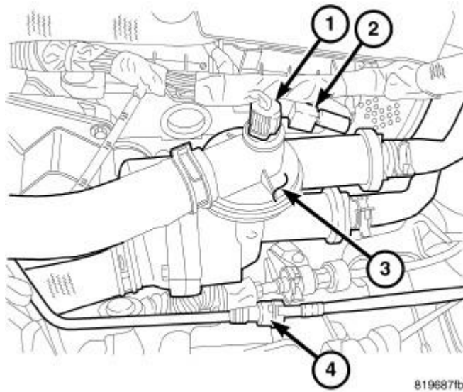
Fig. 133: COOLANT ADAPTER Courtesy of CHRYSLER LLC
