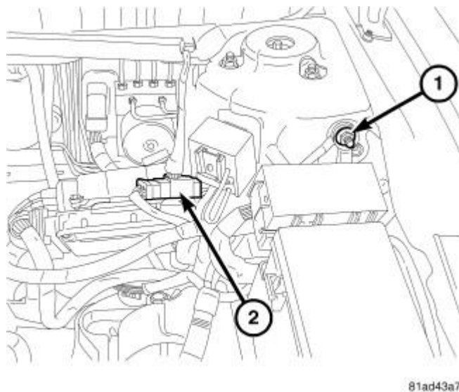
Fig. 378: BATTERY CABLE Courtesy of CHRYSLER LLC
