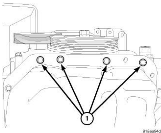
Fig. 418: Timing Chain Cover Lower Bolts Courtesy of CHRYSLER LLC
