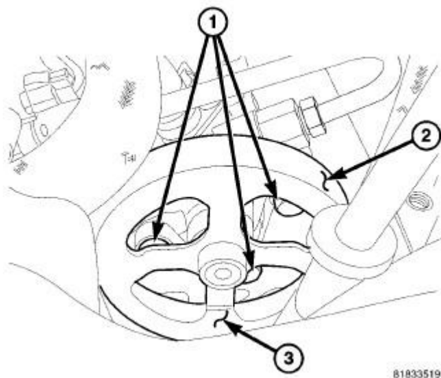
Fig. 86: POWER STEERING PUMP - GAS Courtesy of CHRYSLER LLC
