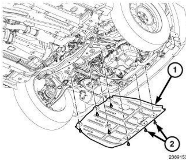
Fig. 336: Removal/Installation Front Skid Plate And Bolts Courtesy of CHRYSLER LLC
