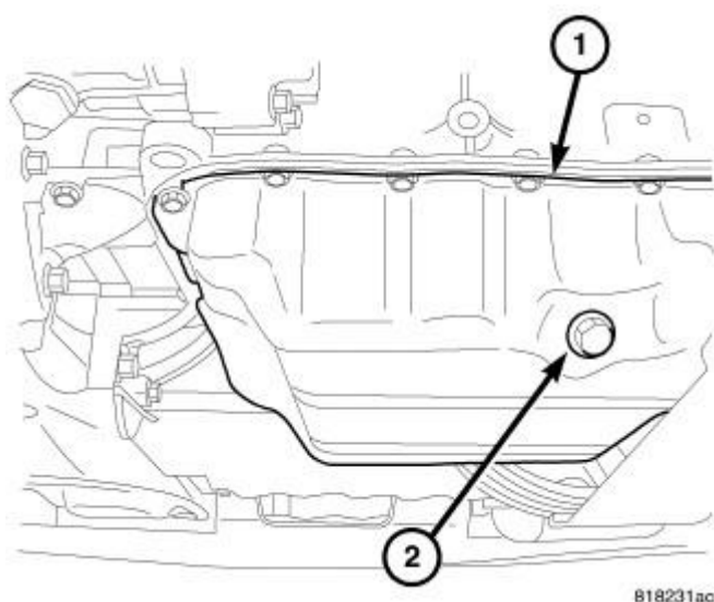
Fig. 302: OIL DRAIN PLUG Courtesy of CHRYSLER LLC
