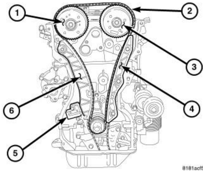
Fig. 408: TIMING DRIVE Courtesy of CHRYSLER LLC
