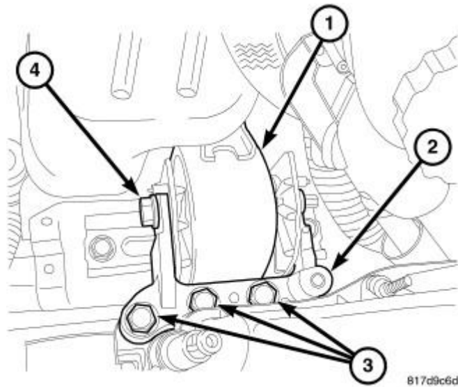
Fig. 419: Right Engine Mount Courtesy of CHRYSLER LLC
