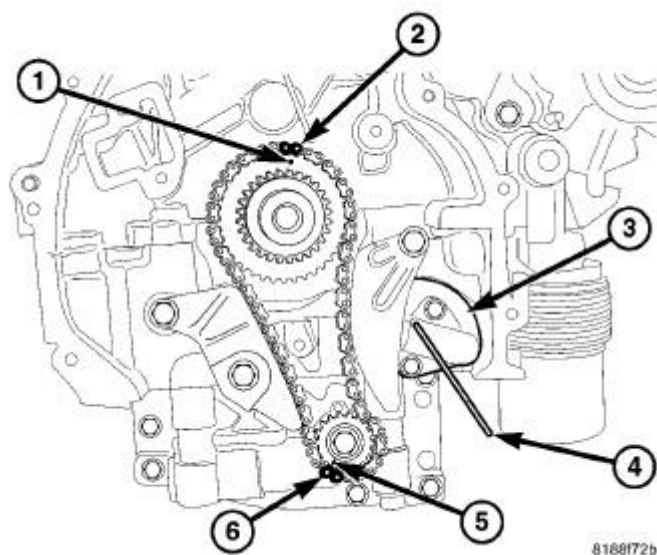
Fig. 323: BSM TENSIONER Courtesy of CHRYSLER LLC
