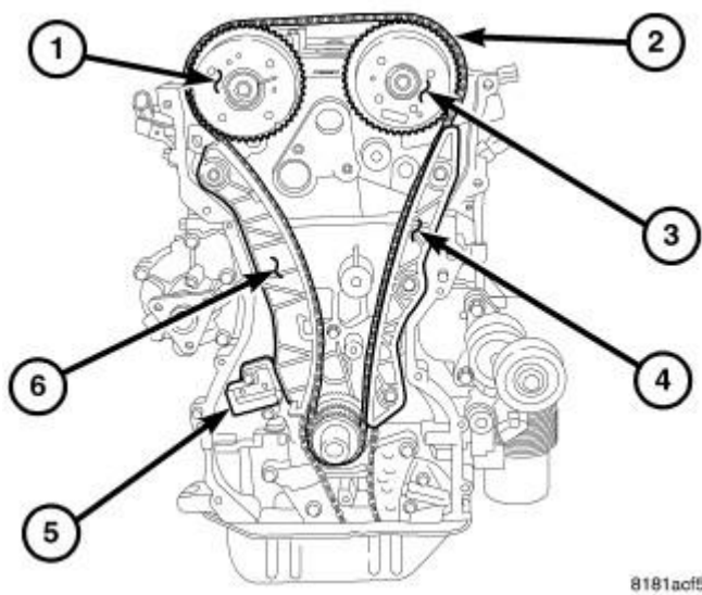
Fig. 442: TIMING DRIVE Courtesy of CHRYSLER LLC
