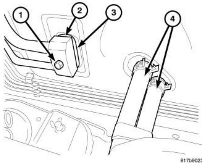
Fig. 364: Refrigerant Lines to Evaporator Bolt Courtesy of CHRYSLER LLC
