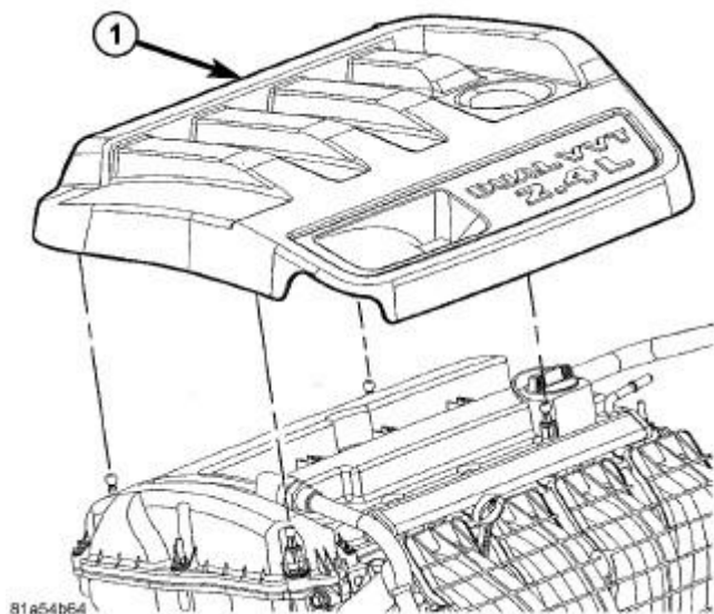
Fig. 149: Engine Cover
