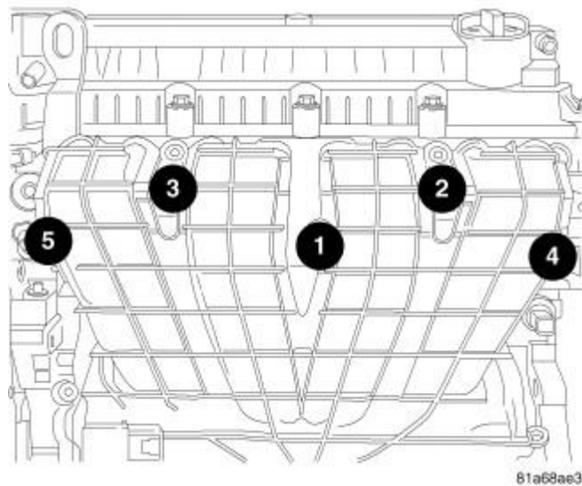
Fig. 105: Removing/Installing Intake Bolts - Torque Sequence Courtesy of CHRYSLER LLC
