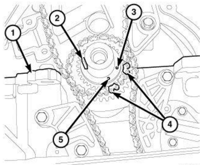
Fig. 407: Crankshaft Timing Marks
