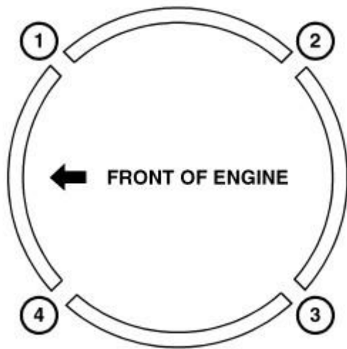
Fig. 257: Piston Ring End Gap Position Courtesy of CHRYSLER LLC
