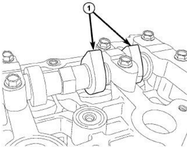
Fig. 140: LOBES VERTICAL Courtesy of CHRYSLER LLC
