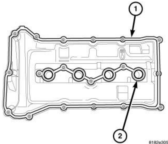
Fig. 177: GASKET LOCATION Courtesy of CHRYSLER LLC
