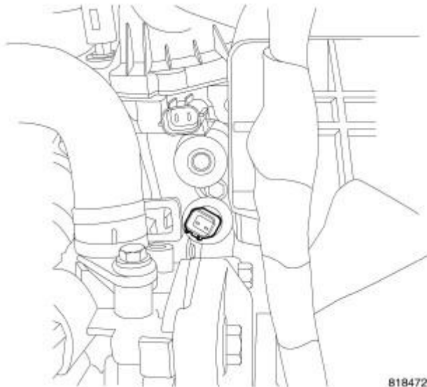
Fig. 291: OIL PRESSURE SENSOR Courtesy of CHRYSLER LLC
