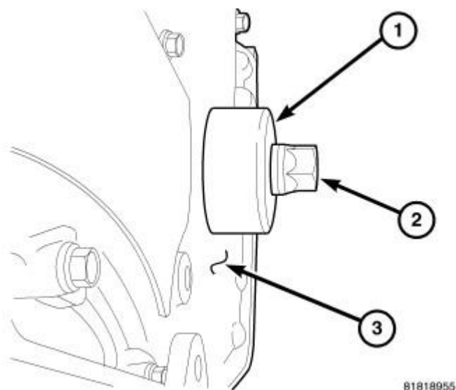
Fig. 266: FRONT SEAL INSTALLED Courtesy of CHRYSLER LLC
