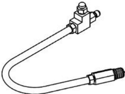
Fig. 63: ADAPTER, PRESSURE PEP - 8116 Courtesy of CHRYSLER LLC
