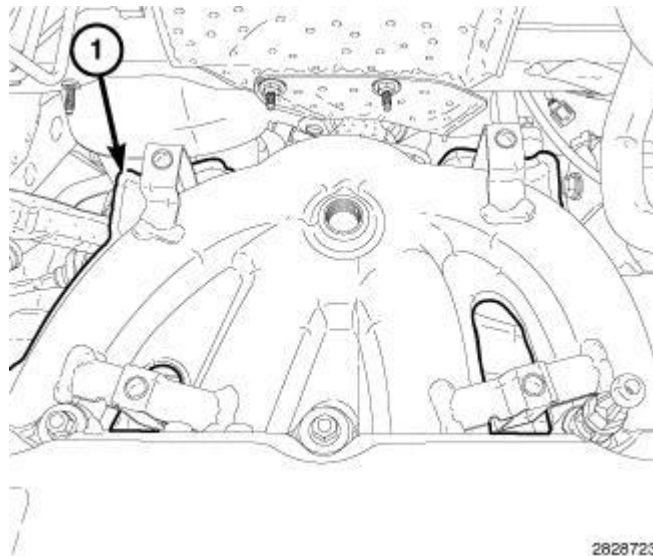
Fig. 362: Lower Maniverter Heatshield Courtesy of CHRYSLER LLC
