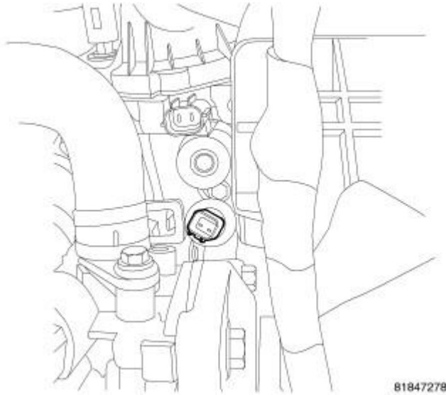
Fig. 284: OIL PRESSURE SENSOR Courtesy of CHRYSLER LLC
