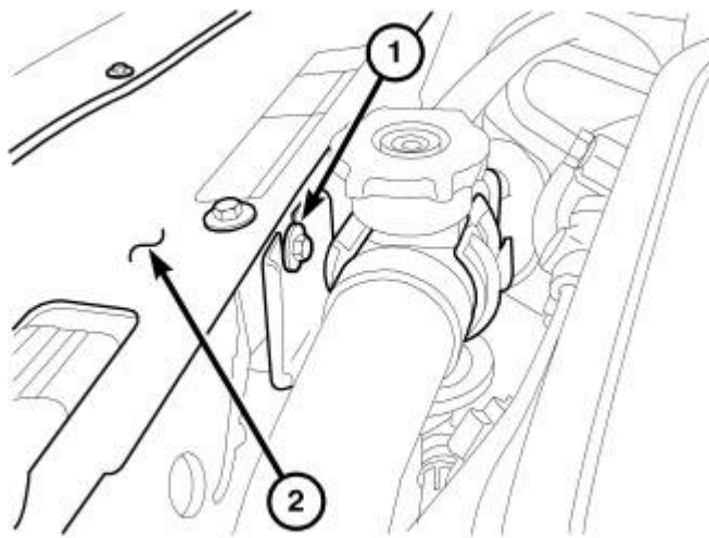
Fig. 15: Radiator Hose Support Courtesy of CHRYSLER LLC
