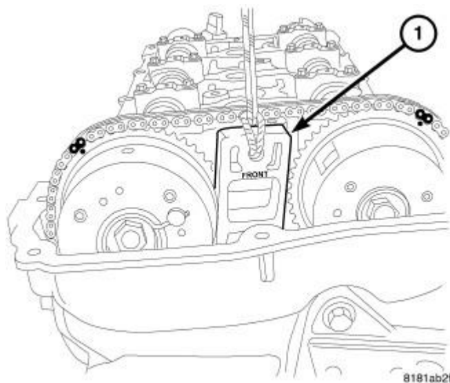
Fig. 154: WEDGE TOOL Courtesy of CHRYSLER LLC
