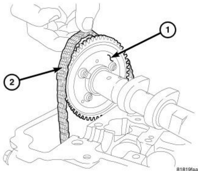
Fig. 159: Identifying Timing Chain & Sprocket Courtesy of CHRYSLER LLC
