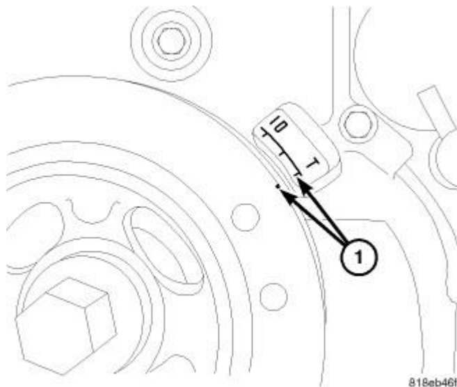
Fig. 414: Setting Crankshaft To Top Dead Center Courtesy of CHRYSLER LLC
