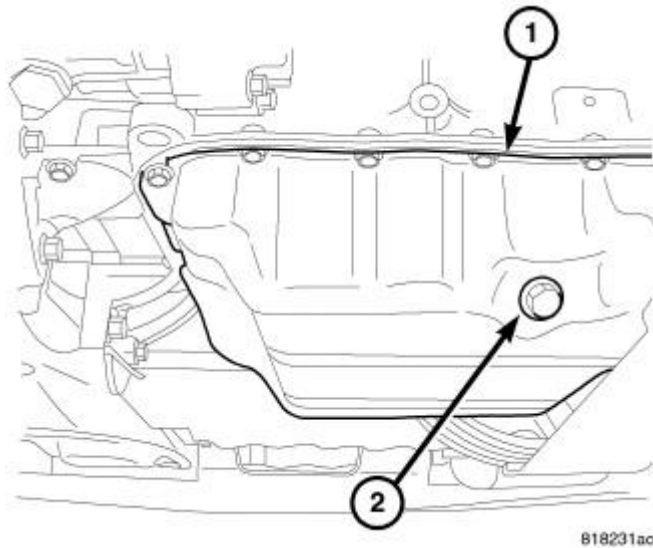
Fig. 311: OIL DRAIN PLUG Courtesy of CHRYSLER LLC
