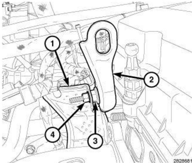
Fig. 345: Heatshield, Stud Bolt, Engine Lift Bracket & Nut Courtesy of CHRYSLER LLC
