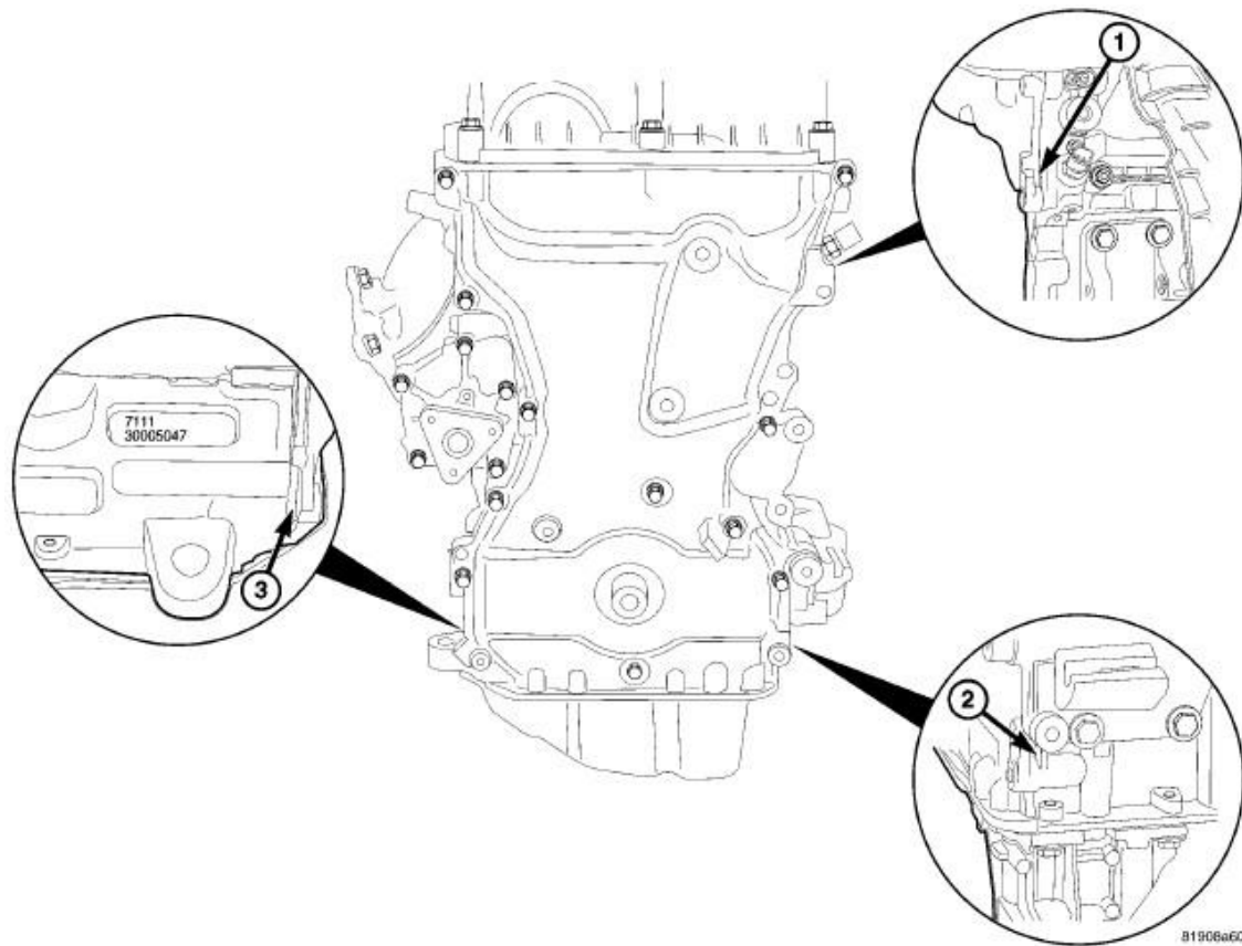
Fig. 97: TIMING CHAIN COVER PRY POINTS Courtesy of CHRYSLER LLC
