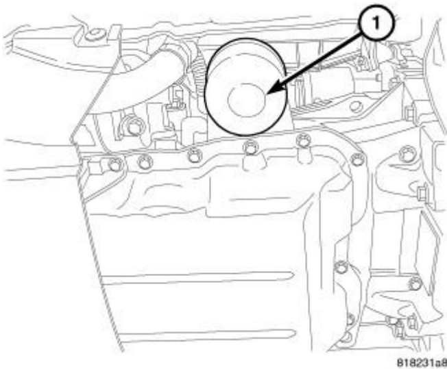
Fig. 298: Oil Filter
