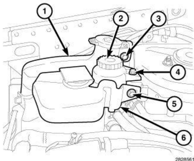
Fig. 359: Coolant Reservoir, Power Steering Fluid Reservoir, Washer Fluid Reservoir & Bolts Courtesy of CHRYSLER LLC
