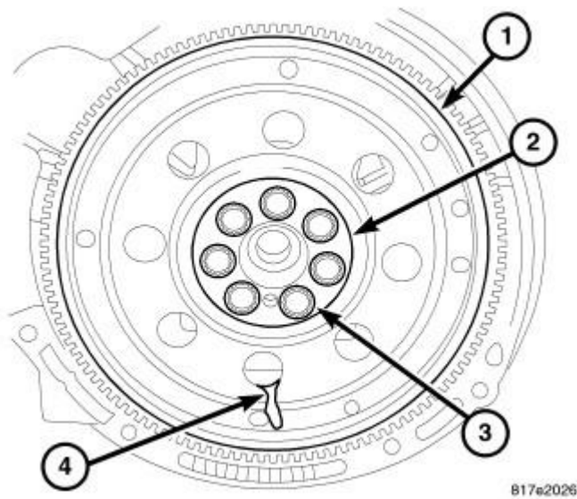
Fig. 240: FLEX PLATE
