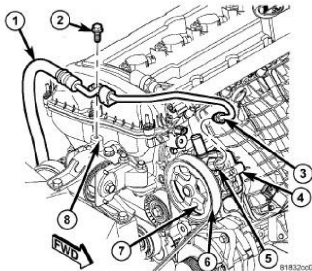
Fig. 85: PRESSURE HOSE Courtesy of CHRYSLER LLC
