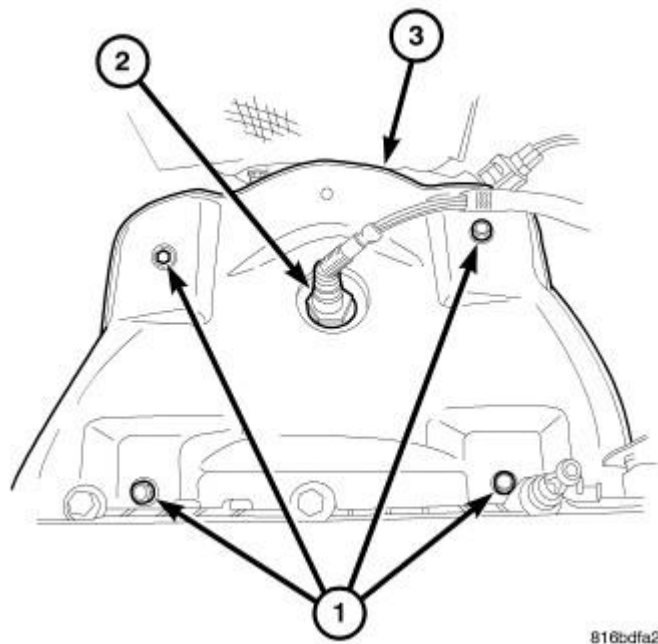
Fig. 335: ManiVerter Heat Shield And Bolts Courtesy of CHRYSLER LLC
