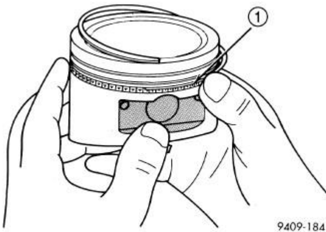
Fig. 248: Installing Side Rail Courtesy of CHRYSLER LLC
