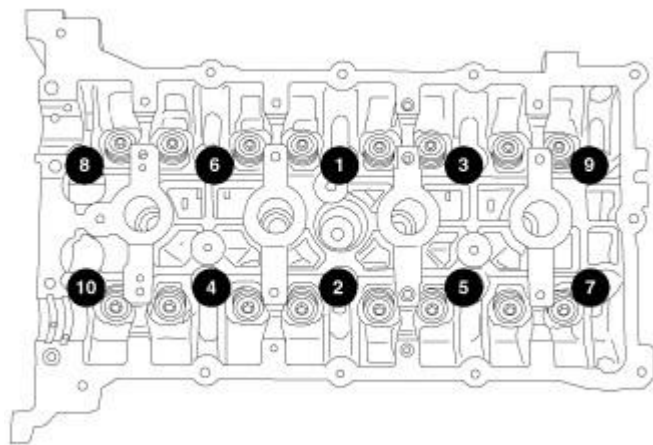
Fig. 119: Cylinder Head Torque Sequence
