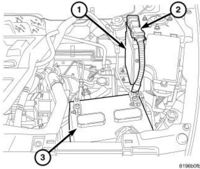
Fig. 193: BATTERY
