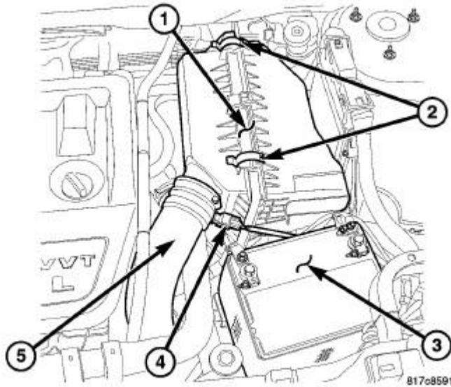
Fig. 79: AIR CLEANER HOUSING Courtesy of CHRYSLER LLC
