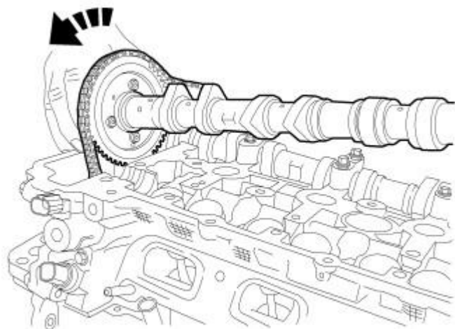
Fig. 158: Rotating Camshaft While Lifting Out Of Front Bearing Cradle Courtesy of CHRYSLER LLC
