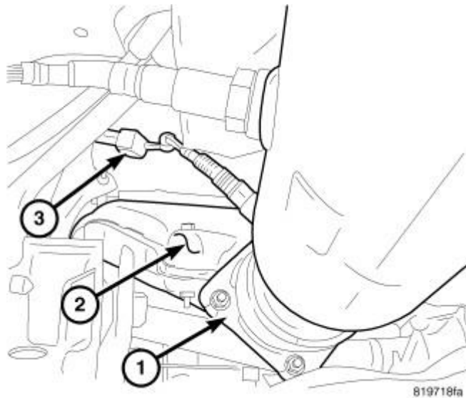
Fig. 24: Exhaust Pipe To Manifold Bolts Courtesy of CHRYSLER LLC
