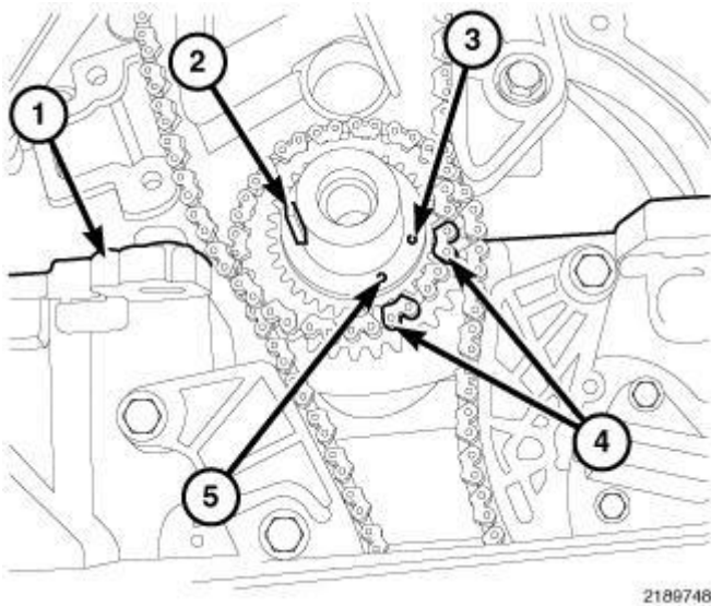
Fig. 395: Crankshaft Timing Marks Courtesy of CHRYSLER LLC
