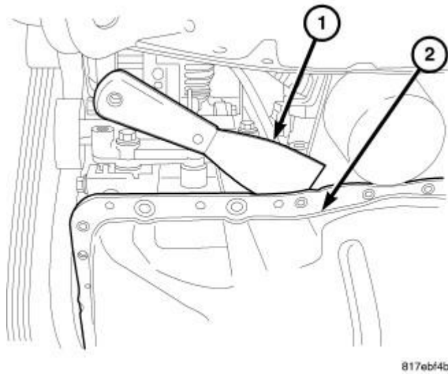
Fig. 220: OIL PAN REMOVAL
