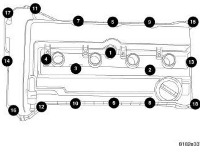
Fig. 172: Cylinder Head Cover Bolt Torque Sequence
