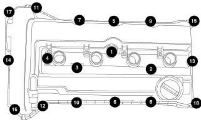
Fig. 413: Cylinder Head Cover Bolt Torque Sequence Courtesy of CHRYSLER LLC
