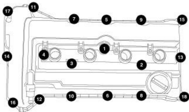
Fig. 143: TORQUE SEQUENCE
