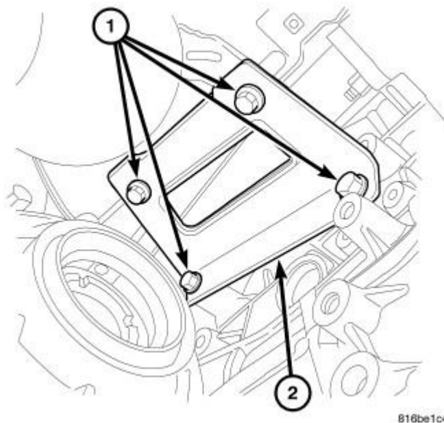
Fig. 341: Maniverter To Block Support Bracket Courtesy of CHRYSLER LLC
