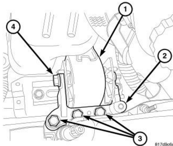
Fig. 94: RIGHT ENGINE MOUNT Courtesy of CHRYSLER LLC
