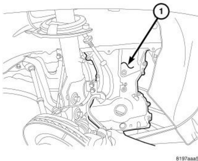
Fig. 423: TIMING CHAIN COVER REMOVAL Courtesy of CHRYSLER LLC
