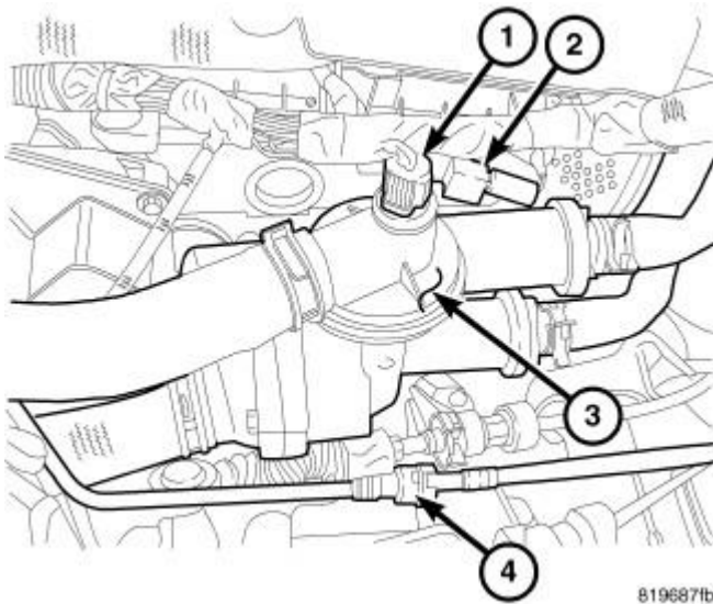
Fig. 102: COOLANT ADAPTER Courtesy of CHRYSLER LLC
