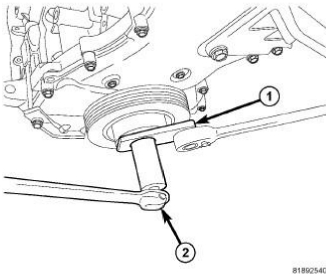
Fig. 238: DAMPER REMOVAL Courtesy of CHRYSLER LLC
