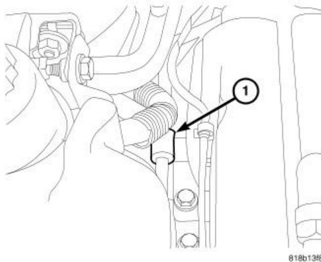
Fig. 204: POWER STEERING LINE SUPPORT Courtesy of CHRYSLER LLC
