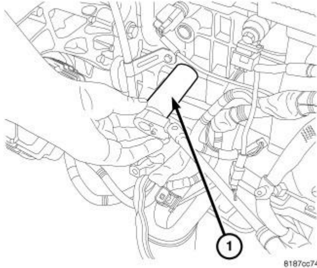
Fig. 327: OIL SENDER Courtesy of CHRYSLER LLC
