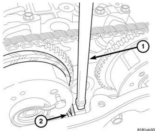
Fig. 155: SEATING WEDGE TOOL
