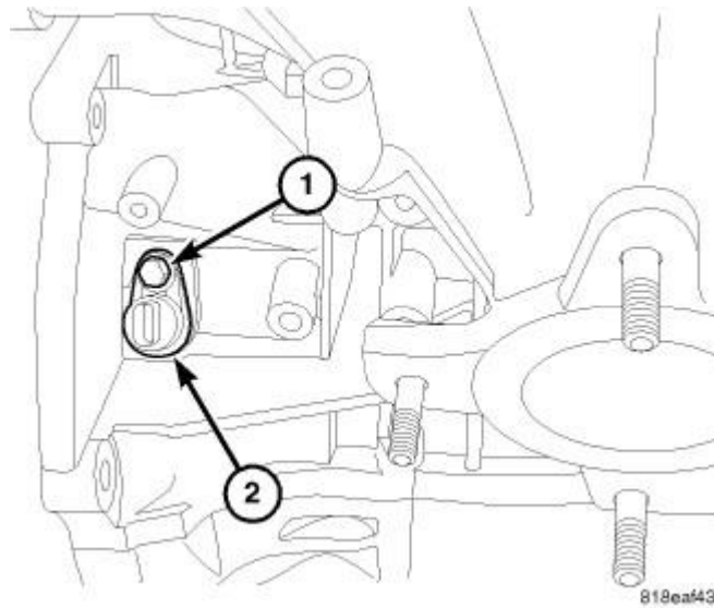
Fig. 37: Crankshaft Position Sensor Courtesy of CHRYSLER LLC
