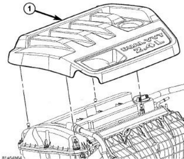
Fig. 351: Engine Cover Courtesy of CHRYSLER LLC
