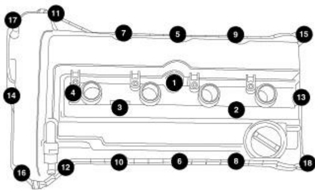
Fig. 176: Cylinder Head Cover Bolt Torque Sequence Courtesy of CHRYSLER LLC
