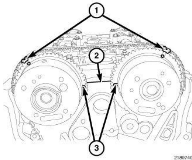
Fig. 406: Timing Chain Timing Marks
