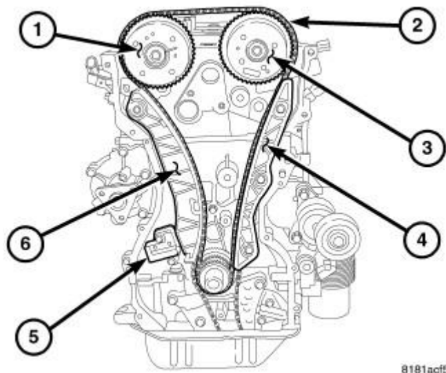
Fig. 98: TIMING DRIVE Courtesy of CHRYSLER LLC
