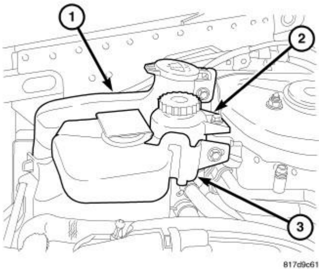
Fig. 200: COOLANT RESERVOIR Courtesy of CHRYSLER LLC
