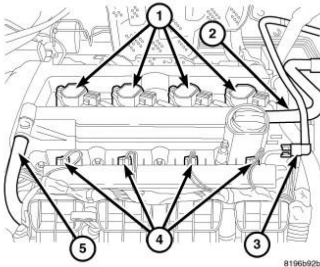
Fig. 175: COIL CONNECTOR Courtesy of CHRYSLER LLC
