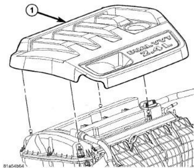
Fig. 409: Engine Cover Courtesy of CHRYSLER LLC
