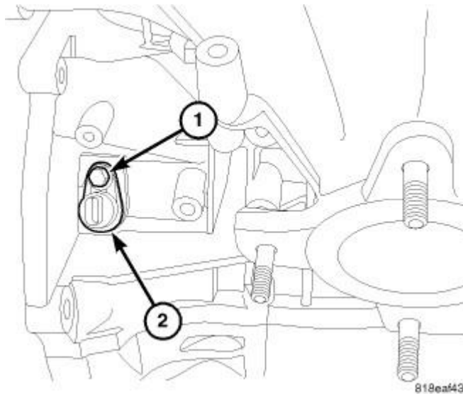
Fig. 29: CRANKSHAFT POSITION SENSOR Courtesy of CHRYSLER LLC
