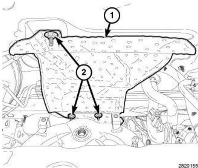
Fig. 343: Dash Panel Heatshield & Nuts Courtesy of CHRYSLER LLC
