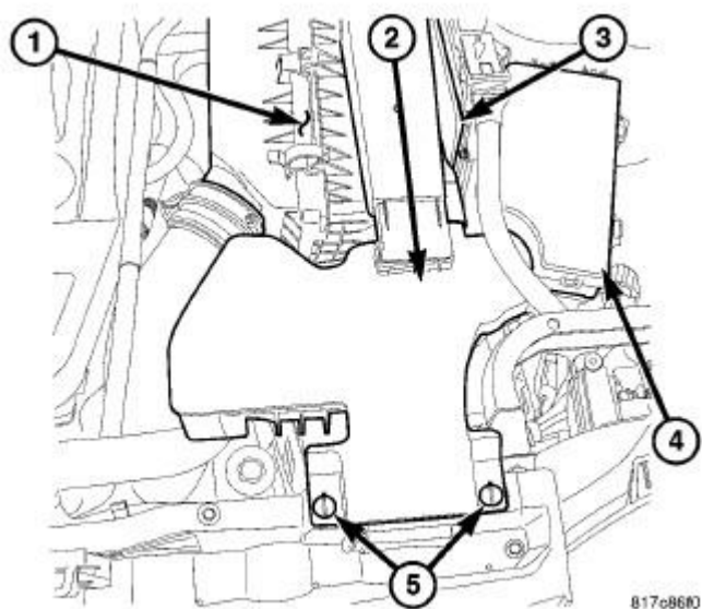
Fig. 373: Air Cleaner Housing, Fresh Air Inlet & Lock Retainers Courtesy of CHRYSLER LLC
