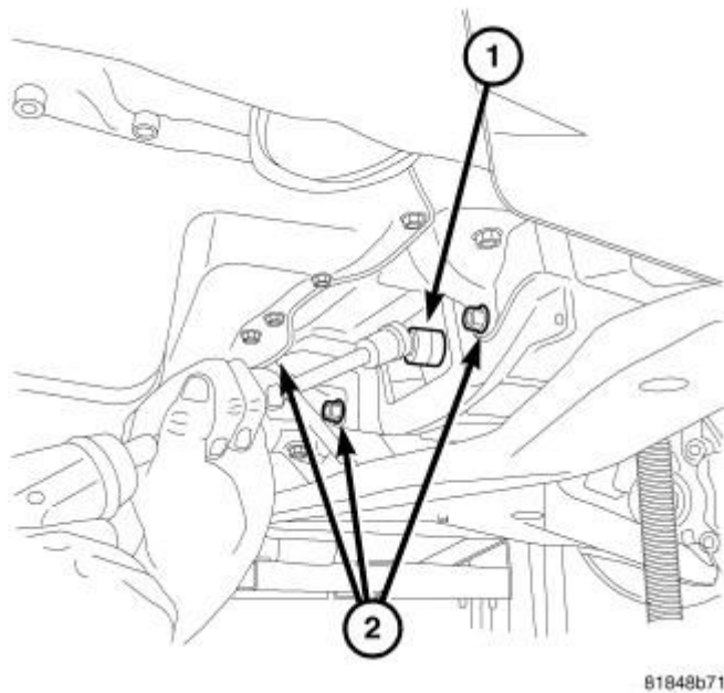
Fig. 27: MODULAR CLUTCH TO FLEX PLATE BOLTS Courtesy of CHRYSLER LLC
