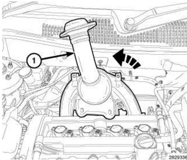
Fig. 350: Rotating Mani-Verter Counterclockwise Courtesy of CHRYSLER LLC
