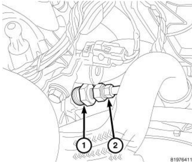
Fig. 275: OIL PRESSURE ADAPTER 9879 Courtesy of CHRYSLER LLC
