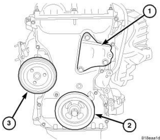
Fig. 234: RIGHT ENGINE MOUNT BRACKET Courtesy of CHRYSLER LLC
