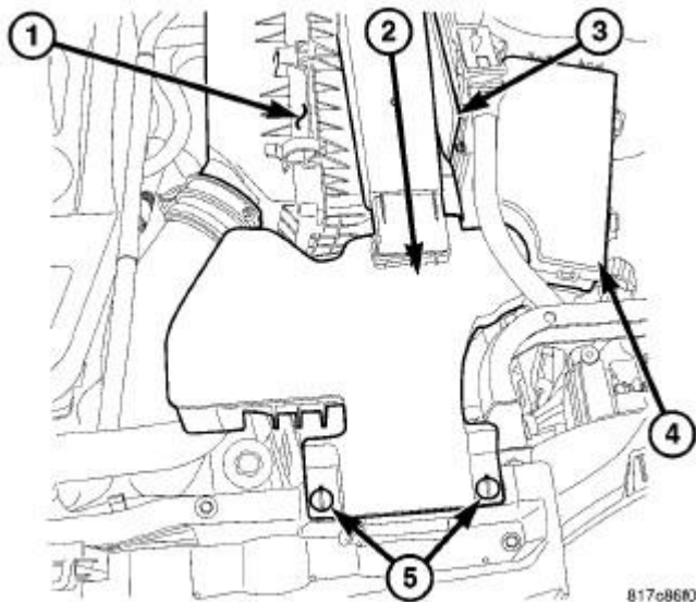
Fig. 72: AIR CLEANER INLET Courtesy of CHRYSLER LLC
