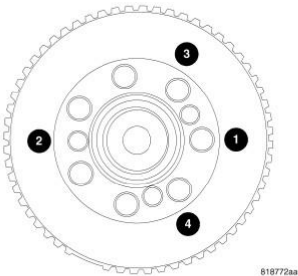
Fig. 227: TARGET WHEEL Courtesy of CHRYSLER LLC
