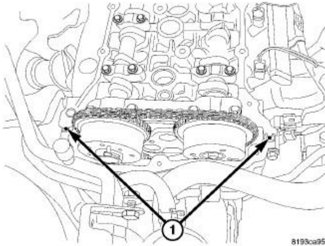
Fig. 179: Applying RTV To Cylinder Head/Front Cover T-Joint Courtesy of CHRYSLER LLC
