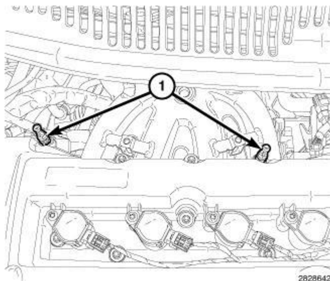
Fig. 360: Engine Cover Mounting Posts Courtesy of CHRYSLER LLC
