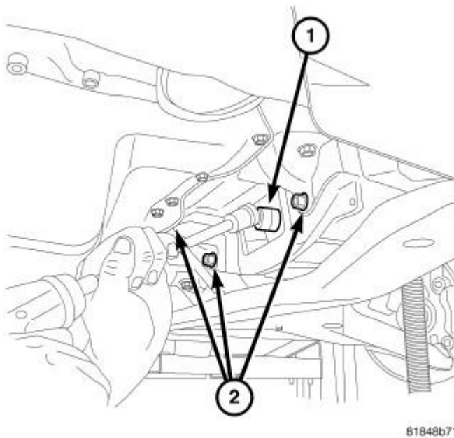
Fig. 35: MODULAR CLUTCH TO FLEX PLATE BOLT Courtesy of CHRYSLER LLC
