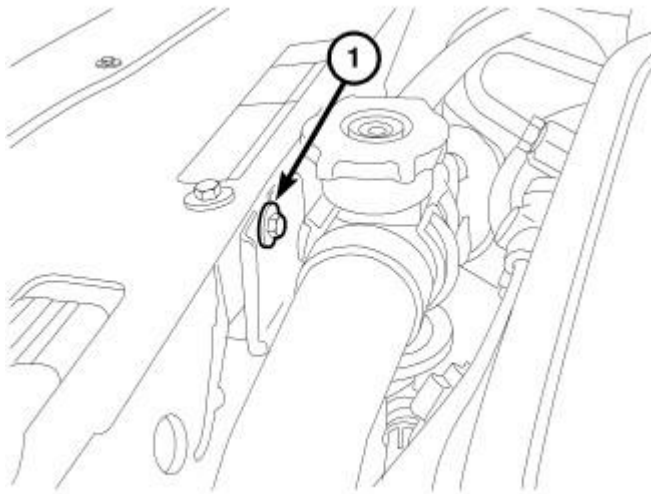
Fig. 386: RADIATOR HOSE SUPPORT Courtesy of CHRYSLER LLC
