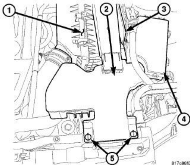
Fig. 381: AIR CLEANER INLET Courtesy of CHRYSLER LLC
