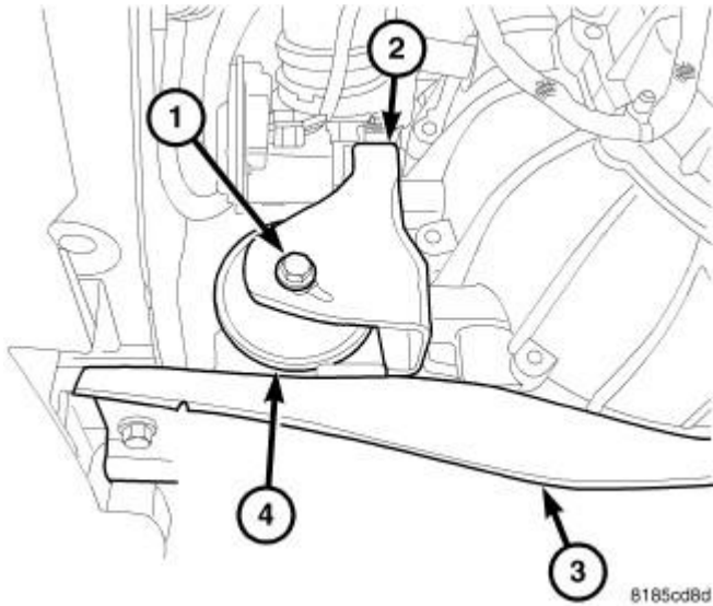
Fig. 190: FRONT MOUNT THROUGH BOLT Courtesy of CHRYSLER LLC
