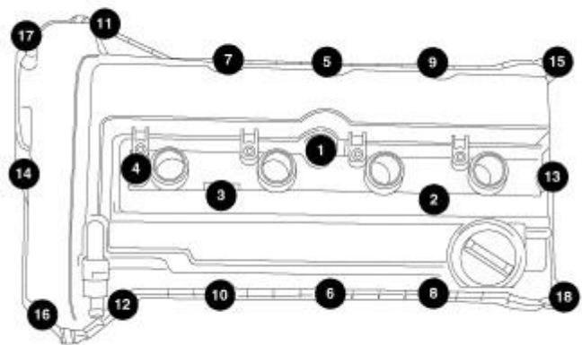
Fig. 436: Remove/Install Cylinder Head Cover Bolts In Sequence Courtesy of CHRYSLER LLC
