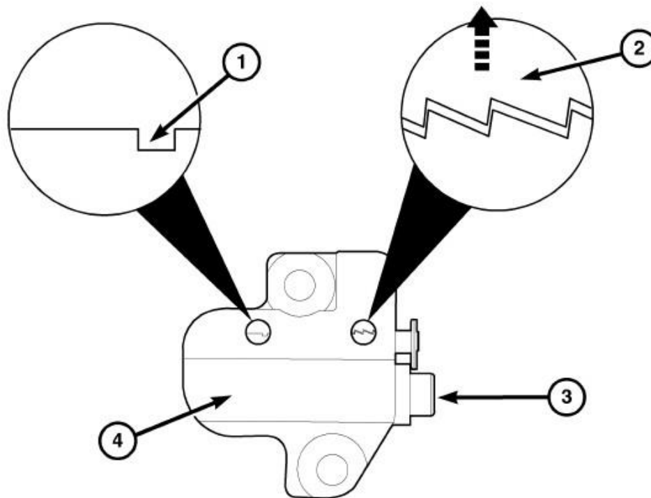
Fig. 153: TENSIONER RESET Courtesy of CHRYSLER LLC
