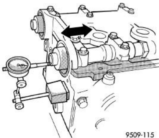
Fig. 148: Camshaft End Play Courtesy of CHRYSLER LLC
