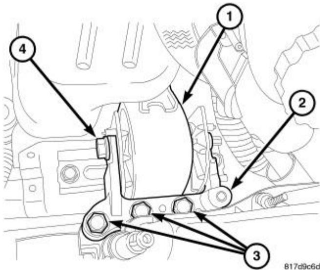
Fig. 203: RIGHT ENGINE MOUNT Courtesy of CHRYSLER LLC
