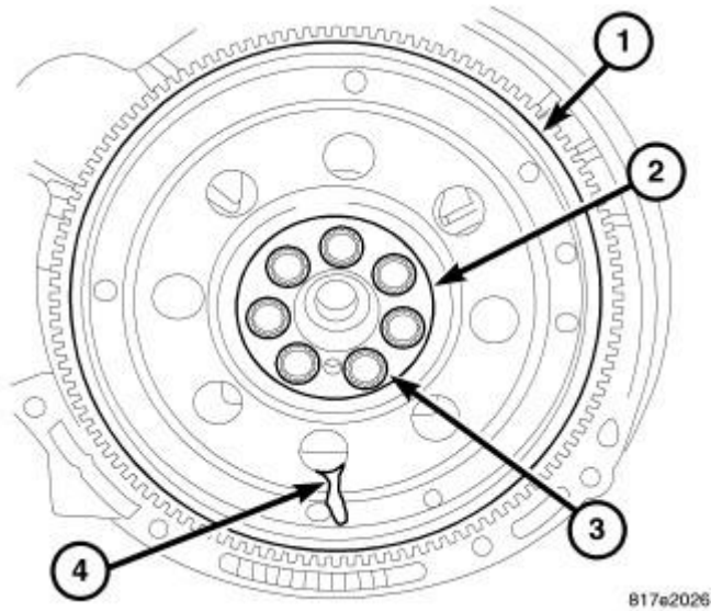
Fig. 271: FLEX PLATE Courtesy of CHRYSLER LLC
