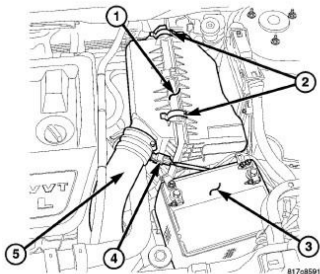
Fig. 390: AIR CLEANER HOUSING
