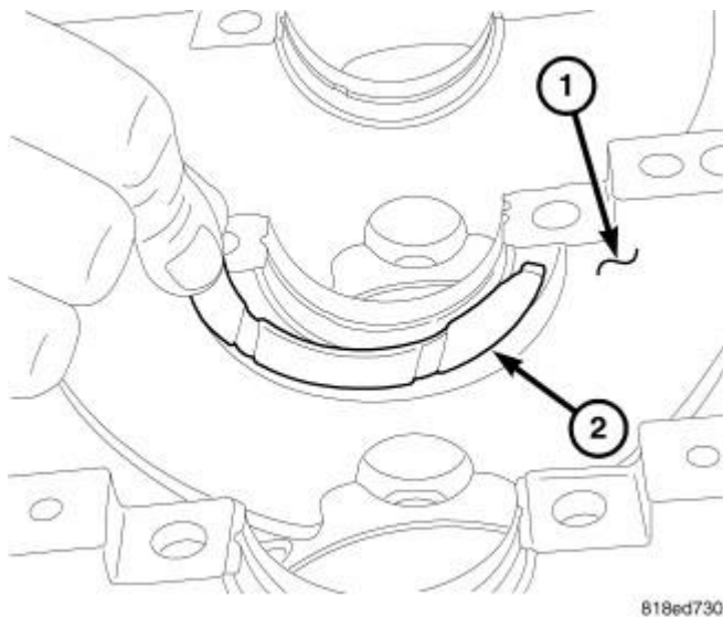
Fig. 228: INSTALLING THRUST BEARING Courtesy of CHRYSLER LLC
