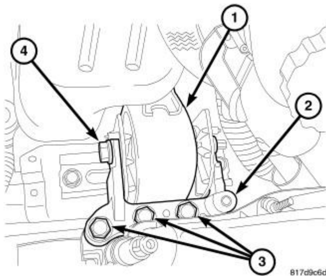
Fig. 34: RIGHT ENGINE MOUNT
