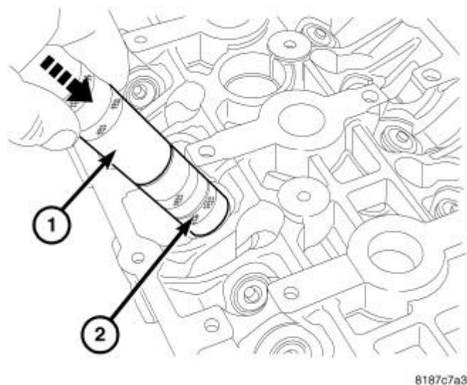
Fig. 186: VALVE INSTALLATION
