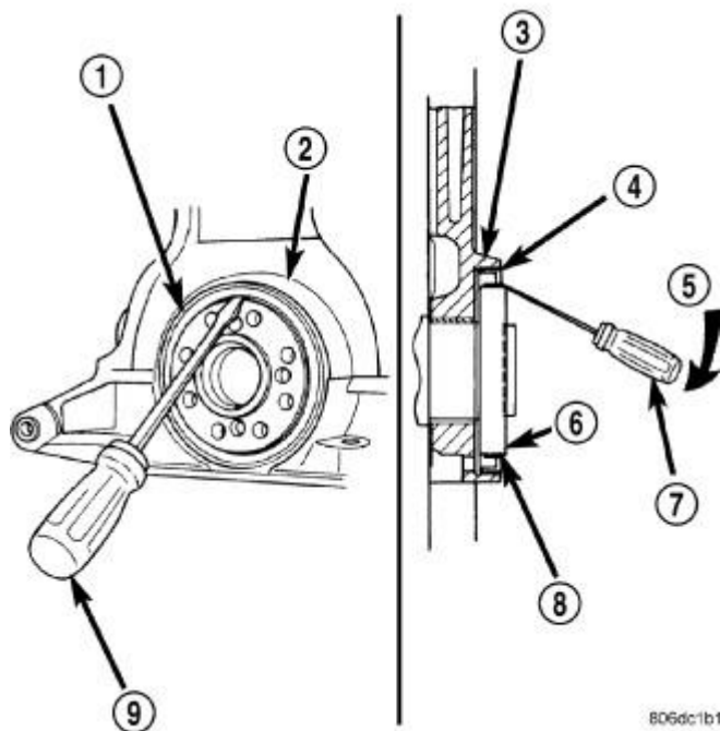
Fig. 269: Rear Crankshaft Oil Seal - Removal
