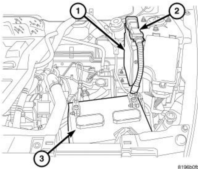
Fig. 11: Battery Courtesy of CHRYSLER LLC
