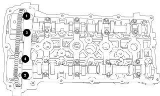
Fig. 108: Removing/Installing Front Camshaft Bearing Caps Courtesy of CHRYSLER LLC
