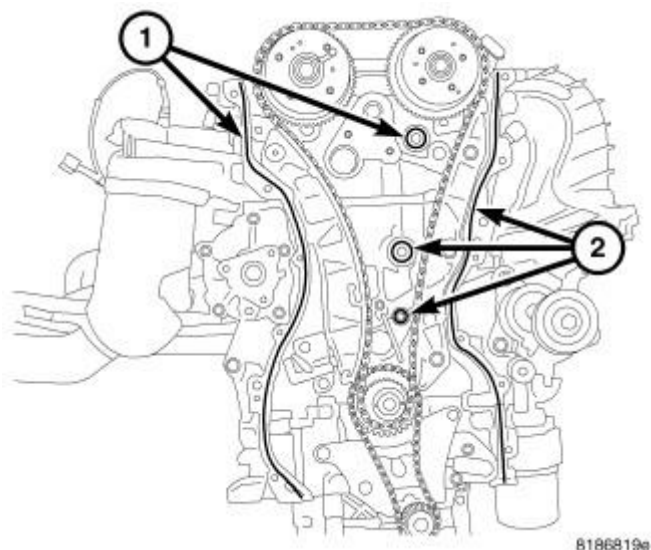
Fig. 427: TIMING CHAIN COVER SEALING Courtesy of CHRYSLER LLC
