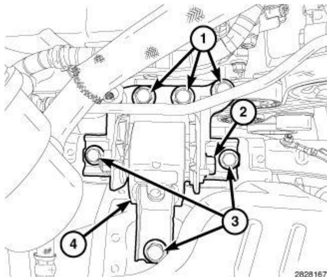
Fig. 357: Engine Mount Isolator, Right Engine Mount & Engine Mount Bracket Retaining Bolts Courtesy of CHRYSLER LLC
