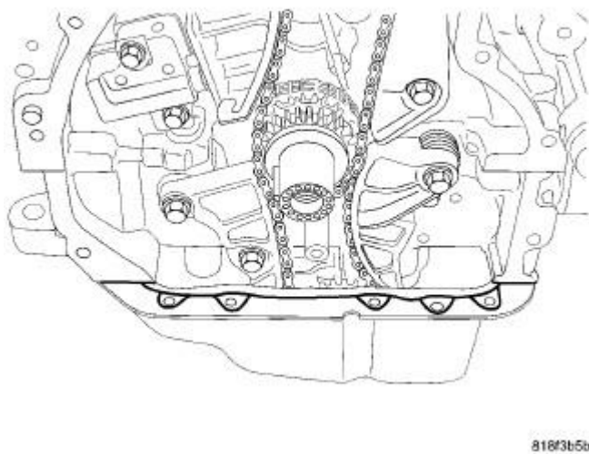
Fig. 426: SEALING OIL PAN Courtesy of CHRYSLER LLC
