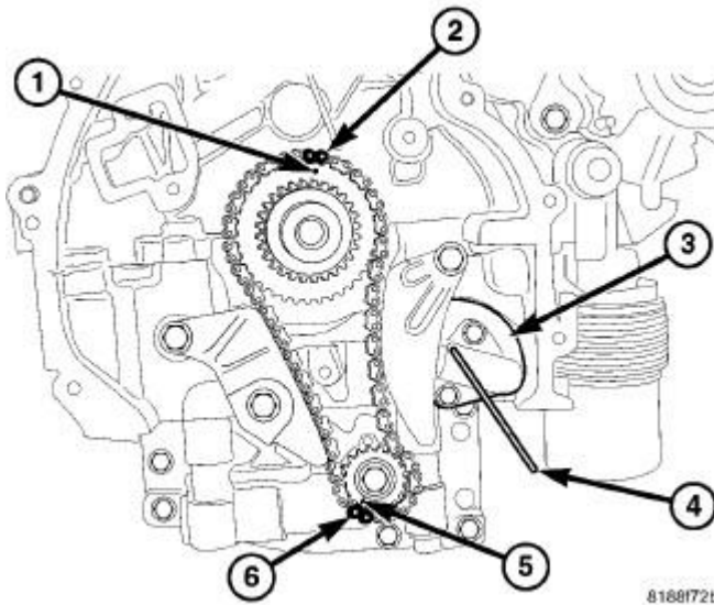
Fig. 317: BSM TENSIONER Courtesy of CHRYSLER LLC
