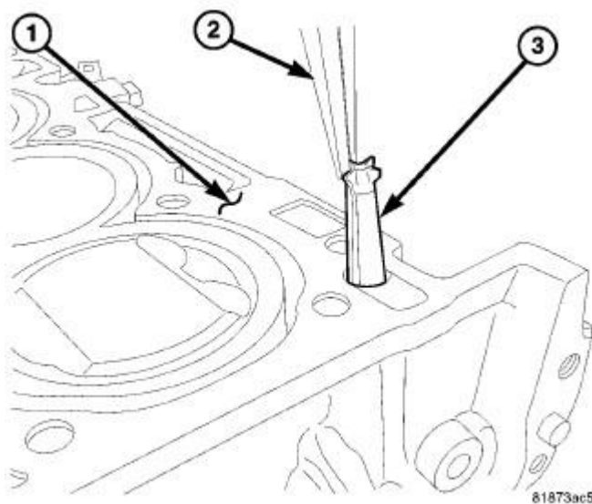
Fig. 113: Removing/Installing VVT Filter Screen Courtesy of CHRYSLER LLC
