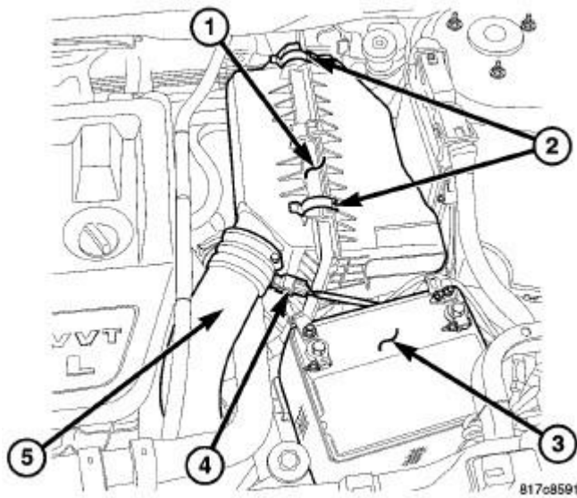
Fig. 382: AIR CLEANER HOUSING Courtesy of CHRYSLER LLC
