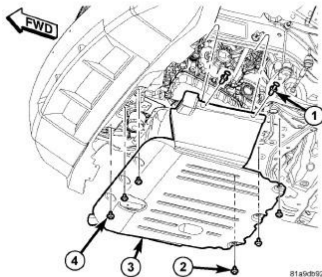
Fig. 337: Belly Pan Courtesy of CHRYSLER LLC
