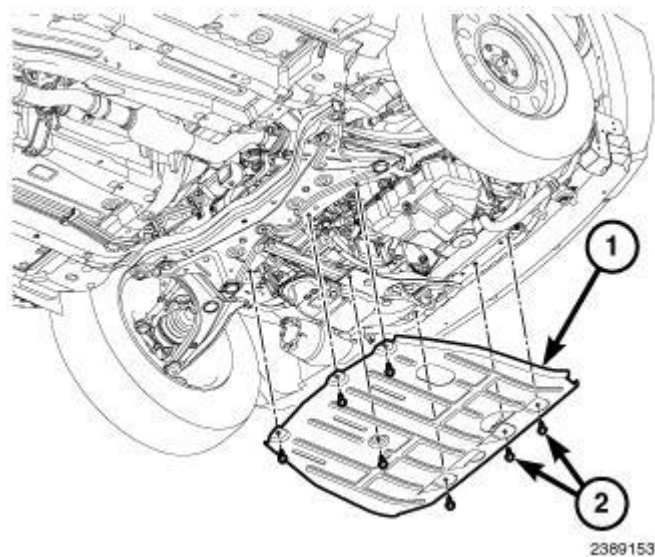
Fig. 370: Removal/Installation Front Skid Plate And Bolts
