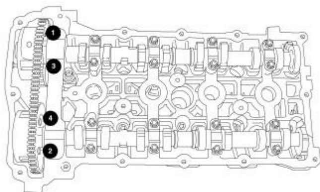
Fig. 156: Removing/Installing Front Camshaft Bearing Caps
