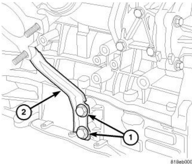
Fig. 376: EXHAUST MANIFOLD SUPPORT BRACKET Courtesy of CHRYSLER LLC
