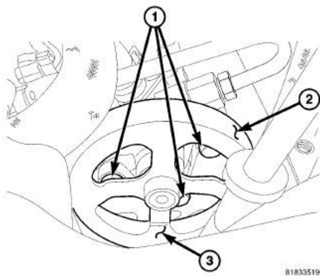
Fig. 437: POWER STEERING PUMP - GAS Courtesy of CHRYSLER LLC
