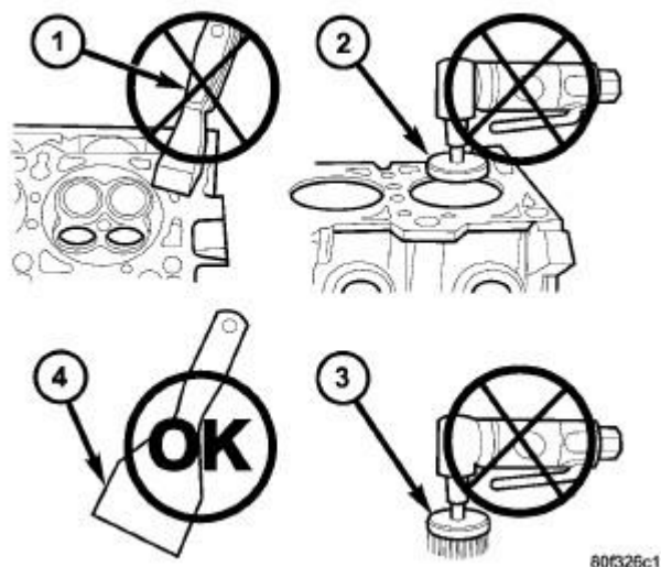
Fig. 110: Proper Tool Usage for Surface Preparation Courtesy of CHRYSLER LLC
