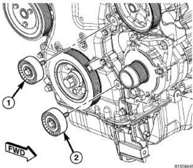
Fig. 434: ACCESSORY DRIVE BELT IDLER PULLEY - 2.4L Courtesy of CHRYSLER LLC
