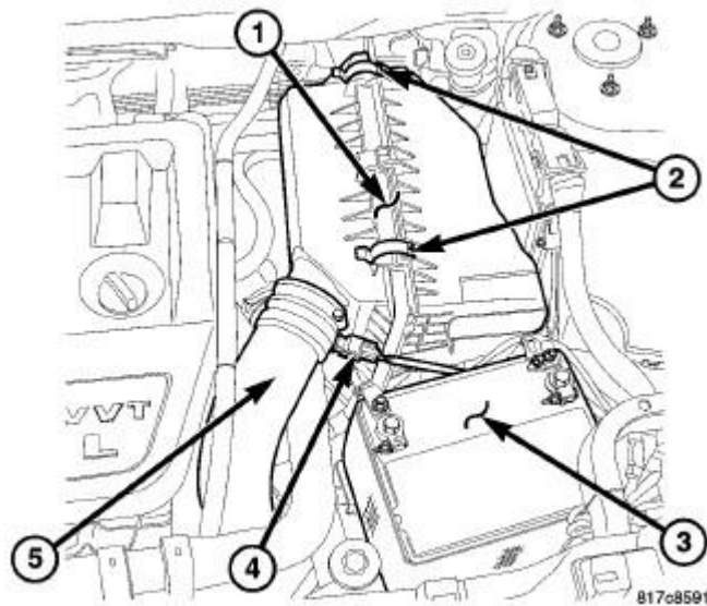
Fig. 55: AIR CLEANER HOUSING Courtesy of CHRYSLER LLC
