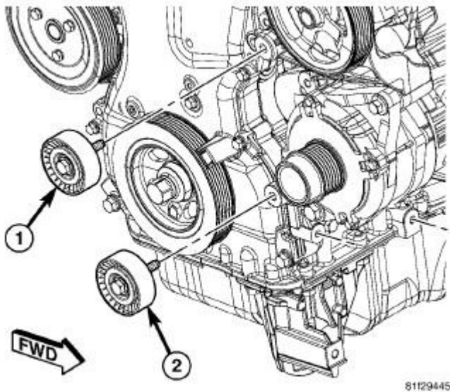
Fig. 430: ACCESSORY DRIVE BELT IDLER PULLEY - 2.4L Courtesy of CHRYSLER LLC
