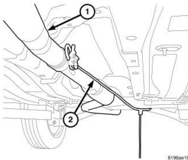
Fig. 25: Exhaust Pipe Courtesy of CHRYSLER LLC
