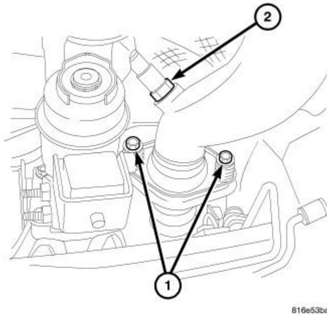
Fig. 338: Exhaust To Maniventer Bolts Courtesy of CHRYSLER LLC
