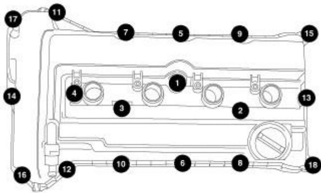
Fig. 139: Cylinder Head Cover Bolt Torque Sequence Courtesy of CHRYSLER LLC
