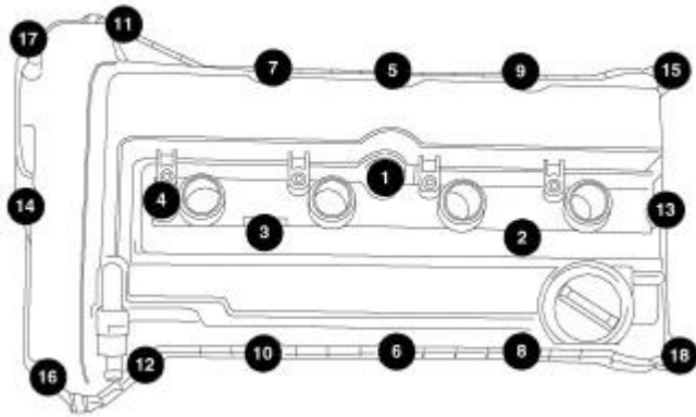
Fig. 128: Cylinder Head Cover Bolt Torque Sequence Courtesy of CHRYSLER LLC
