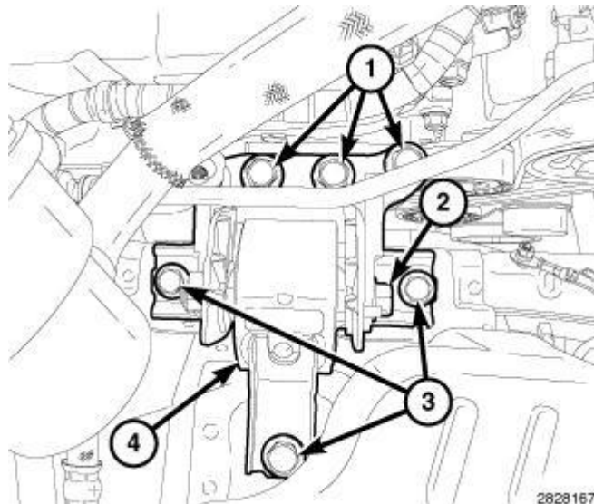
Fig. 349: Engine Mount Isolator, Right Engine Mount & Engine Mount Bracket Retaining Bolts Courtesy of CHRYSLER LLC
