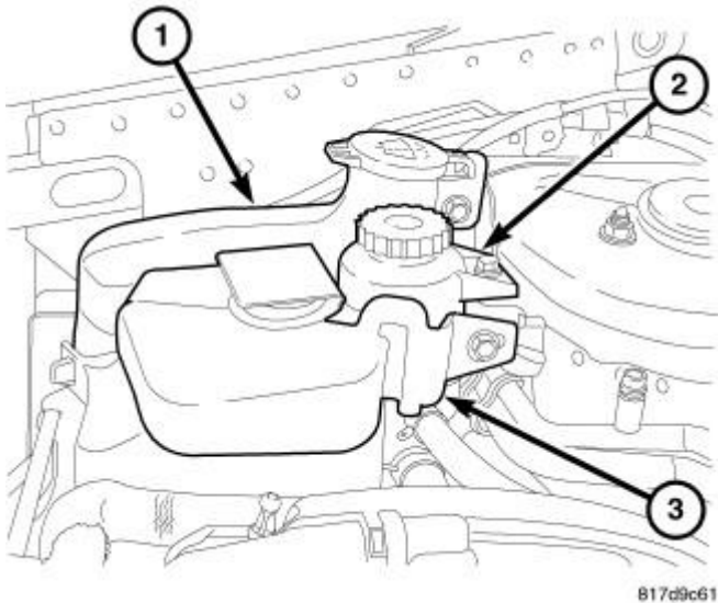
Fig. 13: Coolant Reservoir Courtesy of CHRYSLER LLC
