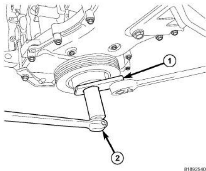
Fig. 267: Damper Removal Courtesy of CHRYSLER LLC
