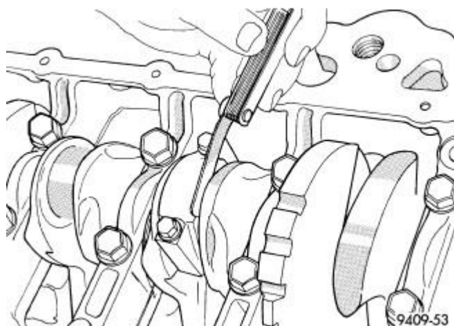
Fig. 260: Connecting Rod Side Clearance Courtesy of CHRYSLER LLC
