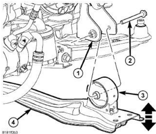
Fig. 340: Fore/Aft Crossmember 2 Courtesy of CHRYSLER LLC
