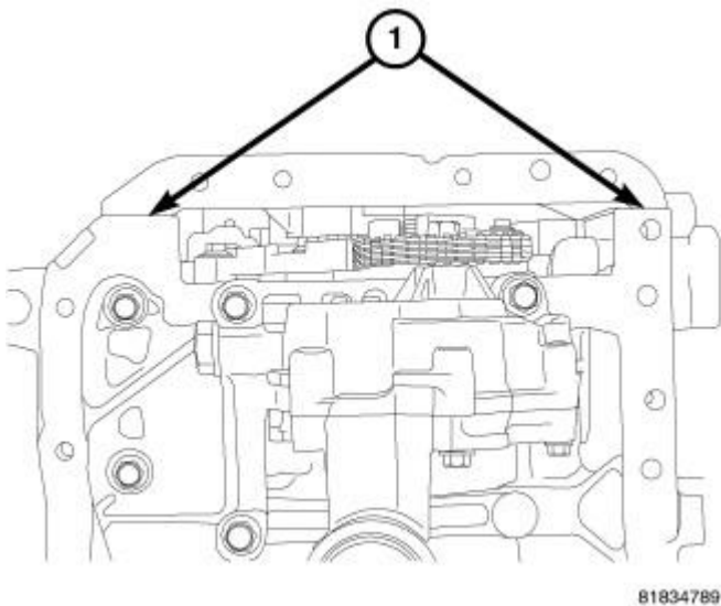
Fig. 309: SEALER LOCATION Courtesy of CHRYSLER LLC
