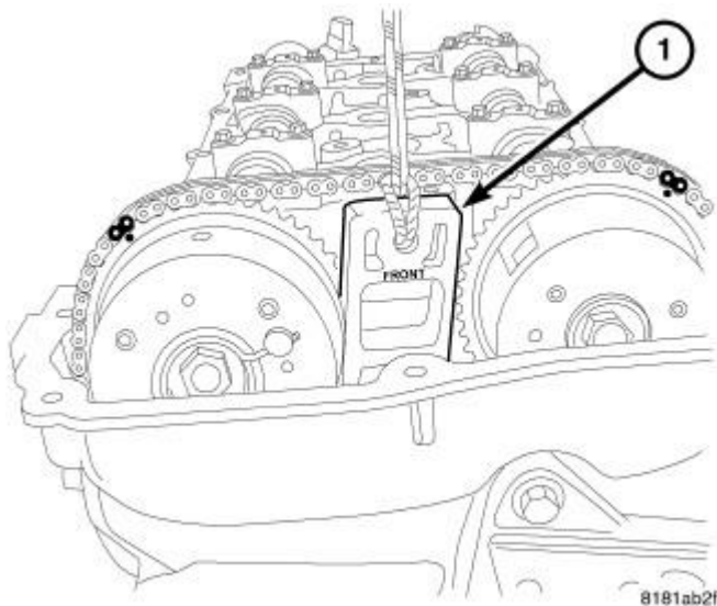
Fig. 168: WEDGE TOOL Courtesy of CHRYSLER LLC
