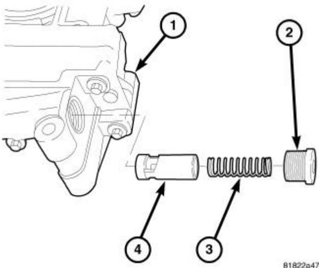
Fig. 332: OIL PRESSURE RELIEF VALVE
