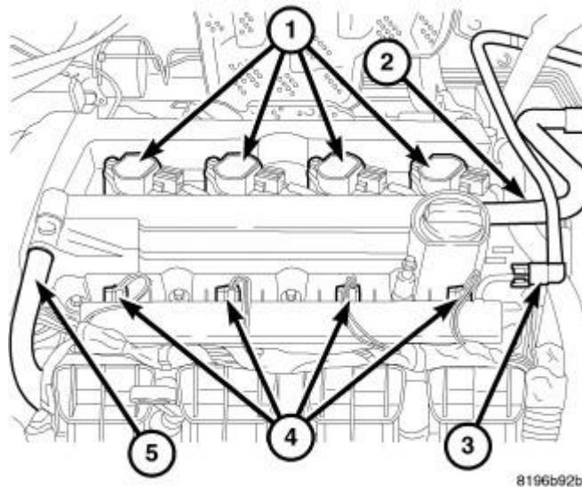
Fig. 181: Coil Connector
