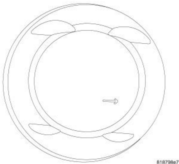
Fig. 258: PISTON INSTALLATION Courtesy of CHRYSLER LLC
