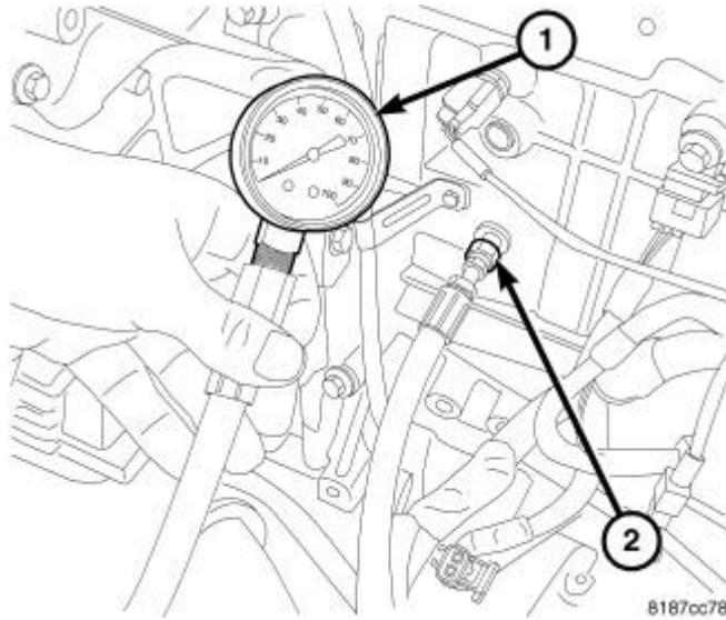
Fig. 281: OIL PRESSURE GAUGE Courtesy of CHRYSLER LLC
