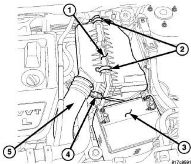
Fig. 83: AIR CLEANER HOUSING
