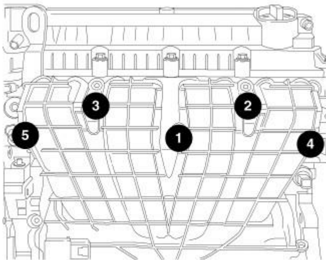
Fig. 387: Removing/Installing Intake Bolts - Torque Sequence Courtesy of CHRYSLER LLC
