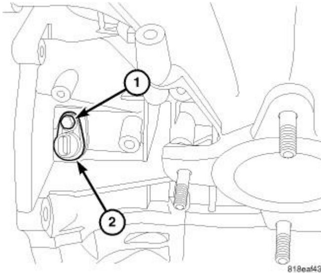
Fig. 222: CRANKSHAFT POSITION SENSOR Courtesy of CHRYSLER LLC
