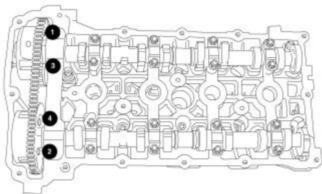
Fig. 126: Front Cam Cap Torque Sequence
