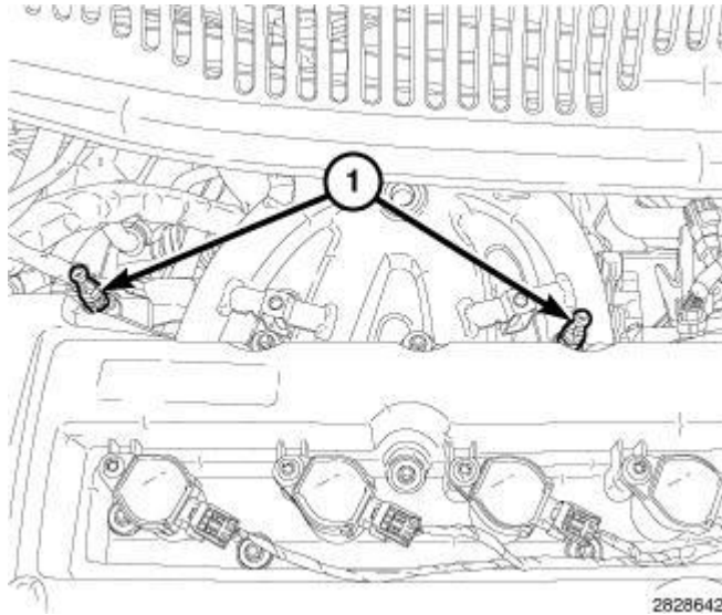
Fig. 346: Engine Cover Mounting Posts Courtesy of CHRYSLER LLC
