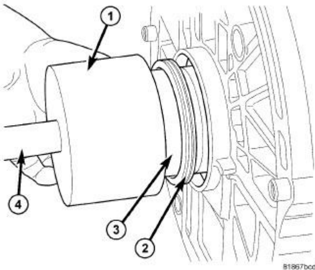
Fig. 270: REAR MAIN INSTALLATION Courtesy of CHRYSLER LLC
