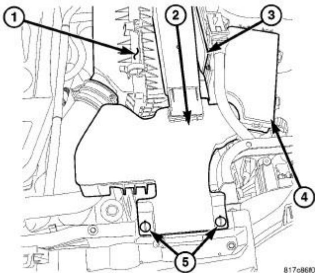
Fig. 192: AIR CLEANER INLET
