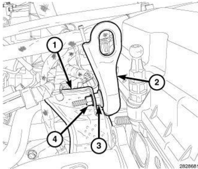
Fig. 361: Heatshield, Stud Bolt, Engine Lift Bracket & Nut Courtesy of CHRYSLER LLC
