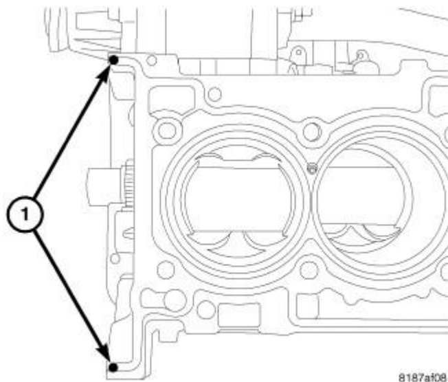
Fig. 115: Cylinder Head Gasket RTV Courtesy of CHRYSLER LLC
