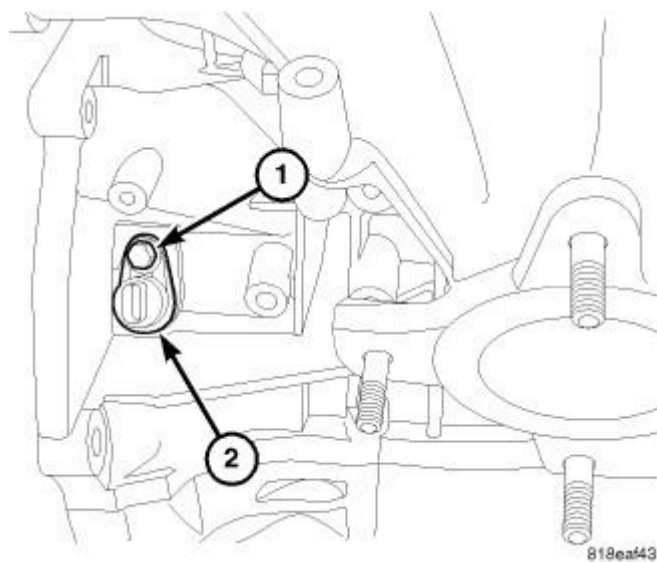
Fig. 232: CRANKSHAFT POSITION SENSOR Courtesy of CHRYSLER LLC
