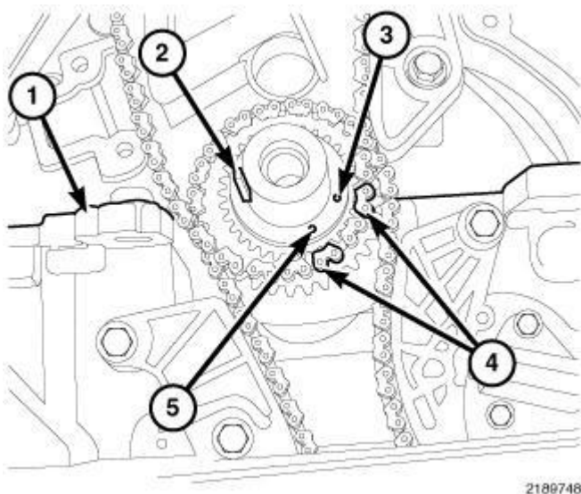
Fig. 405: Crankshaft Timing Marks Courtesy of CHRYSLER LLC
