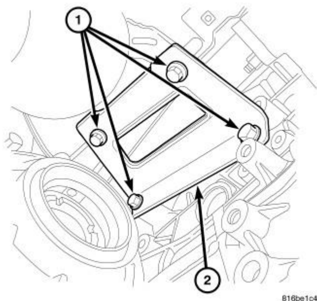
Fig. 365: Maniverter To Block Support Bracket Courtesy of CHRYSLER LLC
