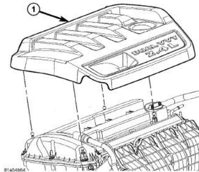
Fig. 173: Engine Cover Courtesy of CHRYSLER LLC
