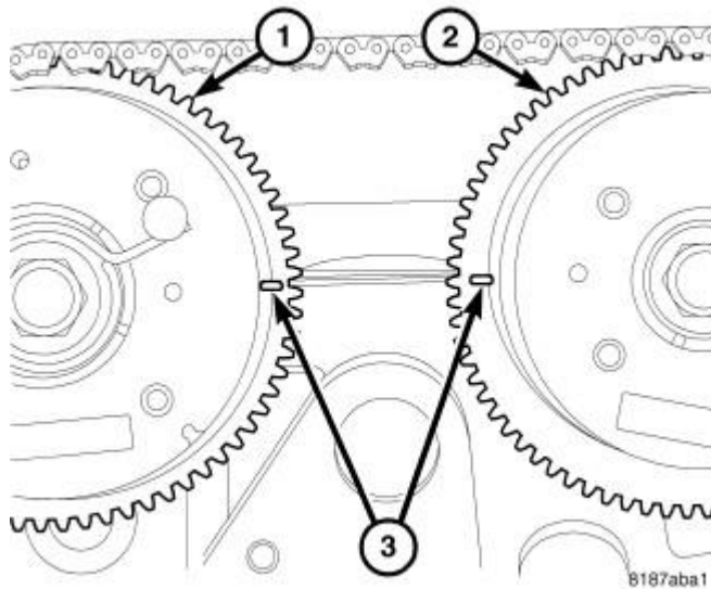
Fig. 394: Camshaft Timing Courtesy of CHRYSLER LLC
