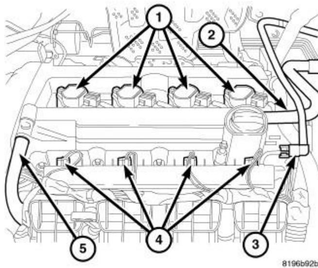
Fig. 8: Coil Connector Courtesy of CHRYSLER LLC
