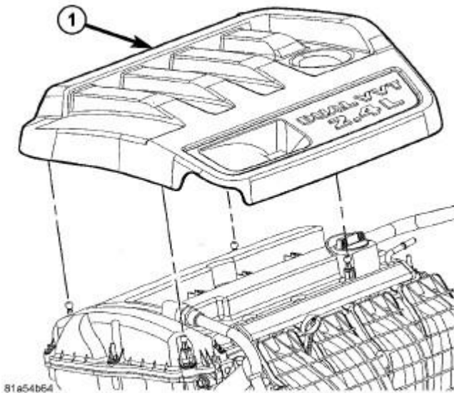
Fig. 32: ENGINE COVER-2.4L Courtesy of CHRYSLER LLC
