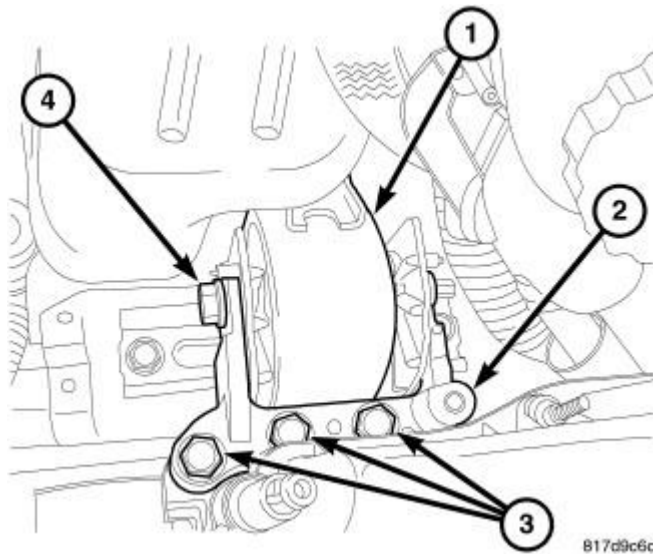
Fig. 202: RIGHT ENGINE MOUNT Courtesy of CHRYSLER LLC
