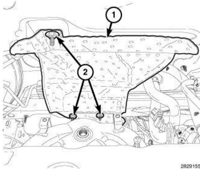
Fig. 363: Dash Panel Heatshield & Nuts Courtesy of CHRYSLER LLC
