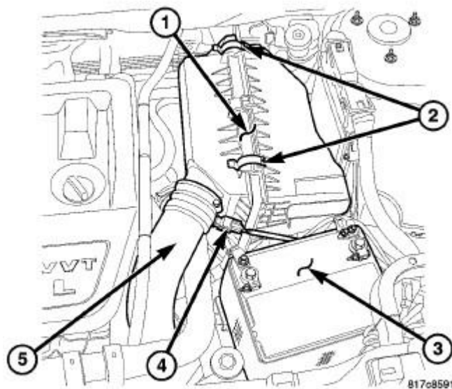
Fig. 76: AIR CLEANER HOUSING
