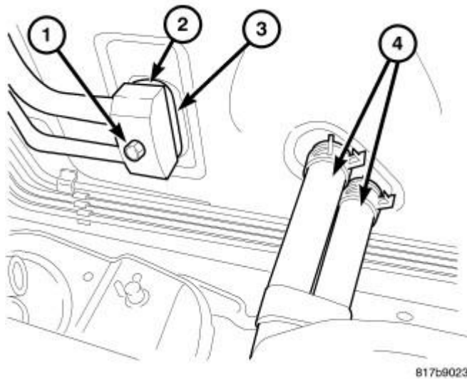
Fig. 342: Refrigerant Lines to Evaporator Bolt Courtesy of CHRYSLER LLC
