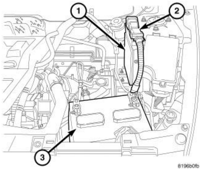
Fig. 54: BATTERY Courtesy of CHRYSLER LLC
