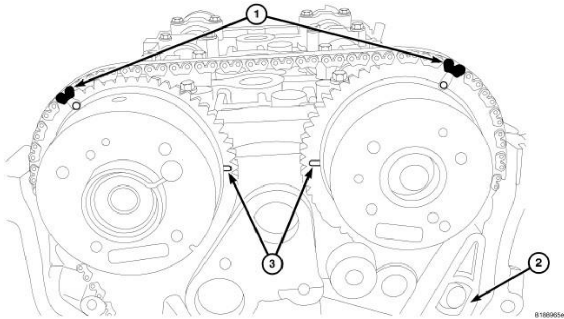
Fig. 167: TIMING CHAIN TIMING MARKS Courtesy of CHRYSLER LLC
