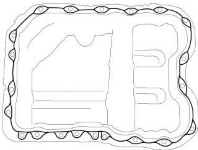
Fig. 310: SEALING OIL PAN Courtesy of CHRYSLER LLC
