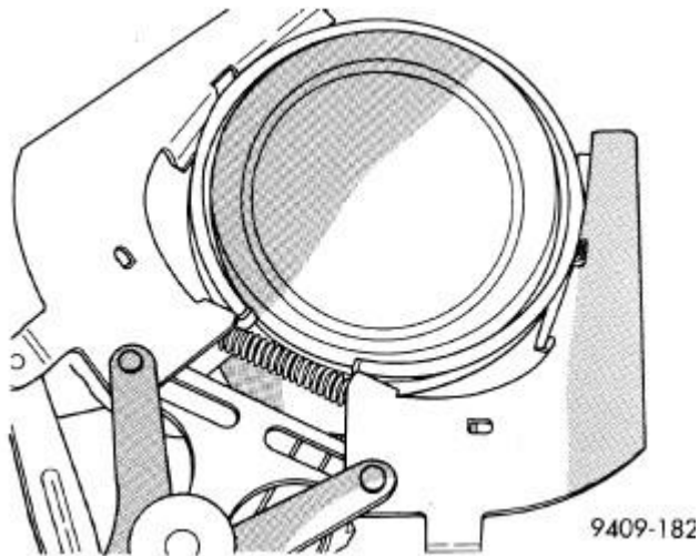
Fig. 247: Piston Rings-Removing and Installing Courtesy of CHRYSLER LLC
