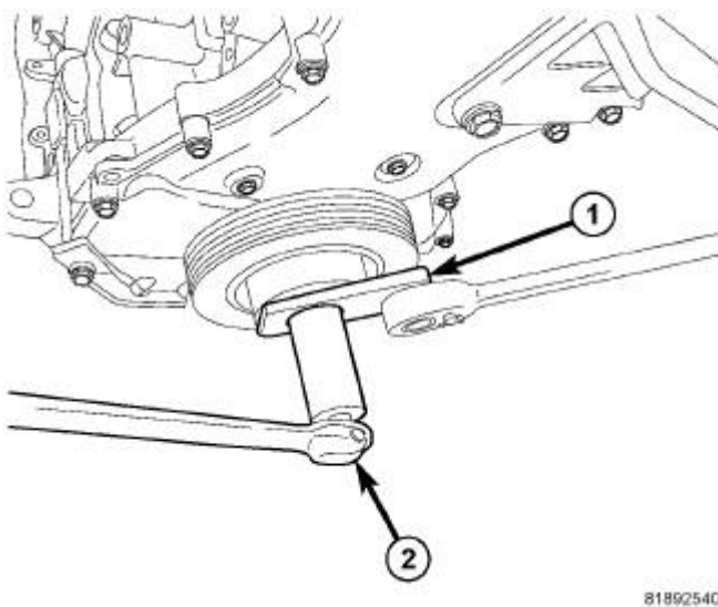
Fig. 237: DAMPER REMOVAL Courtesy of CHRYSLER LLC
