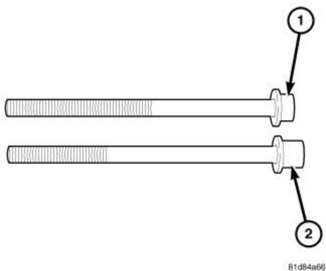
Fig. 120: CYLINDER HEAD BOLT IDENTIFICATION
