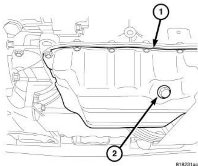
Fig. 304: OIL DRAIN PLUG Courtesy of CHRYSLER LLC
