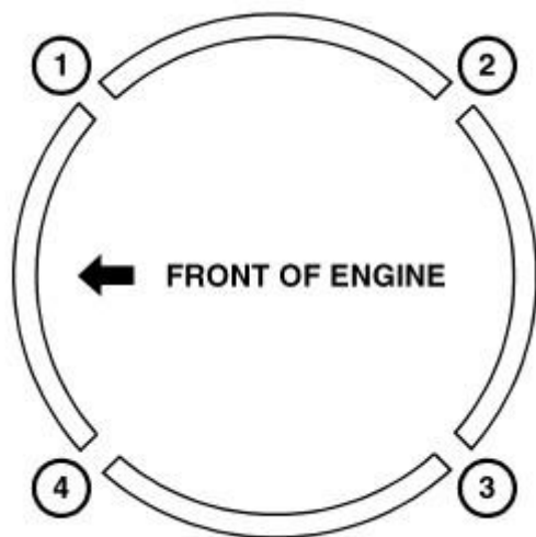
Fig. 249: Piston Ring End Gap Position Courtesy of CHRYSLER LLC
