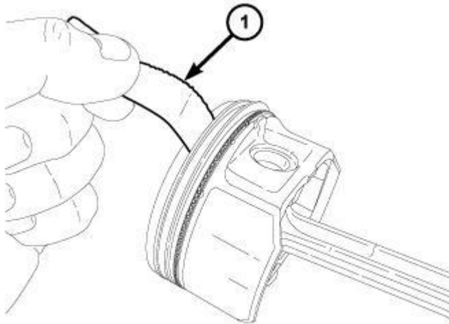
Fig. 246: Checking Piston Ring To Groove Side Clearance Courtesy of CHRYSLER LLC
