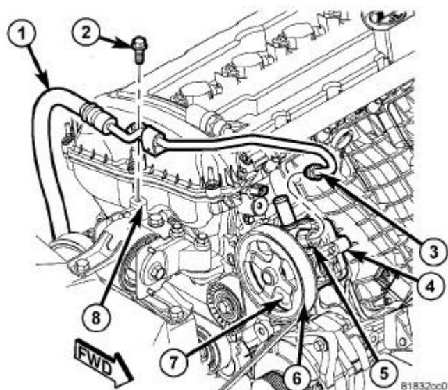
Fig. 411: PRESSURE HOSE Courtesy of CHRYSLER LLC
