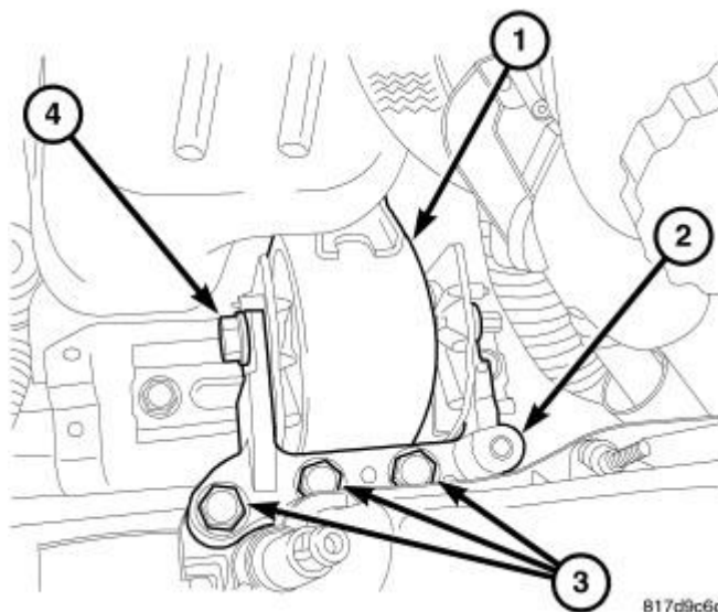
Fig. 31: RIGHT ENGINE MOUNT
