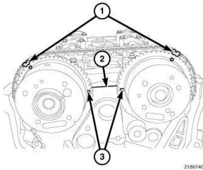
Fig. 162: Timing Chain Timing Marks Courtesy of CHRYSLER LLC
