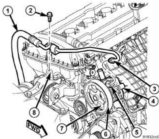
Fig. 348: Pressure Hose Courtesy of CHRYSLER LLC
