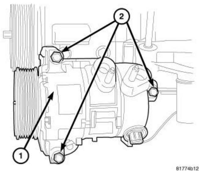
Fig. 329: Removing/Installing A/C Compressor
