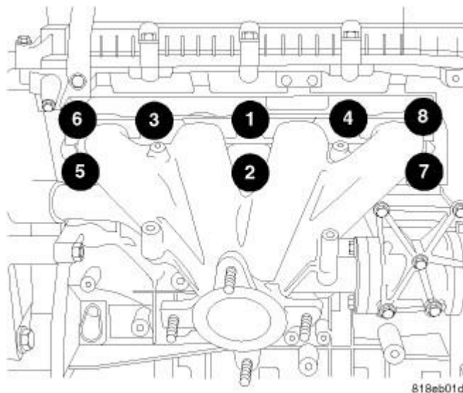
Fig. 355: Exhaust Manifold Bolt Torque Sequence Courtesy of CHRYSLER LLC
