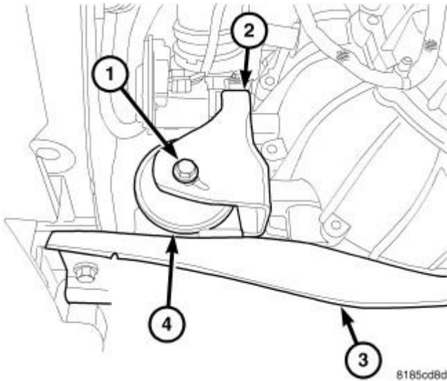
Fig. 191: FRONT MOUNT THROUGH BOLT Courtesy of CHRYSLER LLC
