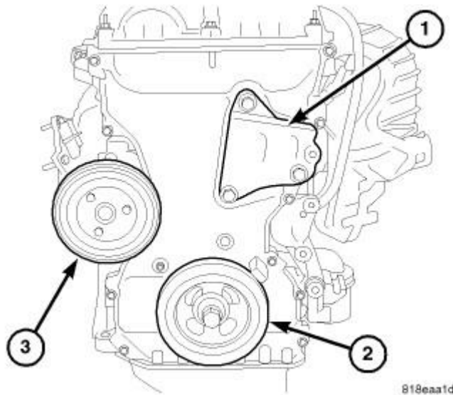
Fig. 429: RIGHT ENGINE MOUNT BRACKET Courtesy of CHRYSLER LLC
