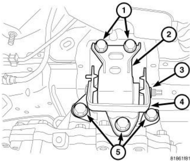
Fig. 195: LEFT MOUNT Courtesy of CHRYSLER LLC
