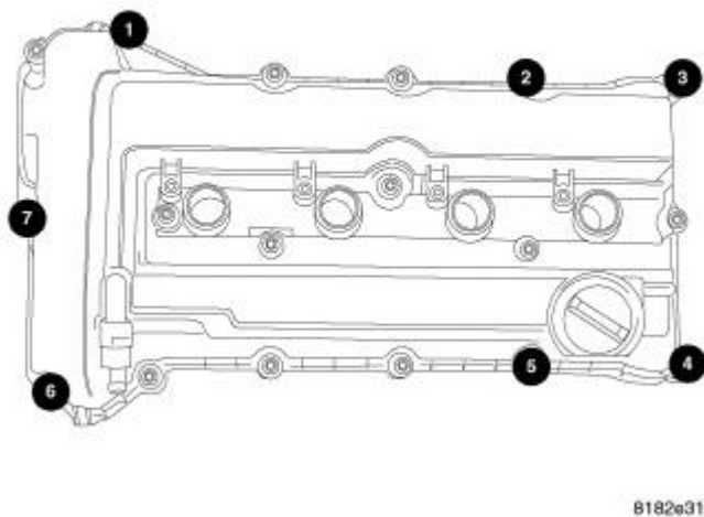
Fig. 178: STUD LOCATION Courtesy of CHRYSLER LLC
