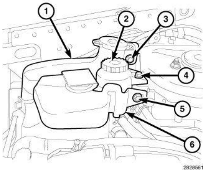
Fig. 347: Coolant Reservoir, Power Steering Fluid Reservoir, Washer Fluid Reservoir & Bolts Courtesy of CHRYSLER LLC
