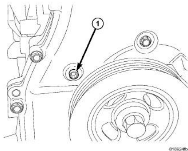
Fig. 169: TENSIONER ACCESS PLUG
