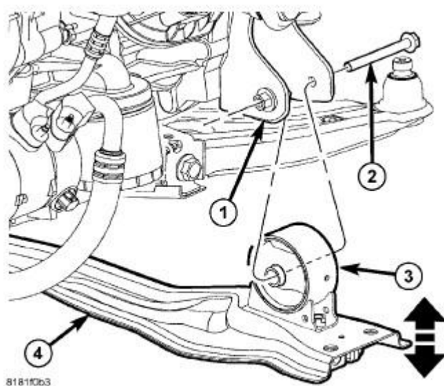
Fig. 366: Fore/Aft Crossmember 2 Courtesy of CHRYSLER LLC
