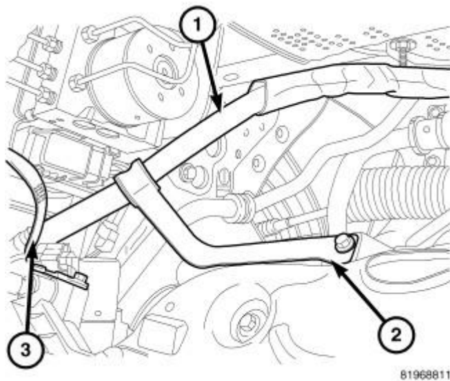
Fig. 20: P/S HOSE SUPPORT-FWD Courtesy of CHRYSLER LLC
