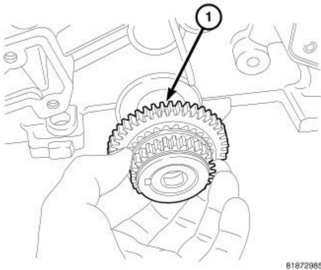
Fig. 398: Crankshaft Sprocket Courtesy of CHRYSLER LLC
