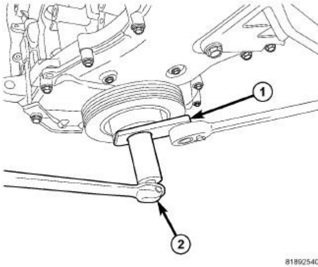
Fig. 262: Damper Removal Courtesy of CHRYSLER LLC
