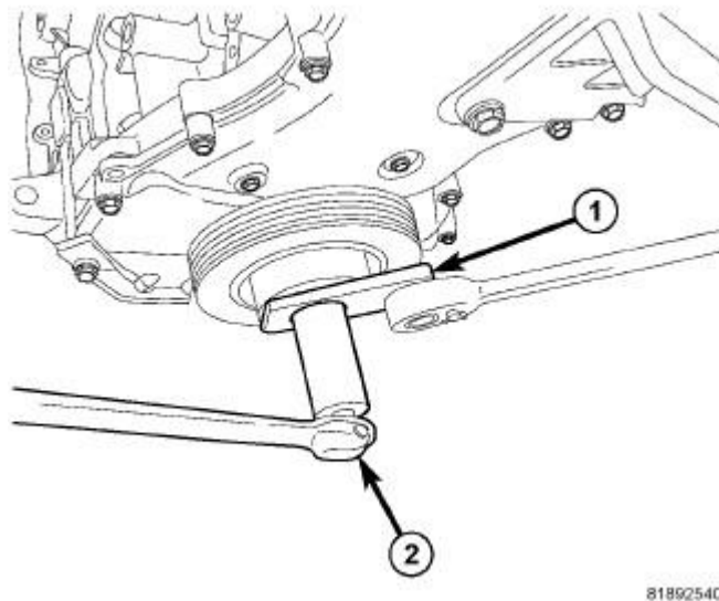
Fig. 43: DAMPER REMOVAL Courtesy of CHRYSLER LLC
