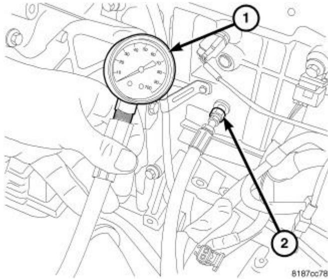
Fig. 280: OIL PRESSURE GAUGE
