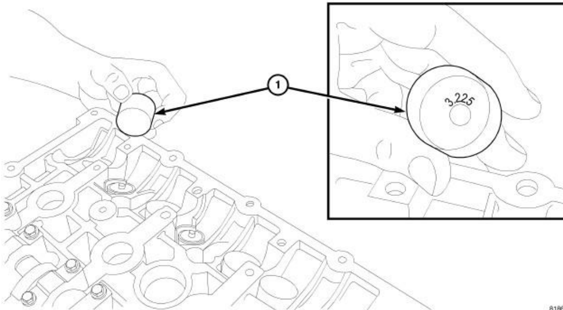
Fig. 142: TAPPET IDENTIFICATION
