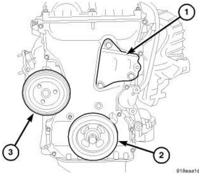
Fig. 219: RIGHT ENGINE MOUNT BRACKET
