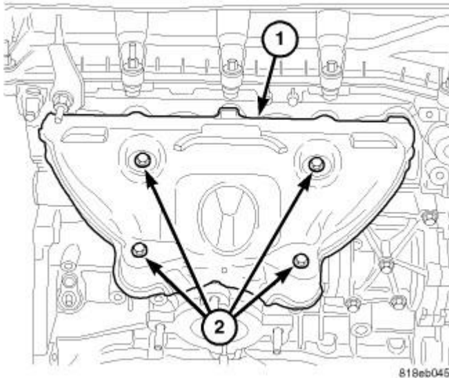
Fig. 375: EXHAUST MANIFOLD HEAT SHIELD Courtesy of CHRYSLER LLC
