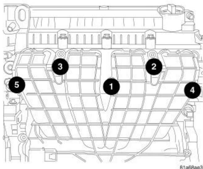
Fig. 47: Removing/Installing Intake Bolts - Torque Sequence Courtesy of CHRYSLER LLC
