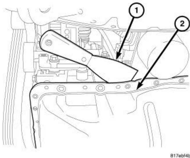
Fig. 308: OIL PAN REMOVAL Courtesy of CHRYSLER LLC
