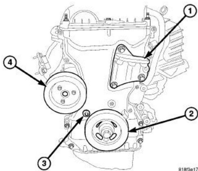
Fig. 417: ENGINE FRONT Courtesy of CHRYSLER LLC
