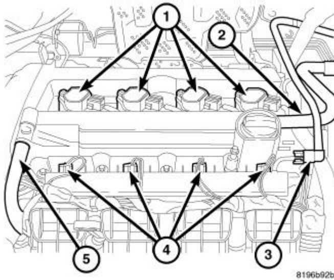
Fig. 49: COIL CONNECTOR Courtesy of CHRYSLER LLC
