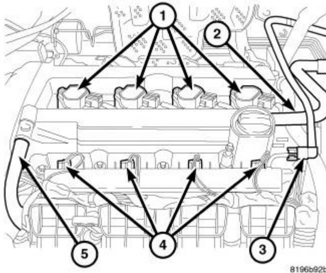
Fig. 383: COIL CONNECTOR Courtesy of CHRYSLER LLC
