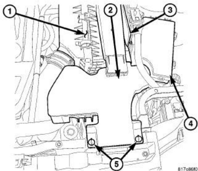
Fig. 77: AIR CLEANER INLET Courtesy of CHRYSLER LLC
