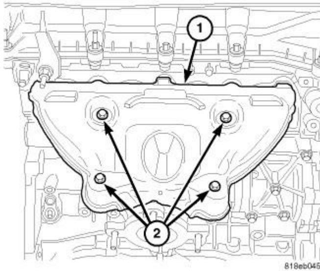
Fig. 352: EXHAUST MANIFOLD HEAT SHIELD Courtesy of CHRYSLER LLC
