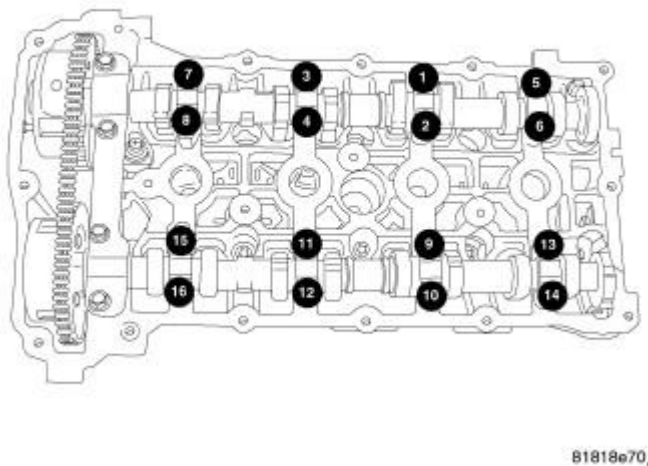
Fig. 125: CAM CAP TORQUE SEQUENCE
