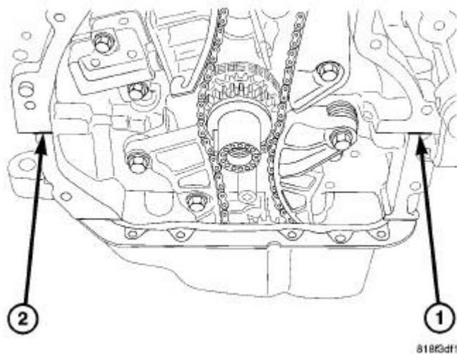
Fig. 425: LOWER T-JOINTS Courtesy of CHRYSLER LLC
