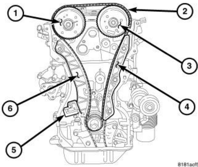
Fig. 392: TIMING DRIVE Courtesy of CHRYSLER LLC
