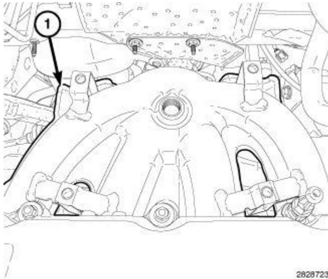
Fig. 344: Lower Maniverter Heatshield Courtesy of CHRYSLER LLC
