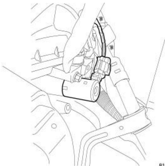
Fig. 293: SOLENOID LOCATION 1/2
