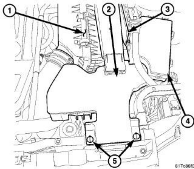
Fig. 56: AIR CLEANER INLET Courtesy of CHRYSLER LLC
