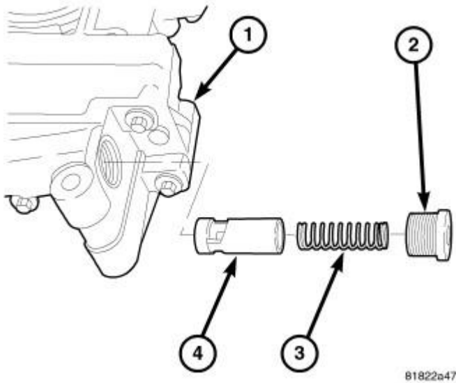
Fig. 330: OIL PRESSURE RELIEF VALVE
