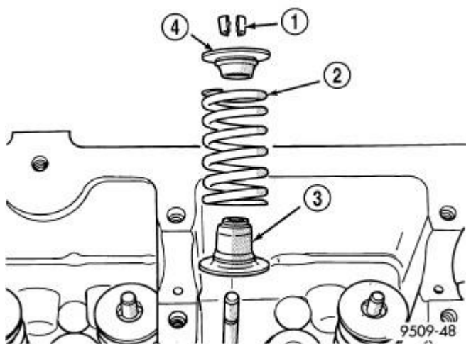
Fig. 187: Valve Spring Assembly
