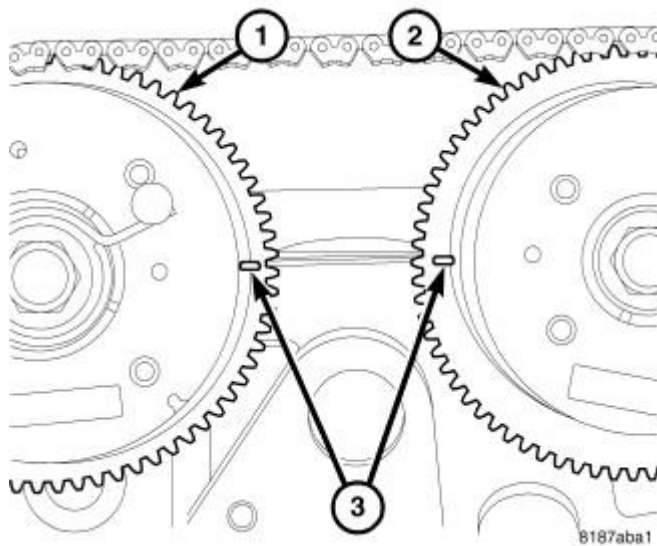
Fig. 124: Camshaft Timing Courtesy of CHRYSLER LLC
