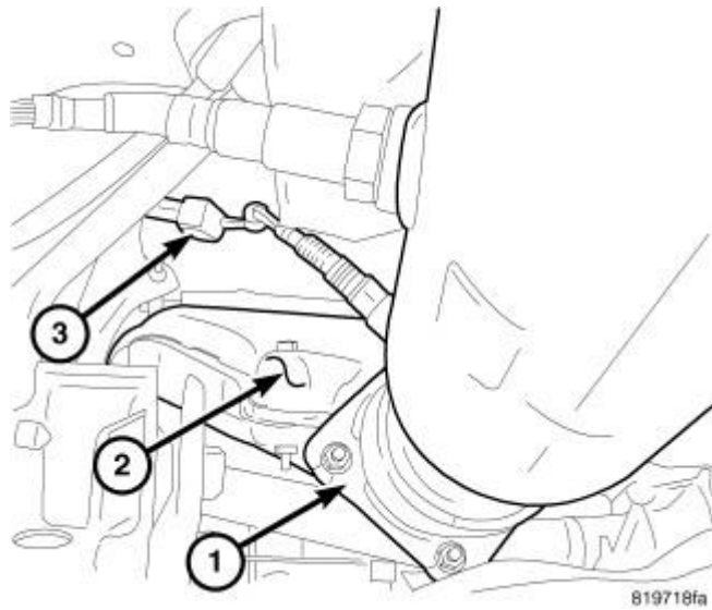
Fig. 41: Manifold To Exhaust Pipe Bolts Courtesy of CHRYSLER LLC
