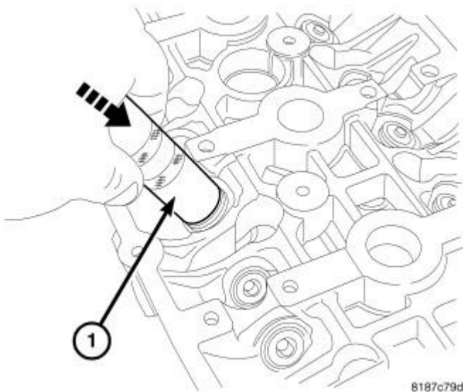
Fig. 183: Valve Removal & Installation Courtesy of CHRYSLER LLC
