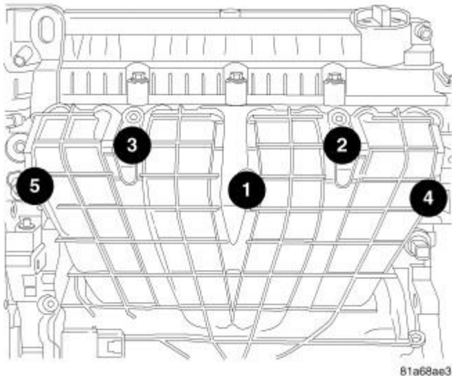
Fig. 388: Removing/Installing Intake Bolts - Torque Sequence Courtesy of CHRYSLER LLC
