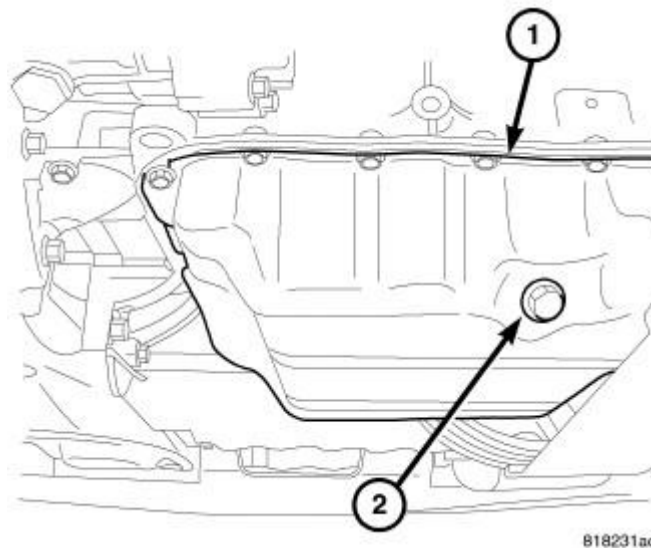
Fig. 23: OIL DRAIN PLUG Courtesy of CHRYSLER LLC
