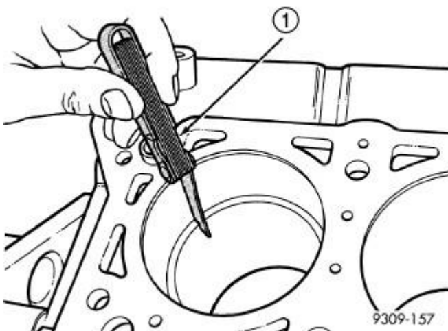
Fig. 245: Check Gap on Piston Rings
