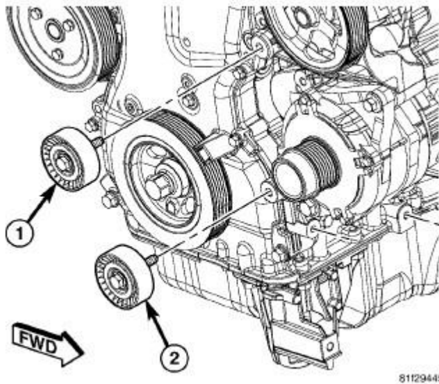
Fig. 416: ACCESSORY DRIVE BELT IDLER PULLEY - 2.4L Courtesy of CHRYSLER LLC
