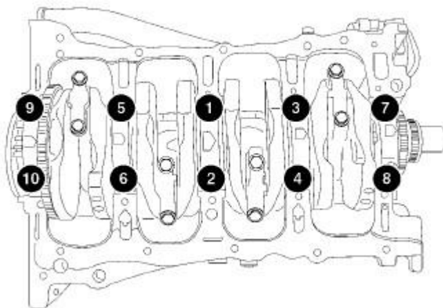
Fig. 231: MAIN BEARING CAP TORQUE SEQUENCE
