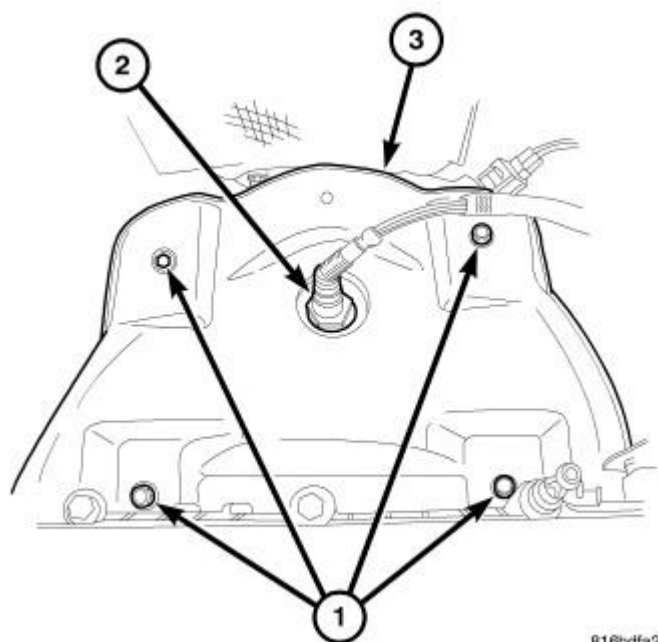
Fig. 371: Manifold Heat Shield And Bolts Courtesy of CHRYSLER LLC
