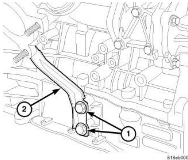
Fig. 354: EXHAUST MANIFOLD SUPPORT BRACKET Courtesy of CHRYSLER LLC
