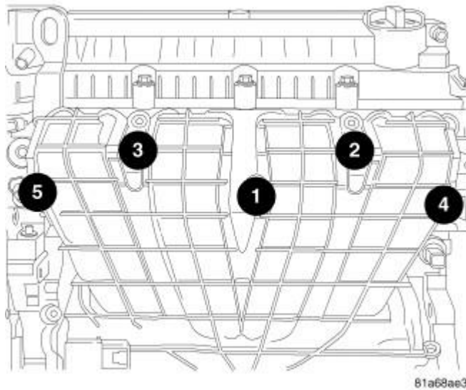
Fig. 130: Removing/Installing Intake Bolts In Sequence Courtesy of CHRYSLER LLC
