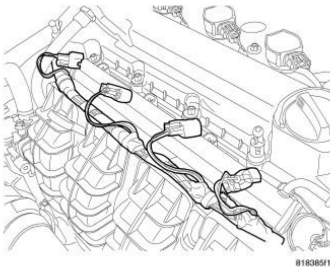
Fig. 100: ELECTRICAL CONNECTORS Courtesy of CHRYSLER LLC
