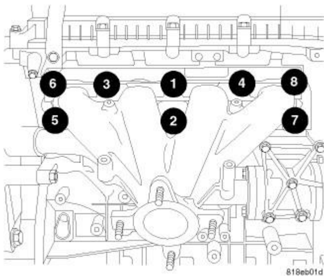
Fig. 374: Exhaust Manifold Bolt Torque Sequence Courtesy of CHRYSLER LLC
