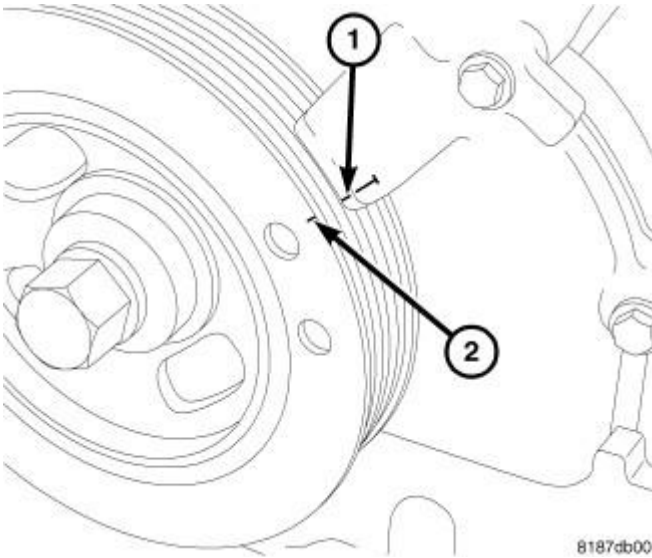
Fig. 316: TDC Courtesy of CHRYSLER LLC
