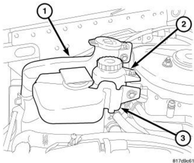
Fig. 410: Coolant Reservoir Courtesy of CHRYSLER LLC
