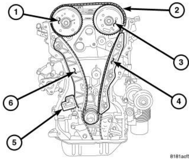
Fig. 364: Removing/Installing Timing Chain, Tensioner, & Guides Courtesy of CHRYSLER LLC
