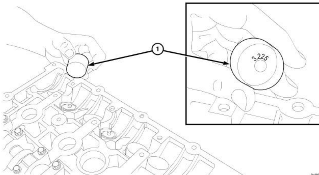
Fig. 130: Tappet Identification
