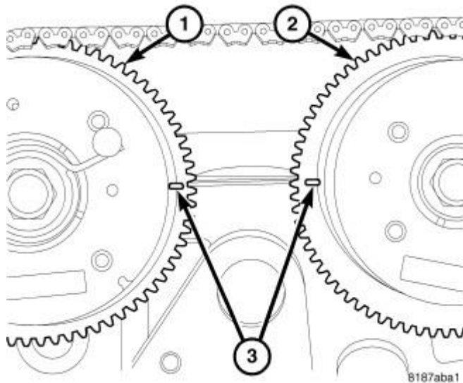
Fig. 365: Camshaft Timing Courtesy of CHRYSLER LLC
