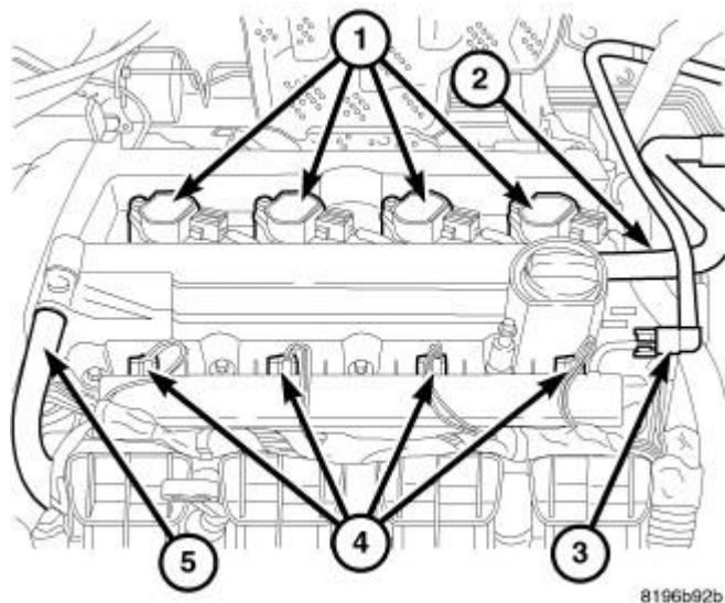
Fig. 16: Coil Connector Courtesy of CHRYSLER LLC
