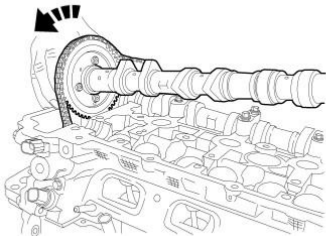
Fig. 147: Rotating Camshaft While Lifting Out Of Front Bearing Cradle Courtesy of CHRYSLER LLC
