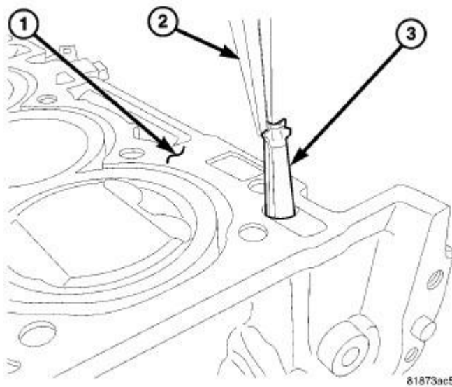
Fig. 100: Removing/Installing VVT Filter Screen Courtesy of CHRYSLER LLC
