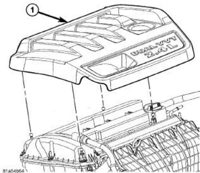
Fig. 68: Engine Cover Courtesy of CHRYSLER LLC
