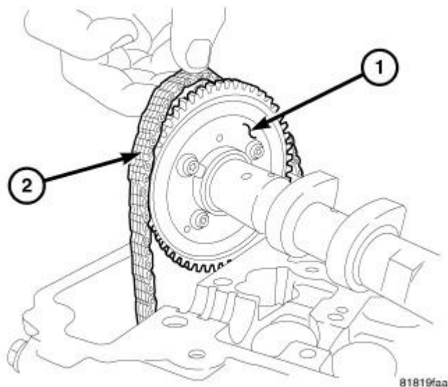
Fig. 148: Chain Removal Courtesy of CHRYSLER LLC
