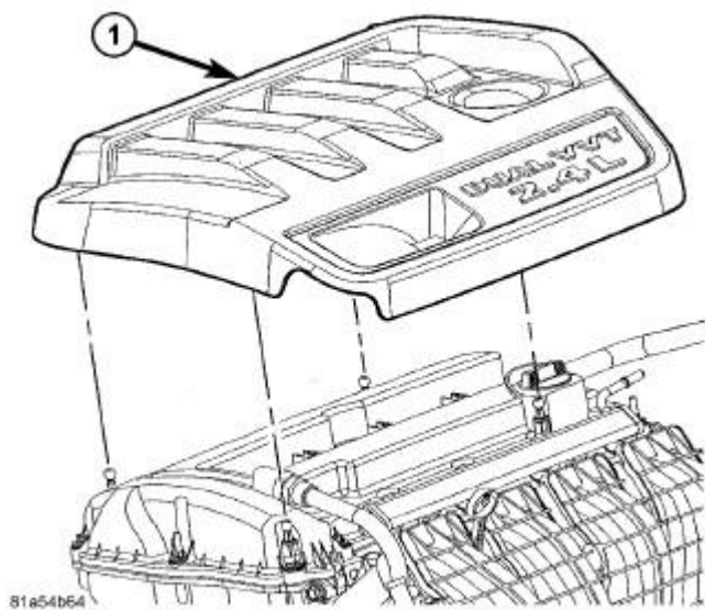
Fig. 366: Engine Cover Courtesy of CHRYSLER LLC
