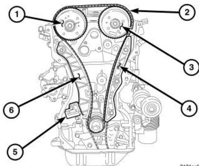
Fig. 114: Removing/Installing Timing Chain, Tensioner, & Guides Courtesy of CHRYSLER LLC
