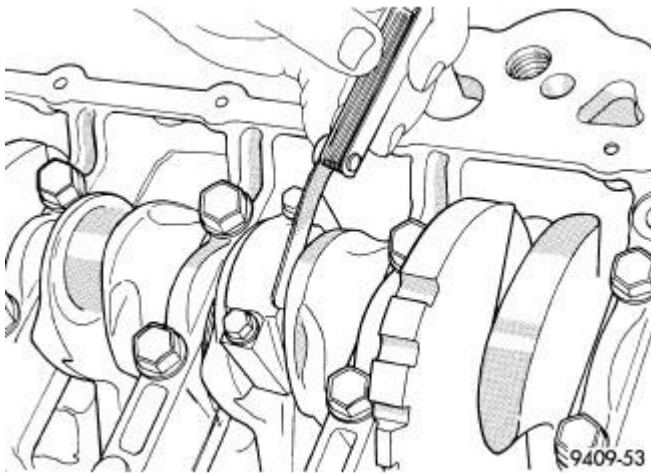
Fig. 231: Connecting Rod Side Clearance Courtesy of CHRYSLER LLC
