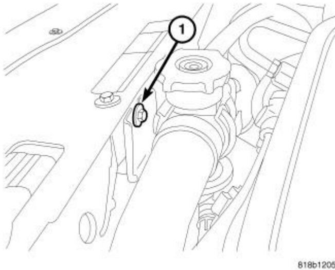
Fig. 340: Radiator Hose Support Courtesy of CHRYSLER LLC
