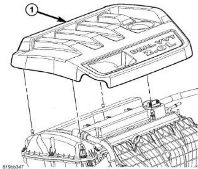
Fig. 8: Engine Cover - 2.0L
