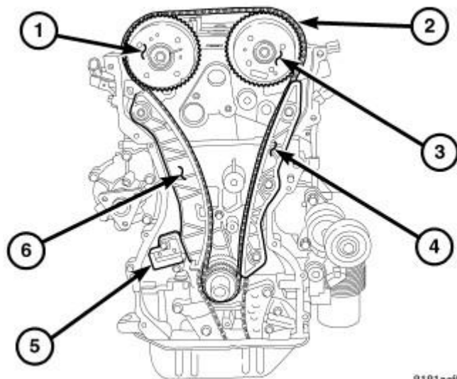
Fig. 353: Removing/Installing Timing Chain Tensioner & Timing Chain
