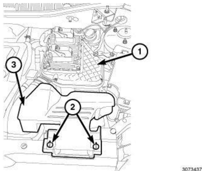
Fig. 53: Retainers, Fresh Air Inlet Duct & Air Cleaner Body Courtesy of CHRYSLER LLC
