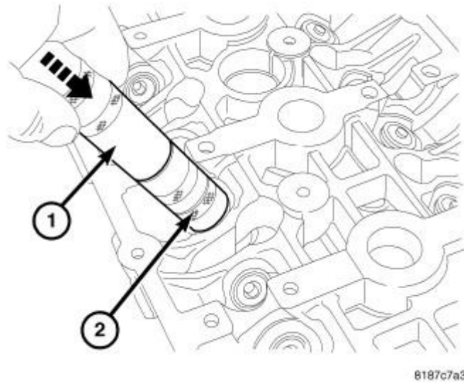
Fig. 177: Valve Installation Courtesy of CHRYSLER LLC
