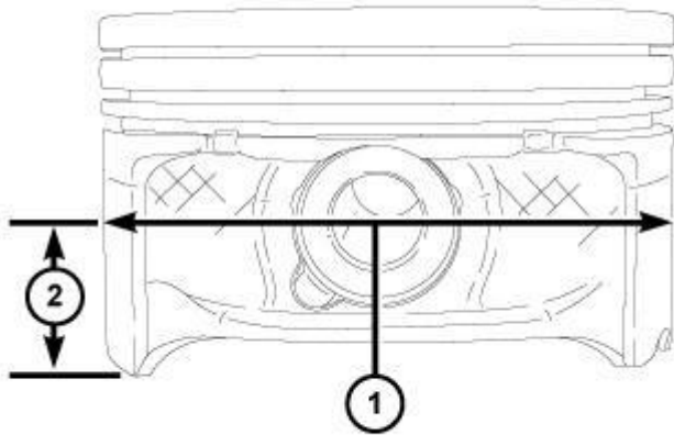
Fig. 225: Piston Pin Measurements Courtesy of CHRYSLER LLC
