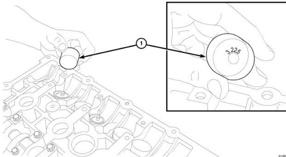
Fig. 134: Tappet Identification
