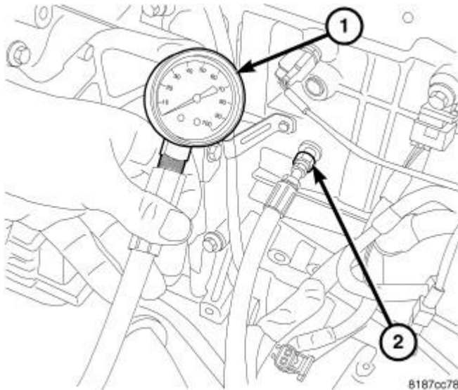
Fig. 263: Oil Pressure Gauge Courtesy of CHRYSLER LLC
