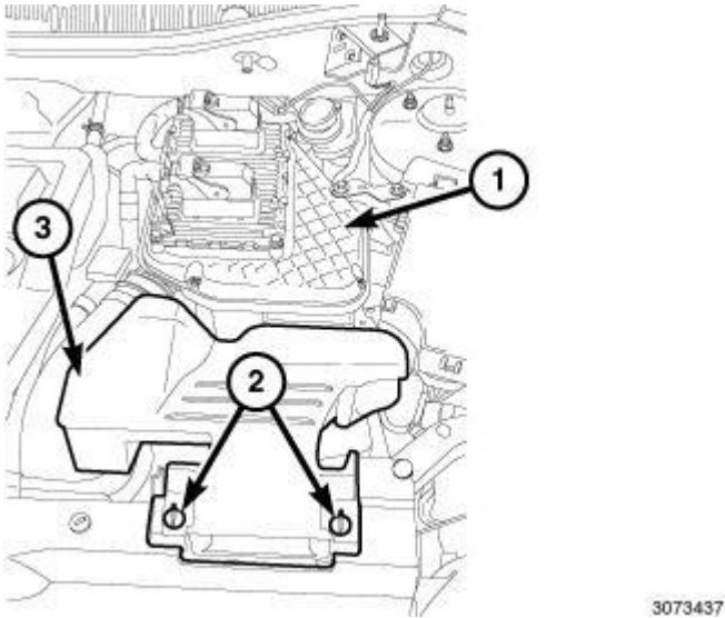
Fig. 56: Retainers, Fresh Air Inlet Duct & Air Cleaner Body Courtesy of CHRYSLER LLC
