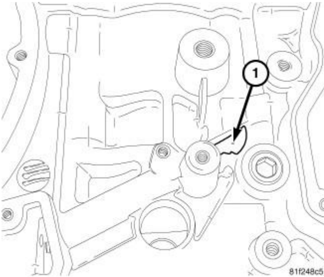
Fig. 261: Oil Hole
