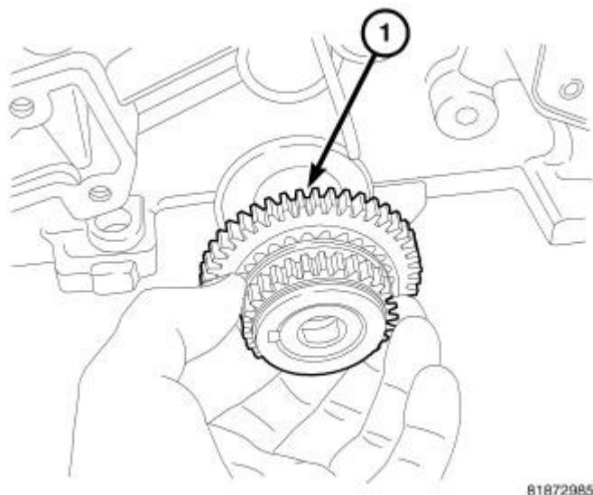
Fig. 354: Crankshaft Sprocket Courtesy of CHRYSLER LLC
