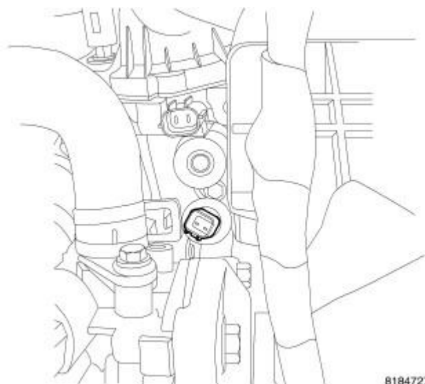
Fig. 280: Oil Pressure Sensor Courtesy of CHRYSLER LLC
