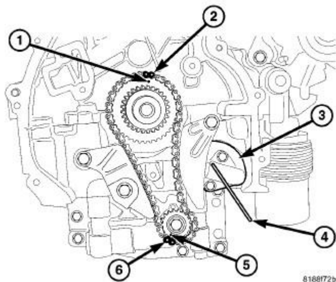
Fig. 357: Marking Chain & Sprocket For Reassembly Courtesy of CHRYSLER LLC
