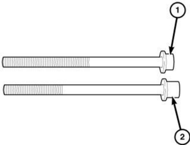
Fig. 103: Cylinder Head Bolt Identification Courtesy of CHRYSLER LLC
