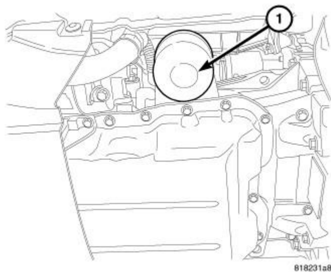
Fig. 290: Oil Filter Courtesy of CHRYSLER LLC
