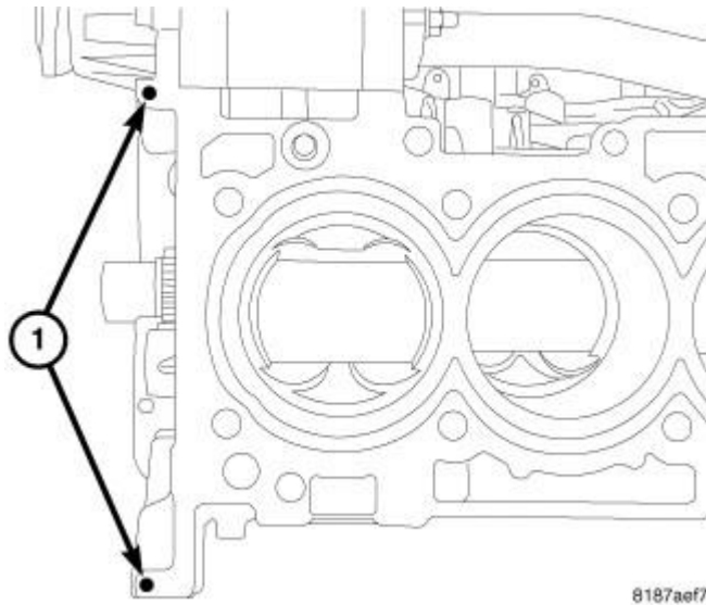
Fig. 101: Applying Cylinder Head RTV On Cylinder Block Courtesy of CHRYSLER LLC
