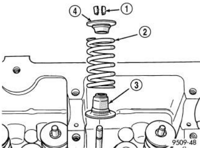
Fig. 181: Valve Spring Assembly
