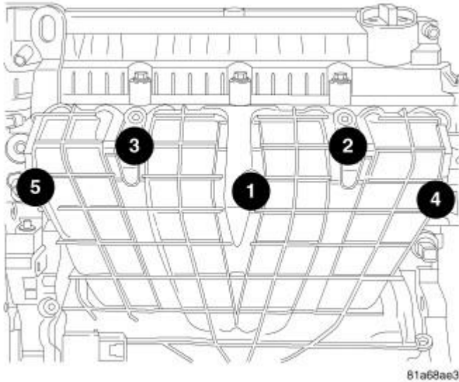
Fig. 122: Removing/Installing Intake Bolts In Sequence Courtesy of CHRYSLER LLC
