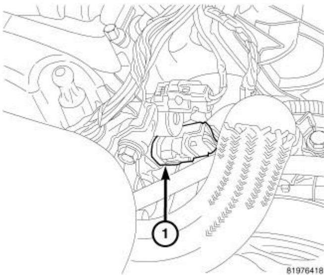
Fig. 314: OIL TEMPERATURE SENSOR
