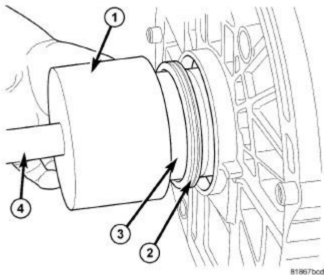
Fig. 243: REAR MAIN INSTALLATION Courtesy of CHRYSLER LLC
