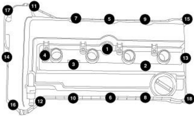
Fig. 176: TORQUE SEQUENCE Courtesy of CHRYSLER LLC
