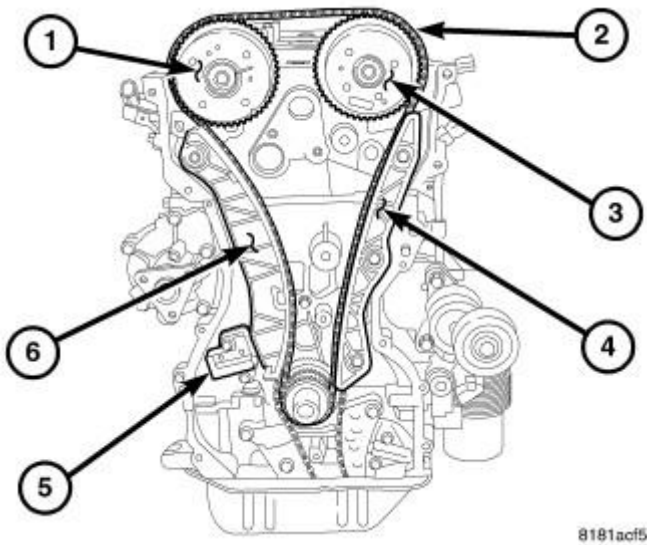
Fig. 344: TIMING DRIVE Courtesy of CHRYSLER LLC
