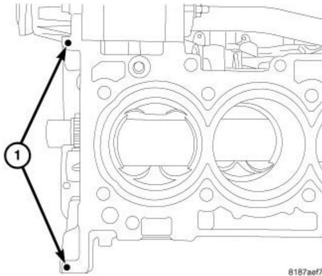
Fig. 106: Applying Cylinder Head RTV On Cylinder Block
