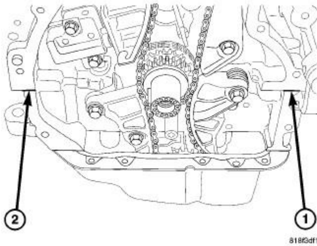
Fig. 377: Applying Mopar(R) Engine Sealant RTV (Or Equivalent) At Ladder Frame To Block Parting Line
