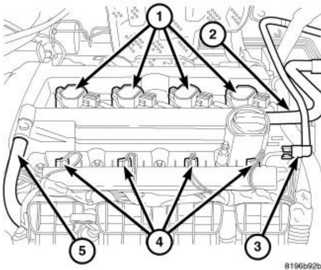
Fig. 13: COIL CONNECTOR Courtesy of CHRYSLER LLC
