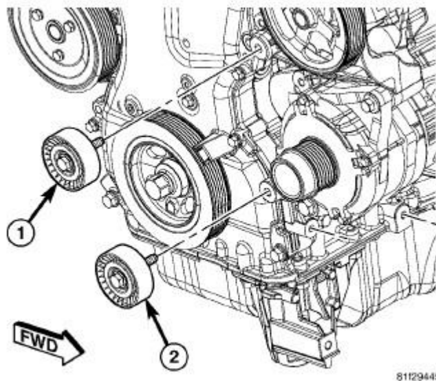
Fig. 83: Removing/Installing Accessory Drive Belt Lower Idler Pulley Courtesy of CHRYSLER LLC
