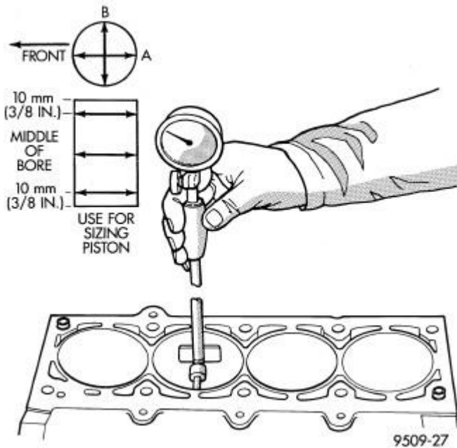
Fig. 186: Checking Cylinder Bore Size
