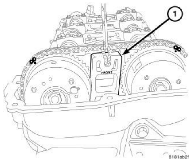
Fig. 160: WEDGE TOOL Courtesy of CHRYSLER LLC
