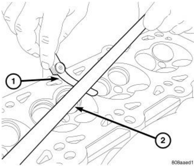
Fig. 103: Checking Cylinder Head Flatness Courtesy of CHRYSLER LLC
