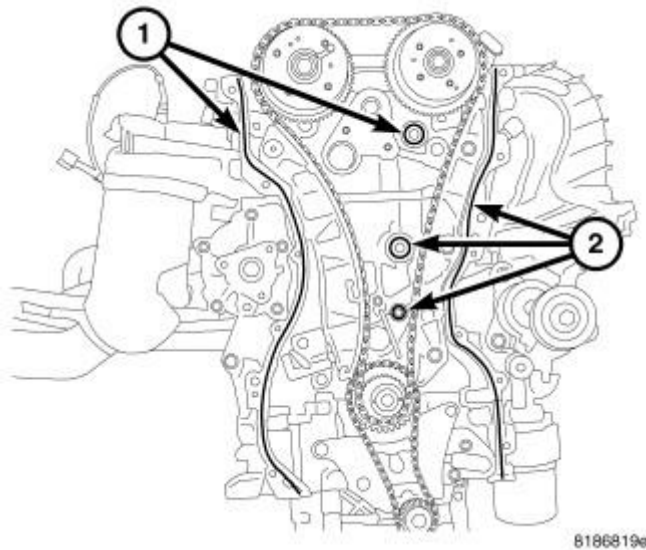
Fig. 379: TIMING CHAIN COVER SEALING Courtesy of CHRYSLER LLC
