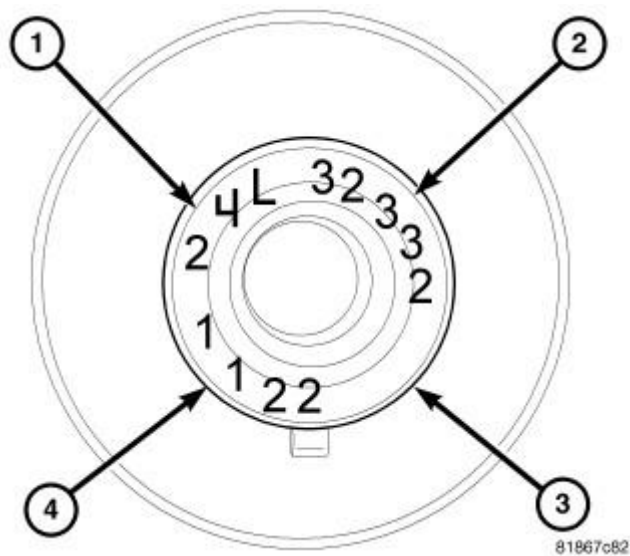
Fig. 187: BEARING SELECTION
