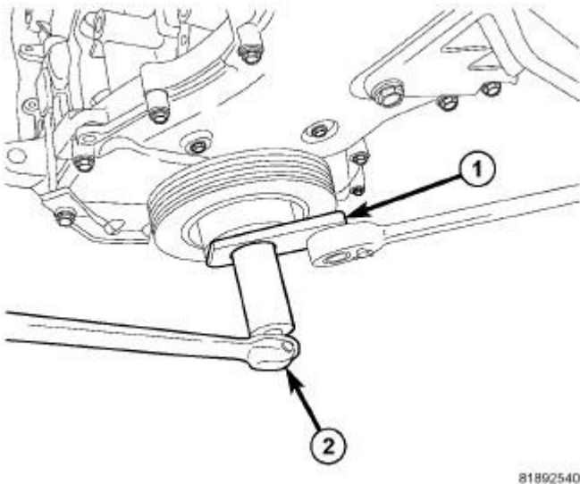
Fig. 216: DAMPER REMOVAL Courtesy of CHRYSLER LLC
