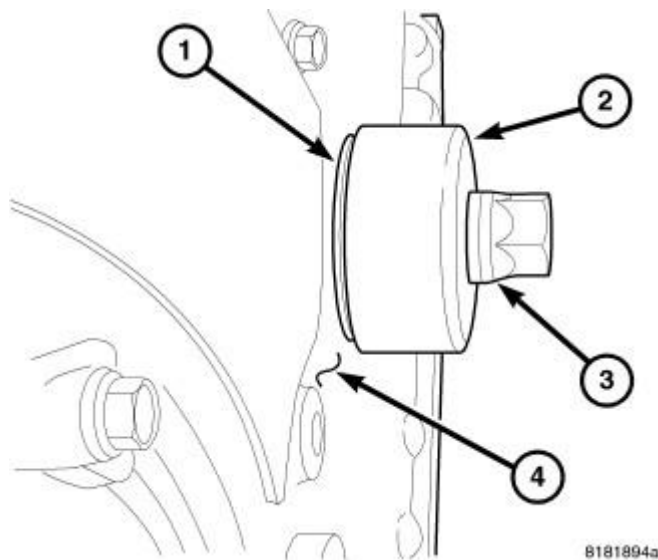
Fig. 238: INSTALLING FRONT SEAL Courtesy of CHRYSLER LLC
