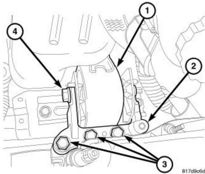
Fig. 257: RIGHT ENGINE MOUNT Courtesy of CHRYSLER LLC
