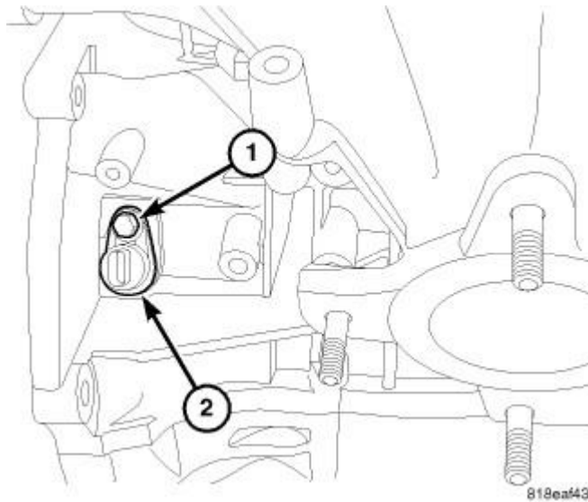
Fig. 31: Crankshaft Position Sensor Courtesy of CHRYSLER LLC
