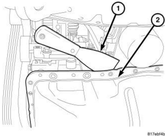
Fig. 297: OIL PAN REMOVAL Courtesy of CHRYSLER LLC
