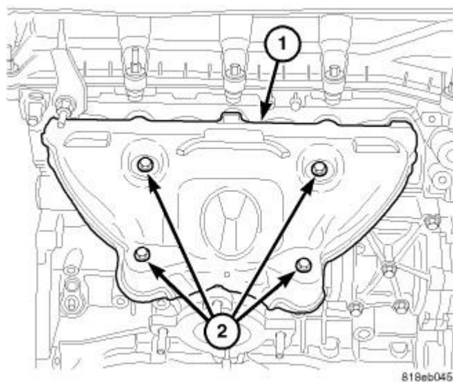
Fig. 324: EXHAUST MANIFOLD HEAT SHIELD Courtesy of CHRYSLER LLC
