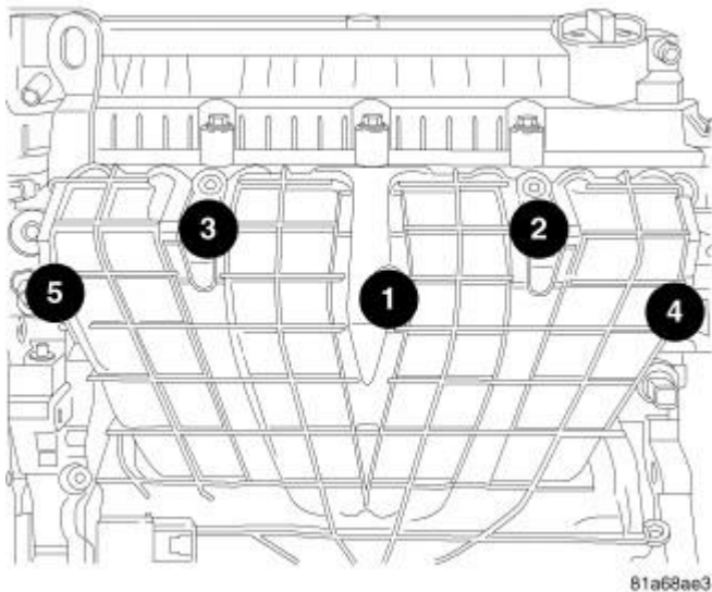
Fig. 340: Removing/Installing Intake Bolts - Torque Sequence Courtesy of CHRYSLER LLC
