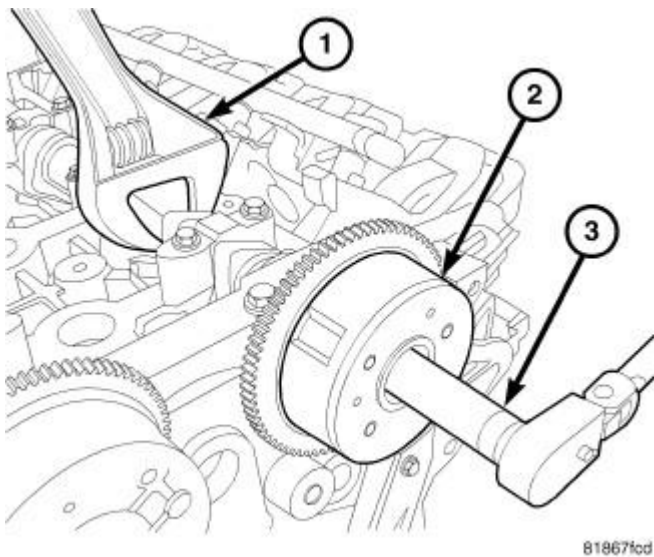
Fig. 129: Removing & Installing Cam Phaser Courtesy of CHRYSLER LLC
