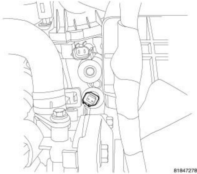
Fig. 280: OIL PRESSURE SENSOR
