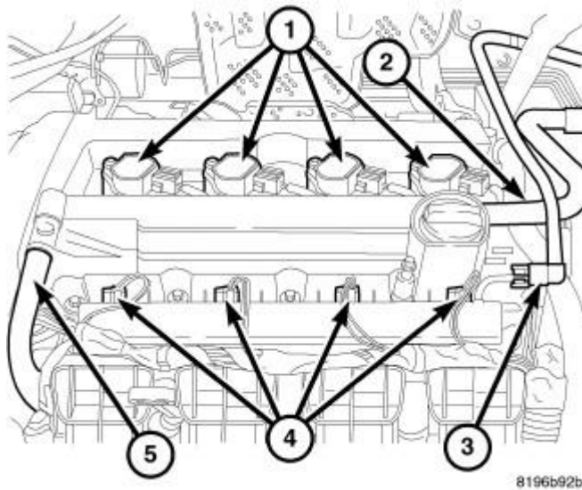
Fig. 341: COIL CONNECTOR Courtesy of CHRYSLER LLC
