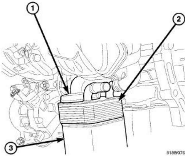
Fig. 283: OIL COOLER
