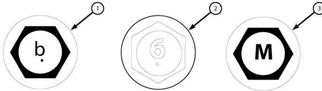
Fig. 208: MAIN BOLT IDENTIFICATION
