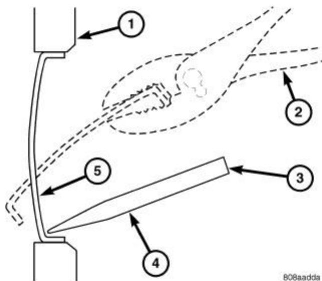
Fig. 3: CORE HOLE PLUG REMOVAL Courtesy of CHRYSLER LLC
