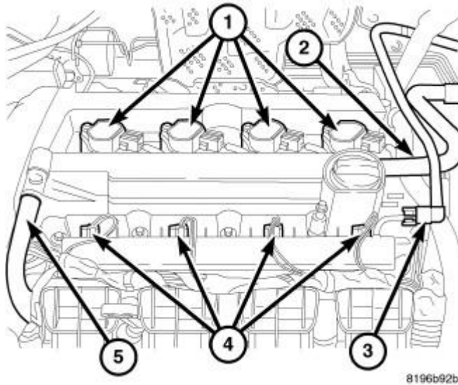
Fig. 173: Coil Connector
