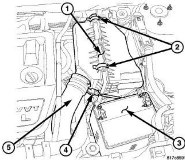
Fig. 49: Removing/Installing Air Cleaner Housing & Clean Air Hose Courtesy of CHRYSLER LLC
