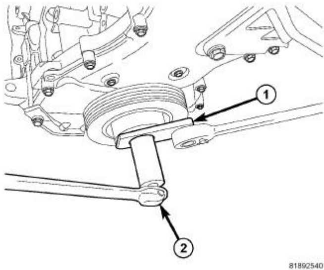
Fig. 35: DAMPER REMOVAL Courtesy of CHRYSLER LLC
