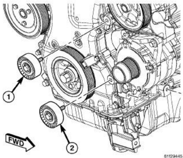
Fig. 368: Removing/Installing Accessory Drive Belt Lower Idler Pulley Courtesy of CHRYSLER LLC
