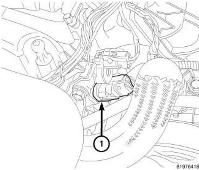
Fig. 263: OIL TEMPERATURE SENSOR
