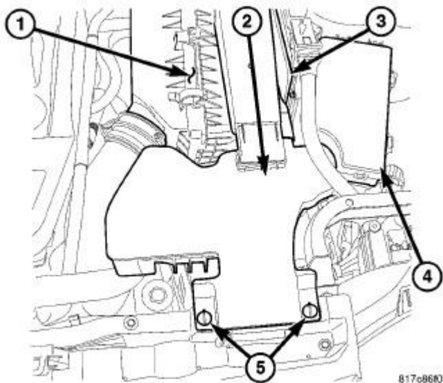
Fig. 65: AIR CLEANER INLET Courtesy of CHRYSLER LLC
