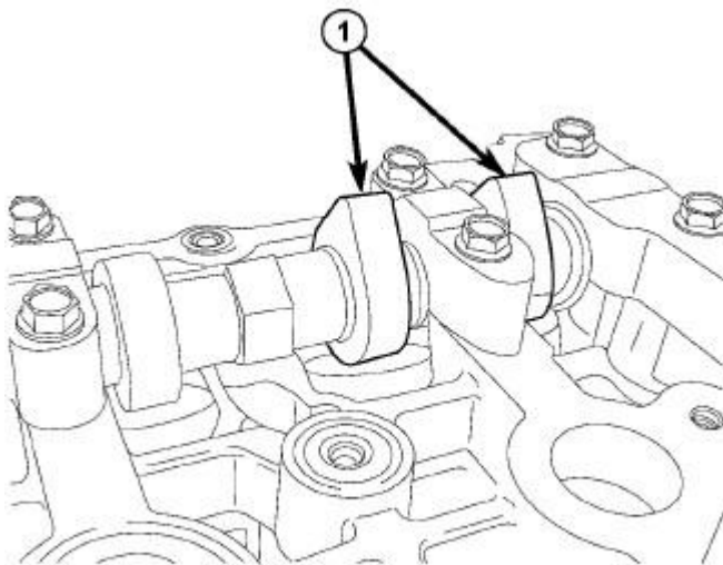
Fig. 132: LOBES VERTICAL Courtesy of CHRYSLER LLC
