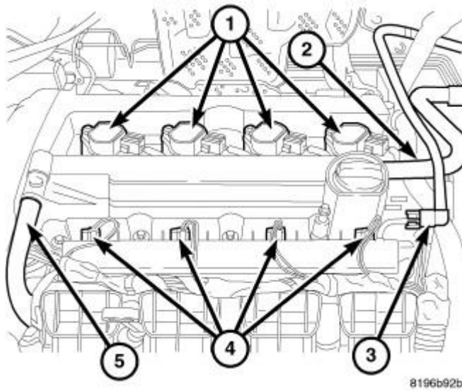
Fig. 42: COIL CONNECTOR Courtesy of CHRYSLER LLC
