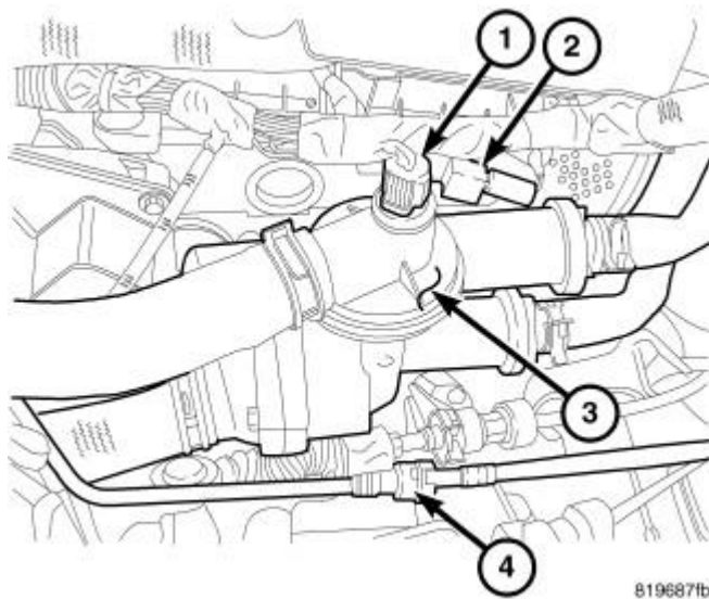
Fig. 125: COOLANT ADAPTER Courtesy of CHRYSLER LLC
