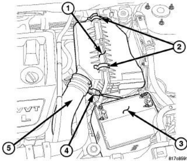
Fig. 127: Air Cleaner Housing Courtesy of CHRYSLER LLC
