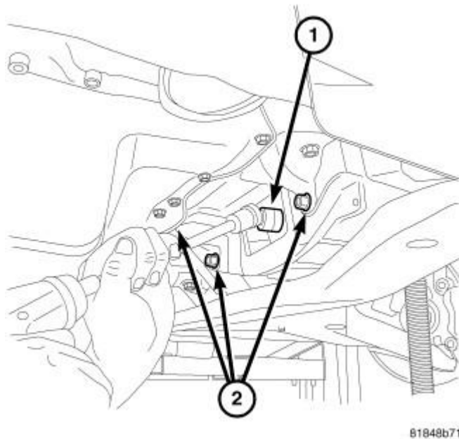
Fig. 33: Removing/Installing Lower Bell Housing Bolts & Torque Converter Bolts Courtesy of CHRYSLER LLC
