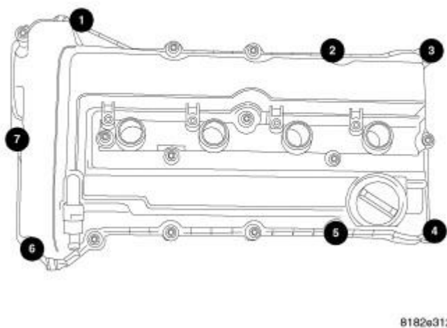
Fig. 170: STUD LOCATION Courtesy of CHRYSLER LLC
