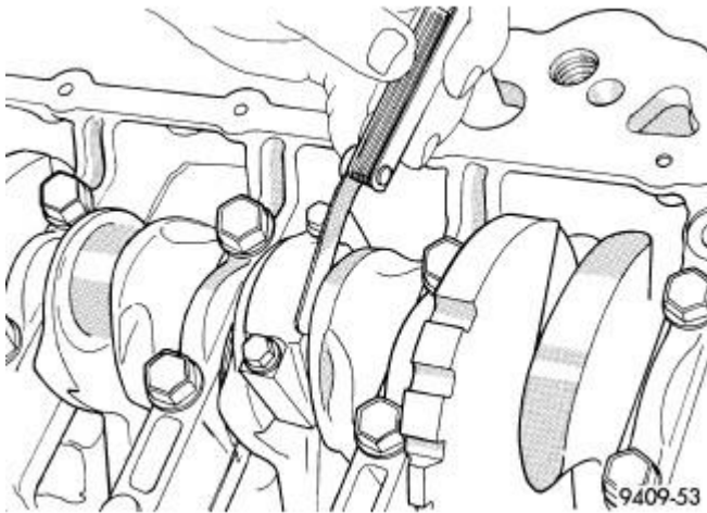
Fig. 189: Connecting Rod Side Clearance Courtesy of CHRYSLER LLC
