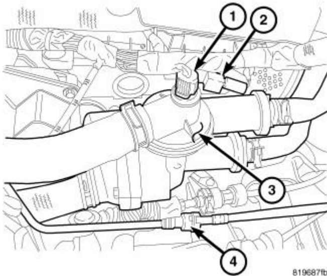
Fig. 113: COOLANT ADAPTER Courtesy of CHRYSLER LLC
