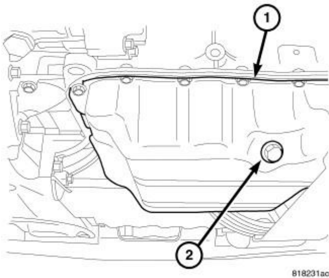
Fig. 230: OIL DRAIN PLUG Courtesy of CHRYSLER LLC
