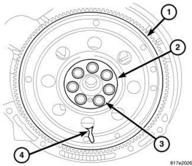
Fig. 218: FLEX PLATE
