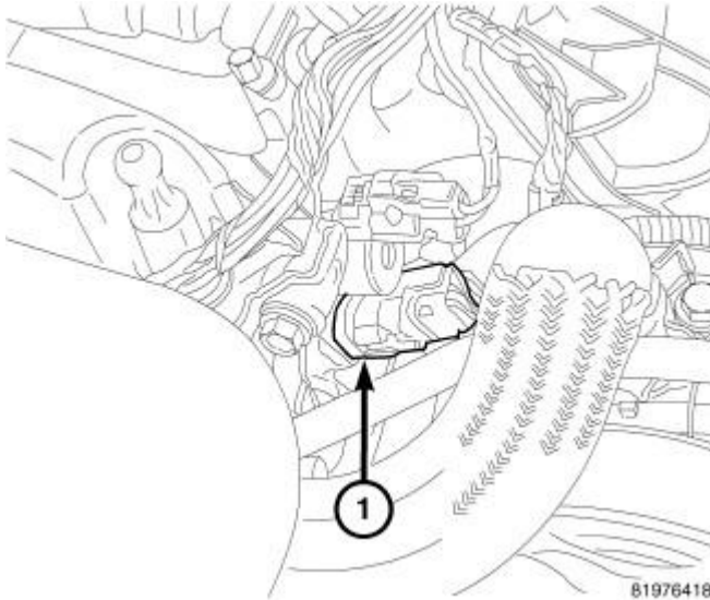
Fig. 336: OIL TEMPERATURE SENSOR Courtesy of CHRYSLER LLC
