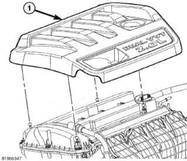
Fig. 6: Engine Cover - 2.0L Courtesy of CHRYSLER LLC
