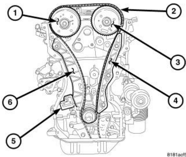
Fig. 394: TIMING DRIVE Courtesy of CHRYSLER LLC
