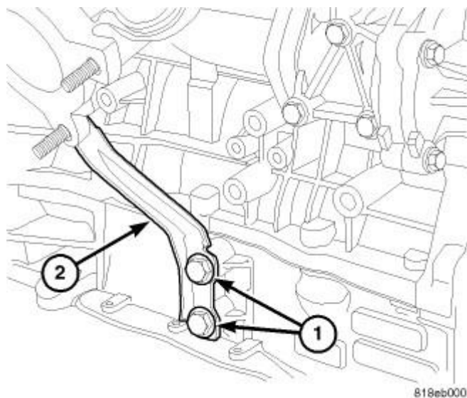
Fig. 329: EXHAUST MANIFOLD SUPPORT BRACKET Courtesy of CHRYSLER LLC
