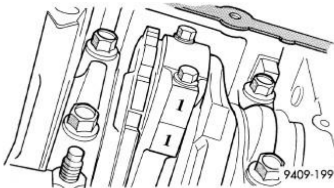
Fig. 232: Identify Connecting Rod to Cylinder-Typical Courtesy of CHRYSLER LLC
