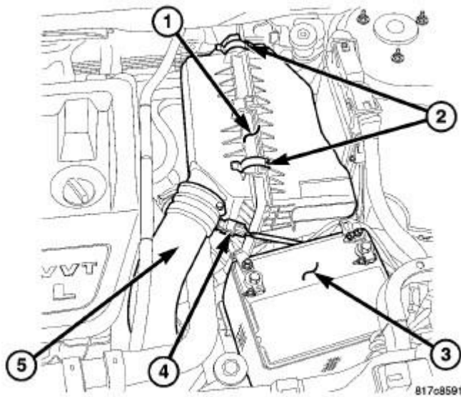
Fig. 334: AIR CLEANER HOUSING Courtesy of CHRYSLER LLC
