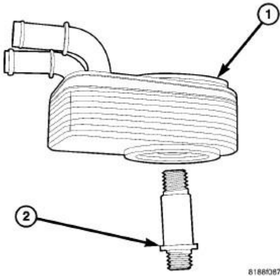
Fig. 284: OIL COOLER MOUNTING
