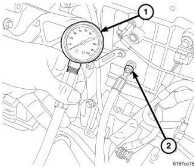
Fig. 270: OIL PRESSURE GAUGE Courtesy of CHRYSLER LLC
