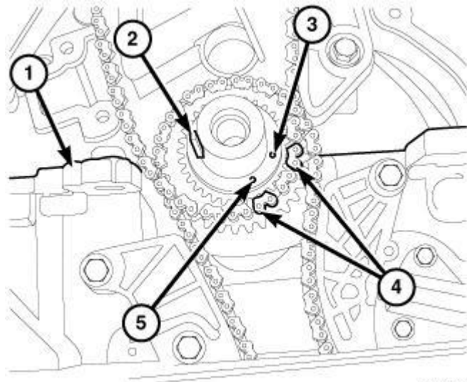
Fig. 359: Crankshaft Timing Marks
