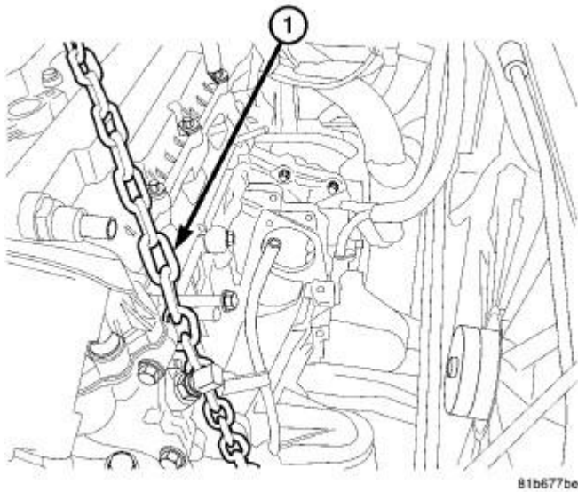
Fig. 24: Removing/Installing Engine Lift Chain Courtesy of CHRYSLER LLC
