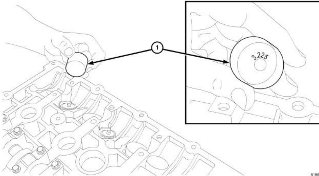
Fig. 133: TAPPET IDENTIFICATION Courtesy of CHRYSLER LLC
