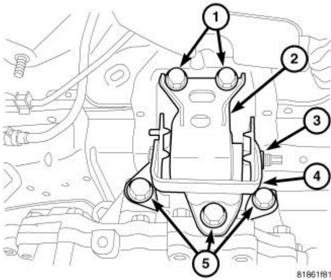
Fig. 250: LEFT MOUNT Courtesy of CHRYSLER LLC
