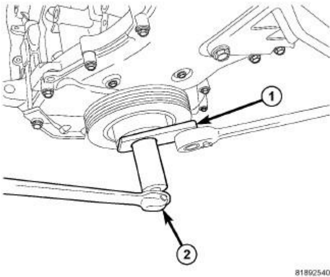
Fig. 235: Damper Removal Courtesy of CHRYSLER LLC
