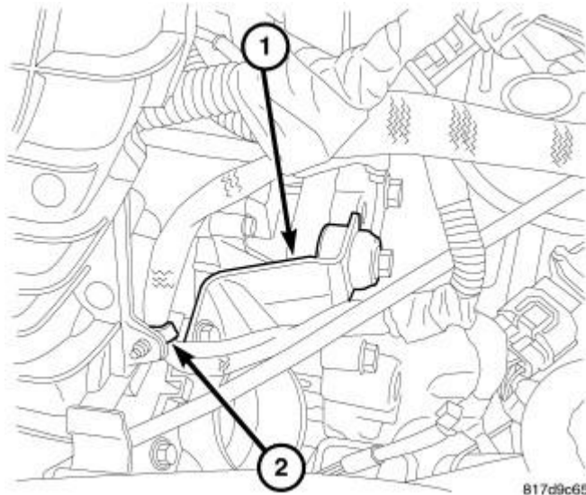
Fig. 337: THROTTLE BODY SUPPORT Courtesy of CHRYSLER LLC
