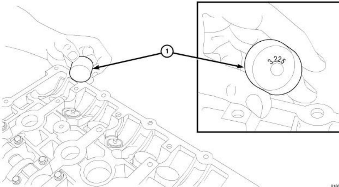
Fig. 134: TAPPET IDENTIFICATION Courtesy of CHRYSLER LLC
