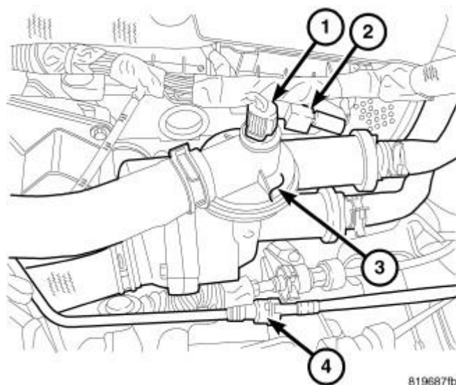
Fig. 37: Removing/Installing Coolant Adapter Assembly Courtesy of CHRYSLER LLC
