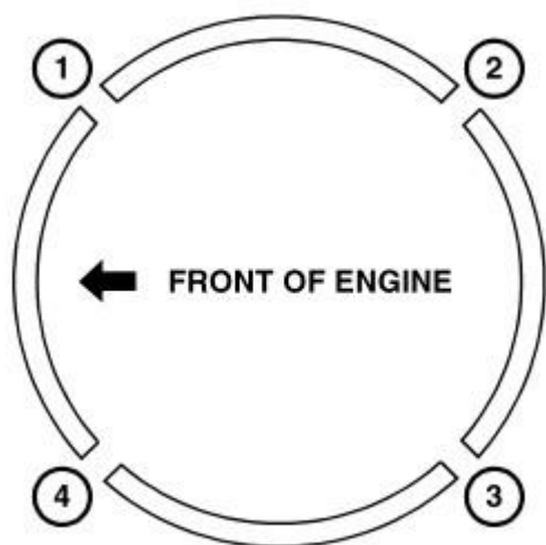
Fig. 233: Piston Ring End Gap Position Courtesy of CHRYSLER LLC
