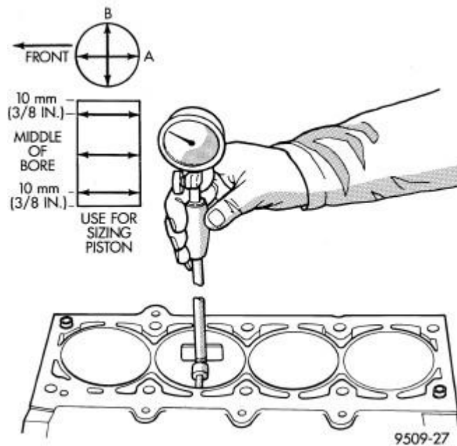
Fig. 229: Checking Cylinder Bore Size
