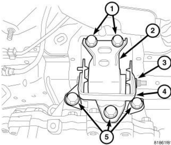
Fig. 249: LEFT MOUNT Courtesy of CHRYSLER LLC
