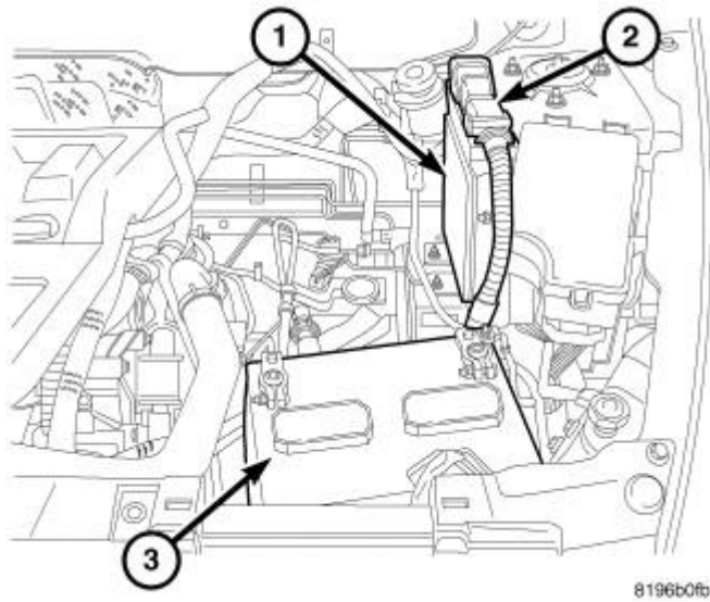
Fig. 48: Removing/Installing Battery Courtesy of CHRYSLER LLC
