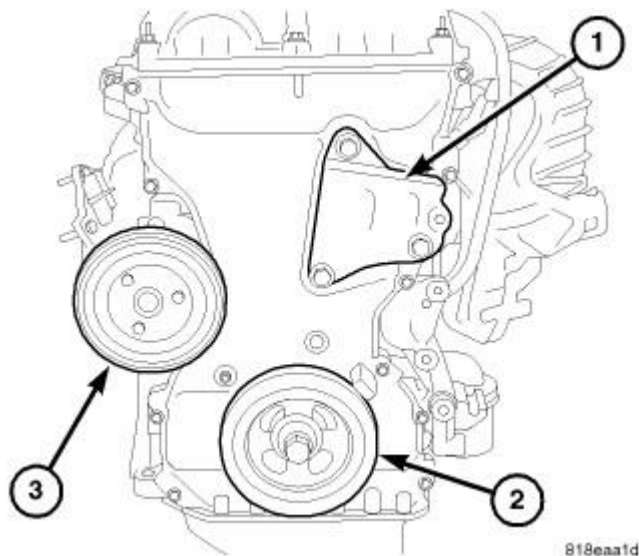
Fig. 381: RIGHT ENGINE MOUNT BRACKET Courtesy of CHRYSLER LLC
