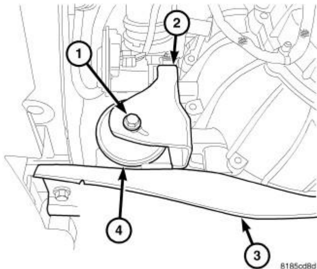
Fig. 246: FRONT MOUNT THROUGH BOLT Courtesy of CHRYSLER LLC
