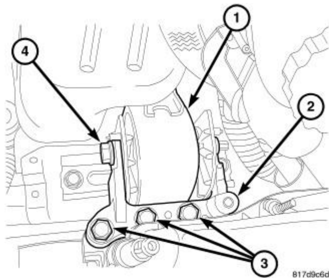
Fig. 371: Right Engine Mount Courtesy of CHRYSLER LLC
