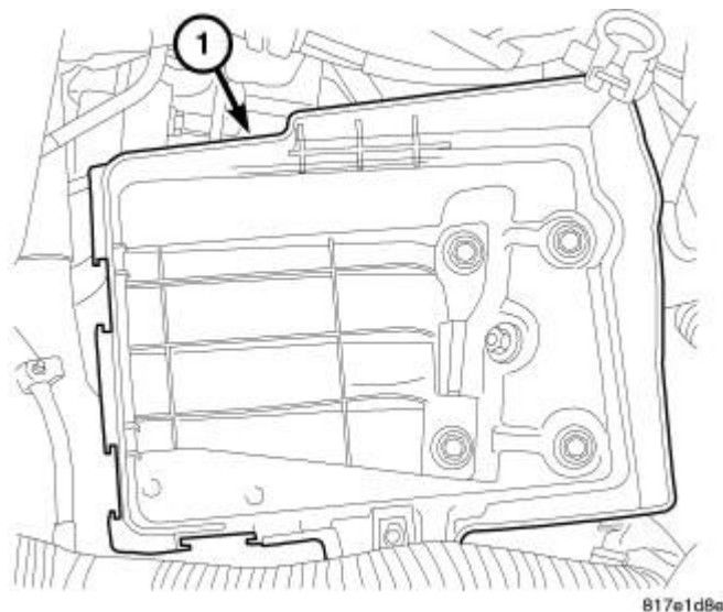
Fig. 9: BATTERY TRAY Courtesy of CHRYSLER LLC
