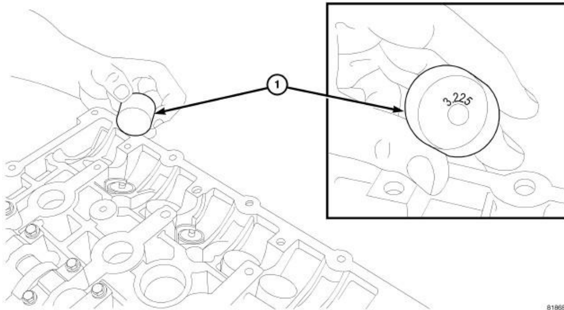
Fig. 136: TAPPET IDENTIFICATION
