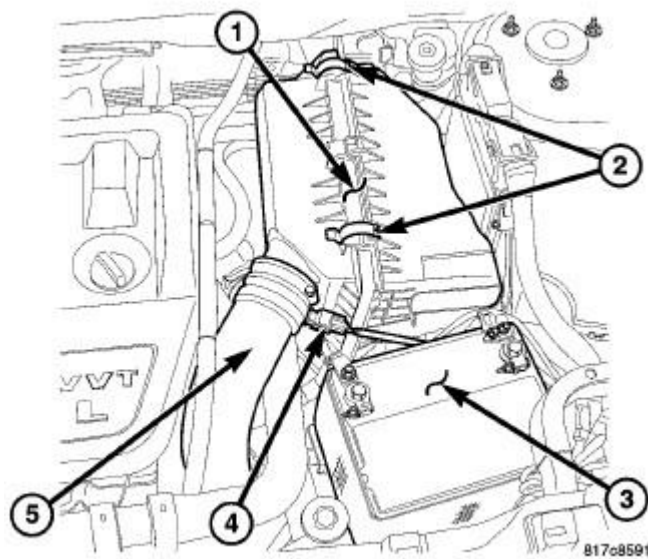
Fig. 69: AIR CLEANER HOUSING
