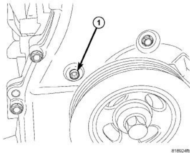
Fig. 144: TENSIONER ACCESS PLUG
