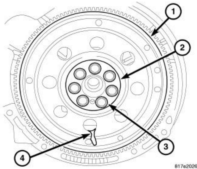
Fig. 244: FLEX PLATE Courtesy of CHRYSLER LLC
