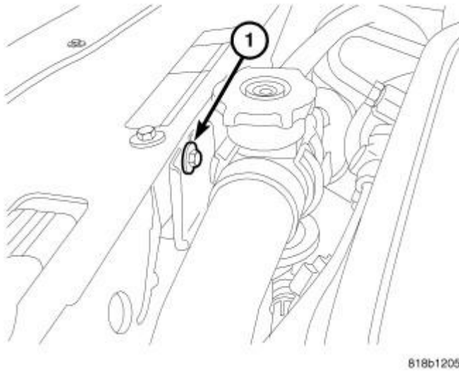
Fig. 12: Removing/Installing Upper Radiator Hose Support Courtesy of CHRYSLER LLC
