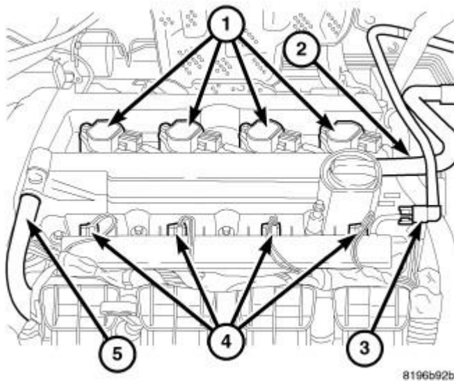
Fig. 333: COIL CONNECTOR Courtesy of CHRYSLER LLC
