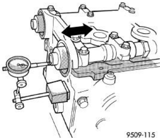
Fig. 140: Camshaft End Play Courtesy of CHRYSLER LLC
