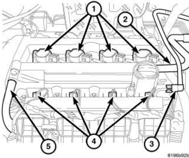
Fig. 167: COIL CONNECTOR Courtesy of CHRYSLER LLC
