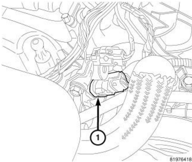
Fig. 315: OIL TEMPERATURE SENSOR
