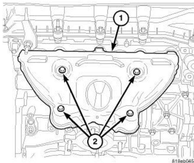
Fig. 328: EXHAUST MANIFOLD HEAT SHIELD Courtesy of CHRYSLER LLC
