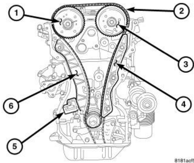
Fig. 91: TIMING DRIVE Courtesy of CHRYSLER LLC
