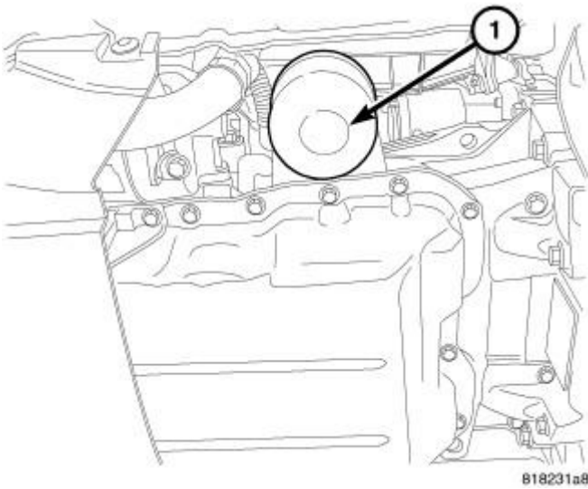
Fig. 288: OIL FILTER
