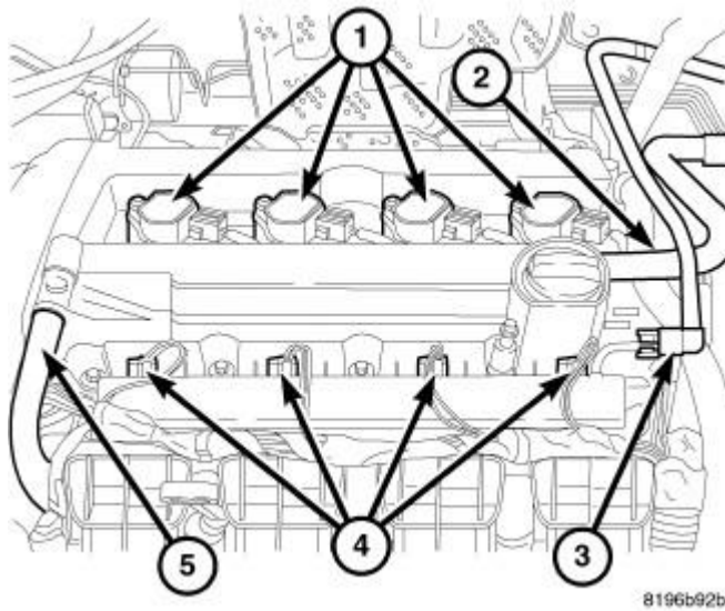
Fig. 43: COIL CONNECTOR Courtesy of CHRYSLER LLC
