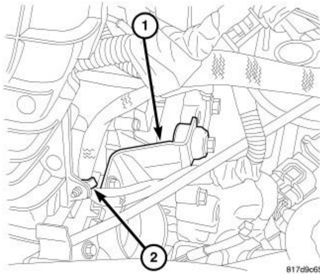
Fig. 14: Removing/Installing Throttle Body Support Bracket Courtesy of CHRYSLER LLC
