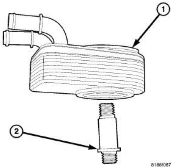
Fig. 285: OIL COOLER MOUNTING
