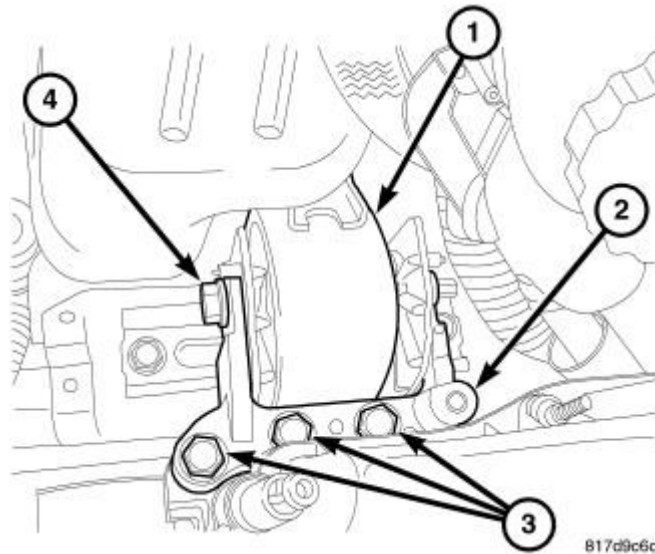
Fig. 87: Removing/Installing Right Engine Mount Adapter Courtesy of CHRYSLER LLC
