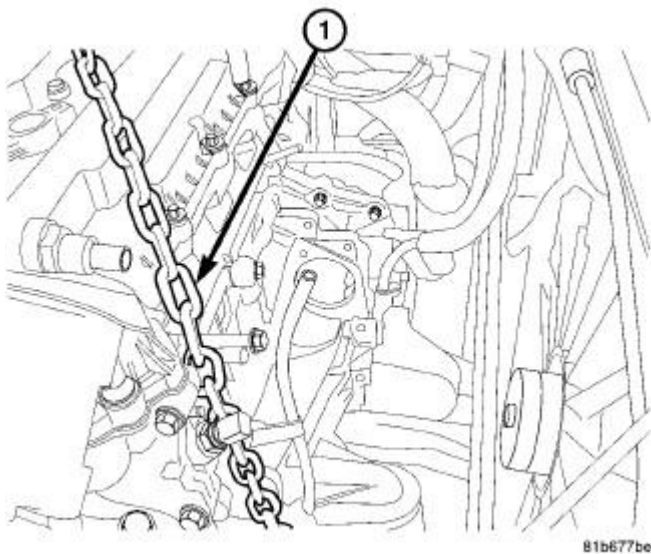
Fig. 194: LIFT CHAIN Courtesy of CHRYSLER LLC
