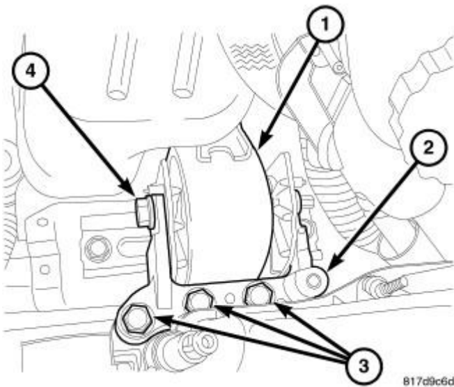
Fig. 258: RIGHT ENGINE MOUNT Courtesy of CHRYSLER LLC
