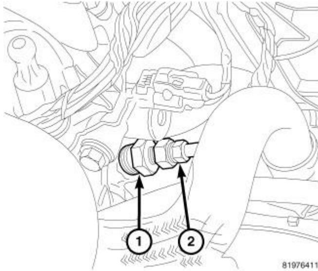
Fig. 266: OIL PRESSURE ADAPTER 9879
