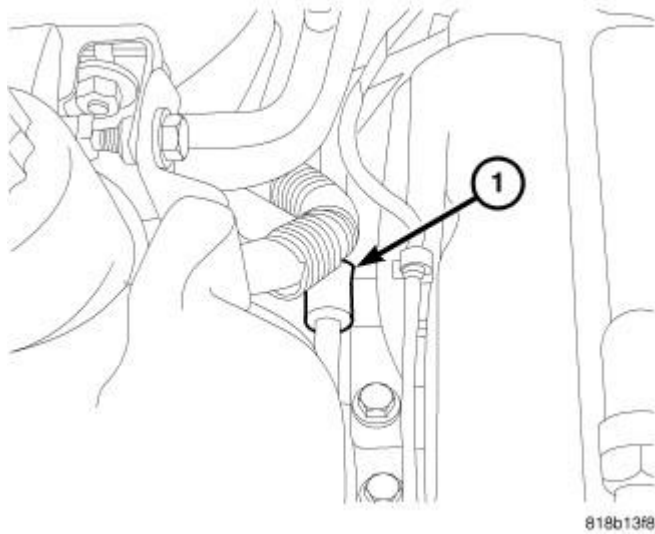
Fig. 17: Removing/Installing Power Steering Line Support At Engine Mount Courtesy of CHRYSLER LLC
