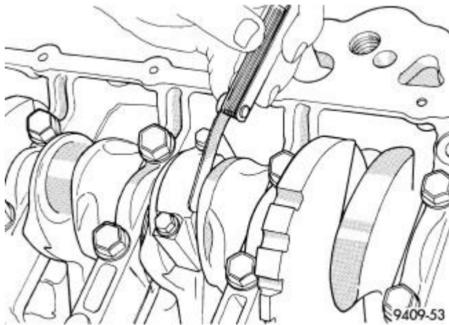
Fig. 234: Connecting Rod Side Clearance Courtesy of CHRYSLER LLC
