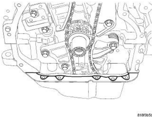
Fig. 378: SEALING OIL PAN
