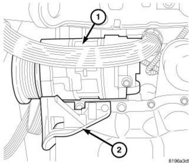
Fig. 82: Removing/Installing Lower A/C Compressor Mount Courtesy of CHRYSLER LLC
