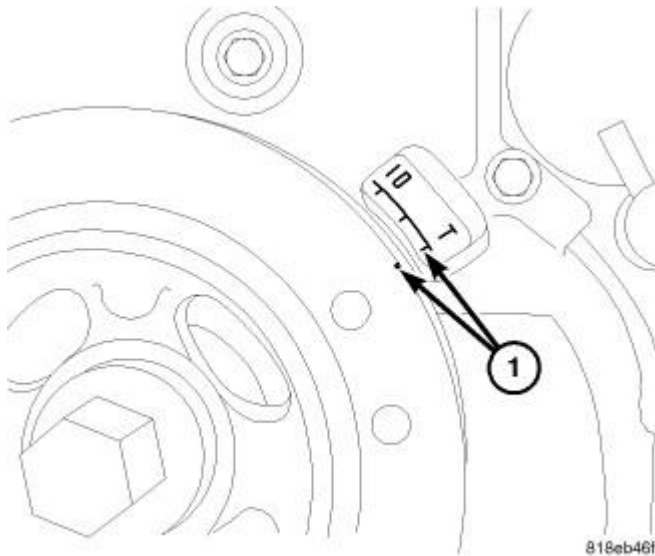
Fig. 366: Setting Engine To Top Dead Center Courtesy of CHRYSLER LLC
