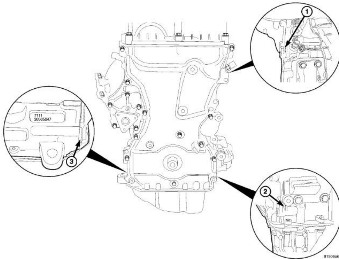
Fig. 90: TIMING CHAIN COVER PRY POINTS Courtesy of CHRYSLER LLC
