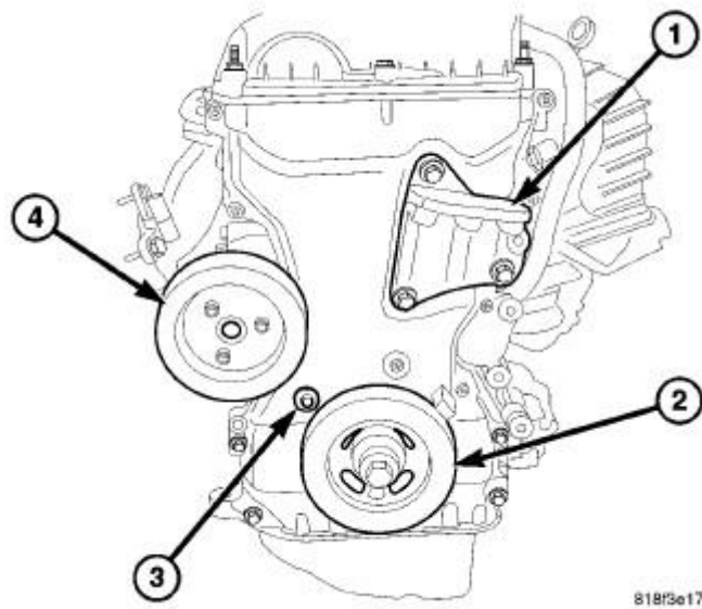
Fig. 89: ENGINE FRONT Courtesy of CHRYSLER LLC
