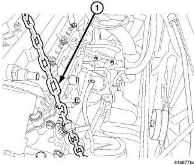
Fig. 28: Removing/Installing Engine Lift Chain Courtesy of CHRYSLER LLC
