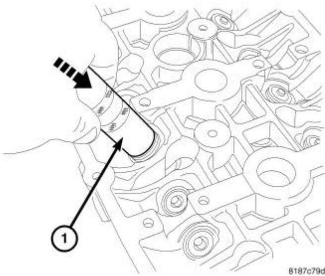
Fig. 178: VALVE REMOVAL Courtesy of CHRYSLER LLC
