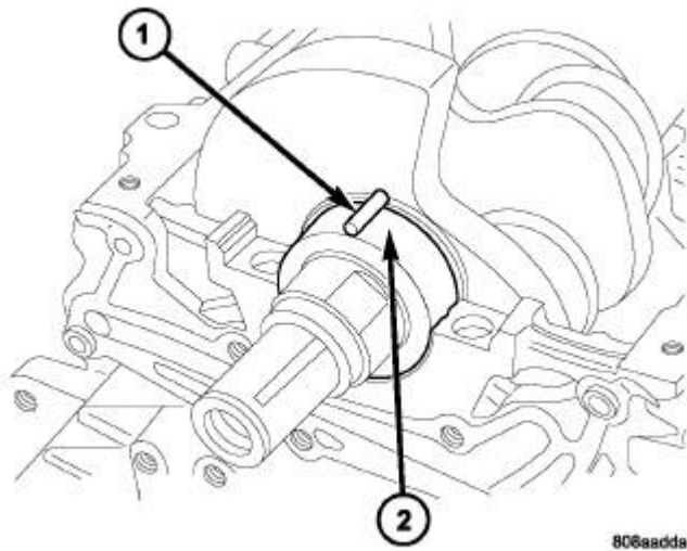
Fig. 4: Plastigage Placed in Lower Shell-Typical Courtesy of CHRYSLER LLC
