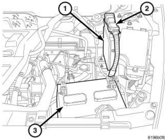
Fig. 251: BATTERY Courtesy of CHRYSLER LLC
