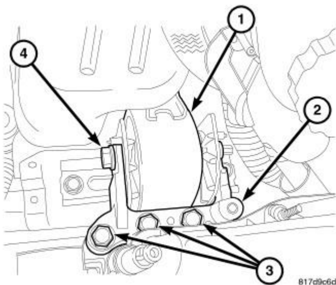
Fig. 27: Removing/Installing Engine Mount Adapter & Engine Mount
