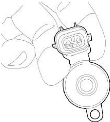
Fig. 275: SOLENOID MOUNTING TAB 1/1 Courtesy of CHRYSLER LLC
