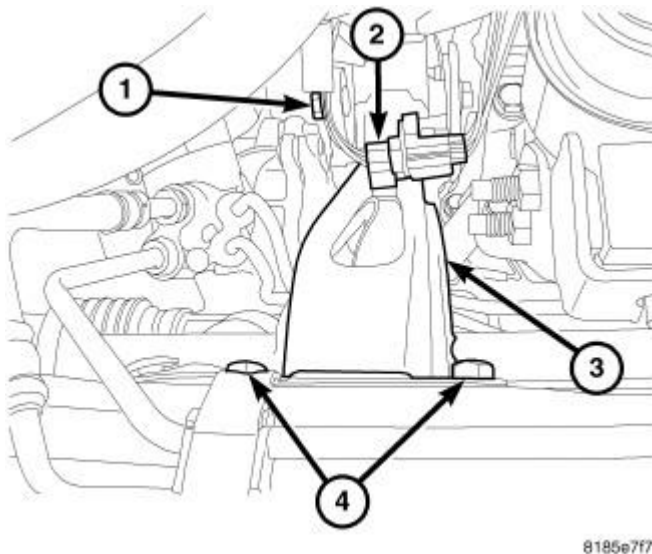
Fig. 254: REAR MOUNT-ATX
