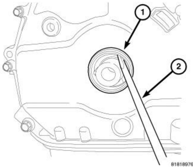
Fig. 236: FRONT CRANKSHAFT SEAL REMOVAL Courtesy of CHRYSLER LLC
