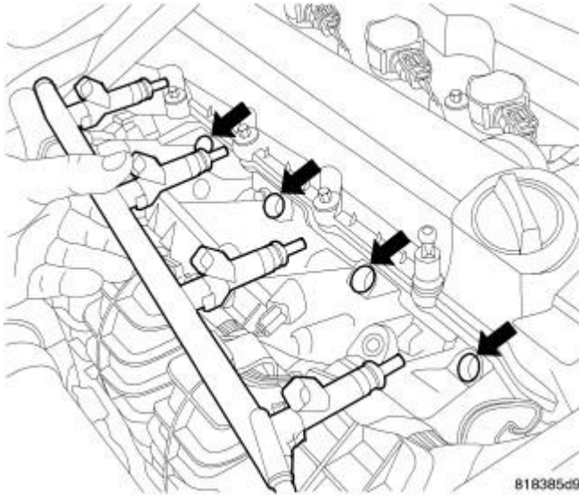
Fig. 94: RAIL REMOVAL/INSTALL Courtesy of CHRYSLER LLC
