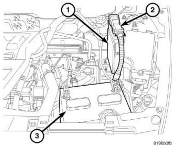
Fig. 8: Removing/Installing Battery Courtesy of CHRYSLER LLC
