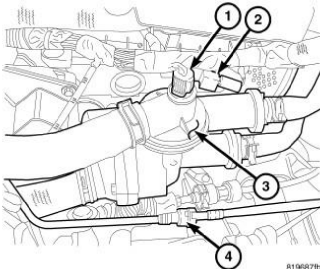
Fig. 45: Removing/Installing Coolant Adapter Assembly Courtesy of CHRYSLER LLC
