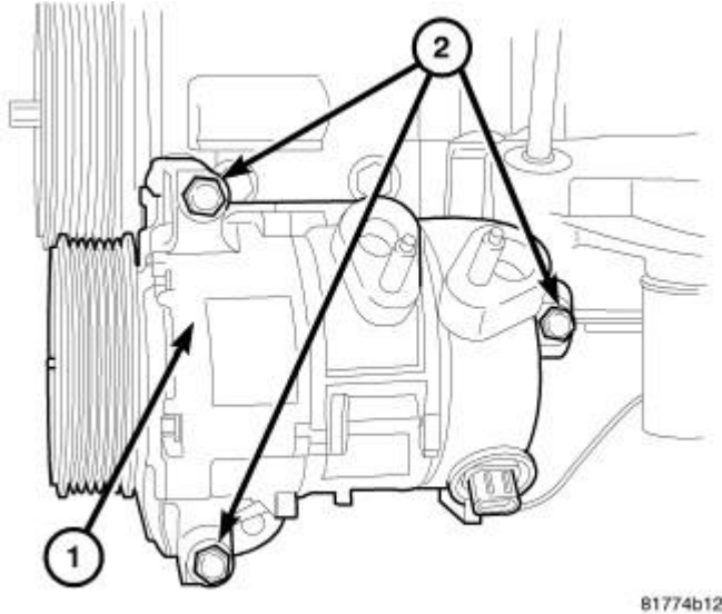
Fig. 319: Removing/Installing A/C Compressor Courtesy of CHRYSLER LLC
