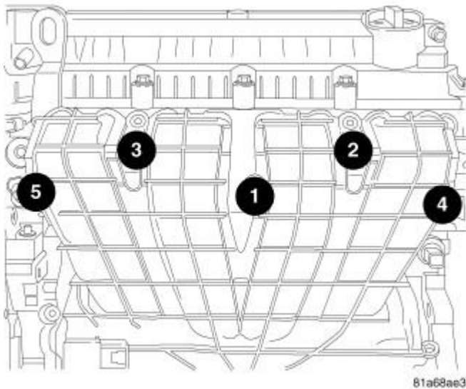
Fig. 339: Removing/Installing Intake Bolts - Torque Sequence Courtesy of CHRYSLER LLC
