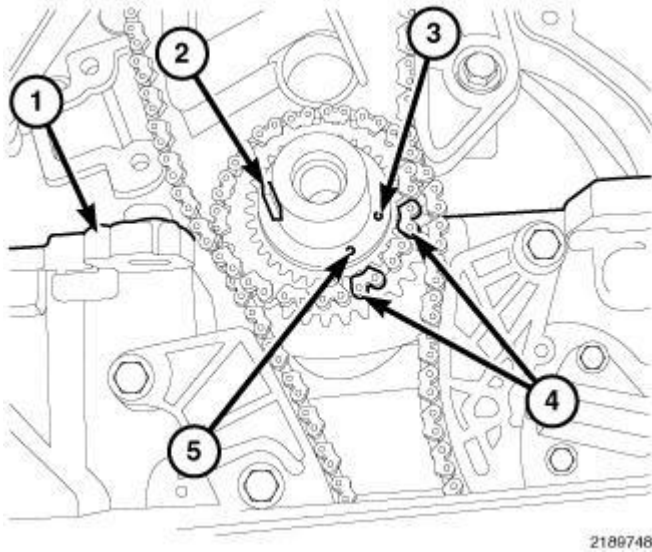
Fig. 347: Crankshaft Timing Marks
