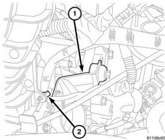
Fig. 41: Removing/Installing Throttle Body Support & Harness Retainer Courtesy of CHRYSLER LLC
