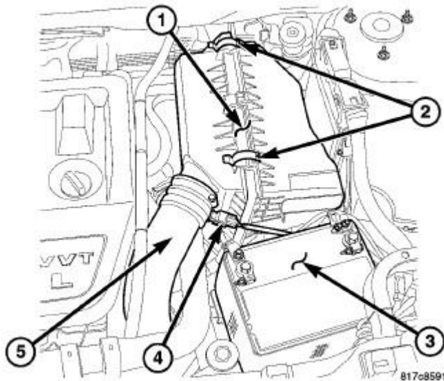
Fig. 342: AIR CLEANER HOUSING Courtesy of CHRYSLER LLC
