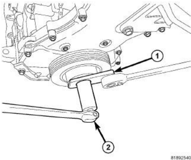
Fig. 215: DAMPER REMOVAL Courtesy of CHRYSLER LLC
