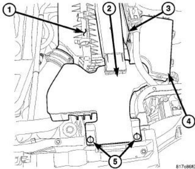
Fig. 7: AIR CLEANER INLET Courtesy of CHRYSLER LLC
