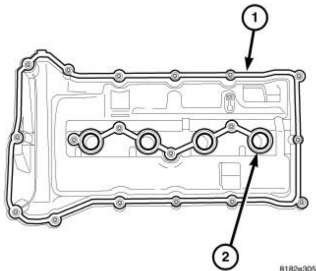
Fig. 169: GASKET LOCATION Courtesy of CHRYSLER LLC
