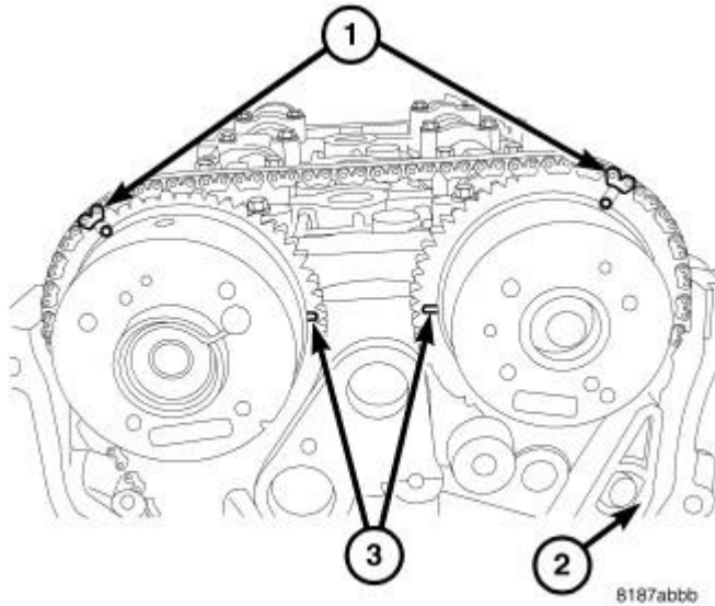
Fig. 143: TIMING CHAIN TIMING MARKS
