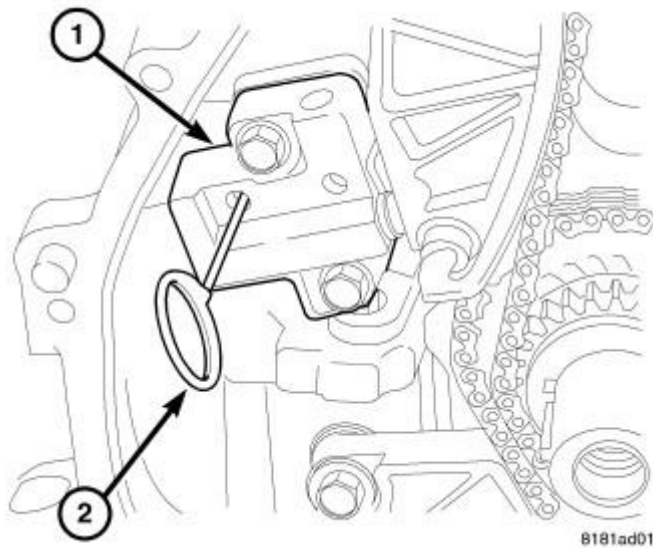
Fig. 396: TIMING CHAIN TENSIONER
