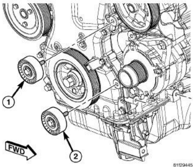
Fig. 382: Removing/Installing Accessory Drive Belt Lower Idler Pulley Courtesy of CHRYSLER LLC
