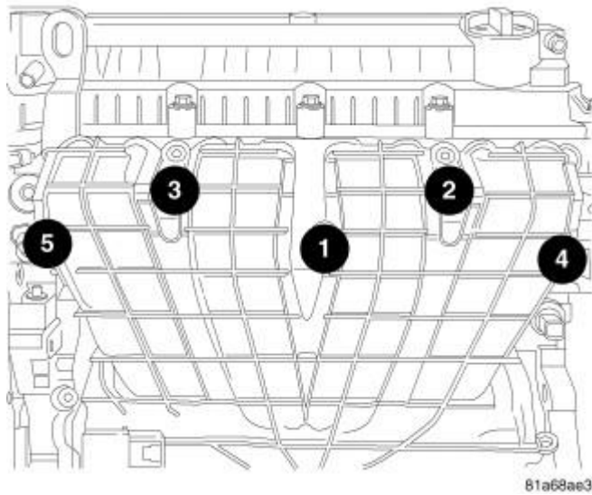
Fig. 16: Removing/Installing Intake Bolts - Torque Sequence Courtesy of CHRYSLER LLC
