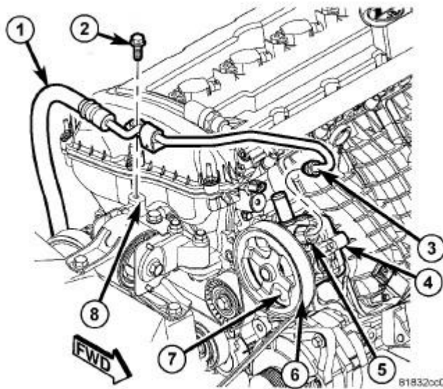
Fig. 390: PRESSURE HOSE Courtesy of CHRYSLER LLC
