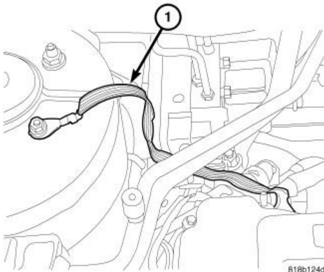
Fig. 121: Ground Strap Courtesy of CHRYSLER LLC
