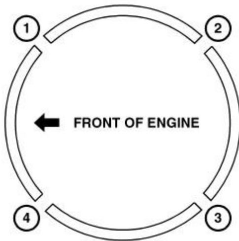
Fig. 227: Piston Ring End Gap Position Courtesy of CHRYSLER LLC
