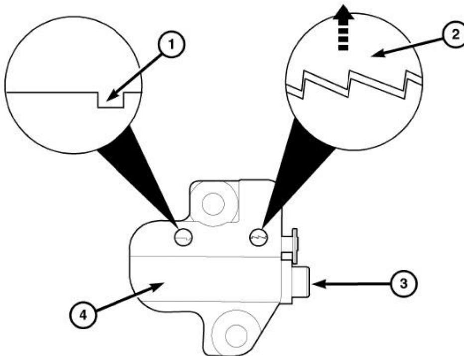
Fig. 145: TENSIONER RESET Courtesy of CHRYSLER LLC
