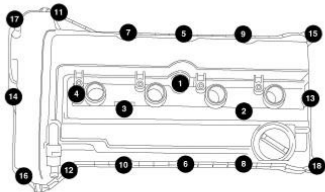
Fig. 135: TORQUE SEQUENCE
