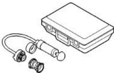
Fig. 54: TESTER, COOLING SYSTEM - 7700-A Courtesy of CHRYSLER LLC
