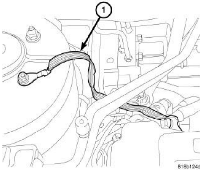
Fig. 100: GROUND STRAP Courtesy of CHRYSLER LLC
