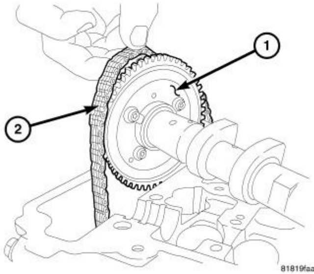
Fig. 151: Identifying Timing Chain & Sprocket Courtesy of CHRYSLER LLC
