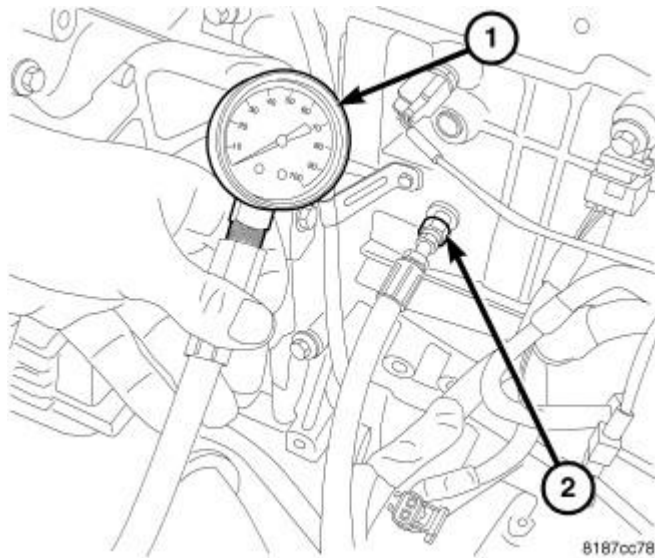
Fig. 269: OIL PRESSURE GAUGE Courtesy of CHRYSLER LLC
