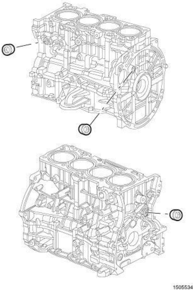
Fig. 301: Engine Block Tapered Plugs Courtesy of CHRYSLER LLC
