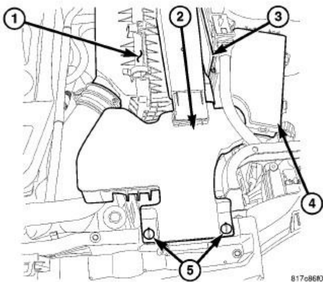
Fig. 247: AIR CLEANER INLET Courtesy of CHRYSLER LLC
