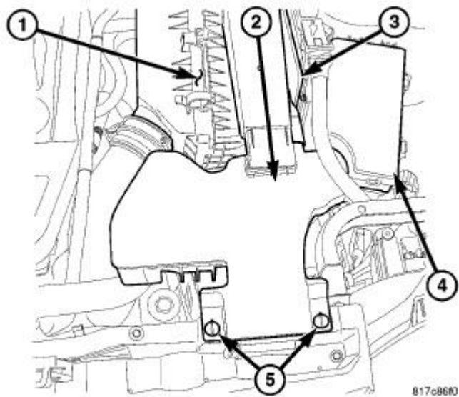
Fig. 252: AIR CLEANER INLET Courtesy of CHRYSLER LLC
