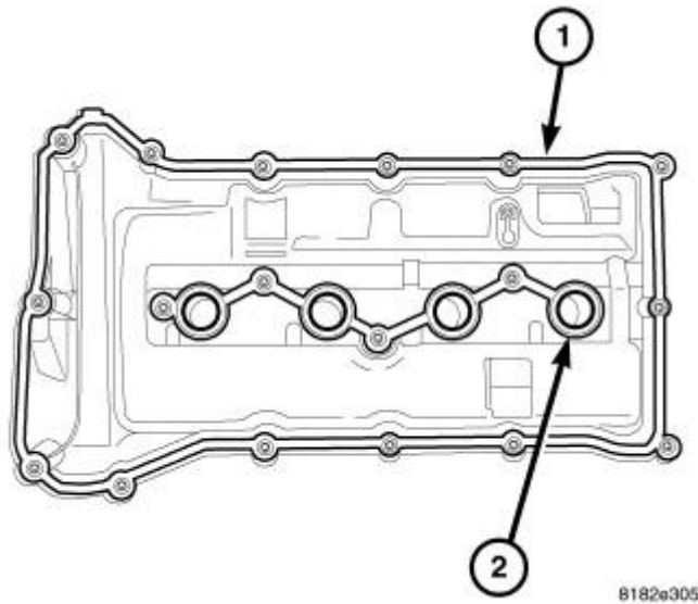
Fig. 163: GASKET LOCATION Courtesy of CHRYSLER LLC
