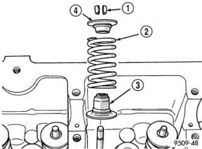
Fig. 179: Valve Spring Assembly Courtesy of CHRYSLER LLC
