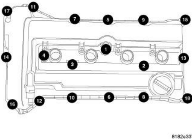
Fig. 164: Cylinder Head Cover Bolt Torque Sequence Courtesy of CHRYSLER LLC
