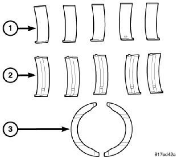
Fig. 207: BEARING IDENTIFICATION Courtesy of CHRYSLER LLC
