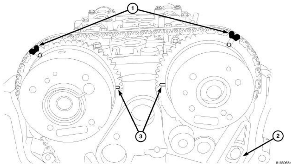
Fig. 159: TIMING CHAIN TIMING MARKS Courtesy of CHRYSLER LLC
