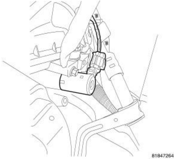
Fig. 276: SOLENOID LOCATION 1/2 Courtesy of CHRYSLER LLC
