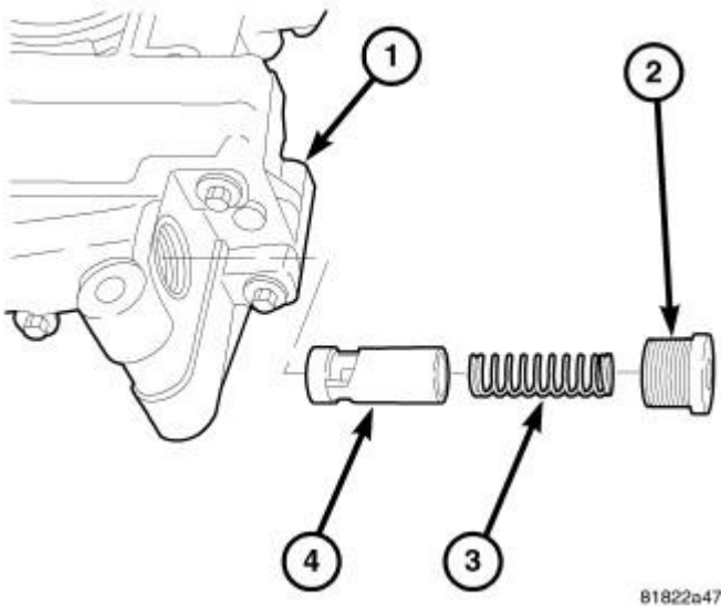
Fig. 321: OIL PRESSURE RELIEF VALVE
