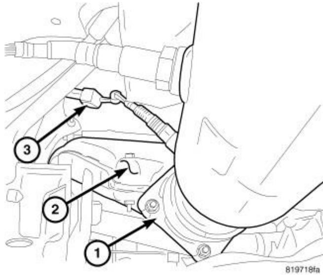
Fig. 86: Removing/Installing Under Floor Catalytic Converter Courtesy of CHRYSLER LLC
