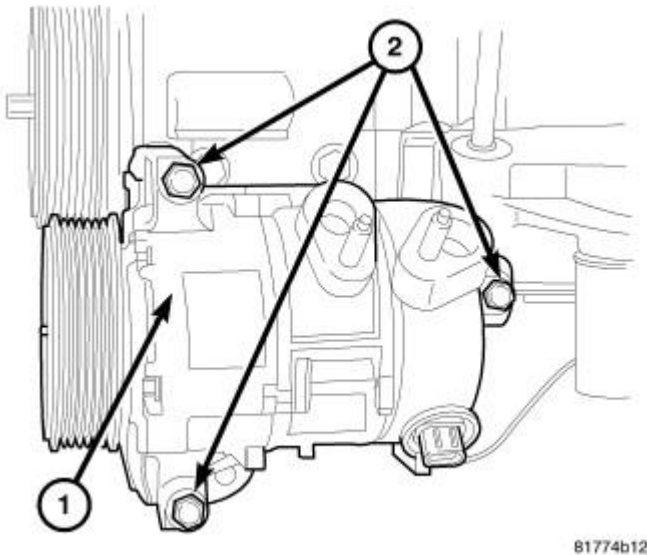
Fig. 316: Removing/Installing A/C Compressor Courtesy of CHRYSLER LLC
