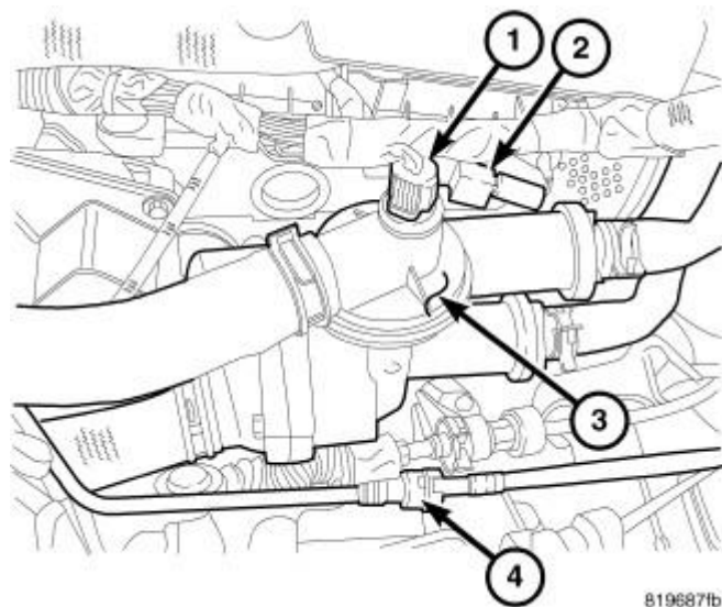
Fig. 11: Removing/Installing Coolant Hoses At Coolant Adapter
