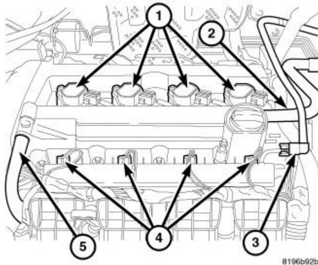
Fig. 335: COIL CONNECTOR Courtesy of CHRYSLER LLC
