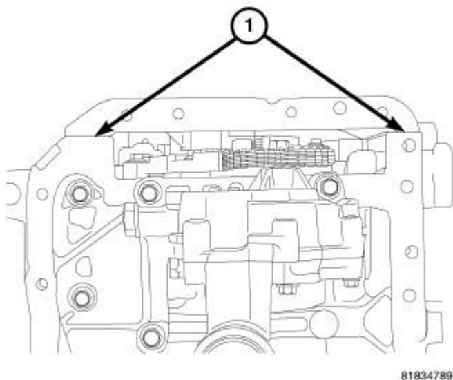
Fig. 298: Sealer Location
