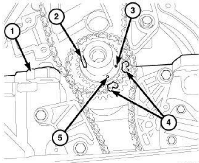
Fig. 360: Crankshaft Timing Marks
