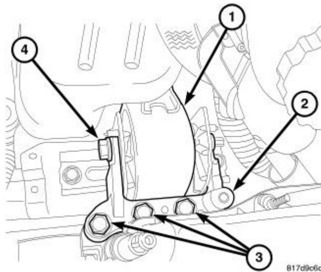
Fig. 87: Right Engine Mount Courtesy of CHRYSLER LLC
