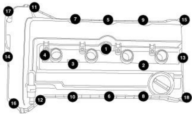
Fig. 389: Torque Sequence Courtesy of CHRYSLER LLC
