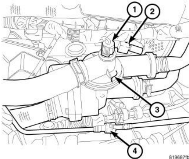
Fig. 45: Coolant Adapter Courtesy of CHRYSLER LLC
