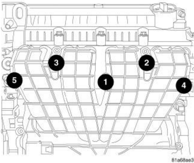
Fig. 340: Torque Sequence Courtesy of CHRYSLER LLC
