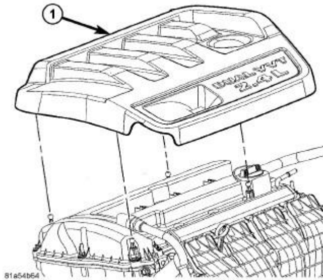
Fig. 394: Engine Cover - 2.4L Courtesy of CHRYSLER LLC
