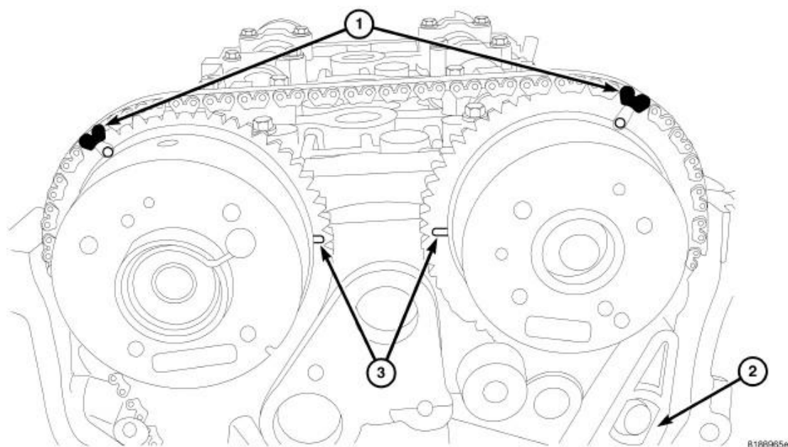
Fig. 348: Timing Chain Timing Marks
