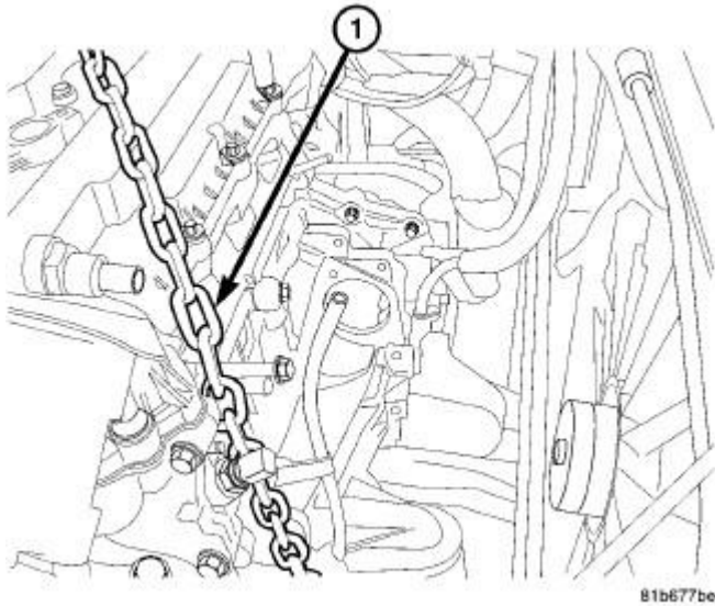
Fig. 24: Lift Chain
