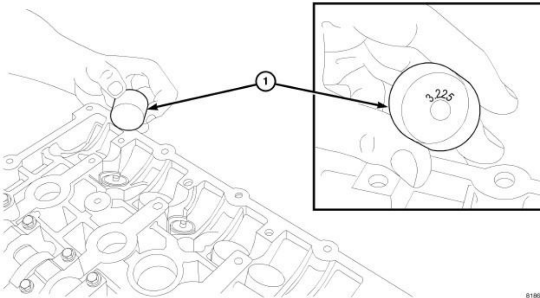
Fig. 137: Tappet Identification Courtesy of CHRYSLER LLC
