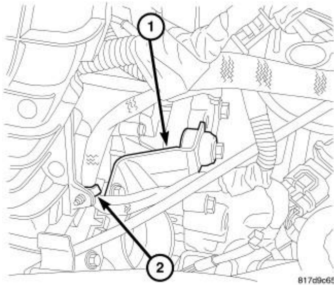
Fig. 14: Throttle Body Support Courtesy of CHRYSLER LLC
