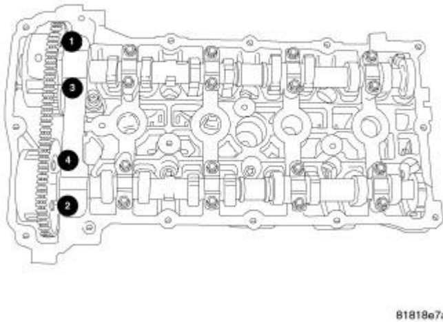
Fig. 148: Front Cam Cap Removal Sequence Courtesy of CHRYSLER LLC
