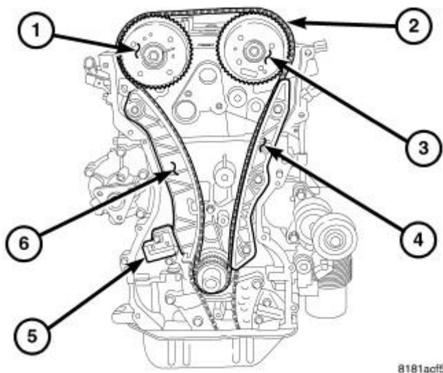
Fig. 350: Timing Drive Courtesy of CHRYSLER LLC
