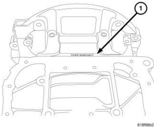
Fig. 64: Serial Number
