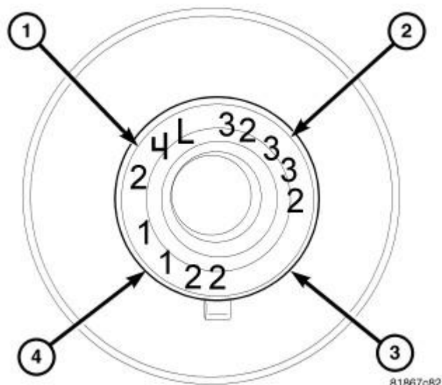
Fig. 190: Lower Main Bearing Identification Courtesy of CHRYSLER LLC
