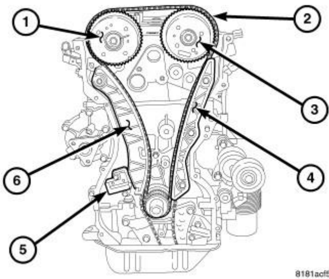
Fig. 395: Timing Drive Courtesy of CHRYSLER LLC
