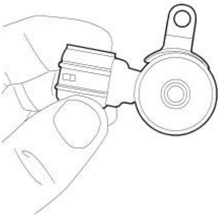
Fig. 281: Solenoid Mounting Tab 1/2 Courtesy of CHRYSLER LLC
