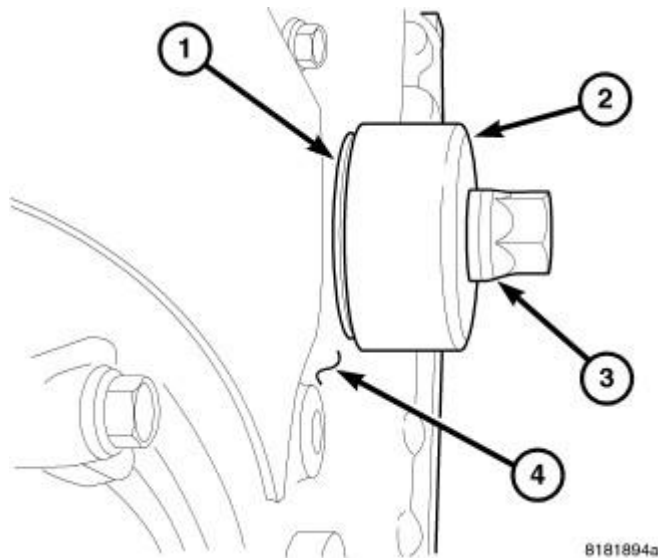
Fig. 238: Front Seal Courtesy of CHRYSLER LLC
