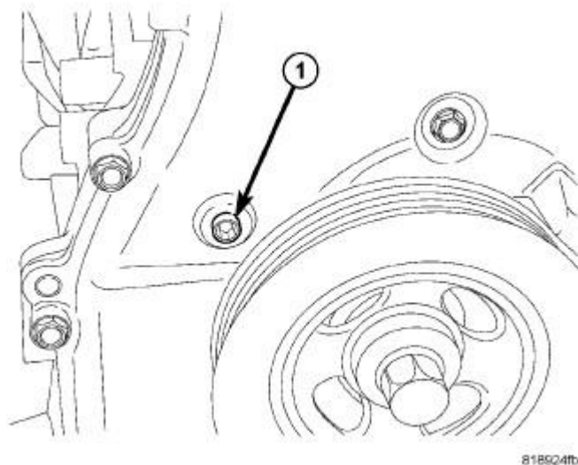
Fig. 144: Tensioner Access Plug Courtesy of CHRYSLER LLC
