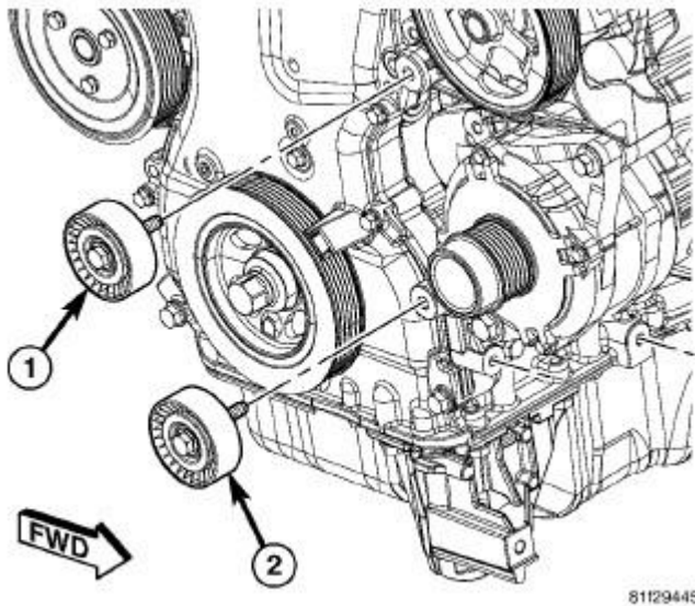
Fig. 387: Accessory Drive Belt Idler Pulley - 2.4L Courtesy of CHRYSLER LLC
