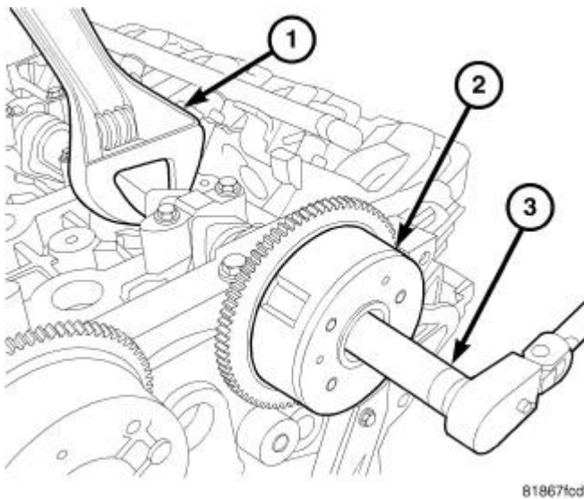
Fig. 129: Cam Phaser Installation Courtesy of CHRYSLER LLC
