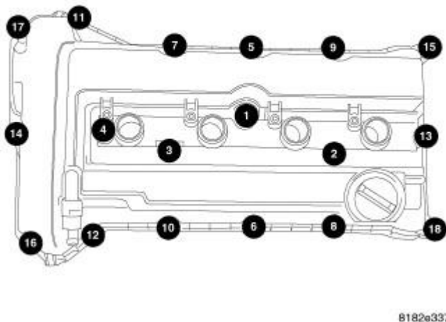
Fig. 172: Torque Sequence
