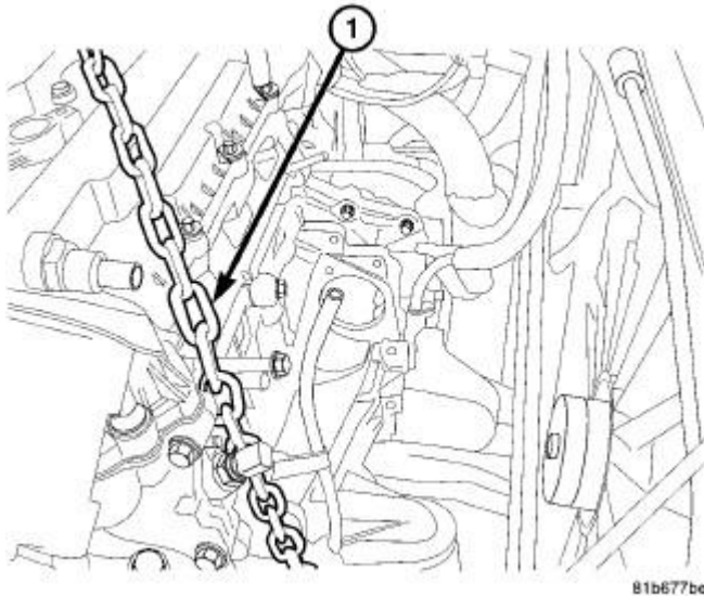
Fig. 213: Lift Chain Courtesy of CHRYSLER LLC
