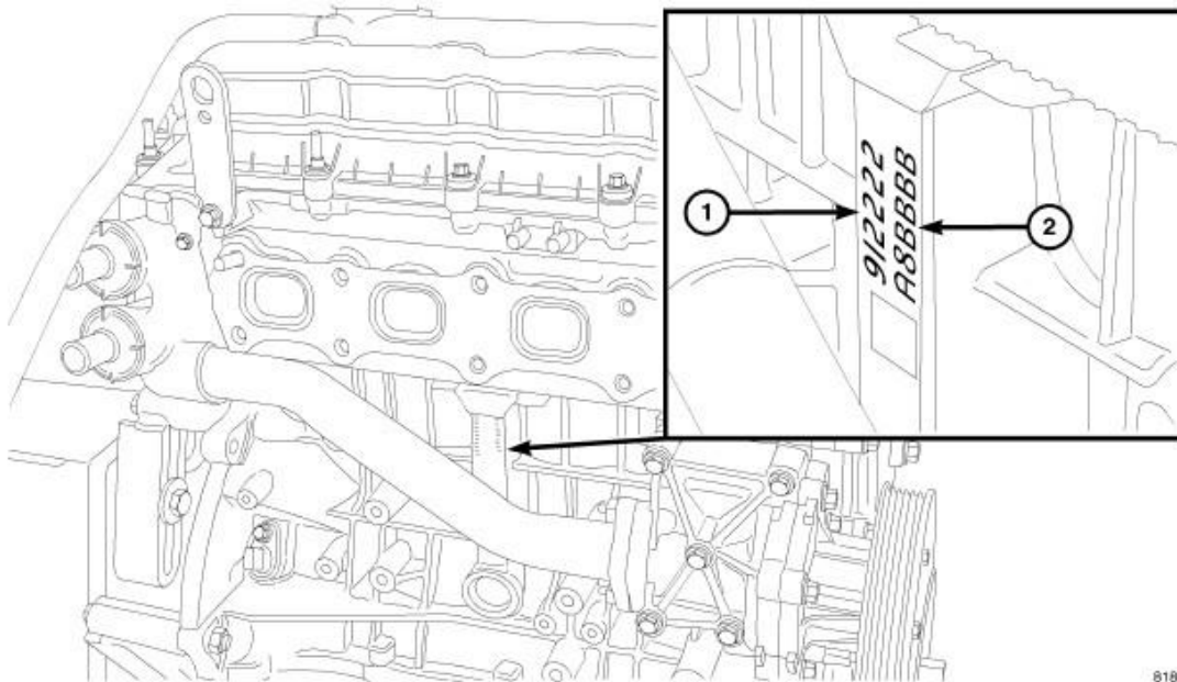
Fig. 191: Upper Main Bearing Shell Identification Courtesy of CHRYSLER LLC
