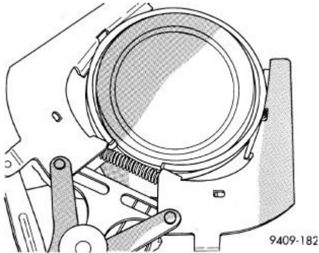
Fig. 225: Piston Rings - Removing & Installing Courtesy of CHRYSLER LLC
