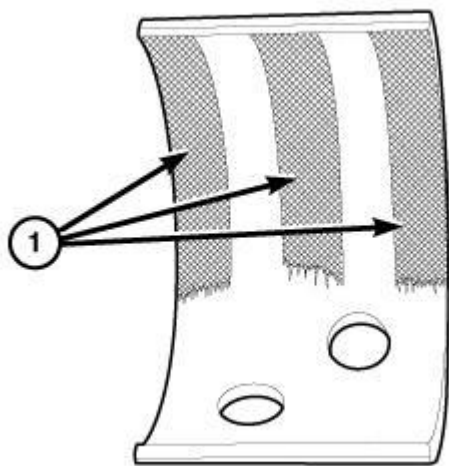
Fig. 139: Uneven Wear Patterns Courtesy of CHRYSLER LLC
