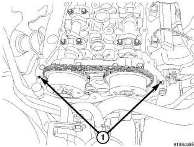
Fig. 171: CYL Head T-Joint Courtesy of CHRYSLER LLC
