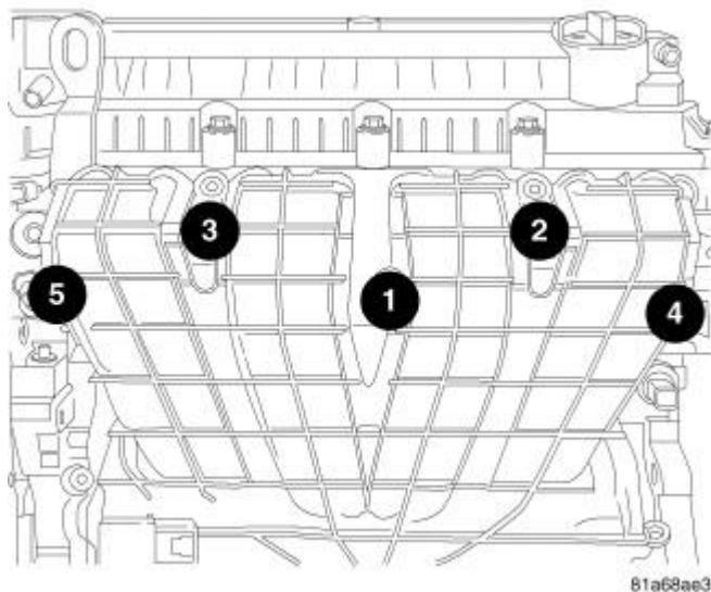
Fig. 339: Torque Sequence Courtesy of CHRYSLER LLC
