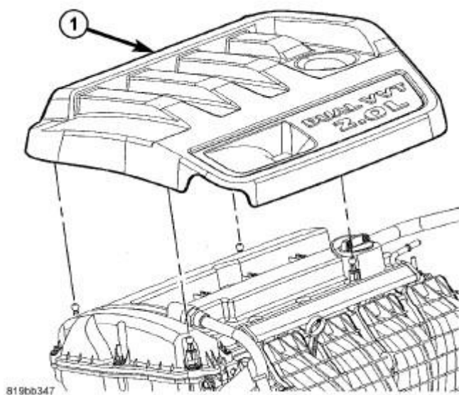
Fig. 166: Engine Cover - 2.0L
