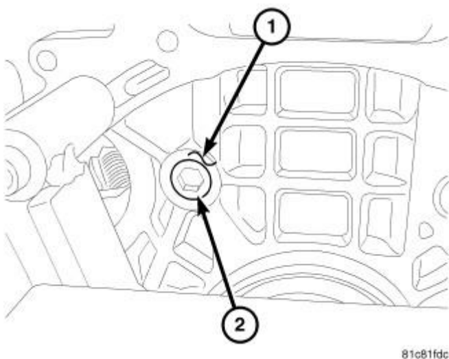
Fig. 302: Gallery Plug
