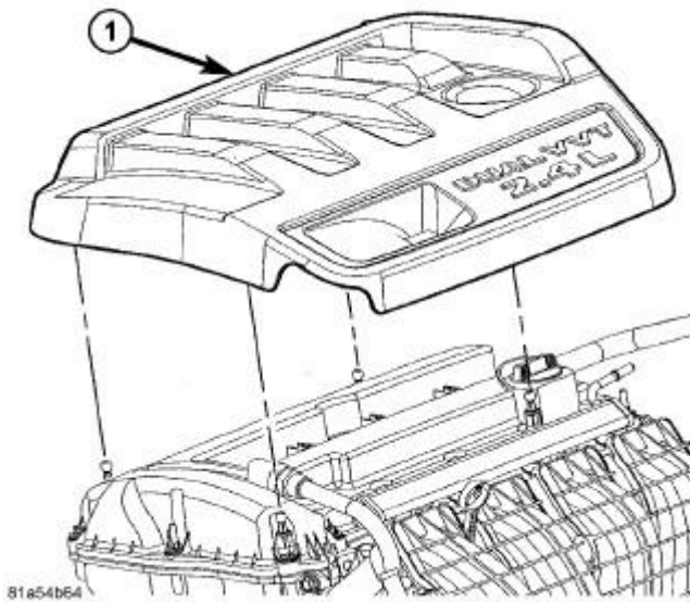
Fig. 141: Engine Cover Courtesy of CHRYSLER LLC
