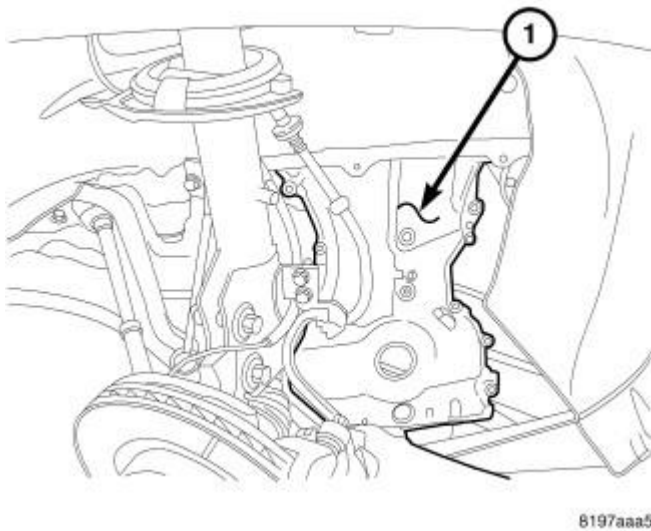
Fig. 381: Timing Chain Cover Removal Courtesy of CHRYSLER LLC
