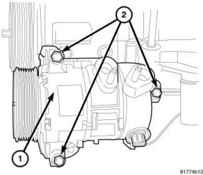
Fig. 316: A/C Compressor - R & I Courtesy of CHRYSLER LLC
