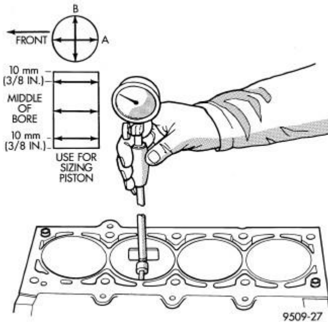
Fig. 186: Checking Cylinder Bore Size Courtesy of CHRYSLER LLC
