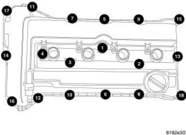
Fig. 164: Torque Sequence Courtesy of CHRYSLER LLC
