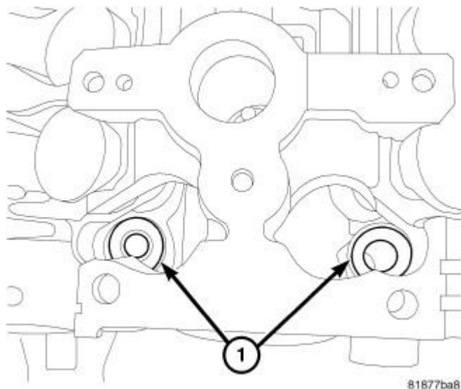
Fig. 102: Front Head Bolt Washers Courtesy of CHRYSLER LLC
