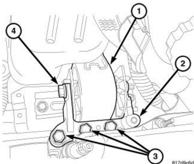
Fig. 27: Right Engine Mount
