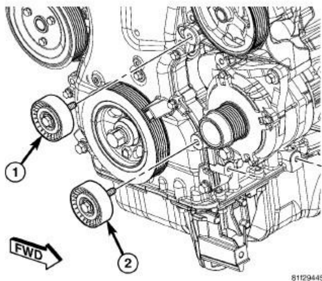
Fig. 83: Accessory Drive Belt Idler Pulley - 2.4L Courtesy of CHRYSLER LLC
