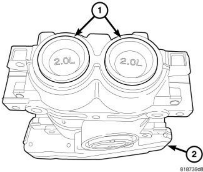
Fig. 304: BSM Identification
