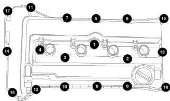
Fig. 120: Torque Sequence Courtesy of CHRYSLER LLC
