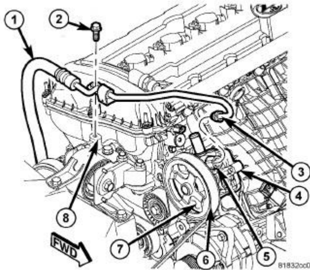
Fig. 364: Pressure Hose Courtesy of CHRYSLER LLC
