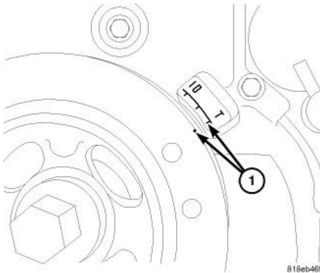
Fig. 142: TDC Courtesy of CHRYSLER LLC
