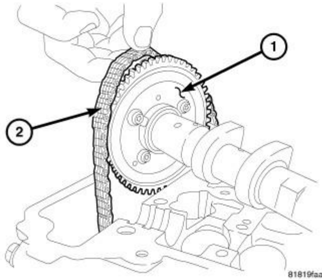
Fig. 151: Chain Removal Courtesy of CHRYSLER LLC
