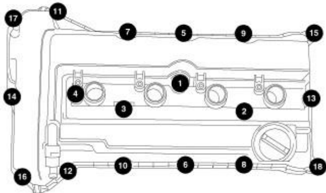
Fig. 135: Torque Sequence
