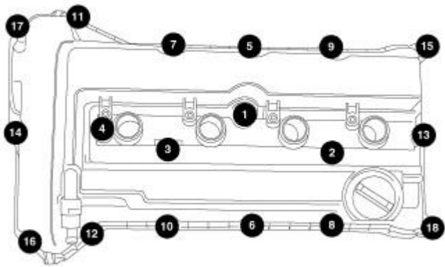
Fig. 168: Torque Sequence Courtesy of CHRYSLER LLC
