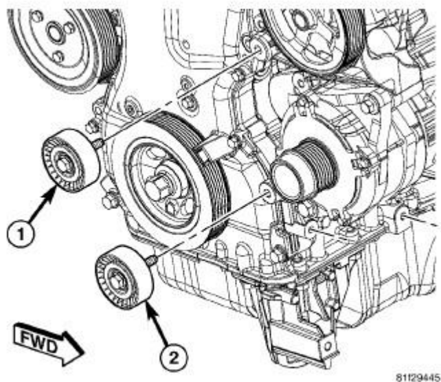
Fig. 88: Accessory Drive Belt Idler Pulley - 2.4L Courtesy of CHRYSLER LLC
