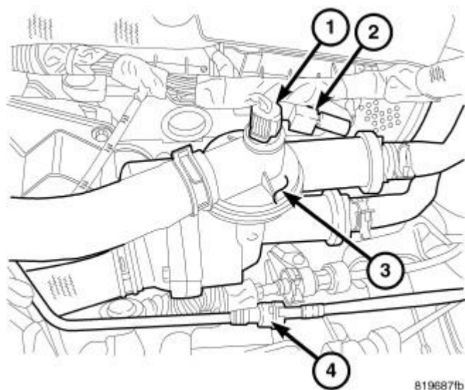
Fig. 11: Coolant Adapter
