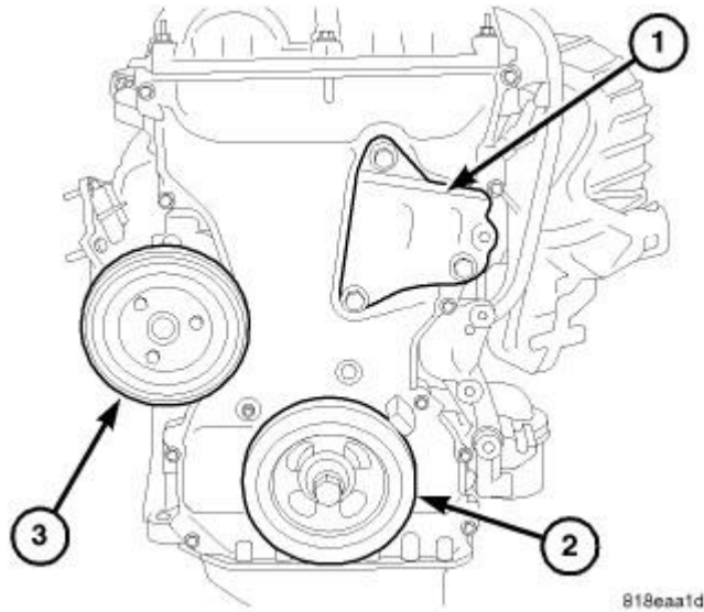
Fig. 197: Right Engine Mount Bracket Courtesy of CHRYSLER LLC
