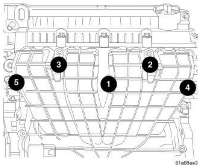
Fig. 40: Torque Sequence Courtesy of CHRYSLER LLC
