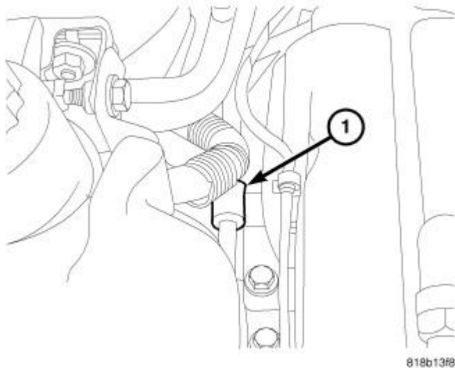
Fig. 256: Power Steering Line Support Bracket Courtesy of CHRYSLER LLC
