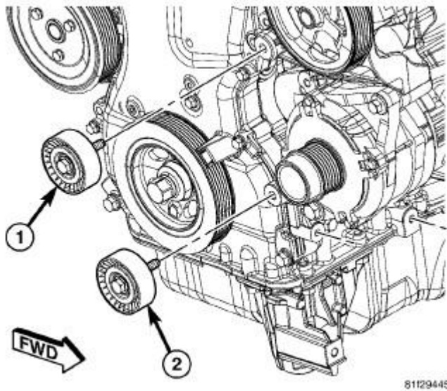
Fig. 373: Accessory Drive Belt Idler Pulley - 2.4L Courtesy of CHRYSLER LLC
