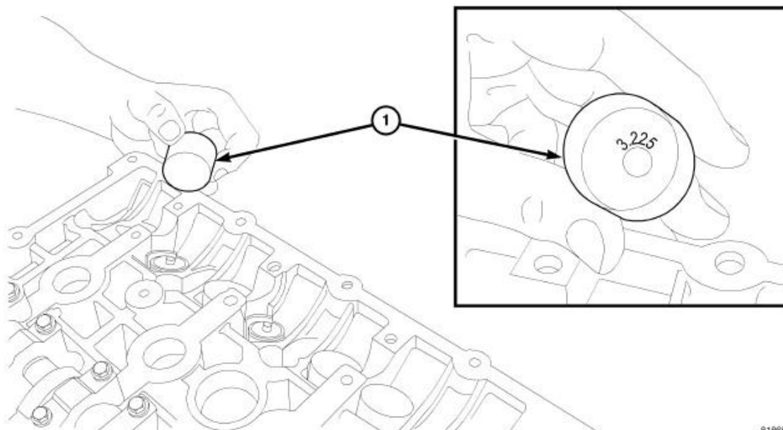
Fig. 133: Tappet Identification
