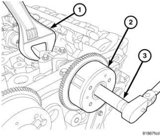
Fig. 130: Cam Phaser Installation Courtesy of CHRYSLER LLC
