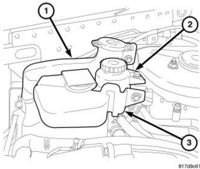
Fig. 392: Coolant Reservoir Courtesy of CHRYSLER LLC
