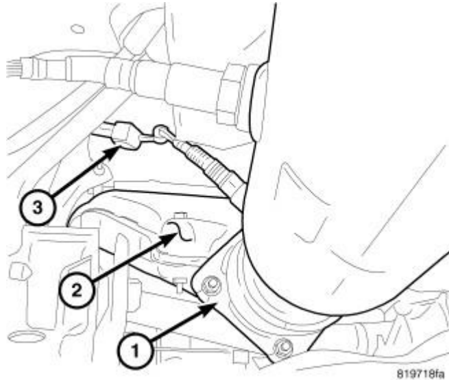
Fig. 30: Manifold To Exhaust Pipe Bolts Courtesy of CHRYSLER LLC
