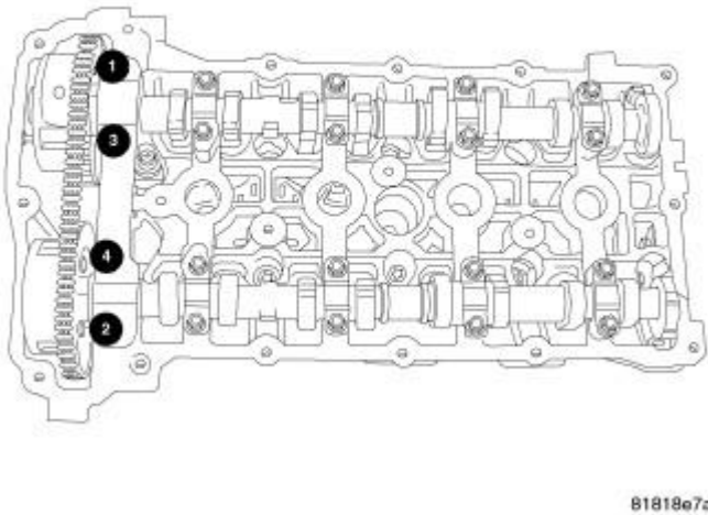
Fig. 101: Front Cam Cap Removal Sequence Courtesy of CHRYSLER LLC
