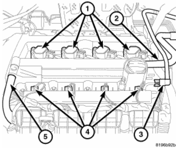
Fig. 310: Coil Connector Courtesy of CHRYSLER LLC
