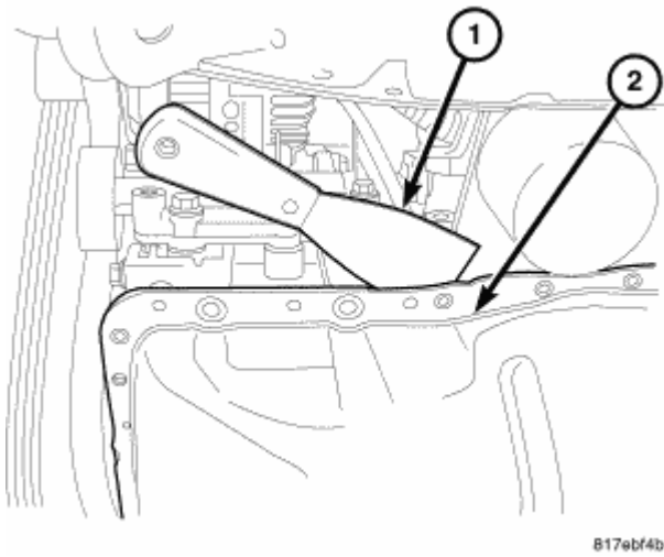
Fig. 178: Oil Pan Removal Courtesy of CHRYSLER LLC
