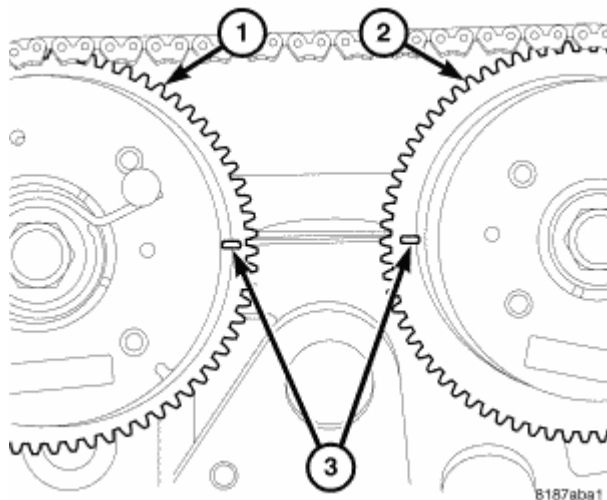
Fig. 133: Camshaft Timing
