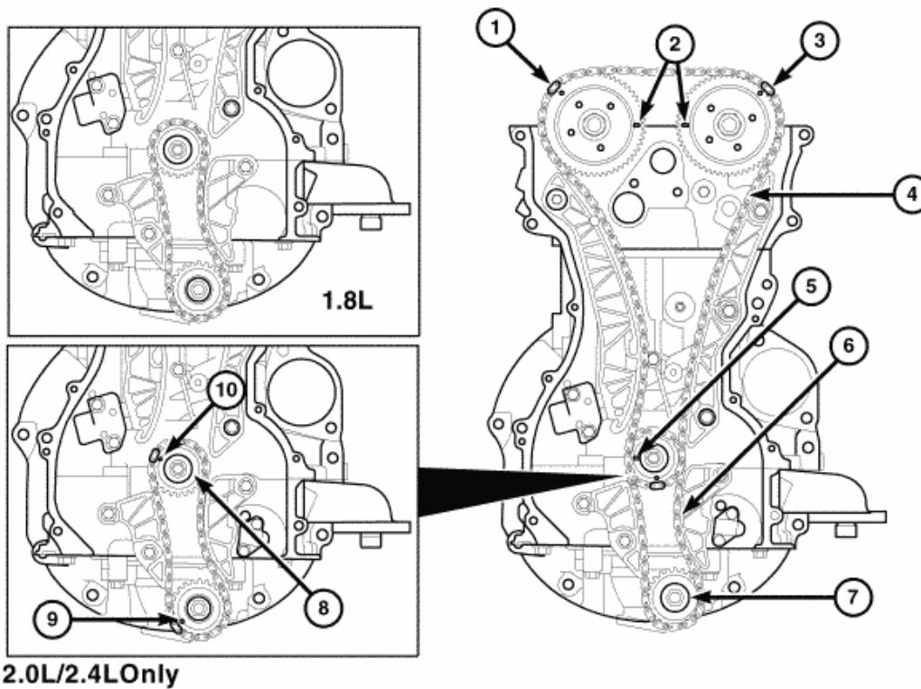
Fig. 323: Timing Marks Courtesy of CHRYSLER LLC
