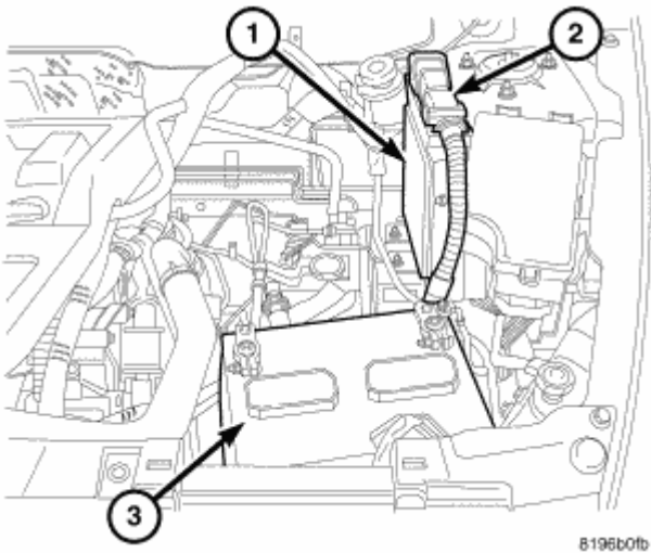
Fig. 117: Battery, Negative Battery Cable & PCM Courtesy of CHRYSLER LLC
