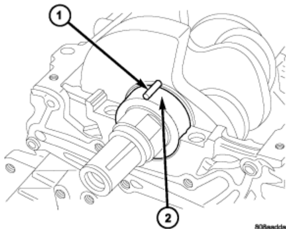
Fig. 5: Identifying Plastigage Courtesy of CHRYSLER LLC
