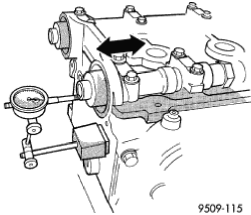
Fig. 116: Measuring Camshaft End Play Courtesy of CHRYSLER LLC
