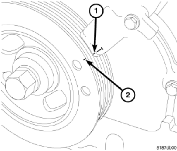
Fig. 322: TDC Courtesy of CHRYSLER LLC
