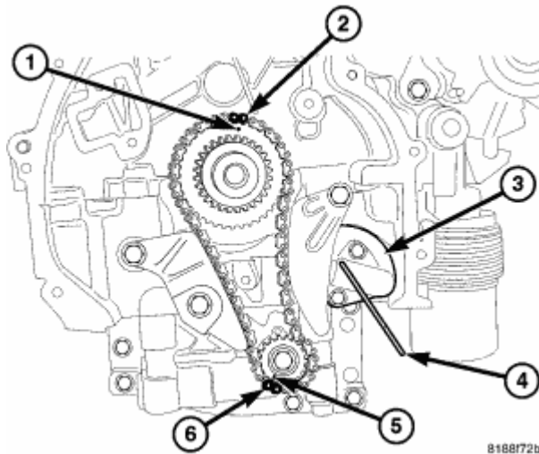
Fig. 362: Oil Pump Drive Chain Courtesy of CHRYSLER LLC
