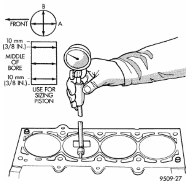
Fig. 206: Checking Cylinder Bore Size Courtesy of CHRYSLER LLC
