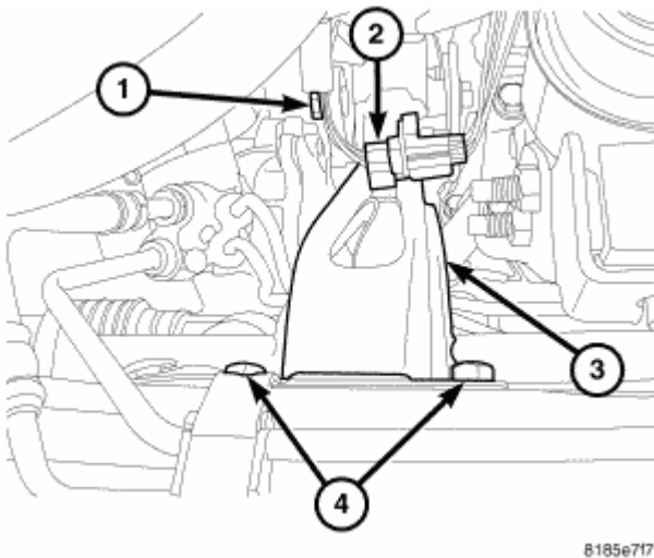
Fig. 242: Rear Mount Courtesy of CHRYSLER LLC
