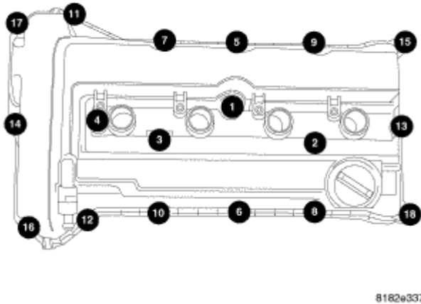
Fig. 160: Torque Sequence
