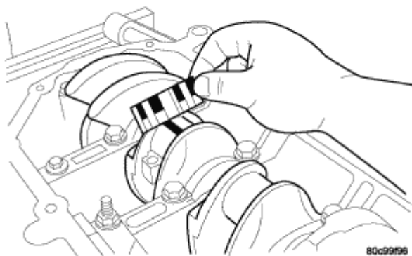
Fig. 215: Connecting Rod Bearing Clearance - Typical Courtesy of CHRYSLER LLC
