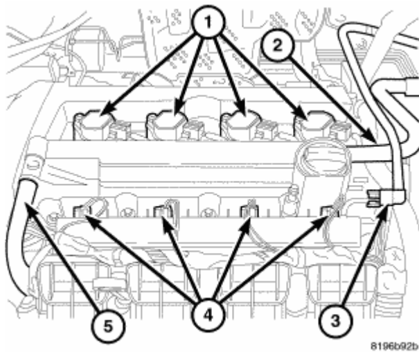
Fig. 318: Coil Connector Courtesy of CHRYSLER LLC
