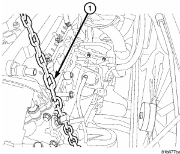
Fig. 28: Lift Chain
