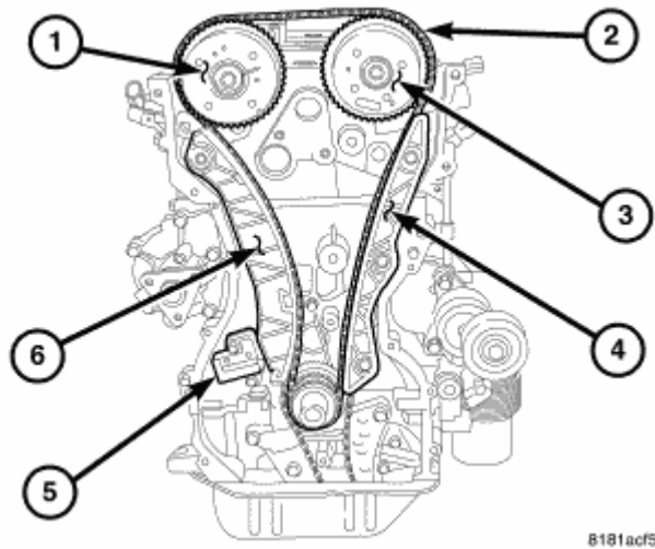
Fig. 356: Timing Drive
