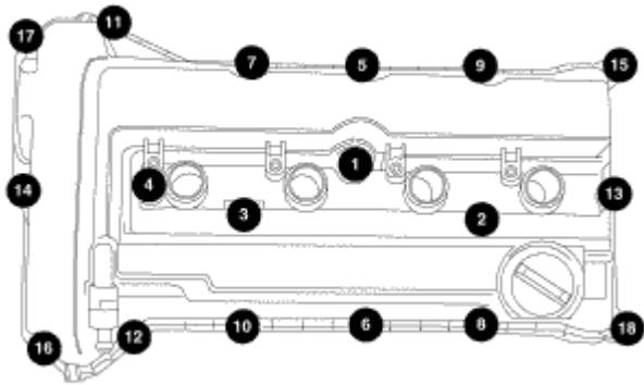
Fig. 150: Torque Sequence Courtesy of CHRYSLER LLC
