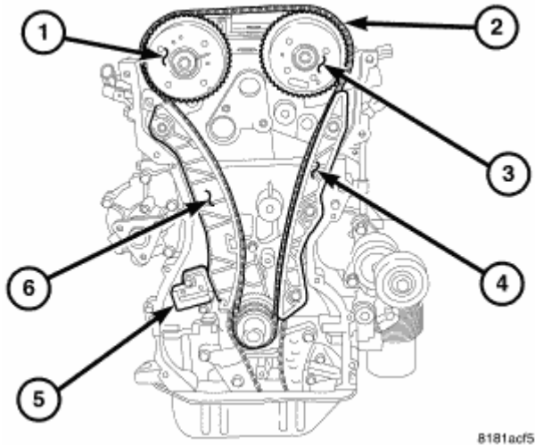
Fig. 88: Timing Drive Courtesy of CHRYSLER LLC
