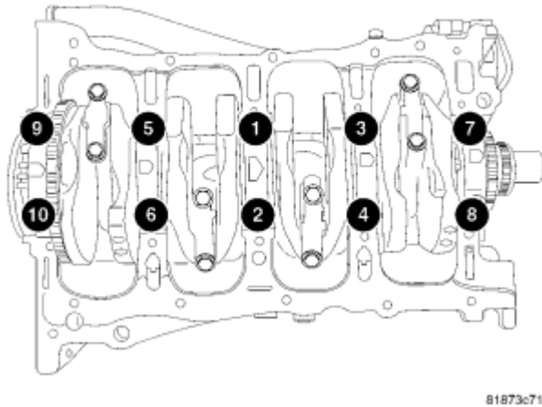
Fig. 182: Main Bearing Cap Torque Sequence Courtesy of CHRYSLER LLC
