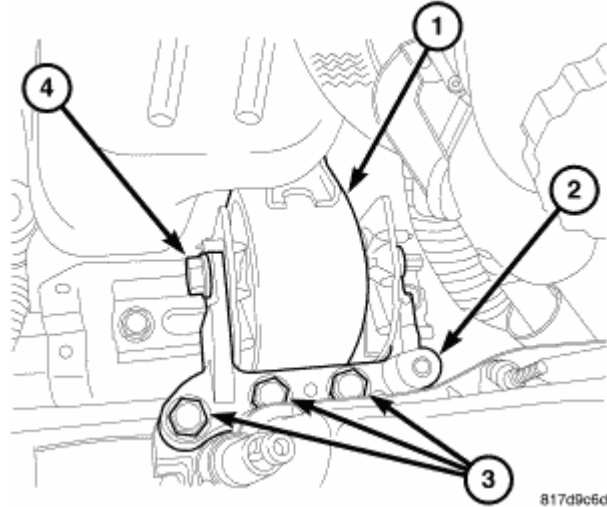
Fig. 84: Right Engine Mount Courtesy of CHRYSLER LLC
