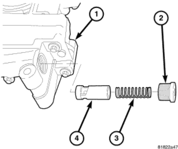
Fig. 281: View Of Pressure Regulating Valve Courtesy of CHRYSLER LLC
