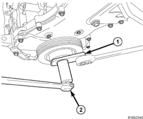
Fig. 223: Removing/Installing Damper Courtesy of CHRYSLER LLC
