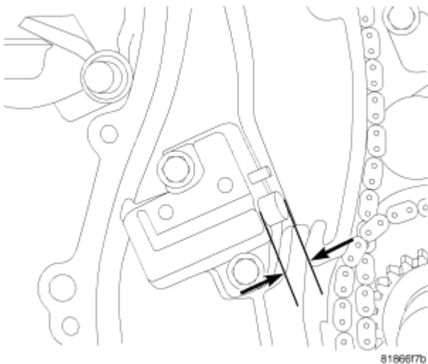
Fig. 357: Checking Timing Chain For Stretching
