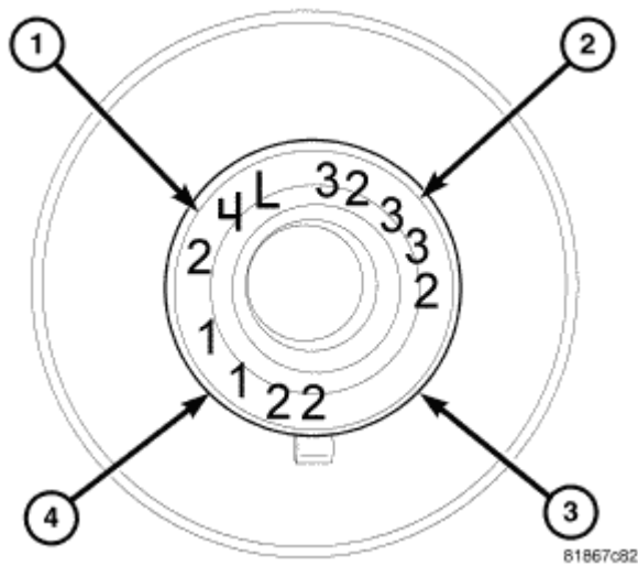
Fig. 212: Lower Main Bearing Identification Courtesy of CHRYSLER LLC
