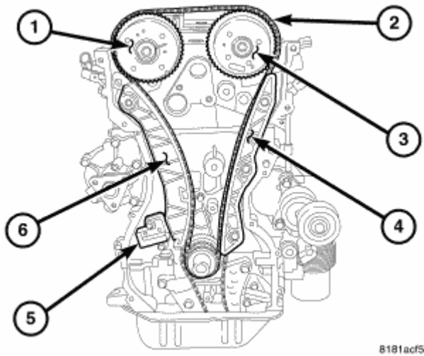
Fig. 321: TIMING DRIVE Courtesy of CHRYSLER LLC
