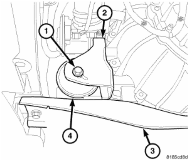
Fig. 241: FRONT MOUNT THROUGH BOLT Courtesy of CHRYSLER LLC
