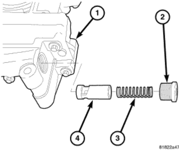
Fig. 282: View Of Pressure Regulating Valve Courtesy of CHRYSLER LLC
