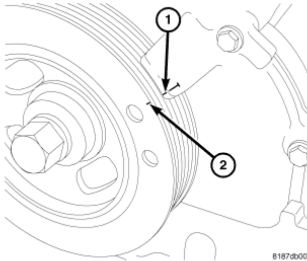
Fig. 373: TDC Courtesy of CHRYSLER LLC
