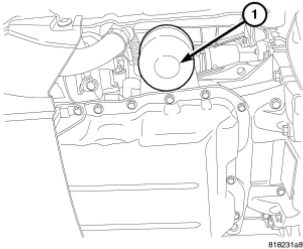
Fig. 260: Oil Filter
