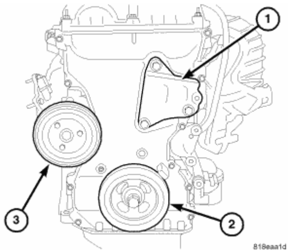
Fig. 177: Right Engine Mount Bracket
