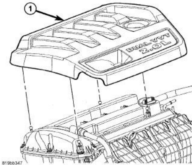
Fig. 138: Engine Cover - 2.0L
