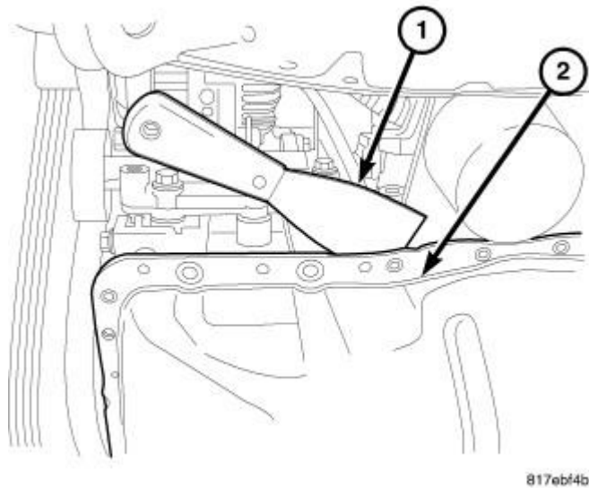
Fig. 195: Oil Pan Removal Courtesy of CHRYSLER GROUP, LLC
