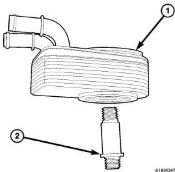
Fig. 284: Oil Cooler & Oil Cooler Connector Bolt Courtesy of CHRYSLER GROUP, LLC
