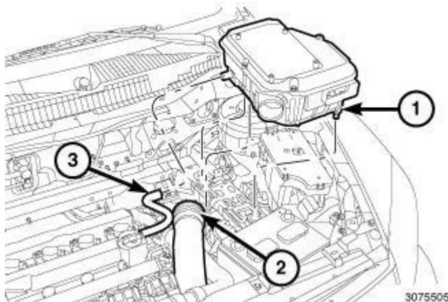
Fig. 246: Air Cleaner Body, Air Inlet Tube & Make-Up Air Hose Courtesy of CHRYSLER GROUP, LLC
