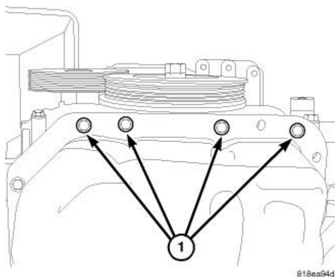
Fig. 80: Timing Chain Cover Lower Bolts Courtesy of CHRYSLER GROUP, LLC
