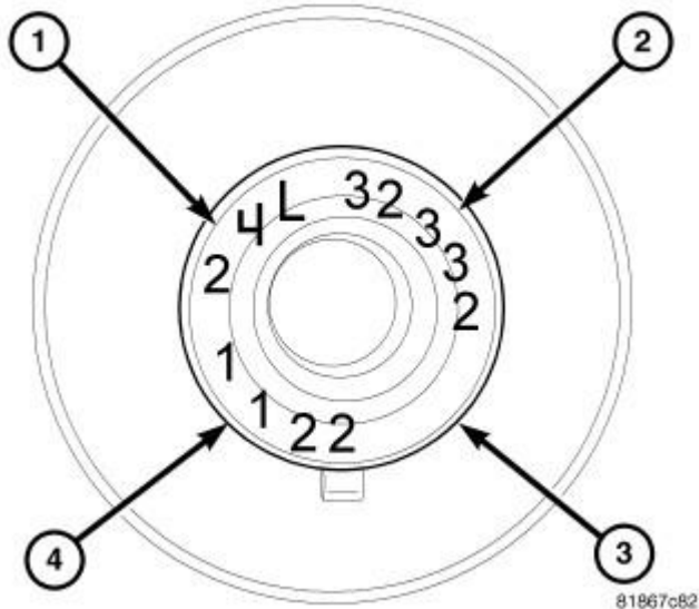
Fig. 187: Lower Main Bearing Identification Courtesy of CHRYSLER GROUP, LLC
