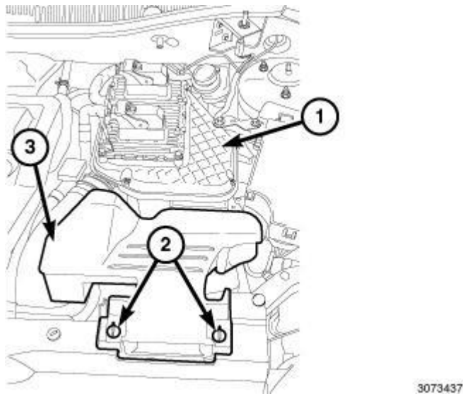
Fig. 346: Retainers, Fresh Air Inlet Duct & Air Cleaner Body Courtesy of CHRYSLER GROUP, LLC
