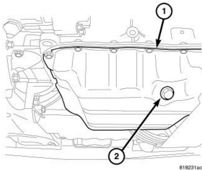
Fig. 289: Oil Drain Plug & Oil Pan
