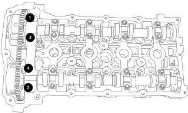
Fig. 96: Front Cam Cap Removal/Tightening Sequence Courtesy of CHRYSLER GROUP, LLC
