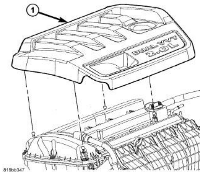
Fig. 347: Engine Cover - 2.0L Courtesy of CHRYSLER GROUP, LLC
