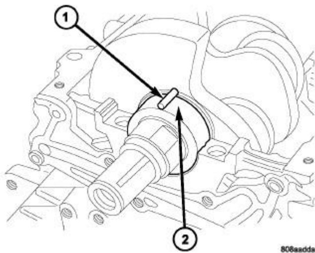
Fig. 6: Plastigage Placed In Lower Shell Courtesy of CHRYSLER GROUP, LLC
