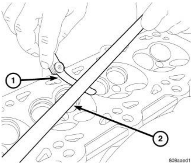
Fig. 98: Checking Cylinder Head Flatness Courtesy of CHRYSLER GROUP, LLC
