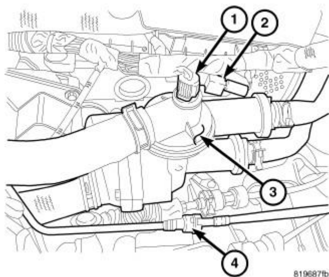
Fig. 14: Coolant Temperature Sensor, Capacitor Electrical Connector & Coolant Adapter Courtesy of CHRYSLER GROUP, LLC
