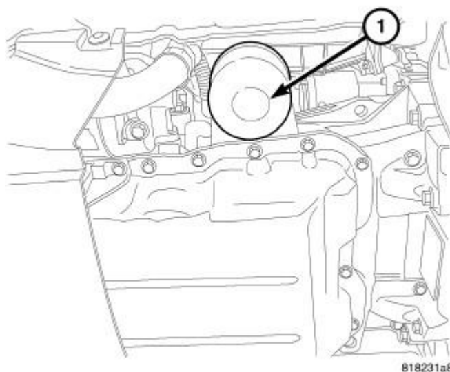
Fig. 211: Oil Filter
