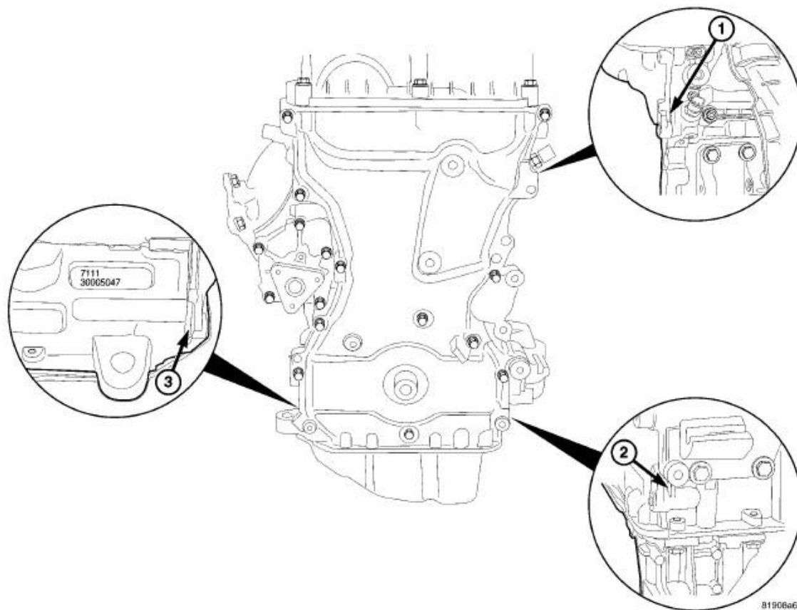
Fig. 85: Timing Chain Cover Pry Points Courtesy of CHRYSLER GROUP, LLC
