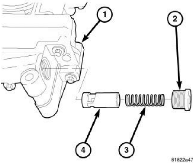
Fig. 318: Oil Pressure Relief Valve Courtesy of CHRYSLER GROUP, LLC
