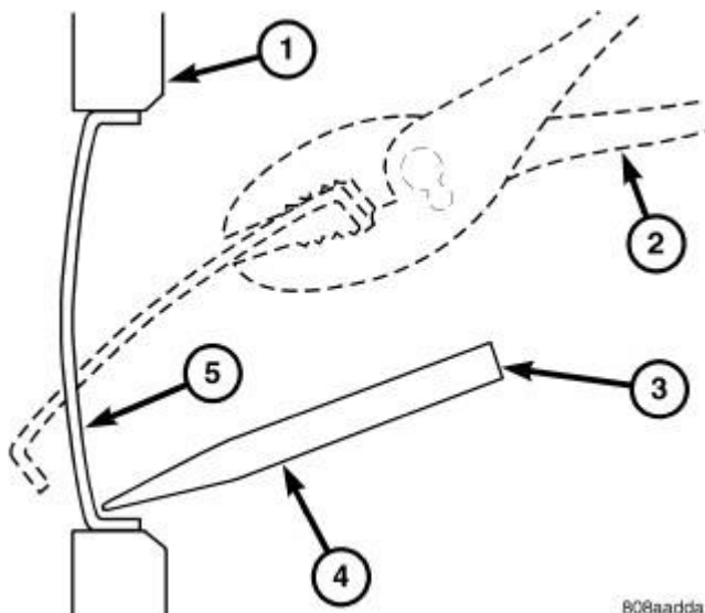
Fig. 5: Core Hole Plug Removal Courtesy of CHRYSLER GROUP, LLC
