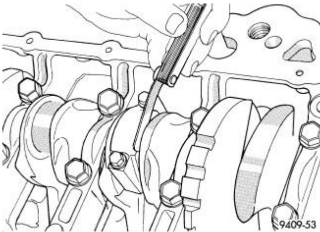
Fig. 231: Connecting Rod Side Clearance Courtesy of CHRYSLER GROUP, LLC
