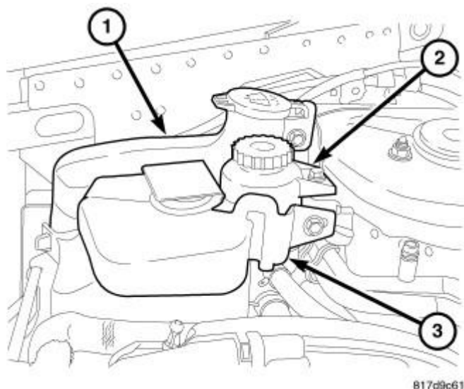
Fig. 72: Windshield Washer Reservoir, Power Steering Reservoir & Coolant Reservoir Courtesy of CHRYSLER GROUP, LLC
