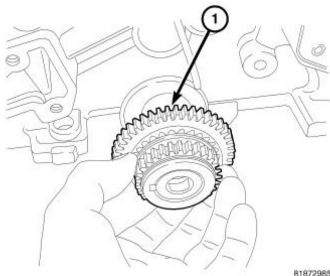
Fig. 196: Crankshaft Sprocket Courtesy of CHRYSLER GROUP, LLC
