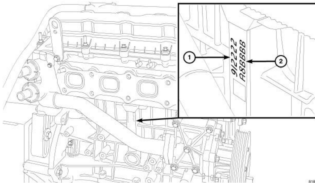
Fig. 188: Upper Main Bearing Shell Identification Courtesy of CHRYSLER GROUP, LLC
