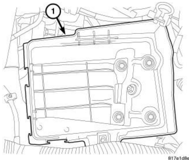
Fig. 12: Battery Tray Courtesy of CHRYSLER GROUP, LLC
