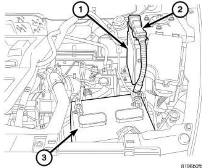
Fig. 329: Negative Battery Cable & Battery Courtesy of CHRYSLER GROUP, LLC
