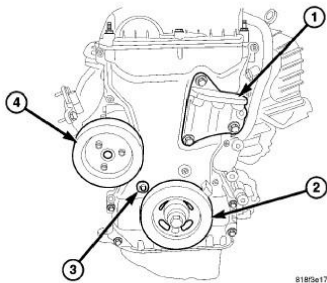
Fig. 374: Right Side Engine Mount Bracket, Crankshaft Damper & Water Pump Pulley Courtesy of CHRYSLER GROUP, LLC
