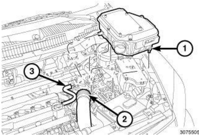
Fig. 344: Air Cleaner Body, Air Inlet Tube & Make-Up Air Hose Courtesy of CHRYSLER GROUP, LLC
