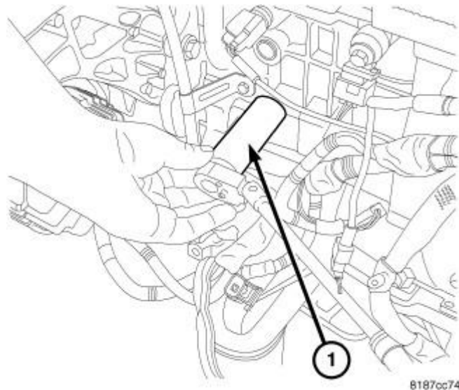
Fig. 315: Remove/Install Oil Pressure Switch Courtesy of CHRYSLER GROUP, LLC
