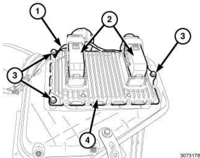
Fig. 52: Electrical Connectors, PCM, Three Mounting Bolts & Ground Wire Courtesy of CHRYSLER GROUP, LLC
