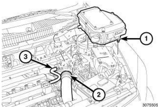
Fig. 333: Air Cleaner Body, Air Inlet Tube & Make-Up Air Hose Courtesy of CHRYSLER GROUP, LLC
