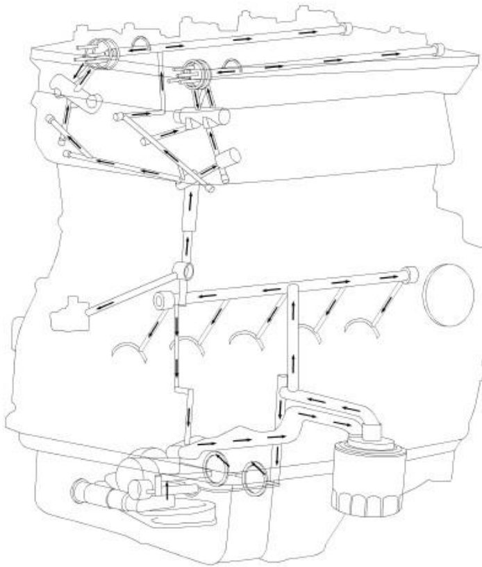
Fig. 260: Oil Flow Diagram
