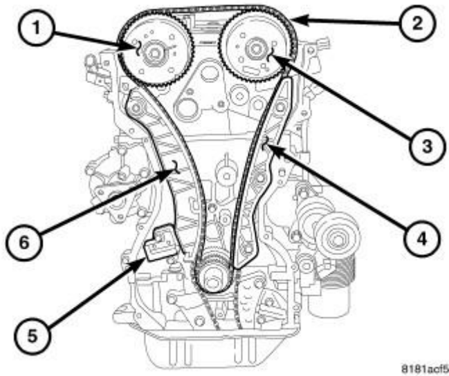
Fig. 348: Timing Drive System
