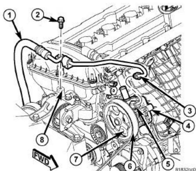
Fig. 73: Power Steering Assembly Components Courtesy of CHRYSLER GROUP, LLC
