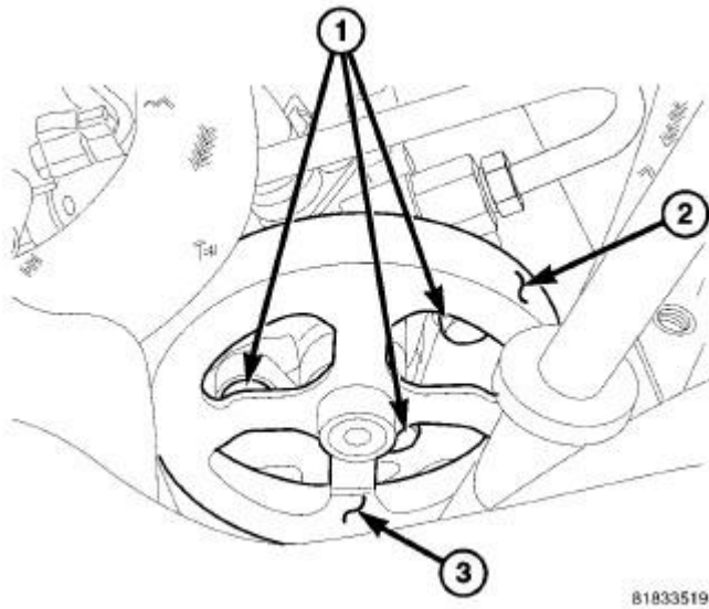
Fig. 369: Power Steering Pump Bolts & Pulley Courtesy of CHRYSLER GROUP, LLC
