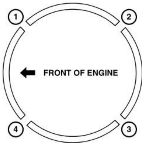
Fig. 224: Piston Ring End Gap Position Courtesy of CHRYSLER GROUP, LLC
