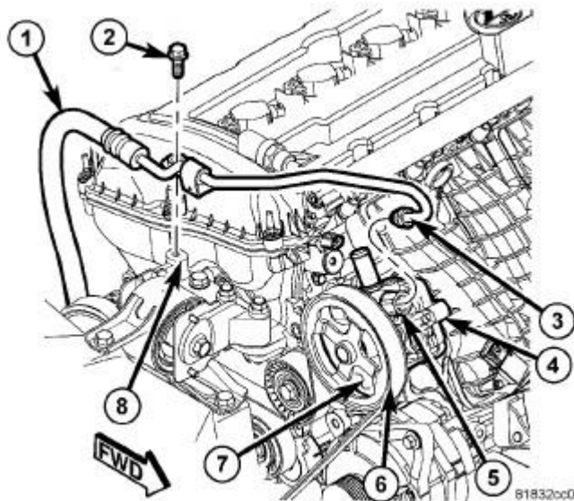
Fig. 368: Power Steering Assembly Components Courtesy of CHRYSLER GROUP, LLC
