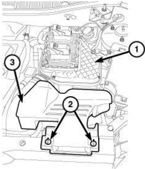
Fig. 9: Retainers, Fresh Air Inlet Duct & Air Cleaner Body Courtesy of CHRYSLER GROUP, LLC
