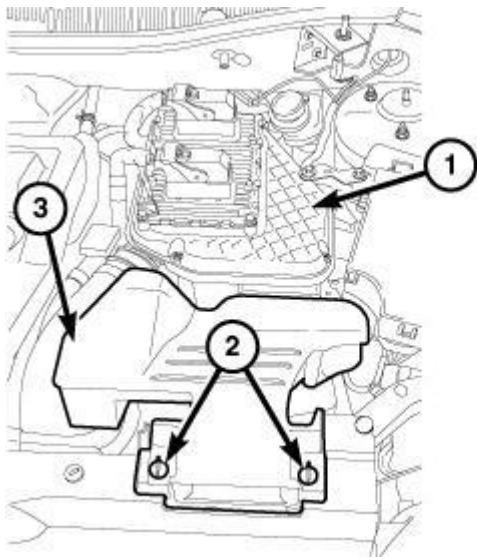
Fig. 62: Retainers, Fresh Air Inlet Duct & Air Cleaner Body Courtesy of CHRYSLER GROUP, LLC
