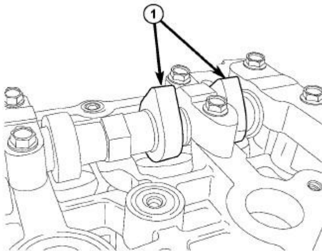
Fig. 129: Identifying Camshaft So Lobes Are Vertical Courtesy of CHRYSLER GROUP, LLC
