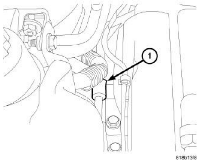
Fig. 255: Power Steering Line Support Bracket Courtesy of CHRYSLER GROUP, LLC
