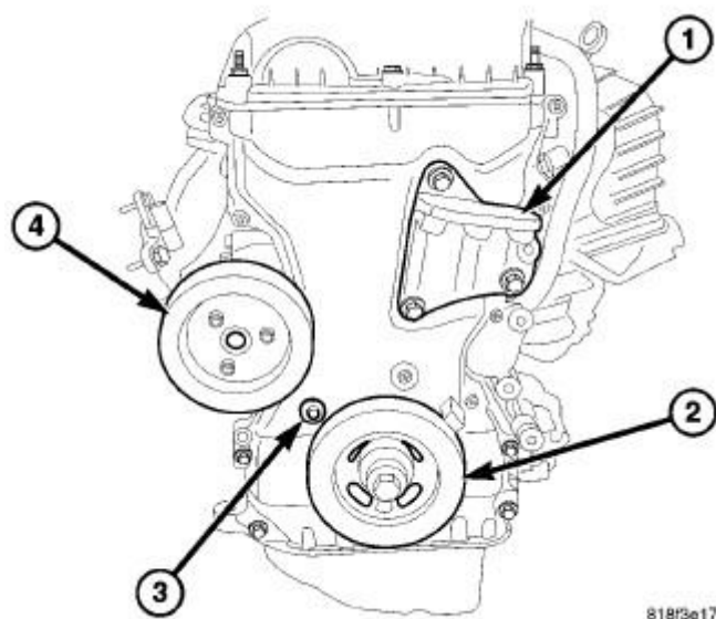
Fig. 378: Right Side Engine Mount Bracket, Crankshaft Damper & Water Pump Pulley Courtesy of CHRYSLER GROUP, LLC
