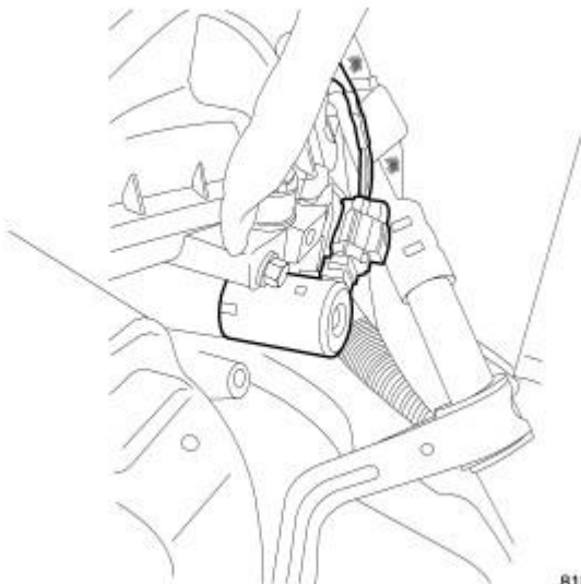
Fig. 282: Solenoid Location 1/2 Courtesy of CHRYSLER GROUP, LLC
