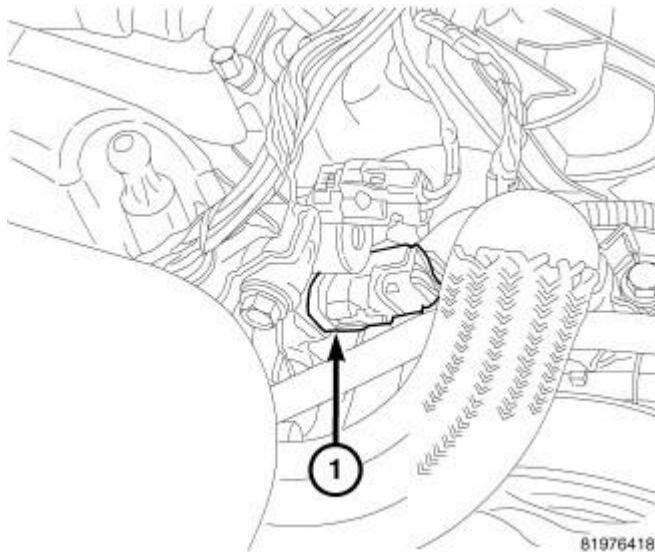
Fig. 342: Oil Temperature Sensor Courtesy of CHRYSLER GROUP, LLC
