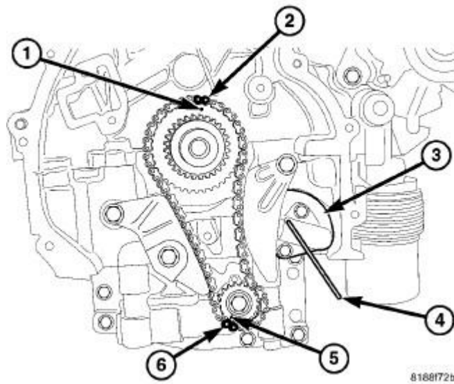
Fig. 306: Oil Pump Drive Chain, Oil Pump Drive Chain Tensioner & Timing Marks On Chain Courtesy of CHRYSLER GROUP, LLC
