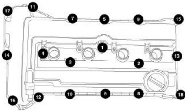
Fig. 115: Removing/Installing Cylinder Head Cover Bolts In Sequence Courtesy of CHRYSLER GROUP, LLC
