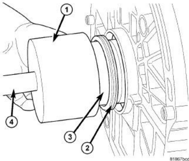
Fig. 240: Rear Main Seal Installation Courtesy of CHRYSLER GROUP, LLC
