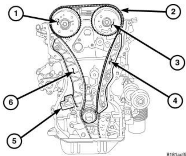
Fig. 364: Timing Drive System
