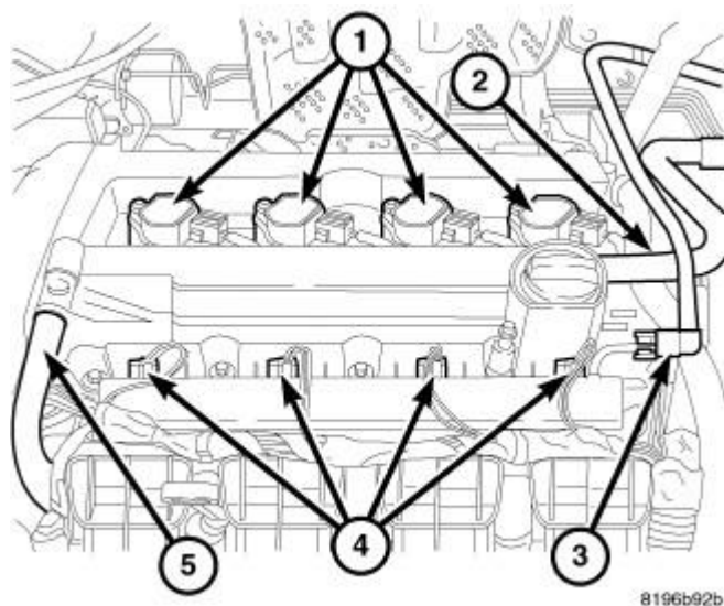
Fig. 46: Ignition Coils, Air Hose, Fuel Line, Injectors & PCV Hose Courtesy of CHRYSLER GROUP, LLC
