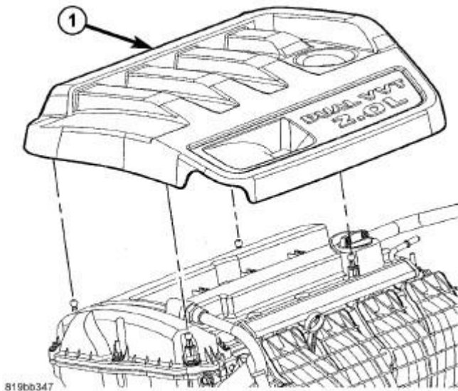
Fig. 29: Engine Cover - 2.0L Courtesy of CHRYSLER GROUP, LLC
