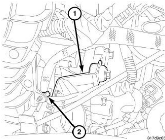
Fig. 17: Throttle Body Support Bracket & Wiring Harness Courtesy of CHRYSLER GROUP, LLC
