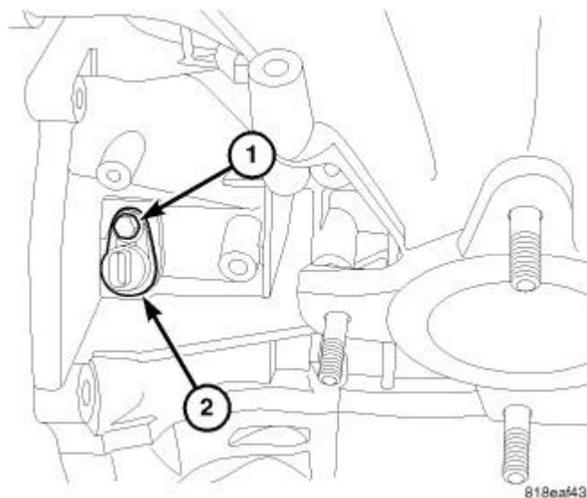
Fig. 197: Crankshaft Position Sensor & Bolt Courtesy of CHRYSLER GROUP, LLC
