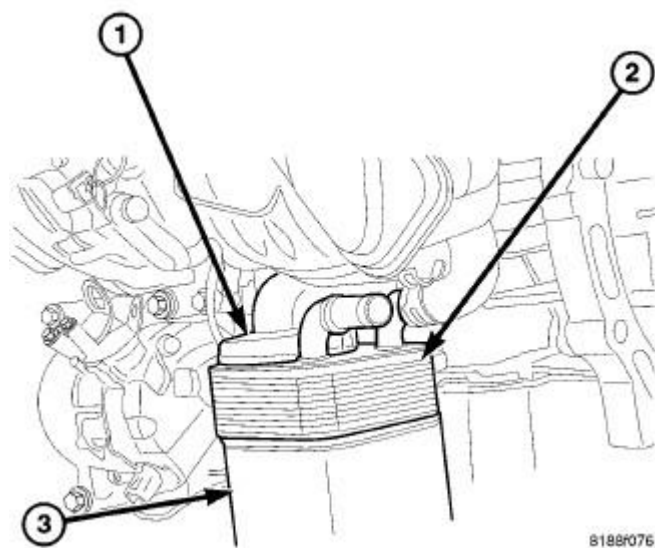
Fig. 39: Oil Cooler Adapter, Oil Cooler & Oil Filter Courtesy of CHRYSLER GROUP, LLC
