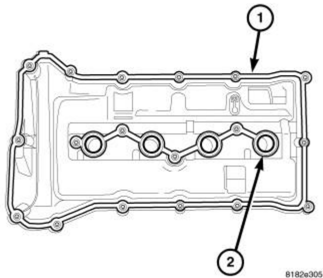
Fig. 160: Cylinder Head Cover Gaskets Location Courtesy of CHRYSLER GROUP, LLC
