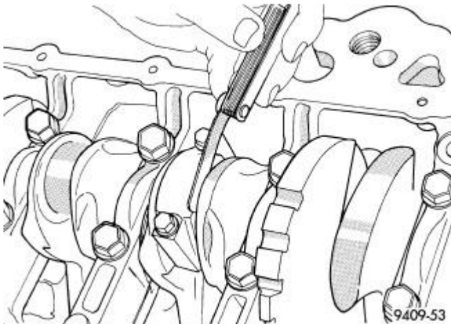
Fig. 186: Checking Connecting Rod Side Clearance Using Feeler Gauge Courtesy of CHRYSLER GROUP, LLC
