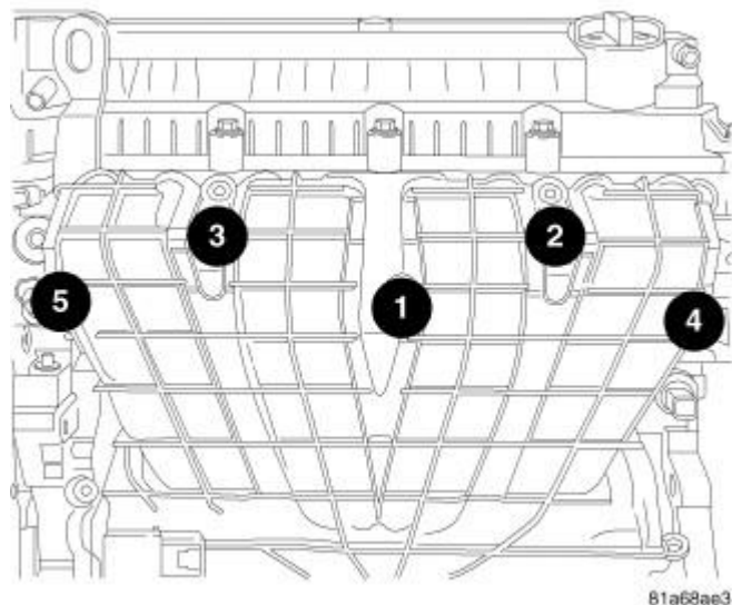
Fig. 117: Intake Manifold Bolt Removal & Tightening Sequence Courtesy of CHRYSLER GROUP, LLC
