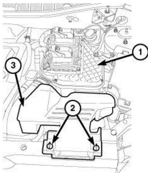
Fig. 331: Retainers, Fresh Air Inlet Duct & Air Cleaner Body
