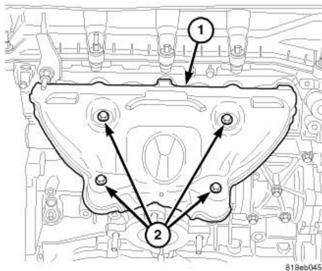
Fig. 322: Exhaust Manifold Heat Shield & Fasteners
