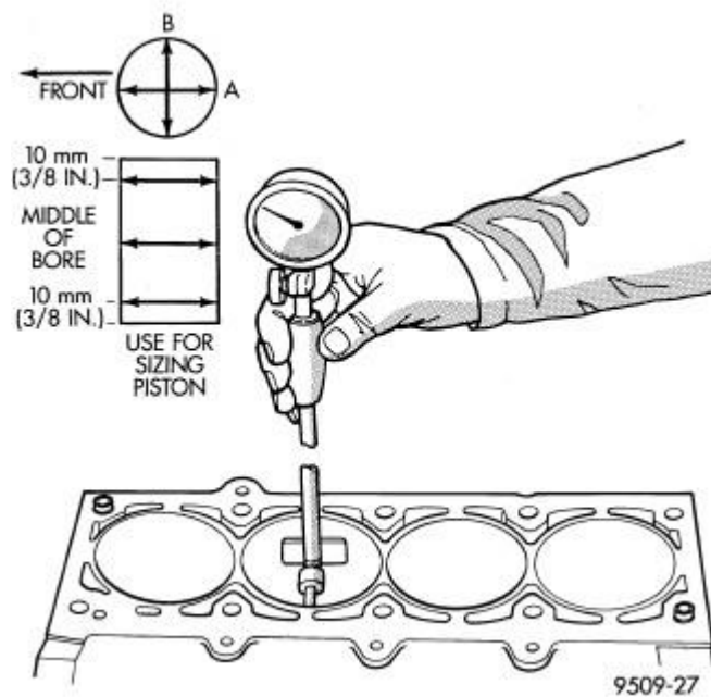
Fig. 226: Checking Cylinder Bore Size Courtesy of CHRYSLER GROUP, LLC
