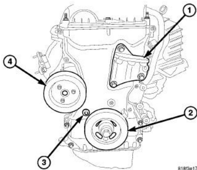
Fig. 390: Right Side Engine Mount Bracket, Crankshaft Damper & Water Pump Pulley Courtesy of CHRYSLER GROUP, LLC
