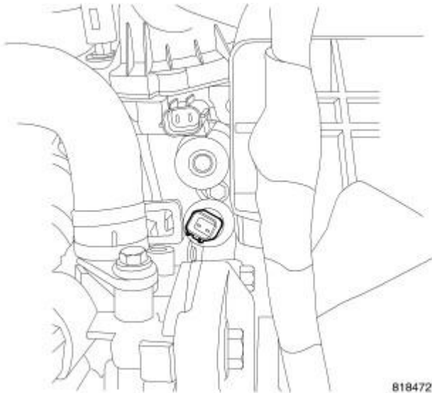
Fig. 280: Oil Pressure Sensor Courtesy of CHRYSLER GROUP, LLC
