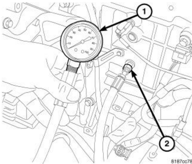
Fig. 264: Oil Pressure Gauge & Adapter Courtesy of CHRYSLER GROUP, LLC
