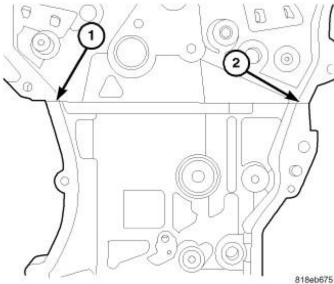
Fig. 381: Front Cover Upper T-Joints Courtesy of CHRYSLER GROUP, LLC
