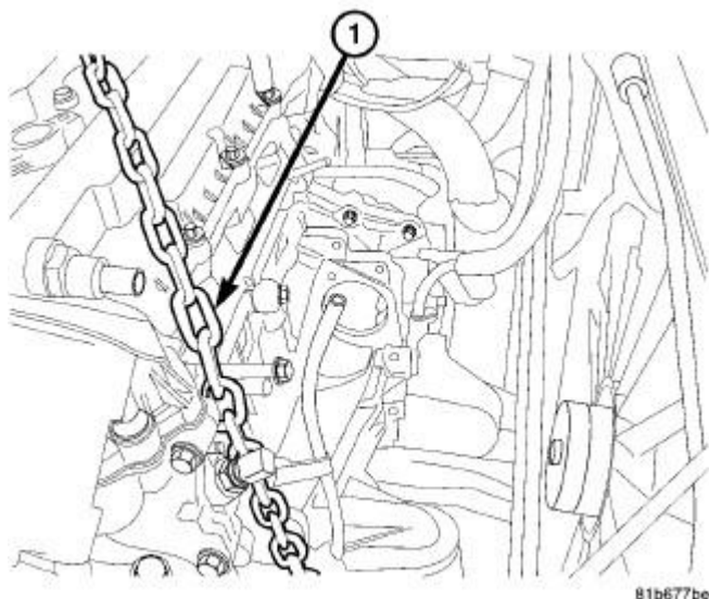
Fig. 210: Lift Chain
