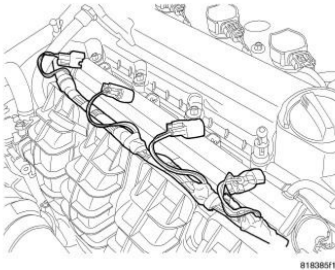
Fig. 88: Fuel Injector Electrical Connectors Courtesy of CHRYSLER GROUP, LLC
