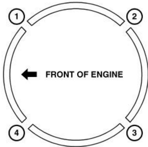
Fig. 230: Piston Ring End Gap Position Courtesy of CHRYSLER GROUP, LLC
