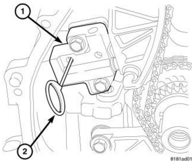
Fig. 401: Timing Chain Tensioner & Pin Courtesy of CHRYSLER GROUP, LLC
