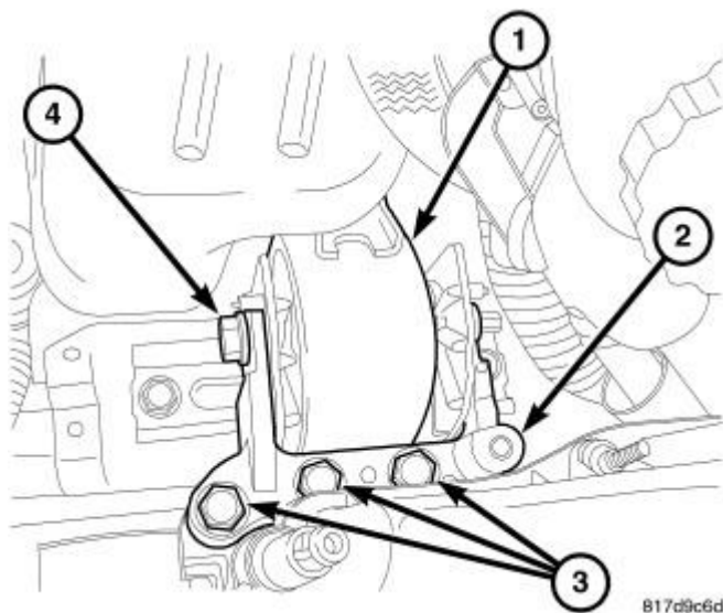
Fig. 257: Right Engine Mount Assembly Courtesy of CHRYSLER GROUP, LLC
