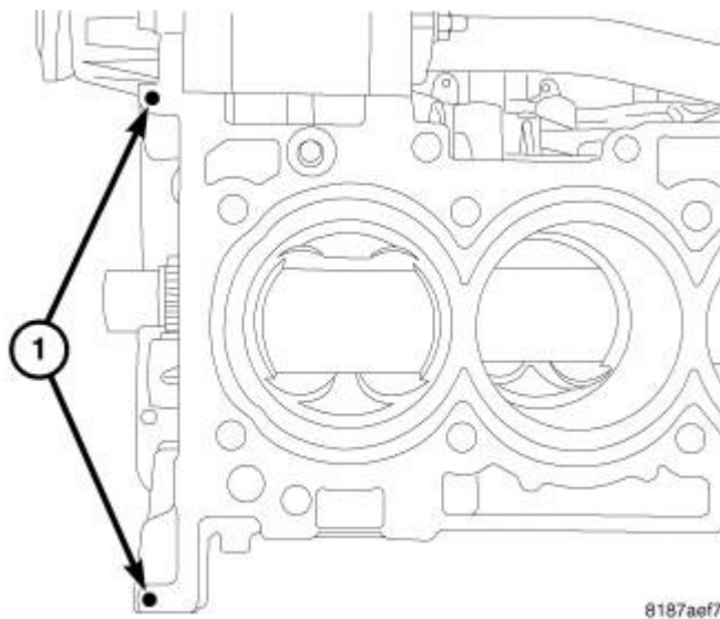
Fig. 101: Cylinder Head RTV
