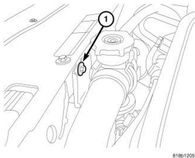
Fig. 118: Upper Radiator Hose Support Courtesy of CHRYSLER GROUP, LLC
