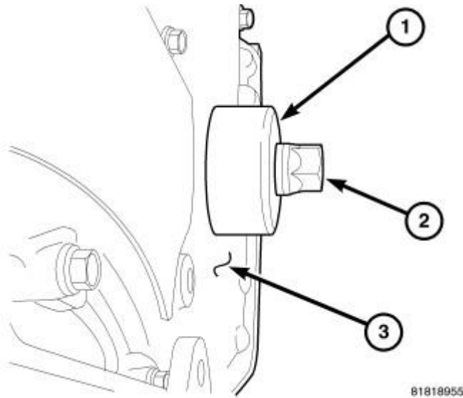
Fig. 236: Front Oil Seal Installed Courtesy of CHRYSLER GROUP, LLC
