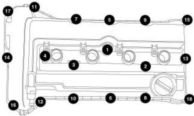
Fig. 370: Removing/Installing Cylinder Head Cover Bolts In Sequence Courtesy of CHRYSLER GROUP, LLC
