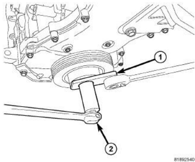
Fig. 38: Removing/Installing Damper Bolt
