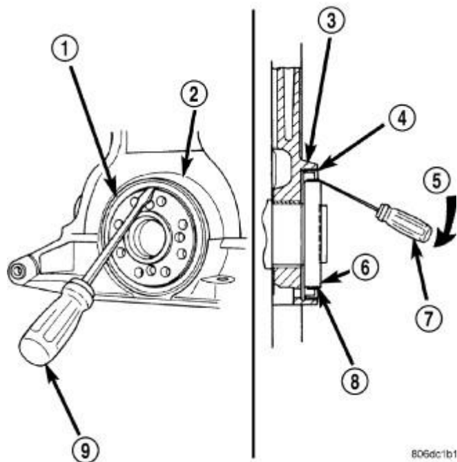
Fig. 239: Removing Rear Crankshaft Oil Seal
