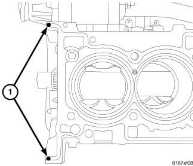
Fig. 102: Cylinder Head Gasket RTV Courtesy of CHRYSLER GROUP, LLC
