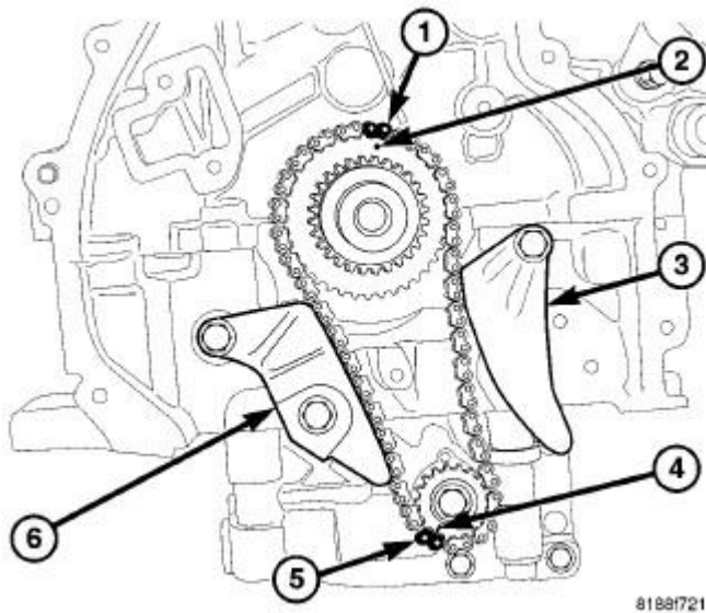
Fig. 309: Aligning Timing Marks On Components Courtesy of CHRYSLER GROUP, LLC
