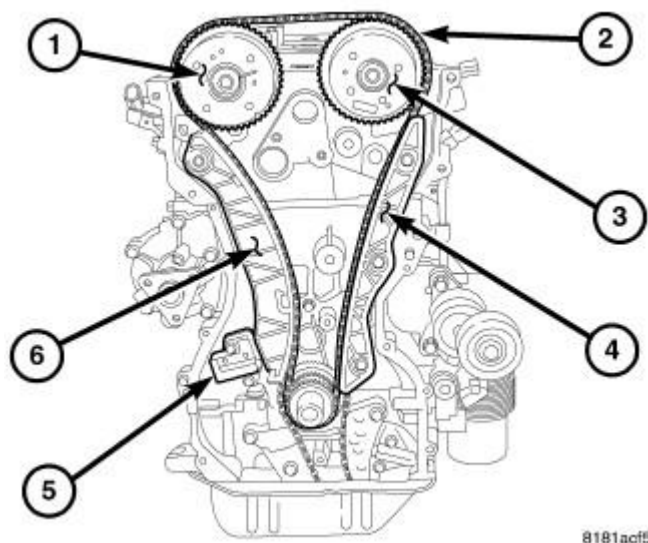
Fig. 86: Timing Drive System Courtesy of CHRYSLER GROUP, LLC
