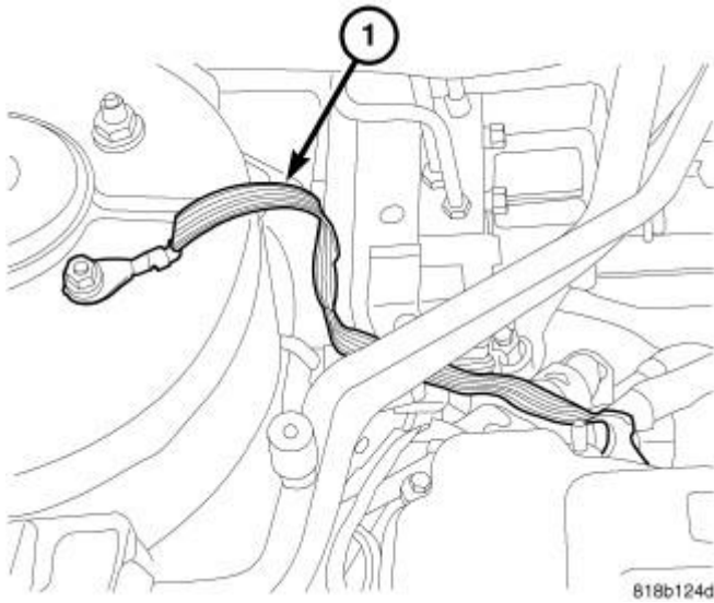
Fig. 41: Ground Strap Courtesy of CHRYSLER GROUP, LLC
