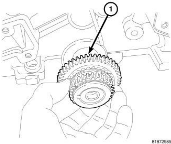
Fig. 354: Crankshaft Sprocket Courtesy of CHRYSLER GROUP, LLC
