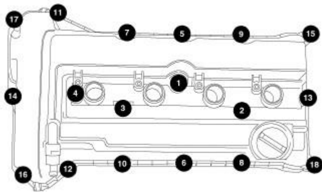
Fig. 393: Removing/Installing Cylinder Head Cover Bolts In Sequence Courtesy of CHRYSLER GROUP, LLC
