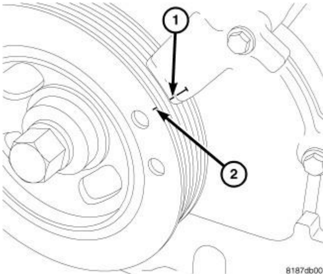
Fig. 303: TDC Courtesy of CHRYSLER GROUP, LLC
