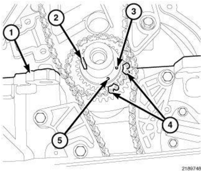
Fig. 351: Crankshaft Timing Marks Courtesy of CHRYSLER GROUP, LLC
