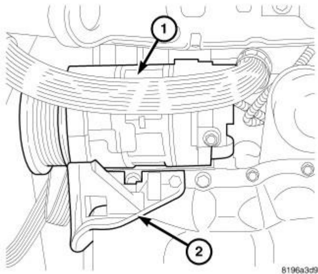
Fig. 77: A/C Compressor & Mounting Bracket
