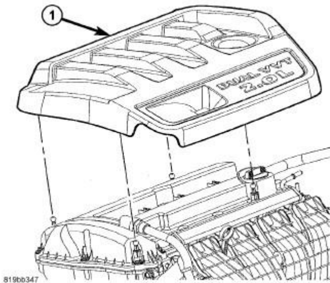
Fig. 68: Engine Cover - 2.0L
