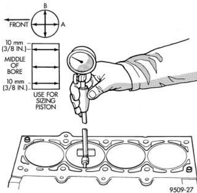
Fig. 183: Checking Cylinder Bore Size Courtesy of CHRYSLER GROUP, LLC
