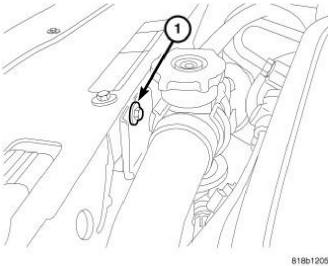
Fig. 337: Upper Radiator Hose Support Courtesy of CHRYSLER GROUP, LLC
