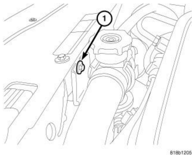
Fig. 340: Upper Radiator Hose Support Courtesy of CHRYSLER GROUP, LLC
