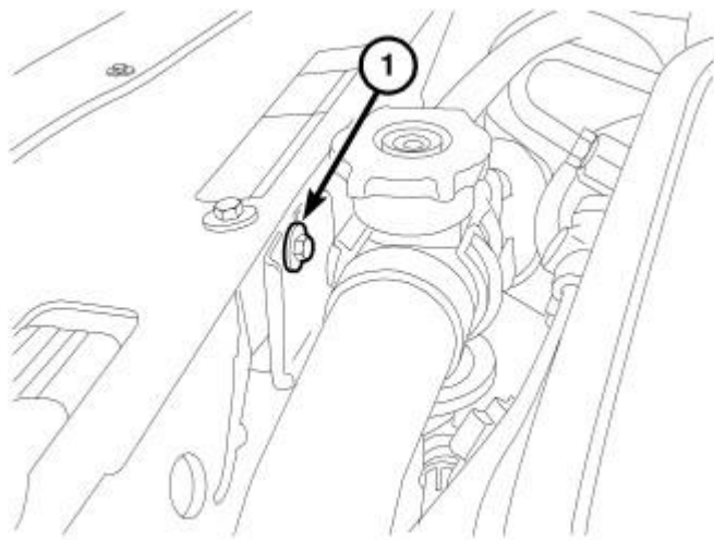
Fig. 47: Upper Radiator Hose Support Courtesy of CHRYSLER GROUP, LLC
