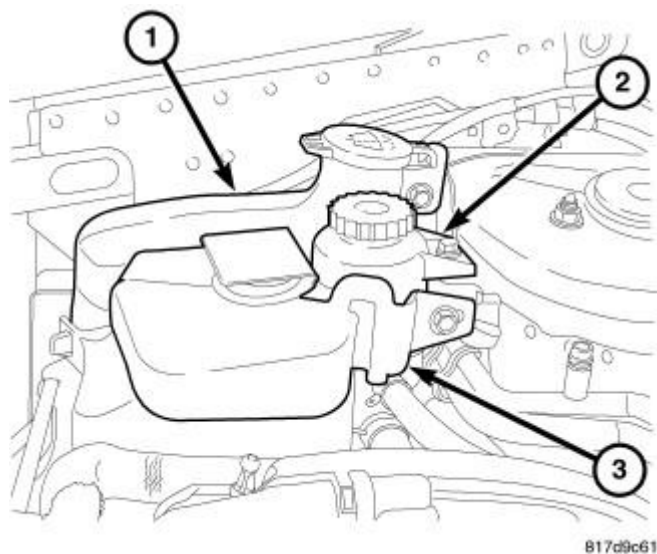
Fig. 13: Windshield Washer Reservoir, Power Steering Reservoir & Coolant Reservoir Courtesy of CHRYSLER GROUP, LLC
