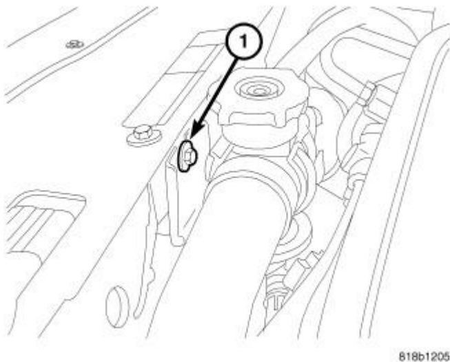
Fig. 92: Upper Radiator Hose Support Courtesy of CHRYSLER GROUP, LLC
