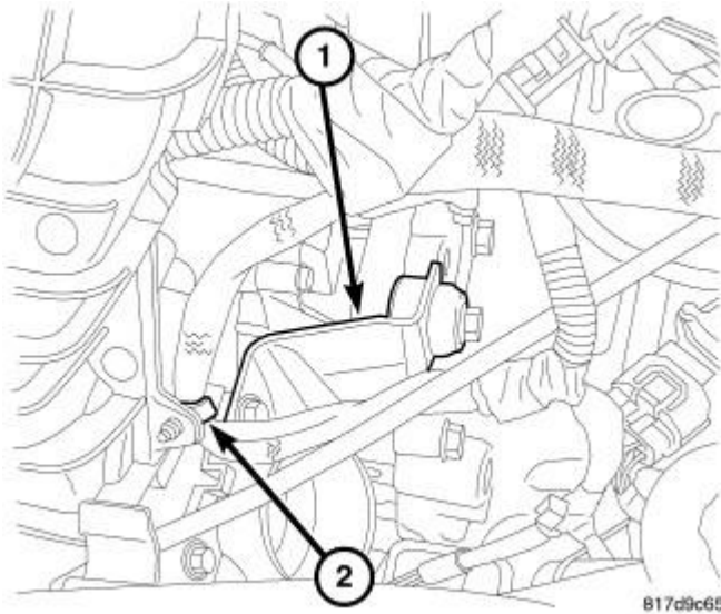
Fig. 336: Throttle Body Support Bracket & Wiring Harness Courtesy of CHRYSLER GROUP, LLC
