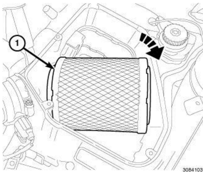
Fig. 59: Air Cleaner Element Courtesy of CHRYSLER GROUP, LLC
