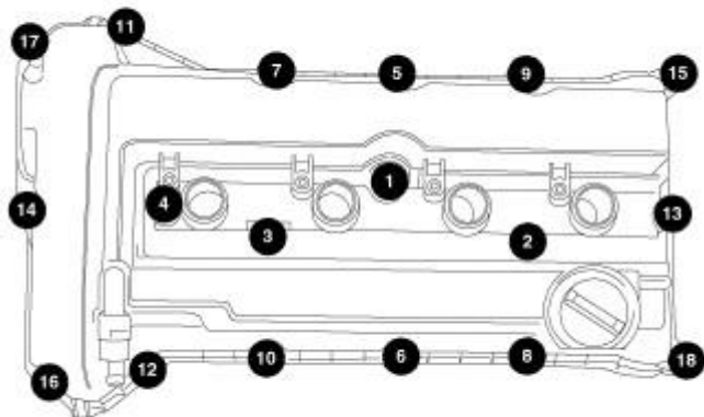
Fig. 132: Removing/Installing Cylinder Head Cover Bolts In Sequence
