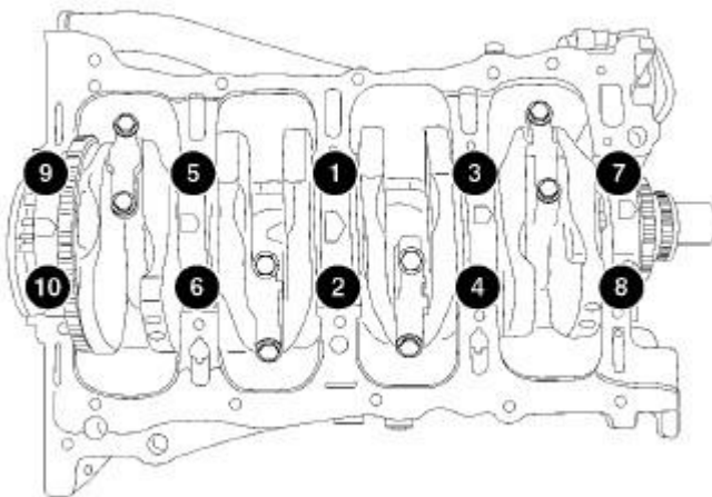
Fig. 206: Main Bearing Cap Removal/Tightening Sequence Courtesy of CHRYSLER GROUP, LLC
