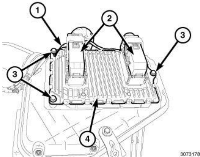
Fig. 66: Electrical Connectors, PCM, Three Mounting Bolts & Ground Wire Courtesy of CHRYSLER GROUP, LLC
