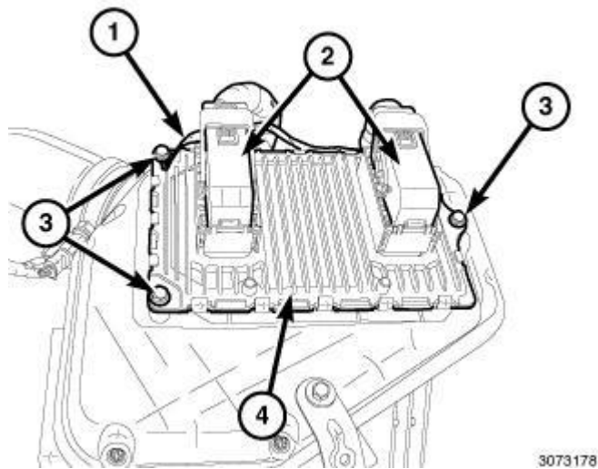
Fig. 70: Electrical Connectors, PCM, Three Mounting Bolts & Ground Wire Courtesy of CHRYSLER GROUP, LLC
