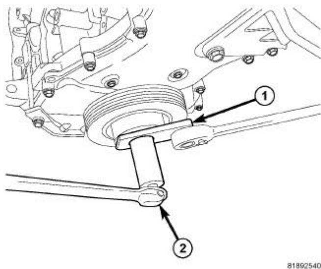
Fig. 213: Damper Removal & Installation Courtesy of CHRYSLER GROUP, LLC
