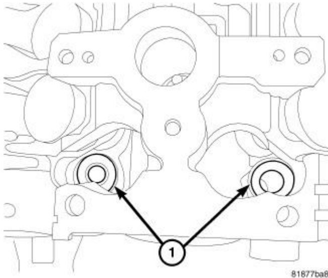
Fig. 97: Front Head Bolt Washers Courtesy of CHRYSLER GROUP, LLC
