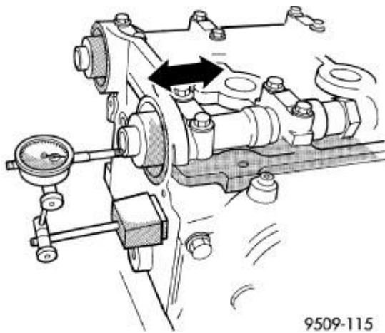
Fig. 137: Measuring Camshaft End Play Courtesy of CHRYSLER GROUP, LLC
