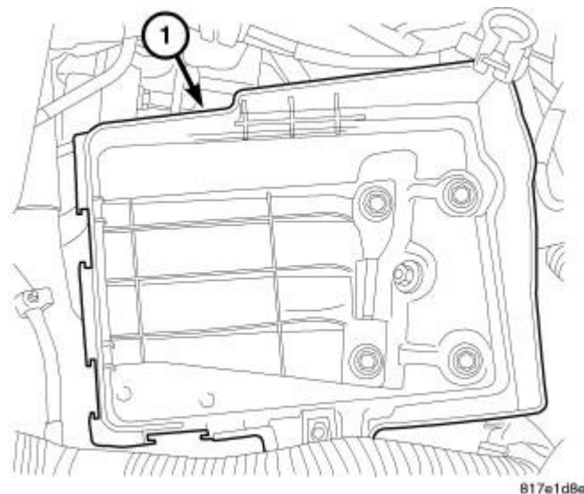
Fig. 50: Battery Tray Courtesy of CHRYSLER GROUP, LLC
