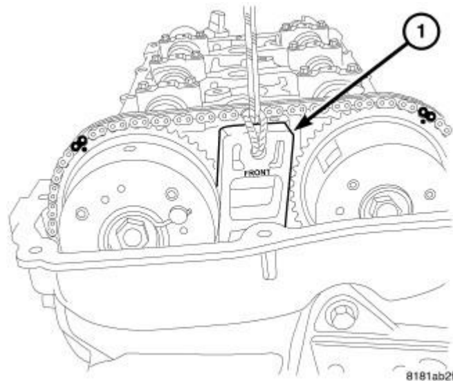
Fig. 157: Wedge 9701 Between Camshaft Phasers Courtesy of CHRYSLER GROUP, LLC
