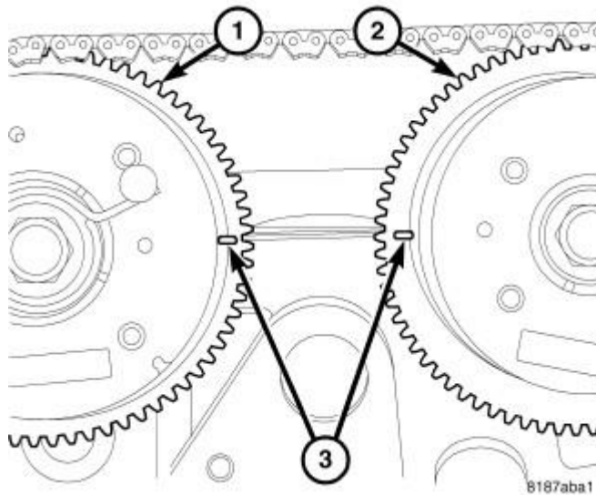
Fig. 111: Camshaft Timing Marks Courtesy of CHRYSLER GROUP, LLC
