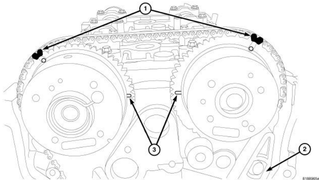
Fig. 156: Timing Chain Timing Marks Courtesy of CHRYSLER GROUP, LLC
