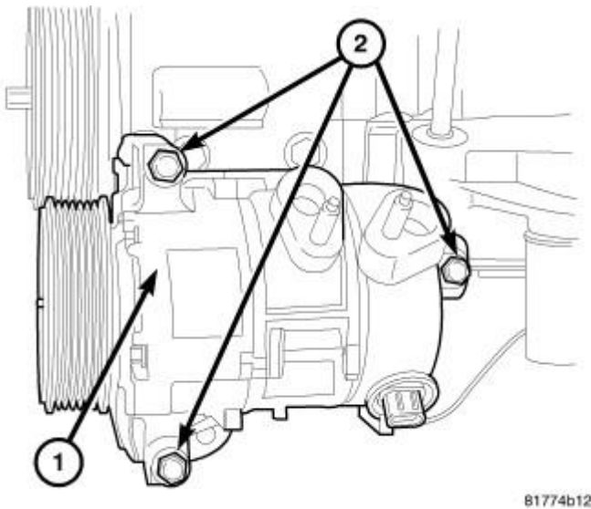
Fig. 314: A/C Compressor & Fasteners Courtesy of CHRYSLER GROUP, LLC
