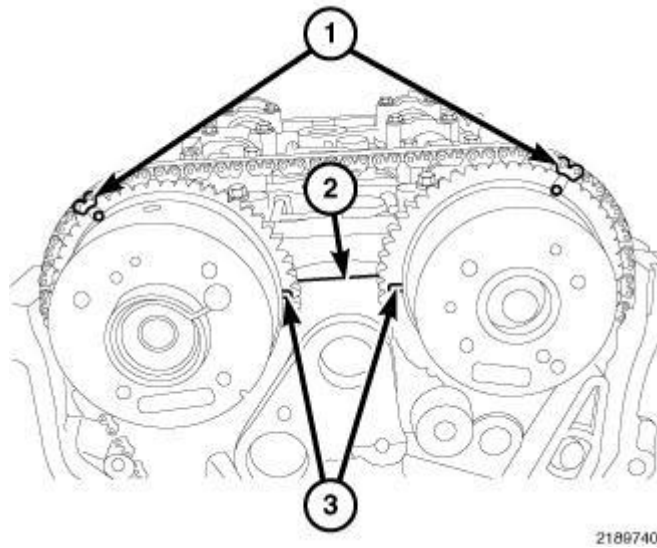
Fig. 153: Timing Chain Timing Marks Courtesy of CHRYSLER GROUP, LLC
