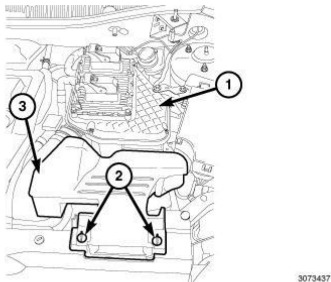
Fig. 124: Retainers, Fresh Air Inlet Duct & Air Cleaner Body Courtesy of CHRYSLER GROUP, LLC
