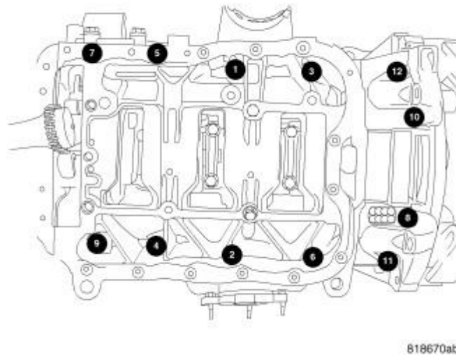
Fig. 219: Ladder Frame Bolts Tightening Sequence Courtesy of CHRYSLER GROUP, LLC
