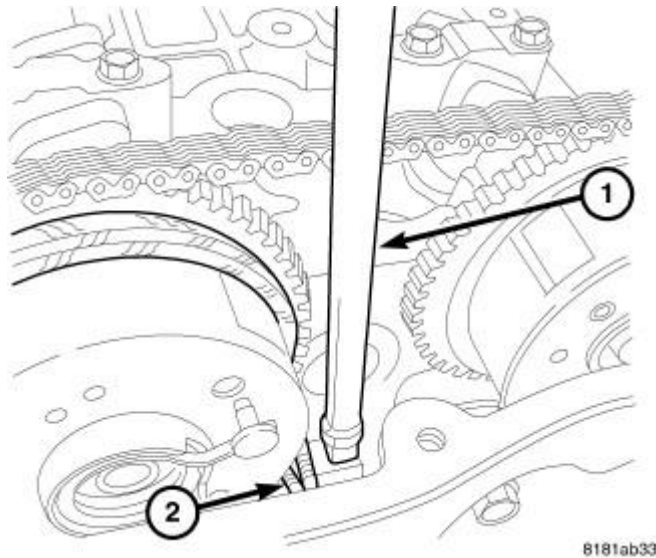
Fig. 144: Seating Wedge Tool 9701 Courtesy of CHRYSLER GROUP, LLC
