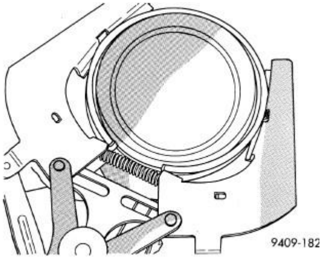
Fig. 222: Piston Rings - Removing & Installing Courtesy of CHRYSLER GROUP, LLC
