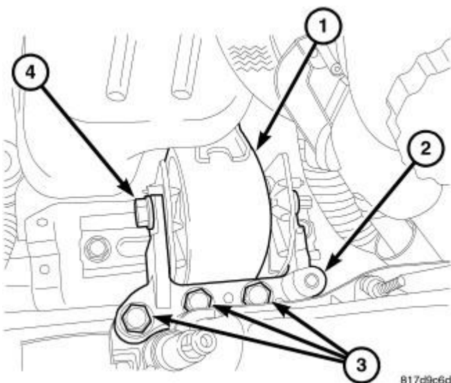
Fig. 30: Right Engine Mount Assembly
