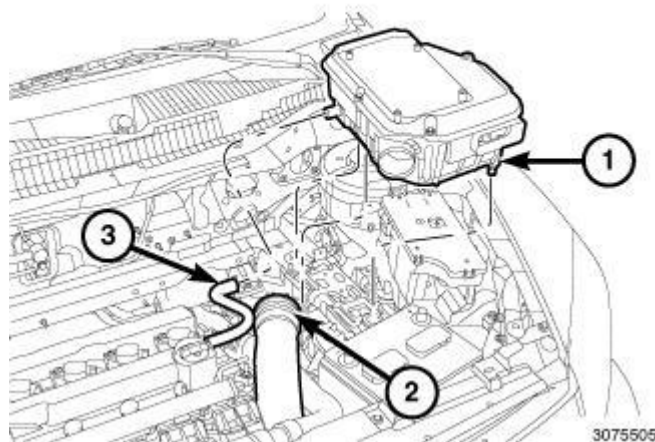
Fig. 122: Air Cleaner Body, Air Inlet Tube & Make-Up Air Hose Courtesy of CHRYSLER GROUP, LLC
