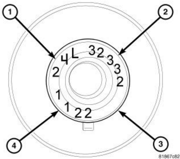
Fig. 184: Connecting Rod Bearing Identification Courtesy of CHRYSLER GROUP, LLC
