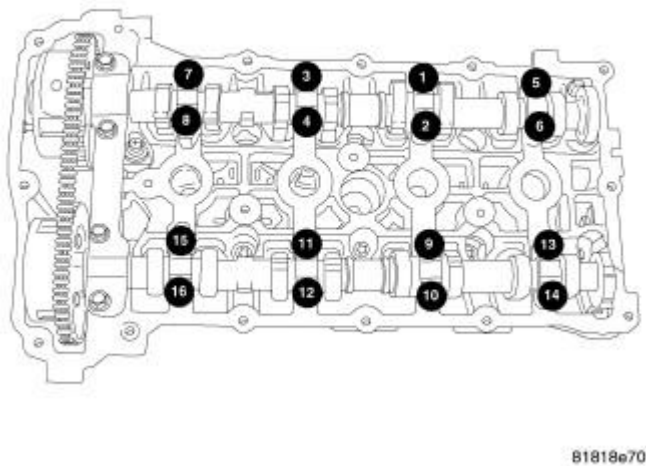
Fig. 112: Camshaft Cap Torque Sequence
