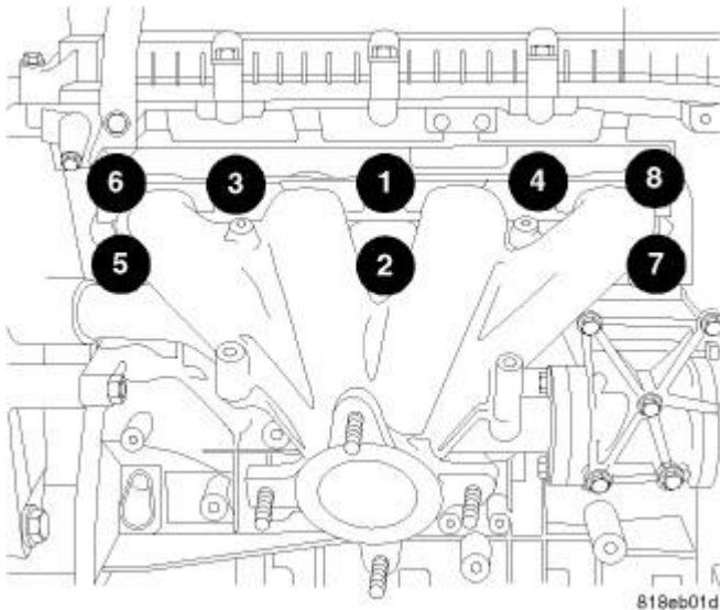
Fig. 325: Exhaust Manifold Retaining Fasteners Removal/Tightening Sequence Courtesy of CHRYSLER GROUP, LLC
