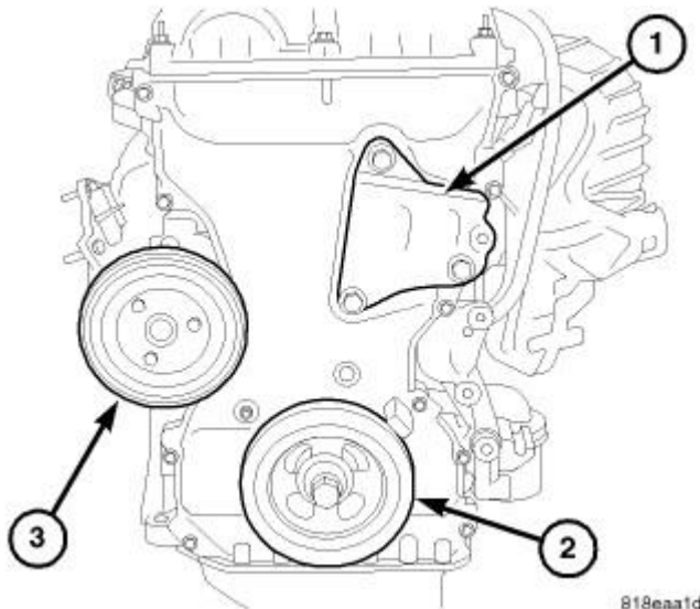
Fig. 209: Right Side Engine Mount Bracket, Crankshaft Damper & Water Pump Pulley Courtesy of CHRYSLER GROUP, LLC
