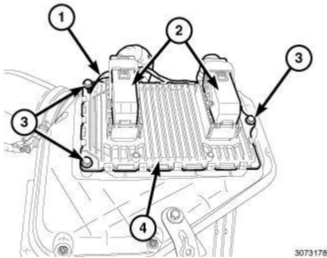
Fig. 250: Electrical Connectors, PCM, Three Mounting Bolts & Ground Wire Courtesy of CHRYSLER GROUP, LLC
