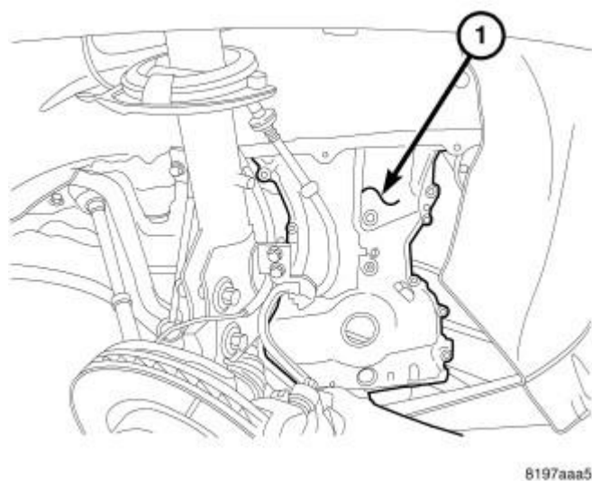
Fig. 380: Removing/Installing Timing Chain Cover Courtesy of CHRYSLER GROUP, LLC
