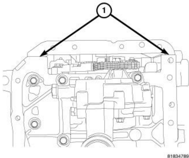
Fig. 296: Sealer Location Courtesy of CHRYSLER GROUP, LLC
