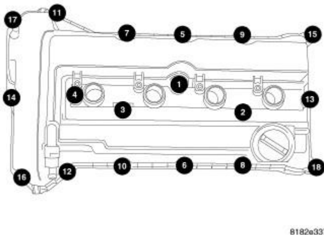
Fig. 161: Removing/Installing Cylinder Head Cover Bolts In Sequence Courtesy of CHRYSLER GROUP, LLC
