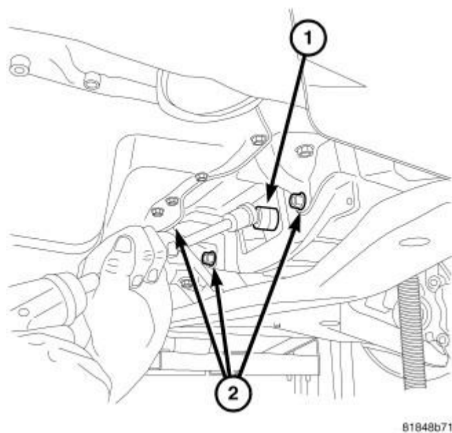
Fig. 36: Removing/Installing Torque Converter Bolts & Lower Bellhousing Bolts Courtesy of CHRYSLER GROUP, LLC
