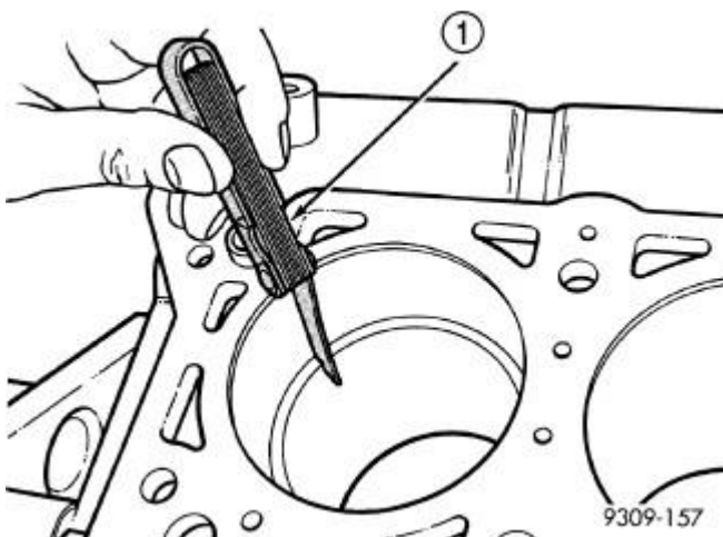
Fig. 220: Measuring Piston Ring Gap Courtesy of CHRYSLER GROUP, LLC
