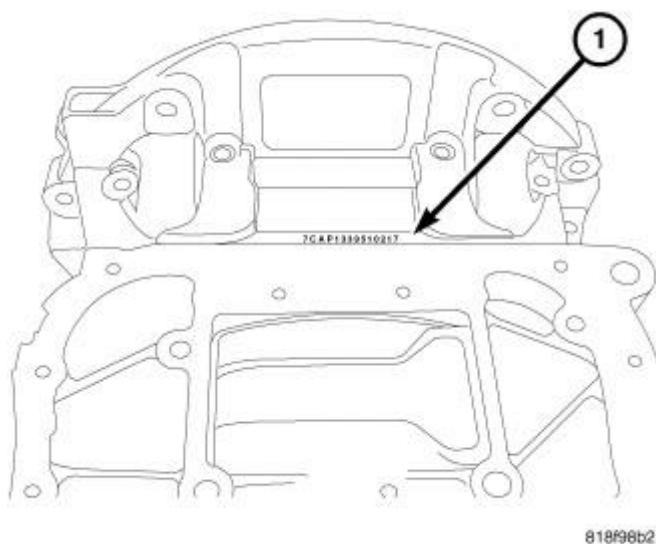
Fig. 55: Locating Engine Serial Number Courtesy of CHRYSLER GROUP, LLC
