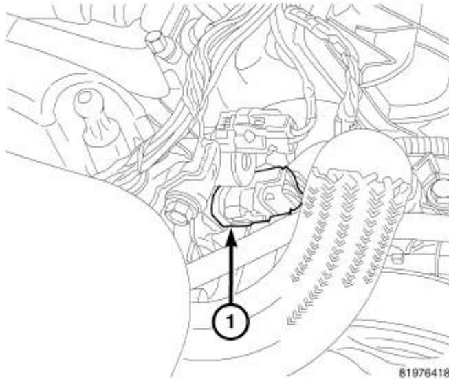
Fig. 271: Oil Temperature Sensor Courtesy of CHRYSLER GROUP, LLC
