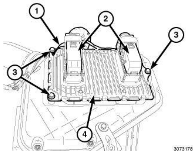
Fig. 63: Electrical Connectors, PCM, Three Mounting Bolts & Ground Wire Courtesy of CHRYSLER GROUP, LLC
