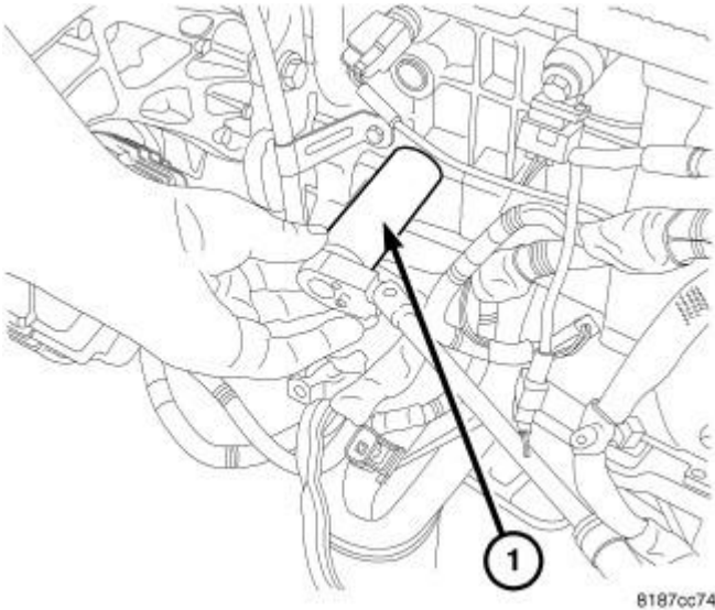
Fig. 262: Remove/Install Oil Pressure Switch Courtesy of CHRYSLER GROUP, LLC
