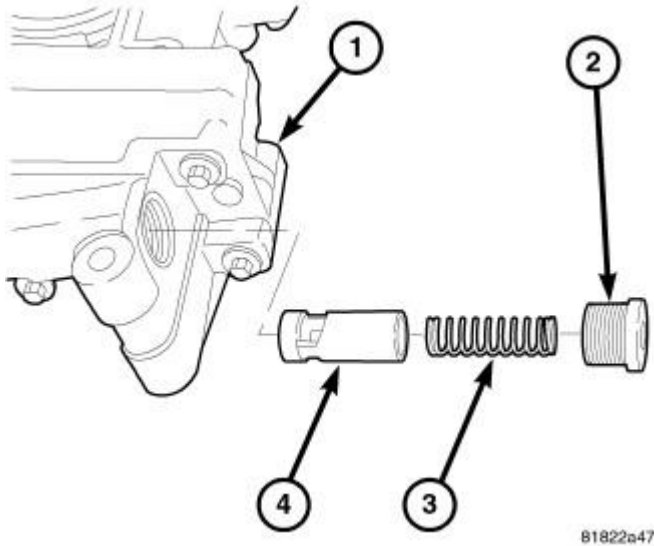
Fig. 320: Oil Pressure Relief Valve Courtesy of CHRYSLER GROUP, LLC
