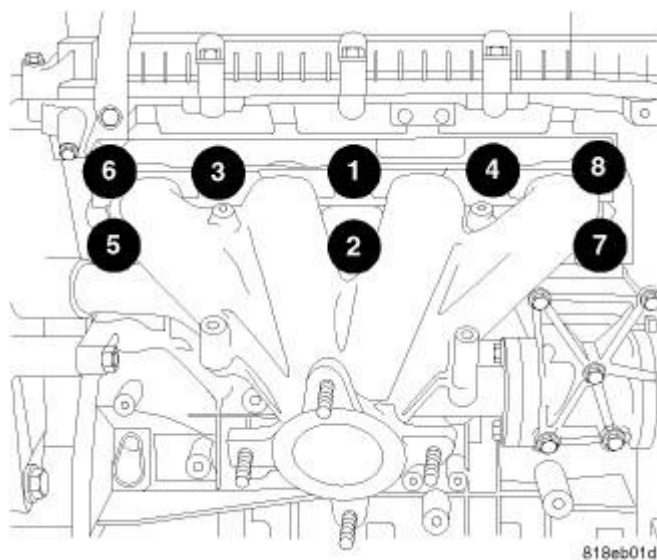
Fig. 324: Exhaust Manifold Retaining Fasteners Removal/Tightening Sequence Courtesy of CHRYSLER GROUP, LLC
