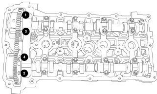
Fig. 145: Front Cam Cap Removal/Tightening Sequence Courtesy of CHRYSLER GROUP, LLC
