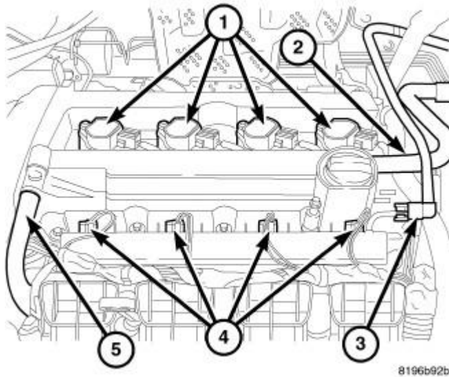
Fig. 334: Ignition Coils, Air Hose, Fuel Line, Injectors & PCV Hose Courtesy of CHRYSLER GROUP, LLC
