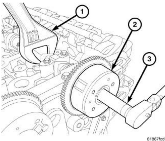
Fig. 360: Removing & Installing Cam Phaser Courtesy of CHRYSLER GROUP, LLC
