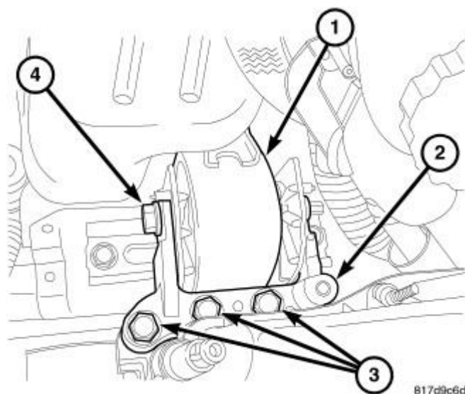
Fig. 28: Right Engine Mount Assembly
