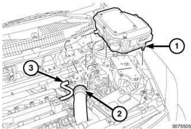
Fig. 64: Air Cleaner Body, Air Inlet Tube & Make-Up Air Hose Courtesy of CHRYSLER GROUP, LLC
