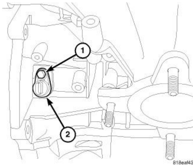
Fig. 207: Crankshaft Position Sensor & Bolt Courtesy of CHRYSLER GROUP, LLC
