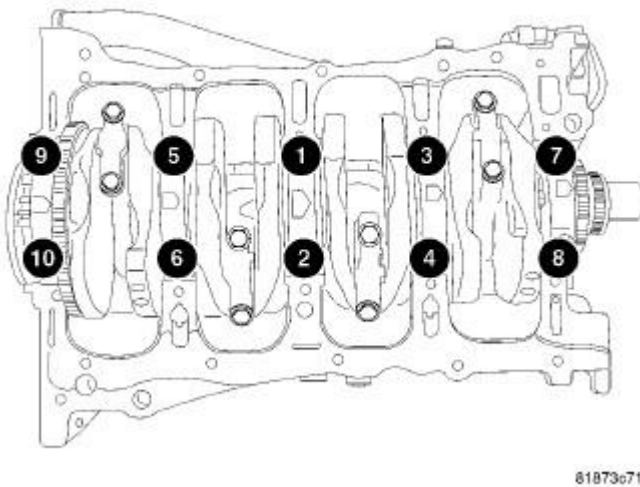
Fig. 199: Main Bearing Cap Removal/Tightening Sequence Courtesy of CHRYSLER GROUP, LLC
