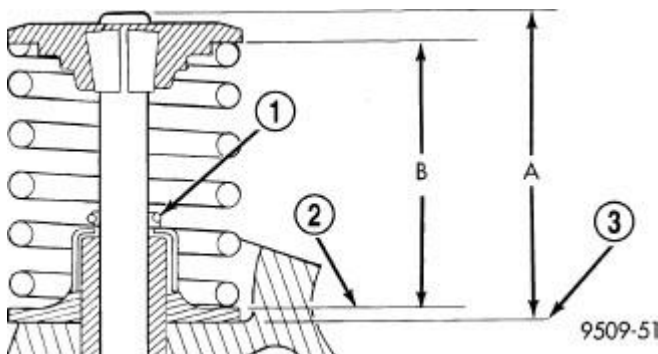
Fig. 180: Spring Installed Height & Valve Tip to Spring Seat Dimensions
