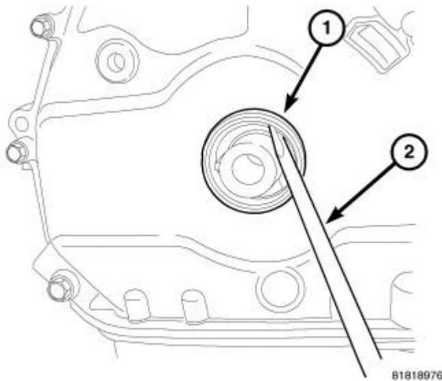
Fig. 233: Front Crankshaft Seal Removal Courtesy of CHRYSLER GROUP, LLC
