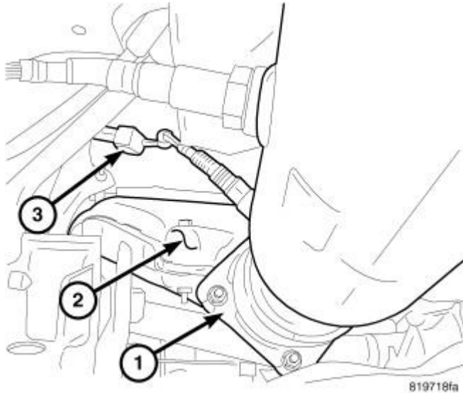
Fig. 33: Exhaust Pipe To Manifold, Heat Shield & Oxygen Sensor Electrical Connector Courtesy of CHRYSLER GROUP, LLC
