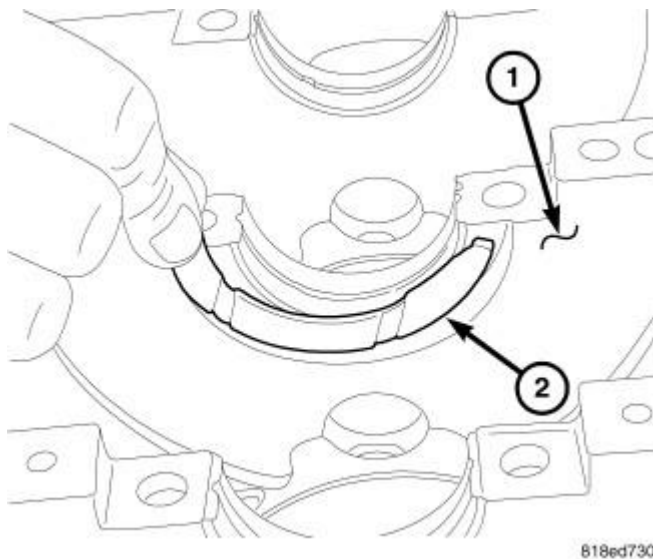
Fig. 203: Installing Thrust Bearing Courtesy of CHRYSLER GROUP, LLC
