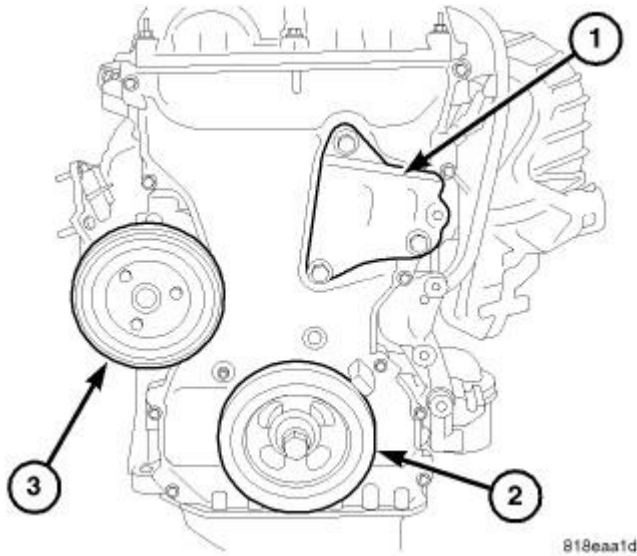
Fig. 194: Right Side Engine Mount Bracket, Crankshaft Damper & Water Pump Pulley Courtesy of CHRYSLER GROUP, LLC
