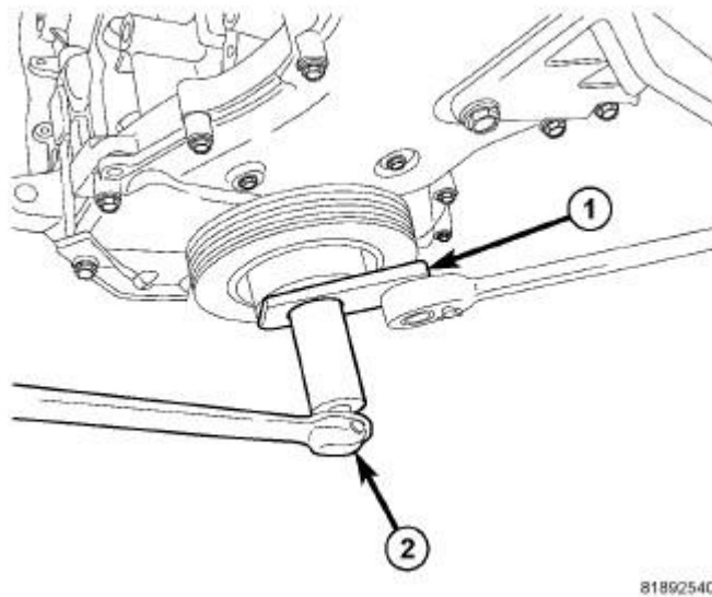
Fig. 237: Damper Removal & Installation Courtesy of CHRYSLER GROUP, LLC
