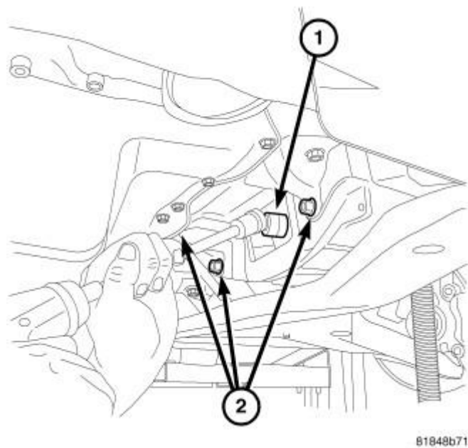
Fig. 24: Removing/Installing Torque Converter Bolts & Lower Bellhousing Bolts
