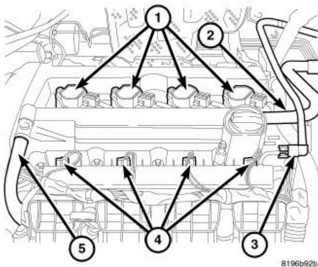
Fig. 343: Ignition Coils, Air Hose, Fuel Line, Injectors & PCV Hose Courtesy of CHRYSLER GROUP, LLC
