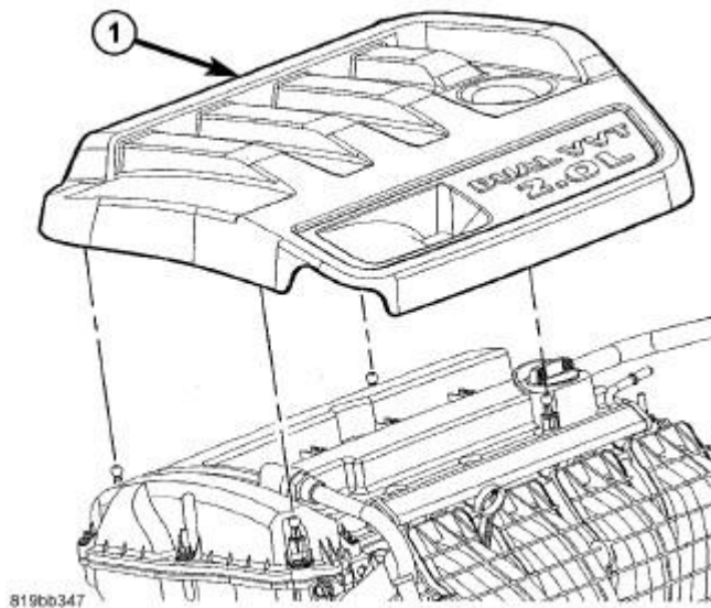
Fig. 125: Engine Cover - 2.0L
