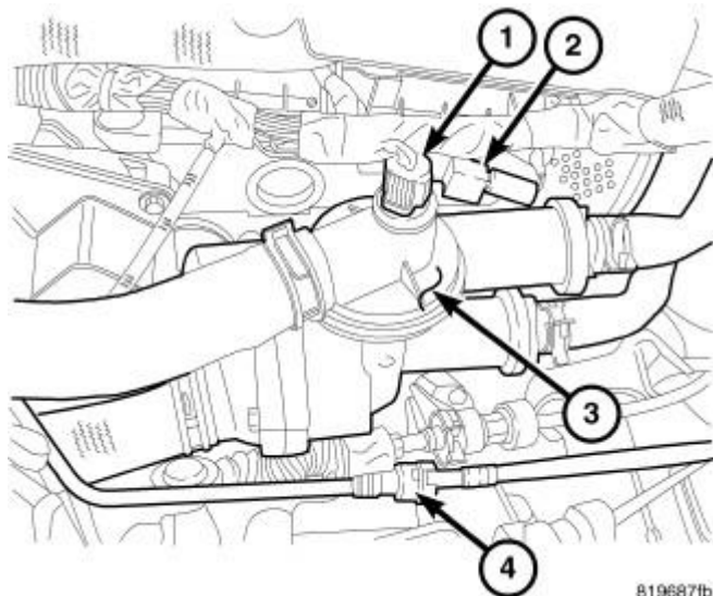
Fig. 48: Coolant Temperature Sensor, Capacitor Electrical Connector & Coolant Adapter Courtesy of CHRYSLER GROUP, LLC
