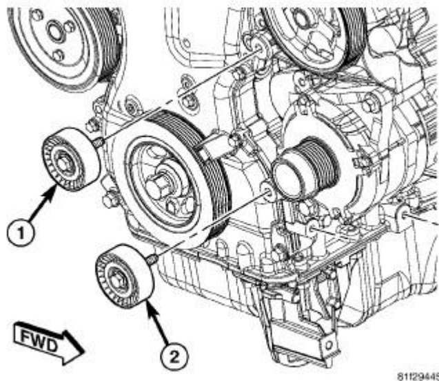
Fig. 373: Removing/Installing Accessory Drive Belt Upper & Lower Idler Pulley Courtesy of CHRYSLER GROUP, LLC
