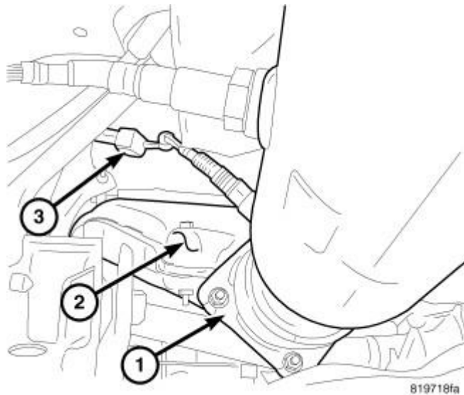
Fig. 328: Exhaust Pipe To Manifold, Heat Shield & Oxygen Sensor Electrical Connector Courtesy of CHRYSLER GROUP, LLC
