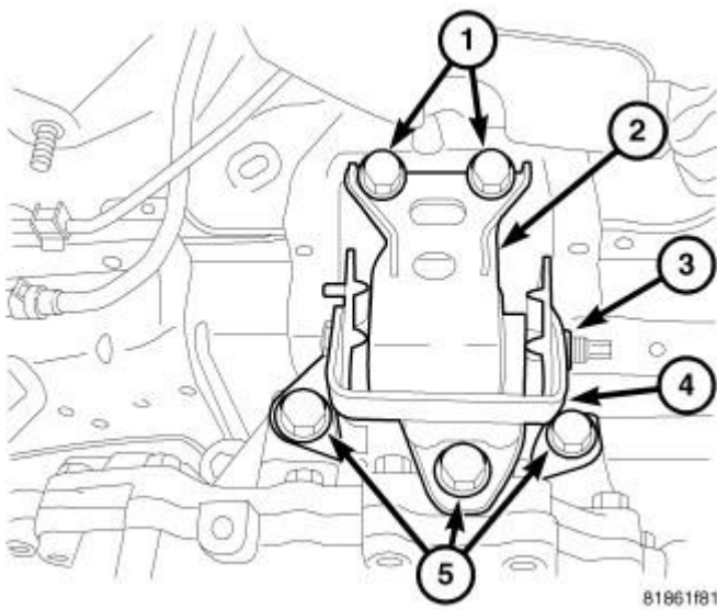
Fig. 248: Left Mount Assembly
