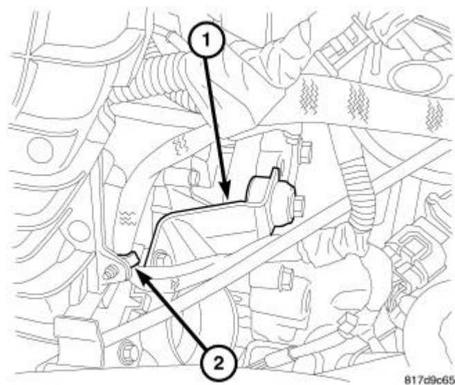
Fig. 341: Throttle Body Support Bracket & Wiring Harness Courtesy of CHRYSLER GROUP, LLC
