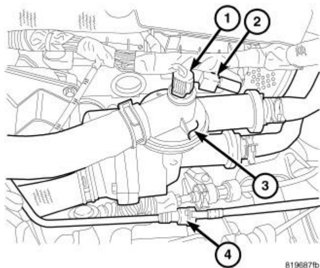
Fig. 94: Coolant Temperature Sensor, Capacitor Electrical Connector & Coolant Adapter Courtesy of CHRYSLER GROUP, LLC
