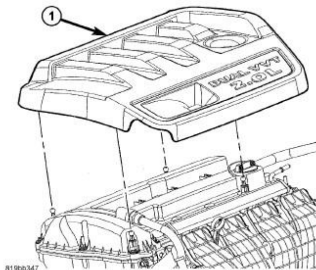
Fig. 398: Engine Cover - 2.0L Courtesy of CHRYSLER GROUP, LLC
