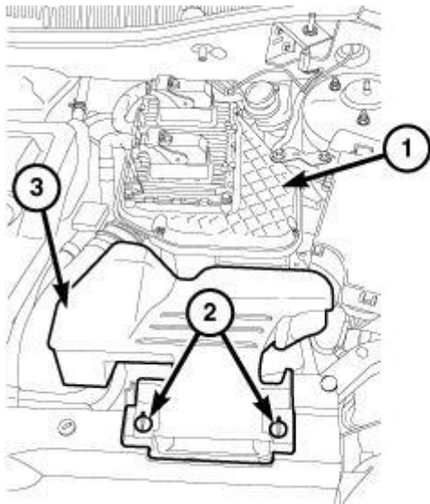
Fig. 244: Retainers, Fresh Air Inlet Duct & Air Cleaner Body Courtesy of CHRYSLER GROUP, LLC
