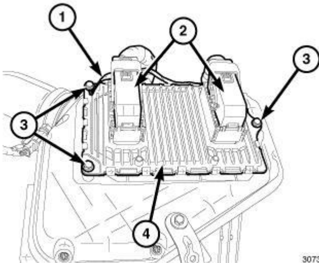
Fig. 10: Electrical Connectors, PCM, Three Mounting Bolts & Ground Wire Courtesy of CHRYSLER GROUP, LLC
