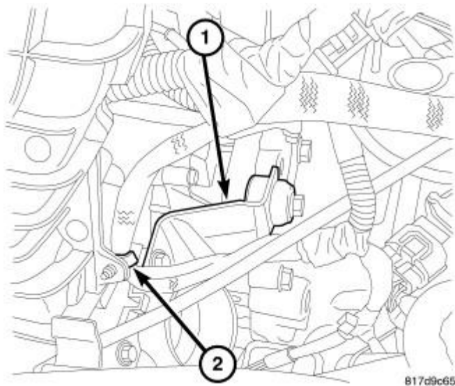
Fig. 91: Throttle Body Support Bracket & Wiring Harness Courtesy of CHRYSLER GROUP, LLC
