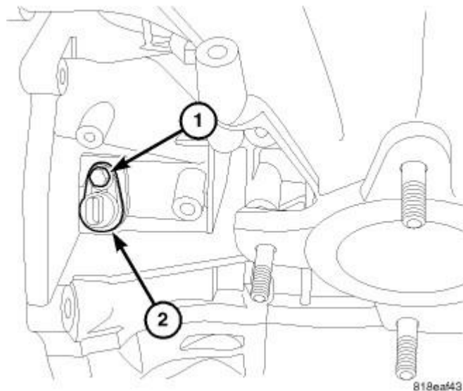
Fig. 26: Crankshaft Position Sensor & Bolt Courtesy of CHRYSLER GROUP, LLC
