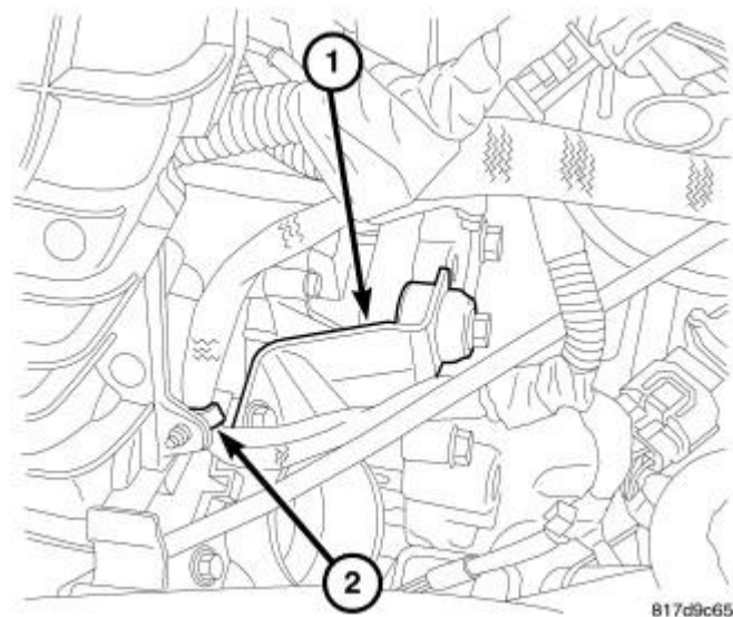
Fig. 44: Throttle Body Support Bracket & Wiring Harness Courtesy of CHRYSLER GROUP, LLC
