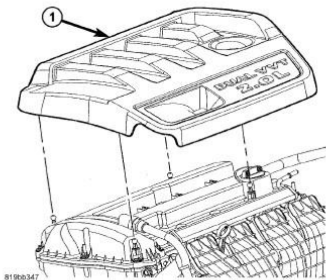
Fig. 163: Engine Cover - 2.0L
