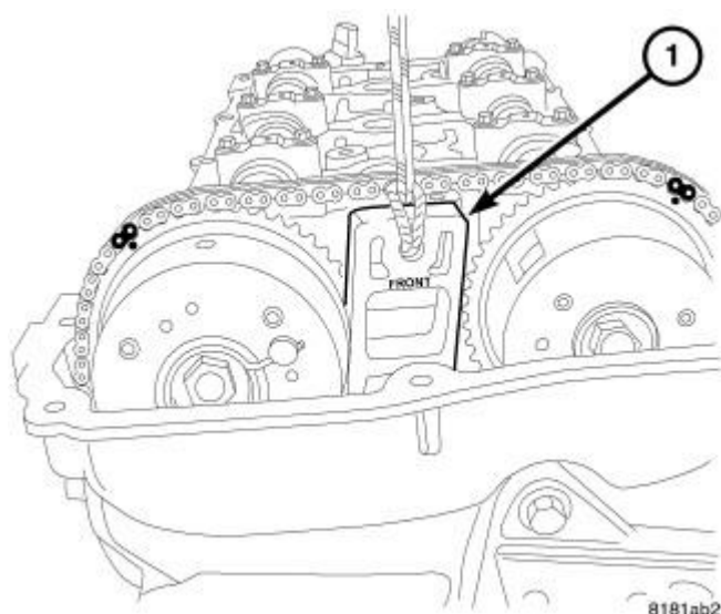
Fig. 143: Wedge 9701 Between Camshaft Phasers
