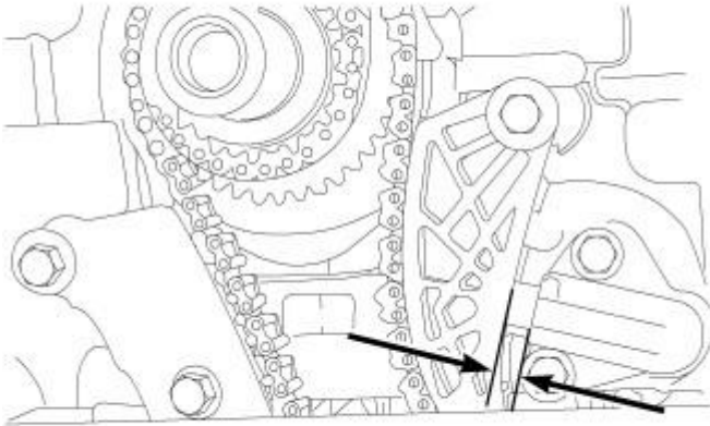
Fig. 307: Measuring Distance Between Tensioner Body & Guide Shoe Courtesy of CHRYSLER GROUP, LLC
