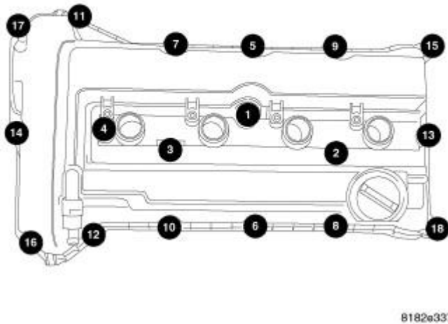
Fig. 75: Cylinder Head Cover Bolt Torque Sequence Courtesy of CHRYSLER LLC
