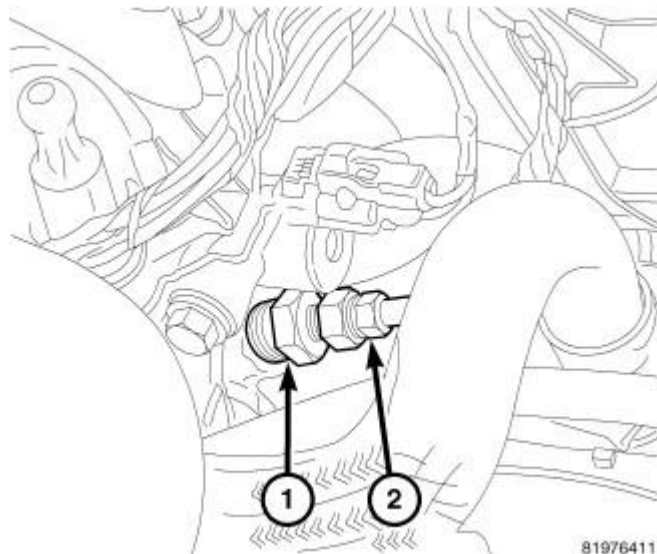
Fig. 267: Oil Pressure Adapter 9879 Courtesy of CHRYSLER LLC
