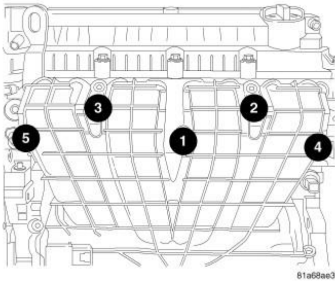
Fig. 19: Intake Manifold Bolt Removal & Tightening Sequence Courtesy of CHRYSLER LLC
