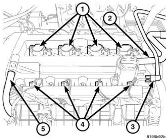
Fig. 334: Coil Connector Courtesy of CHRYSLER LLC
