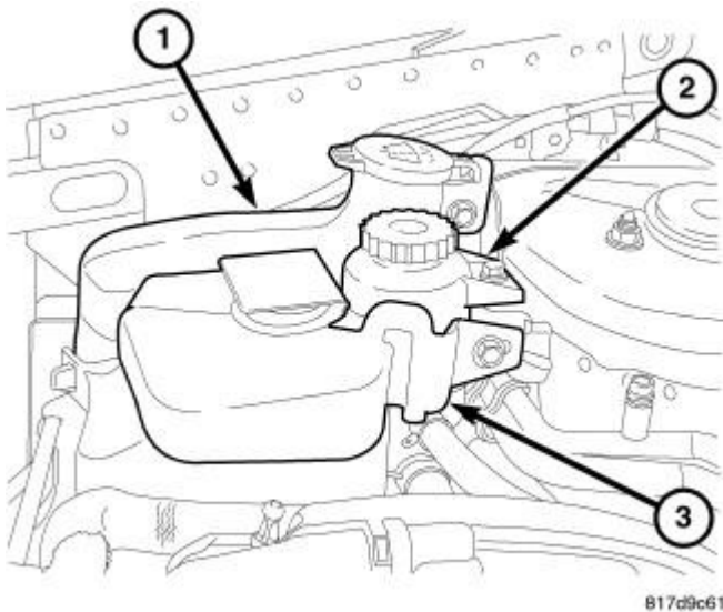
Fig. 259: Coolant Reservoir Courtesy of CHRYSLER LLC
