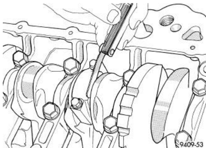
Fig. 186: Connecting Rod Side Clearance Courtesy of CHRYSLER LLC
