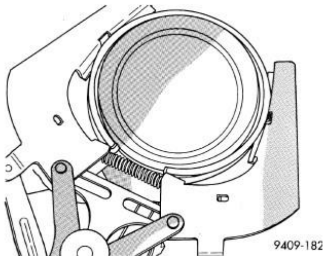
Fig. 222: Piston Rings - Removing & Installing Courtesy of CHRYSLER LLC
