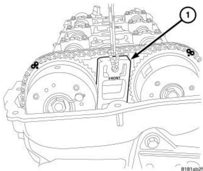
Fig. 143: Inserting Wedge 9701 Between Camshaft Phasers Courtesy of CHRYSLER LLC
