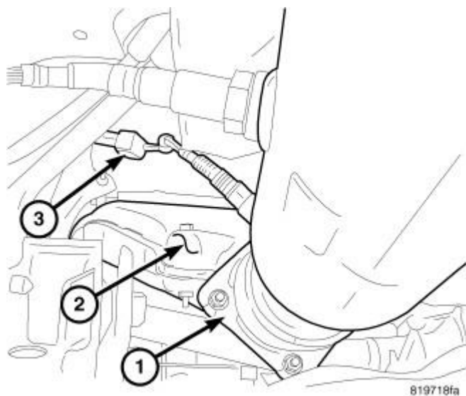
Fig. 81: Removing/Installing Exhaust Pipe, Heat Shields & Oxygen Sensor Courtesy of CHRYSLER LLC
