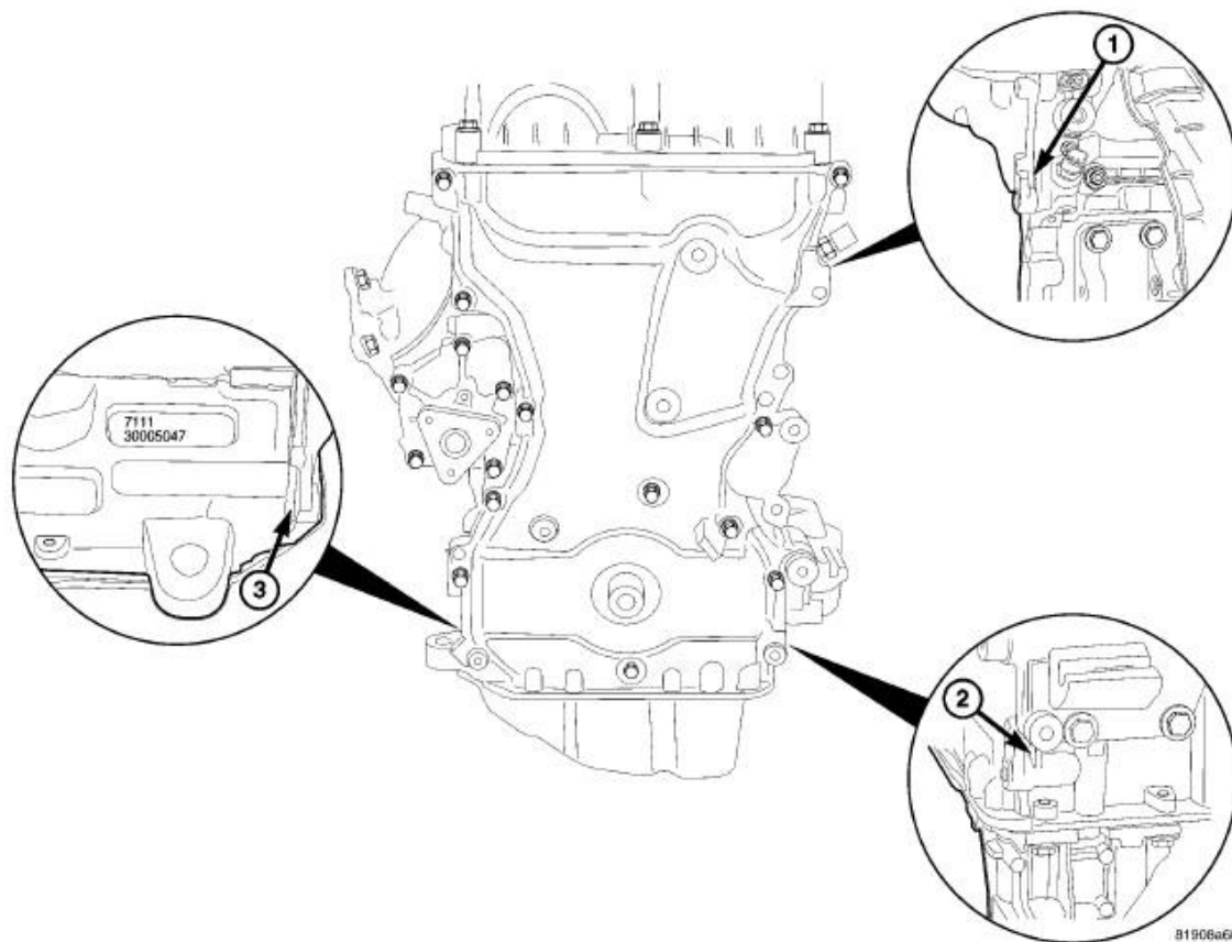
Fig. 379: Timing Chain Cover Pry Points Courtesy of CHRYSLER LLC
