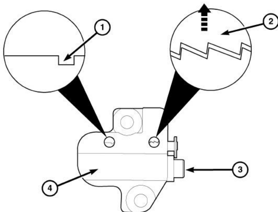
Fig. 400: Tensioner Reset Courtesy of CHRYSLER LLC
