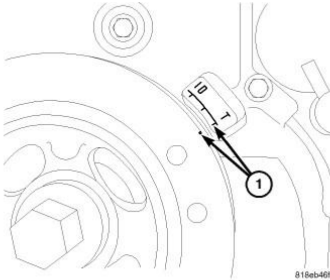
Fig. 76: Setting Crankshaft To Top Dead Center Courtesy of CHRYSLER LLC
