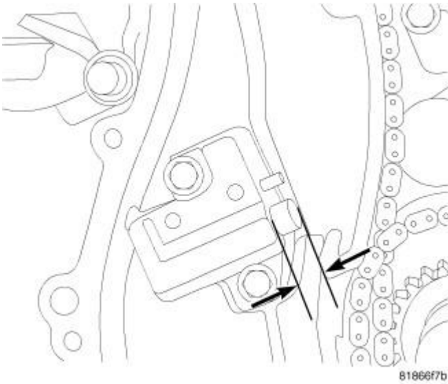
Fig. 355: Checking Timing Chain Stretch Courtesy of CHRYSLER LLC
