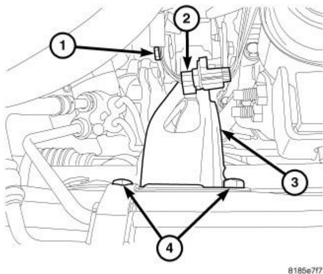
Fig. 253: Rear Mount Through Bolt, Oxygen Sensor Connector, Rear Mount & Rear Mount Retaining Bolts
