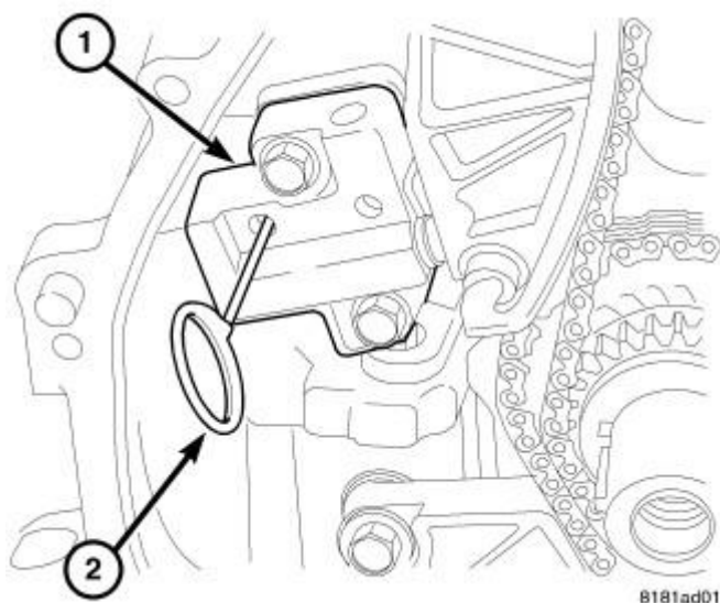
Fig. 401: Timing Chain Tensioner Courtesy of CHRYSLER LLC
