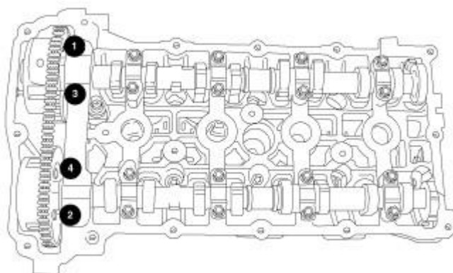
Fig. 155: Removing/Installing Front Intake & Exhaust Bearing Caps - Torque Sequence Courtesy of CHRYSLER LLC
