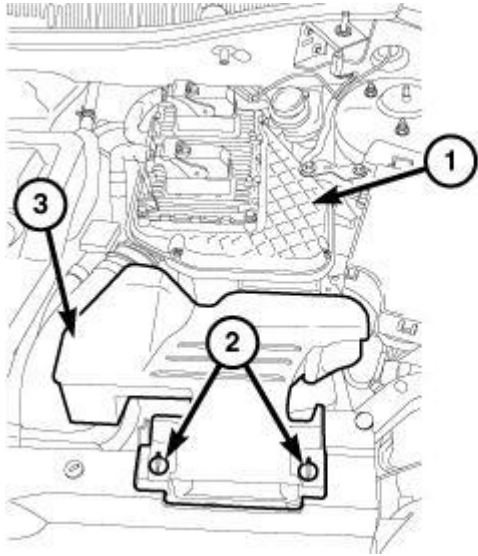
Fig. 346: Retainers, Fresh Air Inlet Duct & Air Cleaner Body Courtesy of CHRYSLER LLC
