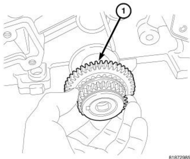
Fig. 196: Crankshaft Sprocket Courtesy of CHRYSLER LLC
