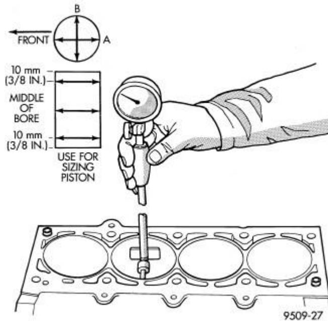
Fig. 226: Checking Cylinder Bore Size Courtesy of CHRYSLER LLC
