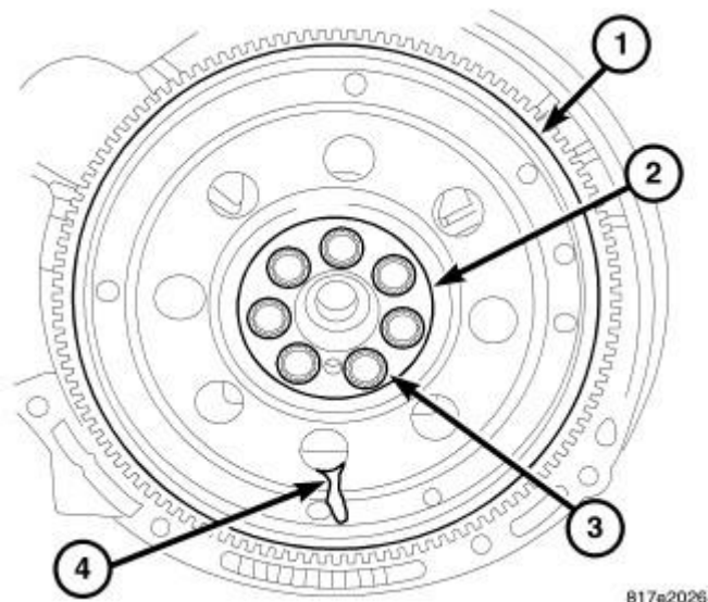
Fig. 241: Flex Plate Courtesy of CHRYSLER LLC
