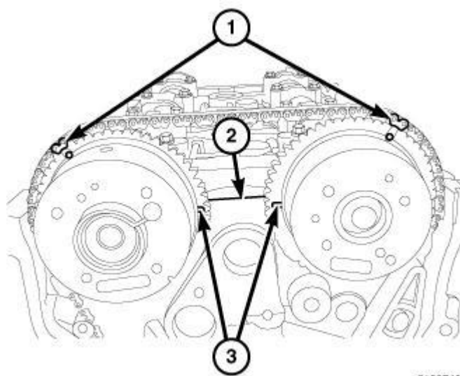
Fig. 153: Timing Chain Timing Marks Courtesy of CHRYSLER LLC
