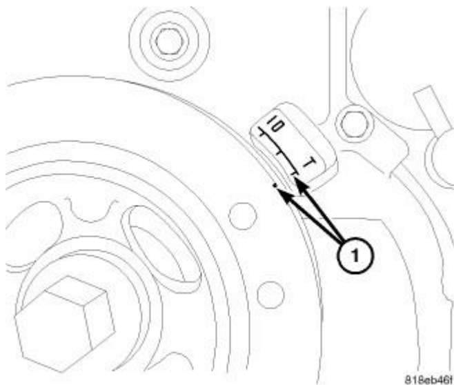
Fig. 172: Setting Crankshaft To Top Dead Center Courtesy of CHRYSLER LLC
