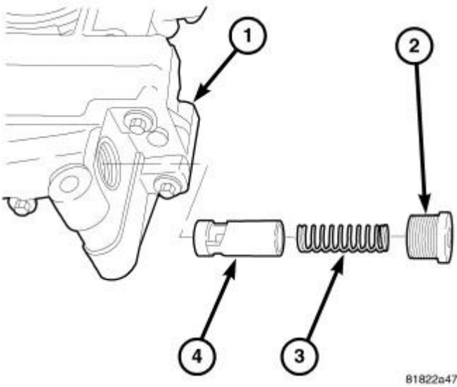
Fig. 318: Oil Pressure Relief Valve Courtesy of CHRYSLER LLC
