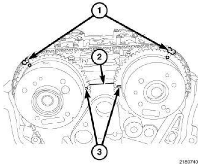
Fig. 151: Timing Chain Timing Marks
