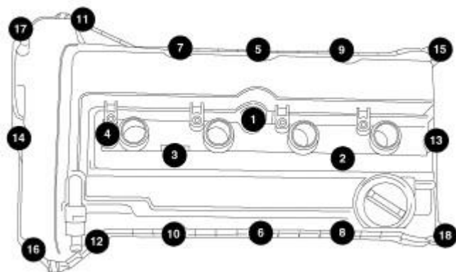
Fig. 161: Cylinder Head Cover Bolt Torque Sequence Courtesy of CHRYSLER LLC
