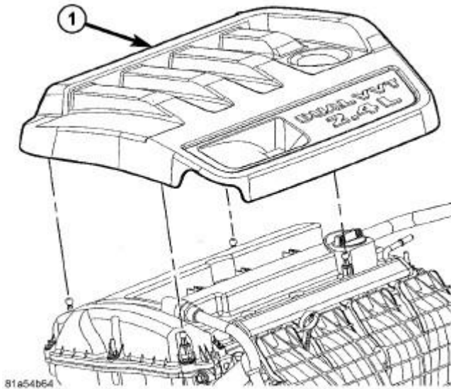
Fig. 330: Engine Cover - 2.4L Courtesy of CHRYSLER LLC
