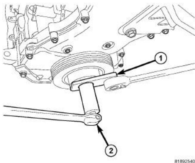
Fig. 212: Damper Removal & Installation Courtesy of CHRYSLER LLC
