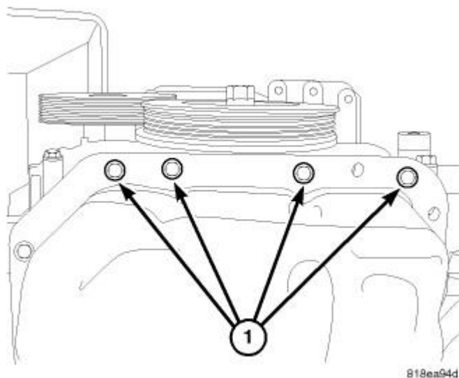
Fig. 80: Timing Chain Cover Lower Bolts Courtesy of CHRYSLER LLC
