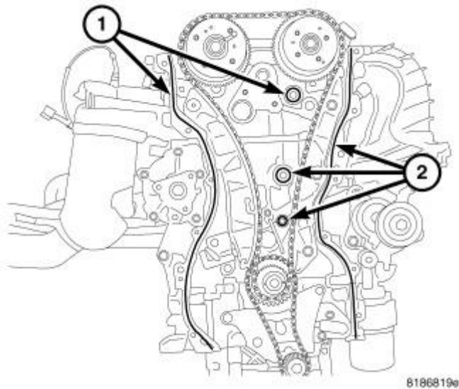
Fig. 384: Timing Chain Cover Sealing Courtesy of CHRYSLER LLC
