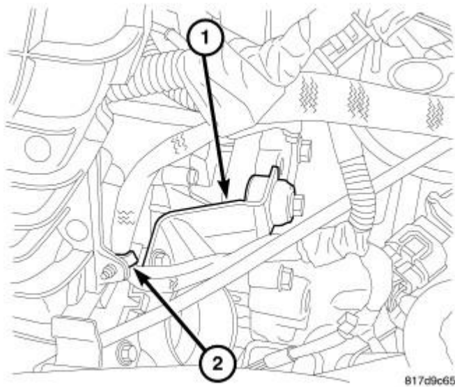
Fig. 341: Throttle Body Support Courtesy of CHRYSLER LLC
