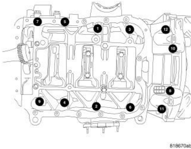
Fig. 219: Ladder Frame Bolts Tightening Sequence Courtesy of CHRYSLER LLC
