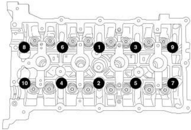
Fig. 106: Cylinder Head Bolt Tightening Sequence
