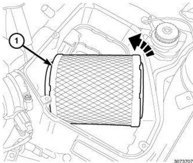
Fig. 58: Air Cleaner Element Courtesy of CHRYSLER LLC
