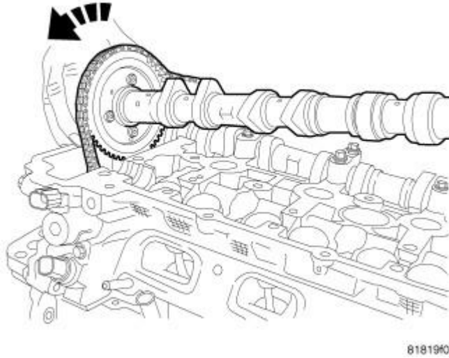
Fig. 147: Rotating Camshaft While Lifting Out Of Front Bearing Cradle Courtesy of CHRYSLER LLC
