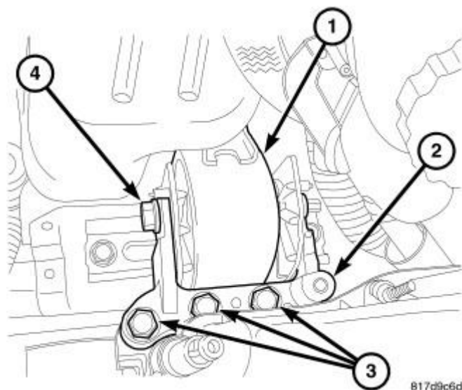
Fig. 82: Right Engine Mount Courtesy of CHRYSLER LLC
