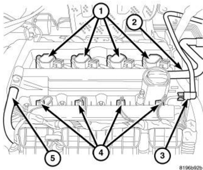
Fig. 170: Coil Connector
