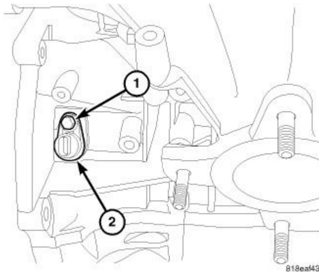
Fig. 34: Crankshaft Position Sensor Courtesy of CHRYSLER LLC
