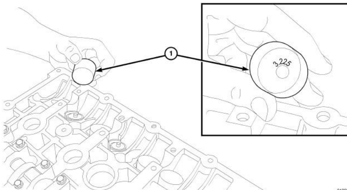
Fig. 131: Tappet Identification Courtesy of CHRYSLER LLC
