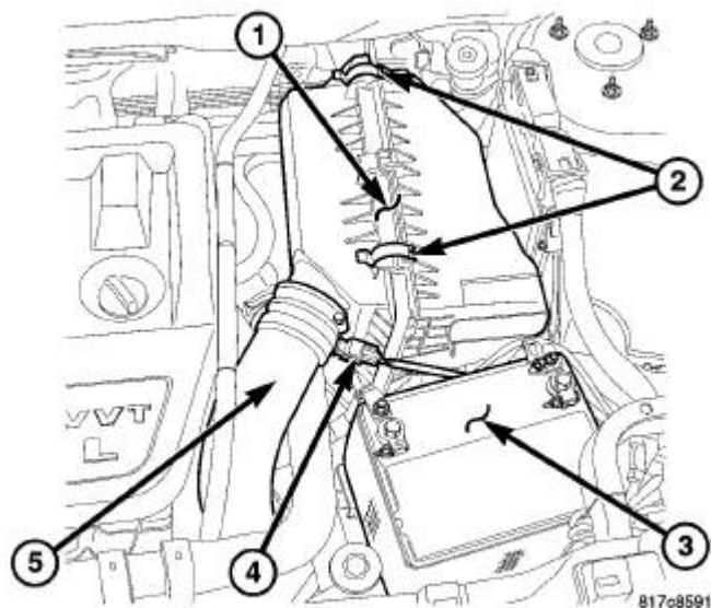
Fig. 397: Air Cleaner Housing Courtesy of CHRYSLER LLC
