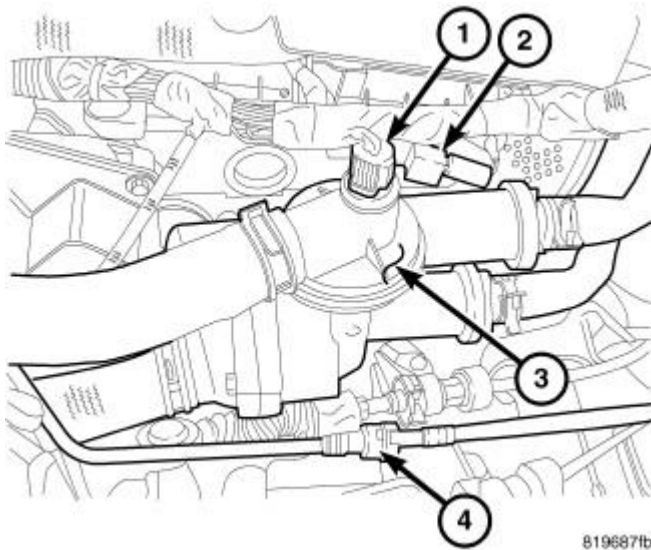
Fig. 90: Coolant Adapter Courtesy of CHRYSLER LLC
