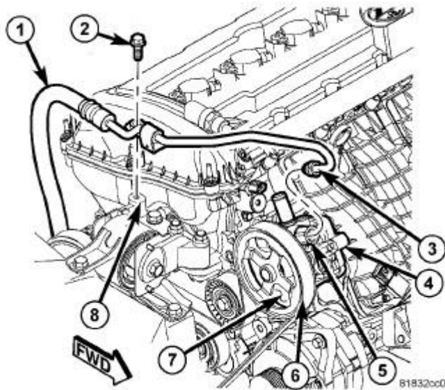
Fig. 368: Pressure Hose Courtesy of CHRYSLER LLC
