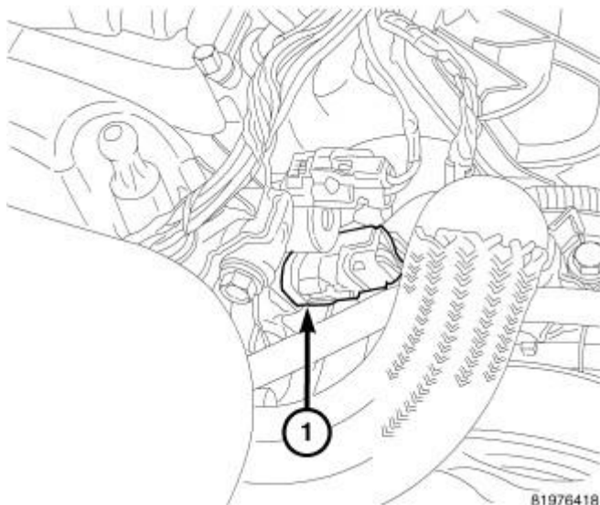
Fig. 266: Oil Temperature Sensor Courtesy of CHRYSLER LLC
