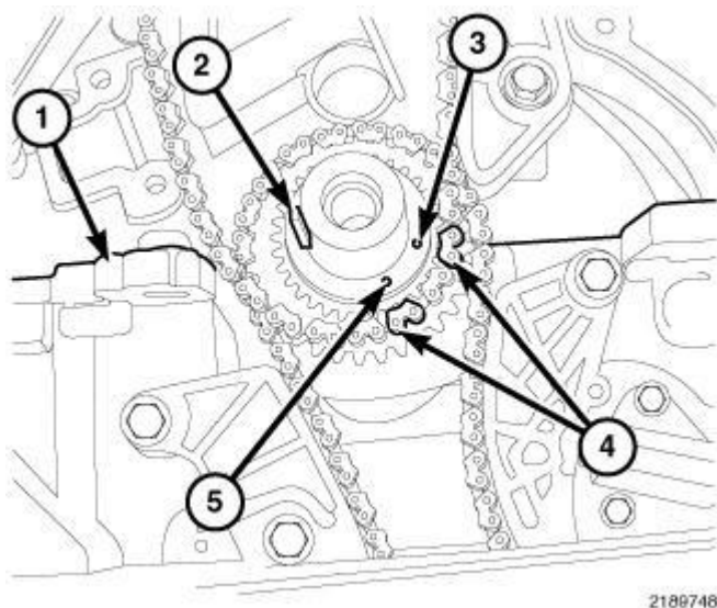
Fig. 351: Crankshaft Timing Marks Courtesy of CHRYSLER LLC
