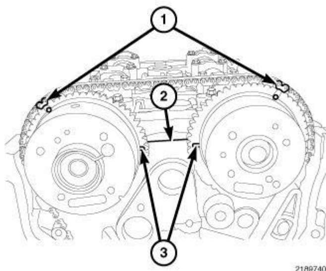
Fig. 352: Timing Chain Timing Marks
