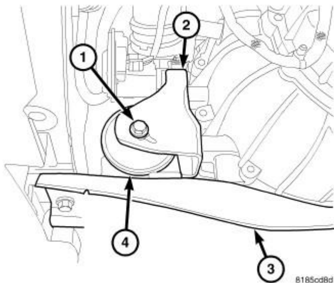
Fig. 243: Front Mount Through Bolt Courtesy of CHRYSLER LLC
