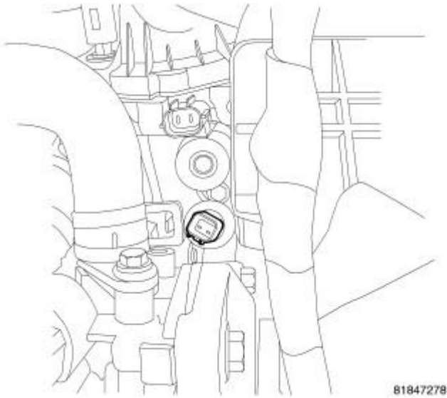
Fig. 273: Oil Pressure Sensor
