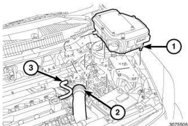
Fig. 51: Air Cleaner Body, Air Inlet Tube & Make-Up Air Hose Courtesy of CHRYSLER LLC
