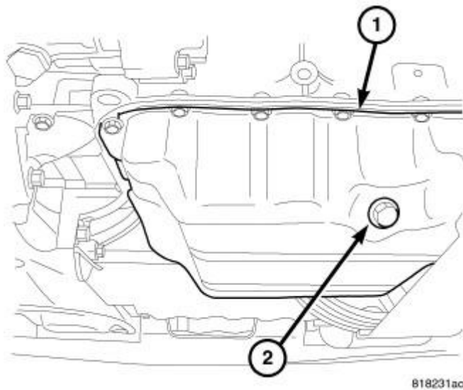
Fig. 192: Oil Drain Plug Courtesy of CHRYSLER LLC
