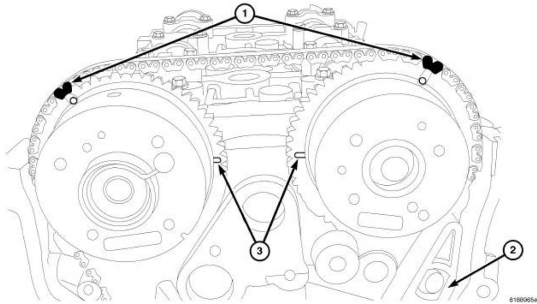
Fig. 156: Timing Chain Timing Marks Courtesy of CHRYSLER LLC
