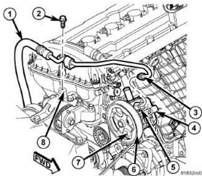
Fig. 395: Pressure Hose Courtesy of CHRYSLER LLC
