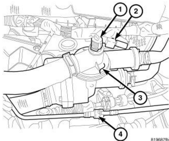
Fig. 108: Coolant Adapter Courtesy of CHRYSLER LLC
