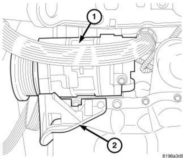
Fig. 32: A/C Compressor
