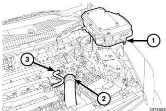
Fig. 333: Air Cleaner Body, Air Inlet Tube & Make-Up Air Hose Courtesy of CHRYSLER LLC
