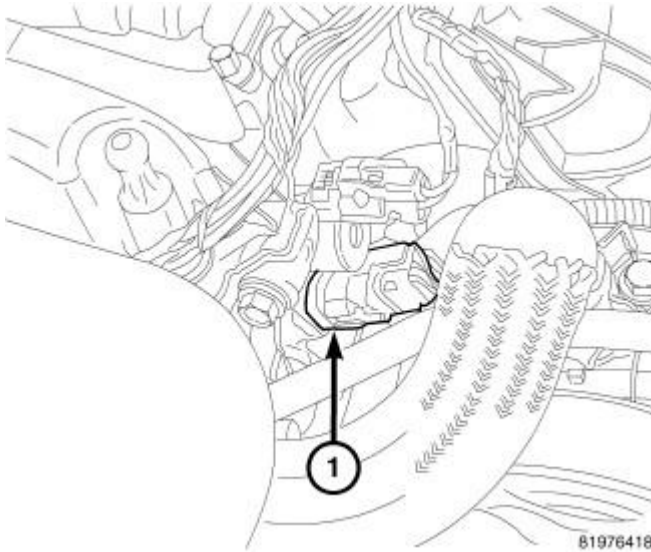
Fig. 342: Oil Temperature Sensor Courtesy of CHRYSLER LLC
