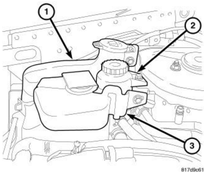
Fig. 254: Coolant Reservoir Courtesy of CHRYSLER LLC
