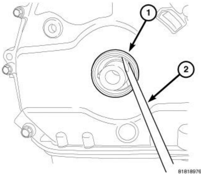
Fig. 233: Front Crankshaft Seal Removal Courtesy of CHRYSLER LLC
