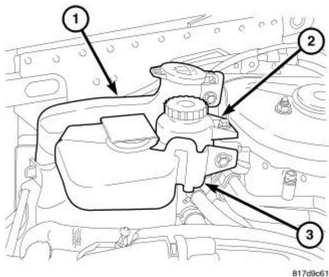
Fig. 49: Coolant Reservoir Courtesy of CHRYSLER LLC
