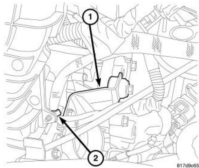
Fig. 44: Throttle Body Support Courtesy of CHRYSLER LLC
