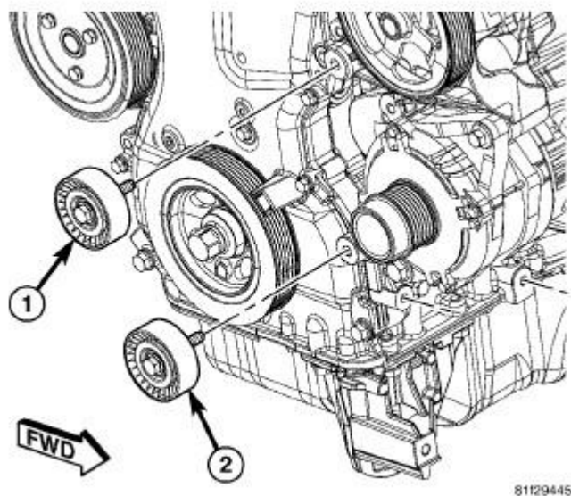
Fig. 78: Removing/Installing Accessory Drive Belt Lower Idler Pulley Courtesy of CHRYSLER LLC
