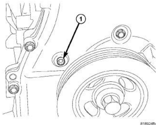
Fig. 141: Tensioner Access Plug Courtesy of CHRYSLER LLC
