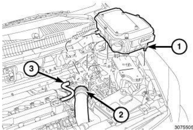
Fig. 246: Air Cleaner Body, Air Inlet Tube & Make-Up Air Hose Courtesy of CHRYSLER LLC
