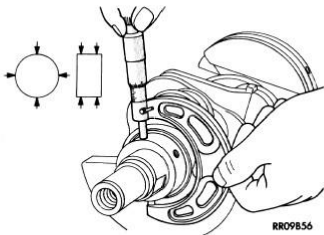
Fig. 200: Crankshaft Journal Measurements - Typical Courtesy of CHRYSLER LLC
