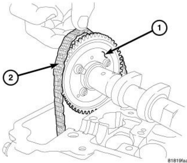
Fig. 148: Chain Removal Courtesy of CHRYSLER LLC
