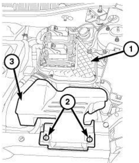
Fig. 331: Retainers, Fresh Air Inlet Duct & Air Cleaner Body Courtesy of CHRYSLER LLC
