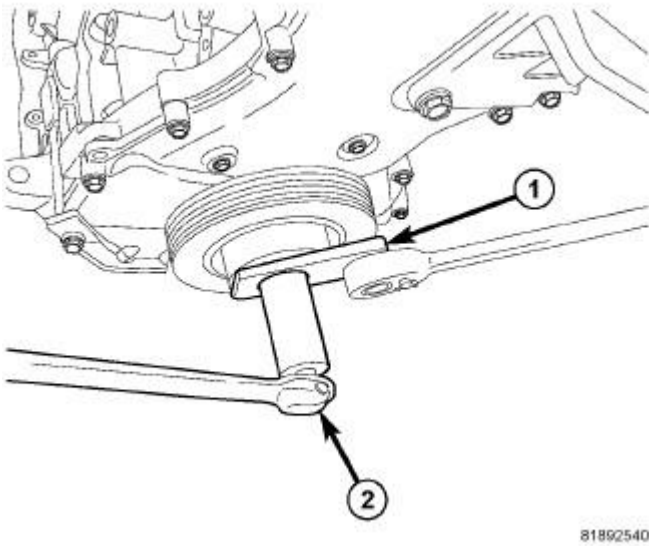
Fig. 232: Damper Removal & Installation Courtesy of CHRYSLER LLC
