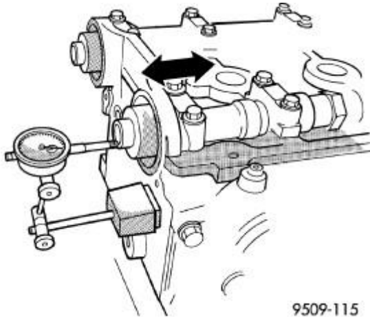
Fig. 137: Camshaft End Play Courtesy of CHRYSLER LLC
