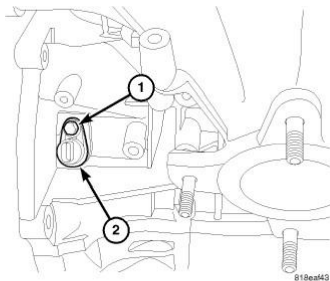
Fig. 207: Crankshaft Position Sensor Courtesy of CHRYSLER LLC
