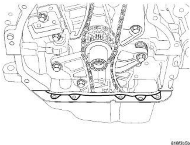
Fig. 383: Sealing Oil Pan
