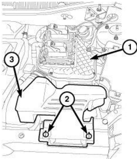
Fig. 69: Retainers, Fresh Air Inlet Duct & Air Cleaner Body
