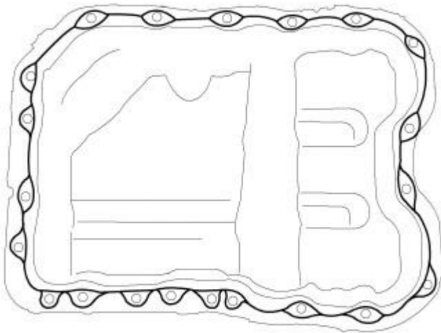
Fig. 297: Sealing Oil Pan Courtesy of CHRYSLER LLC
