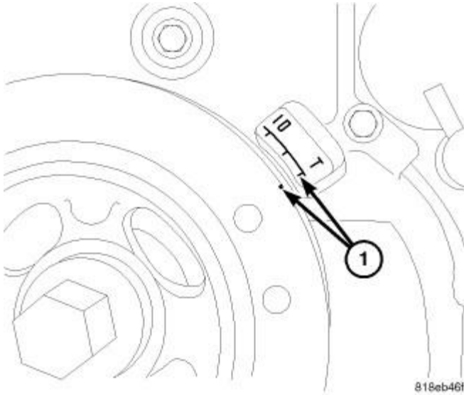
Fig. 139: Setting Engine To Top Dead Center Courtesy of CHRYSLER LLC
