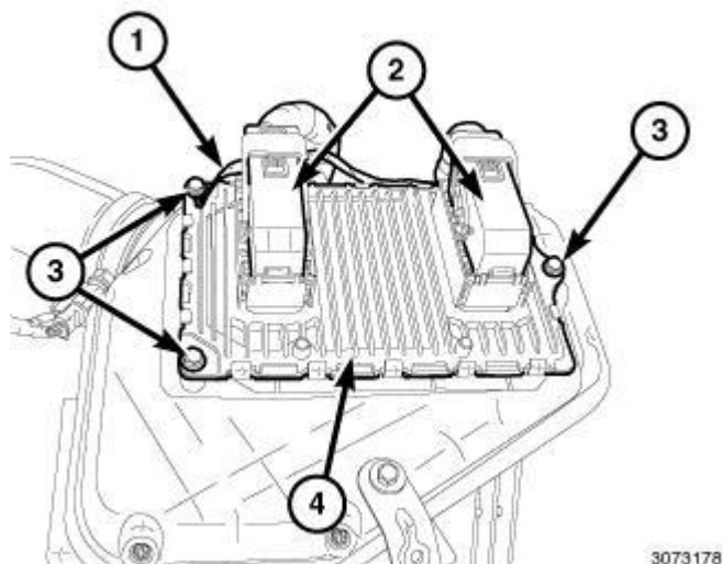
Fig. 123: Electrical Connectors, PCM, Three Mounting Bolts & Ground Wire Courtesy of CHRYSLER LLC
