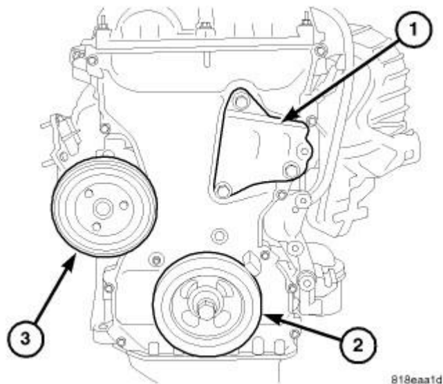
Fig. 386: Right Engine Mount Bracket Courtesy of CHRYSLER LLC
