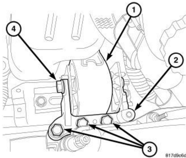
Fig. 376: Right Engine Mount Courtesy of CHRYSLER LLC
