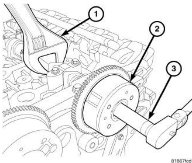
Fig. 126: Removing & Installing Cam Phaser Courtesy of CHRYSLER LLC
