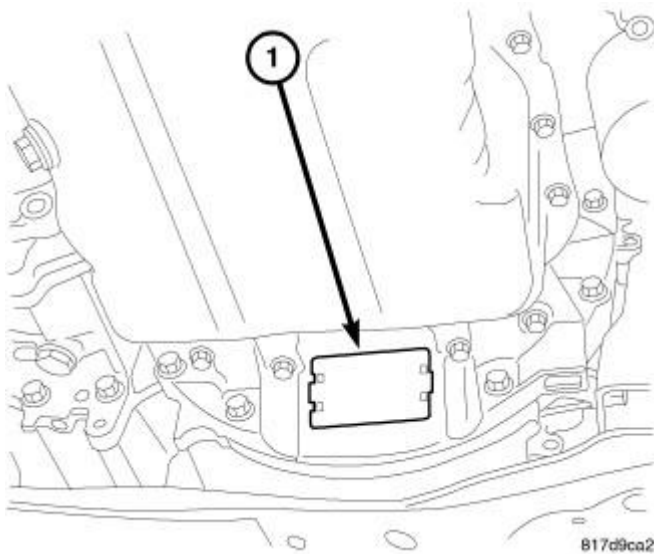
Fig. 23: Inspection Cover Courtesy of CHRYSLER LLC
