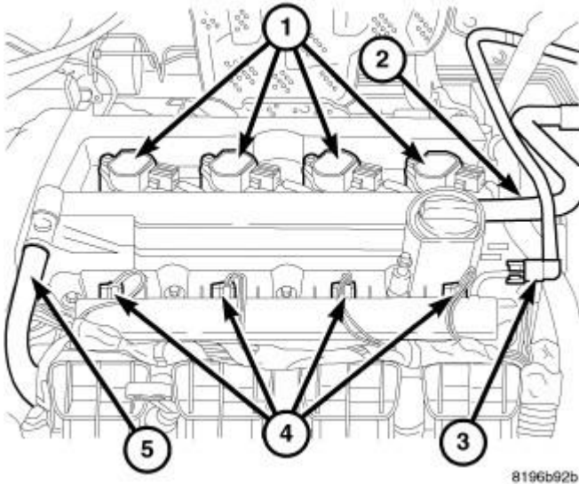
Fig. 18: Coil Connector Courtesy of CHRYSLER LLC
