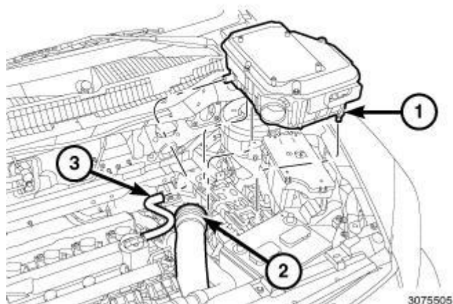
Fig. 344: Air Cleaner Body, Air Inlet Tube & Make-Up Air Hose Courtesy of CHRYSLER LLC
