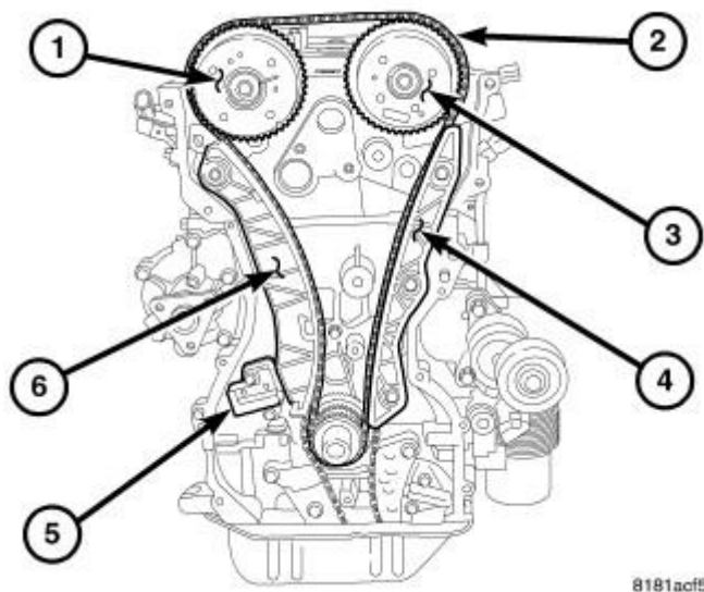
Fig. 348: Identifying Valve Timing Components Courtesy of CHRYSLER LLC
