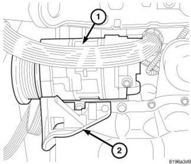
Fig. 372: A/C Compressor Courtesy of CHRYSLER LLC
