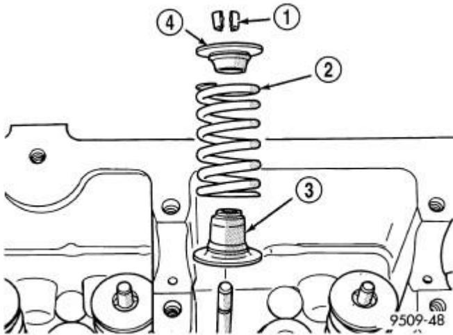
Fig. 176: Valve Spring Assembly Courtesy of CHRYSLER LLC
