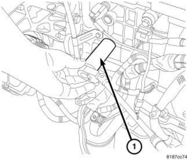
Fig. 262: Oil Sender
