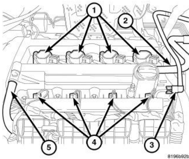
Fig. 119: Coil Connector Courtesy of CHRYSLER LLC
