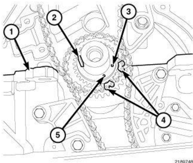
Fig. 361: Crankshaft Timing Marks
