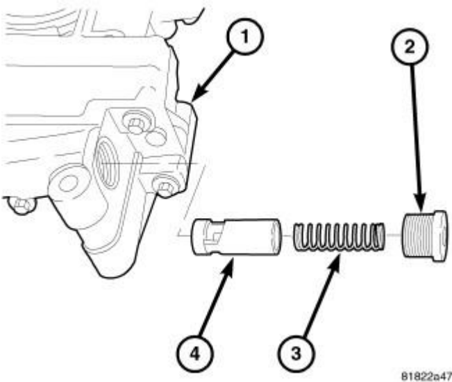
Fig. 319: Oil Pressure Relief Valve Courtesy of CHRYSLER LLC
