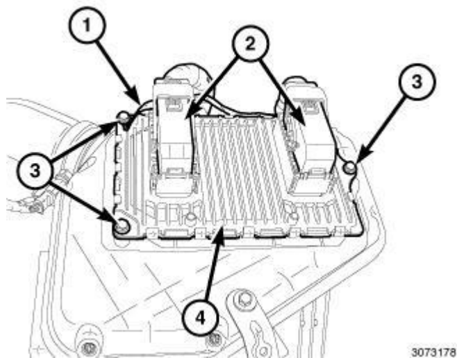
Fig. 10: Electrical Connectors, PCM, Three Mounting Bolts & Ground Wire Courtesy of CHRYSLER LLC
