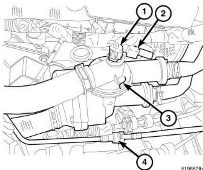
Fig. 48: Coolant Adapter Courtesy of CHRYSLER LLC
