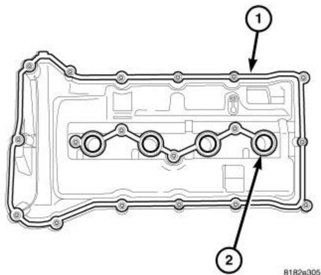
Fig. 160: Cylinder Head Cover Gaskets Location Courtesy of CHRYSLER LLC
