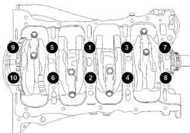
Fig. 206: Main Bearing Cap Torque Sequence
