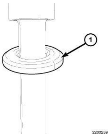
Fig. 104: Washers Must Be Installed With Bevel Edge Up Towards Bolt Head Courtesy of CHRYSLER LLC
