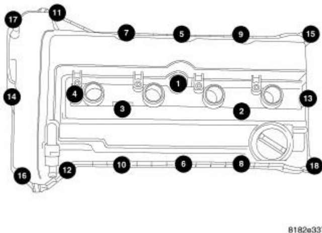
Fig. 169: Cylinder Head Cover Bolts Torque Sequence
