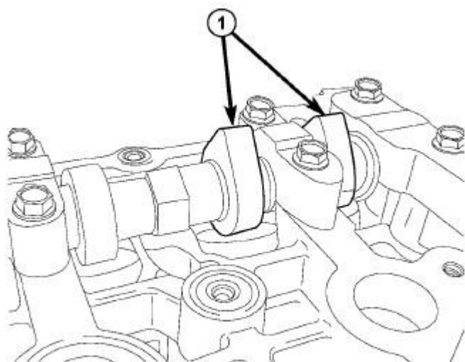
Fig. 129: Identifying Camshaft So Lobes Are Vertical
