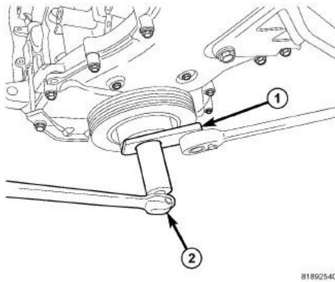
Fig. 237: Damper Removal & Installation Courtesy of CHRYSLER LLC
