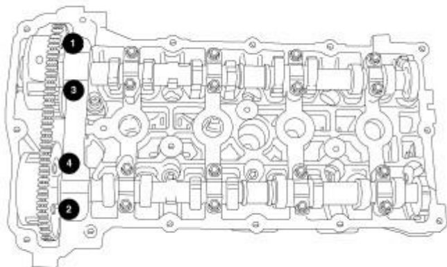
Fig. 145: Removing/Installing Front Camshaft Bearing Caps Courtesy of CHRYSLER LLC
