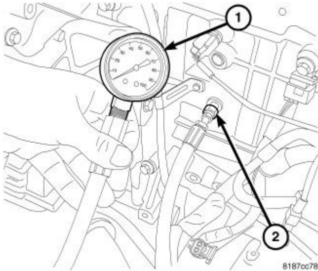
Fig. 264: Oil Pressure Gauge Courtesy of CHRYSLER LLC
