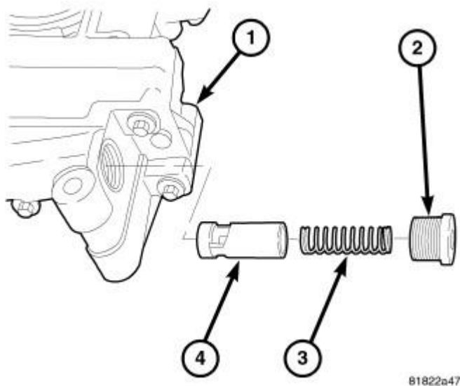
Fig. 320: Oil Pressure Relief Valve Courtesy of CHRYSLER LLC
