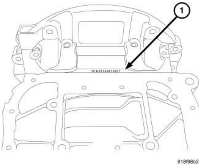
Fig. 55: Locating Engine Serial Number Courtesy of CHRYSLER LLC
