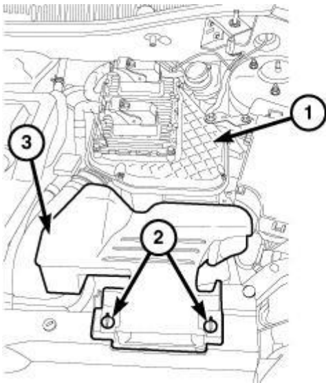
Fig. 244: Retainers, Fresh Air Inlet Duct & Air Cleaner Body Courtesy of CHRYSLER LLC
