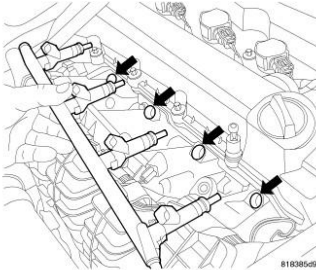
Fig. 89: Removing/Installing Fuel Rail Courtesy of CHRYSLER LLC
