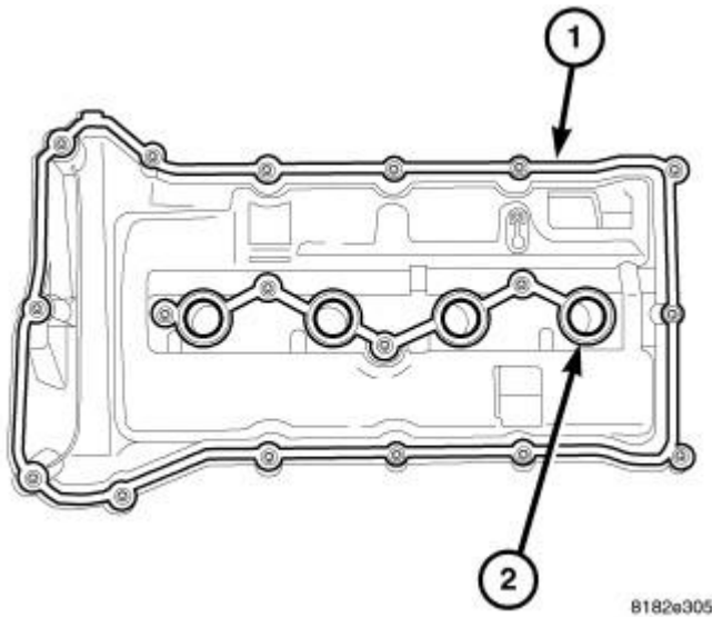
Fig. 166: Cylinder Head Cover Gaskets Location Courtesy of CHRYSLER LLC
