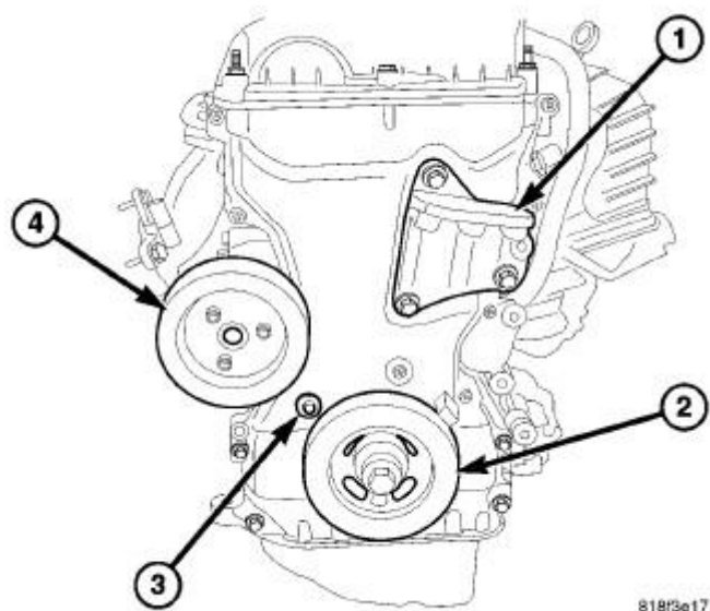
Fig. 79: Engine Front Courtesy of CHRYSLER LLC
