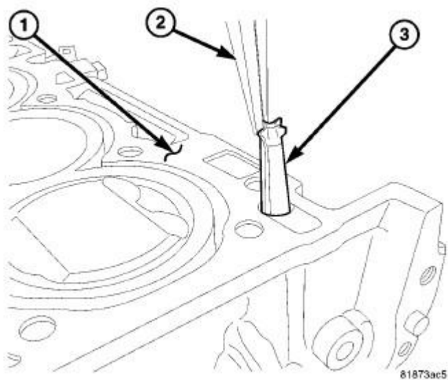
Fig. 269: Removing/Installing VVT Filter Screen Courtesy of CHRYSLER LLC
