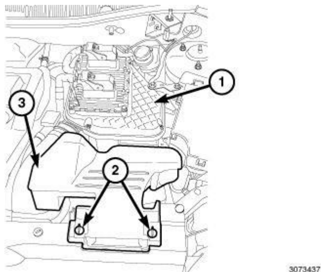
Fig. 9: Retainers, Fresh Air Inlet Duct & Air Cleaner Body Courtesy of CHRYSLER LLC
