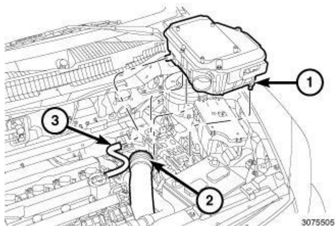
Fig. 71: Air Cleaner Body, Air Inlet Tube & Make-Up Air Hose Courtesy of CHRYSLER LLC
