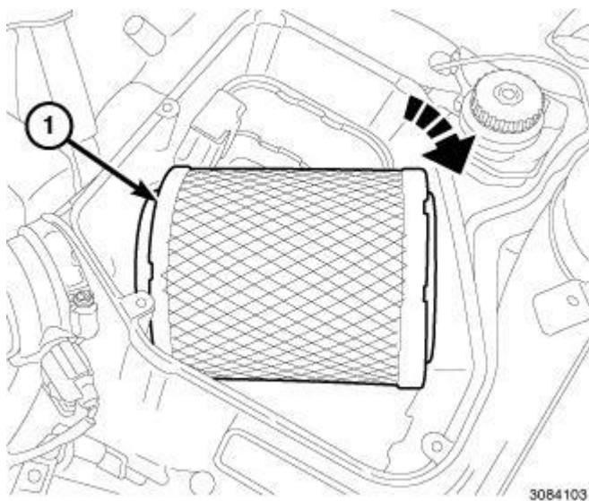
Fig. 59: Air Cleaner Element Courtesy of CHRYSLER LLC
