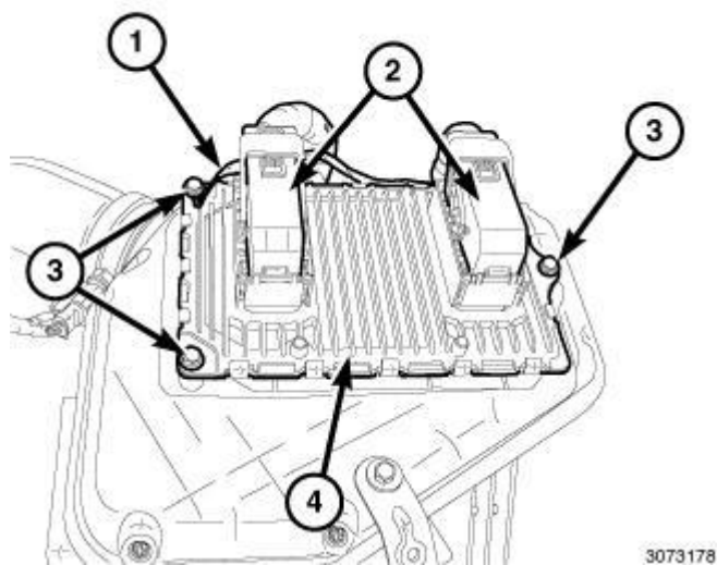
Fig. 52: Electrical Connectors, PCM, Three Mounting Bolts & Ground Wire Courtesy of CHRYSLER LLC
