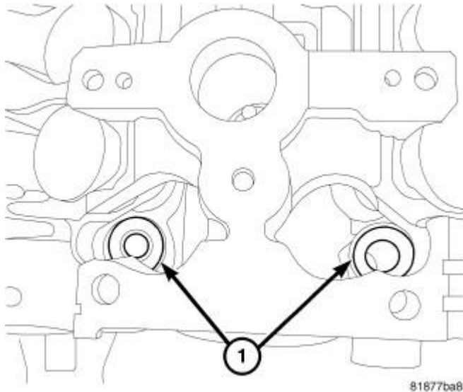
Fig. 97: Front Head Bolt Washers Courtesy of CHRYSLER LLC
