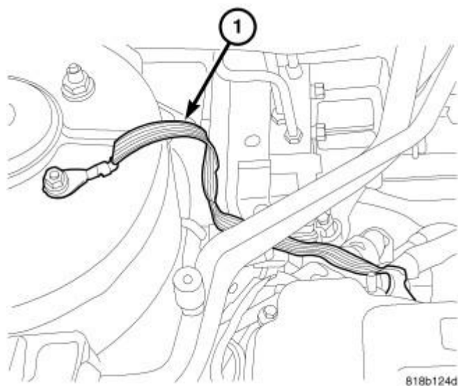
Fig. 21: Ground Strap Courtesy of CHRYSLER LLC
