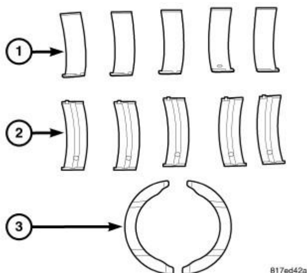
Fig. 201: Bearing Identification Courtesy of CHRYSLER LLC
