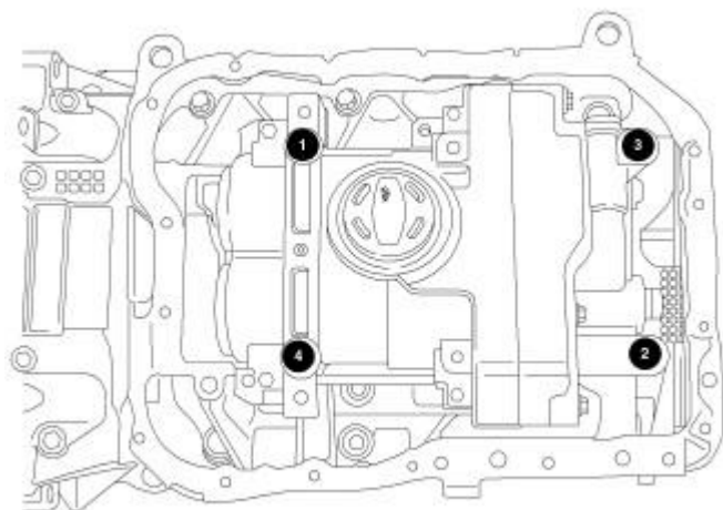
Fig. 310: BSM Mounting Bolts Tightening Sequence Courtesy of CHRYSLER LLC
