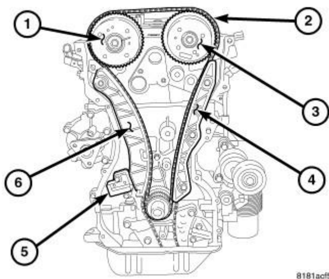
Fig. 399: Removing/Installing Timing Chain Tensioner Courtesy of CHRYSLER LLC
