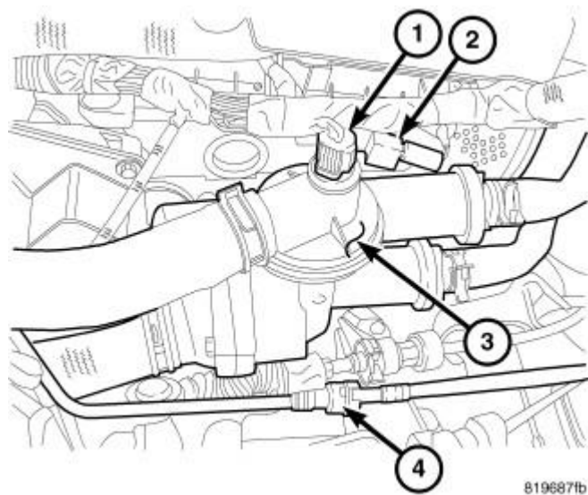
Fig. 94: Coolant Adapter Courtesy of CHRYSLER LLC
