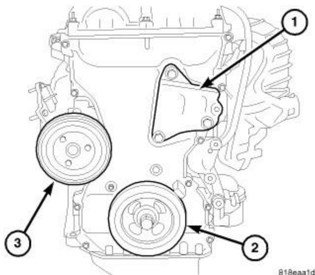
Fig. 209: Right Engine Mount Bracket Courtesy of CHRYSLER LLC
