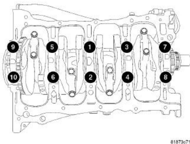
Fig. 199: Main Bearing Cap Torque Sequence Courtesy of CHRYSLER LLC
