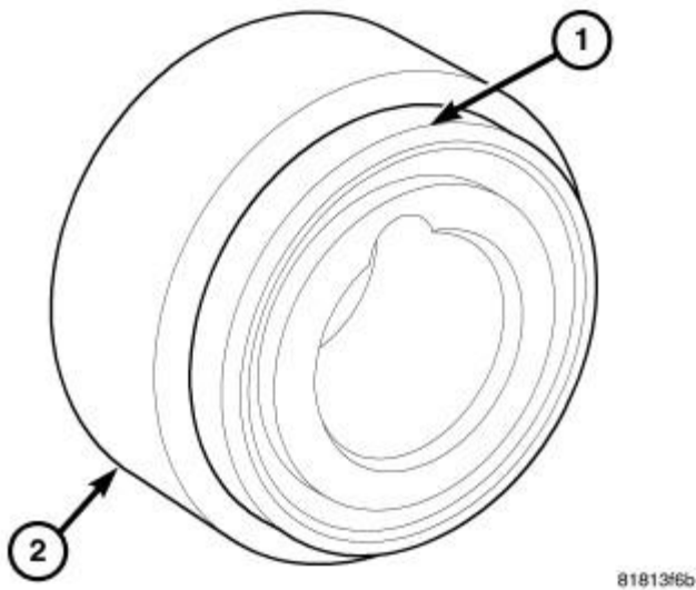
Fig. 234: Crankshaft Oil Seal & Seal Installer 9506 Courtesy of CHRYSLER LLC
