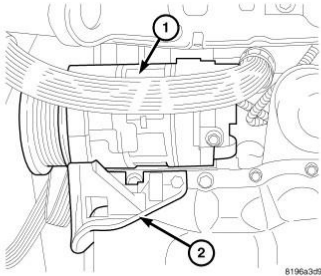
Fig. 392: A/C Compressor Courtesy of CHRYSLER LLC
