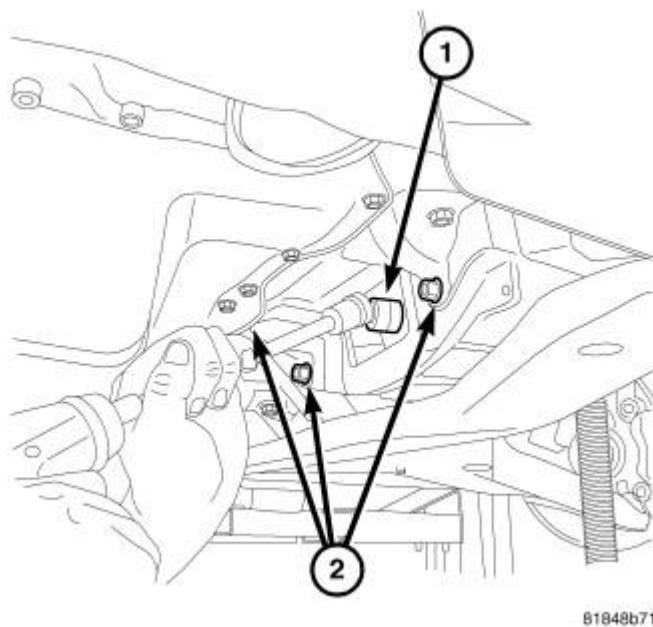
Fig. 36: Modular Clutch To Flex Plate Bolts Courtesy of CHRYSLER LLC
