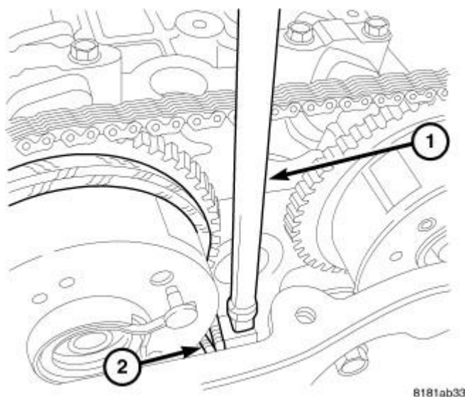
Fig. 144: Seating Wedge Tool 9701 Courtesy of CHRYSLER LLC
