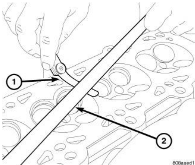
Fig. 98: Checking Cylinder Head Flatness
