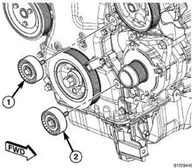
Fig. 373: Removing/Installing Accessory Drive Belt Lower Idler Pulley Courtesy of CHRYSLER LLC
