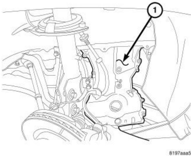
Fig. 385: Timing Chain Cover Removal & Installation Courtesy of CHRYSLER LLC
