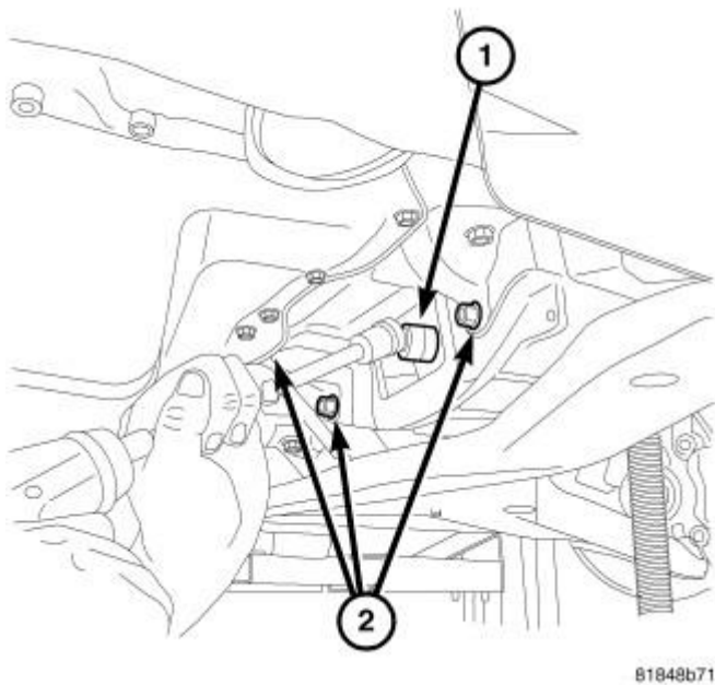
Fig. 24: Modular Clutch To Flex Plate Bolts Courtesy of CHRYSLER LLC
