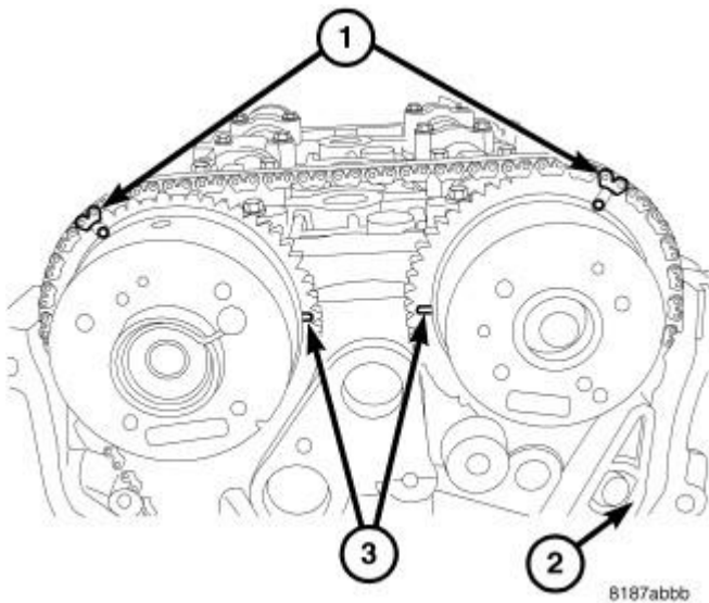
Fig. 140: Timing Chain Timing Marks Courtesy of CHRYSLER LLC
