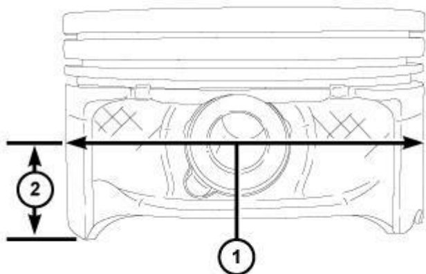
Fig. 225: Piston Pin Measurements
