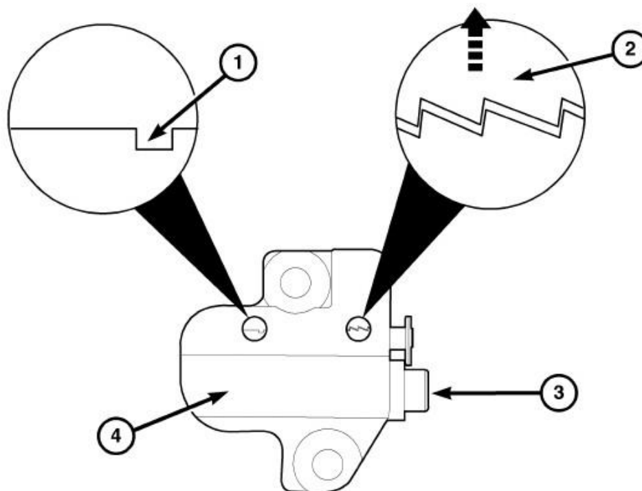
Fig. 142: Tensioner Reset Courtesy of CHRYSLER LLC
