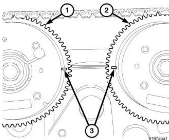
Fig. 350: Camshaft Timing Courtesy of CHRYSLER LLC
