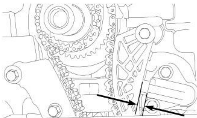
Fig. 307: Oil Pump Chain Stretch
