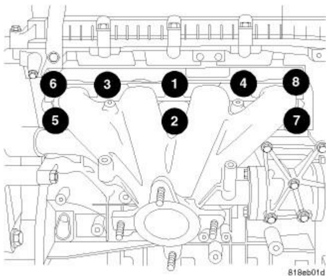
Fig. 325: Exhaust Manifold Retaining Fasteners Tightening Sequence Courtesy of CHRYSLER LLC
