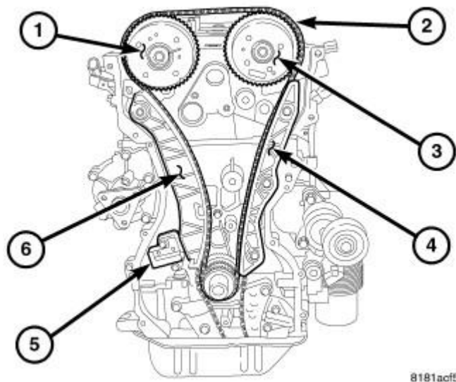
Fig. 353: Removing/Installing Timing Chain Tensioner & Timing Chain
