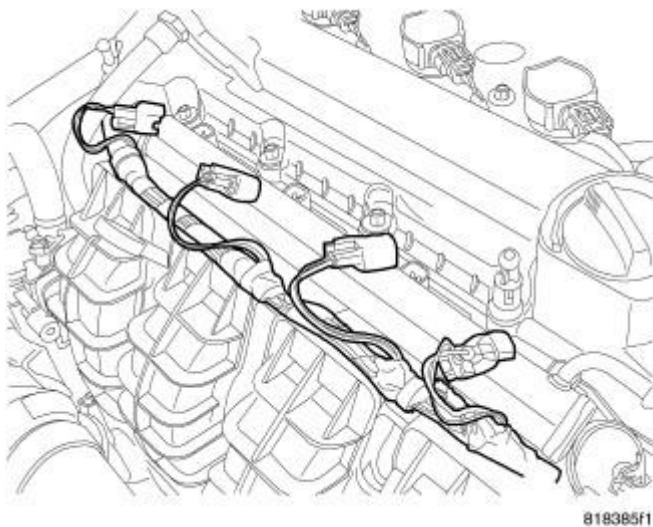
Fig. 88: Identifying Fuel Injector Electrical Connectors Courtesy of CHRYSLER LLC
