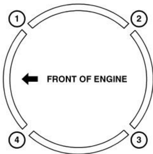
Fig. 224: Identifying Piston Ring End Gap Positions Courtesy of CHRYSLER LLC
