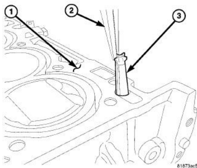
Fig. 100: Removing/Installing VVT Filter Screen
