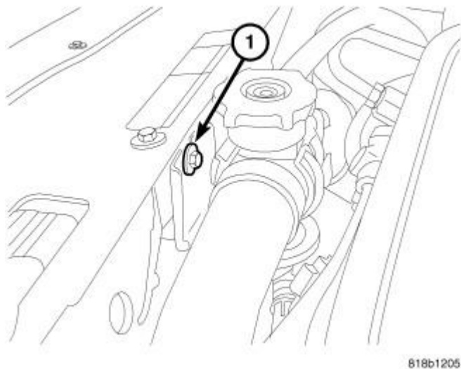
Fig. 92: Radiator Hose Support Courtesy of CHRYSLER LLC
