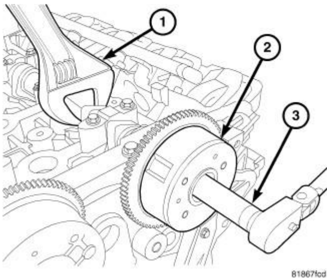
Fig. 360: Cam Phaser Installation Courtesy of CHRYSLER LLC
