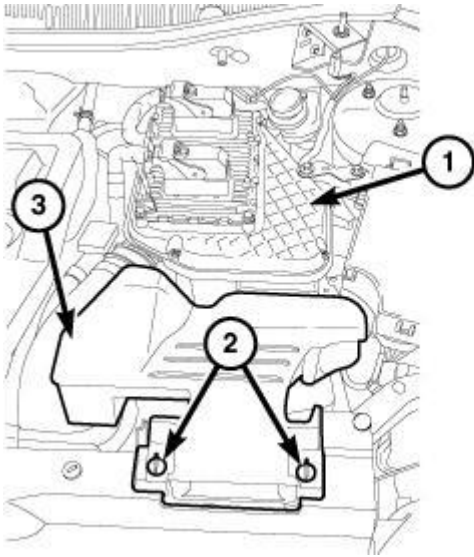
Fig. 62: Retainers, Fresh Air Inlet Duct & Air Cleaner Body Courtesy of CHRYSLER LLC
