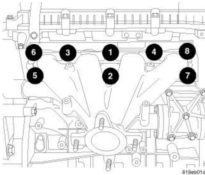
Fig. 324: Exhaust Manifold Retaining Fasteners Tightening Sequence Courtesy of CHRYSLER LLC
