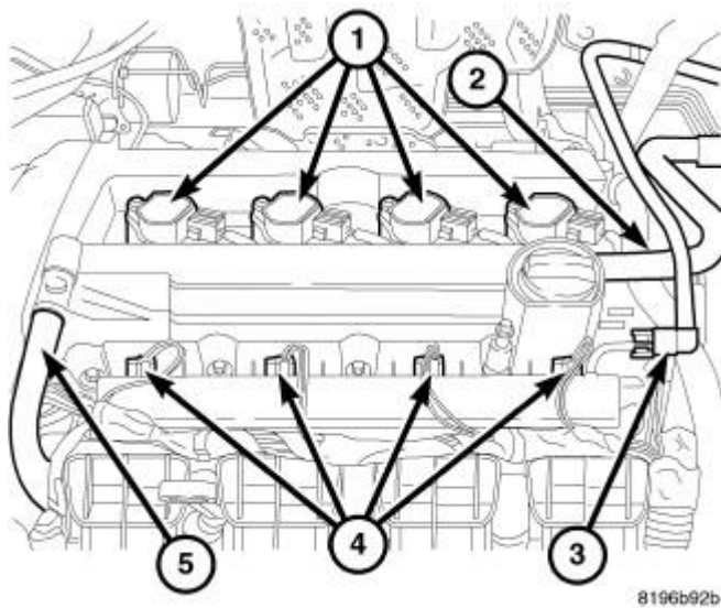
Fig. 45: Coil Connector Courtesy of CHRYSLER LLC
