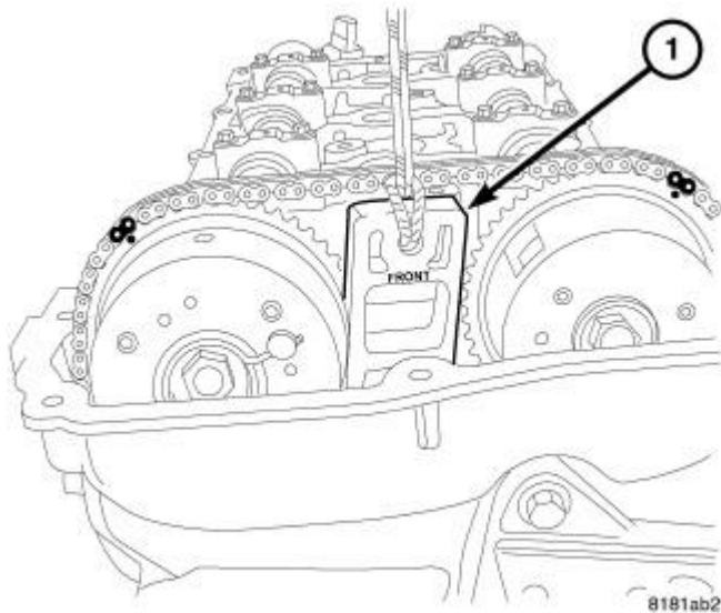
Fig. 157: Inserting Wedge 9701 Between Camshaft Phasers Courtesy of CHRYSLER LLC
