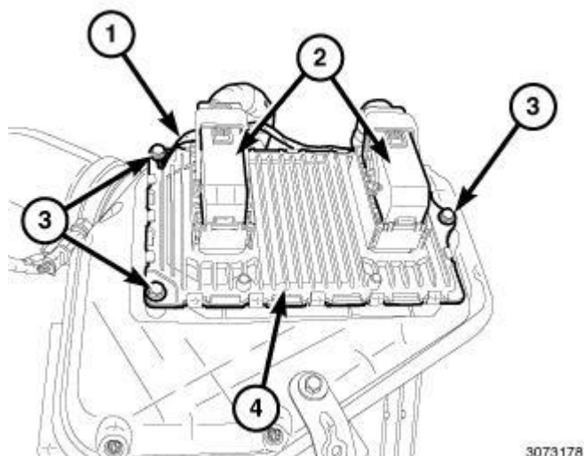
Fig. 332: Electrical Connectors, PCM, Three Mounting Bolts & Ground Wire Courtesy of CHRYSLER LLC
