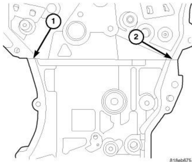
Fig. 381: Applying Mopar® Engine Sealant RTV (Or Equivalent) At Cylinder Head To Block Parting Line
