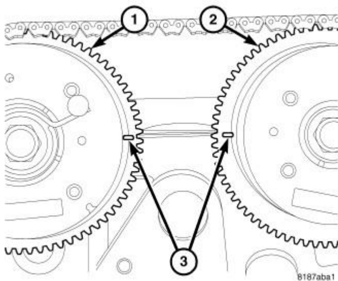
Fig. 159: Camshaft Timing Courtesy of CHRYSLER LLC
