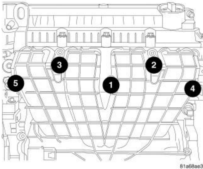
Fig. 117: Intake Manifold Retaining Bolts Torque Sequence Courtesy of CHRYSLER LLC
