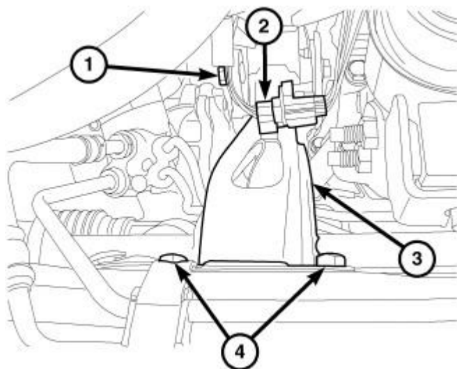
Fig. 252: Rear Mount Through Bolt, Oxygen Sensor Connector, Rear Mount & Rear Mount Retaining Bolts
