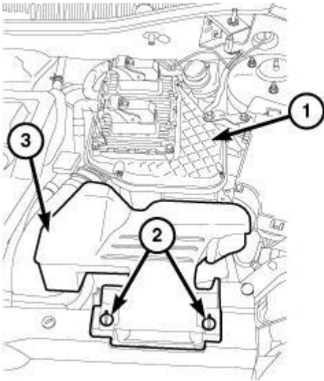
Fig. 56: Retainers, Fresh Air Inlet Duct & Air Cleaner Body Courtesy of CHRYSLER LLC
