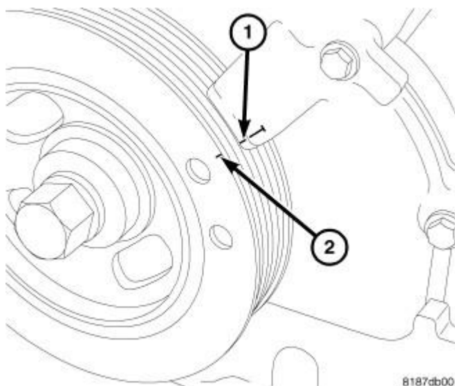
Fig. 349: Setting Engine To Top Dead Center Courtesy of CHRYSLER LLC
