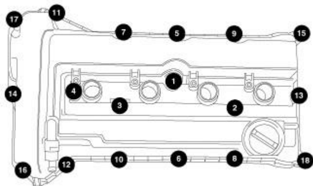
Fig. 173: Cylinder Head Cover Bolts Torque Sequence Courtesy of CHRYSLER LLC
