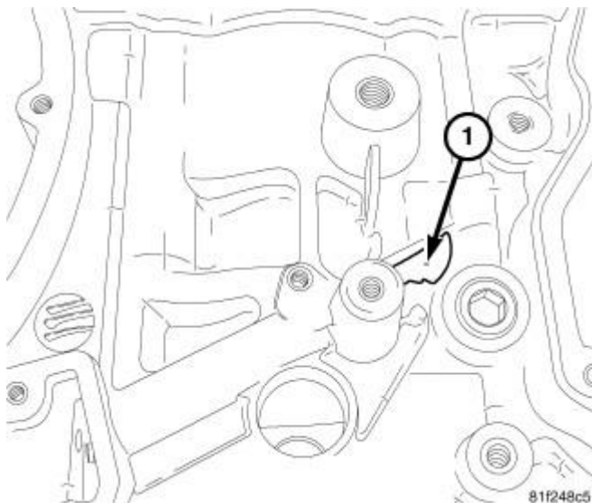
Fig. 261: Oil Hole
