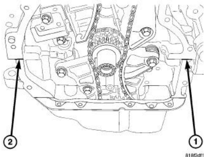
Fig. 382: Applying Mopar® Engine Sealant RTV (Or Equivalent) At Ladder Frame To Block Parting Line
