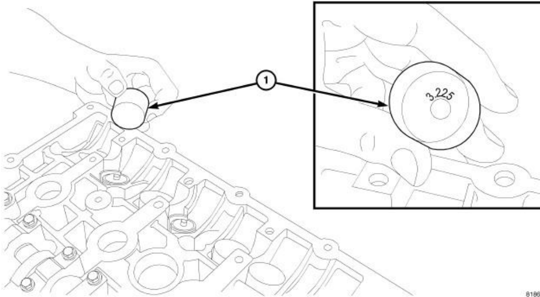
Fig. 134: Tappet Identification
