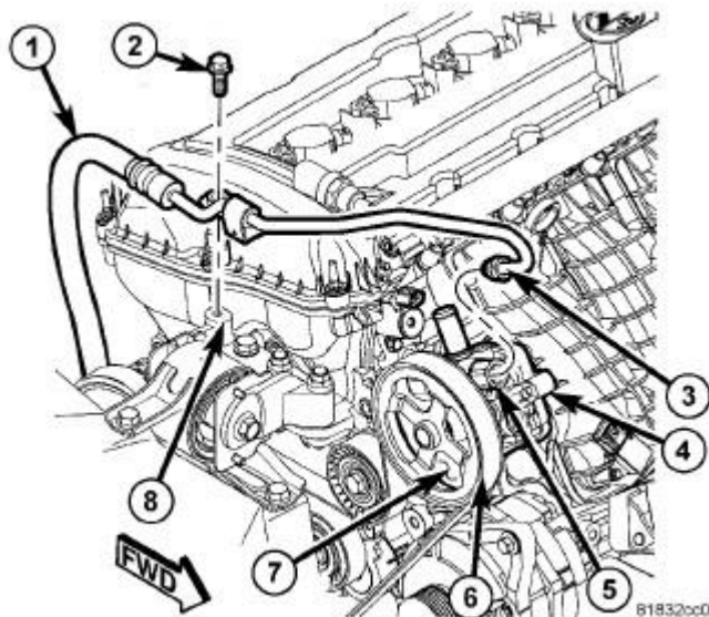
Fig. 73: Pressure Hose Courtesy of CHRYSLER LLC
