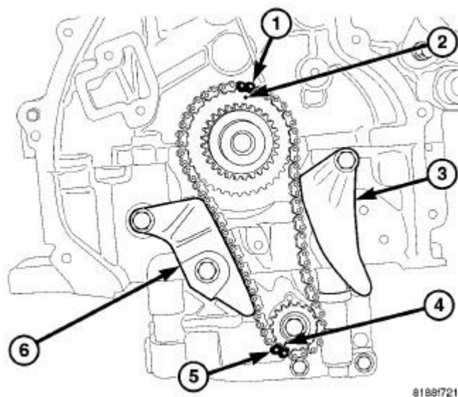
Fig. 309: Balance Shaft Module Timing Courtesy of CHRYSLER LLC
