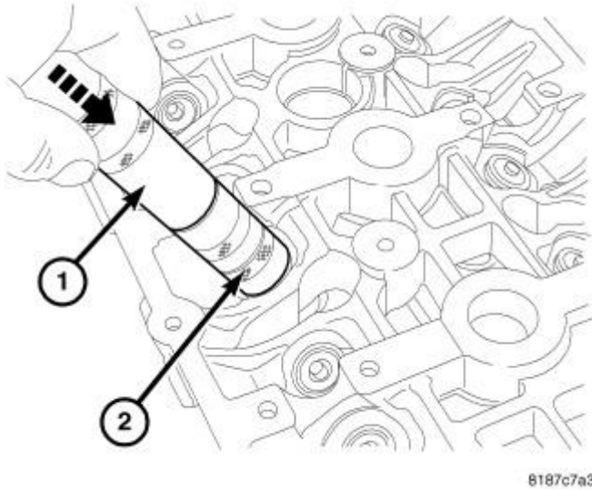
Fig. 179: Valve Installation Courtesy of CHRYSLER LLC
