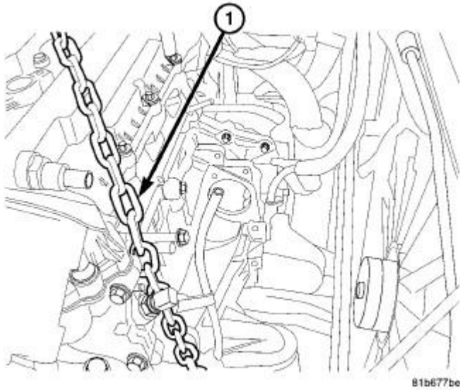
Fig. 31: Identifying Lift Chain Courtesy of CHRYSLER LLC
