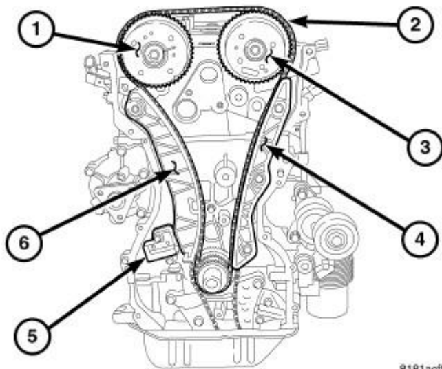
Fig. 114: Removing/Installing Timing Chain, Tensioner, & Guides
