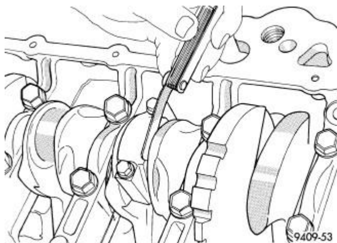
Fig. 231: Connecting Rod Side Clearance Courtesy of CHRYSLER LLC
