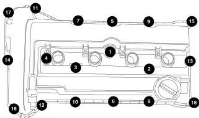
Fig. 128: Cylinder Head Cover Bolt Torque Sequence
