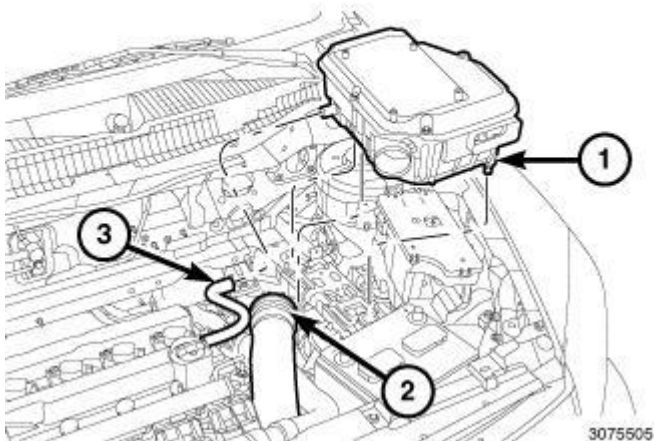
Fig. 65: Air Cleaner Body, Air Inlet Tube & Make-Up Air Hose Courtesy of CHRYSLER LLC
