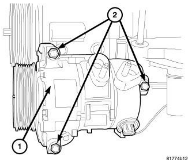
Fig. 317: Removing/Installing A/C Compressor Courtesy of CHRYSLER LLC
