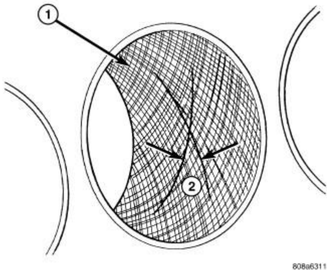
Fig. 182: Cylinder Bore Cross-Hatch Pattern Courtesy of CHRYSLER LLC
