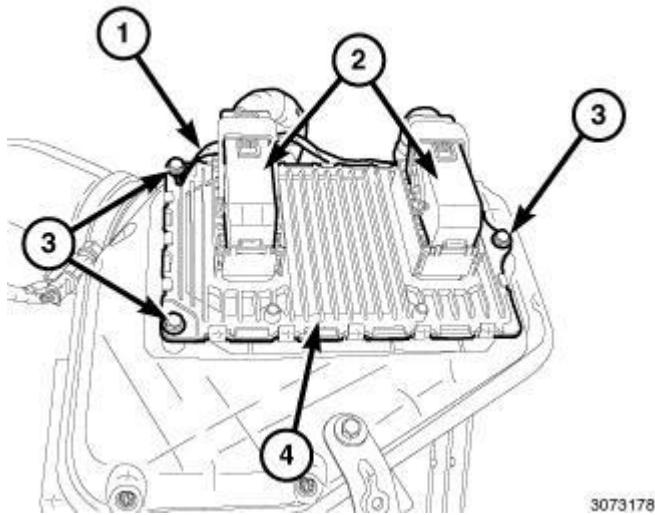
Fig. 63: Electrical Connectors, PCM, Three Mounting Bolts & Ground Wire Courtesy of CHRYSLER LLC
