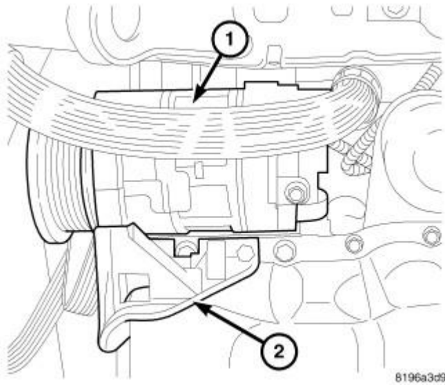
Fig. 294: A/C Compressor
