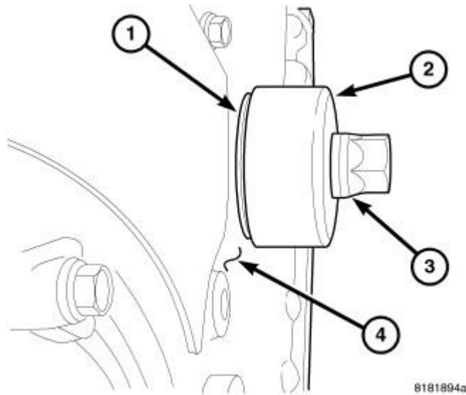
Fig. 235: Installing Front Seal Courtesy of CHRYSLER LLC
