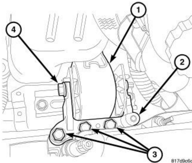
Fig. 28: Right Engine Mount Courtesy of CHRYSLER LLC
