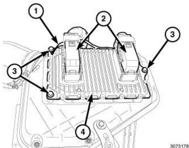
Fig. 345: Electrical Connectors, PCM, Three Mounting Bolts & Ground Wire
