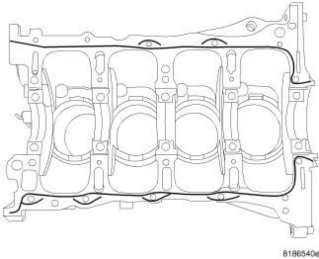
Fig. 218: Sealing Ladder Frame Courtesy of CHRYSLER LLC
