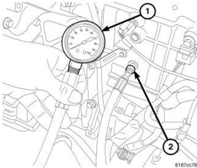
Fig. 263: Oil Pressure Gauge
