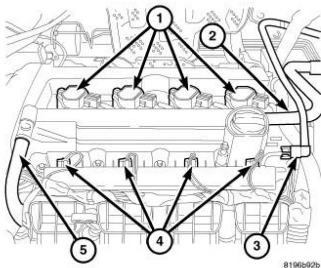
Fig. 16: Coil Connector Courtesy of CHRYSLER LLC
