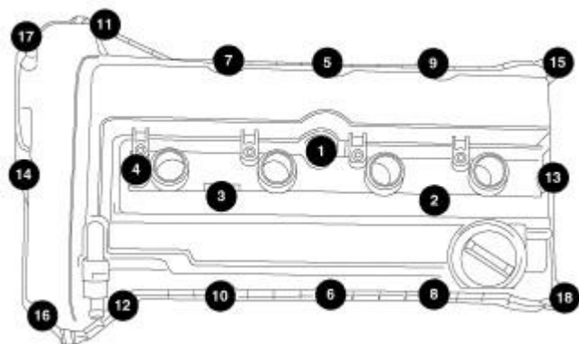
Fig. 115: Cylinder Head Cover Bolt Torque Sequence Courtesy of CHRYSLER LLC
