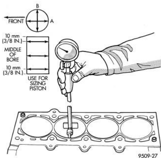
Fig. 183: Checking Cylinder Bore Size
