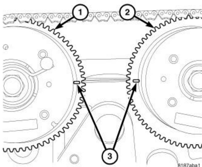
Fig. 111: Camshaft Timing Courtesy of CHRYSLER LLC
