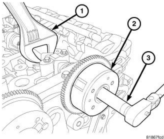
Fig. 127: Cam Phaser Installation Courtesy of CHRYSLER LLC
