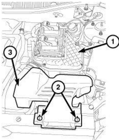
Fig. 61: Retainers, Fresh Air Inlet Duct & Air Cleaner Body Courtesy of CHRYSLER LLC
