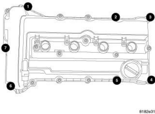
Fig. 167: Cylinder Head Stud Installation Sequence Courtesy of CHRYSLER LLC
