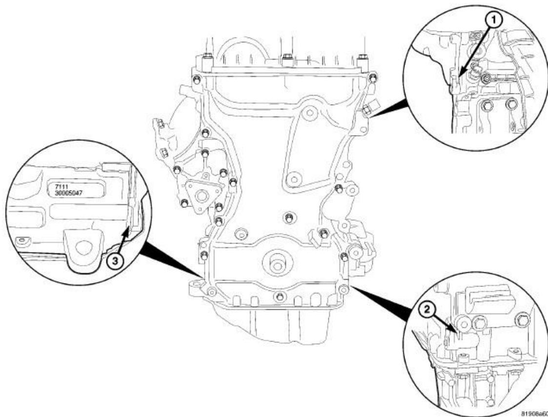
Fig. 85: Timing Chain Cover Pry Points Courtesy of CHRYSLER LLC
