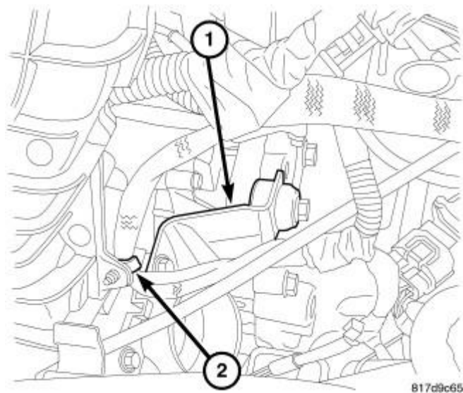
Fig. 91: Throttle Body Support Courtesy of CHRYSLER LLC
