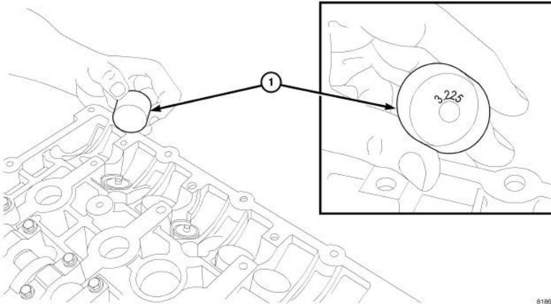
Fig. 130: Tappet Identification
