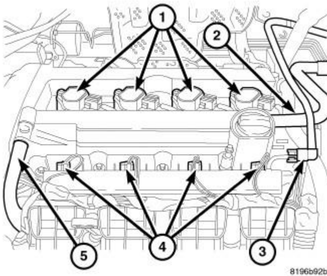
Fig. 343: Coil Connector Courtesy of CHRYSLER LLC
