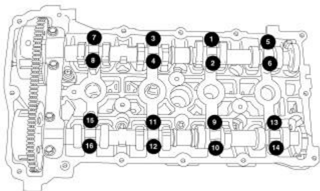
Fig. 154: Removing/Installing Intake & Exhaust Camshaft Bearing Caps - Torque Sequence Courtesy of CHRYSLER LLC
