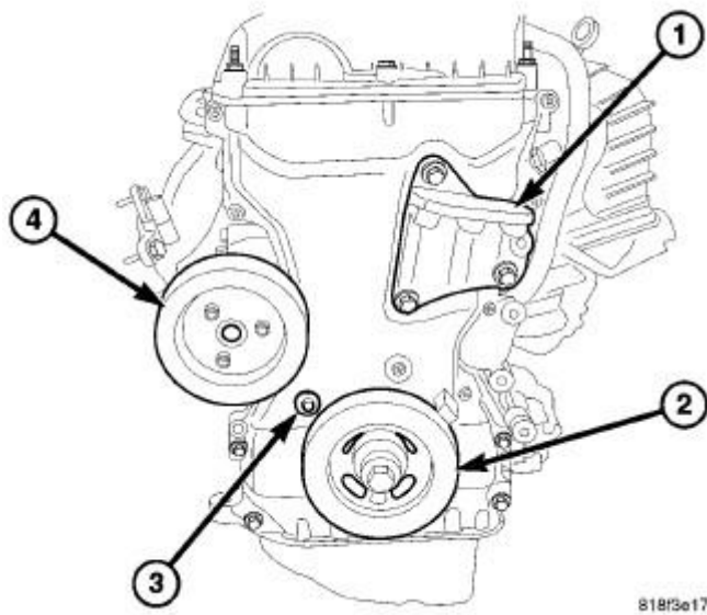
Fig. 374: Engine Front Courtesy of CHRYSLER LLC
