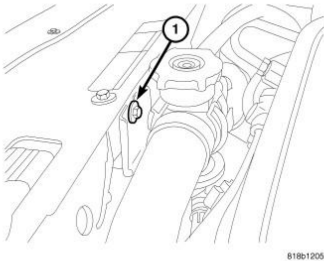
Fig. 118: Radiator Hose Support Courtesy of CHRYSLER LLC
