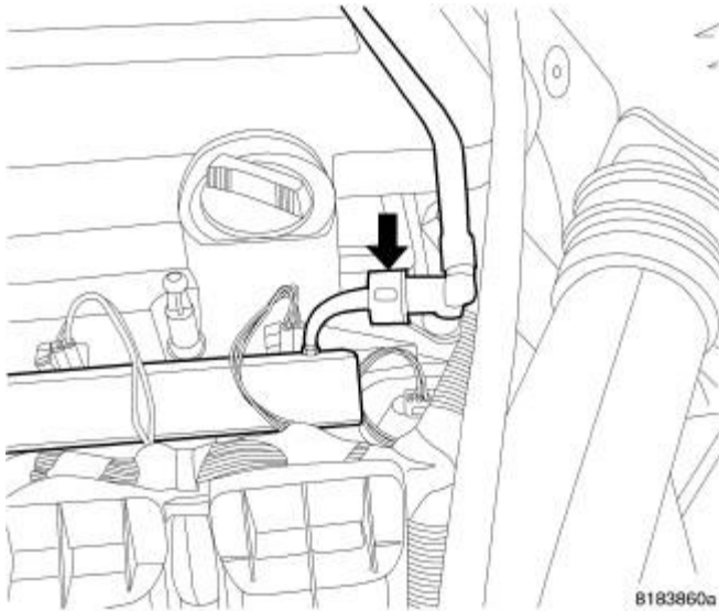
Fig. 87: Disconnecting/Connecting Fuel Line At Fuel Rail Courtesy of CHRYSLER LLC
