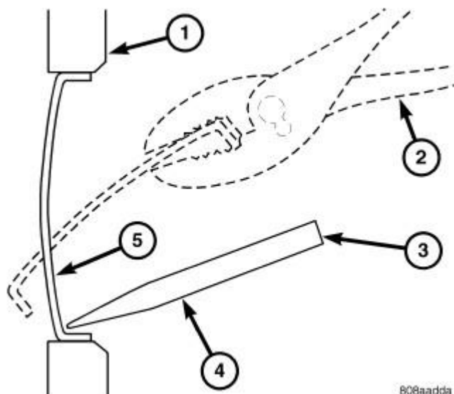
Fig. 5: Core Hole Plug Removal Courtesy of CHRYSLER LLC
