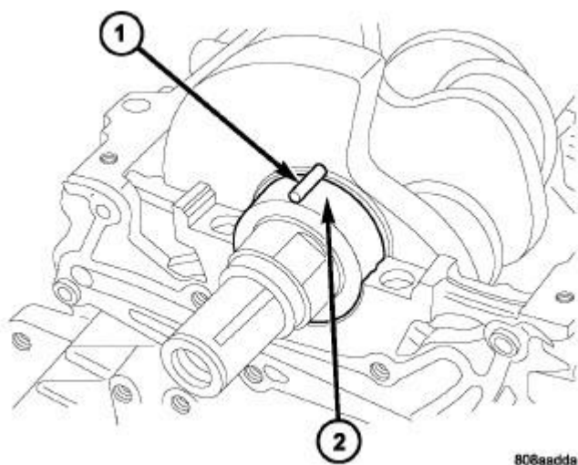
Fig. 6: Plastigage Placed in Lower Shell-Typical Courtesy of CHRYSLER LLC
