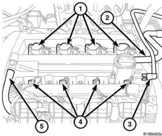
Fig. 46: Coil Connector Courtesy of CHRYSLER LLC
