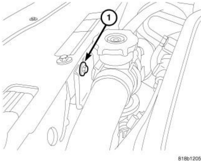
Fig. 340: Radiator Hose Support Courtesy of CHRYSLER LLC
