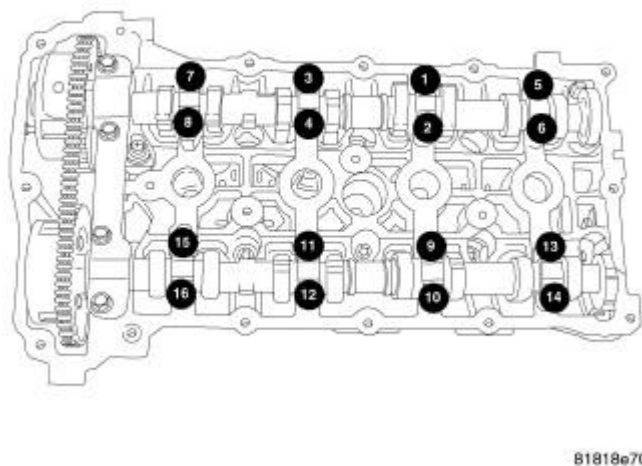
Fig. 112: Removing/Installing Intake & Exhaust Camshaft Bearing Caps - Torque Sequence
