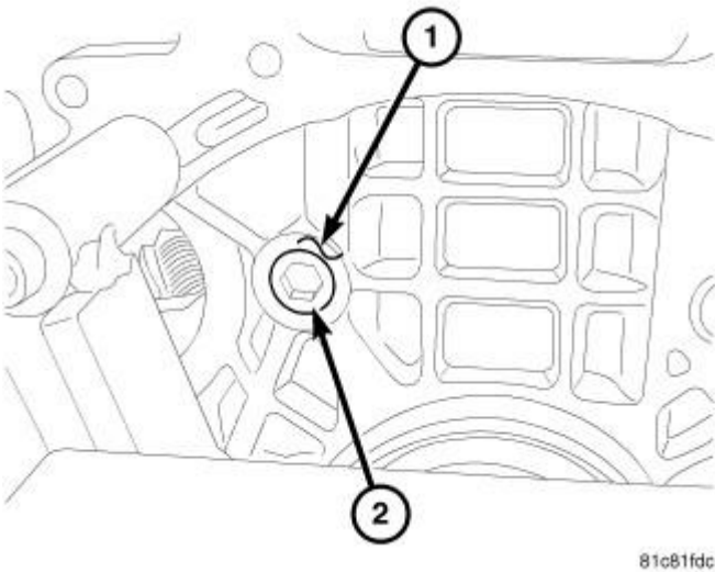
Fig. 301: Gallery Plug
