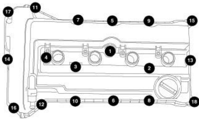
Fig. 132: Cylinder Head Cover Bolts Torque Sequence Courtesy of CHRYSLER LLC
