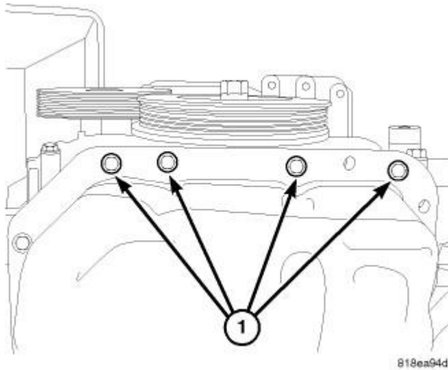
Fig. 375: Timing Chain Cover Lower Bolts Courtesy of CHRYSLER LLC
