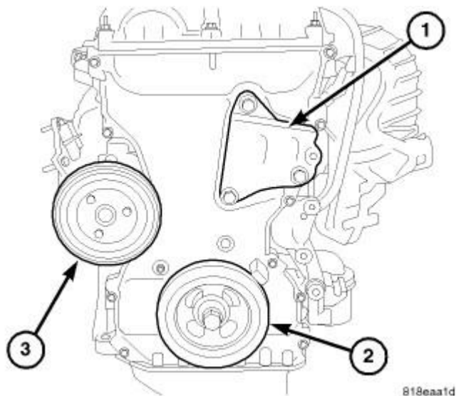
Fig. 194: Right Engine Mount Bracket Courtesy of CHRYSLER LLC
