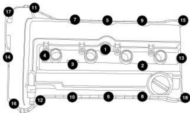
Fig. 80: Cylinder Head Cover Bolt Torque Sequence
