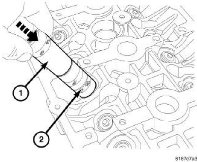
Fig. 182: VALVE INSTALLATION
