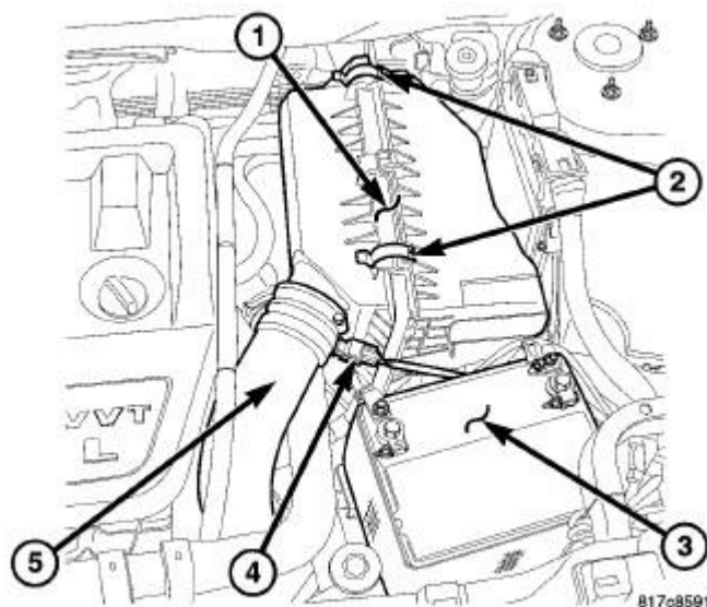
Fig. 342: AIR CLEANER HOUSING
