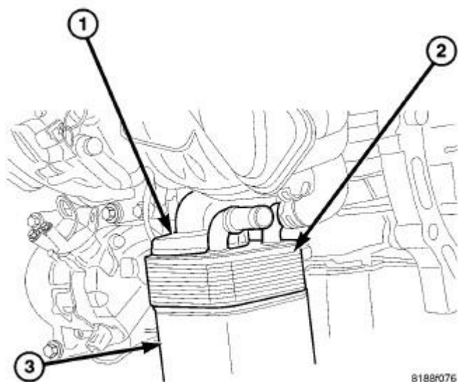
Fig. 283: OIL COOLER
