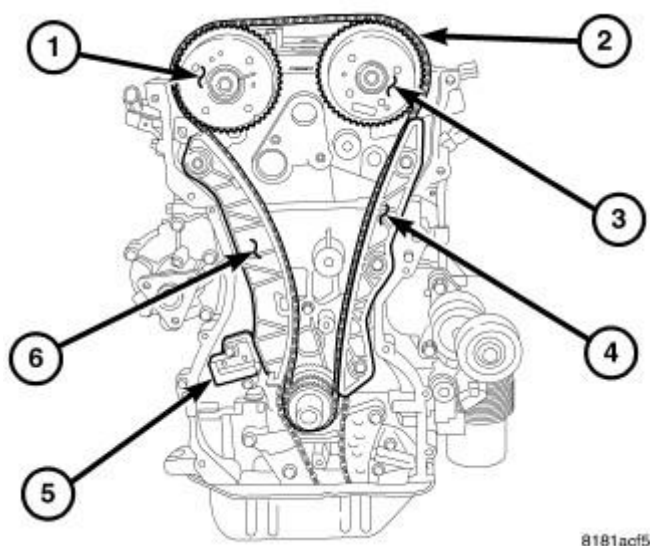
Fig. 344: TIMING DRIVE
