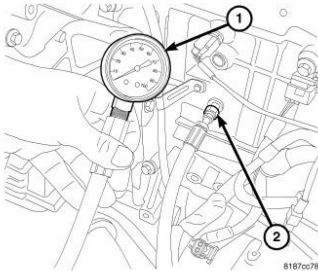
Fig. 269: OIL PRESSURE GAUGE
