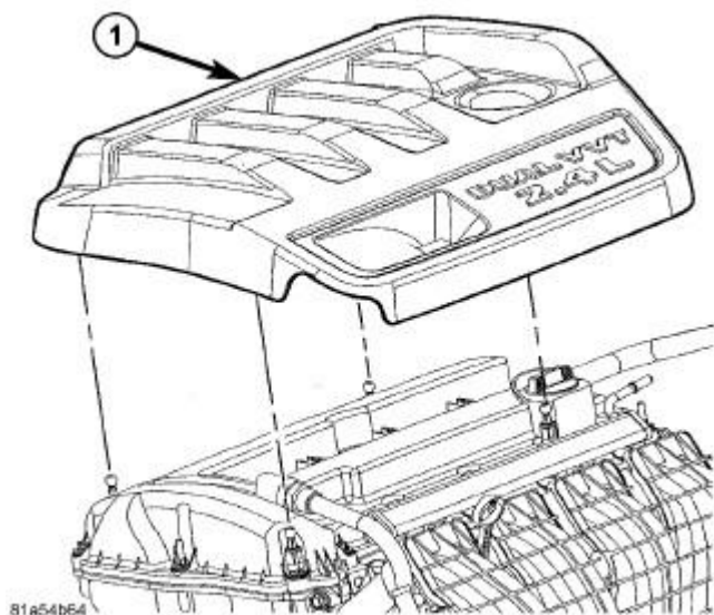
Fig. 75: Engine Cover
