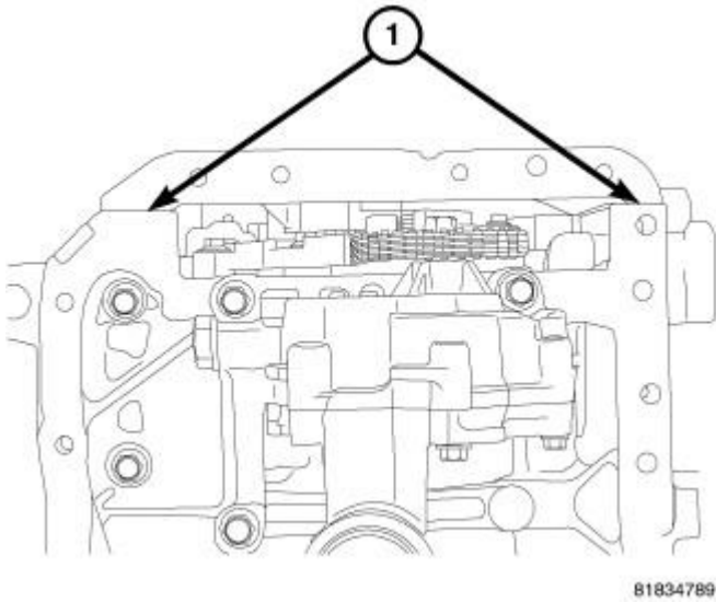
Fig. 298: SEALER LOCATION Courtesy of CHRYSLER LLC
