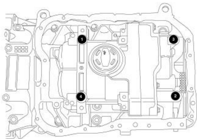
Fig. 312: BSM TORQUE SEQUENCE
