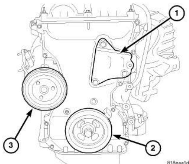
Fig. 197: RIGHT ENGINE MOUNT BRACKET
