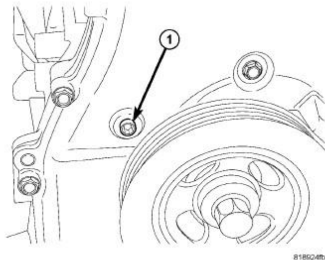
Fig. 144: TENSIONER ACCESS PLUG
