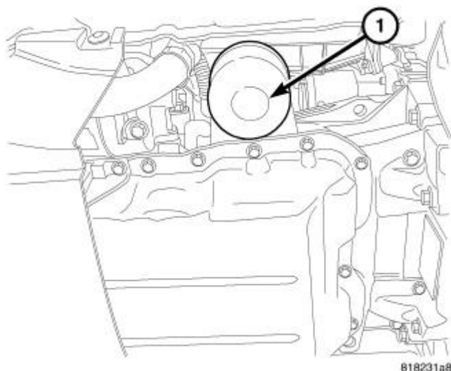
Fig. 287: Oil Filter
