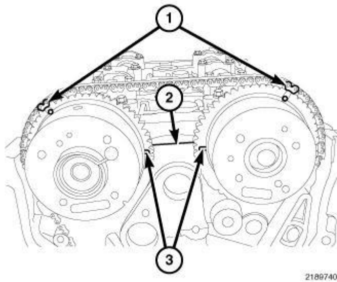
Fig. 154: Timing Chain Timing Marks
