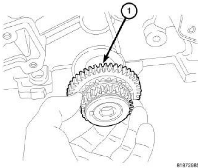
Fig. 199: CRANKSHAFT SPROCKET Courtesy of CHRYSLER LLC
