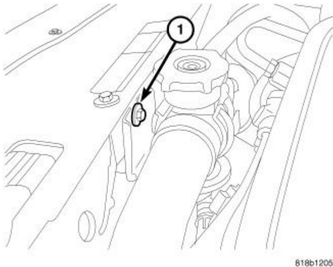
Fig. 97: RADIATOR HOSE SUPPORT
