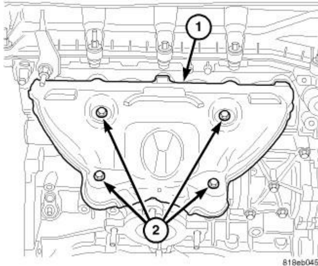
Fig. 324: EXHAUST MANIFOLD HEAT SHIELD Courtesy of CHRYSLER LLC
