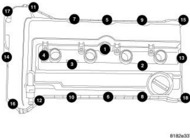
Fig. 168: Cylinder Head Cover Bolt Torque Sequence Courtesy of CHRYSLER LLC
