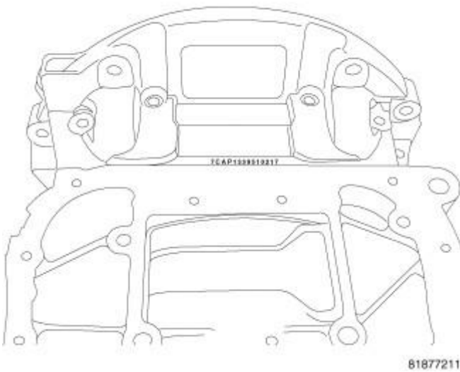
Fig. 184: SERIAL NUMBER Courtesy of CHRYSLER LLC
