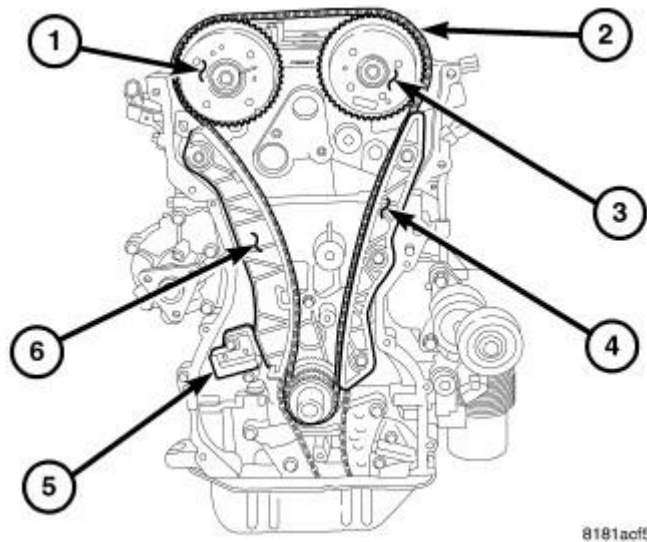
Fig. 349: Timing Drive Courtesy of CHRYSLER LLC
