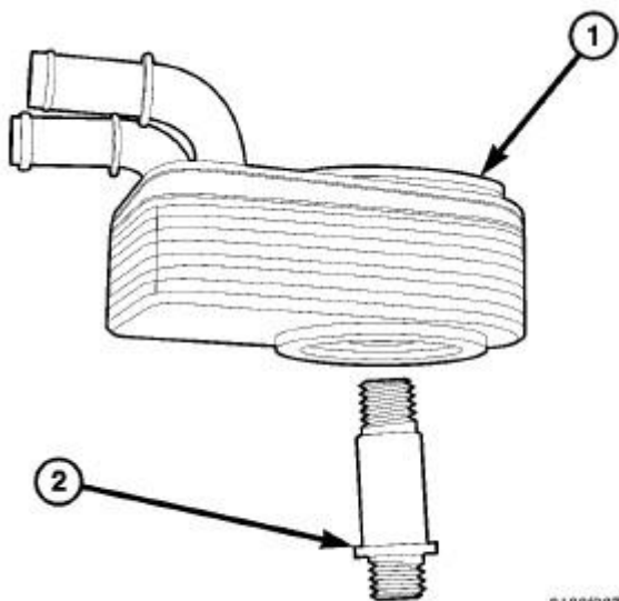
Fig. 284: OIL COOLER MOUNTING
