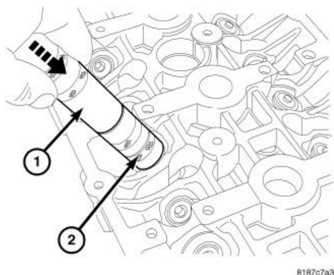
Fig. 180: VALVE INSTALLATION
