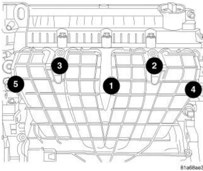
Fig. 16: Removing/Installing Intake Bolts - Torque Sequence Courtesy of CHRYSLER LLC
