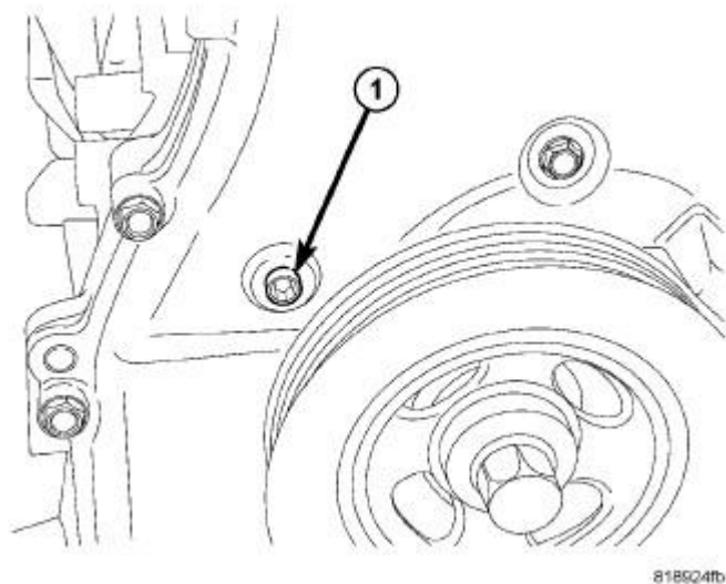
Fig. 161: TENSIONER ACCESS PLUG
