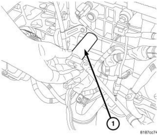
Fig. 268: OIL SENDER
