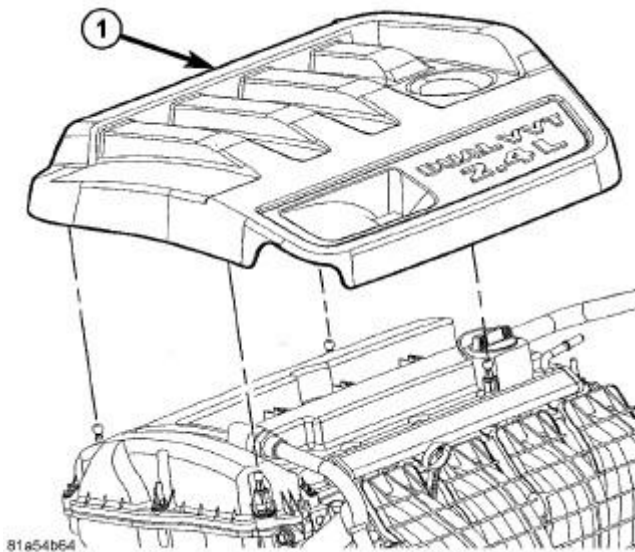
Fig. 141: Engine Cover
