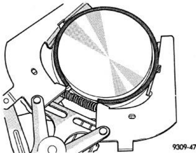
Fig. 121: Upper and Intermediate Rings - Installation Courtesy of CHRYSLER LLC
