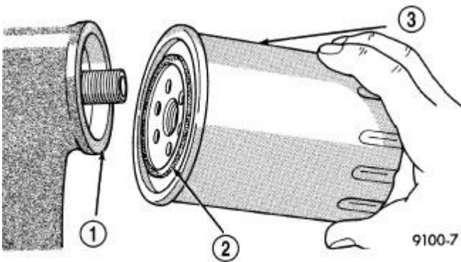
Fig. 146: Oil Filter Sealing Surface-Typical Courtesy of CHRYSLER LLC
