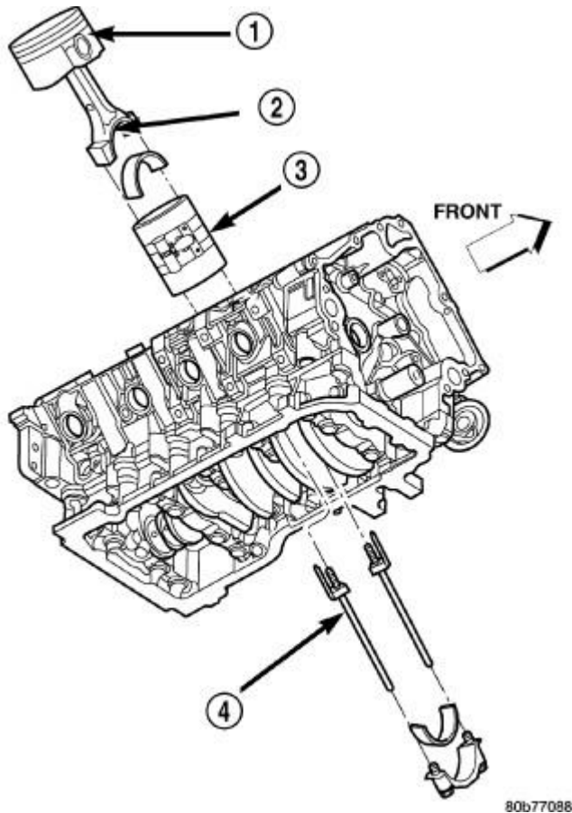
Fig. 131: Piston and Connecting Rod - Installation - Typical Courtesy of CHRYSLER LLC
