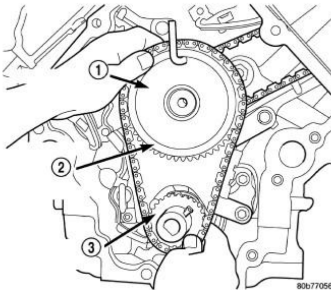
Fig. 190: INSTALLING IDLER GEAR, PRIMARY AND SECONDARY TIMING CHAINS Courtesy of CHRYSLER LLC
