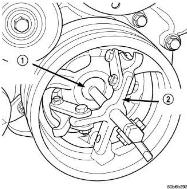
Fig. 133: Crankshaft Damper - Removal
