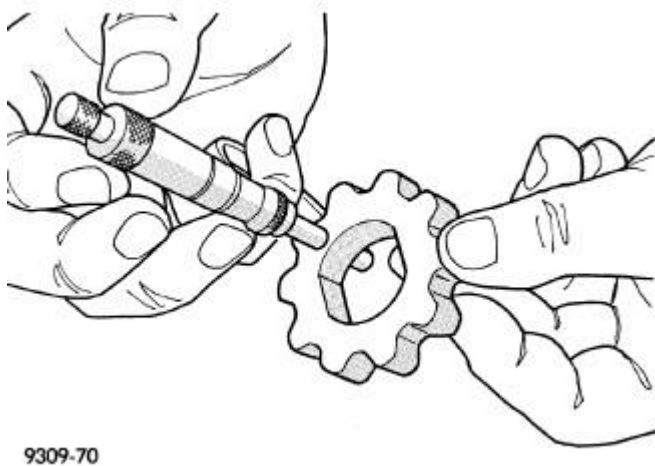
Fig. 153: Measuring Inner Rotor Thickness Courtesy of CHRYSLER LLC
