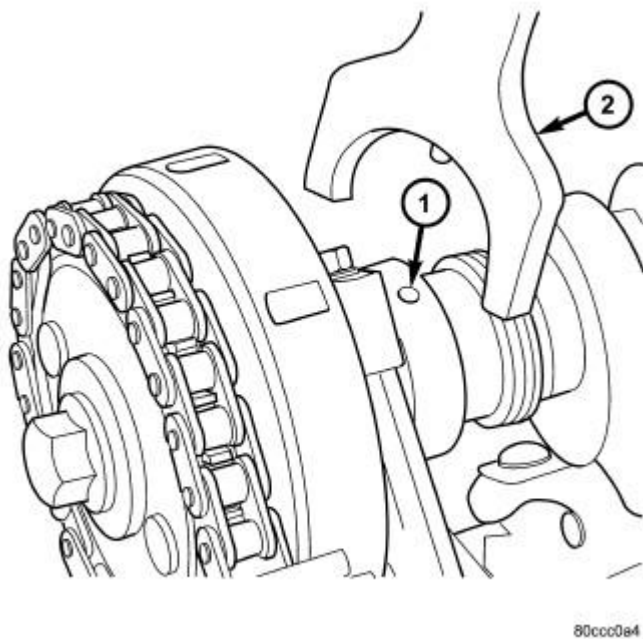
Fig. 56: Special Tool 8428A
