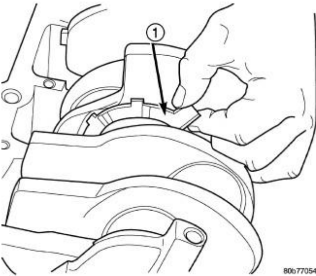
Fig. 107: Crankshaft Thrust Washer Installation Courtesy of CHRYSLER LLC
