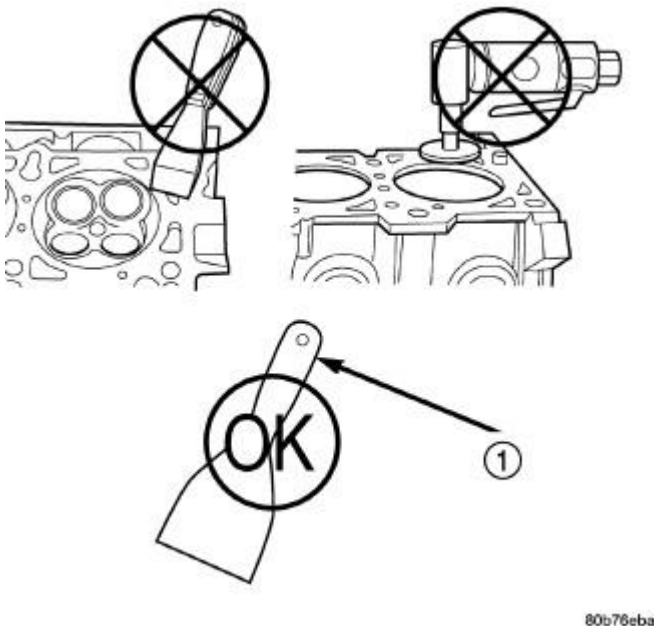
Fig. 76: Proper Tool Usage For Surface Preparation
