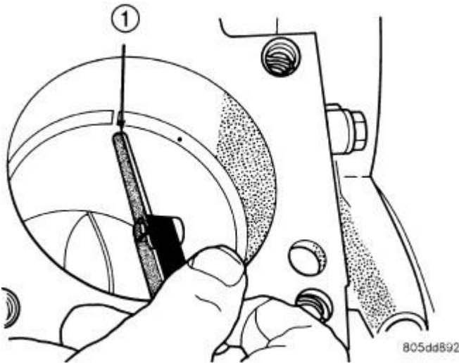
Fig. 119: Ring End Gap Measurement - Typical Courtesy of CHRYSLER LLC
