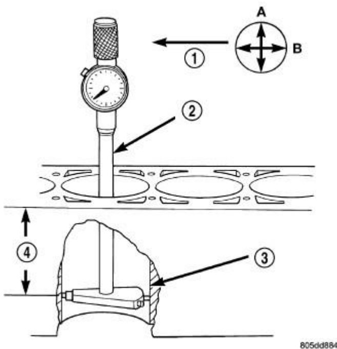
Fig. 101: Bore Gauge - Typical
