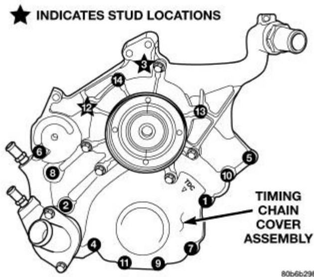
Fig. 200: Timing Chain Cover Fasteners - Typical Courtesy of CHRYSLER LLC
