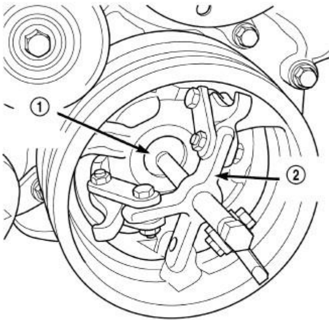
Fig. 110: Crankshaft Damper - Removal
