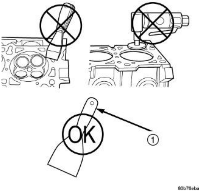
Fig. 53: Proper Tool Usage For Surface Preparation
