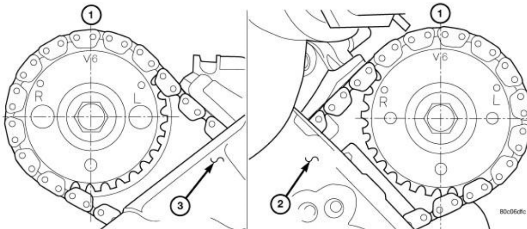
Fig. 192: Camshaft Sprocket V6 Marks Courtesy of CHRYSLER LLC
