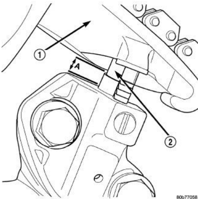
Fig. 176: Measuring Secondary Timing Chains For Wear Courtesy of CHRYSLER LLC
