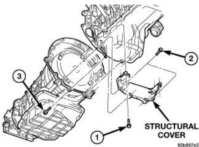
Fig. 104: Structural Cover Courtesy of CHRYSLER LLC
