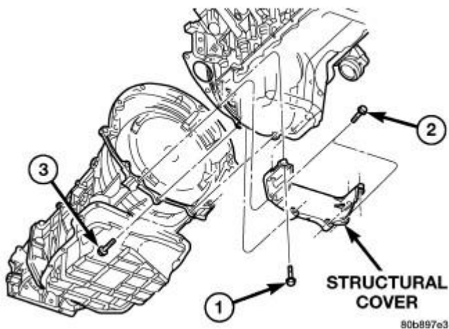
Fig. 103: Structural Cover Courtesy of CHRYSLER LLC
