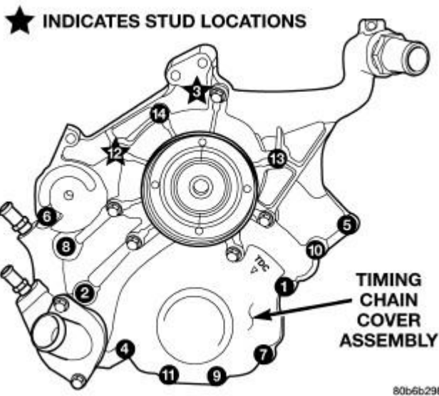
Fig. 198: Timing Chain Cover Fasteners - Typical Courtesy of CHRYSLER LLC
