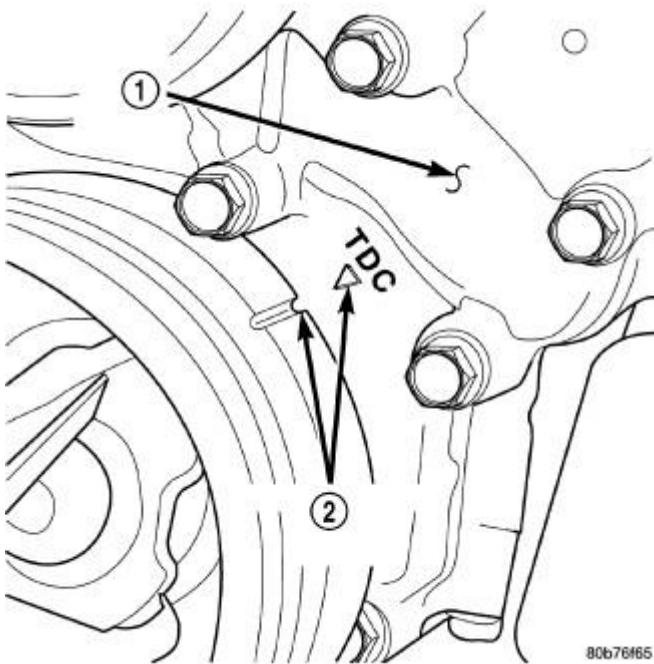
Fig. 177: Engine Top Dead Center (TDC) Indicator Mark
