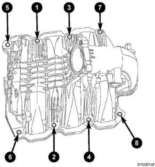
Fig. 164: 3.7L INTAKE TORQUE SEQUENCE Courtesy of CHRYSLER LLC
