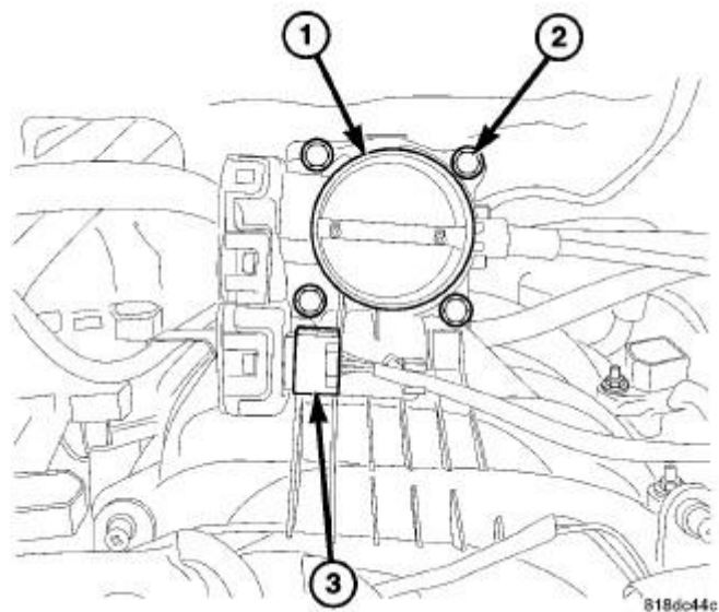
Fig. 172: THROTTLE BODY 3.7L
