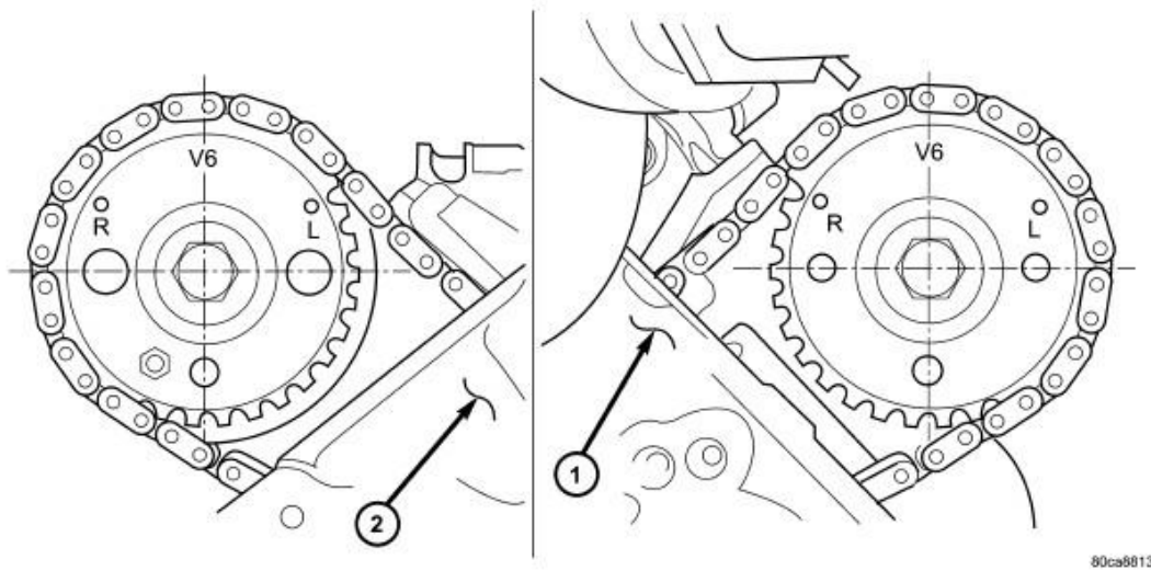
Fig. 183: CAMSHAFT SPROCKET V6 MARKS, (#1 TDC EXHAUST STROKE) Courtesy of CHRYSLER LLC
