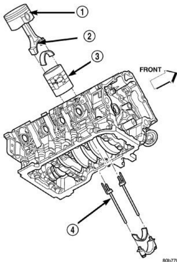
Fig. 126: Piston and Connecting Rod - Installation - Typical Courtesy of CHRYSLER LLC
