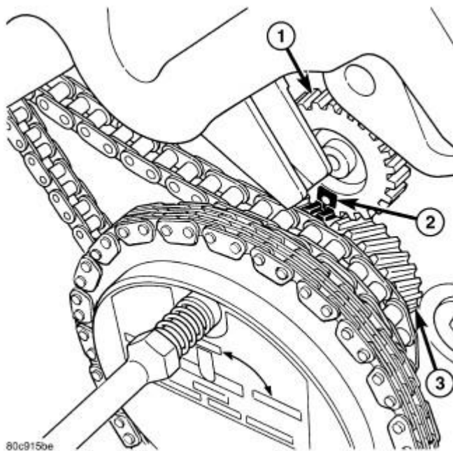
Fig. 191: COUNTERBALANCE SHAFT ALIGNMENT MARKS
