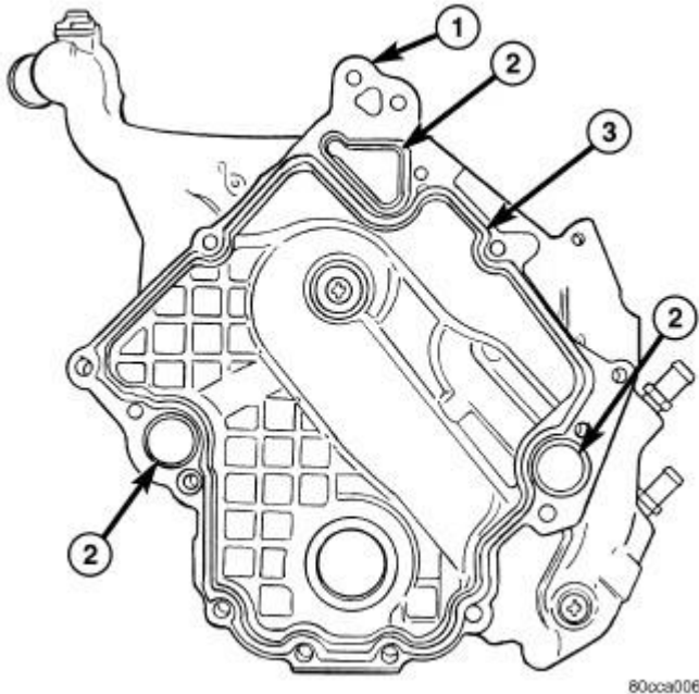
Fig. 199: Timing Cover Sealant Courtesy of CHRYSLER LLC
