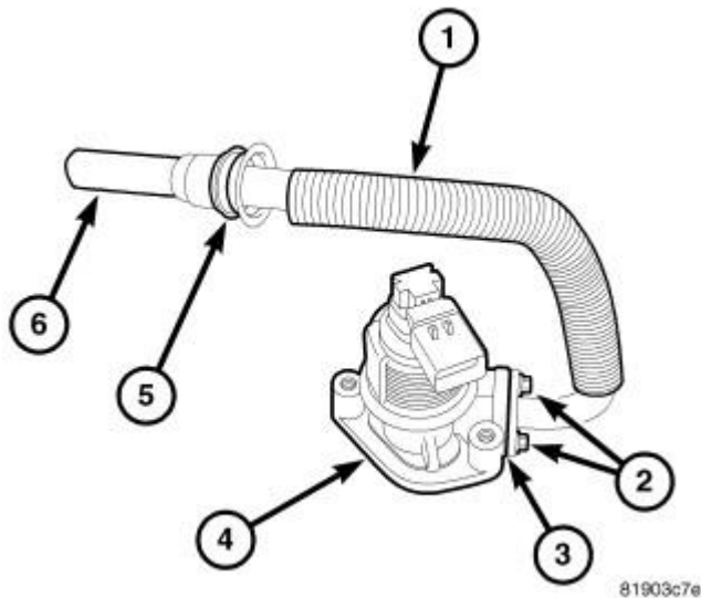
Fig. 173: EGR SOLENOID/TUBE ASSEMBLY Courtesy of CHRYSLER LLC
