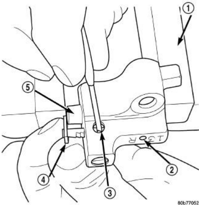
Fig. 189: RESETTING SECONDARY CHAIN TENSIONERS Courtesy of CHRYSLER LLC
