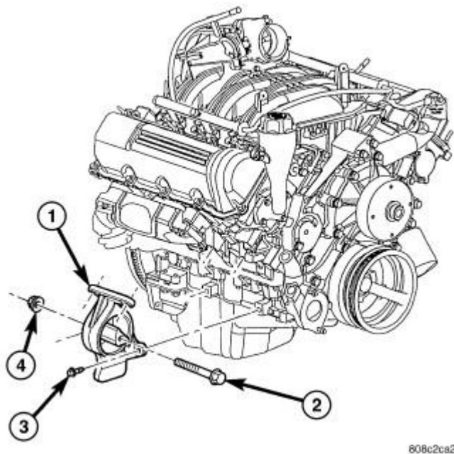
Fig. 140: Engine Insulator Mount 3.7 Right Courtesy of CHRYSLER LLC
