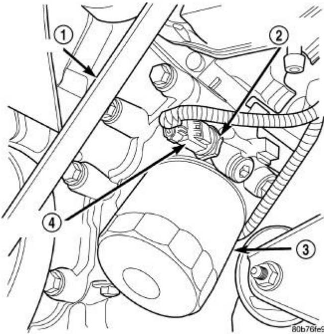
Fig. 159: Identifying Engine Oil Pressure Sensor Courtesy of CHRYSLER LLC
