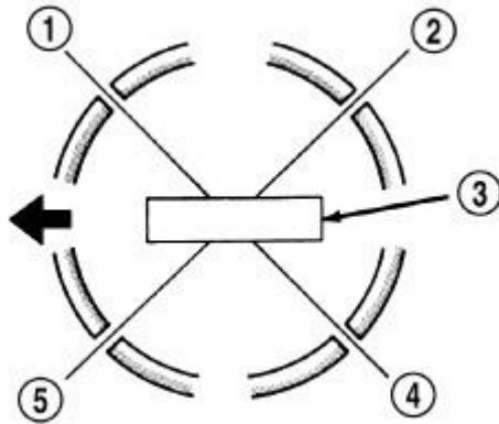
Fig. 122: Piston Ring End Gap Position Courtesy of CHRYSLER LLC
