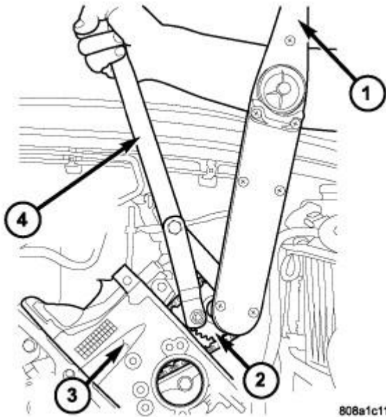
Fig. 193: Tightening Left Side Cam Sprocket Retaining Bolt Courtesy of CHRYSLER LLC
