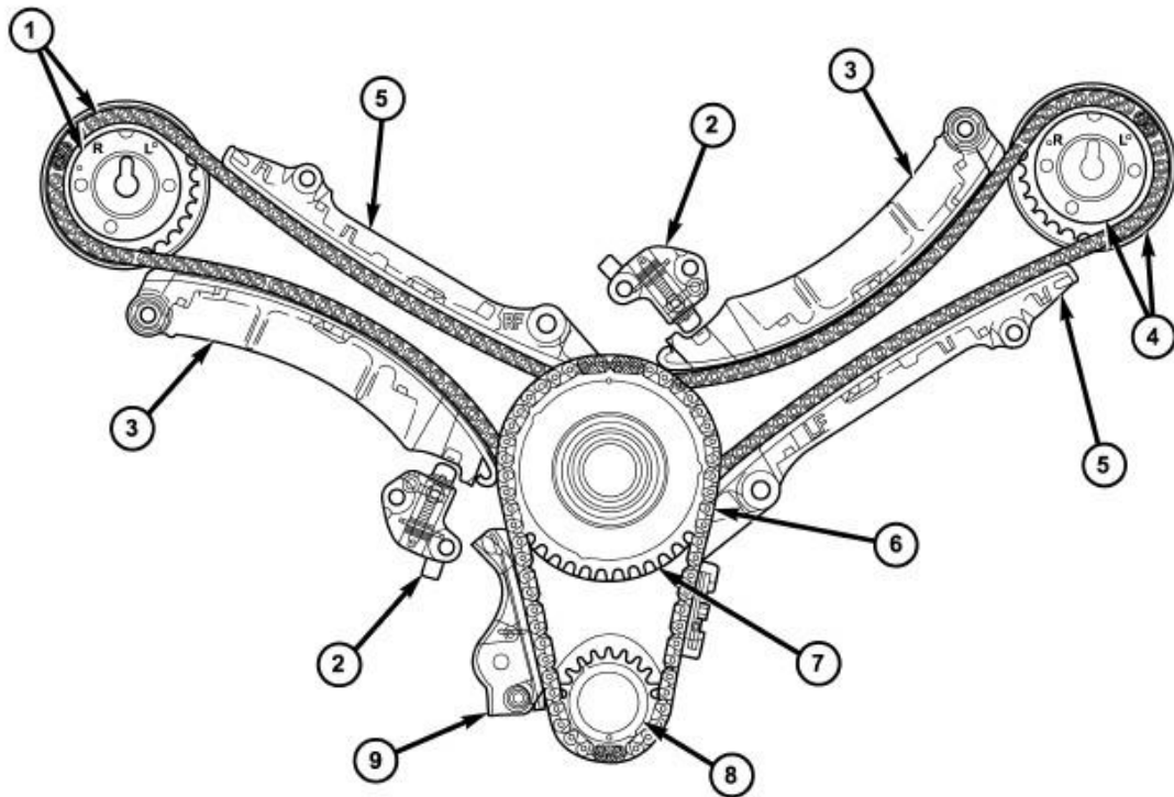
Fig. 175: Timing Drive System Courtesy of CHRYSLER LLC
