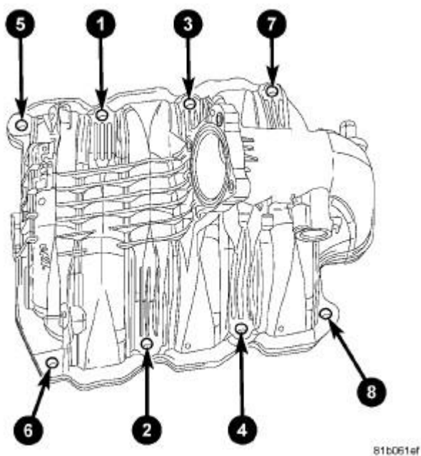
Fig. 170: 3.7L INTAKE TORQUE SEQUENCE Courtesy of CHRYSLER LLC
