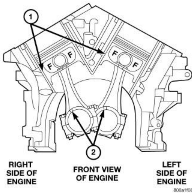
Fig. 132: Piston and Connecting Rod Orientation Courtesy of CHRYSLER LLC
