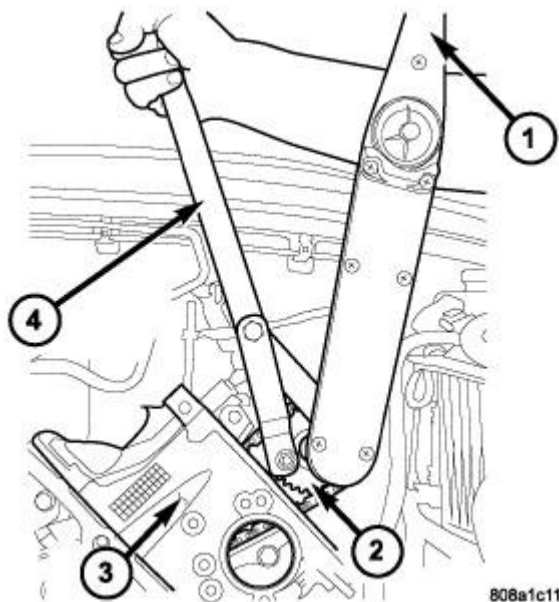
Fig. 91: Tightening Left Side Cam Sprocket Retaining Bolt Courtesy of CHRYSLER LLC
