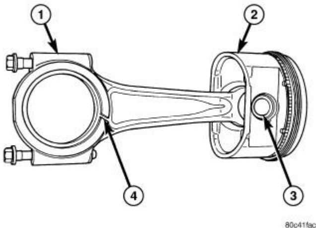
Fig. 123: PISTON AND ROD ASSEMBLY
