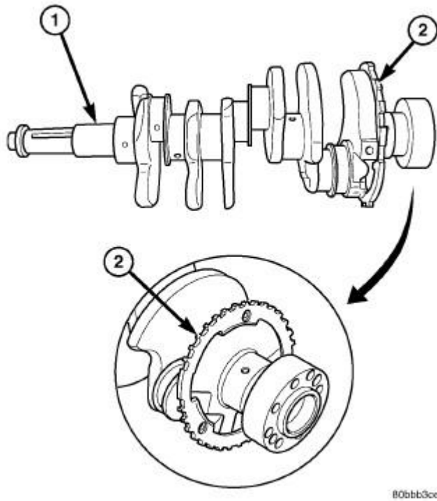
Fig. 105: Crankshaft and Target Ring Courtesy of CHRYSLER LLC
