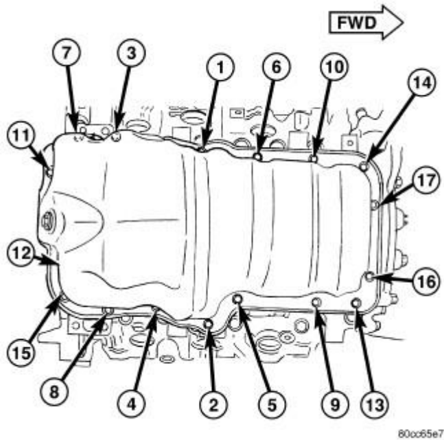
Fig. 150: Oil Pan Mounting Bolt Sequence Courtesy of CHRYSLER LLC
