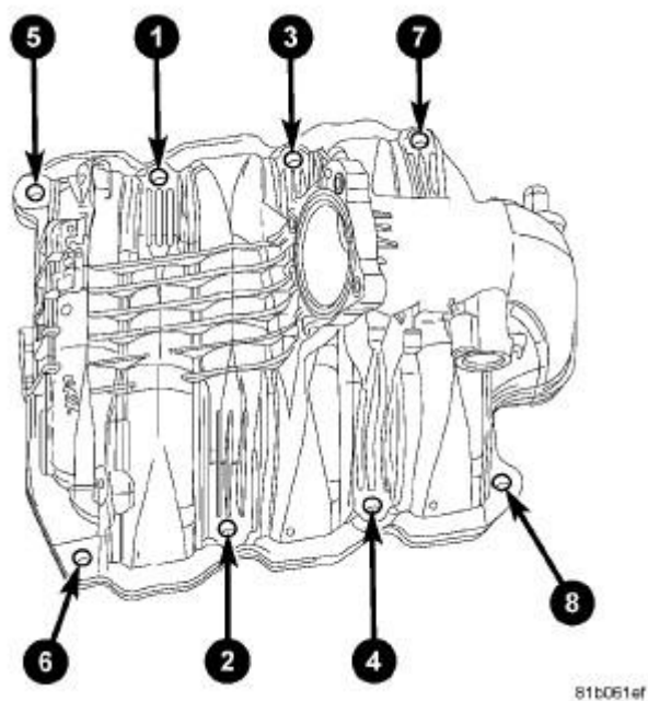
Fig. 171: 3.7L INTAKE TORQUE SEQUENCE
