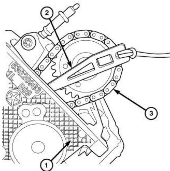
Fig. 180: SECURING TIMING CHAIN TENSIONER USING TIMING CHAIN WEDGE Courtesy of CHRYSLER LLC
