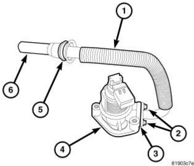
Fig. 168: EGR SOLENOID/TUBE ASSEMBLY
