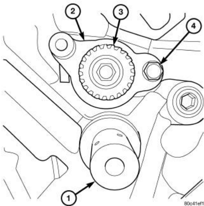
Fig. 115: Counterbalance Shaft Retaining Plate Courtesy of CHRYSLER LLC
