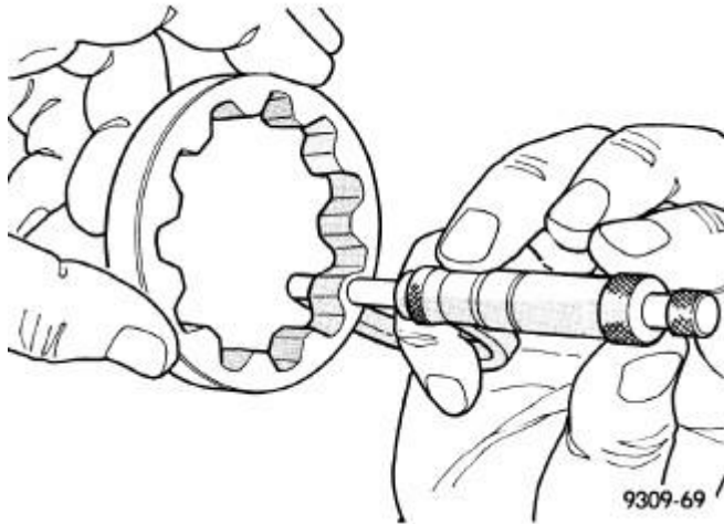
Fig. 152: Measuring Outer Rotor Thickness Courtesy of CHRYSLER LLC
