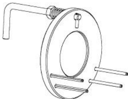
Fig. 34: HOLDER, SECONDARY CAMSHAFT CHAIN - 8429
