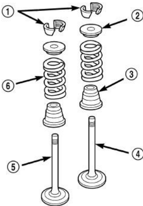
Fig. 64: Valve Assembly Configuration Courtesy of CHRYSLER LLC
