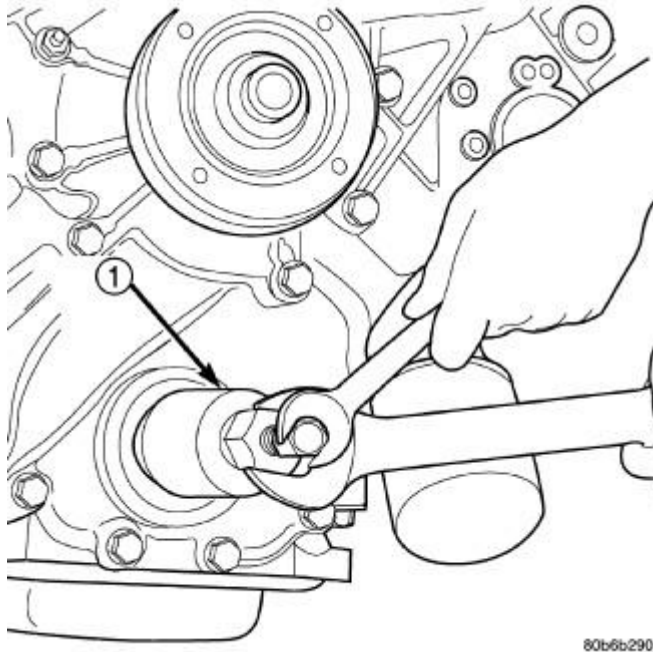
Fig. 134: Crankshaft Front Seal Removal Courtesy of CHRYSLER LLC
