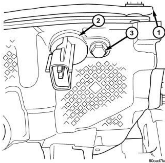
Fig. 187: Camshaft Position Sensor Courtesy of CHRYSLER LLC
