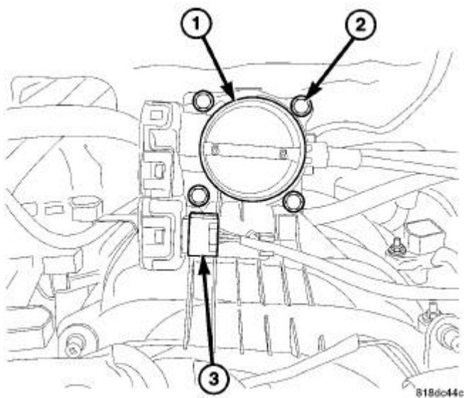
Fig. 169: THROTTLE BODY 3.7L
