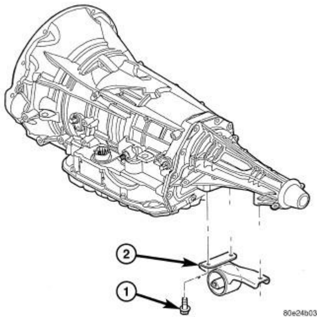
Fig. 142: TRANSMISSION MOUNT - 3.7L 2WD AUTO TRANS Courtesy of CHRYSLER LLC
