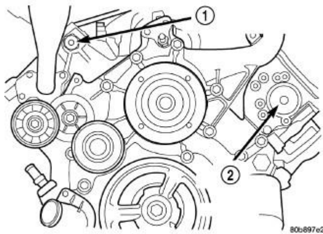
Fig. 185: Cylinder Head Access Plugs Courtesy of CHRYSLER LLC
