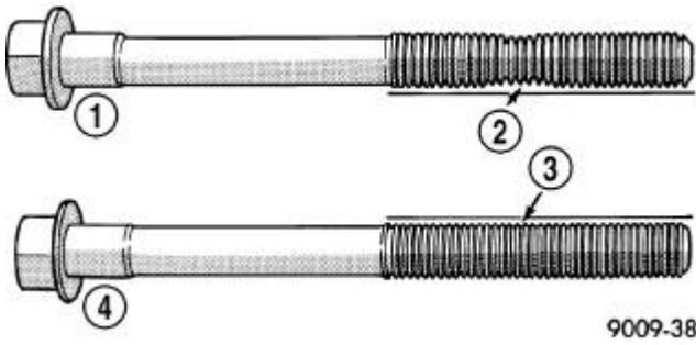
Fig. 52: Checking Cylinder Head Bolts for Stretching (Necking)
