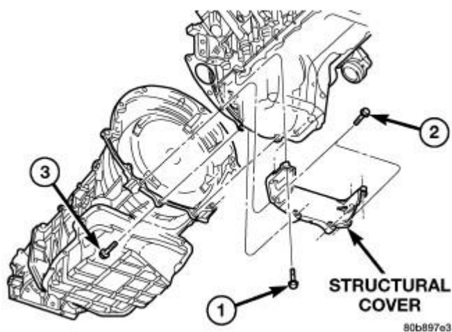
Fig. 79: Structural Cover
