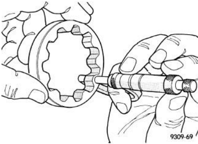
Fig. 128: Measuring Outer Rotor Thickness Courtesy of CHRYSLER LLC
