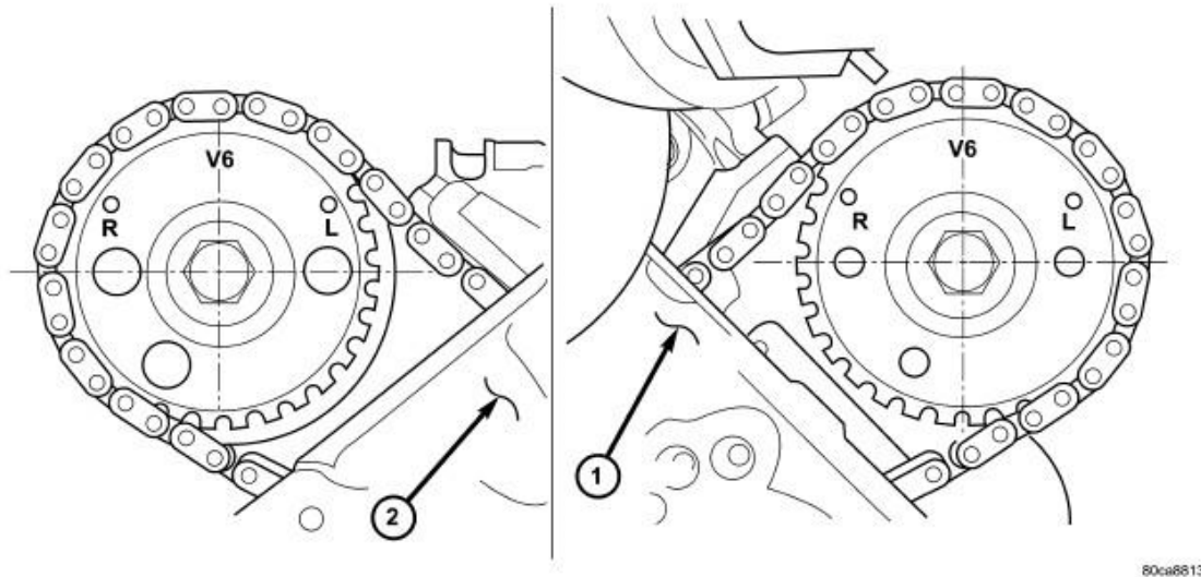
Fig. 158: Camshaft Sprocket V6 Marks (#1 TDC, Exhaust Stroke) Courtesy of CHRYSLER LLC
