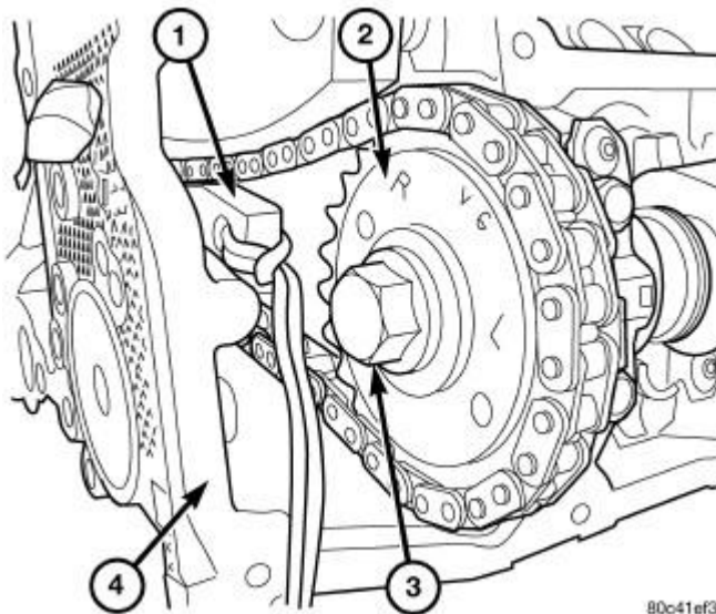
Fig. 29: Timing Chain Tensioners Secured With Timing Chain Wedge Courtesy of CHRYSLER LLC
