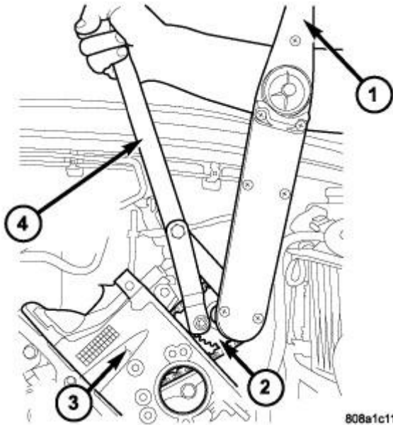
Fig. 169: Tightening Left Side Camshaft Sprocket Bolt Courtesy of CHRYSLER LLC
