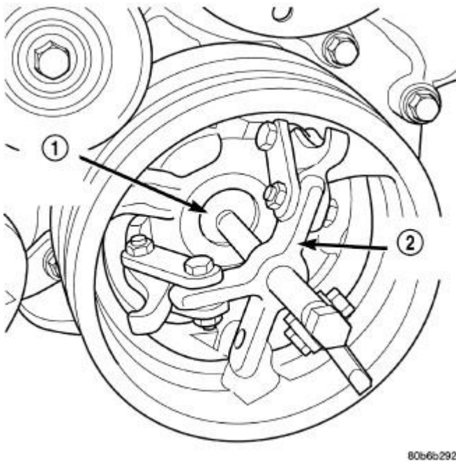
Fig. 109: Removing Crankshaft Damper Courtesy of CHRYSLER LLC
