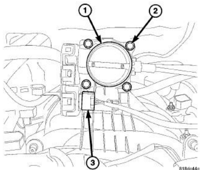
Fig. 145: Throttle Body 3.7L, Mounting Bolts & Connector Courtesy of CHRYSLER LLC
