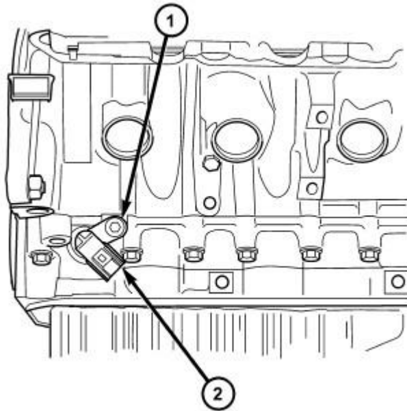
Fig. 17: Crankshaft Position Sensor Courtesy of CHRYSLER LLC
