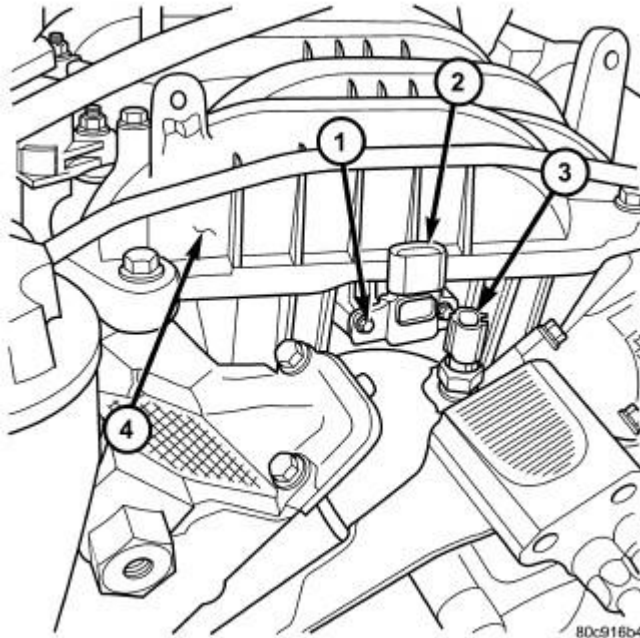
Fig. 143: MAP Sensor, ECT Sensor, Intake Manifold & Screw - 3.7L V-6 Courtesy of CHRYSLER LLC
