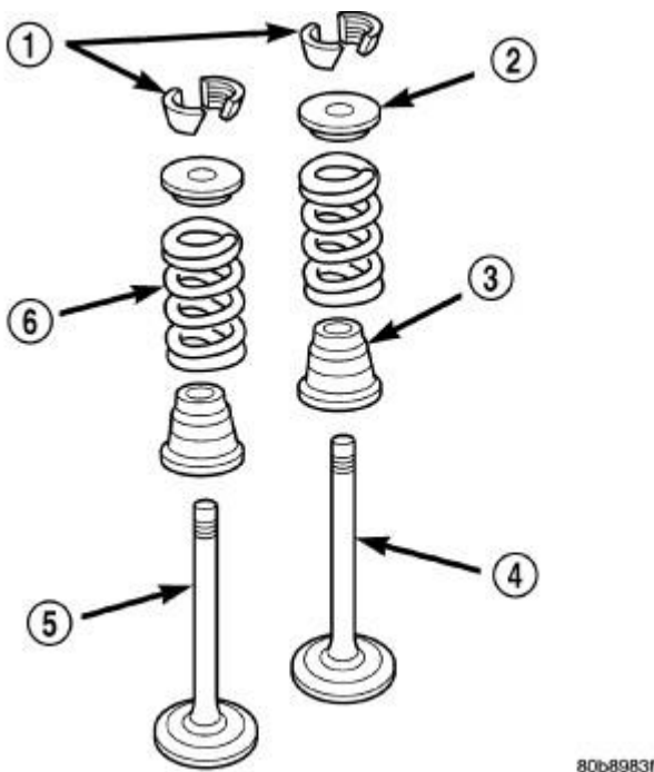
Fig. 69: Valve Assembly Configuration Courtesy of CHRYSLER LLC
