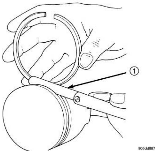
Fig. 95: Measuring Piston Ring Side Clearance Courtesy of CHRYSLER LLC
