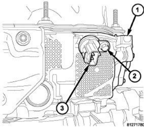
Fig. 66: Camshaft Position Sensor Courtesy of CHRYSLER LLC
