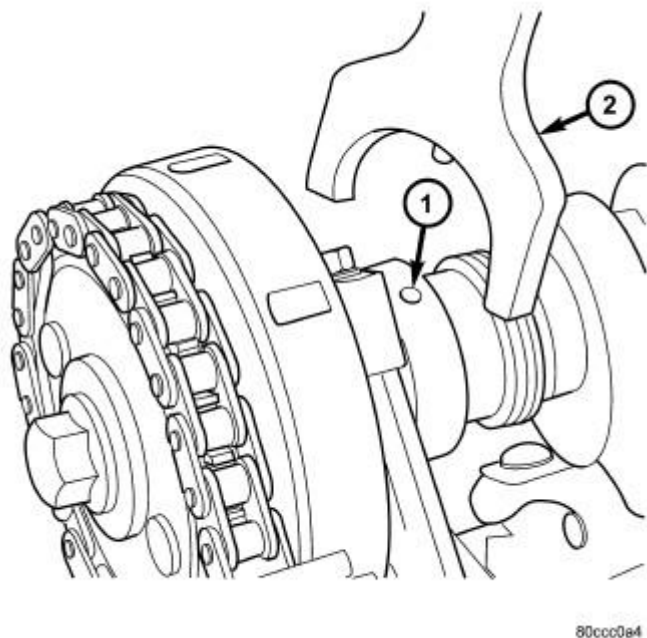
Fig. 63: Camshaft & Camshaft Holder Courtesy of CHRYSLER LLC
