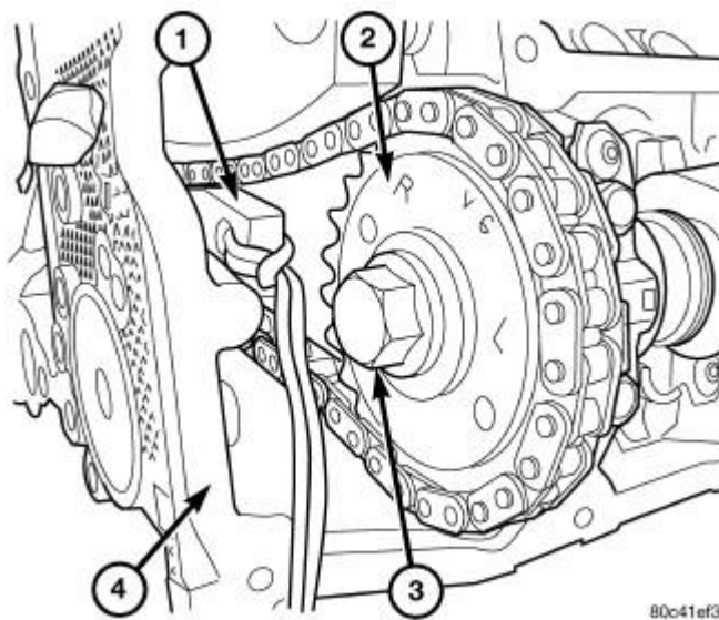
Fig. 57: Timing Chain Tensioners Secured With Timing Chain Wedge Courtesy of CHRYSLER LLC
