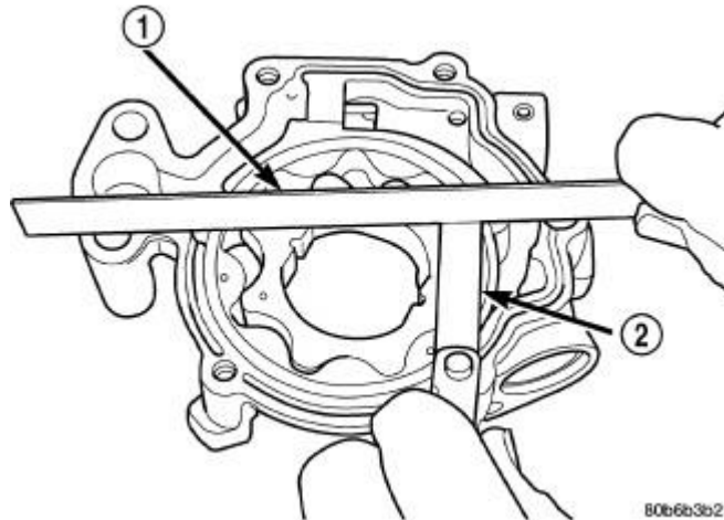
Fig. 132: Measuring Clearance Over Rotors Courtesy of CHRYSLER LLC
