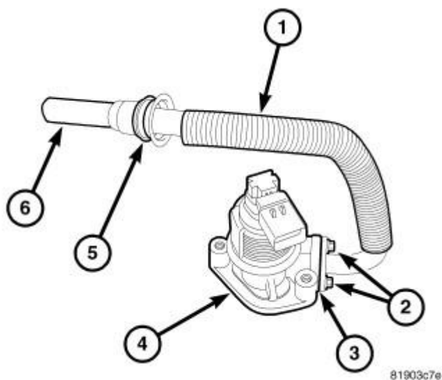
Fig. 144: EGR Solenoid/Tube Assembly Courtesy of CHRYSLER LLC
