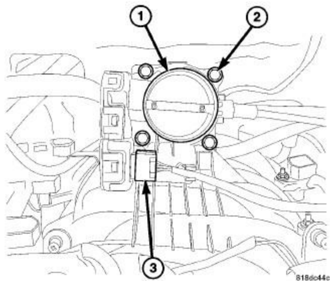
Fig. 148: Throttle Body 3.7L, Mounting Bolts & Connector Courtesy of CHRYSLER LLC
