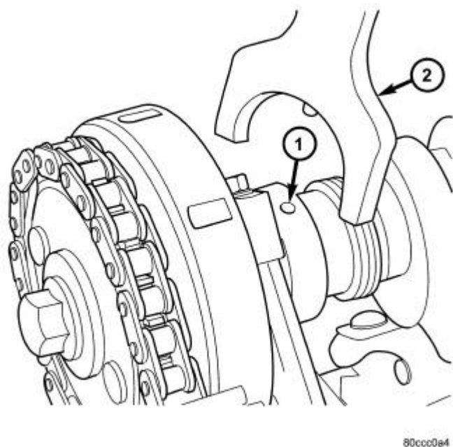
Fig. 32: Camshaft & Camshaft Holder Courtesy of CHRYSLER LLC
