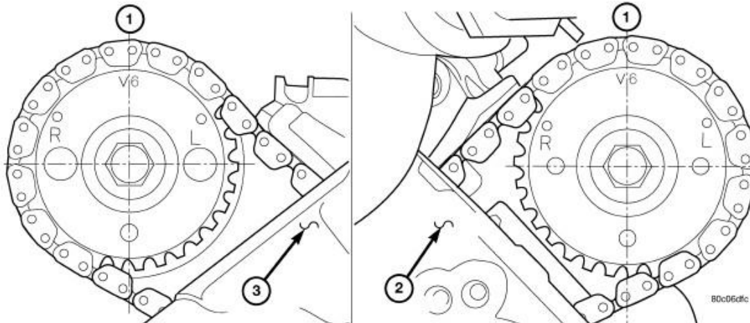
Fig. 55: Camshaft Sprocket V6 Marks Courtesy of CHRYSLER LLC
