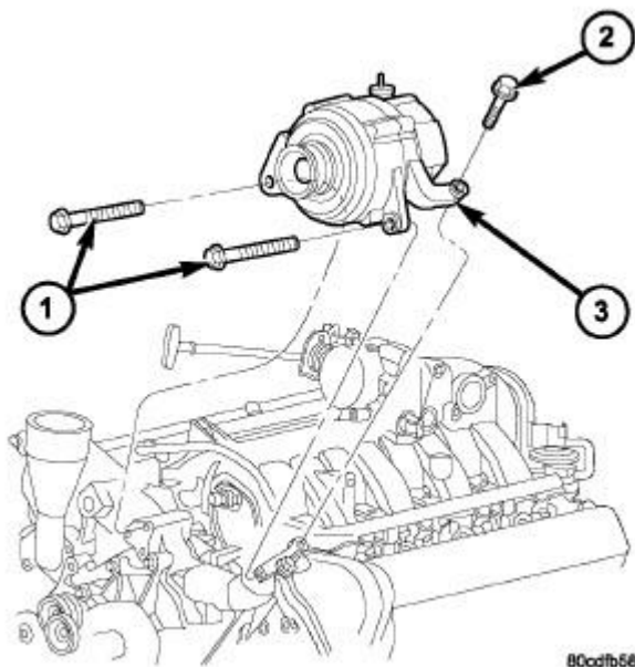
Fig. 18: Removing/Installing Generator - 3.7L/4.7L Courtesy of CHRYSLER LLC
