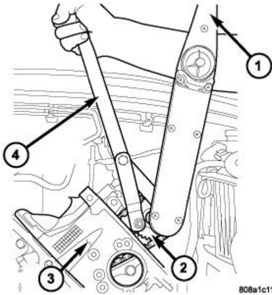
Fig. 33: Tightening Left Side Camshaft Sprocket Bolt Courtesy of CHRYSLER LLC
