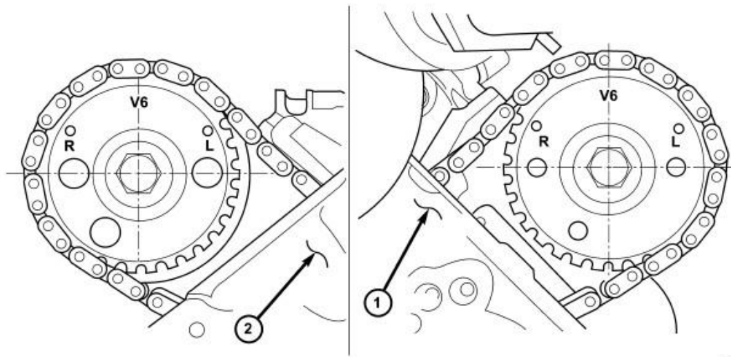
Fig. 22: Camshaft Sprocket V6 Marks (#1 TDC, Exhaust Stroke) Courtesy of CHRYSLER LLC
