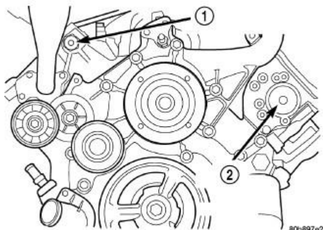
Fig. 53: Access Plugs From Left And Right Cylinder Heads Courtesy of CHRYSLER LLC
