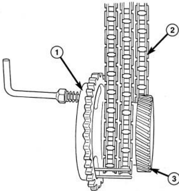
Fig. 23: Locked Secondary Timing Chains Courtesy of CHRYSLER LLC
