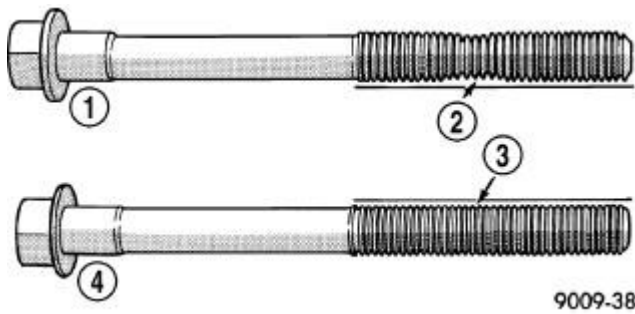
Fig. 49: Checking Cylinder Head Bolts For Stretching (Necking)
