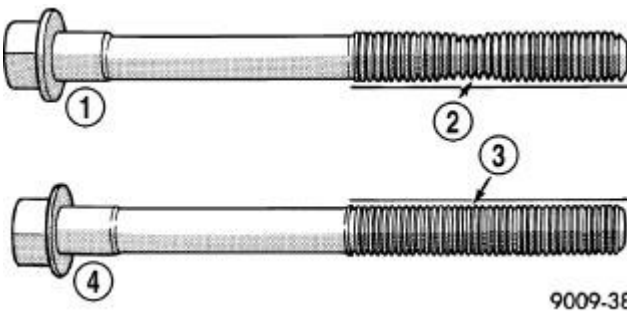
Fig. 26: Checking Cylinder Head Bolts For Stretching (Necking) Courtesy of CHRYSLER LLC
