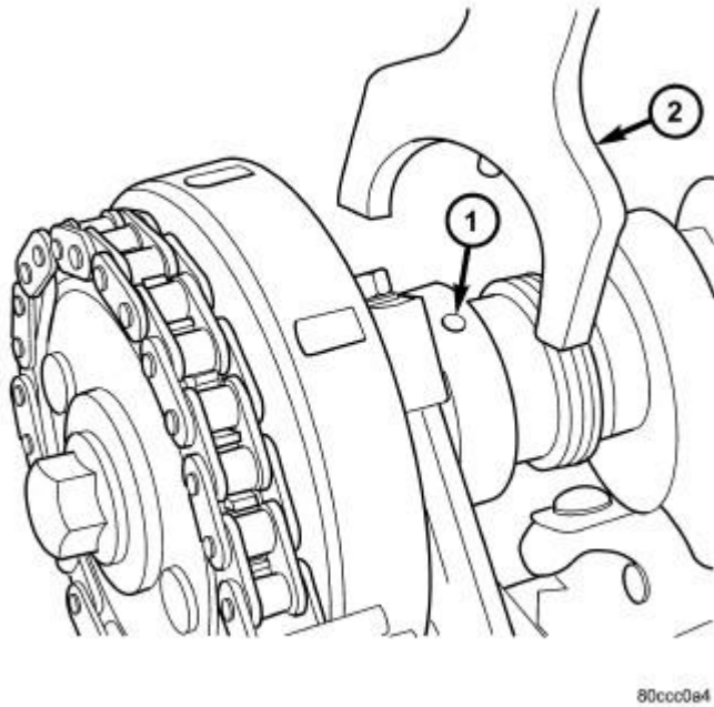
Fig. 164: Camshaft & Camshaft Holder Courtesy of CHRYSLER LLC
