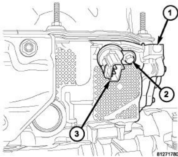
Fig. 58: Camshaft Position Sensor Courtesy of CHRYSLER LLC
