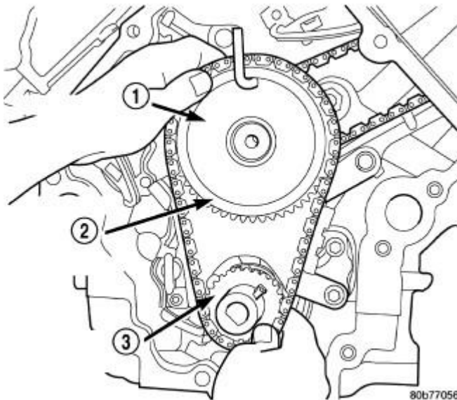
Fig. 166: Installing Idler Gear, Primary And Secondary Timing Chains Courtesy of CHRYSLER LLC
