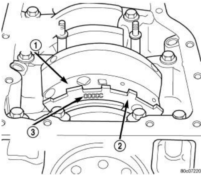
Fig. 77: Markings On Target Wheel Courtesy of CHRYSLER LLC
