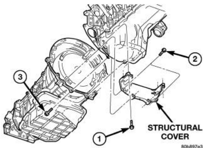
Fig. 78: Structural Cover
