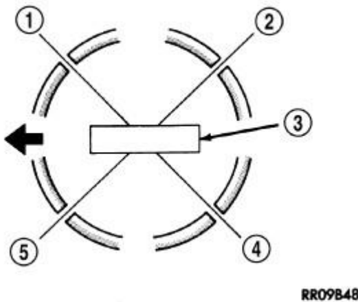
Fig. 98: Piston Ring End Gap Position Courtesy of CHRYSLER LLC
