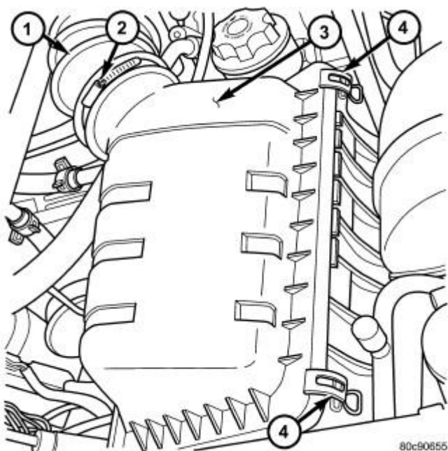
Fig. 20: Air Cleaner Element - 3.7L
