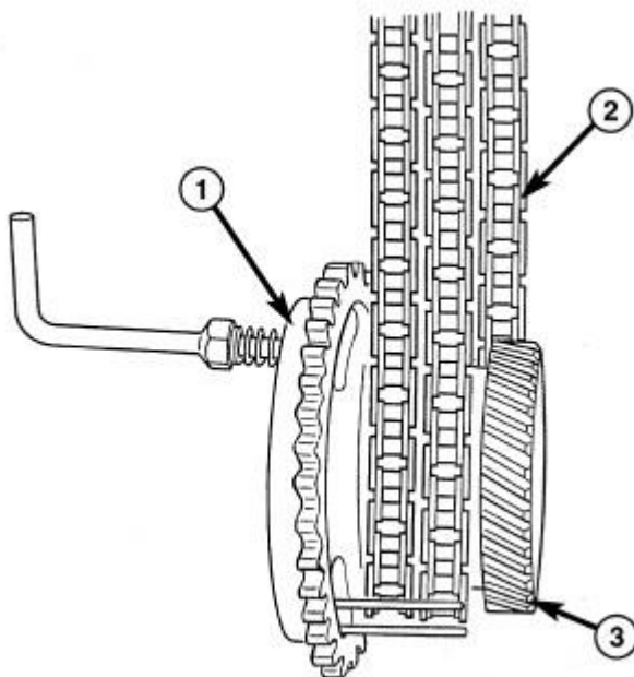
Fig. 45: Locked Secondary Timing Chains Courtesy of CHRYSLER LLC
