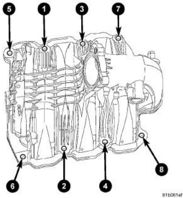
Fig. 140: 3.7L Intake Loosening/Tightening Sequence Courtesy of CHRYSLER LLC
