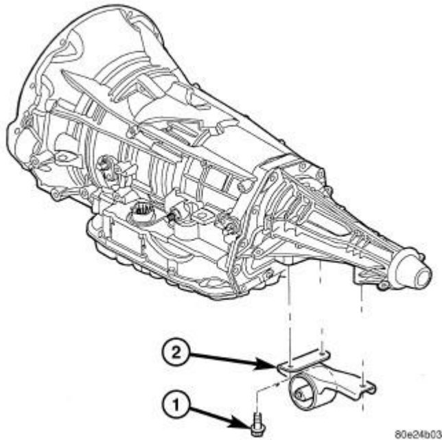
Fig. 118: Automatic Transmission Mount Assembly - 3.7L 2WD Courtesy of CHRYSLER LLC
