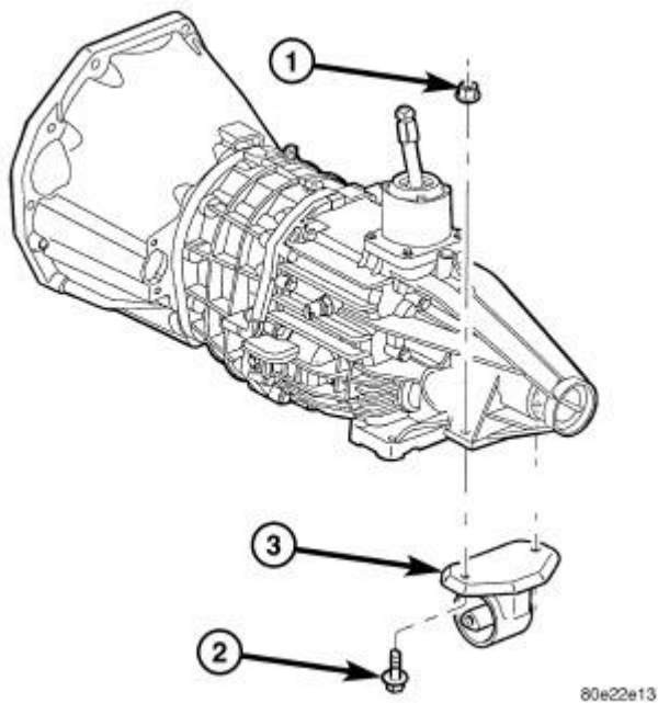
Fig. 117: Manual Transmission Mount Assembly - 3.7L 2WD Courtesy of CHRYSLER LLC
