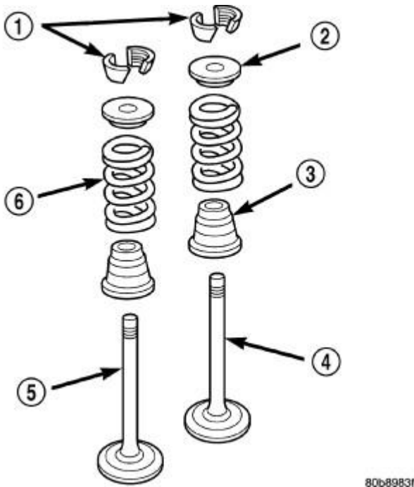
Fig. 41: Valve Assembly Configuration Courtesy of CHRYSLER LLC
