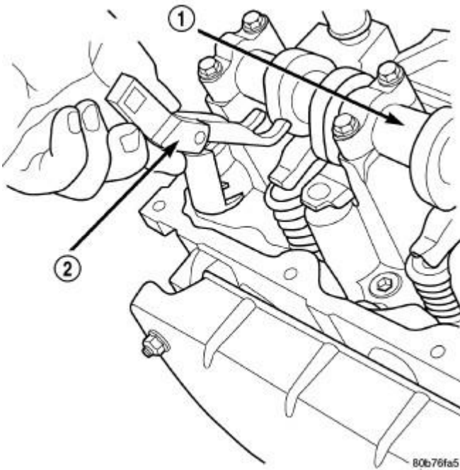
Fig. 39: Rocker Arm - Removal/Installation Courtesy of CHRYSLER LLC
