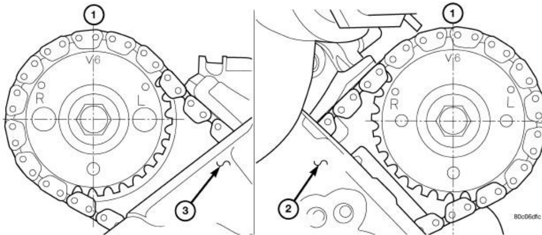
Fig. 168: Camshaft Sprocket V6 Marks Courtesy of CHRYSLER LLC
