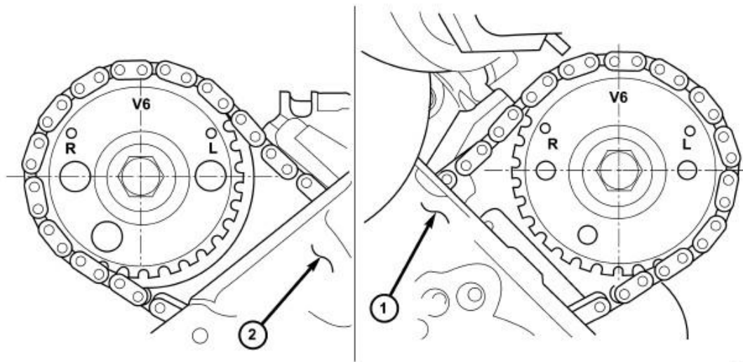
Fig. 154: Camshaft Sprocket V6 Marks (#1 TDC, Exhaust Stroke) Courtesy of CHRYSLER LLC
