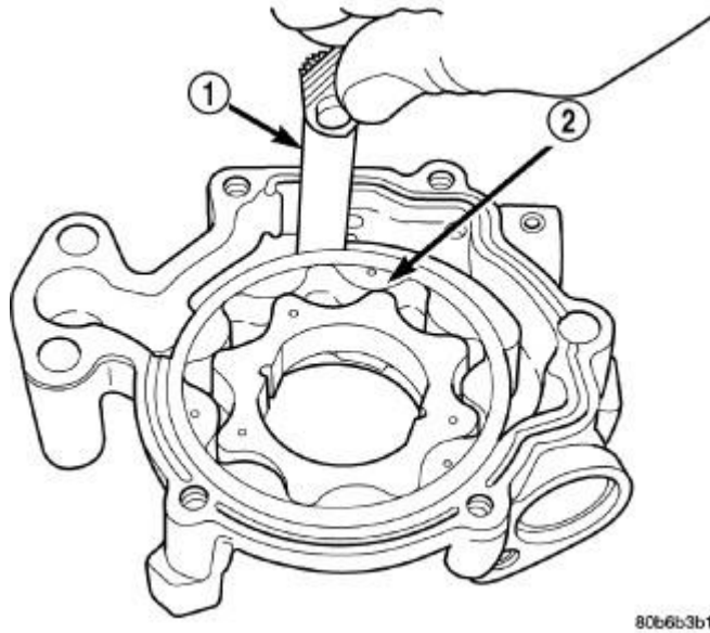
Fig. 130: Measuring Outer Rotor Clearance Courtesy of CHRYSLER LLC
