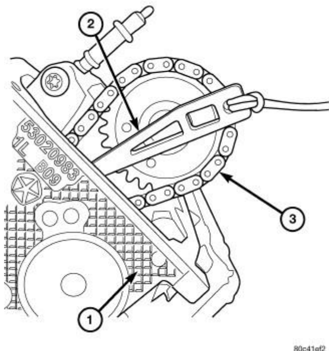
Fig. 156: Securing Timing Chain Tensioner Using Timing Chain Wedge Courtesy of CHRYSLER LLC
