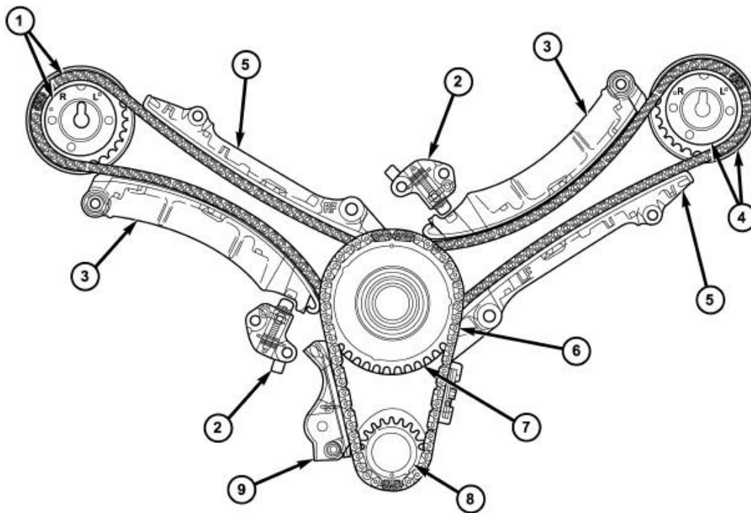
Fig. 151: Timing Drive System Courtesy of CHRYSLER LLC
