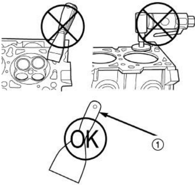
Fig. 48: Proper Tool Usage For Surface Preparation Courtesy of CHRYSLER LLC
