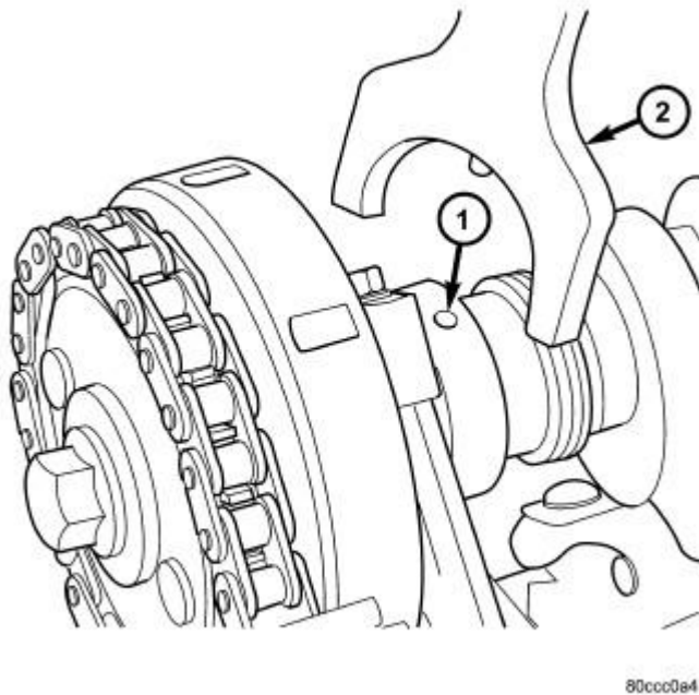
Fig. 59: Camshaft & Camshaft Holder Courtesy of CHRYSLER LLC
