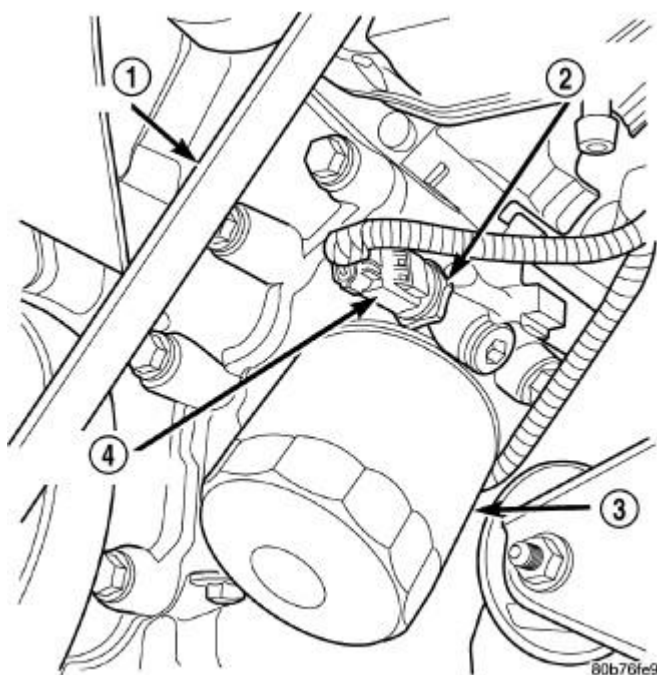
Fig. 135: Belt, Oil Pressure Sensor, Oil Filter & Connector Courtesy of CHRYSLER LLC
