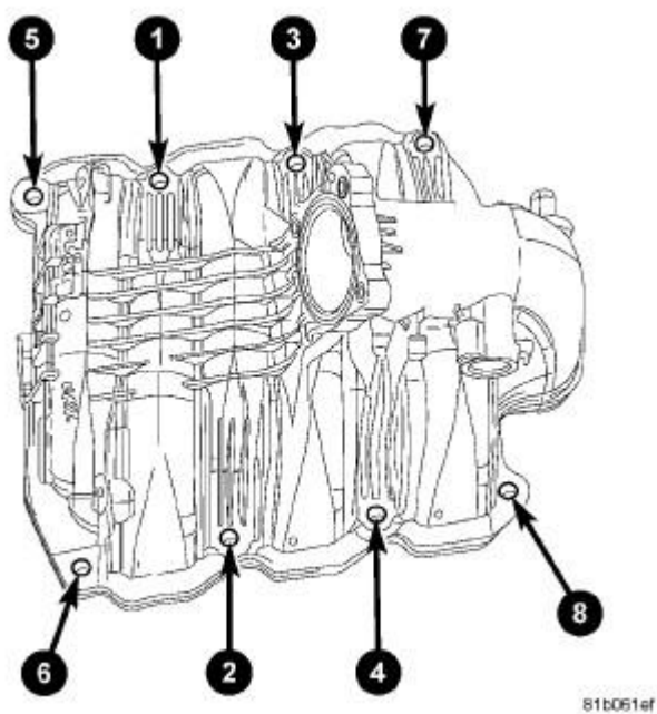
Fig. 16: 3.7L Intake Loosening/Tightening Sequence Courtesy of CHRYSLER LLC
