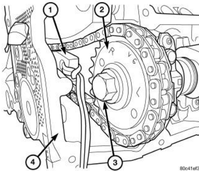
Fig. 64: Timing Chain Tensioners Secured With Timing Chain Wedge Courtesy of CHRYSLER LLC
