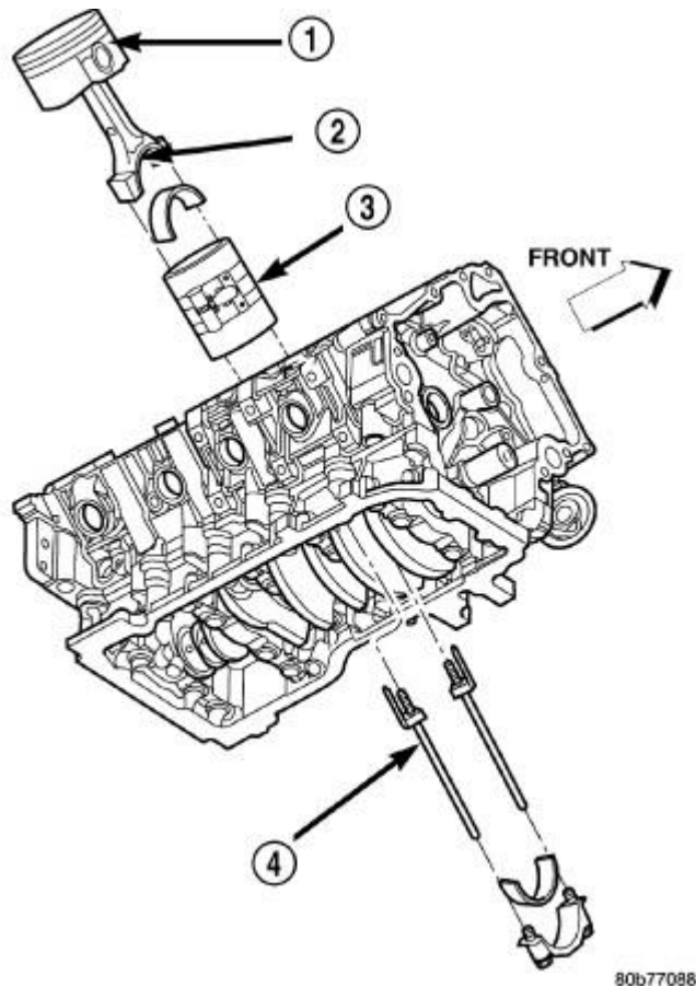
Fig. 102: Piston, Oil Slinger Slot, Ring Compressor & Special Tool Courtesy of CHRYSLER LLC
