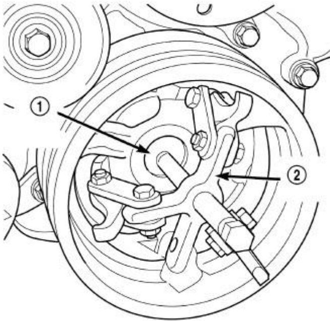
Fig. 85: Removing Crankshaft Damper Courtesy of CHRYSLER LLC
