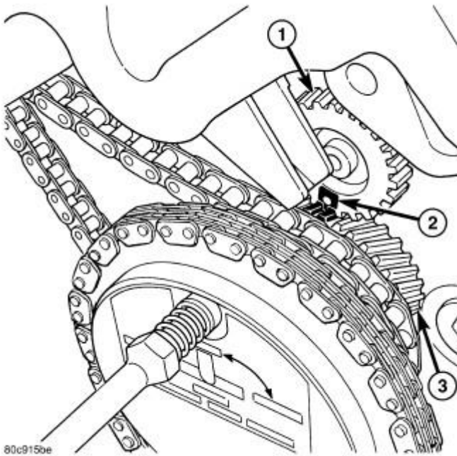
Fig. 155: Counterbalance Shaft Alignment Marks Courtesy of CHRYSLER LLC
