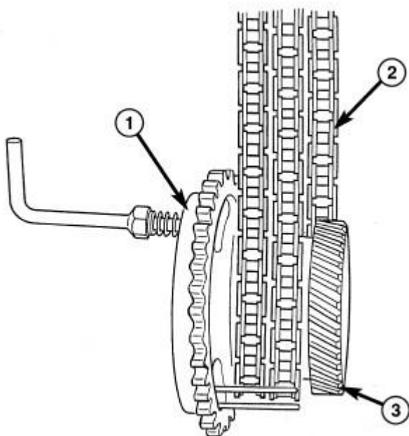
Fig. 54: Locked Secondary Timing Chains Courtesy of CHRYSLER LLC
