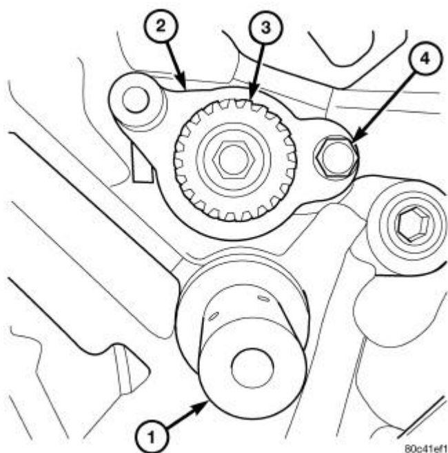
Fig. 90: Idler Shaft, Counterbalance Shaft Thrust Plate And Drive Gear & Retaining Bolt Courtesy of CHRYSLER LLC
