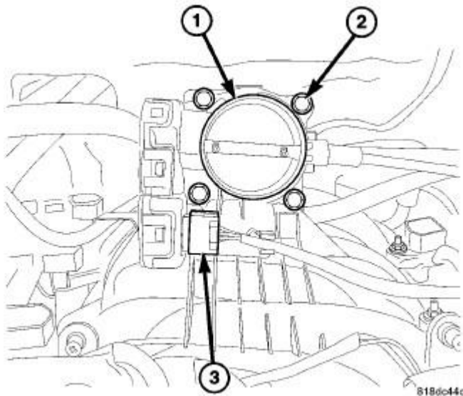
Fig. 142: Throttle Body 3.7L, Mounting Bolts & Connector Courtesy of CHRYSLER LLC
