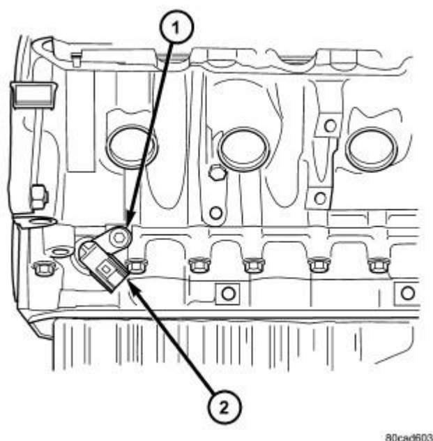
Fig. 8: Crankshaft Position Sensor Courtesy of CHRYSLER LLC
