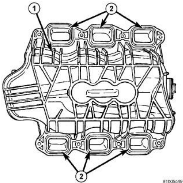
Fig. 141: Intake Manifold Seals Courtesy of CHRYSLER LLC
