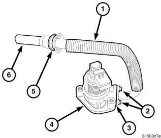
Fig. 149: EGR Solenoid/Tube Assembly Courtesy of CHRYSLER LLC
