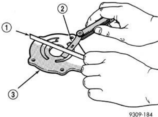
Fig. 127: Checking Oil Pump Cover Flatness Courtesy of CHRYSLER LLC
