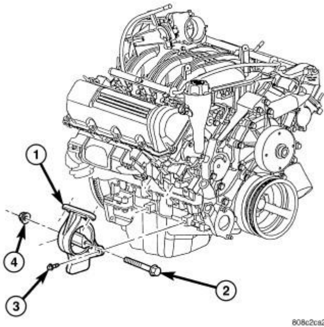
Fig. 116: Engine Insulator Mount Assembly 3.7L Right Courtesy of CHRYSLER LLC
