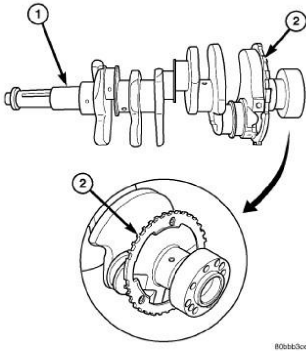
Fig. 80: Crankshaft & Target Ring Courtesy of CHRYSLER LLC
