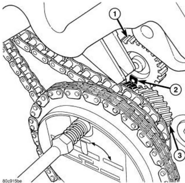
Fig. 167: Counterbalance Shaft Alignment Marks Courtesy of CHRYSLER LLC
