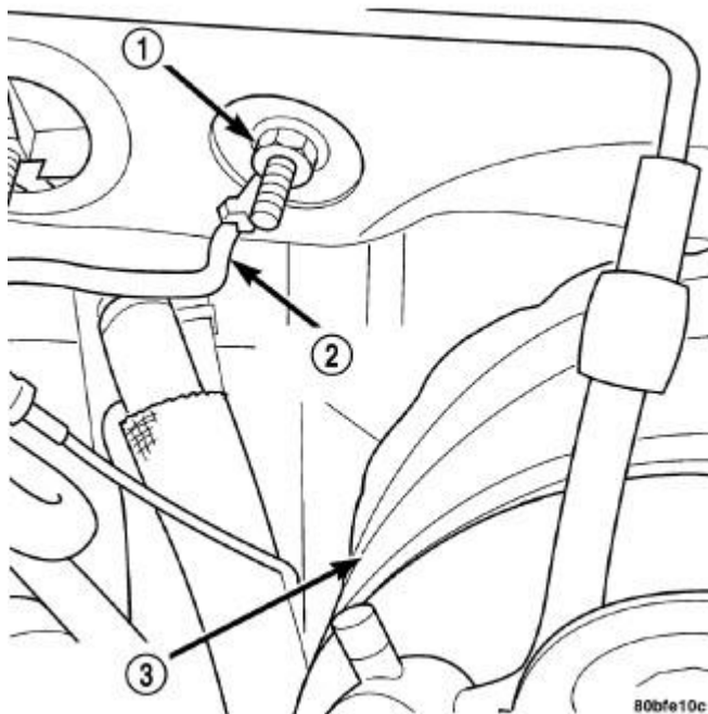
Fig. 15: Body Ground Strap, Brake Booster & Nut
