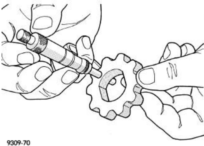
Fig. 129: Measuring Inner Rotor Thickness Courtesy of CHRYSLER LLC
