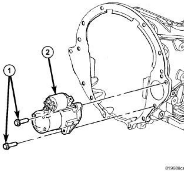
Fig. 11: Starter Motor - 3.7L Courtesy of CHRYSLER LLC
