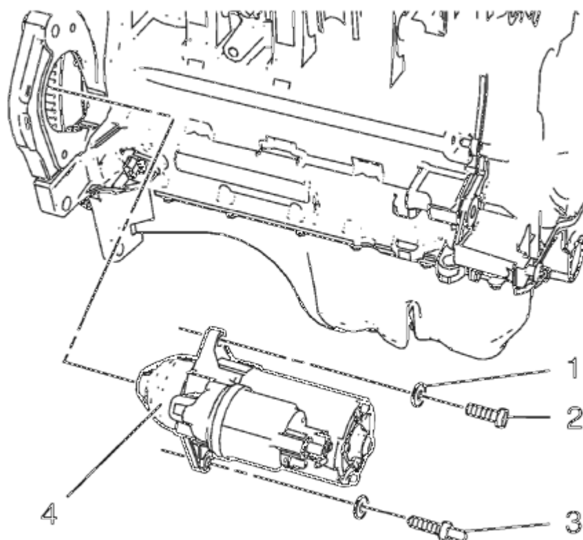
Fig. 280: Starter, Bolt, Stud And Washer Courtesy of GENERAL MOTORS COMPANY
