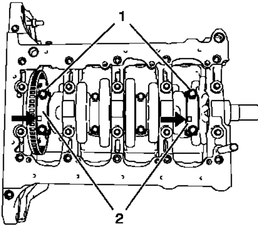
Fig. 397: Rod Bearing Caps And Bolts Courtesy of GENERAL MOTORS COMPANY
