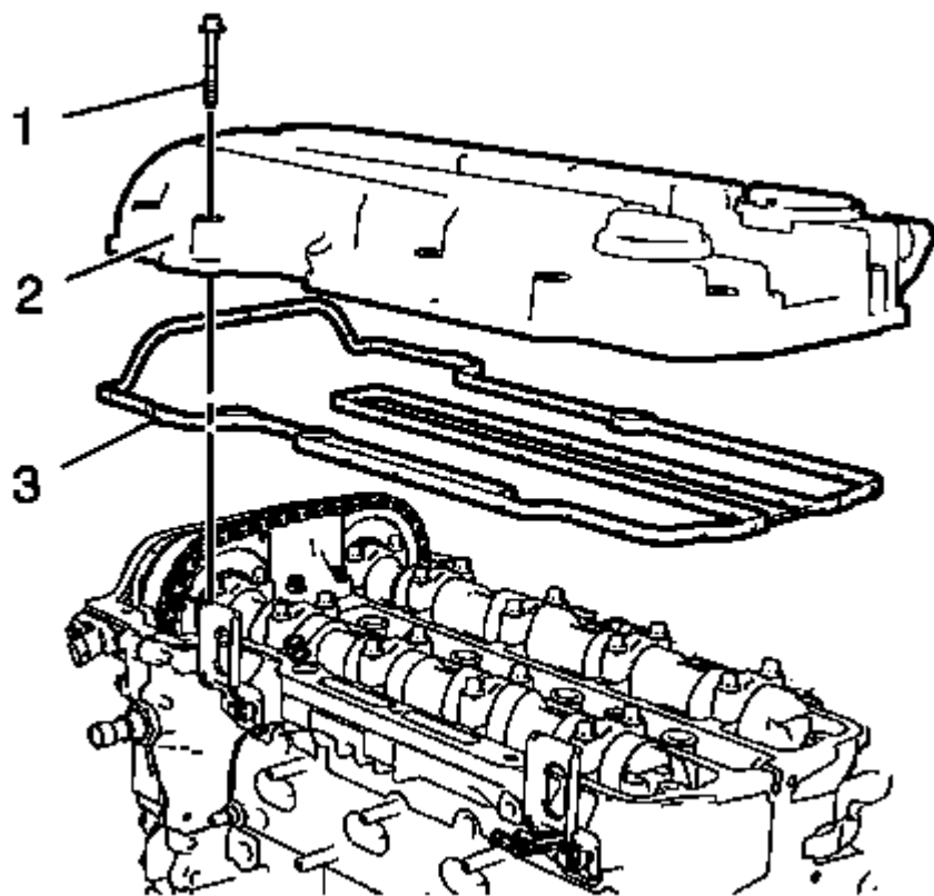
Fig. 429: Camshaft Cover And Gasket
