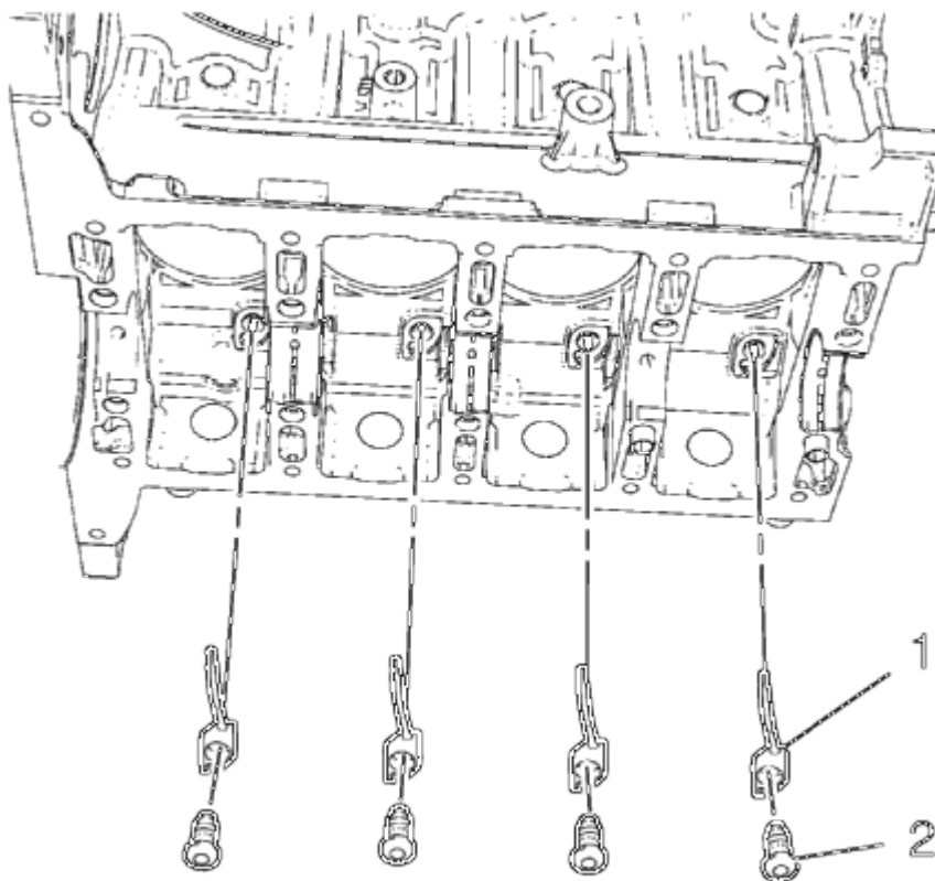
Fig. 333: Piston Oil Nozzles And Bolts
