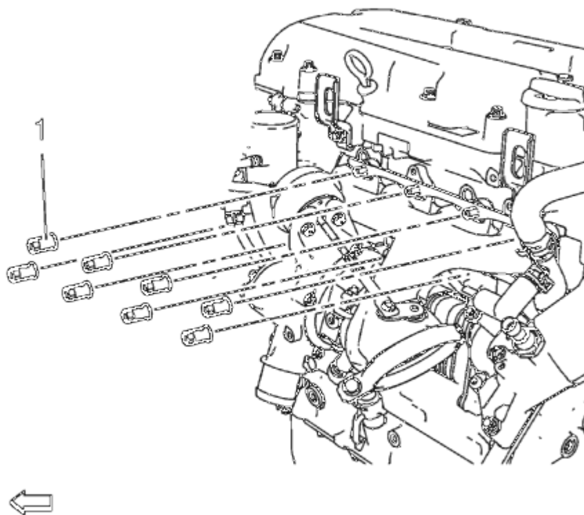
Fig. 204: Turbocharger Nuts
