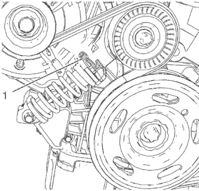
Fig. 21: Locking Pin
