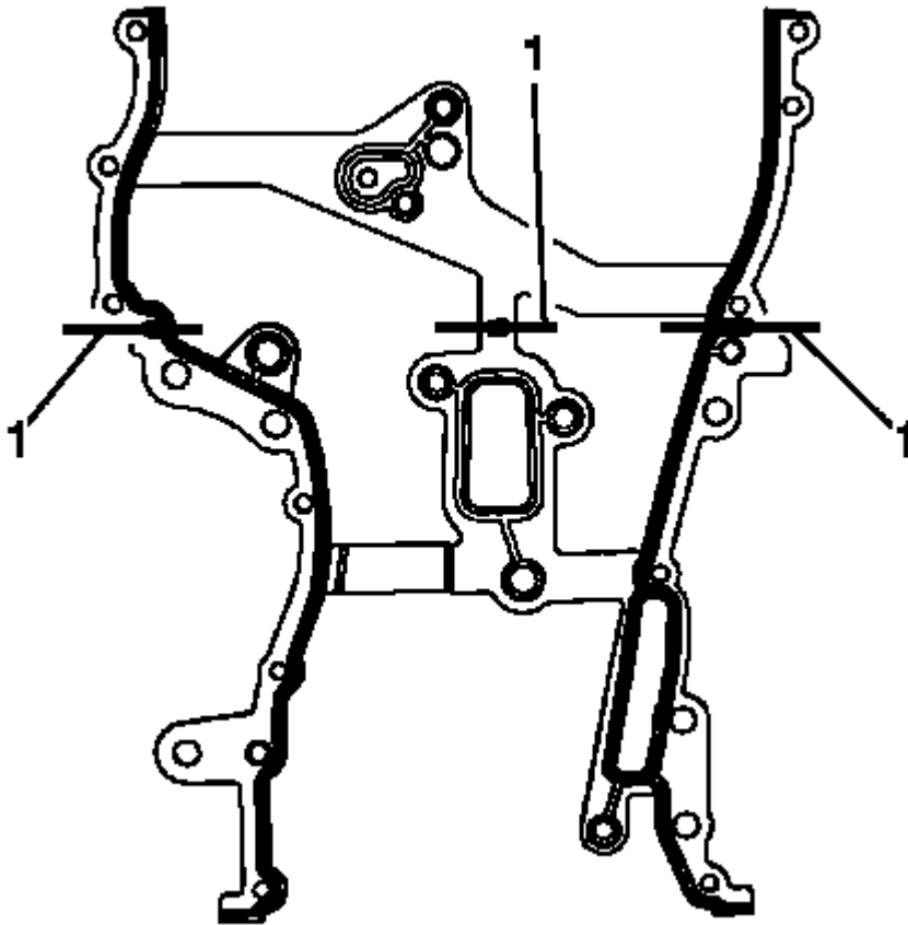
Fig. 83: engine front cover gasket
