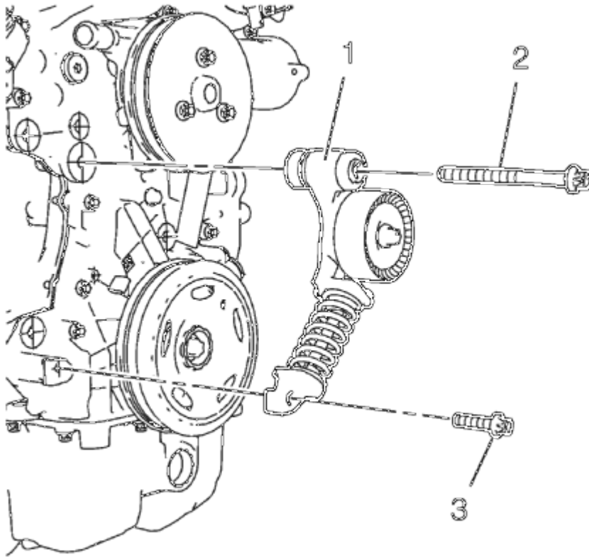
Fig. 270: Drive Belt Tensioner And Bolts
