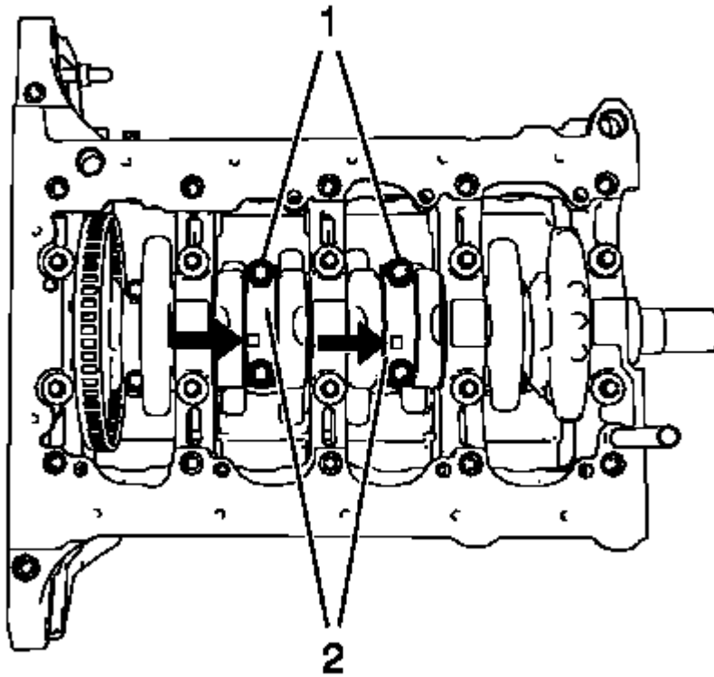
Fig. 311: Rod Bearing Caps And Bolts Courtesy of GENERAL MOTORS COMPANY
