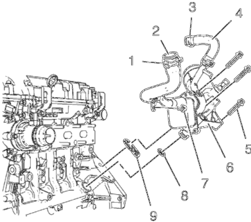
Fig. 267: Locating Engine Oil Cooler Components Courtesy of GENERAL MOTORS COMPANY
