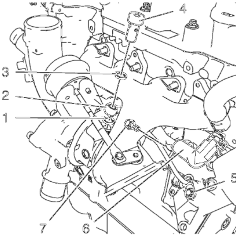
Fig. 264: Turbocharger Oil Feed Pipe Components
