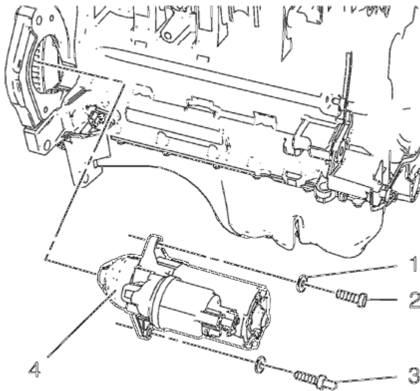
Fig. 437: Starter, Bolt, Stud And Washer Courtesy of GENERAL MOTORS COMPANY
