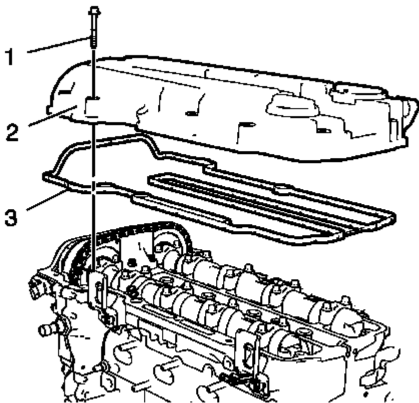
Fig. 286: Camshaft Cover And Gasket
