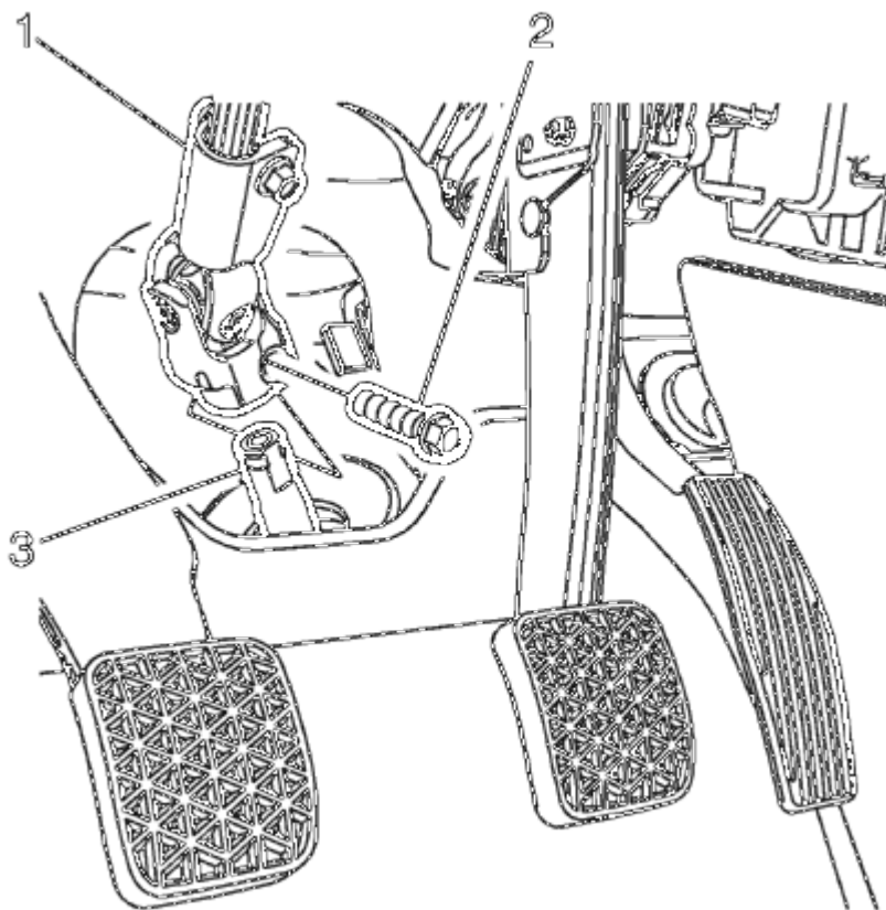
Fig. 140: Intermediate Steering Shaft And Bolt
