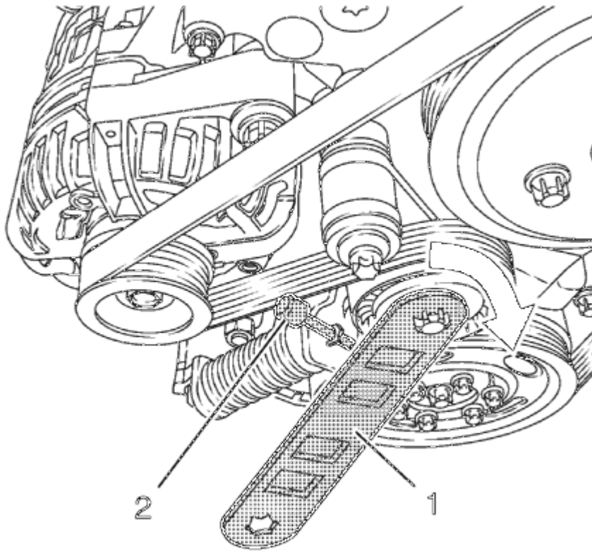
Fig. 474: Locking Pin And Wrench
