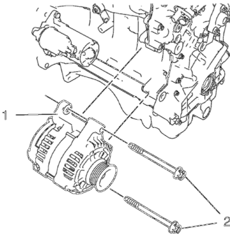
Fig. 436: Generator And Bolts
