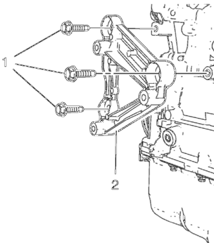
Fig. 271: Power Steering Pump Bracket/Air Conditioning Compressor Bracket And Bolts Courtesy of GENERAL MOTORS COMPANY
