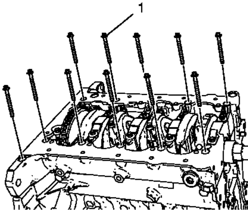
Fig. 315: Outer Crankshaft Bearing Cap Tie Plate Bolts Courtesy of GENERAL MOTORS COMPANY
