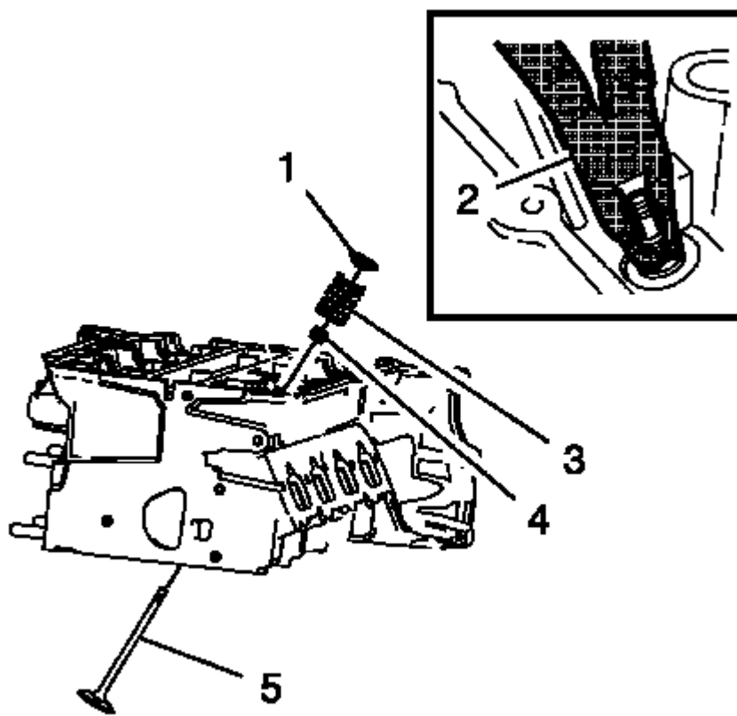
Fig. 322: Spring Compressor
