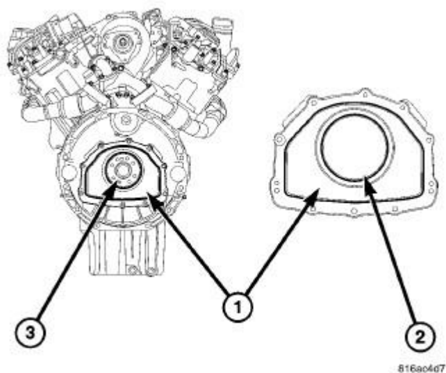
Fig. 407: REAR MAIN SEAL CARRIER
