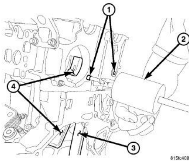
Fig. 567: LEFT UPPER TIMING CHAIN GUIDE PIN EXTRACTION Courtesy of CHRYSLER LLC
