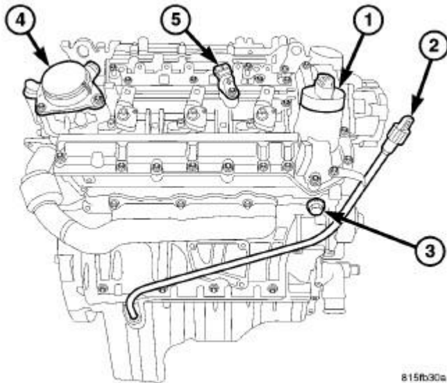
Fig. 605: Timing Chain Tensioner Courtesy of CHRYSLER LLC
