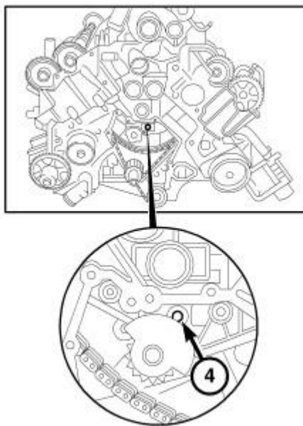
Fig. 379: BALANCE SHAFT ALIGNMENT FRONT
