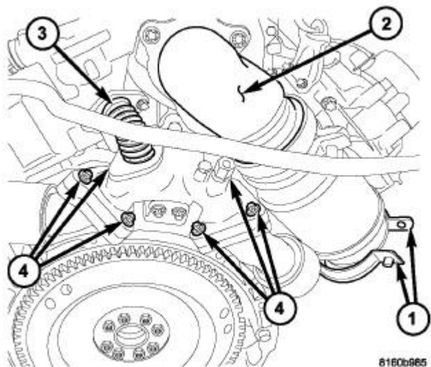
Fig. 490: Removing/Installing Air Intake, Turbo & Exhaust System Components Courtesy of CHRYSLER LLC
