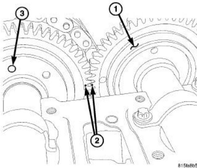
Fig. 113: CAMSHAFT GEAR ALIGNMENT Courtesy of CHRYSLER LLC
