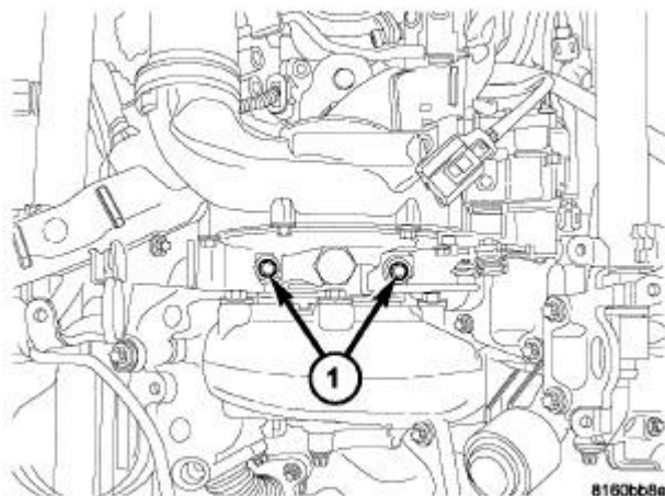
Fig. 552: Removing/Installing Air Intake Tube (Air Cleaner To Turbo) Courtesy of CHRYSLER LLC
