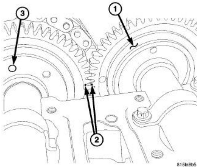
Fig. 163: CAMSHAFT GEAR ALIGNMENT
