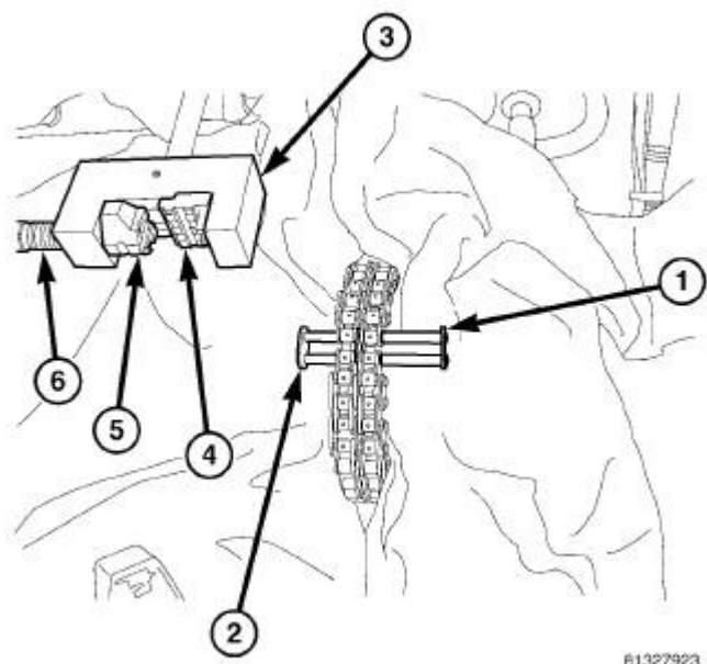
Fig. 588: Removal/Installation Chain Link Courtesy of CHRYSLER LLC
