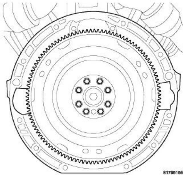
Fig. 461: FLEX PLATE Courtesy of CHRYSLER LLC
