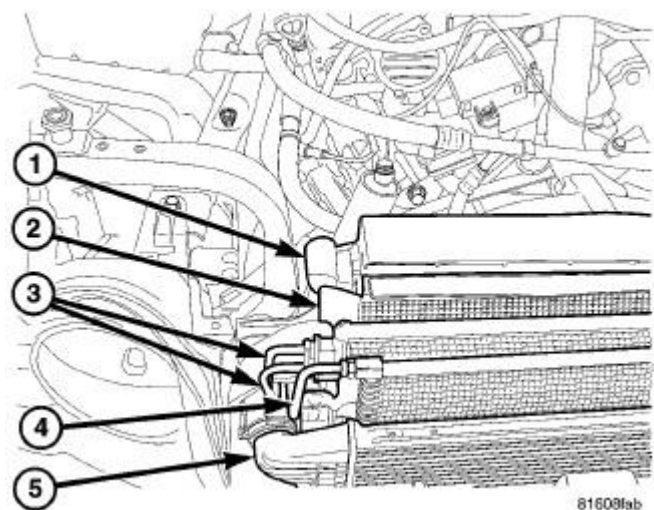
Fig. 15: COOLANT MODULE Courtesy of CHRYSLER LLC
