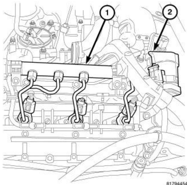
Fig. 266: EGR Valve & Fuel Rail Equalizing Line Courtesy of CHRYSLER LLC
