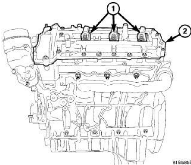
Fig. 247: Left Cylinder Head Cover Courtesy of CHRYSLER LLC
