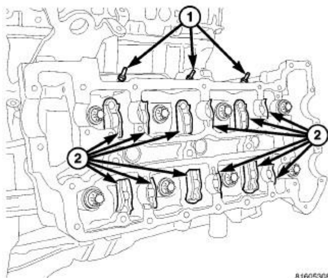
Fig. 161: RIGHT TAPPET/CAMSHAFT FOLLOWER POSITION
