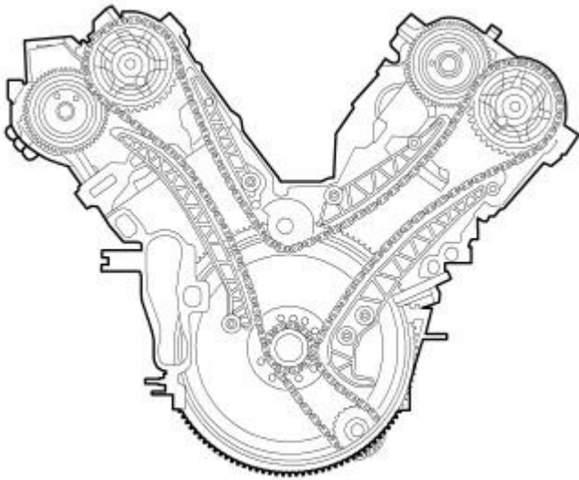
Fig. 572: TIMING
