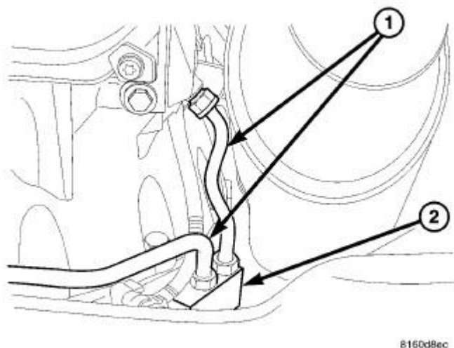
Fig. 397: TRANSMISSION THERMO-BLOCK Courtesy of CHRYSLER LLC
