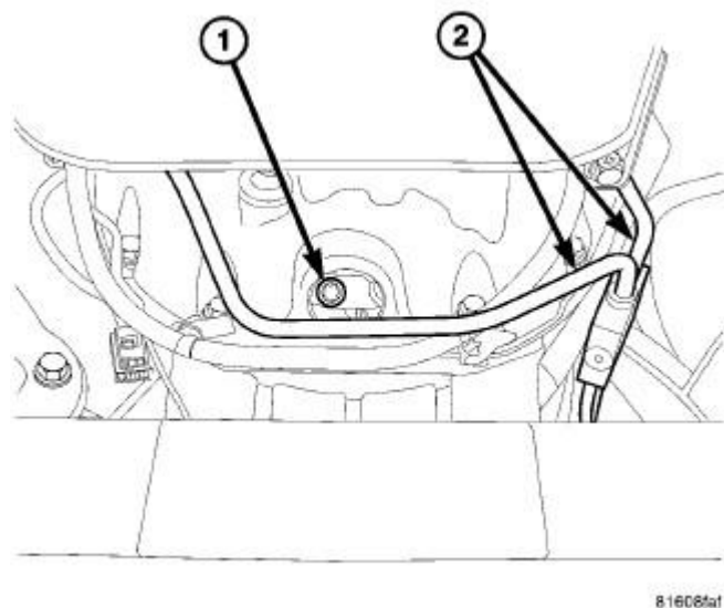
Fig. 13: TORQUE CONVERTER TO FLEX PLATE BOLTS Courtesy of CHRYSLER LLC
