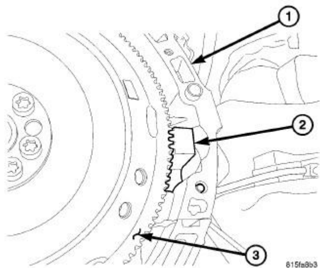
Fig. 87: FLYWHEEL LOCK 9102 Courtesy of CHRYSLER LLC
