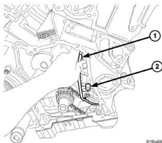
Fig. 95: LEFT LOWER TIMING CHAIN GUIDE AND FASTENER
