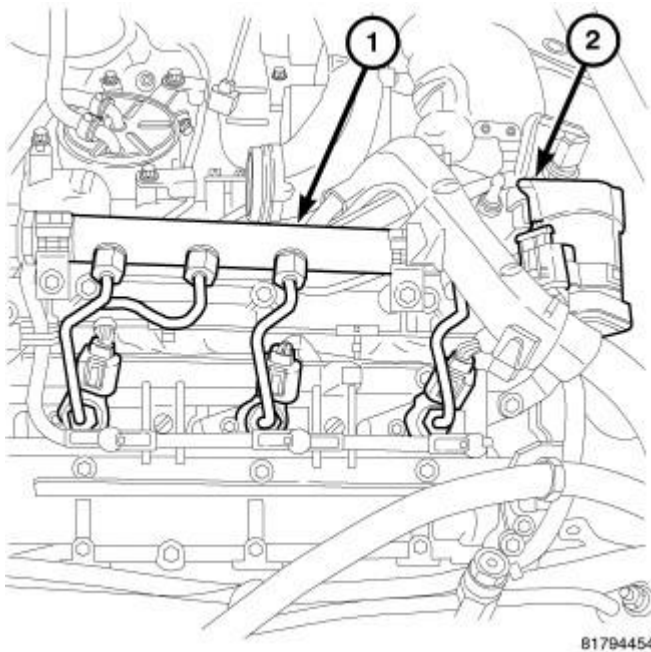
Fig. 597: EGR Valve & Fuel Rail Equalizing Line Courtesy of CHRYSLER LLC
