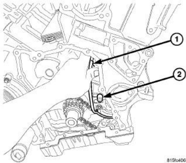
Fig. 581: Left Lower Timing Chain Guide And Fastener Courtesy of CHRYSLER LLC
