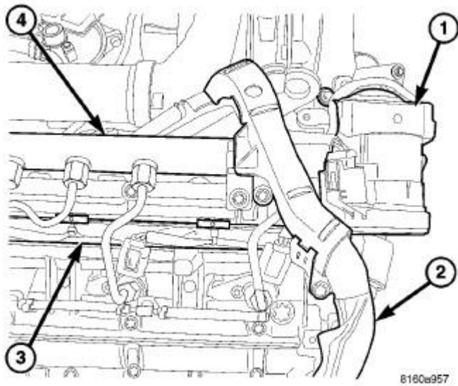
Fig. 207: EGR VALVE WITH MAIN ENGINE WIRING HARNESS Courtesy of CHRYSLER LLC
