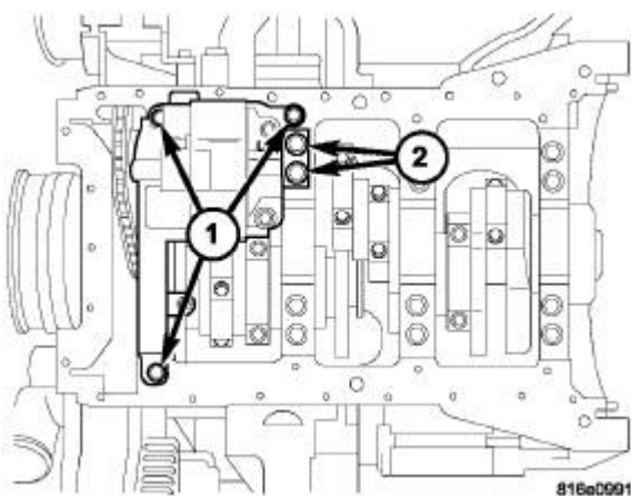
Fig. 392: OIL PUMP
