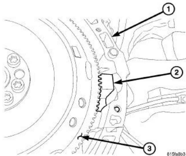
Fig. 156: SPECIAL TOOL # 9102
