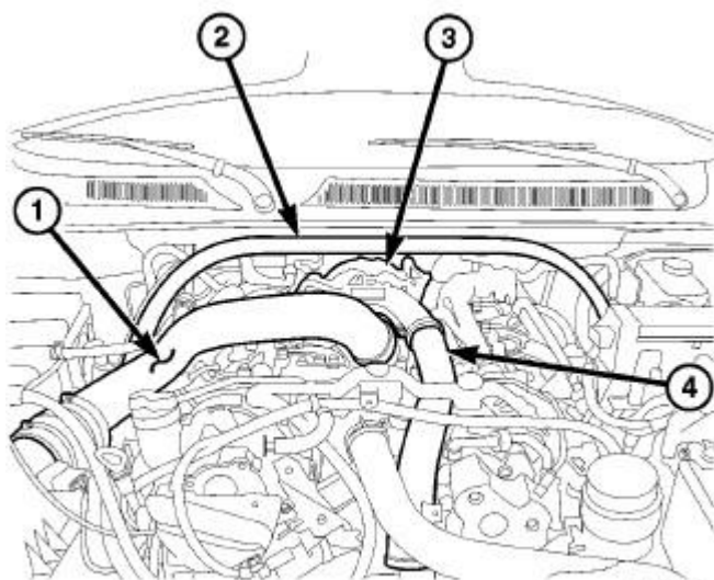
Fig. 506: STRUT TOWER SUPPORT
