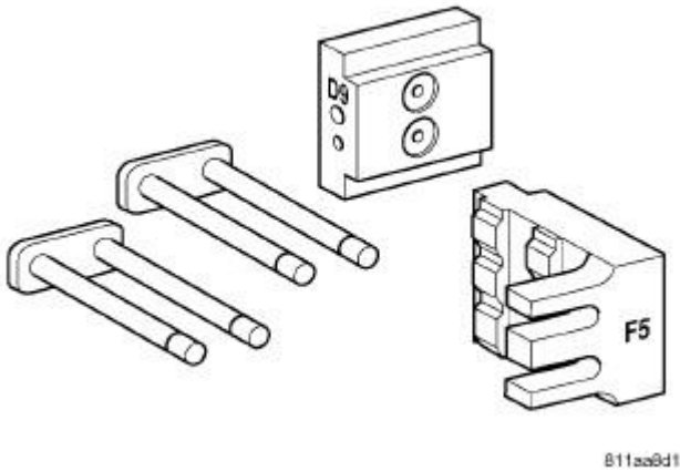
Fig. 41: INSERTS, ASSEMBLY - 8952A Courtesy of CHRYSLER LLC
