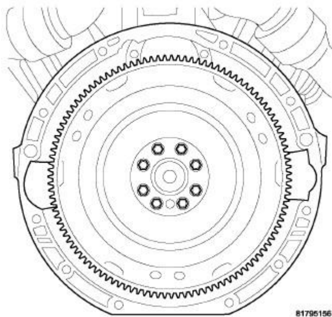
Fig. 324: FLEX PLATE
