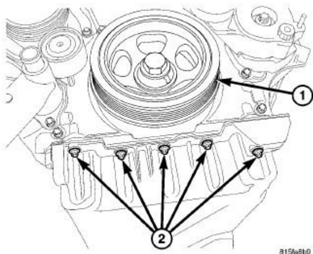
Fig. 601: Vibration Damper & Front Oil Pan Bolts Courtesy of CHRYSLER LLC
