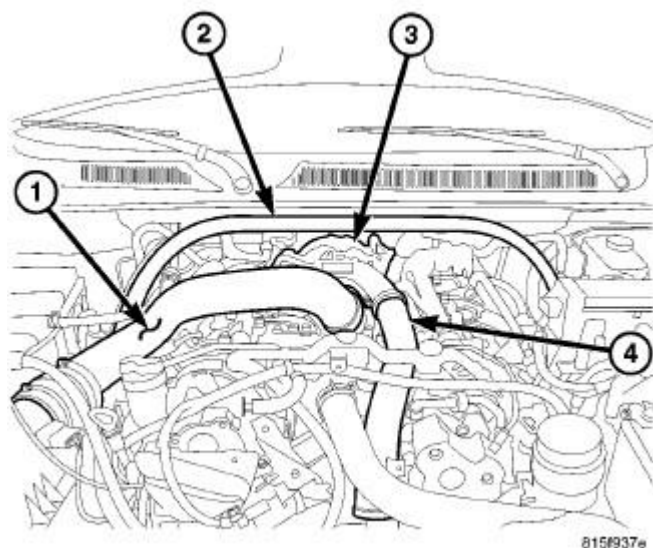
Fig. 53: STRUT TOWER SUPPORT
