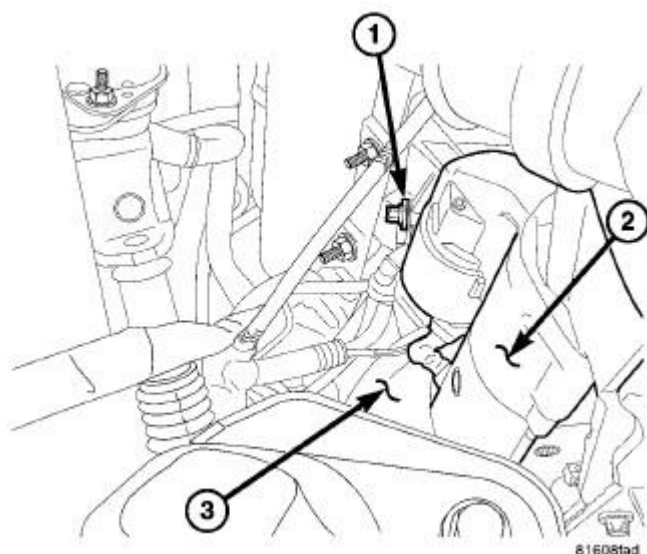
Fig. 22: STARTER AND MAIN ENGINE HARNESS GROUND
