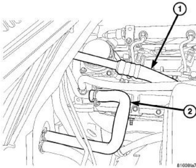
Fig. 16: HEATER HOSES Courtesy of CHRYSLER LLC
