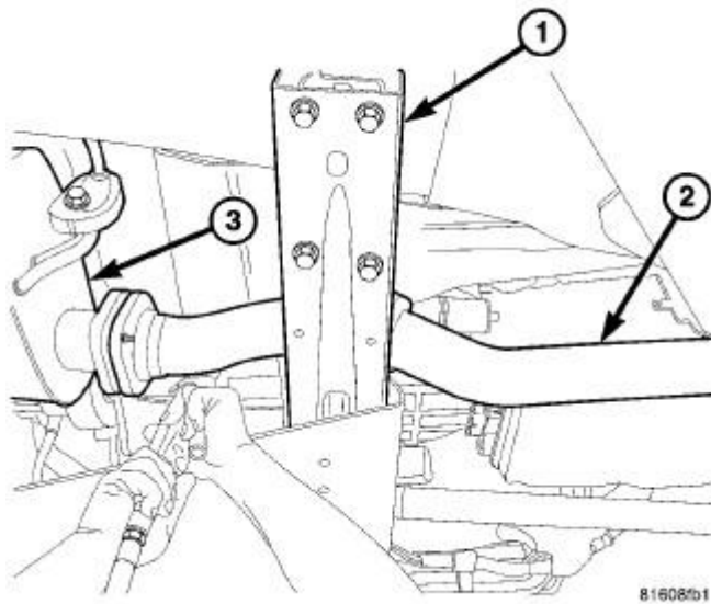
Fig. 12: FRONT EXHAUST PIPE AT MUFFLER Courtesy of CHRYSLER LLC
