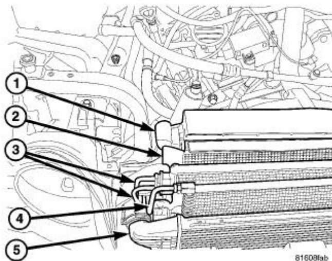
Fig. 28: COOLANT MODULE Courtesy of CHRYSLER LLC
