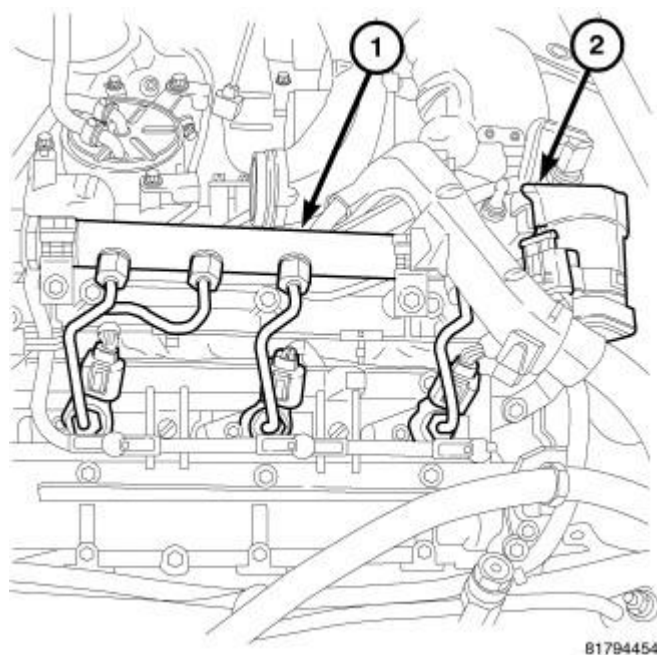
Fig. 603: EGR Valve & Fuel Rail Equalizing Line Courtesy of CHRYSLER LLC
