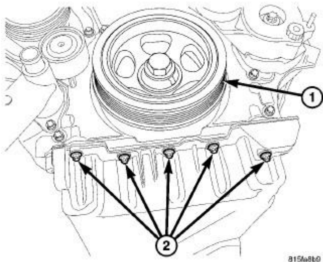
Fig. 172: FRONT OIL PAN Courtesy of CHRYSLER LLC
