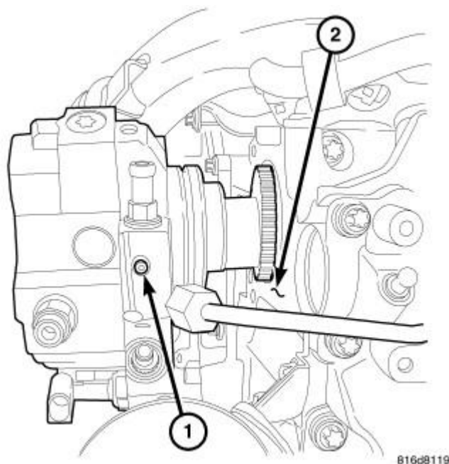
Fig. 146: HIGH PRESSURE PUMP INSTALLATION Courtesy of CHRYSLER LLC
