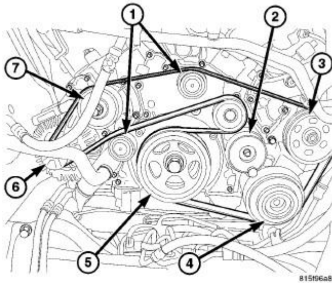
Fig. 366: ACCESSORY DRIVE BELT Courtesy of CHRYSLER LLC
