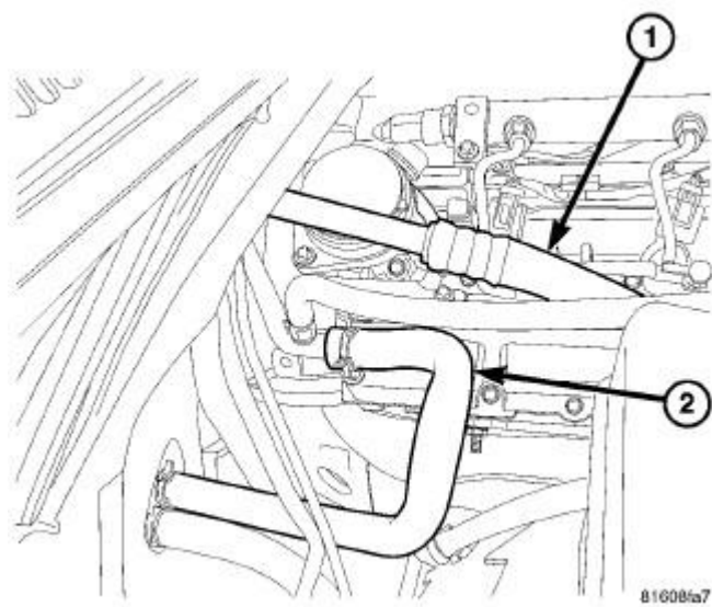
Fig. 26: HEATER HOSES
