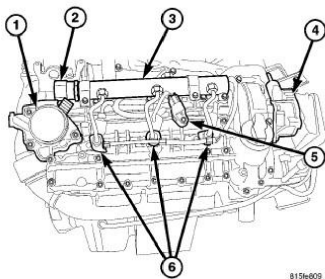
Fig. 233: RIGHT CYLINDER HEAD
