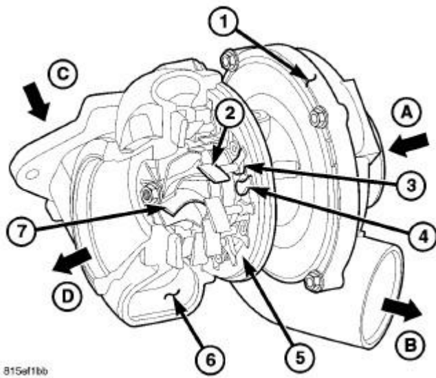
Fig. 549: TURBOCHARGER COMPONENTS Courtesy of CHRYSLER LLC
