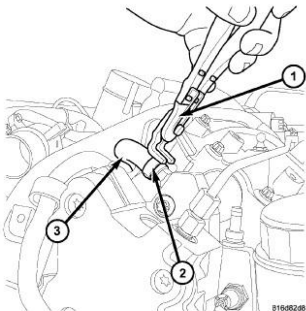
Fig. 244: PUMP FUEL LINE PLIERS Courtesy of CHRYSLER LLC
