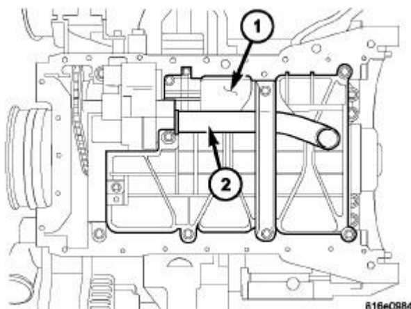
Fig. 338: OIL PUMP COVER REMOVAL Courtesy of CHRYSLER LLC
