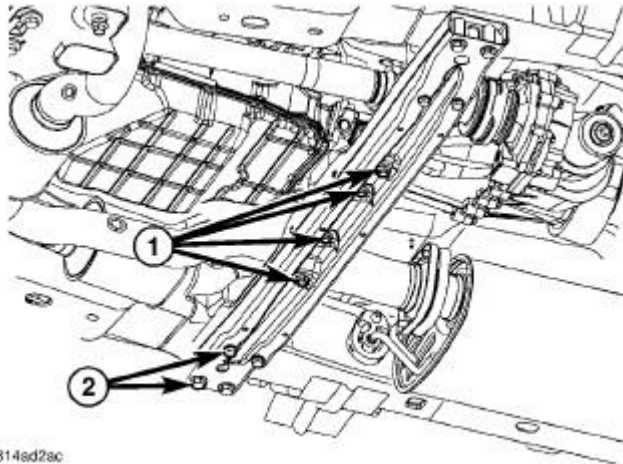
Fig. 502: TRANSFER CASE SKID PLATE Courtesy of CHRYSLER LLC
