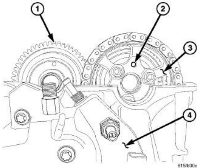
Fig. 578: LEFT EXHAUST CAMSHAFT DRIVE GEAR ALIGNMENT DOWEL Courtesy of CHRYSLER LLC
