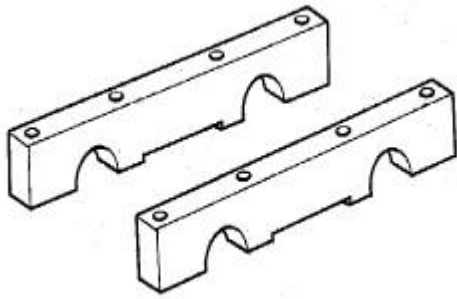
Fig. 49: Retainer, Camshafts - 9555
