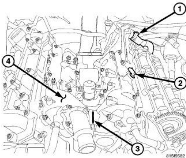
Fig. 178: INTAKE MANIFOLD
