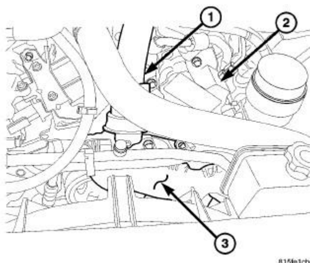
Fig. 152: CHARGE AIR COOLER INLET WITH RESONATOR
