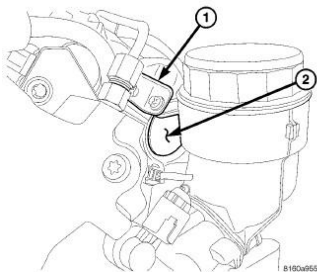
Fig. 145: LEFT FRONT CAMSHAFT SEAL WITH OIL FILTER HOUSING BRACKET
