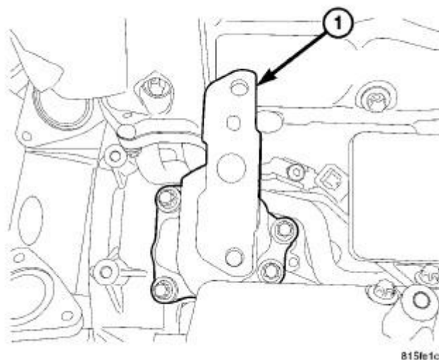
Fig. 99: TURBOCHARGER ADAPTOR
