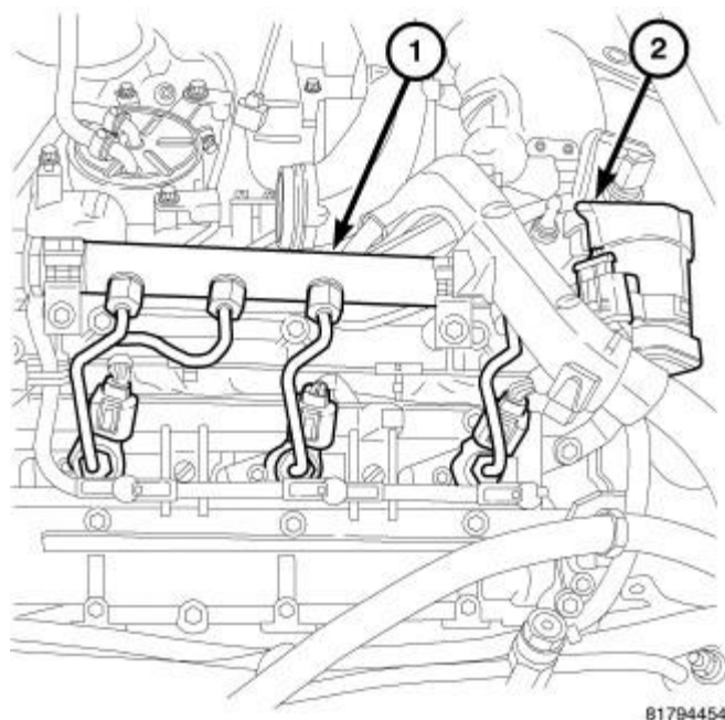
Fig. 245: EGR Valve & Fuel Rail Equalizing Line Courtesy of CHRYSLER LLC
