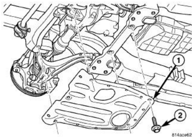
Fig. 101: UPDATED SKID PLATE Courtesy of CHRYSLER LLC
