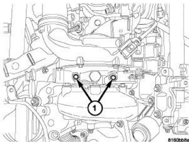
Fig. 557: Removing/Installing Air Intake Tube (Air Cleaner To Turbo)
