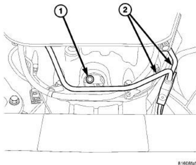
Fig. 21: TORQUE CONVERTER TO FLEX PLATE BOLTS
