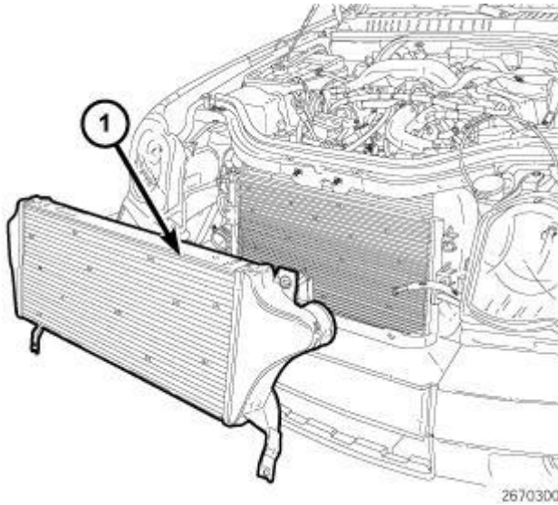
Fig. 546: Charge Air Cooler Courtesy of CHRYSLER LLC
