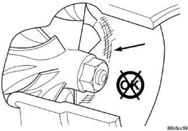
Fig. 554: Inspect Compressor Housing for Impeller Rubbing Condition Courtesy of CHRYSLER LLC
