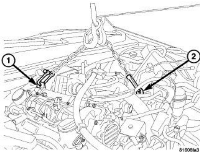
Fig. 350: ENGINE LIFTING POINTS Courtesy of CHRYSLER LLC
