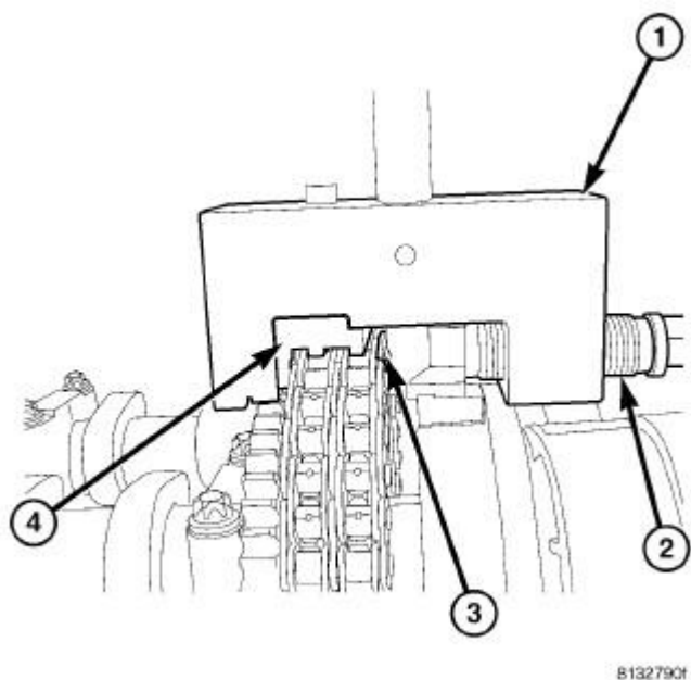
Fig. 592: Riveting Link Pins Courtesy of CHRYSLER LLC
