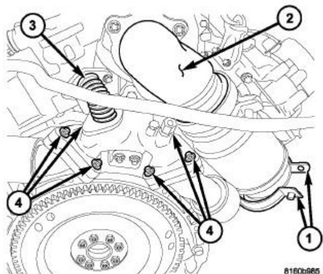
Fig. 347: Removing/Installing Air Intake, Turbo & Exhaust System Components Courtesy of CHRYSLER LLC
