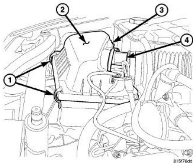
Fig. 241: AIR CLEANER COVER
