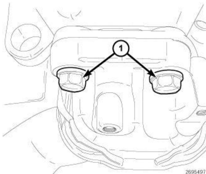
Fig. 431: Right Upper Engine Mount Retaining Bolts Courtesy of CHRYSLER LLC
