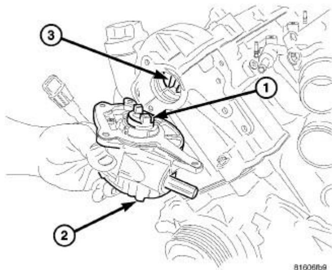
Fig. 235: VACUUM PUMP Courtesy of CHRYSLER LLC
