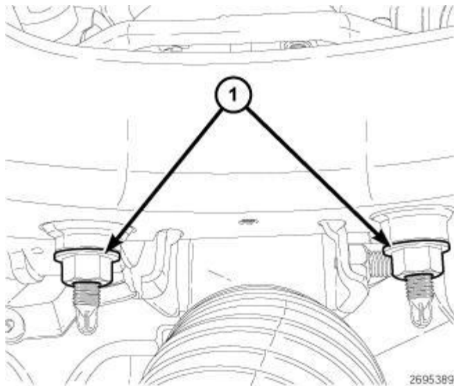
Fig. 422: Left Lower Engine Mount Retaining Nuts
