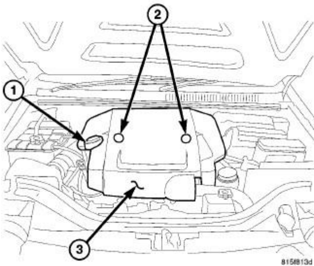
Fig. 19: ENGINE COVER
