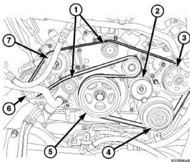
Fig. 602: Accessory Drive Belt Routing Courtesy of CHRYSLER LLC
