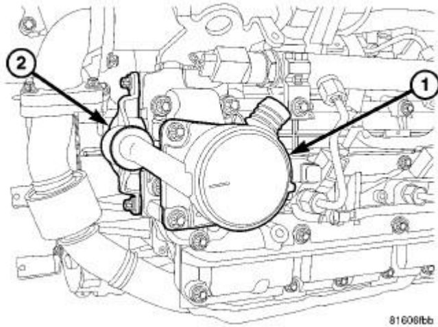
Fig. 250: OIL SEPARATOR Courtesy of CHRYSLER LLC
