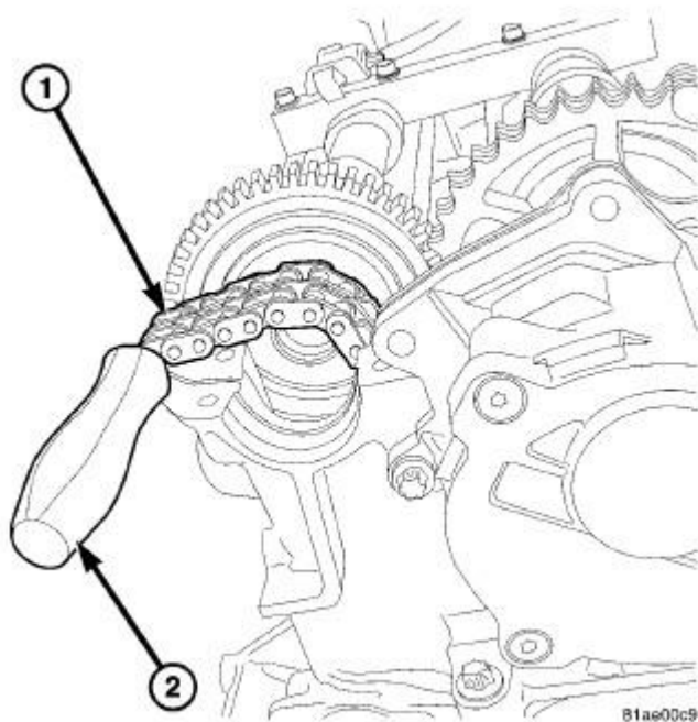
Fig. 582: PREVENT CHAIN FROM FALLING Courtesy of CHRYSLER LLC
