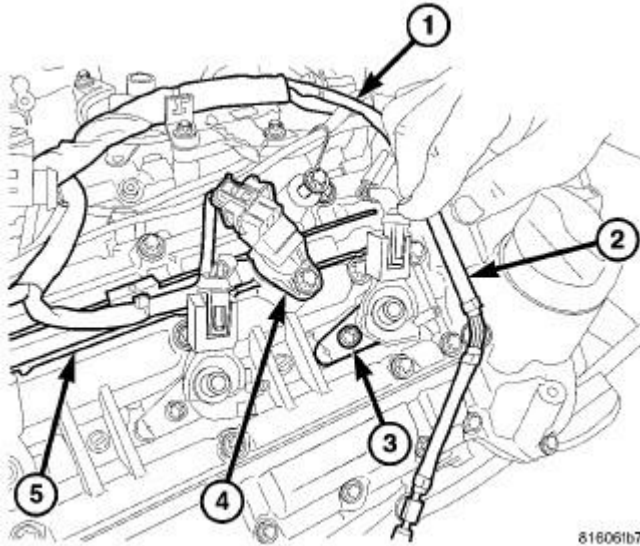
Fig. 257: RIGHT FUEL INJECTORS
