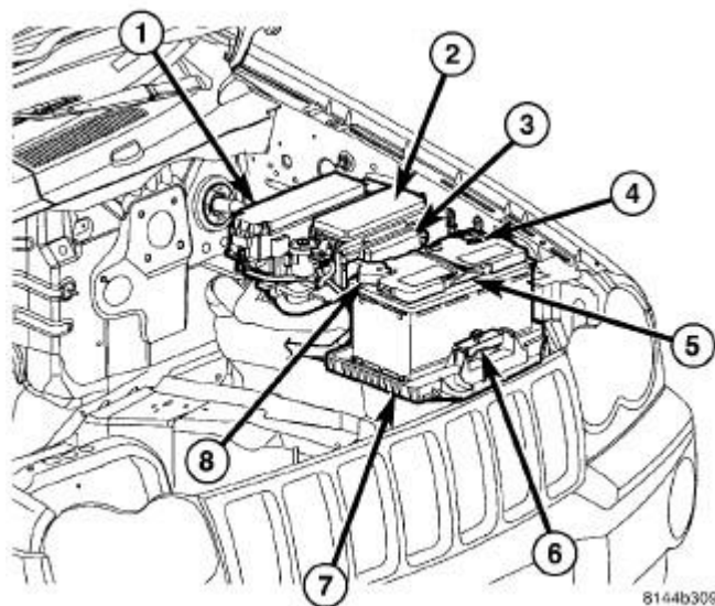
Fig. 428: Identifying Battery System Components, Power Distribution Center & Integrated Power Module
