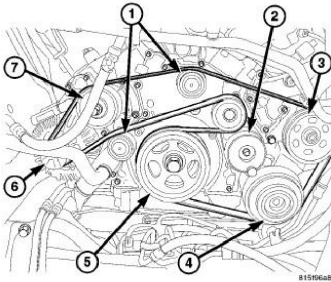
Fig. 77: ACCESSORY DRIVE BELT Courtesy of CHRYSLER LLC
