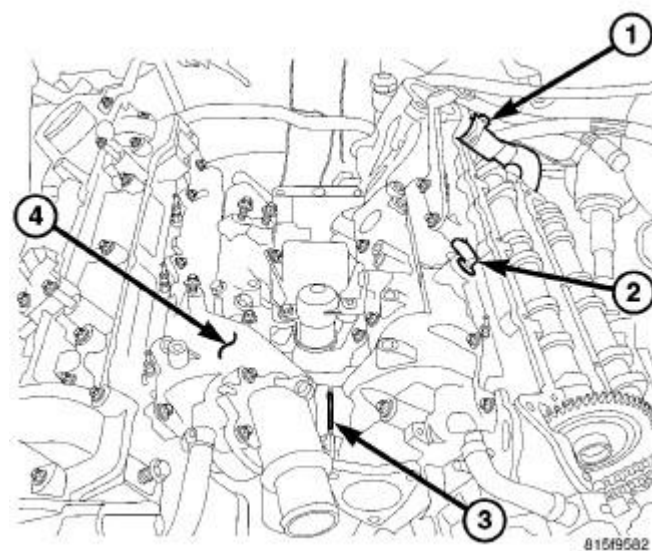
Fig. 76: INTAKE MANIFOLD Courtesy of CHRYSLER LLC
