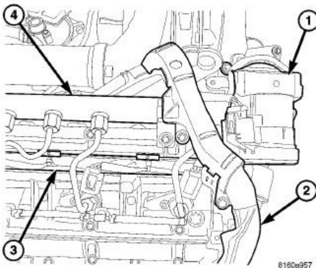
Fig. 302: EGR VALVE WITH MAIN ENGINE WIRING HARNESS
