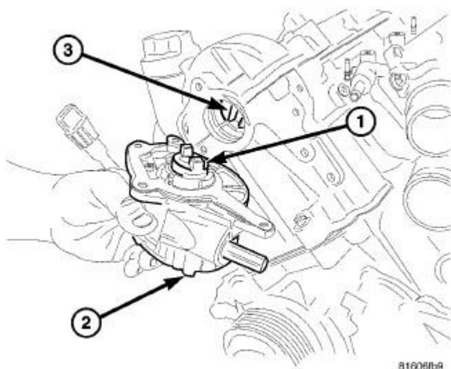
Fig. 384: Vacuum Pump
