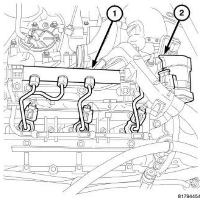
Fig. 486: EGR Valve & Fuel Rail Equalizing Line Courtesy of CHRYSLER LLC
