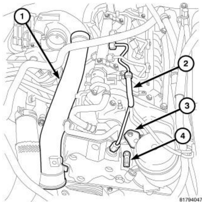
Fig. 242: Charge Air Cooler Inlet Pipe, High Pressure Line, Oil Filter Housing Bracket & Fuel Temperature Sensor Connector Courtesy of CHRYSLER LLC
