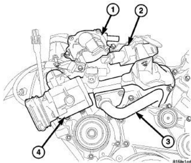
Fig. 153: AIR CONTROL VALVE
