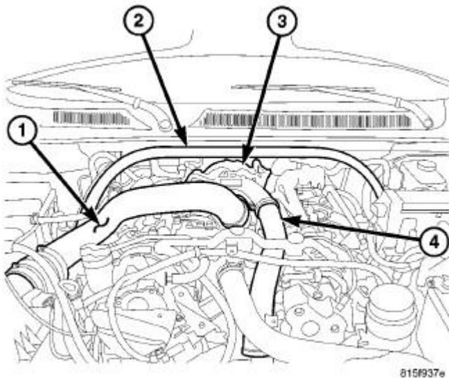
Fig. 550: STRUT TOWER SUPPORT
