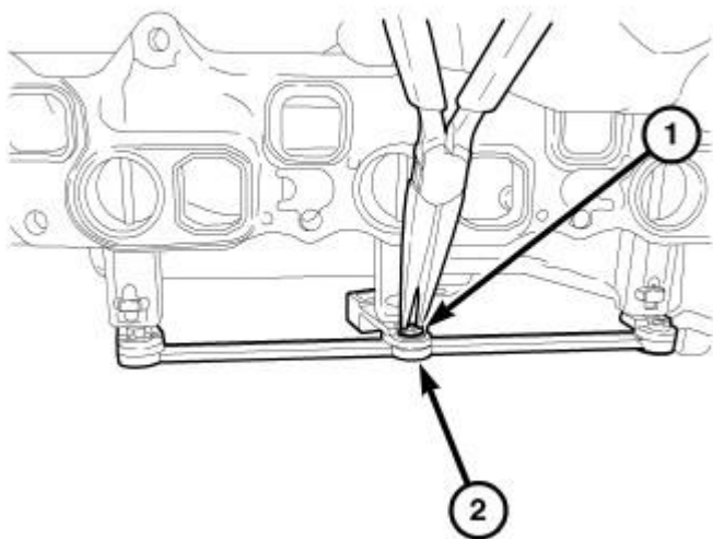
Fig. 489: REMOVE/INSTALL ROUND CLIPS Courtesy of CHRYSLER LLC
