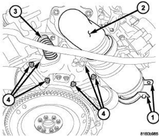
Fig. 484: Removing/Installing Air Intake, Turbo & Exhaust System Components
