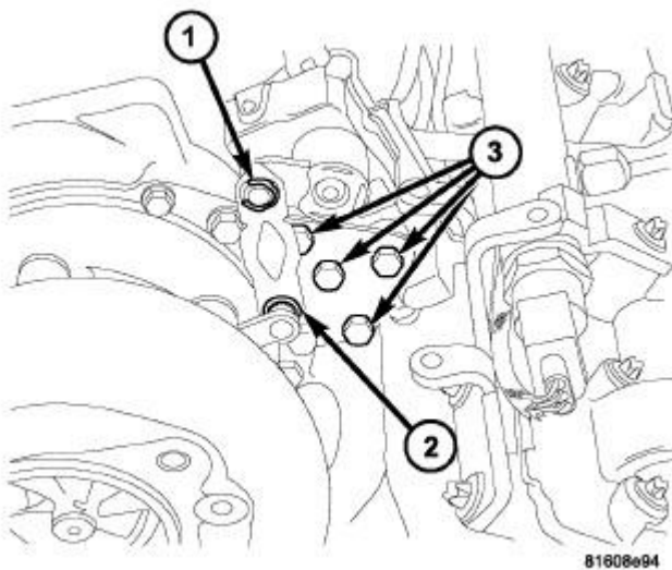
Fig. 543: Identifying Actuator Rod Circlip (1), Actuator Rod At Turbocharger End Circlip (2) & Servomotor & Actuator Rod Courtesy of CHRYSLER LLC
