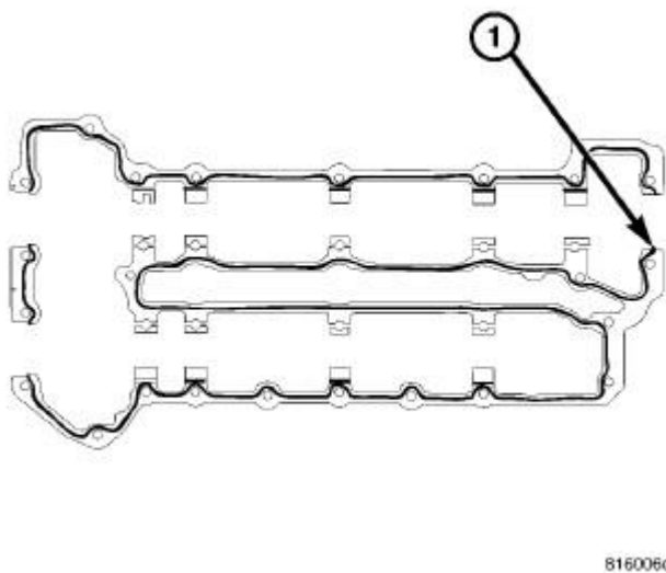
Fig. 306: RIGHT CYLINDER HEAD COVER SEALANT
