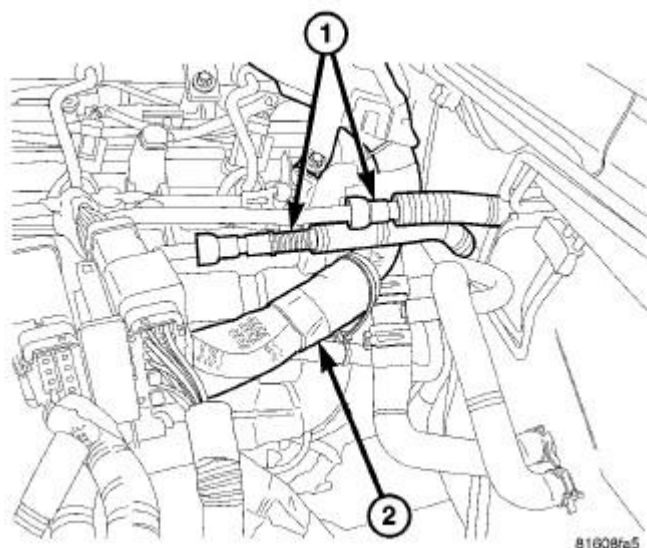
Fig. 17: FUEL LINES Courtesy of CHRYSLER LLC
