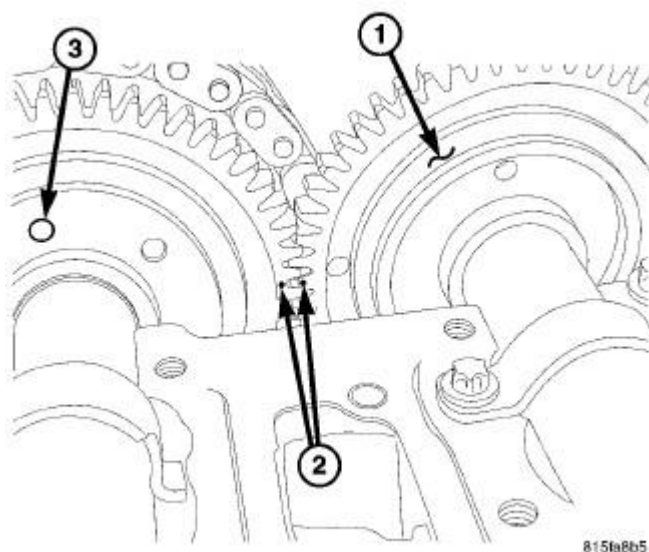
Fig. 91: LEFT CAMSHAFT GEAR ALIGNMENT Courtesy of CHRYSLER LLC
