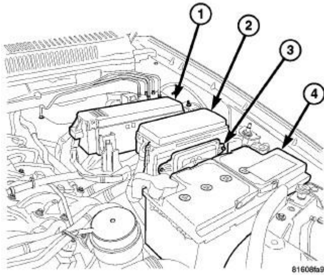
Fig. 27: POWER DISTRIBUTION CENTER AND FRONT CONTROL MODULE Courtesy of CHRYSLER LLC
