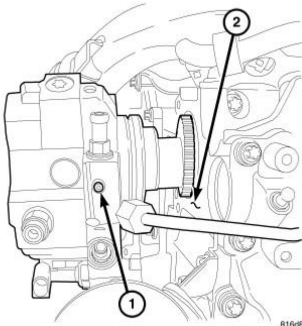
Fig. 80: HIGH PRESSURE PUMP INSTALLATION Courtesy of CHRYSLER LLC
