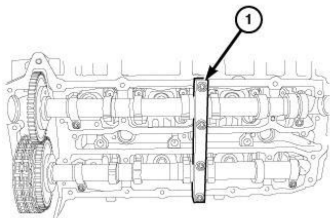
Fig. 137: Camshaft Holding Fixture 9555 Courtesy of CHRYSLER LLC
