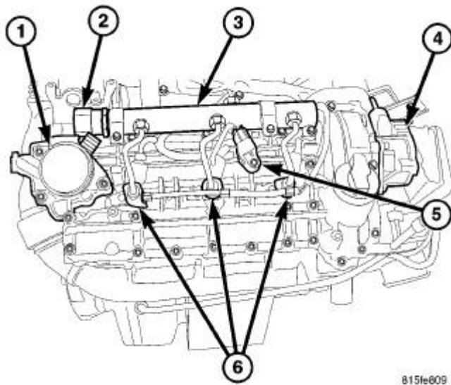
Fig. 244: RIGHT CYLINDER HEAD
