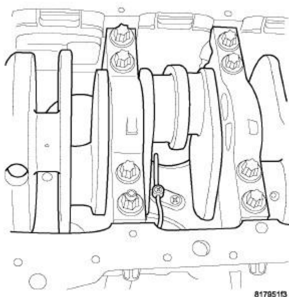
Fig. 336: OIL JET
