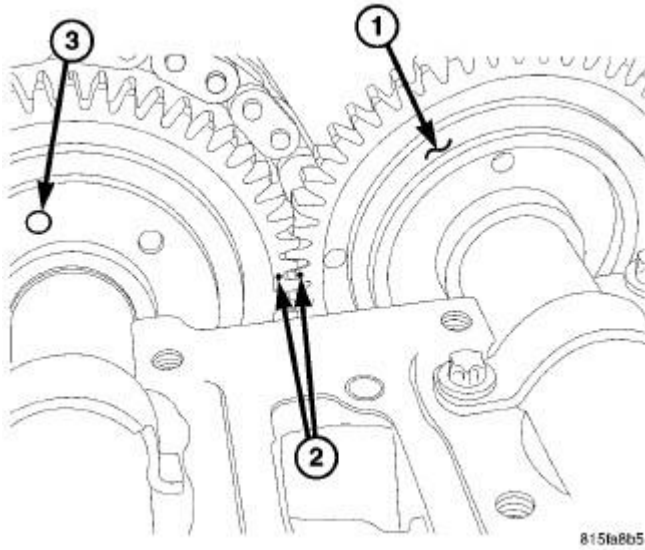
Fig. 369: Camshaft Gear Alignment Courtesy of CHRYSLER LLC
