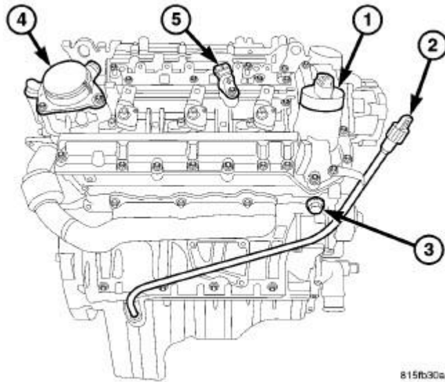
Fig. 381: Timing Chain Tensioner Courtesy of CHRYSLER LLC
