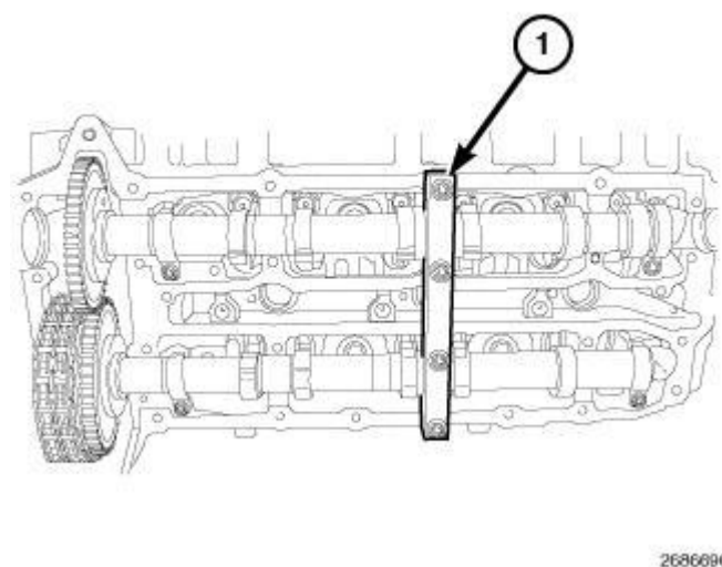
Fig. 174: Camshaft Holding Fixture 9555 Courtesy of CHRYSLER LLC
