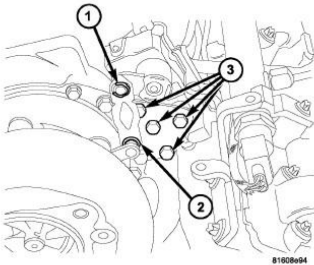
Fig. 544: Identifying Actuator Rod Circlip (1), Actuator Rod At Turbocharger End Circlip (2) & Servomotor & Actuator Rod Courtesy of CHRYSLER LLC
