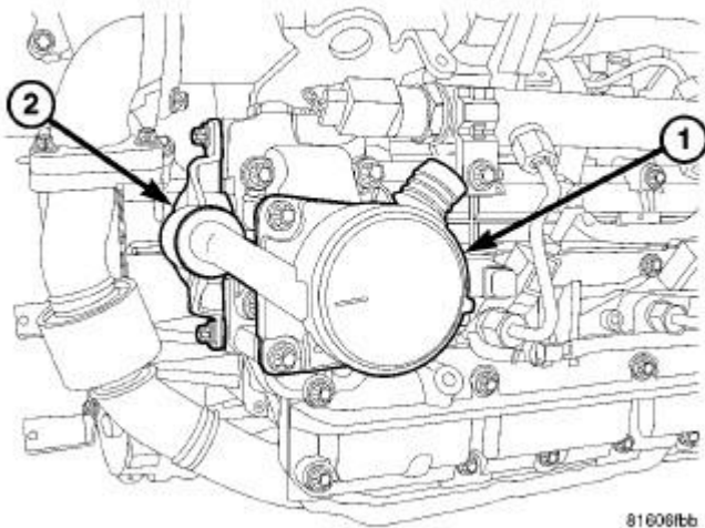
Fig. 531: OIL SEPARATOR
