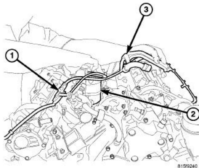
Fig. 326: FUEL FILTER, LINES AND HOSES
