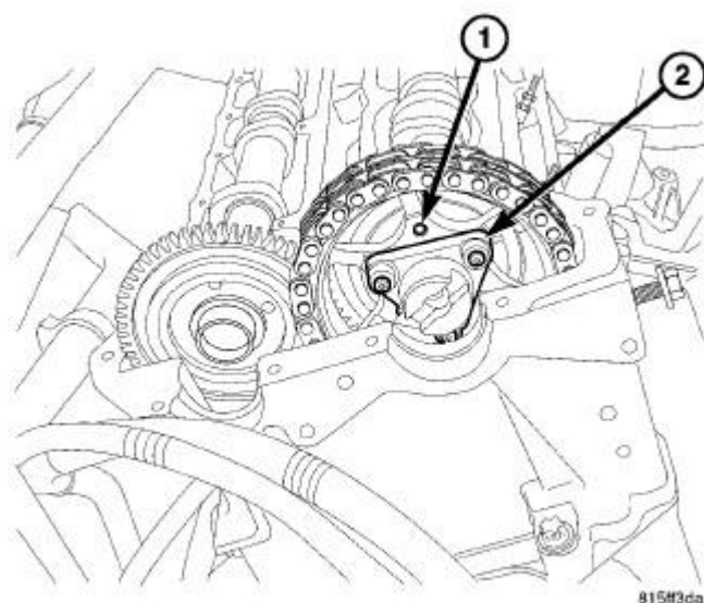
Fig. 165: RIGHT INTAKE CAMSHAFT DRIVE GEAR Courtesy of CHRYSLER LLC
