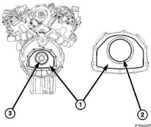
Fig. 409: REAR MAIN SEAL CARRIER Courtesy of CHRYSLER LLC
