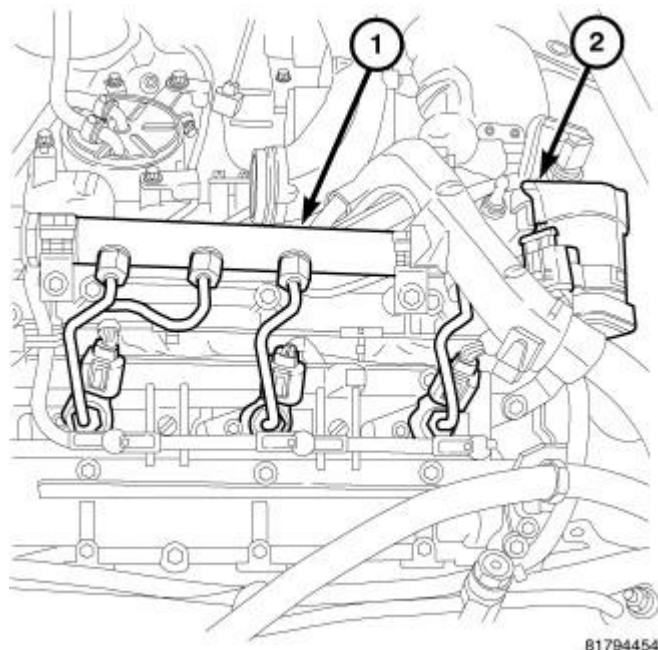
Fig. 266: Exhaust Gas Recirculation Valve Courtesy of CHRYSLER LLC
