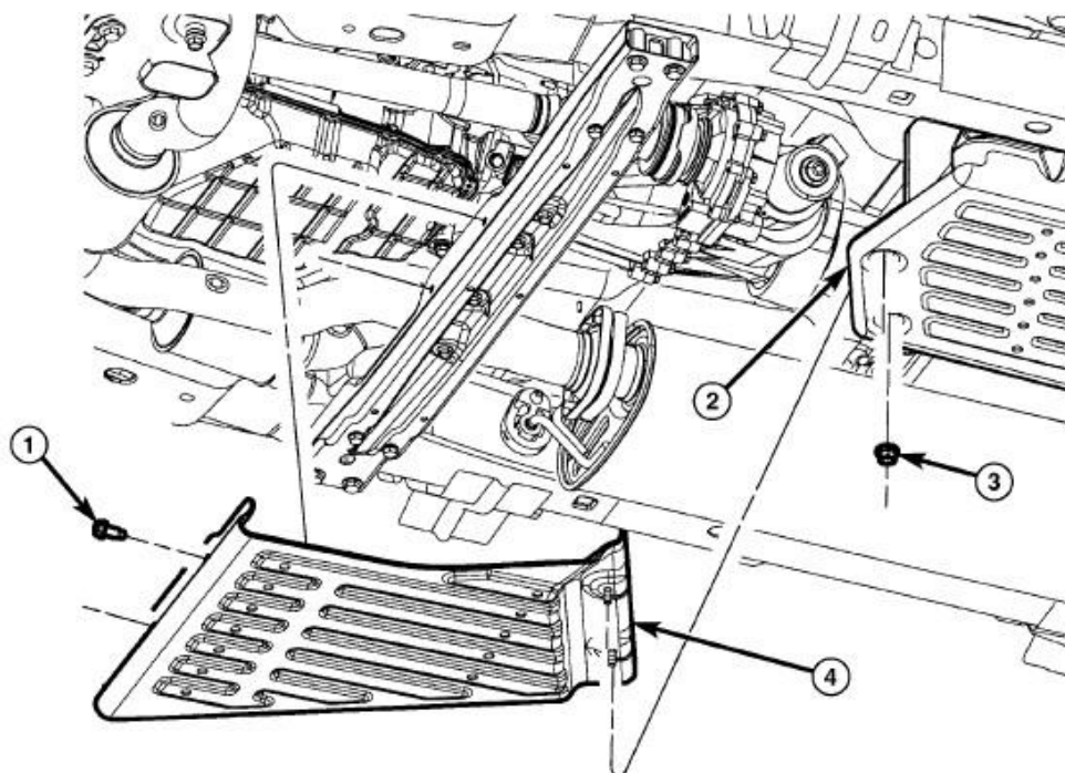
Fig. 511: TRANSFER CASE SKID PLATE Courtesy of CHRYSLER LLC
