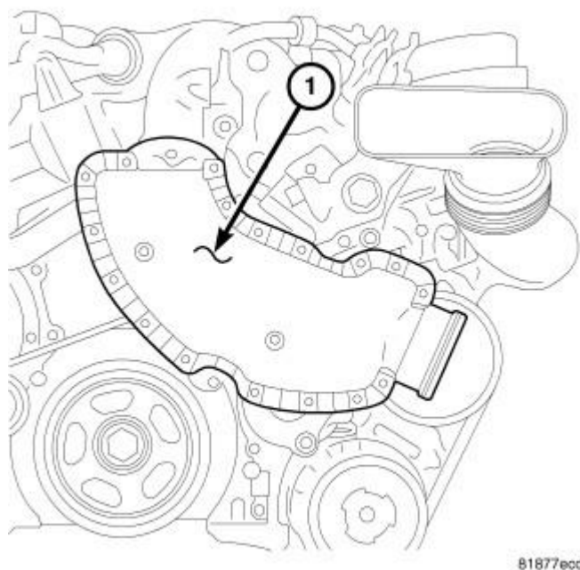
Fig. 60: MIXING CHAMBER Courtesy of CHRYSLER LLC
