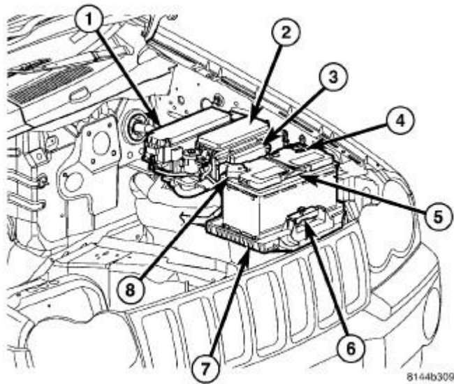
Fig. 237: Identifying Battery System Components, Power Distribution Center & Integrated Power Module
