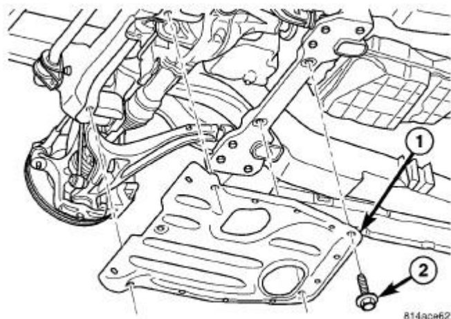
Fig. 101: UPDATED SKID PLATE Courtesy of CHRYSLER LLC
