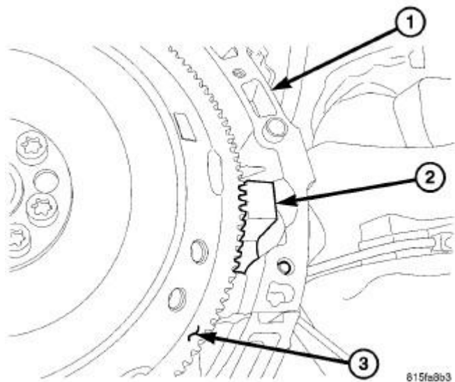
Fig. 87: SPECIAL TOOL 9102 Courtesy of CHRYSLER LLC
