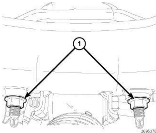
Fig. 432: Right Lower Engine Mount Retaining Nuts Courtesy of CHRYSLER LLC
