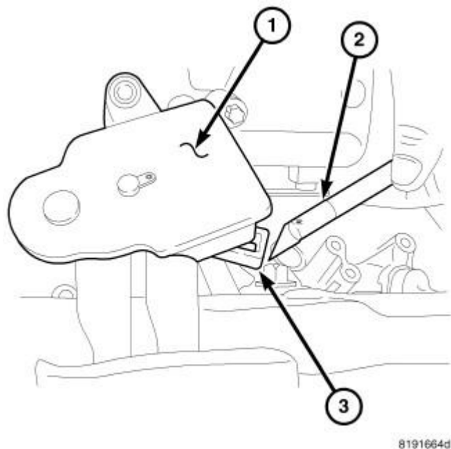
Fig. 478: REMOVE O-RINGS Courtesy of CHRYSLER LLC
