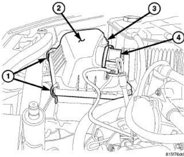
Fig. 595: AIR CLEANER COVER Courtesy of CHRYSLER LLC
