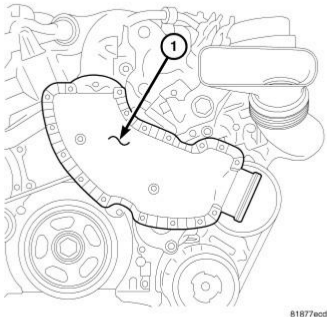
Fig. 52: MIXING CHAMBER Courtesy of CHRYSLER LLC
