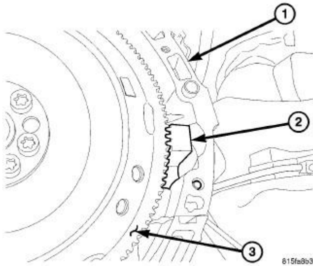
Fig. 605: SPECIAL TOOL 9102 Courtesy of CHRYSLER LLC
