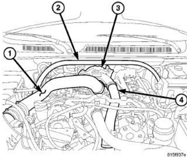
Fig. 66: Strut Tower Support Courtesy of CHRYSLER LLC
