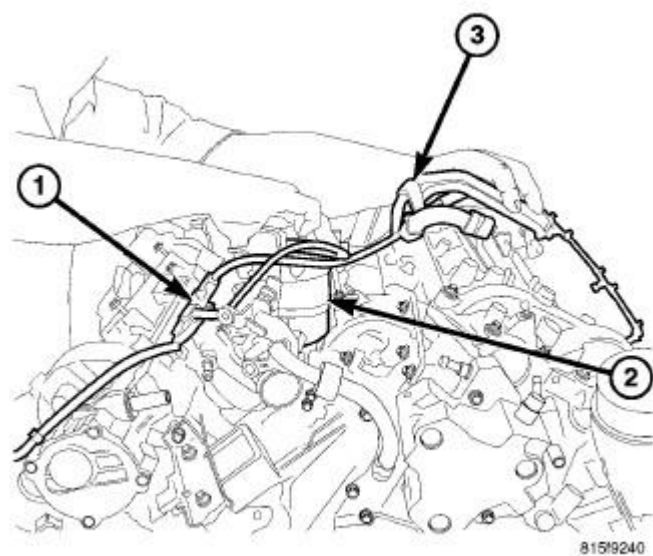
Fig. 284: FUEL FILTER, LINES AND HOSES Courtesy of CHRYSLER LLC
