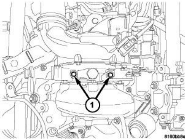
Fig. 558: Removing/Installing Air Intake Tube (Air Cleaner To Turbo)
