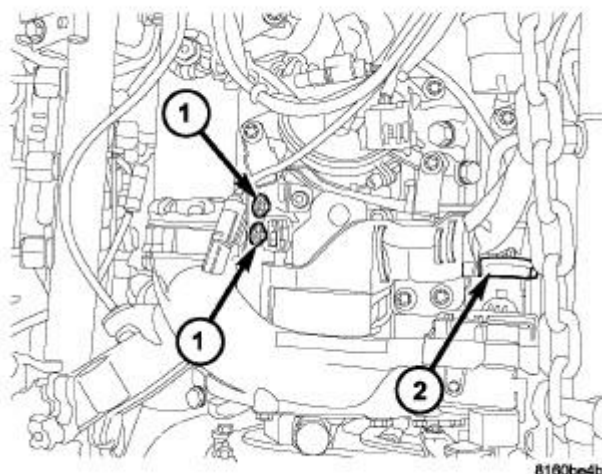
Fig. 560: Removing/Installing Turbo, Shields, Exhaust System & Support Bracket Components Courtesy of CHRYSLER LLC
