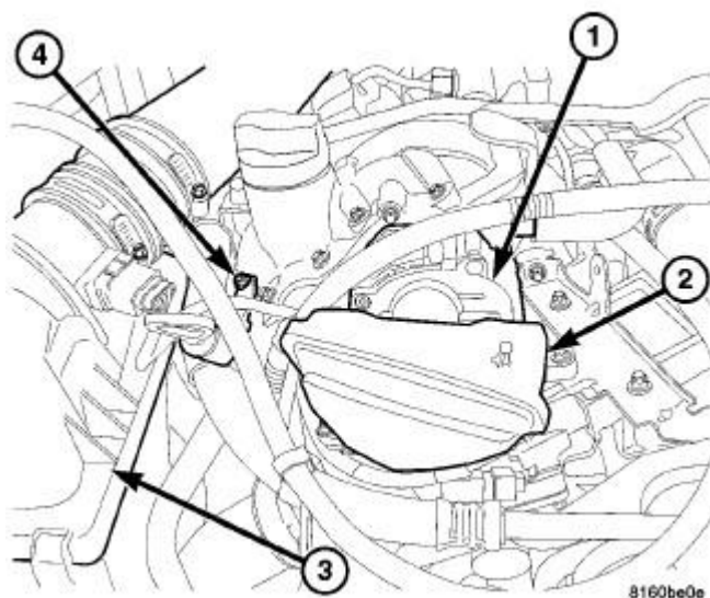
Fig. 293: AIR CONTROL VALVE RESONATOR Courtesy of CHRYSLER LLC
