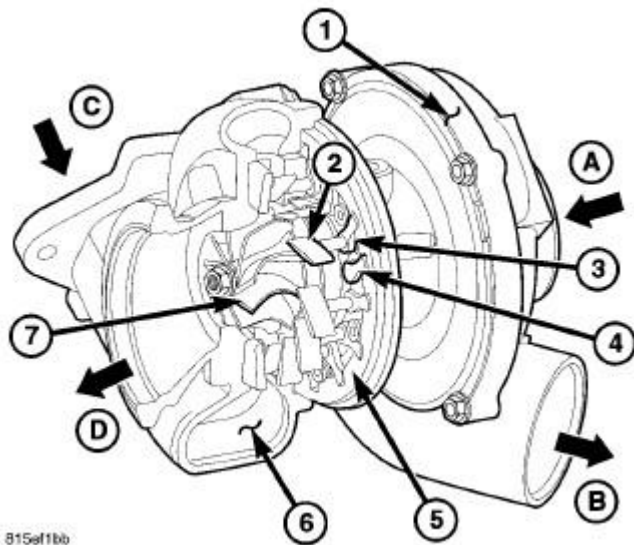
Fig. 543: Turbocharger Components Courtesy of CHRYSLER LLC
