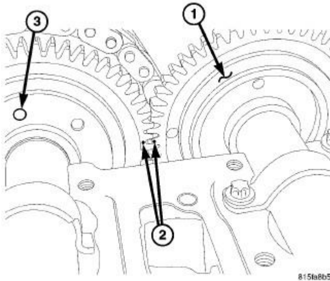
Fig. 82: Camshaft Gear Alignment Courtesy of CHRYSLER LLC
