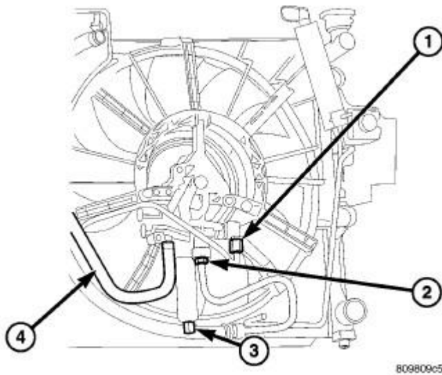
Fig. 71: HYDRAULIC LINES/HOSES AND ELECTRICAL CONNECTOR
