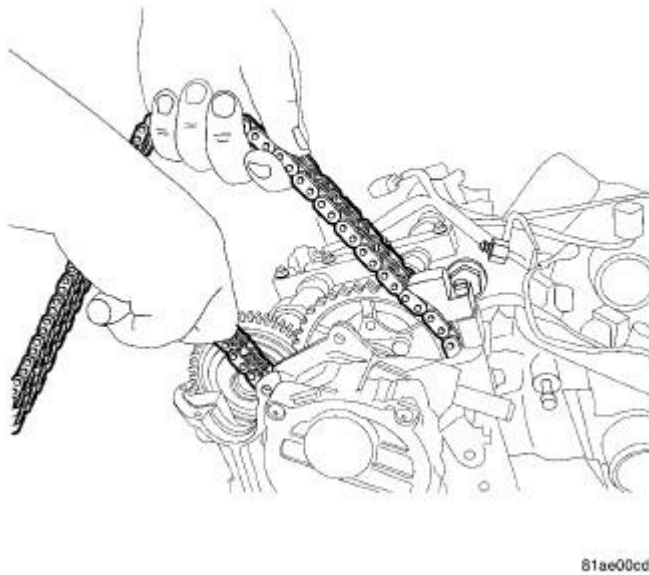
Fig. 588: FEED THE CHAINS THROUGH
