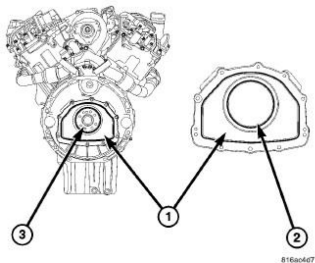
Fig. 333: REAR MAIN SEAL CARRIER
