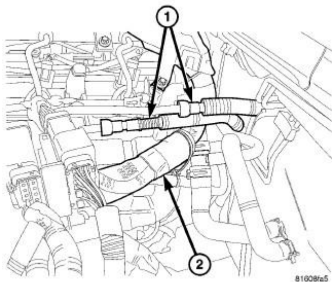
Fig. 283: FUEL LINES Courtesy of CHRYSLER LLC
