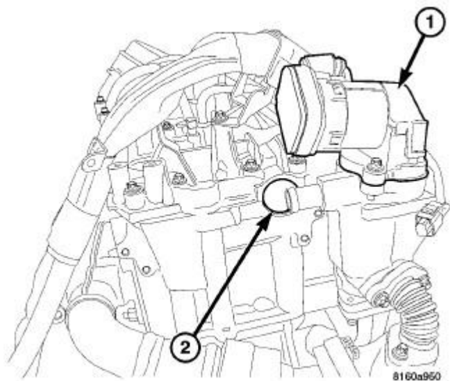
Fig. 204: LEFT REAR CAMSHAFT SEAL Courtesy of CHRYSLER LLC
