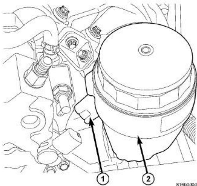
Fig. 449: Oil Filter Housing Courtesy of CHRYSLER LLC
