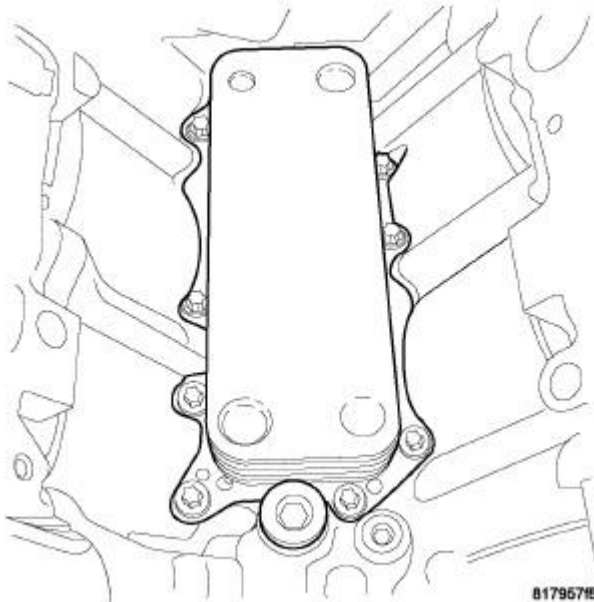
Fig. 445: Heat Exchanger Courtesy of CHRYSLER LLC
