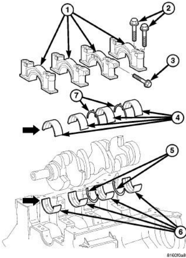
Fig. 321: CRANKSHAFT MAIN BEARINGS AND CAPS Courtesy of CHRYSLER LLC
