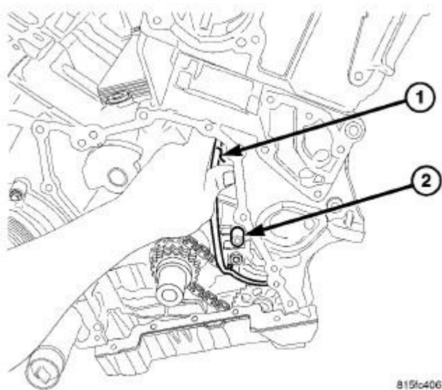
Fig. 582: Left Lower Timing Chain Guide And Fastener Courtesy of CHRYSLER LLC
