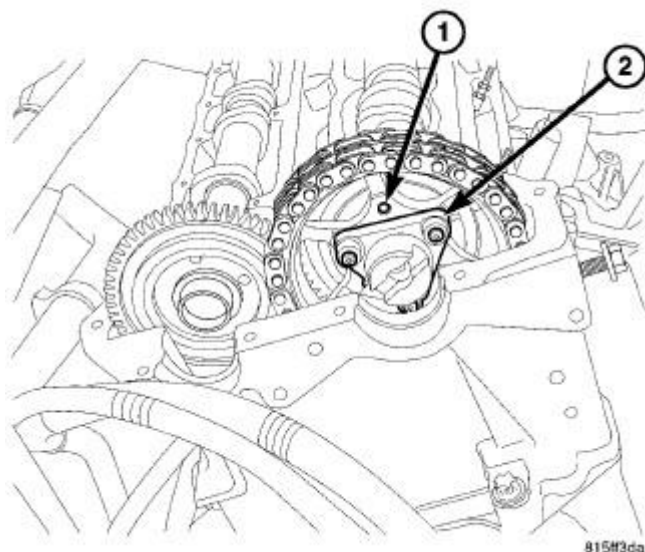
Fig. 214: Right Intake Camshaft Drive Gear Courtesy of CHRYSLER LLC
