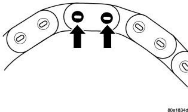
Fig. 594: RIVET INSPECTION Courtesy of CHRYSLER LLC
