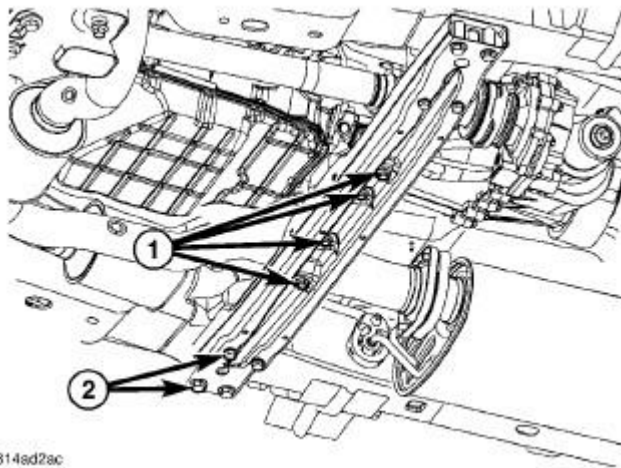
Fig. 515: TRANSFER CASE SKID PLATE
