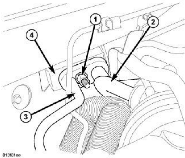
Fig. 68: A/C Expansion Valve Lines Removal/Installation Courtesy of CHRYSLER LLC
