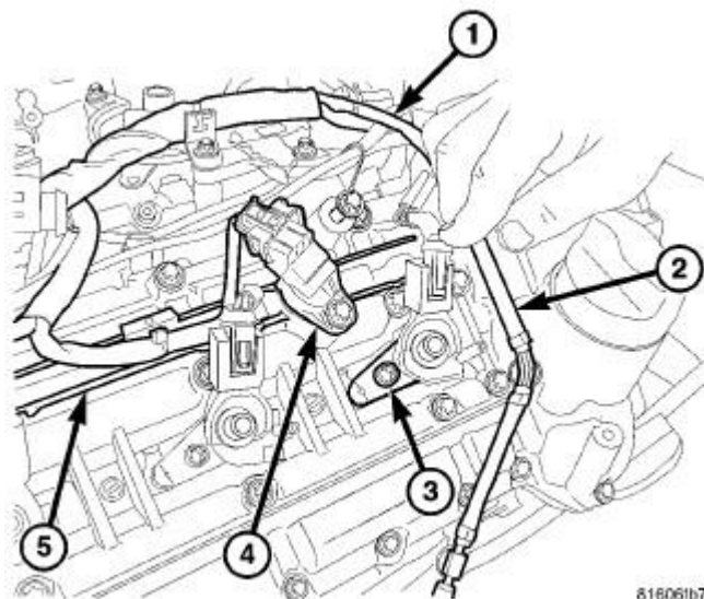
Fig. 257: RIGHT FUEL INJECTORS Courtesy of CHRYSLER LLC
