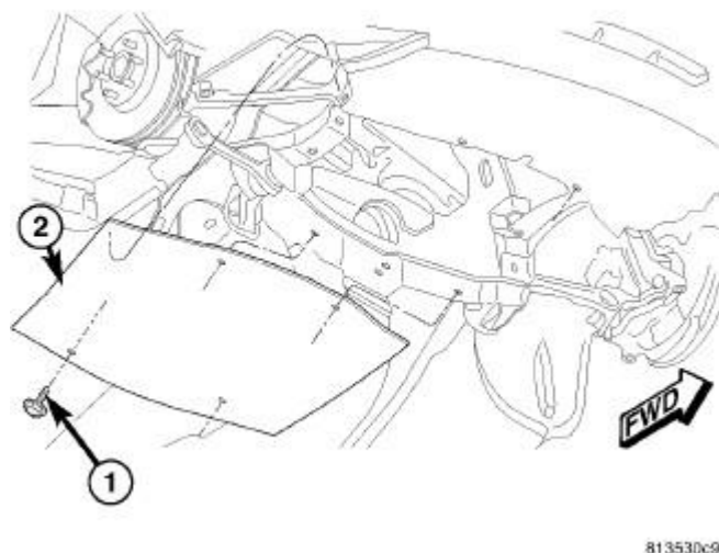
Fig. 435: Rear Belly Pan Courtesy of CHRYSLER LLC
