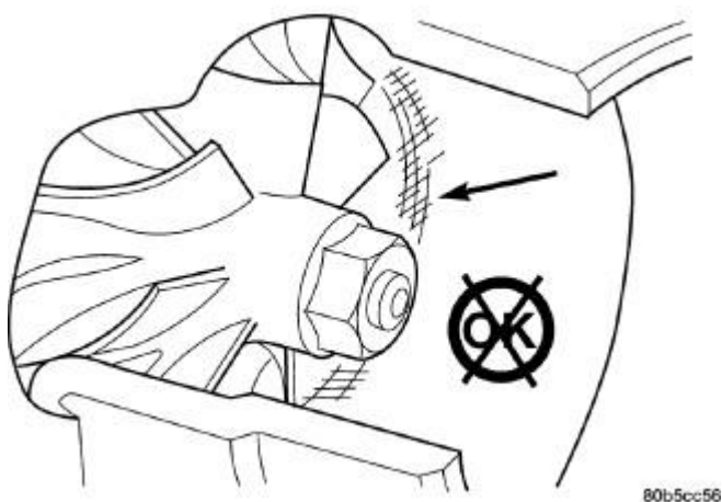
Fig. 555: Inspect Compressor Housing for Impeller Rubbing Condition Courtesy of CHRYSLER LLC
