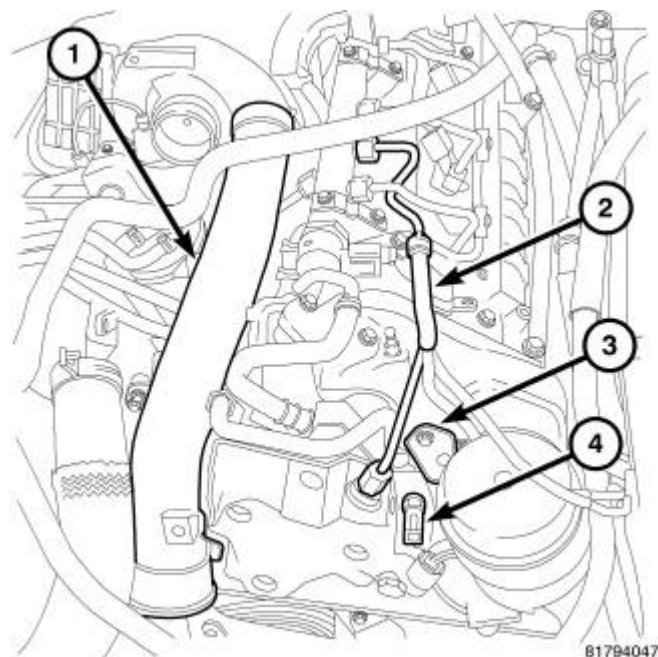
Fig. 229: SENSORS LINE AIRTUBE
