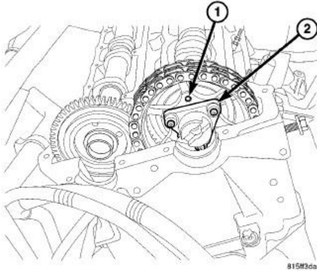
Fig. 372: RIGHT INTAKE CAMSHAFT DRIVE GEAR Courtesy of CHRYSLER LLC
