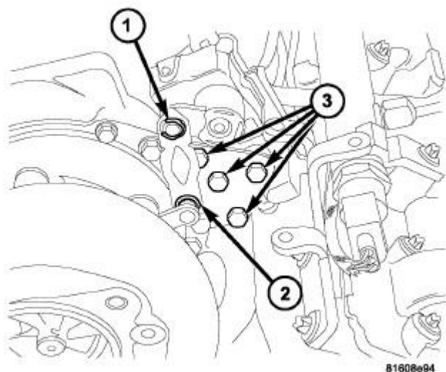
Fig. 545: Identifying Actuator Rod Circlip (1), Actuator Rod At Turbocharger End Circlip (2) & Servomotor & Actuator Rod Courtesy of CHRYSLER LLC
