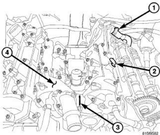
Fig. 539: Intake Manifold & Connections Courtesy of CHRYSLER LLC
