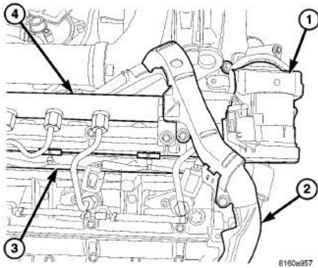
Fig. 207: EXHAUST GAS RECIRCULATION VALVE WITH MAIN ENGINE WIRING HARNESS
