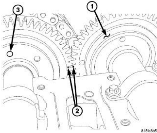
Fig. 201: Camshaft Gear Alignment Courtesy of CHRYSLER LLC
