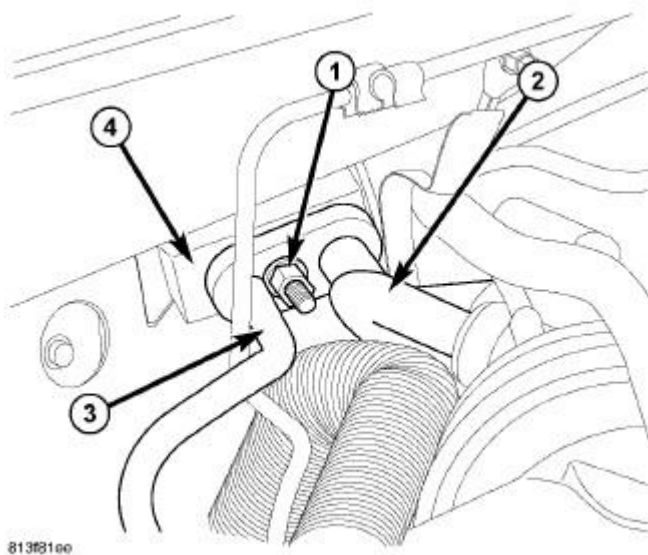
Fig. 150: A/C Expansion Valve Lines - Removal/Installation Courtesy of CHRYSLER LLC
