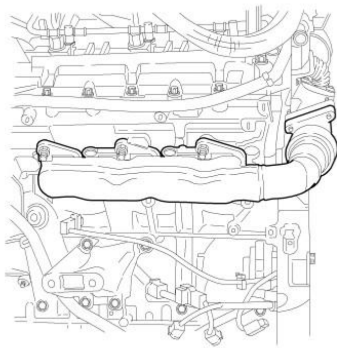
Fig. 513: Exhaust Manifold - Left Courtesy of CHRYSLER LLC
