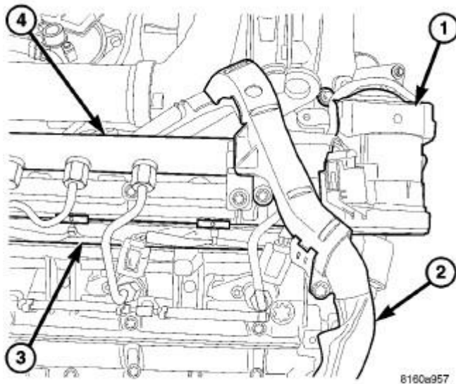
Fig. 286: EXHAUST GAS RECIRCULATION VALVE WITH MAIN ENGINE WIRING HARNESS
