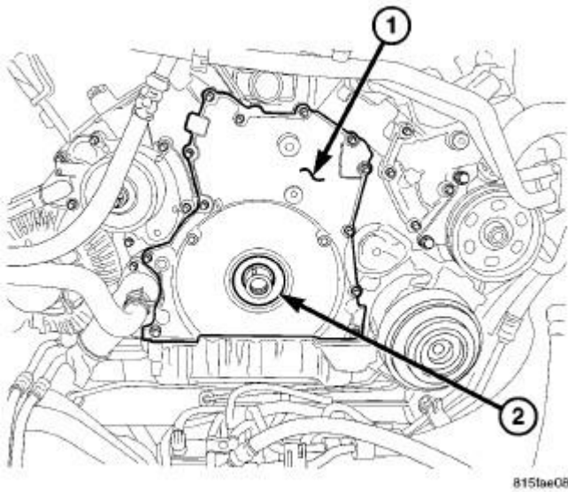
Fig. 401: FRONT TIMING COVER
