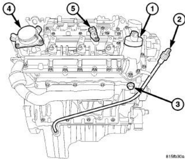
Fig. 166: Timing Chain Tensioner Courtesy of CHRYSLER LLC
