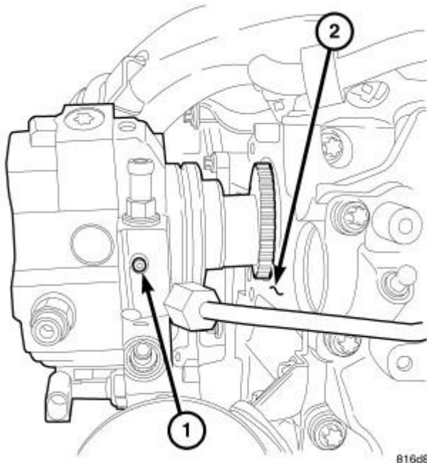
Fig. 80: Removing/Installing High Pressure Pump Courtesy of CHRYSLER LLC
