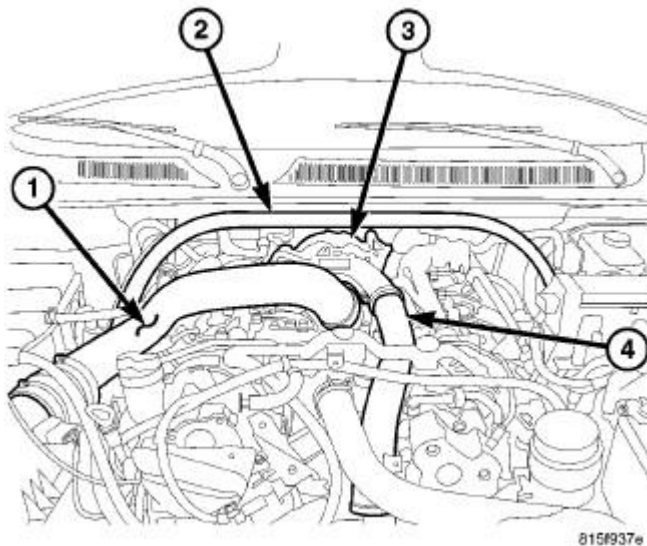
Fig. 480: Strut Tower Support Courtesy of CHRYSLER LLC
