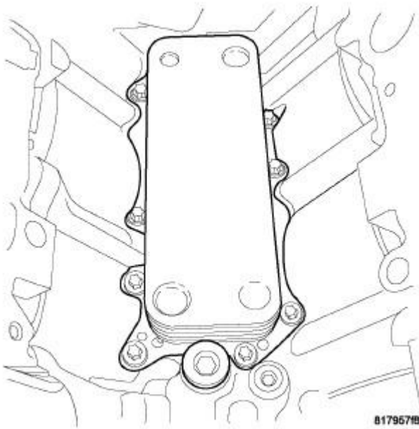
Fig. 441: Heat Exchanger Courtesy of CHRYSLER LLC
