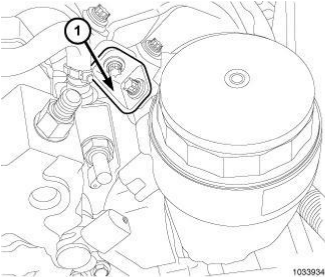
Fig. 452: Oil Filter Housing Upper Bracket
