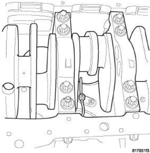
Fig. 393: Oil Jet
