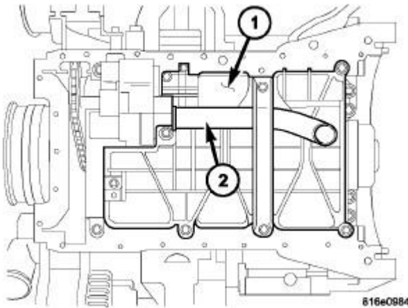
Fig. 467: OIL PUMP COVER REMOVAL
