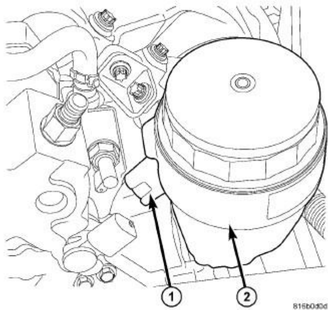
Fig. 345: OIL FILTER HOUSING Courtesy of CHRYSLER LLC
