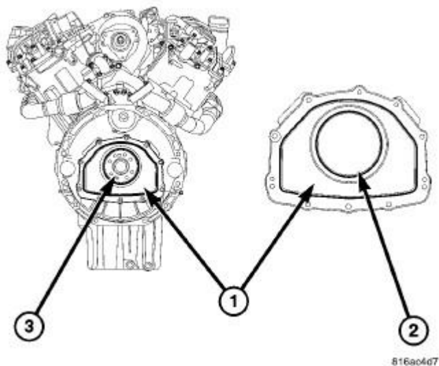
Fig. 406: REAR MAIN SEAL CARRIER
