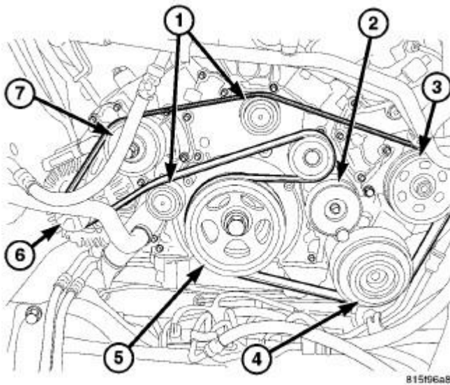
Fig. 77: Accessory Drive Belt Routing Courtesy of CHRYSLER LLC
