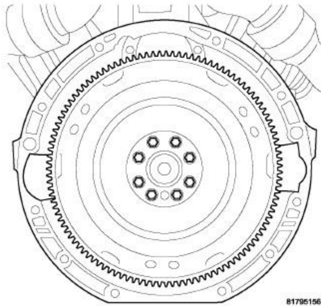
Fig. 461: Flex Plate
