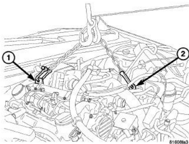
Fig. 350: ENGINE LIFTING POINTS
