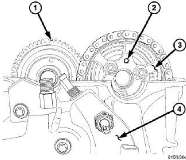
Fig. 579: LEFT EXHAUST CAMSHAFT DRIVE GEAR ALIGNMENT DOWEL Courtesy of CHRYSLER LLC
