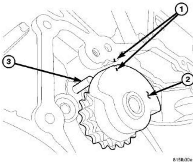
Fig. 371: BALANCE SHAFT INDEXING
