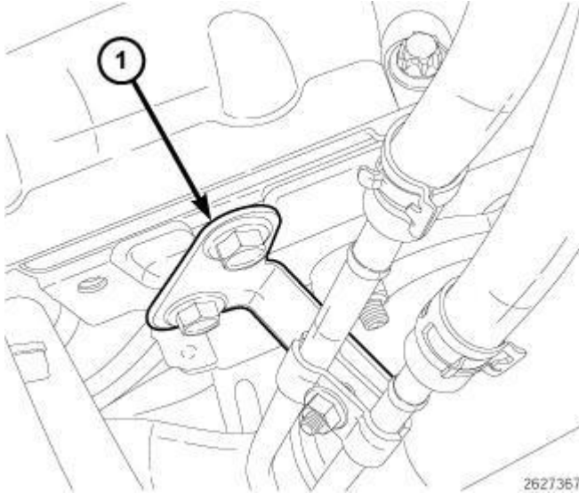
Fig. 516: Differential Pressure Sensor Port Bracket Courtesy of CHRYSLER LLC
