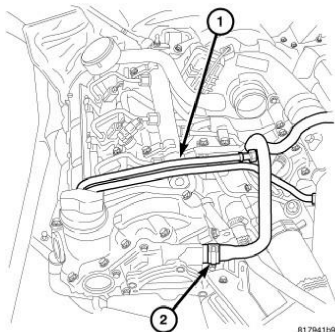
Fig. 256: Power Brake Booster Vacuum Line Courtesy of CHRYSLER LLC
