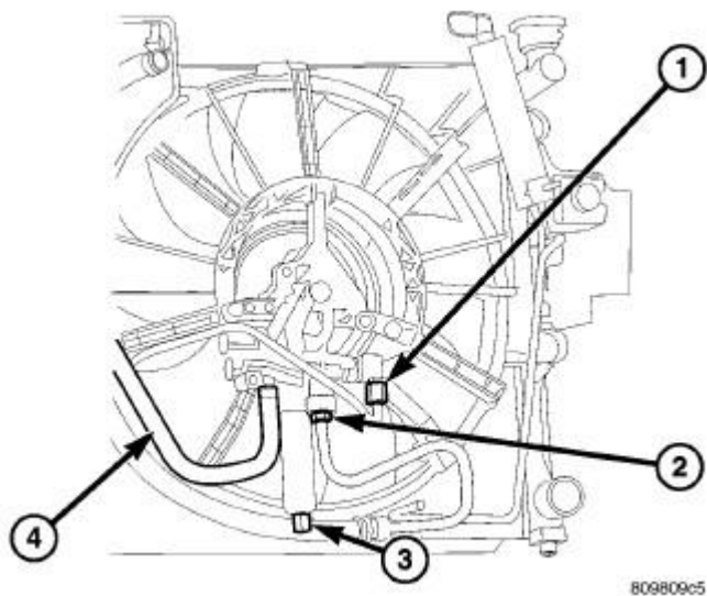
Fig. 184: HYDRAULIC LINES/HOSES AND ELECTRICAL CONNECTOR
