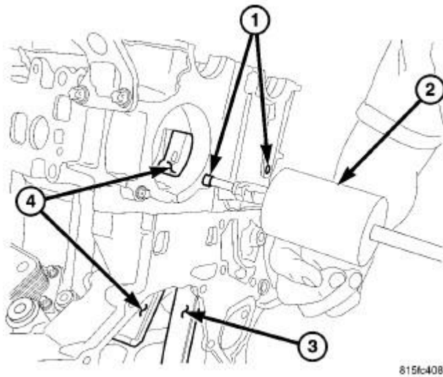
Fig. 565: LEFT UPPER TIMING CHAIN GUIDE PIN EXTRACTION Courtesy of CHRYSLER LLC
