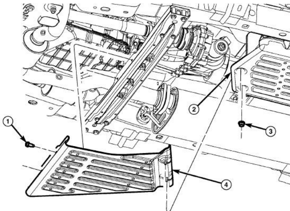
Fig. 499: TRANSFER CASE SKID PLATE Courtesy of CHRYSLER LLC
