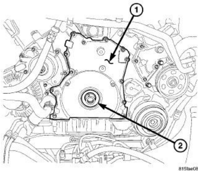
Fig. 171: FRONT TIMING COVER Courtesy of CHRYSLER LLC
