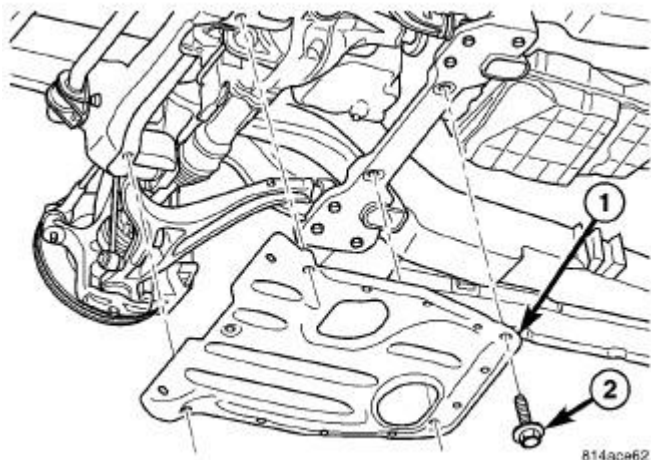
Fig. 498: UPDATED SKID PLATE Courtesy of CHRYSLER LLC
