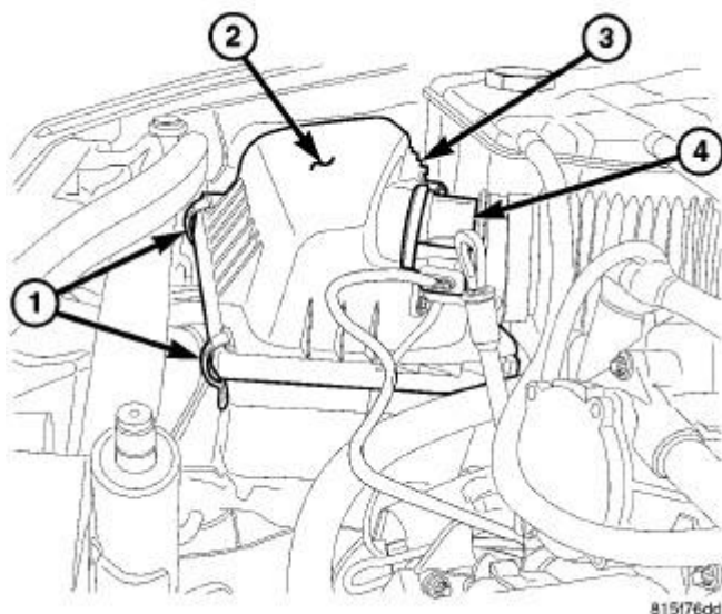
Fig. 57: AIR CLEANER COVER Courtesy of CHRYSLER LLC
