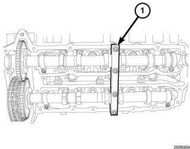
Fig. 92: Camshaft Holding Fixture 9555
