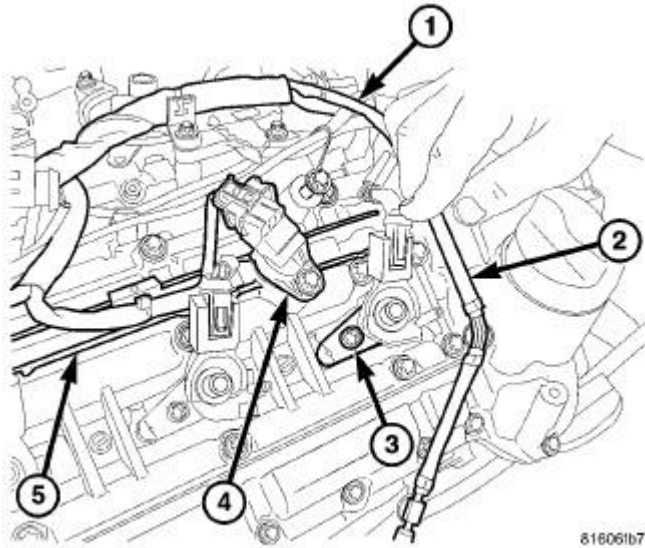
Fig. 242: RIGHT FUEL INJECTORS
