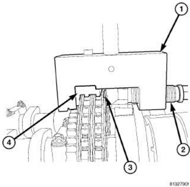
Fig. 593: Install Moving Assembly Insert 9312-11A To 9312-1 Courtesy of CHRYSLER LLC
