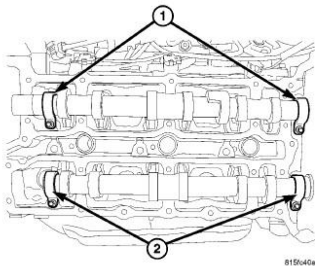
Fig. 199: CAMSHAFT RETAINERS Courtesy of CHRYSLER LLC
