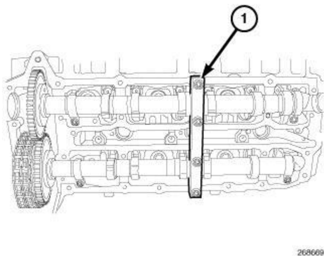
Fig. 365: Camshaft Holding Fixture 9555 Courtesy of CHRYSLER LLC
