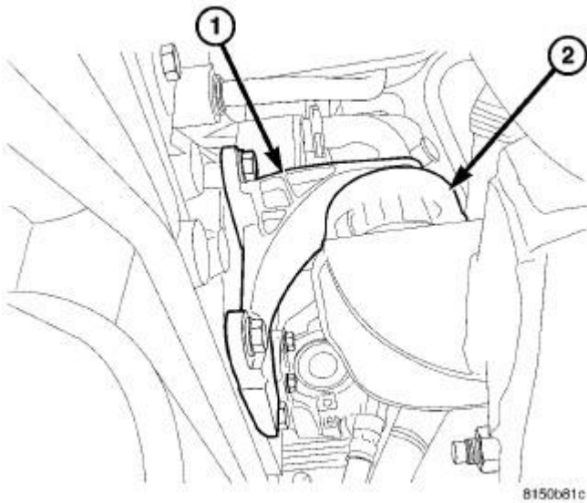
Fig. 430: RIGHT ENGINE MOUNT Courtesy of CHRYSLER LLC
