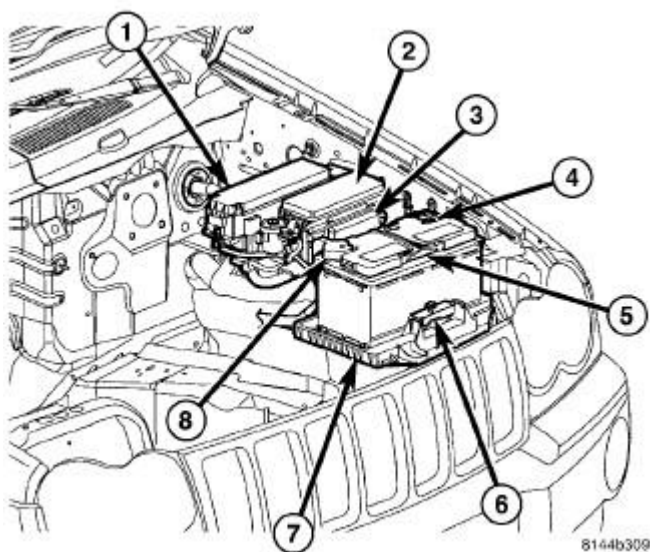
Fig. 492: Identifying Battery System Components, Power Distribution Center & Integrated Power Module
