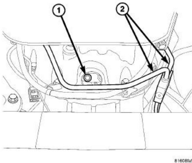
Fig. 19: TORQUE CONVERTER TO FLEX PLATE BOLTS
