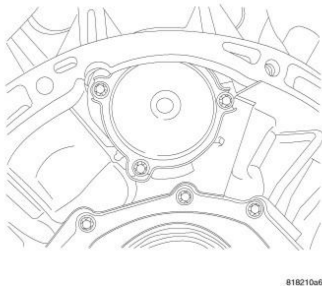
Fig. 377: BALANCE SHAFT REAR COVER
