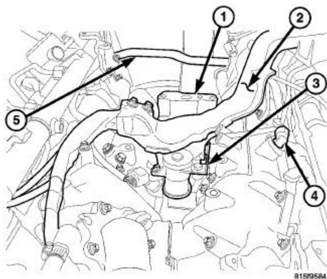
Fig. 491: MAIN ENGINE WIRING HARNESS
