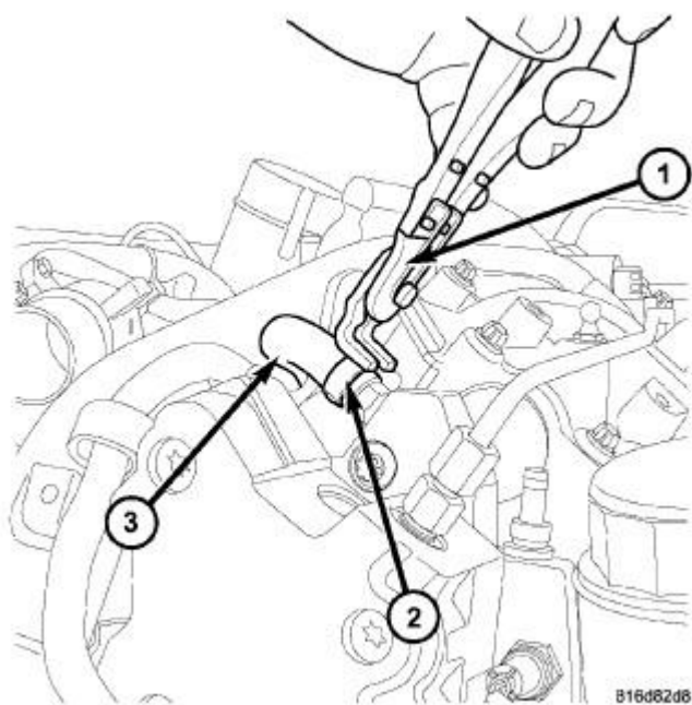
Fig. 267: PUMP FUEL LINE PLIERS
