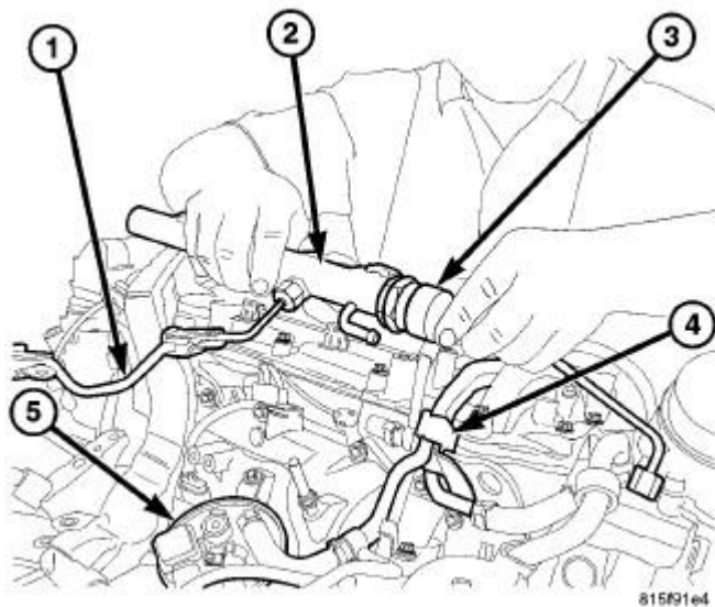
Fig. 265: LEFT FUEL RAIL Courtesy of CHRYSLER LLC
