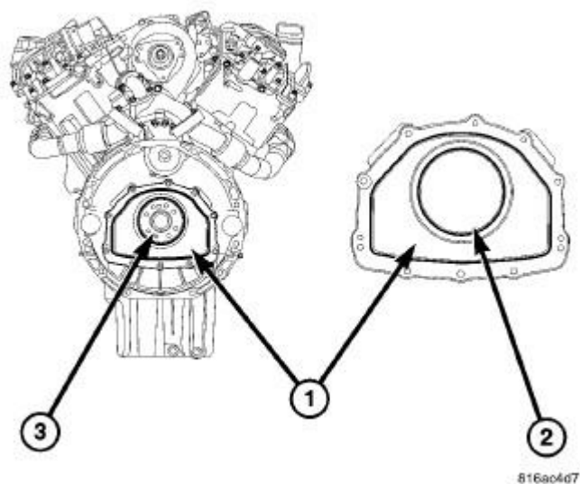
Fig. 337: REAR MAIN SEAL CARRIER Courtesy of CHRYSLER LLC
