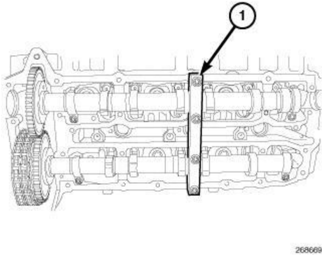
Fig. 81: Camshaft Holding Fixture 9555 Courtesy of CHRYSLER LLC
