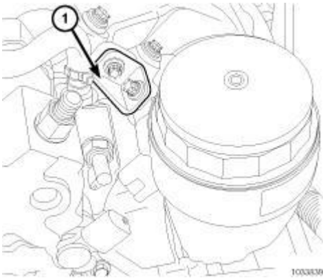
Fig. 451: Oil Filter Housing Upper Bracket Courtesy of CHRYSLER LLC
