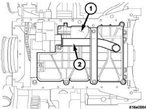
Fig. 463: OIL PUMP COVER REMOVAL
