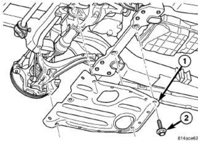
Fig. 530: UPDATED SKID PLATE
