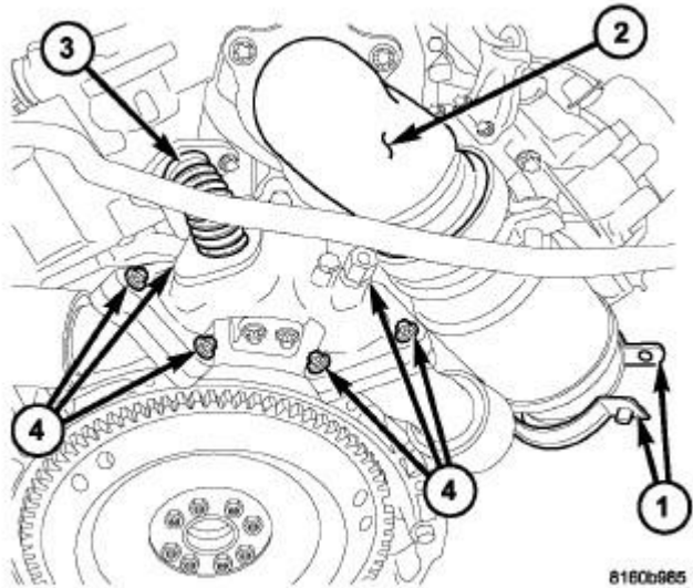
Fig. 347: REAR OF ENGINE TURBO Courtesy of CHRYSLER LLC
