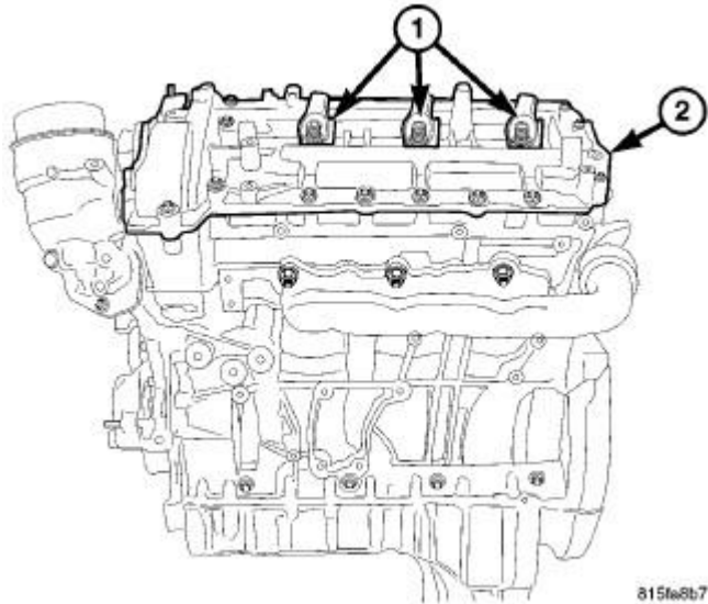
Fig. 299: LEFT CYLINDER HEAD COVER Courtesy of CHRYSLER LLC
