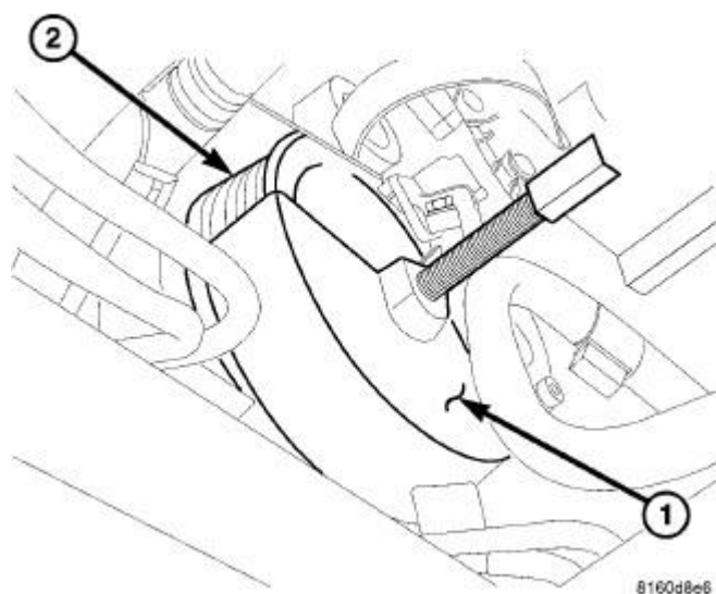
Fig. 400: SPECIAL TOOL #9544 VIBRATION DAMPER PULLER Courtesy of CHRYSLER LLC
