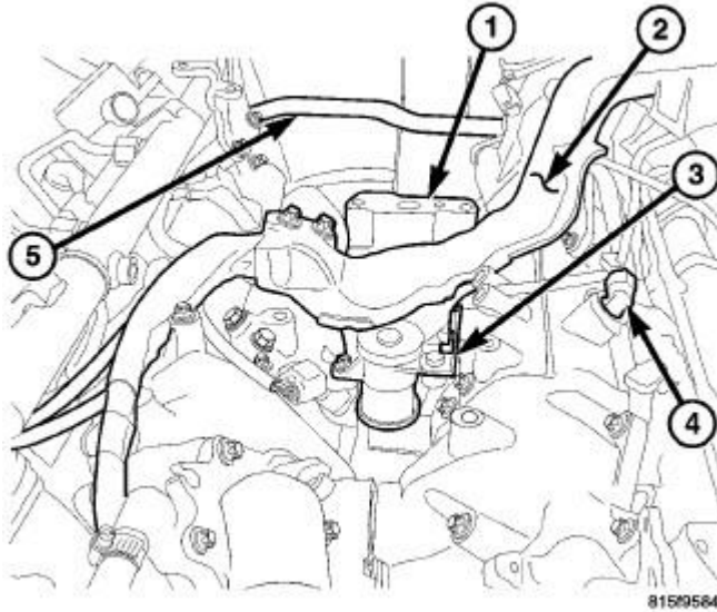
Fig. 179: MAIN ENGINE WIRING HARNESS Courtesy of CHRYSLER LLC
