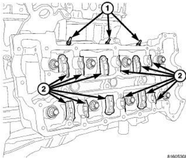
Fig. 161: RIGHT TAPPET/CAMSHAFT FOLLOWER POSITION Courtesy of CHRYSLER LLC
