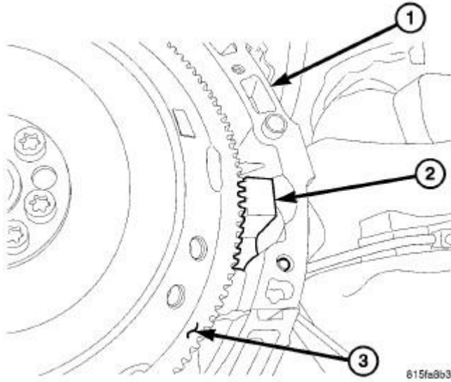
Fig. 143: SPECIAL TOOL 9102 Courtesy of CHRYSLER LLC
