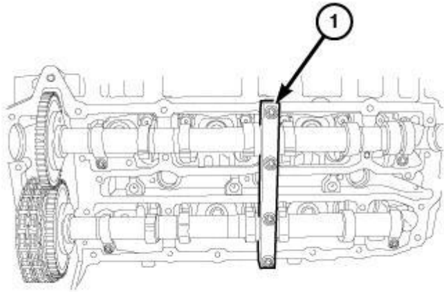
Fig. 144: Camshaft Holding Fixture 9555
