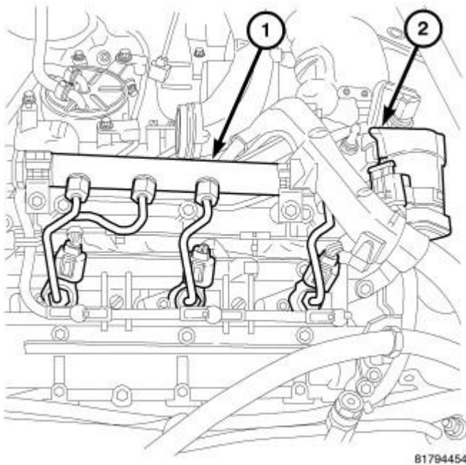
Fig. 598: Exhaust Gas Recirculation Valve Courtesy of CHRYSLER LLC
