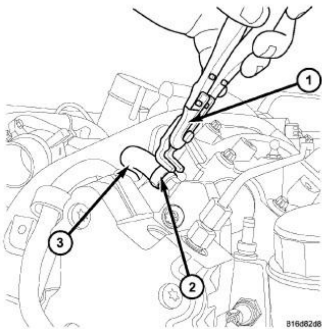
Fig. 255: PUMP FUEL LINE PLIERS
