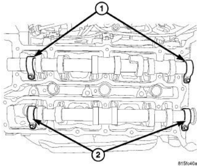
Fig. 124: CAMSHAFT RETAINERS
