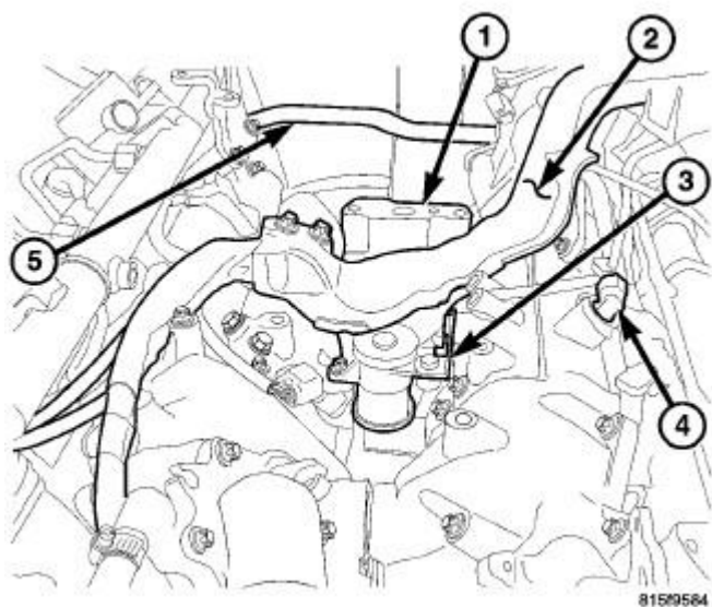
Fig. 479: MAIN ENGINE WIRING HARNESS Courtesy of CHRYSLER LLC
