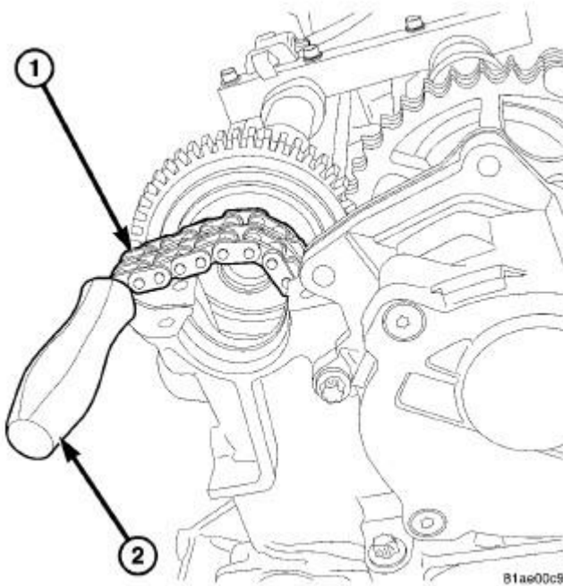
Fig. 583: PREVENT CHAIN FROM FALLING Courtesy of CHRYSLER LLC
