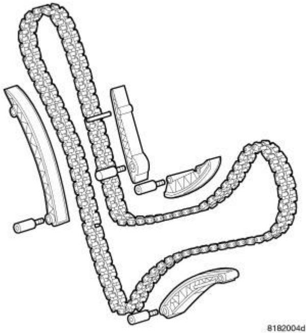
Fig. 562: TIMING CHAIN AND GUIDES
