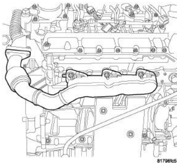
Fig. 328: RIGHT EXHAUST MANIFOLD Courtesy of CHRYSLER LLC
