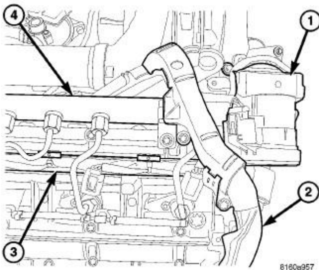
Fig. 302: EXHAUST GAS RECIRCULATION VALVE WITH MAIN ENGINE WIRING
