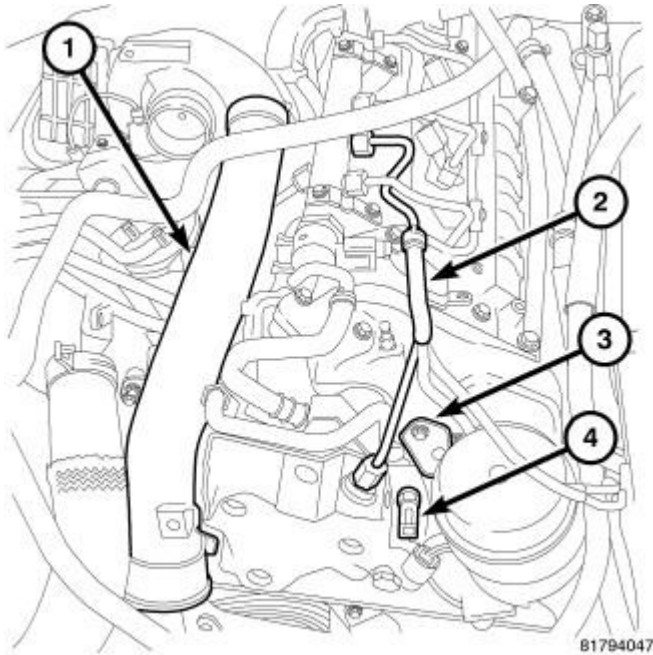
Fig. 269: SENSORS LINE AIRTUBE
