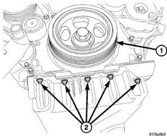
Fig. 602: Vibration Damper & Front Oil Pan Bolts Courtesy of CHRYSLER LLC
