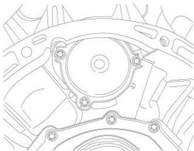
Fig. 383: BALANCE SHAFT REAR COVER Courtesy of CHRYSLER LLC
