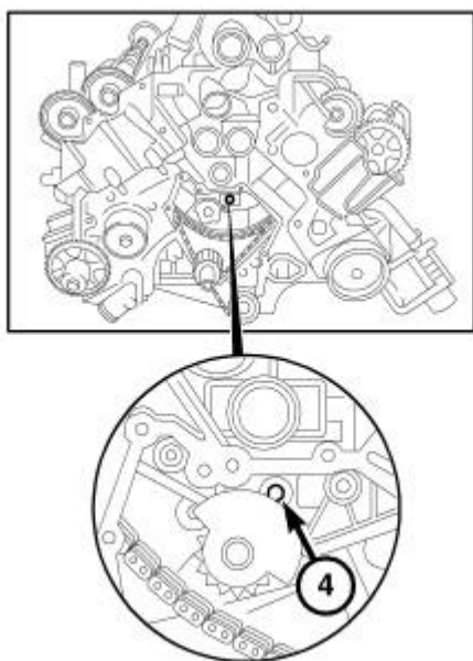
Fig. 382: BALANCE SHAFT ALIGNMENT FRONT Courtesy of CHRYSLER LLC
