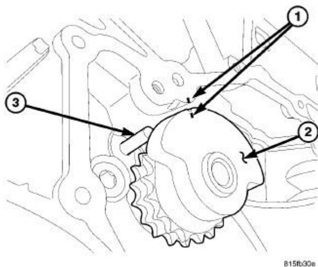
Fig. 86: BALANCE SHAFT INDEXING Courtesy of CHRYSLER LLC
