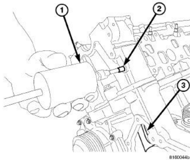
Fig. 125: UPPER TIMING CHAIN GUIDE AND PIN Courtesy of CHRYSLER LLC
