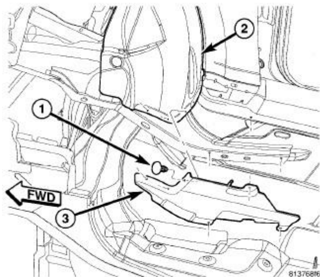
Fig. 416: Removing/Installing Shield Courtesy of CHRYSLER LLC
