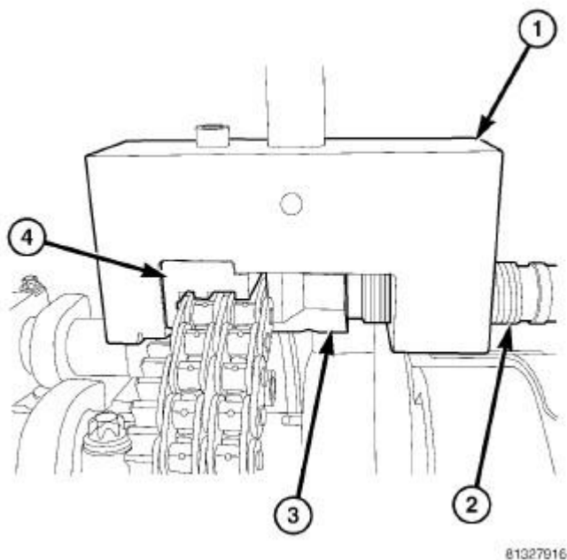
Fig. 592: Installing Moving Assembly Insert 9312-11A To 9312-1 Courtesy of CHRYSLER LLC
