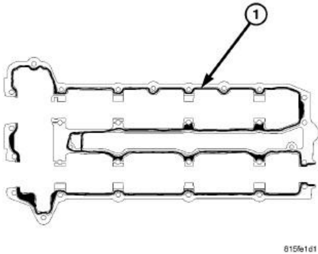
Fig. 262: Applying Cylinder Head Cover Sealant Courtesy of CHRYSLER LLC
