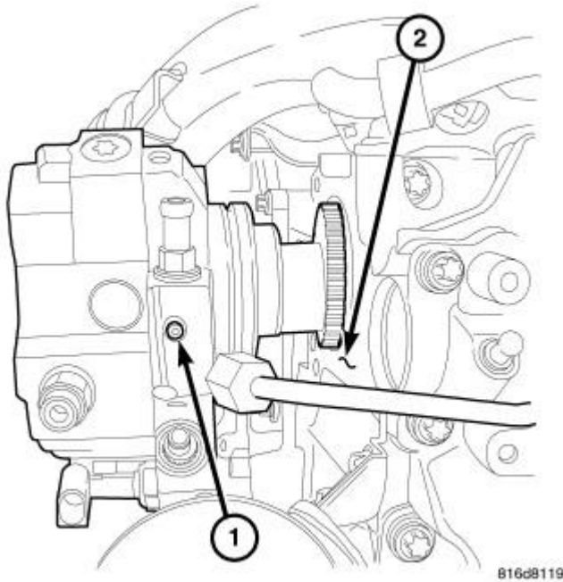
Fig. 146: Removing/Installing High Pressure Pump Courtesy of CHRYSLER LLC
