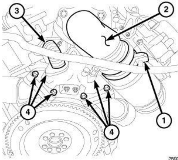
Fig. 527: Left Exhaust Manifold To Crossover Pipe Retaining Bolts Courtesy of CHRYSLER LLC
