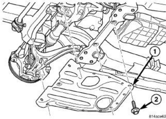
Fig. 69: UPDATED SKID PLATE Courtesy of CHRYSLER LLC
