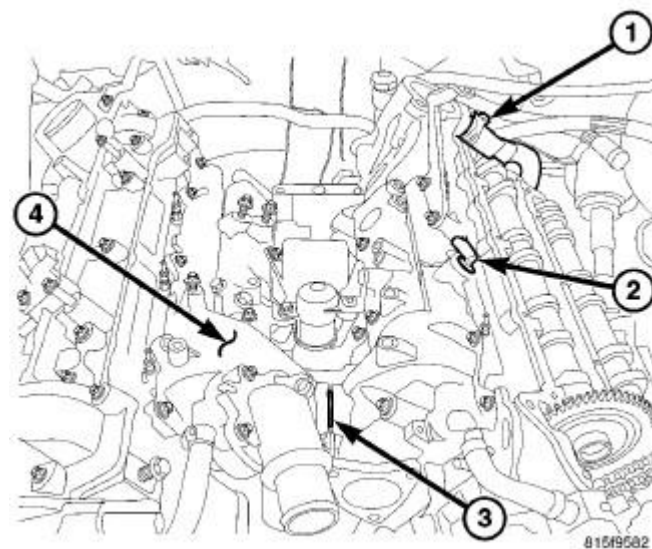
Fig. 76: INTAKE MANIFOLD
