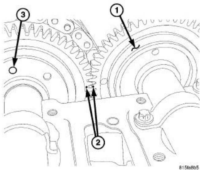
Fig. 580: Camshaft Gear Alignment Courtesy of CHRYSLER LLC
