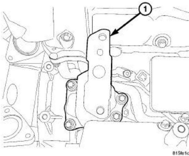
Fig. 181: TURBOCHARGER ADAPTOR Courtesy of CHRYSLER LLC
