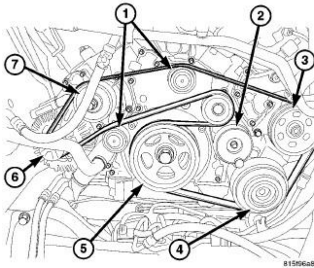
Fig. 366: Accessory Drive Belt Routing Courtesy of CHRYSLER LLC
