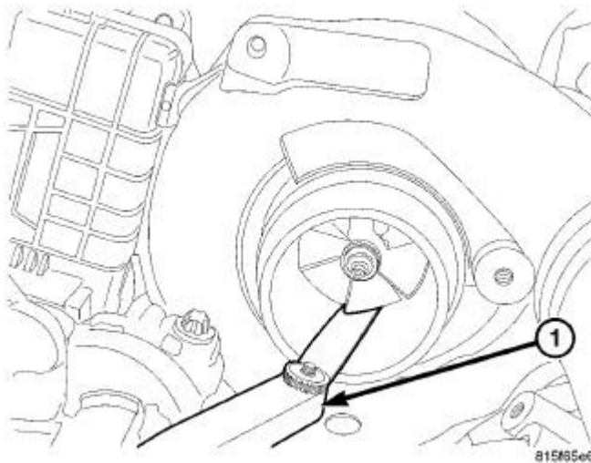
Fig. 557: TURBOCHARGER RADIAL BEARING CLEARANCE Courtesy of CHRYSLER LLC
