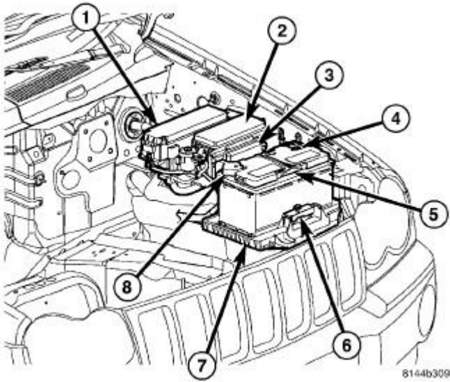
Fig. 504: Identifying Battery System Components, Power Distribution Center & Integrated Power Module
