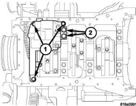
Fig. 464: OIL PUMP
