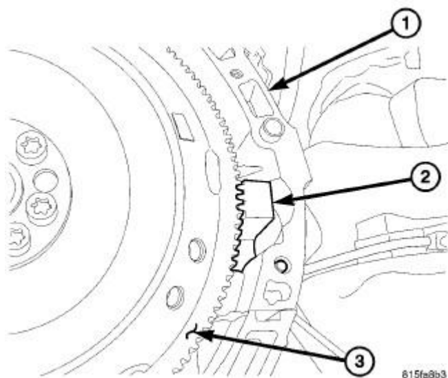
Fig. 185: SPECIAL TOOL 9102 Courtesy of CHRYSLER LLC
