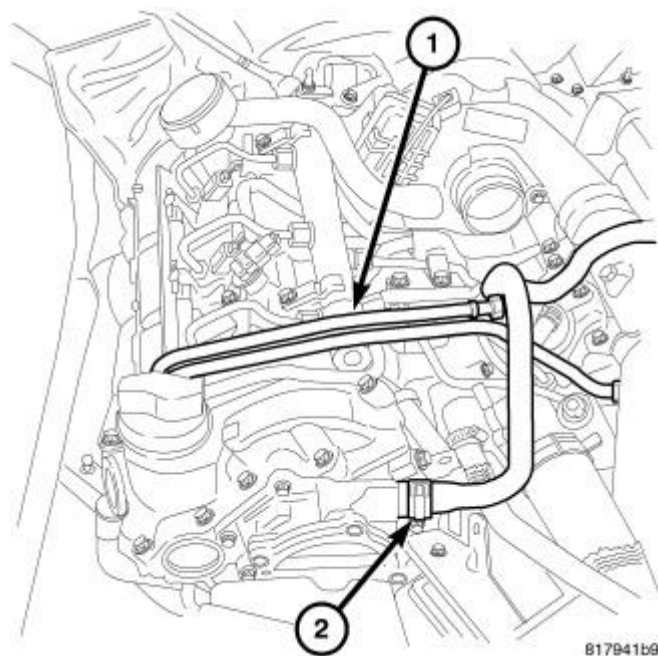
Fig. 268: Power Brake Booster Vacuum Line
