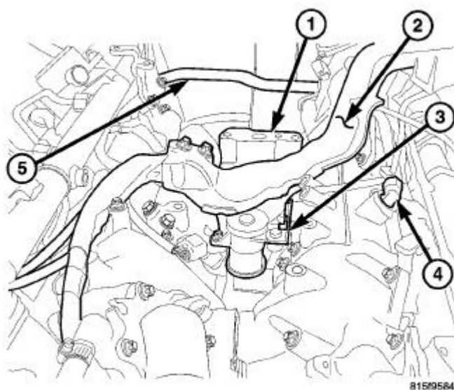
Fig. 73: MAIN ENGINE WIRING HARNESS Courtesy of CHRYSLER LLC
