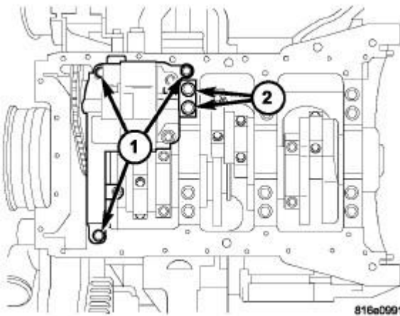
Fig. 392: OIL PUMP
