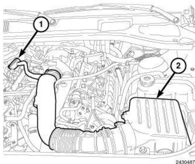
Fig. 442: Air Cleaner Assembly Courtesy of CHRYSLER LLC
