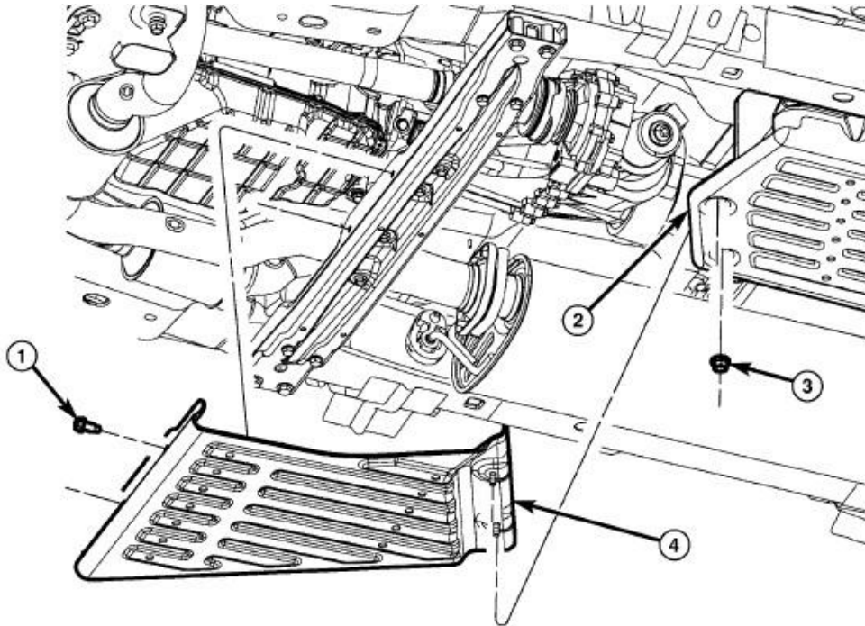
Fig. 529: TRANSFER CASE SKID PLATE Courtesy of CHRYSLER LLC
