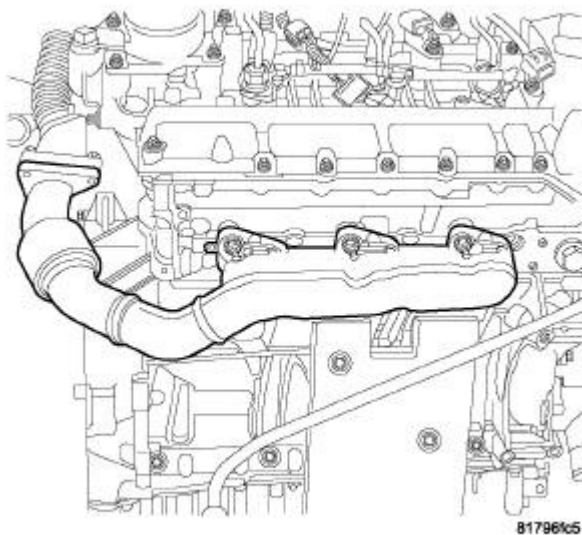
Fig. 497: RIGHT EXHAUST MANIFOLD
