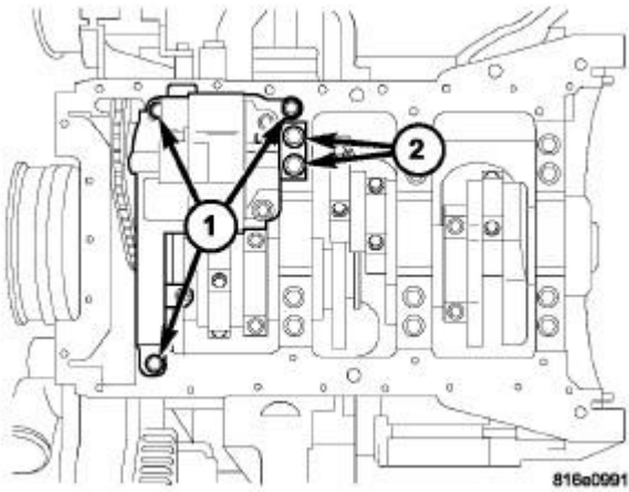
Fig. 466: OIL PUMP
