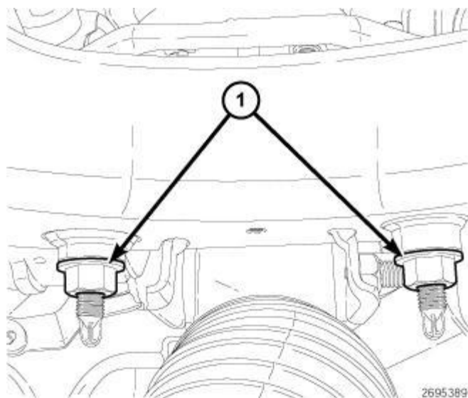
Fig. 422: Left Lower Engine Mount Retaining Nuts Courtesy of CHRYSLER LLC
