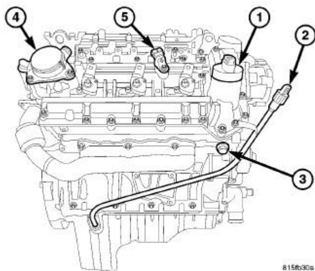
Fig. 253: Timing Chain Tensioner Courtesy of CHRYSLER LLC
