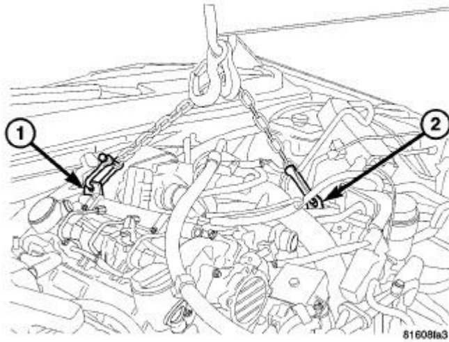
Fig. 391: ENGINE LIFTING POINTS
