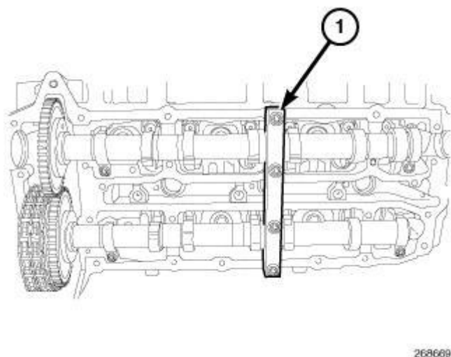
Fig. 123: Camshaft Holding Fixture 9555
