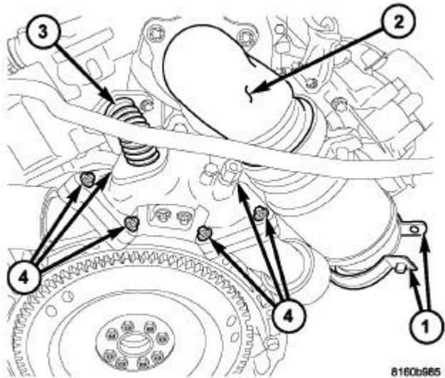
Fig. 484: REAR OF ENGINE TURBO Courtesy of CHRYSLER LLC
