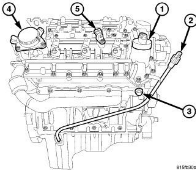
Fig. 196: Timing Chain Tensioner Courtesy of CHRYSLER LLC
