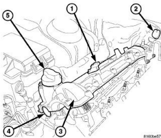
Fig. 297: RIGHT CYLINDER HEAD COVER
