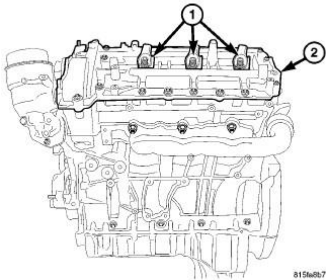
Fig. 301: LEFT CYLINDER HEAD COVER Courtesy of CHRYSLER LLC
