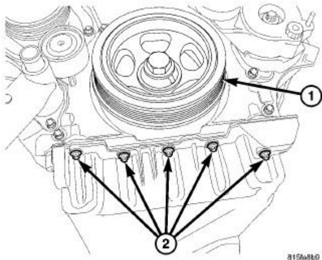
Fig. 172: Vibration Damper & Front Oil Pan Bolts Courtesy of CHRYSLER LLC
