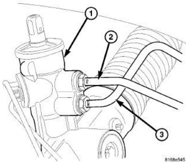
Fig. 102: LINES AT GEAR Courtesy of CHRYSLER LLC
