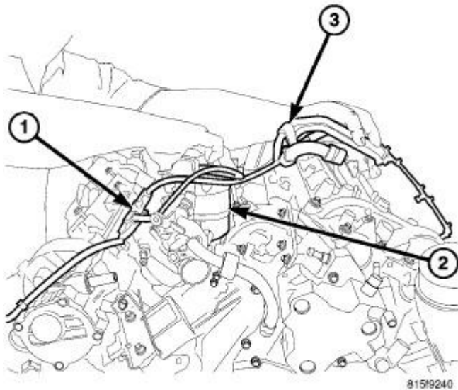
Fig. 348: FUEL FILTER, LINES AND HOSES Courtesy of CHRYSLER LLC
