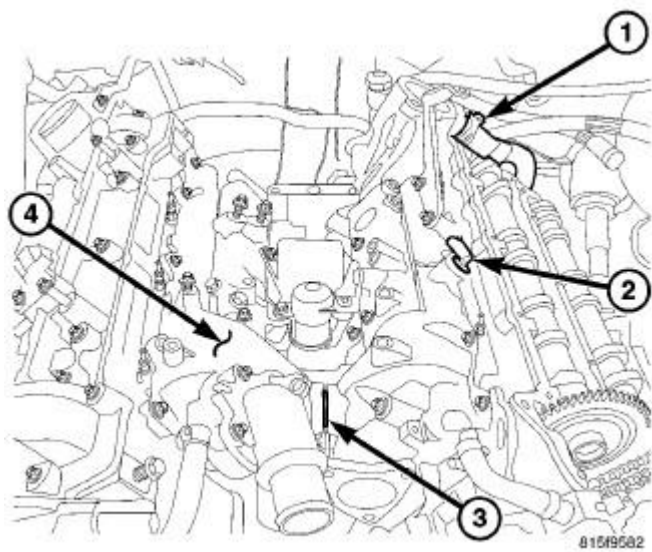
Fig. 341: INTAKE MANIFOLD Courtesy of CHRYSLER LLC
