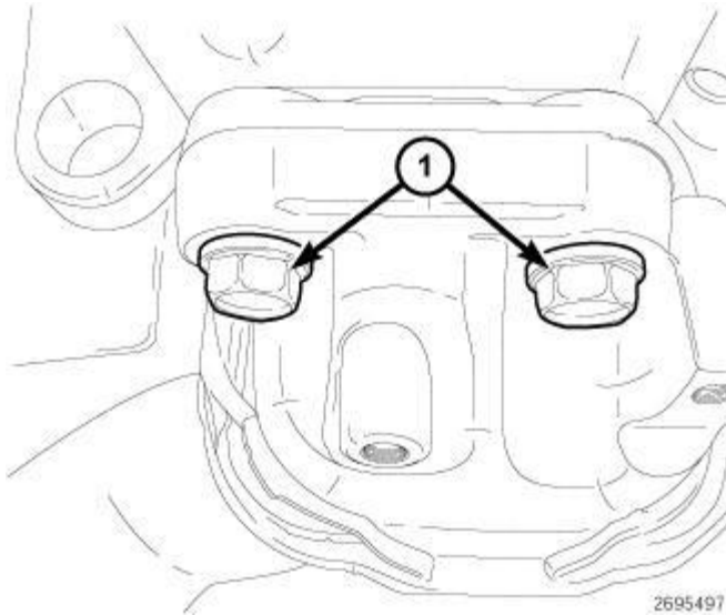
Fig. 431: Right Engine Mount Retaining Bolts Courtesy of CHRYSLER LLC
