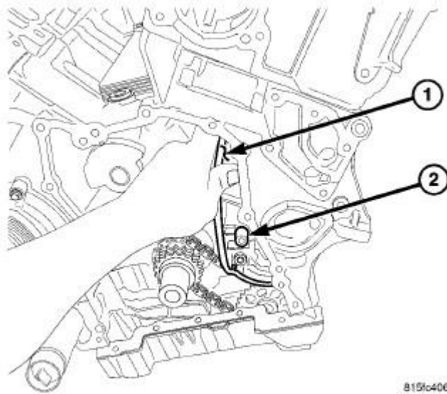
Fig. 95: LEFT LOWER TIMING CHAIN GUIDE AND FASTENER Courtesy of CHRYSLER LLC
