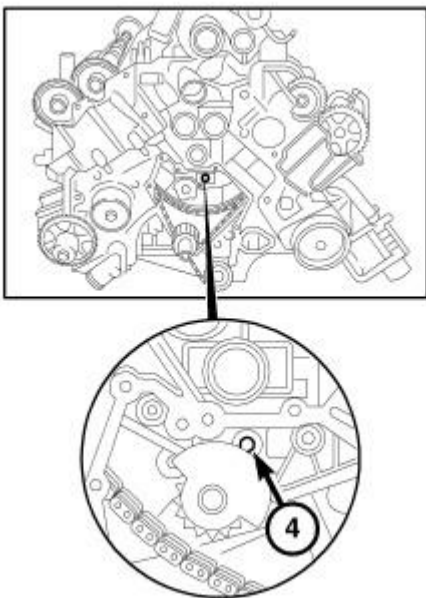
Fig. 380: BALANCE SHAFT ALIGNMENT FRONT
