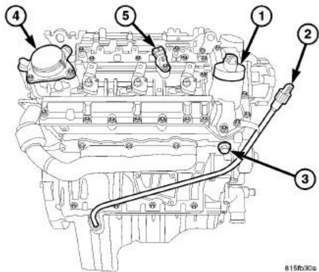
Fig. 581: Timing Chain Tensioner Courtesy of CHRYSLER LLC
