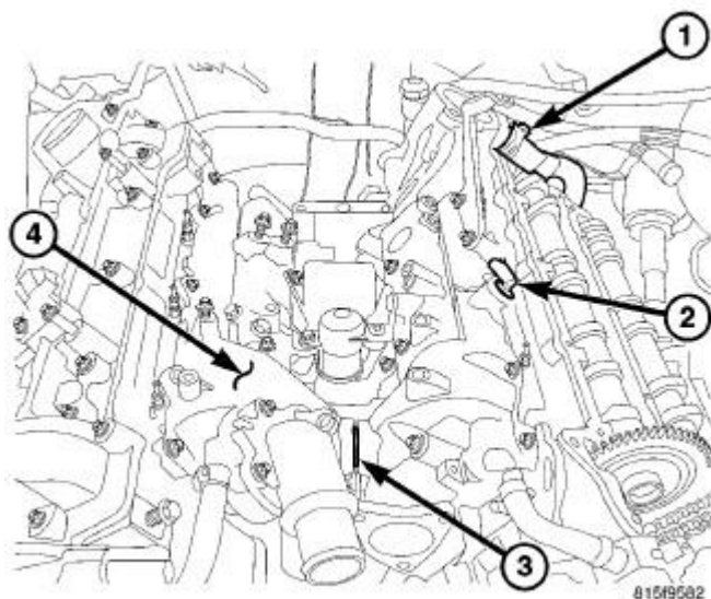
Fig. 444: Intake Manifold & Connections Courtesy of CHRYSLER LLC
