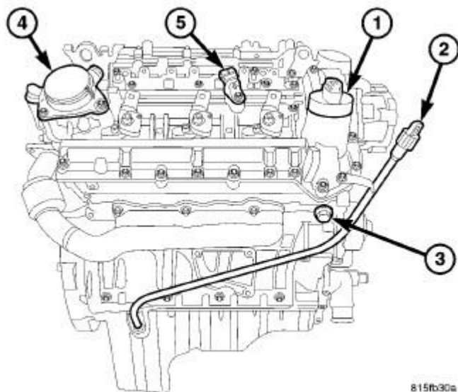
Fig. 575: Timing Chain Tensioner Courtesy of CHRYSLER LLC
