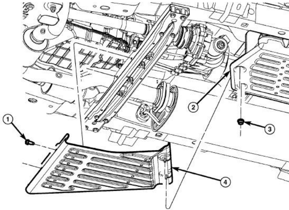
Fig. 519: TRANSFER CASE SKID PLATE
