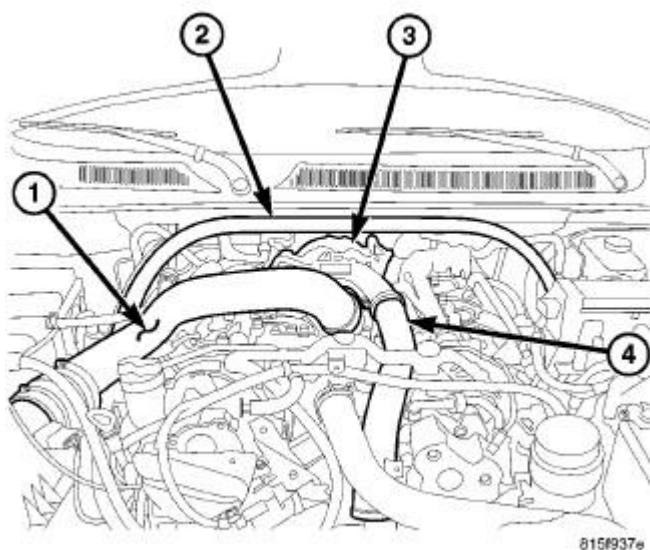
Fig. 50: Strut Tower Support Courtesy of CHRYSLER LLC
