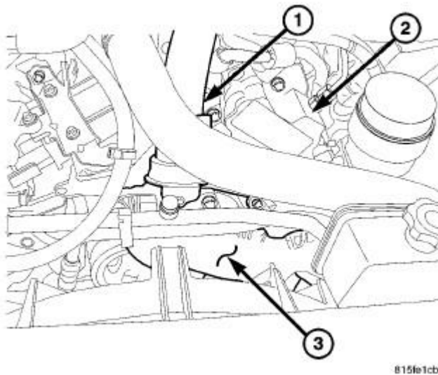
Fig. 105: CHARGE AIR COOLER INLET WITH RESONATOR
