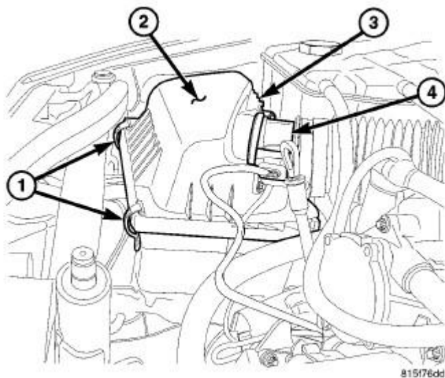
Fig. 495: AIR CLEANER COVER Courtesy of CHRYSLER LLC
