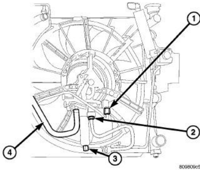
Fig. 103: HYDRAULIC LINES/HOSES AND ELECTRICAL CONNECTOR Courtesy of CHRYSLER LLC
