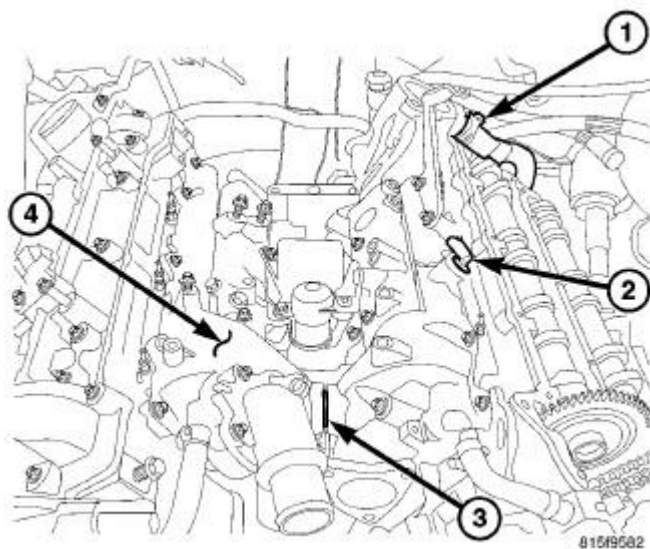
Fig. 107: INTAKE MANIFOLD
