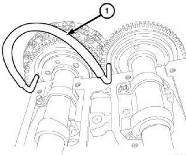
Fig. 168: Camshaft Locking Pins 8929 Courtesy of CHRYSLER LLC
