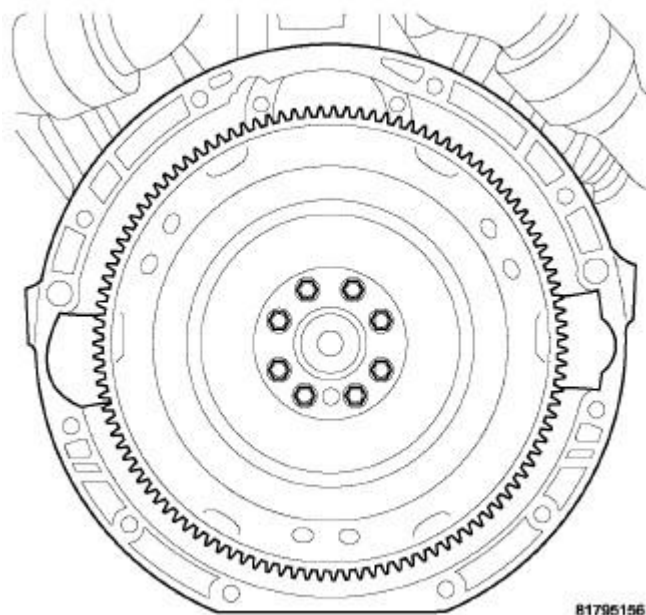
Fig. 376: Flex Plate
