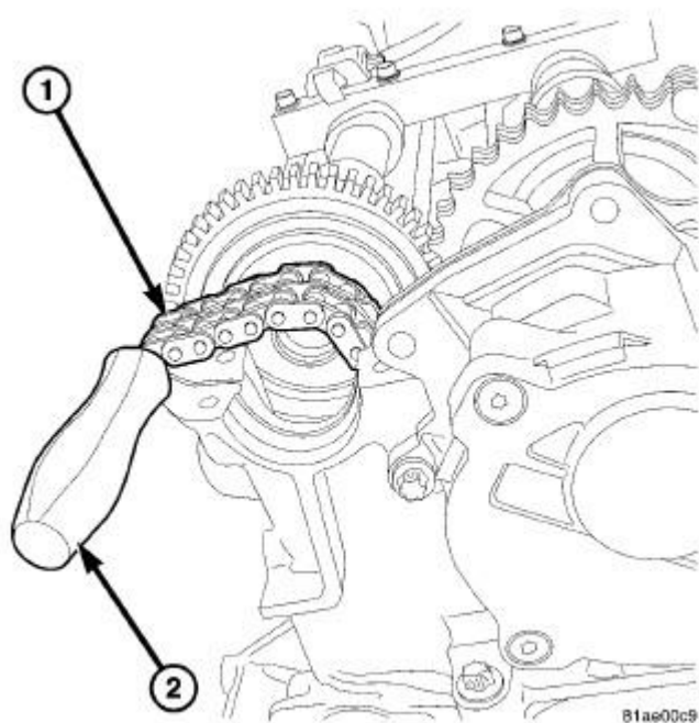
Fig. 572: PREVENT CHAIN FROM FALLING Courtesy of CHRYSLER LLC
