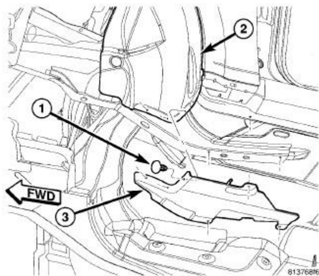
Fig. 434: Removing/Installing Shield Courtesy of CHRYSLER LLC
