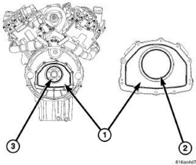
Fig. 460: REAR MAIN SEAL CARRIER
