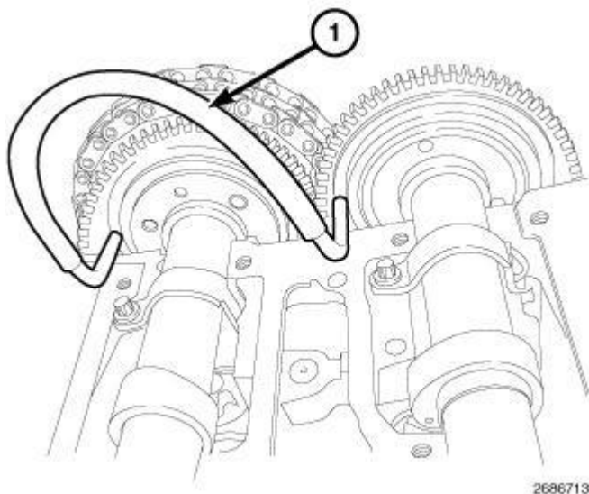
Fig. 138: Camshaft Locking Pins 8929 Courtesy of CHRYSLER LLC
