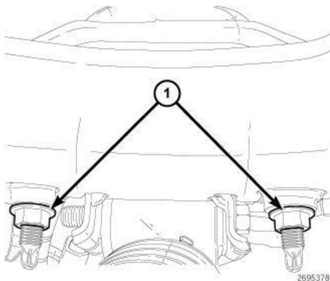
Fig. 421: Right Lower Engine Mount Retaining Nuts Courtesy of CHRYSLER LLC
