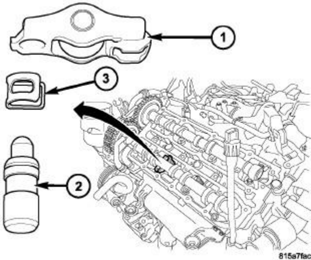
Fig. 278: ROCKER ARMS Courtesy of CHRYSLER LLC
