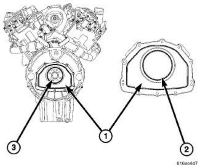
Fig. 458: REAR MAIN SEAL CARRIER Courtesy of CHRYSLER LLC
