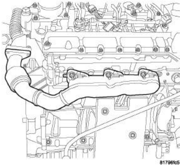
Fig. 518: RIGHT EXHAUST MANIFOLD Courtesy of CHRYSLER LLC
