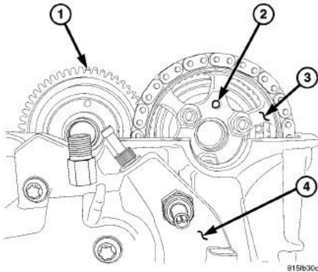
Fig. 88: LEFT EXHAUST CAMSHAFT DRIVE GEAR ALIGNMENT DOWEL Courtesy of CHRYSLER LLC
