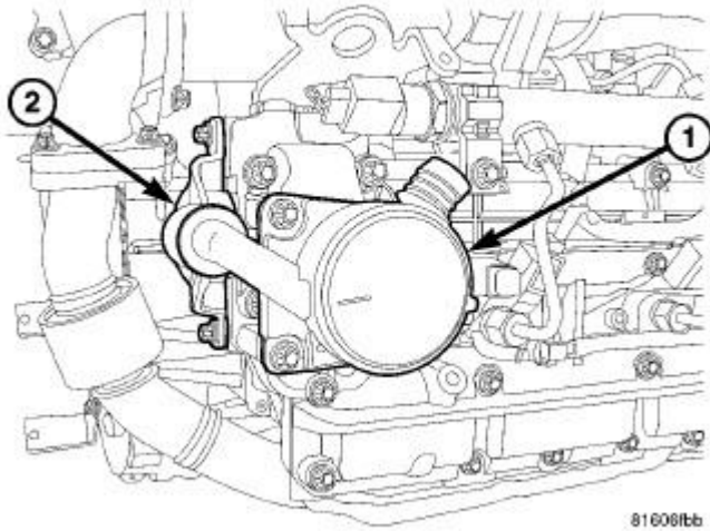
Fig. 521: OIL SEPARATOR Courtesy of CHRYSLER LLC
