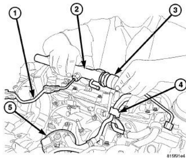
Fig. 285: LEFT FUEL RAIL Courtesy of CHRYSLER LLC
