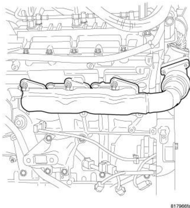
Fig. 346: EXHAUST MANIFOLD - LEFT Courtesy of CHRYSLER LLC
