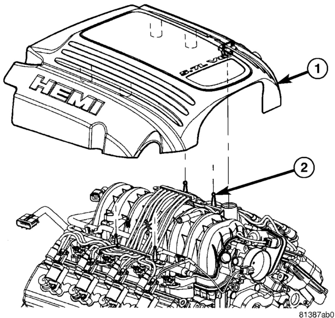
Fig. 206: Engine Cover & Attaching Studs Courtesy of CHRYSLER LLC
