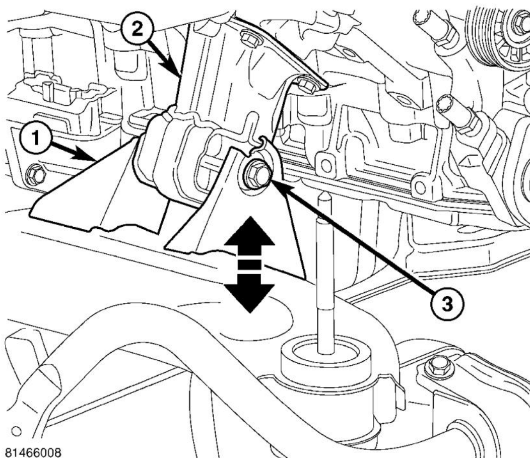
Fig. 8: Removing Engine Front Mount To Frame Bolts/Nuts Courtesy of CHRYSLER LLC
