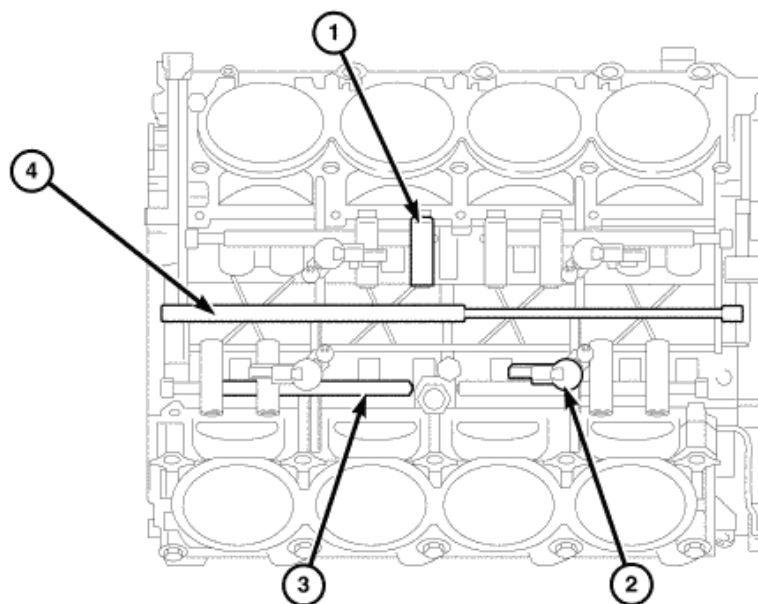
Fig. 53: MDS Cylinder View Courtesy of CHRYSLER LLC
