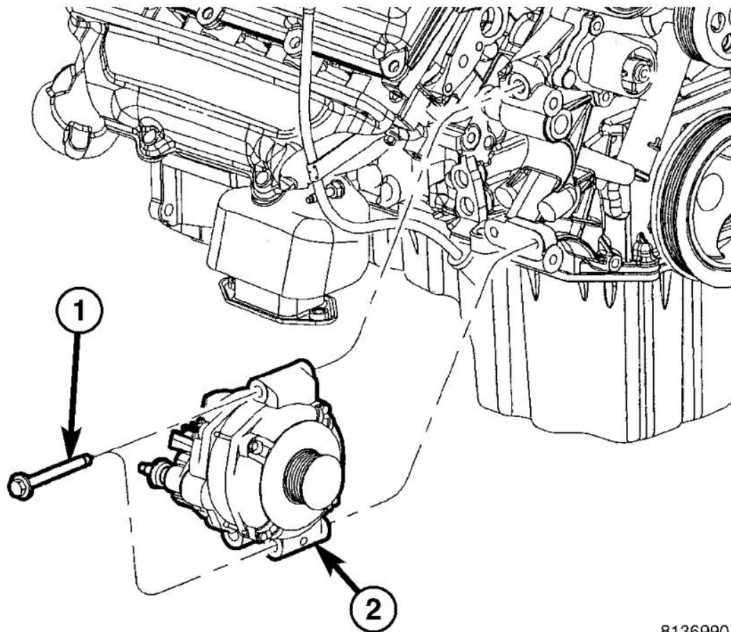
Fig. 5: Generator-5.7L Courtesy of CHRYSLER LLC
