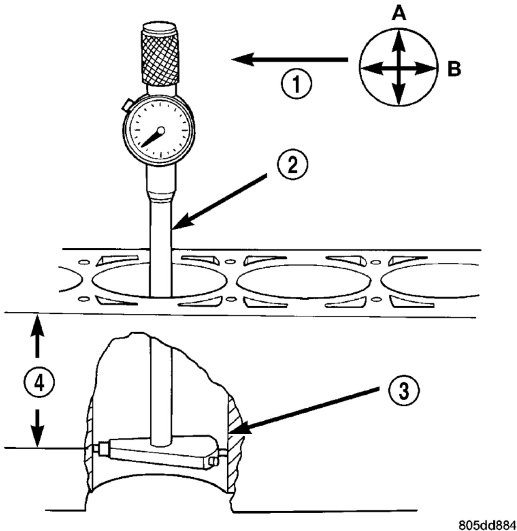
Fig. 149: Measuring Inside Diameter Of Cylinder Bore Using Bore Gauge - Typical Courtesy of CHRYSLER LLC
