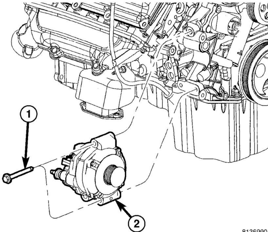
Fig. 27: Generator-5.7L Courtesy of CHRYSLER LLC
