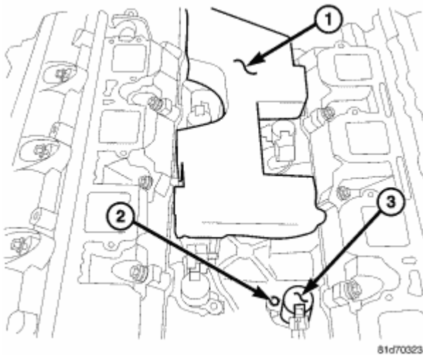
Fig. 165: Foam Insulator Pad, Hold Down Bolt & MDS Solenoid(s) Courtesy of CHRYSLER LLC
