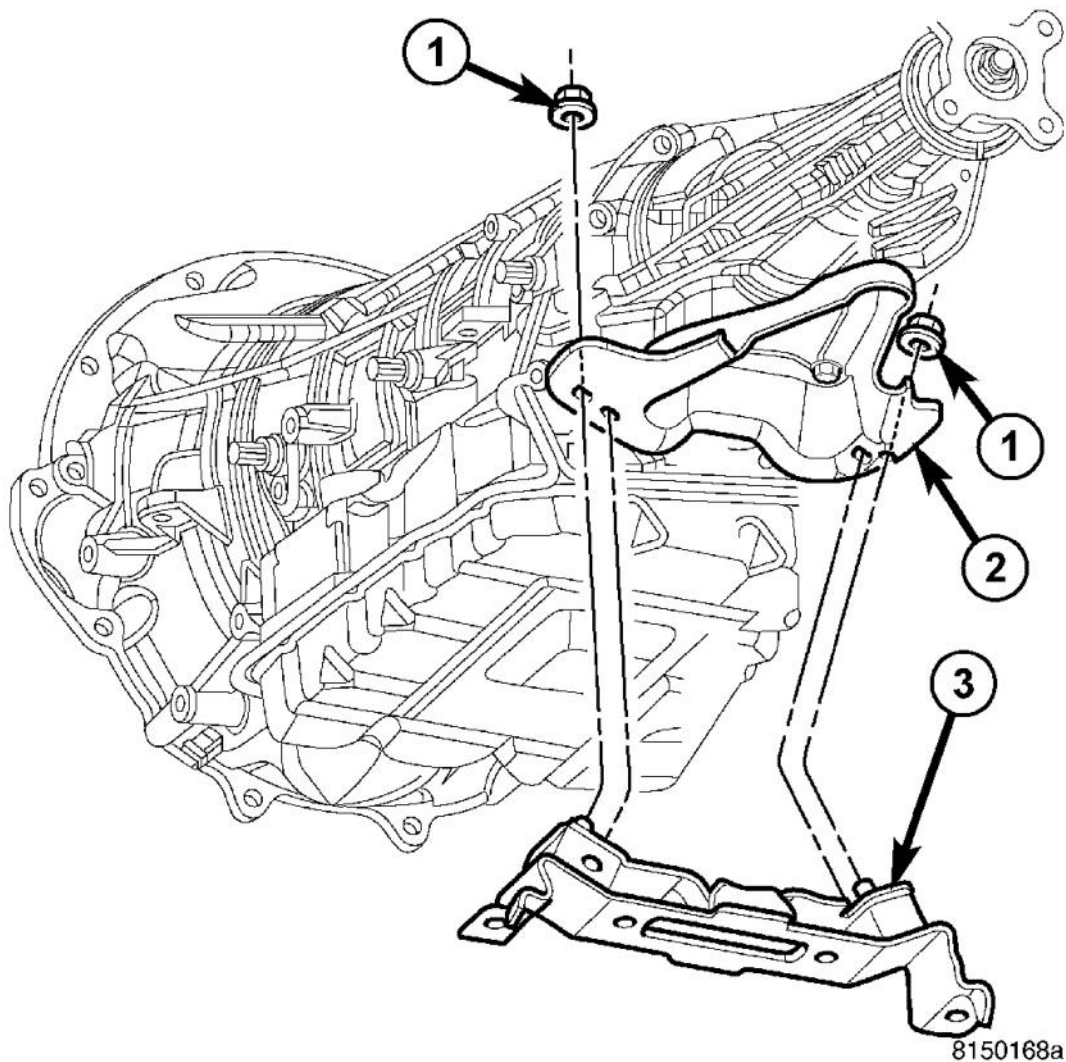
Fig. 171: Removing/Installing Engine Rear Mount (4X2) Courtesy of CHRYSLER LLC
