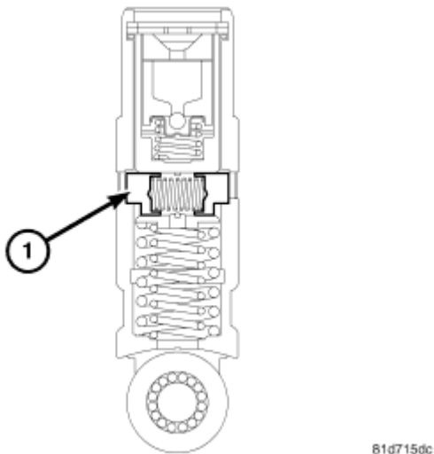
Fig. 54: MDS System Latching Pin Courtesy of CHRYSLER LLC
