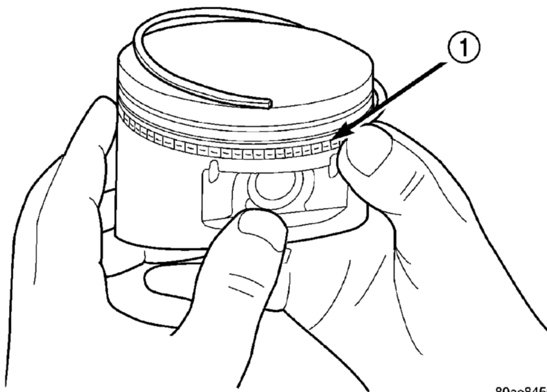
Fig. 157: Installing Upper Side Rail By Placing One End Between Piston Ring Groove And Expander Ring
