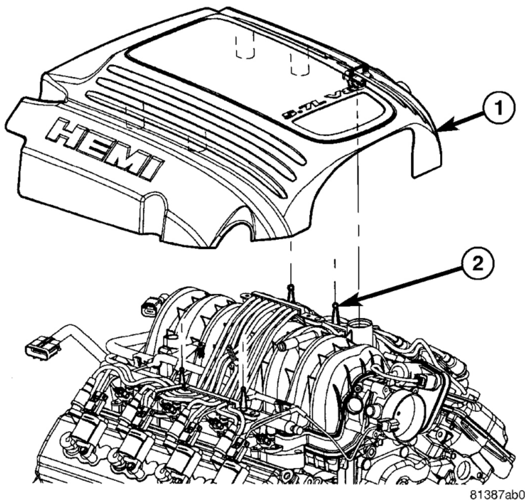
Fig. 201: Engine Cover & Attaching Studs Courtesy of CHRYSLER LLC
