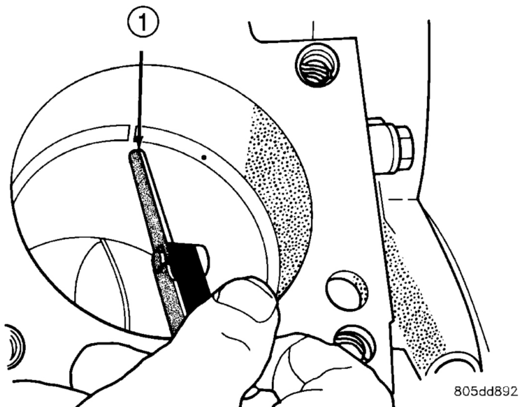
Fig. 155: Using Feeler Gauge To Check Ring End Gap Courtesy of CHRYSLER LLC
