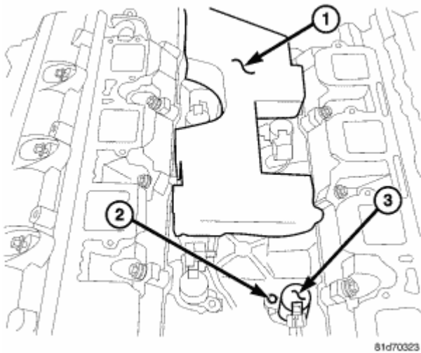
Fig. 168: Foam Insulator Pad, Hold Down Bolt & MDS Solenoid(s) Courtesy of CHRYSLER LLC
