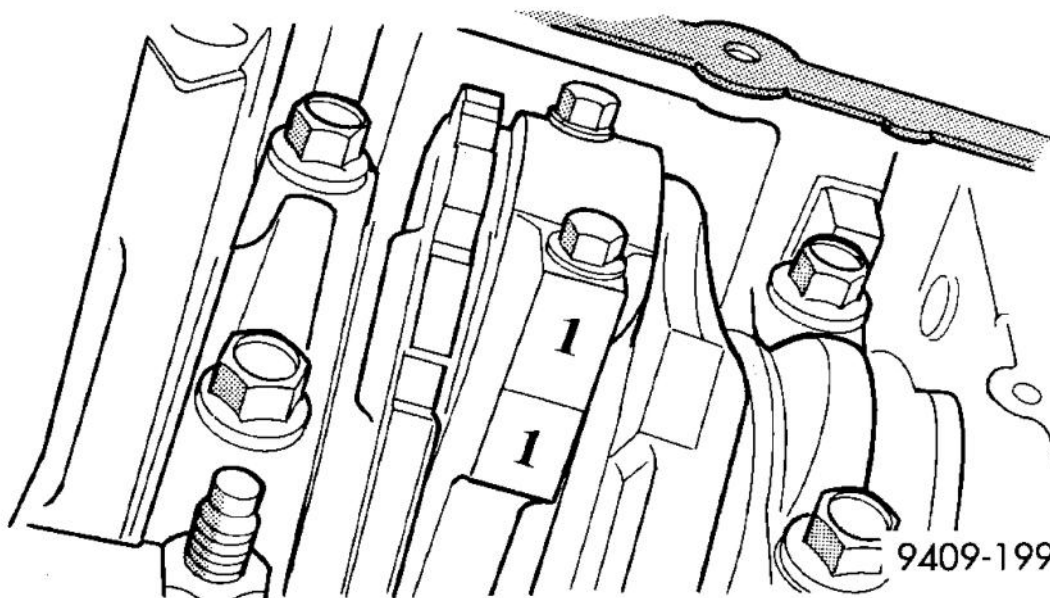
Fig. 151: Marking Connecting Rod And Bearing Cap Positions Courtesy of CHRYSLER LLC
