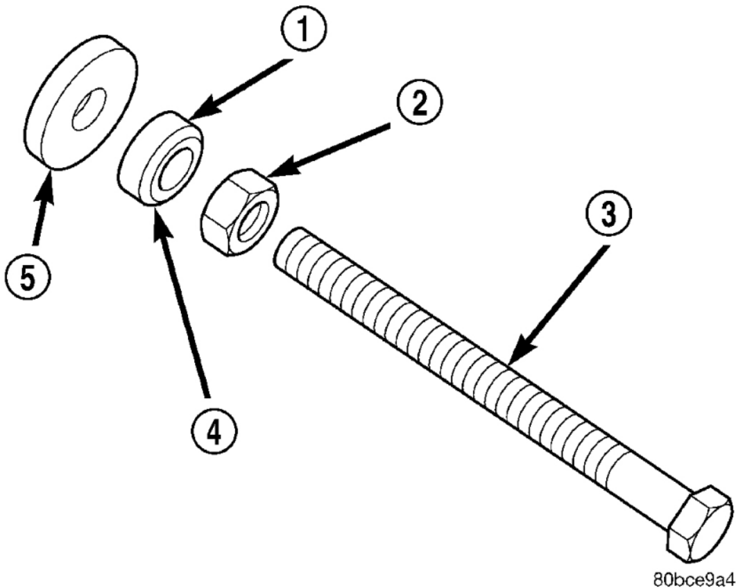
Fig. 161: Bearing, Nut, Threaded Rod, Bearing Hardened Surface & Hardened Washer Courtesy of CHRYSLER LLC
