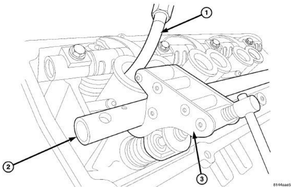
Fig. 121: SPECIAL TOOL 9065A COMPONENTS Courtesy of CHRYSLER LLC
