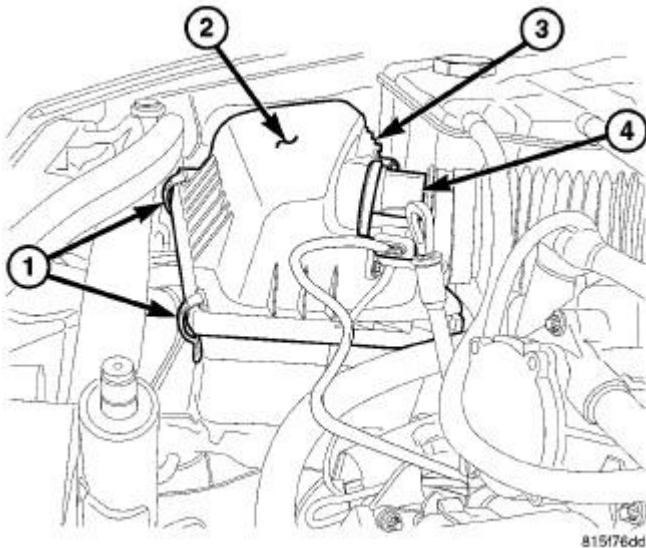
Fig. 263: AIR CLEANER COVER
