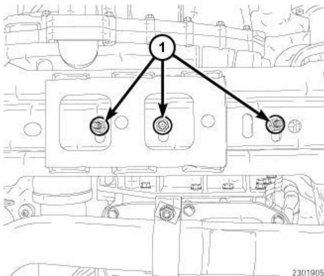
Fig. 159: Transmission Mount To Crossmember Retaining Nuts Courtesy of CHRYSLER LLC
