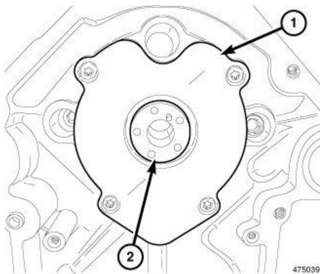
Fig. 148: Camshaft Thrust Plate Courtesy of CHRYSLER LLC
