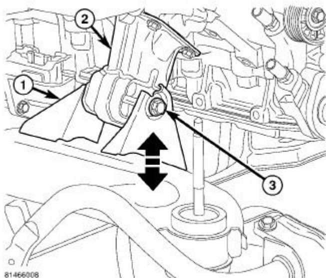
Fig. 222: ENGINE MOUNT BOLT Courtesy of CHRYSLER LLC
