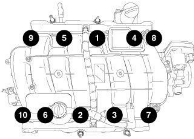
Fig. 284: Intake Manifold Removal & Tightening Sequence Courtesy of CHRYSLER LLC
