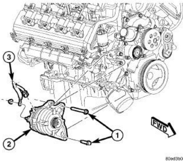
Fig. 314: REMOVE / INSTALL GENERATOR - 5.7L Courtesy of CHRYSLER LLC
