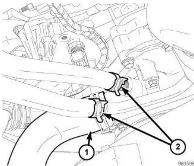
Fig. 81: Heater & Lower Radiator Hose
