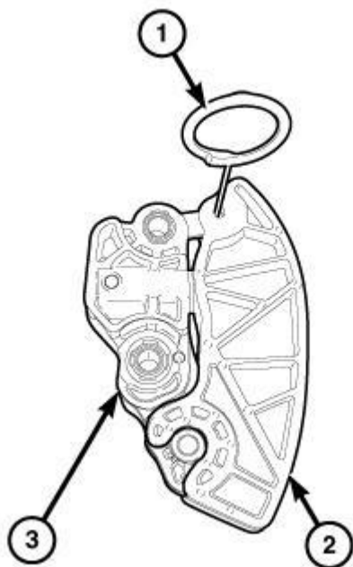
Fig. 323: Installing Tensioner Pin Courtesy of CHRYSLER LLC
