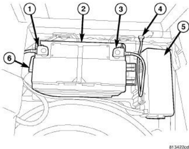
Fig. 205: Battery System Components And PDC Cover
