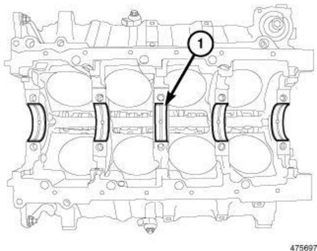
Fig. 173: Main Bearings
