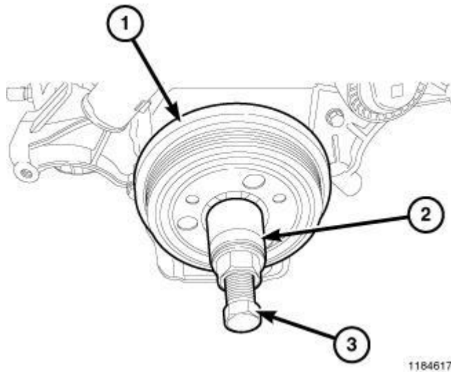
Fig. 186: Pressing Damper Onto Crankshaft Courtesy of CHRYSLER LLC
