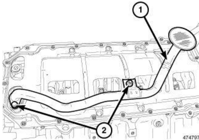
Fig. 166: Oil Pick Up Tube Courtesy of CHRYSLER LLC
