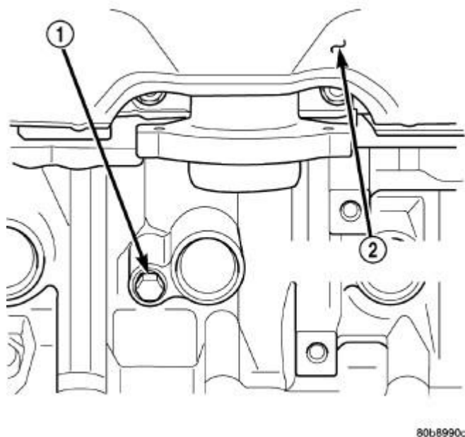
Fig. 309: Drain Plug Courtesy of CHRYSLER LLC
