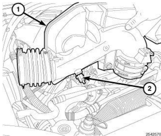
Fig. 76: Air Cleaner Resonator Courtesy of CHRYSLER LLC
