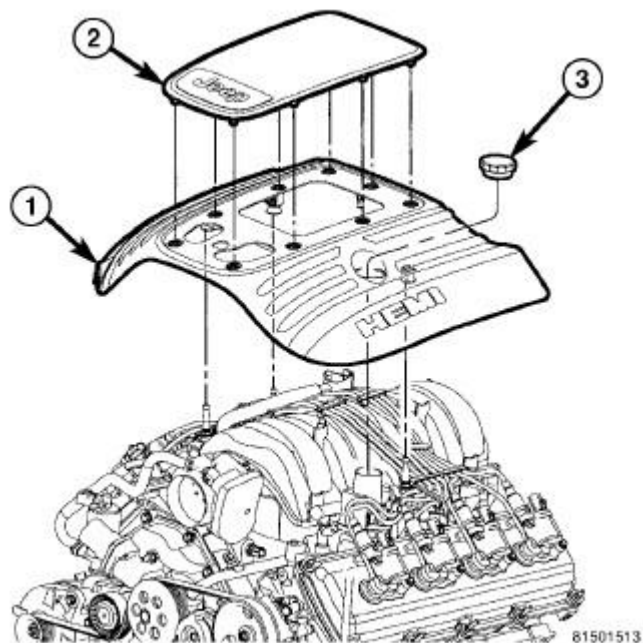
Fig. 308: Engine Cover Courtesy of CHRYSLER LLC
