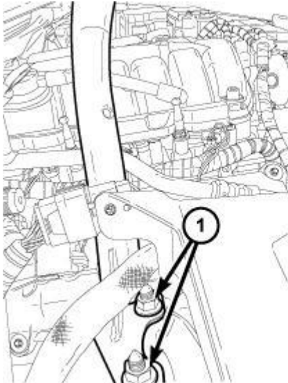
Fig. 253: Right Side Strut Tower Support Beam Retaining Nuts Courtesy of CHRYSLER LLC
