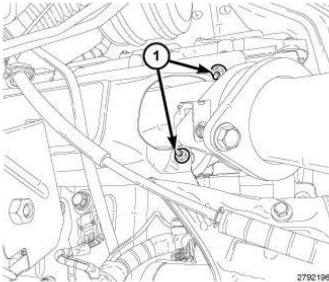
Fig. 260: Rear Exhaust Manifold Heat Shield Retaining Nuts Courtesy of CHRYSLER LLC
