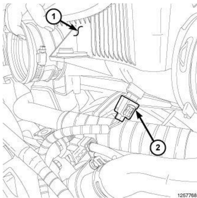
Fig. 307: IAT Sensor Electrical Connector Courtesy of CHRYSLER LLC
