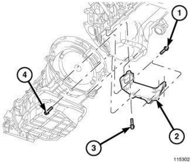
Fig. 6: Structural Cover
