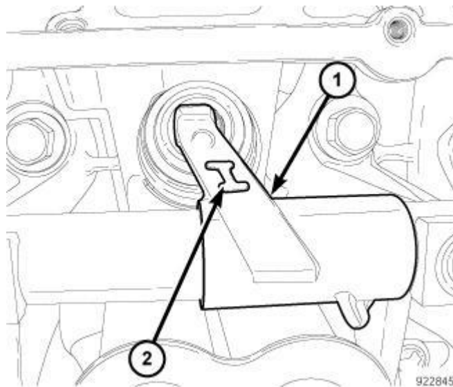
Fig. 109: Intake Rocker Arm Marking
