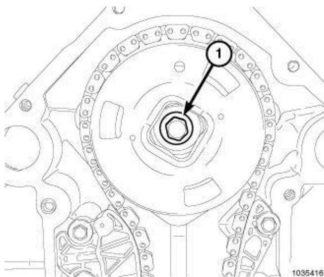
Fig. 302: Camshaft Phaser Retaining Bolt Courtesy of CHRYSLER LLC
