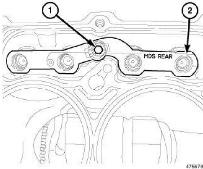
Fig. 153: Rear MDS Lifter Assembly Courtesy of CHRYSLER LLC
