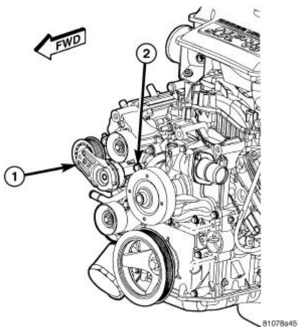
Fig. 316: Automatic Belt Tensioner Courtesy of CHRYSLER LLC
