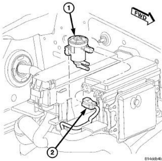
Fig. 275: EVAP SOLENOID LOCATION Courtesy of CHRYSLER LLC
