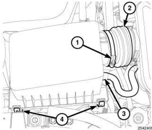
Fig. 79: Air Duct Clamp At Air Cleaner Cover Courtesy of CHRYSLER LLC
