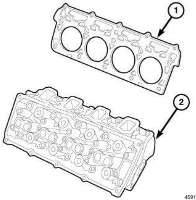
Fig. 86: Cylinder Head & Gasket Courtesy of CHRYSLER LLC
