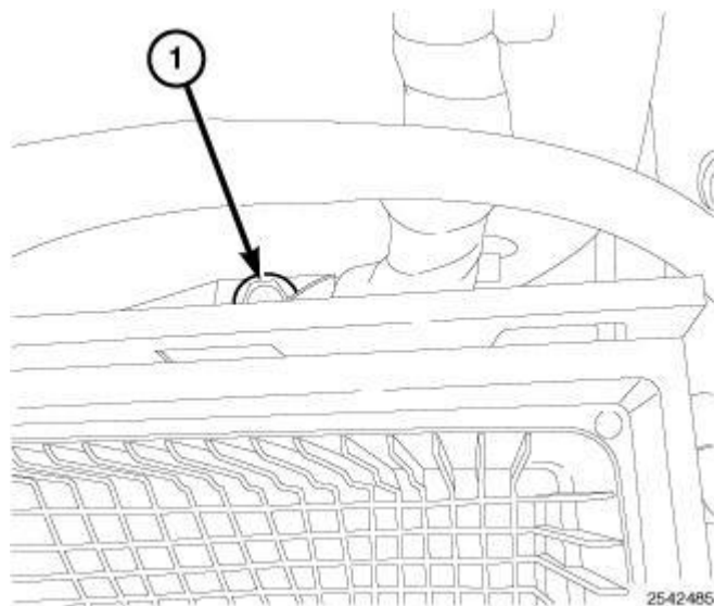
Fig. 70: Housing Assembly Retaining Bolt Courtesy of CHRYSLER LLC
