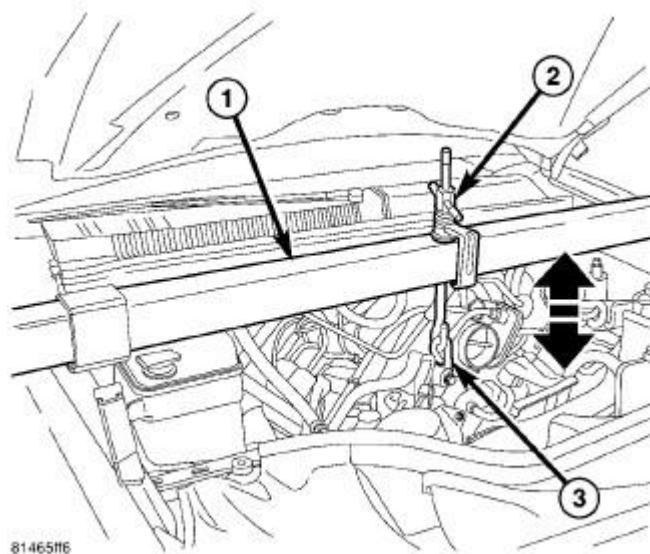
Fig. 243: ENGINE SUPPORT TOOL Courtesy of CHRYSLER LLC
