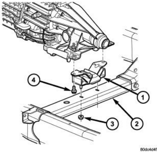
Fig. 229: TRANSMISSION MOUNT Courtesy of CHRYSLER LLC
