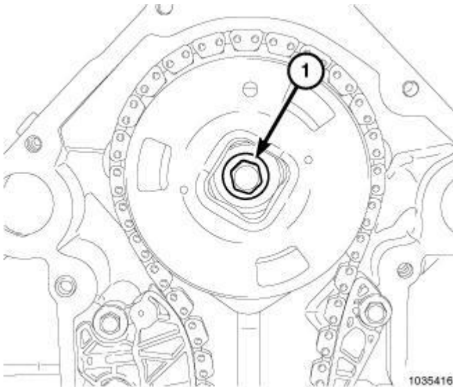
Fig. 298: Camshaft Phaser Retaining Bolt Courtesy of CHRYSLER LLC
