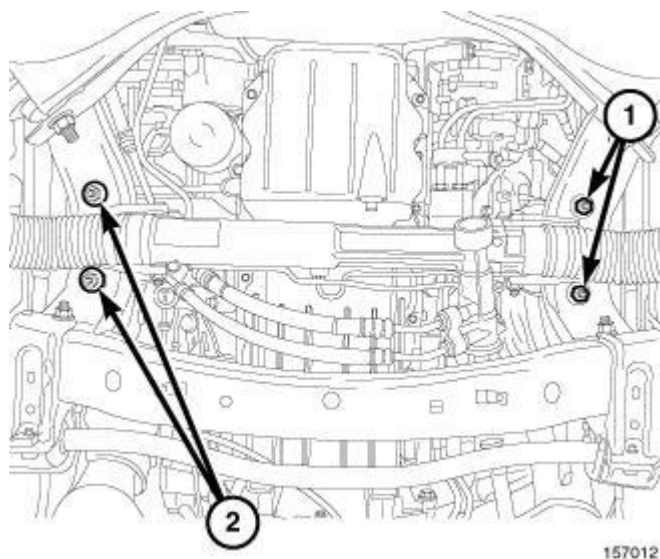
Fig. 208: Engine Mount Nuts Courtesy of CHRYSLER LLC
