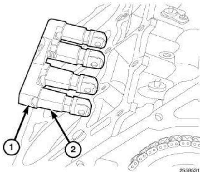
Fig. 192: Tappet Guide Holder Assembly Courtesy of CHRYSLER LLC
