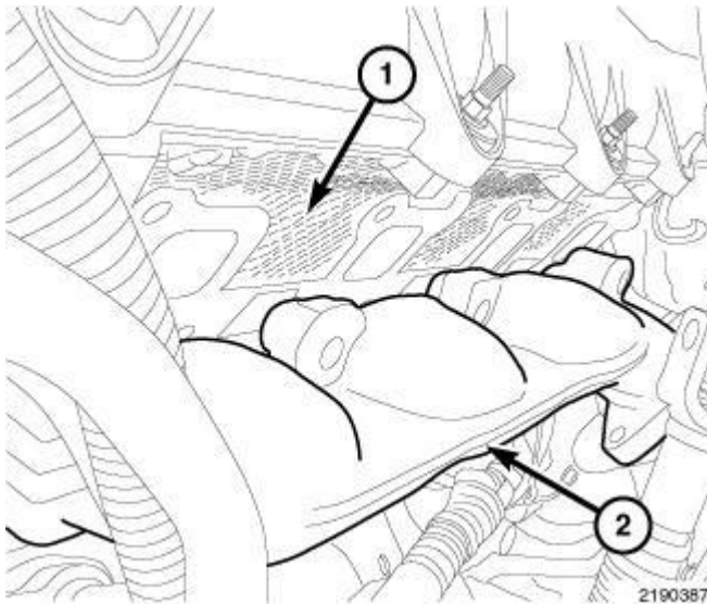
Fig. 262: Locating Exhaust Manifold & Gasket Courtesy of CHRYSLER LLC
