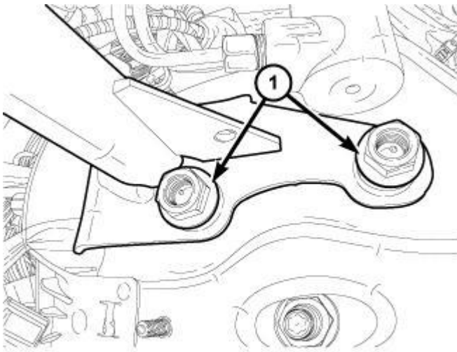
Fig. 254: Left Side Strut Tower Support Beam Retaining Nuts Courtesy of CHRYSLER LLC
