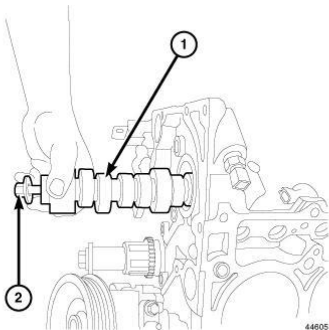
Fig. 147: Removing/Installing Camshaft Courtesy of CHRYSLER LLC
