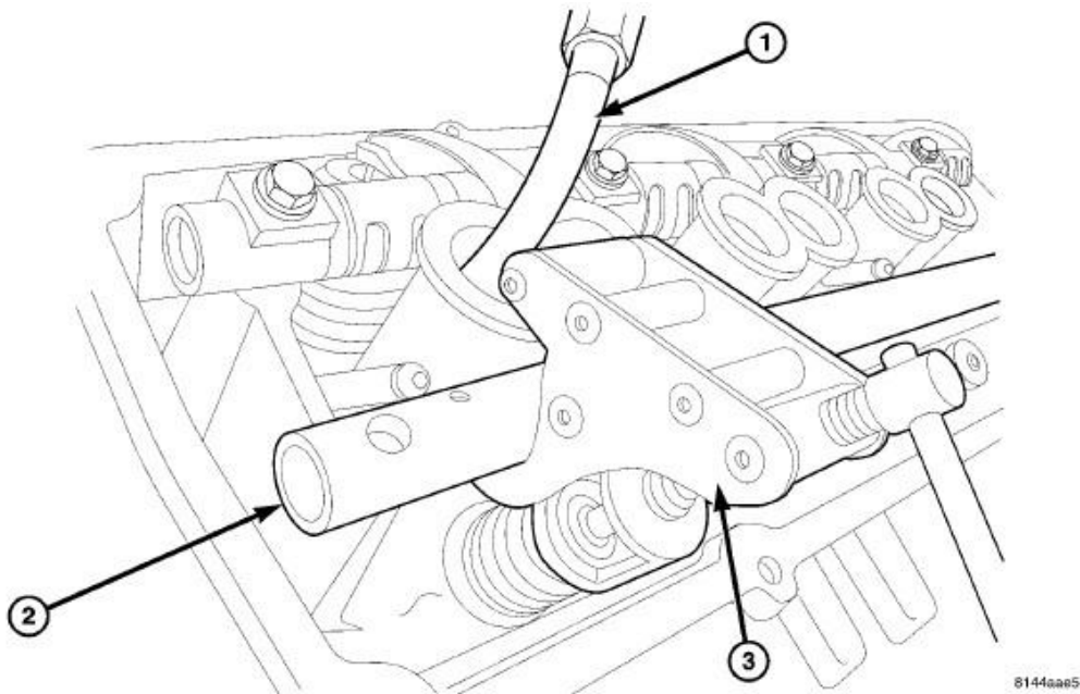
Fig. 123: SPECIAL TOOL 9065A COMPONENTS Courtesy of CHRYSLER LLC
