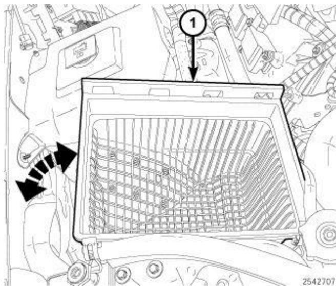
Fig. 72: Lifting Housing Assembly While Rotating Up Toward Engine Courtesy of CHRYSLER LLC
