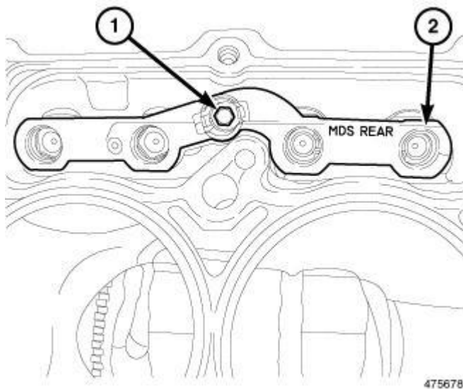
Fig. 191: Rear MDS Lifter Assembly Courtesy of CHRYSLER LLC
