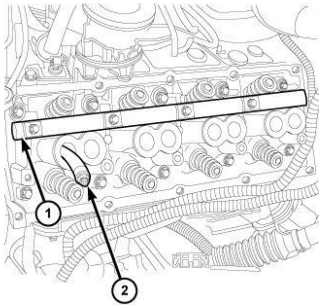
Fig. 119: ROCKER SHAFT Courtesy of CHRYSLER LLC
