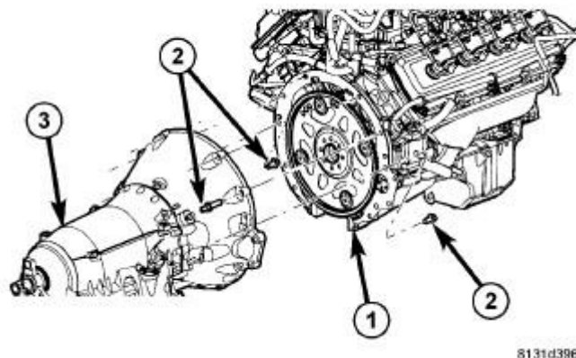
Fig. 20: Removing/Installing Transmission to Engine Bolts
