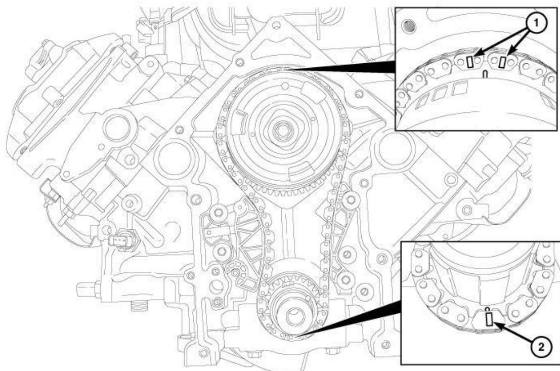
Fig. 301: Aligning Timing Marks With Timing Chain Sprockets Courtesy of CHRYSLER LLC
