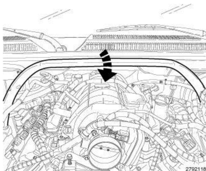
Fig. 276: Rotating Strut Tower Support Beam Forward/Rearward To Remove/Install Beam Courtesy of CHRYSLER LLC
