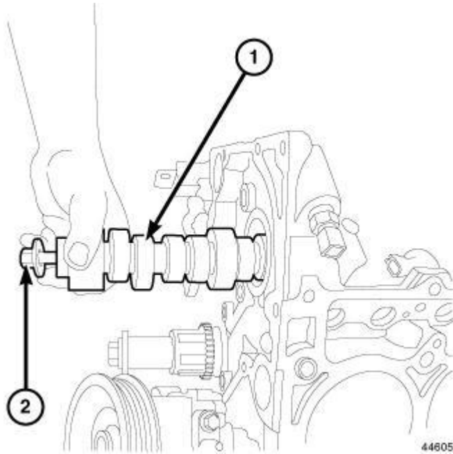
Fig. 145: Removing/Installing Camshaft Courtesy of CHRYSLER LLC
