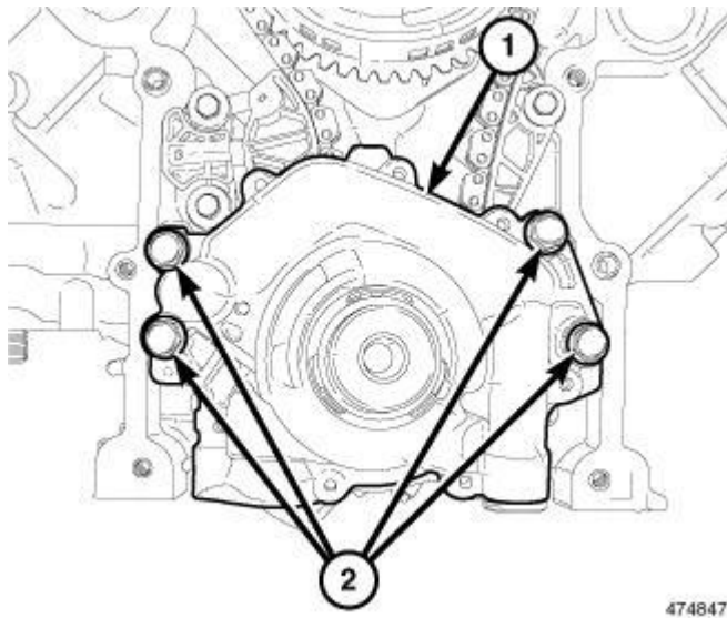
Fig. 167: Oil Pump Retaining Bolts Courtesy of CHRYSLER LLC
