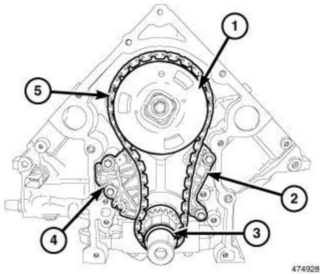
Fig. 168: Timing Chain Courtesy of CHRYSLER LLC
