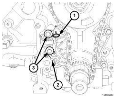
Fig. 300: Timing Chain Tensioner Pin Courtesy of CHRYSLER LLC
