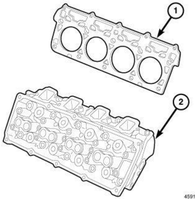
Fig. 96: Cylinder Head & Gasket Courtesy of CHRYSLER LLC
