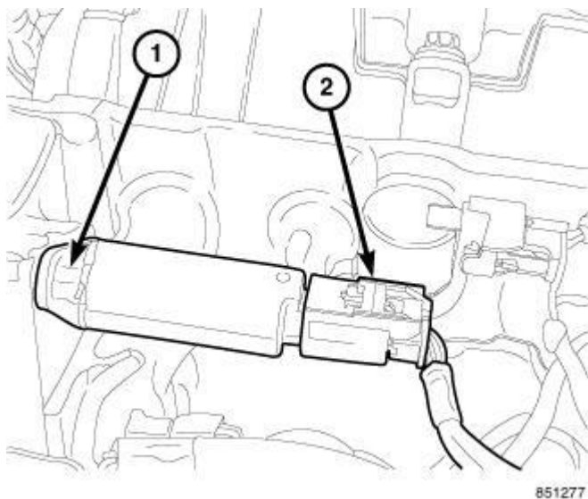
Fig. 231: Oil Control Valve Courtesy of CHRYSLER LLC
