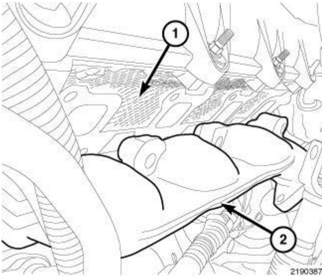
Fig. 267: Locating Exhaust Manifold & Gasket Courtesy of CHRYSLER LLC
