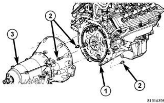
Fig. 7: Remove/Install Transmission To Engine Bolts
