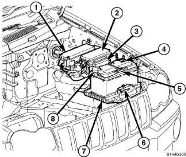
Fig. 274: Identifying Battery System Components, Power Distribution Center & Integrated Power Module Courtesy of CHRYSLER LLC
