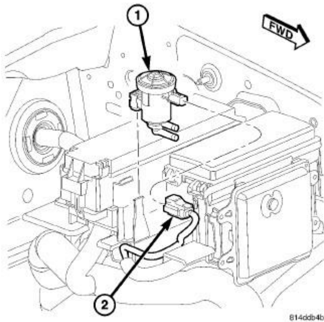
Fig. 251: EVAP SOLENOID LOCATION
