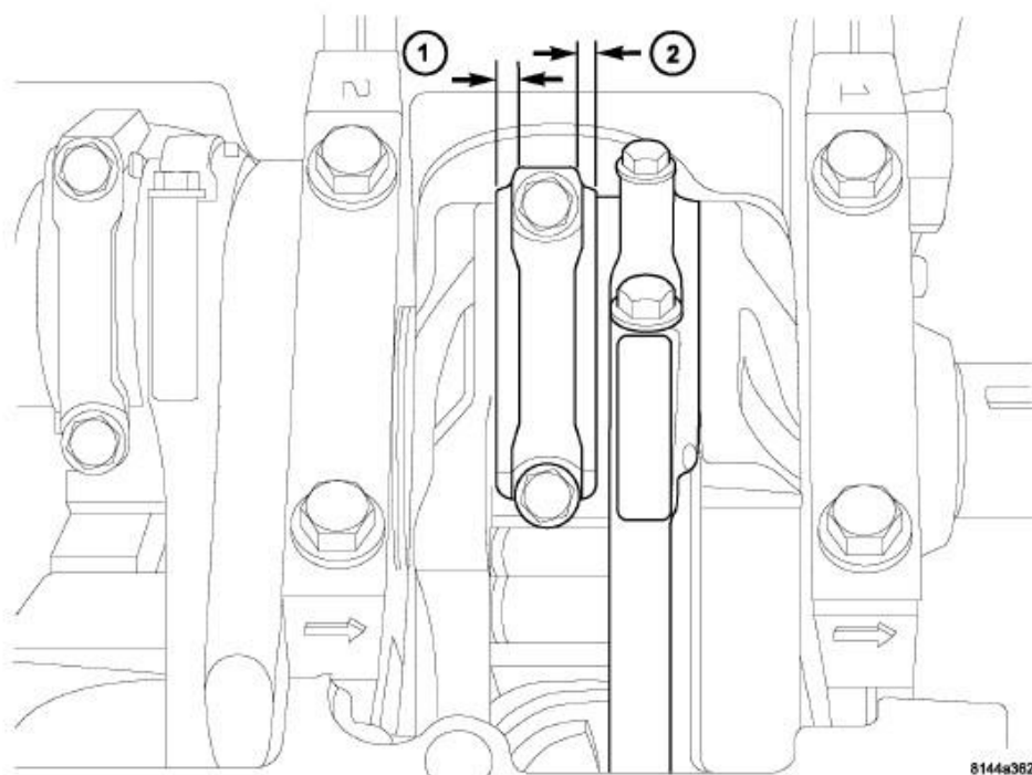
Fig. 214: CONNECTING ROD REMOVAL/INSTALLATION
