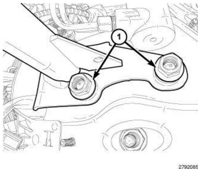
Fig. 277: Left Side Strut Tower Support Beam Retaining Nuts Courtesy of CHRYSLER LLC
