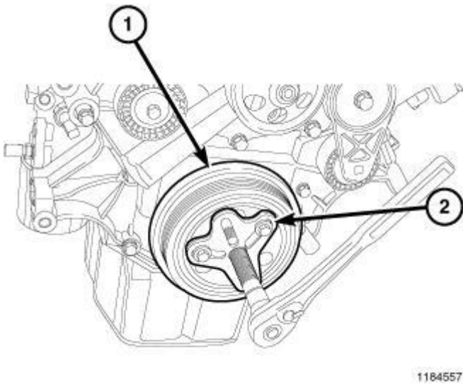
Fig. 215: Vibration Damper & Bolt Grip Puller Courtesy of CHRYSLER LLC
