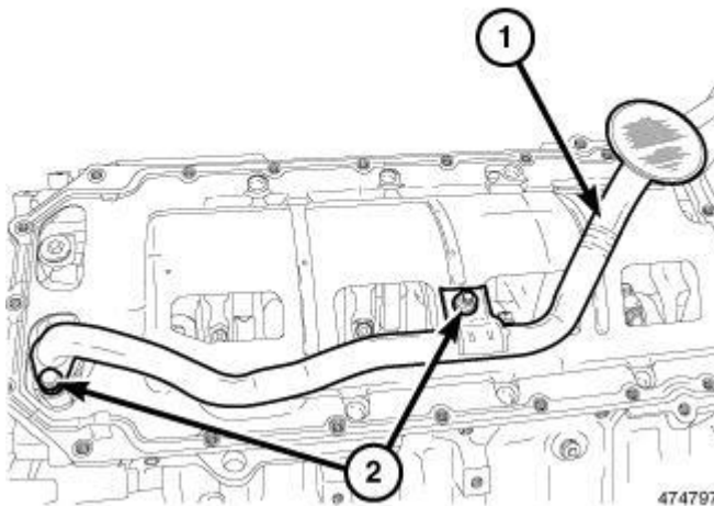
Fig. 152: Oil Pick Up Tube Courtesy of CHRYSLER LLC
