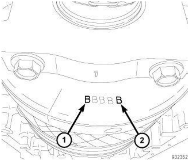
Fig. 136: Crankshaft Counterweight Stamped Grade Identification Marks Courtesy of CHRYSLER LLC
