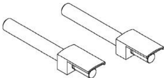
Fig. 52: Guides, Connecting Rod 8507 Courtesy of CHRYSLER LLC
