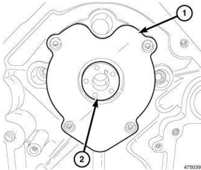
Fig. 144: Camshaft Thrust Plate Courtesy of CHRYSLER LLC
