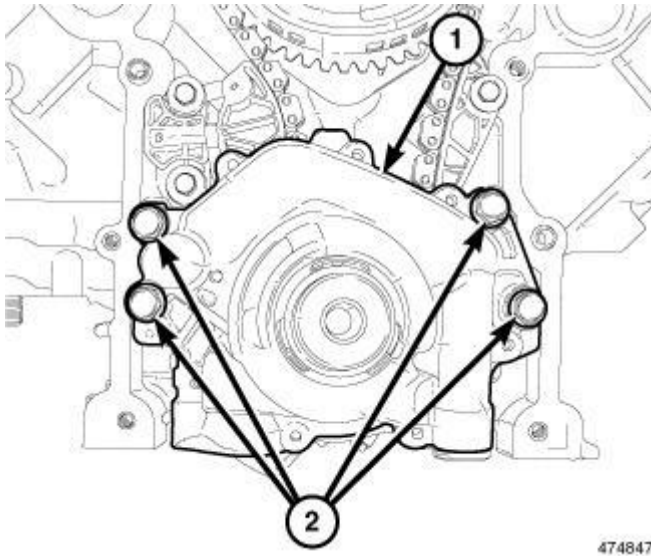
Fig. 151: Oil Pump Retaining Bolts Courtesy of CHRYSLER LLC
