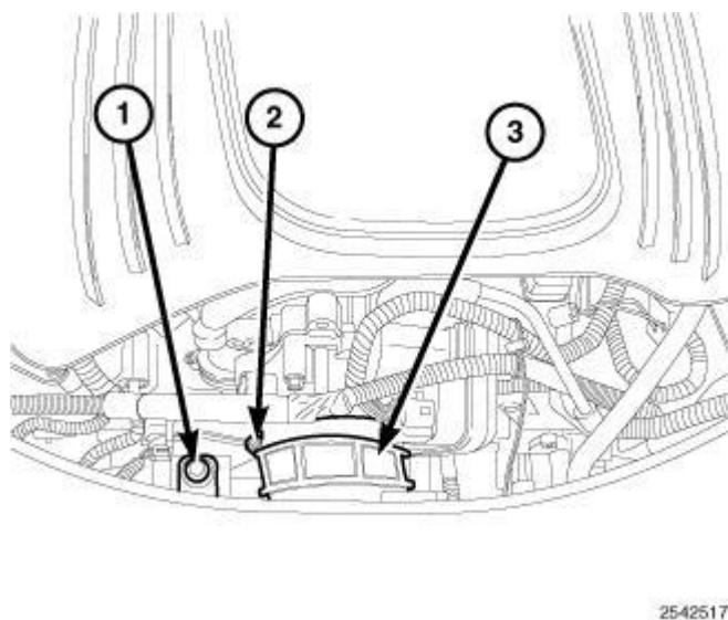
Fig. 66: Air Cleaner Resonator Air Duct Clamp Courtesy of CHRYSLER LLC
