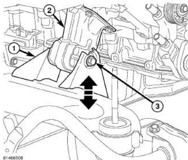
Fig. 226: ENGINE MOUNT BOLT Courtesy of CHRYSLER LLC
