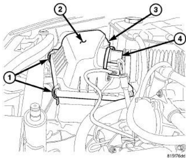
Fig. 282: AIR CLEANER COVER
