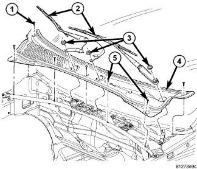
Fig. 80: Removing/Installing Cowl Grille Courtesy of CHRYSLER LLC
