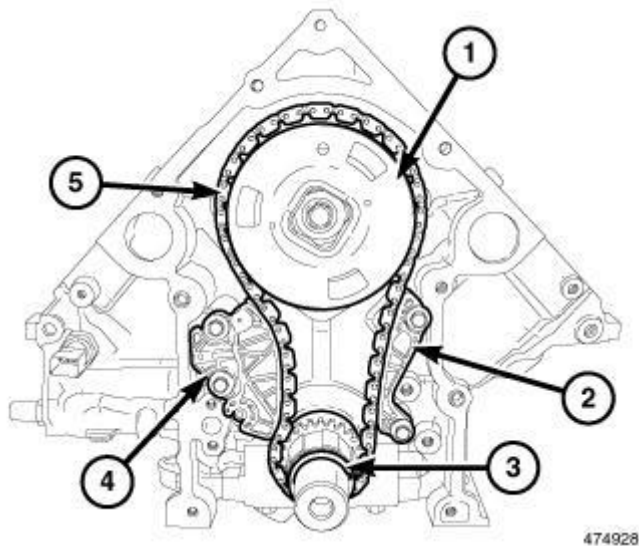
Fig. 180: Timing Chain
