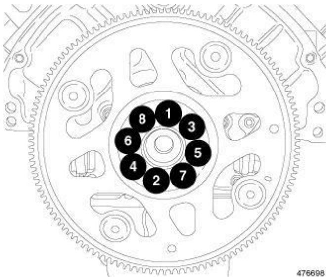
Fig. 187: Flexplate Retaining Bolt Removal & Tightening Sequence Courtesy of CHRYSLER LLC
