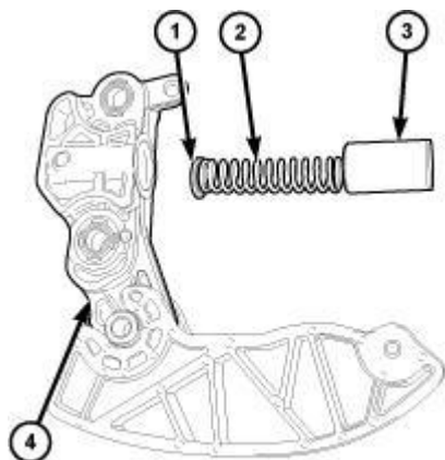
Fig. 322: Tensioner Body, Washer, Spring & Plunger Courtesy of CHRYSLER LLC
