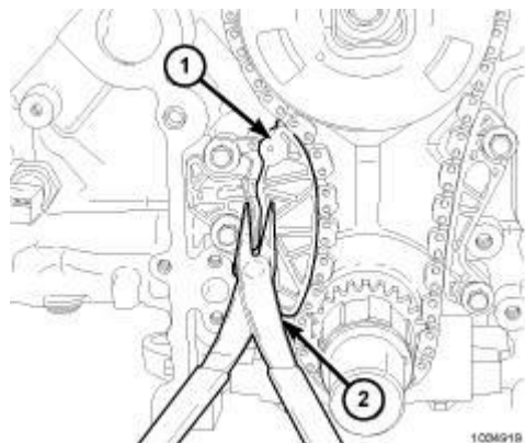
Fig. 290: Chain Tensioner Arm Courtesy of CHRYSLER LLC
