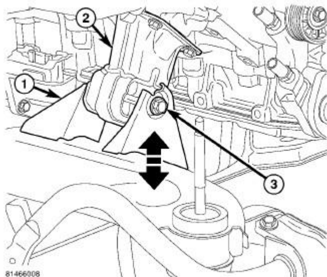
Fig. 224: ENGINE MOUNT BOLT Courtesy of CHRYSLER LLC
