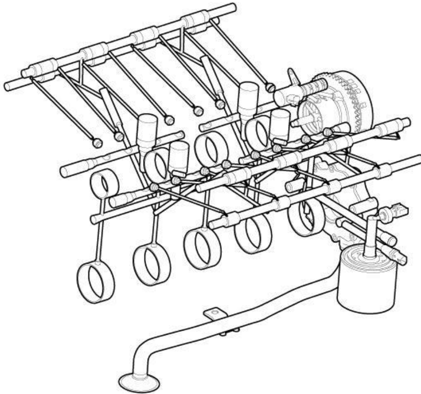
Fig. 230: 5.7L MDS Lubrication System Courtesy of CHRYSLER LLC
