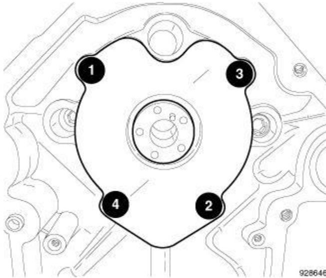
Fig. 149: Camshaft Thrust Plate Bolt Tightening Sequence Courtesy of CHRYSLER LLC
