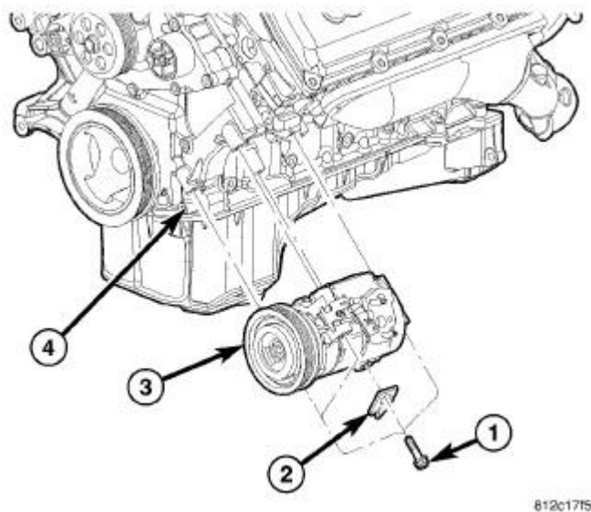
Fig. 33: COMPRESSOR-A/C 5.7L REMOVAL/INSTALLATION Courtesy of CHRYSLER LLC
