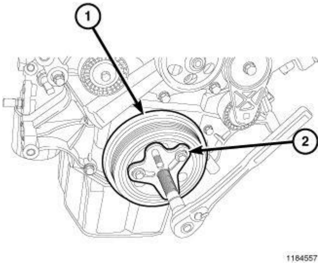
Fig. 184: Vibration Damper & Bolt Grip Puller Courtesy of CHRYSLER LLC
