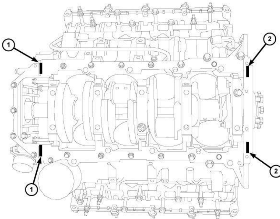
Fig. 240: T-JOINT RTV APPLICATION
