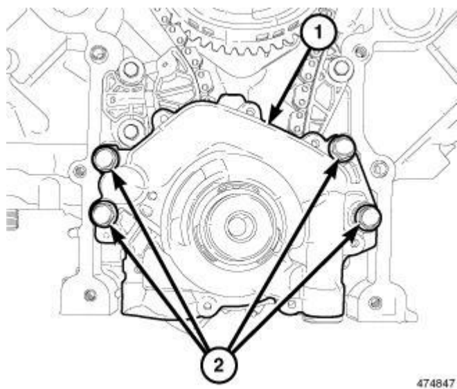
Fig. 142: Oil Pump Retaining Bolts Courtesy of CHRYSLER LLC
