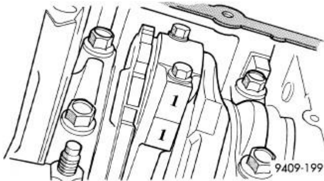
Fig. 169: Identifying Mark On Connecting Rod And Bearing Cap Courtesy of CHRYSLER LLC
