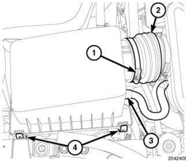
Fig. 64: Air Duct Clamp At Air Cleaner Cover
