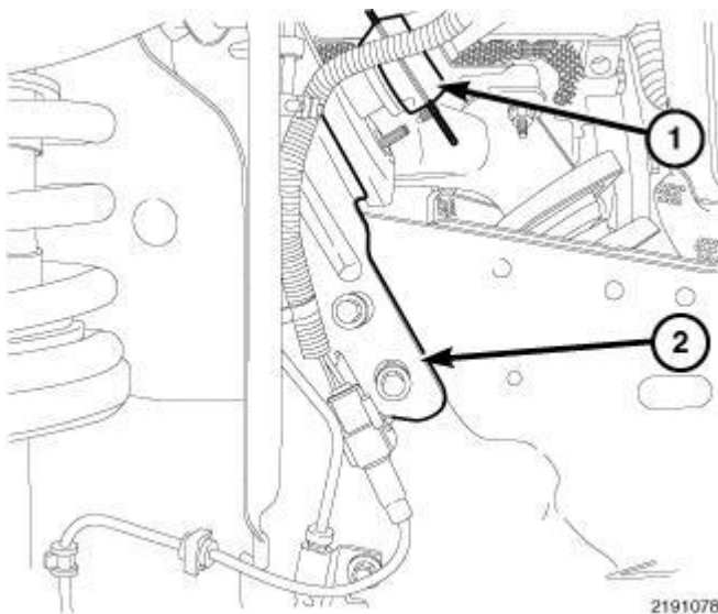
Fig. 258: Intermediate Steering Shaft Support Bracket Courtesy of CHRYSLER LLC
