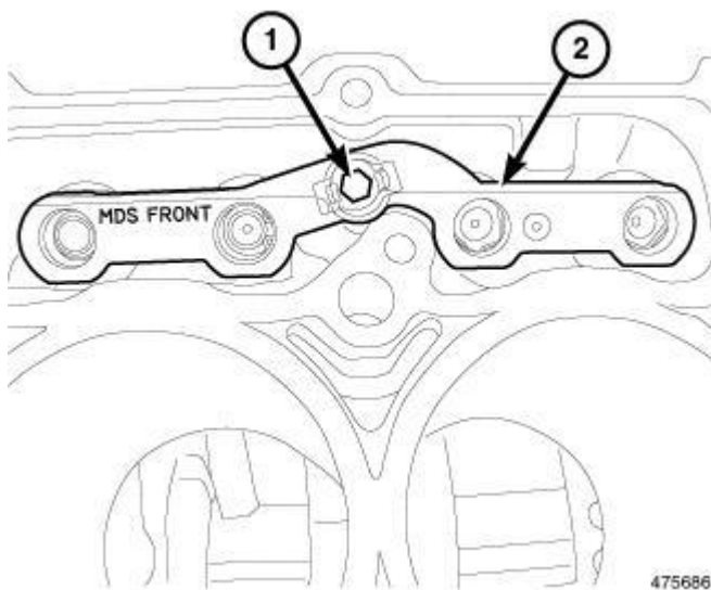
Fig. 154: Front MDS Lifter Assembly Courtesy of CHRYSLER LLC
