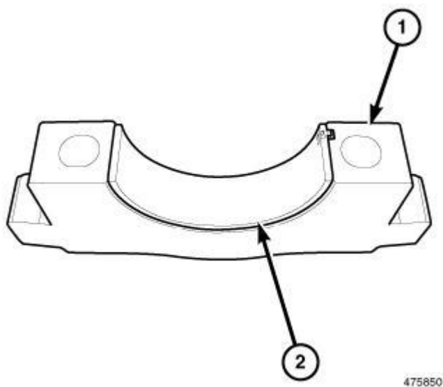
Fig. 174: Main Bearing Shells In The Bearing Caps
