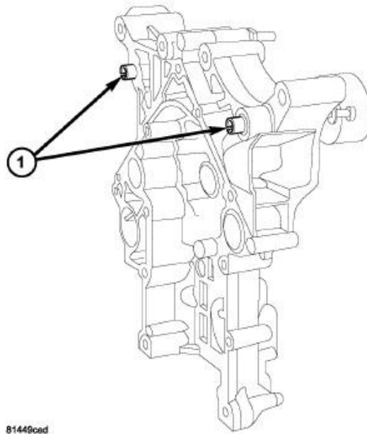
Fig. 287: FRONT COVER SLIDE BUSHINGS
