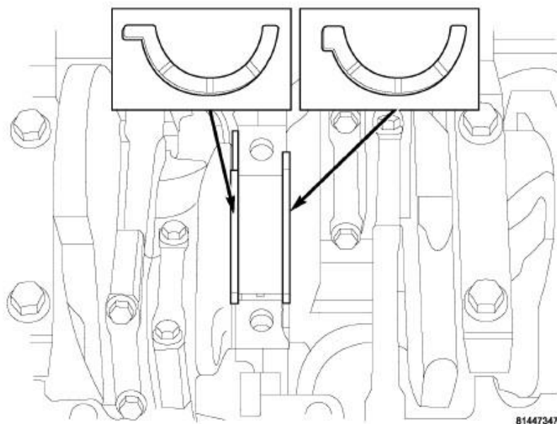
Fig. 172: THRUST WASHER LOCATION Courtesy of CHRYSLER LLC
