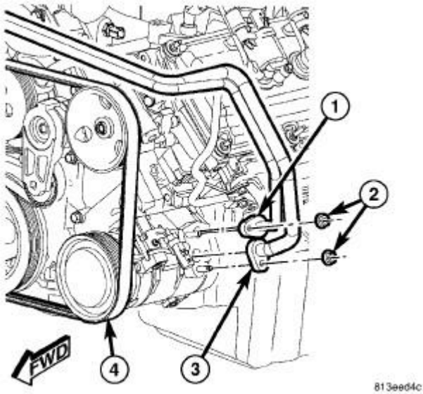
Fig. 34: Compressor Refrigerant Lines Removal/Installation Courtesy of CHRYSLER LLC
