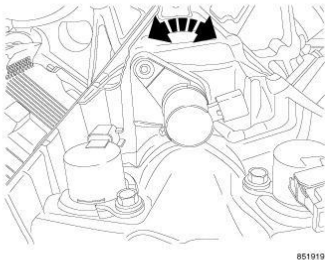
Fig. 233: Removing OCV By Rotating OCV To Break Seal
