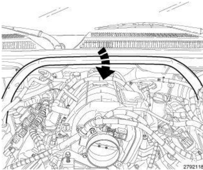
Fig. 255: Rotating Strut Tower Support Beam Forward/Rearward To Remove/Install Beam Courtesy of CHRYSLER LLC
