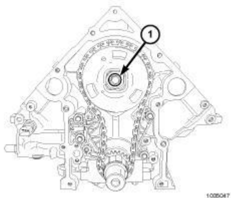
Fig. 292: Camshaft Phaser Retaining Bolt Courtesy of CHRYSLER LLC
