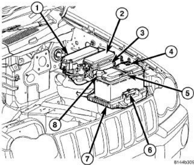
Fig. 250: Identifying Battery System Components, Power Distribution Center & Integrated Power Module
