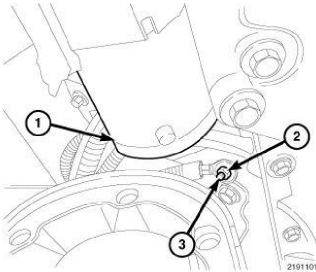
Fig. 259: Starter, Harness Retaining Nut & Lower Stud/Bolt Courtesy of CHRYSLER LLC
