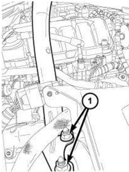
Fig. 278: Right Side Strut Tower Support Beam Retaining Nuts Courtesy of CHRYSLER LLC
