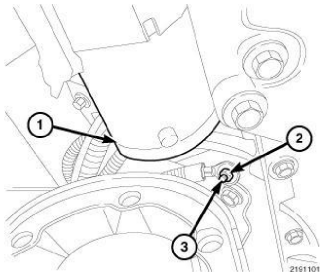
Fig. 270: Starter, Harness Retaining Nut & Lower Stud/Bolt Courtesy of CHRYSLER LLC
