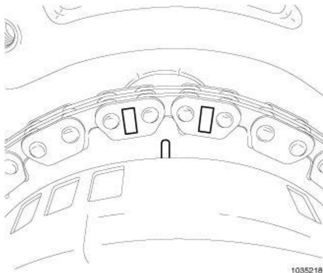
Fig. 296: Aligning Timing Chain & Camshaft Phaser Marks Courtesy of CHRYSLER LLC
