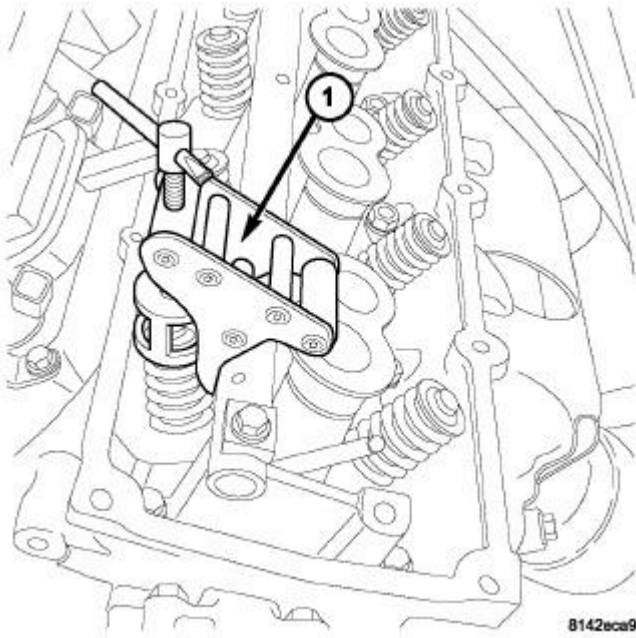
Fig. 122: Remove/Install Valve Spring Intake Courtesy of CHRYSLER LLC
