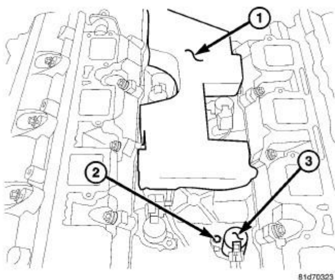
Fig. 218: MDS SOLENOIDS Courtesy of CHRYSLER LLC
