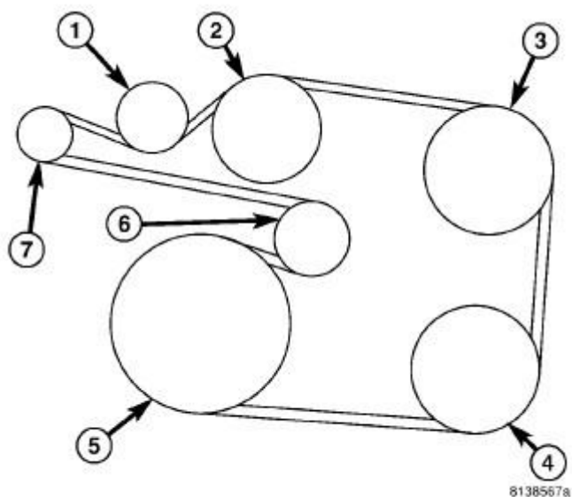
Fig. 310: 5.7L/6.1L ENGINE ACCESSORY DRIVE BELT ROUTING Courtesy of CHRYSLER LLC
