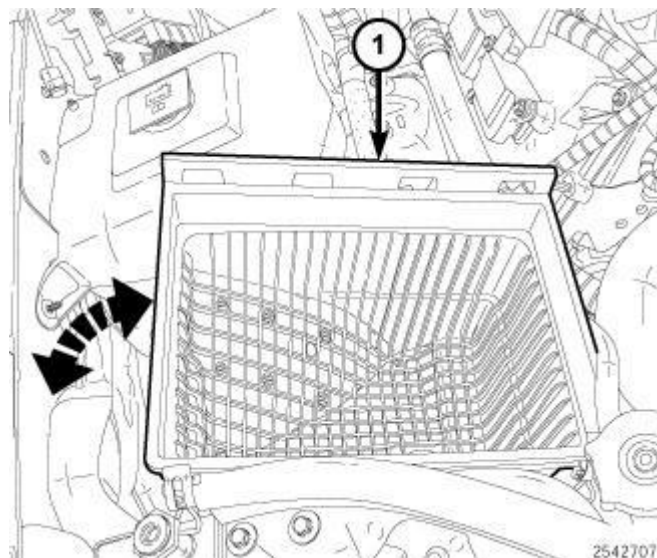
Fig. 71: Lifting Housing Assembly While Rotating Up Toward Engine Courtesy of CHRYSLER LLC
