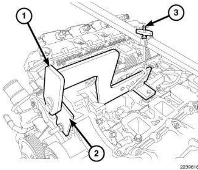
Fig. 210: Engine Lift Fixture & Adapter Courtesy of CHRYSLER LLC
