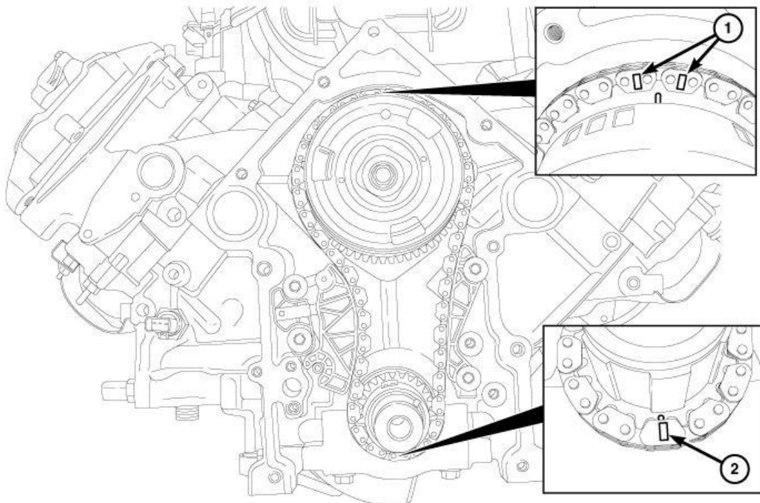
Fig. 289: Aligning Timing Marks With Timing Chain Sprockets Courtesy of CHRYSLER LLC
