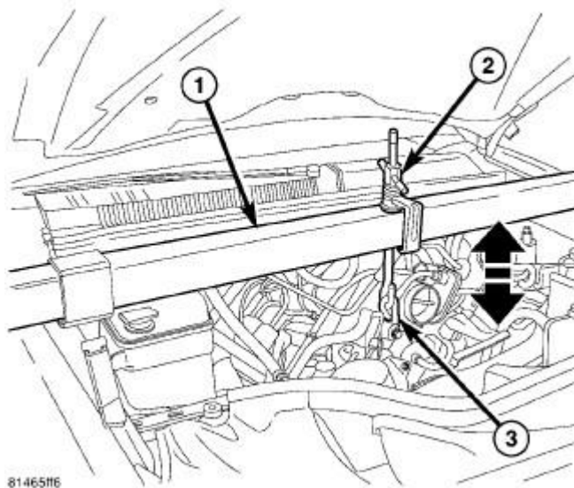
Fig. 244: ENGINE SUPPORT TOOL Courtesy of CHRYSLER LLC
