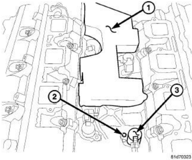
Fig. 221: MDS SOLENOIDS
