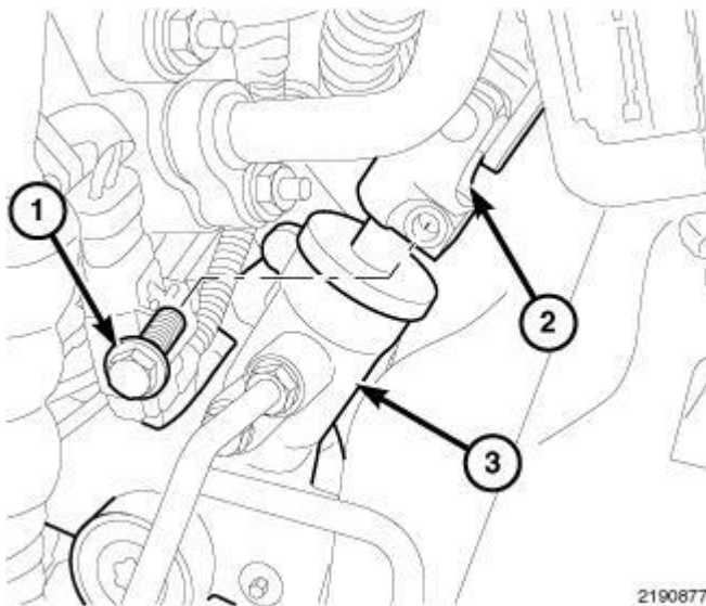
Fig. 256: Intermediate Steering Shaft Courtesy of CHRYSLER LLC
