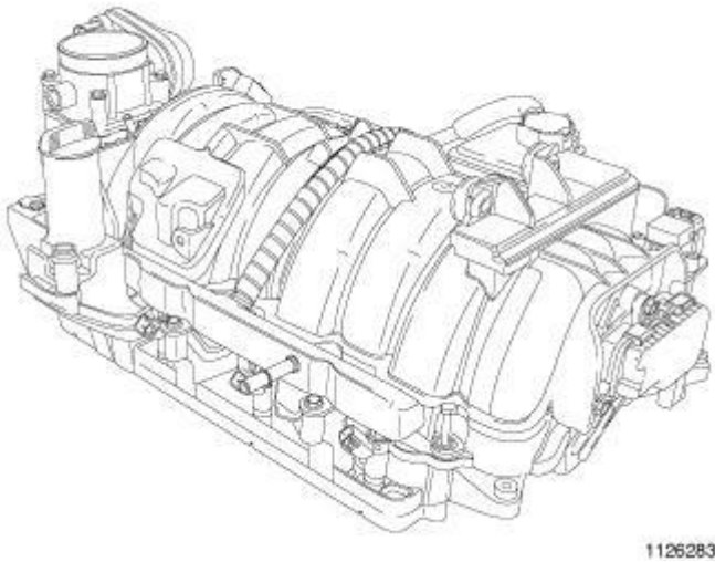
Fig. 283: Intake Manifold Courtesy of CHRYSLER LLC
