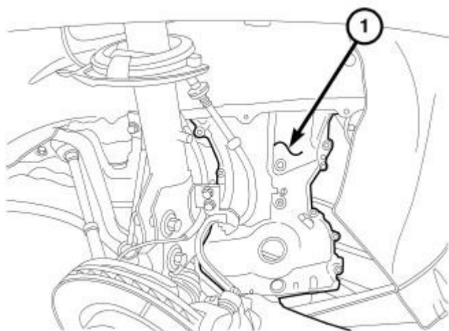
Fig. 73: Timing Chain Cover Removal/Installation Courtesy of CHRYSLER GROUP, LLC
