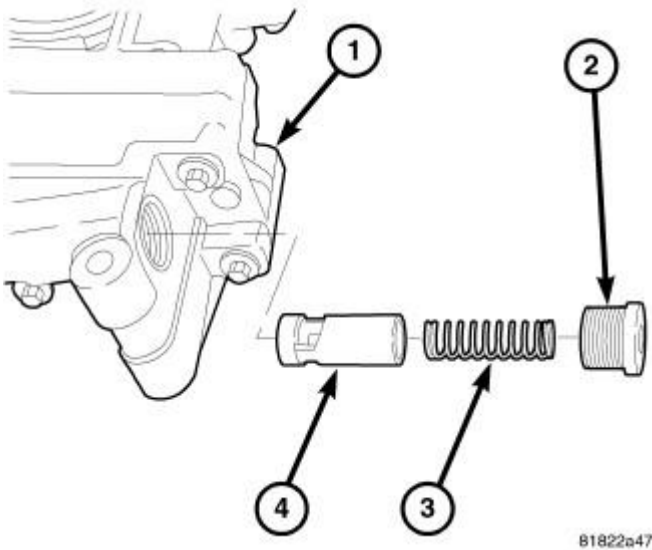
Fig. 388: Oil Pressure Relief Valve Courtesy of CHRYSLER GROUP, LLC
