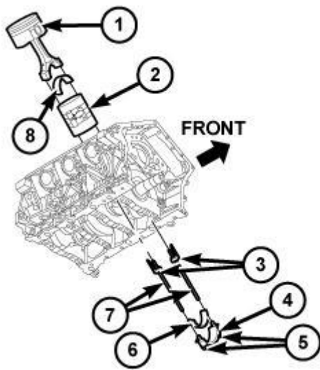
Fig. 272: Piston, Connecting Rod Cap, Bolts, Plastic Guide Plates & Guide Pins Courtesy of CHRYSLER GROUP, LLC
