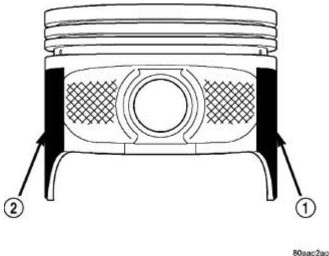
Fig. 267: Coating Material On Piston
