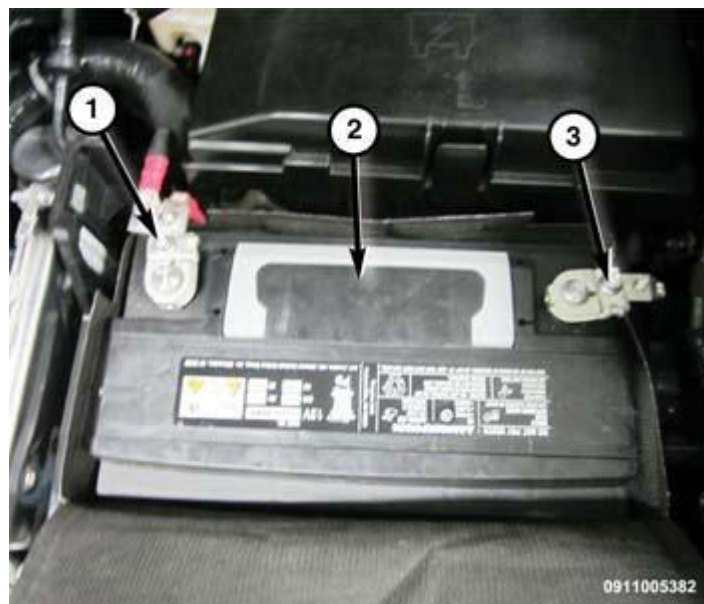
Fig. 49: Battery & Cables
