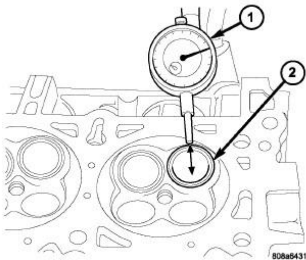
Fig. 165: Measuring Valve Guide Wear
