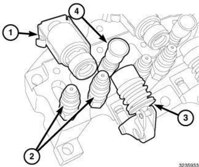
Fig. 177: Solenoid Valve, Hydraulic Brake Pumping Element/Hydraulic Lash Adjusters, Upper Pumping Element & Oil Accumulator
