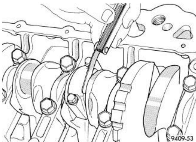
Fig. 269: Connecting Rod Side Clearance Courtesy of CHRYSLER GROUP, LLC
