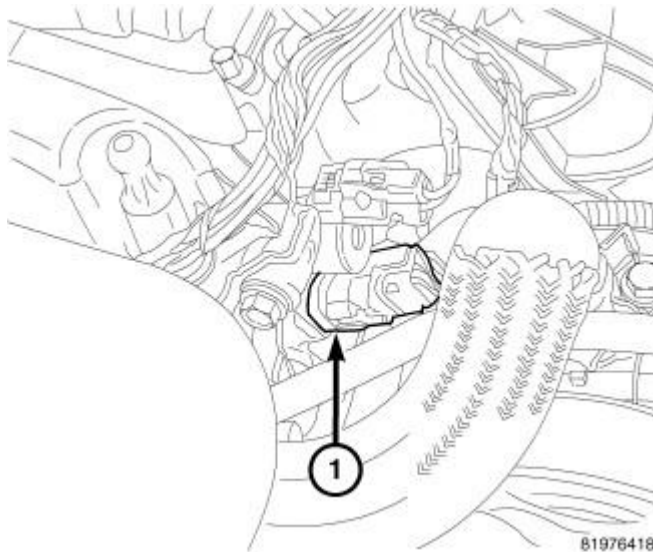
Fig. 343: Oil Temperature Sensor Courtesy of CHRYSLER GROUP, LLC
