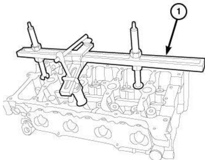
Fig. 149: Valve Spring Compressor Courtesy of CHRYSLER GROUP, LLC
