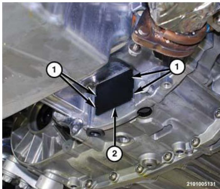
Fig. 32: Access Door In Splash Shield Courtesy of CHRYSLER GROUP, LLC
