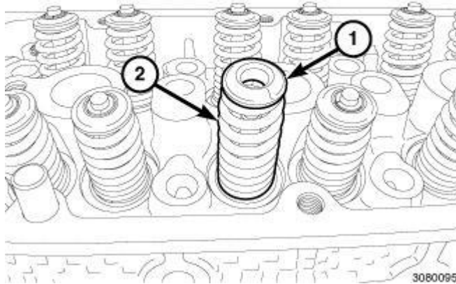
Fig. 168: Valve Spring & Retainer Courtesy of CHRYSLER GROUP, LLC
