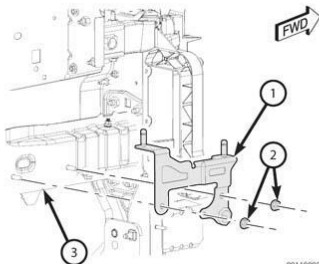
Fig. 333: Removing/Installing Airbox Bracket
