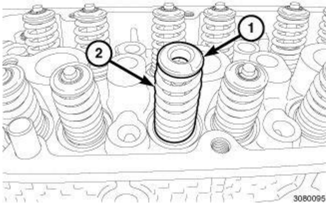
Fig. 161: Valve Spring & Retainer
