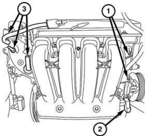
Fig. 322: MAP Sensor Connector & Fittings Courtesy of CHRYSLER GROUP, LLC
