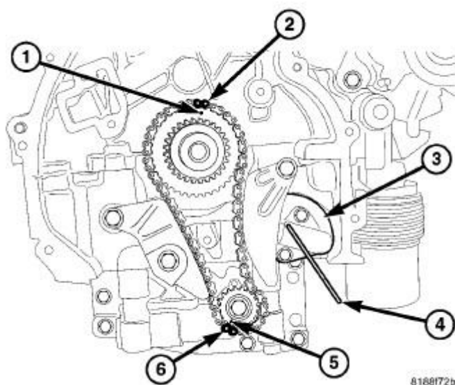
Fig. 398: BSM Timing Chain Marks Courtesy of CHRYSLER GROUP, LLC
