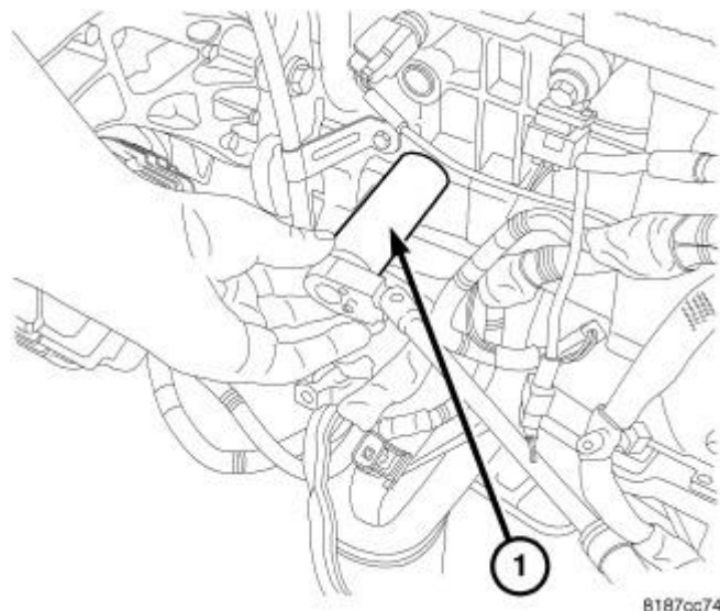
Fig. 347: Oil Sender
