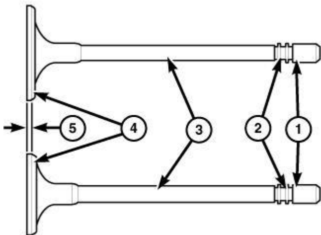
Fig. 154: Inspecting Valve Margin
