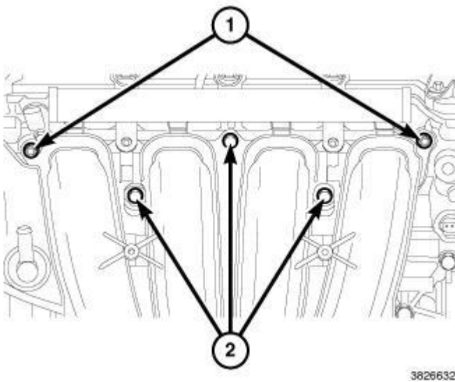
Fig. 324: Intake Manifold Retaining Bolts & Nuts Courtesy of CHRYSLER GROUP, LLC
