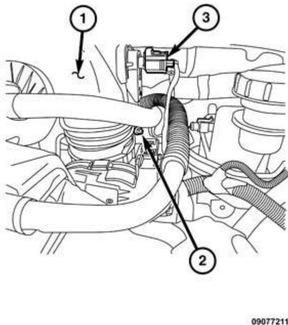
Fig. 312: Resonator, Clamp & Connector
