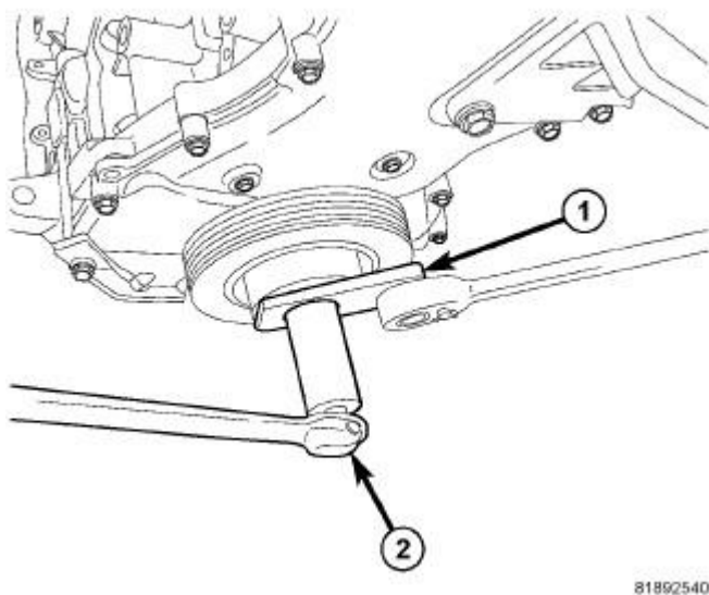
Fig. 245: Removing/Installing Crankshaft Damper Bolt
