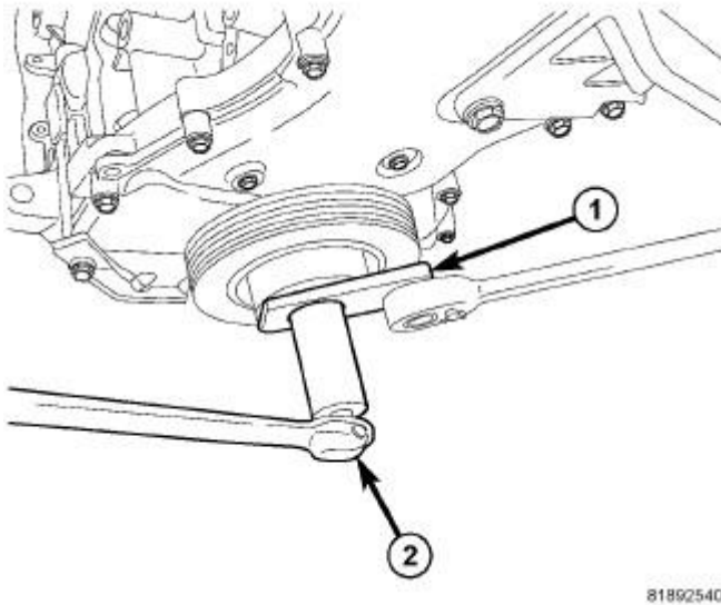
Fig. 278: Removing/Installing Crankshaft Damper Courtesy of CHRYSLER GROUP, LLC
