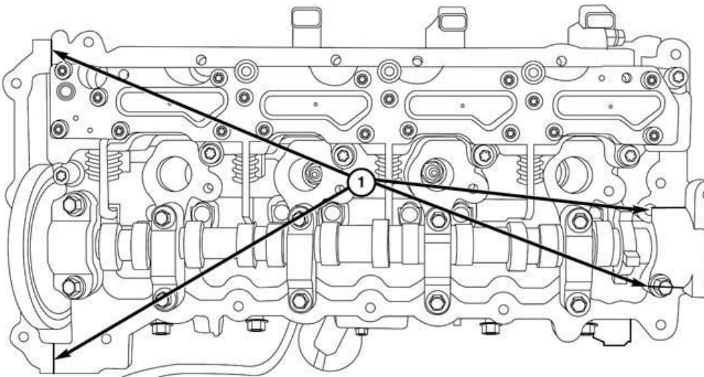
Fig. 116: Sealant Application Areas Courtesy of CHRYSLER GROUP, LLC
