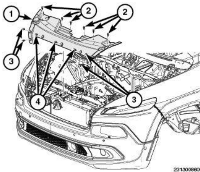
Fig. 46: Upper Close Out Panel Cover Components
