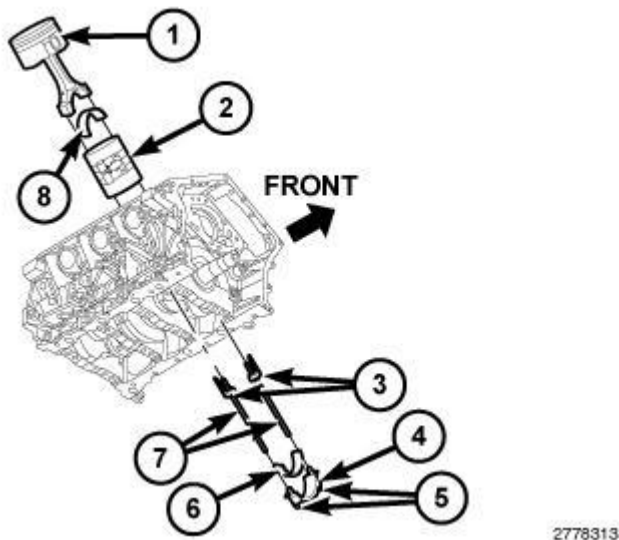
Fig. 222: Piston, Connecting Rod Cap, Bolts, Plastic Guide Plates & Guide Pins Courtesy of CHRYSLER GROUP, LLC
