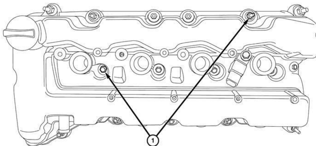
Fig. 120: Cylinder Head Cover Bolts Courtesy of CHRYSLER GROUP, LLC
