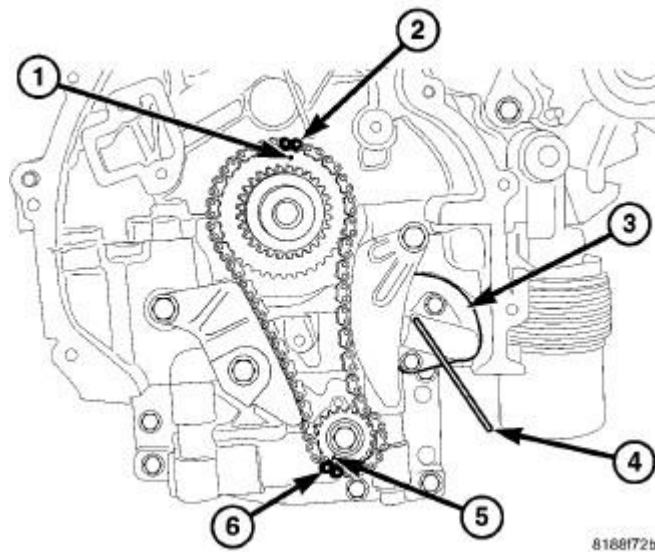
Fig. 410: BSM Timing Chain Marks
