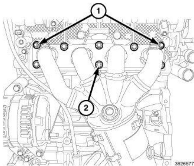
Fig. 70: Exhaust Manifold Bolts Courtesy of CHRYSLER GROUP, LLC
