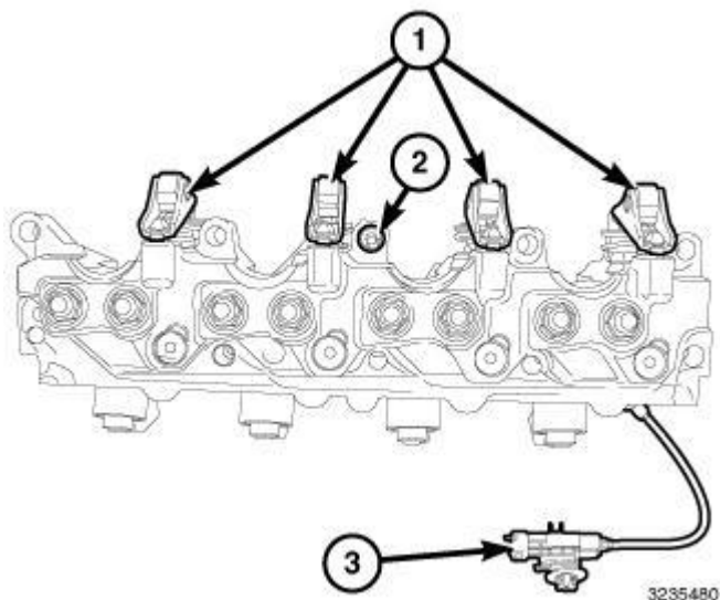
Fig. 190: Valve Rocker Arms, Oil Supply O-Ring & Oil Temperature Sensor
