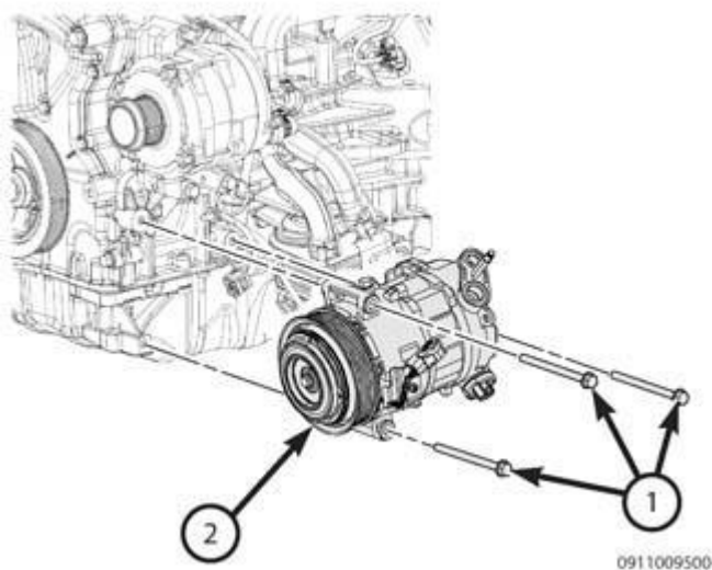
Fig. 41: Air Conditioning Compressor & Bolts Courtesy of CHRYSLER GROUP, LLC
