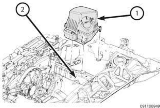
Fig. 58: Removing/Installing Air Cleaner Body
