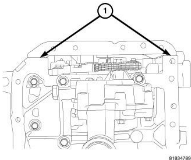
Fig. 363: Sealer Location
