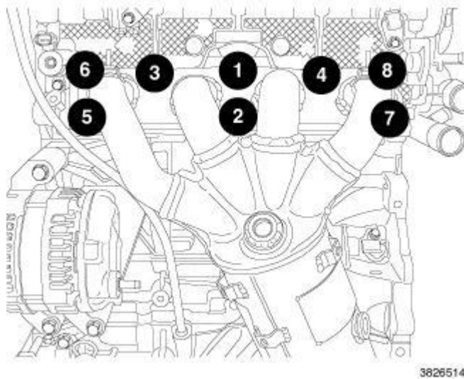
Fig. 94: Exhaust Manifold Bolts Tightening Sequence Courtesy of CHRYSLER GROUP, LLC
