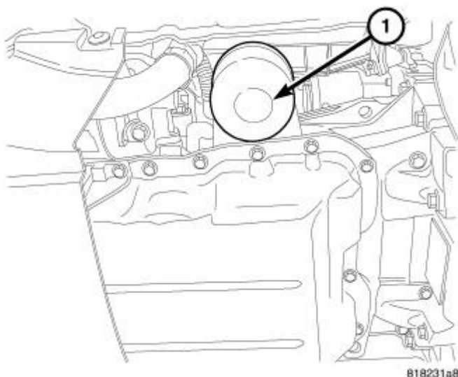
Fig. 352: Oil Filter
