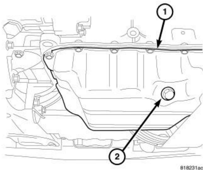
Fig. 360: Oil Drain Plug & Oil Pan
