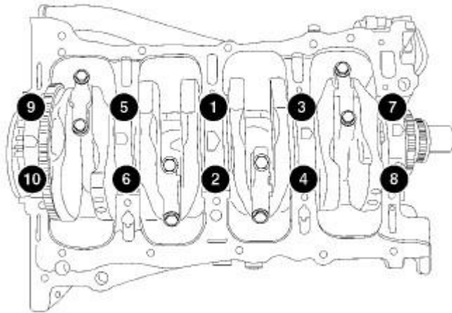
Fig. 234: Main Bearing Cap Removal/Installation Sequence Courtesy of CHRYSLER GROUP, LLC
