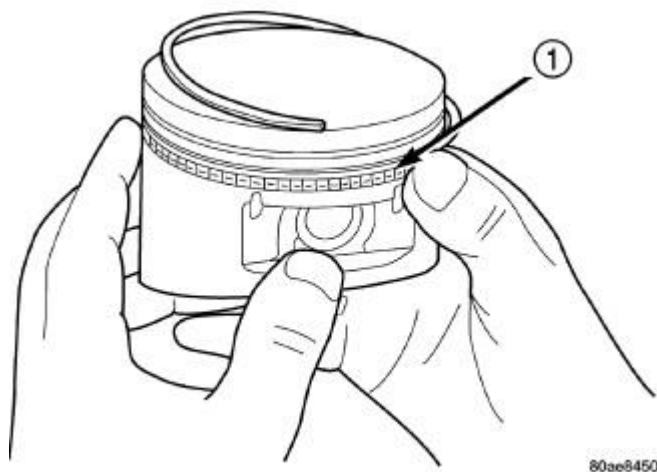
Fig. 257: Removing/Installing Piston Ring Side Rail Courtesy of CHRYSLER GROUP, LLC
