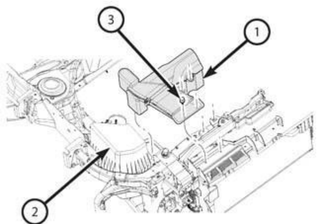
Fig. 13: Removing/Installing Inlet Assembly Courtesy of CHRYSLER GROUP, LLC
