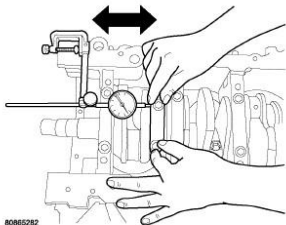
Fig. 268: Measuring Connecting Rod Side Clearance Courtesy of CHRYSLER GROUP, LLC
