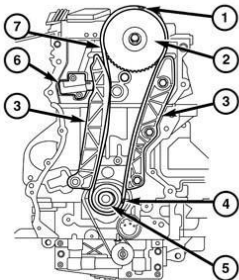
Fig. 74: Timing Chain, Sprockets, Tensioner & Guides
