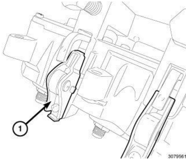
Fig. 192: Rocker Arms Courtesy of CHRYSLER GROUP, LLC
