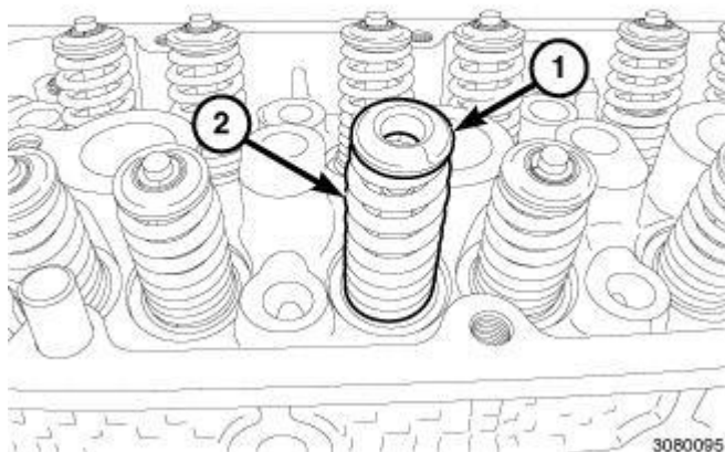
Fig. 126: Valve Spring & Retainer
