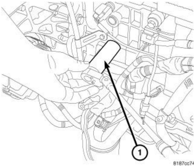
Fig. 344: Oil Sender
