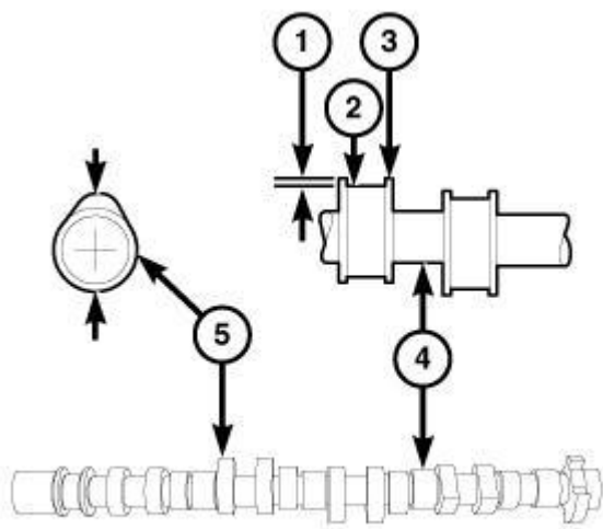
Fig. 109: Inspecting Camshaft Wear Areas Courtesy of CHRYSLER GROUP, LLC
