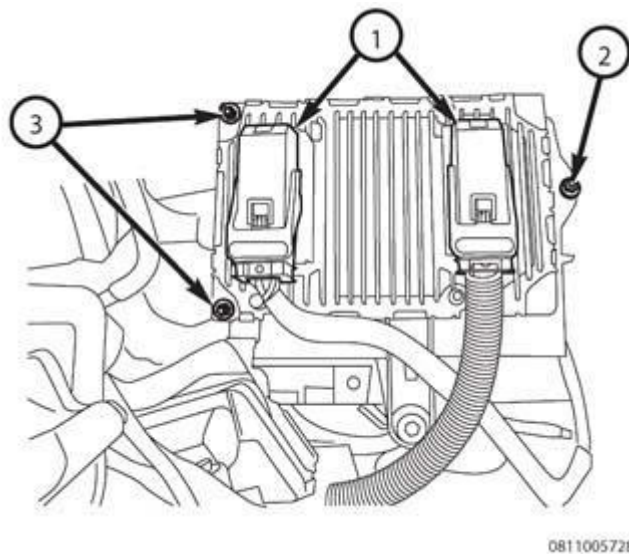
Fig. 11: Powertrain Control Module Electrical Connectors & Nuts Courtesy of CHRYSLER GROUP, LLC
