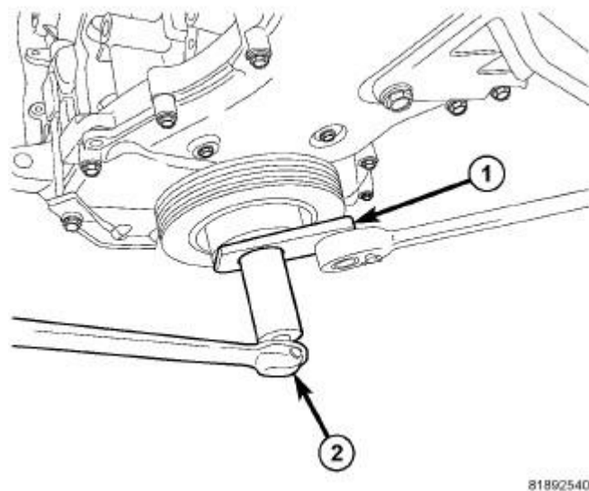
Fig. 283: Installing Damper Holder 9707 Courtesy of CHRYSLER GROUP, LLC
