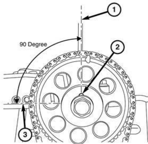
Fig. 104: Vertical Center Line Of Camshaft, Dowel & Cylinder Head Courtesy of CHRYSLER GROUP, LLC
