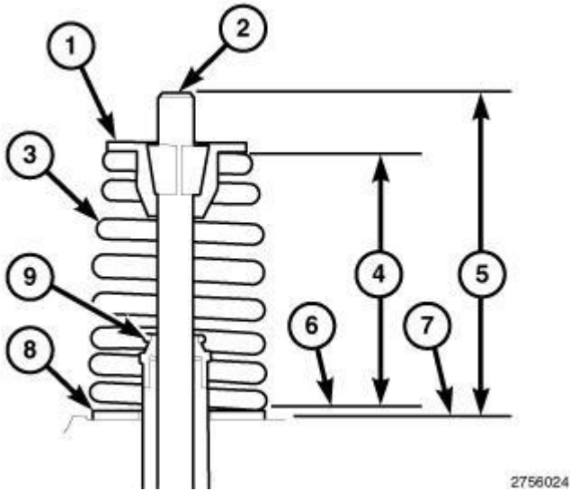
Fig. 156: Checking Valve Spring Installed Height
