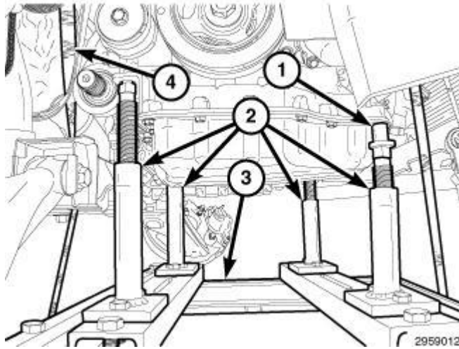
Fig. 28: Adapter, Engine Support Cradle, Power Train Dolly & Safety Straps Courtesy of CHRYSLER GROUP, LLC
