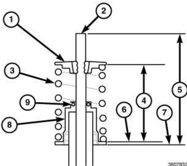
Fig. 151: Valve Spring Component Measurements
