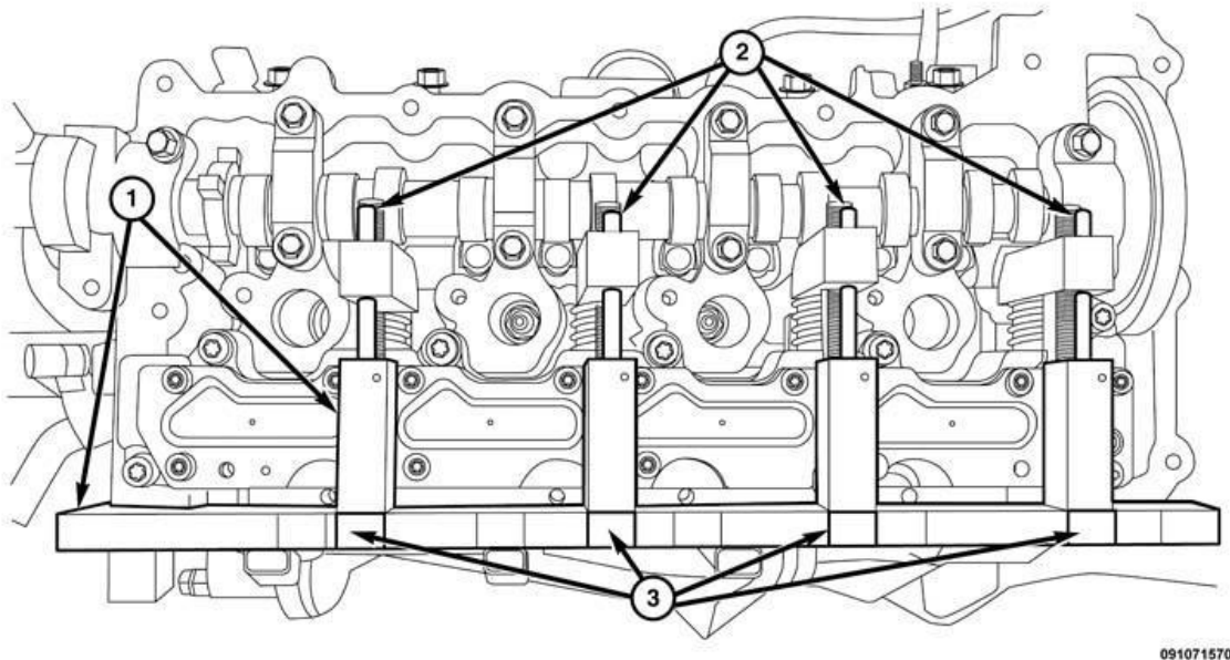
Fig. 193: Special Tool, Spring Compressor & Indicators Courtesy of CHRYSLER GROUP, LLC
