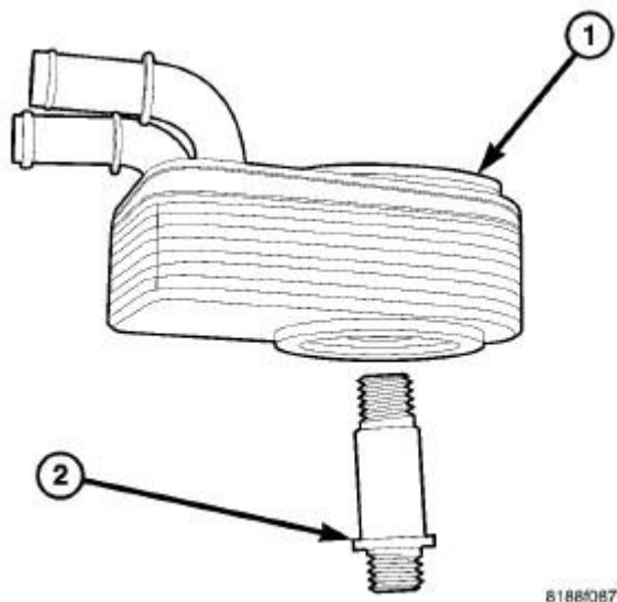
Fig. 350: Oil Cooler Mounting Courtesy of CHRYSLER GROUP, LLC
