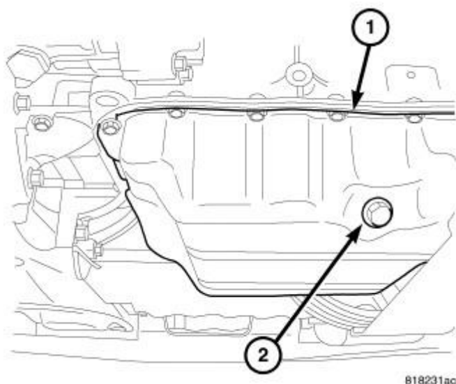
Fig. 356: Oil Drain Plug & Oil Pan Courtesy of CHRYSLER GROUP, LLC
