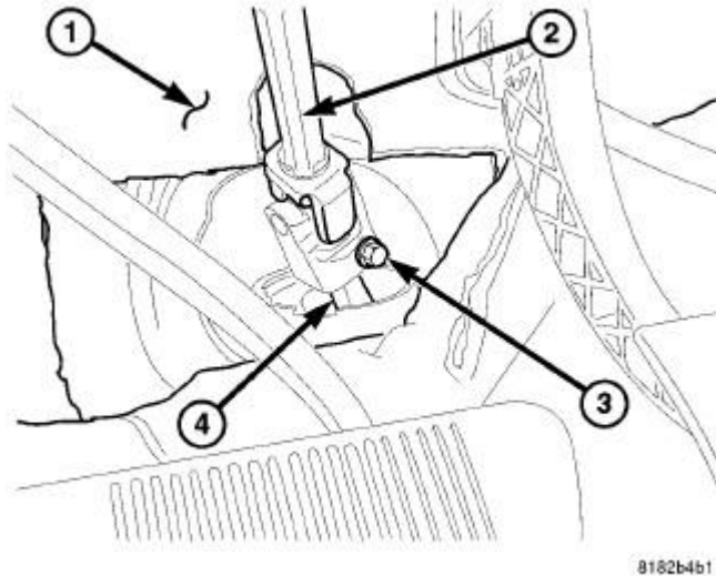
Fig. 8: Lower Coupling Bolt
