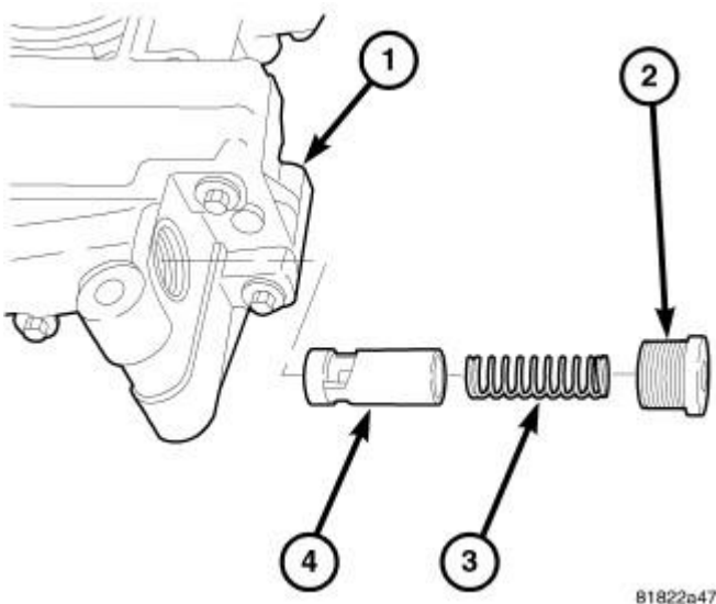
Fig. 389: Oil Pressure Relief Valve Courtesy of CHRYSLER GROUP, LLC
