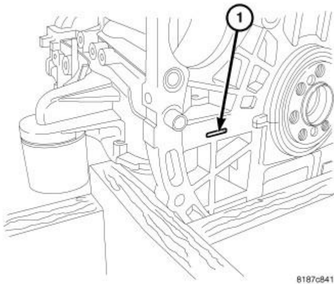
Fig. 249: Pry Point 1
