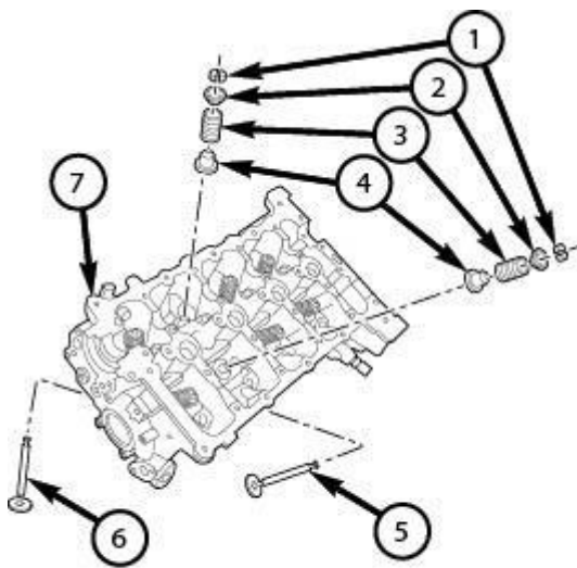
Fig. 152: Cylinder Head, Valves & Springs Courtesy of CHRYSLER GROUP, LLC
