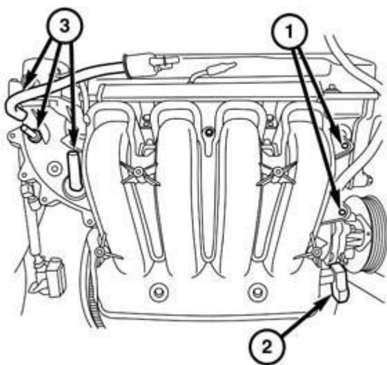
Fig. 328: MAP Sensor Connector & Fittings
