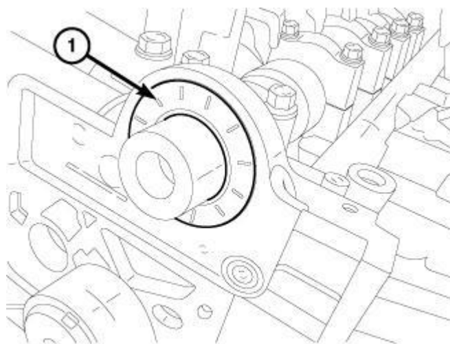
Fig. 112: Camshaft Seal Courtesy of CHRYSLER GROUP, LLC
