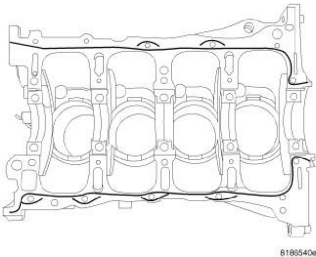
Fig. 251: Sealing Ladder Frame
