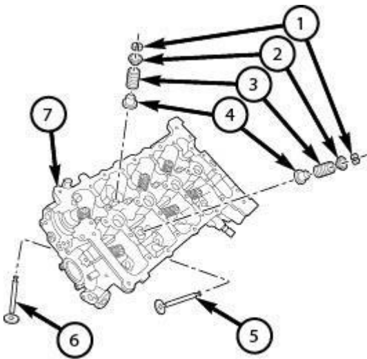
Fig. 65: Cylinder Head, Valves & Springs Courtesy of CHRYSLER GROUP, LLC
