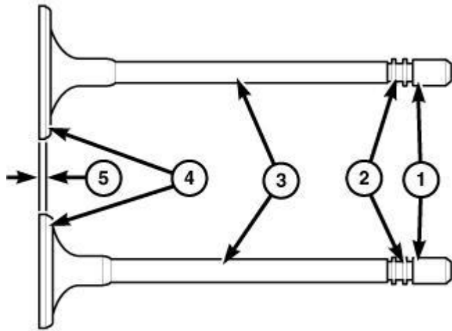
Fig. 162: Inspecting Valve Margin Courtesy of CHRYSLER GROUP, LLC
