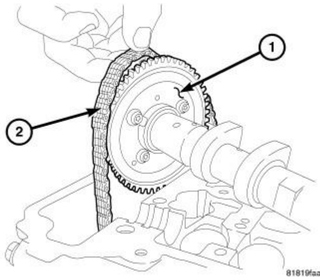
Fig. 108: Chain Removal Courtesy of CHRYSLER GROUP, LLC
