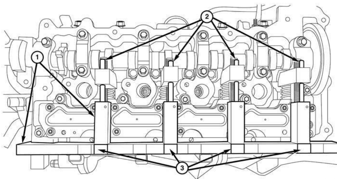
Fig. 122: Special Tool, Spring Compressor & Indicators
