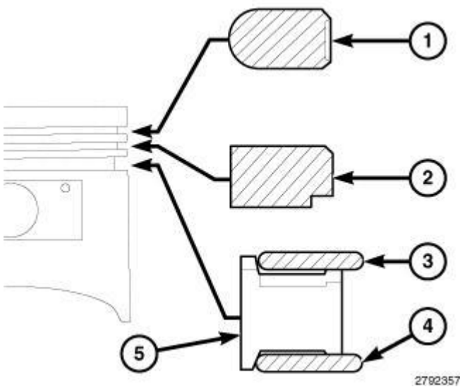
Fig. 255: Piston Ring Removal/Installation Sequence
