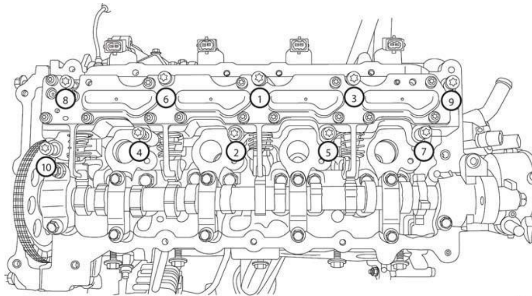
Fig. 197: Variable Valve Actuation Assembly Tightening Sequence Courtesy of CHRYSLER GROUP, LLC
