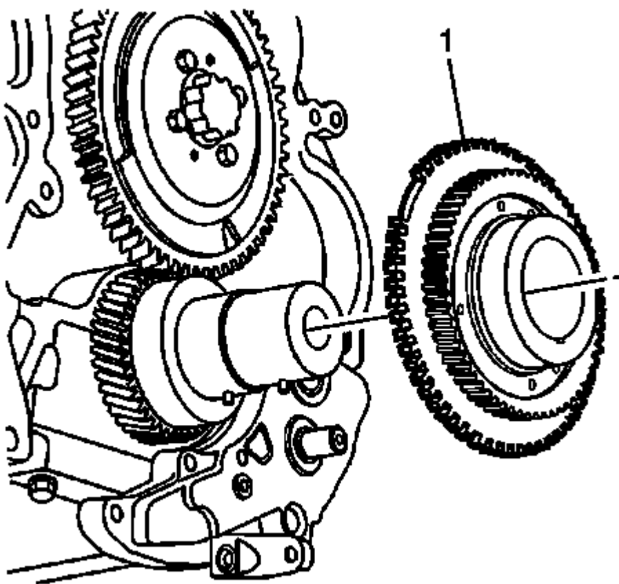
Fig. 126: View Of Oil Pump Drive Gear Courtesy of GENERAL MOTORS COMPANY
