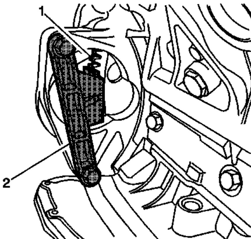
Fig. 143: Locking Flywheel Using Special Tool Courtesy of GENERAL MOTORS COMPANY
