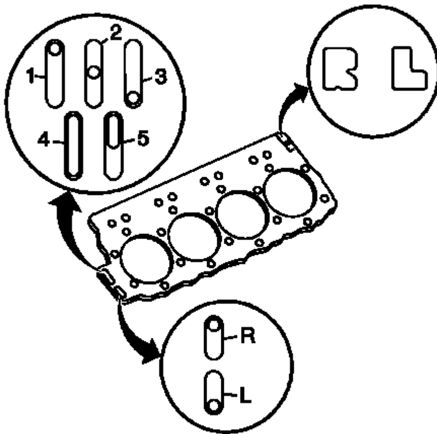
Fig. 82: View Of Cylinder Head Gasket Markings Courtesy of GENERAL MOTORS COMPANY
