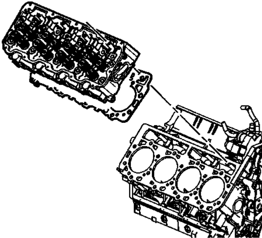
Fig. 92: View Of Cylinder Head & Gasket (Right) Courtesy of GENERAL MOTORS COMPANY
