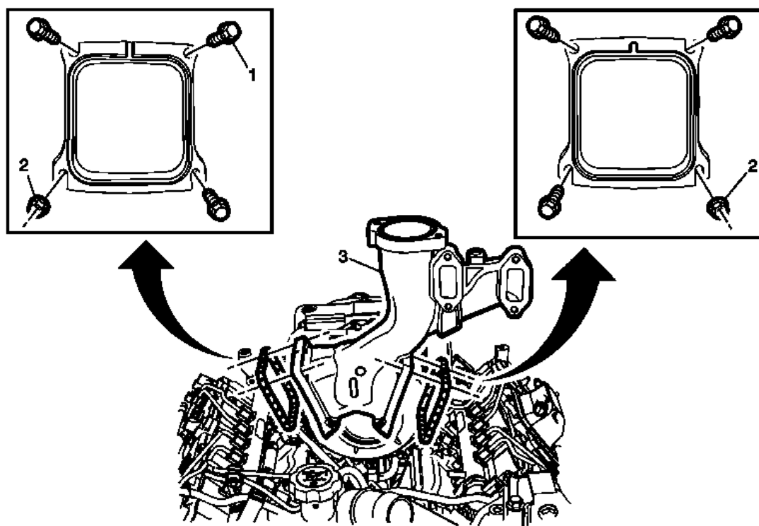
Fig. 37: Identifying Center Intake Manifold And Fasteners Courtesy of GENERAL MOTORS COMPANY
