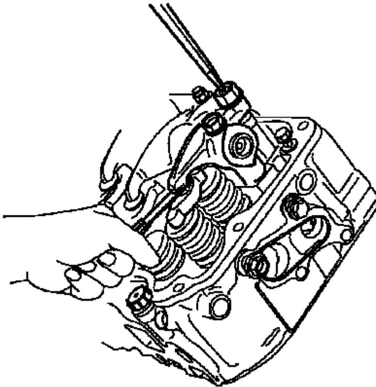
Fig. 62: View Of Feeler Gage Between Tip Of Rocker Arm & Valve Lifter Bridge Courtesy of GENERAL MOTORS COMPANY
