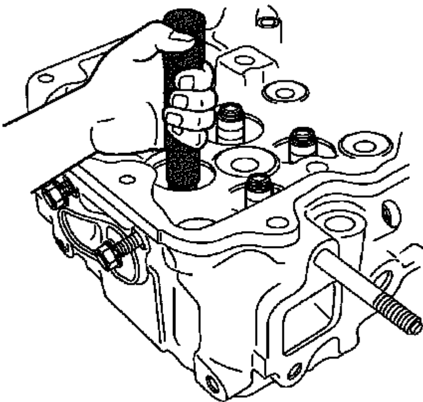
Fig. 99: Installing Valve Stem Seal Courtesy of GENERAL MOTORS COMPANY
