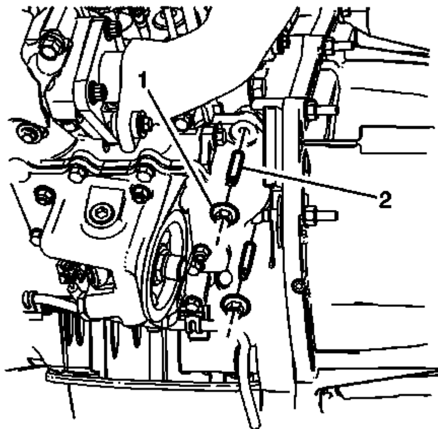
Fig. 252: Oil Cooler Adapter Nuts And Studs Courtesy of GENERAL MOTORS COMPANY
