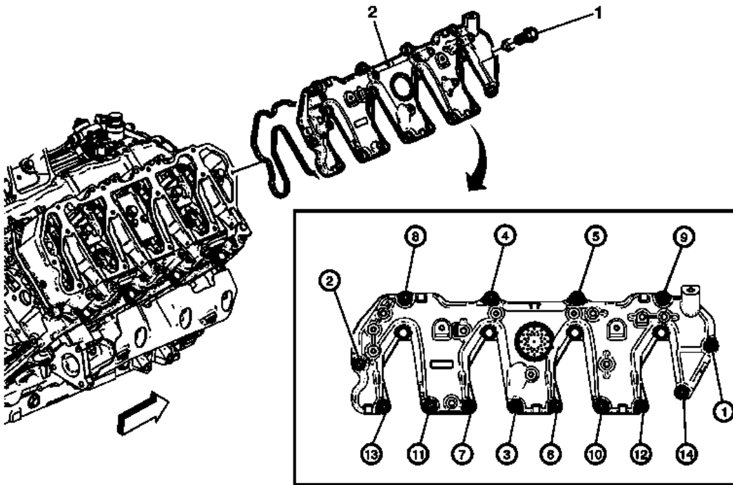
Fig. 49: Valve Rocker Arm Upper Cover And Fasteners With Tightening Sequence - Right Side Courtesy of GENERAL MOTORS COMPANY
