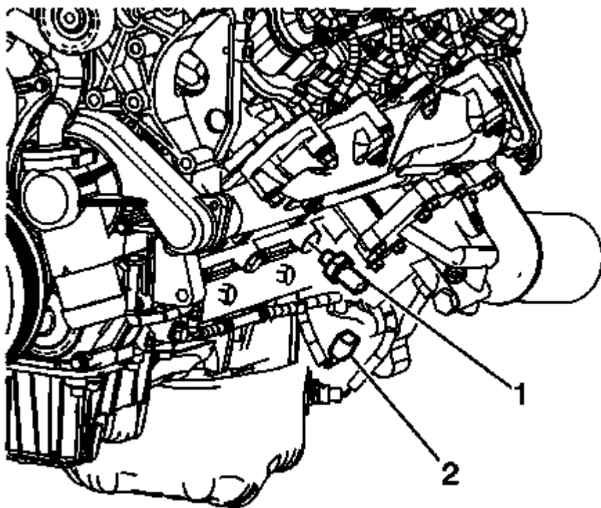
Fig. 208: View Of Engine Harness Electrical Connector Courtesy of GENERAL MOTORS COMPANY
