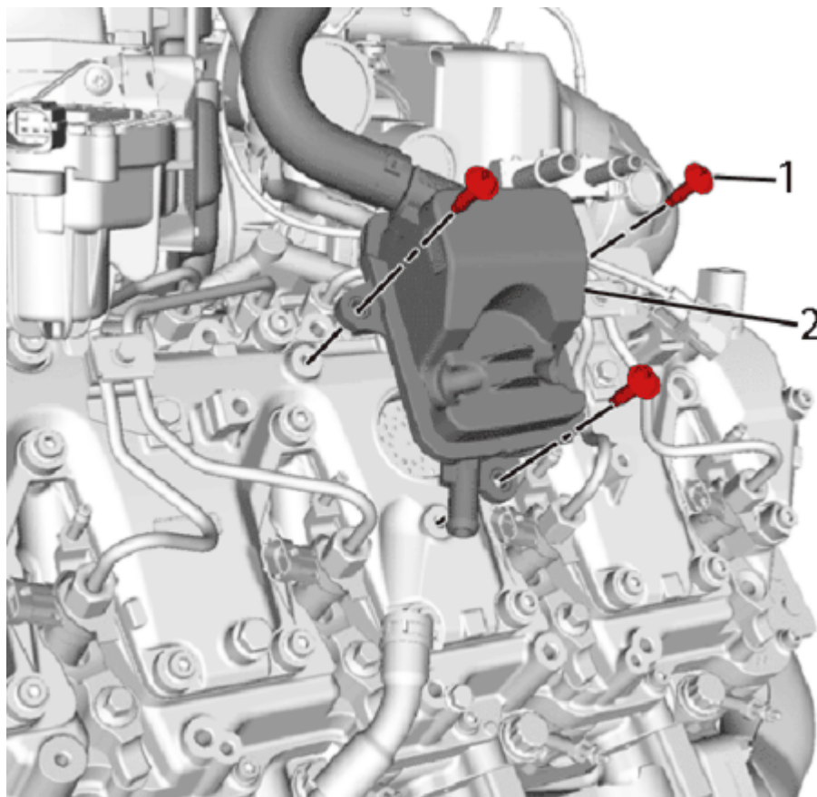
Fig. 29: Oil Separator
