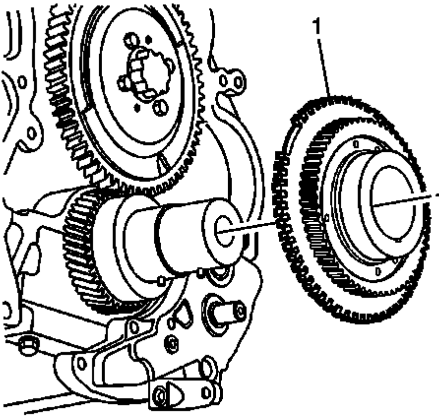
Fig. 159: View Of Oil Pump Drive Gear Courtesy of GENERAL MOTORS COMPANY
