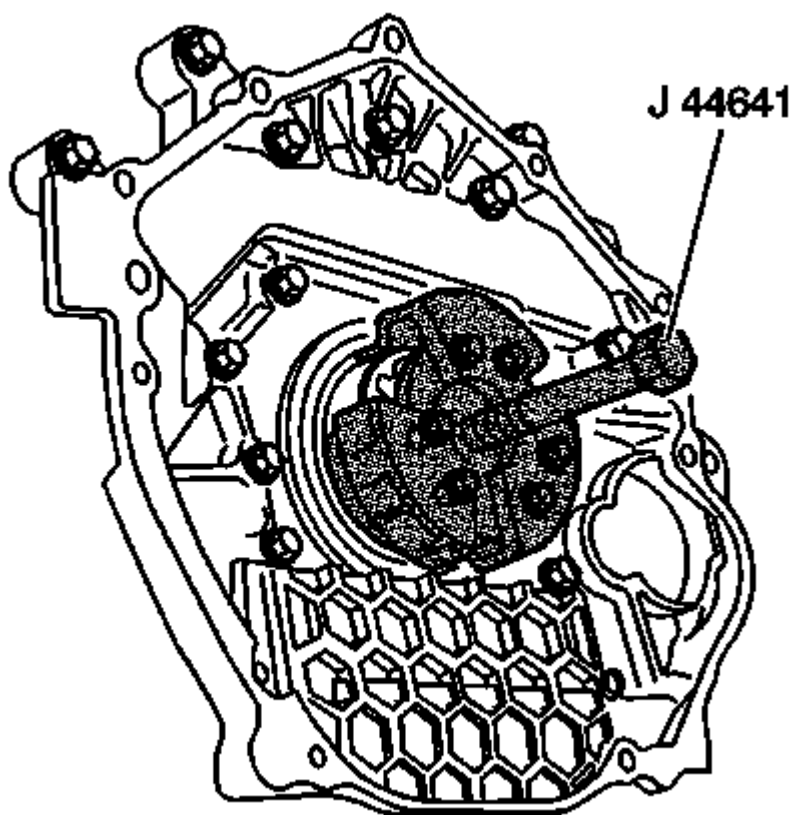
Fig. 161: Crankshaft Rear Oil Seal And Special Tool Courtesy of GENERAL MOTORS COMPANY
