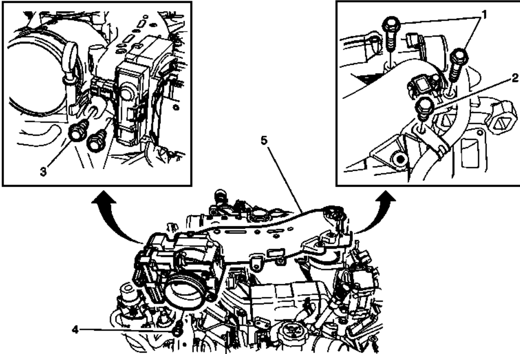
Fig. 36: Intake Manifold Tube And Fasteners Courtesy of GENERAL MOTORS COMPANY
