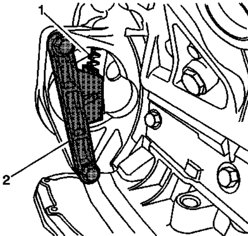
Fig. 173: Locking Flywheel Using Special Tool Courtesy of GENERAL MOTORS COMPANY
