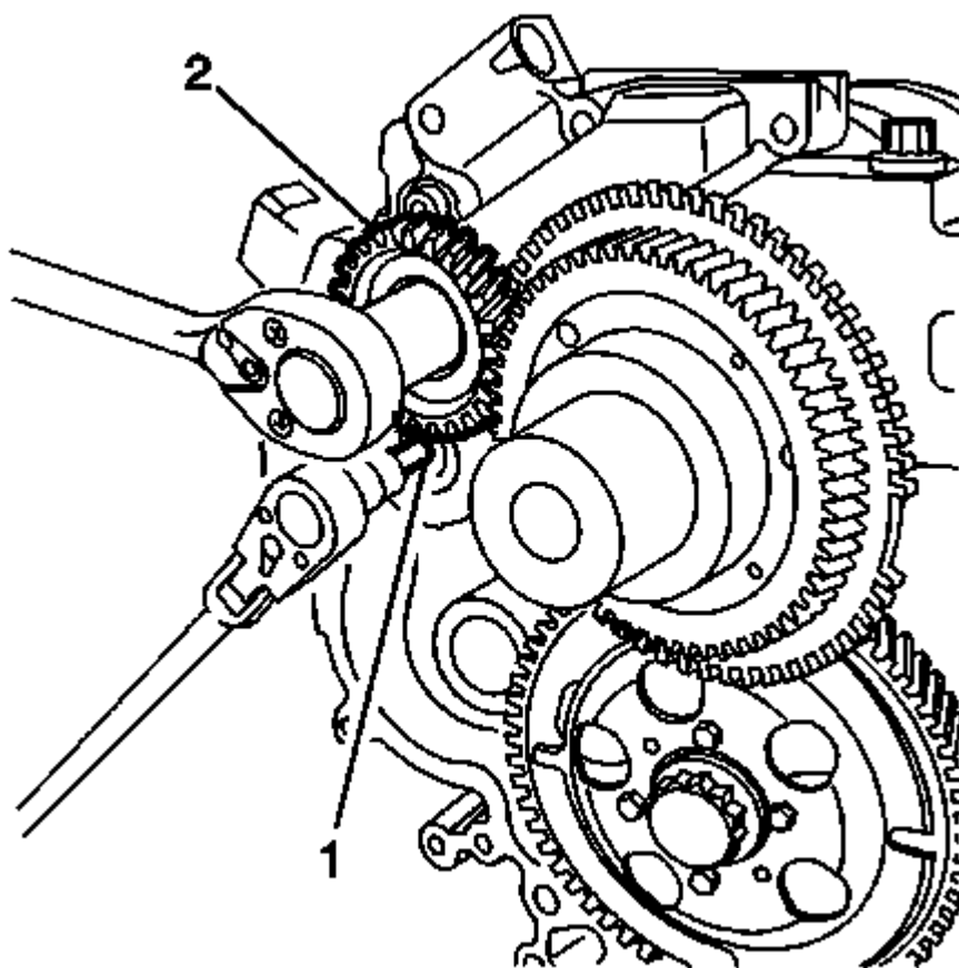
Fig. 199: View of Secondary Oil Pump Driven Gear Nut While Holding Oil Pump Shaft Courtesy of GENERAL MOTORS COMPANY
