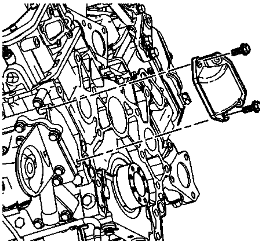
Fig. 166: View Of Oil Cooler Adapter Courtesy of GENERAL MOTORS COMPANY
