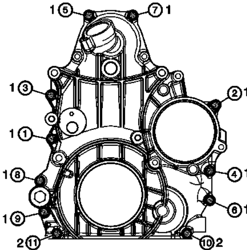
Fig. 120: Identifying Engine Front Cover Bolt Tightening Sequence Courtesy of GENERAL MOTORS COMPANY
