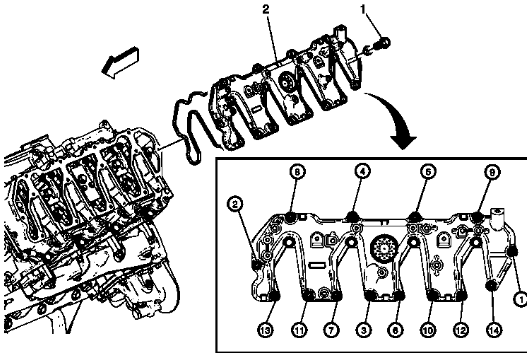
Fig. 48: Valve Rocker Arm Upper Cover And Fasteners With Tightening Sequence - Left Side Courtesy of GENERAL MOTORS COMPANY
