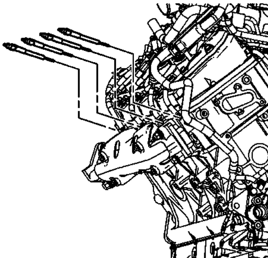
Fig. 87: View Of Right Glow Plugs Courtesy of GENERAL MOTORS COMPANY
