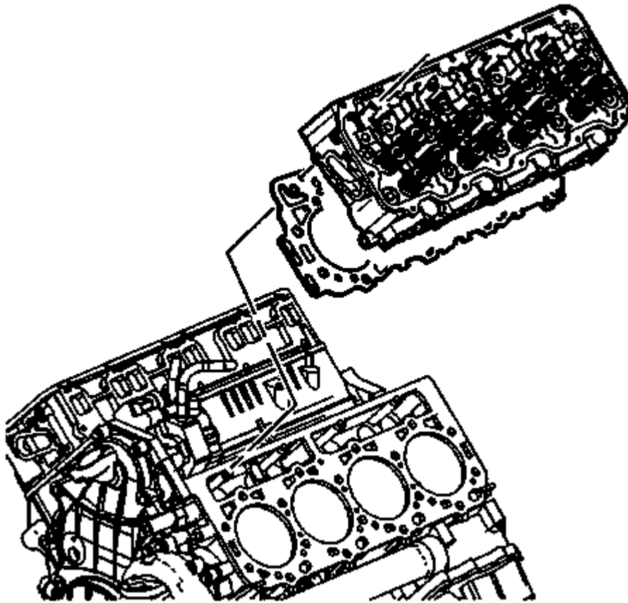
Fig. 83: View Of Left Cylinder Head Gasket Courtesy of GENERAL MOTORS COMPANY
