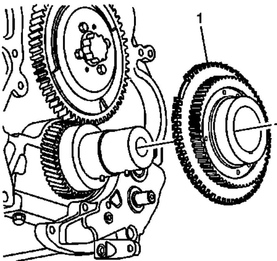
Fig. 194: View Of Oil Pump Drive Gear Courtesy of GENERAL MOTORS COMPANY
