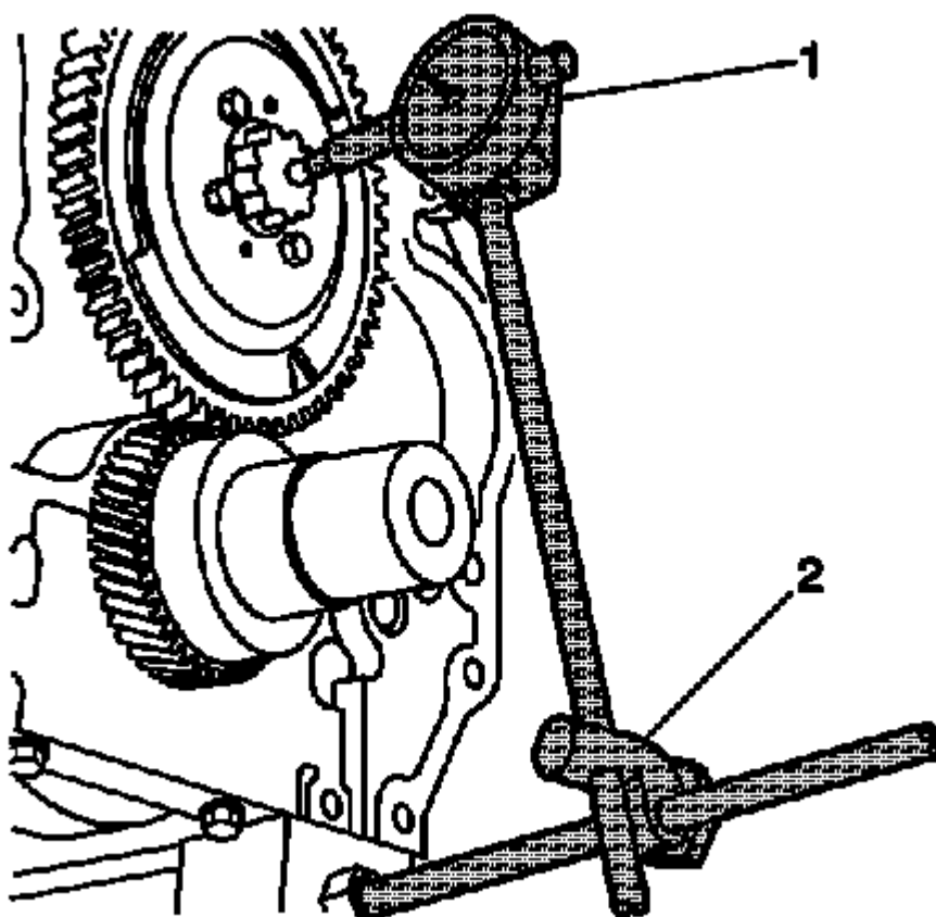
Fig. 158: Camshaft End Play Dial Indicator And Magnetic Base Courtesy of GENERAL MOTORS COMPANY
