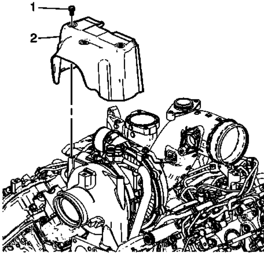
Fig. 76: Turbocharger Upper Heat Shield And Bolts Courtesy of GENERAL MOTORS COMPANY
