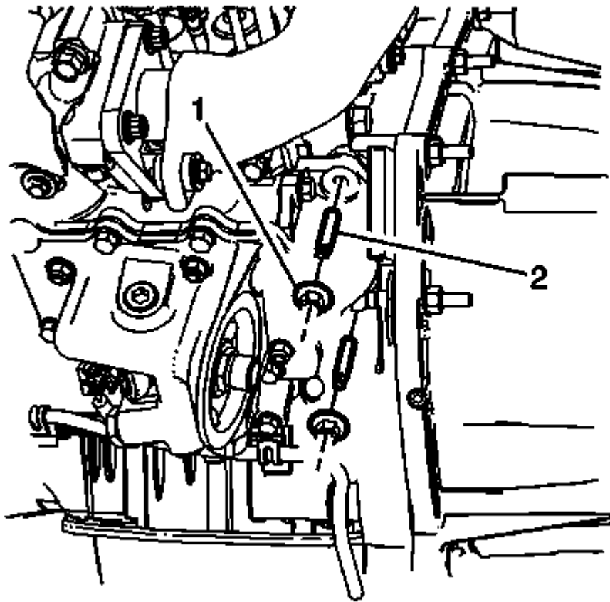
Fig. 202: Oil Cooler Adapter Nuts And Studs Courtesy of GENERAL MOTORS COMPANY
