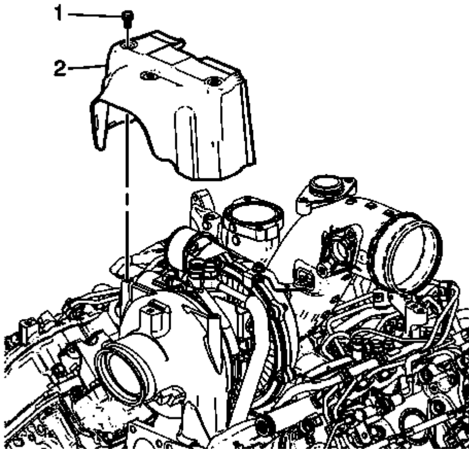
Fig. 66: Turbocharger Upper Heat Shield And Bolts Courtesy of GENERAL MOTORS COMPANY
