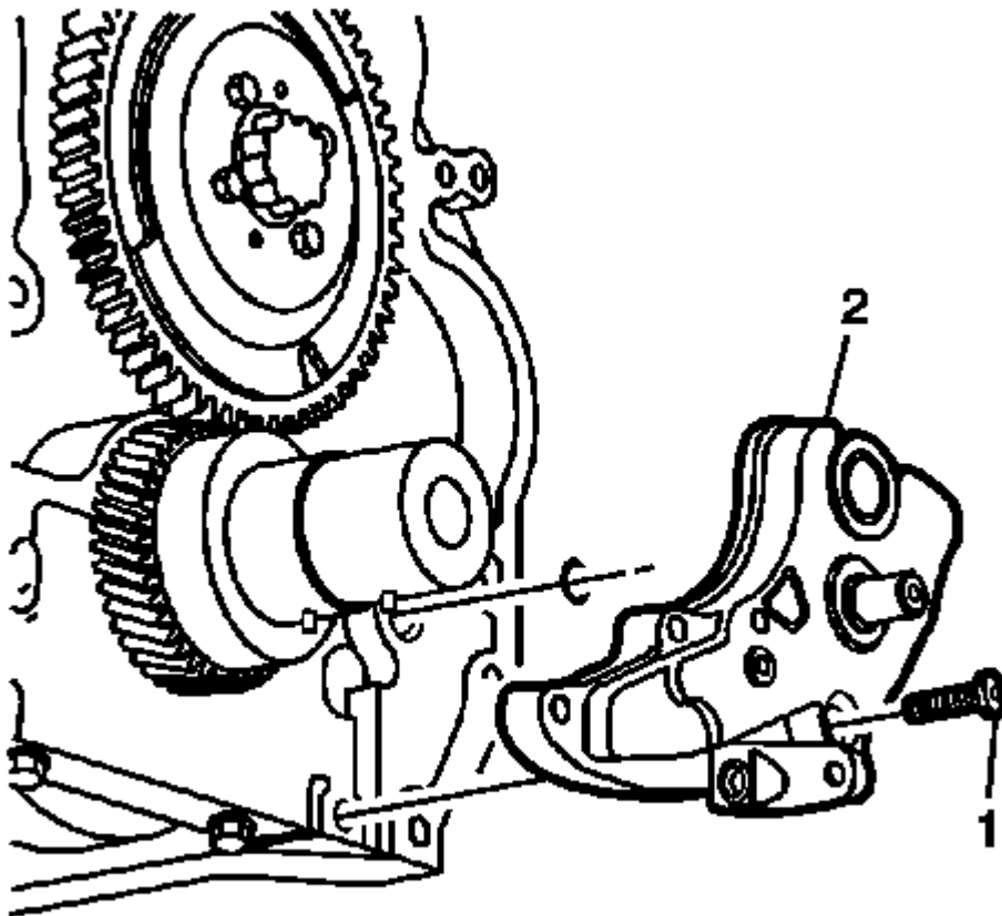
Fig. 195: View Of Oil Pump, O-Ring Seal & Bolt Courtesy of GENERAL MOTORS COMPANY
