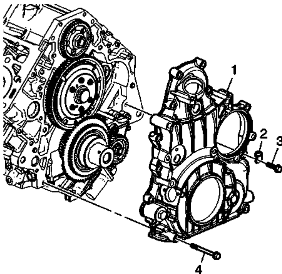
Fig. 116: View Of Engine Front Cover & Bolts Courtesy of GENERAL MOTORS COMPANY
