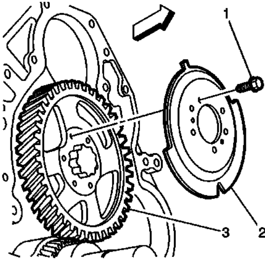
Fig. 127: View Of Camshaft Reluctor & Bolts Courtesy of GENERAL MOTORS COMPANY
