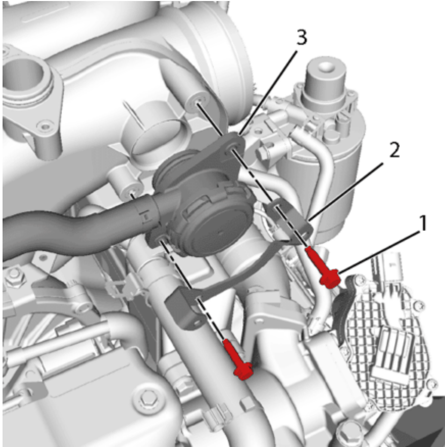
Fig. 31: Crankcase Depression Regulator Valve Courtesy of GENERAL MOTORS COMPANY
