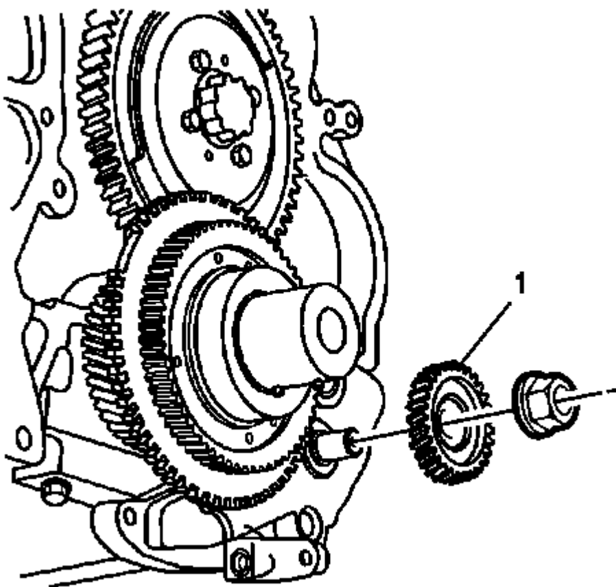
Fig. 135: View Of Oil Pump Driven Gear & Nut Courtesy of GENERAL MOTORS COMPANY
