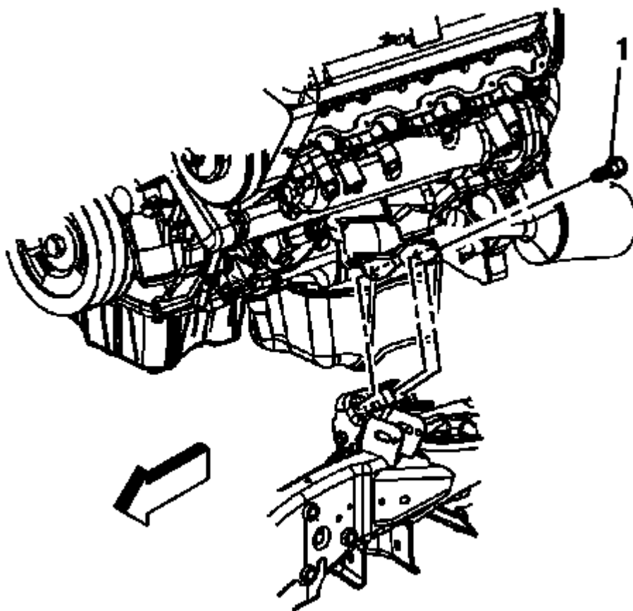
Fig. 235: Left Side Engine Mount And Bolt Courtesy of GENERAL MOTORS COMPANY
