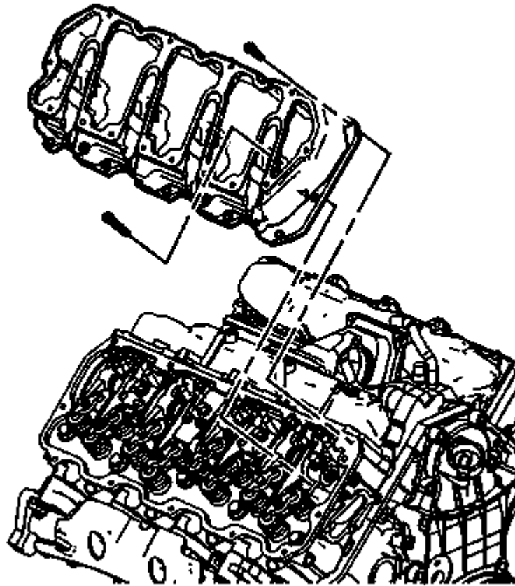
Fig. 88: View Of Lower Valve Rocker Arm Cover (Right) Courtesy of GENERAL MOTORS COMPANY
