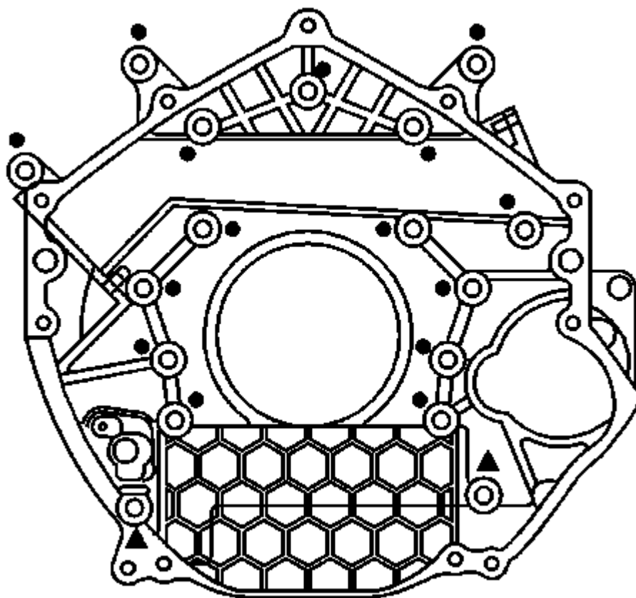
Fig. 165: View Of Engine Rear Cover Bolts & Flywheel Housing To Upper Oil Pan Bolts Courtesy of GENERAL MOTORS COMPANY
