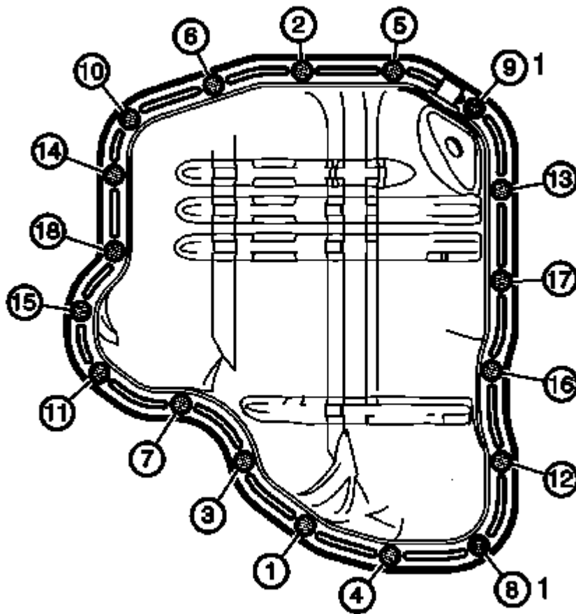
Fig. 182: Lower Oil Pan Bolt Tightening Sequence Courtesy of GENERAL MOTORS COMPANY
