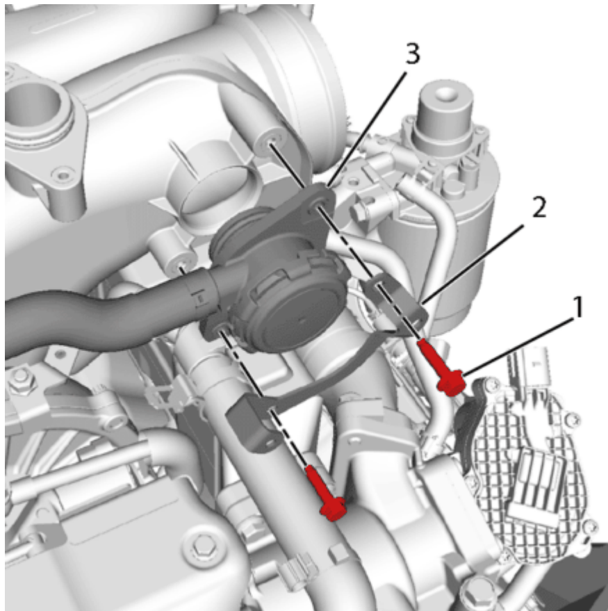
Fig. 32: Crankcase Depression Regulator Valve Courtesy of GENERAL MOTORS COMPANY
