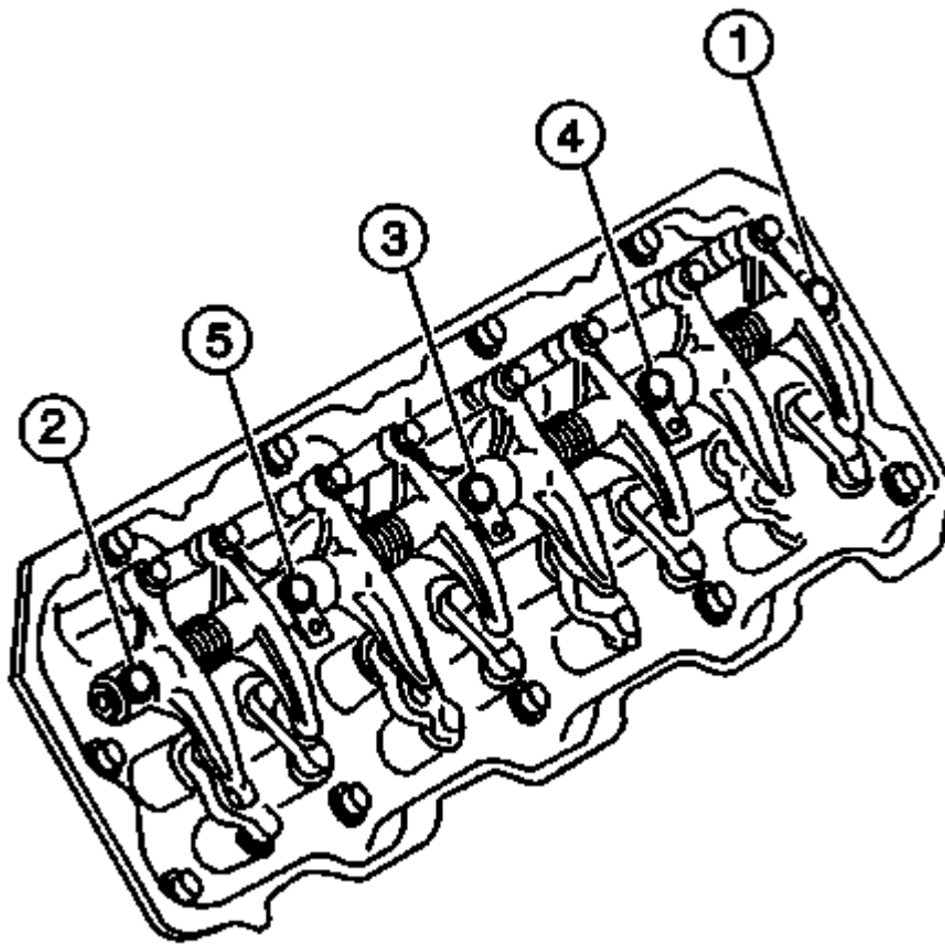
Fig. 53: Rocker Arm Shaft Bolts Loosening Sequence Courtesy of GENERAL MOTORS COMPANY
