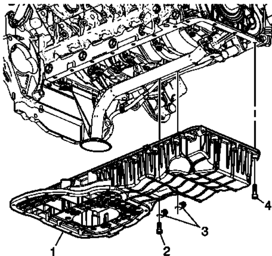
Fig. 185: View Of Upper Oil Pan & Bolts Courtesy of GENERAL MOTORS COMPANY
