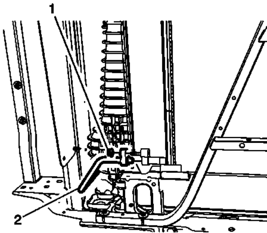
Fig. 220: Identifying Evaporator Tube And Nut Courtesy of GENERAL MOTORS COMPANY
