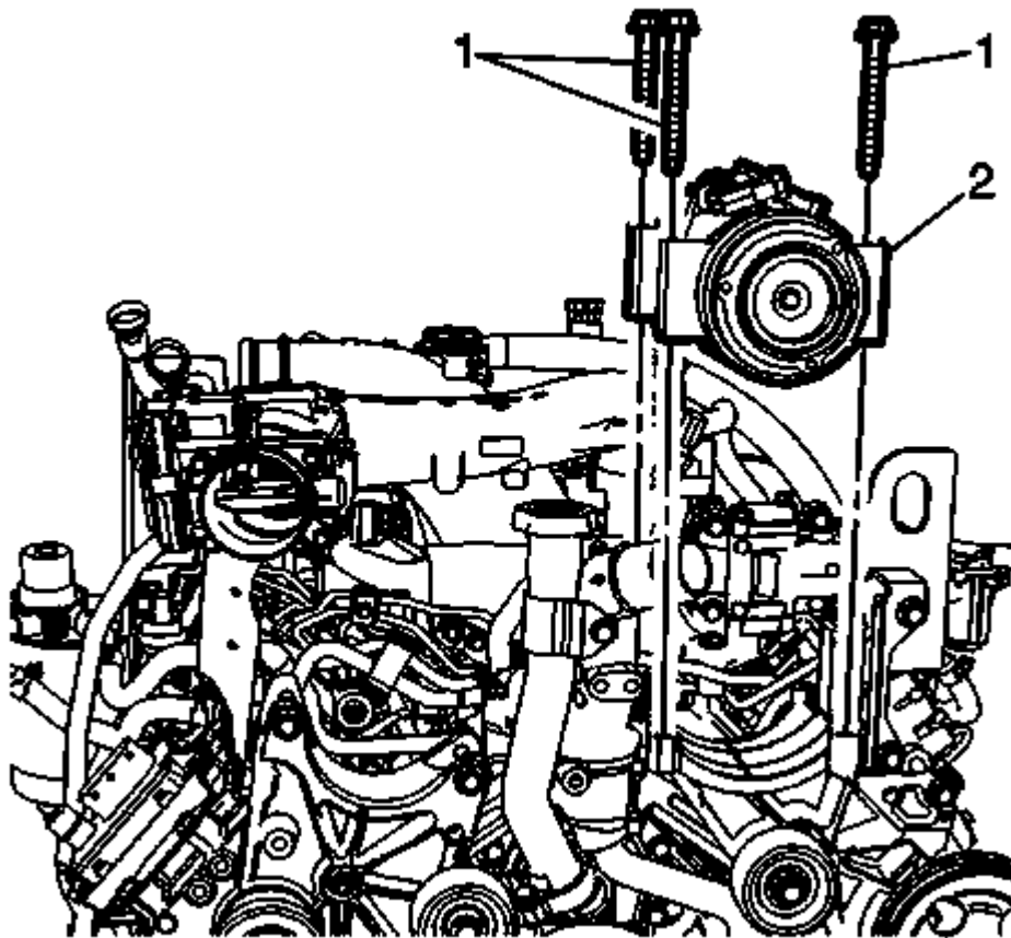
Fig. 226: Air Conditioning Compressor Courtesy of GENERAL MOTORS COMPANY
