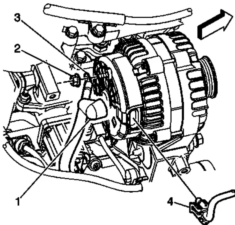
Fig. 227: View Of Generator Positive Terminal & Protective Boot Courtesy of GENERAL MOTORS COMPANY
