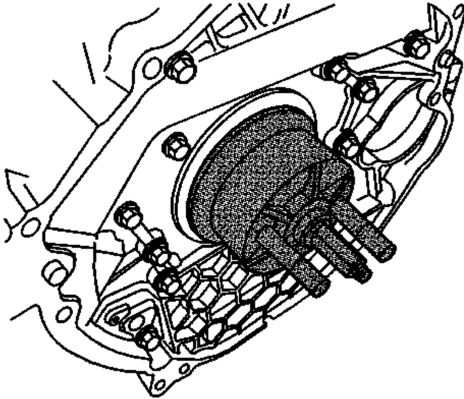
Fig. 162: Crankshaft Rear Oil Seal Installer Courtesy of GENERAL MOTORS COMPANY
