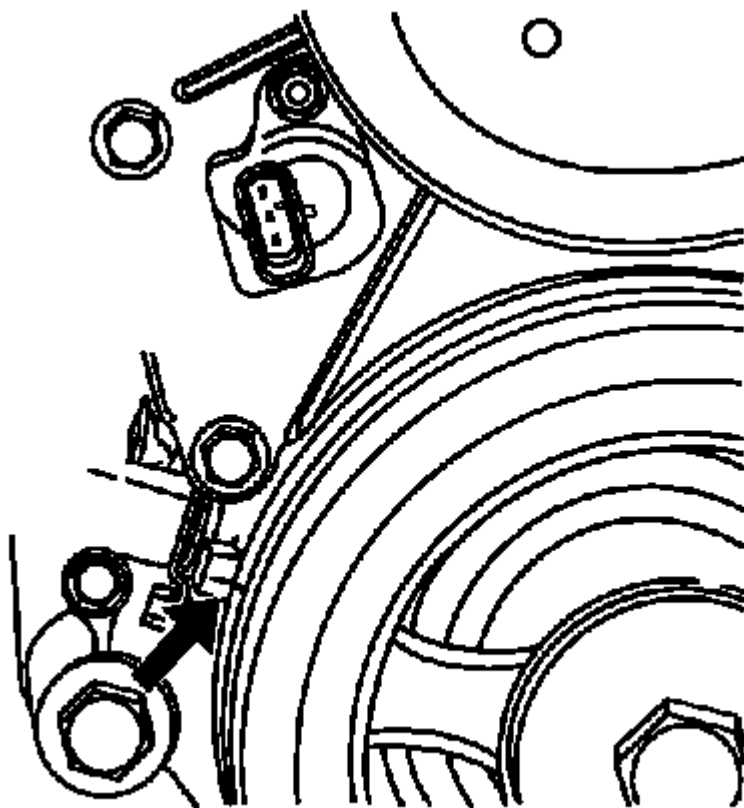
Fig. 61: View Of Crankshaft Balancer Mark Aligned With Engine Mark Courtesy of GENERAL MOTORS COMPANY
