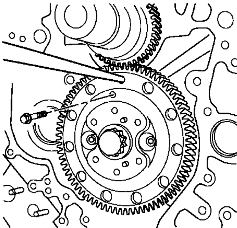
Fig. 128: Using Exciter Ring Bolt To Secure Spring Tension Courtesy of GENERAL MOTORS COMPANY
