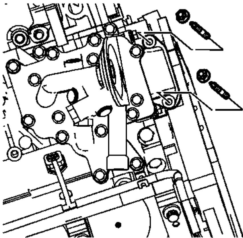
Fig. 163: View Of Turbocharger Oil Return Pipe Nuts Courtesy of GENERAL MOTORS COMPANY
