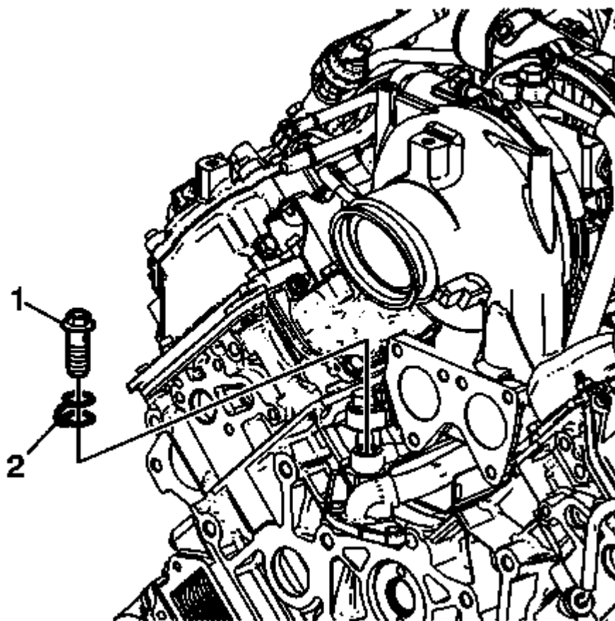
Fig. 75: View Of Turbocharger Oil Feed Pipe Eye Bolt & Washer Courtesy of GENERAL MOTORS COMPANY
