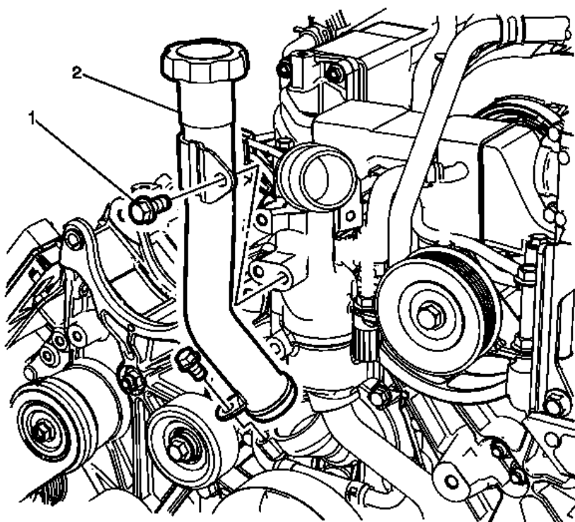
Fig. 46: Oil Filler Tube
