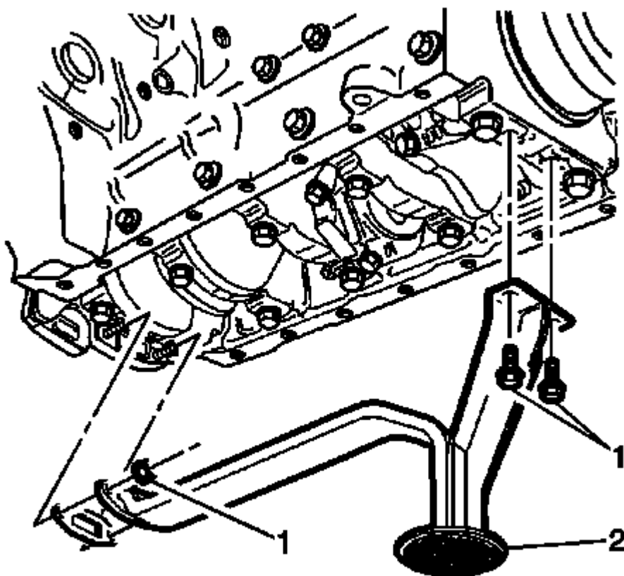
Fig. 190: View Of Oil Pump Screen, Bolts, Nuts & Gasket Courtesy of GENERAL MOTORS COMPANY
