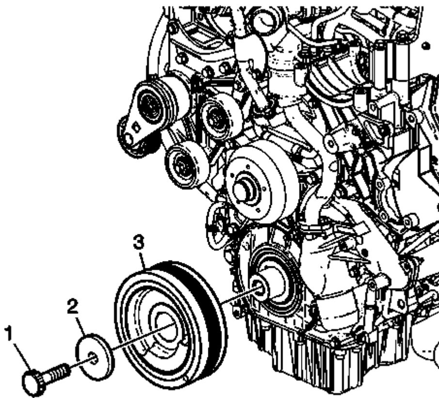
Fig. 107: Identifying Crankshaft Balancer, Washer And Bolt Courtesy of GENERAL MOTORS COMPANY
