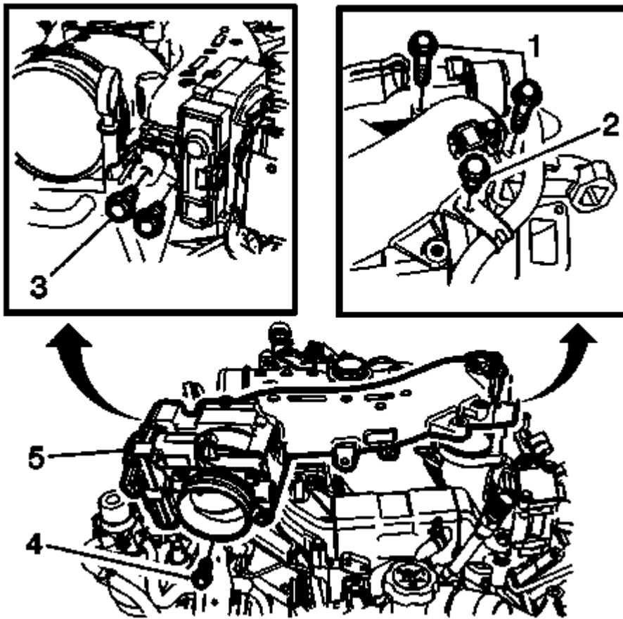
Fig. 254: Intake Manifold Tube
