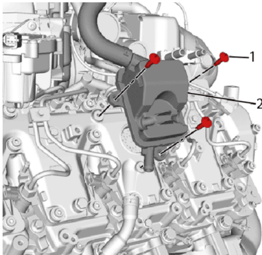
Fig. 34: Oil Separator
