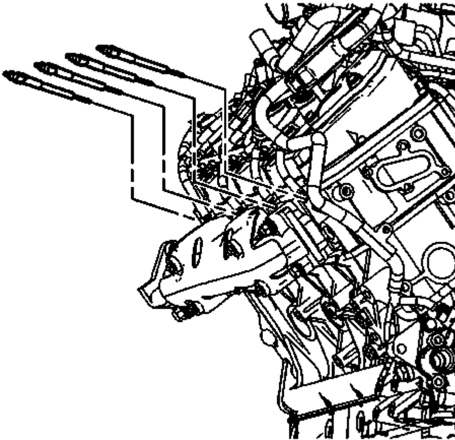
Fig. 78: View Of Right Glow Plugs Courtesy of GENERAL MOTORS COMPANY
