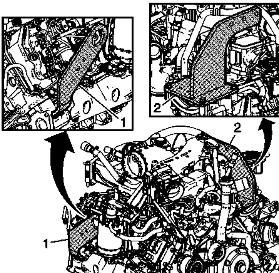
Fig. 231: Lift Brackets
