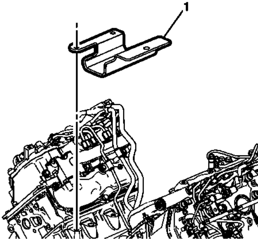
Fig. 72: Turbocharger Lower Heat Shield Courtesy of GENERAL MOTORS COMPANY
