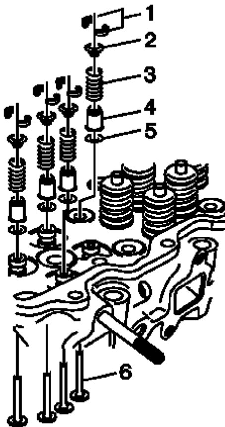
Fig. 100: View Of Valve Stem Oil Seal & Valve Spring Courtesy of GENERAL MOTORS COMPANY
