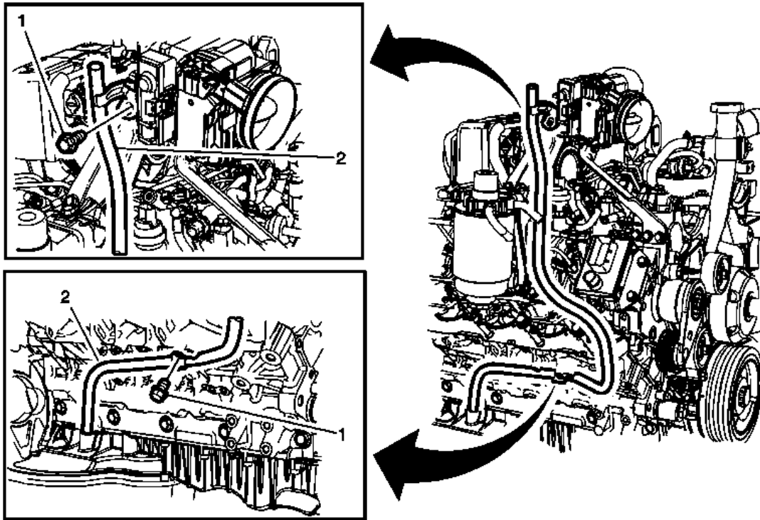
Fig. 47: Oil Level Indicator Tube
