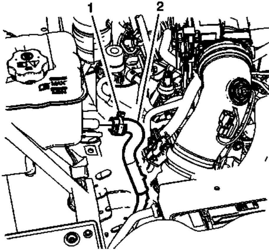
Fig. 242: Radiator Outlet Hose And Clamp Courtesy of GENERAL MOTORS COMPANY
