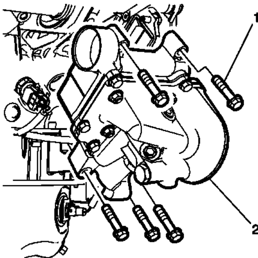
Fig. 205: Oil Cooler And Bolts
