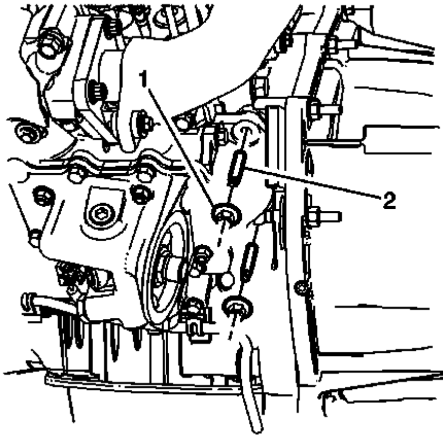
Fig. 214: Oil Cooler Adapter Nuts And Studs Courtesy of GENERAL MOTORS COMPANY
