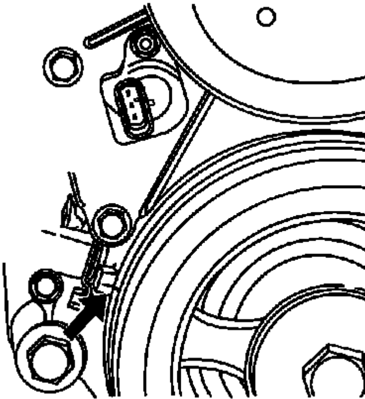
Fig. 64: View Of Crankshaft Balancer Mark Aligned With Engine Mark Courtesy of GENERAL MOTORS COMPANY
