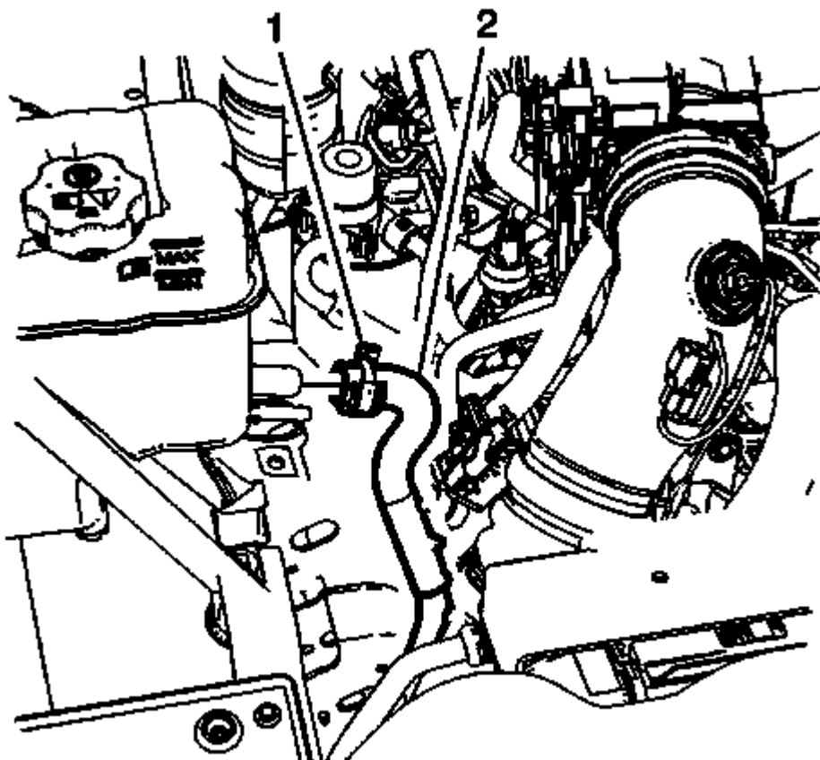
Fig. 224: Radiator Outlet Hose And Clamp Courtesy of GENERAL MOTORS COMPANY
