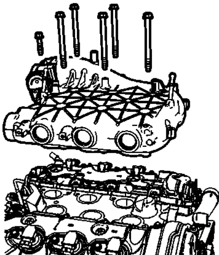
Fig. 20: View Of Intake Manifold & Bolts
