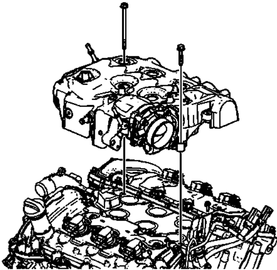
Fig. 60: View Of Intake Manifold & Bolts Courtesy of GENERAL MOTORS COMPANY
