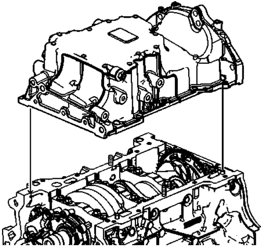
Fig. 205: View Of Oil Pan & Block
