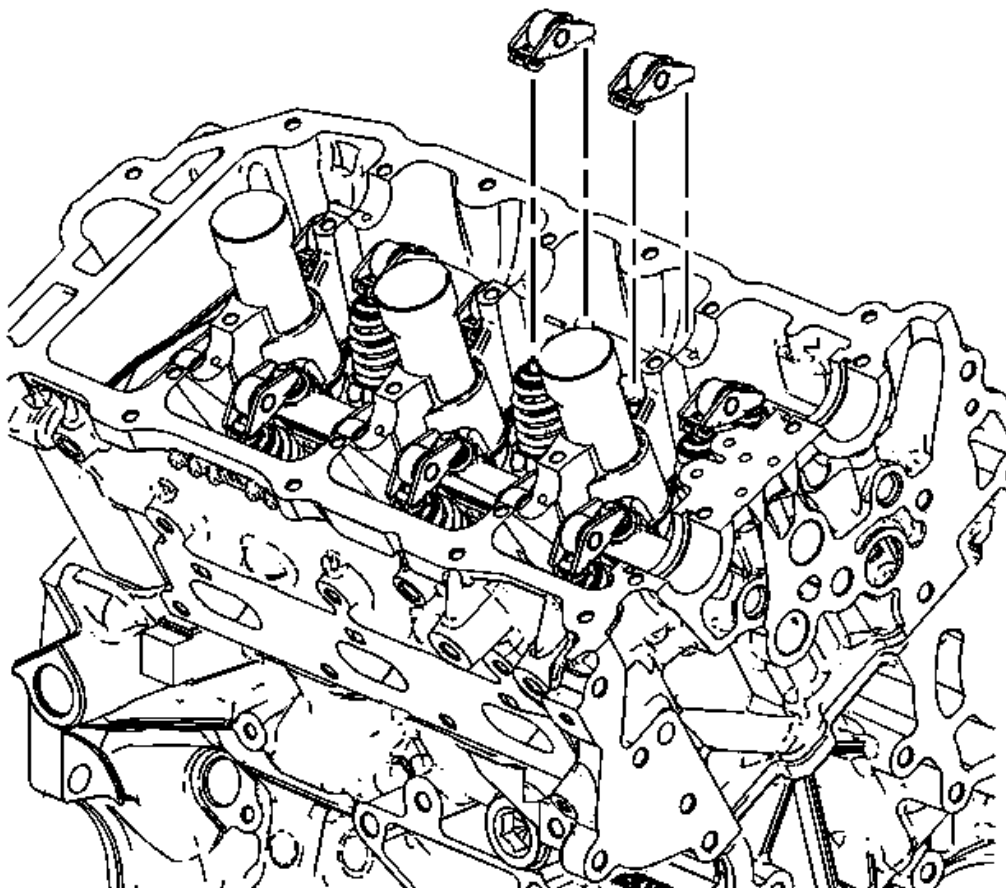
Fig. 163: Identifying Valve Rocker Arms Courtesy of GENERAL MOTORS COMPANY
