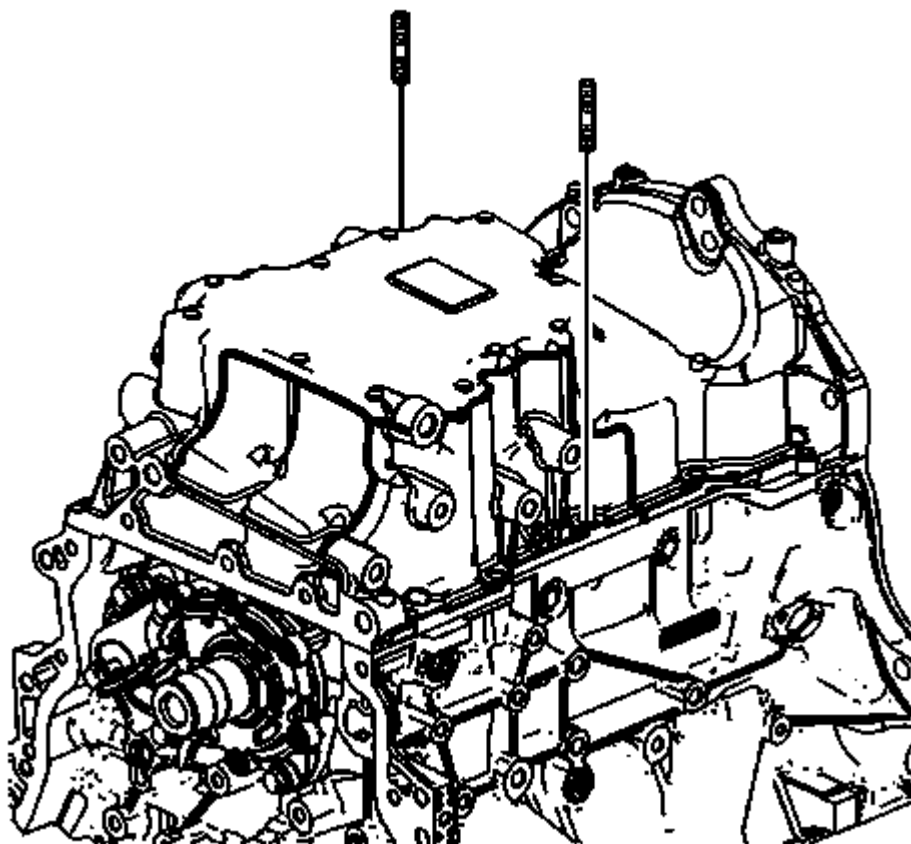
Fig. 209: Identifying Special Tools - EN 46109 Courtesy of GENERAL MOTORS COMPANY
