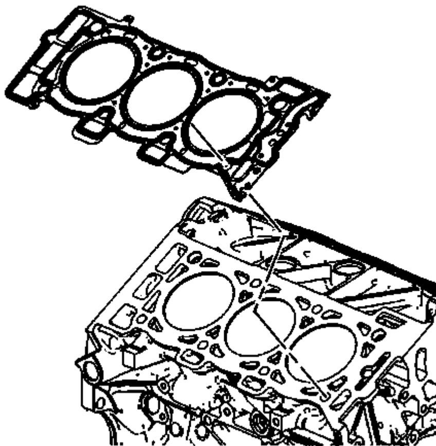
Fig. 195: View Of Right Cylinder Head Gasket Courtesy of GENERAL MOTORS COMPANY
