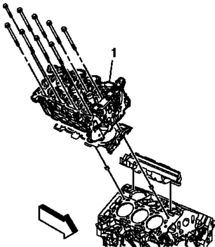
Fig. 210: Cylinder Head And Exhaust Manifold Courtesy of GENERAL MOTORS COMPANY
