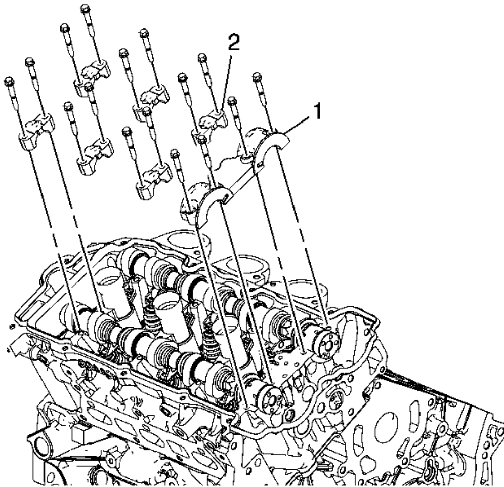
Fig. 175: Camshaft Bearing Caps And Bolts Courtesy of GENERAL MOTORS COMPANY
