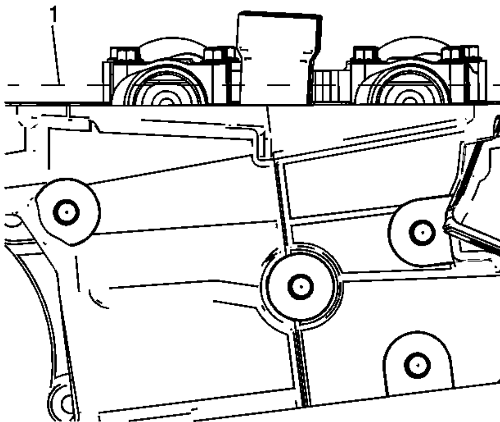
Fig. 145: Camshaft Flats Parallel With Camshaft Cover Rail Courtesy of GENERAL MOTORS COMPANY
