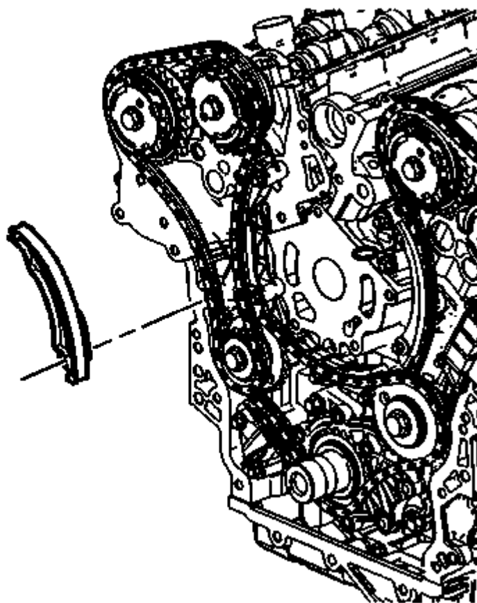
Fig. 94: Right Secondary Camshaft Drive Chain Shoe Courtesy of GENERAL MOTORS COMPANY
