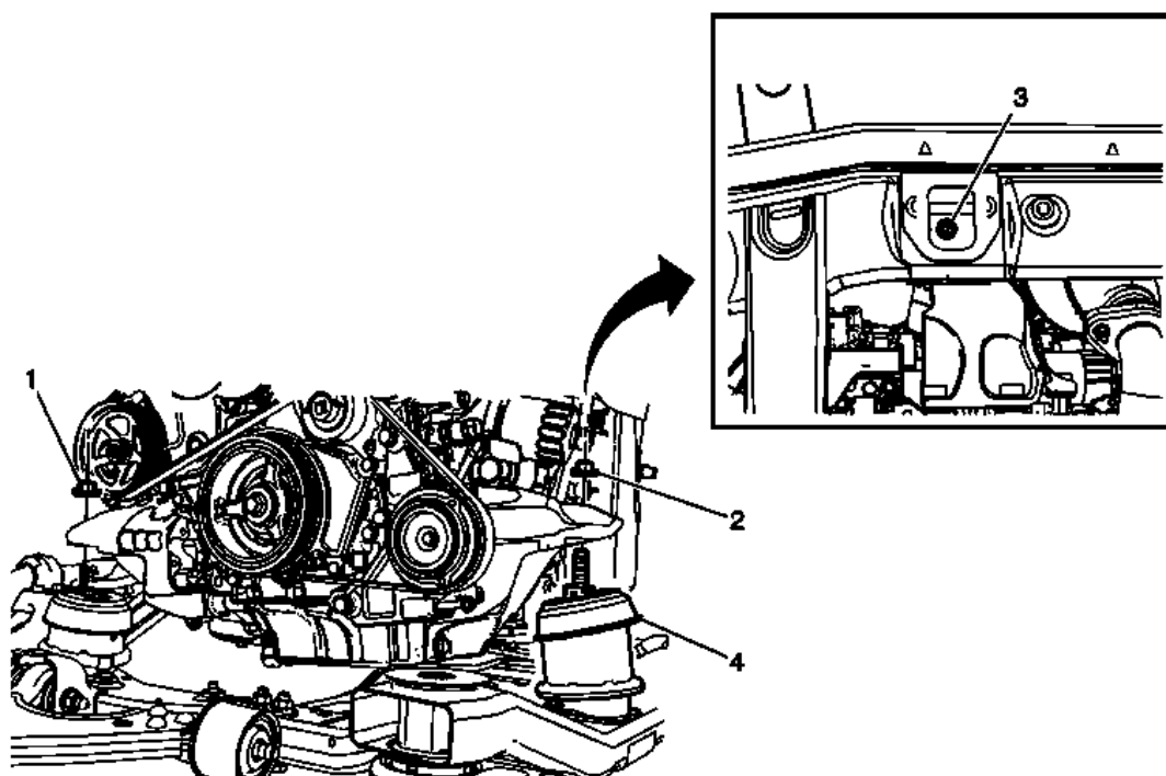
Fig. 5: Engine Front Mount Assembly Courtesy of GENERAL MOTORS COMPANY
