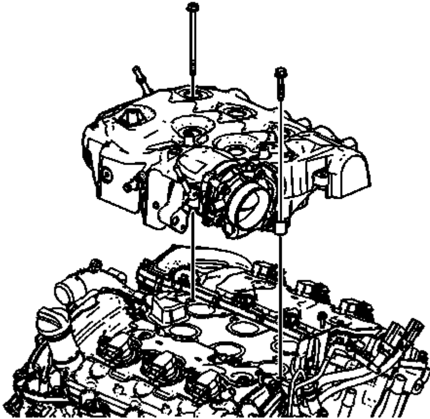
Fig. 79: Intake Manifold And Bolts Courtesy of GENERAL MOTORS COMPANY
