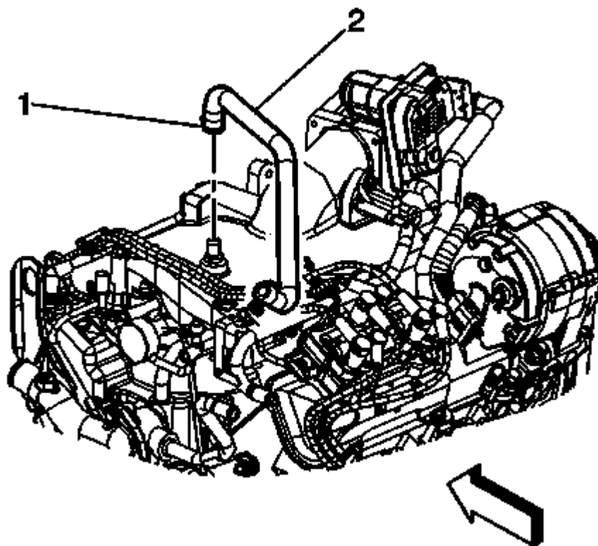
Fig. 277: Brake Booster Vacuum Hose Courtesy of GENERAL MOTORS COMPANY
