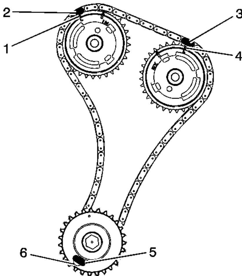
Fig. 146: Left Secondary Camshaft Drive Chain Timing Marks Courtesy of GENERAL MOTORS COMPANY
