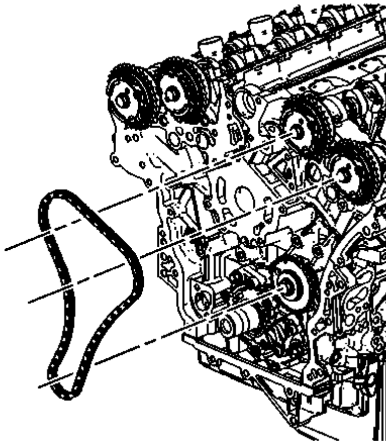
Fig. 81: Left Bank Secondary Camshaft Drive Chain Courtesy of GENERAL MOTORS COMPANY
