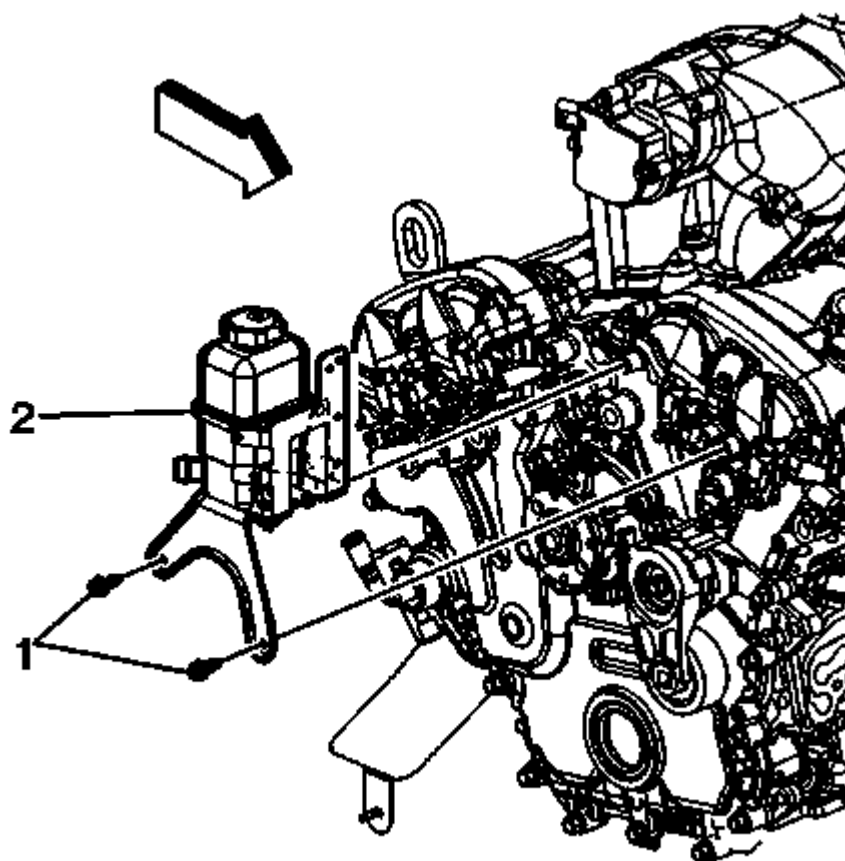
Fig. 78: Power Steering Fluid Reservoir Bracket And Bolts Courtesy of GENERAL MOTORS COMPANY
