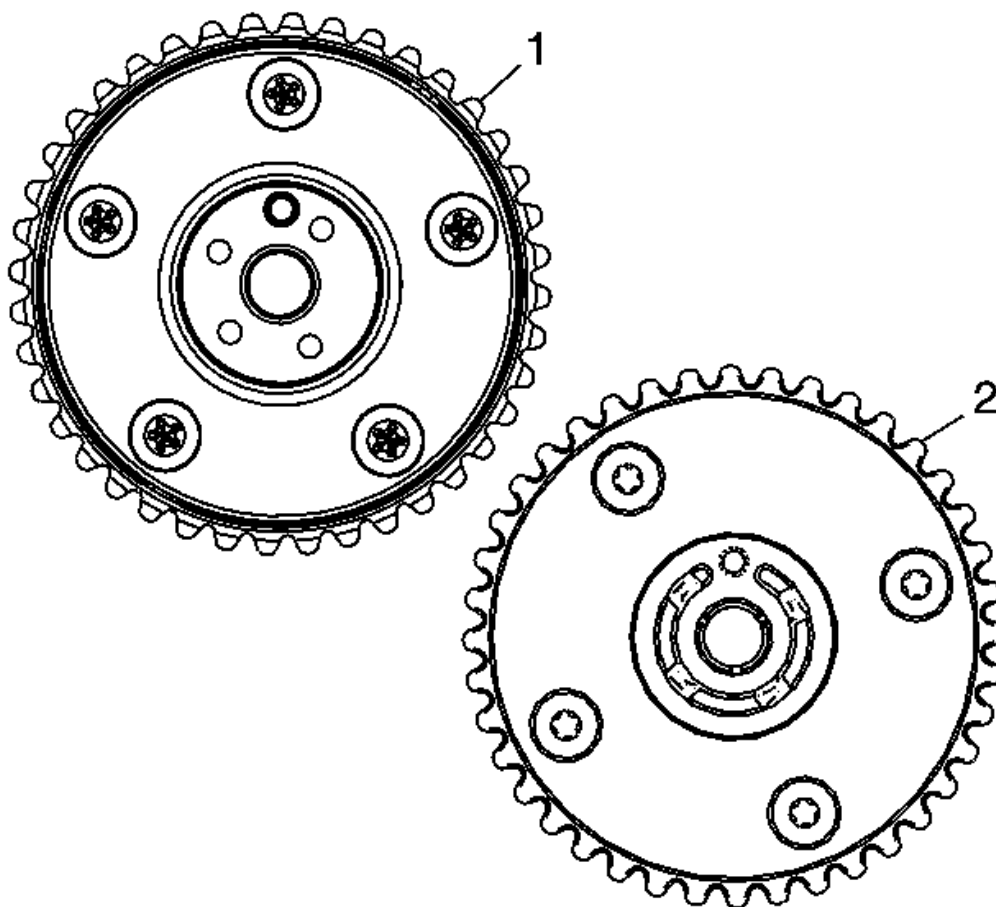
Fig. 153: Camshaft Position Actuators Courtesy of GENERAL MOTORS COMPANY
