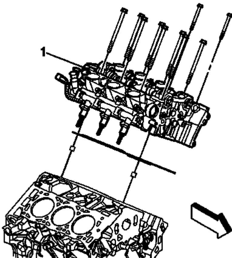
Fig. 203: Cylinder Head And Exhaust Manifold Assembly Courtesy of GENERAL MOTORS COMPANY
