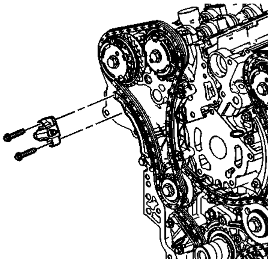
Fig. 87: Right Bank Secondary Camshaft Drive Chain Tensioner Courtesy of GENERAL MOTORS COMPANY
