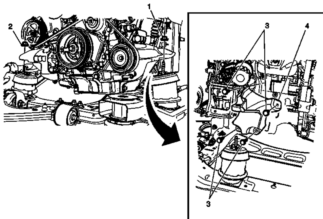
Fig. 7: Engine Front Mount Assembly Courtesy of GENERAL MOTORS COMPANY
