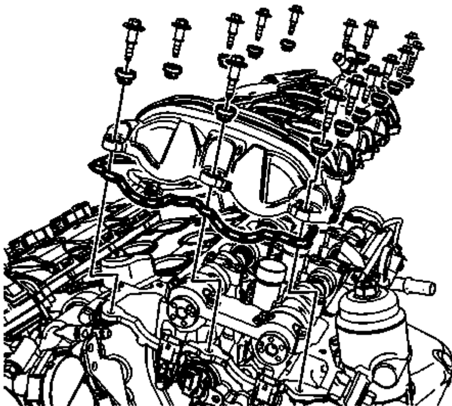
Fig. 44: Camshaft Cover Seal And Grommets Courtesy of GENERAL MOTORS COMPANY
