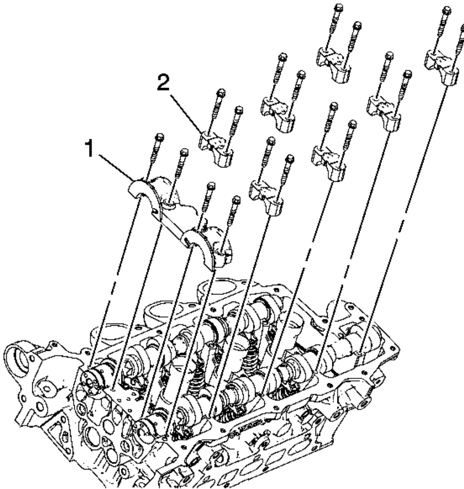
Fig. 164: Camshaft Bearing Caps And Bolts Courtesy of GENERAL MOTORS COMPANY
