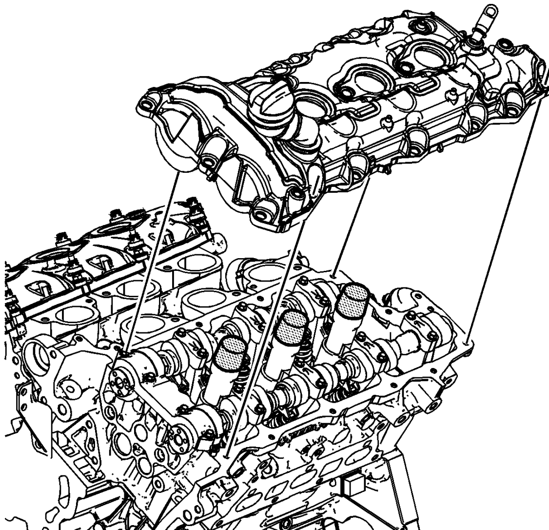
Fig. 48: Camshaft Cover And Cylinder Head Courtesy of GENERAL MOTORS COMPANY
