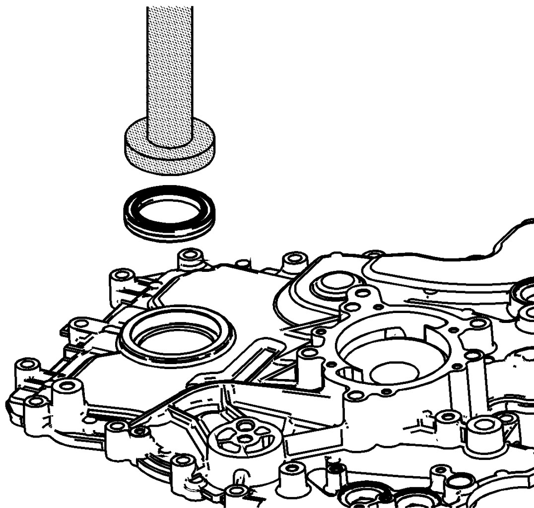
Fig. 43: Crankshaft Front Oil Seal And Installer Courtesy of GENERAL MOTORS COMPANY
