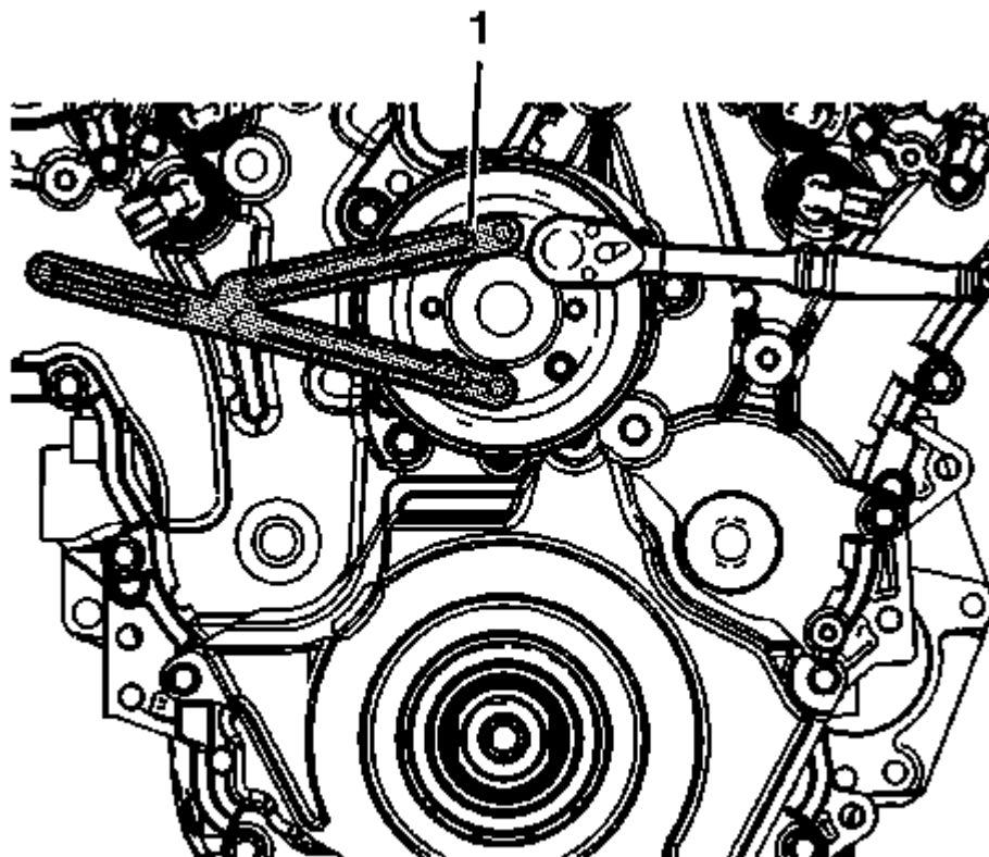
Fig. 74: Water Pump Pulley Holding Tool
