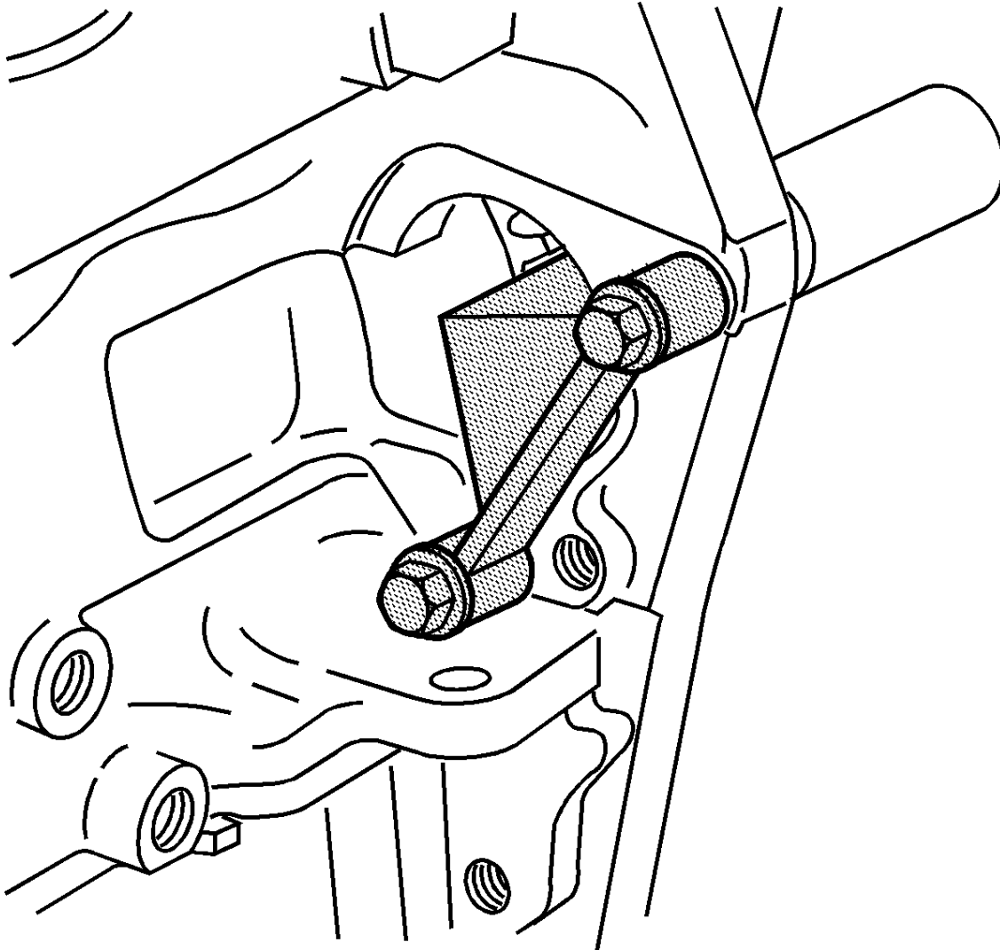
Fig. 34: Engine Flywheel Holding Tool Courtesy of GENERAL MOTORS COMPANY
