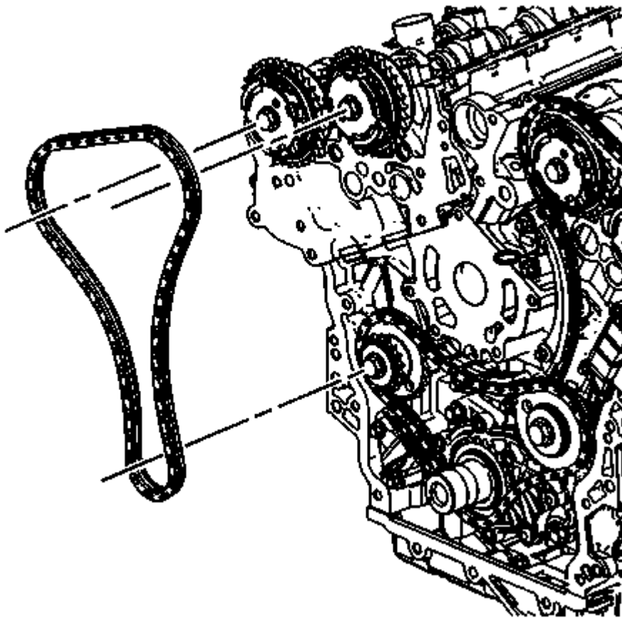
Fig. 82: Right Bank Secondary Camshaft Drive Chain Courtesy of GENERAL MOTORS COMPANY
