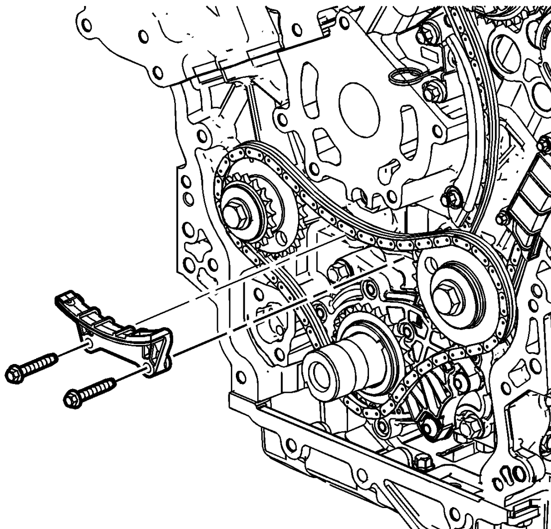
Fig. 115: Upper Primary Camshaft Drive Chain Guide Courtesy of GENERAL MOTORS COMPANY
