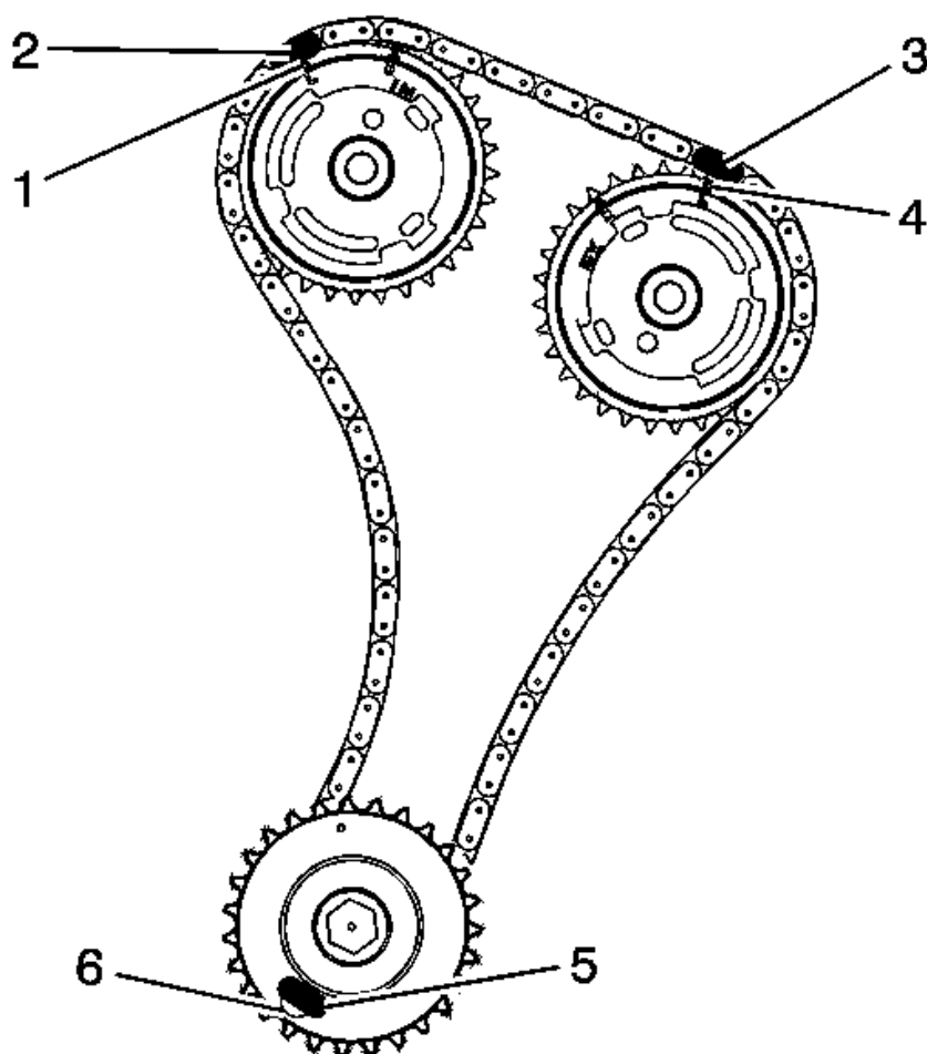
Fig. 152: Left Secondary Camshaft Drive Chain Timing Marks Courtesy of GENERAL MOTORS COMPANY
