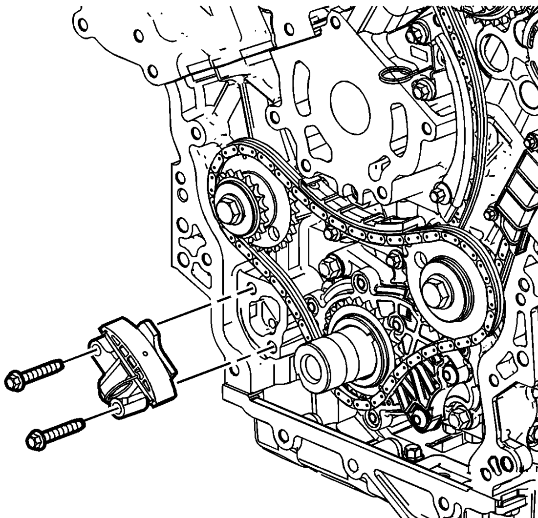
Fig. 111: Primary Camshaft Drive Chain Tensioner Courtesy of GENERAL MOTORS COMPANY
