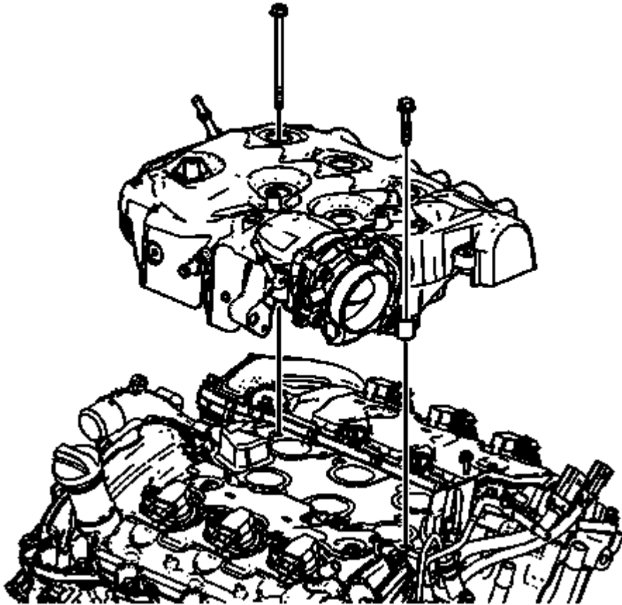
Fig. 60: Intake Manifold And Bolts Courtesy of GENERAL MOTORS COMPANY
