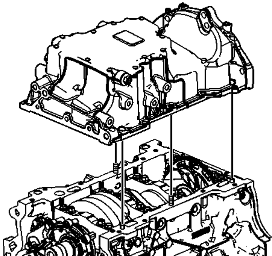
Fig. 222: Engine Oil Pan
