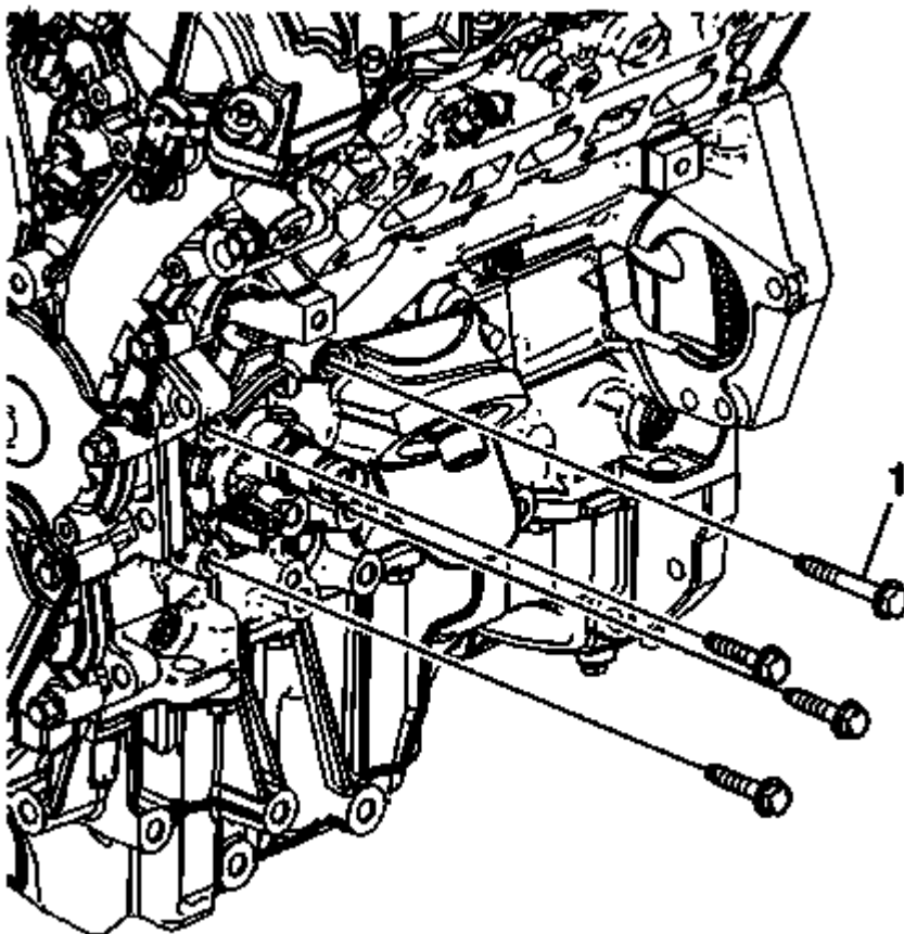
Fig. 33: Correct Position Of Longer Bolt Courtesy of GENERAL MOTORS COMPANY
