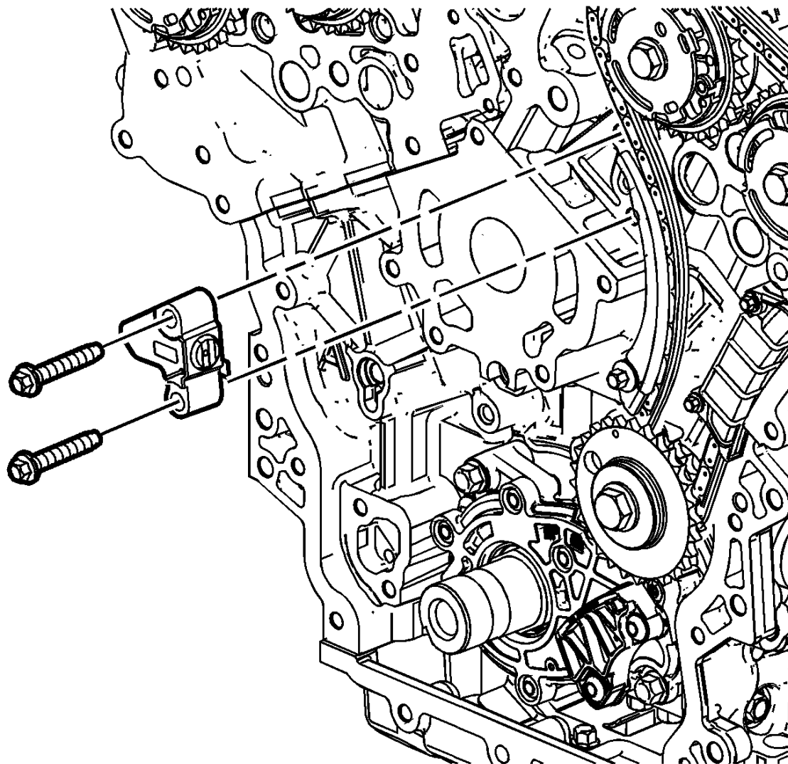
Fig. 85: Left Bank Secondary Camshaft Drive Chain Tensioner Courtesy of GENERAL MOTORS COMPANY
