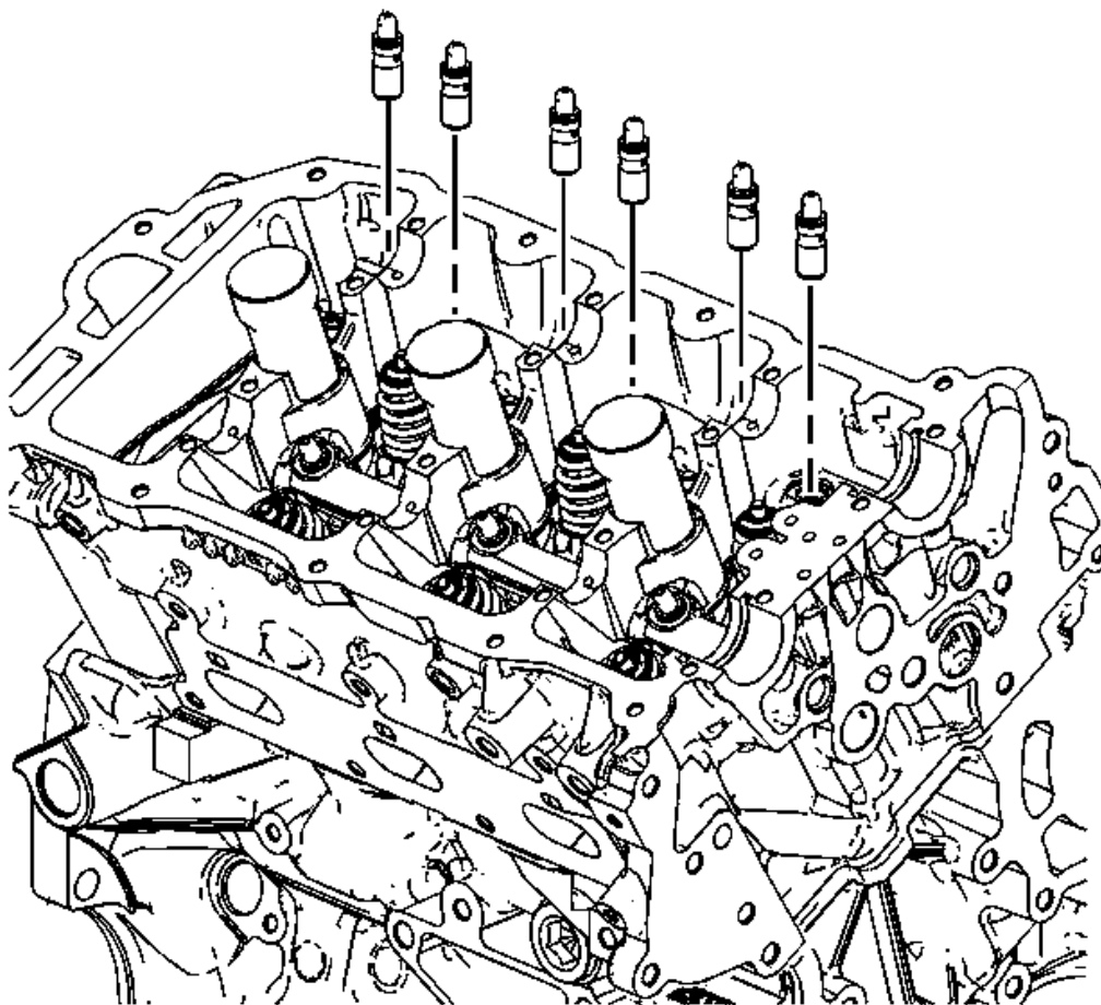
Fig. 182: Stationary Hydraulic Lash Adjuster (SHLA) Courtesy of GENERAL MOTORS COMPANY
