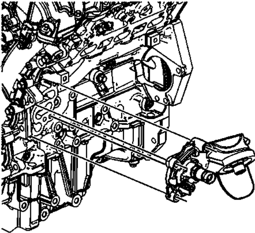
Fig. 29: Oil Filter Adapter
