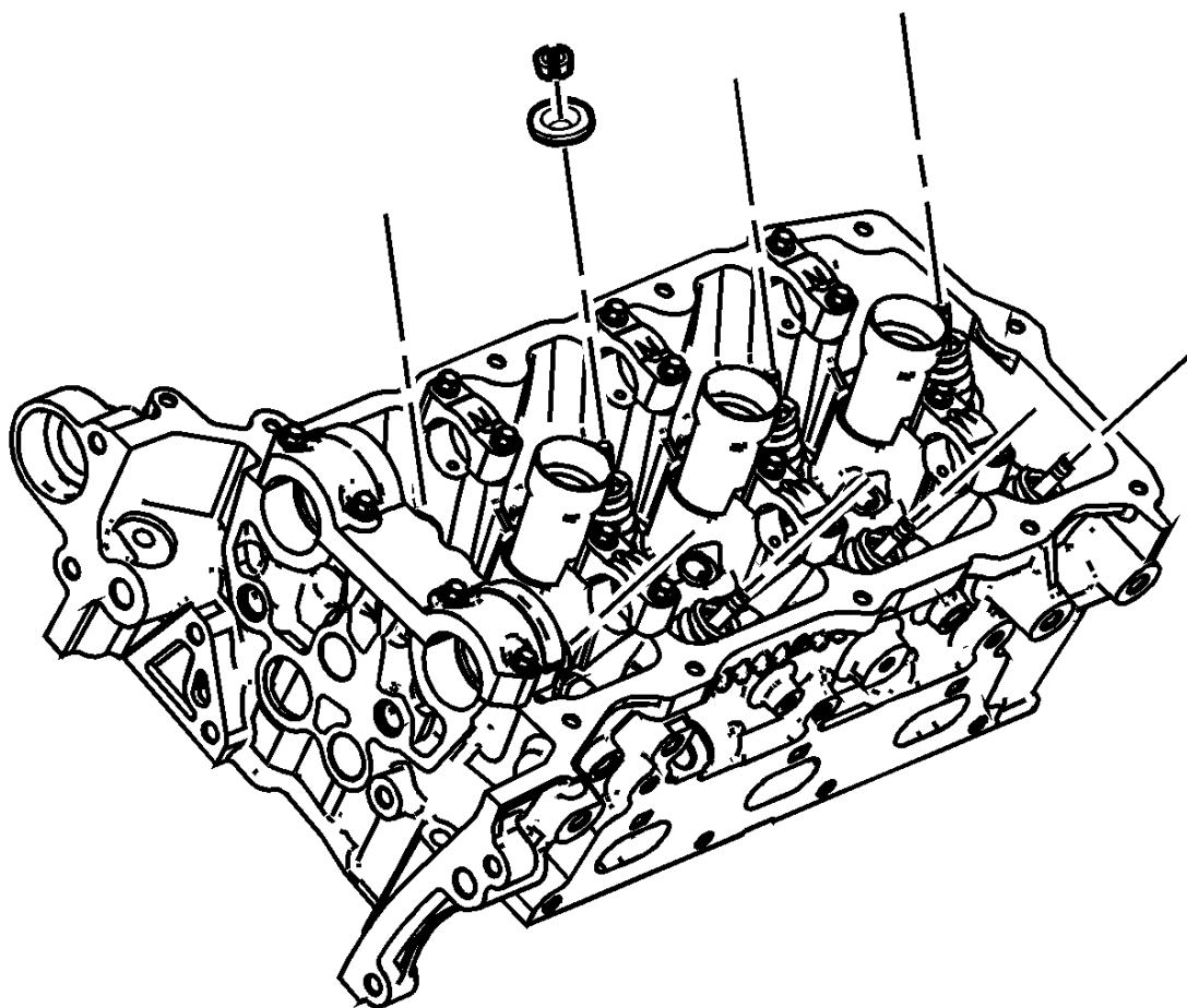
Fig. 193: Valve Spring Keepers And Valve Spring Retainers Courtesy of GENERAL MOTORS COMPANY
