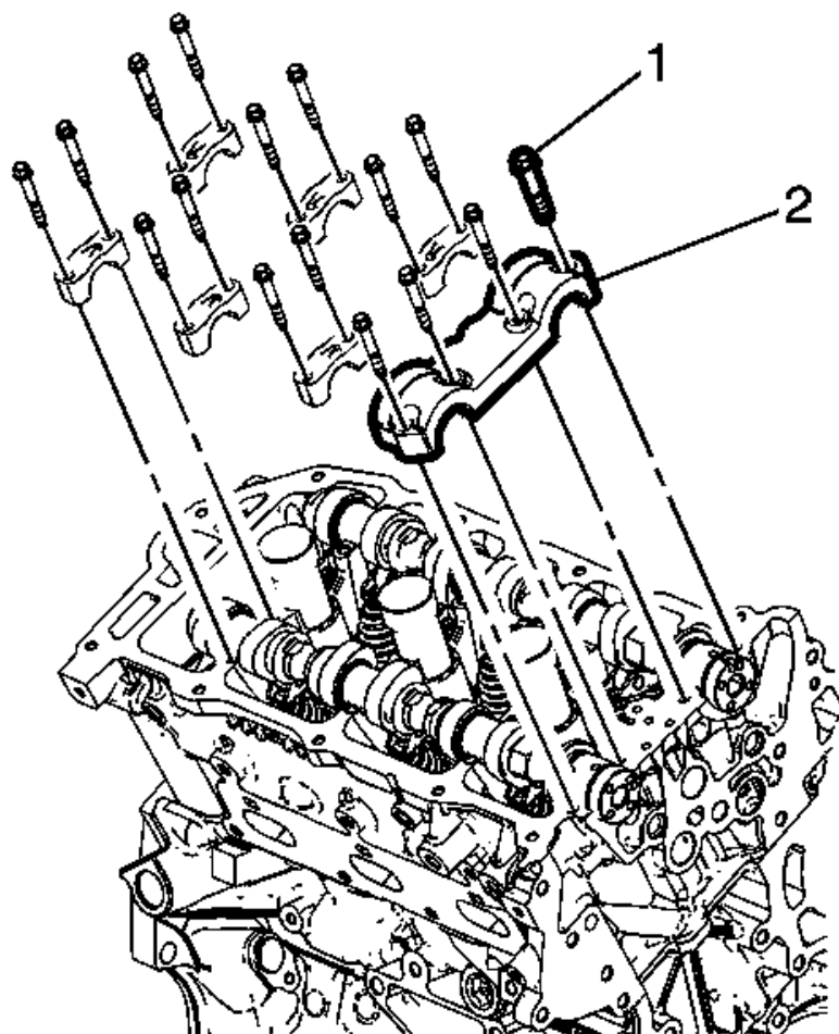
Fig. 167: Camshaft Bearing Caps And Bolts Courtesy of GENERAL MOTORS COMPANY
