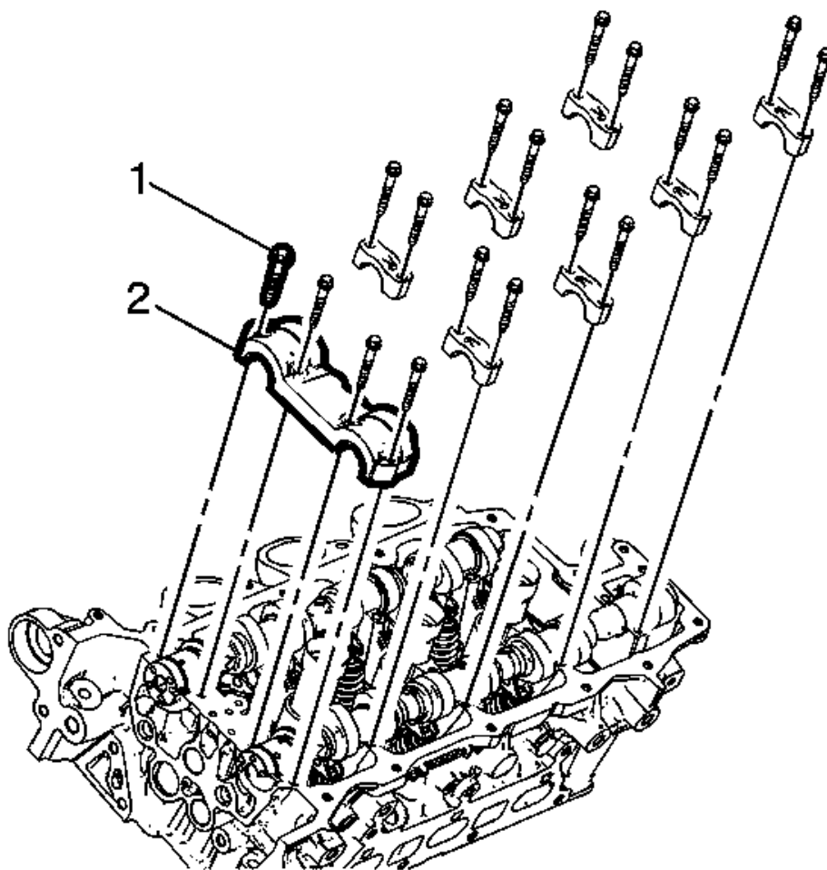
Fig. 156: Bearing Cap Bolts
