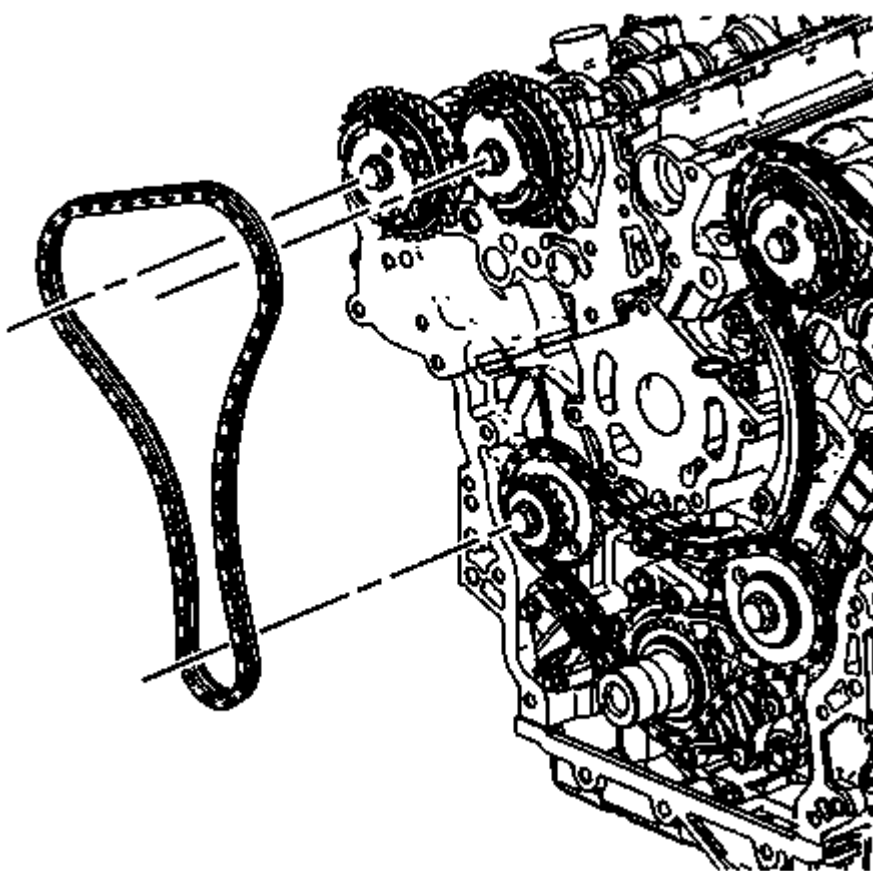
Fig. 83: Right Bank Secondary Camshaft Drive Chain Courtesy of GENERAL MOTORS COMPANY
