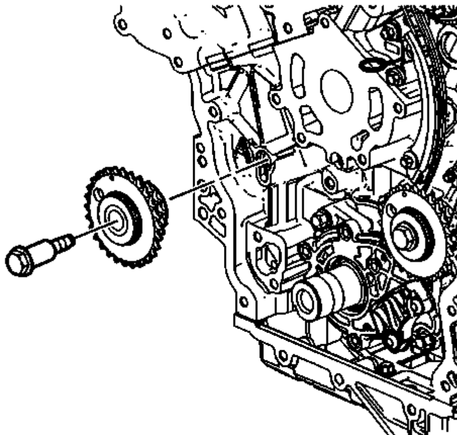
Fig. 107: Left Bank Camshaft Intermediate Drive Chain Idler Courtesy of GENERAL MOTORS COMPANY
