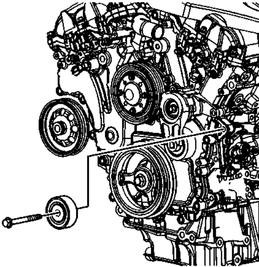
Fig. 73: Drive Belt Idler Pulley Bolt Courtesy of GENERAL MOTORS COMPANY
