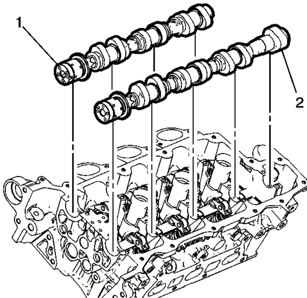
Fig. 160: Camshaft Intake And Exhaust Positioning Points Courtesy of GENERAL MOTORS COMPANY
