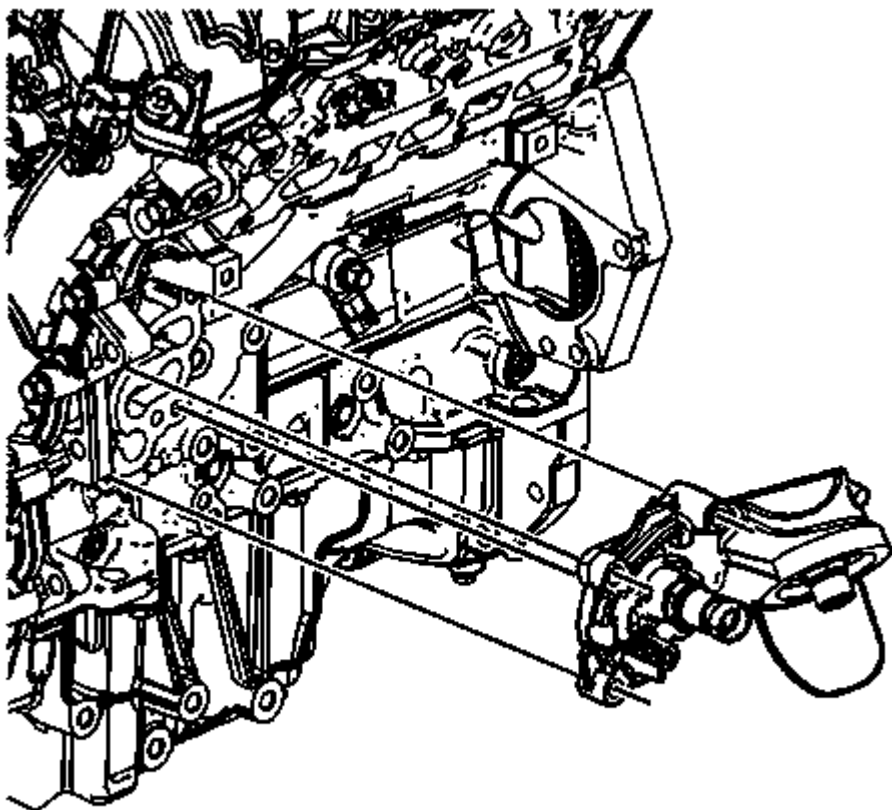
Fig. 32: Oil Filter Adapter
