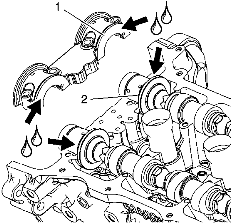
Fig. 174: Camshaft Bearing Cap And Camshaft Thrust Surface Courtesy of GENERAL MOTORS COMPANY
