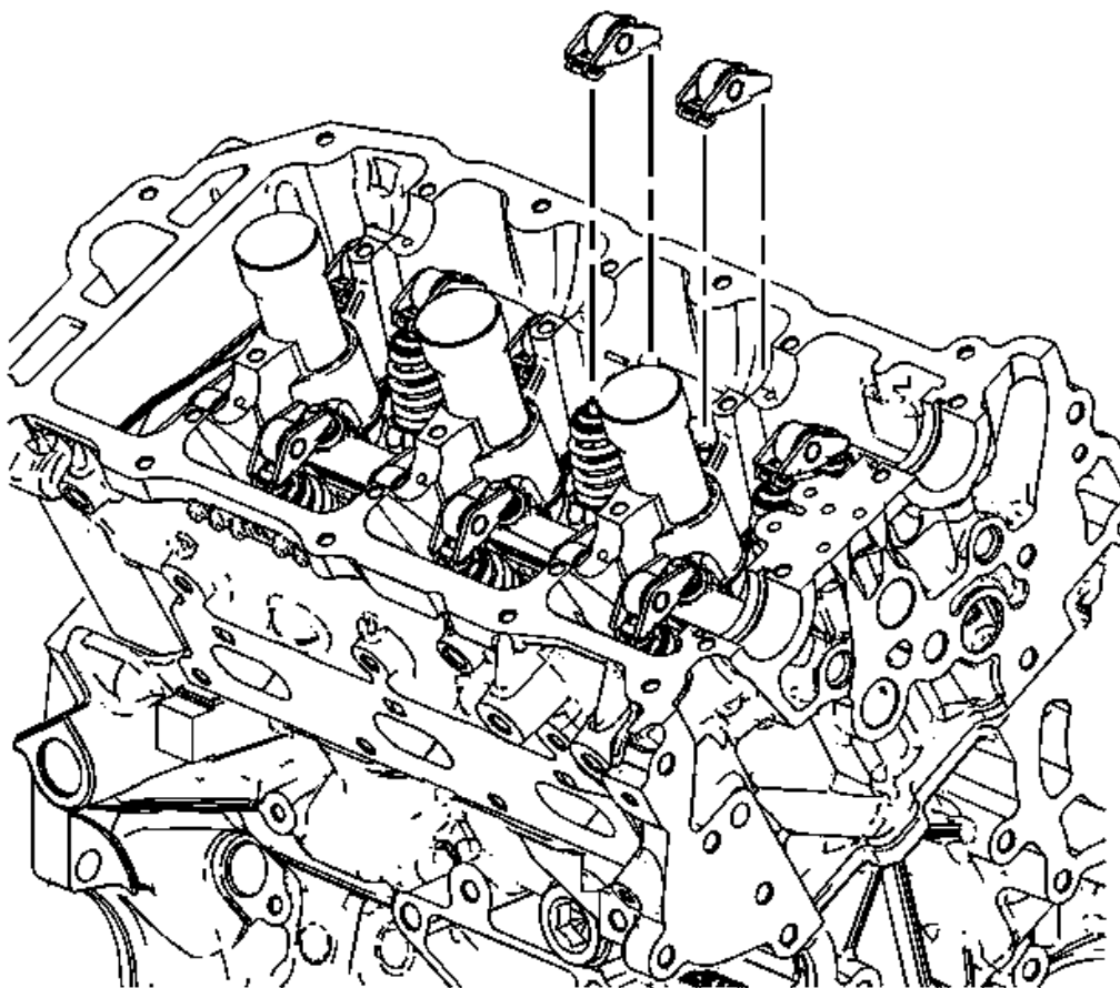
Fig. 178: Valve Rocker Arms
