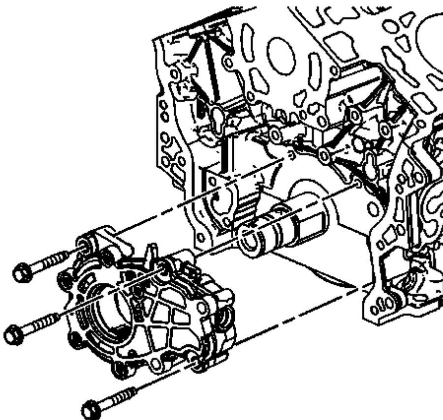
Fig. 216: Oil Pump And Bolts
