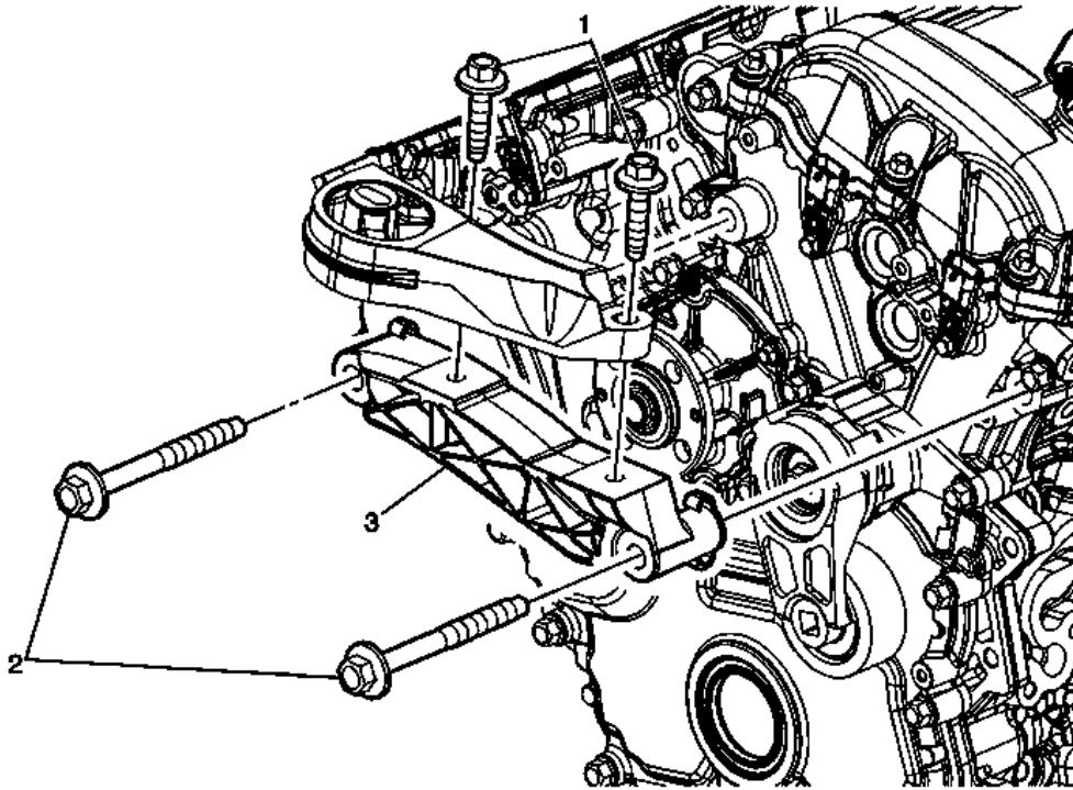
Fig. 11: Right Side Engine Mount Strut Bracket Courtesy of GENERAL MOTORS COMPANY
