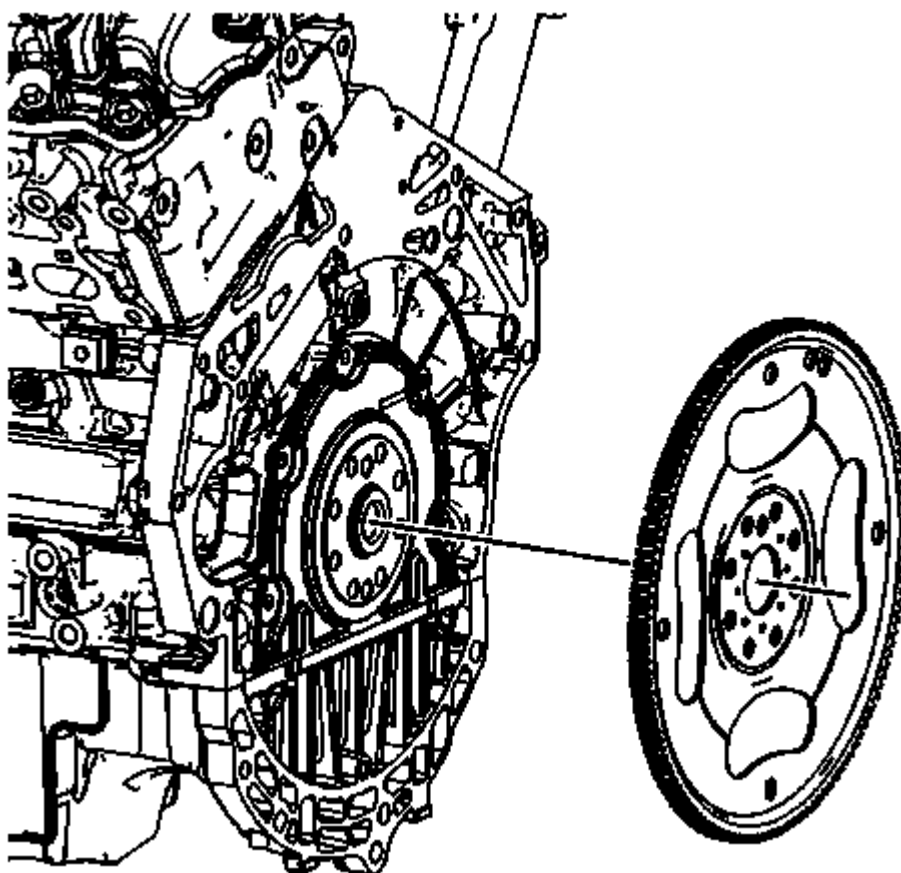
Fig. 211: Engine Flywheel
