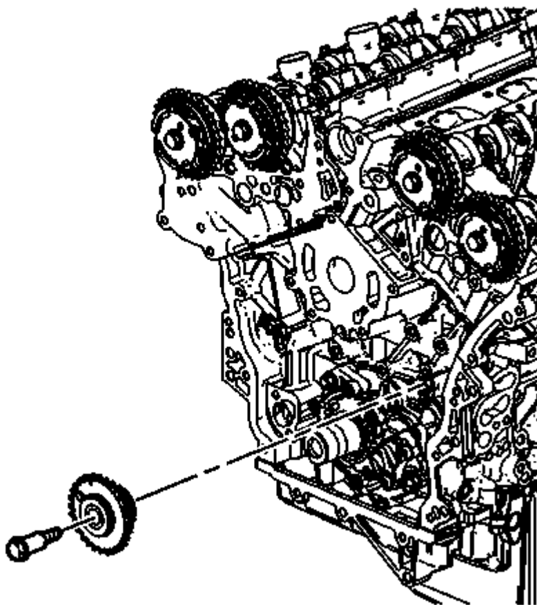
Fig. 108: Left Timing Chain Idler Sprocket Courtesy of GENERAL MOTORS COMPANY
