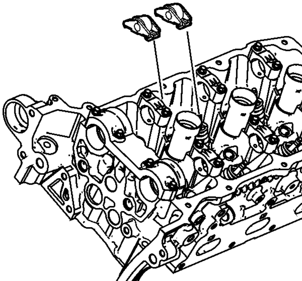
Fig. 180: Valve Rocker Arm
