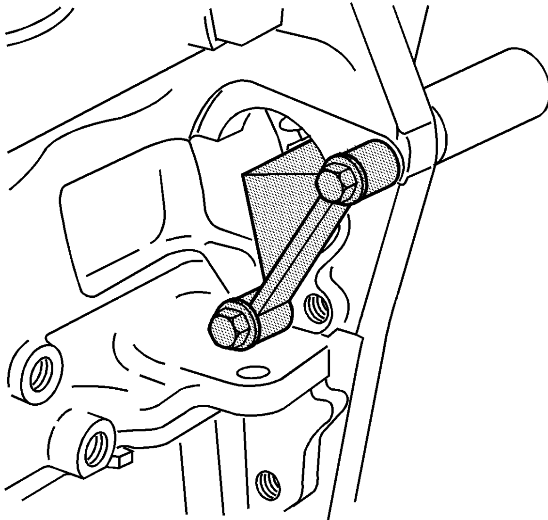
Fig. 185: Engine Flywheel Holding Tool Courtesy of GENERAL MOTORS COMPANY
