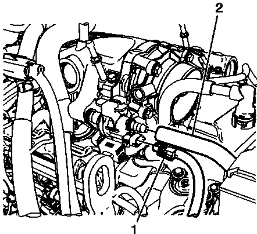
Fig. 25: Purge Solenoid Valve Electrical Connector Courtesy of GENERAL MOTORS COMPANY
