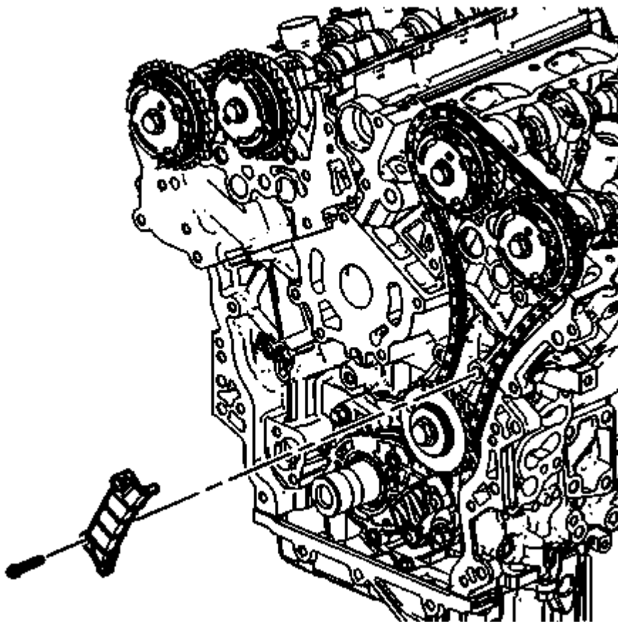
Fig. 96: Left Bank Secondary Camshaft Drive Chain Guide Courtesy of GENERAL MOTORS COMPANY
