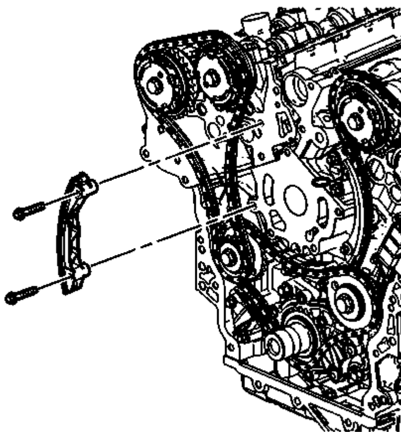
Fig. 97: Right Secondary Camshaft Drive Chain Guide And Bolts Courtesy of GENERAL MOTORS COMPANY
