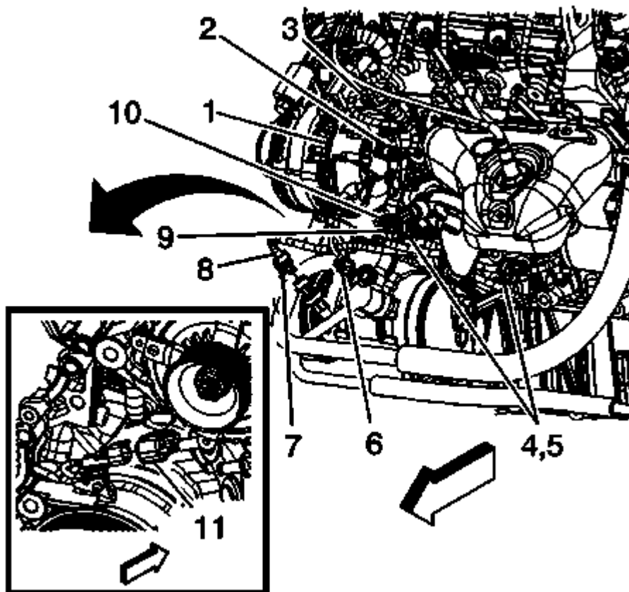
Fig. 262: Generator, A/C Compressor, Oil Pressure Switch And Retainer Clips Courtesy of GENERAL MOTORS COMPANY
