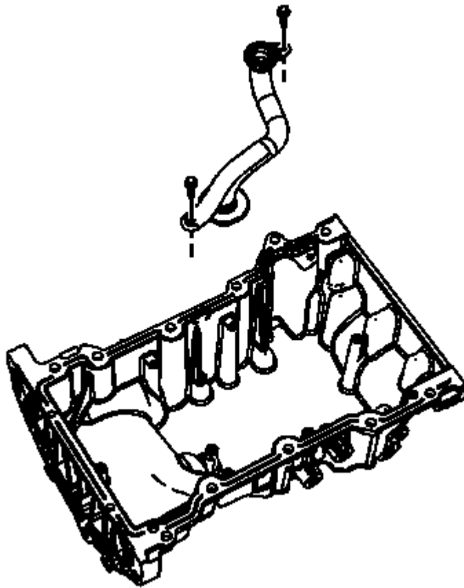
Fig. 229: Oil Suction Pipe And Bolts Courtesy of GENERAL MOTORS COMPANY
