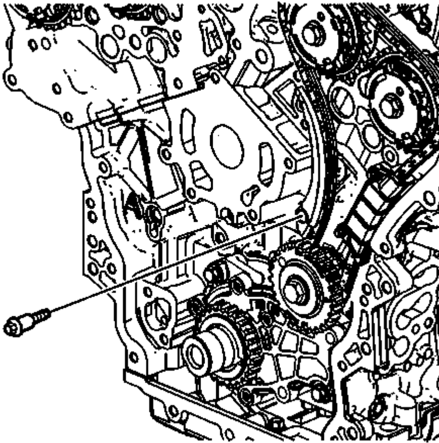
Fig. 92: Secondary Camshaft Drive Chain Shoe Bolt Courtesy of GENERAL MOTORS COMPANY
