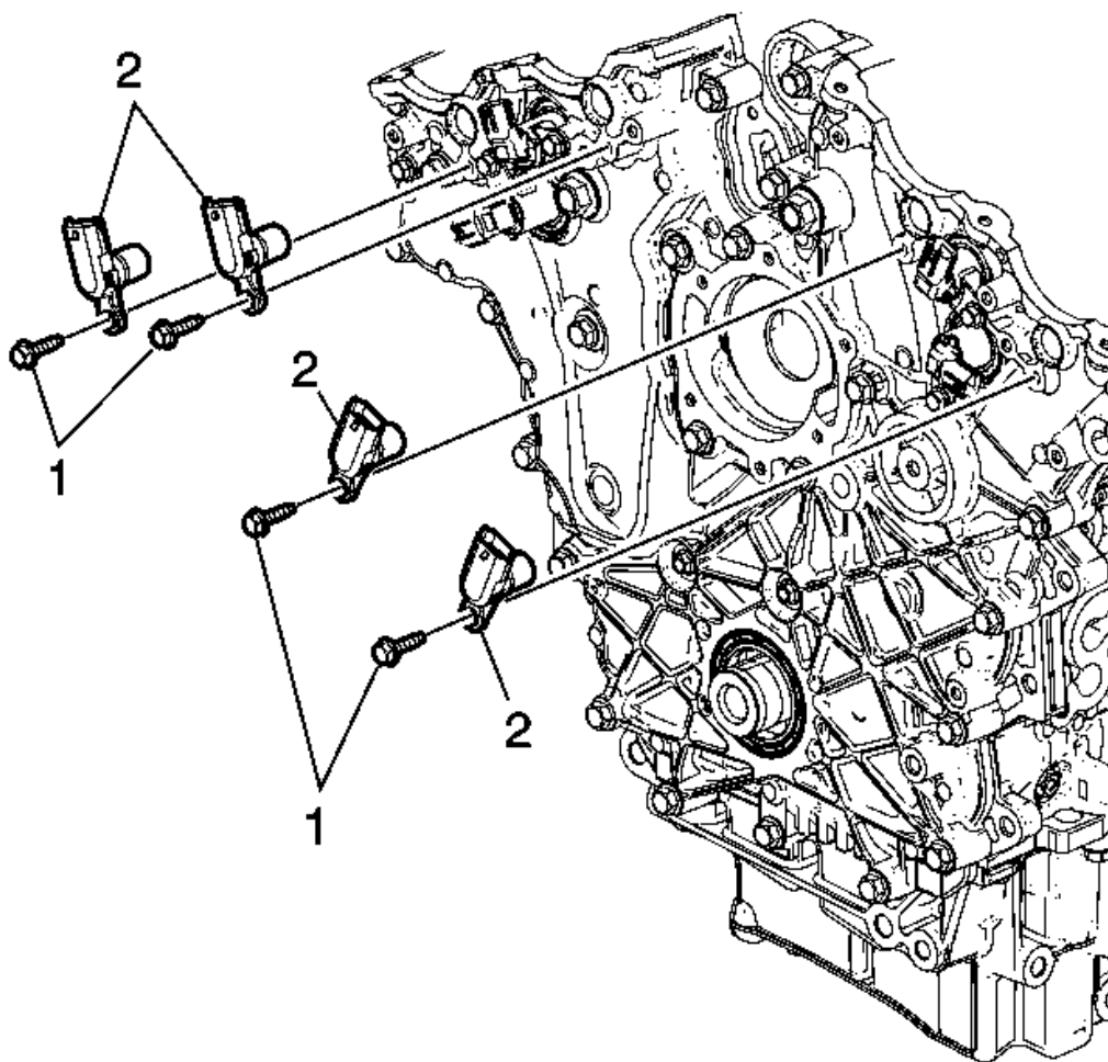
Fig. 67: Camshaft Position Sensors And Bolts Courtesy of GENERAL MOTORS COMPANY
