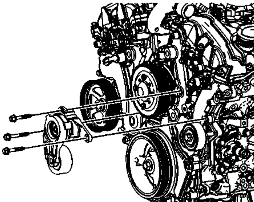
Fig. 75: Drive Belt Tensioner
