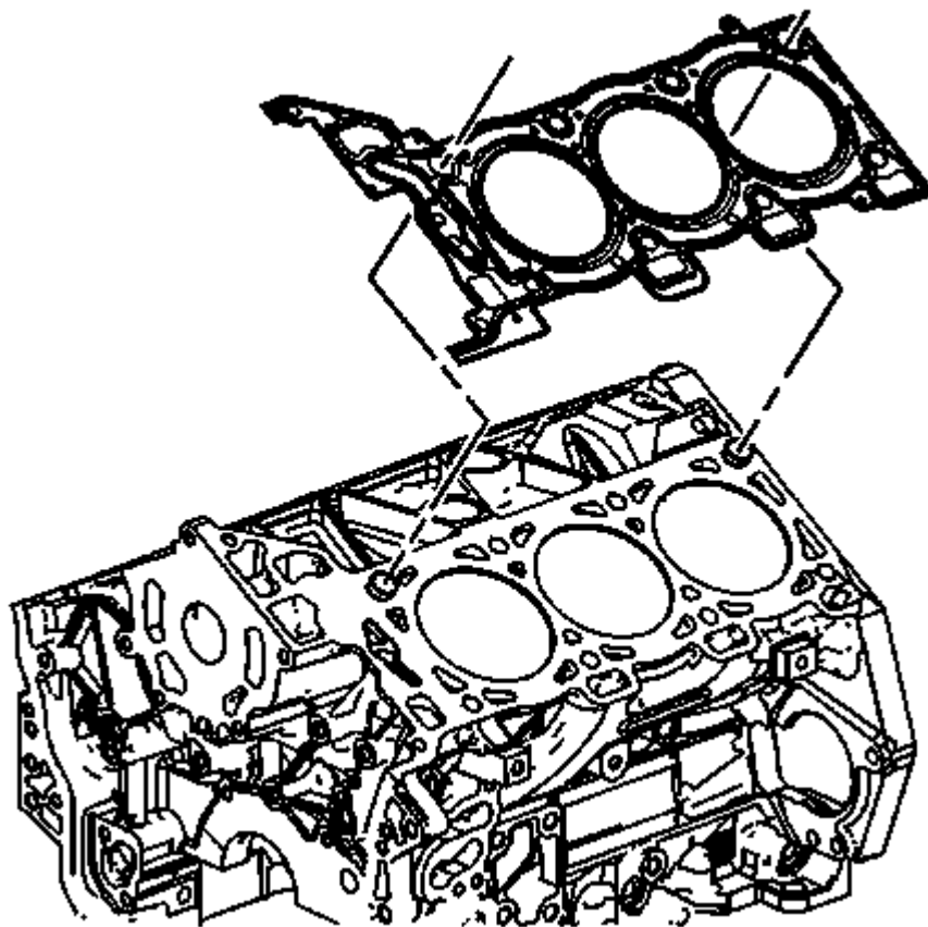
Fig. 204: Left Cylinder Head Gasket
