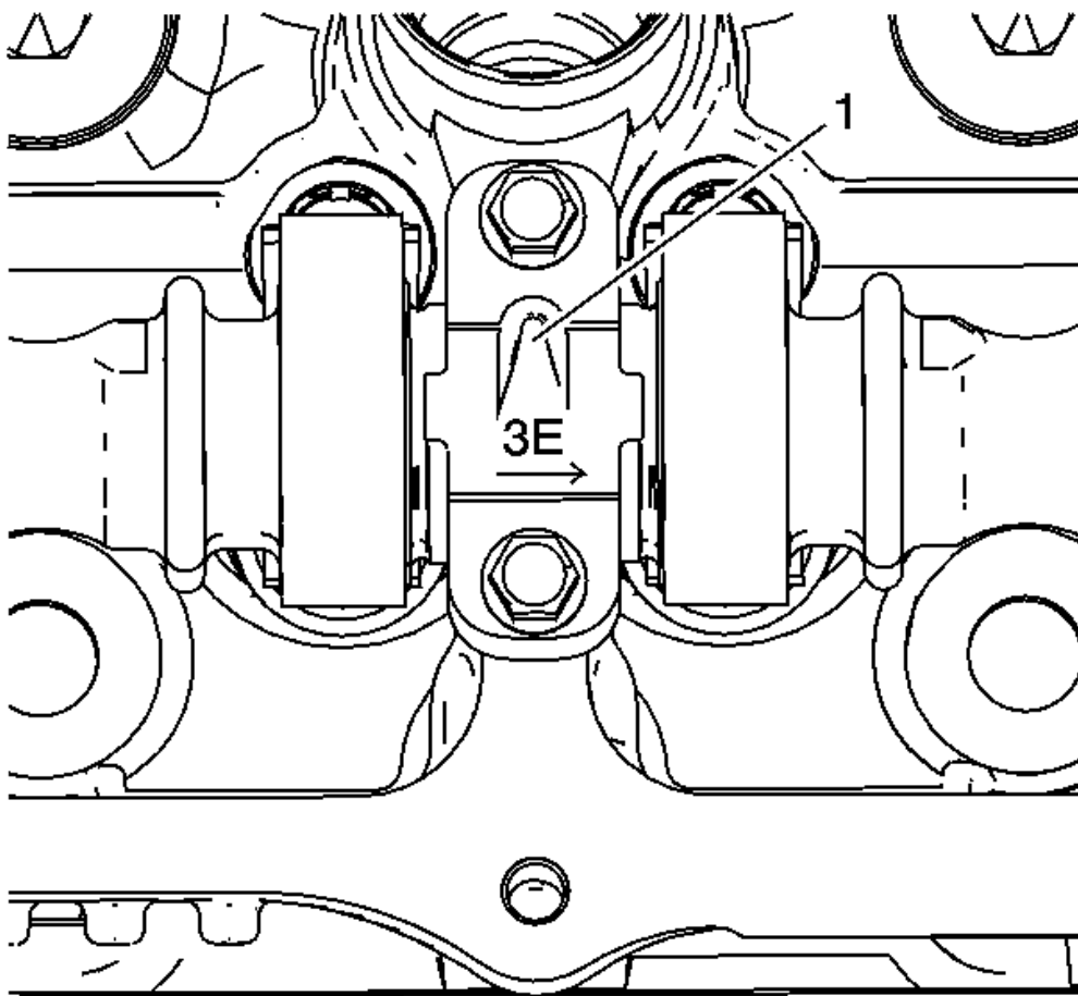
Fig. 173: Right Cylinder Head Camshaft Bearing Cap Markings Courtesy of GENERAL MOTORS COMPANY
