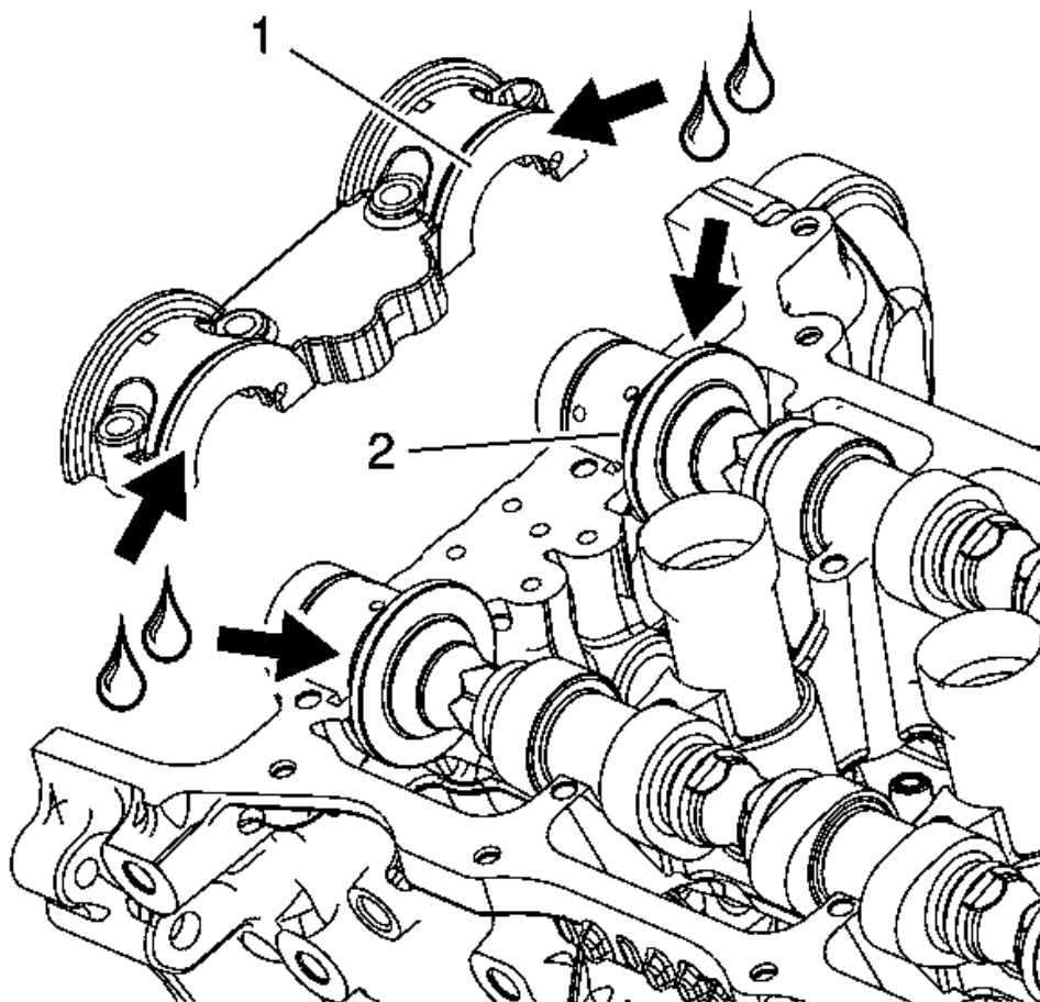
Fig. 163: Camshaft Bearing Cap And Camshaft Thrust Surface Courtesy of GENERAL MOTORS COMPANY
