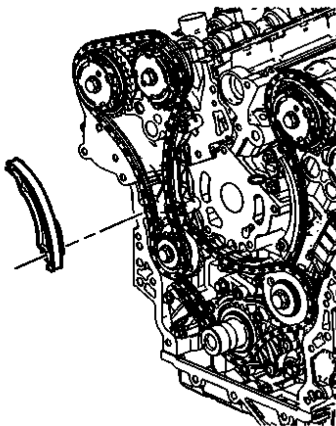
Fig. 93: Right Secondary Camshaft Drive Chain Shoe Courtesy of GENERAL MOTORS COMPANY
