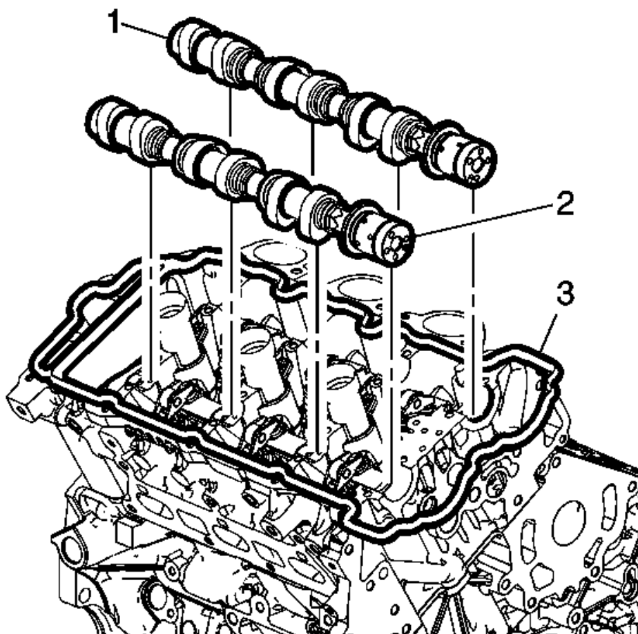
Fig. 171: Right Cylinder Head Camshaft Intake And Exhaust Positioning Points Courtesy of GENERAL MOTORS COMPANY
