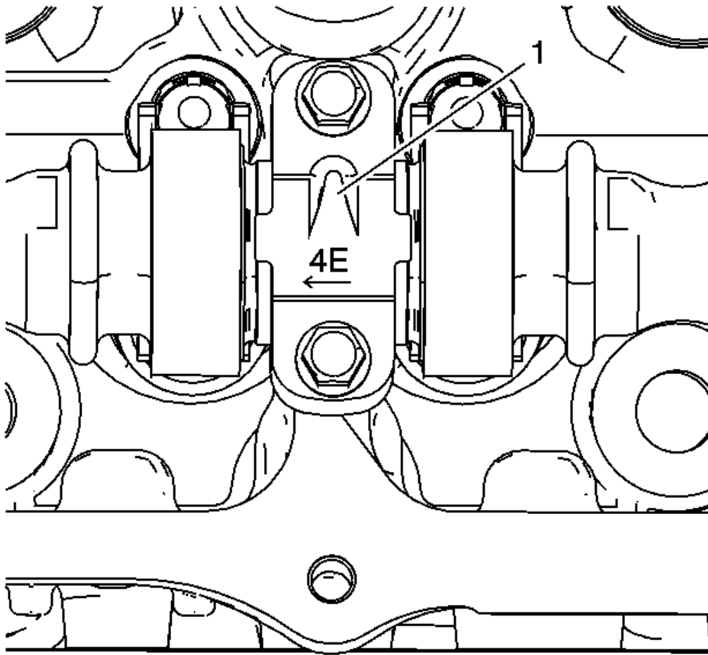
Fig. 162: Left Cylinder Head Camshaft Bearing Cap Markings Courtesy of GENERAL MOTORS COMPANY
