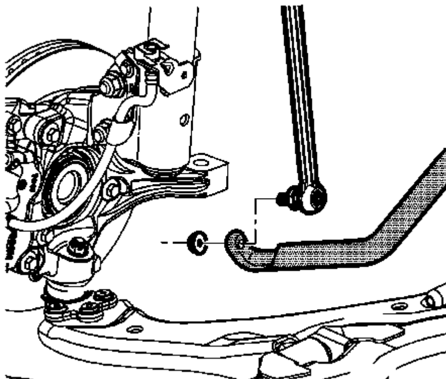
Fig. 270: Stabilizer Shaft And Link
