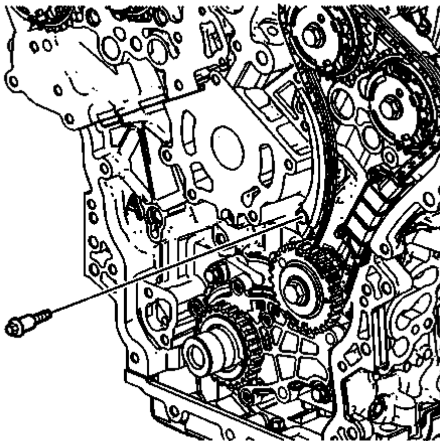
Fig. 88: Secondary Camshaft Drive Chain Shoe Bolt Courtesy of GENERAL MOTORS COMPANY
