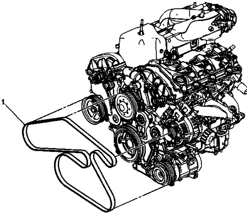
Fig. 1: Drive Belt Routing
