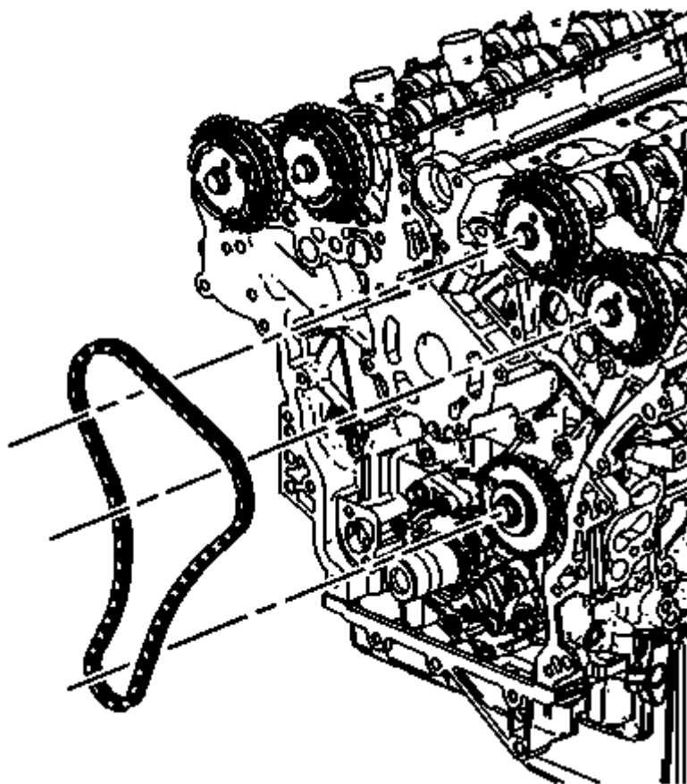
Fig. 80: Left Bank Secondary Camshaft Drive Chain Courtesy of GENERAL MOTORS COMPANY
