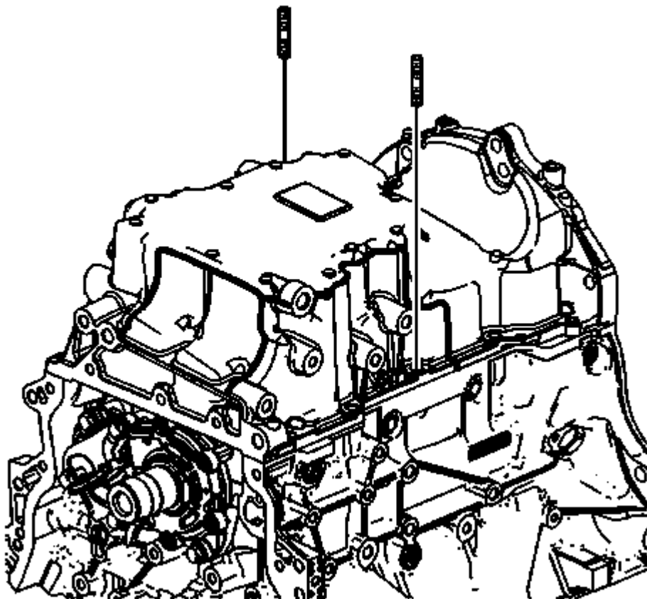
Fig. 223: Engine Block Guide Pins
