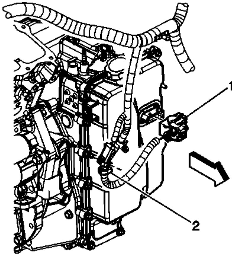
Fig. 261: Wire Harness Retainer And TCM Electrical Connector Courtesy of GENERAL MOTORS COMPANY
