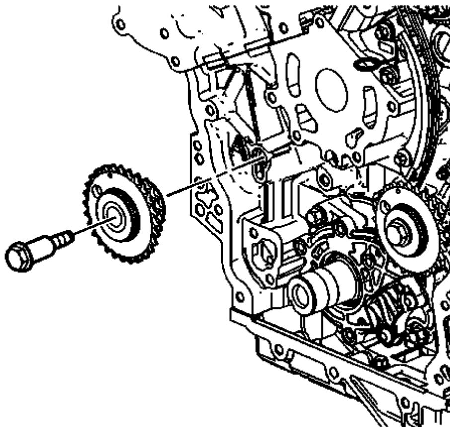
Fig. 106: Left Bank Camshaft Intermediate Drive Chain Idler Courtesy of GENERAL MOTORS COMPANY
