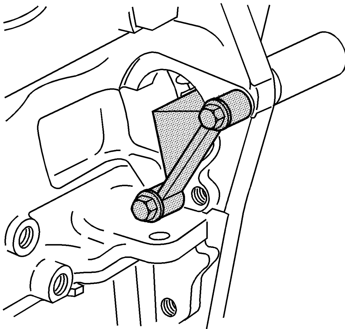
Fig. 194: Engine Flywheel Holding Tool Courtesy of GENERAL MOTORS COMPANY
