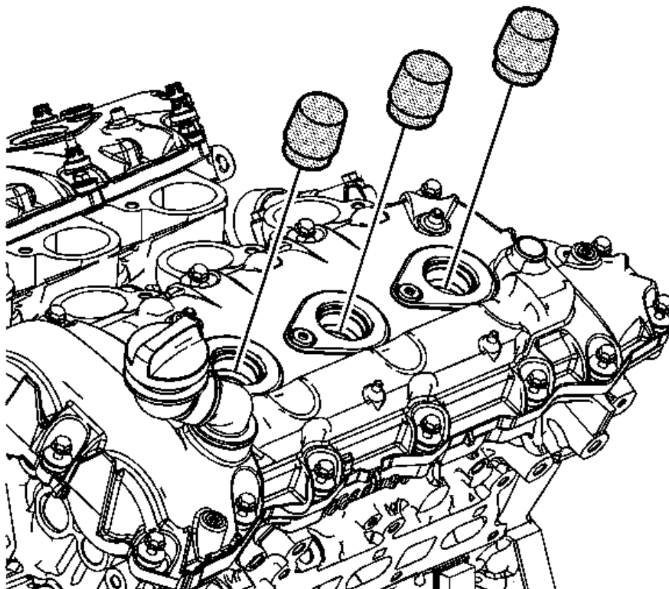
Fig. 51: Spark Plug Tubes And Cylinder Head Courtesy of GENERAL MOTORS COMPANY
