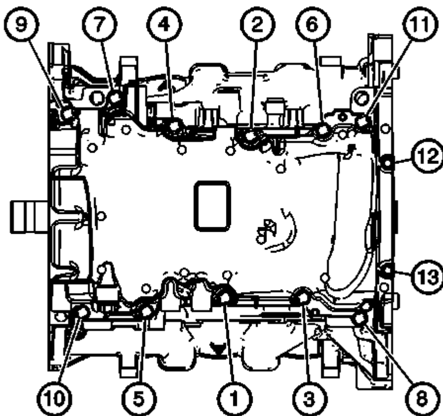
Fig. 225: Oil Pan Bolts - Tightening Sequence Courtesy of GENERAL MOTORS COMPANY
