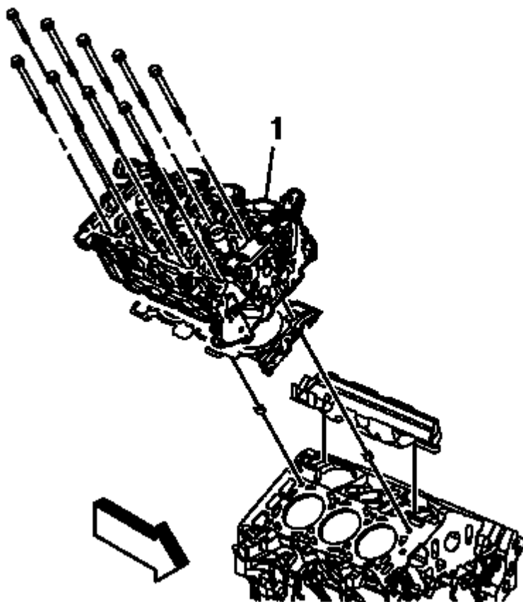
Fig. 207: Cylinder Head And Exhaust Manifold Courtesy of GENERAL MOTORS COMPANY
