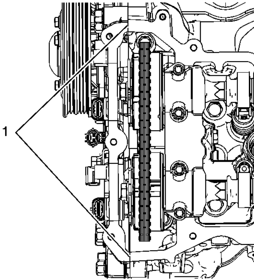
Fig. 47: Engine Front Cover Split Lines Courtesy of GENERAL MOTORS COMPANY
