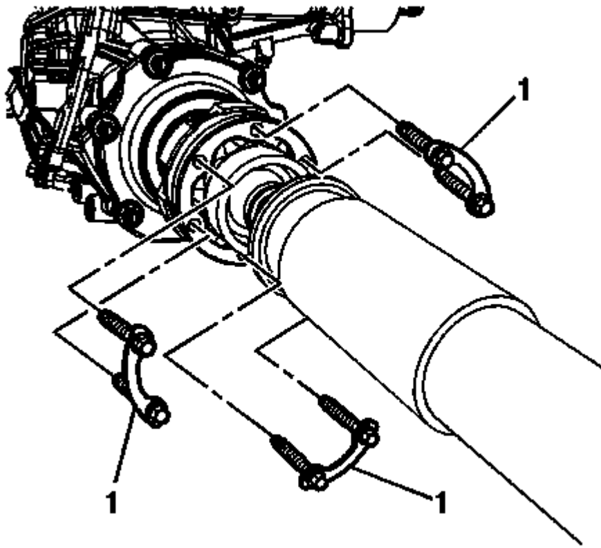
Fig. 243: Propeller Shaft Bolts And Washers Courtesy of GENERAL MOTORS COMPANY
