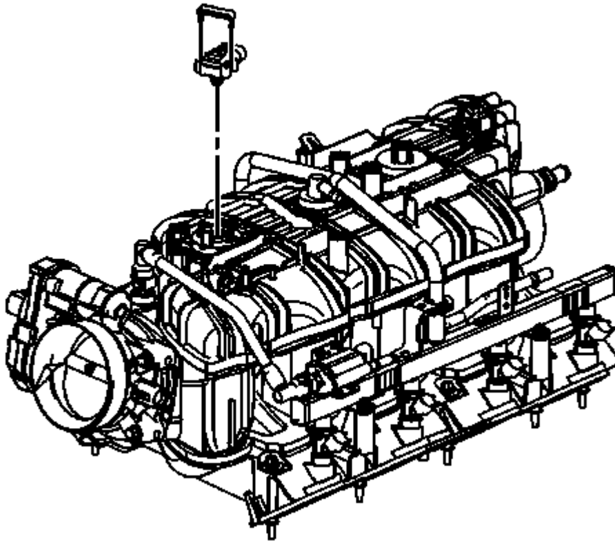
Fig. 65: View Of MAP Sensor & Retainer Courtesy of GENERAL MOTORS COMPANY
