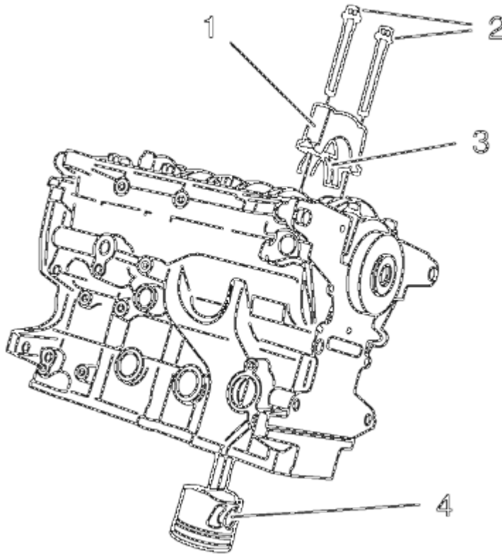
Fig. 242: View Of Valve Lifters & Guides
