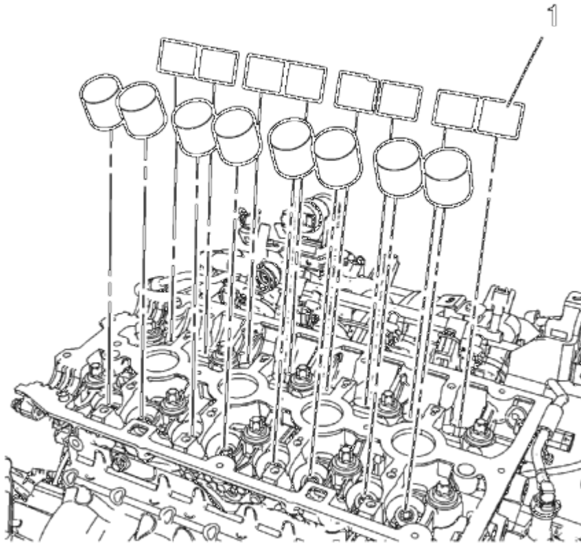
Fig. 165: Retaining Strap
