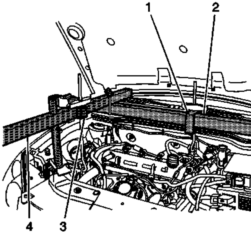
Fig. 351: View Of Oil Pan Drain Plug & Seal Courtesy of GENERAL MOTORS COMPANY
