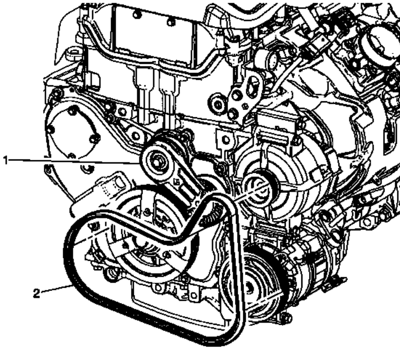
Fig. 340: View Of Oil Cooler Line Clip & Bolt Courtesy of GENERAL MOTORS COMPANY
