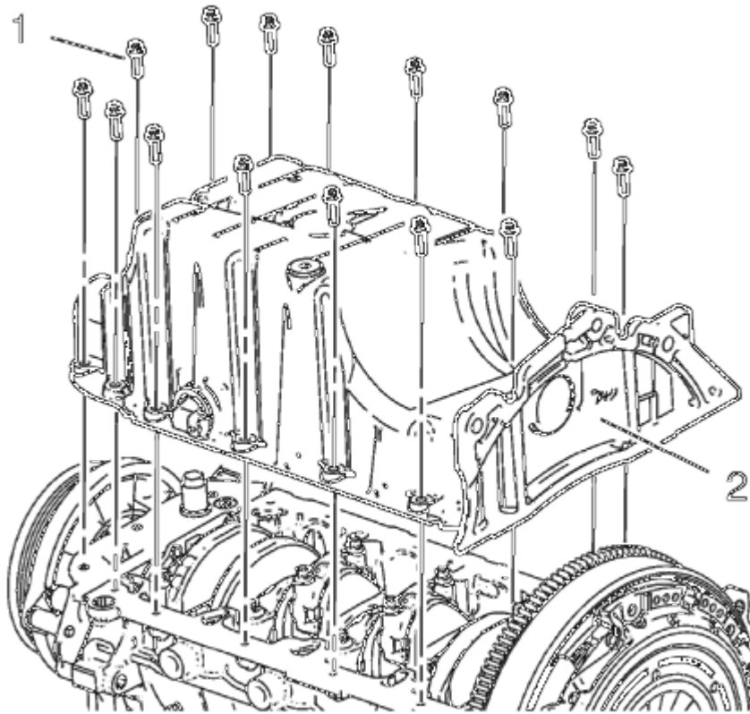
Fig. 157: View Of Engine Valley Cover & Gasket Courtesy of GENERAL MOTORS COMPANY
