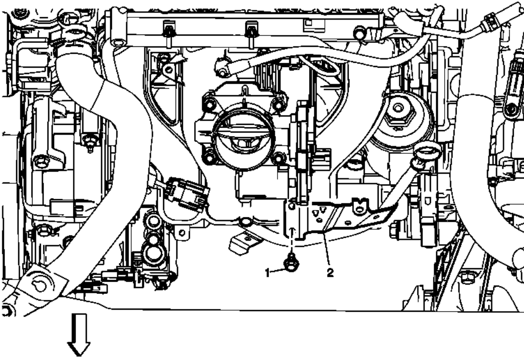
Fig. 352: View Of Oil Pan Skid Plate & Bolts Courtesy of GENERAL MOTORS COMPANY
