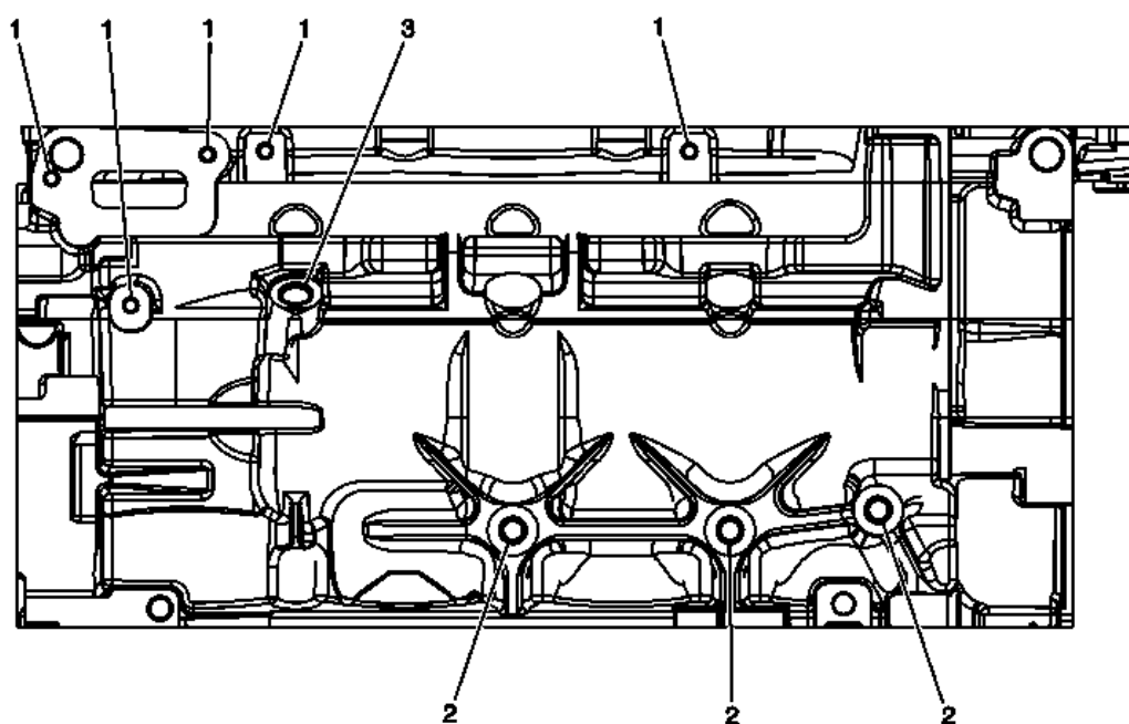
Fig. 318: View Of Left Side Transmission Cover Bolt
