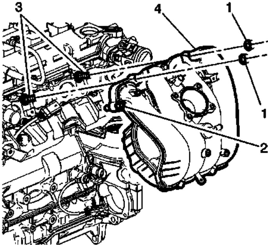
Fig. 362: View Of Lower Transmission Bolts Courtesy of GENERAL MOTORS COMPANY
