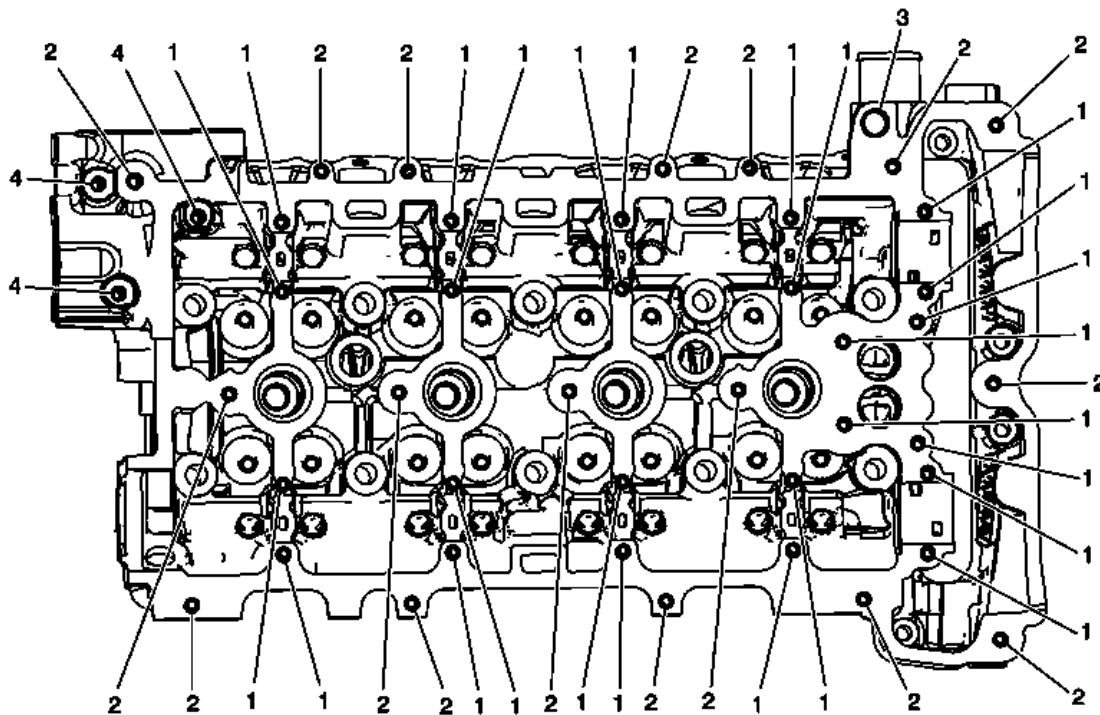
Fig. 327: View Of Oil Cooler Line Clip Courtesy of GENERAL MOTORS COMPANY
