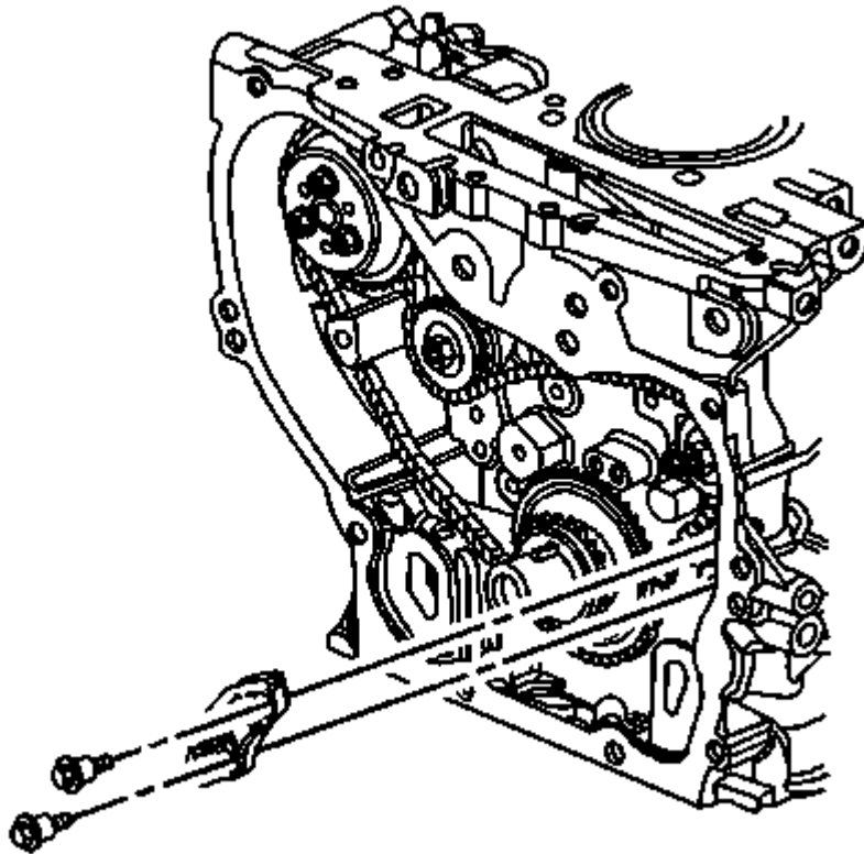
Fig. 411: View Of Special Tool & Bolts Courtesy of GENERAL MOTORS COMPANY
