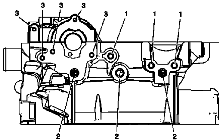
Fig. 331: View Of Oil Pan & Bolts Courtesy of GENERAL MOTORS COMPANY
