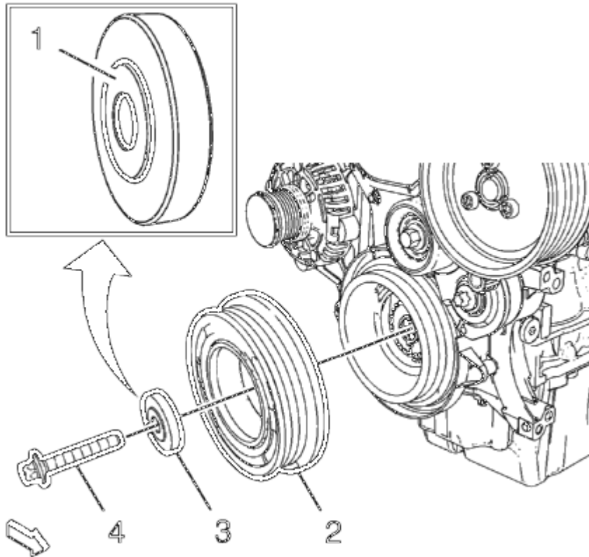
Fig. 292: Crankshaft Rear Oil Seal & Housing Courtesy of GENERAL MOTORS COMPANY
