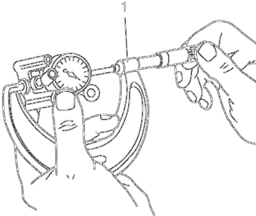
Fig. 213: Compress The Valve Spring (Cylinder Head Installed) Using Special Tools Courtesy of GENERAL MOTORS COMPANY
