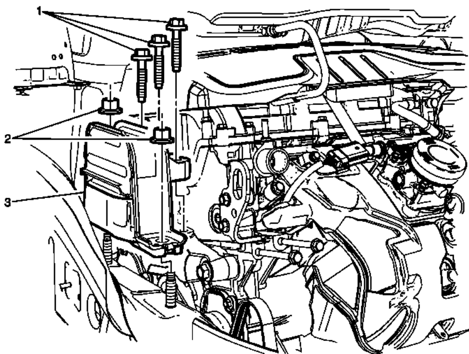
Fig. 344: View Of Electrical Connector, Cable Channel Bolt & Pin Courtesy of GENERAL MOTORS COMPANY
