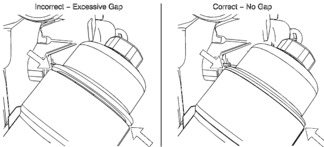
Fig. 13: View Of Drive Belt Tensioner & Bolts Courtesy of GENERAL MOTORS COMPANY
