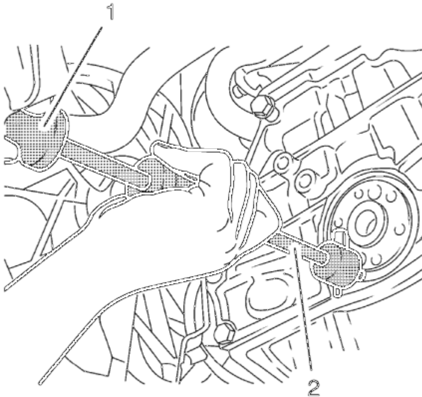
Fig. 115: View Of Brake Booster Vacuum Hose & Booster Fitting Courtesy of GENERAL MOTORS COMPANY
