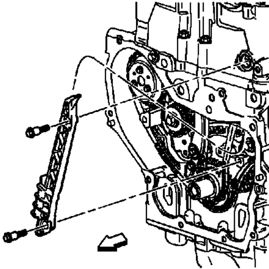
Fig. 389: View Of Vehicle Crossbar, Bolts & Nuts Courtesy of GENERAL MOTORS COMPANY
