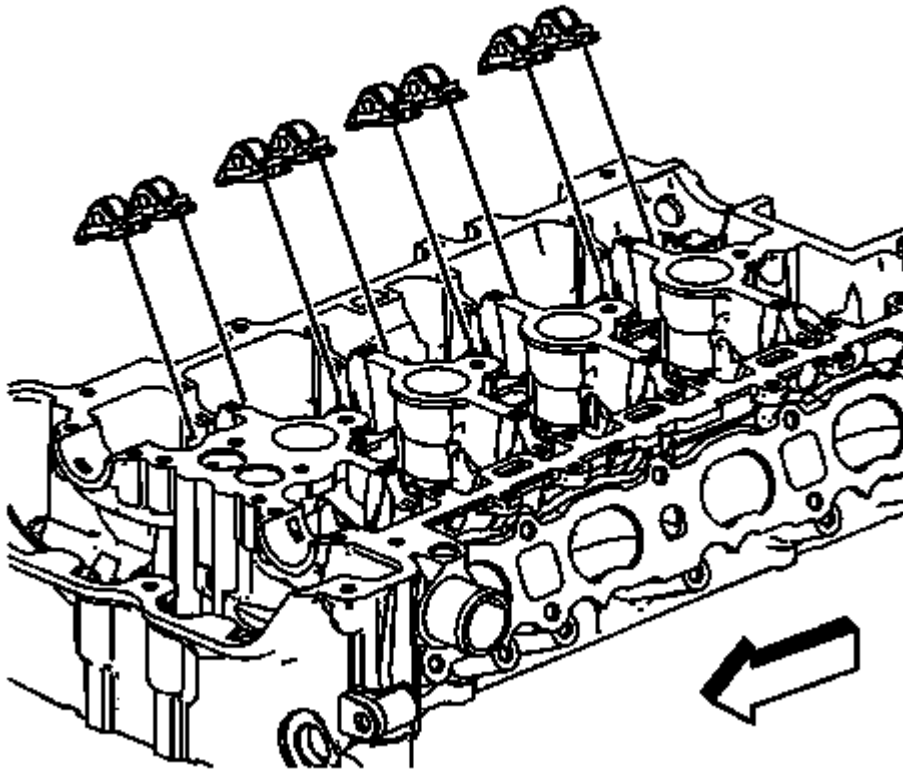
Fig. 444: View Of Engine Wiring Harness Electrical Connector & Components Courtesy of GENERAL MOTORS COMPANY
