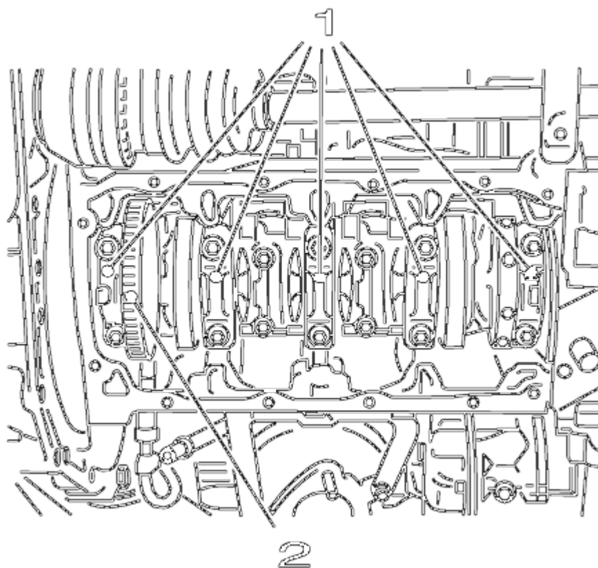
Fig. 239: Valve Lifter Guides & Bolts
