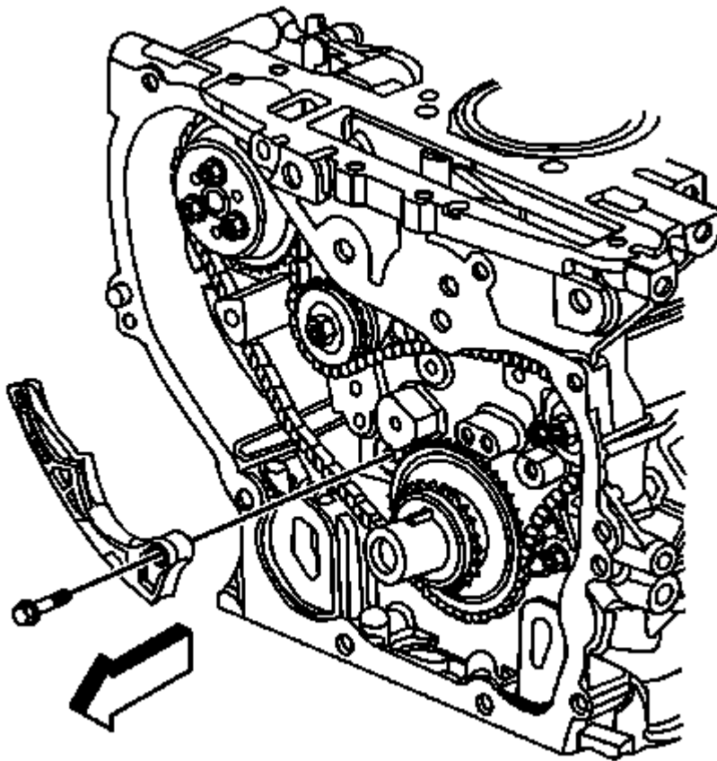
Fig. 417: View Of Installed Crankshaft Key Courtesy of GENERAL MOTORS COMPANY
