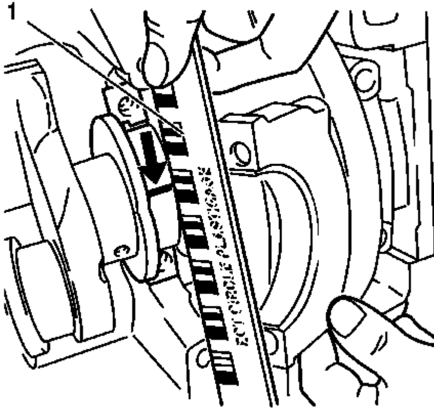
Fig. 212: Applying Compressed Air To J 22794 Courtesy of GENERAL MOTORS COMPANY
