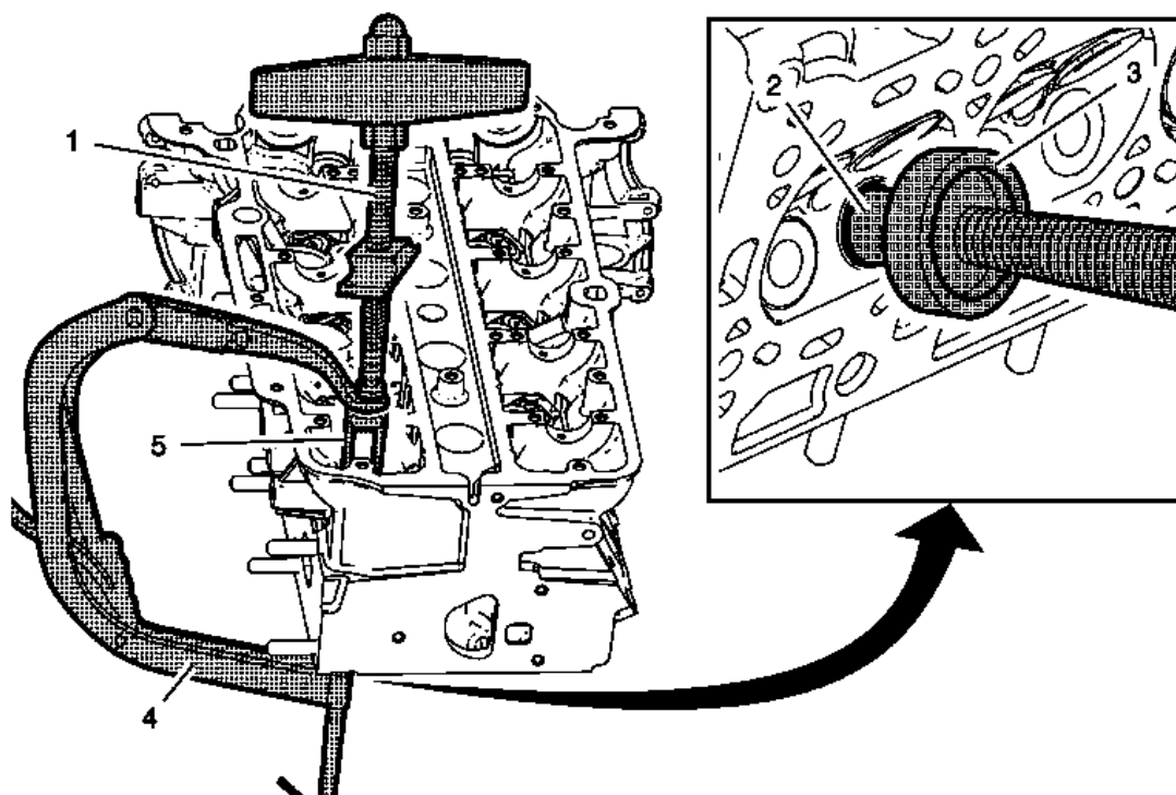
Fig. 231: View Of Cylinder Head Gasket & Locating Pins Courtesy of GENERAL MOTORS COMPANY
