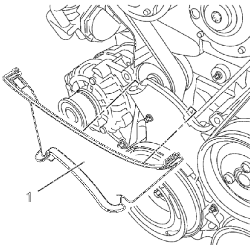
Fig. 293: Identifying Oil Seal
