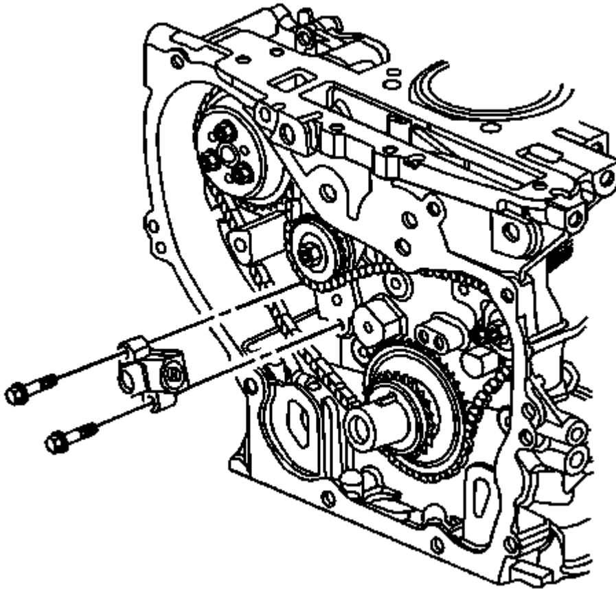
Fig. 410: View Of Oil Pump Screen & O-Ring Seal Courtesy of GENERAL MOTORS COMPANY
