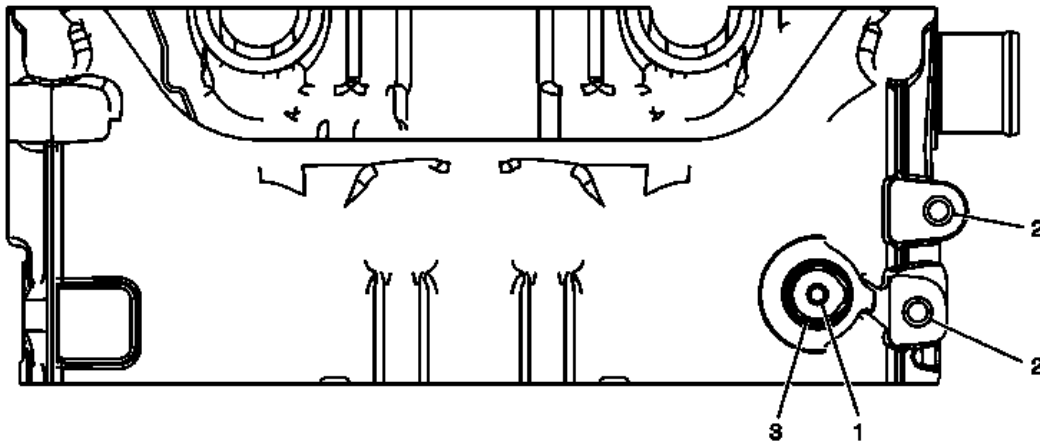
Fig. 330: View Of Oil Cooler Line Clip & Bolt Courtesy of GENERAL MOTORS COMPANY
