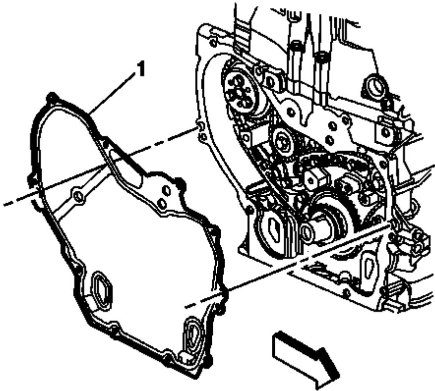
Fig. 380: View Of Lower Transmission Bolt Courtesy of GENERAL MOTORS COMPANY
