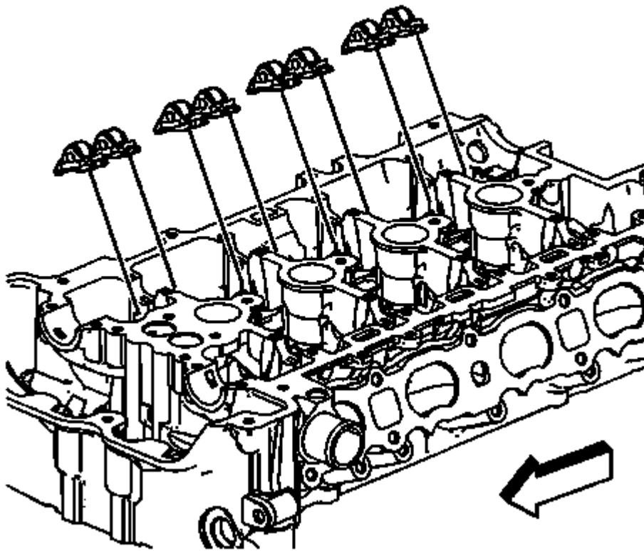
Fig. 448: View Of Transmission Oil Level Indicator Tube Nut Courtesy of GENERAL MOTORS COMPANY
