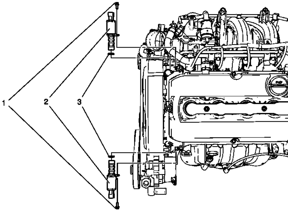
Fig. 50: View Of PCV Tube & Right Valve Rocker Arm Cover Fitting Courtesy of GENERAL MOTORS COMPANY
