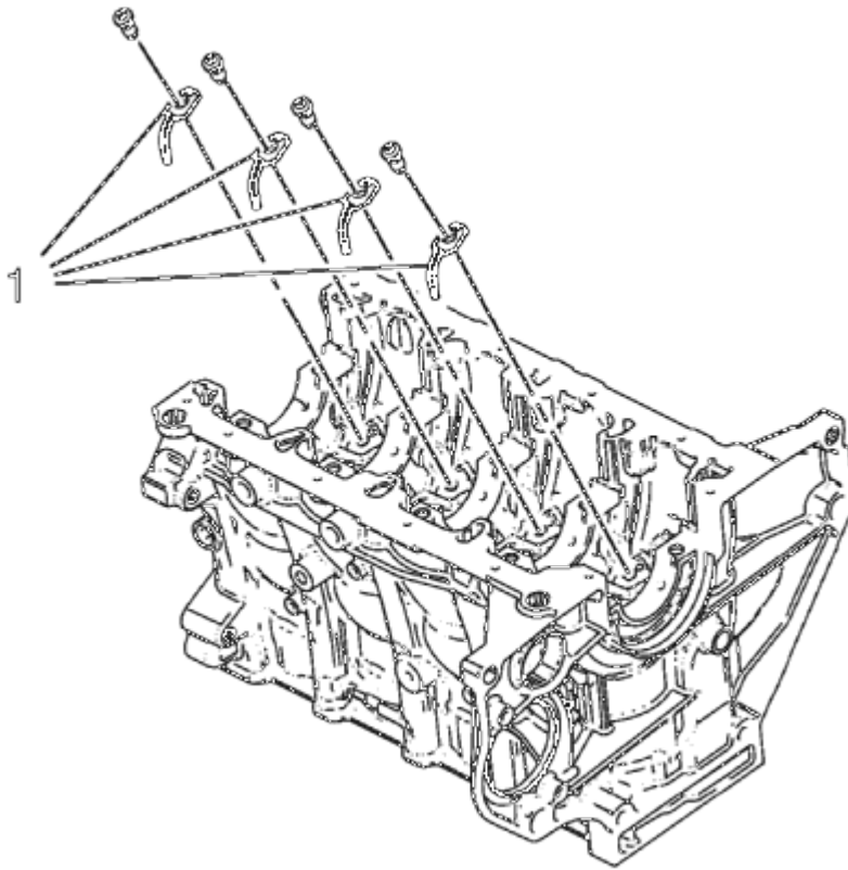
Fig. 222: View Of Cylinder Head & Bolts Courtesy of GENERAL MOTORS COMPANY
