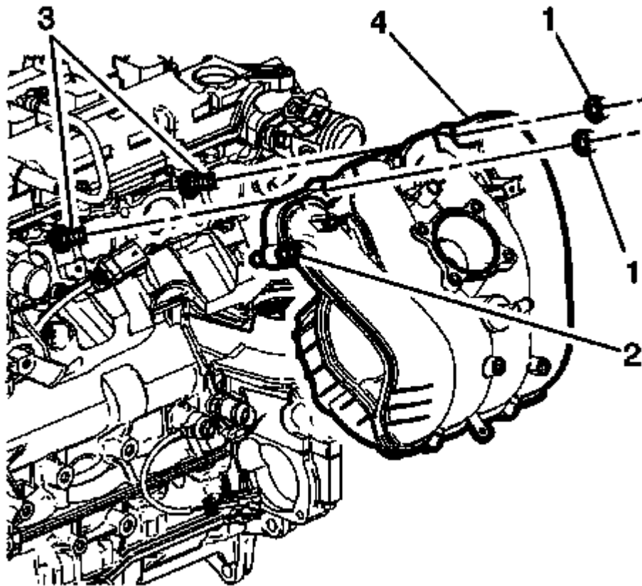
Fig. 361: View Of Vehicle Crossbar, Bolts & Nuts Courtesy of GENERAL MOTORS COMPANY
