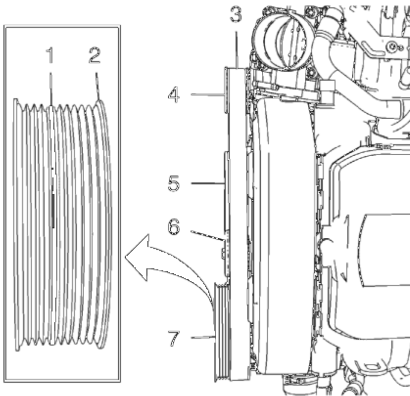
Fig. 296: Identifying Rear Oil Seal Housing Components Courtesy of GENERAL MOTORS COMPANY
