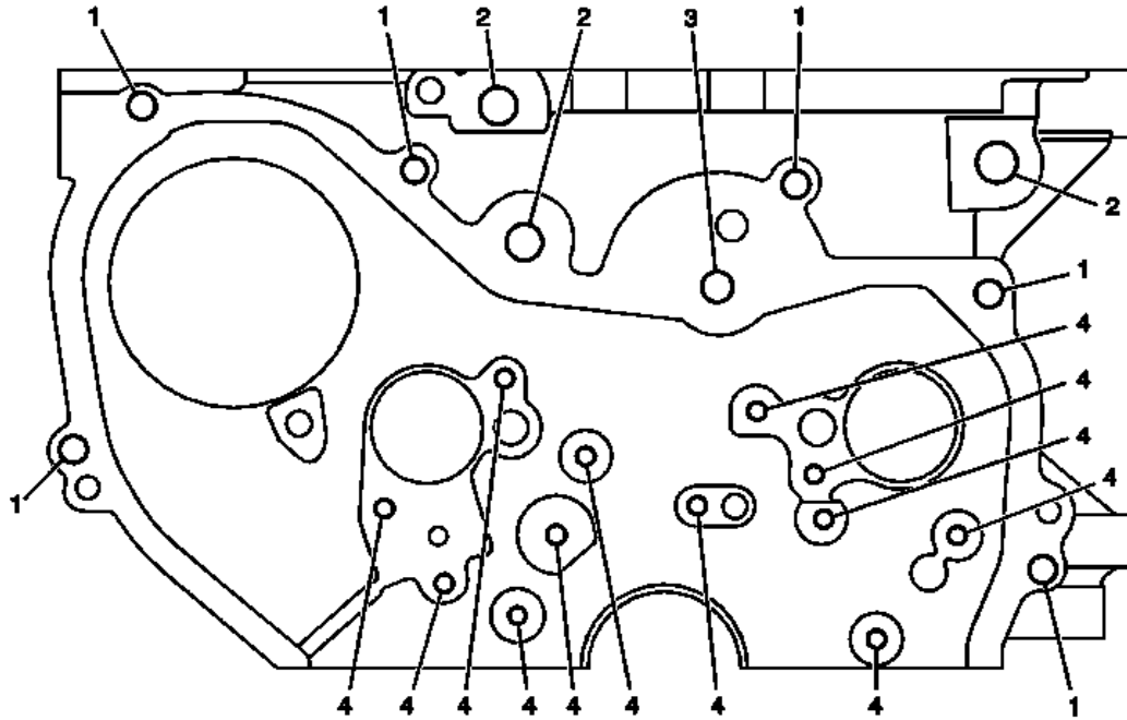
Fig. 316: View Of Engine Oil Filter
