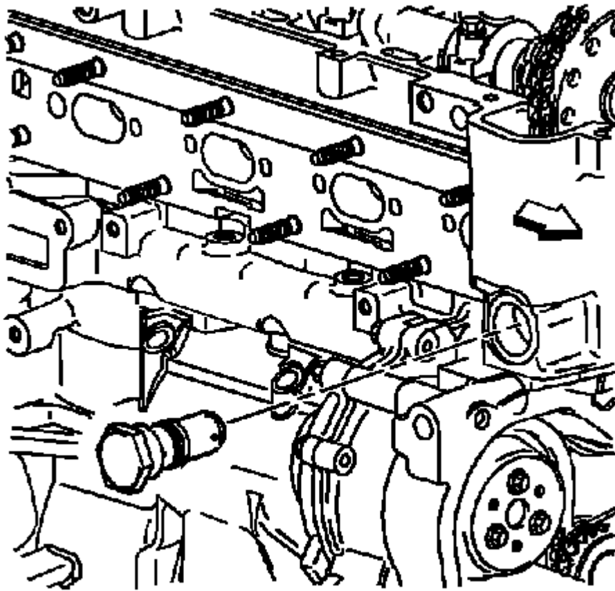
Fig. 420: View Of Compressed Tensioner Courtesy of GENERAL MOTORS COMPANY
