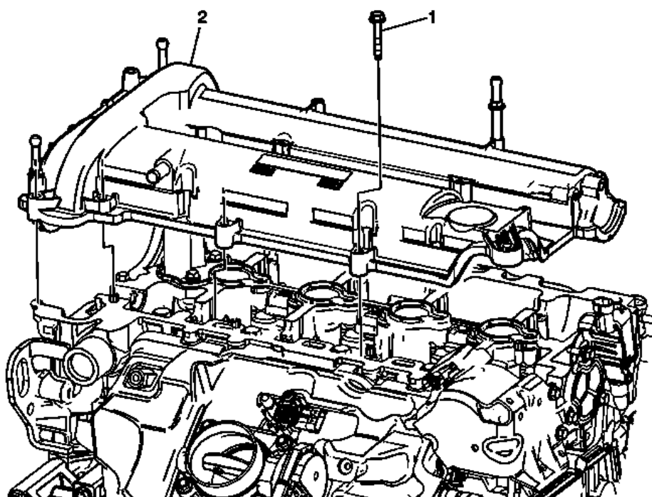
Fig. 419: View Of Crankshaft Sprocket & Installer Courtesy of GENERAL MOTORS COMPANY
