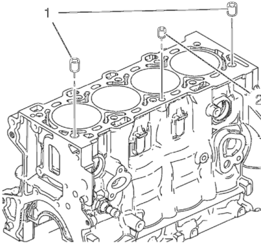
Fig. 228: View Of Engine Ground Strap & Bolt Courtesy of GENERAL MOTORS COMPANY
