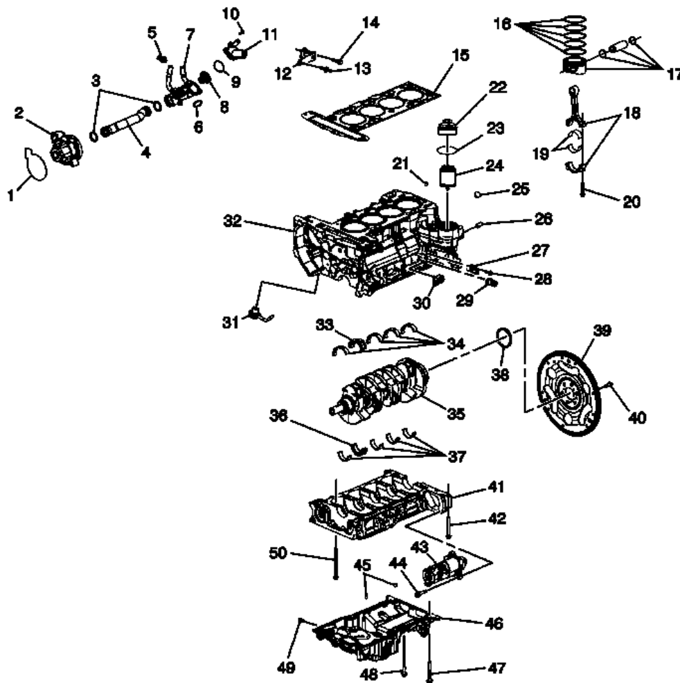
Fig. 335: View Of Oil Pan & Bolts
