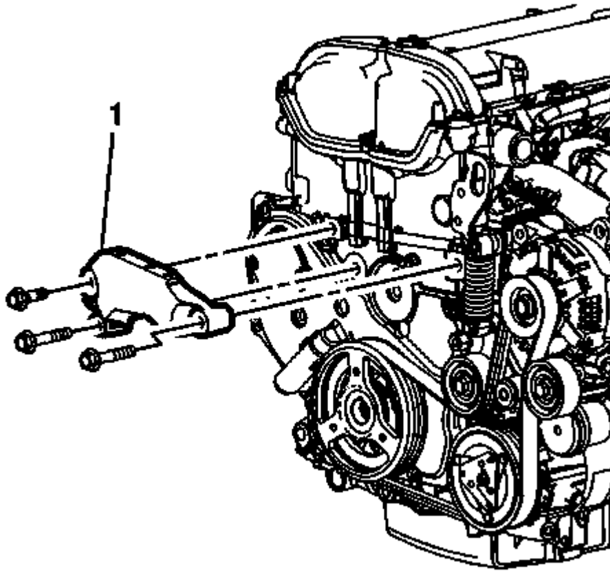
Fig. 383: View Of Oil Cooler Line Clip & Bolt Courtesy of GENERAL MOTORS COMPANY
