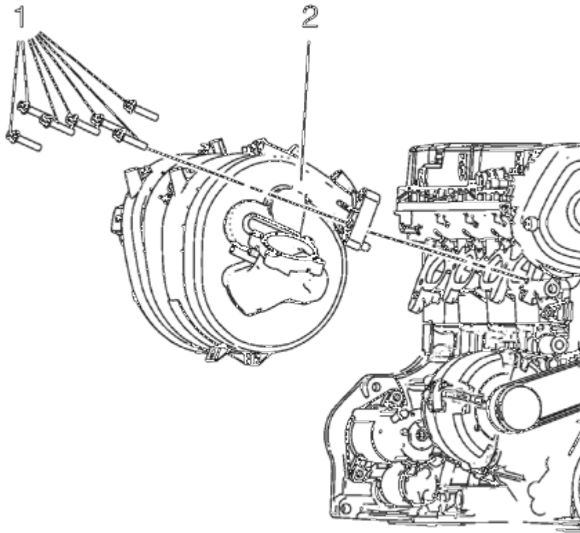
Fig. 146: View Of PCV Hose
