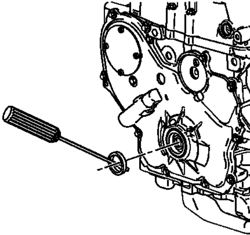
Fig. 374: Drilling Oil Pan Gasket Retaining Rivets Courtesy of GENERAL MOTORS COMPANY
