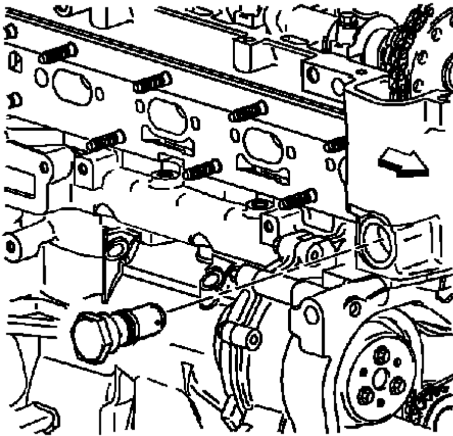
Fig. 457: View Of Oil Pan Drain Plug & Seal Courtesy of GENERAL MOTORS COMPANY
