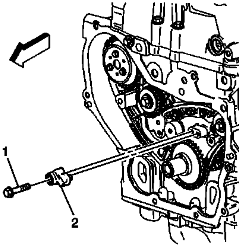
Fig. 408: View Of Oil Pump & Bolts
