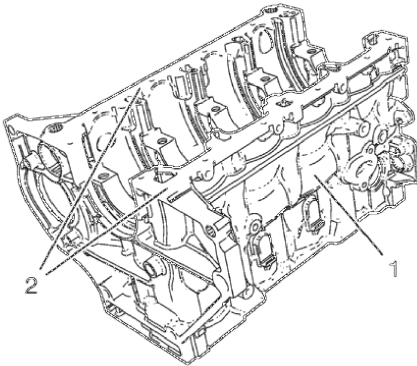
Fig. 216: Compress The Valve Spring (Cylinder Head Installed) Using Special Tools Courtesy of GENERAL MOTORS COMPANY
