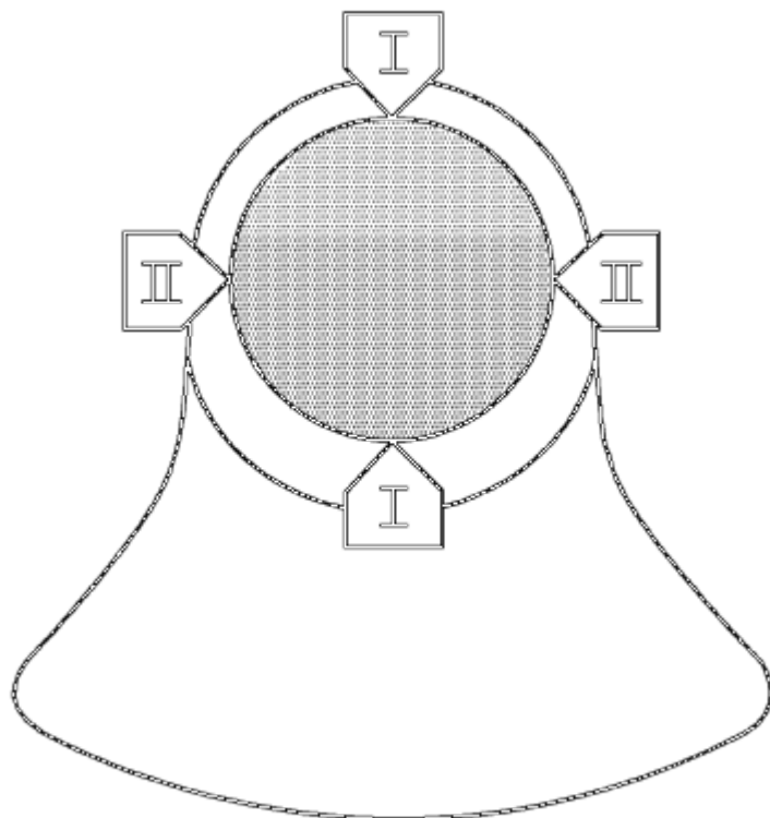
Fig. 215: Valve Stem Keys, Valve Spring Cap & Valve Spring Courtesy of GENERAL MOTORS COMPANY
