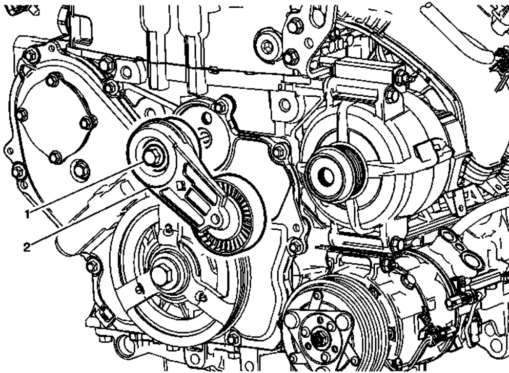
Fig. 341: View Of Oil Cooler Line Clip Courtesy of GENERAL MOTORS COMPANY
