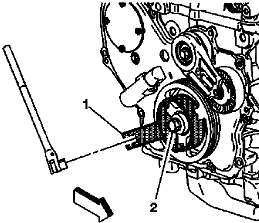
Fig. 370: View Of Oil Cooler Line Clip
