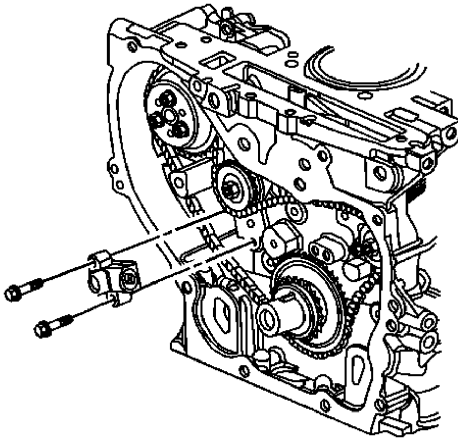
Fig. 418: View Of Crankshaft Sprocket Courtesy of GENERAL MOTORS COMPANY
