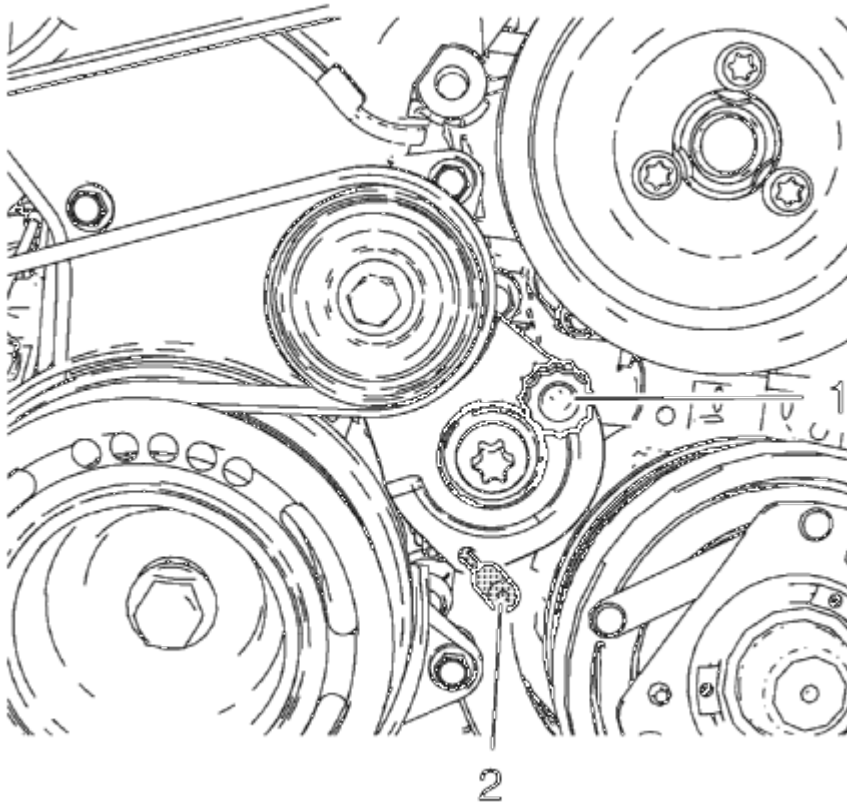
Fig. 120: View Of Engine Harness Retainer Nut & Electrical Connectors Courtesy of GENERAL MOTORS COMPANY
