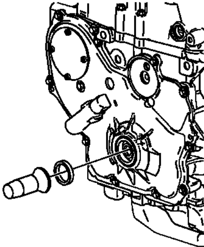
Fig. 375: View Of Sealant Applied To Front Oil Pan-To-Engine Block Junction Courtesy of GENERAL MOTORS COMPANY
