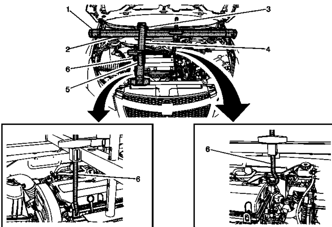
Fig. 74: View Of MAP Sensor & Retainer Courtesy of GENERAL MOTORS COMPANY
