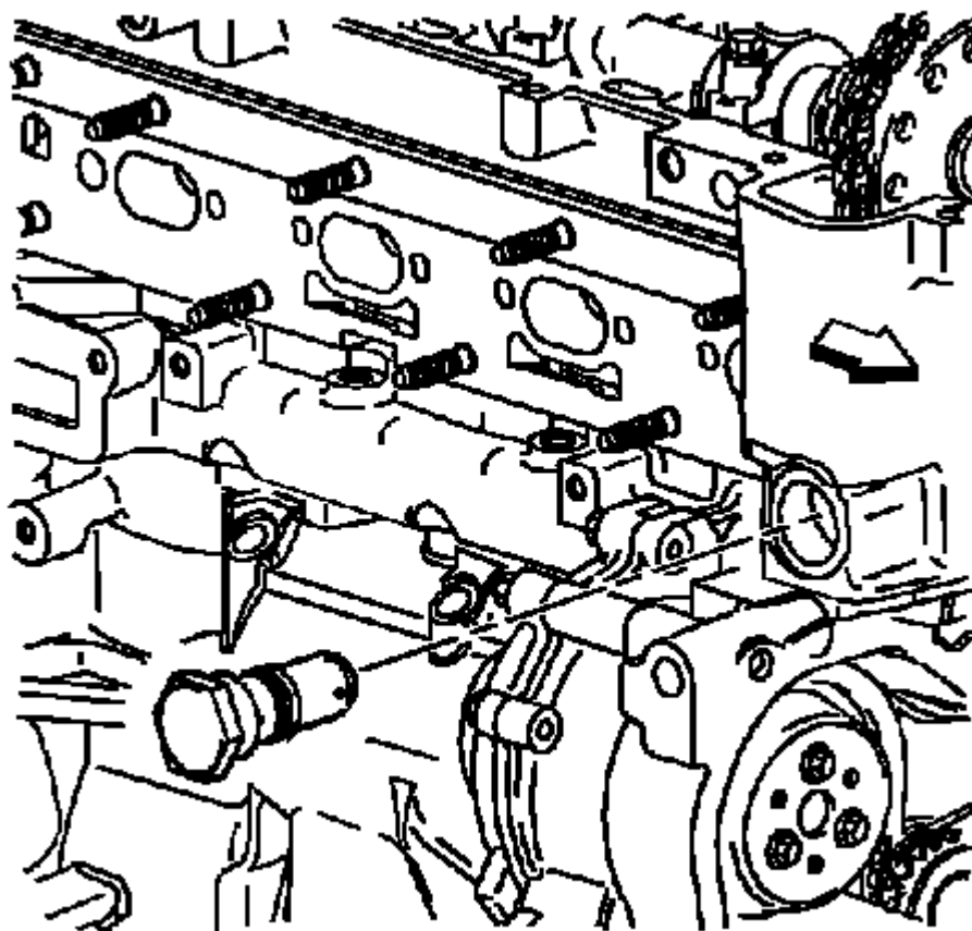
Fig. 487: View Of Engine Ground Strap & Bolt Courtesy of GENERAL MOTORS COMPANY
