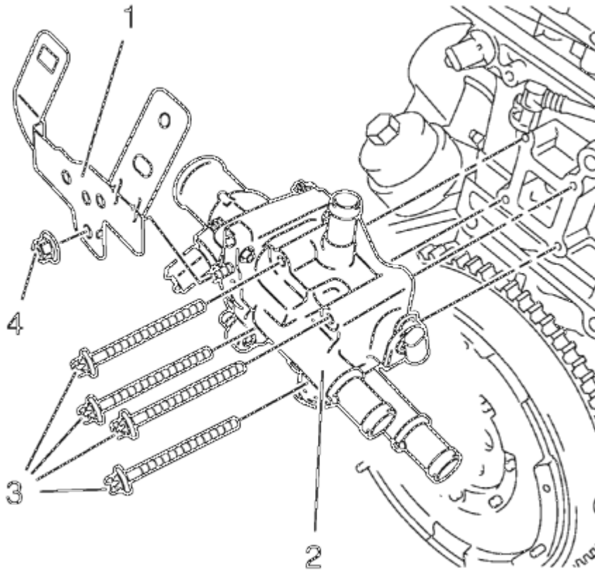
Fig. 265: View Of CMP Sensor Wire Harness & Bolts Courtesy of GENERAL MOTORS COMPANY
