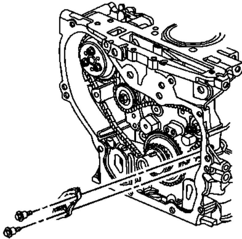
Fig. 416: View Of Crankshaft Key & Keyway Courtesy of GENERAL MOTORS COMPANY
