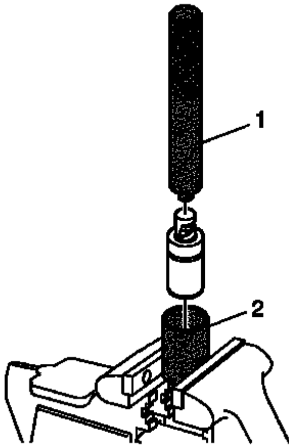
Fig. 422: View Of Special Tool & Bolts Courtesy of GENERAL MOTORS COMPANY
