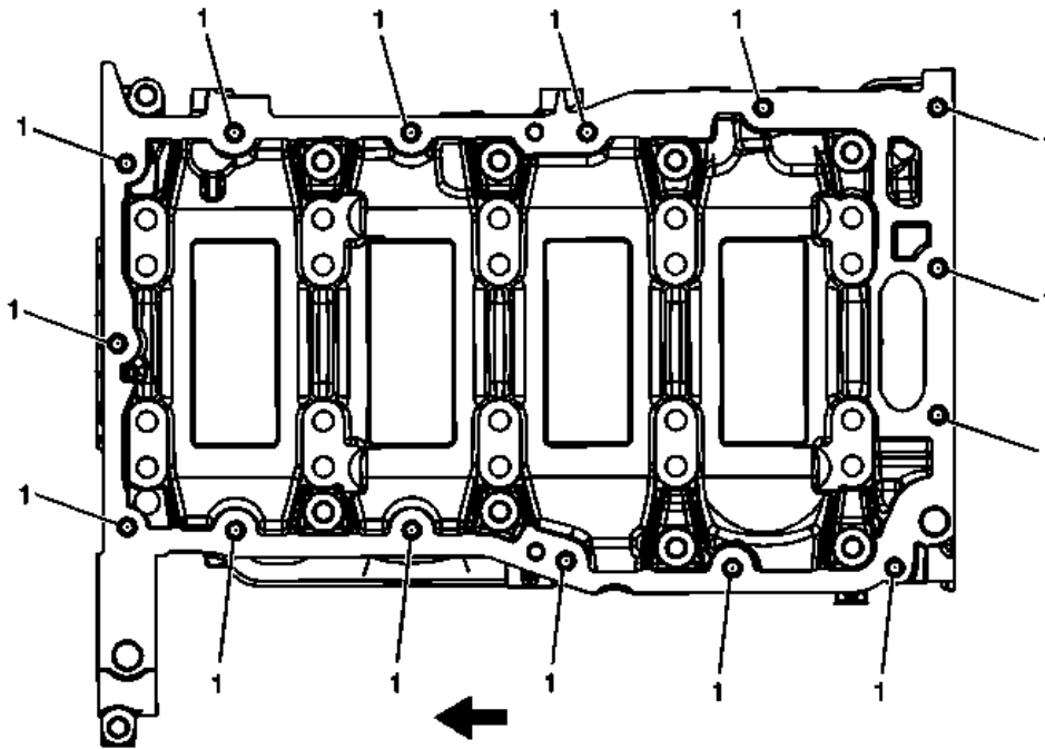
Fig. 324: View Of Lower Transmission Stud Courtesy of GENERAL MOTORS COMPANY
