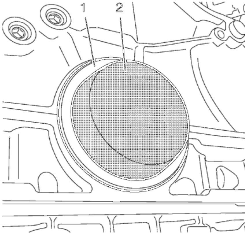
Fig. 310: View Of Oil Pan Skid Plate & Bolts Courtesy of GENERAL MOTORS COMPANY
