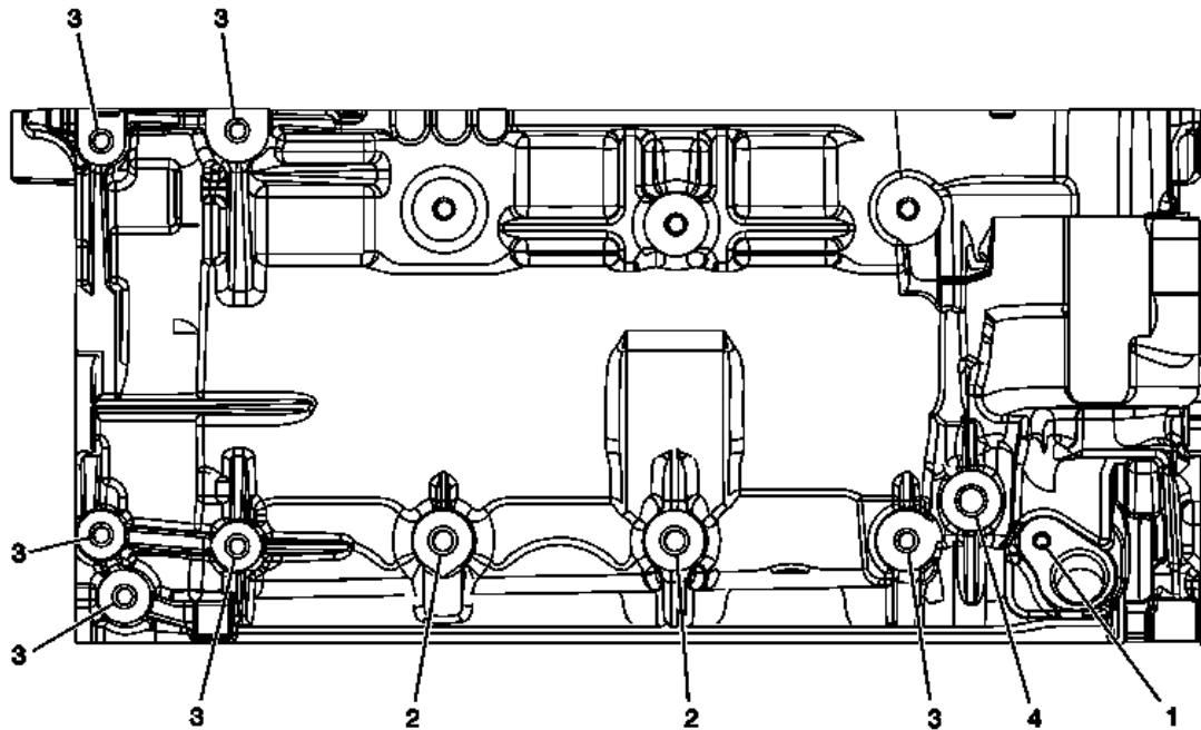
Fig. 319: View Of Vehicle Crossbar, Bolts & Nuts Courtesy of GENERAL MOTORS COMPANY
