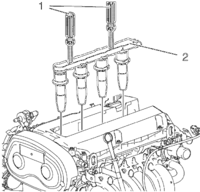
Fig. 160: View Of Engine Valley Cover & Gasket Courtesy of GENERAL MOTORS COMPANY
