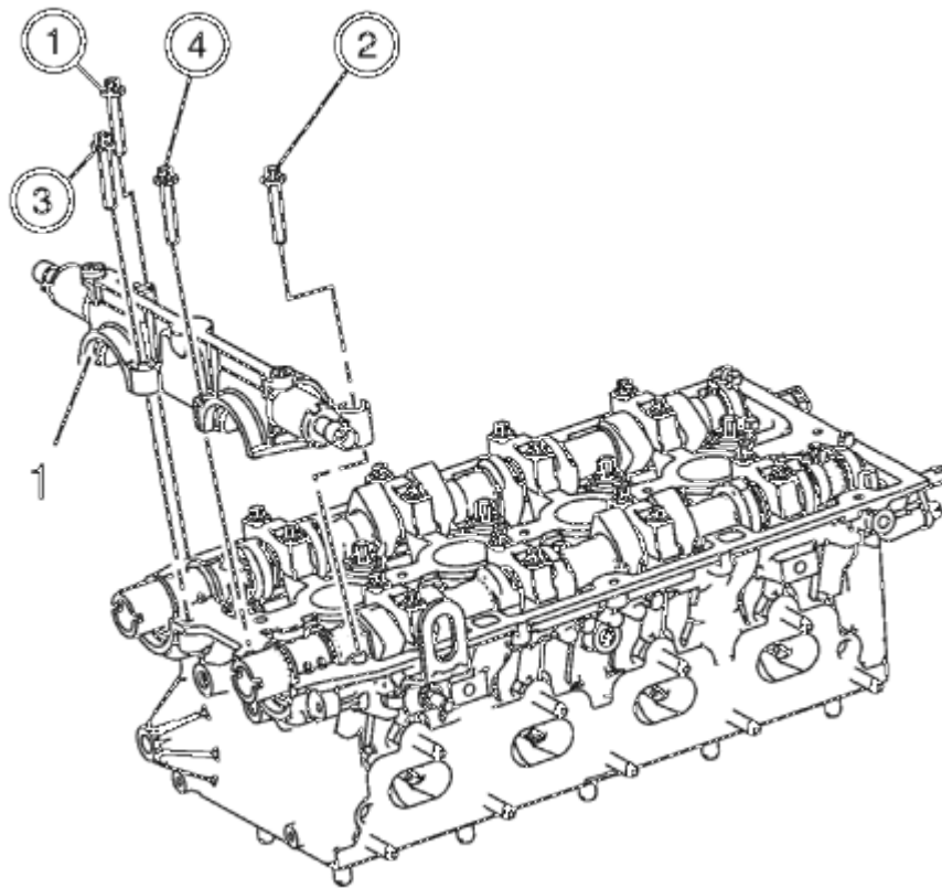
Fig. 162: Valve Lifter Oil Manifold
