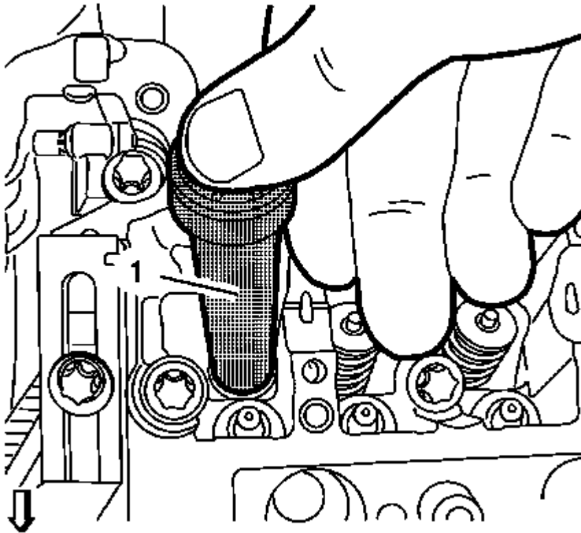
Fig. 64: View Of Upper Intake Manifold Cover & Nut Courtesy of GENERAL MOTORS COMPANY
