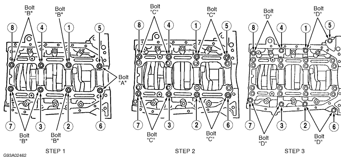
Fig. 38: Identifying Lower Cylinder Block Bolt Location & Installation Sequence Courtesy of MAZDA MOTORS CORP.
