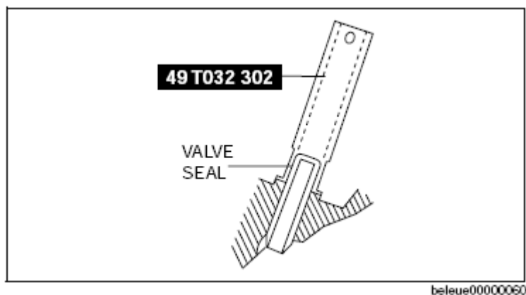
Fig. 112: Tapping SST Using Plastic Hammer
