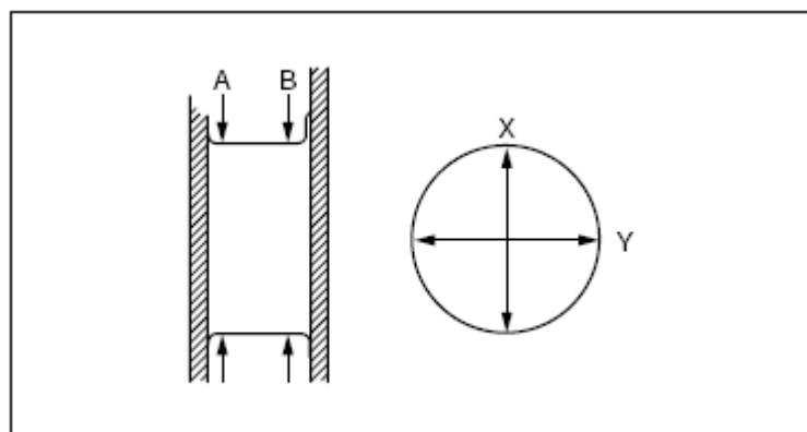
Fig. 61: Measuring Journal Diameter In X And Y Directions At Two Points (A And B)
