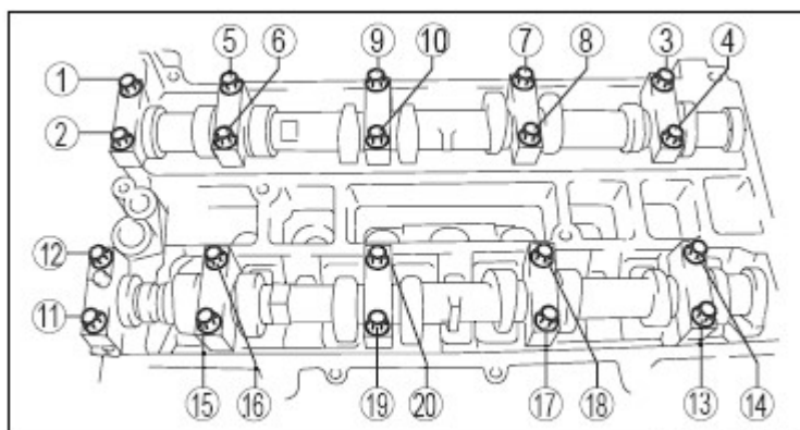
Fig. 78: Identifying Camshaft Cap Bolt Loosening Order
